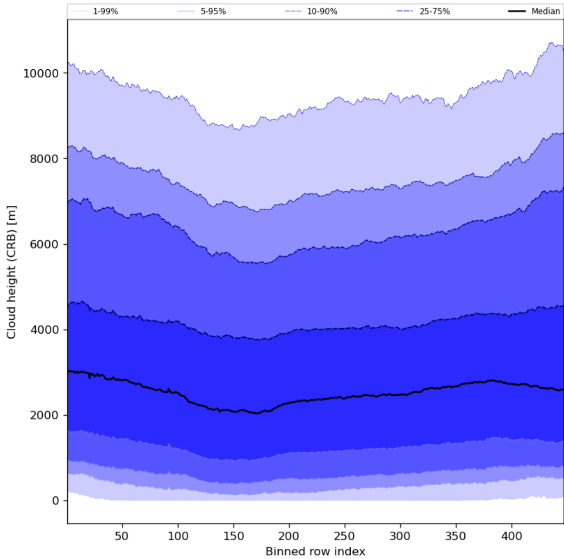
Figure 59: Along track statistics of “Cloud height (CRB)” for 2024-01-05 to 2024-01-06
