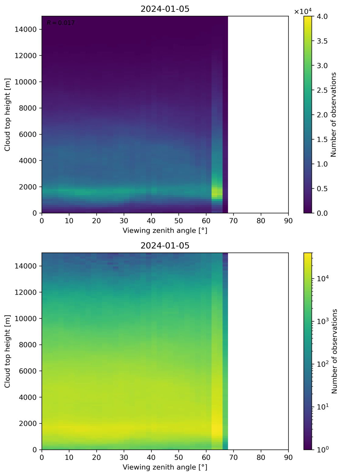
Figure 112: Scatter density plot of “Viewing zenith angle” against “Cloud top height” for 2024-01-05 to 2024-01-06.
