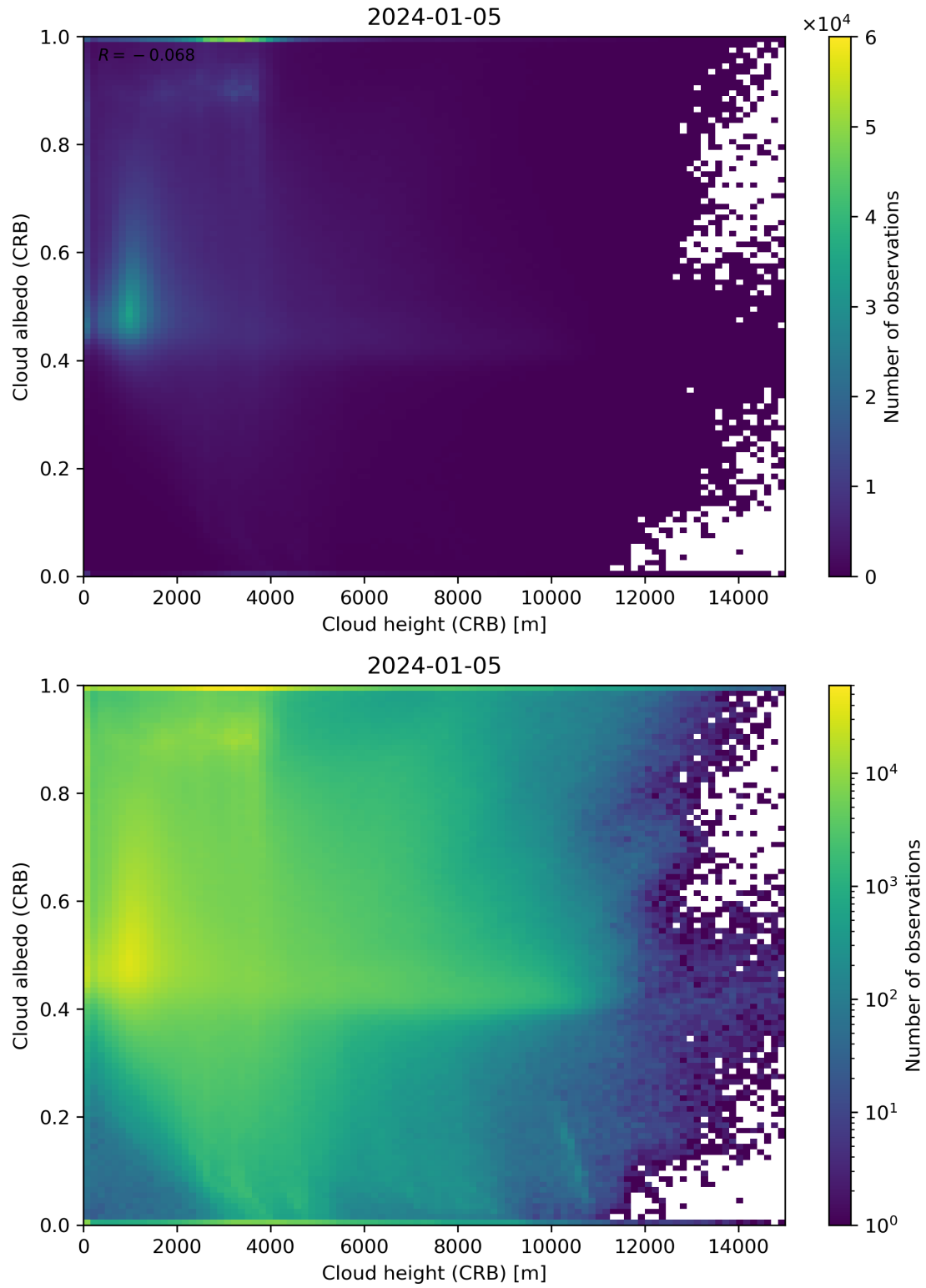
Figure 80: Scatter density plot of “Cloud height (CRB)” against “Cloud albedo (CRB)” for 2024-01-05 to 2024-01-06.
