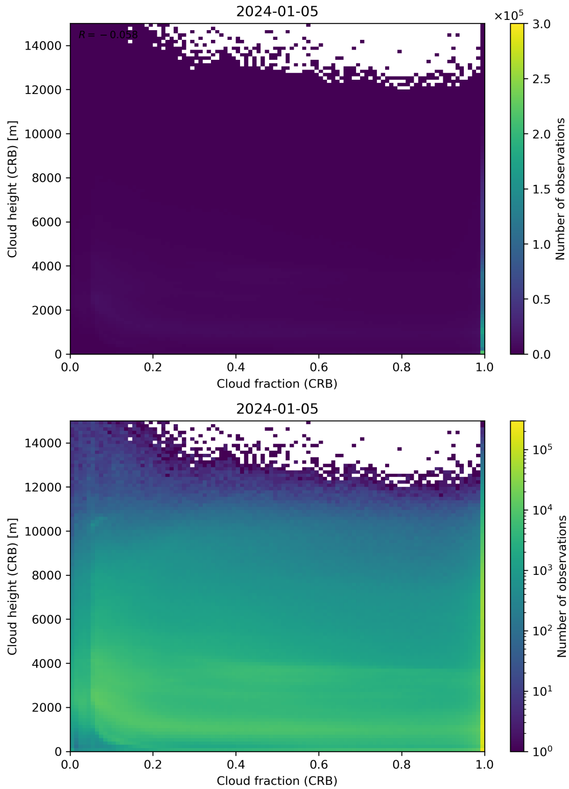
Figure 79: Scatter density plot of “Cloud fraction (CRB)” against “Cloud height (CRB)” for 2024-01-05 to 2024-01-06.
