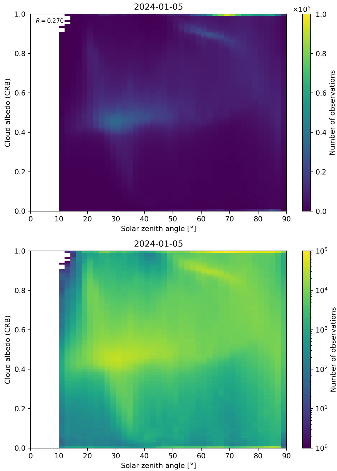
Figure 98: Scatter density plot of “Solar zenith angle” against “Cloud albedo (CRB)” for 2024-01-05 to 2024-01-06.
