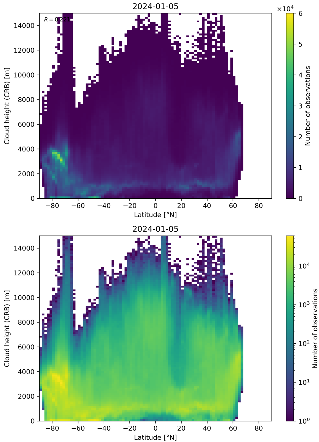
Figure 95: Scatter density plot of “Latitude” against “Cloud height (CRB)” for 2024-01-05 to 2024-01-06.
