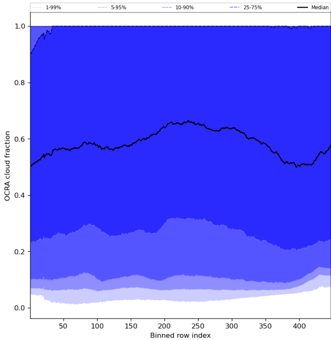
Figure 66: Along track statistics of “OCRA cloud fraction” for 2024-01-05 to 2024-01-06
