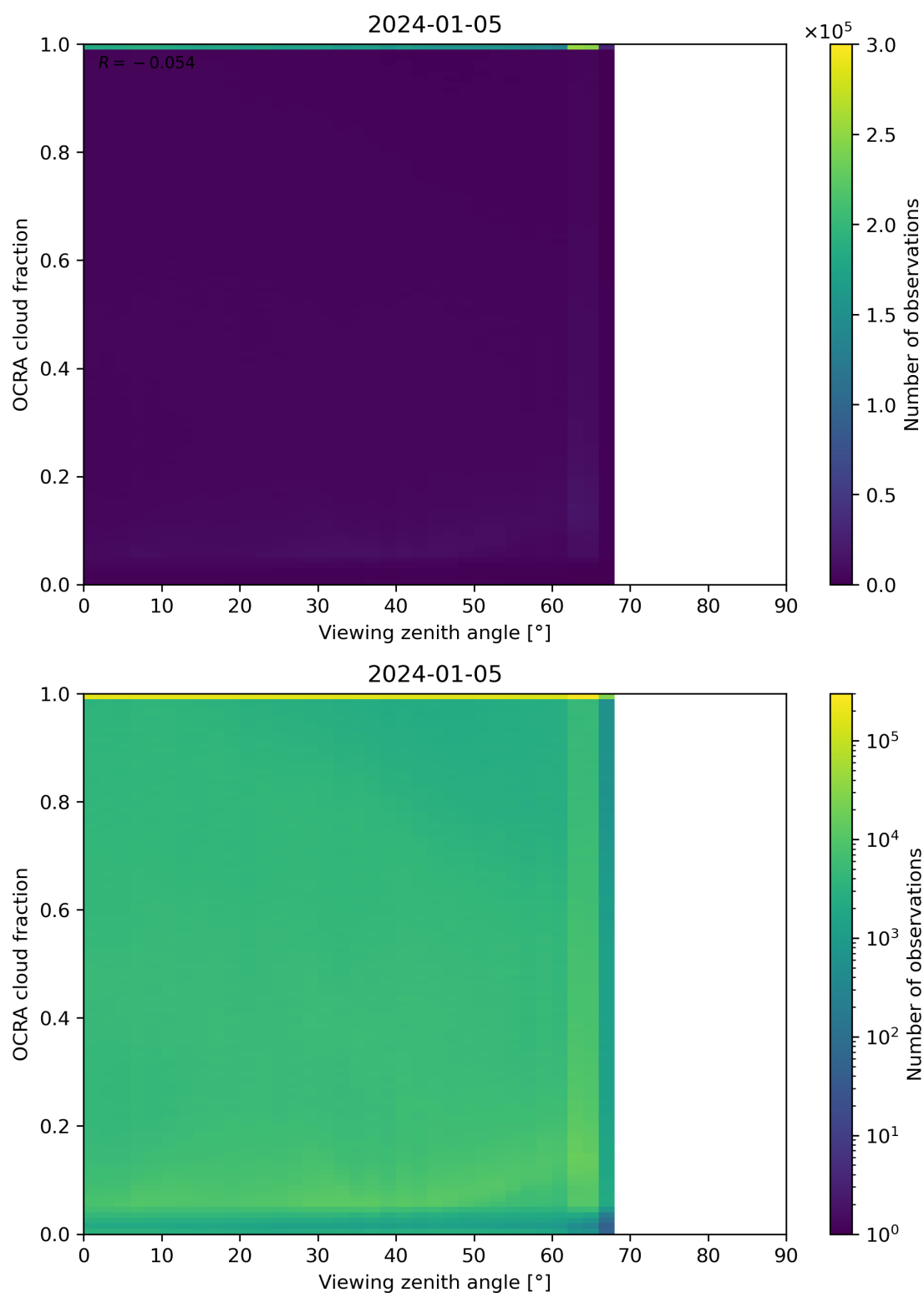
Figure 108: Scatter density plot of “Viewing zenith angle” against “OCRA cloud fraction” for 2024-01-05 to 2024-01-06.
