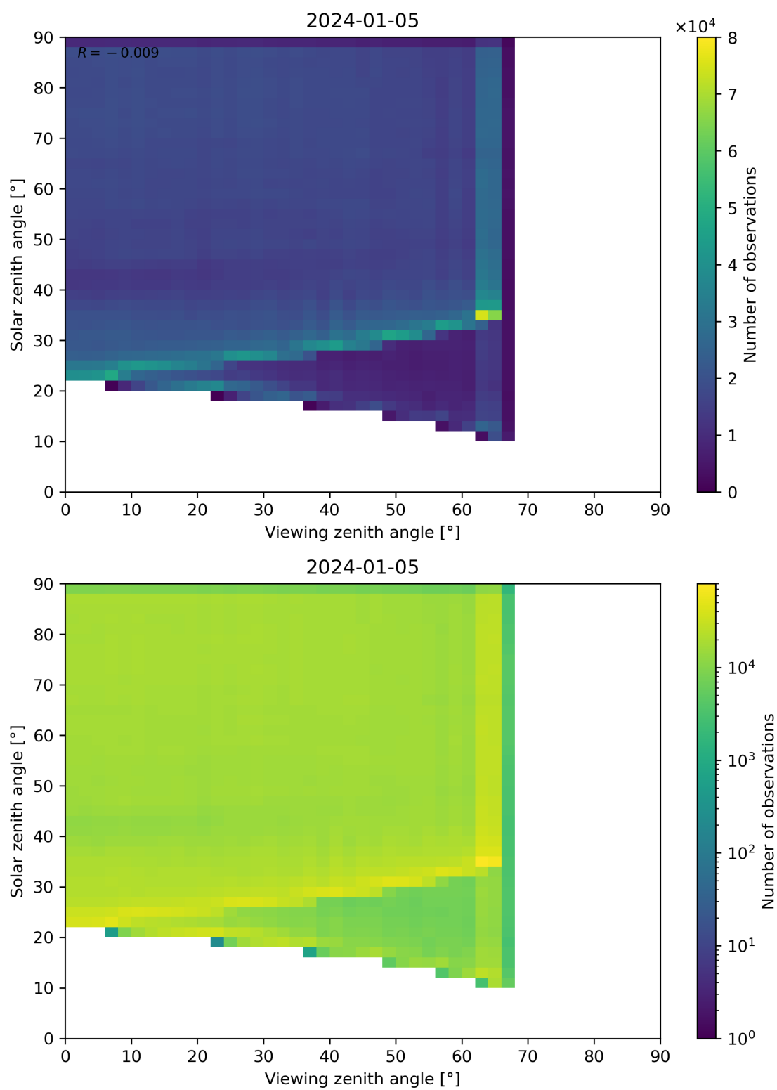
Figure 114: Scatter density plot of “Viewing zenith angle” against “Solar zenith angle” for 2024-01-05 to 2024-01-06.
