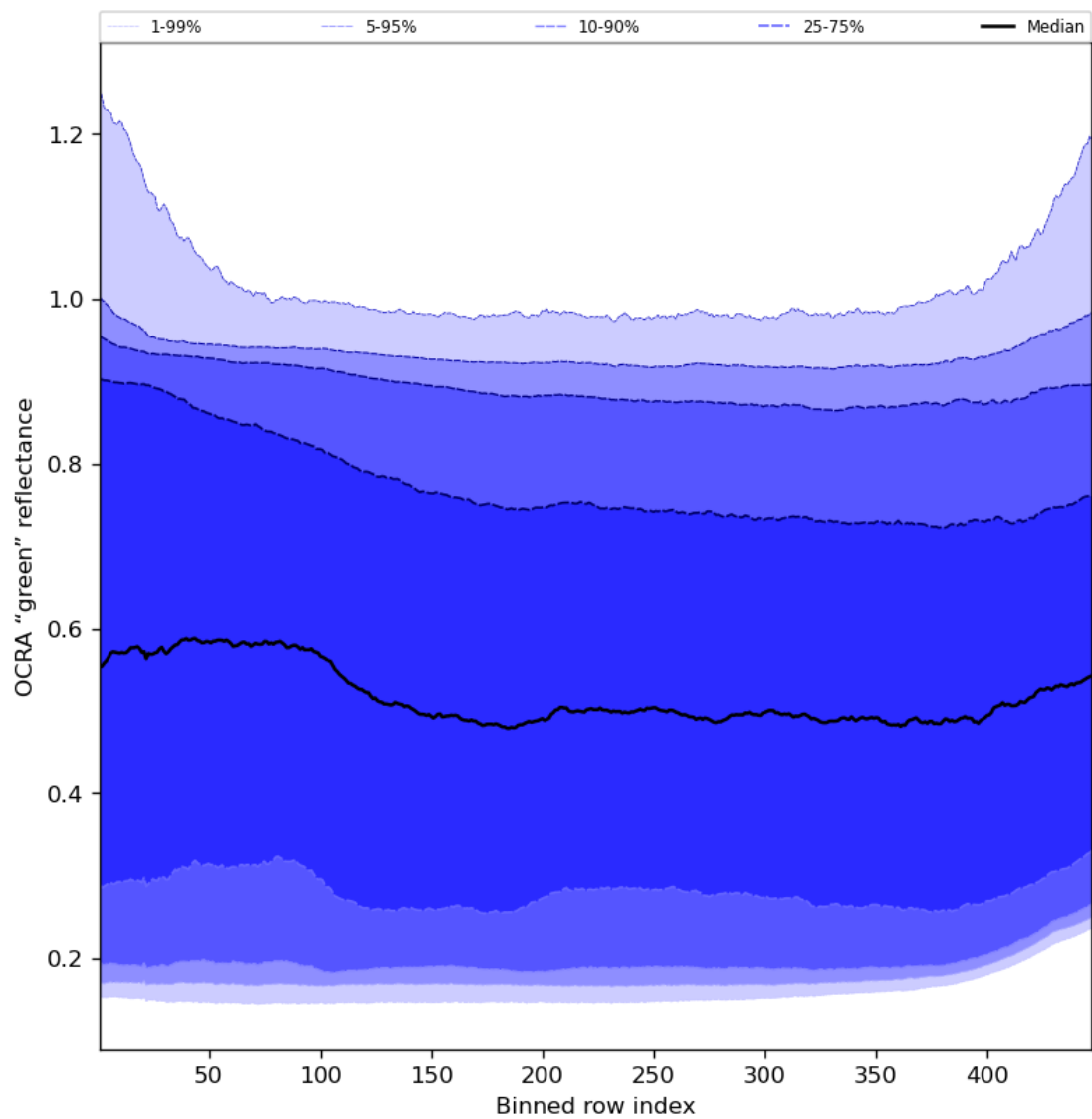
Figure 68: Along track statistics of "OCRA "green" reflectance" for 2024-01-05 to 2024-01-06
