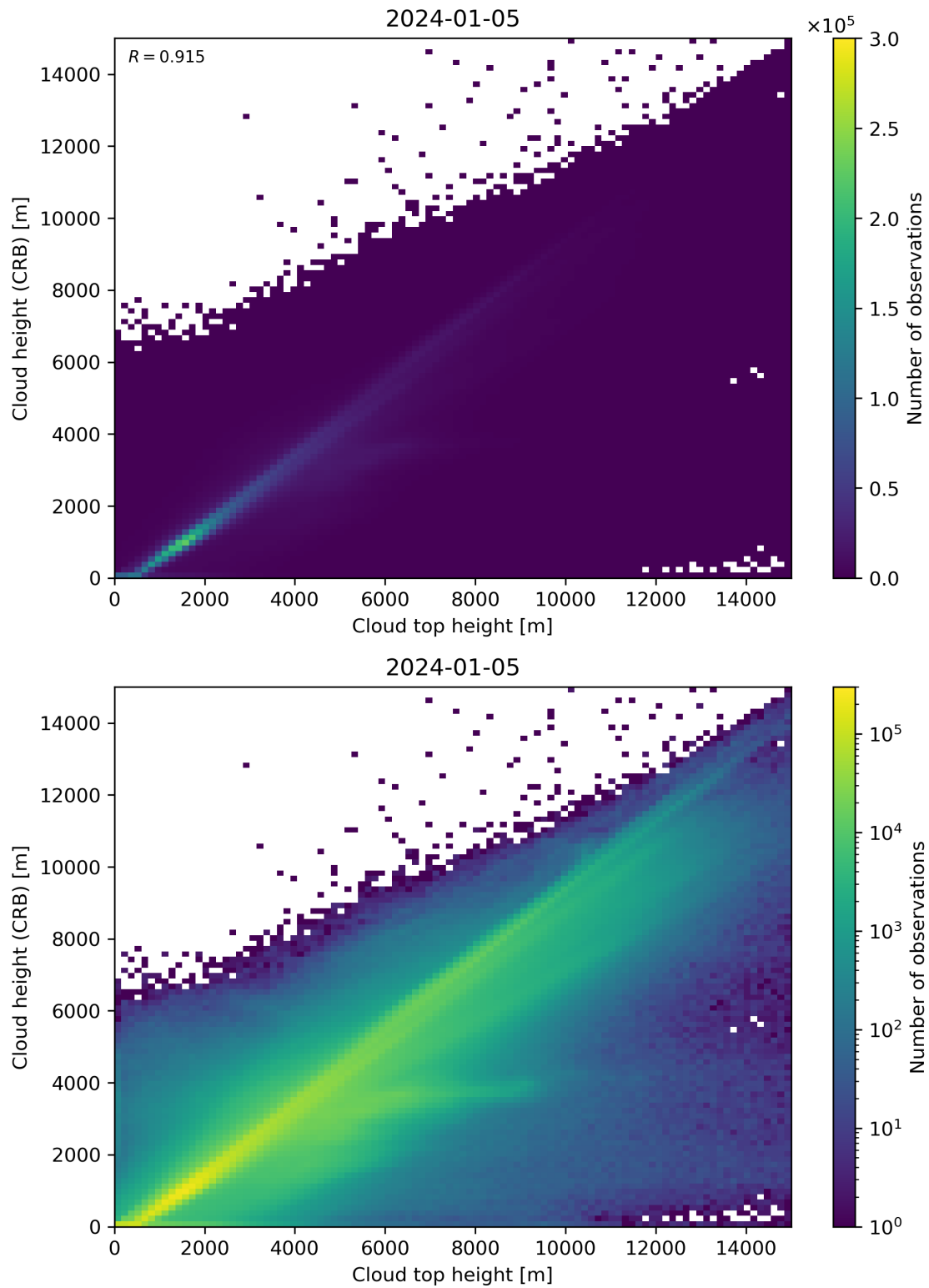
Figure 89: Scatter density plot of “Cloud top height” against “Cloud height (CRB)” for 2024-01-05 to 2024-01-06.
