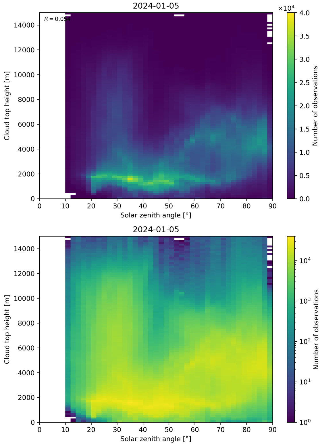
Figure 104: Scatter density plot of “Solar zenith angle” against “Cloud top height” for 2024-01-05 to 2024-01-06.
