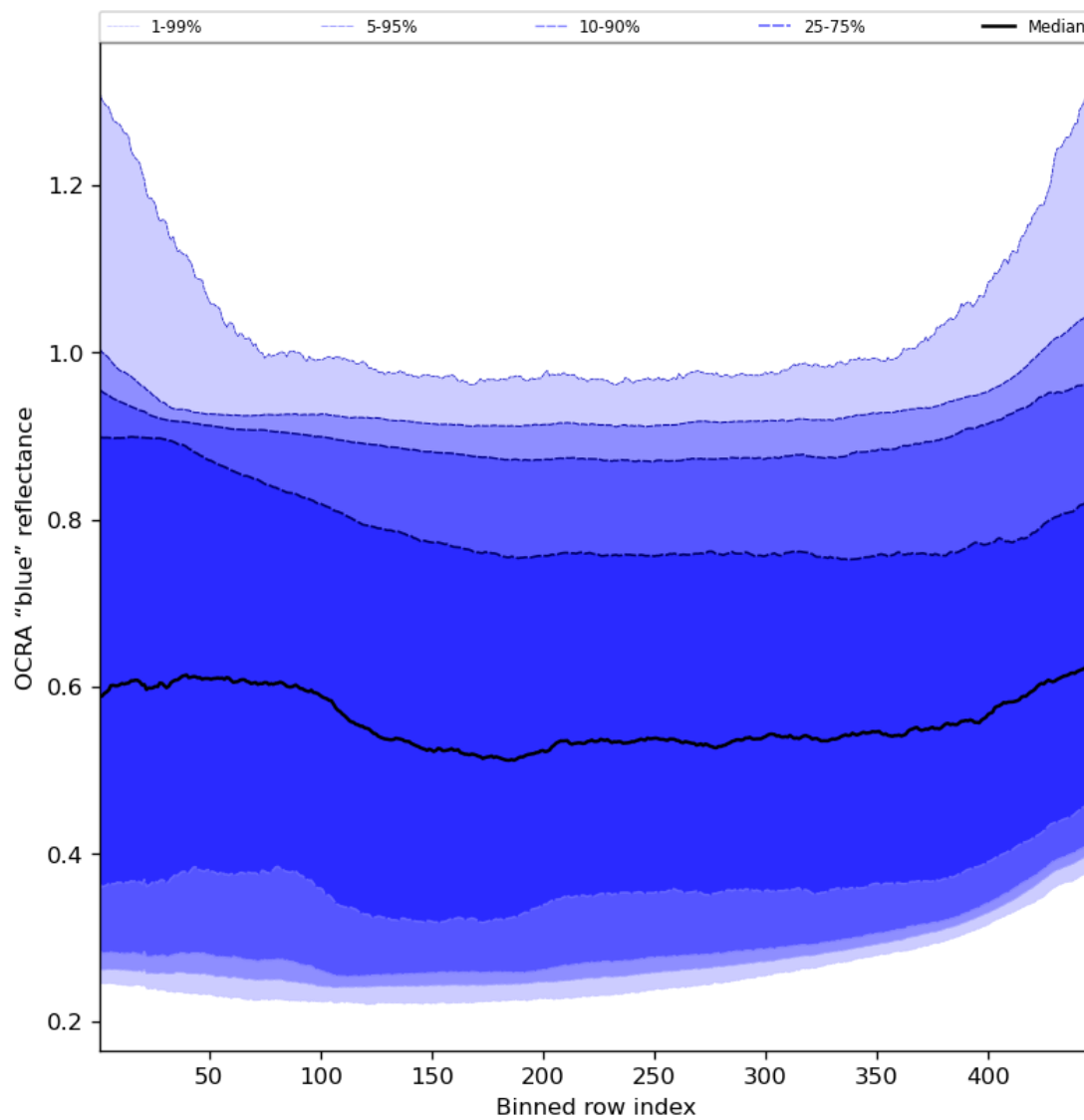
Figure 67: Along track statistics of “OCRA “blue” reflectance” for 2024-01-05 to 2024-01-06
