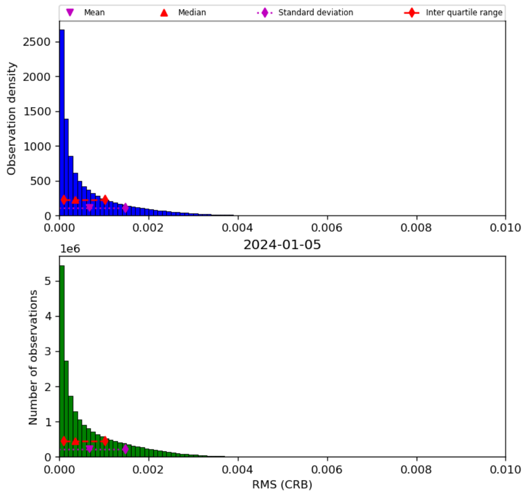
Figure 48: Histogram of “RMS (CRB)” for 2024-01-05 to 2024-01-06
