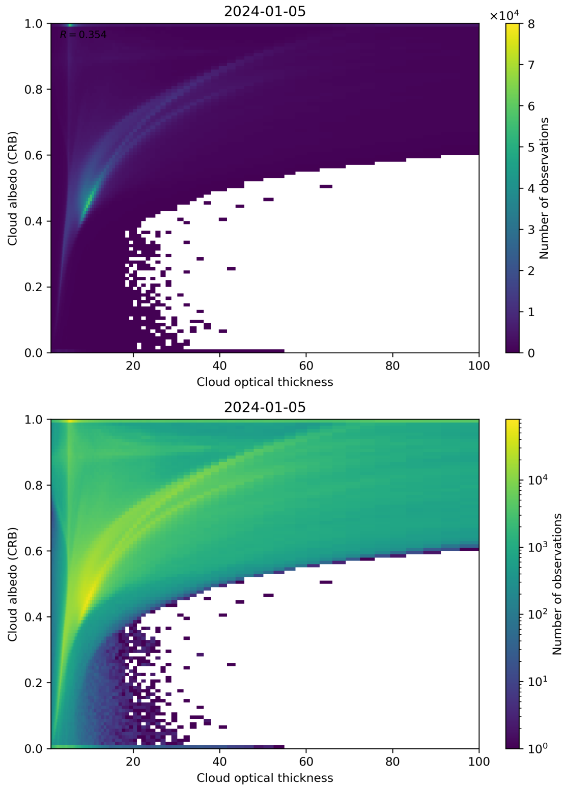
Figure 82: Scatter density plot of “Cloud optical thickness” against “Cloud albedo (CRB)” for 2024-01-05 to 2024-01-06.
