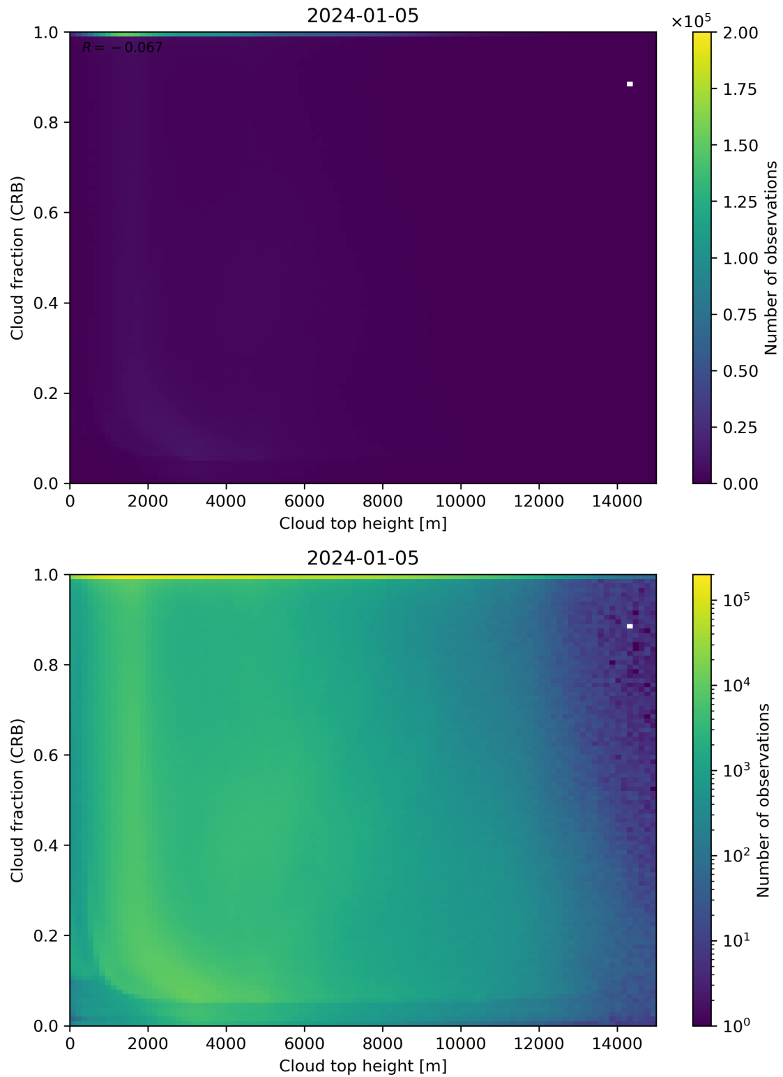
Figure 88: Scatter density plot of “Cloud top height” against “Cloud fraction (CRB)” for 2024-01-05 to 2024-01-06.
