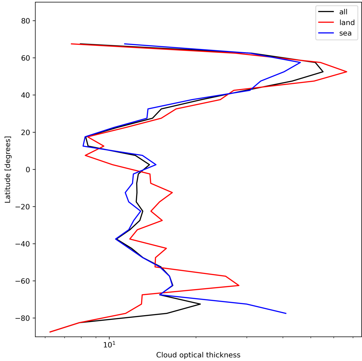
Figure 25: Zonal average of “Cloud optical thickness” for 2024-01-05 to 2024-01-06.
