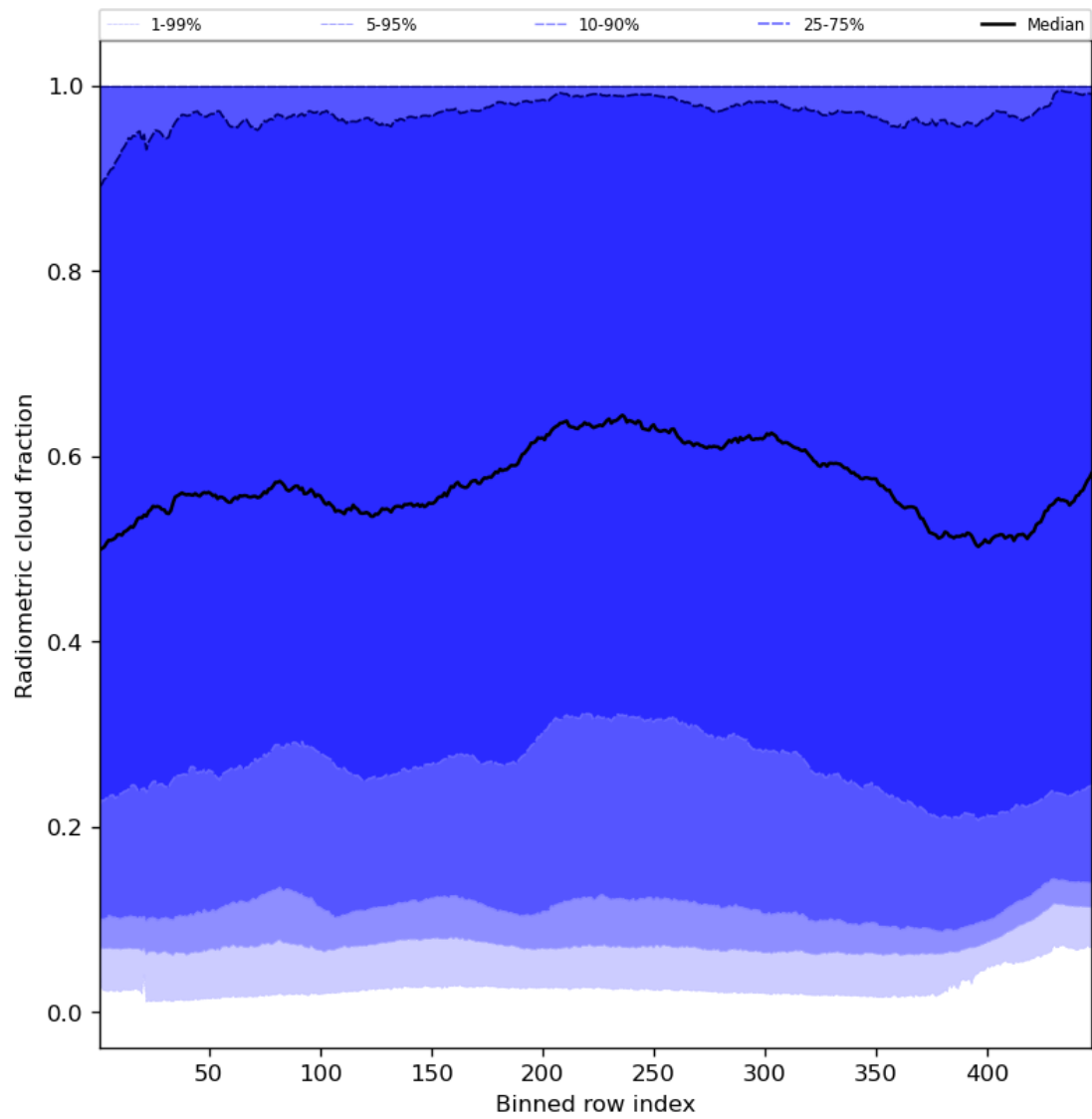
Figure 55: Along track statistics of “Radiometric cloud fraction” for 2024-01-05 to 2024-01-06
