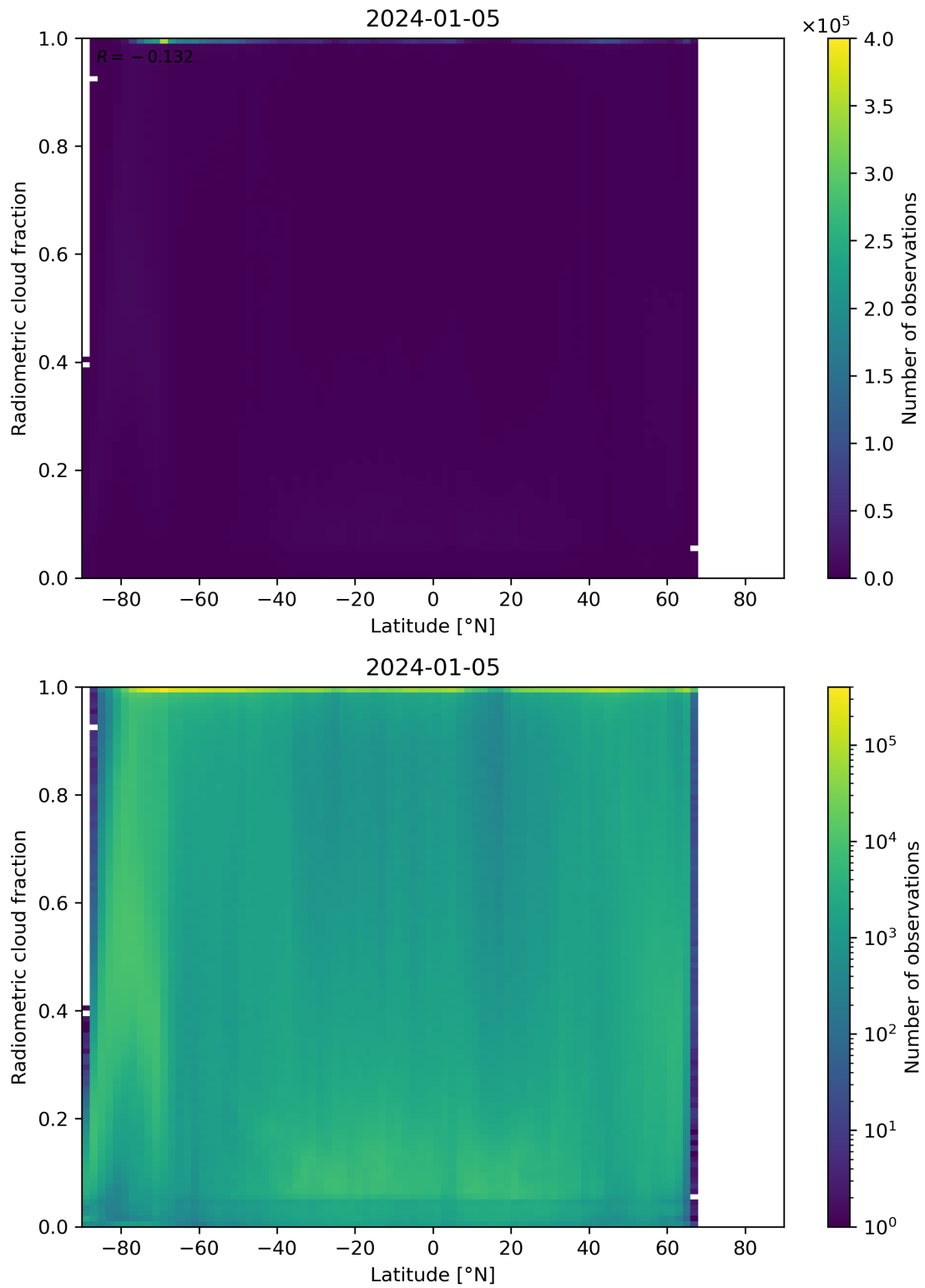
Figure 92: Scatter density plot of “Latitude” against “Radiometric cloud fraction” for 2024-01-05 to 2024-01-06.
