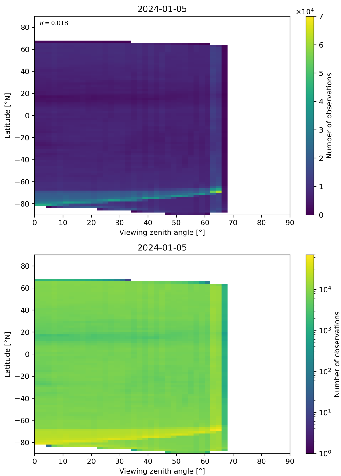
Figure 113: Scatter density plot of “Viewing zenith angle” against “Latitude” for 2024-01-05 to 2024-01-06.
