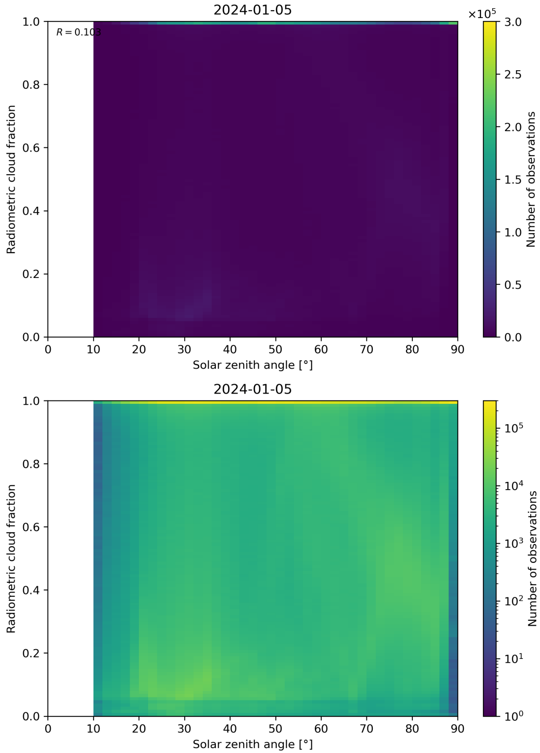
Figure 99: Scatter density plot of “Solar zenith angle” against “Radiometric cloud fraction” for 2024-01-05 to 2024-01-06.
