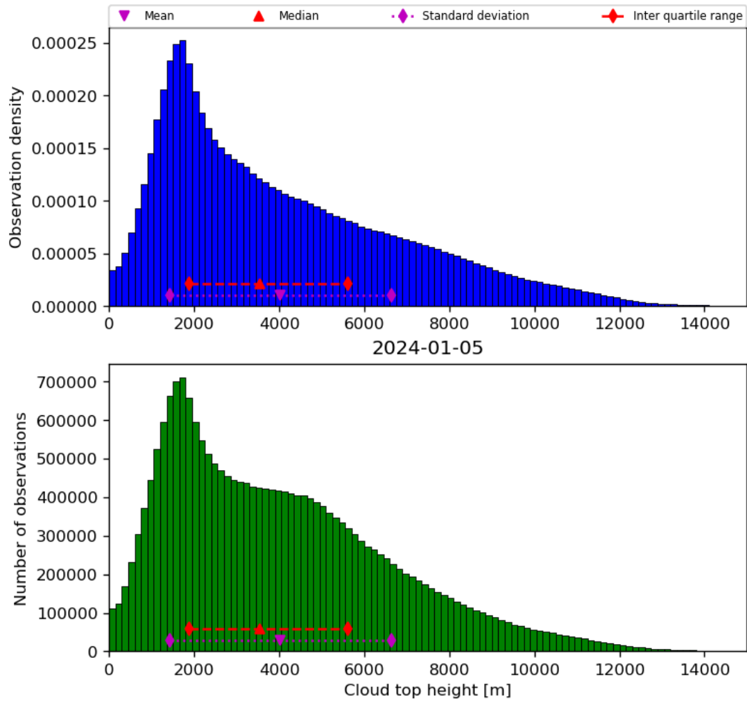
Figure 40: Histogram of “Cloud top height” for 2024-01-05 to 2024-01-06
