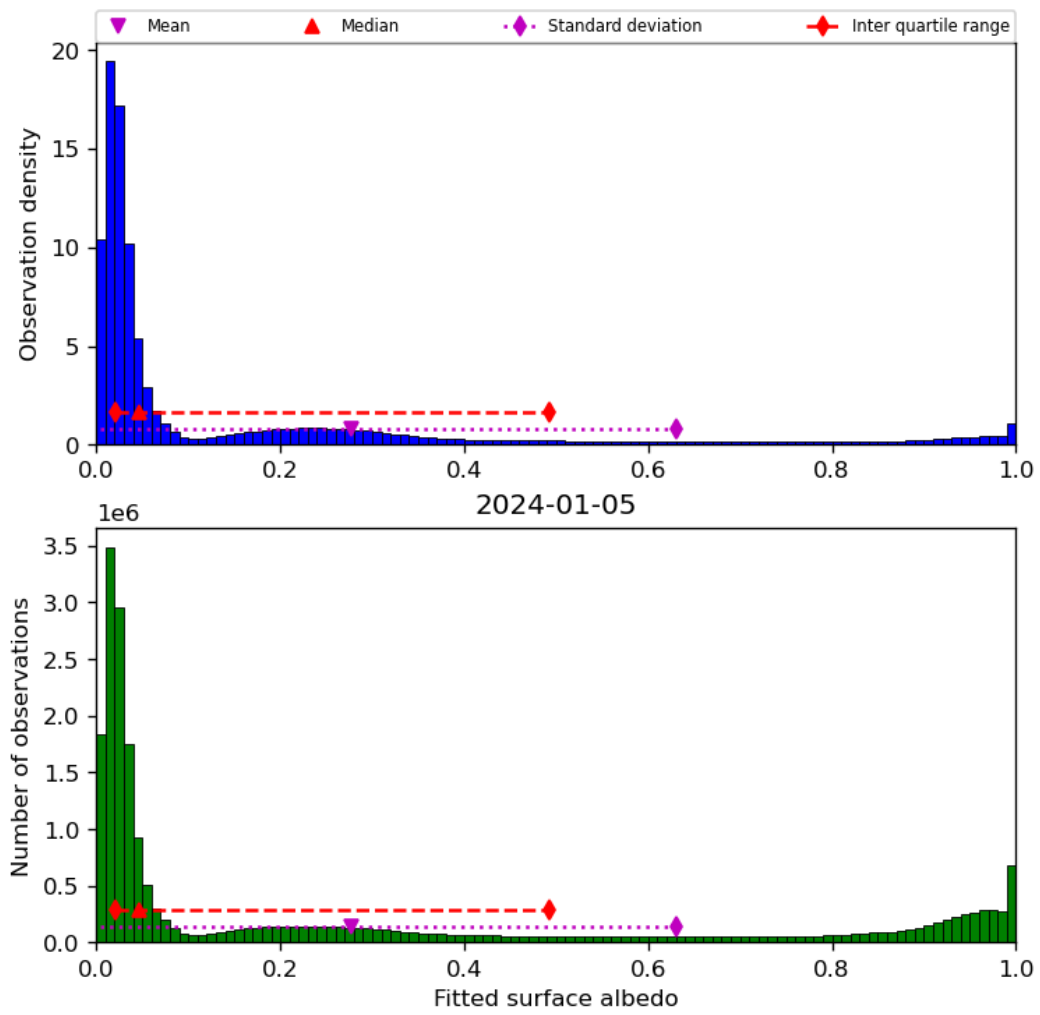
Figure 45: Histogram of “Fitted surface albedo” for 2024-01-05 to 2024-01-06
