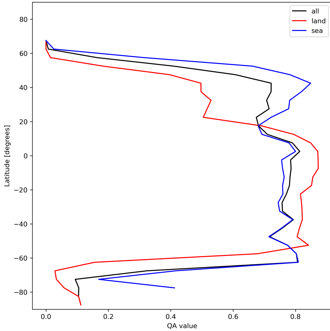
Figure 22: Zonal average of “QA value” for 2024-01-05 to 2024-01-06.
