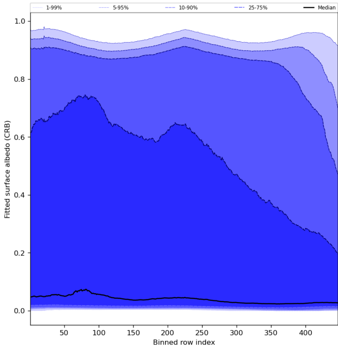
Figure 62: Along track statistics of “Fitted surface albedo (CRB)” for 2024-01-05 to 2024-01-06
