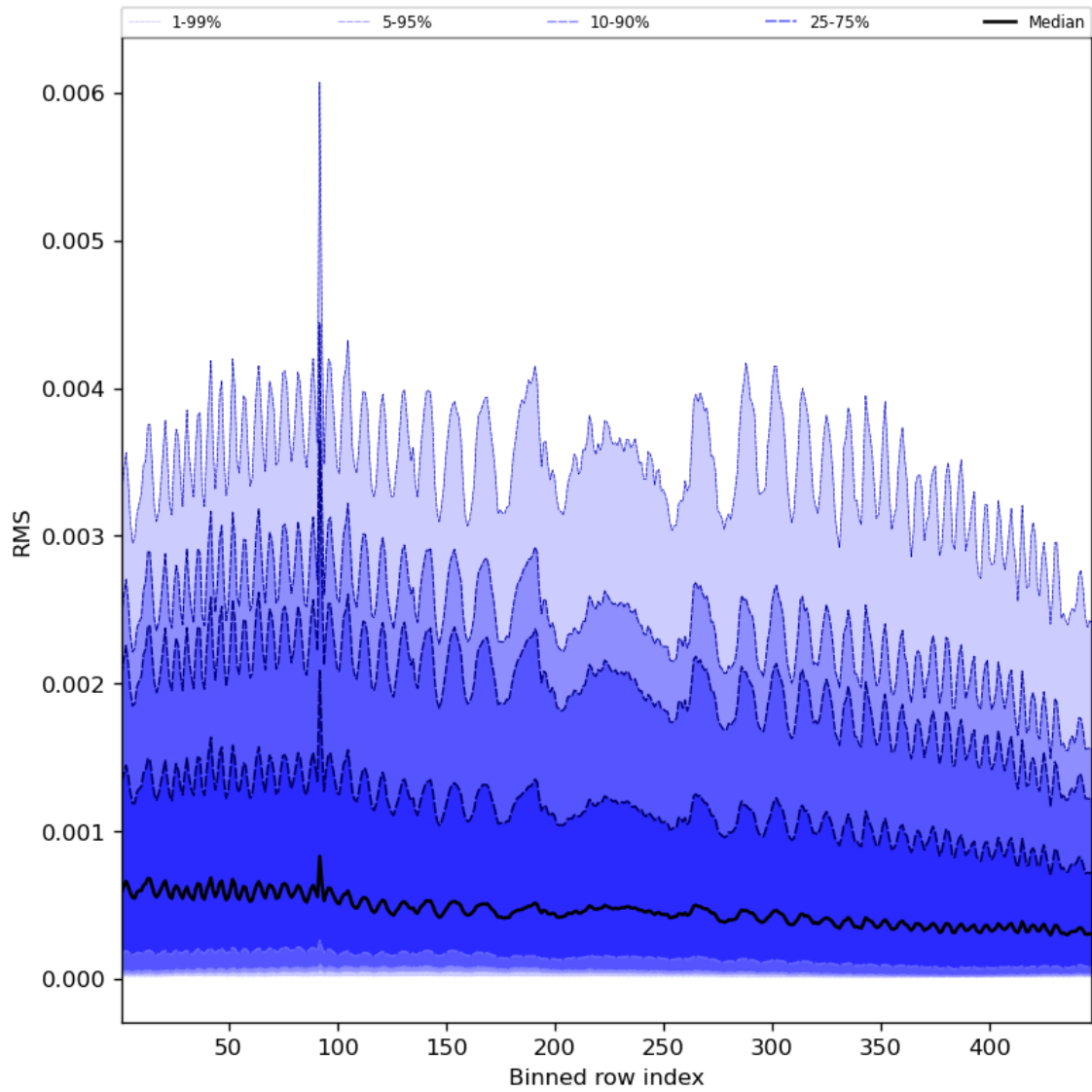
Figure 63: Along track statistics of “RMS” for 2024-01-05 to 2024-01-06
