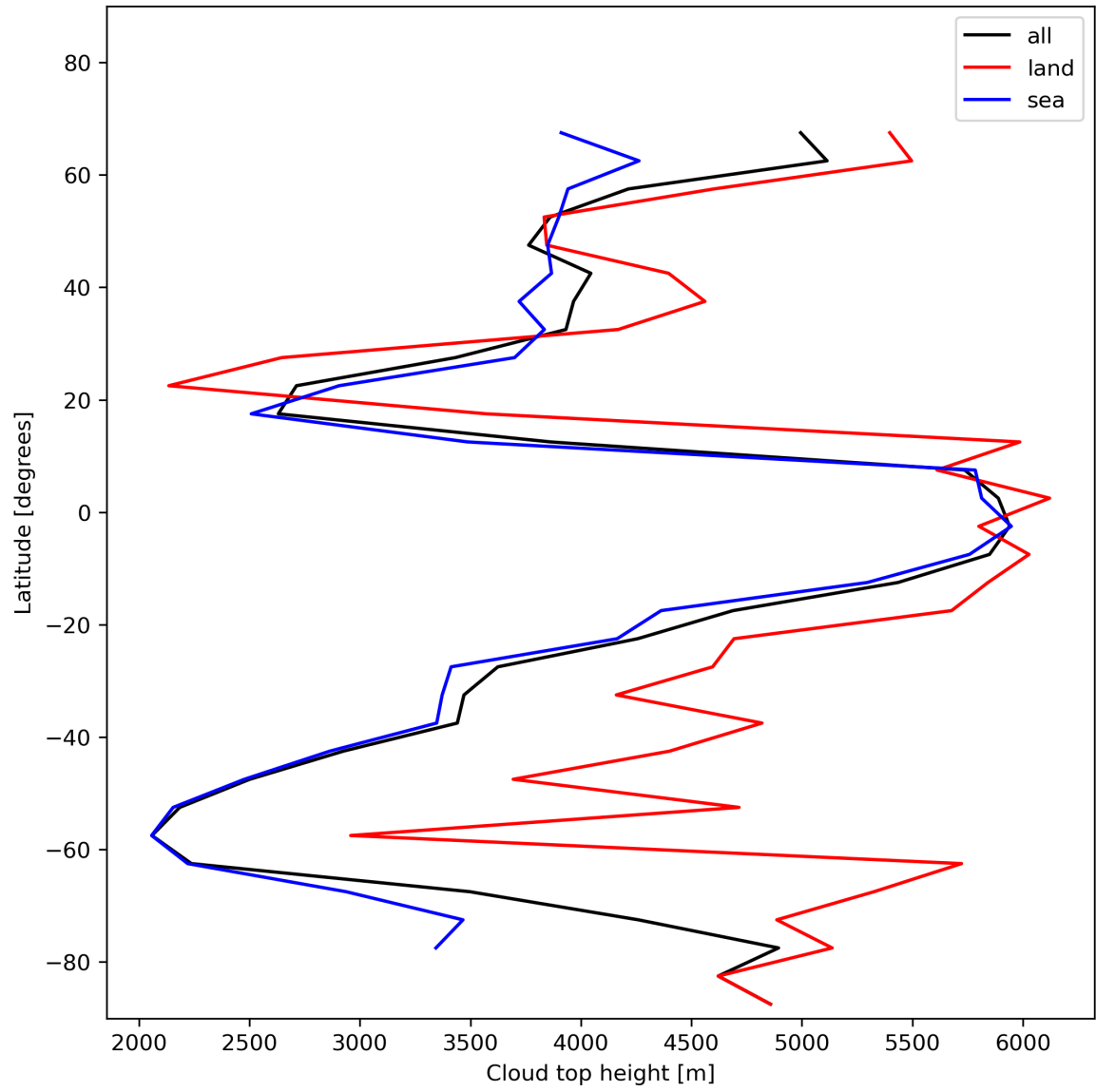
Figure 24: Zonal average of “Cloud top height” for 2024-01-05 to 2024-01-06.
