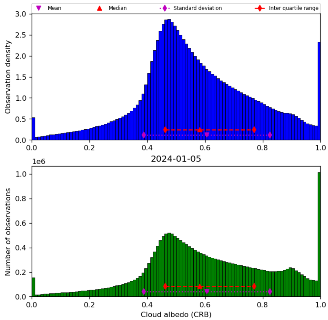
Figure 44: Histogram of “Cloud albedo (CRB)” for 2024-01-05 to 2024-01-06
