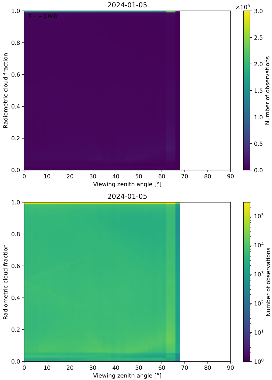
Figure 107: Scatter density plot of “Viewing zenith angle” against “Radiometric cloud fraction” for 2024-01-05 to 2024-01-06.
