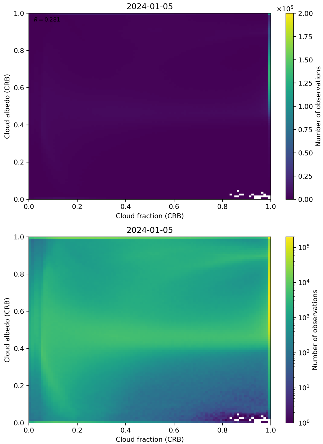
Figure 77: Scatter density plot of “Cloud fraction (CRB)” against “Cloud albedo (CRB)” for 2024-01-05 to 2024-01-06.
