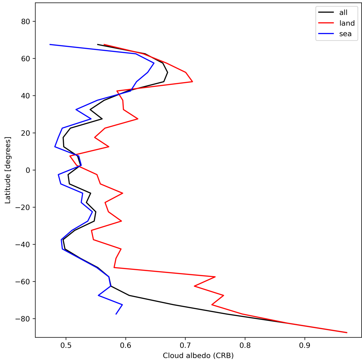
Figure 28: Zonal average of “Cloud albedo (CRB)” for 2024-01-05 to 2024-01-06.
