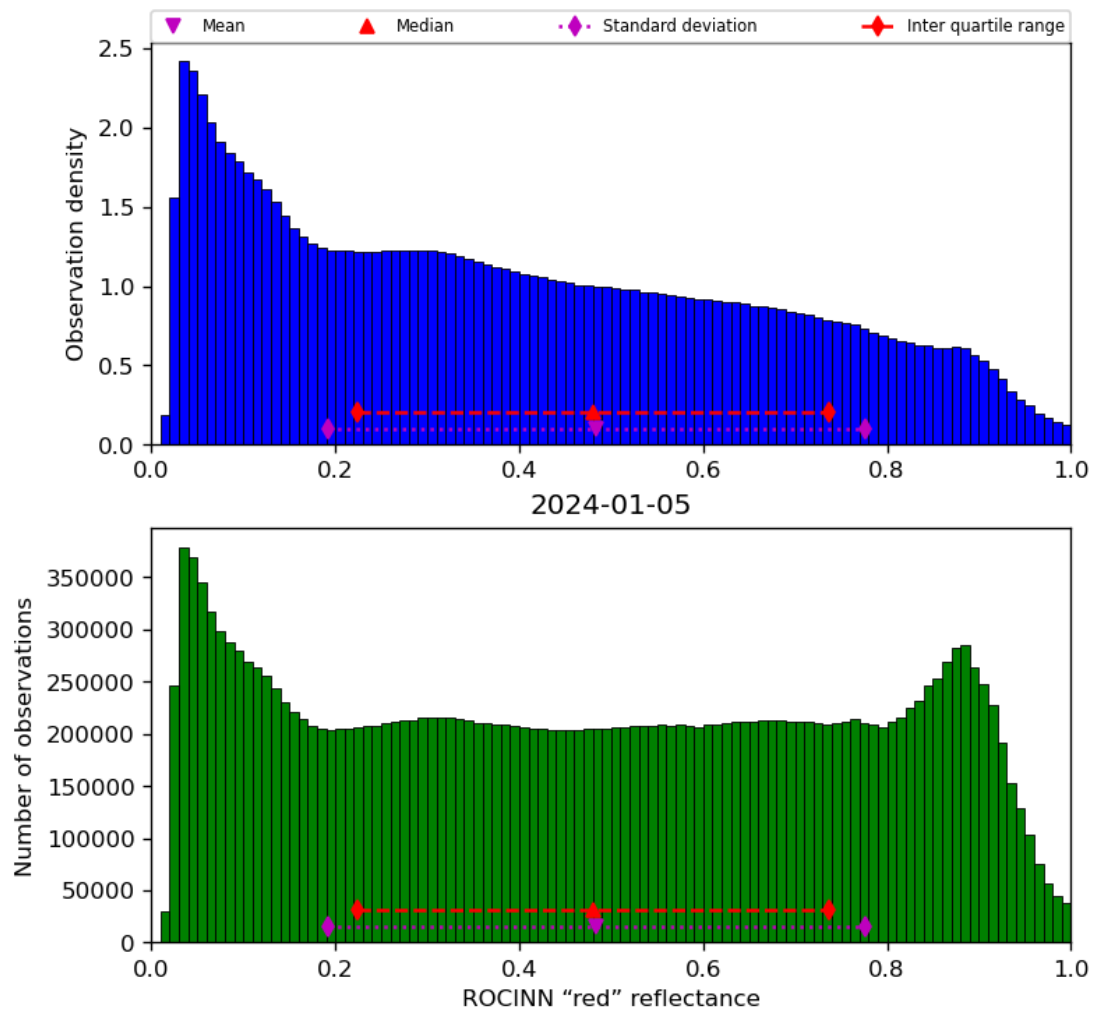
Figure 53: Histogram of “ROCINN “red” reflectance” for 2024-01-05 to 2024-01-06
