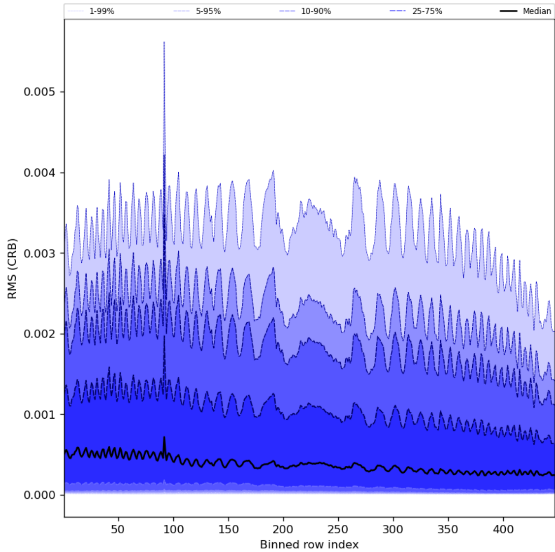
Figure 64: Along track statistics of “RMS (CRB)” for 2024-01-05 to 2024-01-06
