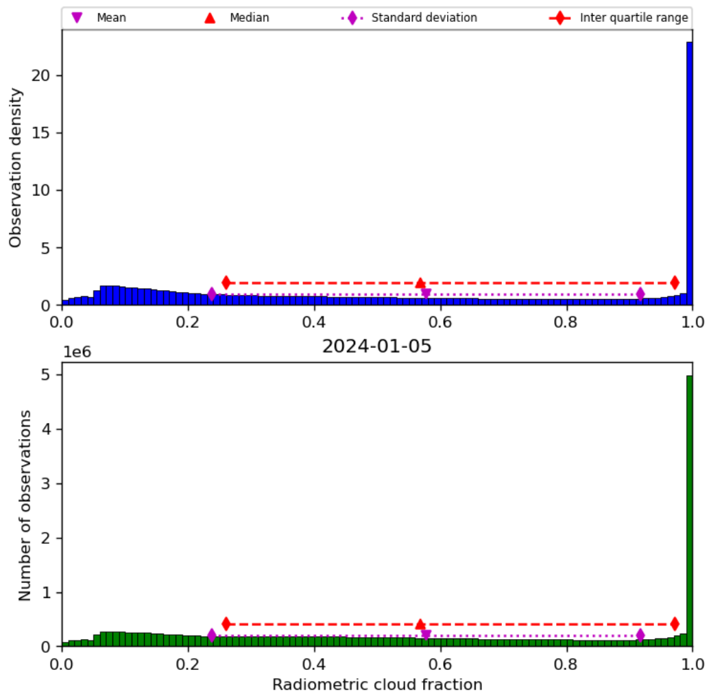
Figure 39: Histogram of “Radiometric cloud fraction” for 2024-01-05 to 2024-01-06
