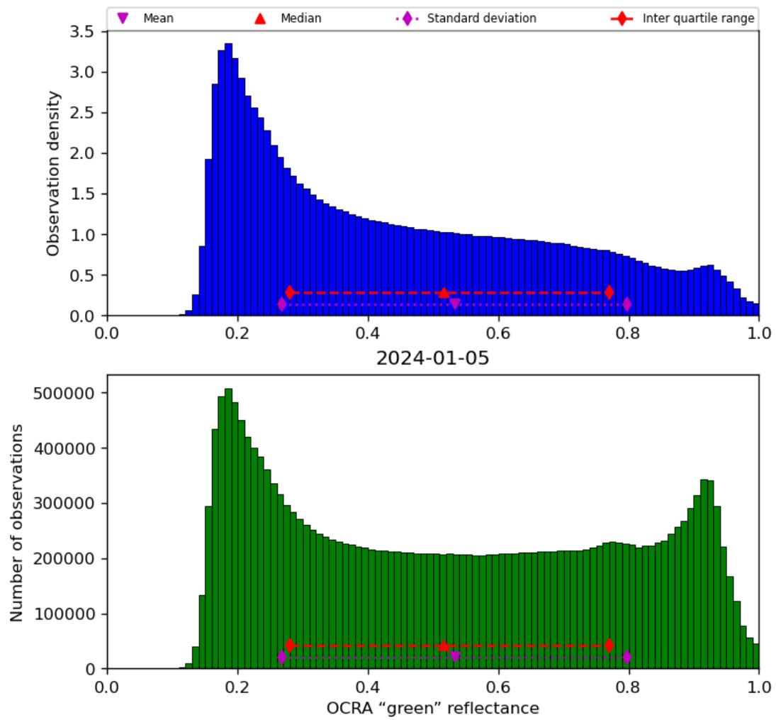
Figure 52: Histogram of “OCRA “green” reflectance” for 2024-01-05 to 2024-01-06
