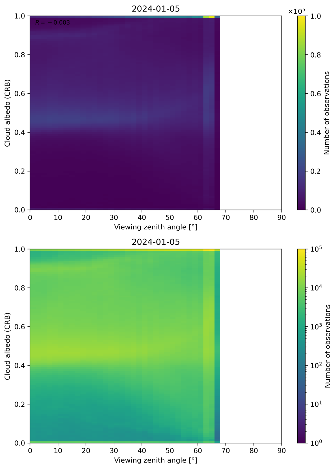
Figure 106: Scatter density plot of “Viewing zenith angle” against “Cloud albedo (CRB)” for 2024-01-05 to 2024-01-06.
