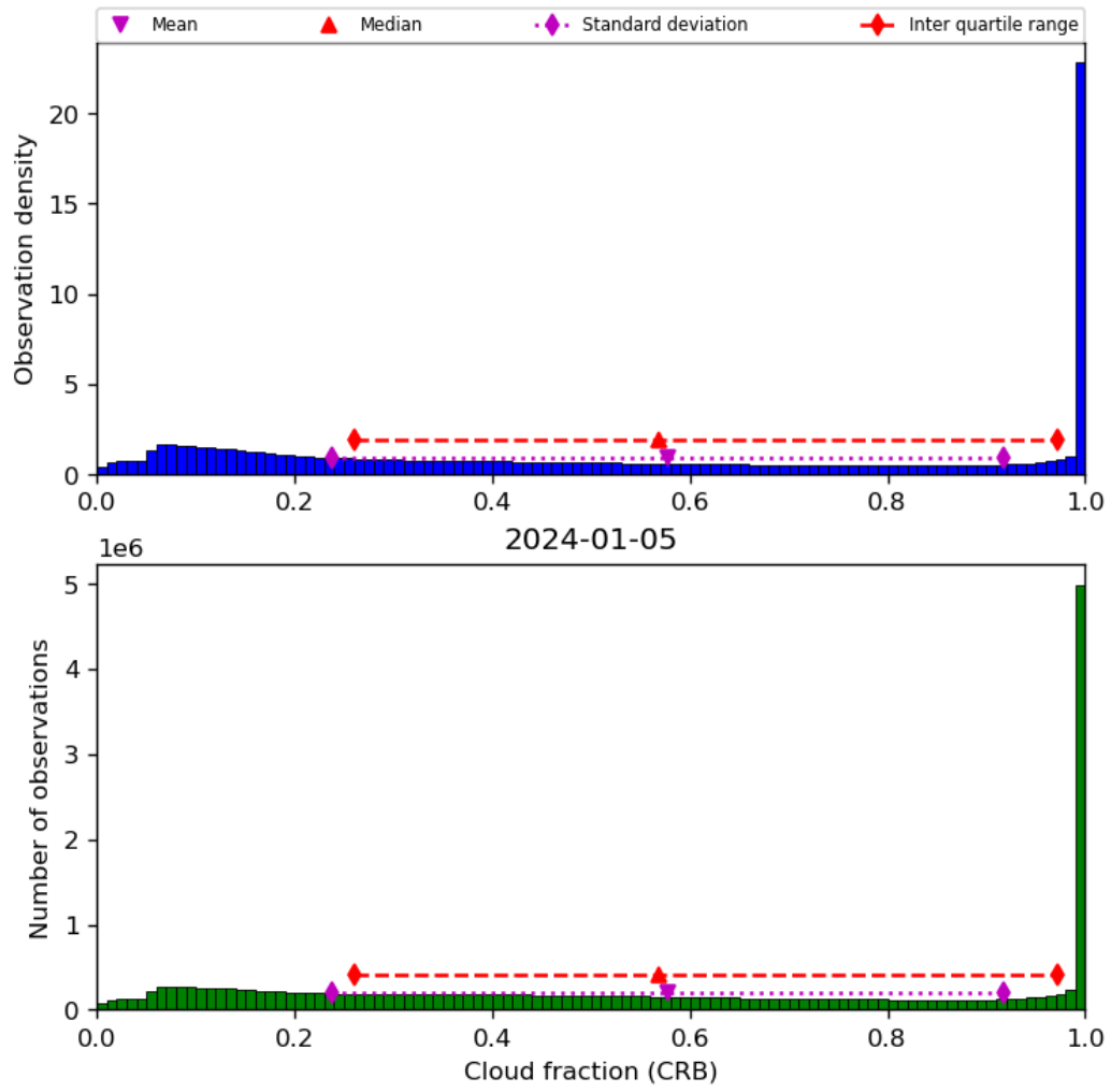
Figure 42: Histogram of “Cloud fraction (CRB)” for 2024-01-05 to 2024-01-06
