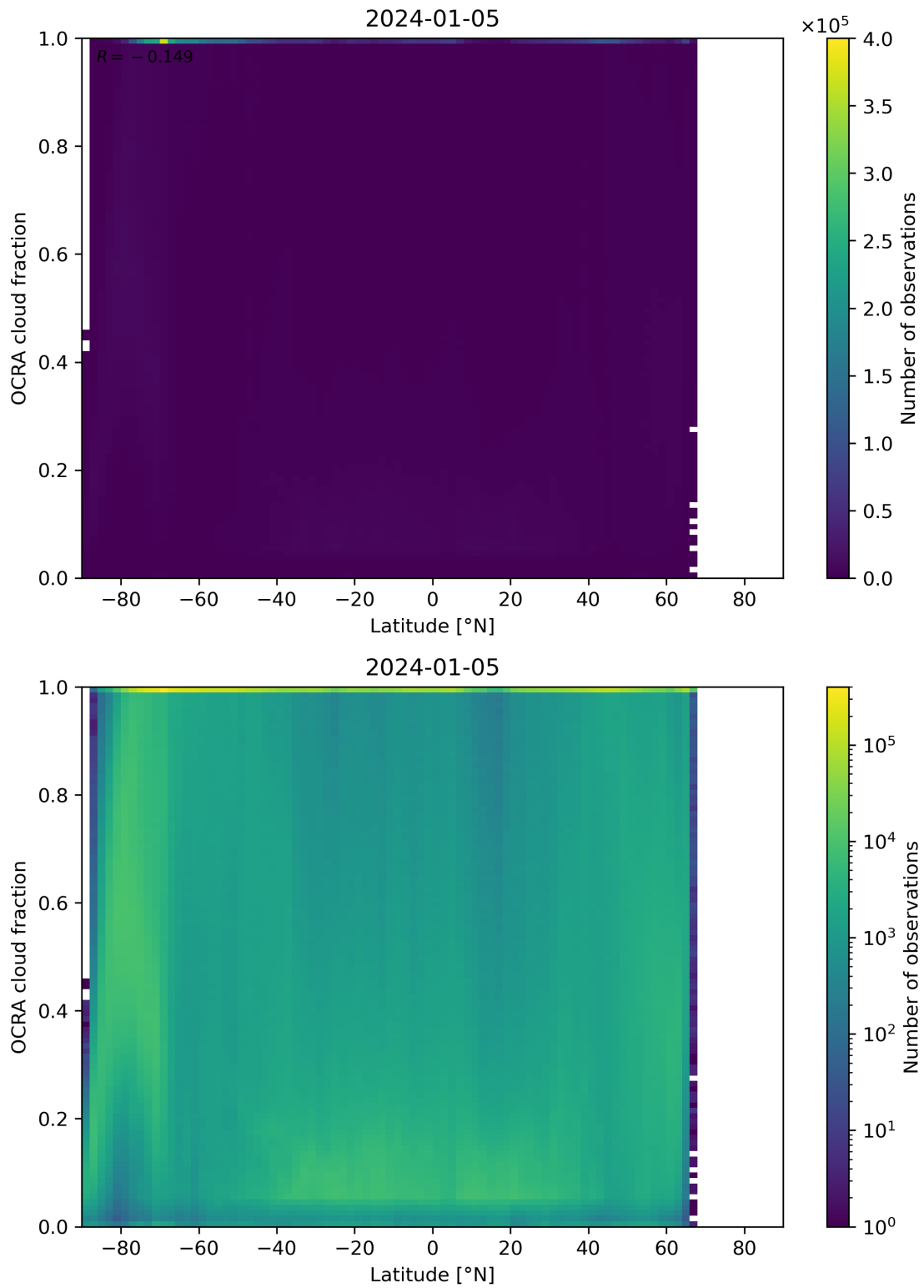
Figure 93: Scatter density plot of “Latitude” against “OCRA cloud fraction” for 2024-01-05 to 2024-01-06.
