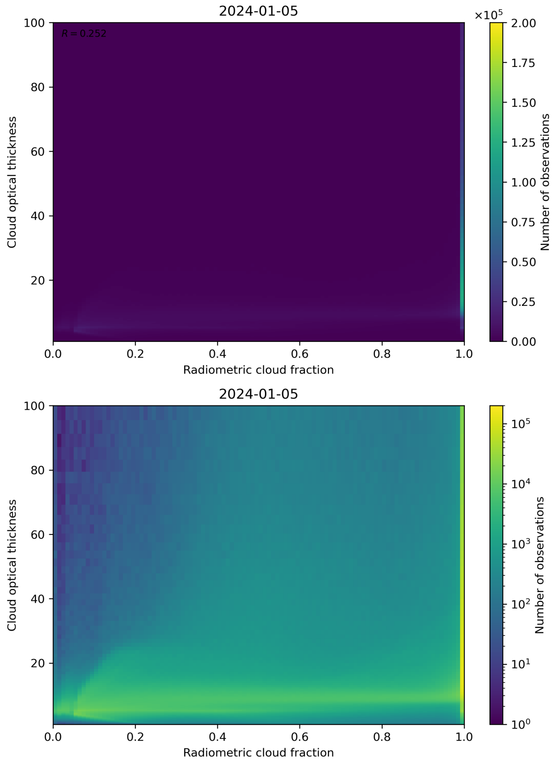
Figure 75: Scatter density plot of “Radiometric cloud fraction” against “Cloud optical thickness” for 2024-01-05 to 2024-01-06.
