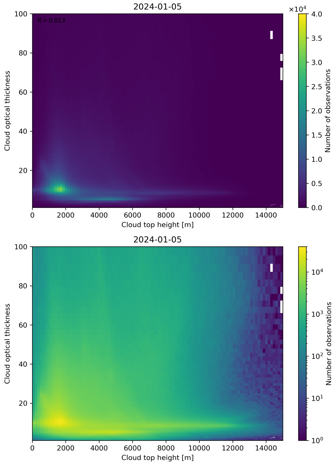
Figure 90: Scatter density plot of “Cloud top height” against “Cloud optical thickness” for 2024-01-05 to 2024-01-06.
