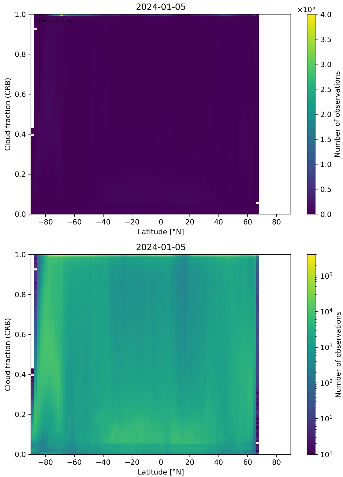
Figure 94: Scatter density plot of “Latitude” against “Cloud fraction (CRB)” for 2024-01-05 to 2024-01-06.
