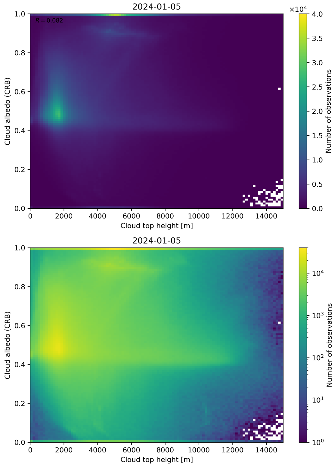
Figure 86: Scatter density plot of “Cloud top height” against “Cloud albedo (CRB)” for 2024-01-05 to 2024-01-06.
