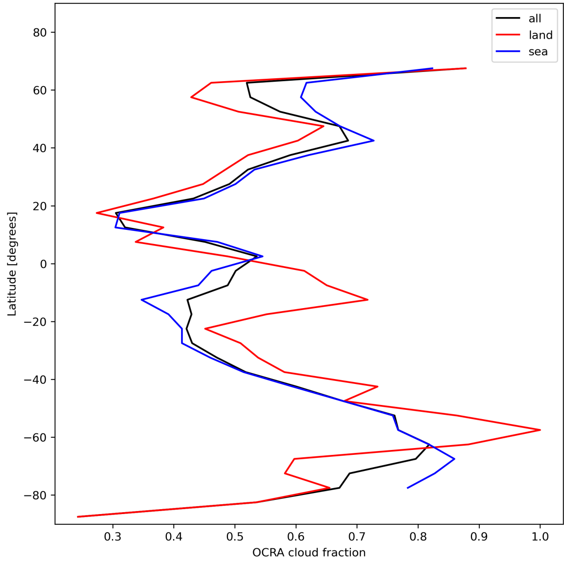
Figure 34: Zonal average of “OCRA cloud fraction” for 2024-01-05 to 2024-01-06.
