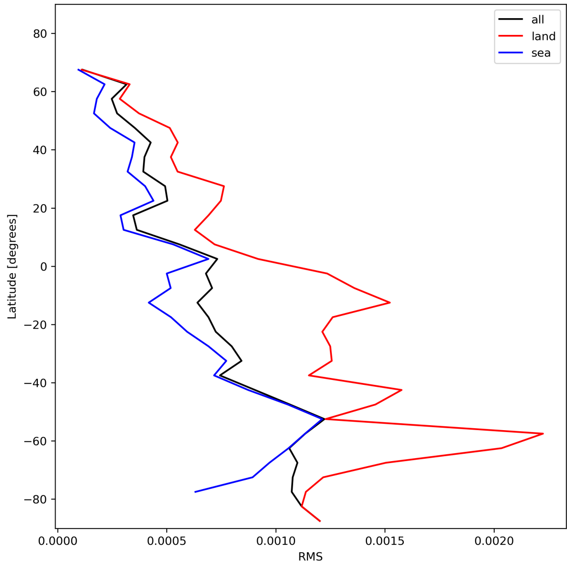
Figure 31: Zonal average of “RMS” for 2024-01-05 to 2024-01-06.
