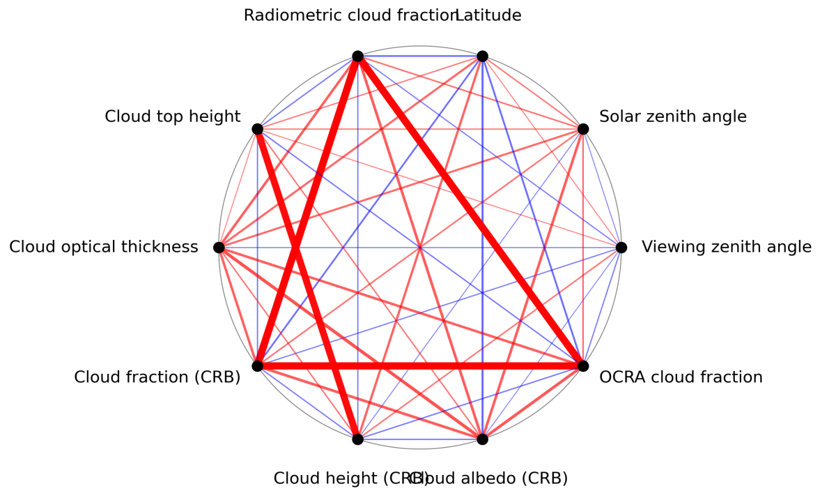
Figure 1: Map of correlation graph for 2024-01-05 to 2024-01-06.
