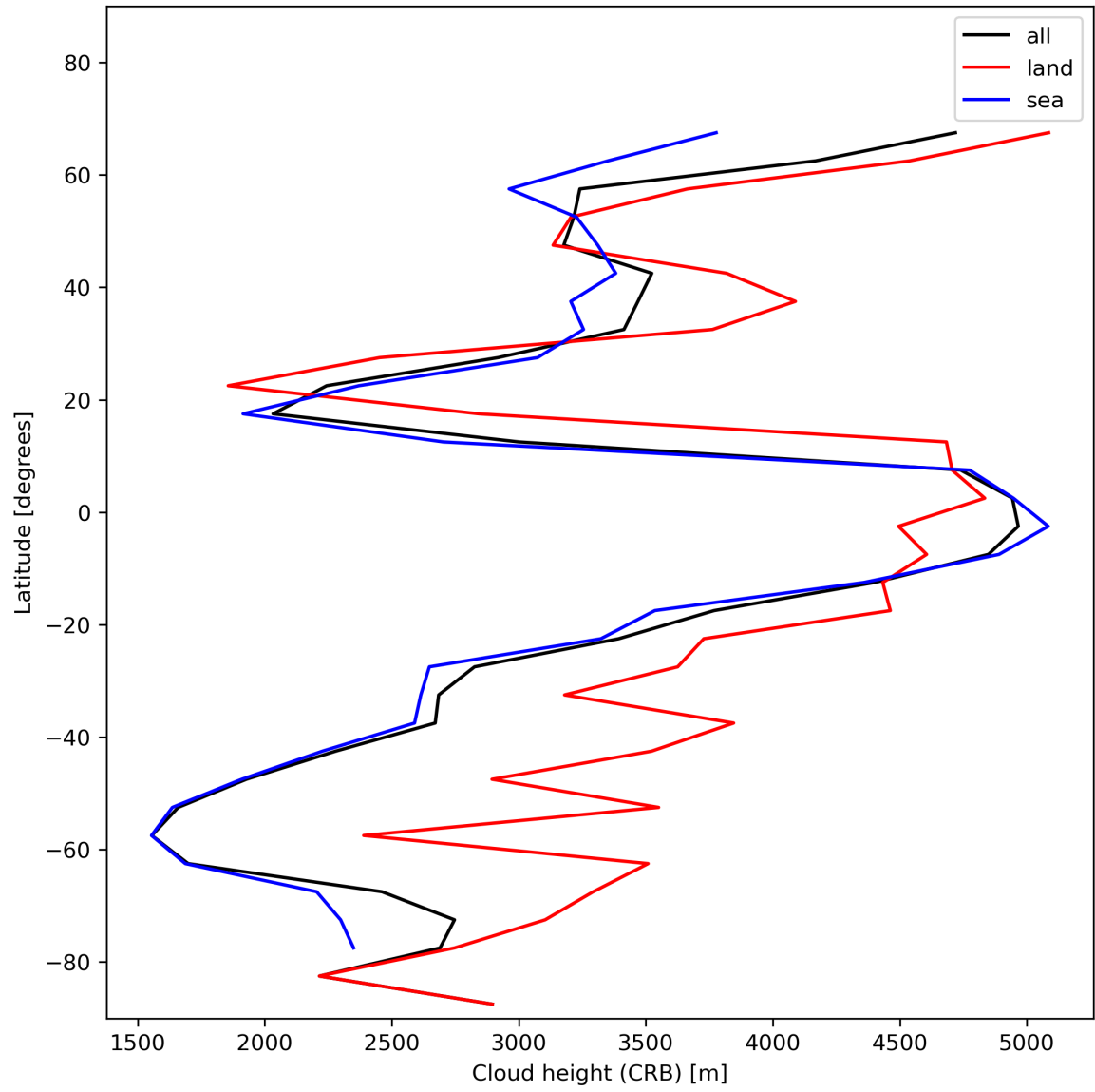
Figure 27: Zonal average of “Cloud height (CRB)” for 2024-01-05 to 2024-01-06.
