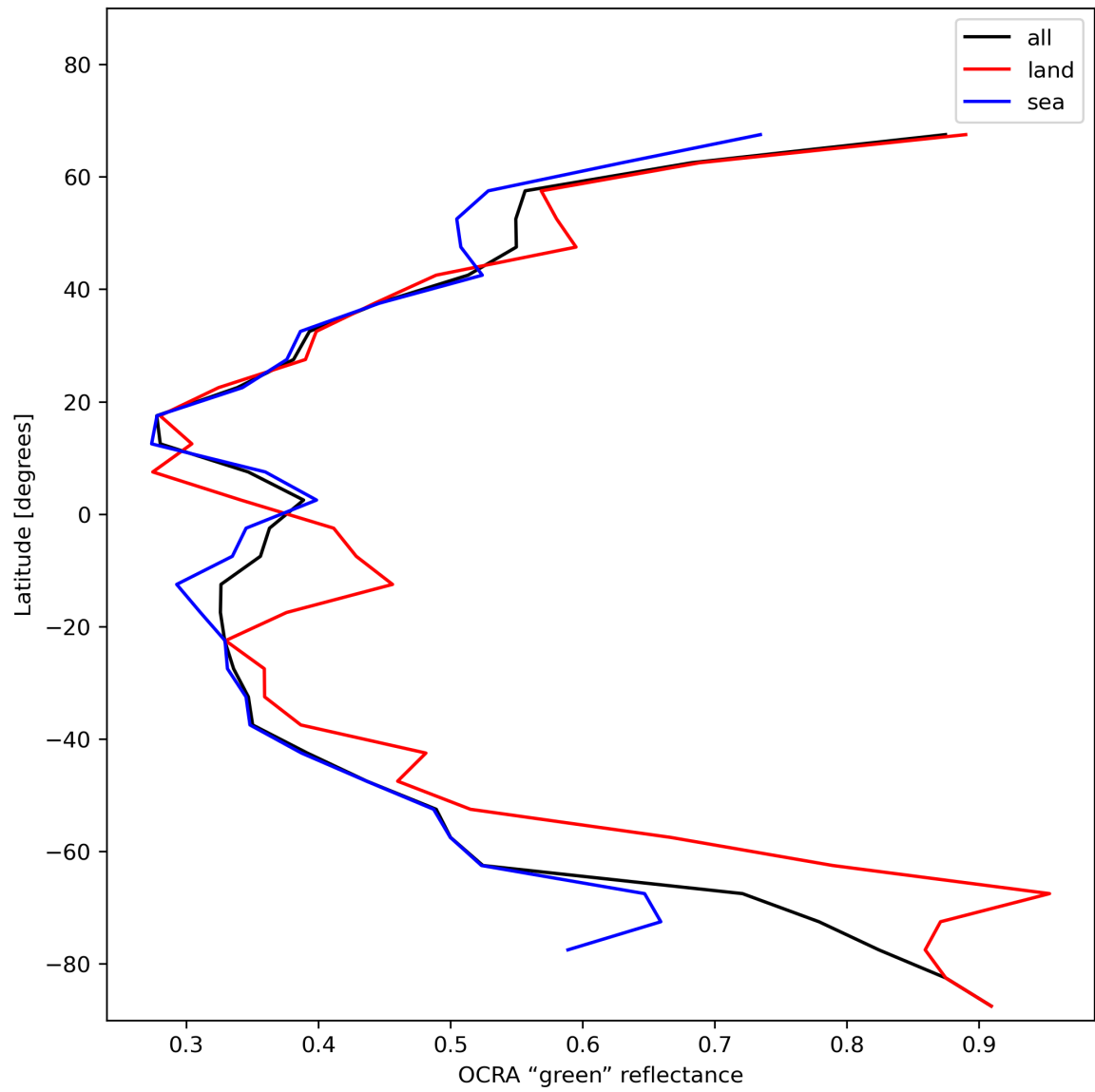
Figure 36: Zonal average of “OCRA “green” reflectance” for 2024-01-05 to 2024-01-06.
