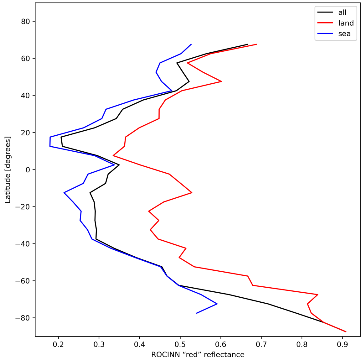
Figure 37: Zonal average of “ROCINN “red” reflectance” for 2024-01-05 to 2024-01-06.
