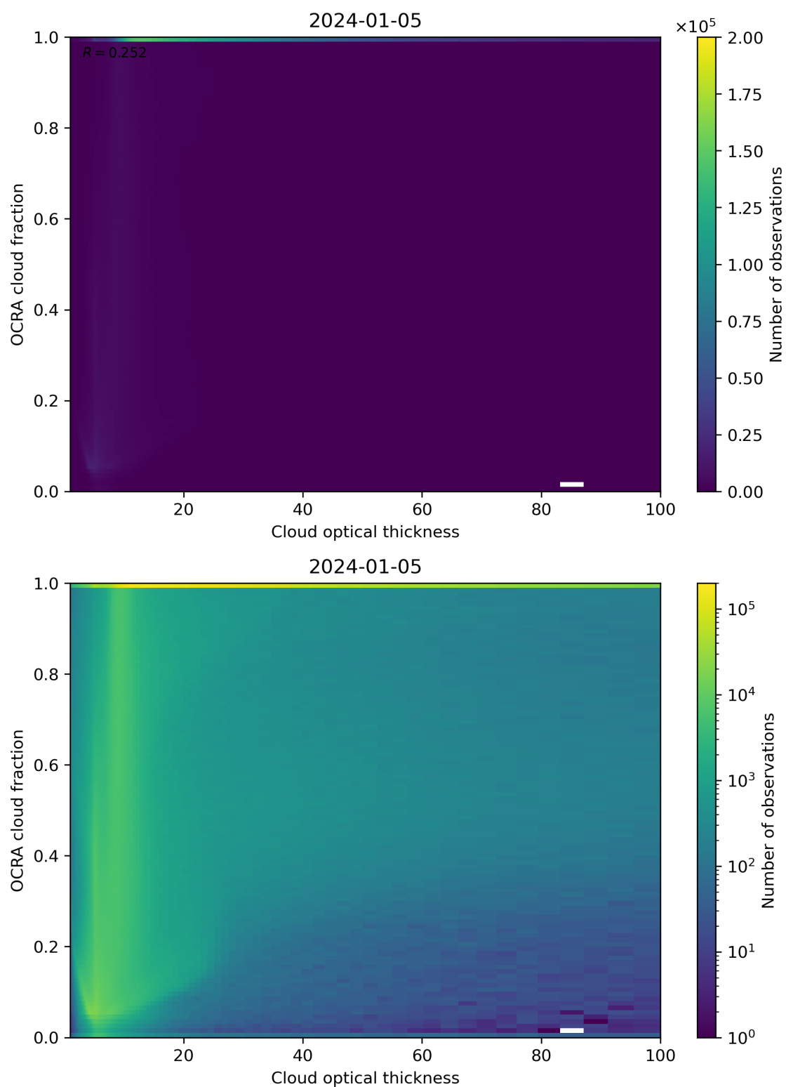
Figure 83: Scatter density plot of “Cloud optical thickness” against “OCRA cloud fraction” for 2024-01-05 to 2024-01-06.
