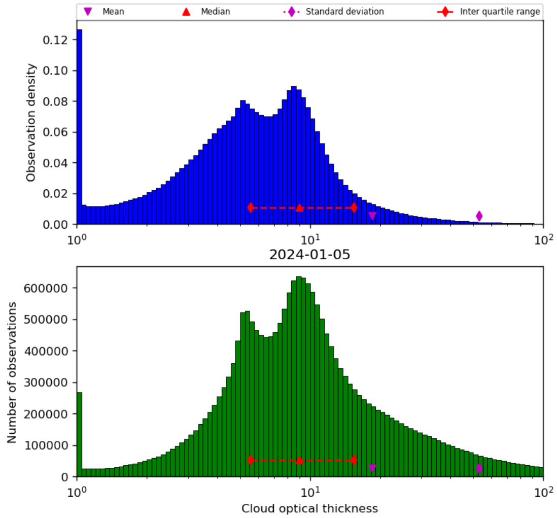
Figure 41: Histogram of “Cloud optical thickness” for 2024-01-05 to 2024-01-06
