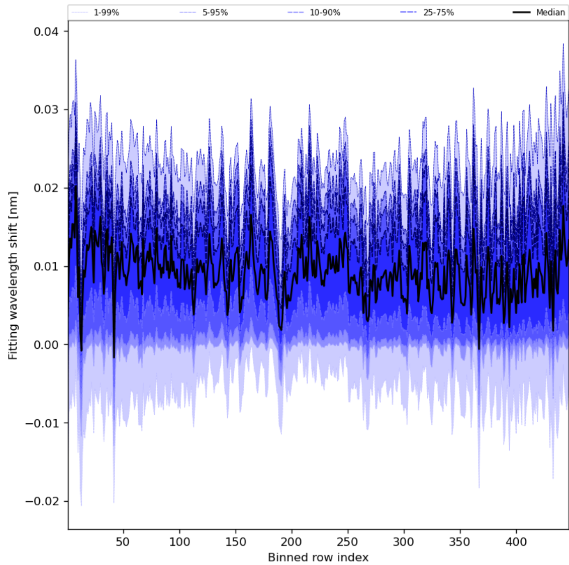
Figure 65: Along track statistics of “Fitting wavelength shift” for 2024-01-05 to 2024-01-06
