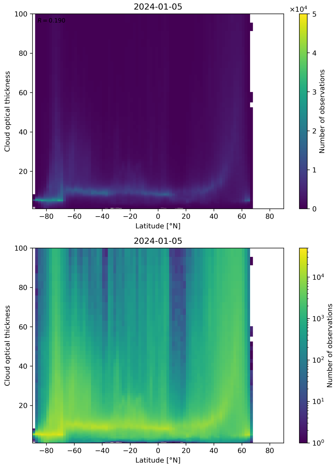
Figure 96: Scatter density plot of “Latitude” against “Cloud optical thickness” for 2024-01-05 to 2024-01-06.
