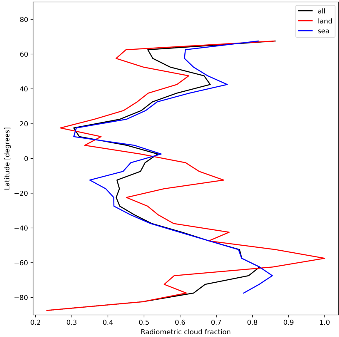
Figure 23: Zonal average of “Radiometric cloud fraction” for 2024-01-05 to 2024-01-06.
