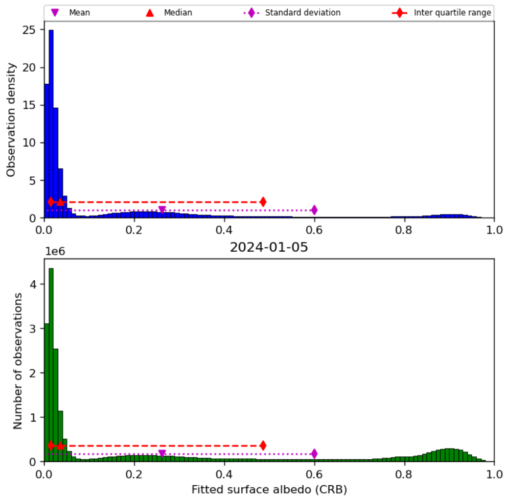
Figure 46: Histogram of “Fitted surface albedo (CRB)” for 2024-01-05 to 2024-01-06
