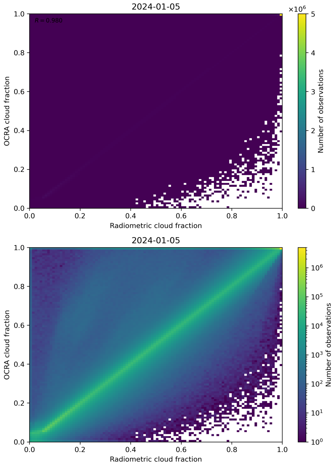
Figure 72: Scatter density plot of “Radiometric cloud fraction” against “OCRA cloud fraction” for 2024-01-05 to 2024-01-06.
