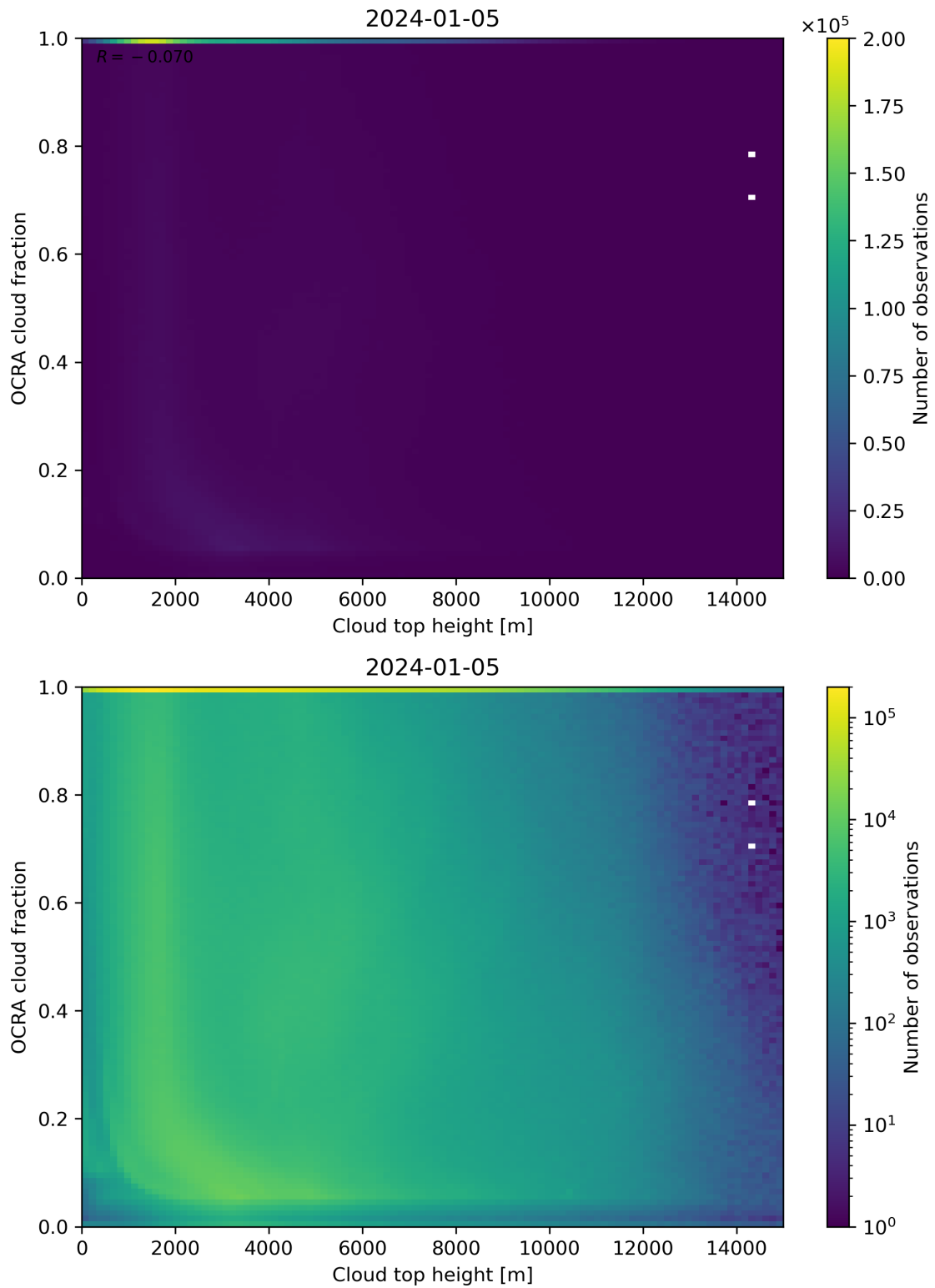
Figure 87: Scatter density plot of “Cloud top height” against “OCRA cloud fraction” for 2024-01-05 to 2024-01-06.
