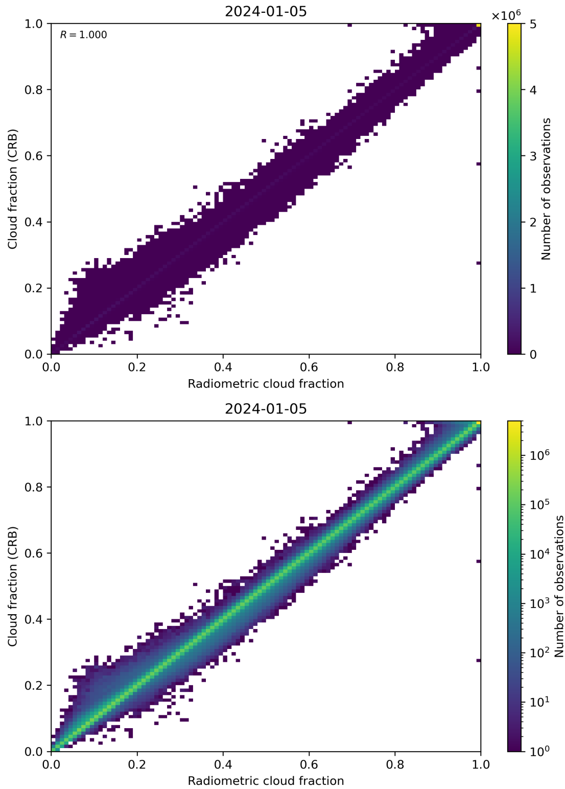
Figure 73: Scatter density plot of “Radiometric cloud fraction” against “Cloud fraction (CRB)” for 2024-01-05 to 2024-01-06.
