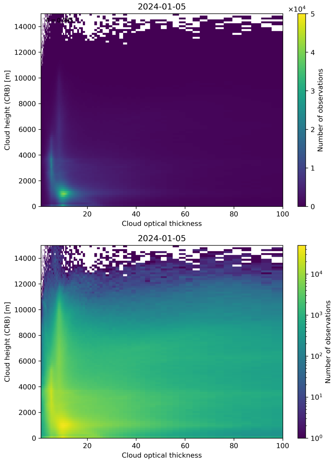
Figure 85: Scatter density plot of “Cloud optical thickness” against “Cloud height (CRB)” for 2024-01-05 to 2024-01-06.
