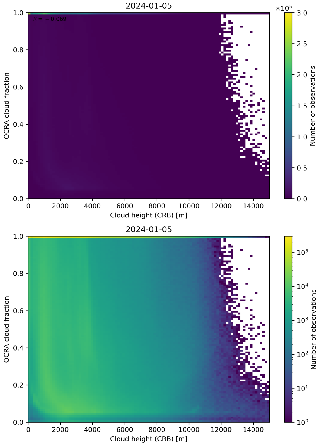
Figure 81: Scatter density plot of “Cloud height (CRB)” against “OCRA cloud fraction” for 2024-01-05 to 2024-01-06.
