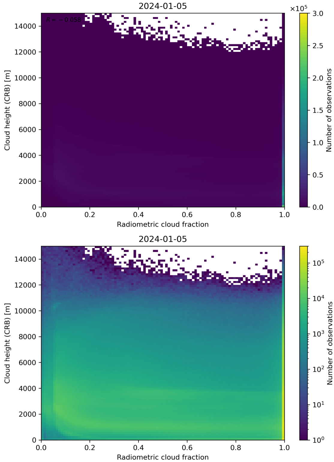
Figure 74: Scatter density plot of “Radiometric cloud fraction” against “Cloud height (CRB)” for 2024-01-05 to 2024-01-06.
