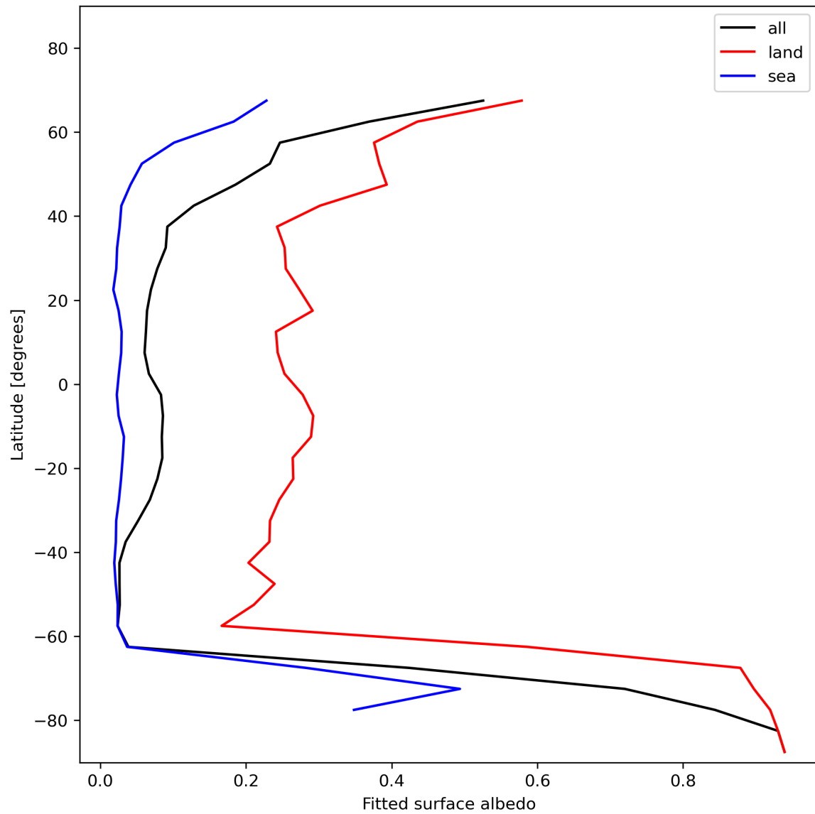
Figure 29: Zonal average of “Fitted surface albedo” for 2024-01-05 to 2024-01-06.
