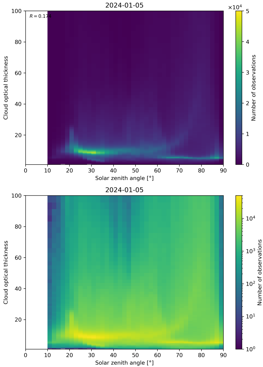
Figure 103: Scatter density plot of “Solar zenith angle” against “Cloud optical thickness” for 2024-01-05 to 2024-01-06.
