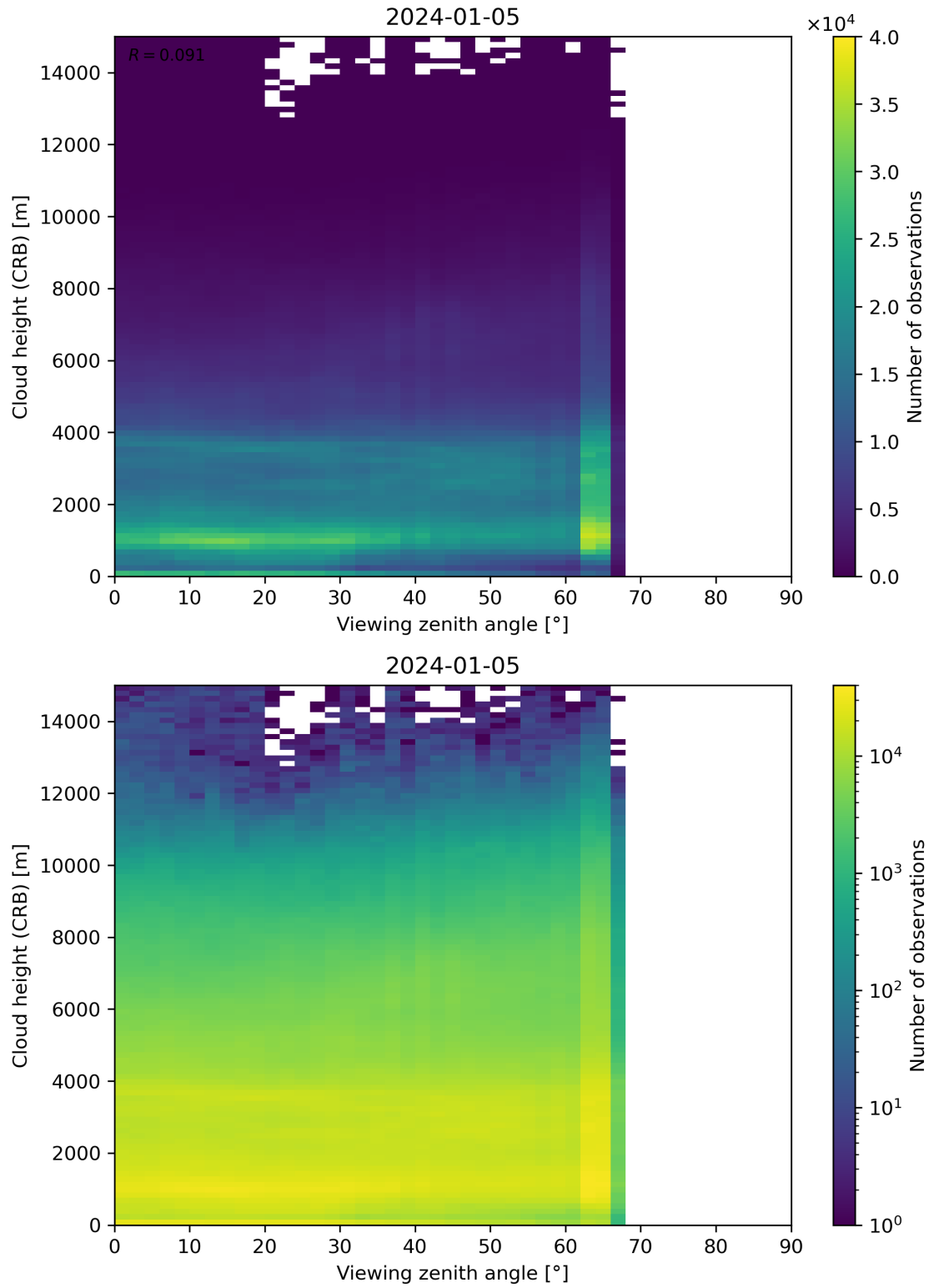
Figure 110: Scatter density plot of “Viewing zenith angle” against “Cloud height (CRB)” for 2024-01-05 to 2024-01-06.
