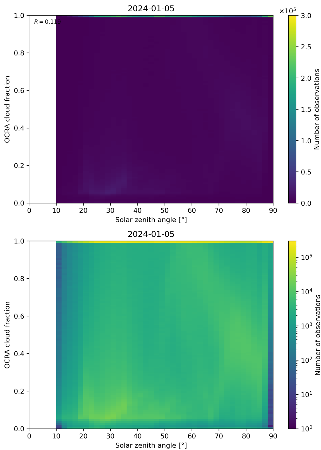
Figure 100: Scatter density plot of “Solar zenith angle” against “OCRA cloud fraction” for 2024-01-05 to 2024-01-06.
