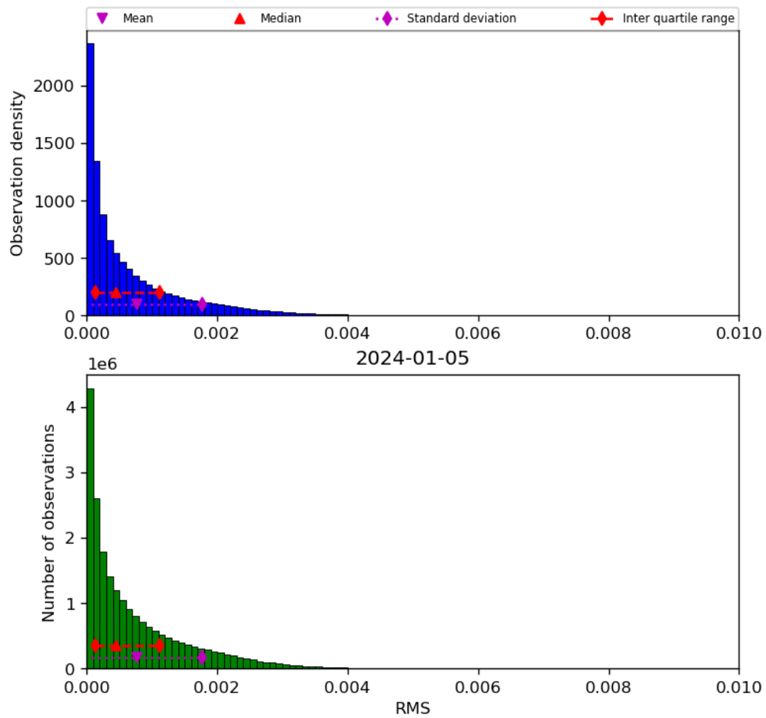
Figure 47: Histogram of “RMS” for 2024-01-05 to 2024-01-06
