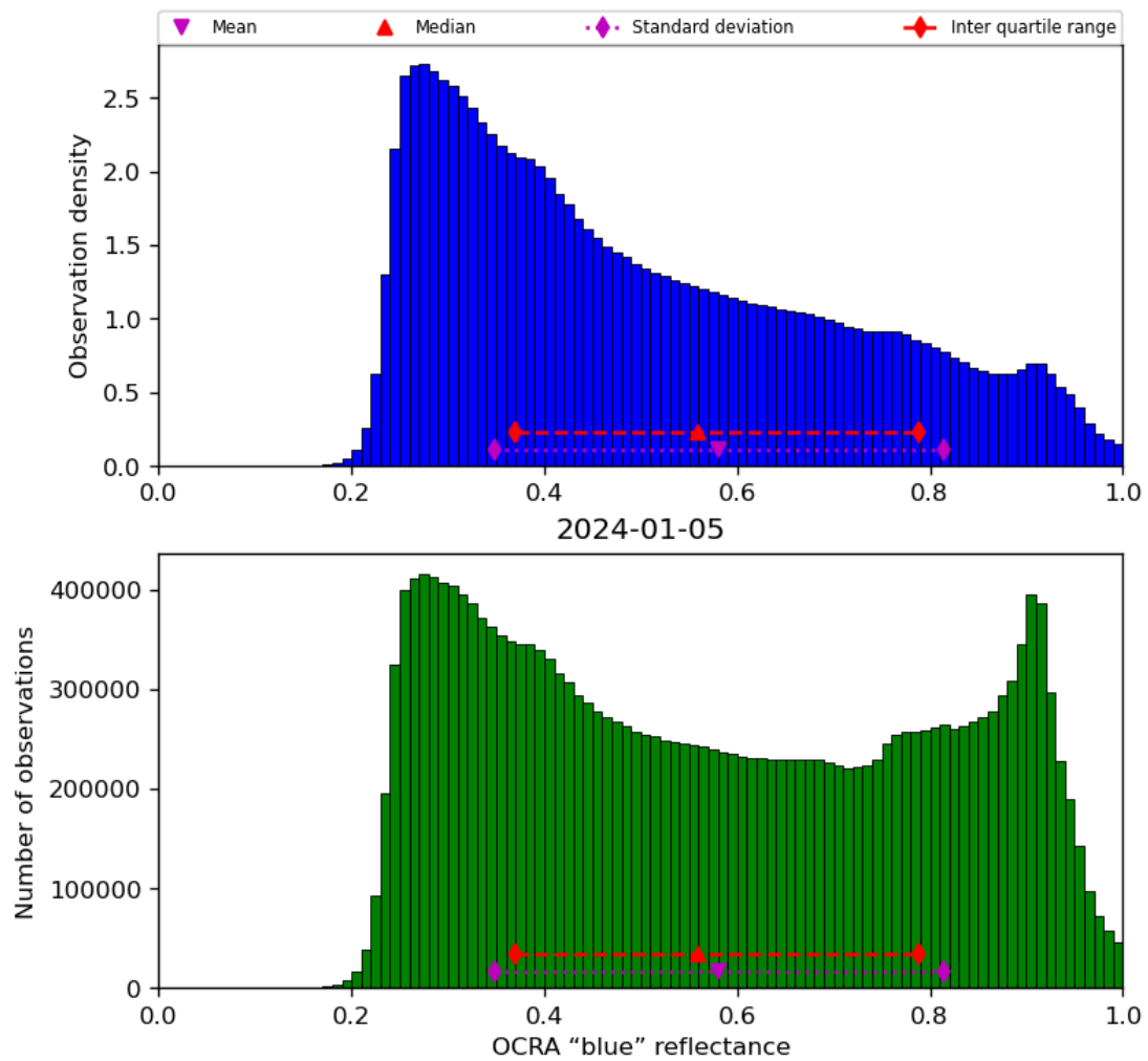
Figure 51: Histogram of “OCRA “blue” reflectance” for 2024-01-05 to 2024-01-06
