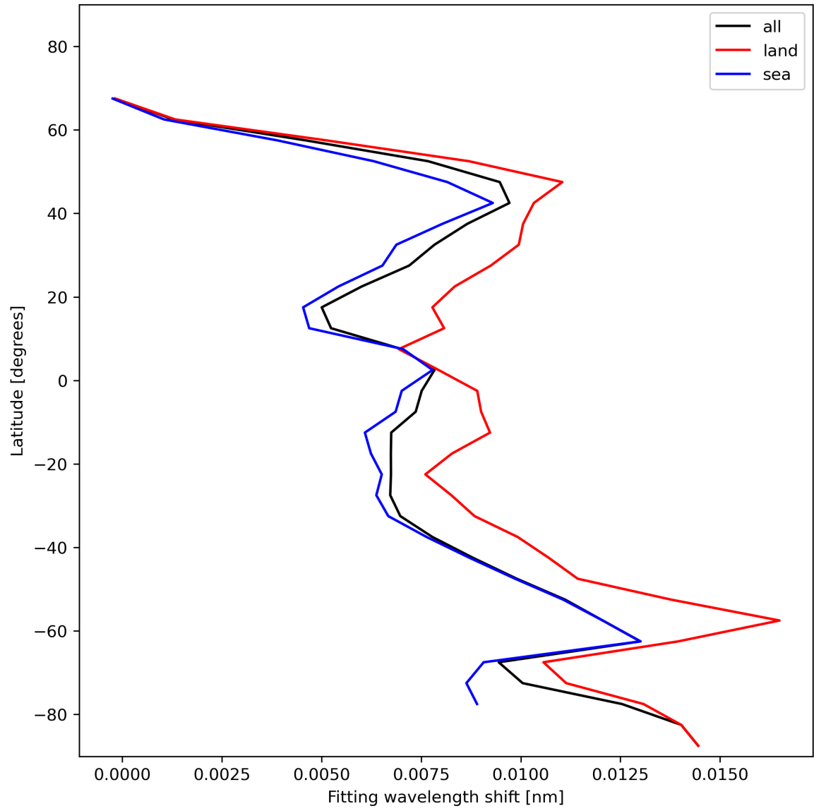
Figure 33: Zonal average of “Fitting wavelength shift” for 2024-01-05 to 2024-01-06.
