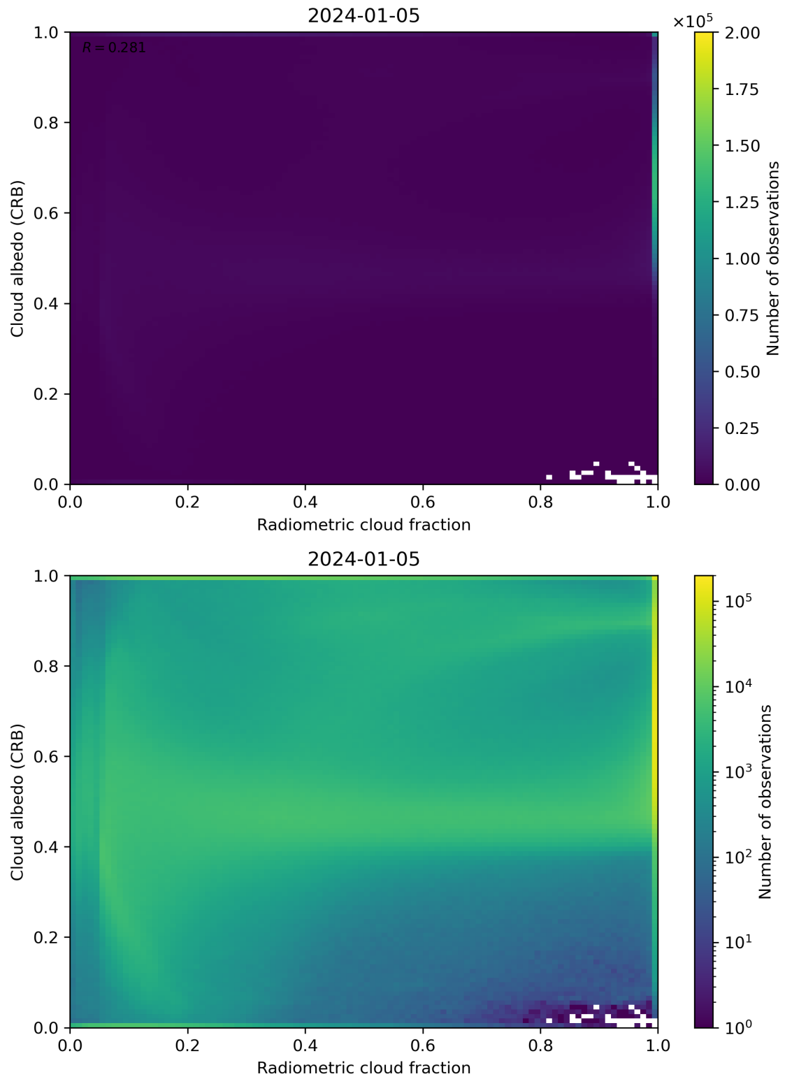
Figure 71: Scatter density plot of “Radiometric cloud fraction” against “Cloud albedo (CRB)” for 2024-01-05 to 2024-01-06.
