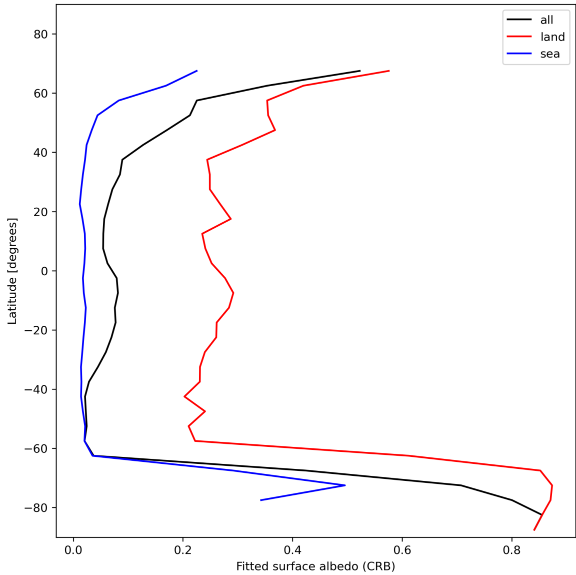
Figure 30: Zonal average of “Fitted surface albedo (CRB)” for 2024-01-05 to 2024-01-06.
