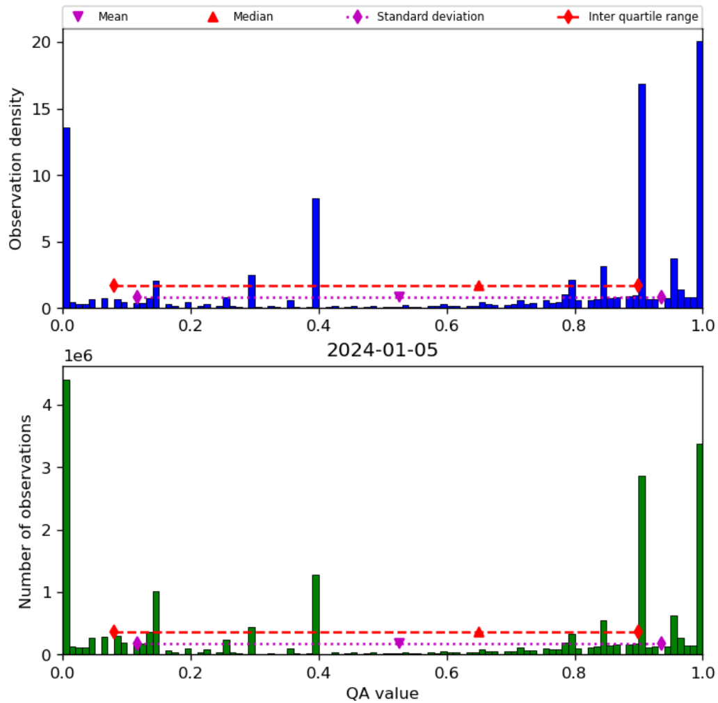
Figure 38: Histogram of “QA value” for 2024-01-05 to 2024-01-06
