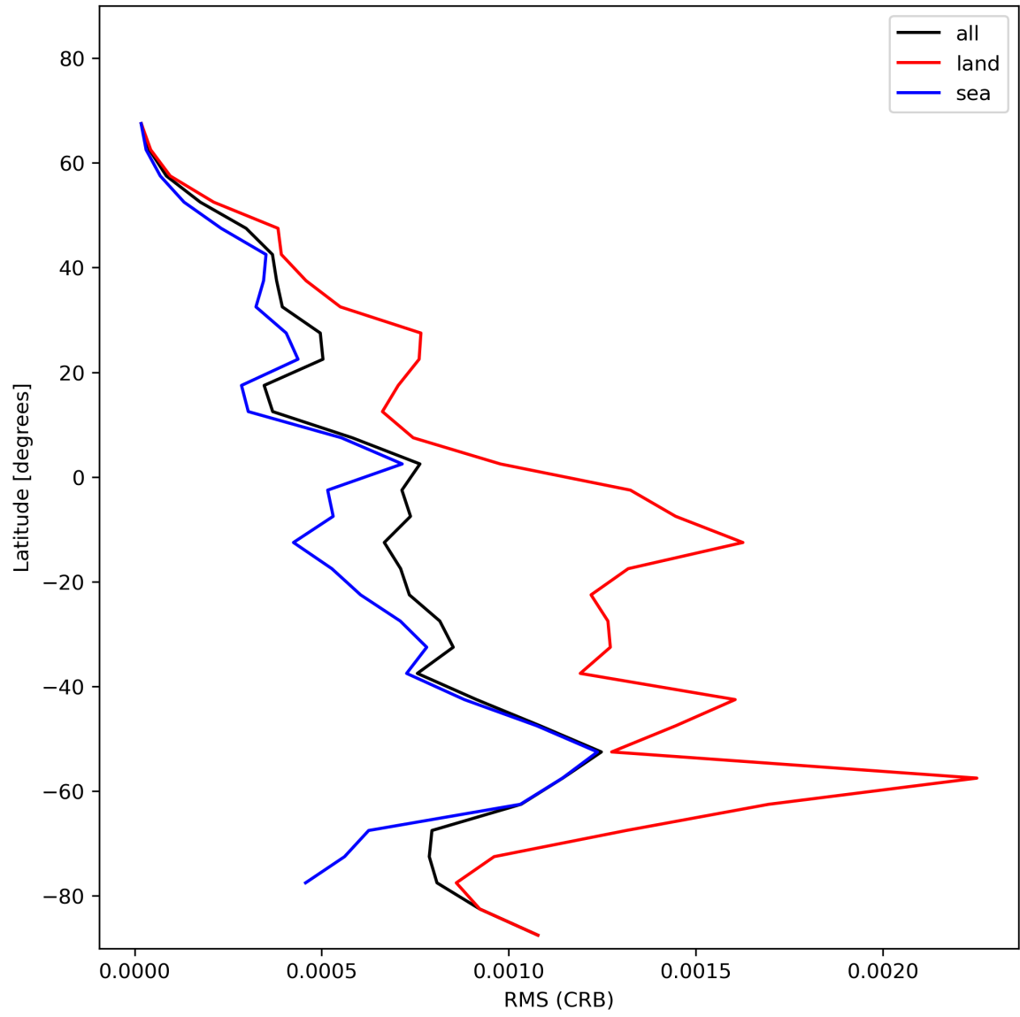
Figure 32: Zonal average of “RMS (CRB)” for 2024-01-05 to 2024-01-06.
