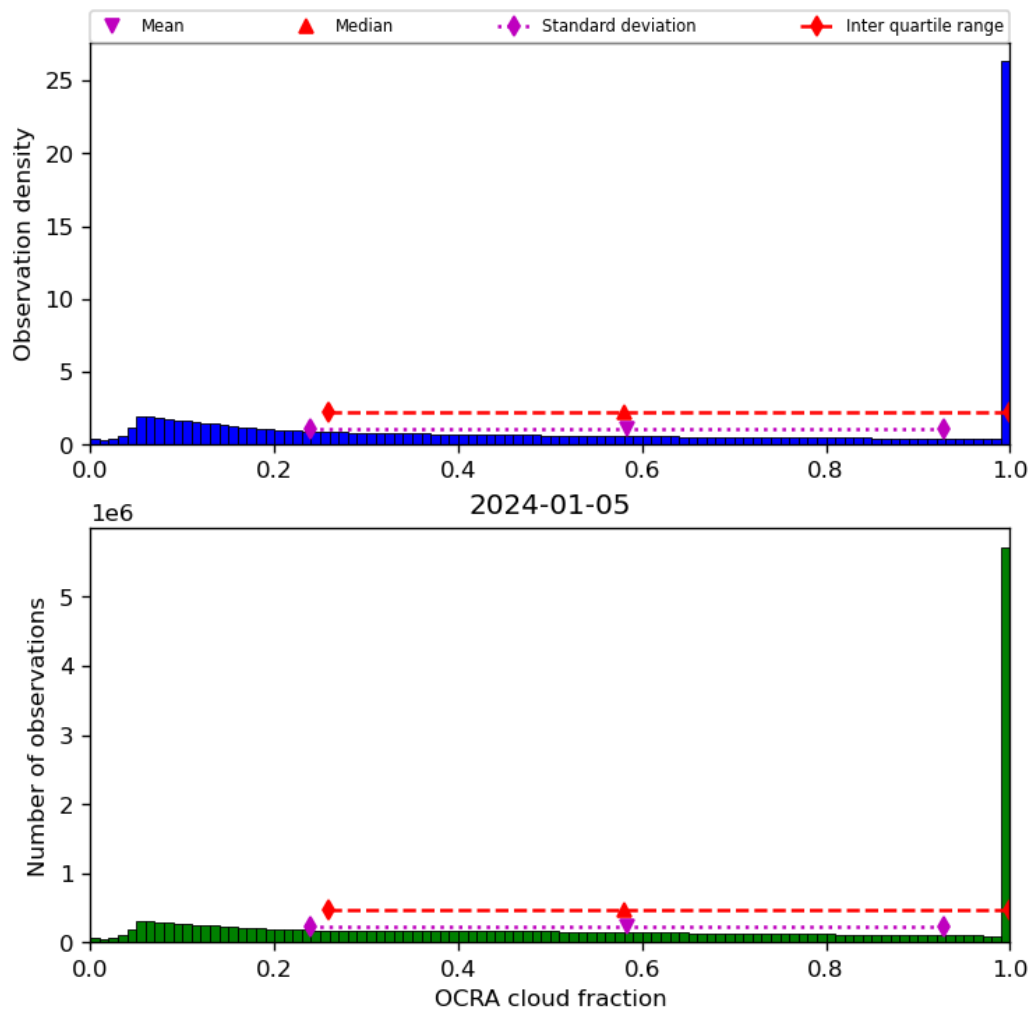
Figure 50: Histogram of “OCRA cloud fraction” for 2024-01-05 to 2024-01-06
