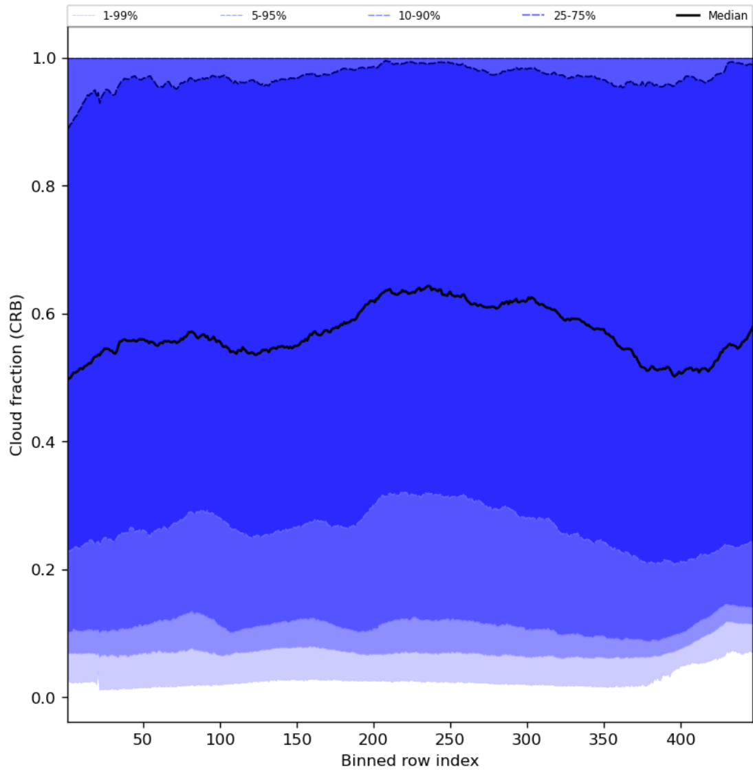
Figure 58: Along track statistics of “Cloud fraction (CRB)” for 2024-01-05 to 2024-01-06
