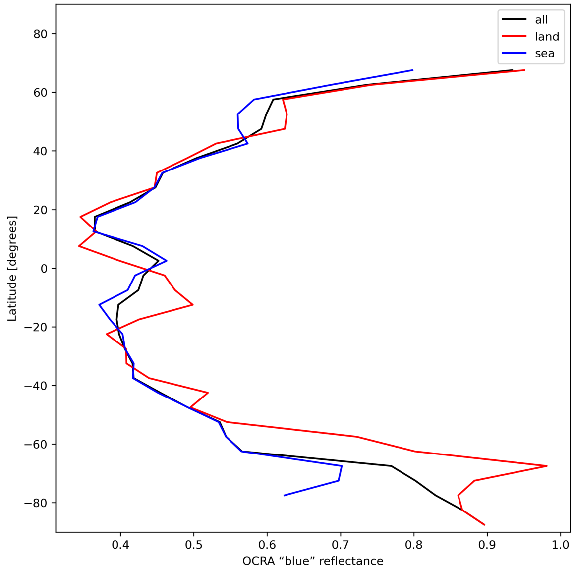
Figure 35: Zonal average of “OCRA “blue” reflectance” for 2024-01-05 to 2024-01-06.
