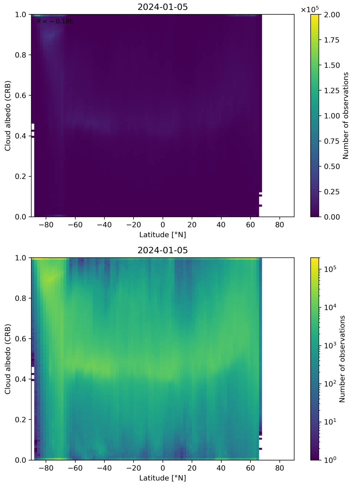
Figure 91: Scatter density plot of “Latitude” against “Cloud albedo (CRB)” for 2024-01-05 to 2024-01-06.
