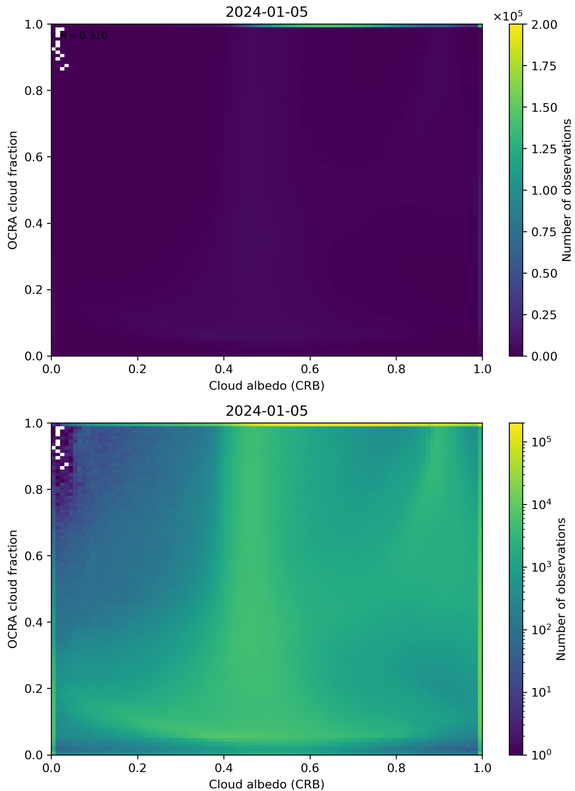
Figure 70: Scatter density plot of “Cloud albedo (CRB)” against “OCRA cloud fraction” for 2024-01-05 to 2024-01-06.
