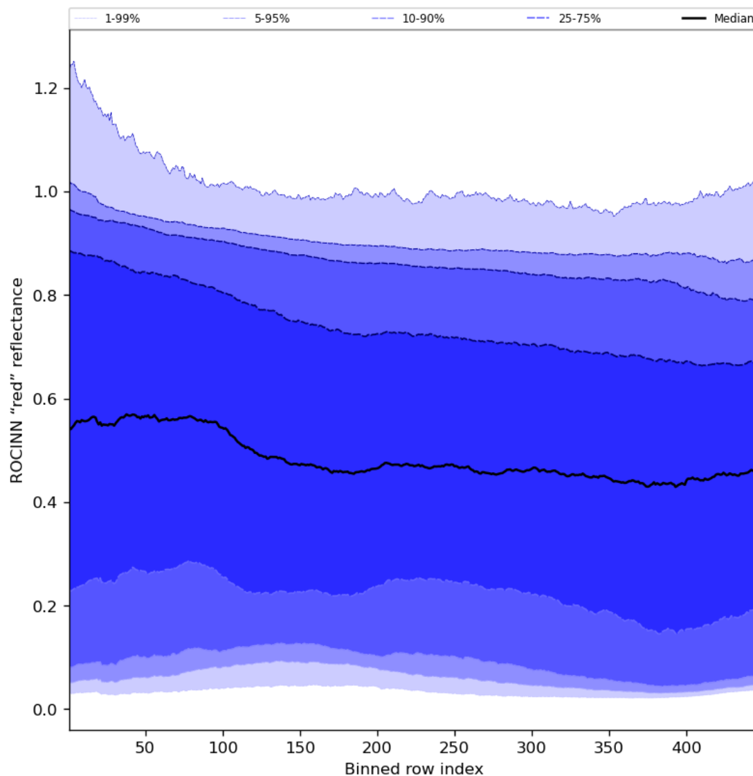
Figure 69: Along track statistics of “ROCINN “red” reflectance” for 2024-01-05 to 2024-01-06
