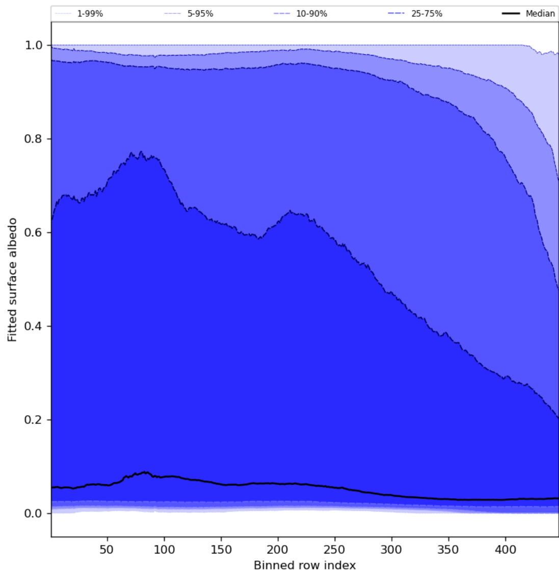
Figure 61: Along track statistics of “Fitted surface albedo” for 2024-01-05 to 2024-01-06
