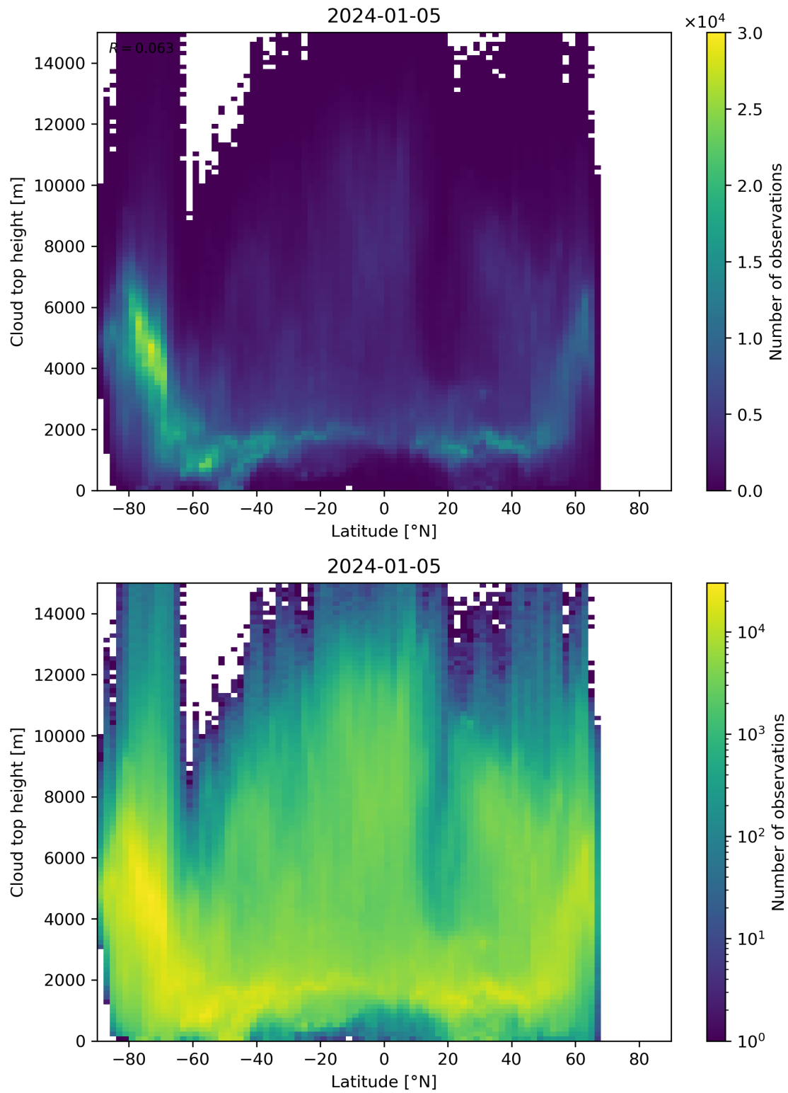
Figure 97: Scatter density plot of “Latitude” against “Cloud top height” for 2024-01-05 to 2024-01-06.
