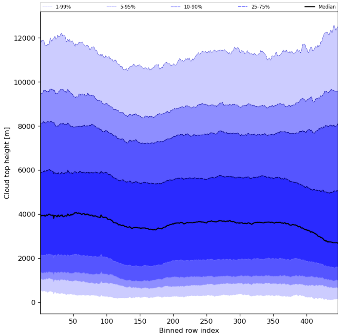
Figure 56: Along track statistics of “Cloud top height” for 2024-01-05 to 2024-01-06
