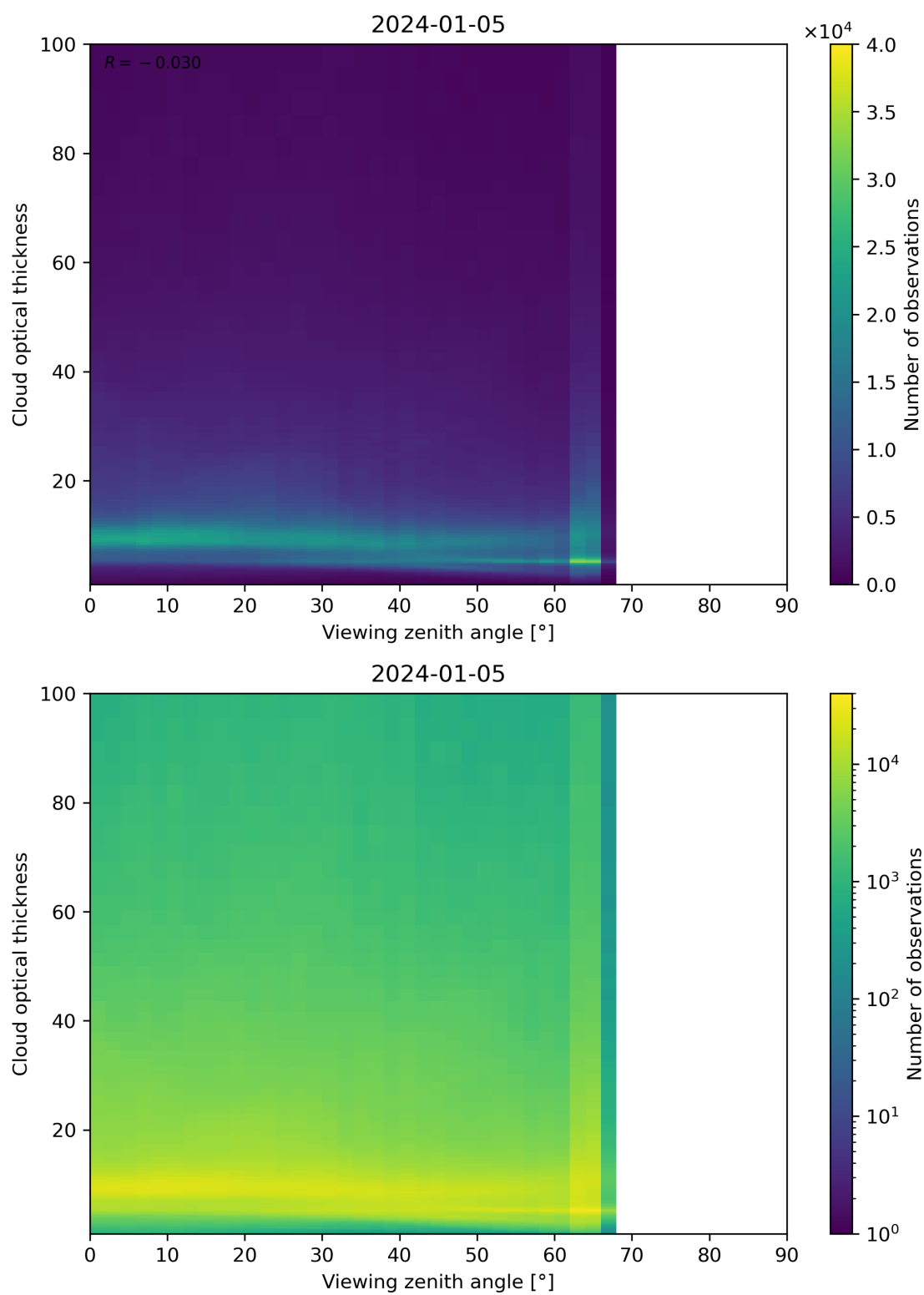
Figure 111: Scatter density plot of “Viewing zenith angle” against “Cloud optical thickness” for 2024-01-05 to 2024-01-06.
