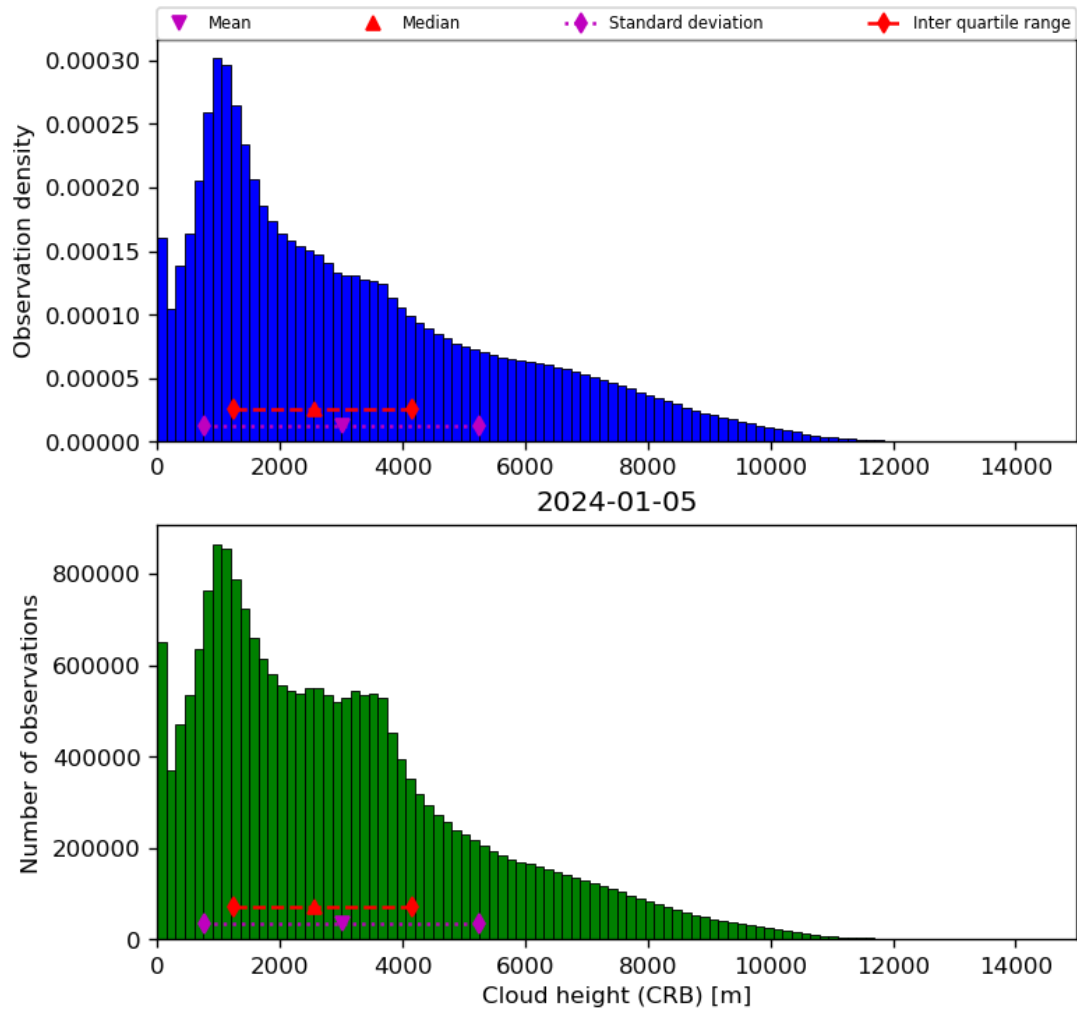
Figure 43: Histogram of “Cloud height (CRB)” for 2024-01-05 to 2024-01-06
