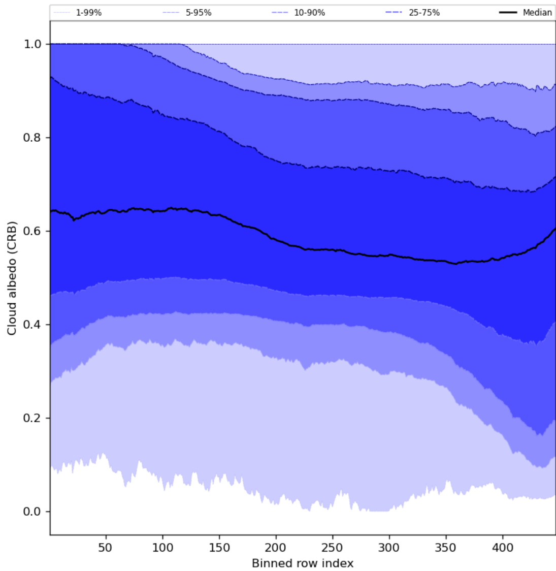
Figure 60: Along track statistics of “Cloud albedo (CRB)” for 2024-01-05 to 2024-01-06
