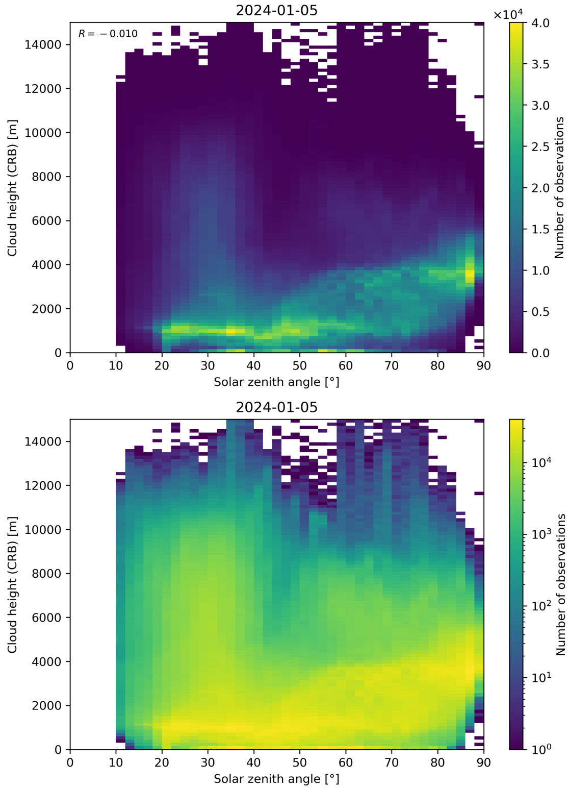
Figure 102: Scatter density plot of “Solar zenith angle” against “Cloud height (CRB)” for 2024-01-05 to 2024-01-06.
