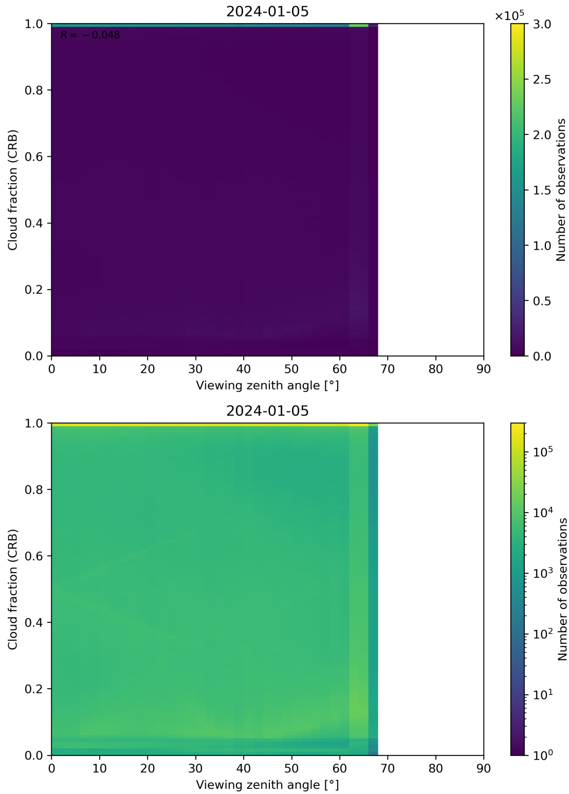
Figure 109: Scatter density plot of “Viewing zenith angle” against “Cloud fraction (CRB)” for 2024-01-05 to 2024-01-06.
