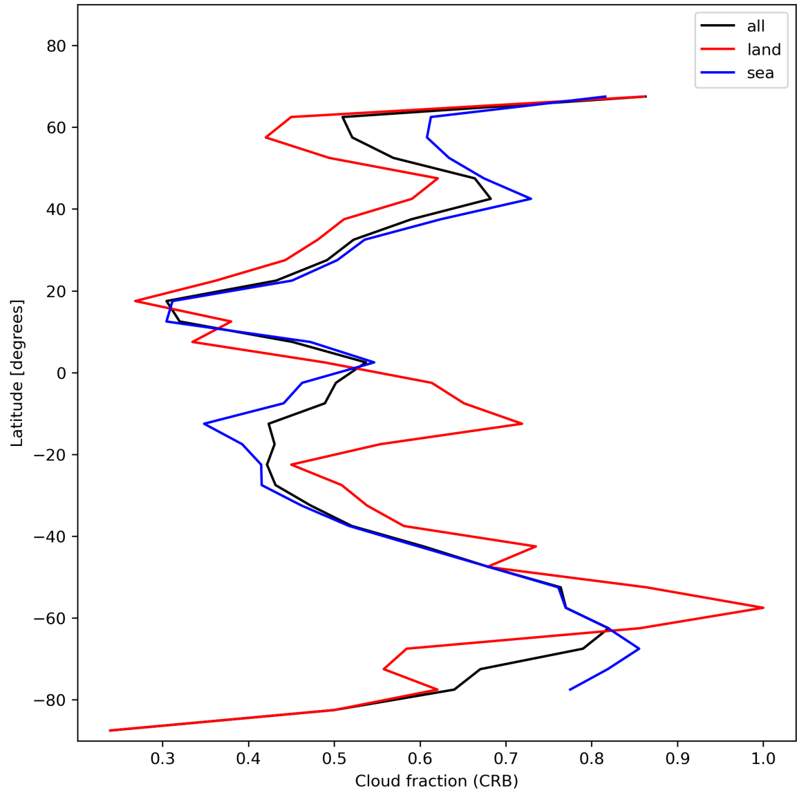
Figure 26: Zonal average of “Cloud fraction (CRB)” for 2024-01-05 to 2024-01-06.
