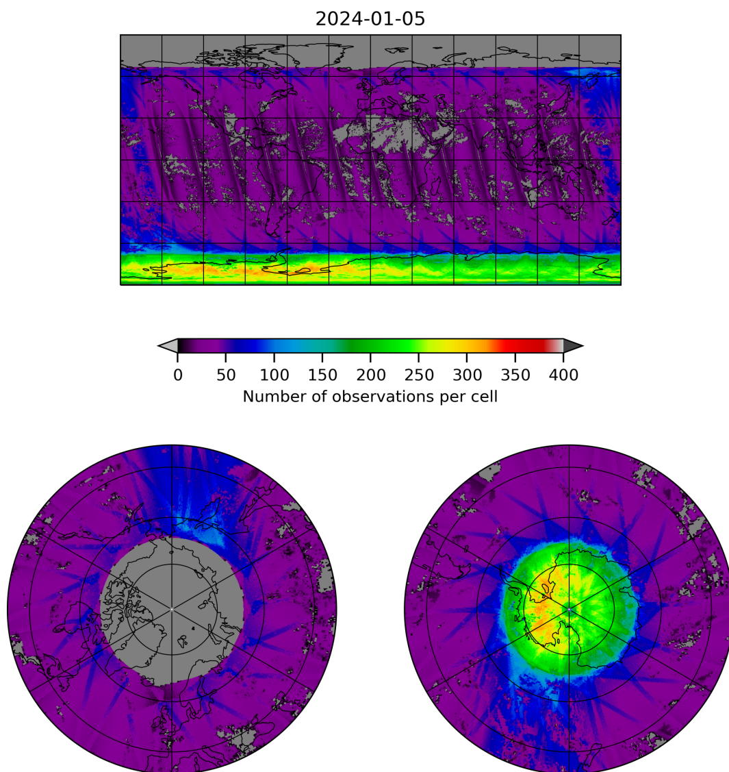
Figure 21: Map of the number of observations for 2024-01-05 to 2024-01-06
