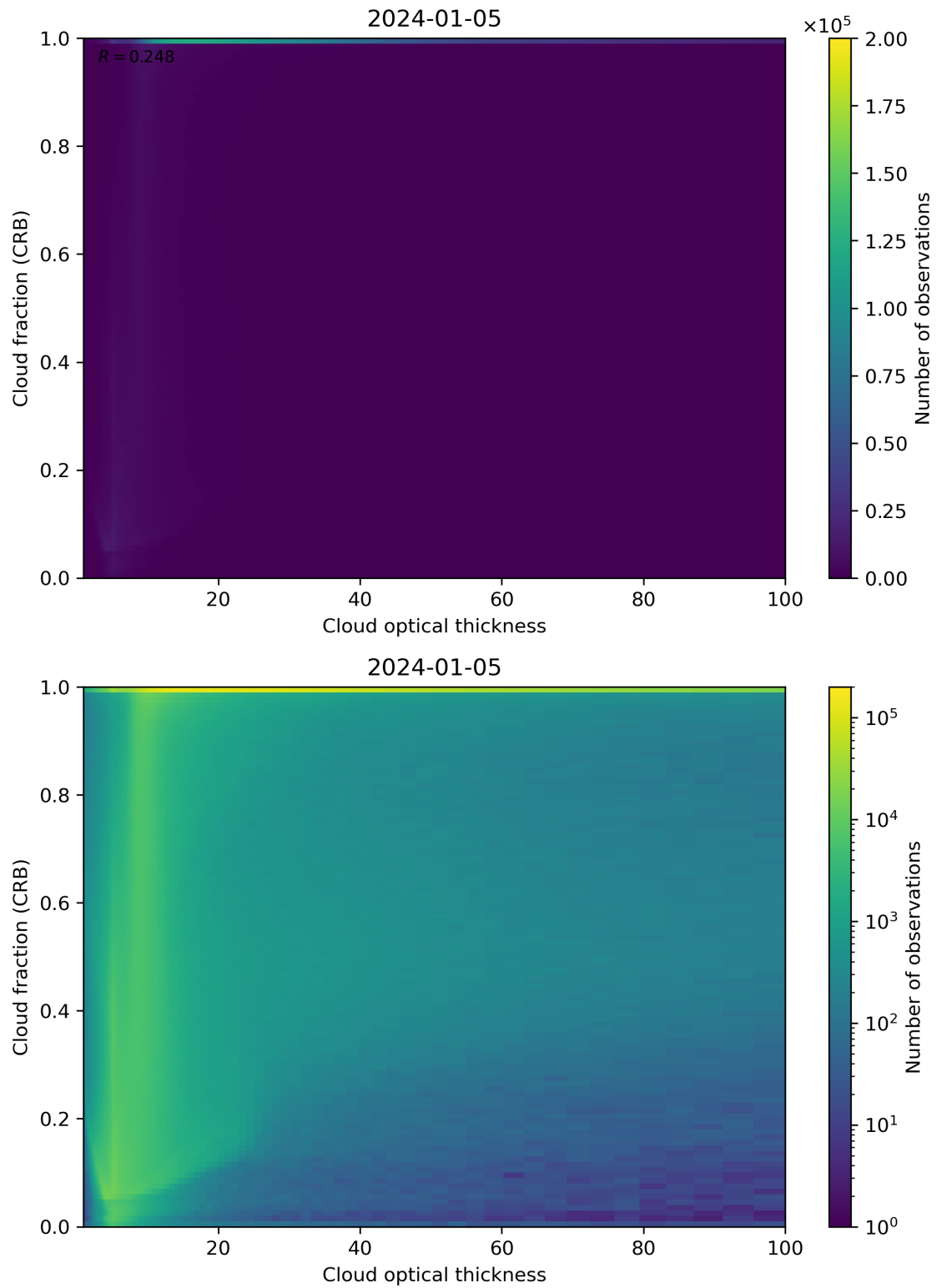
Figure 84: Scatter density plot of “Cloud optical thickness” against “Cloud fraction (CRB)” for 2024-01-05 to 2024-01-06.
