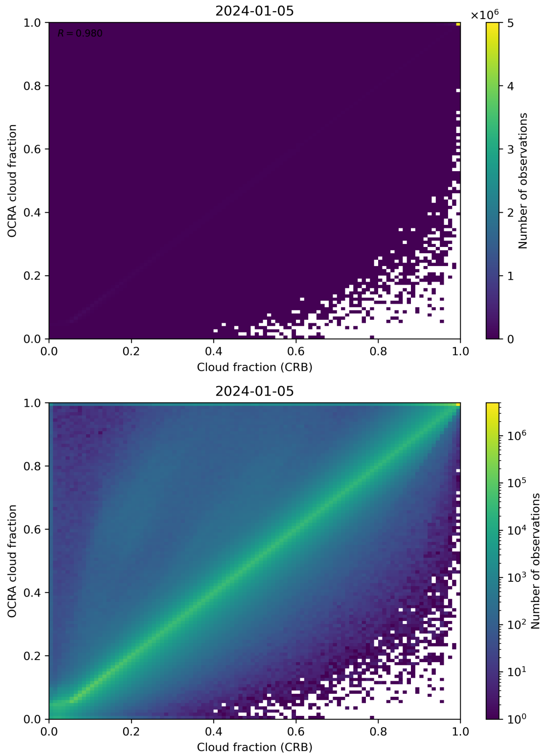
Figure 78: Scatter density plot of “Cloud fraction (CRB)” against “OCRA cloud fraction” for 2024-01-05 to 2024-01-06.
