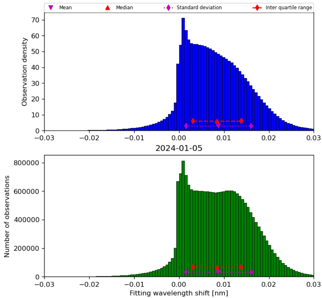
Figure 49: Histogram of “Fitting wavelength shift” for 2024-01-05 to 2024-01-06
