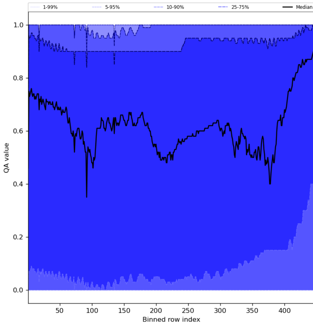
Figure 54: Along track statistics of “QA value” for 2024-01-05 to 2024-01-06
