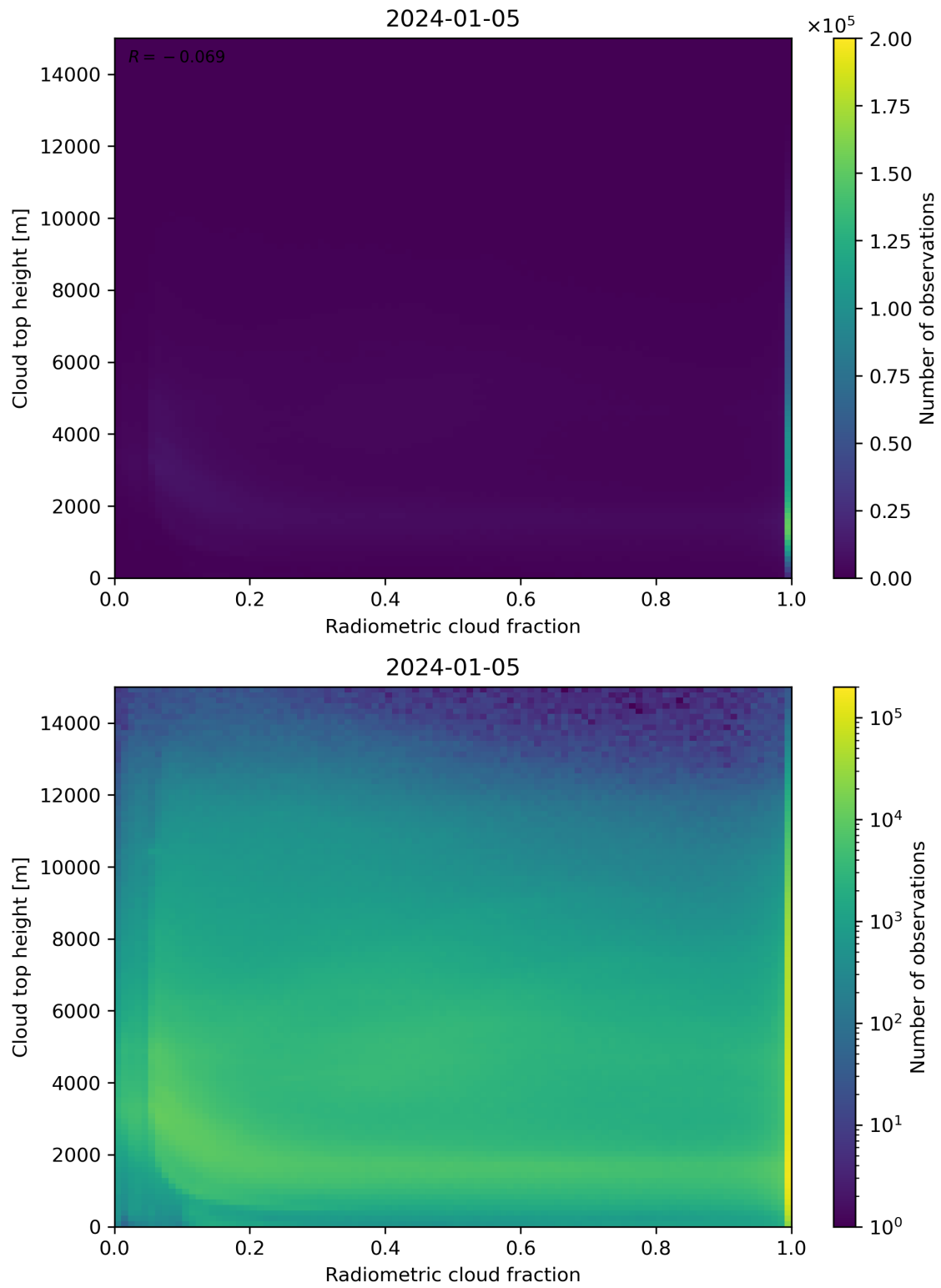
Figure 76: Scatter density plot of “Radiometric cloud fraction” against “Cloud top height” for 2024-01-05 to 2024-01-06.
