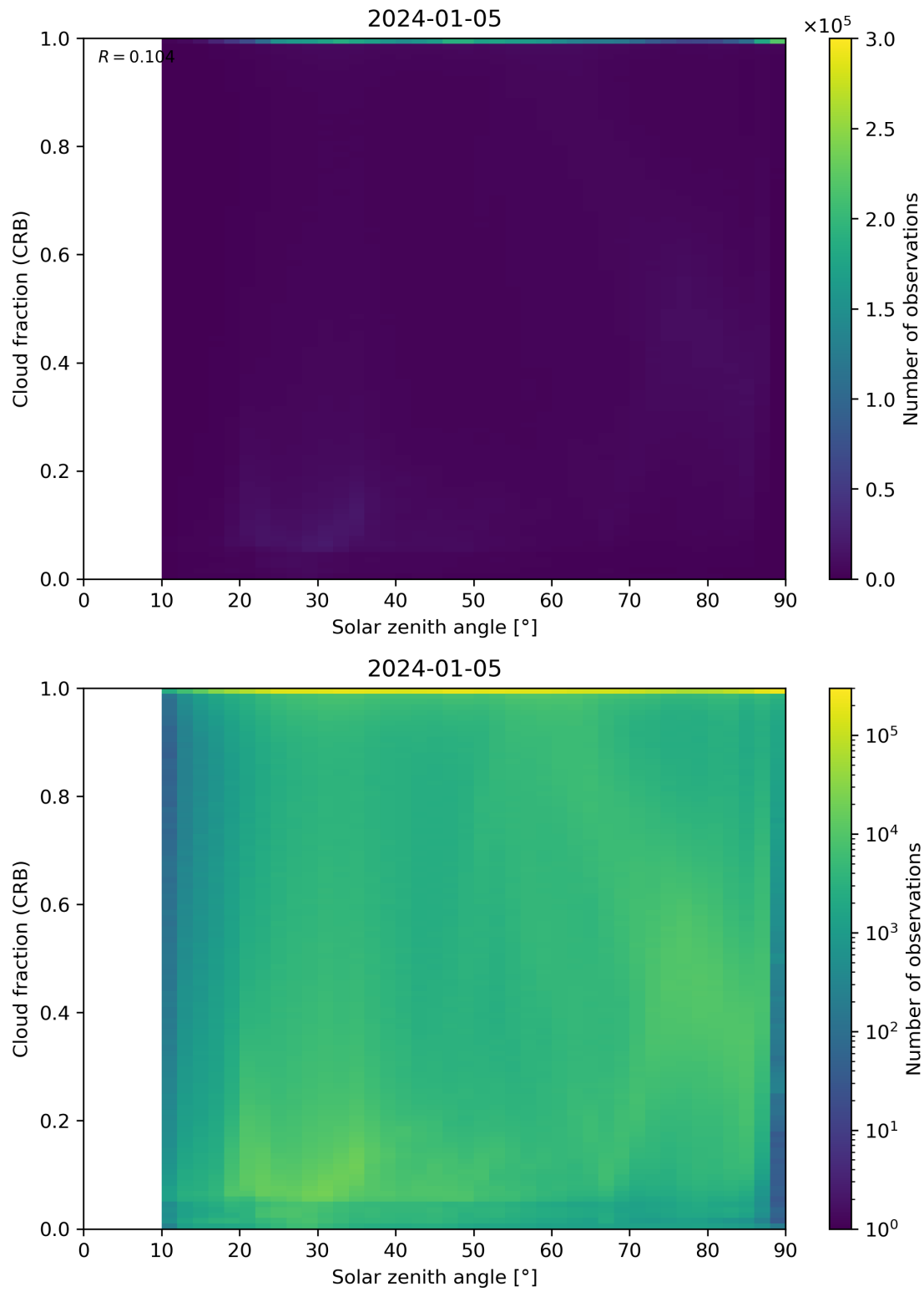
Figure 101: Scatter density plot of “Solar zenith angle” against “Cloud fraction (CRB)” for 2024-01-05 to 2024-01-06.
