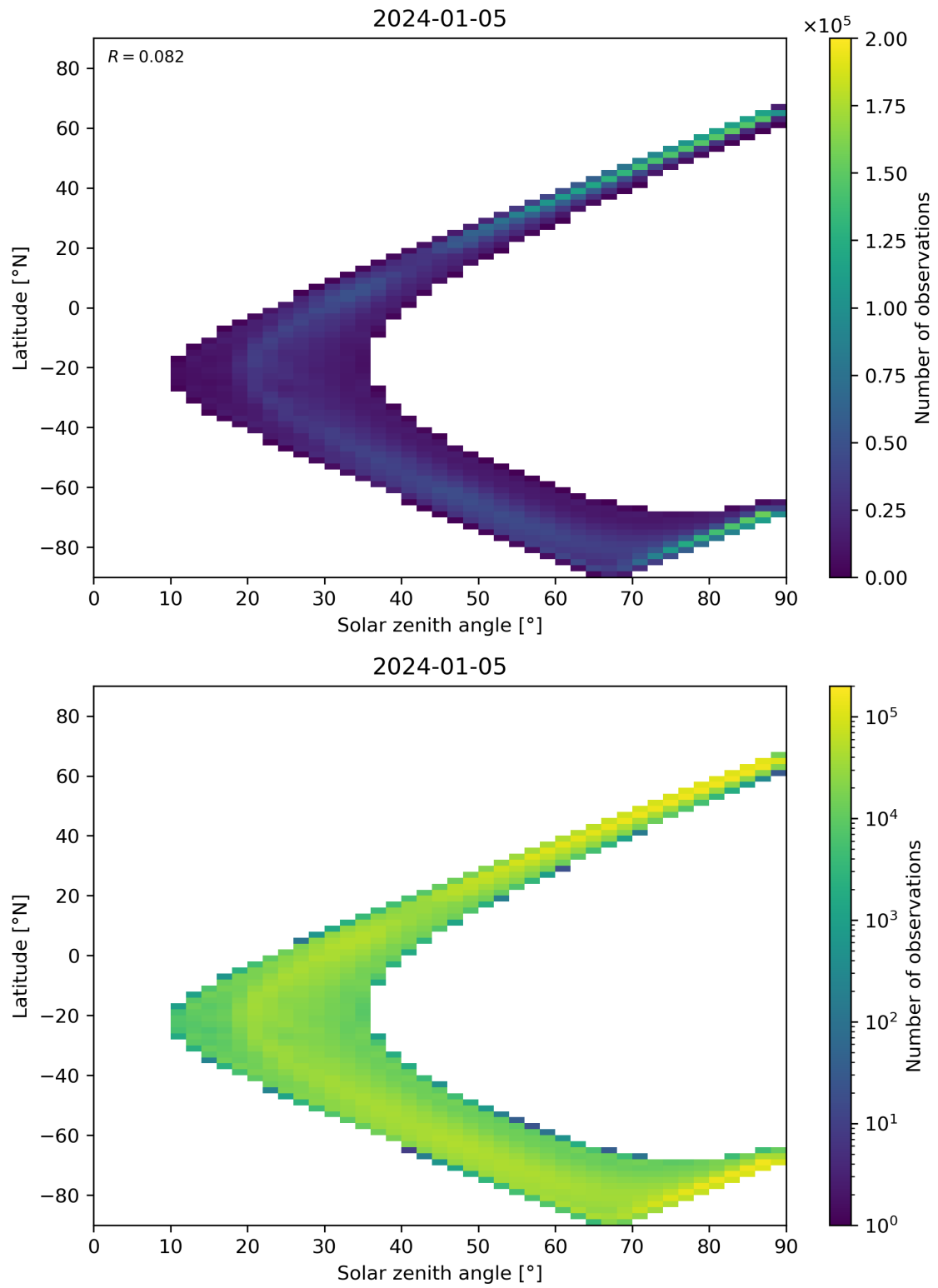
Figure 105: Scatter density plot of “Solar zenith angle” against “Latitude” for 2024-01-05 to 2024-01-06.
