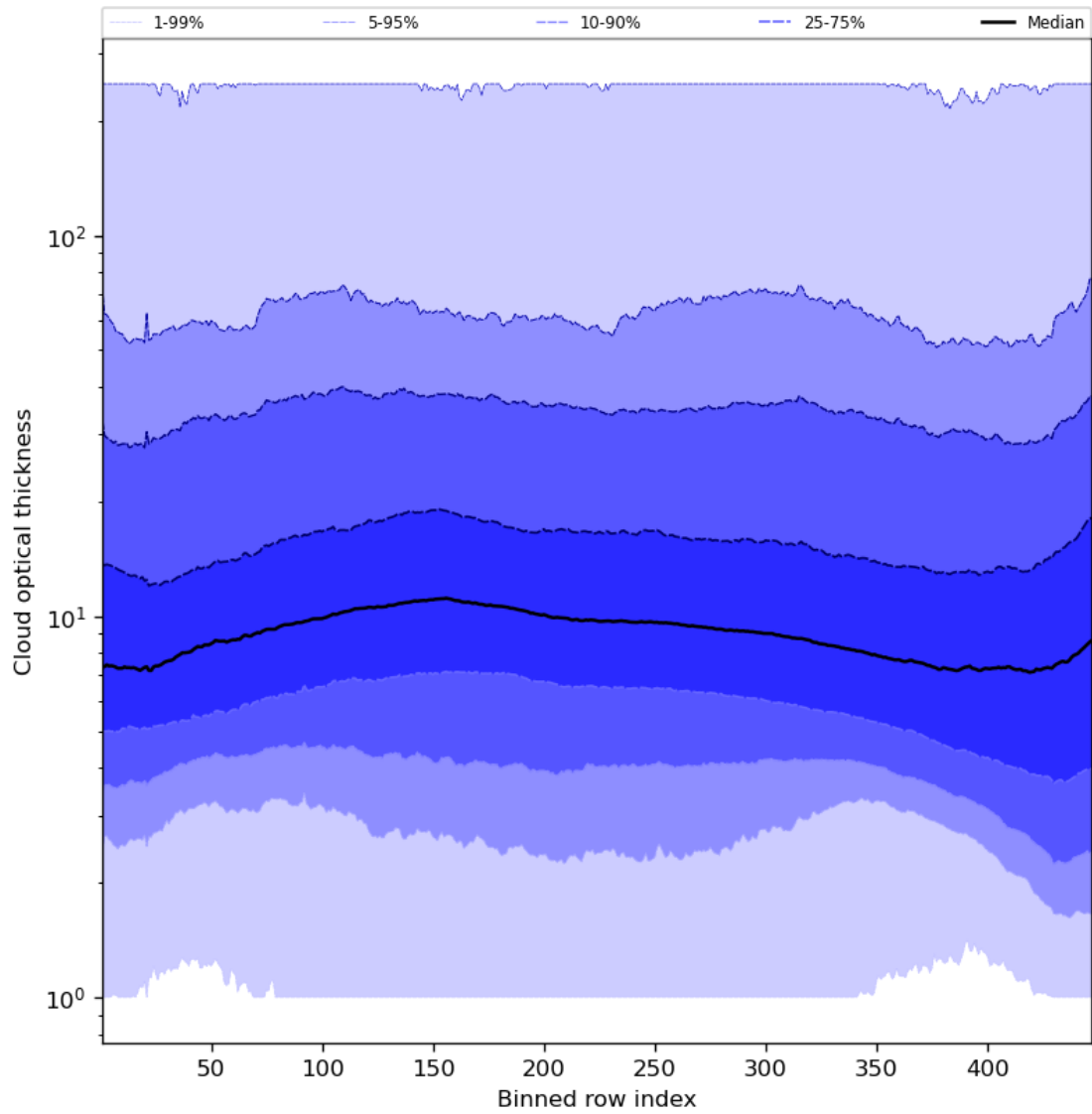
Figure 57: Along track statistics of “Cloud optical thickness” for 2024-01-05 to 2024-01-06
