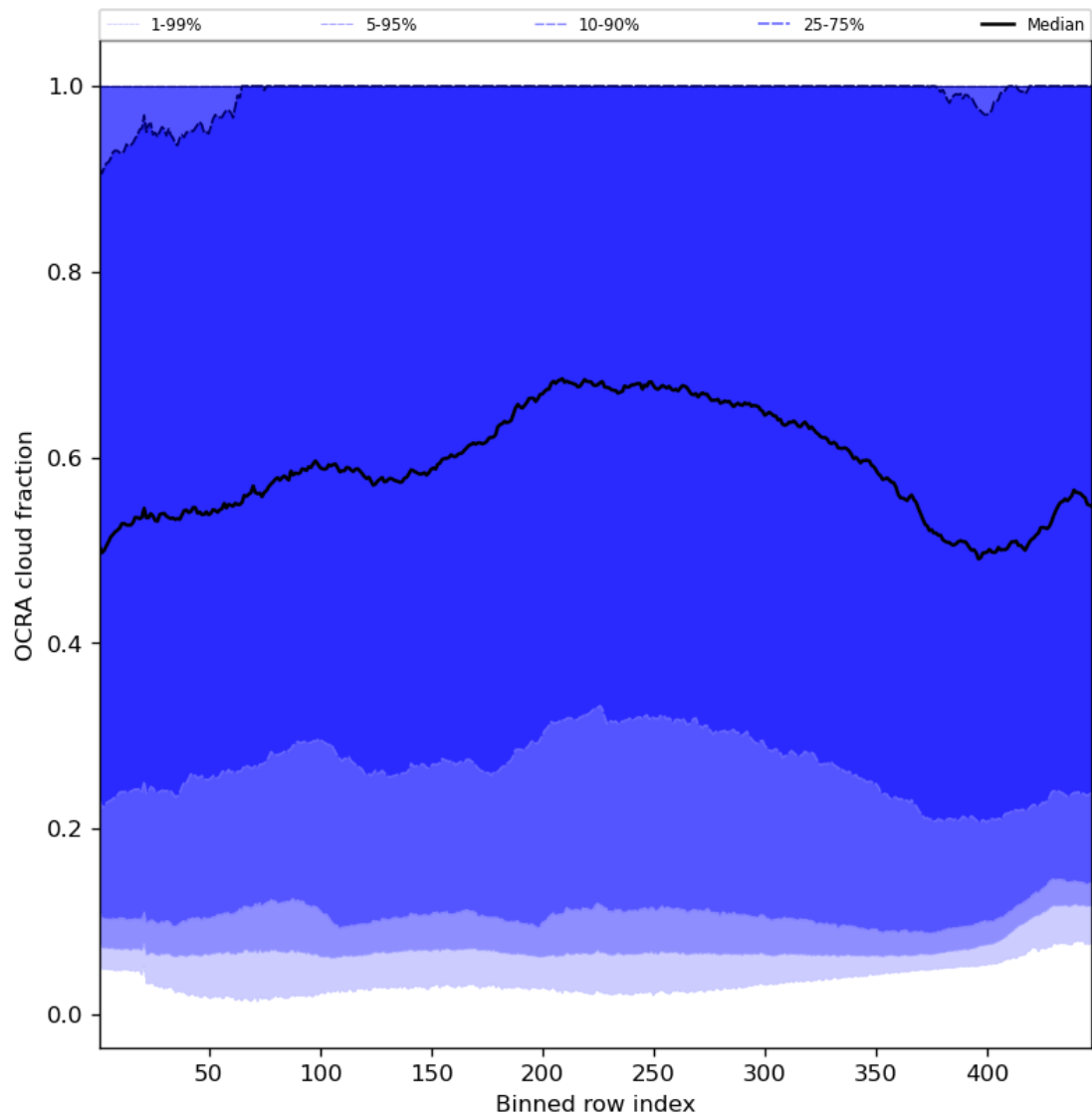
Figure 66: Along track statistics of “OCRA cloud fraction” for 2024-01-05 to 2024-01-07
