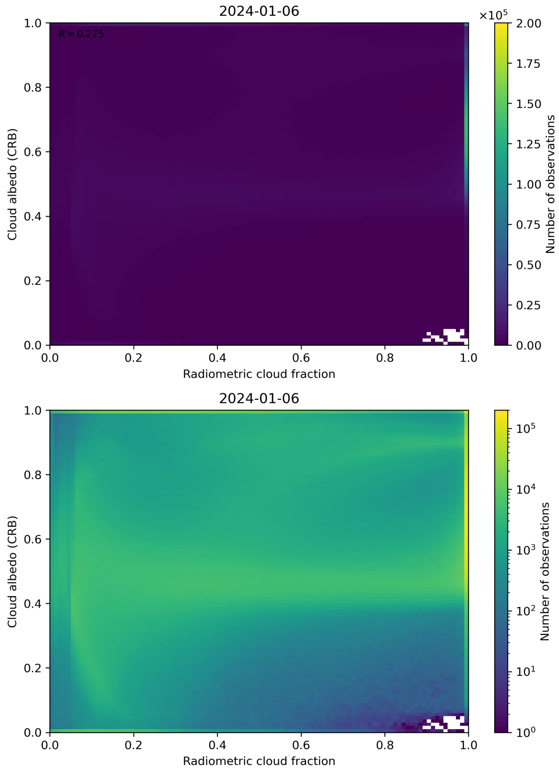
Figure 71: Scatter density plot of “Radiometric cloud fraction” against “Cloud albedo (CRB)” for 2024-01-05 to 2024-01-07.
