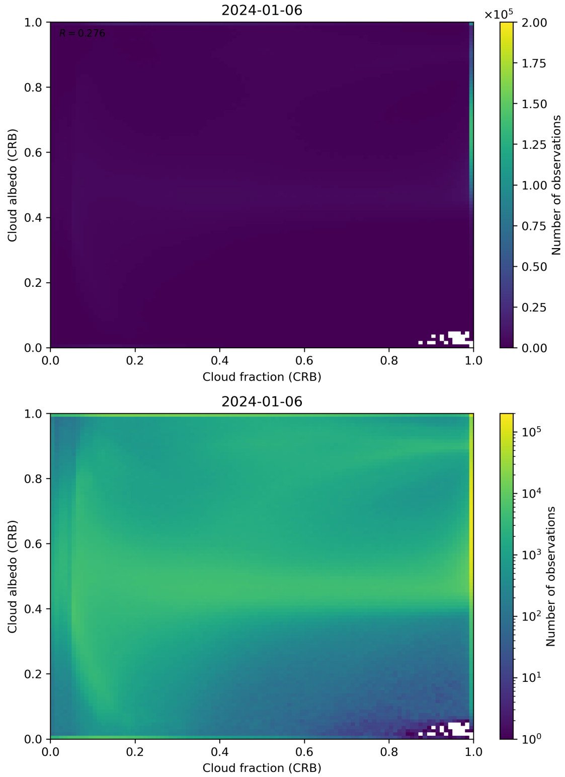
Figure 77: Scatter density plot of “Cloud fraction (CRB)” against “Cloud albedo (CRB)” for 2024-01-05 to 2024-01-07.
