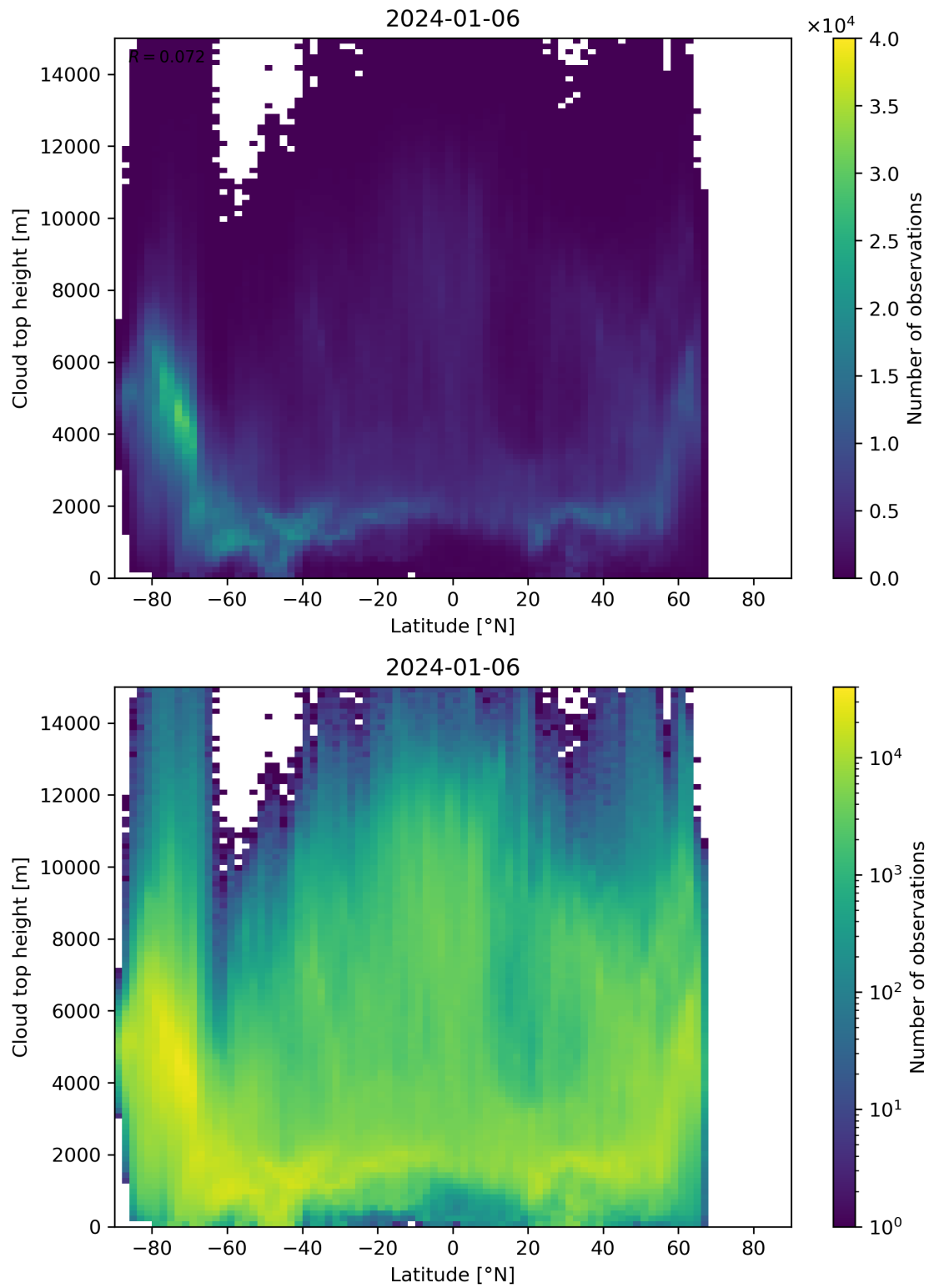
Figure 97: Scatter density plot of “Latitude” against “Cloud top height” for 2024-01-05 to 2024-01-07.
