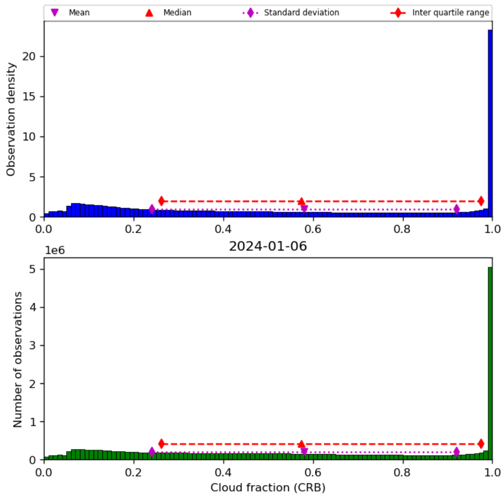
Figure 42: Histogram of “Cloud fraction (CRB)” for 2024-01-05 to 2024-01-07
