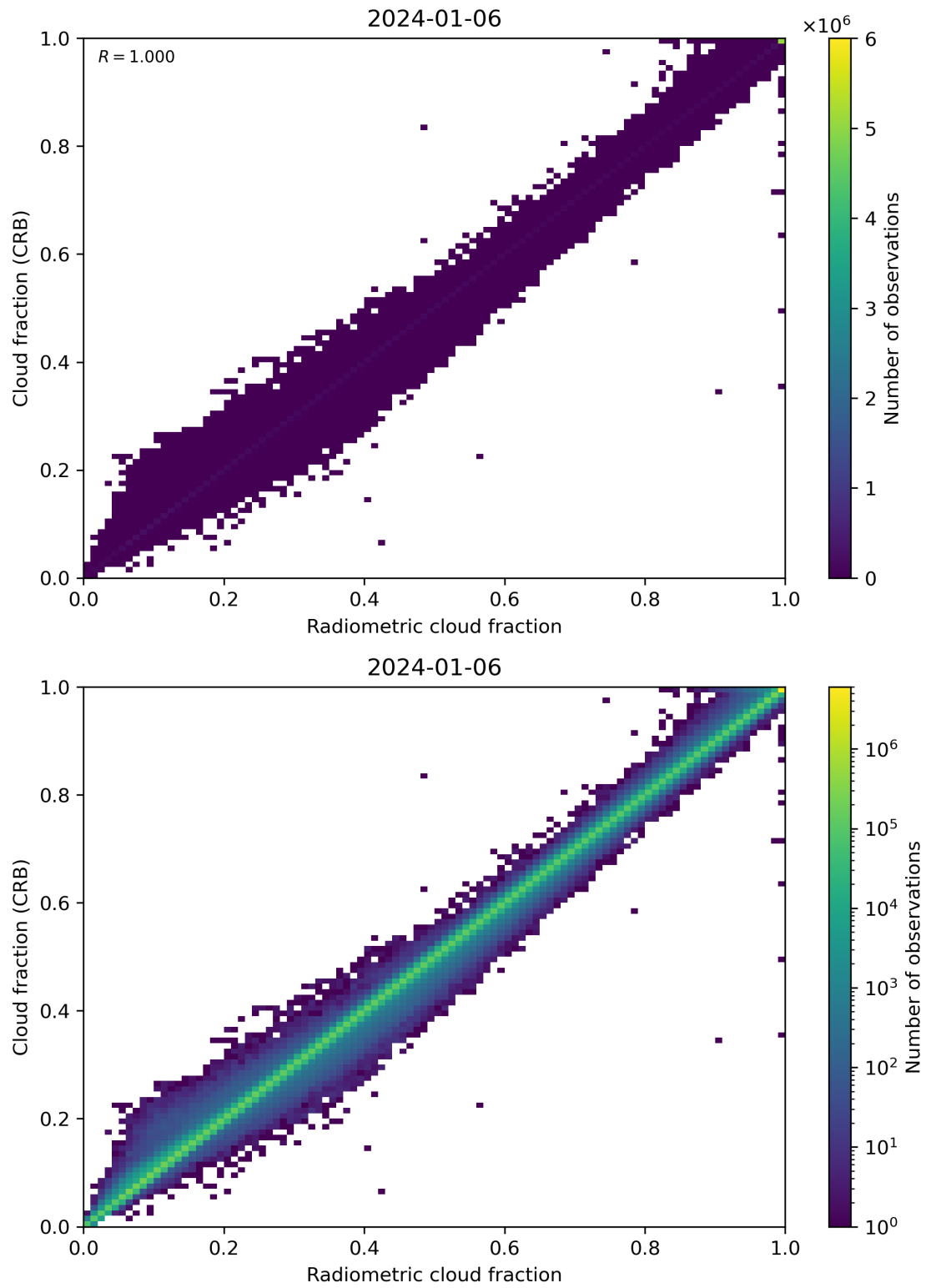
Figure 73: Scatter density plot of “Radiometric cloud fraction” against “Cloud fraction (CRB)” for 2024-01-05 to 2024-01-07.
