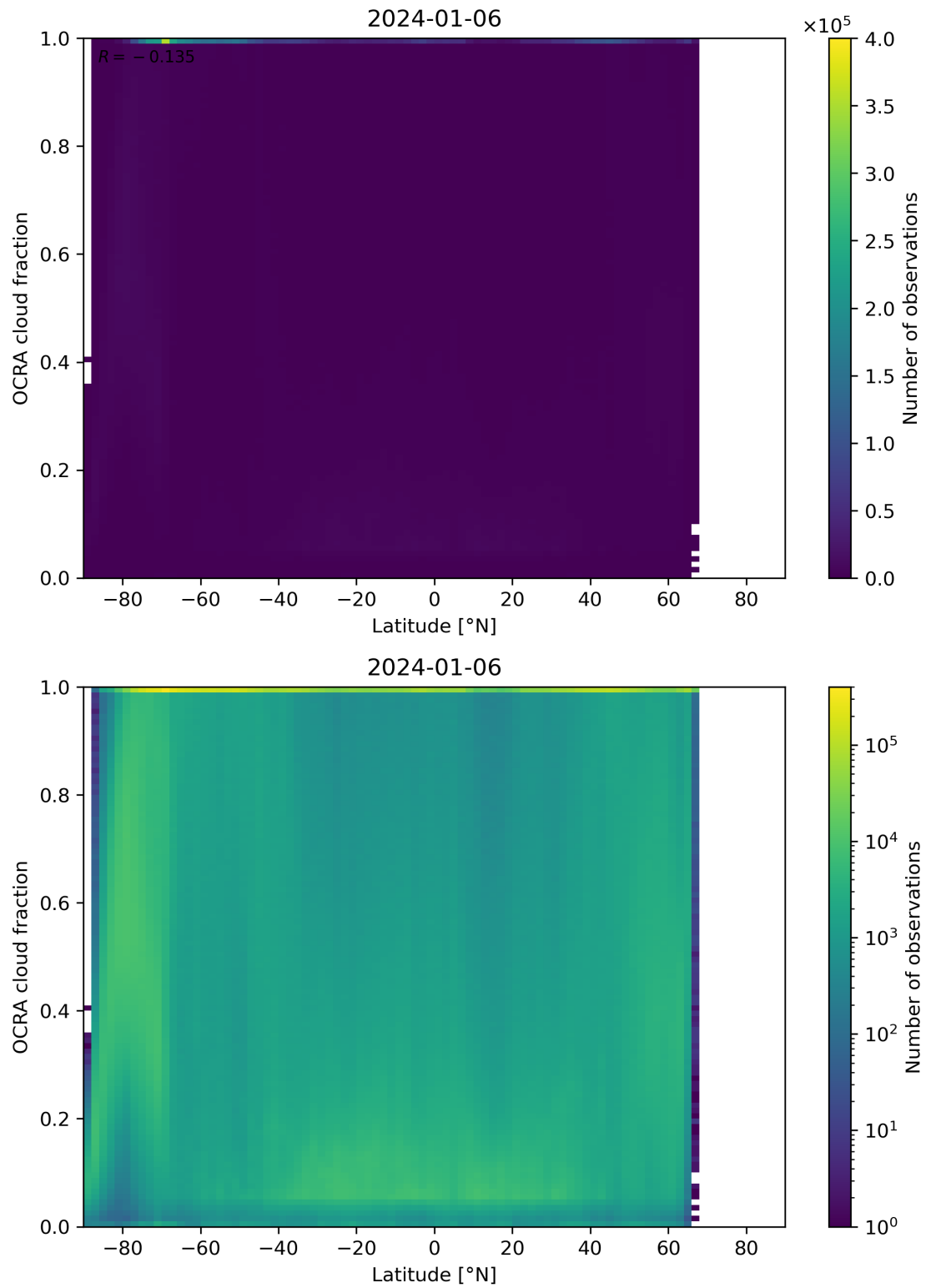
Figure 93: Scatter density plot of “Latitude” against “OCRA cloud fraction” for 2024-01-05 to 2024-01-07.
