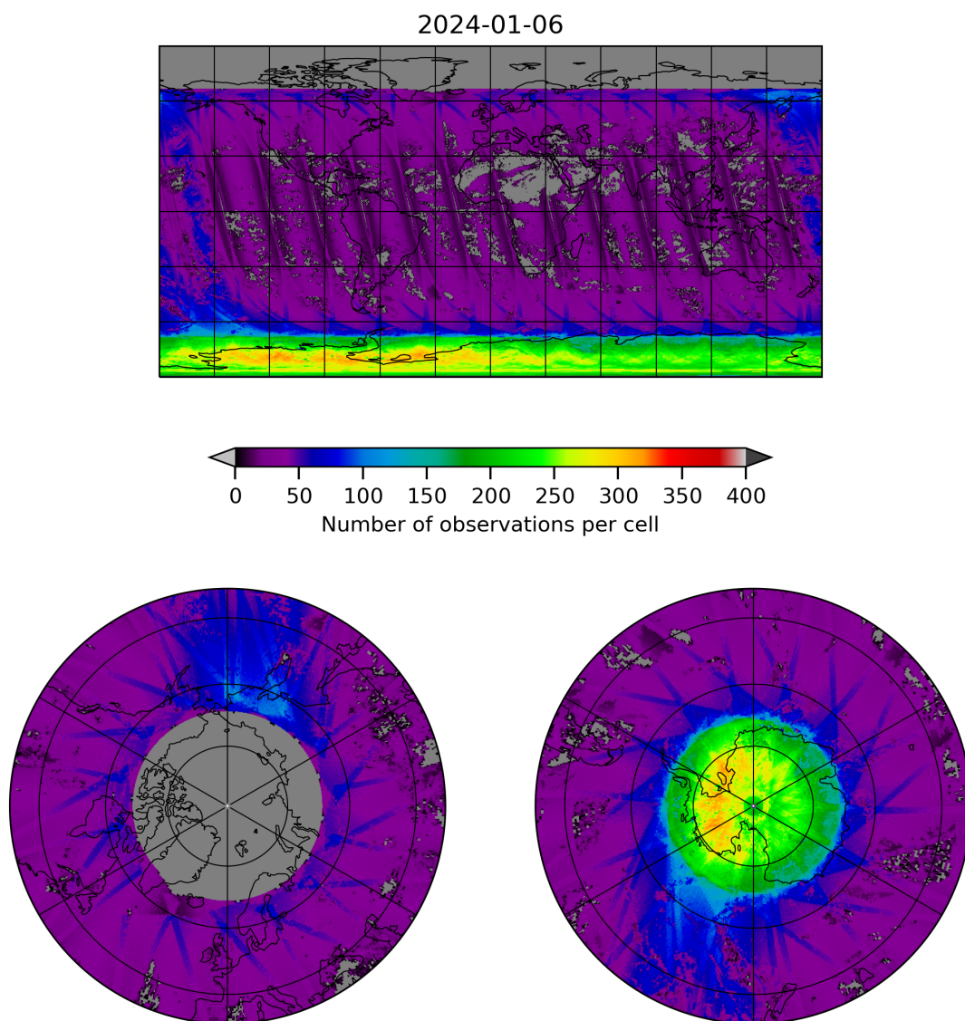
Figure 21: Map of the number of observations for 2024-01-05 to 2024-01-07
