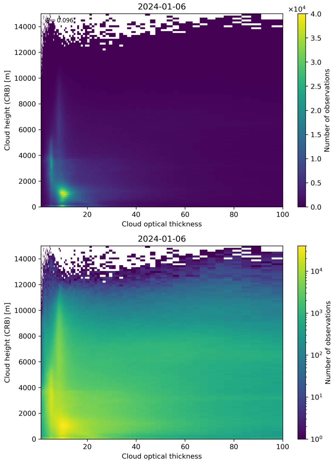
Figure 85: Scatter density plot of “Cloud optical thickness” against “Cloud height (CRB)” for 2024-01-05 to 2024-01-07.
