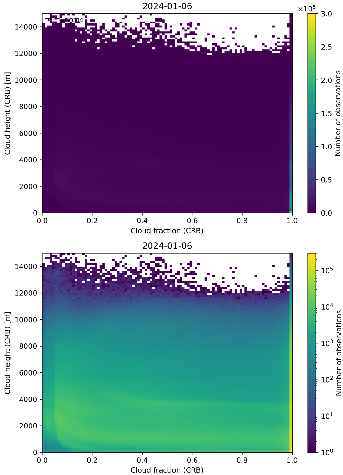
Figure 79: Scatter density plot of “Cloud fraction (CRB)” against “Cloud height (CRB)” for 2024-01-05 to 2024-01-07.
