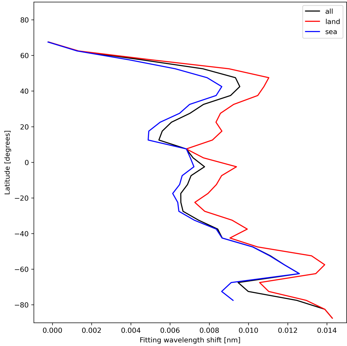
Figure 33: Zonal average of “Fitting wavelength shift” for 2024-01-05 to 2024-01-07.
