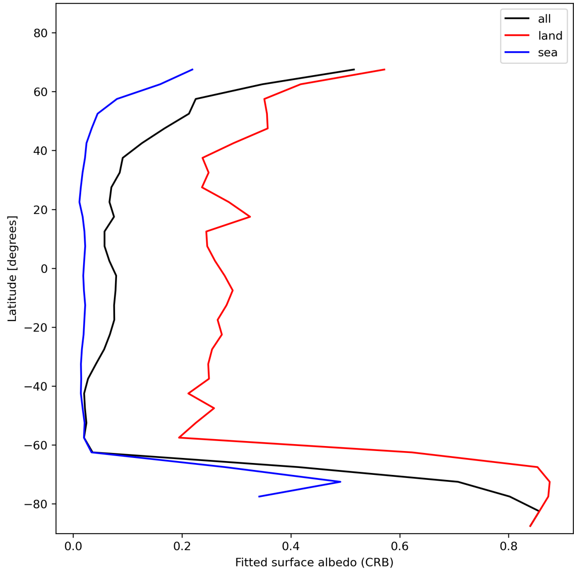
Figure 30: Zonal average of “Fitted surface albedo (CRB)” for 2024-01-05 to 2024-01-07.
