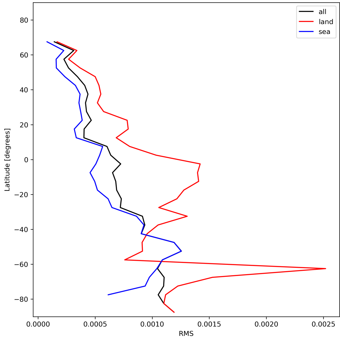
Figure 31: Zonal average of “RMS” for 2024-01-05 to 2024-01-07.
