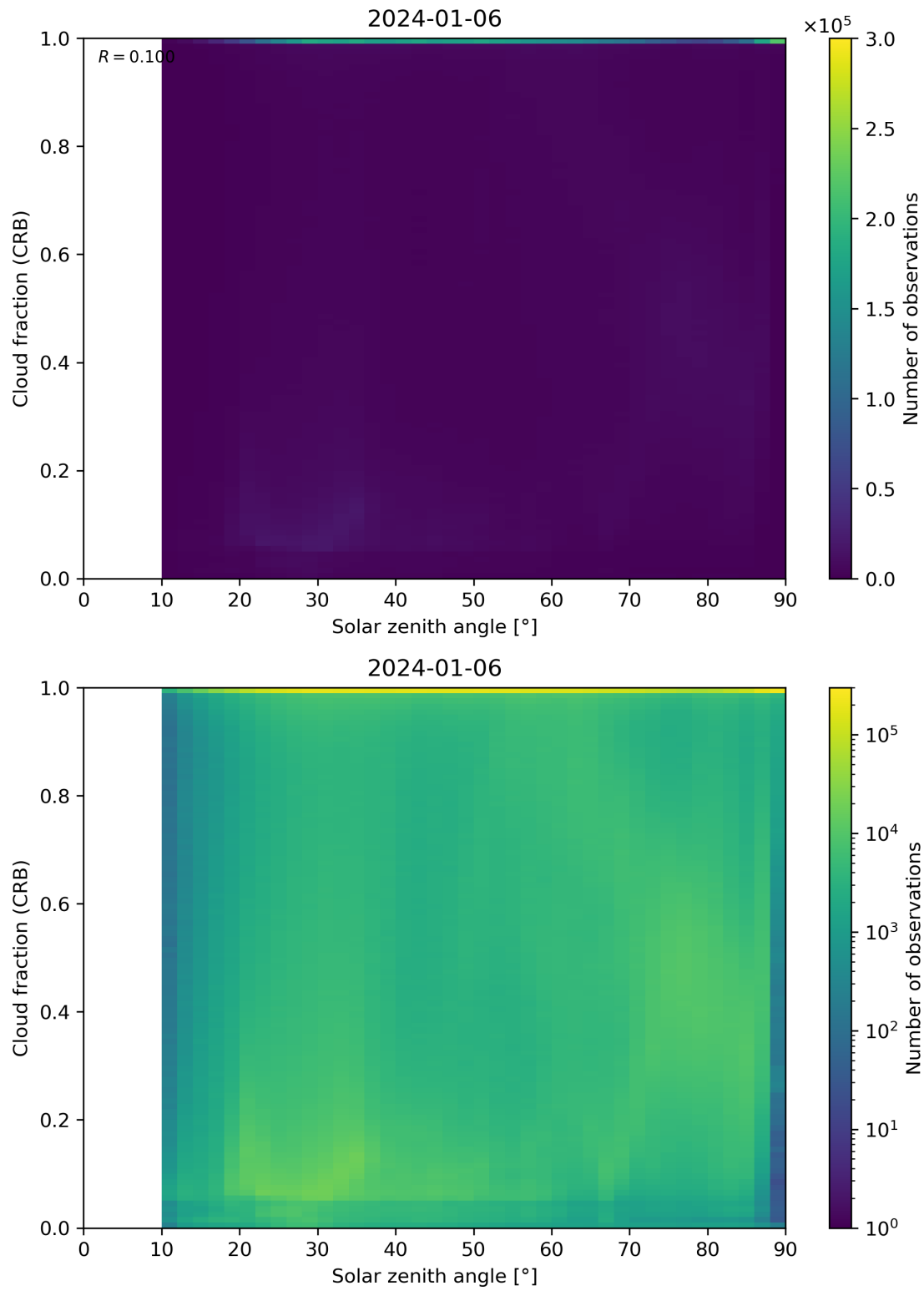
Figure 101: Scatter density plot of “Solar zenith angle” against “Cloud fraction (CRB)” for 2024-01-05 to 2024-01-07.
