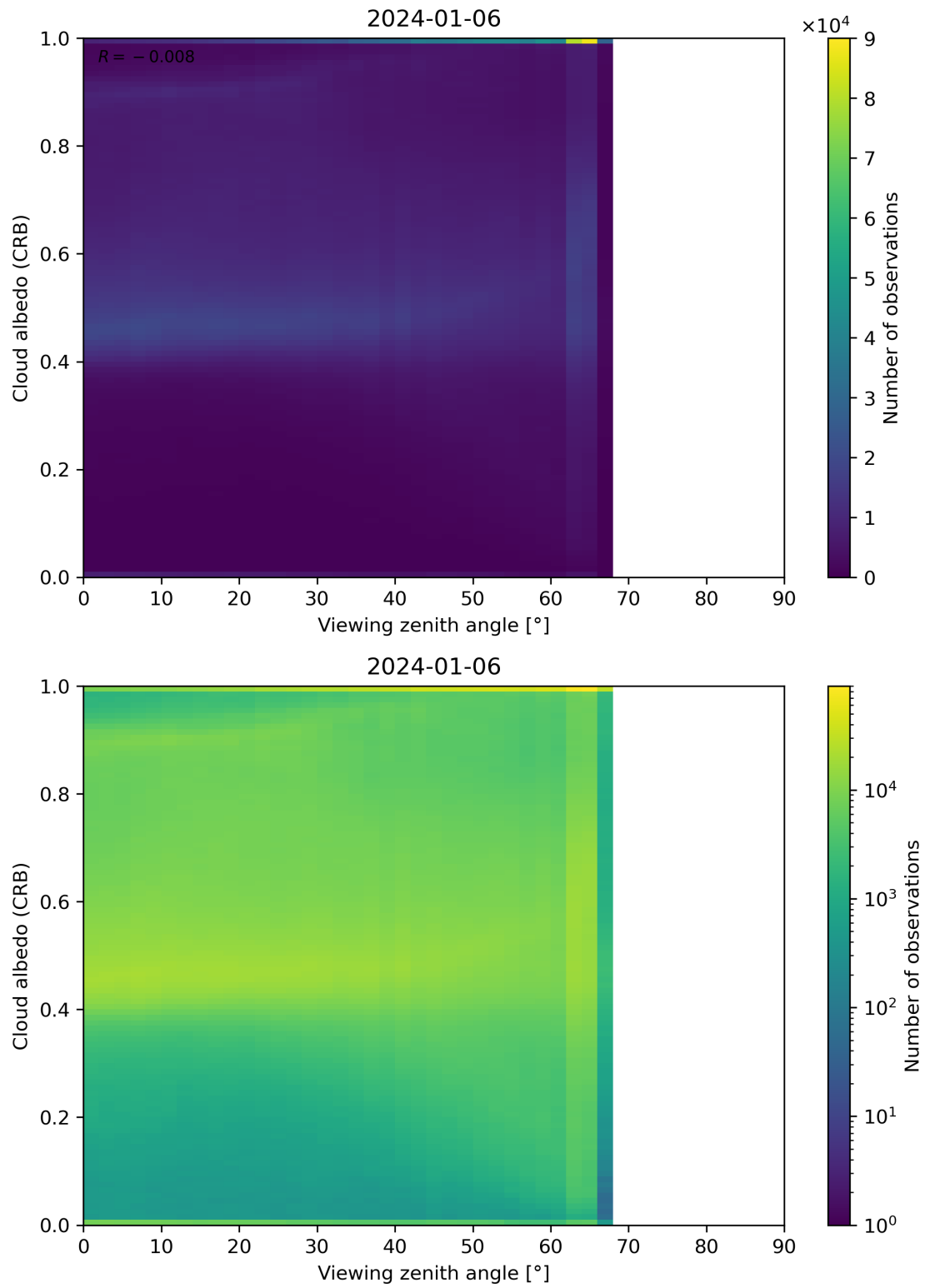
Figure 106: Scatter density plot of “Viewing zenith angle” against “Cloud albedo (CRB)” for 2024-01-05 to 2024-01-07.
