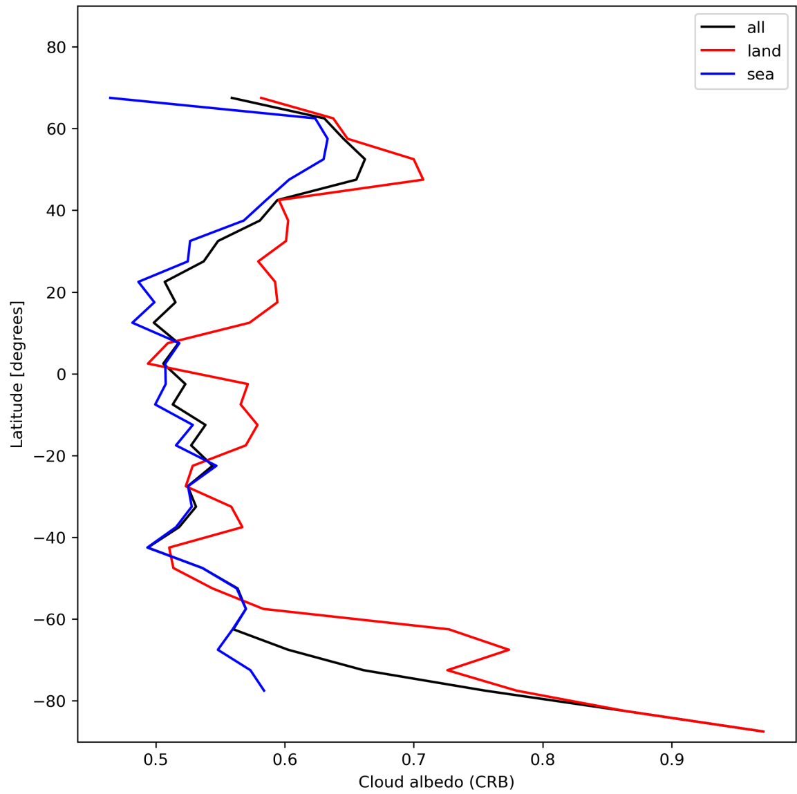
Figure 28: Zonal average of “Cloud albedo (CRB)” for 2024-01-05 to 2024-01-07.
