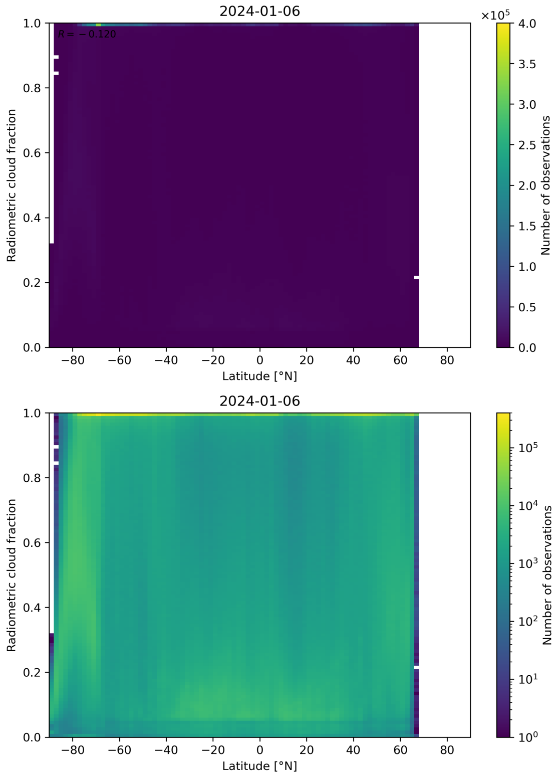
Figure 92: Scatter density plot of “Latitude” against “Radiometric cloud fraction” for 2024-01-05 to 2024-01-07.
