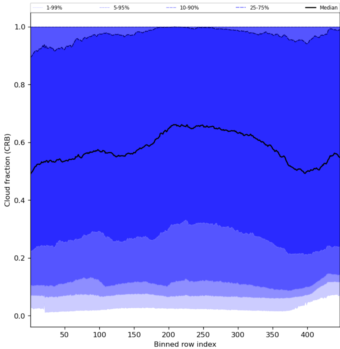
Figure 58: Along track statistics of “Cloud fraction (CRB)” for 2024-01-05 to 2024-01-07
