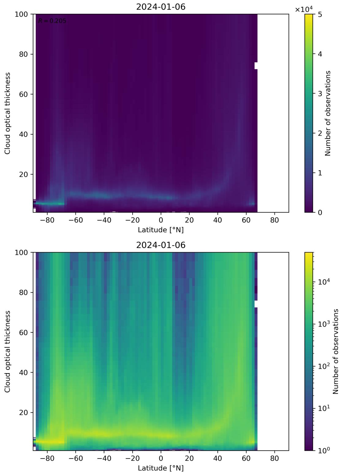
Figure 96: Scatter density plot of “Latitude” against “Cloud optical thickness” for 2024-01-05 to 2024-01-07.
