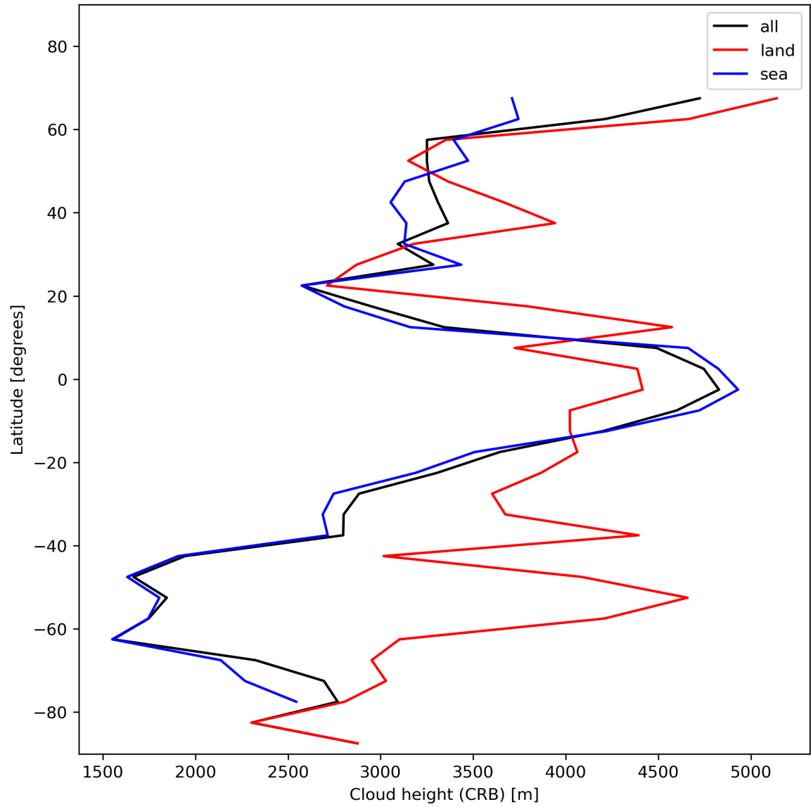
Figure 27: Zonal average of “Cloud height (CRB)” for 2024-01-05 to 2024-01-07.
