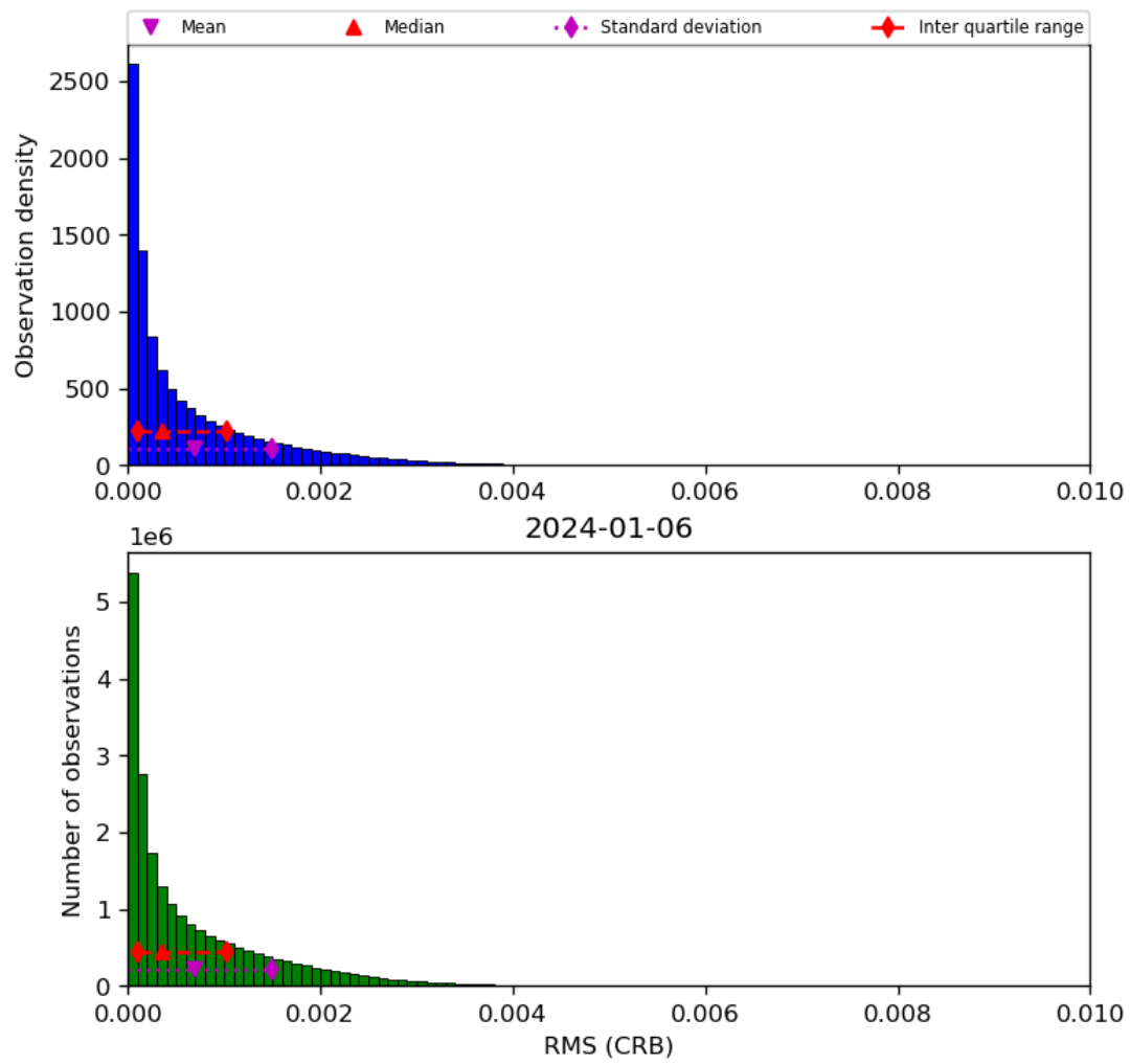
Figure 48: Histogram of “RMS (CRB)” for 2024-01-05 to 2024-01-07
