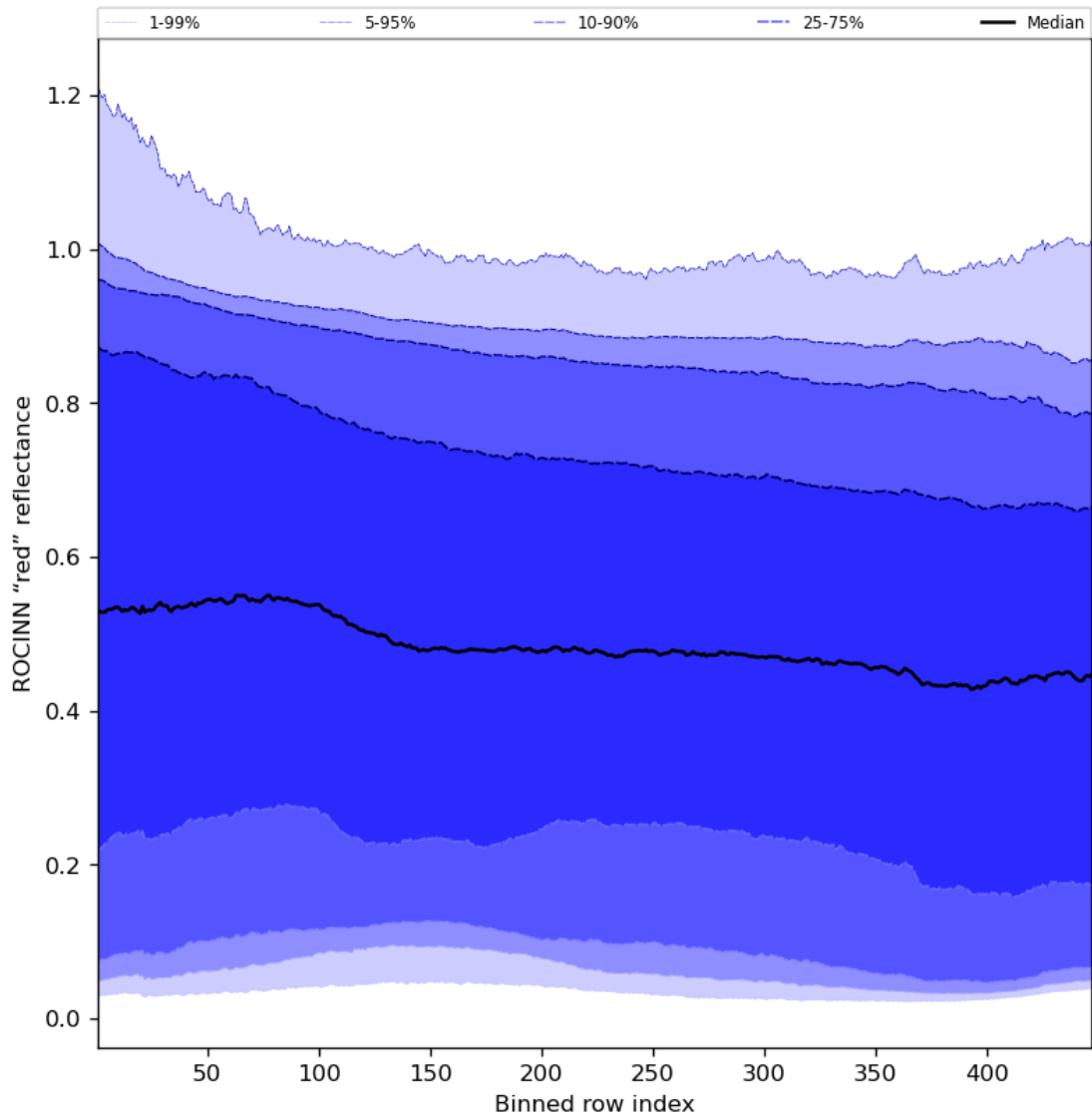
Figure 69: Along track statistics of "ROCINN "red" reflectance" for 2024-01-05 to 2024-01-07
