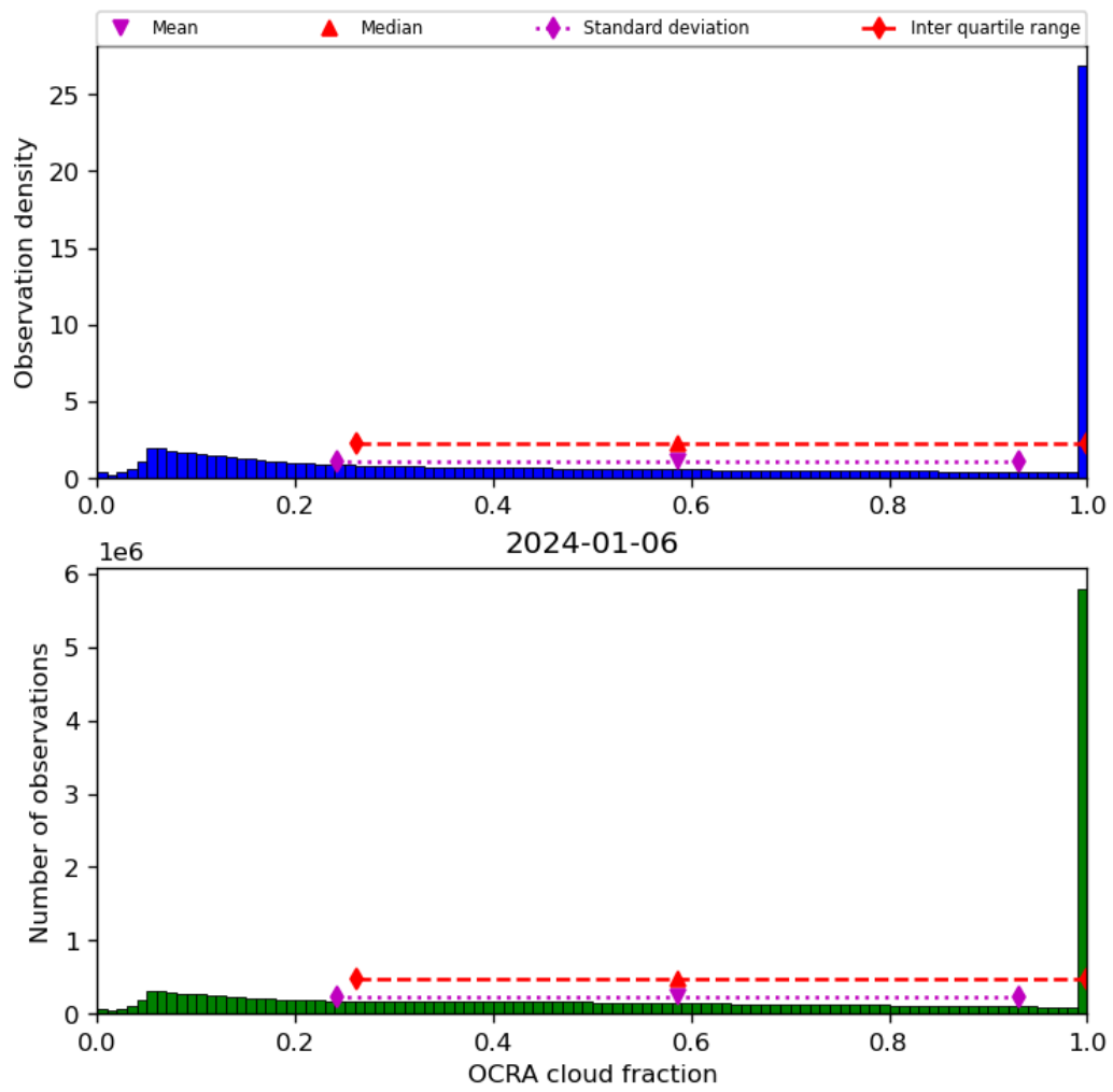
Figure 50: Histogram of “OCRA cloud fraction” for 2024-01-05 to 2024-01-07
