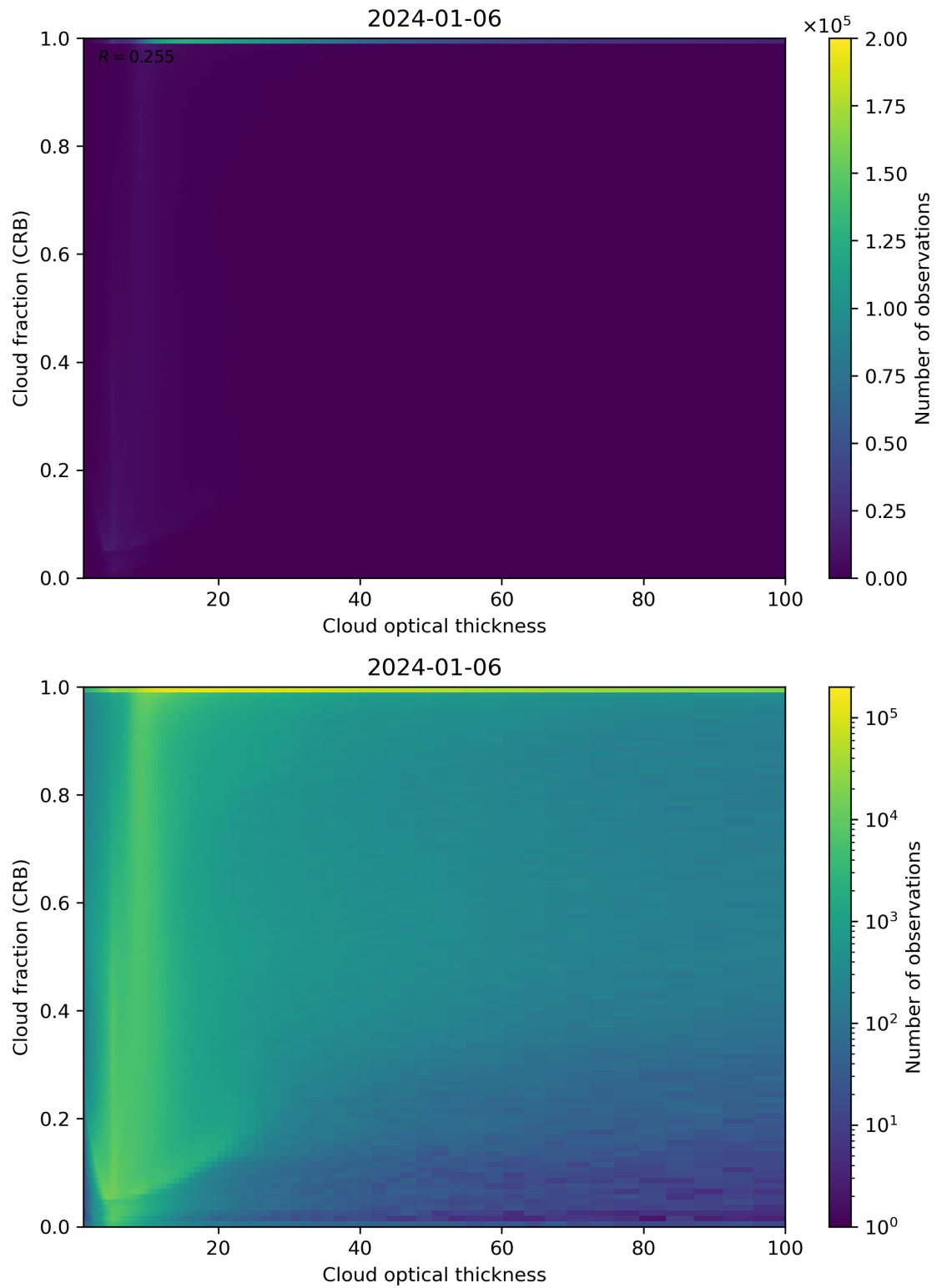
Figure 84: Scatter density plot of “Cloud optical thickness” against “Cloud fraction (CRB)” for 2024-01-05 to 2024-01-07.
