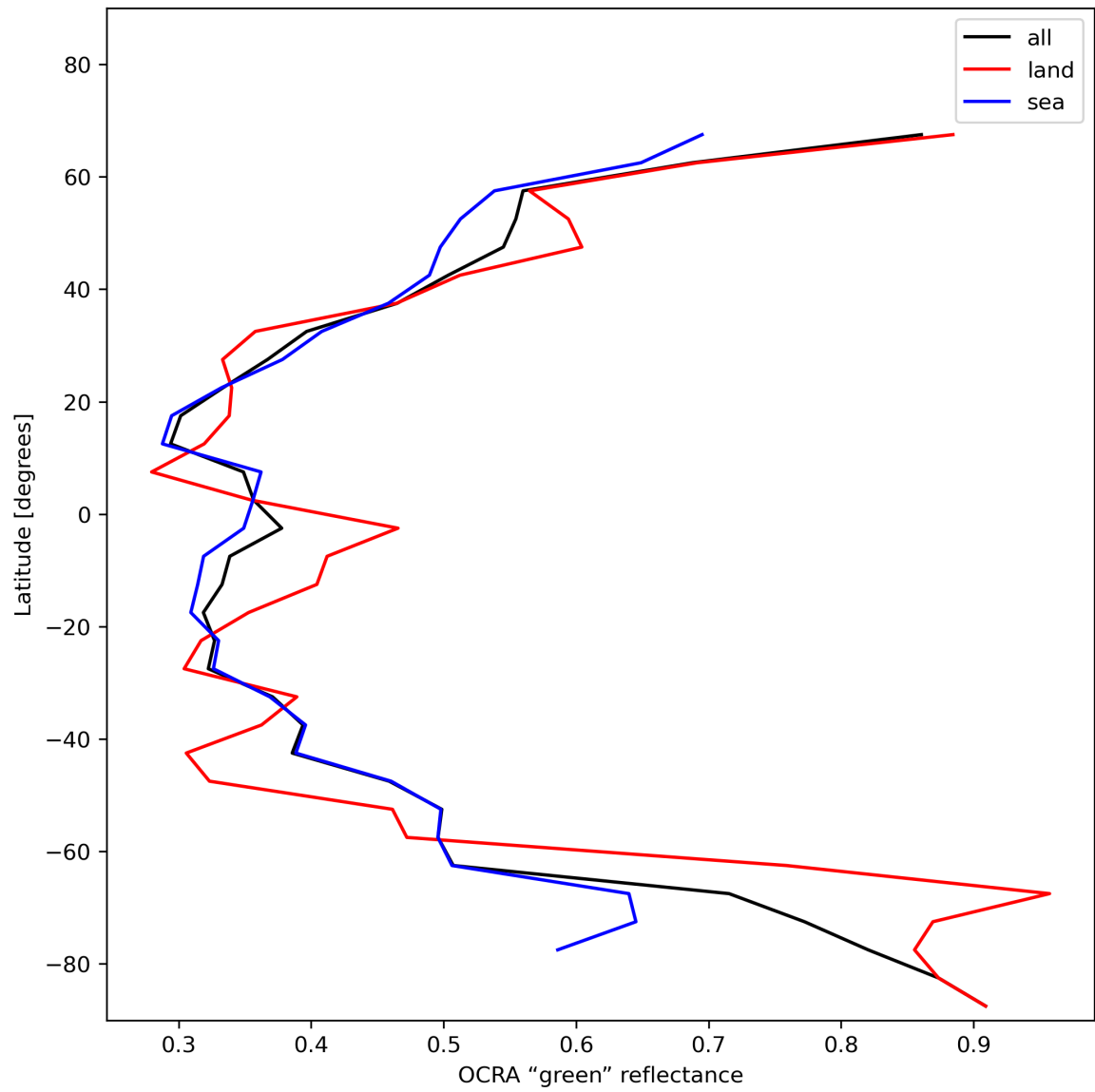
Figure 36: Zonal average of “OCRA “green” reflectance” for 2024-01-05 to 2024-01-07.
