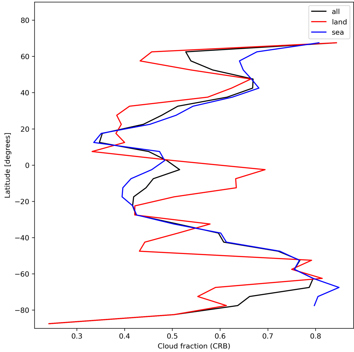
Figure 26: Zonal average of “Cloud fraction (CRB)” for 2024-01-05 to 2024-01-07.
