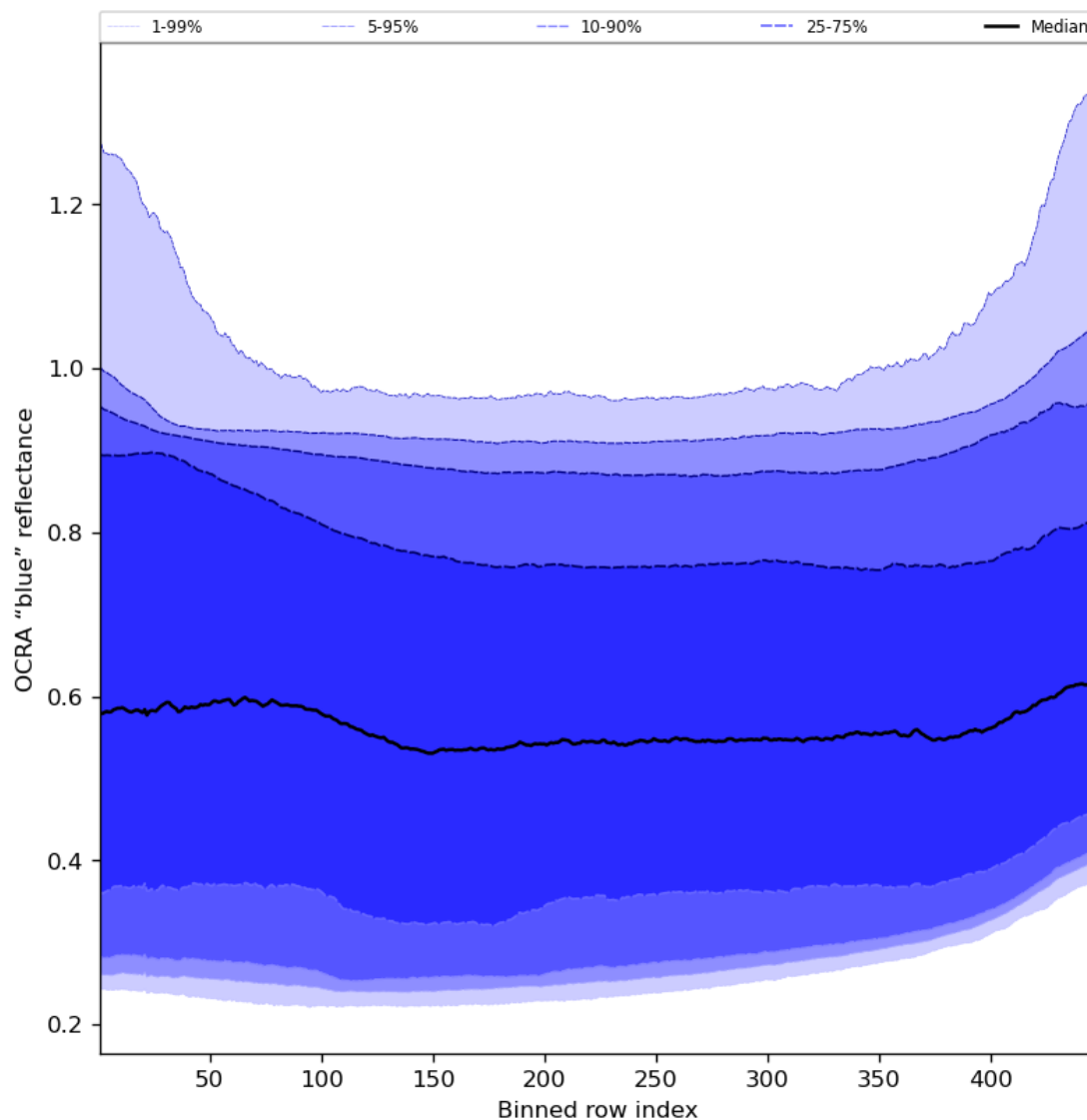
Figure 67: Along track statistics of “OCRA “blue” reflectance” for 2024-01-05 to 2024-01-07
