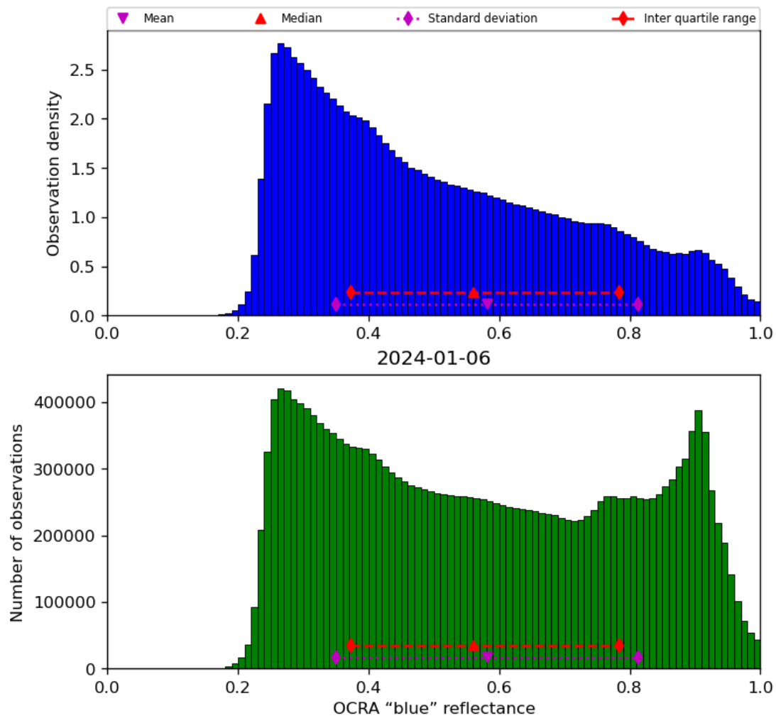
Figure 51: Histogram of "OCRA "blue" reflectance" for 2024-01-05 to 2024-01-07
