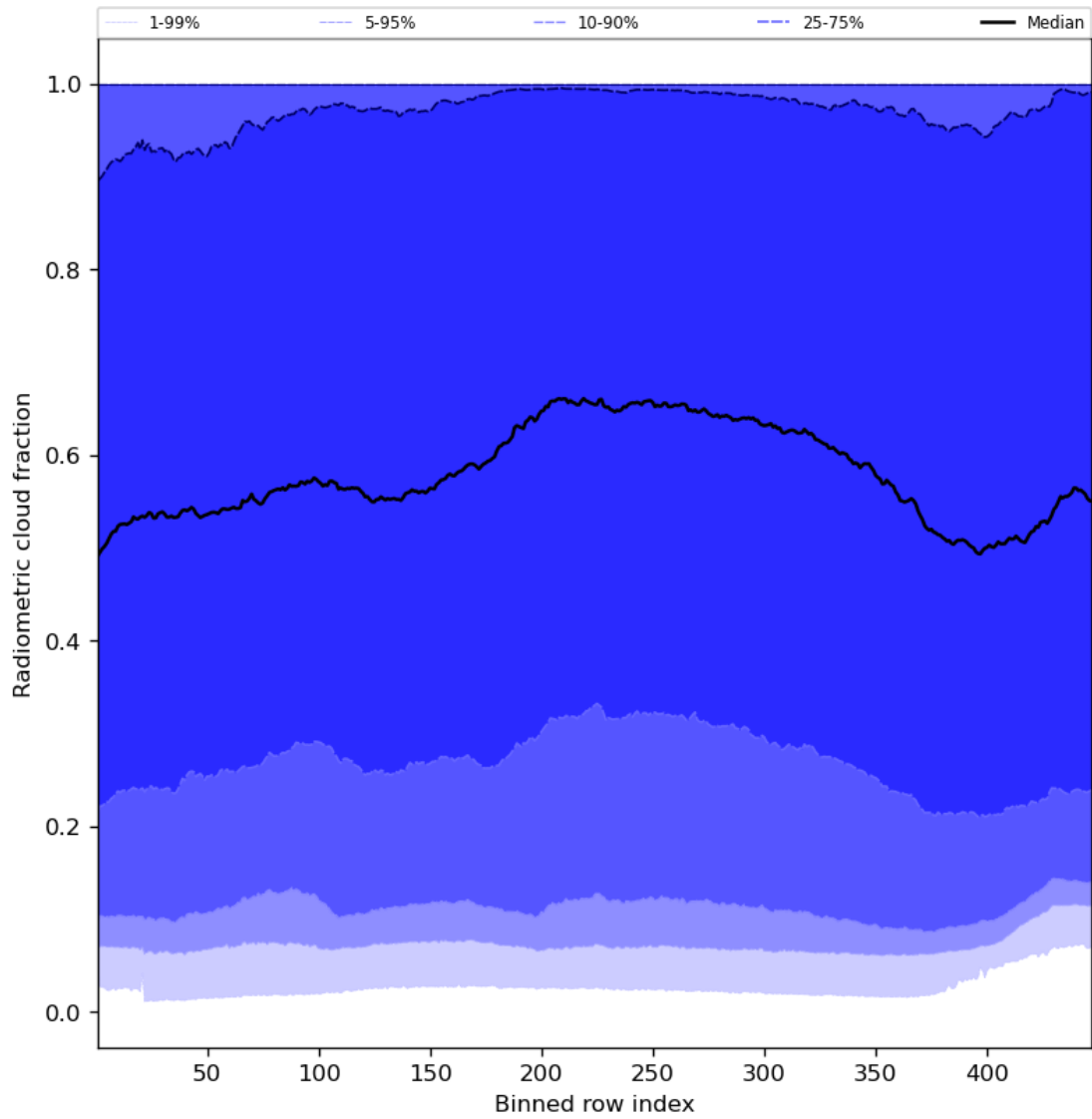
Figure 55: Along track statistics of “Radiometric cloud fraction” for 2024-01-05 to 2024-01-07
