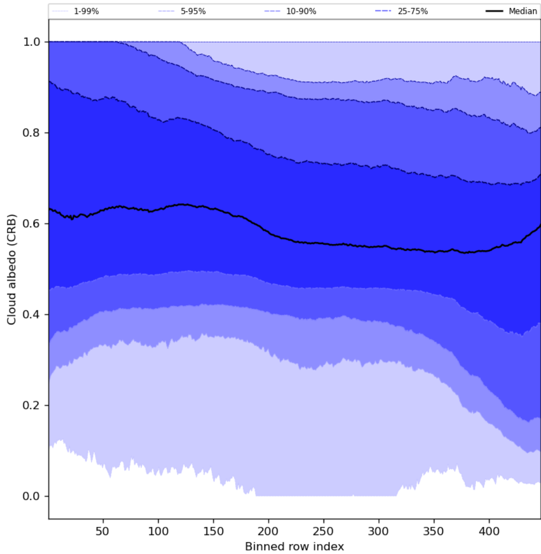
Figure 60: Along track statistics of “Cloud albedo (CRB)” for 2024-01-05 to 2024-01-07
