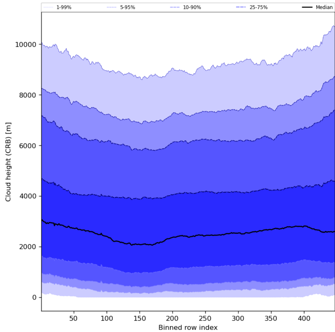
Figure 59: Along track statistics of “Cloud height (CRB)” for 2024-01-05 to 2024-01-07
