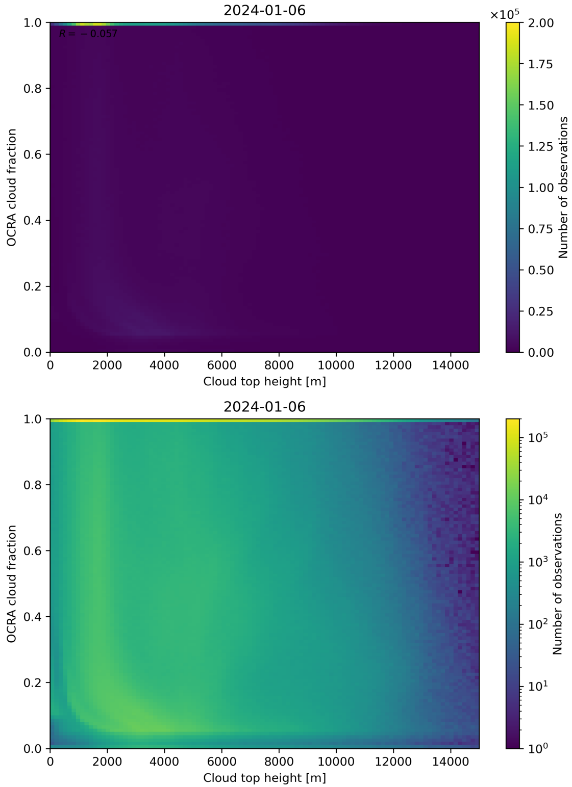
Figure 87: Scatter density plot of “Cloud top height” against “OCRA cloud fraction” for 2024-01-05 to 2024-01-07.
