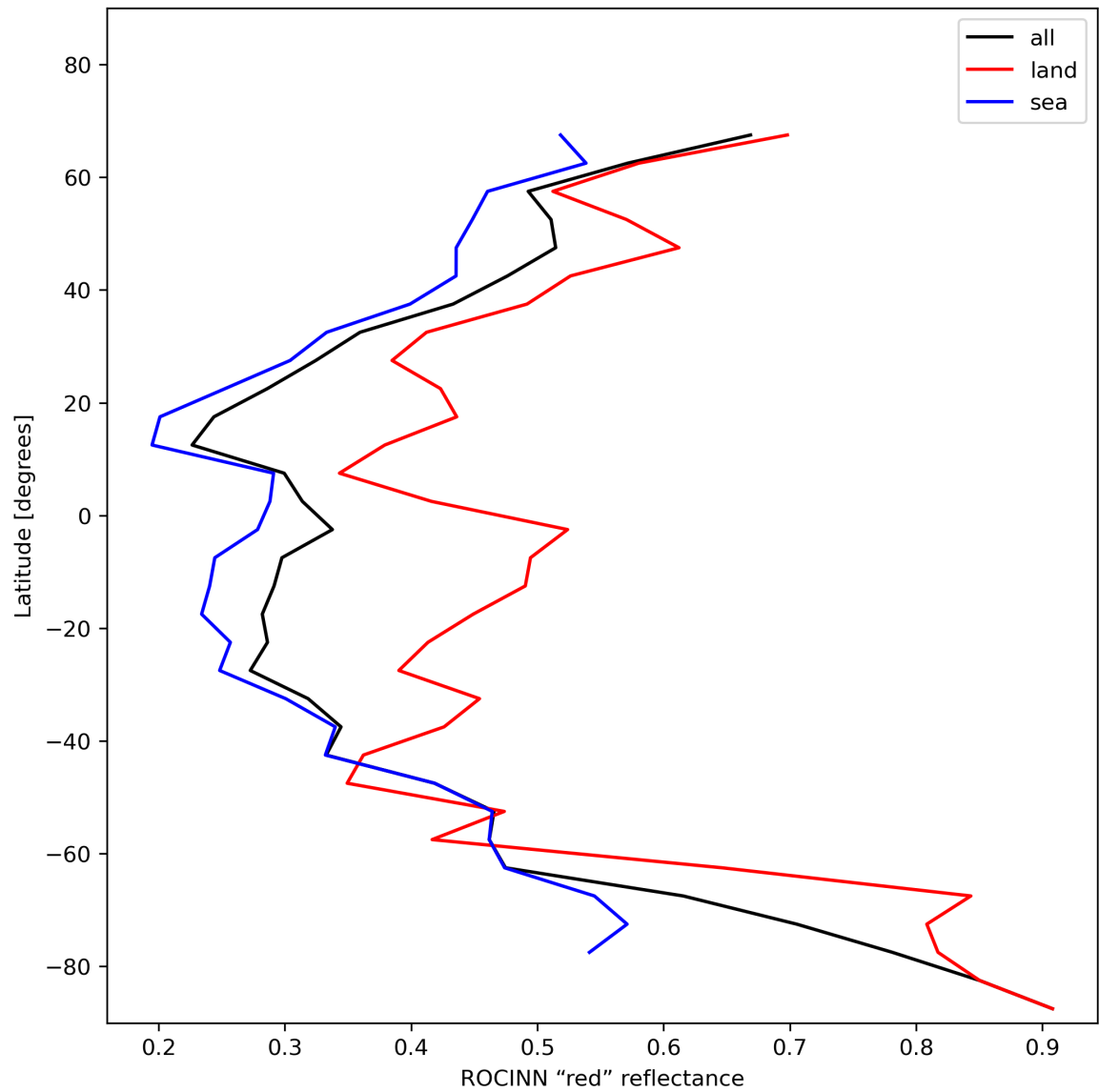
Figure 37: Zonal average of “ROCINN “red” reflectance” for 2024-01-05 to 2024-01-07.
