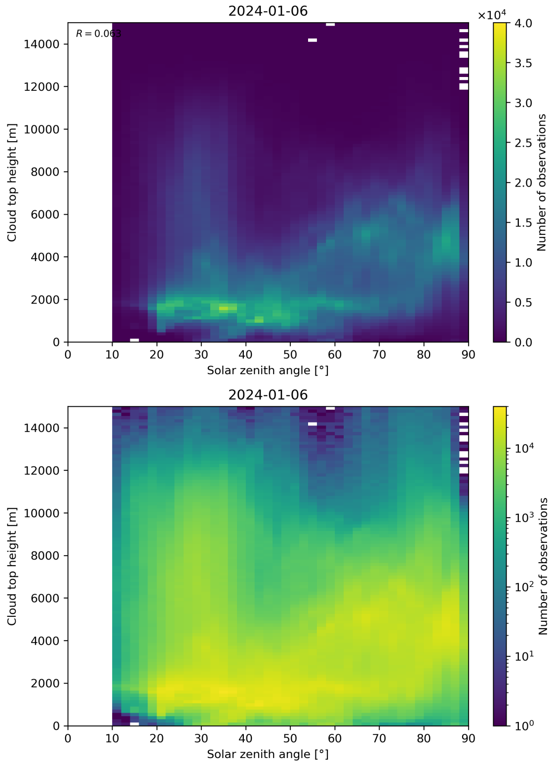
Figure 104: Scatter density plot of “Solar zenith angle” against “Cloud top height” for 2024-01-05 to 2024-01-07.
