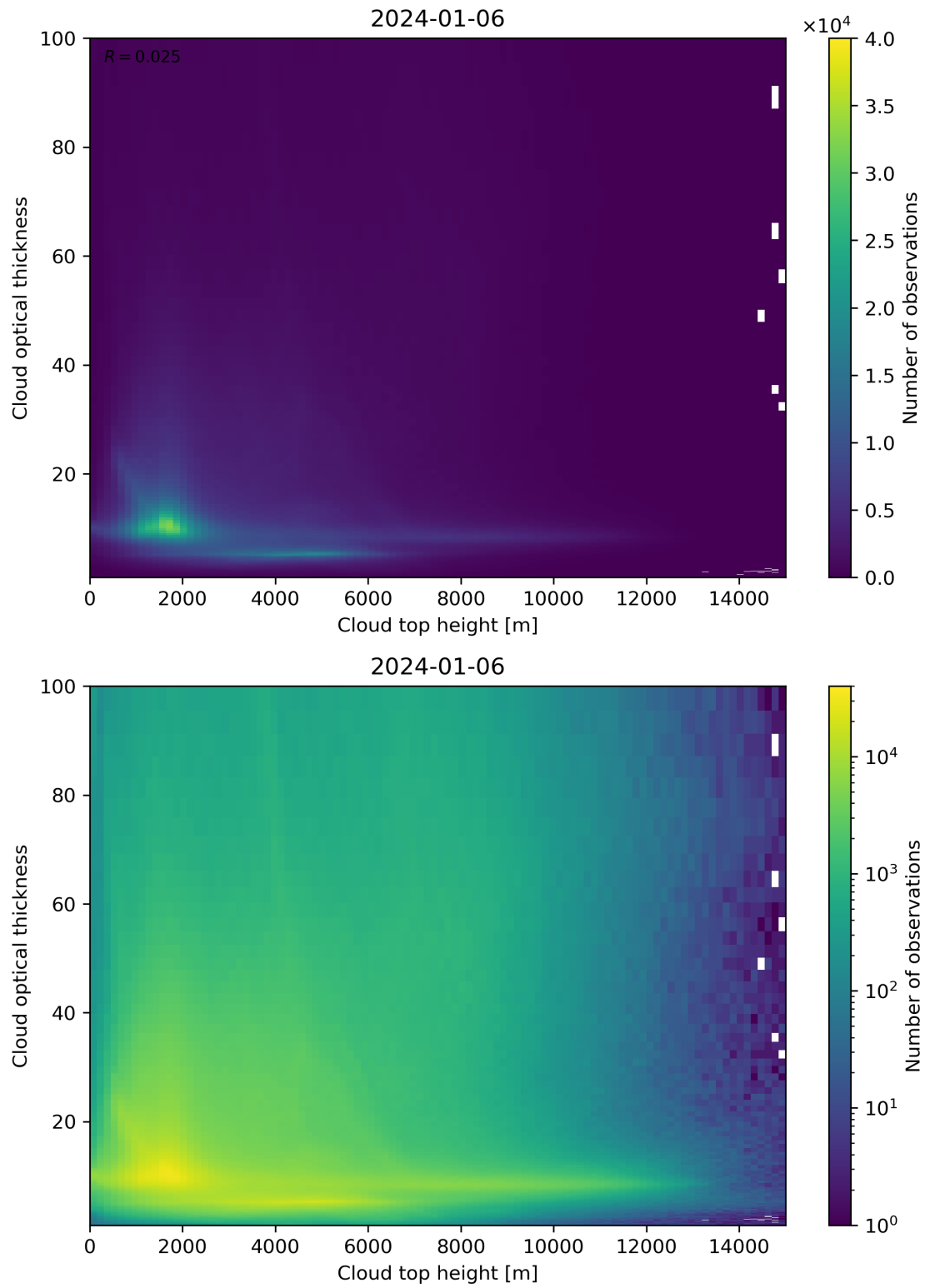
Figure 90: Scatter density plot of “Cloud top height” against “Cloud optical thickness” for 2024-01-05 to 2024-01-07.
