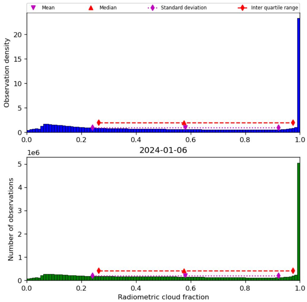
Figure 39: Histogram of “Radiometric cloud fraction” for 2024-01-05 to 2024-01-07
