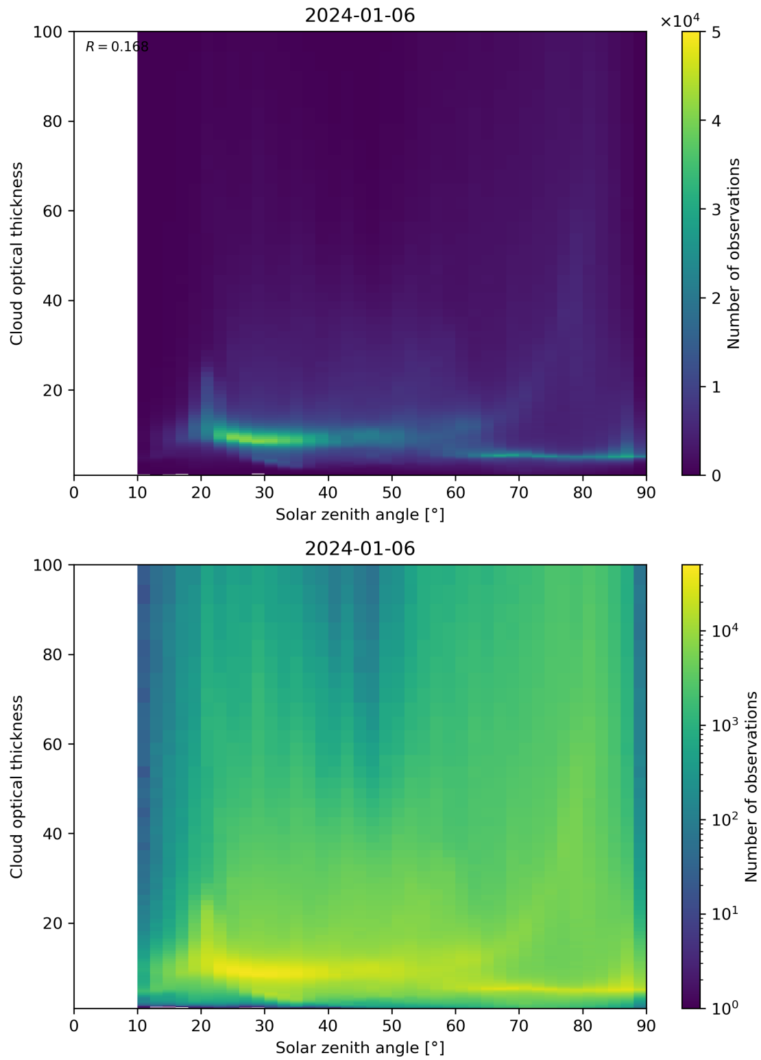
Figure 103: Scatter density plot of “Solar zenith angle” against “Cloud optical thickness” for 2024-01-05 to 2024-01-07.
