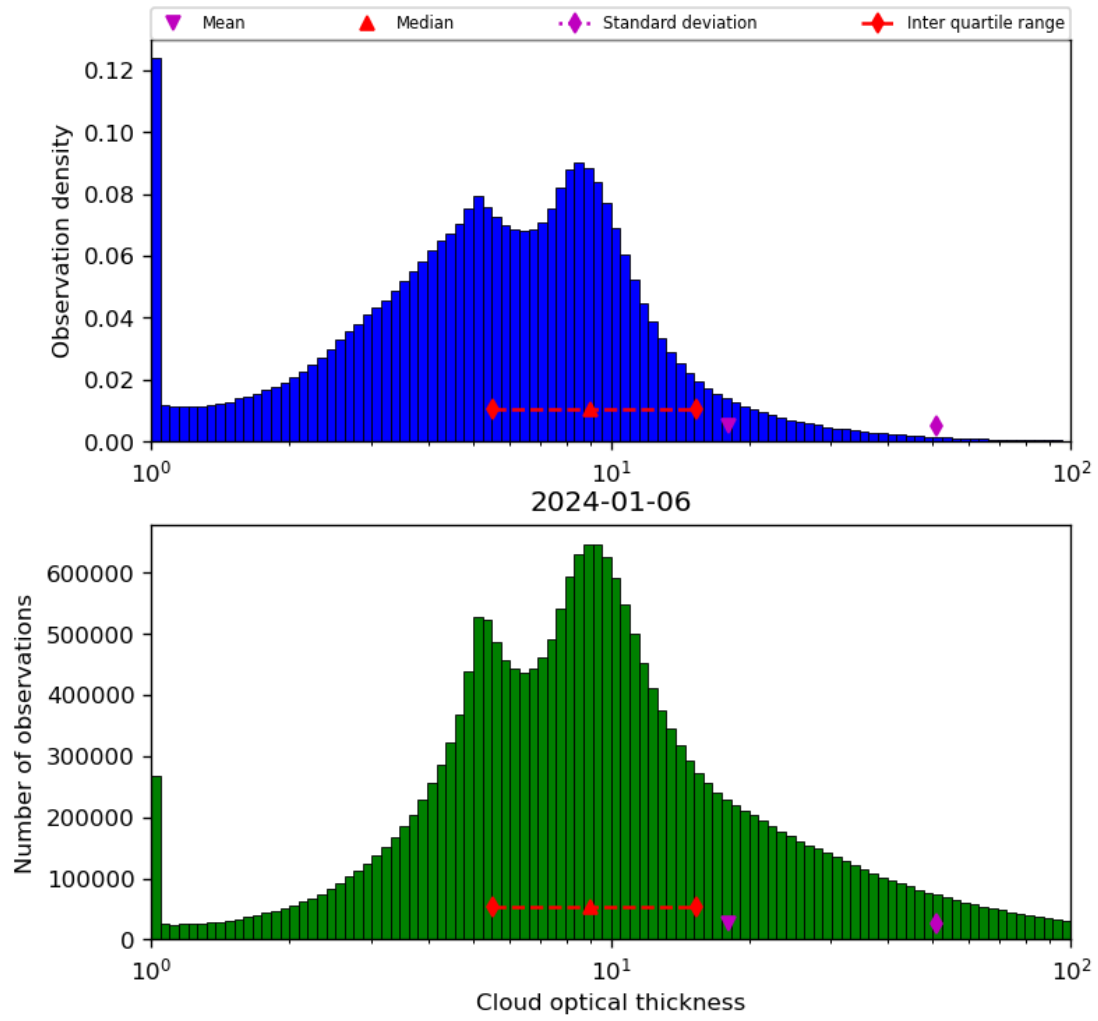
Figure 41: Histogram of “Cloud optical thickness” for 2024-01-05 to 2024-01-07
