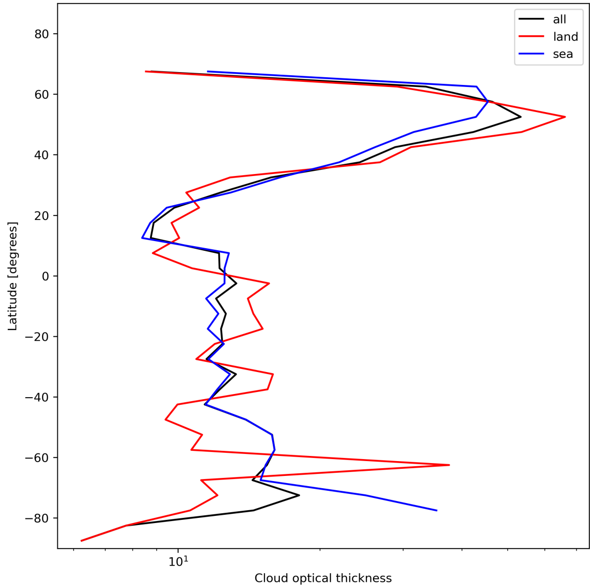
Figure 25: Zonal average of “Cloud optical thickness” for 2024-01-05 to 2024-01-07.
