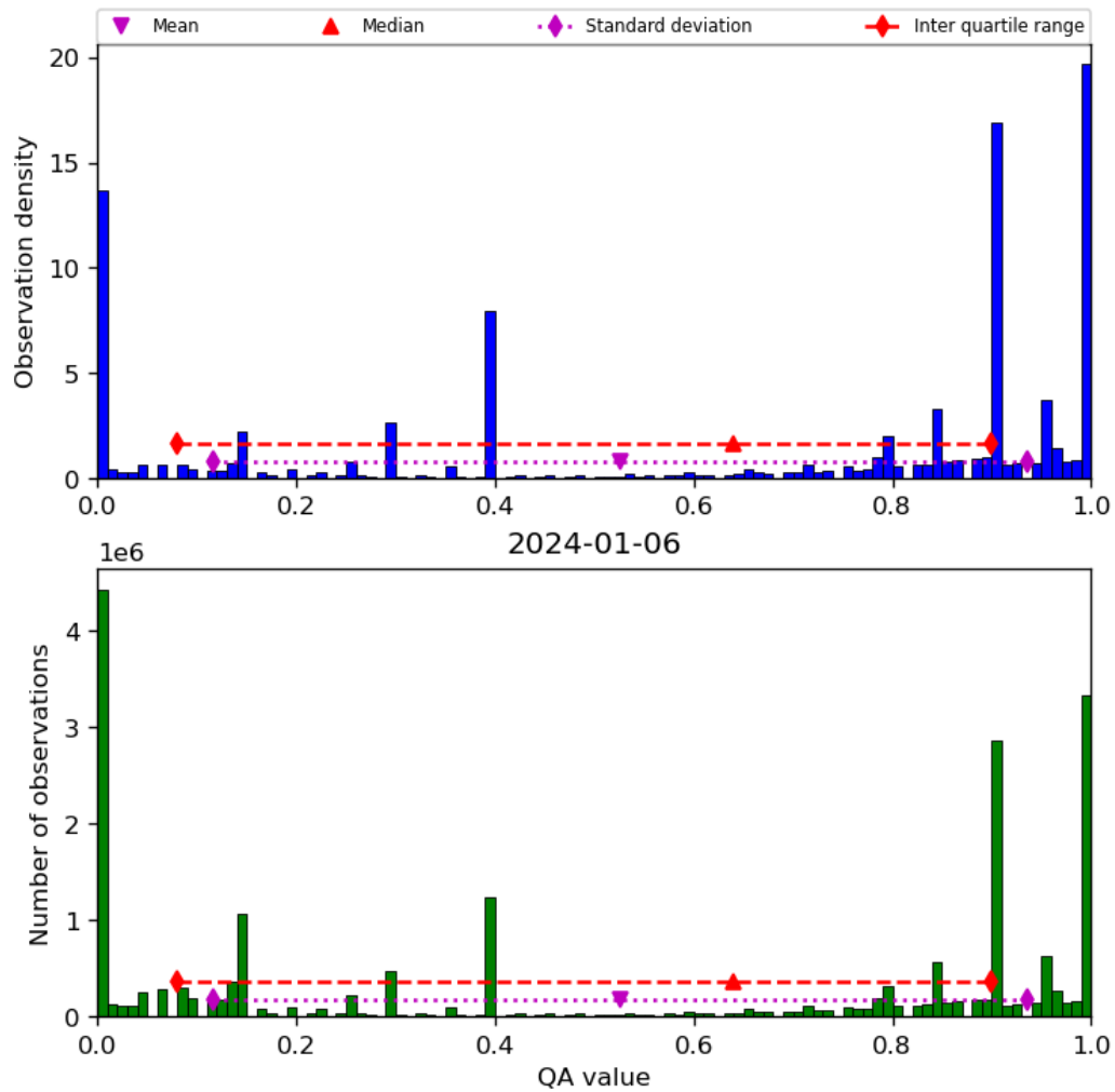
Figure 38: Histogram of “QA value” for 2024-01-05 to 2024-01-07
