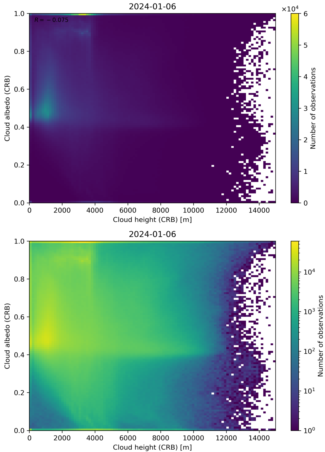
Figure 80: Scatter density plot of “Cloud height (CRB)” against “Cloud albedo (CRB)” for 2024-01-05 to 2024-01-07.
