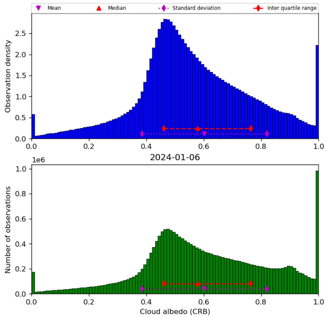
Figure 44: Histogram of “Cloud albedo (CRB)” for 2024-01-05 to 2024-01-07
