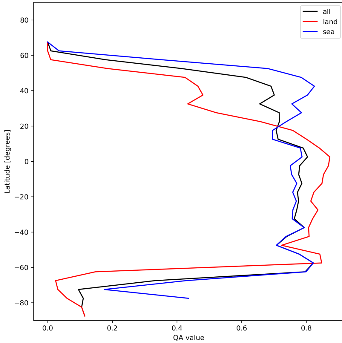
Figure 22: Zonal average of “QA value” for 2024-01-05 to 2024-01-07.
