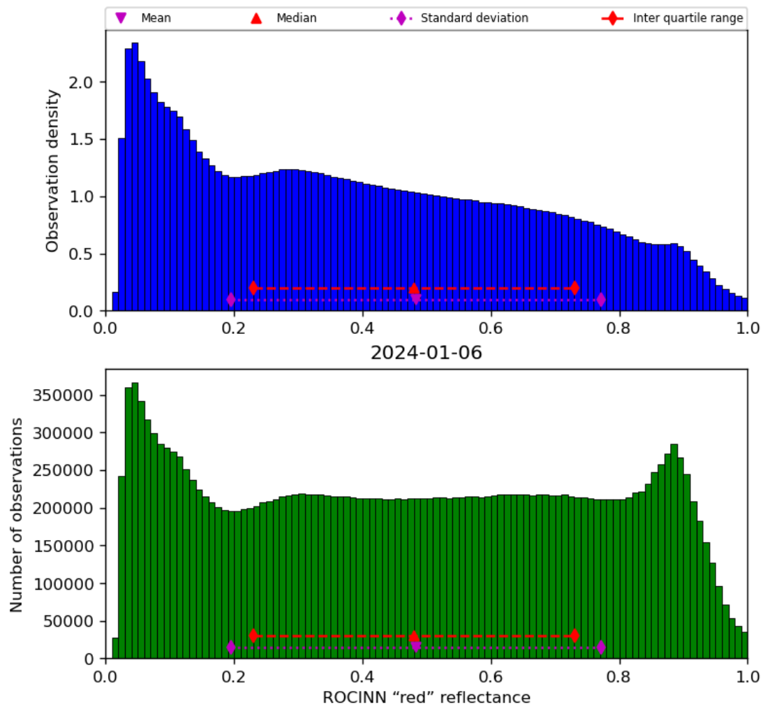
Figure 53: Histogram of “ROCINN “red” reflectance” for 2024-01-05 to 2024-01-07
