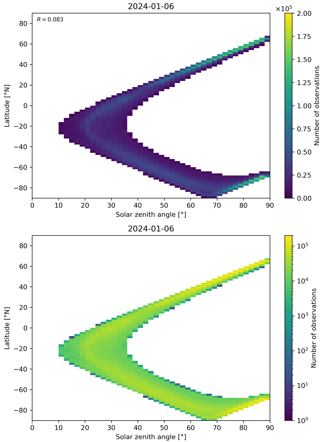
Figure 105: Scatter density plot of “Solar zenith angle” against “Latitude” for 2024-01-05 to 2024-01-07.
