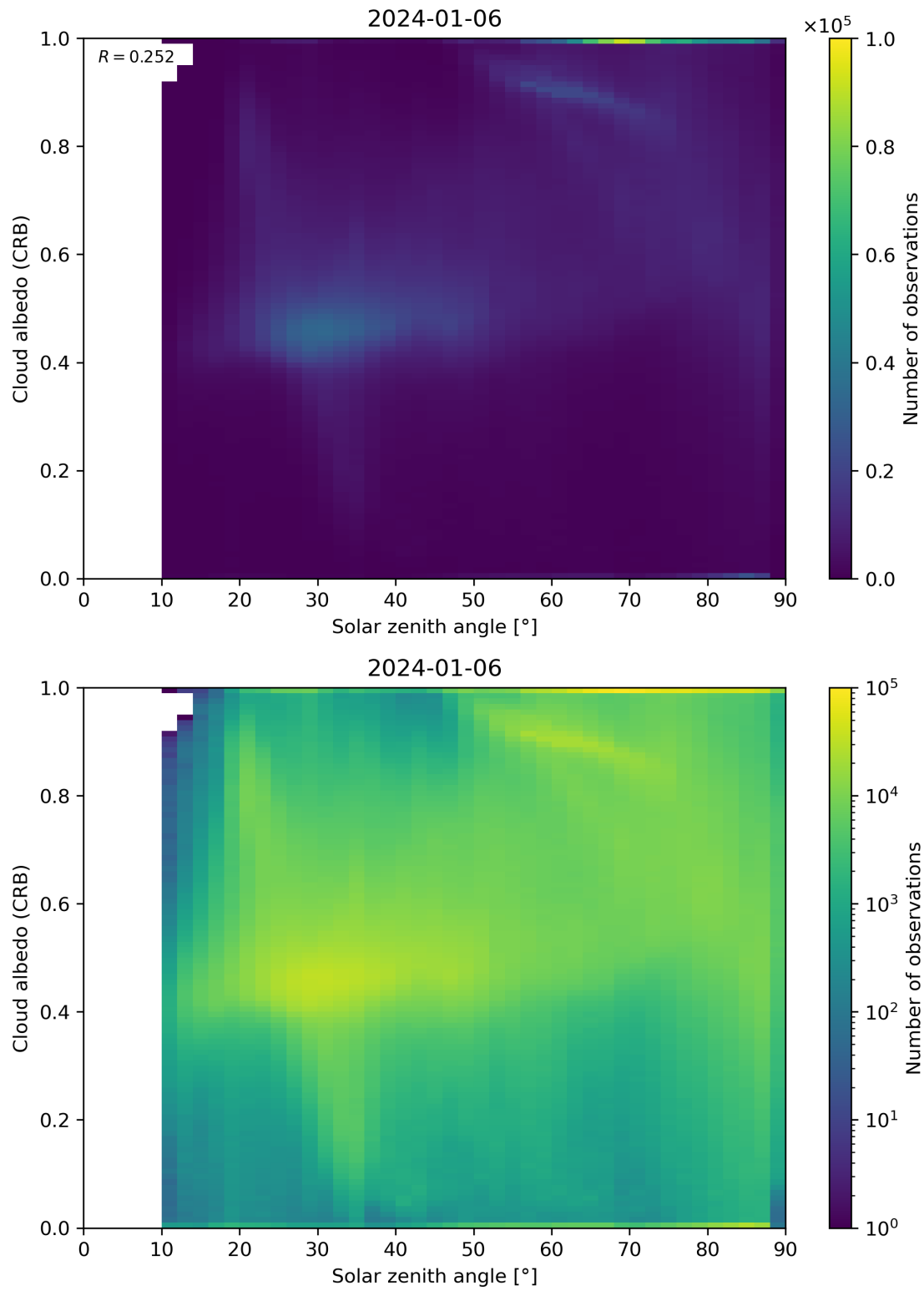
Figure 98: Scatter density plot of “Solar zenith angle” against “Cloud albedo (CRB)” for 2024-01-05 to 2024-01-07.
