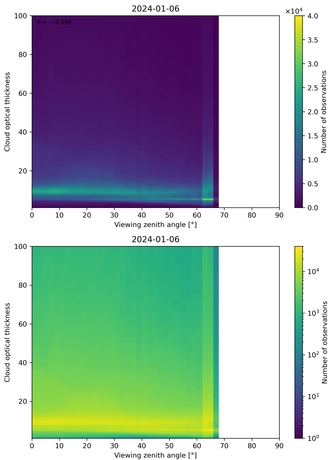
Figure 111: Scatter density plot of “Viewing zenith angle” against “Cloud optical thickness” for 2024-01-05 to 2024-01-07.
