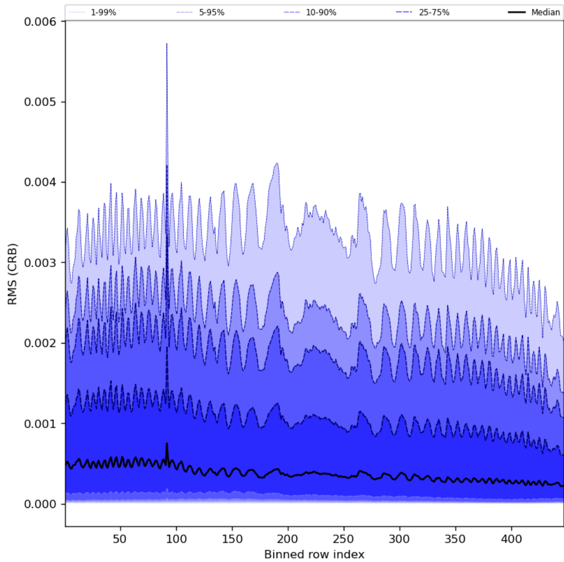
Figure 64: Along track statistics of “RMS (CRB)” for 2024-01-05 to 2024-01-07
