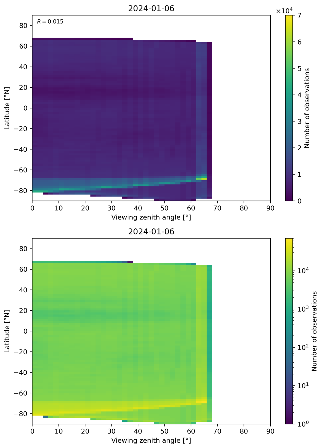
Figure 113: Scatter density plot of “Viewing zenith angle” against “Latitude” for 2024-01-05 to 2024-01-07.
