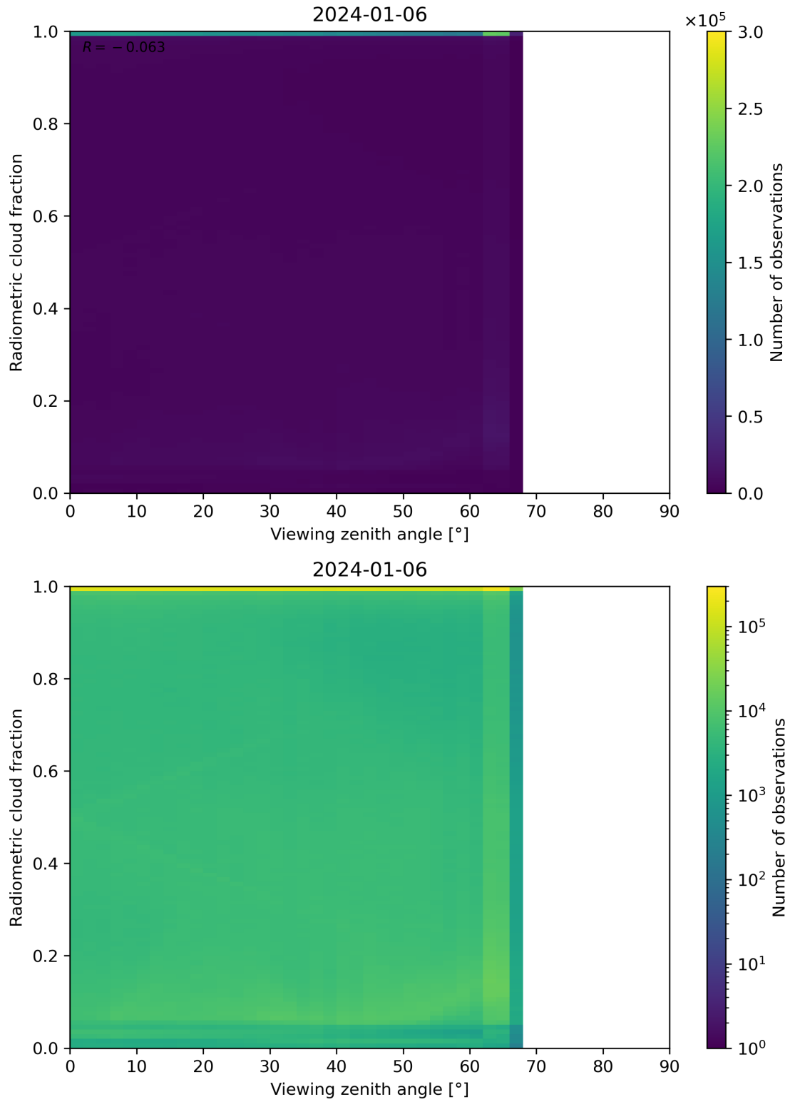
Figure 107: Scatter density plot of “Viewing zenith angle” against “Radiometric cloud fraction” for 2024-01-05 to 2024-01-07.
