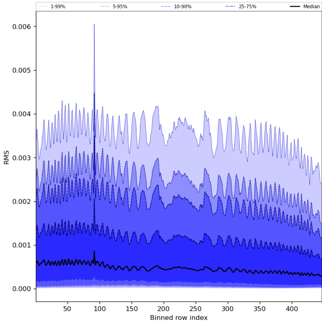
Figure 63: Along track statistics of “RMS” for 2024-01-05 to 2024-01-07
