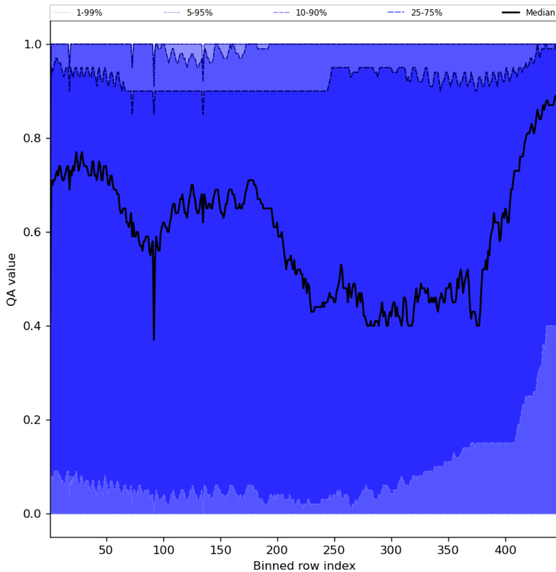
Figure 54: Along track statistics of “QA value” for 2024-01-05 to 2024-01-07
