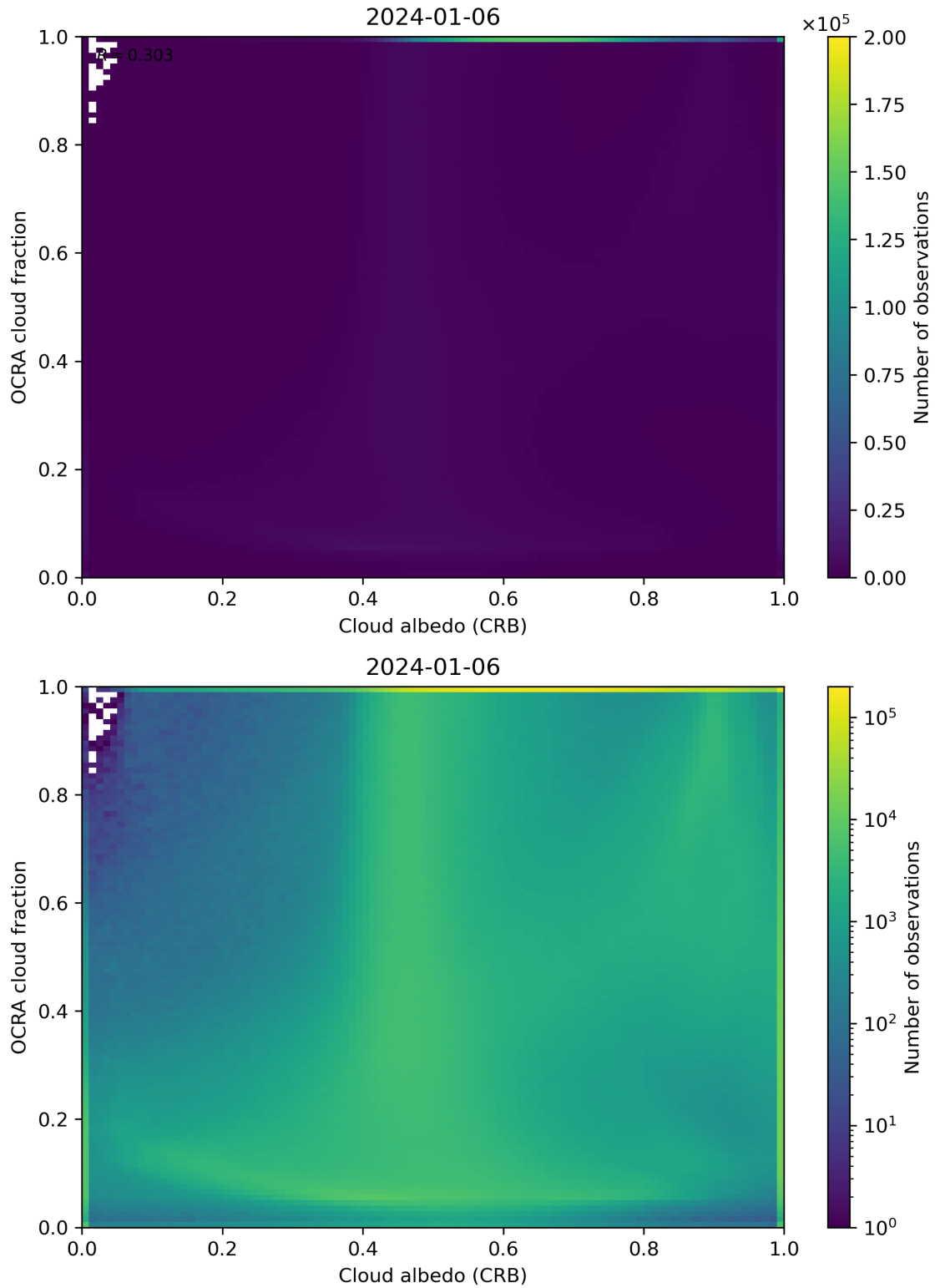
Figure 70: Scatter density plot of “Cloud albedo (CRB)” against “OCRA cloud fraction” for 2024-01-05 to 2024-01-07.
