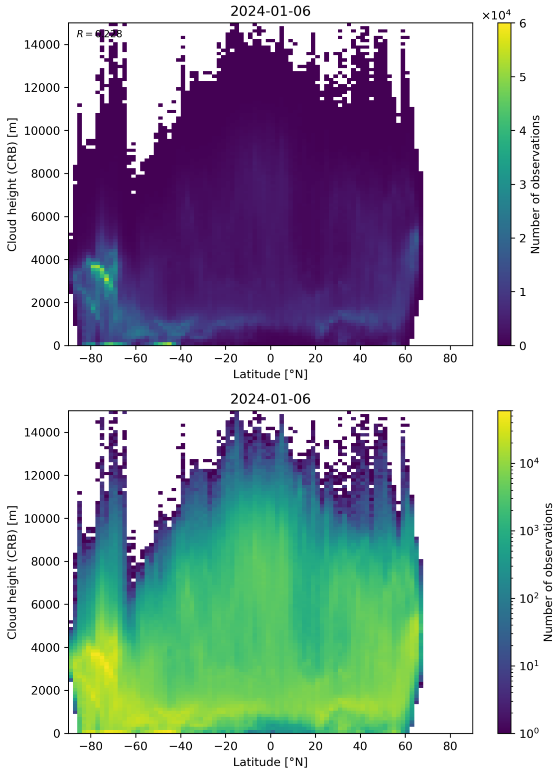
Figure 95: Scatter density plot of “Latitude” against “Cloud height (CRB)” for 2024-01-05 to 2024-01-07.
