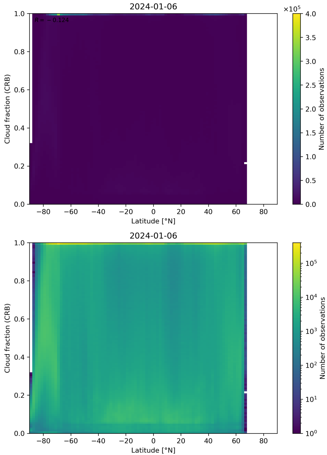
Figure 94: Scatter density plot of “Latitude” against “Cloud fraction (CRB)” for 2024-01-05 to 2024-01-07.
