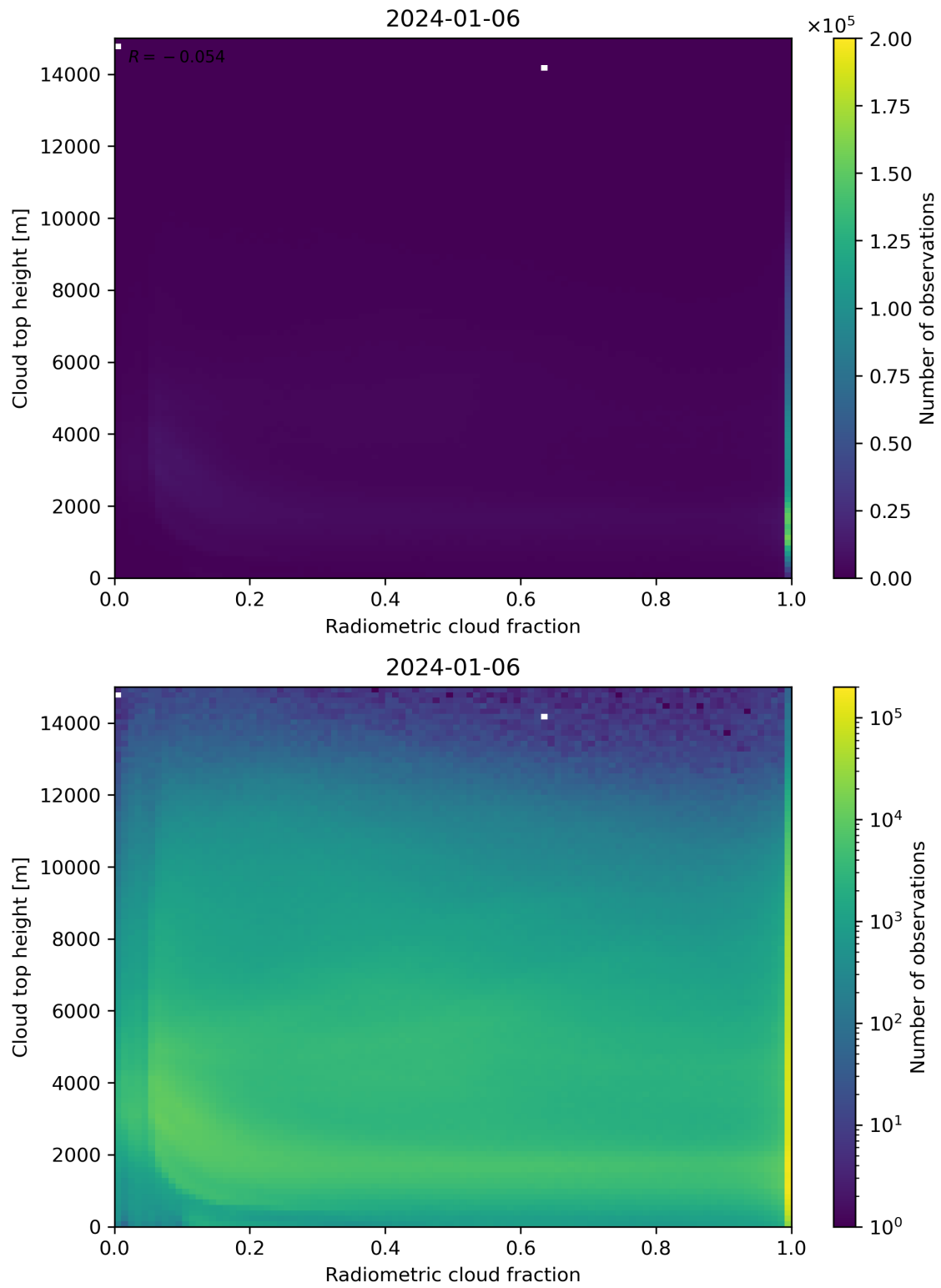
Figure 76: Scatter density plot of “Radiometric cloud fraction” against “Cloud top height” for 2024-01-05 to 2024-01-07.
