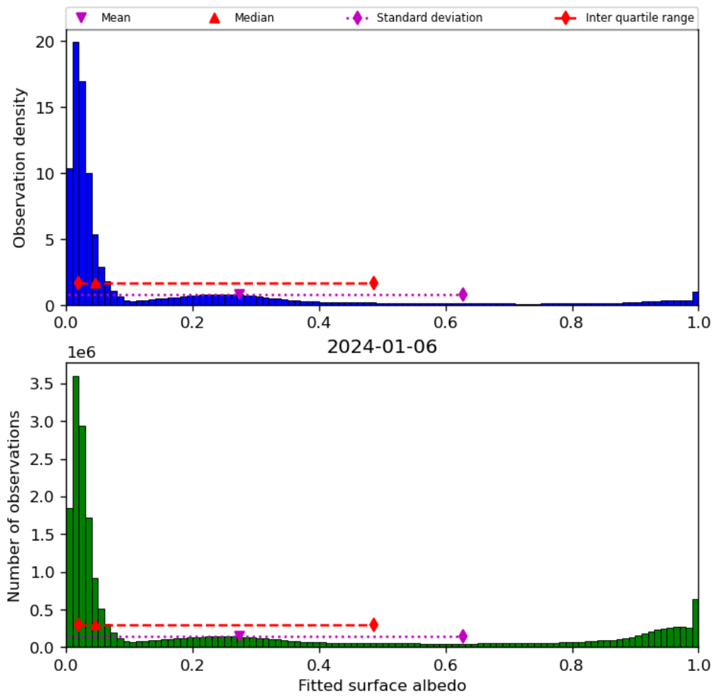
Figure 45: Histogram of “Fitted surface albedo” for 2024-01-05 to 2024-01-07
