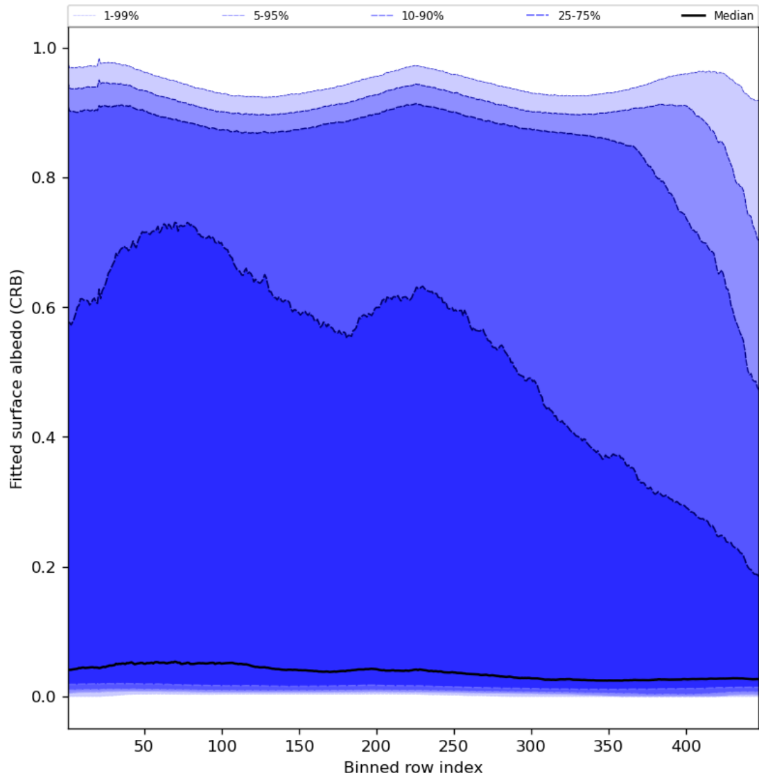
Figure 62: Along track statistics of “Fitted surface albedo (CRB)” for 2024-01-05 to 2024-01-07
