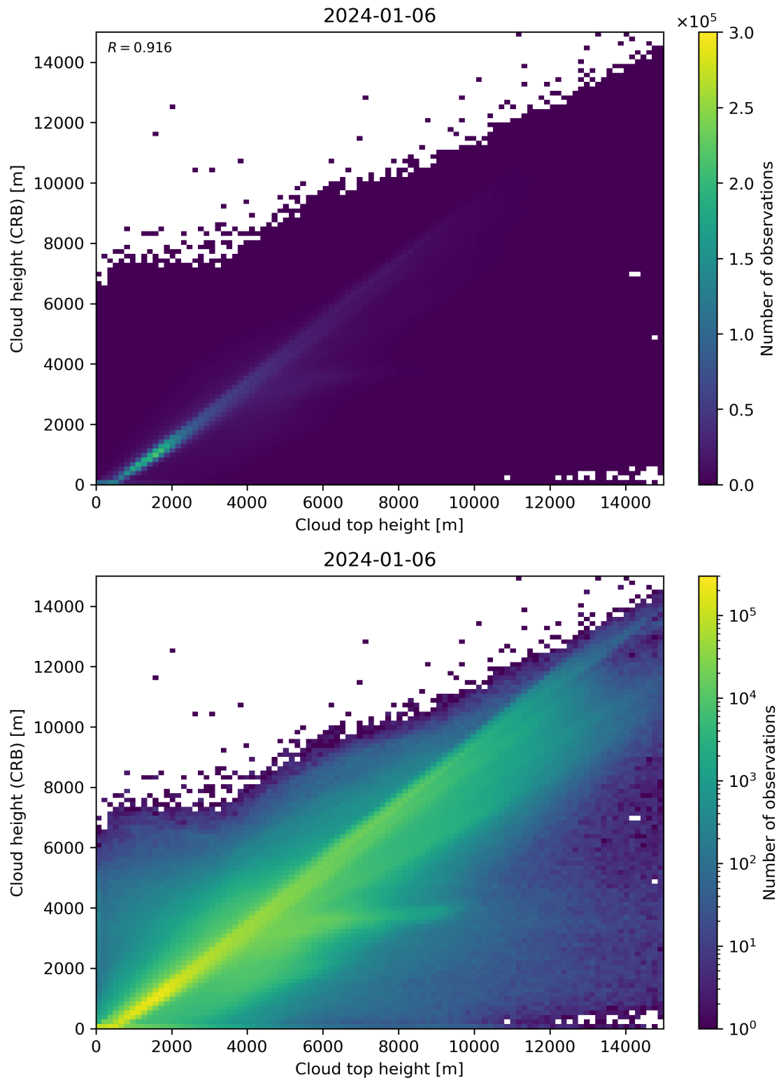
Figure 89: Scatter density plot of “Cloud top height” against “Cloud height (CRB)” for 2024-01-05 to 2024-01-07.
