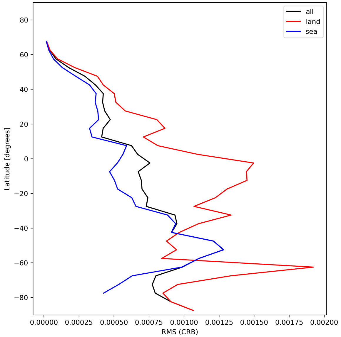
Figure 32: Zonal average of “RMS (CRB)” for 2024-01-05 to 2024-01-07.
