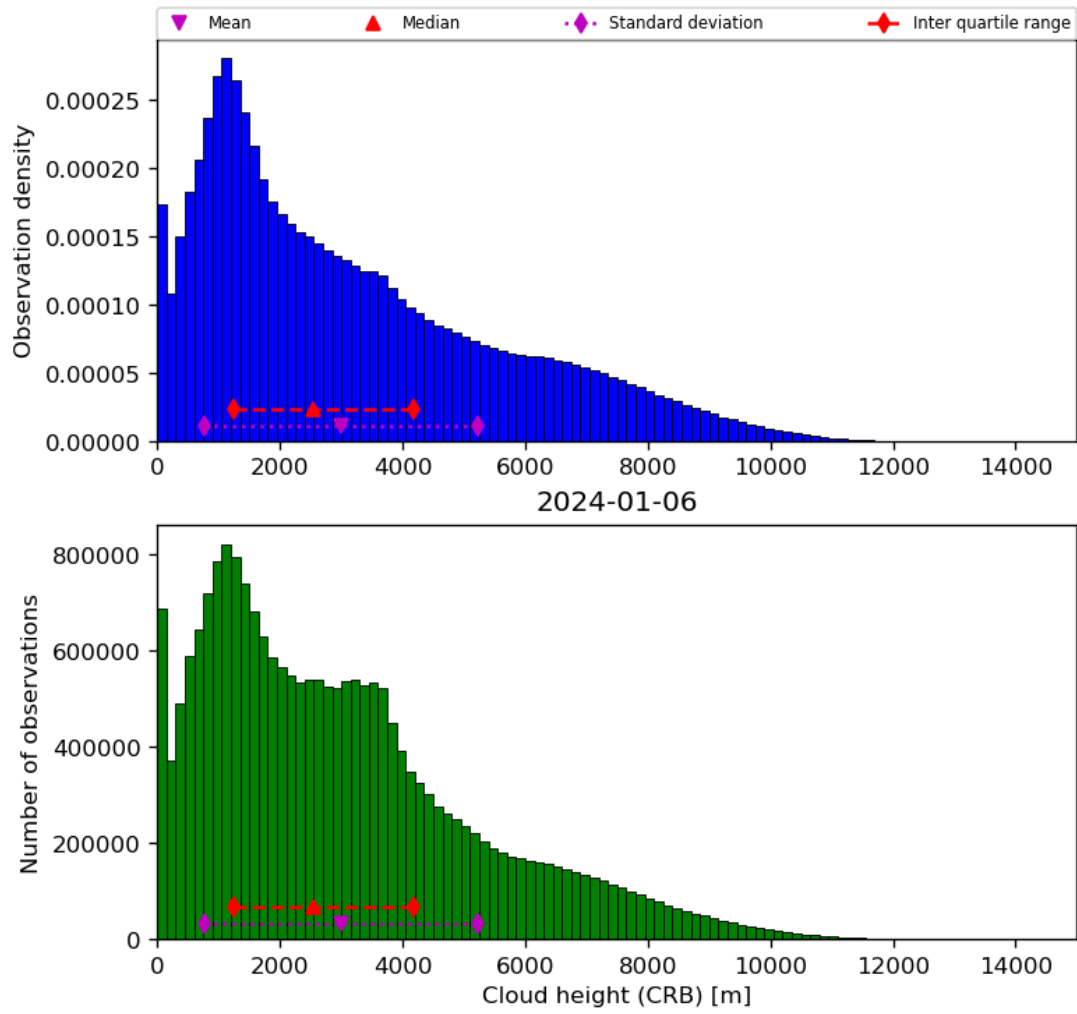
Figure 43: Histogram of “Cloud height (CRB)” for 2024-01-05 to 2024-01-07
