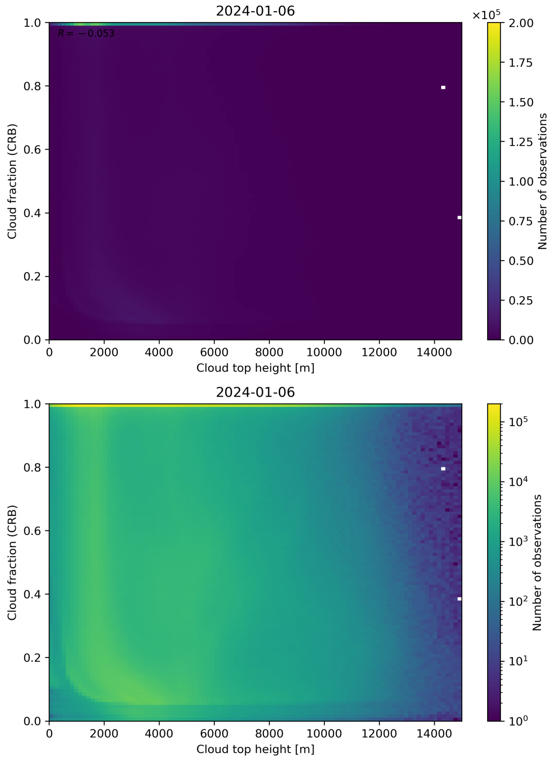
Figure 88: Scatter density plot of “Cloud top height” against “Cloud fraction (CRB)” for 2024-01-05 to 2024-01-07.
