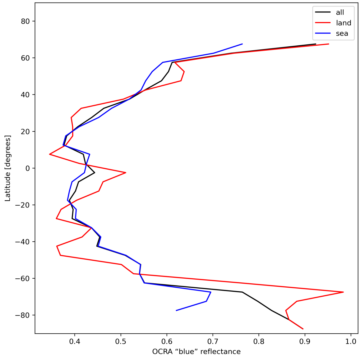
Figure 35: Zonal average of “OCRA “blue” reflectance” for 2024-01-05 to 2024-01-07.
