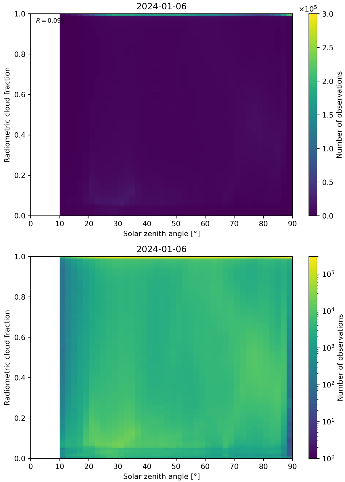
Figure 99: Scatter density plot of “Solar zenith angle” against “Radiometric cloud fraction” for 2024-01-05 to 2024-01-07.
