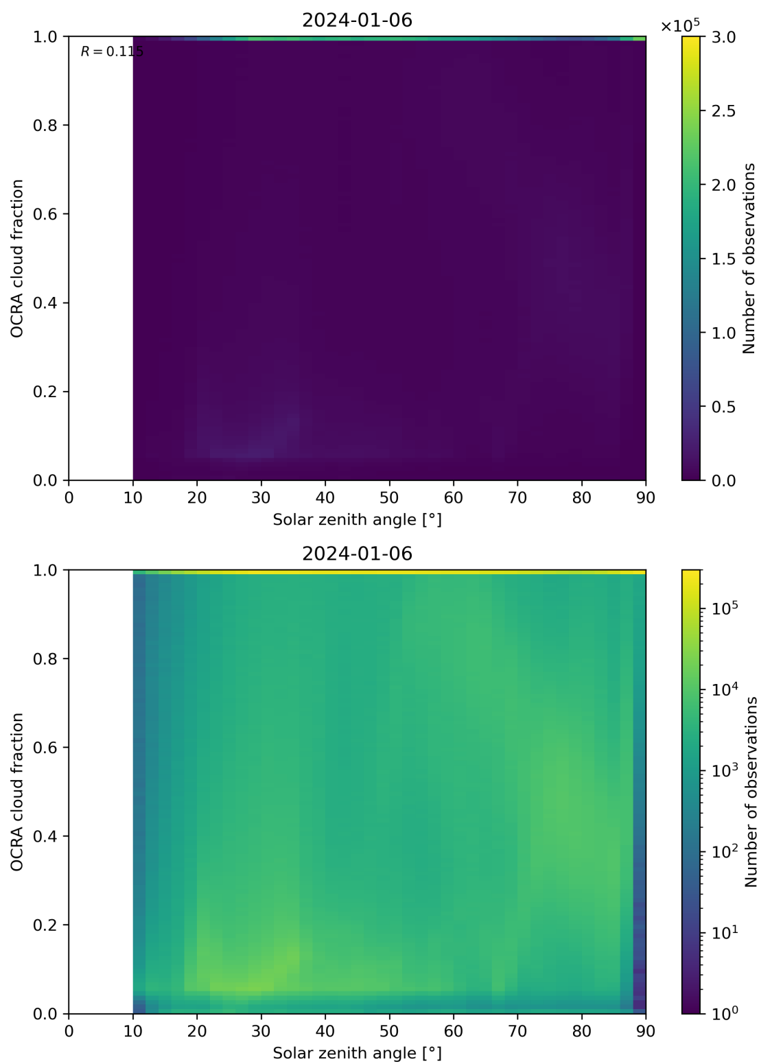
Figure 100: Scatter density plot of “Solar zenith angle” against “OCRA cloud fraction” for 2024-01-05 to 2024-01-07.
