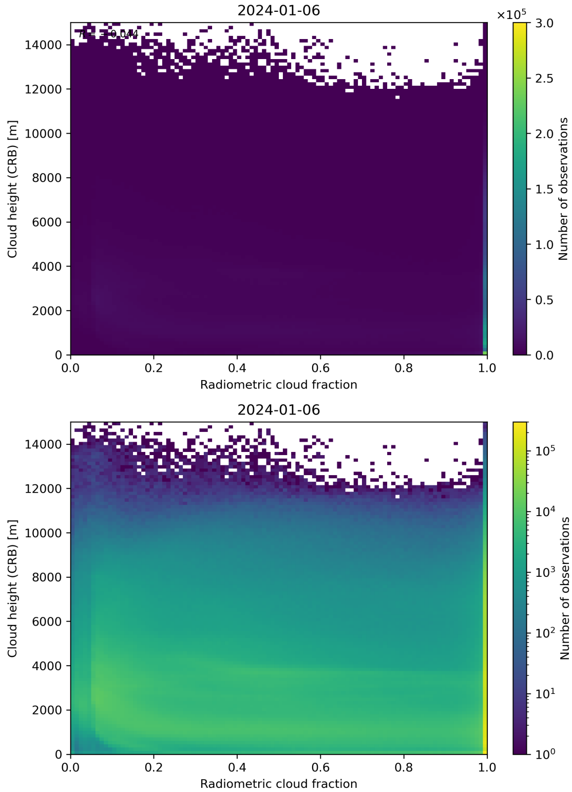
Figure 74: Scatter density plot of “Radiometric cloud fraction” against “Cloud height (CRB)” for 2024-01-05 to 2024-01-07.
