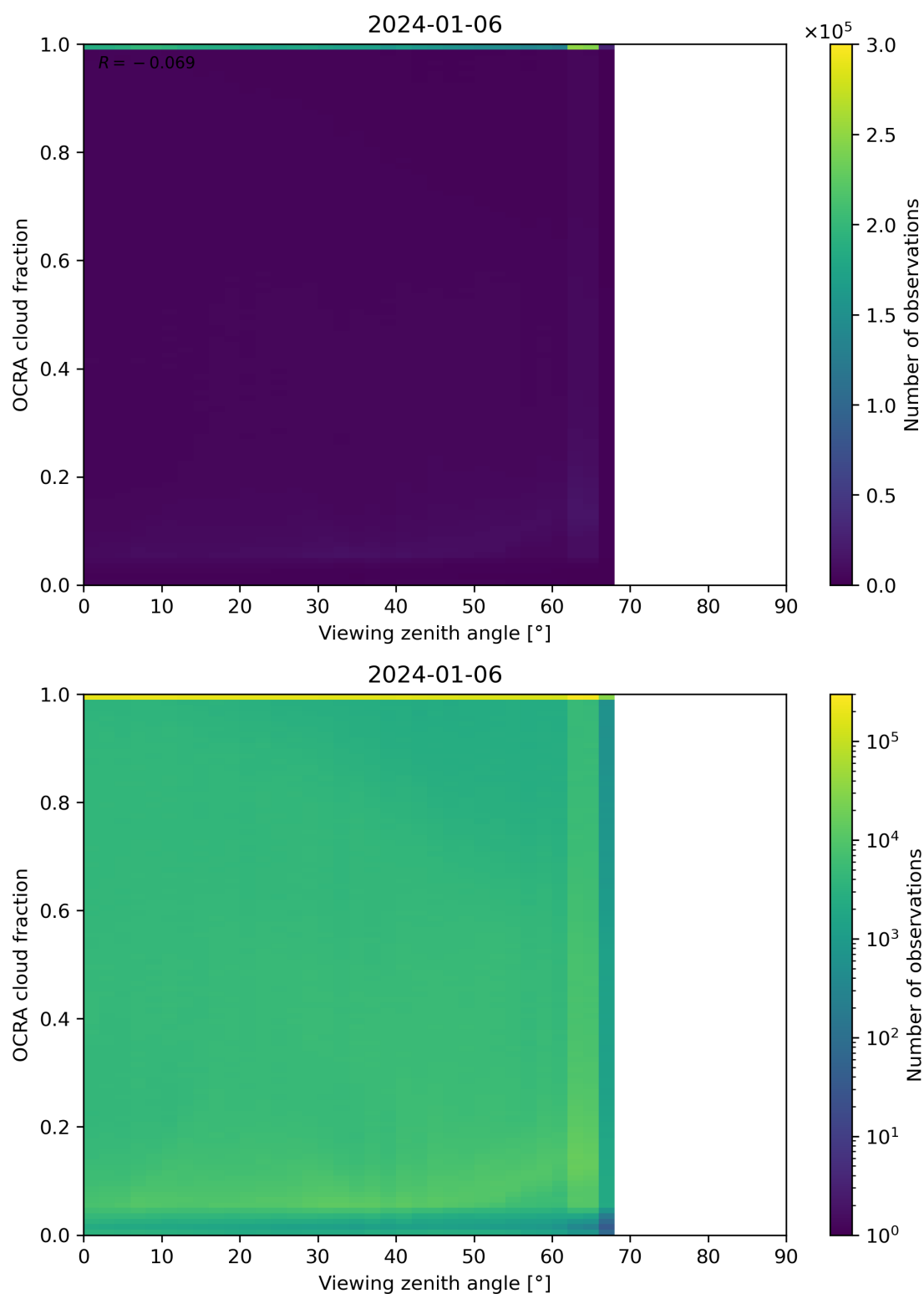
Figure 108: Scatter density plot of “Viewing zenith angle” against “OCRA cloud fraction” for 2024-01-05 to 2024-01-07.
