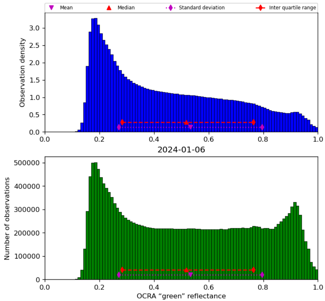
Figure 52: Histogram of “OCRA “green” reflectance” for 2024-01-05 to 2024-01-07
