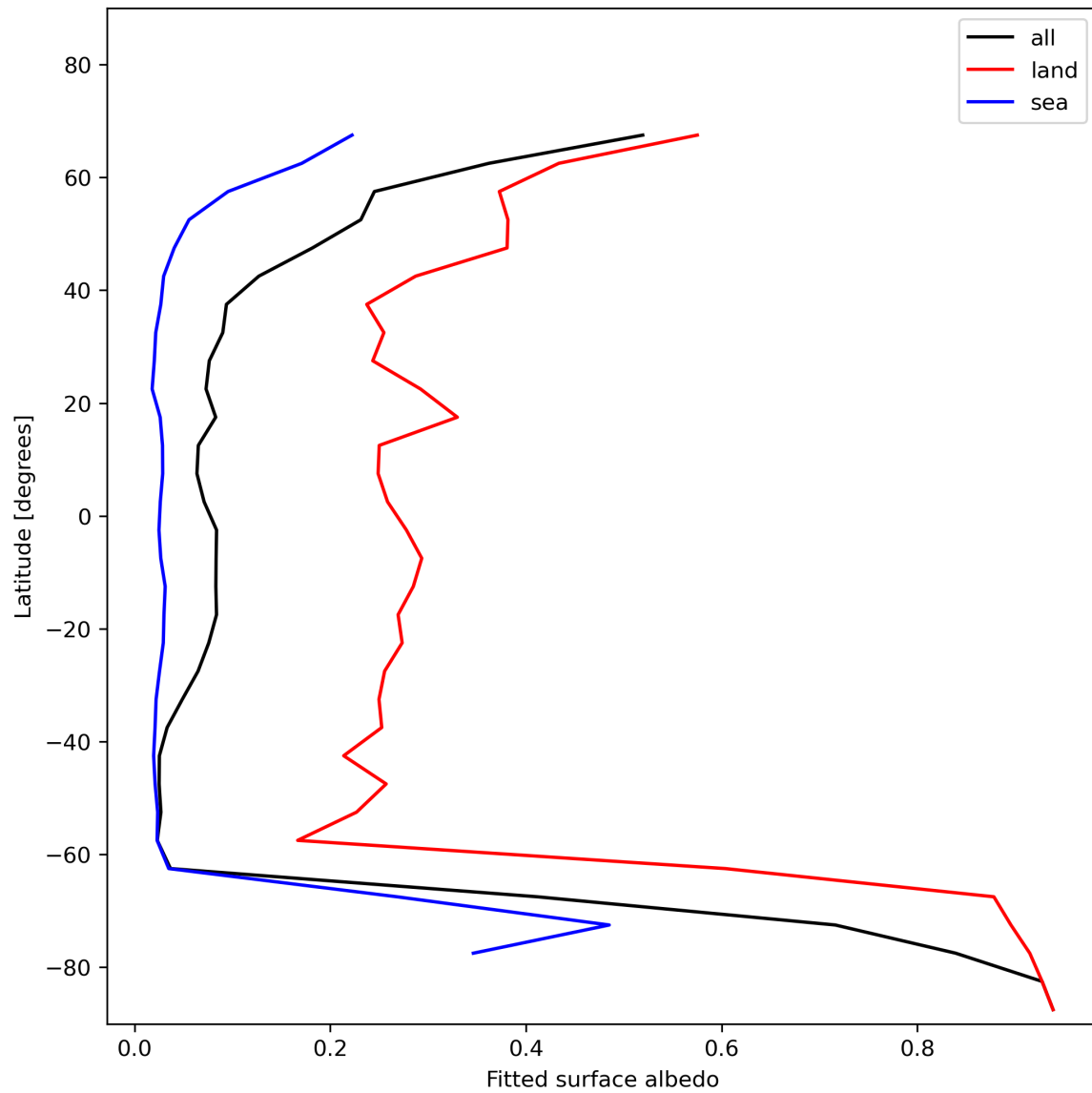
Figure 29: Zonal average of “Fitted surface albedo” for 2024-01-05 to 2024-01-07.
