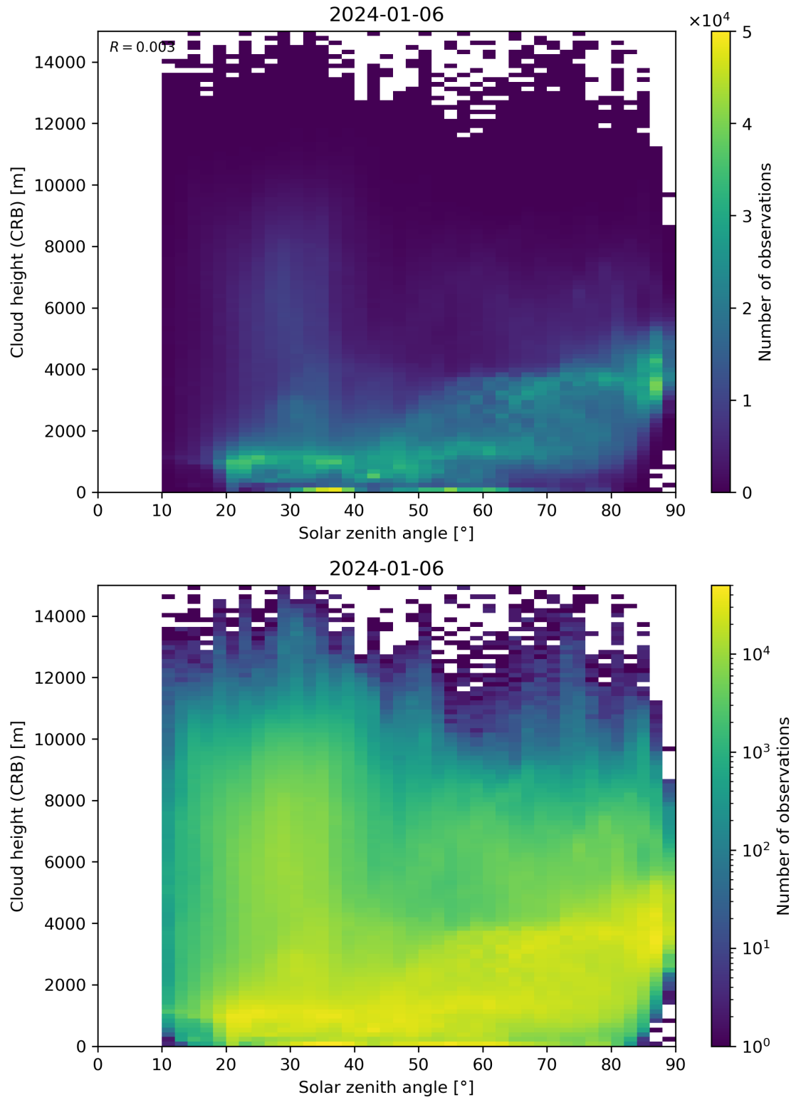
Figure 102: Scatter density plot of “Solar zenith angle” against “Cloud height (CRB)” for 2024-01-05 to 2024-01-07.
