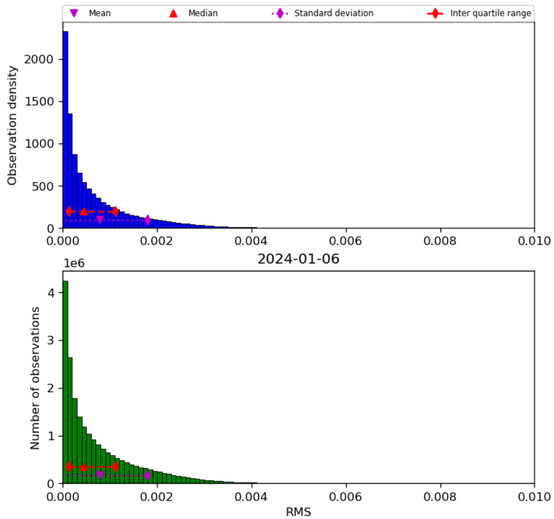
Figure 47: Histogram of “RMS” for 2024-01-05 to 2024-01-07
