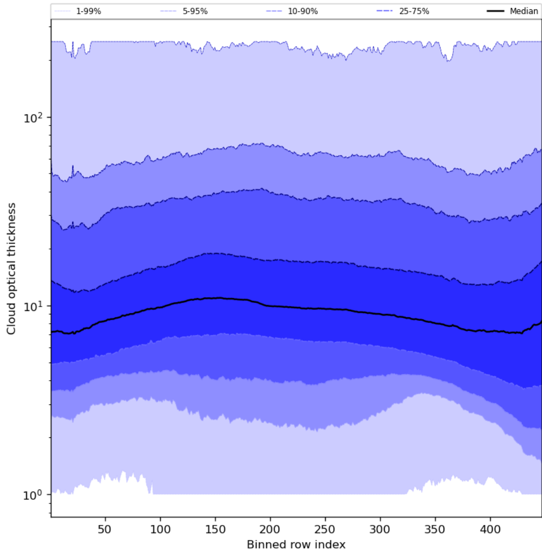
Figure 57: Along track statistics of “Cloud optical thickness” for 2024-01-05 to 2024-01-07
