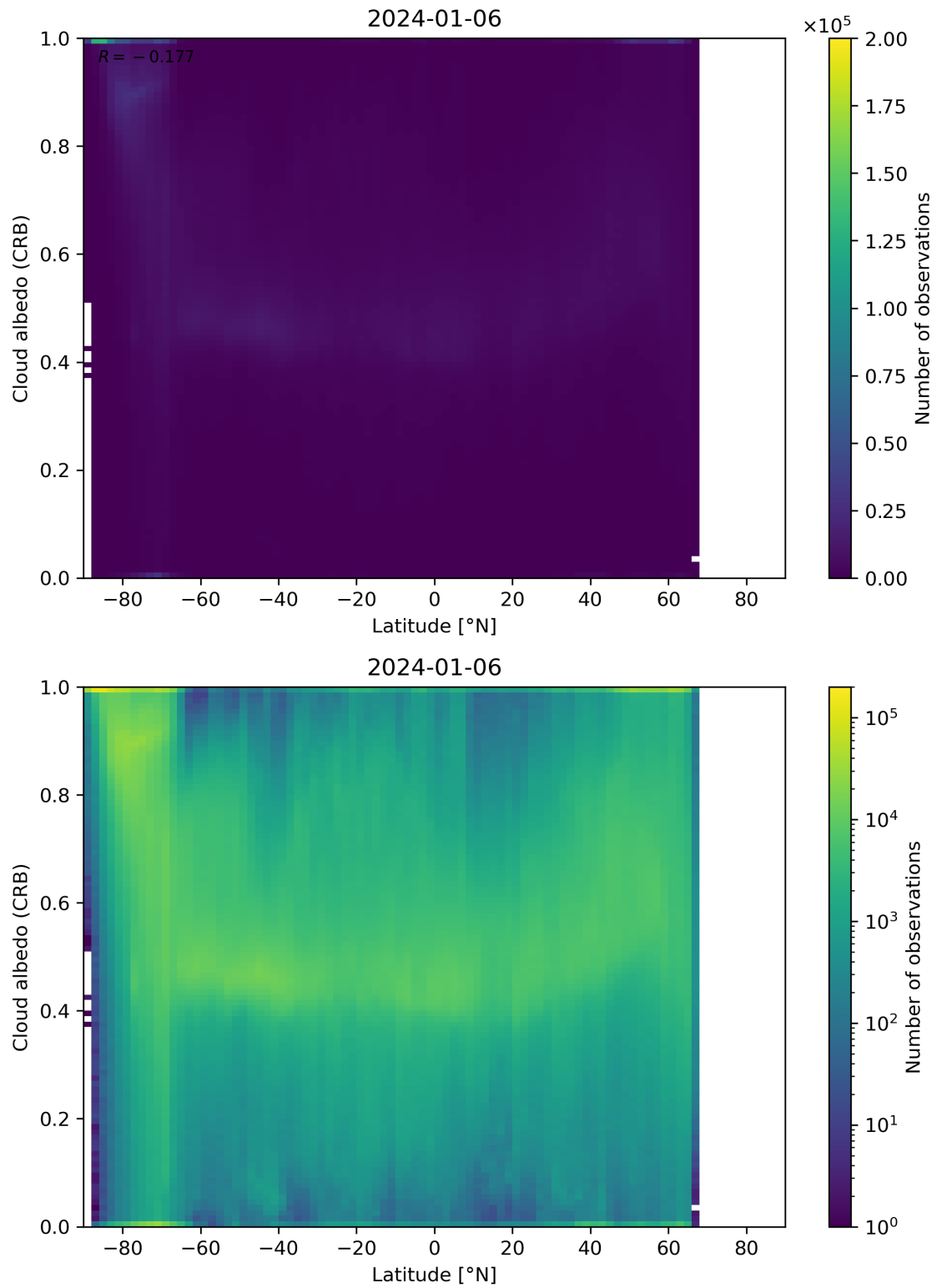
Figure 91: Scatter density plot of “Latitude” against “Cloud albedo (CRB)” for 2024-01-05 to 2024-01-07.
