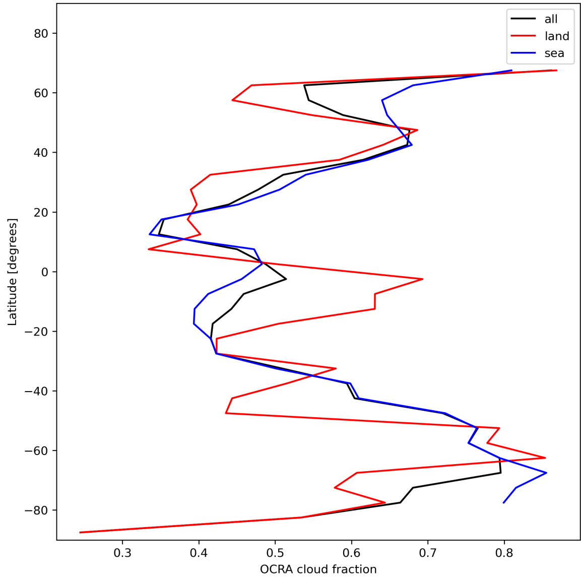
Figure 34: Zonal average of “OCRA cloud fraction” for 2024-01-05 to 2024-01-07.
