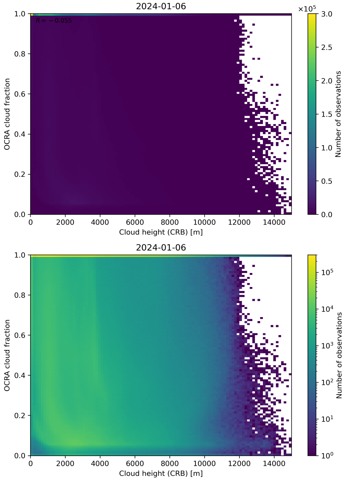
Figure 81: Scatter density plot of “Cloud height (CRB)” against “OCRA cloud fraction” for 2024-01-05 to 2024-01-07.
