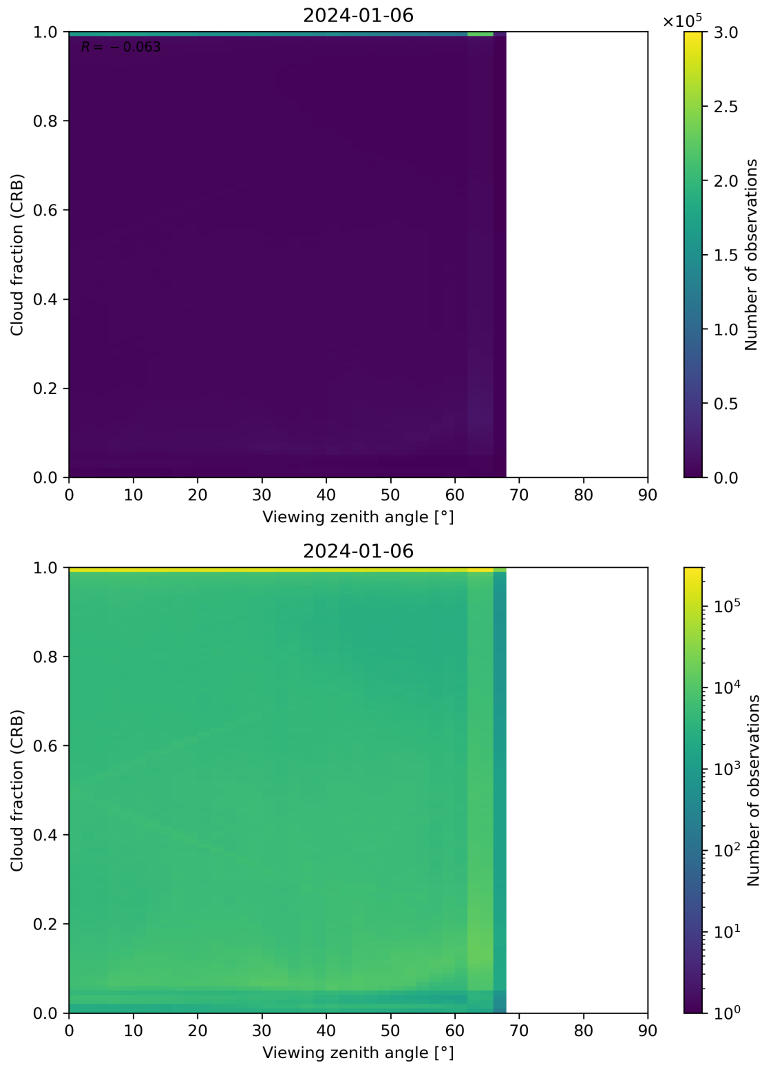
Figure 109: Scatter density plot of “Viewing zenith angle” against “Cloud fraction (CRB)” for 2024-01-05 to 2024-01-07.
