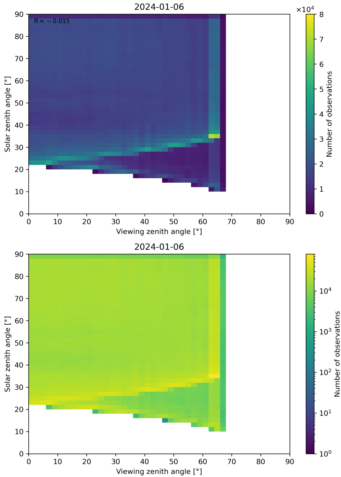
Figure 114: Scatter density plot of “Viewing zenith angle” against “Solar zenith angle” for 2024-01-05 to 2024-01-07.
