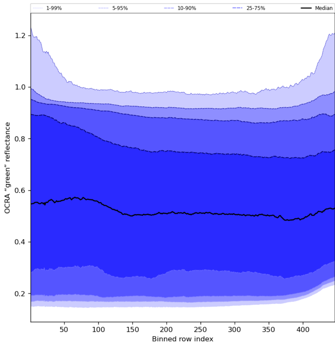
Figure 68: Along track statistics of "OCRA "green" reflectance" for 2024-01-05 to 2024-01-07
