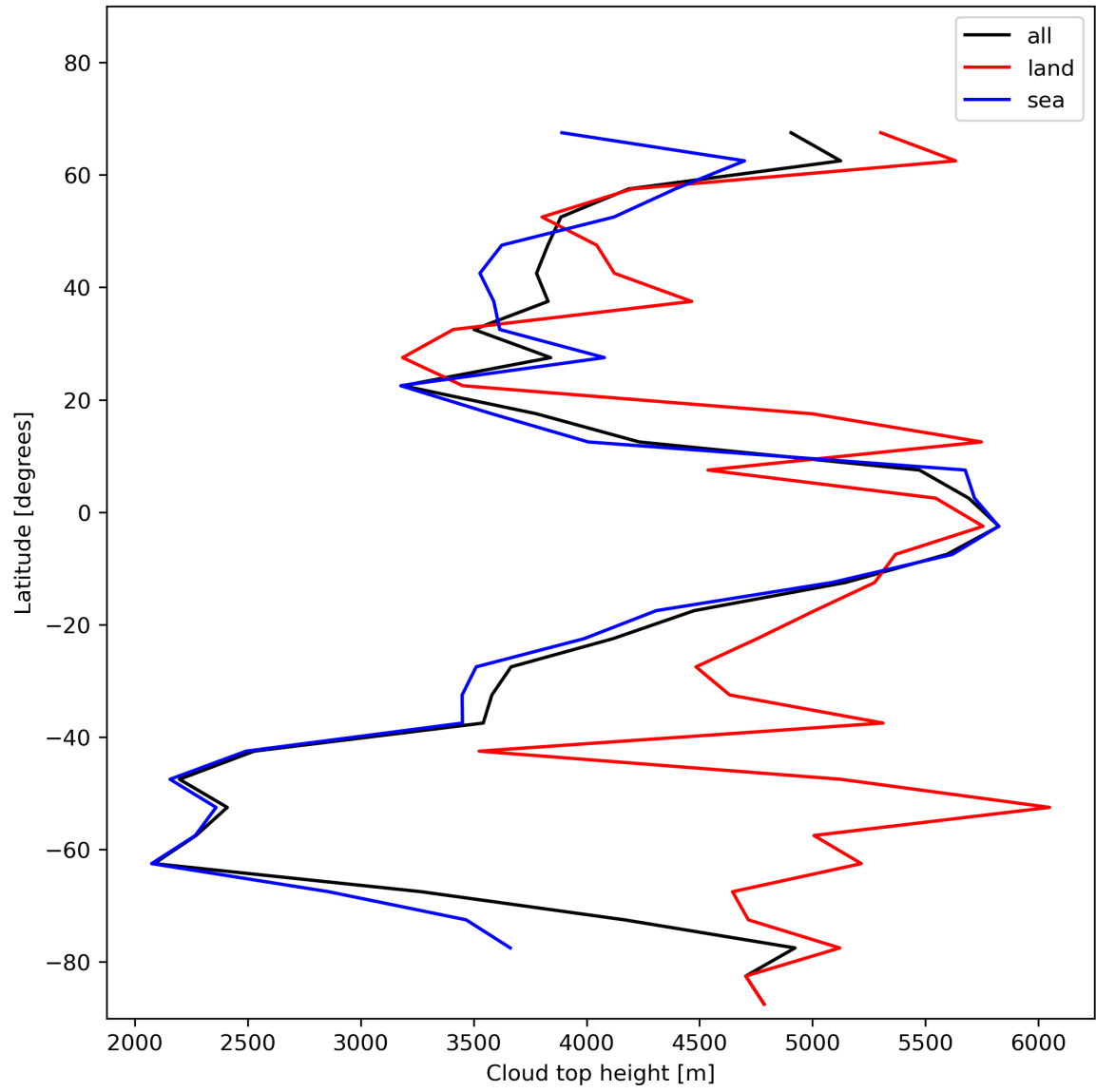
Figure 24: Zonal average of “Cloud top height” for 2024-01-05 to 2024-01-07.
