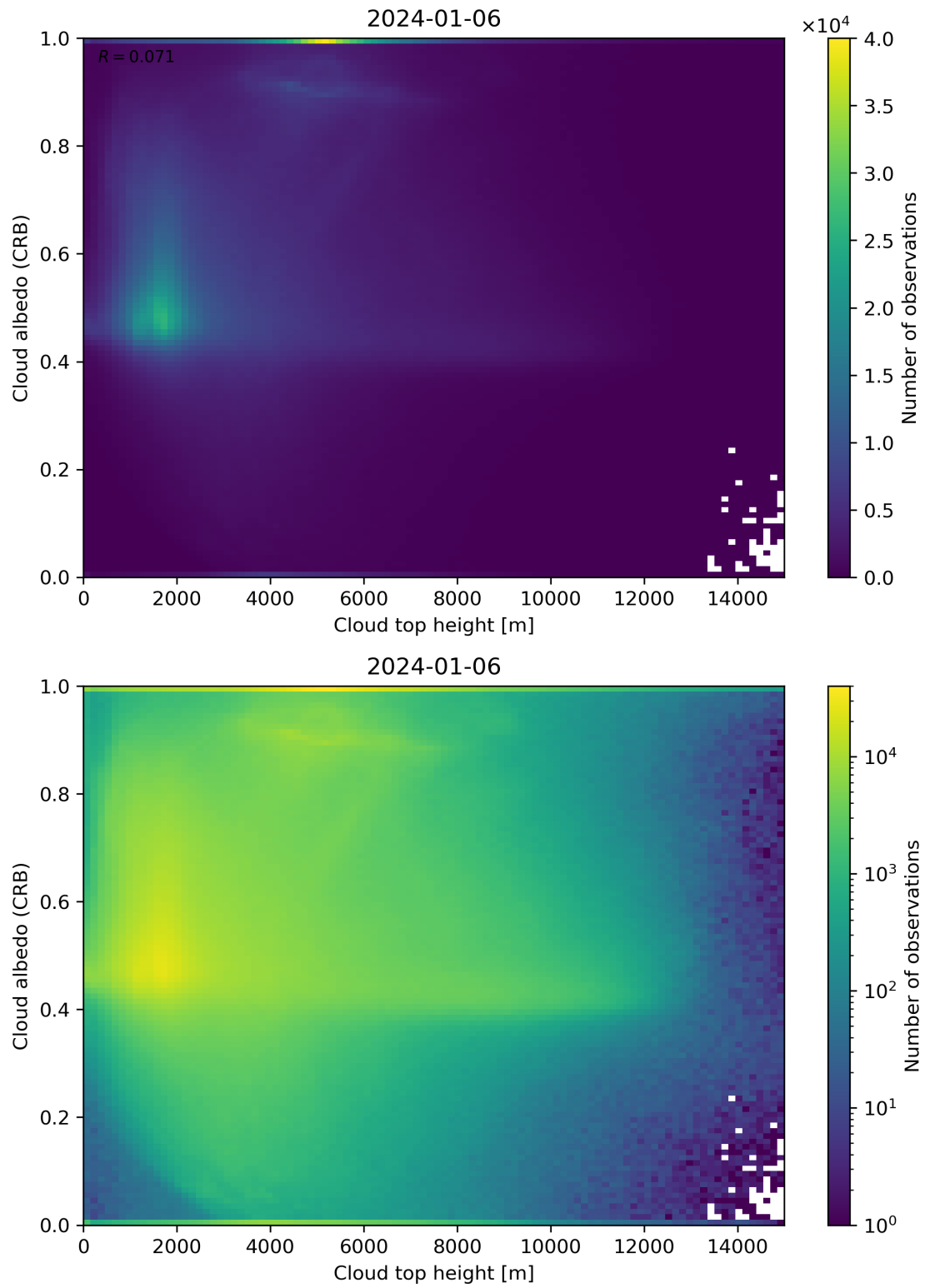
Figure 86: Scatter density plot of “Cloud top height” against “Cloud albedo (CRB)” for 2024-01-05 to 2024-01-07.
