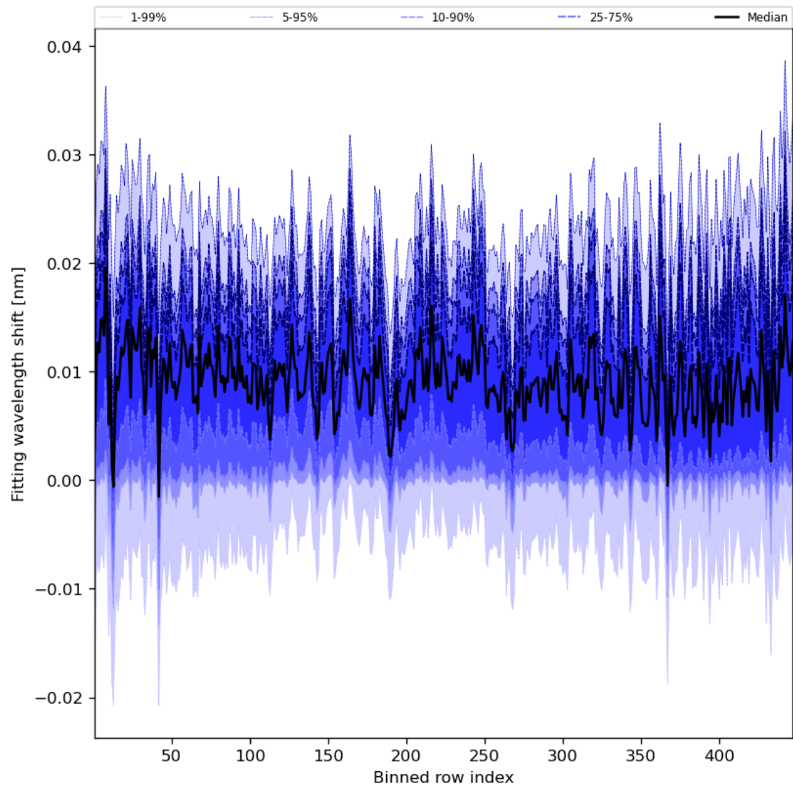
Figure 65: Along track statistics of “Fitting wavelength shift” for 2024-01-05 to 2024-01-07
