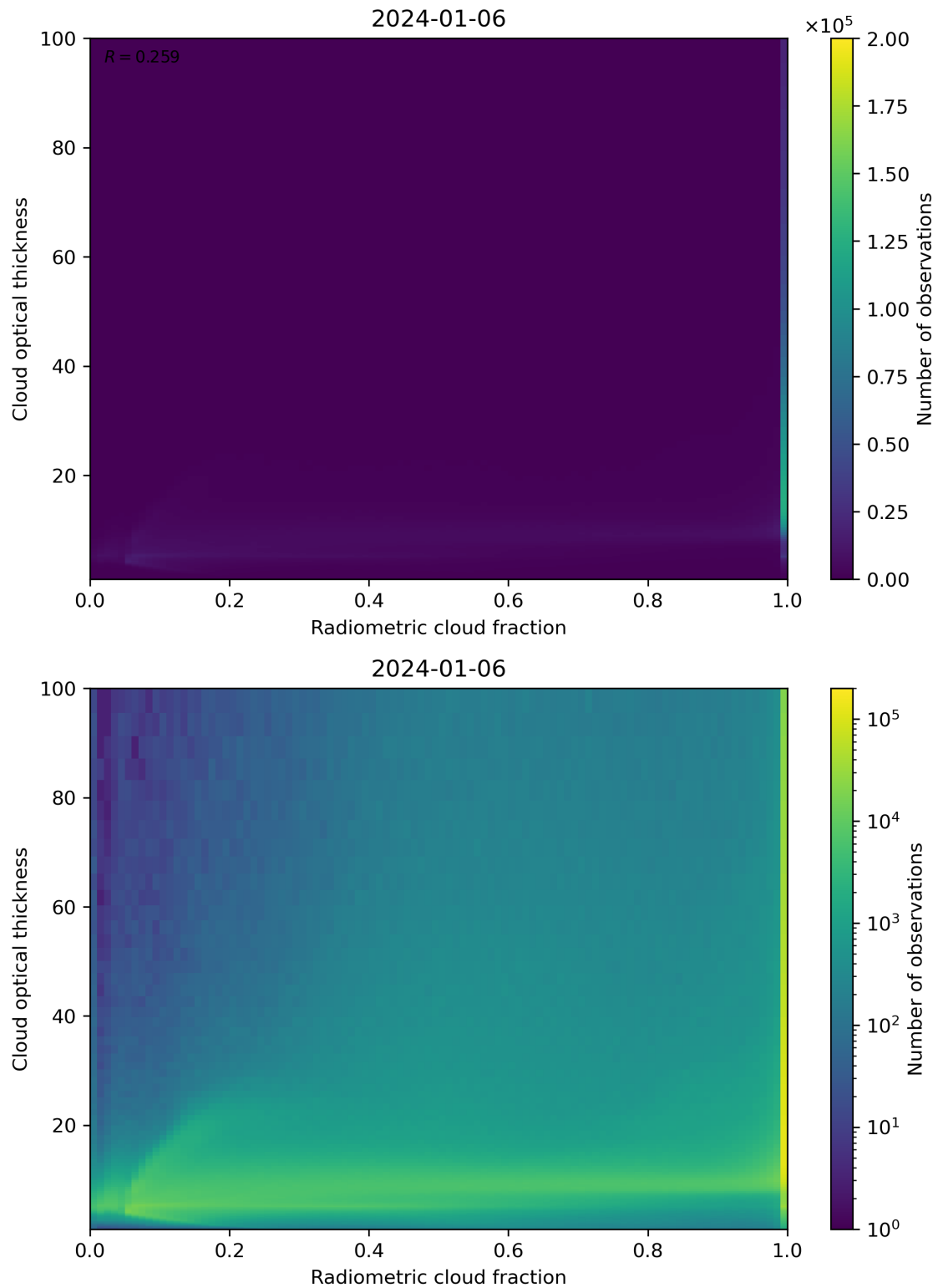
Figure 75: Scatter density plot of “Radiometric cloud fraction” against “Cloud optical thickness” for 2024-01-05 to 2024-01-07.
