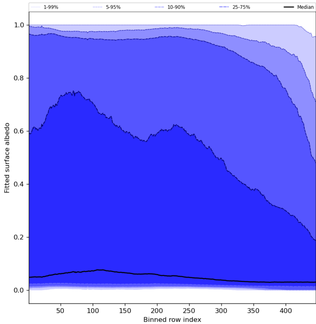
Figure 61: Along track statistics of “Fitted surface albedo” for 2024-01-05 to 2024-01-07
