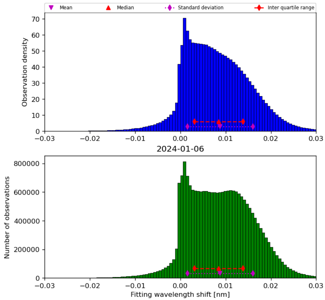
Figure 49: Histogram of “Fitting wavelength shift” for 2024-01-05 to 2024-01-07
