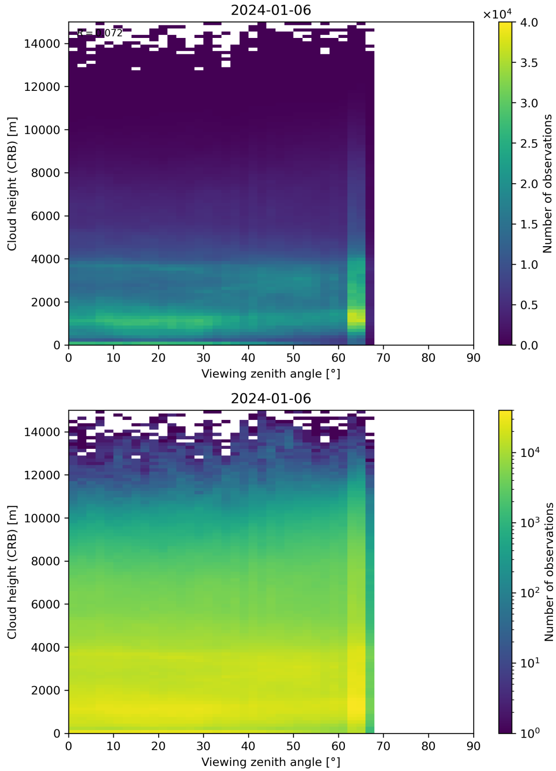
Figure 110: Scatter density plot of “Viewing zenith angle” against “Cloud height (CRB)” for 2024-01-05 to 2024-01-07.
