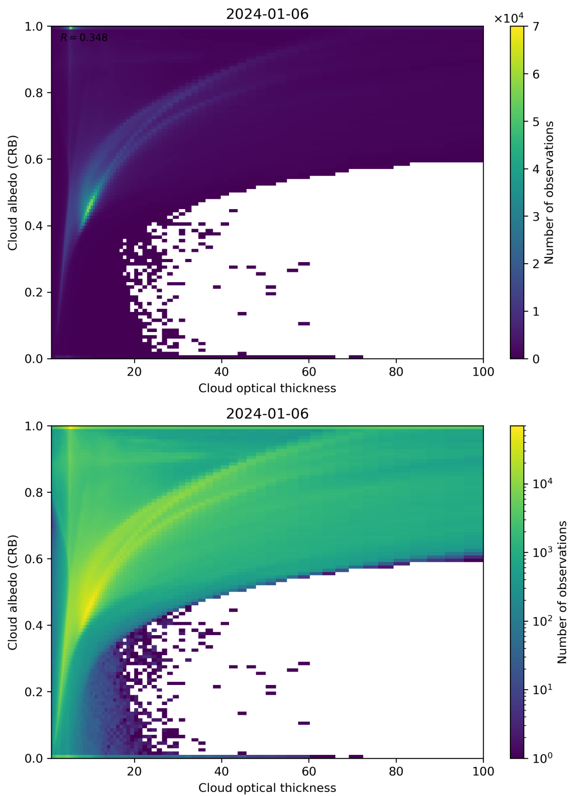
Figure 82: Scatter density plot of “Cloud optical thickness” against “Cloud albedo (CRB)” for 2024-01-05 to 2024-01-07.
