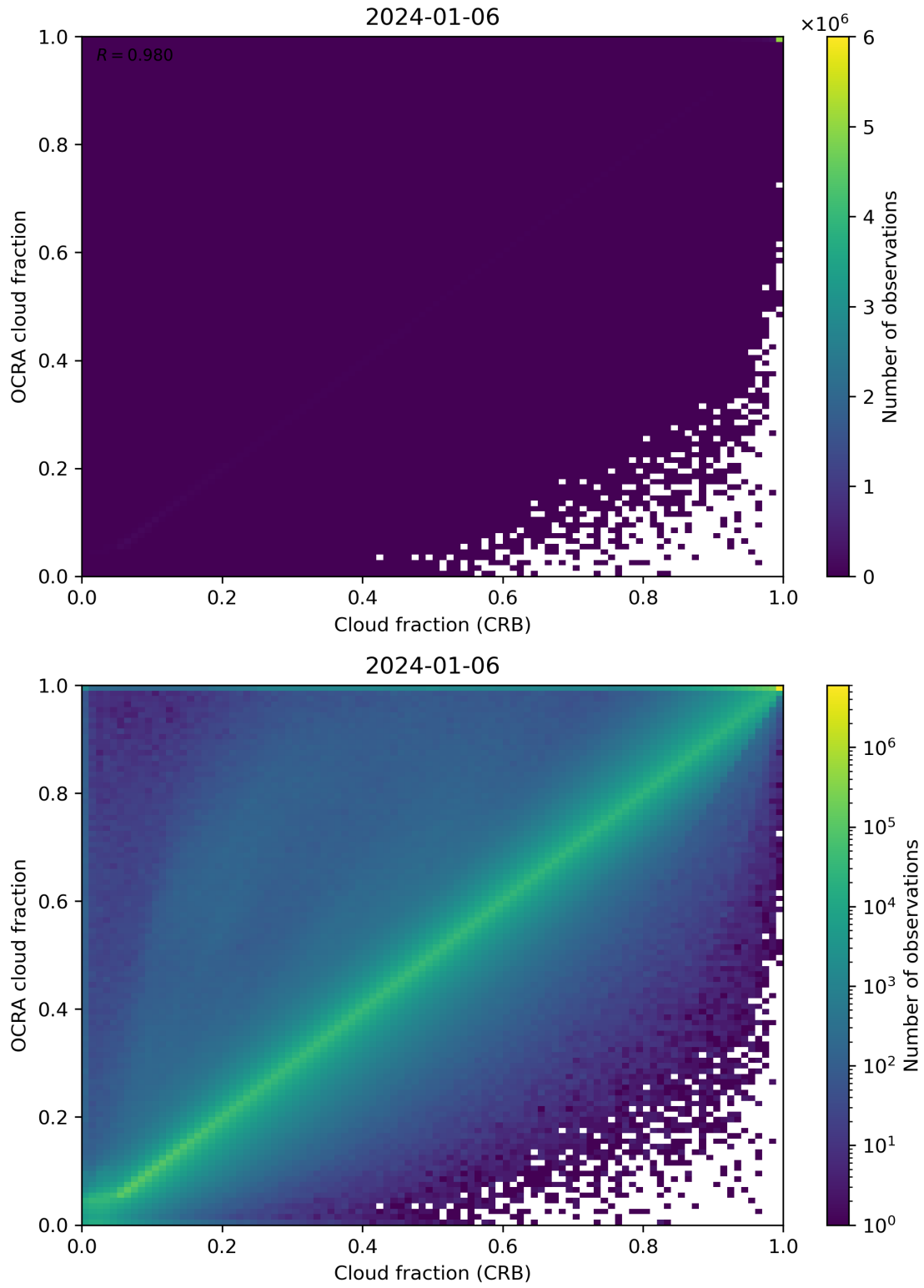
Figure 78: Scatter density plot of “Cloud fraction (CRB)” against “OCRA cloud fraction” for 2024-01-05 to 2024-01-07.
