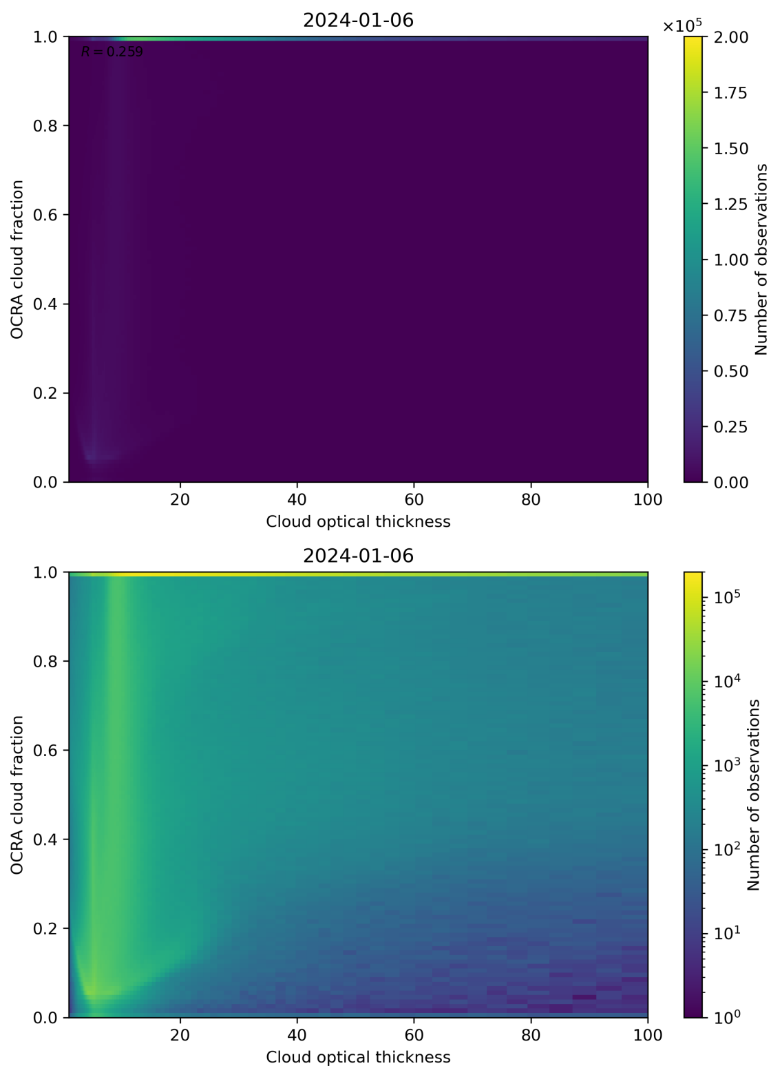
Figure 83: Scatter density plot of “Cloud optical thickness” against “OCRA cloud fraction” for 2024-01-05 to 2024-01-07.
