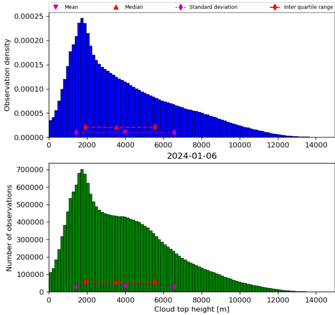
Figure 40: Histogram of “Cloud top height” for 2024-01-05 to 2024-01-07
