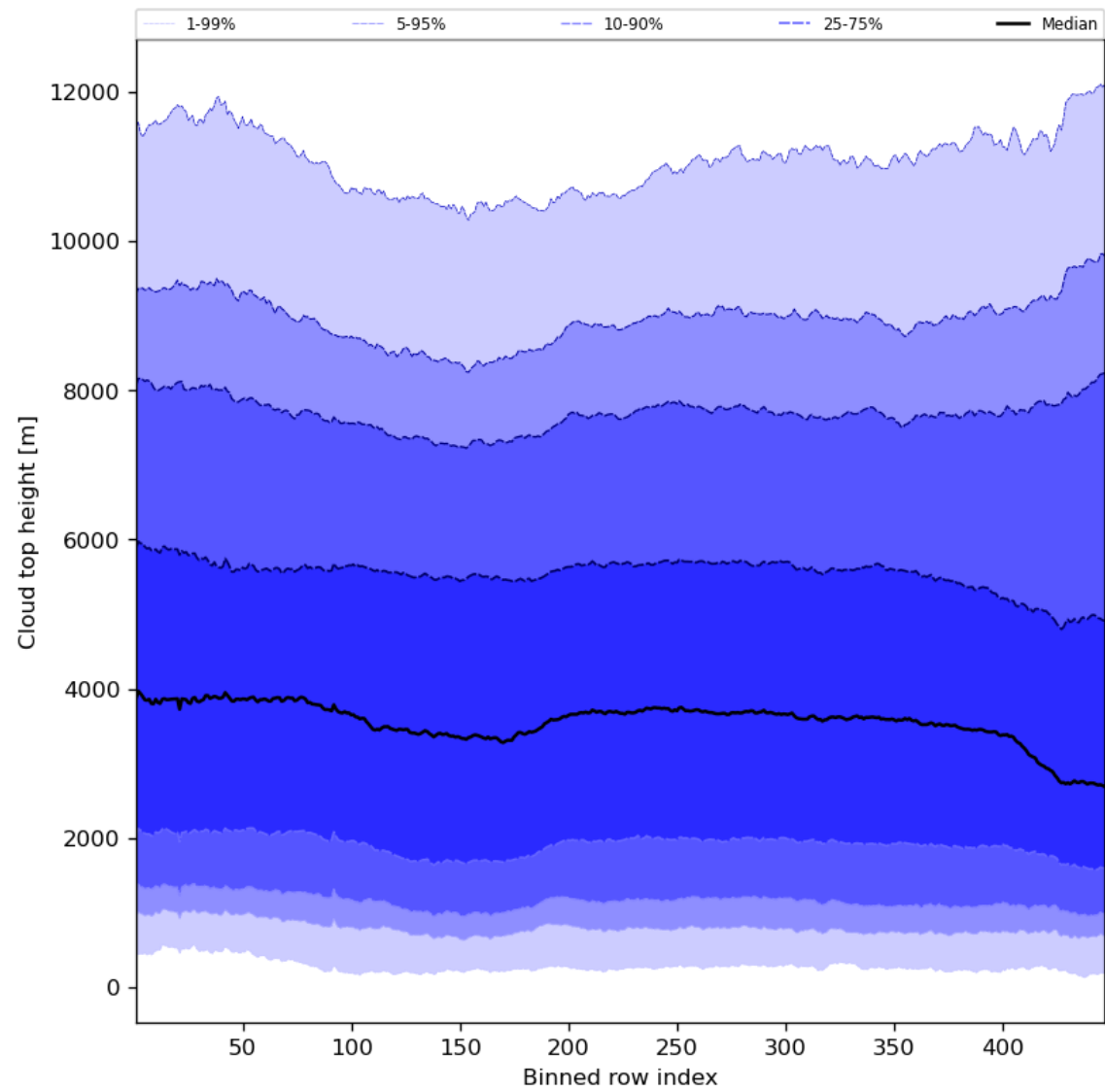
Figure 56: Along track statistics of “Cloud top height” for 2024-01-05 to 2024-01-07
