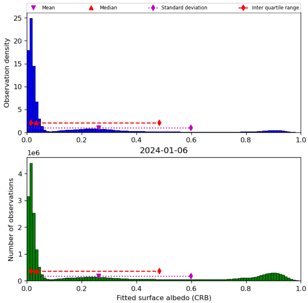
Figure 46: Histogram of “Fitted surface albedo (CRB)” for 2024-01-05 to 2024-01-07
