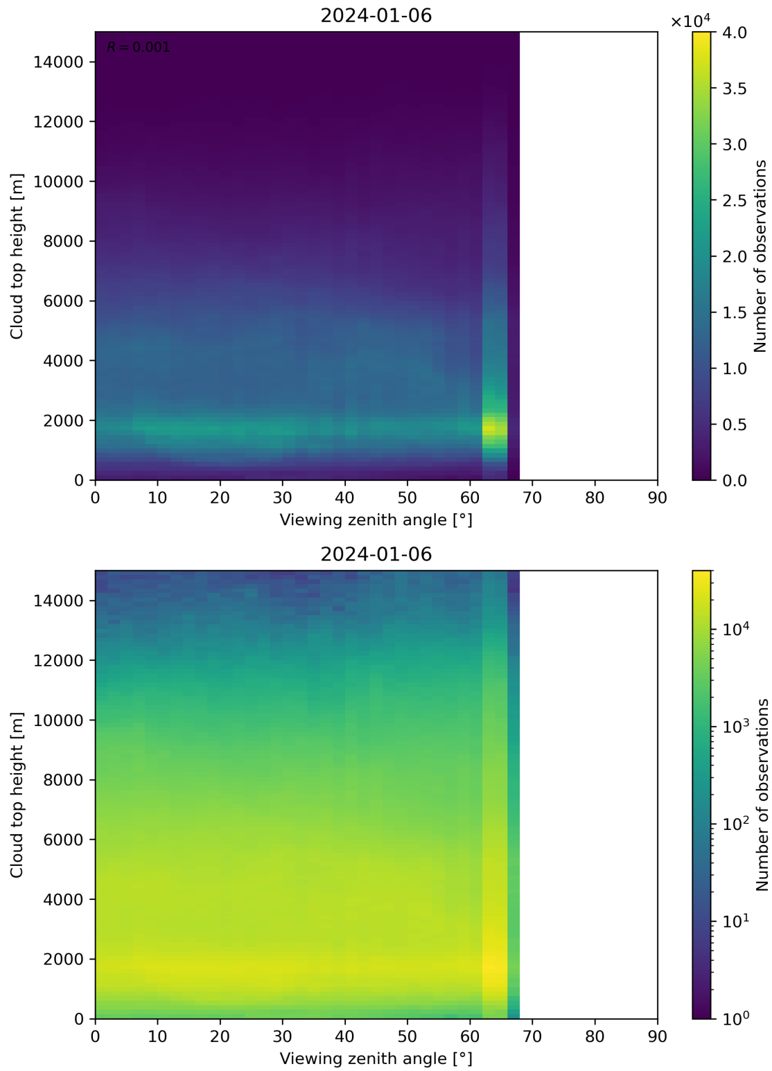
Figure 112: Scatter density plot of “Viewing zenith angle” against “Cloud top height” for 2024-01-05 to 2024-01-07.
