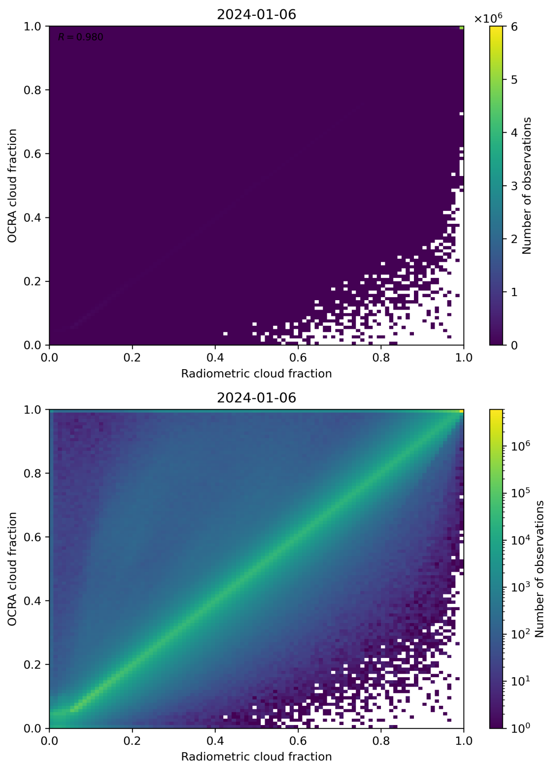
Figure 72: Scatter density plot of “Radiometric cloud fraction” against “OCRA cloud fraction” for 2024-01-05 to 2024-01-07.
