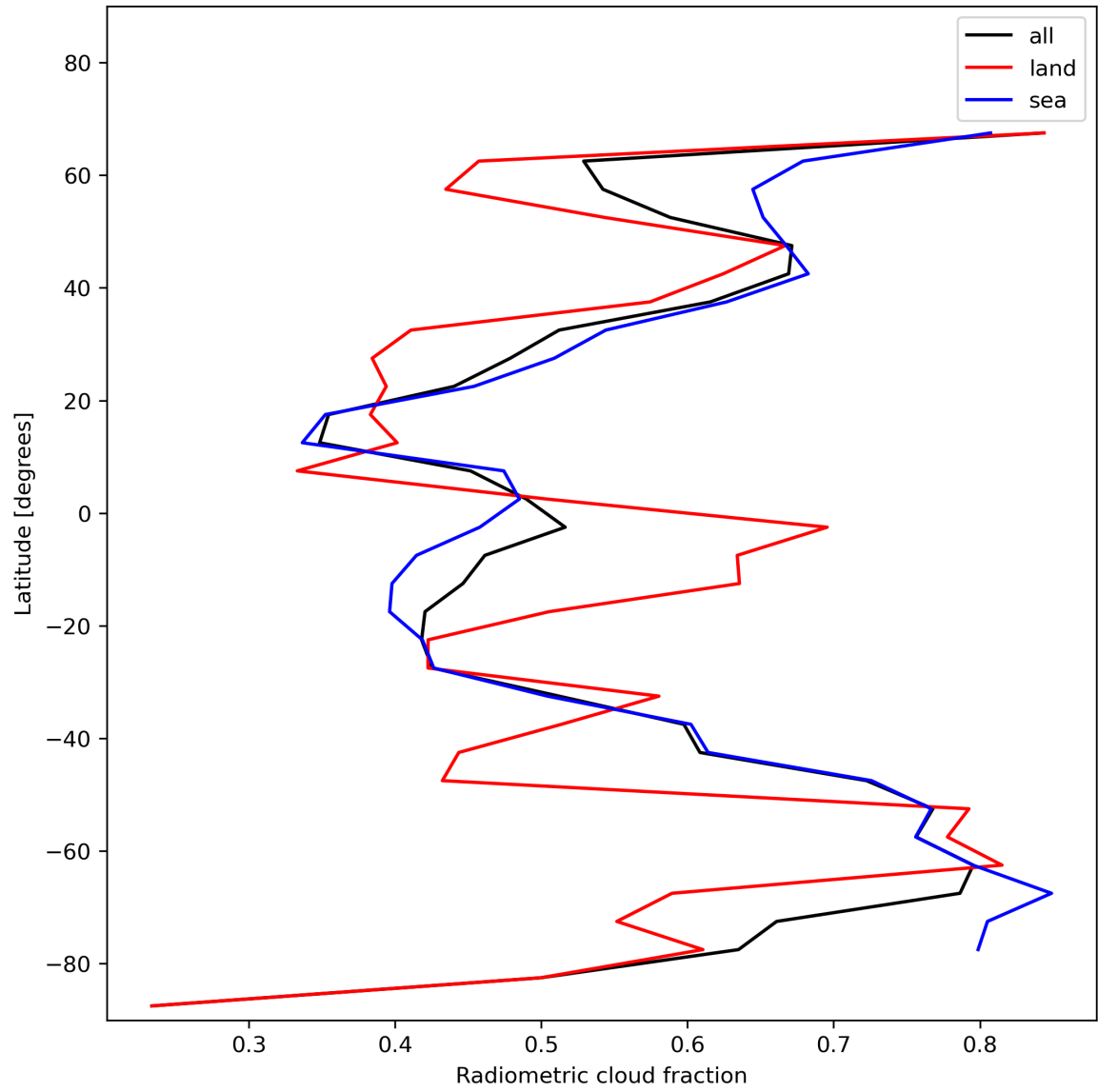
Figure 23: Zonal average of “Radiometric cloud fraction” for 2024-01-05 to 2024-01-07.
