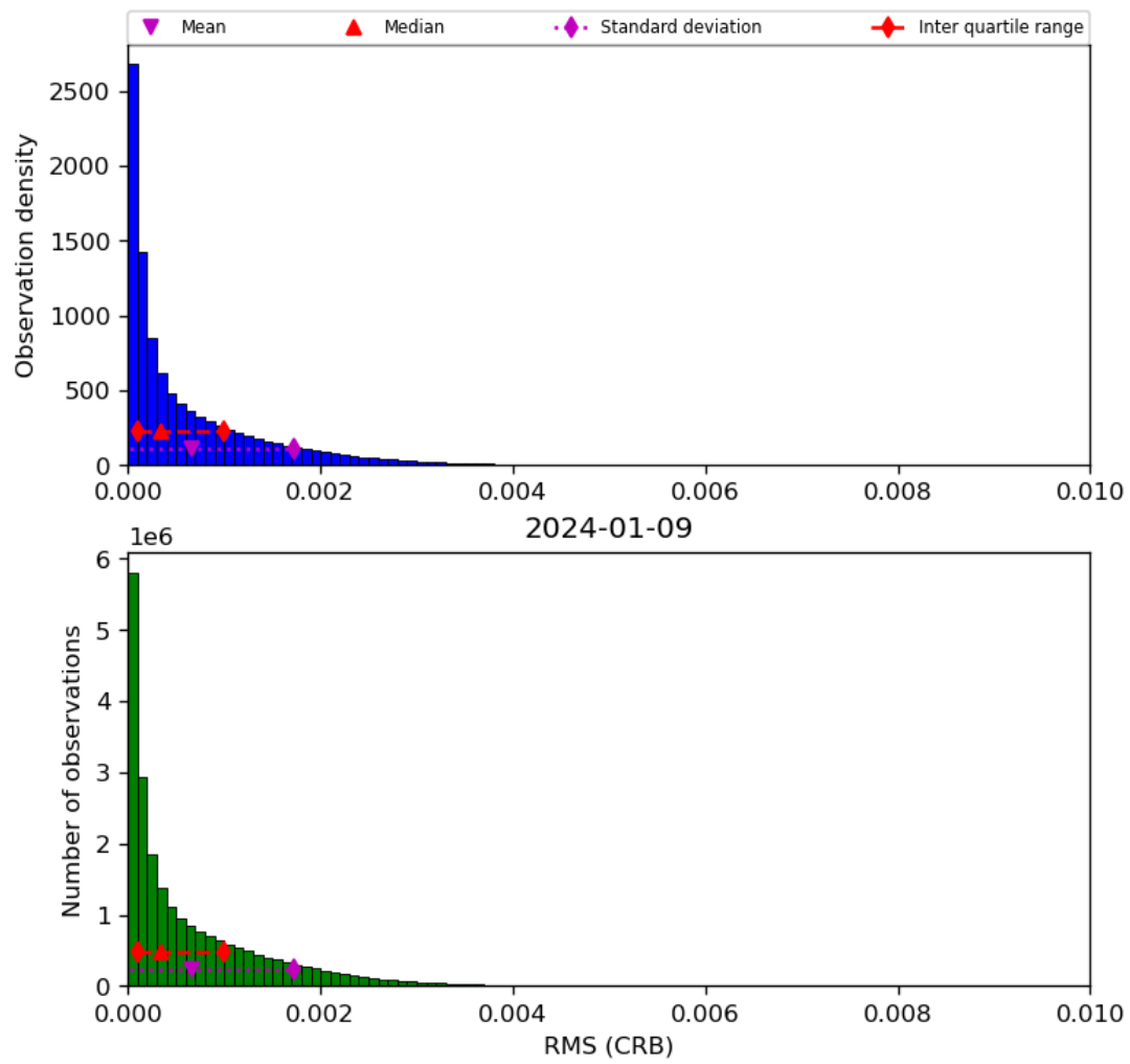
Figure 48: Histogram of “RMS (CRB)” for 2024-01-08 to 2024-01-10
