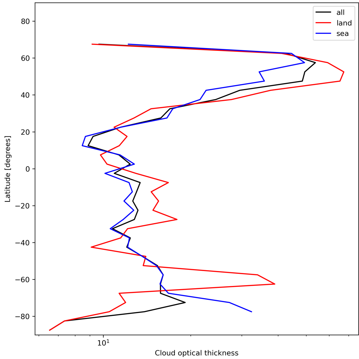
Figure 25: Zonal average of “Cloud optical thickness” for 2024-01-08 to 2024-01-10.
