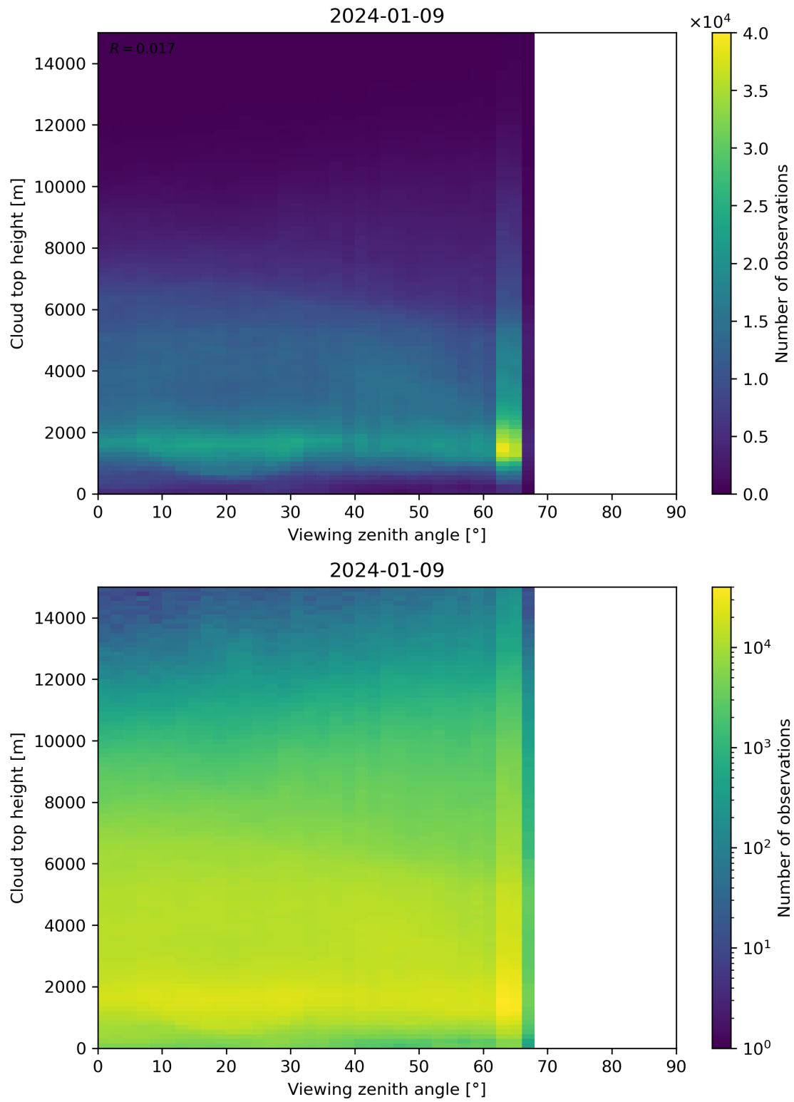
Figure 112: Scatter density plot of “Viewing zenith angle” against “Cloud top height” for 2024-01-08 to 2024-01-10.
