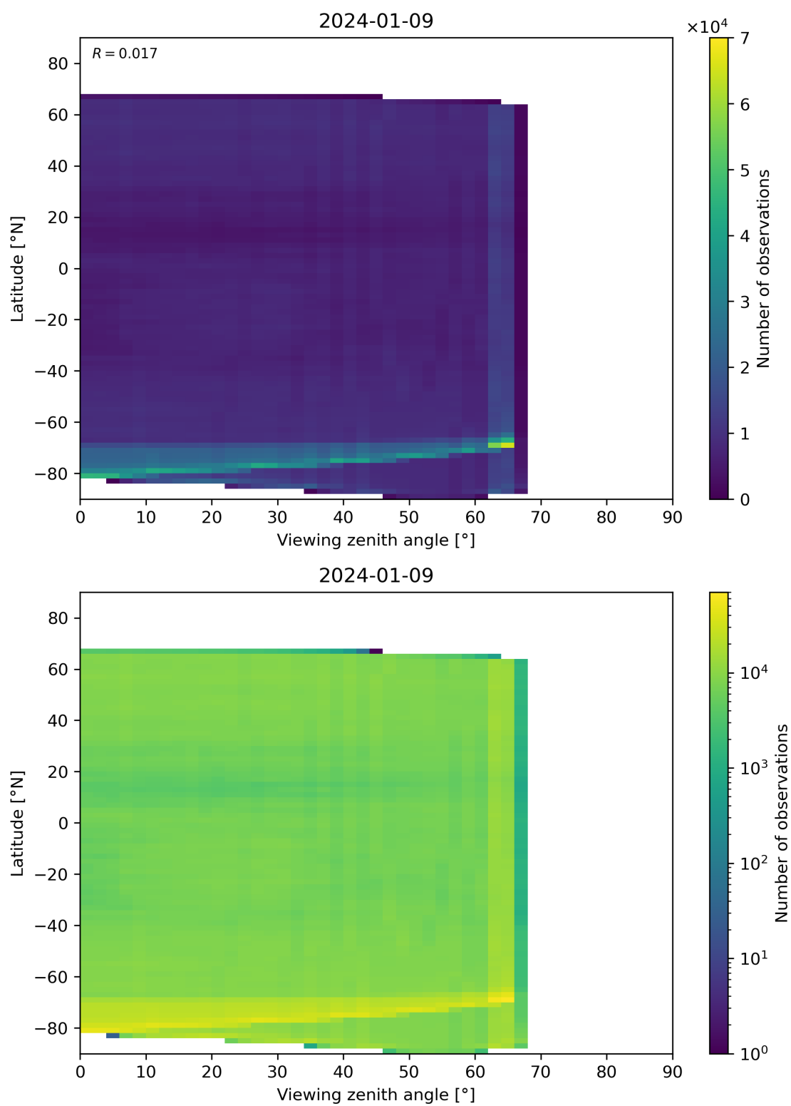
Figure 113: Scatter density plot of “Viewing zenith angle” against “Latitude” for 2024-01-08 to 2024-01-10.
