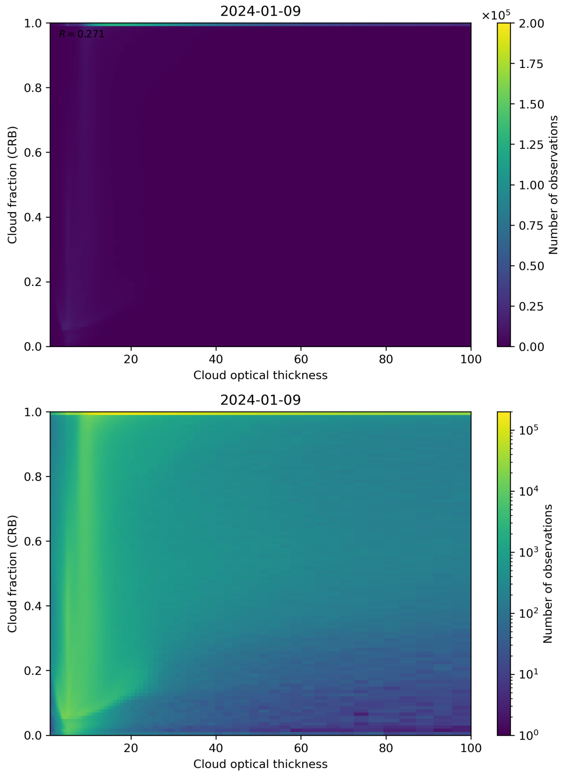
Figure 84: Scatter density plot of “Cloud optical thickness” against “Cloud fraction (CRB)” for 2024-01-08 to 2024-01-10.
