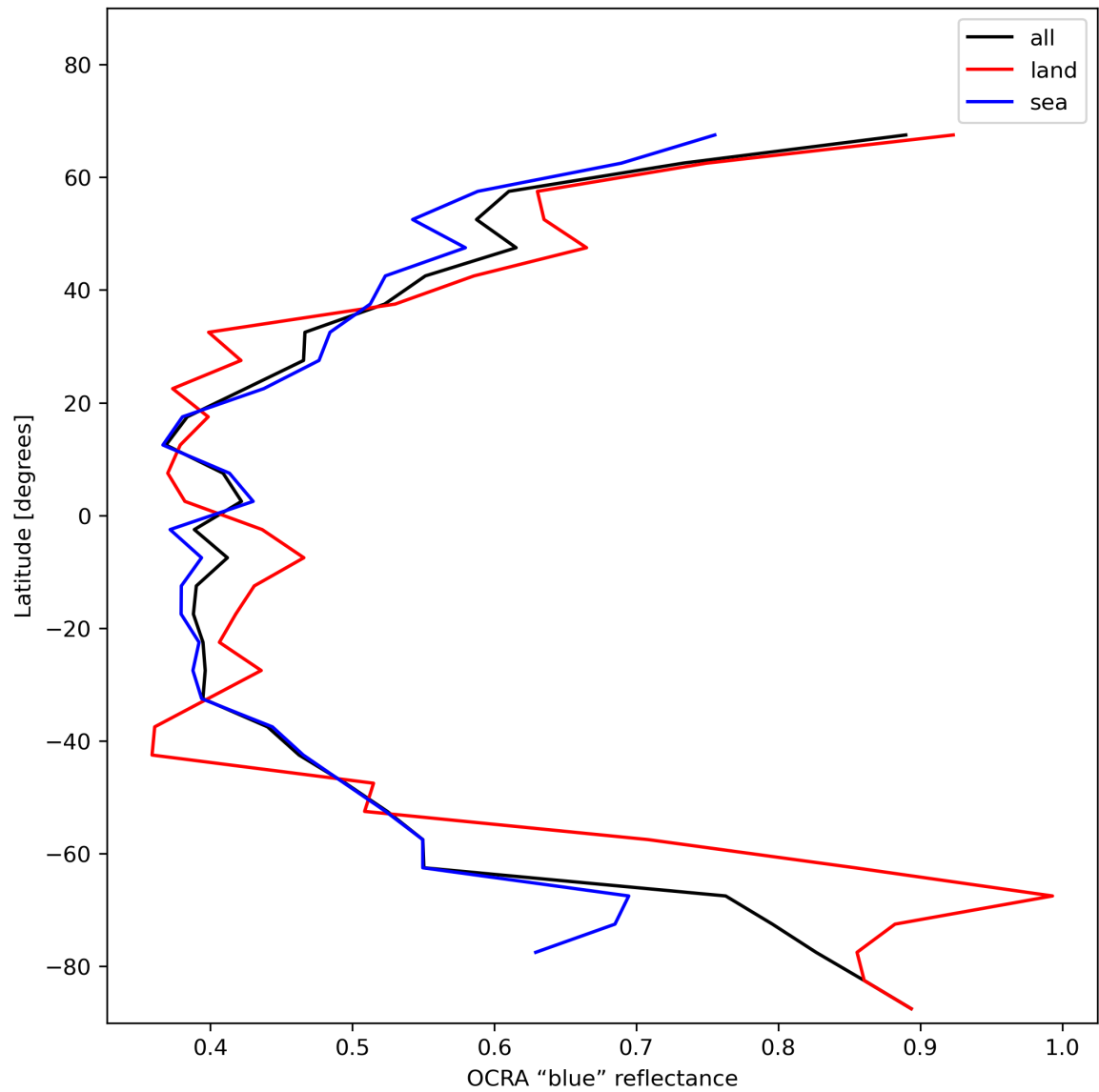
Figure 35: Zonal average of “OCRA “blue” reflectance” for 2024-01-08 to 2024-01-10.
