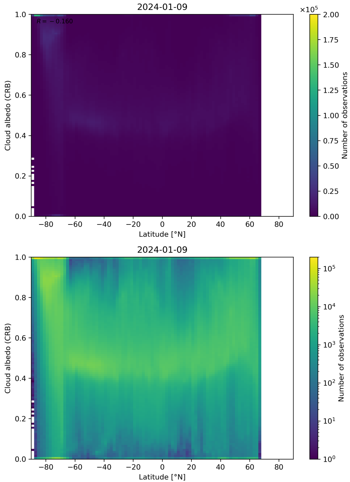
Figure 91: Scatter density plot of “Latitude” against “Cloud albedo (CRB)” for 2024-01-08 to 2024-01-10.
