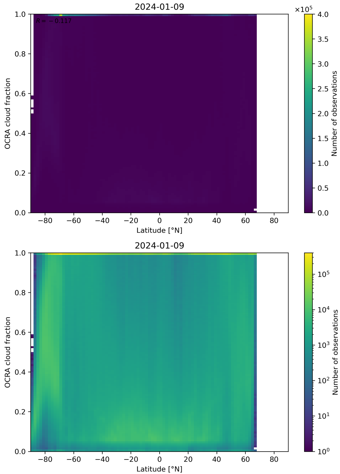
Figure 93: Scatter density plot of “Latitude” against “OCRA cloud fraction” for 2024-01-08 to 2024-01-10.
