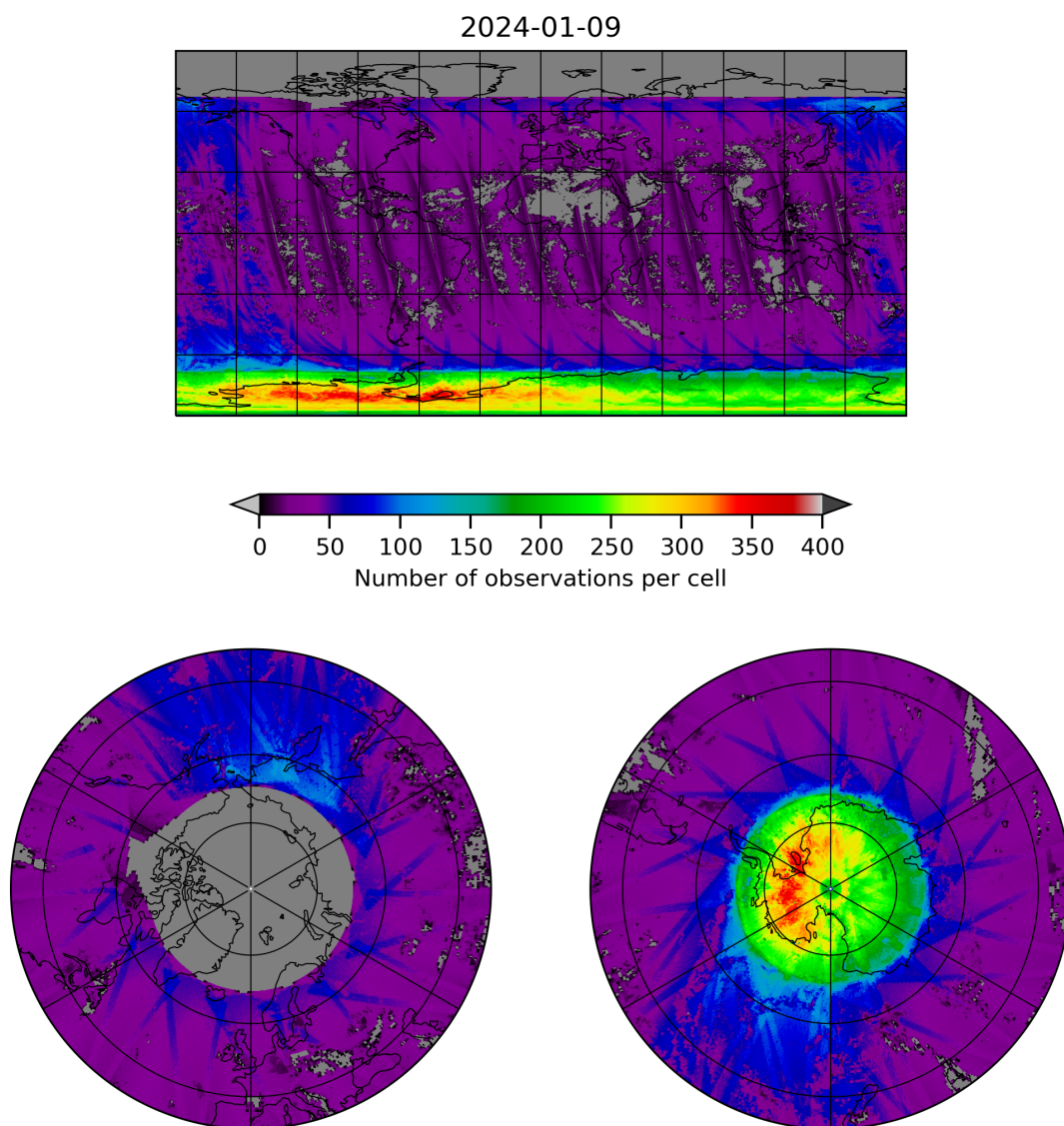
Figure 21: Map of the number of observations for 2024-01-08 to 2024-01-10
