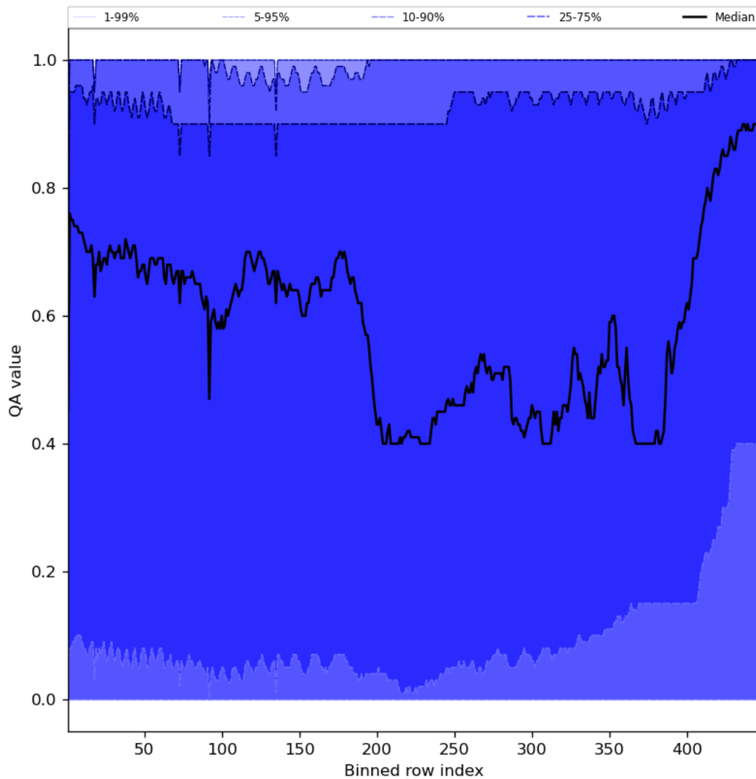
Figure 54: Along track statistics of “QA value” for 2024-01-08 to 2024-01-10
