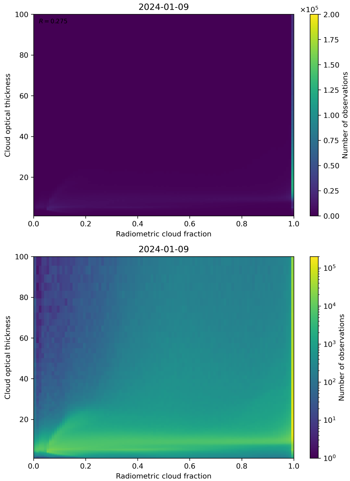
Figure 75: Scatter density plot of “Radiometric cloud fraction” against “Cloud optical thickness” for 2024-01-08 to 2024-01-10.
