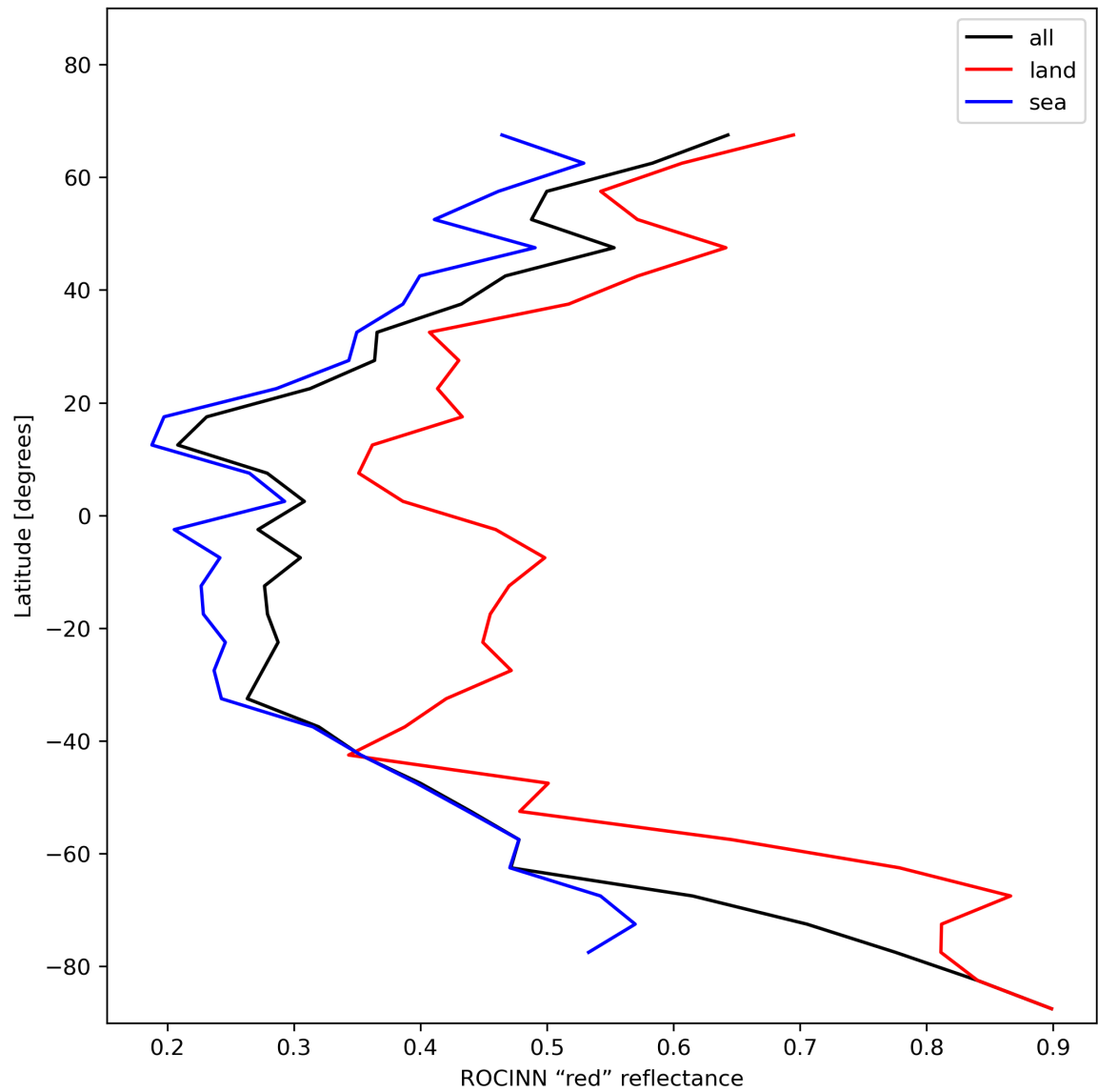
Figure 37: Zonal average of “ROCINN “red” reflectance” for 2024-01-08 to 2024-01-10.
