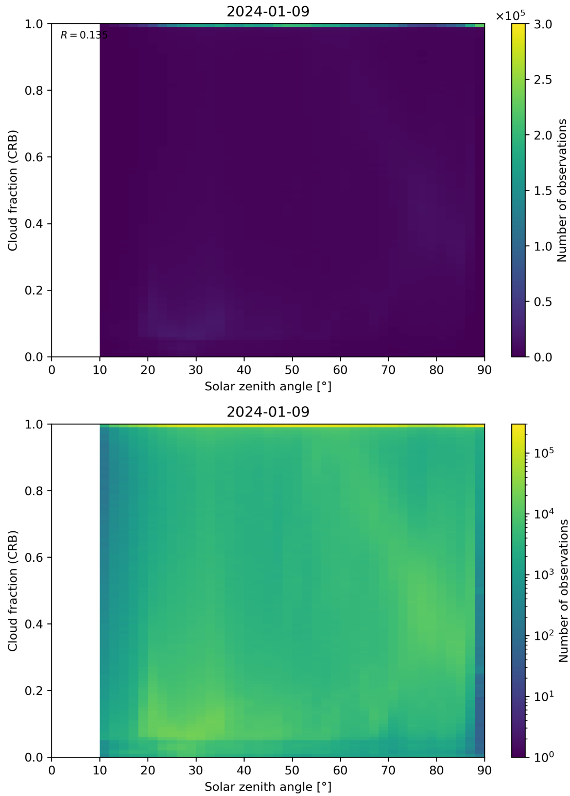
Figure 101: Scatter density plot of “Solar zenith angle” against “Cloud fraction (CRB)” for 2024-01-08 to 2024-01-10.
