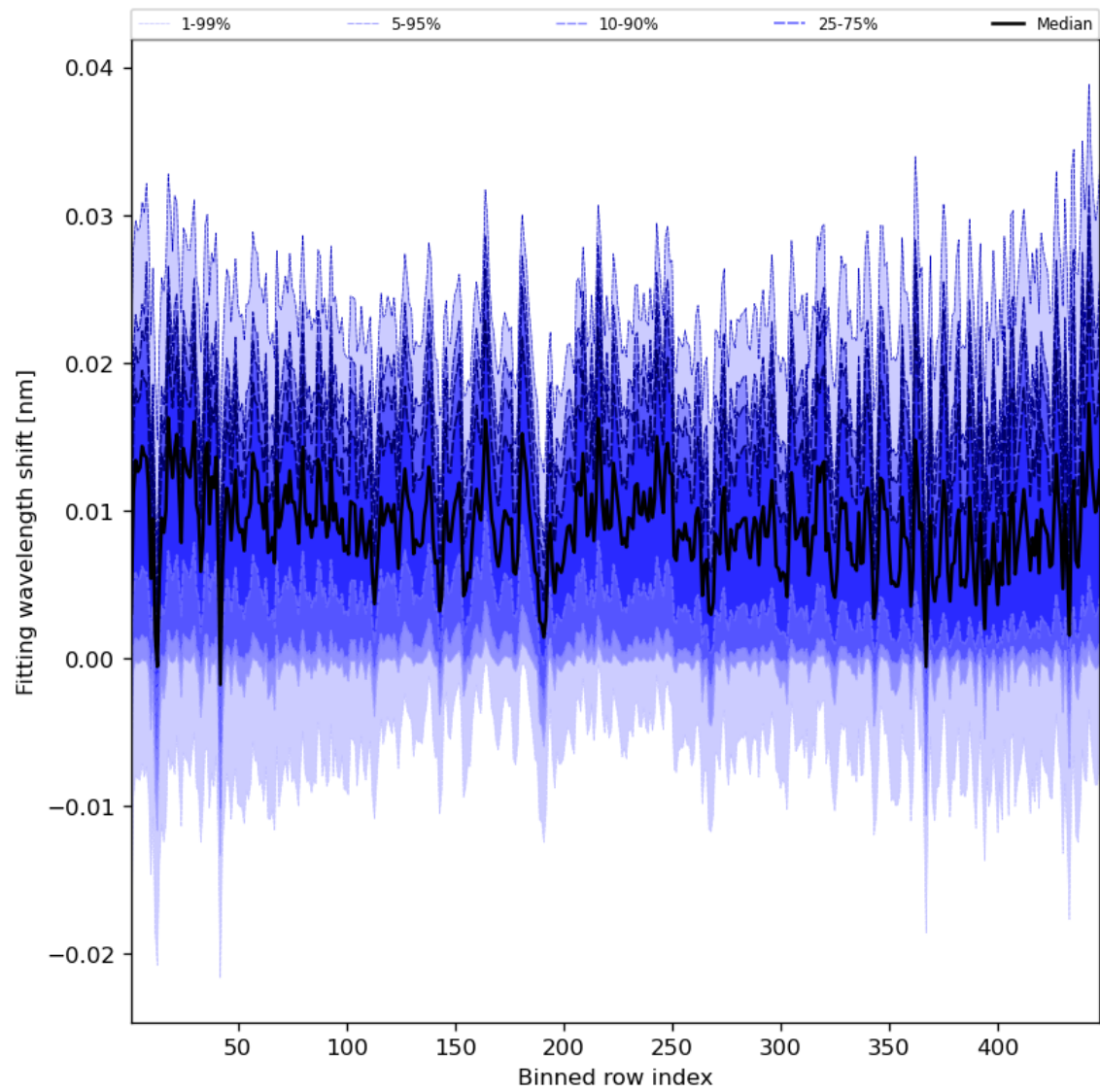
Figure 65: Along track statistics of “Fitting wavelength shift” for 2024-01-08 to 2024-01-10
