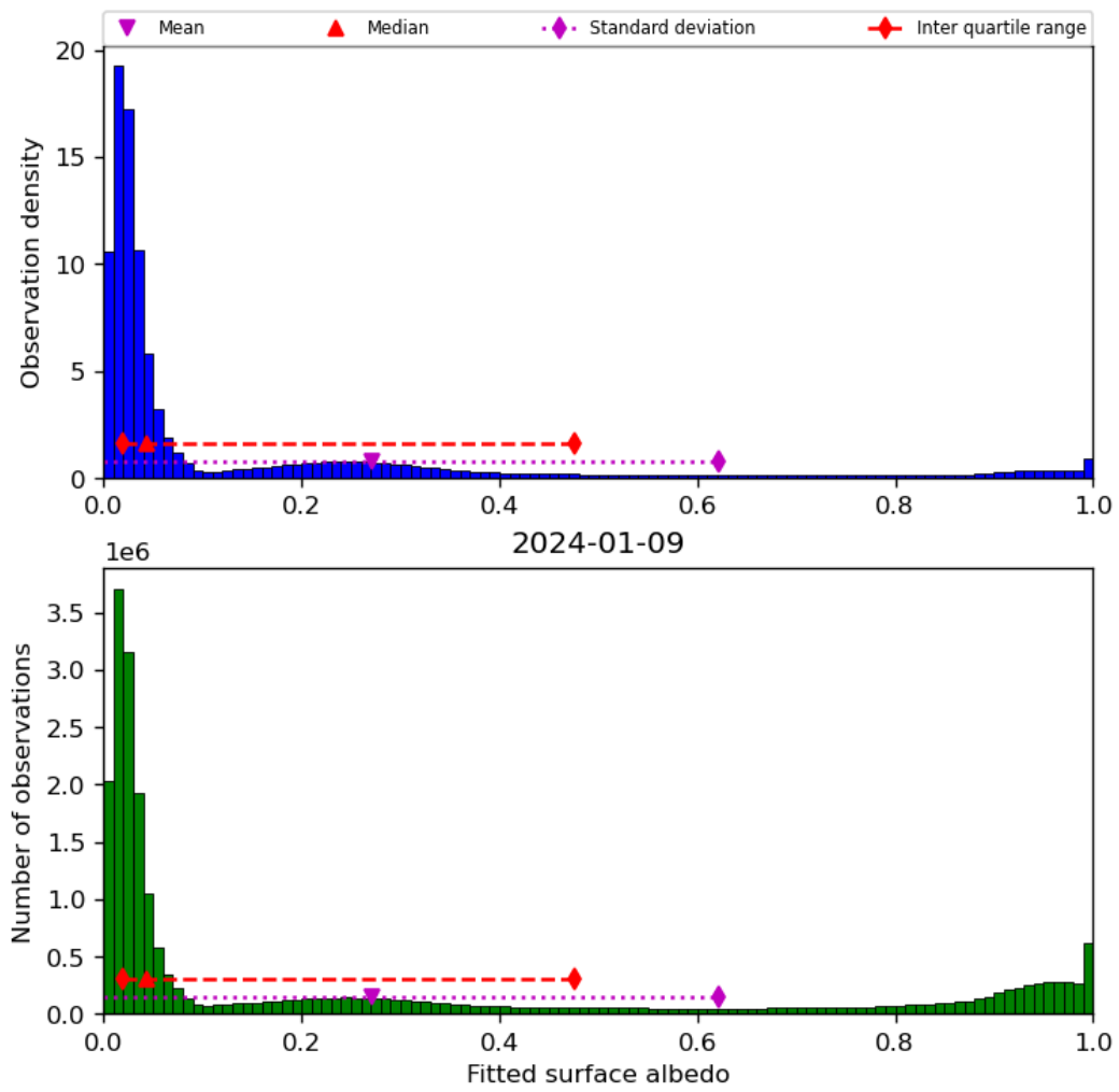
Figure 45: Histogram of “Fitted surface albedo” for 2024-01-08 to 2024-01-10
