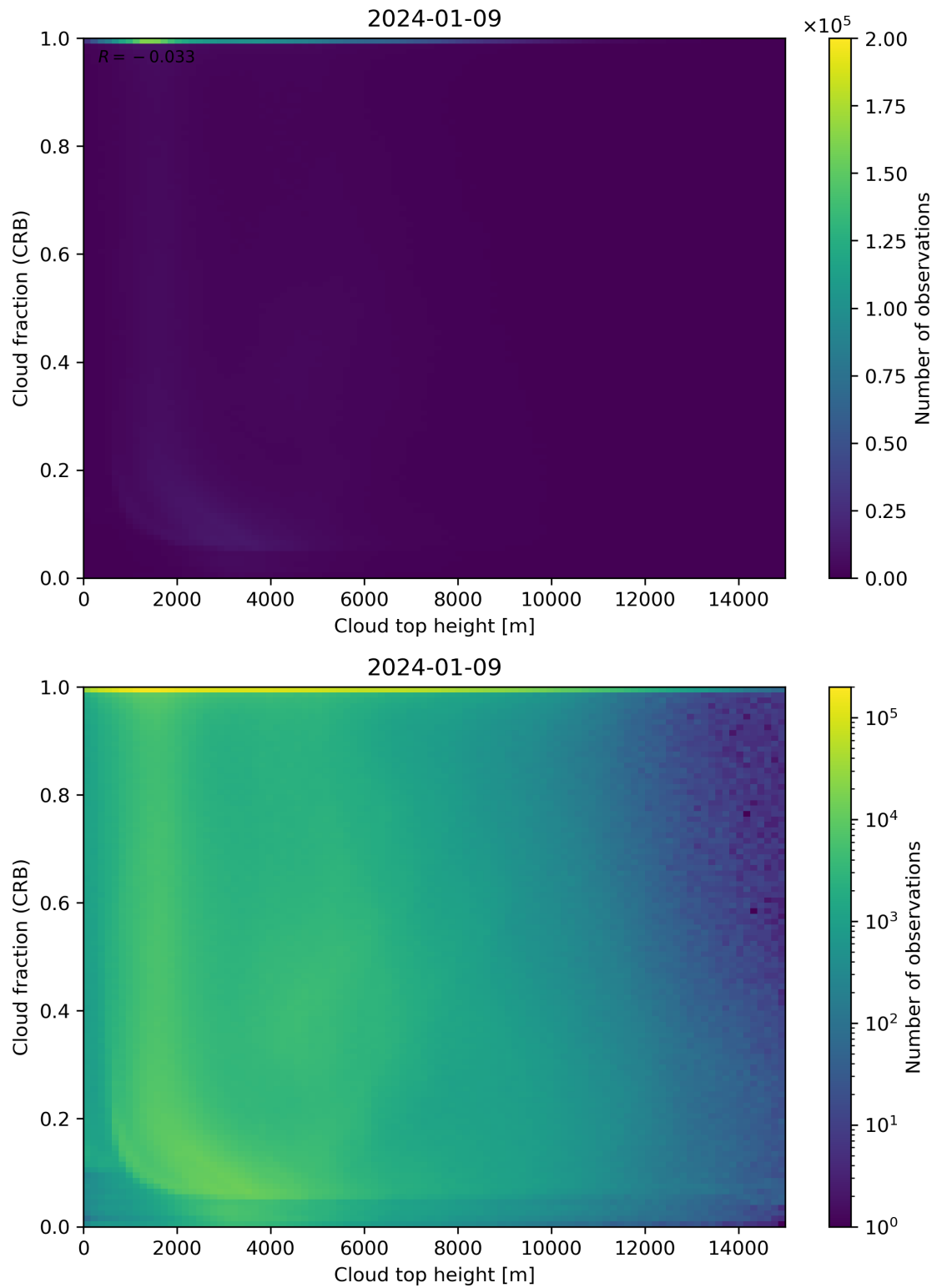
Figure 88: Scatter density plot of “Cloud top height” against “Cloud fraction (CRB)” for 2024-01-08 to 2024-01-10.
