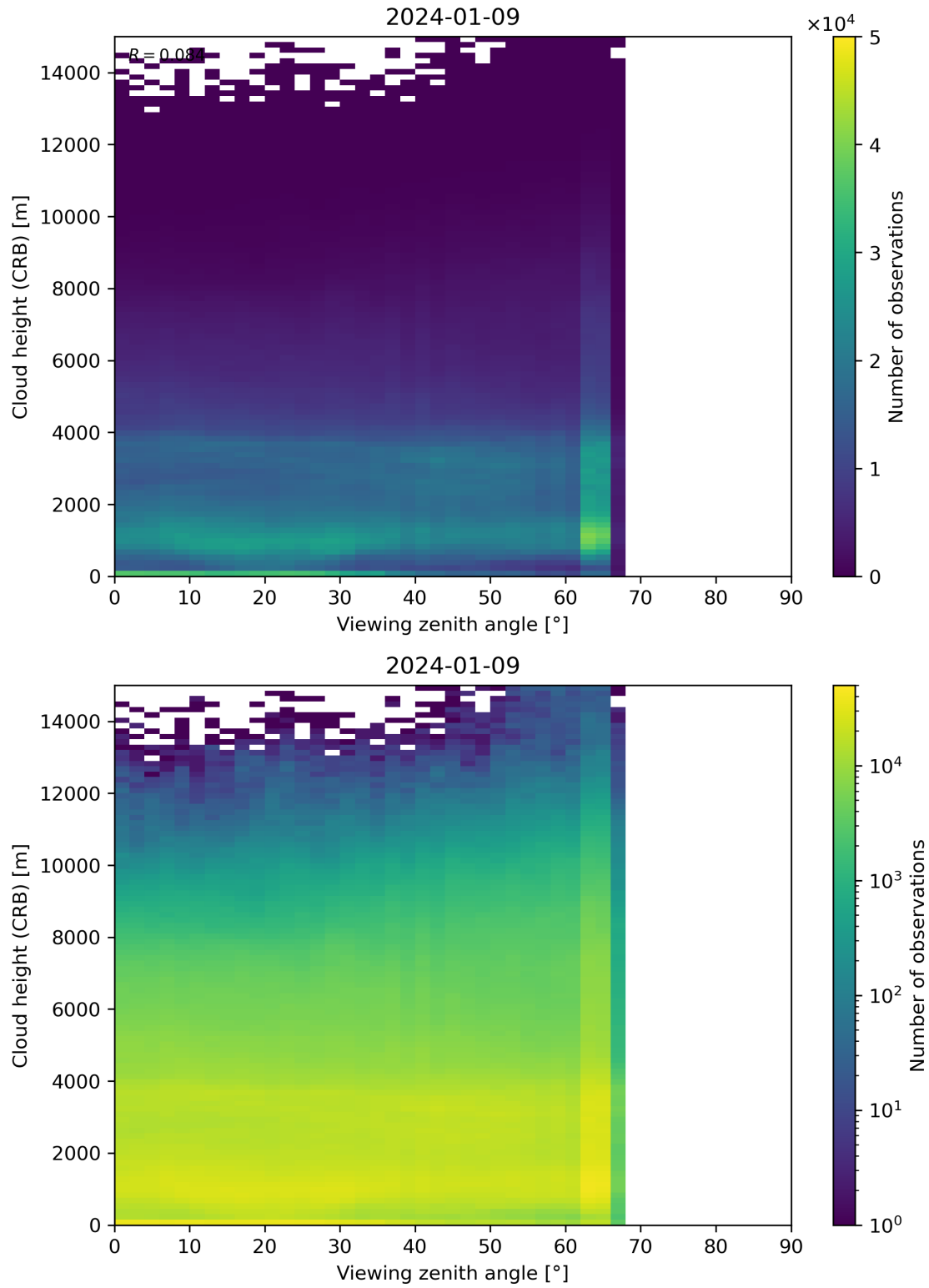
Figure 110: Scatter density plot of “Viewing zenith angle” against “Cloud height (CRB)” for 2024-01-08 to 2024-01-10.
