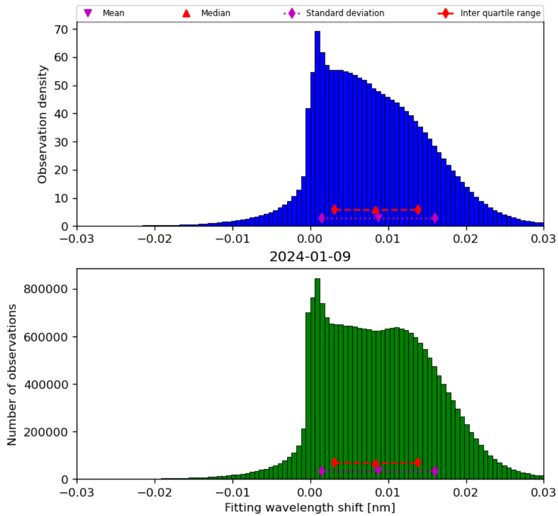
Figure 49: Histogram of “Fitting wavelength shift” for 2024-01-08 to 2024-01-10
