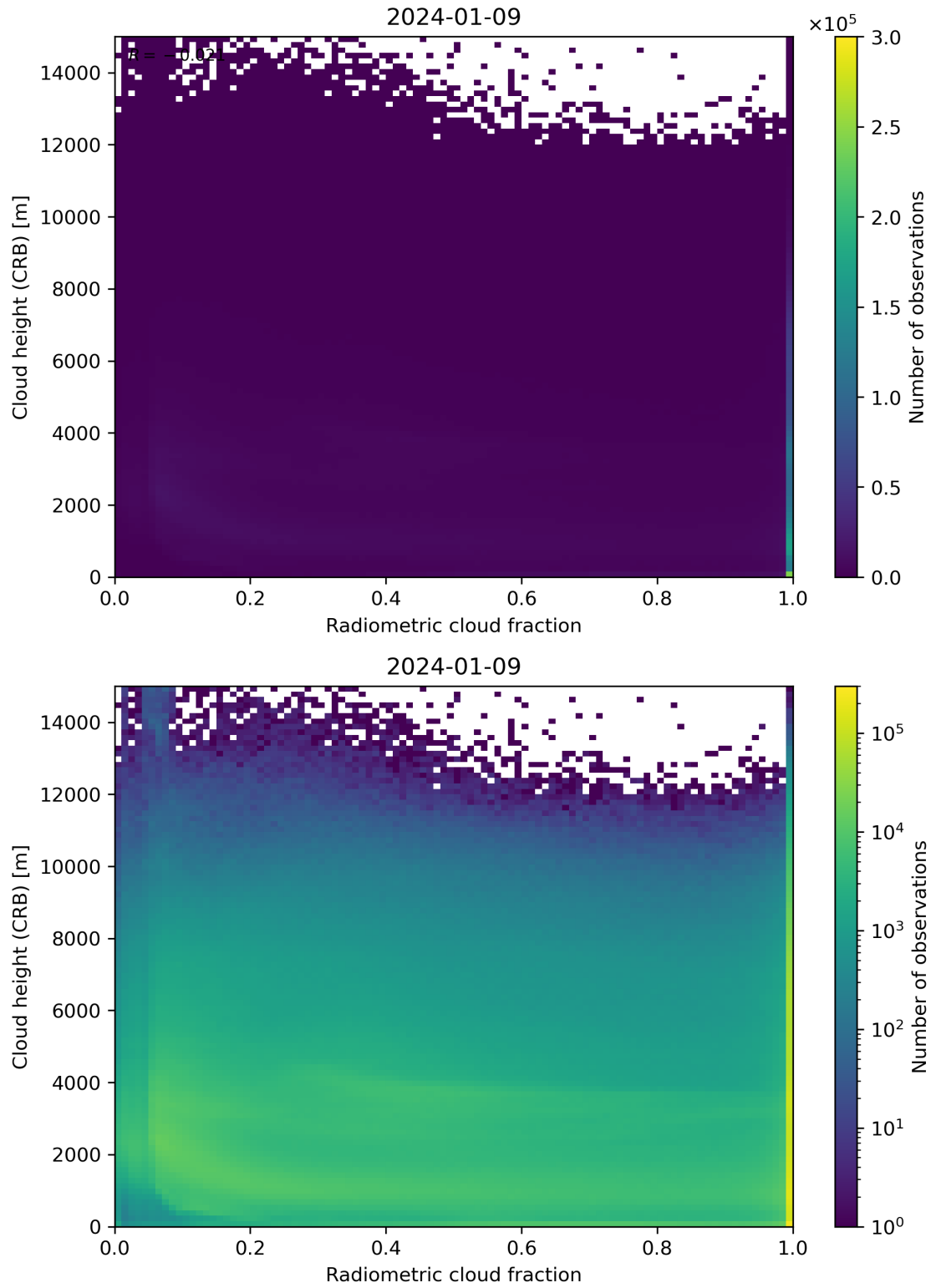
Figure 74: Scatter density plot of “Radiometric cloud fraction” against “Cloud height (CRB)” for 2024-01-08 to 2024-01-10.
