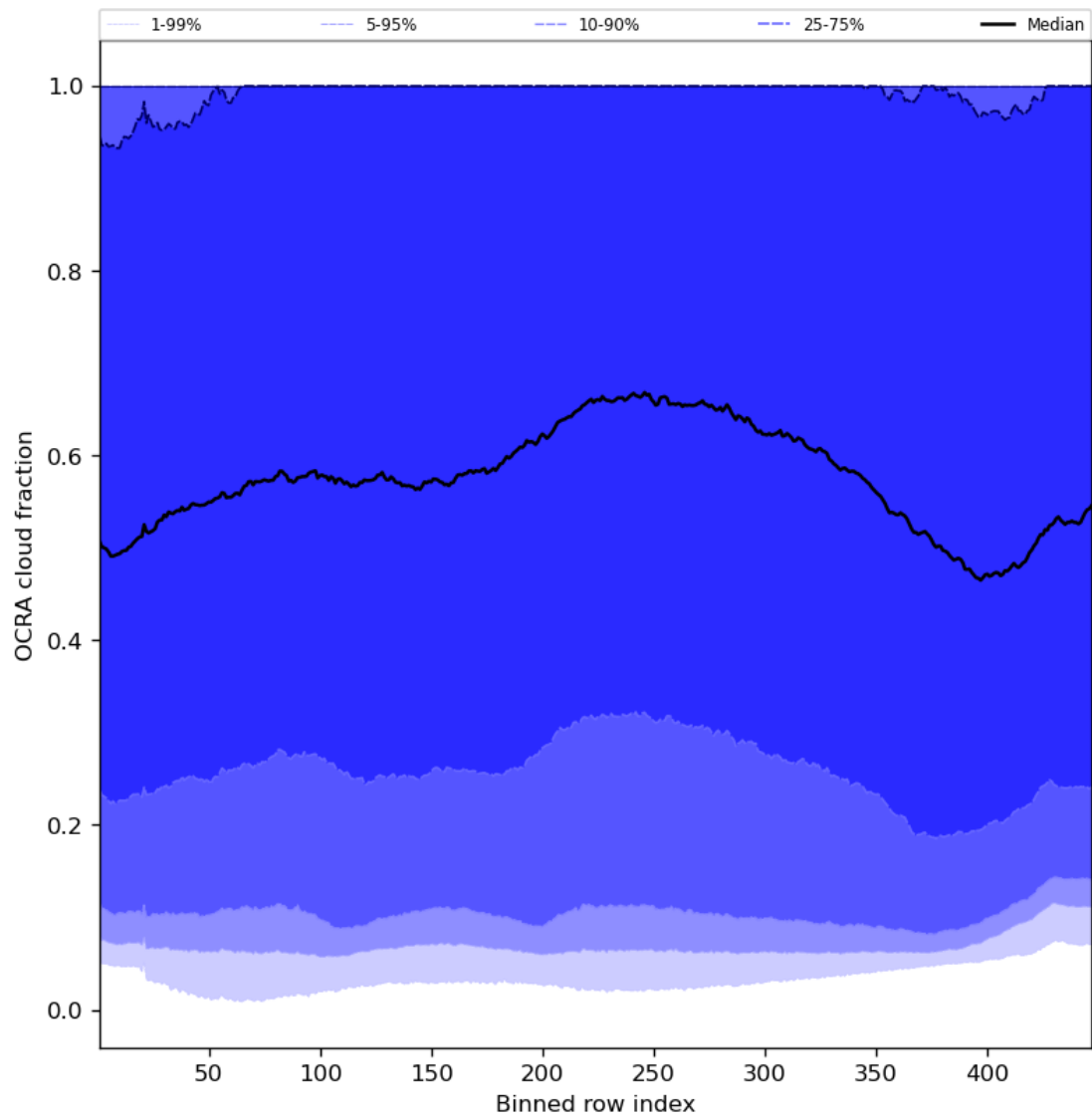
Figure 66: Along track statistics of “OCRA cloud fraction” for 2024-01-08 to 2024-01-10
