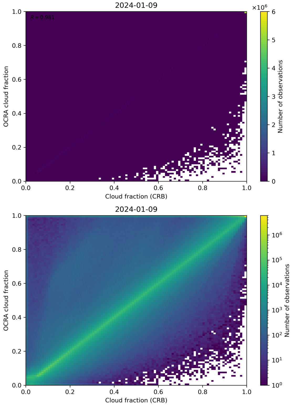
Figure 78: Scatter density plot of “Cloud fraction (CRB)” against “OCRA cloud fraction” for 2024-01-08 to 2024-01-10.
