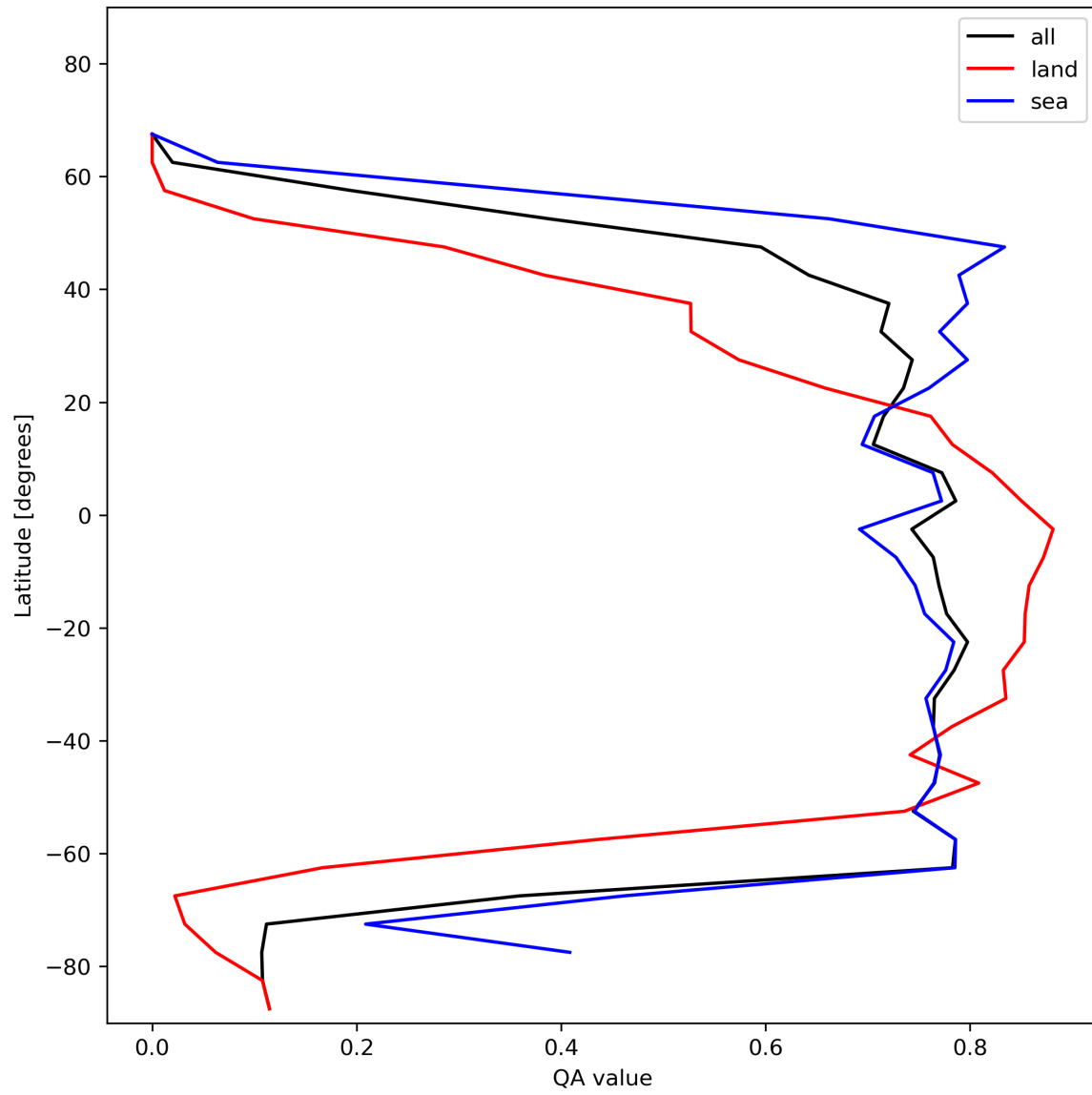
Figure 22: Zonal average of “QA value” for 2024-01-08 to 2024-01-10.
