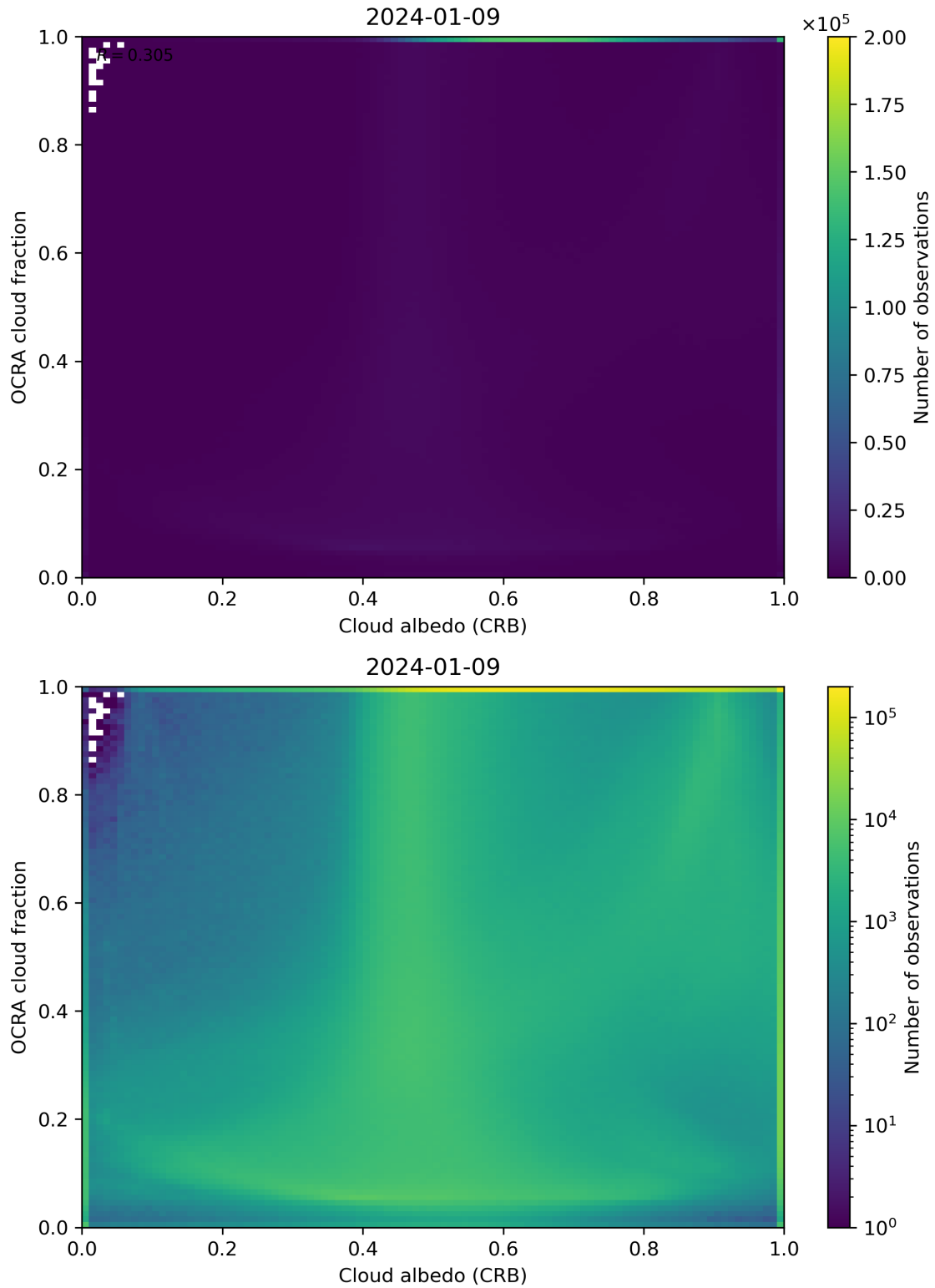
Figure 70: Scatter density plot of “Cloud albedo (CRB)” against “OCRA cloud fraction” for 2024-01-08 to 2024-01-10.
