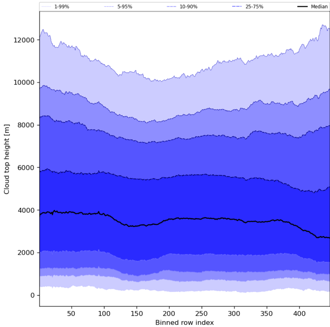
Figure 56: Along track statistics of “Cloud top height” for 2024-01-08 to 2024-01-10
