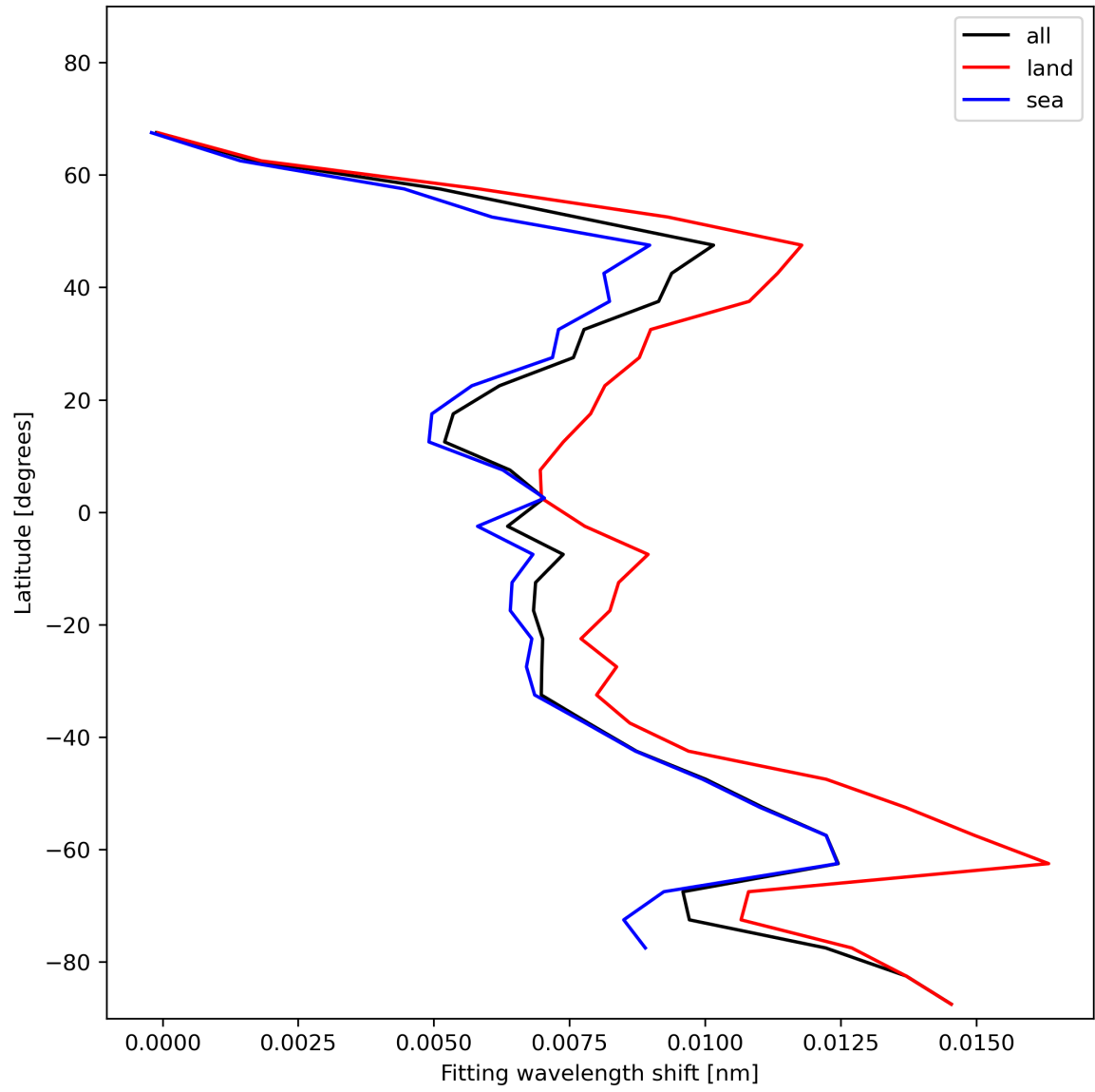
Figure 33: Zonal average of “Fitting wavelength shift” for 2024-01-08 to 2024-01-10.
