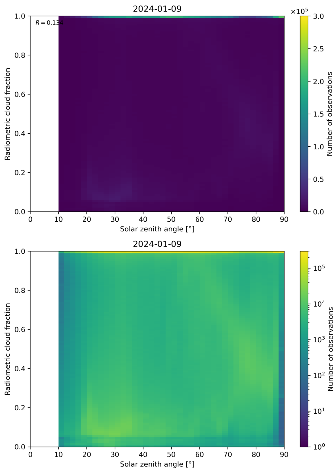
Figure 99: Scatter density plot of “Solar zenith angle” against “Radiometric cloud fraction” for 2024-01-08 to 2024-01-10.
