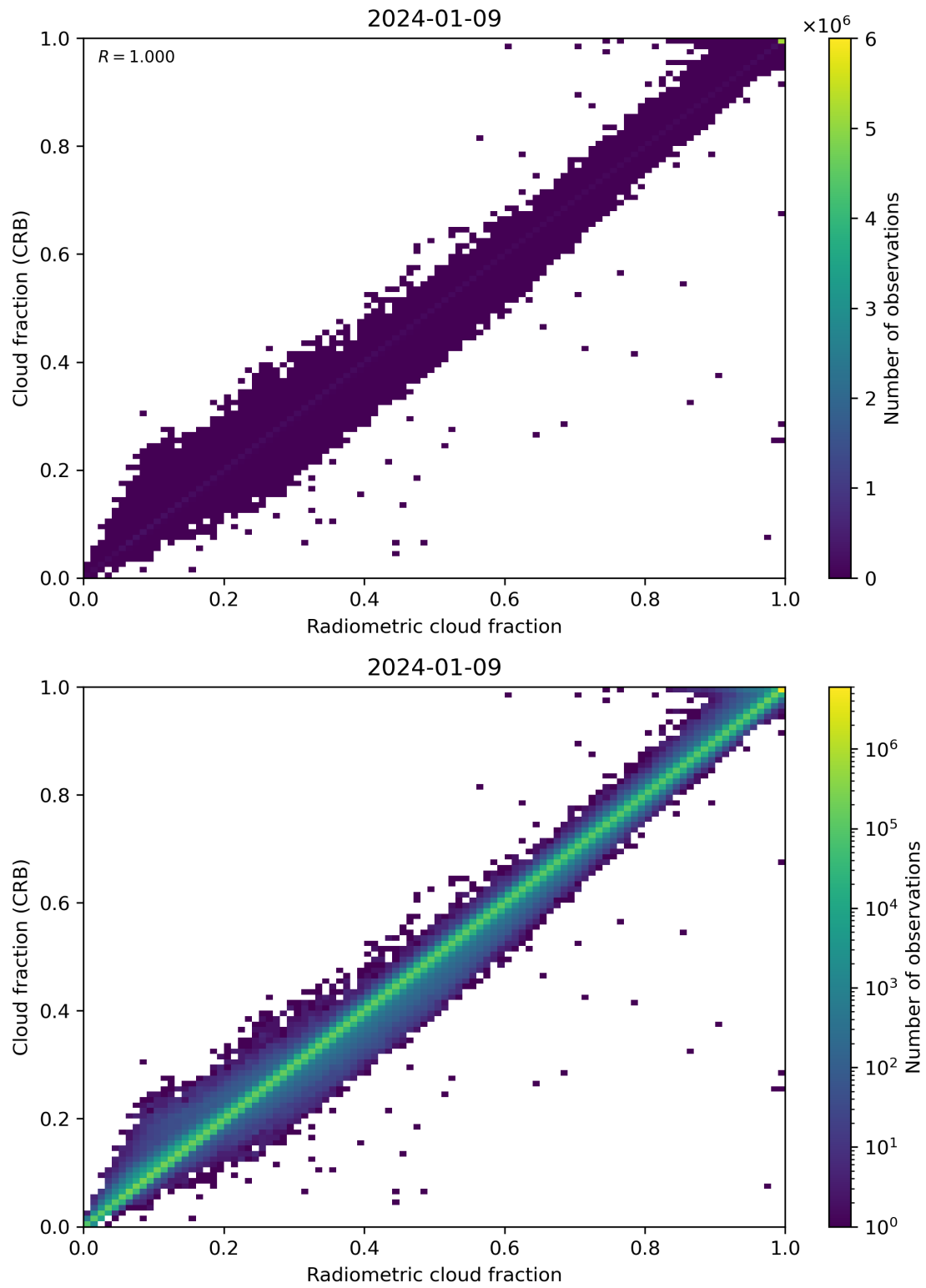
Figure 73: Scatter density plot of “Radiometric cloud fraction” against “Cloud fraction (CRB)” for 2024-01-08 to 2024-01-10.
