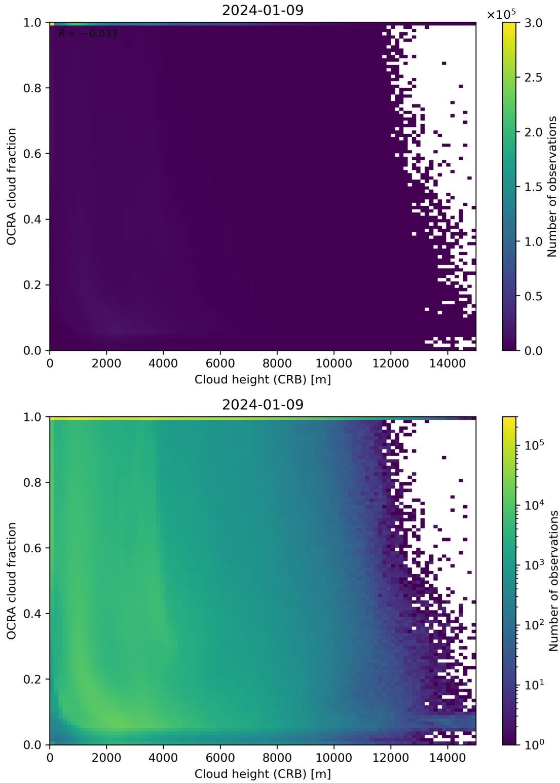
Figure 81: Scatter density plot of “Cloud height (CRB)” against “OCRA cloud fraction” for 2024-01-08 to 2024-01-10.
