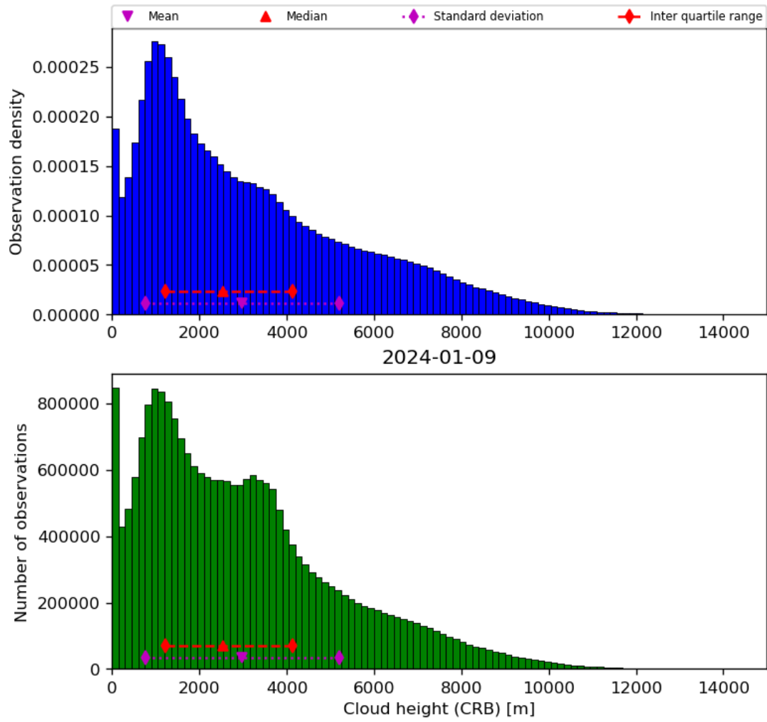
Figure 43: Histogram of “Cloud height (CRB)” for 2024-01-08 to 2024-01-10
