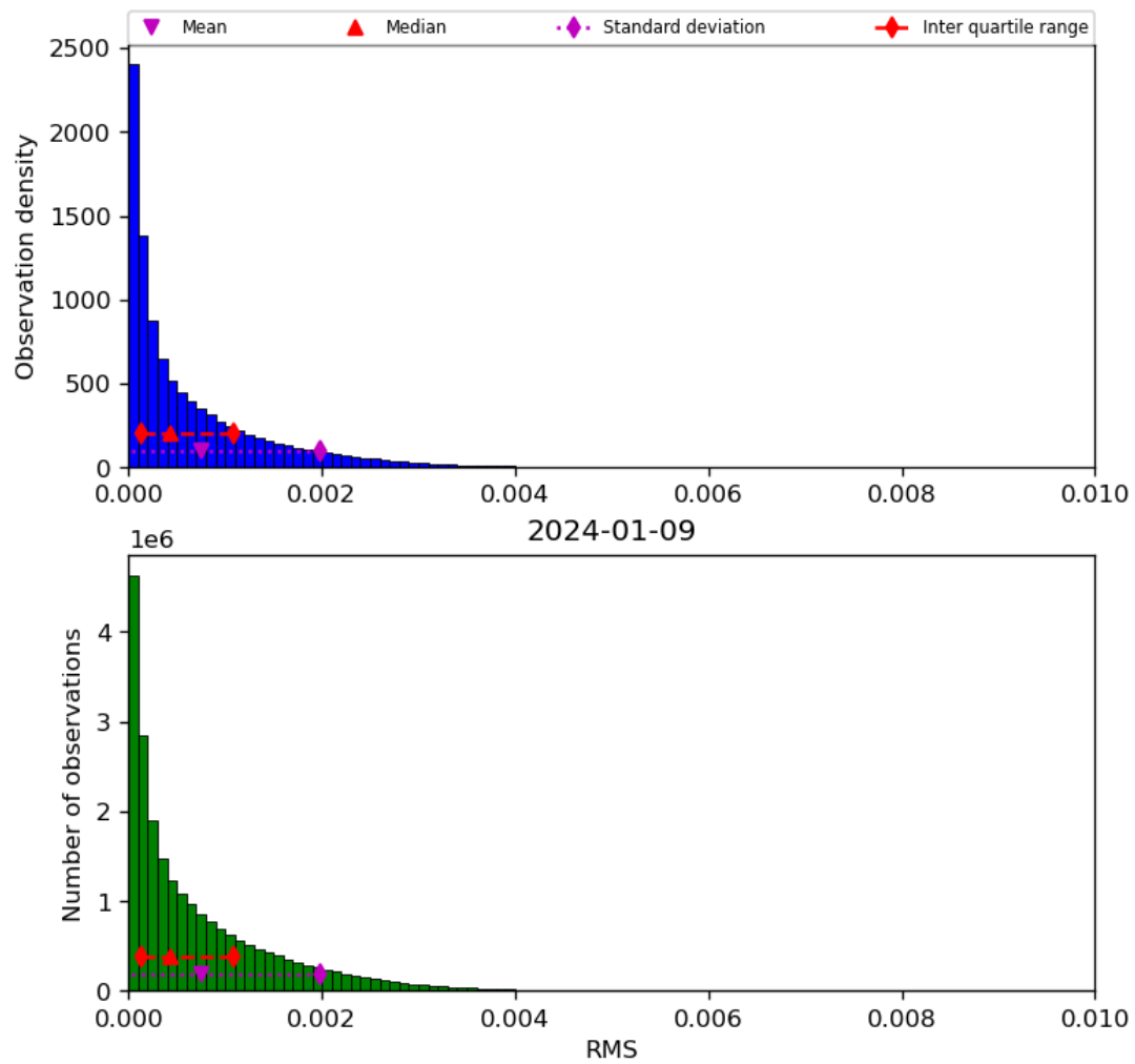
Figure 47: Histogram of “RMS” for 2024-01-08 to 2024-01-10
