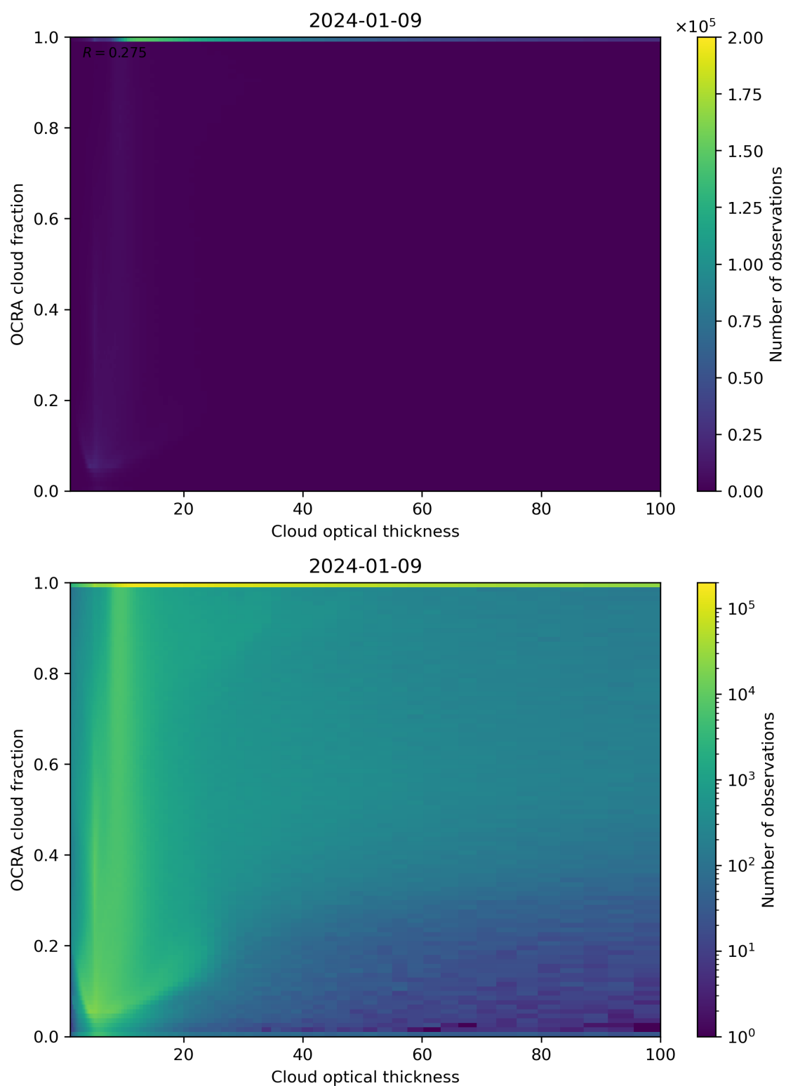
Figure 83: Scatter density plot of “Cloud optical thickness” against “OCRA cloud fraction” for 2024-01-08 to 2024-01-10.
