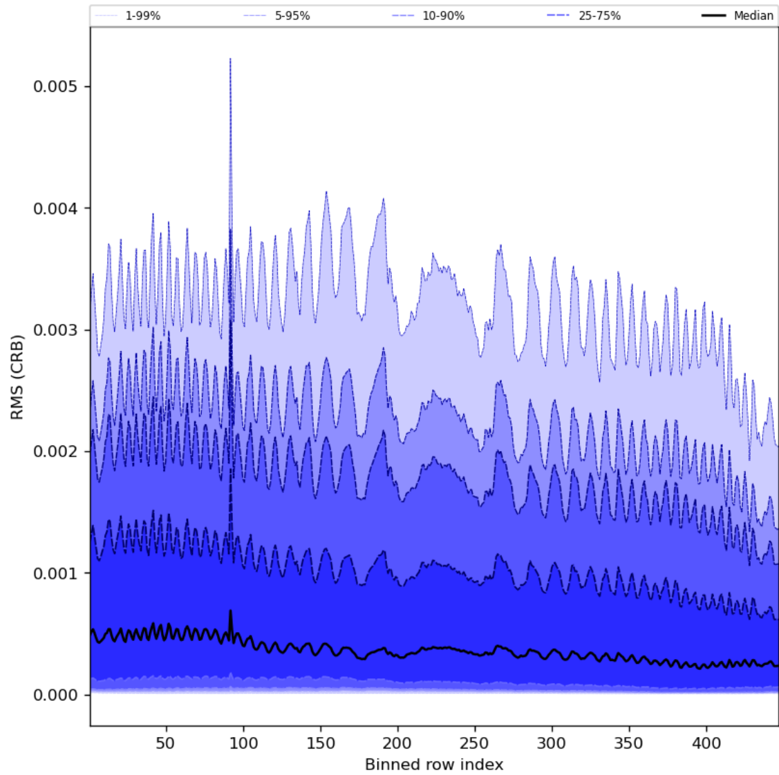
Figure 64: Along track statistics of “RMS (CRB)” for 2024-01-08 to 2024-01-10
