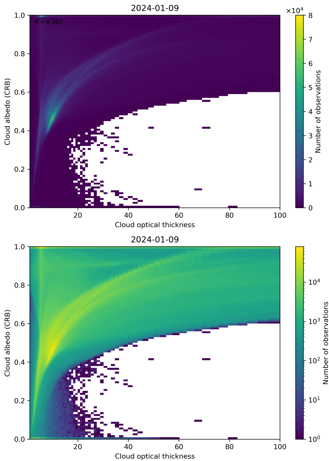
Figure 82: Scatter density plot of “Cloud optical thickness” against “Cloud albedo (CRB)” for 2024-01-08 to 2024-01-10.
