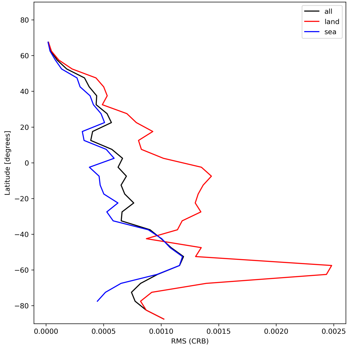
Figure 32: Zonal average of “RMS (CRB)” for 2024-01-08 to 2024-01-10.
