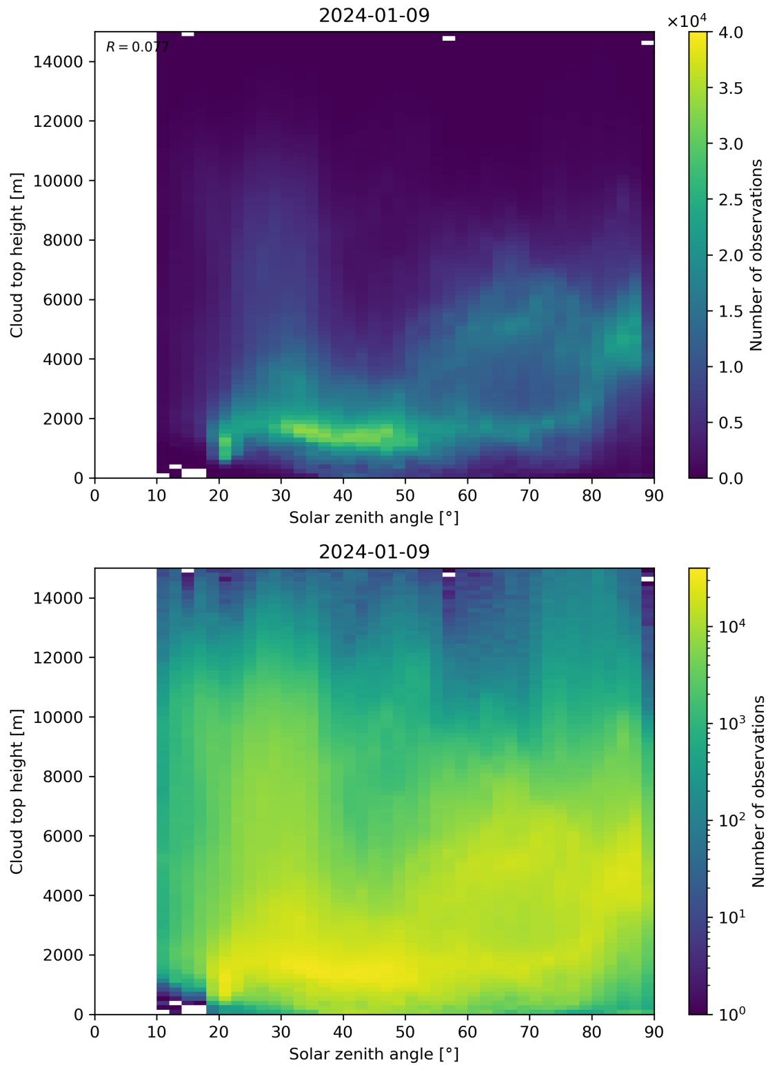
Figure 104: Scatter density plot of “Solar zenith angle” against “Cloud top height” for 2024-01-08 to 2024-01-10.
