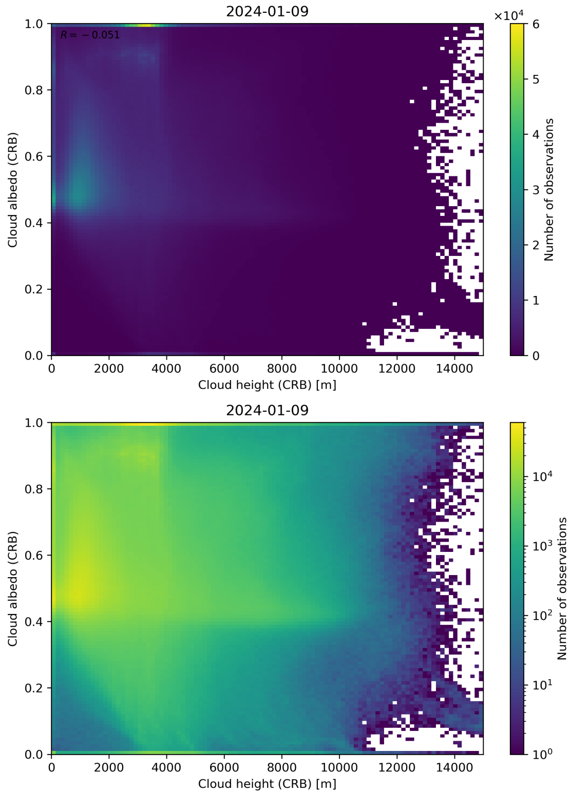
Figure 80: Scatter density plot of “Cloud height (CRB)” against “Cloud albedo (CRB)” for 2024-01-08 to 2024-01-10.
