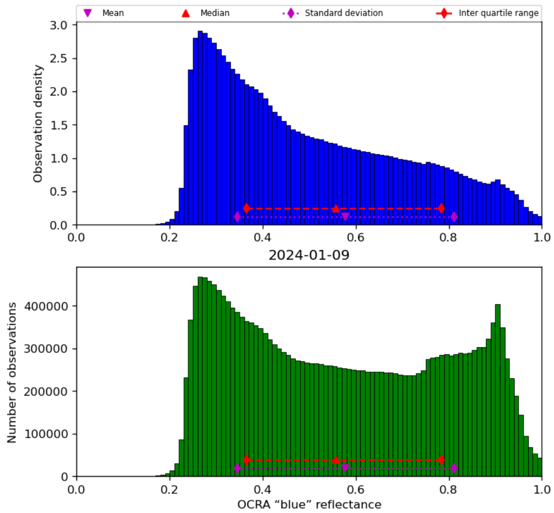
Figure 51: Histogram of “OCRA “blue” reflectance” for 2024-01-08 to 2024-01-10
