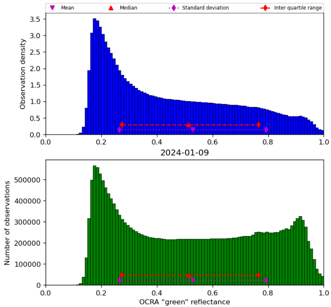
Figure 52: Histogram of “OCRA “green” reflectance” for 2024-01-08 to 2024-01-10
