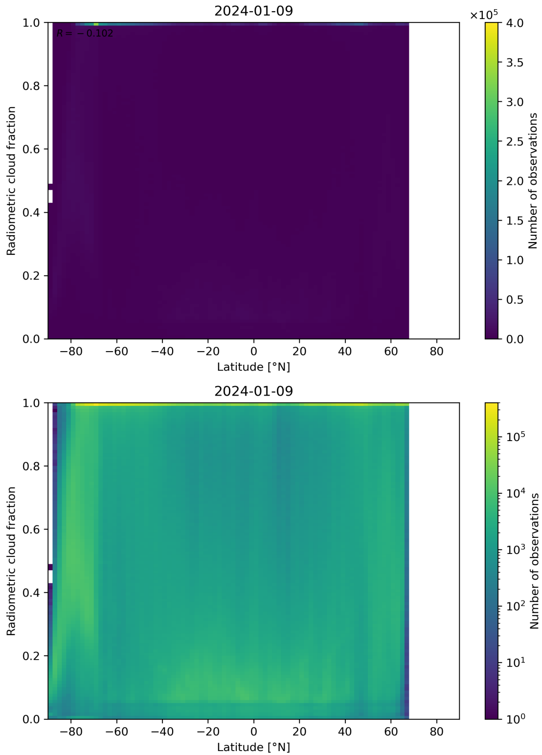
Figure 92: Scatter density plot of “Latitude” against “Radiometric cloud fraction” for 2024-01-08 to 2024-01-10.
