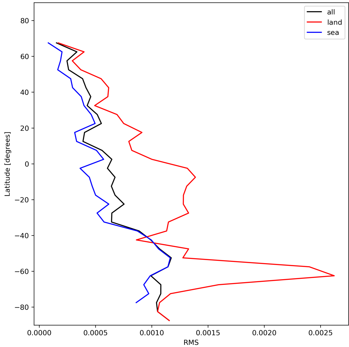
Figure 31: Zonal average of “RMS” for 2024-01-08 to 2024-01-10.
