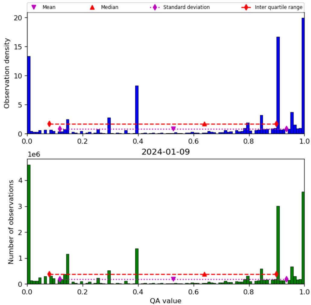
Figure 38: Histogram of “QA value” for 2024-01-08 to 2024-01-10
