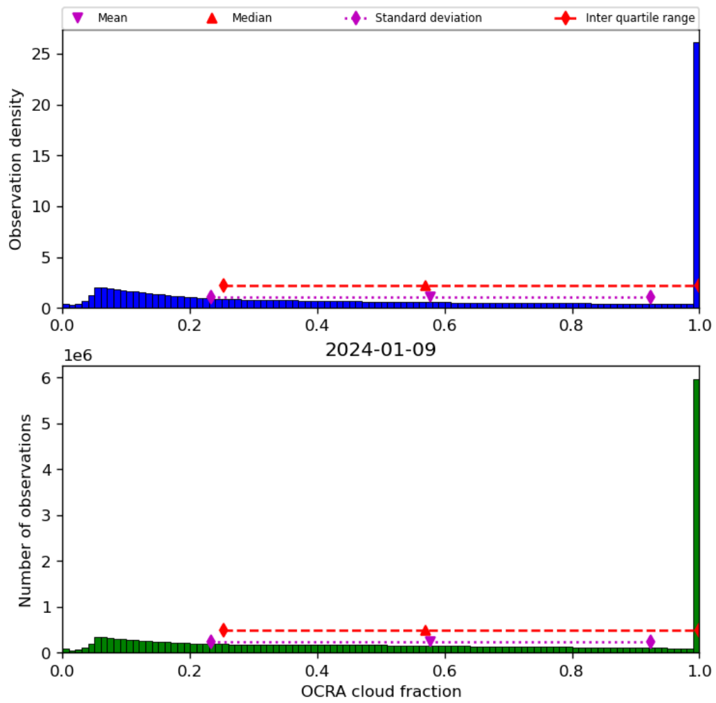
Figure 50: Histogram of “OCRA cloud fraction” for 2024-01-08 to 2024-01-10
