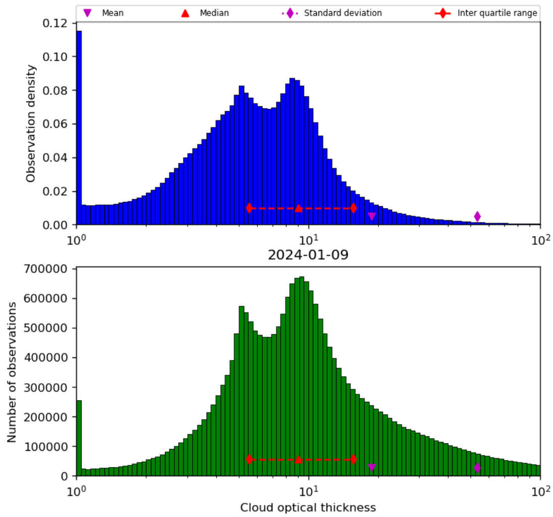
Figure 41: Histogram of “Cloud optical thickness” for 2024-01-08 to 2024-01-10
