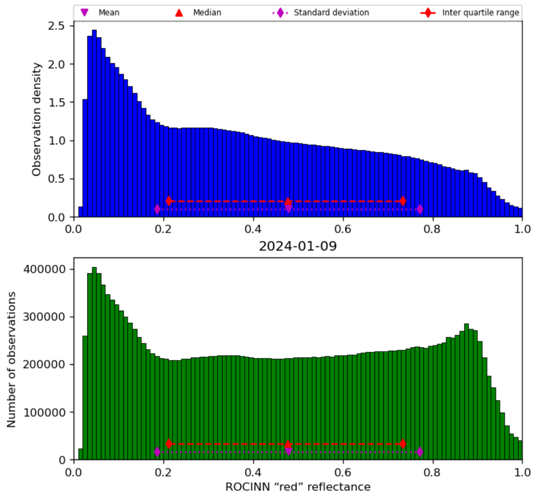
Figure 53: Histogram of “ROCINN “red” reflectance” for 2024-01-08 to 2024-01-10
