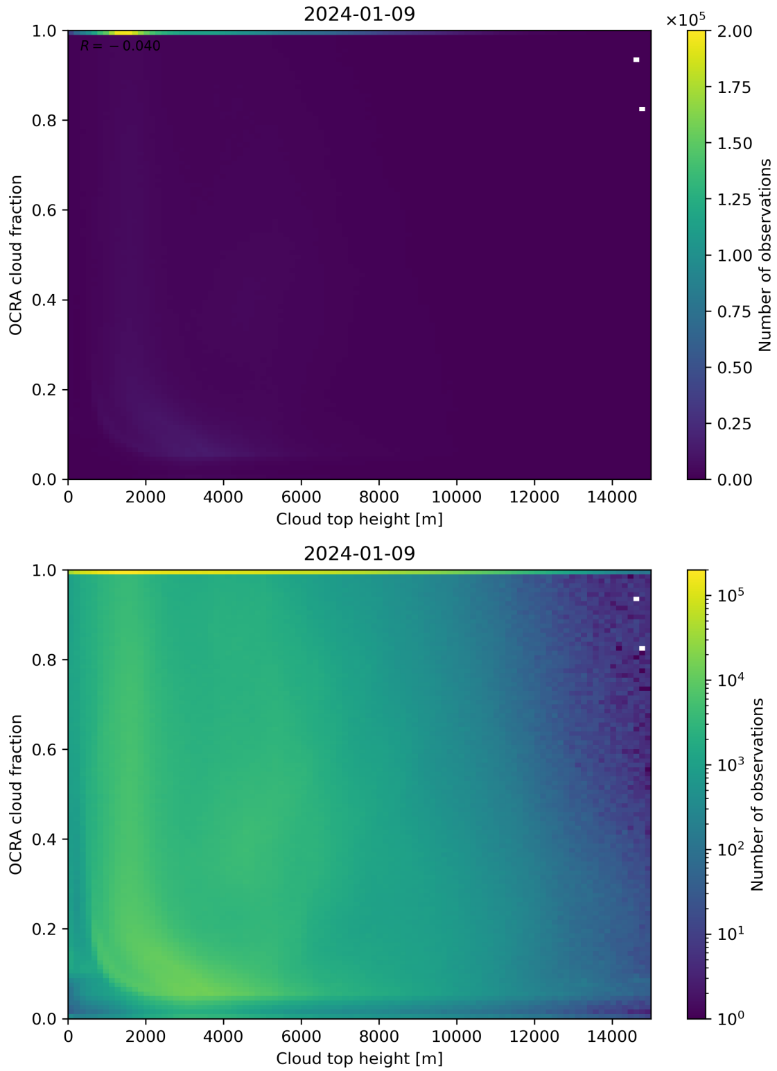
Figure 87: Scatter density plot of “Cloud top height” against “OCRA cloud fraction” for 2024-01-08 to 2024-01-10.
