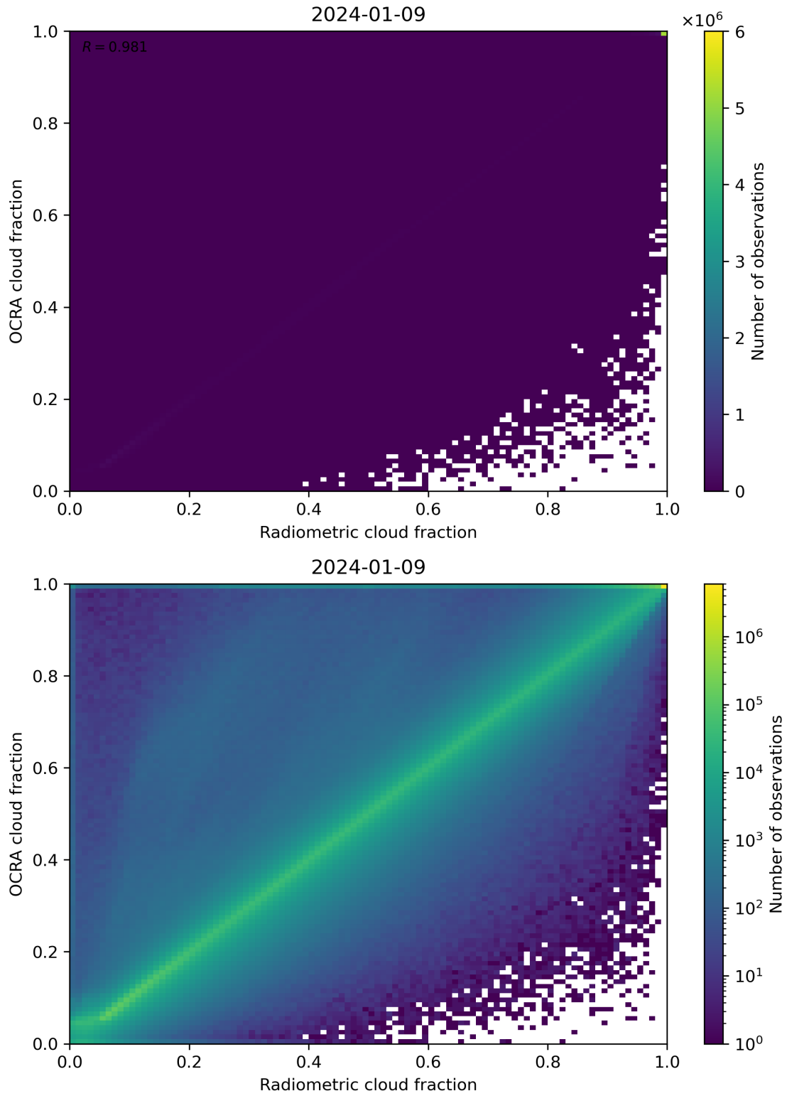
Figure 72: Scatter density plot of “Radiometric cloud fraction” against “OCRA cloud fraction” for 2024-01-08 to 2024-01-10.
