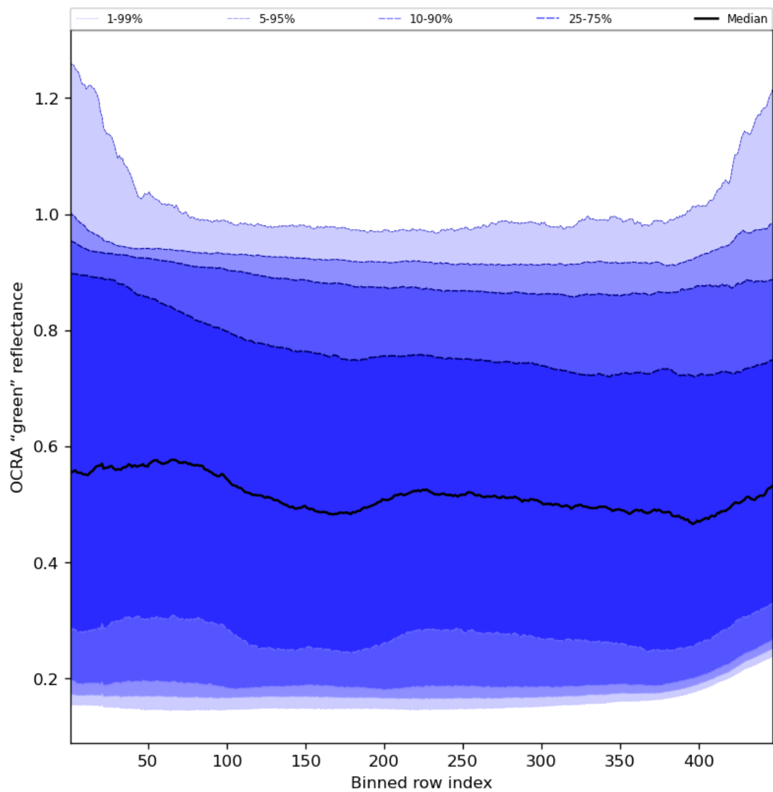
Figure 68: Along track statistics of "OCRA "green" reflectance" for 2024-01-08 to 2024-01-10
