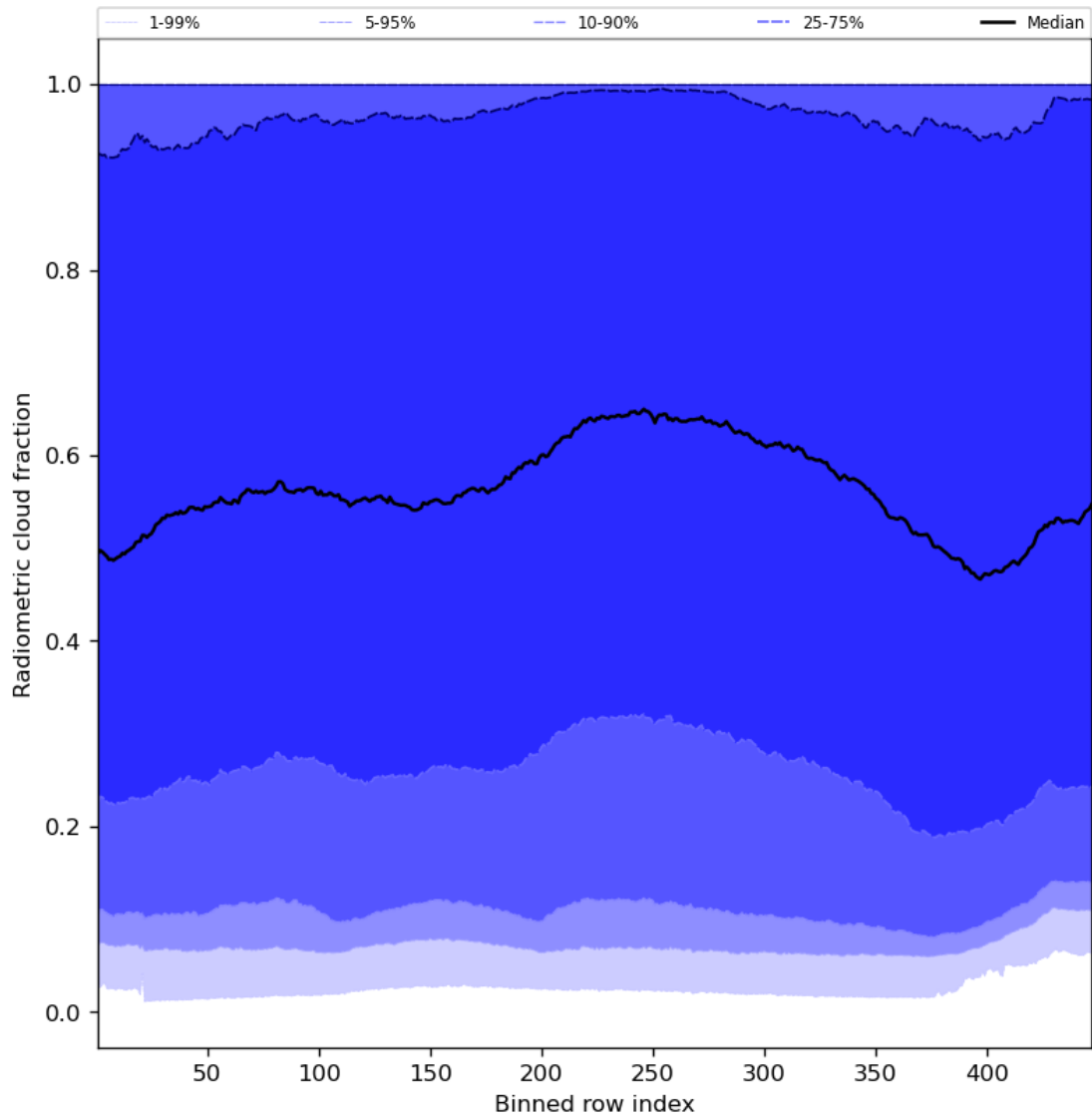
Figure 55: Along track statistics of “Radiometric cloud fraction” for 2024-01-08 to 2024-01-10
