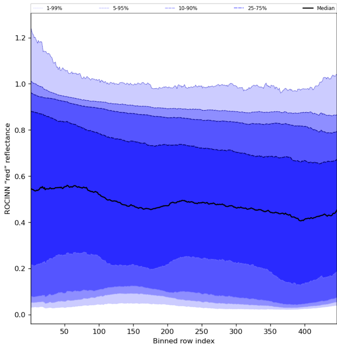
Figure 69: Along track statistics of “ROCINN “red” reflectance” for 2024-01-08 to 2024-01-10
