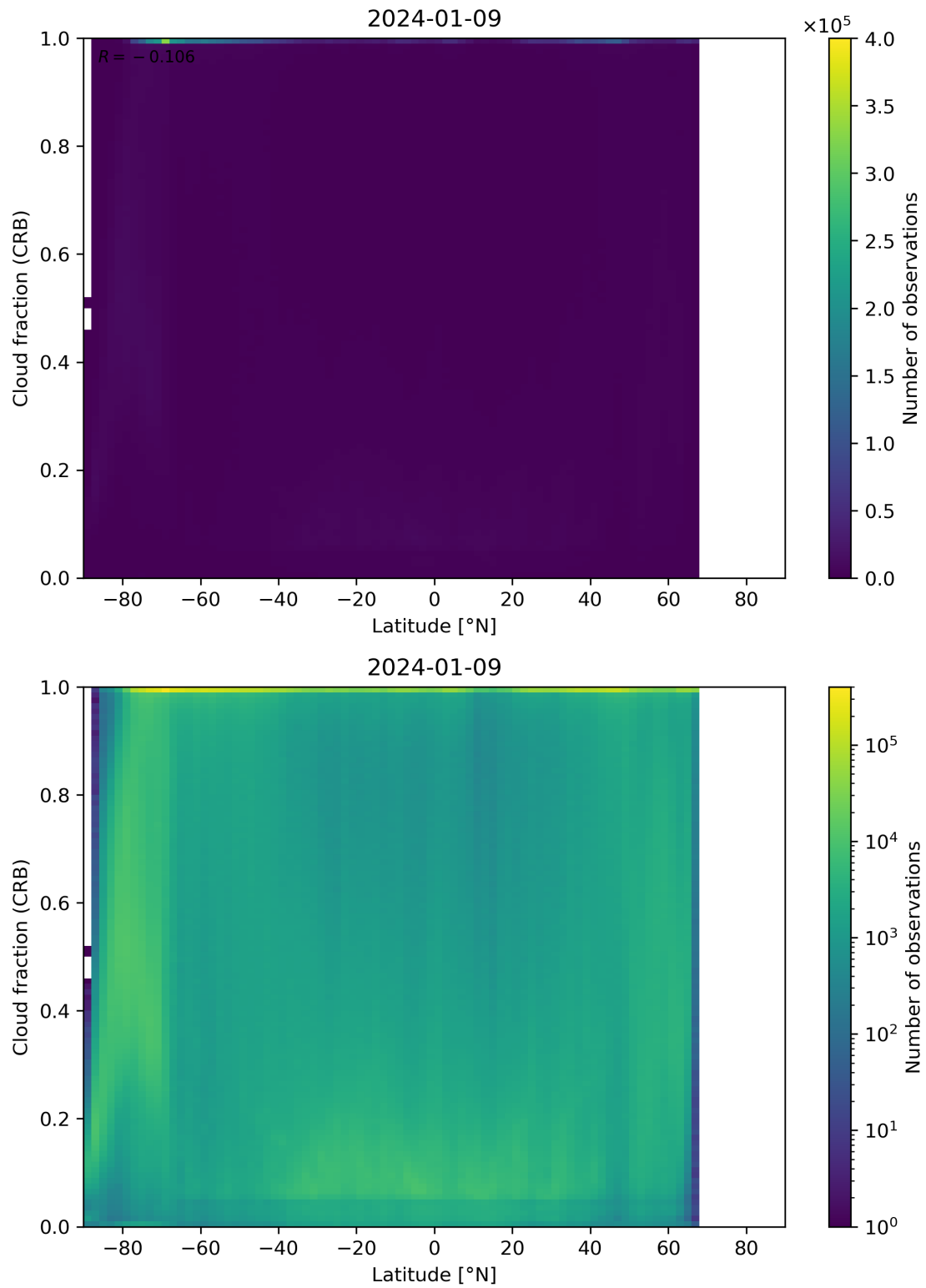
Figure 94: Scatter density plot of “Latitude” against “Cloud fraction (CRB)” for 2024-01-08 to 2024-01-10.
