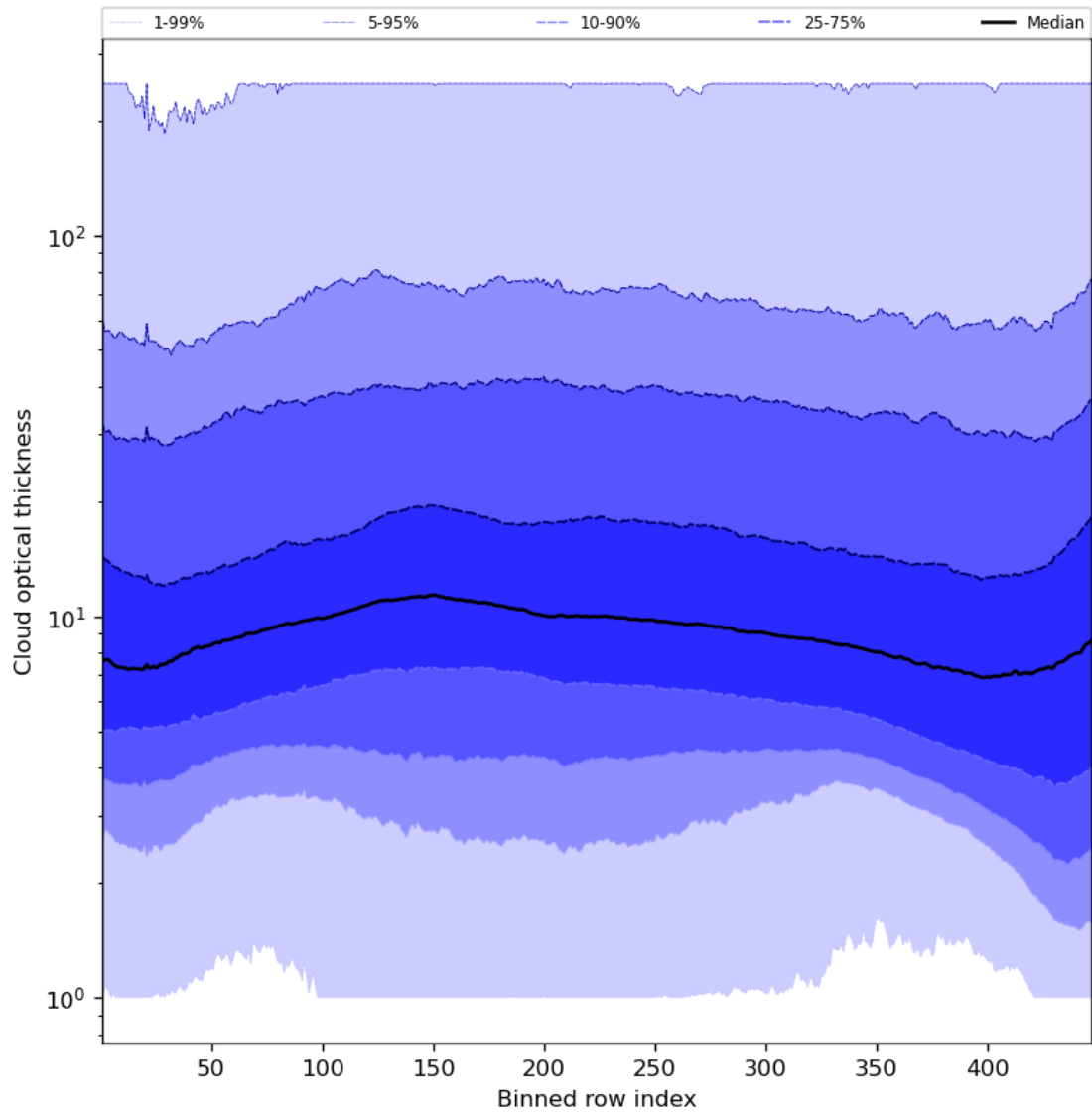
Figure 57: Along track statistics of “Cloud optical thickness” for 2024-01-08 to 2024-01-10
