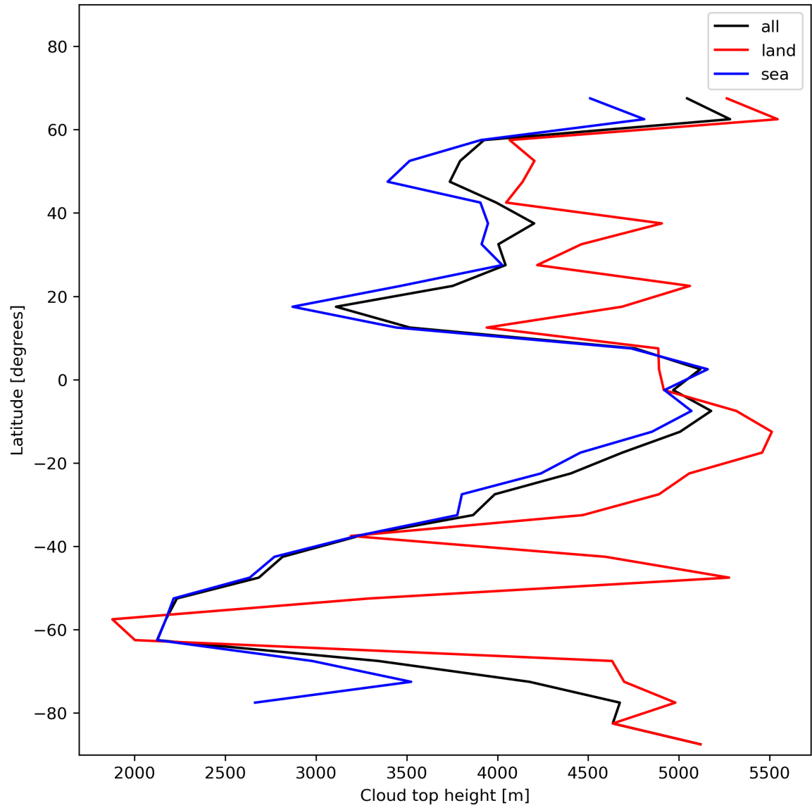
Figure 24: Zonal average of “Cloud top height” for 2024-01-08 to 2024-01-10.
