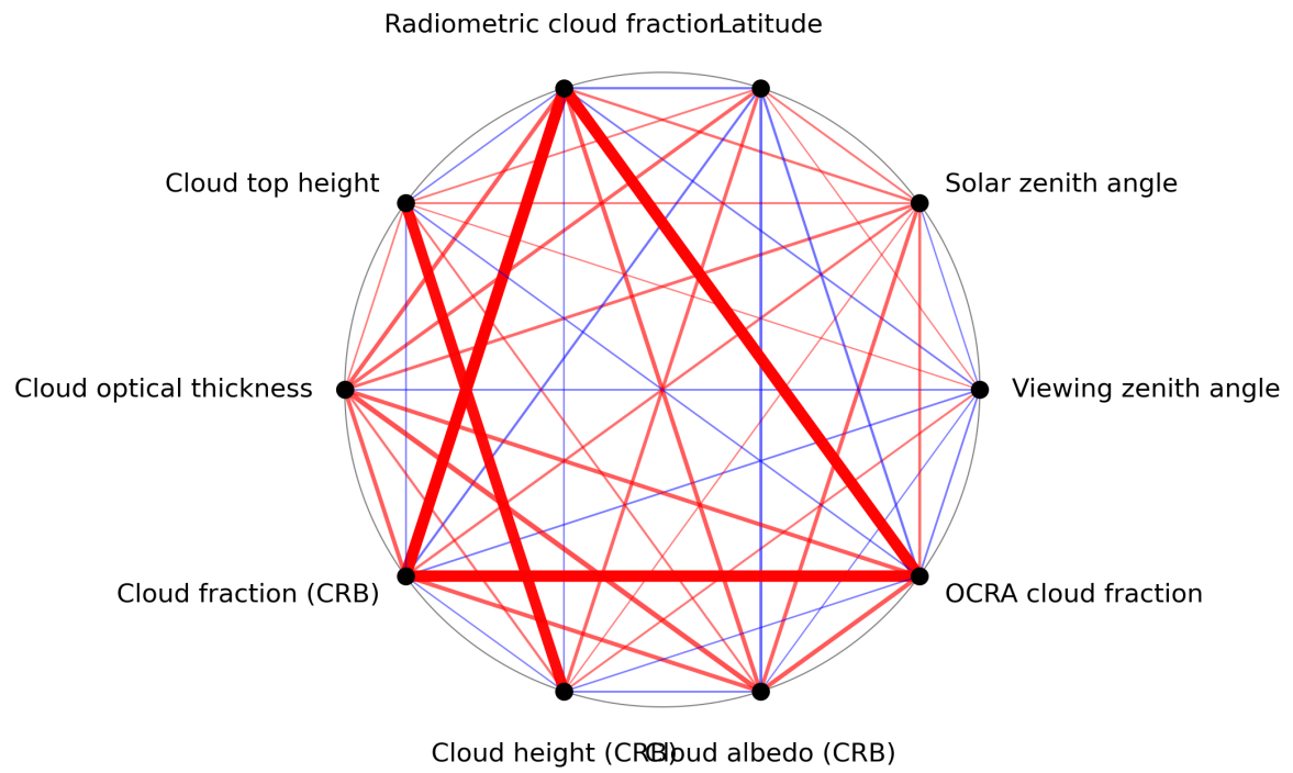
Figure 1: Map of correlation graph for 2024-01-08 to 2024-01-10.
