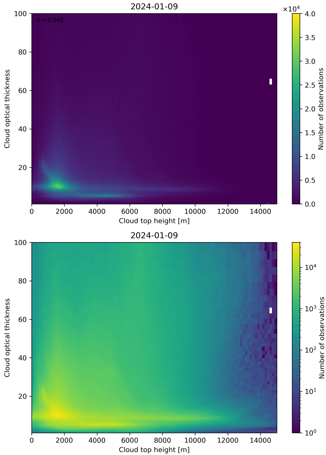
Figure 90: Scatter density plot of “Cloud top height” against “Cloud optical thickness” for 2024-01-08 to 2024-01-10.
