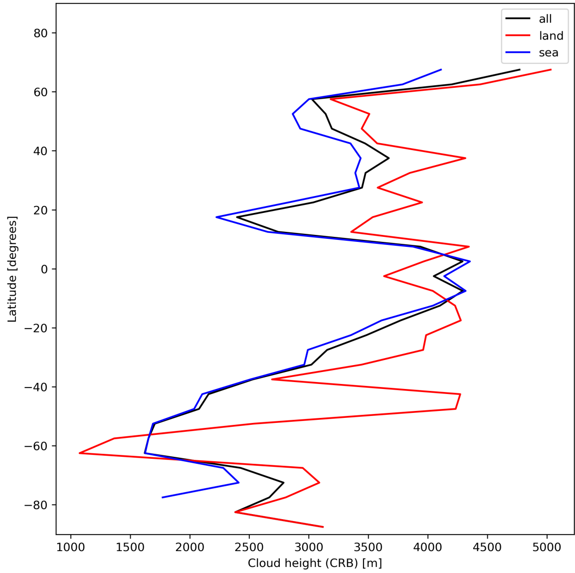
Figure 27: Zonal average of “Cloud height (CRB)” for 2024-01-08 to 2024-01-10.
