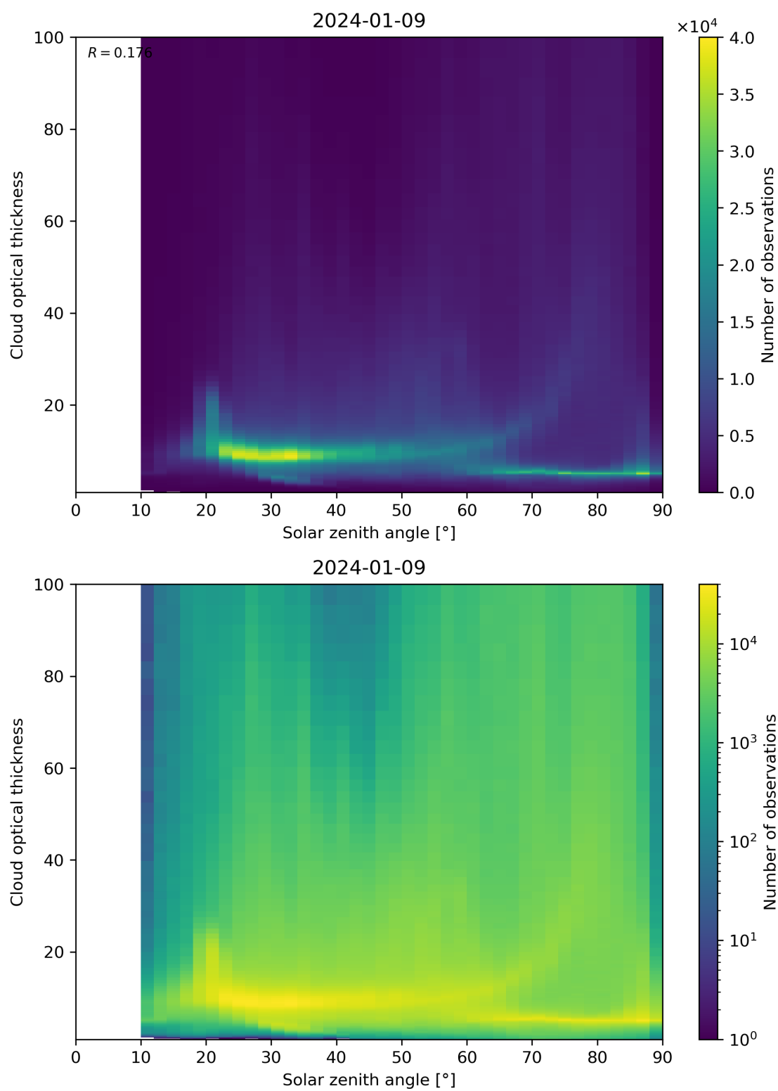
Figure 103: Scatter density plot of “Solar zenith angle” against “Cloud optical thickness” for 2024-01-08 to 2024-01-10.
