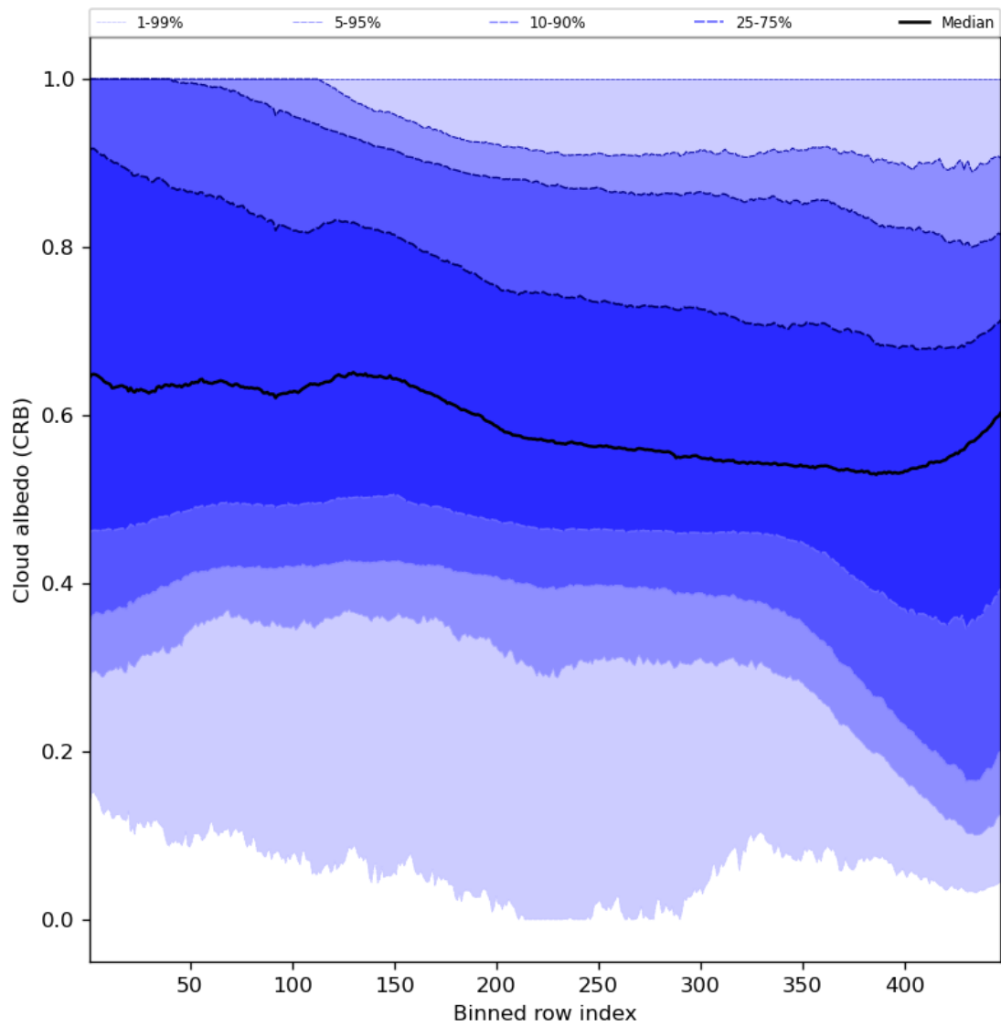
Figure 60: Along track statistics of “Cloud albedo (CRB)” for 2024-01-08 to 2024-01-10
