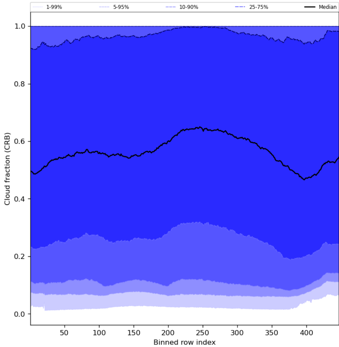
Figure 58: Along track statistics of “Cloud fraction (CRB)” for 2024-01-08 to 2024-01-10
