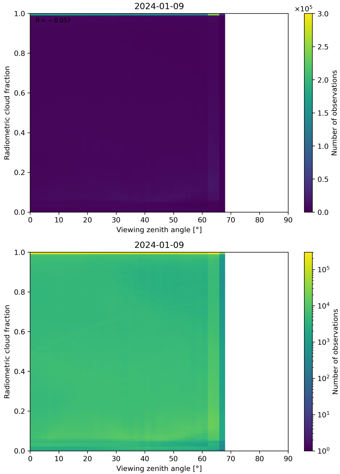
Figure 107: Scatter density plot of “Viewing zenith angle” against “Radiometric cloud fraction” for 2024-01-08 to 2024-01-10.
