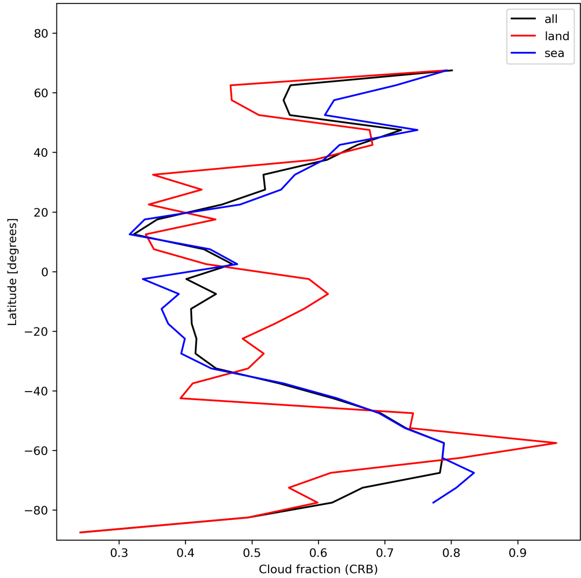
Figure 26: Zonal average of “Cloud fraction (CRB)” for 2024-01-08 to 2024-01-10.
