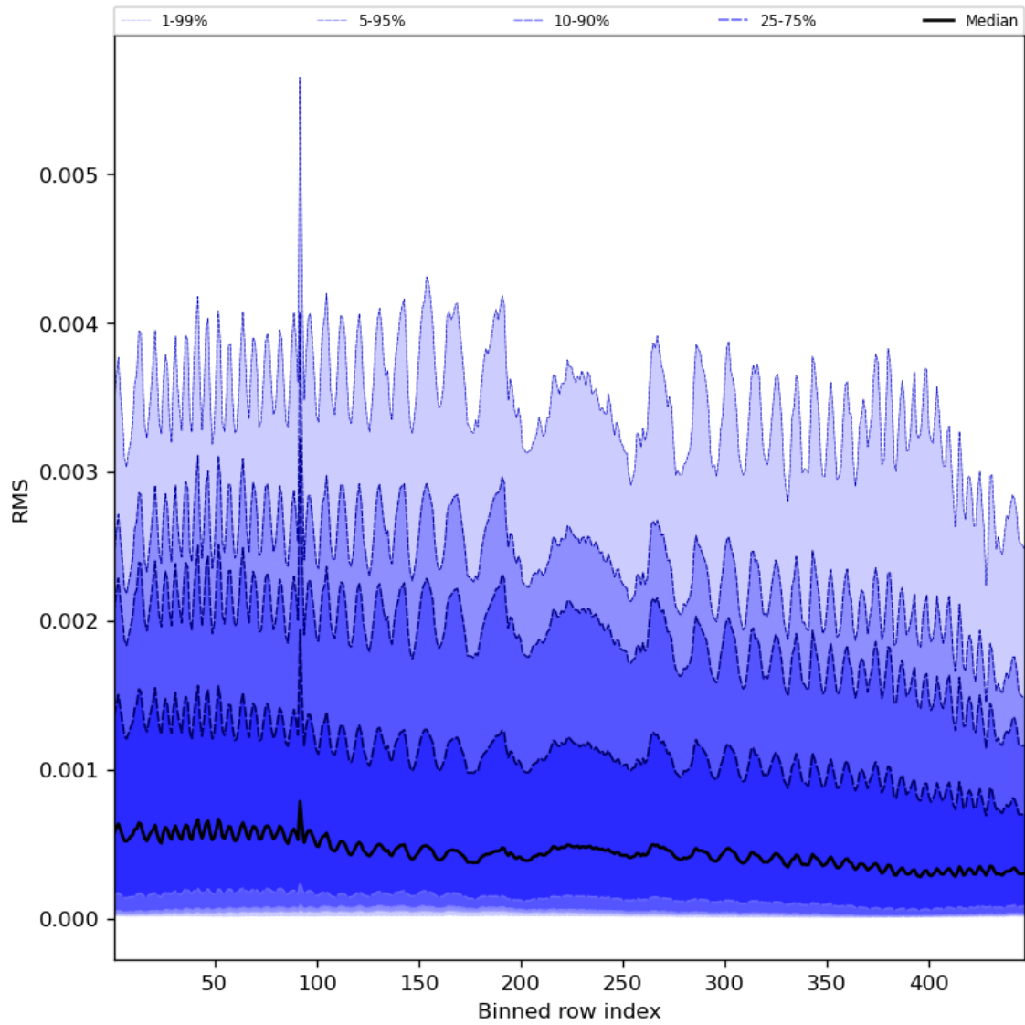
Figure 63: Along track statistics of “RMS” for 2024-01-08 to 2024-01-10
