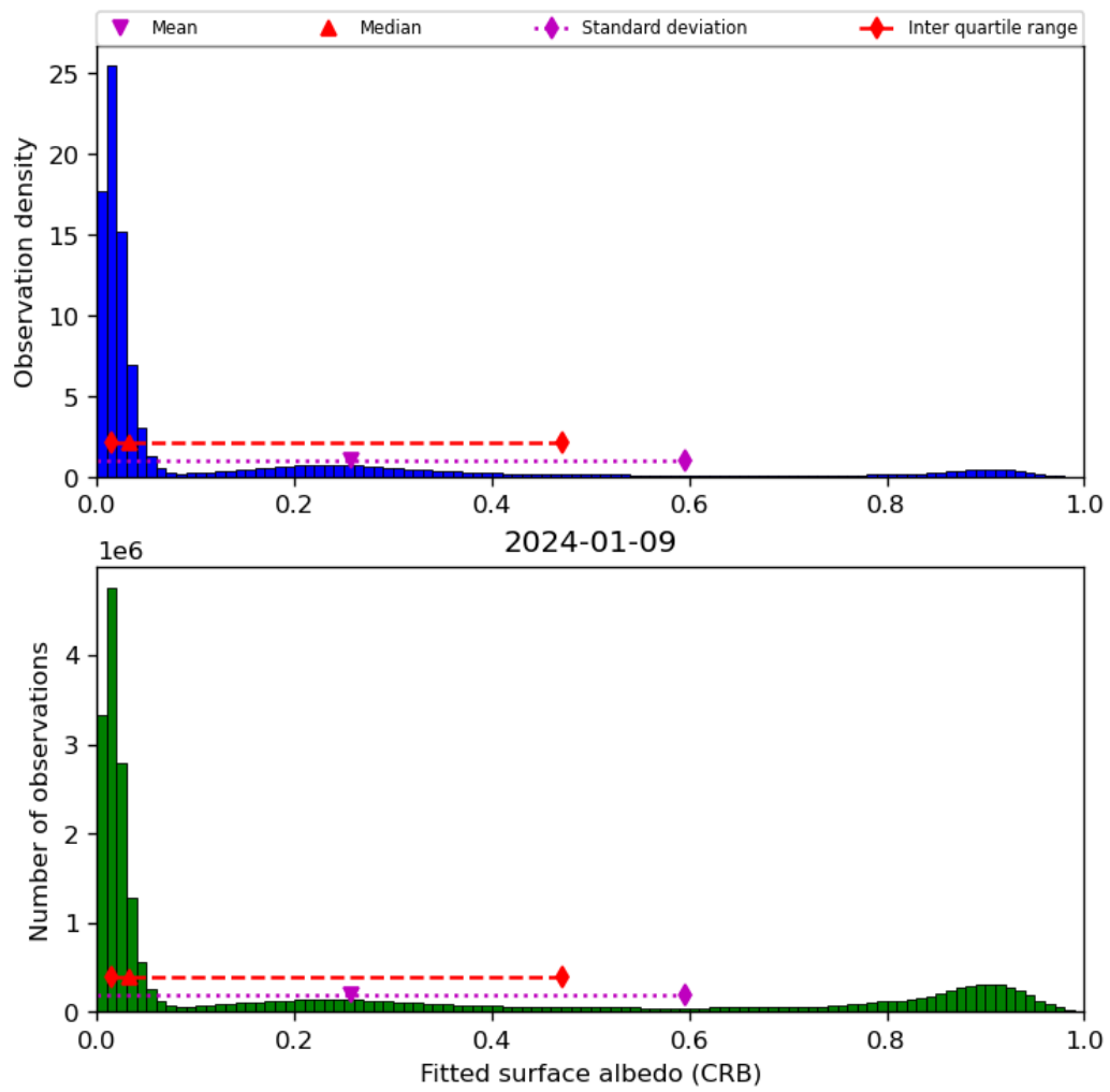
Figure 46: Histogram of “Fitted surface albedo (CRB)” for 2024-01-08 to 2024-01-10
