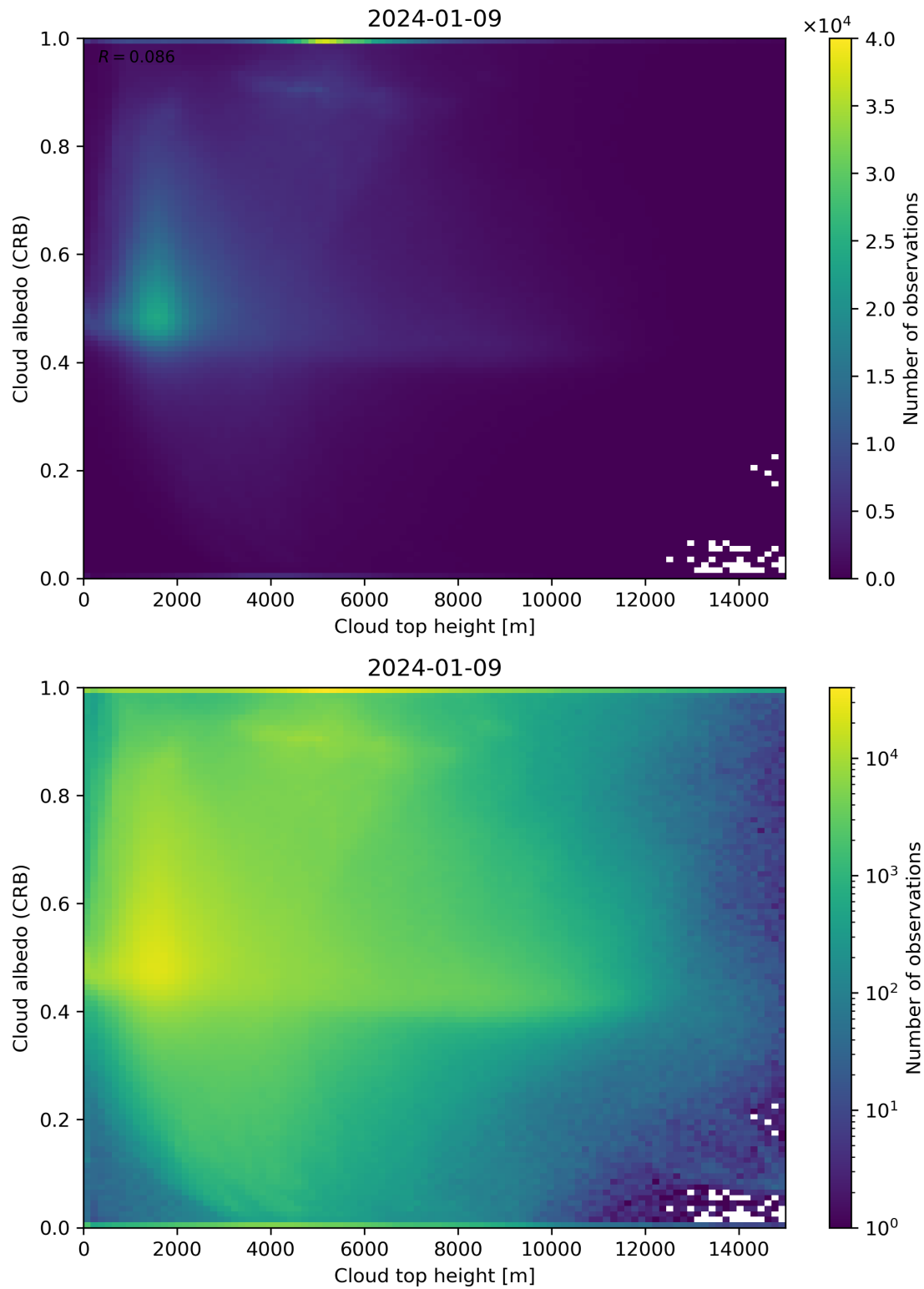
Figure 86: Scatter density plot of “Cloud top height” against “Cloud albedo (CRB)” for 2024-01-08 to 2024-01-10.
