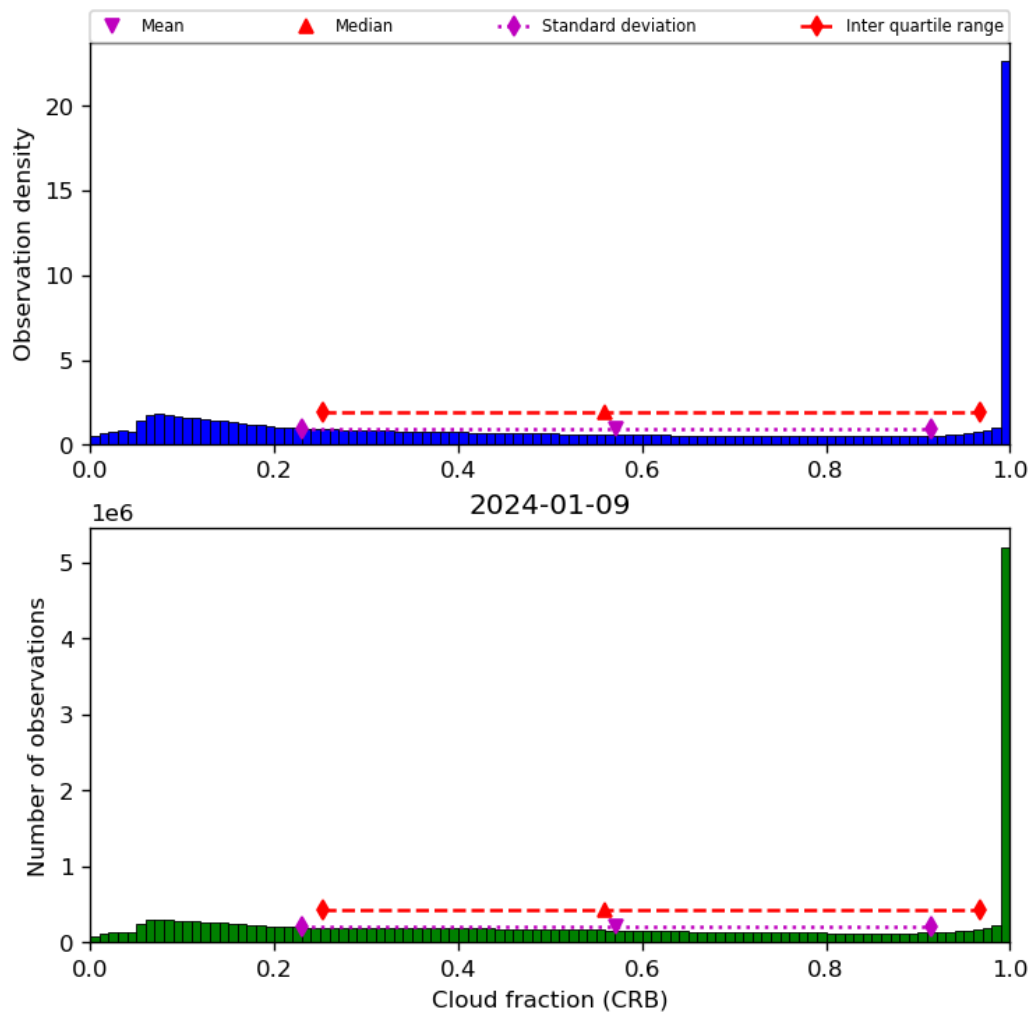
Figure 42: Histogram of “Cloud fraction (CRB)” for 2024-01-08 to 2024-01-10
