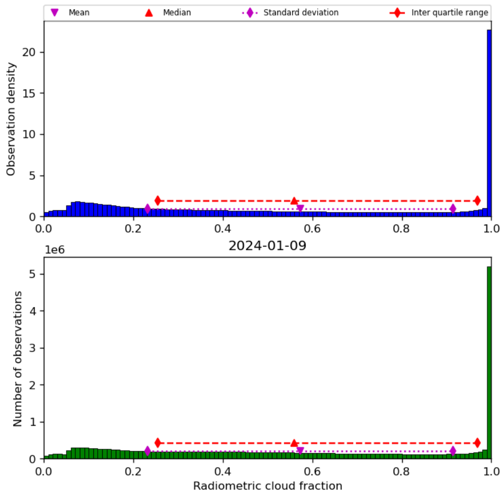
Figure 39: Histogram of “Radiometric cloud fraction” for 2024-01-08 to 2024-01-10
