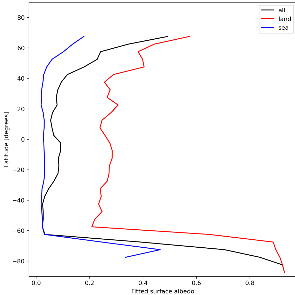
Figure 29: Zonal average of “Fitted surface albedo” for 2024-01-08 to 2024-01-10.
