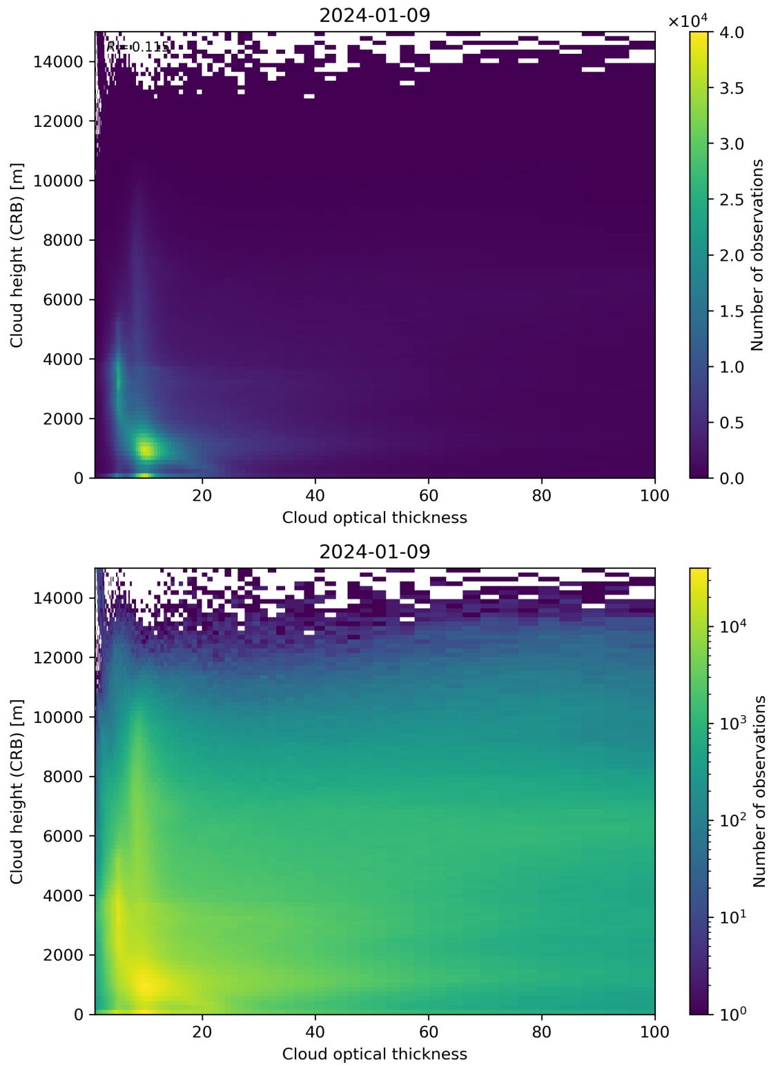
Figure 85: Scatter density plot of “Cloud optical thickness” against “Cloud height (CRB)” for 2024-01-08 to 2024-01-10.
