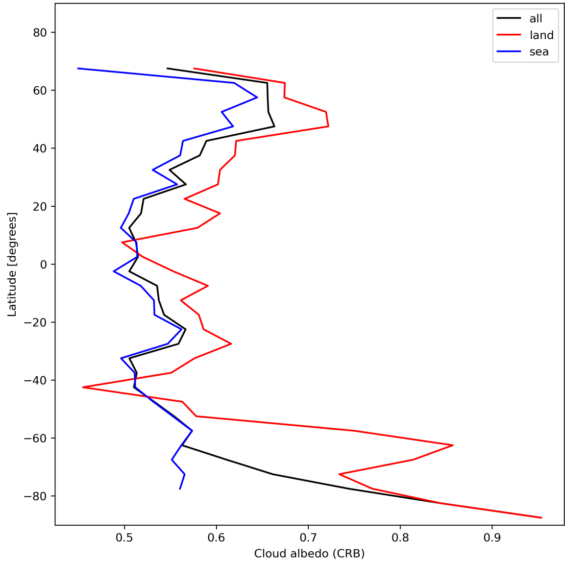
Figure 28: Zonal average of “Cloud albedo (CRB)” for 2024-01-08 to 2024-01-10.
