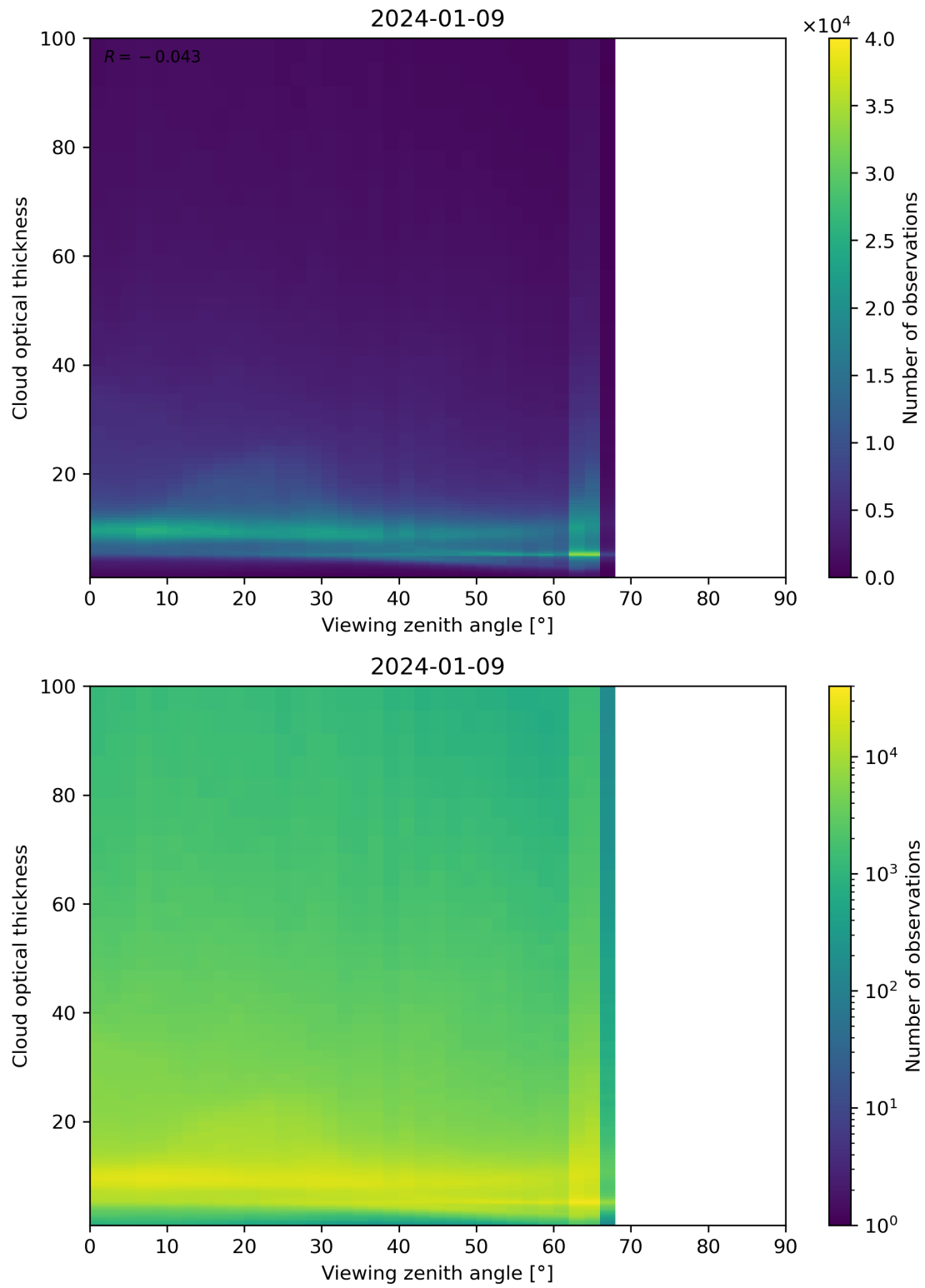
Figure 111: Scatter density plot of “Viewing zenith angle” against “Cloud optical thickness” for 2024-01-08 to 2024-01-10.
