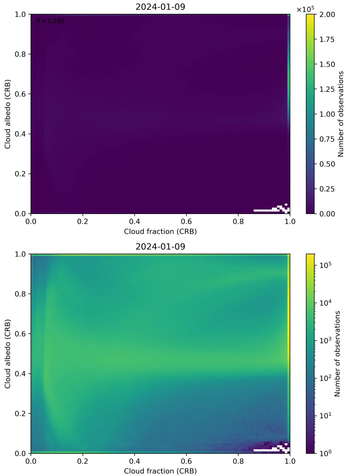
Figure 77: Scatter density plot of “Cloud fraction (CRB)” against “Cloud albedo (CRB)” for 2024-01-08 to 2024-01-10.
