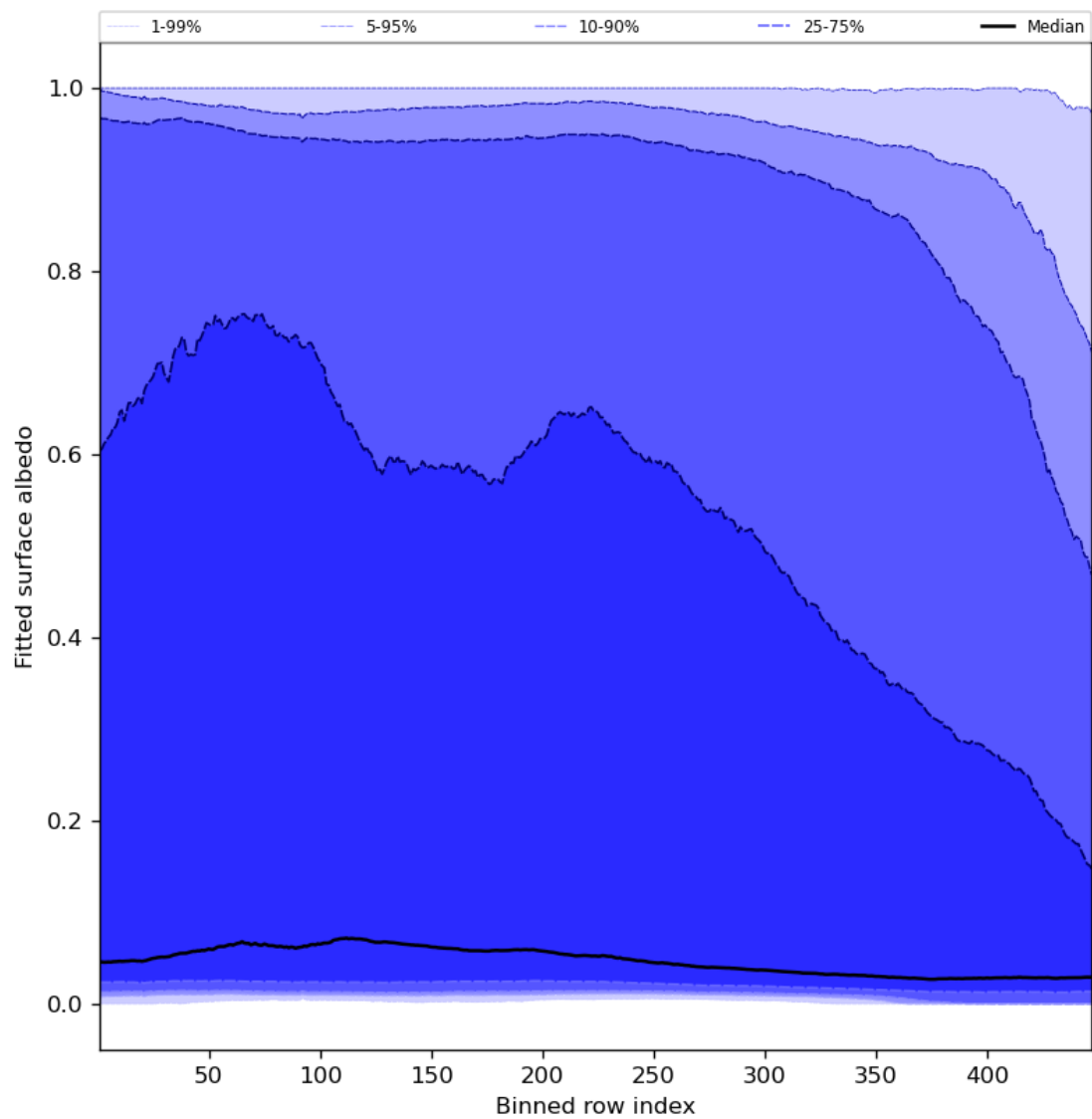
Figure 61: Along track statistics of “Fitted surface albedo” for 2024-01-08 to 2024-01-10
