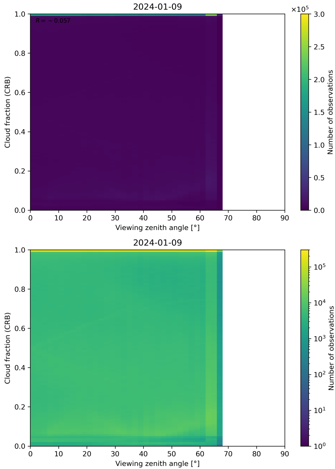
Figure 109: Scatter density plot of “Viewing zenith angle” against “Cloud fraction (CRB)” for 2024-01-08 to 2024-01-10.
