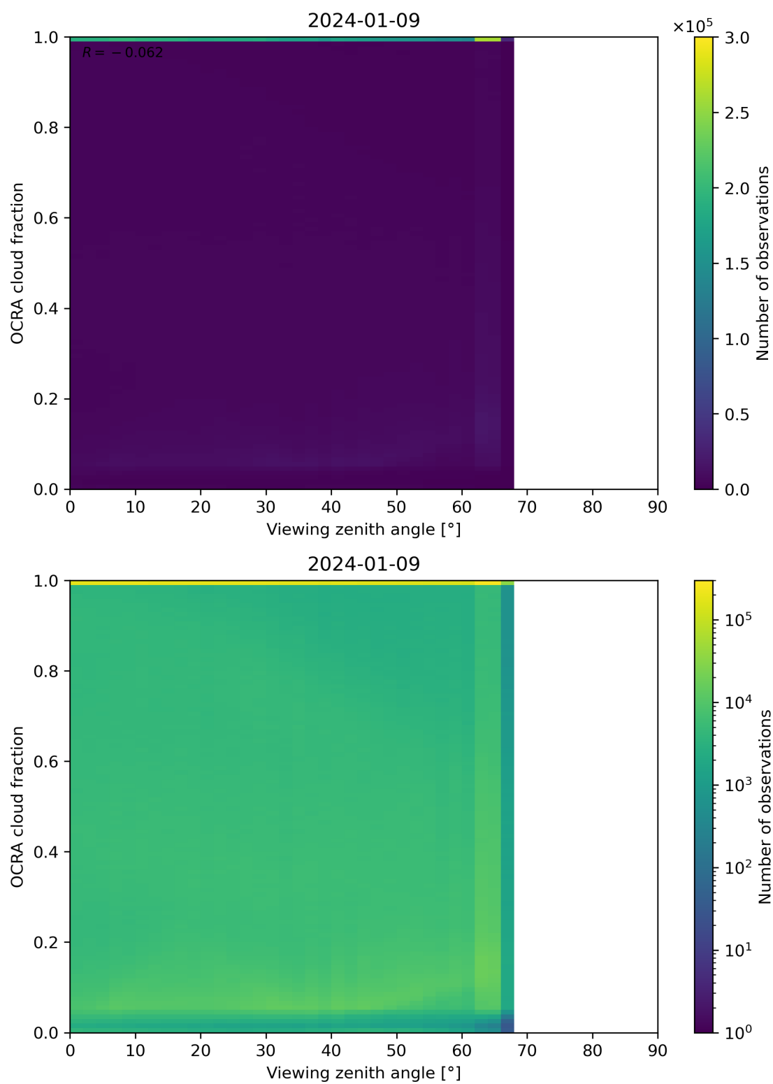
Figure 108: Scatter density plot of “Viewing zenith angle” against “OCRA cloud fraction” for 2024-01-08 to 2024-01-10.
