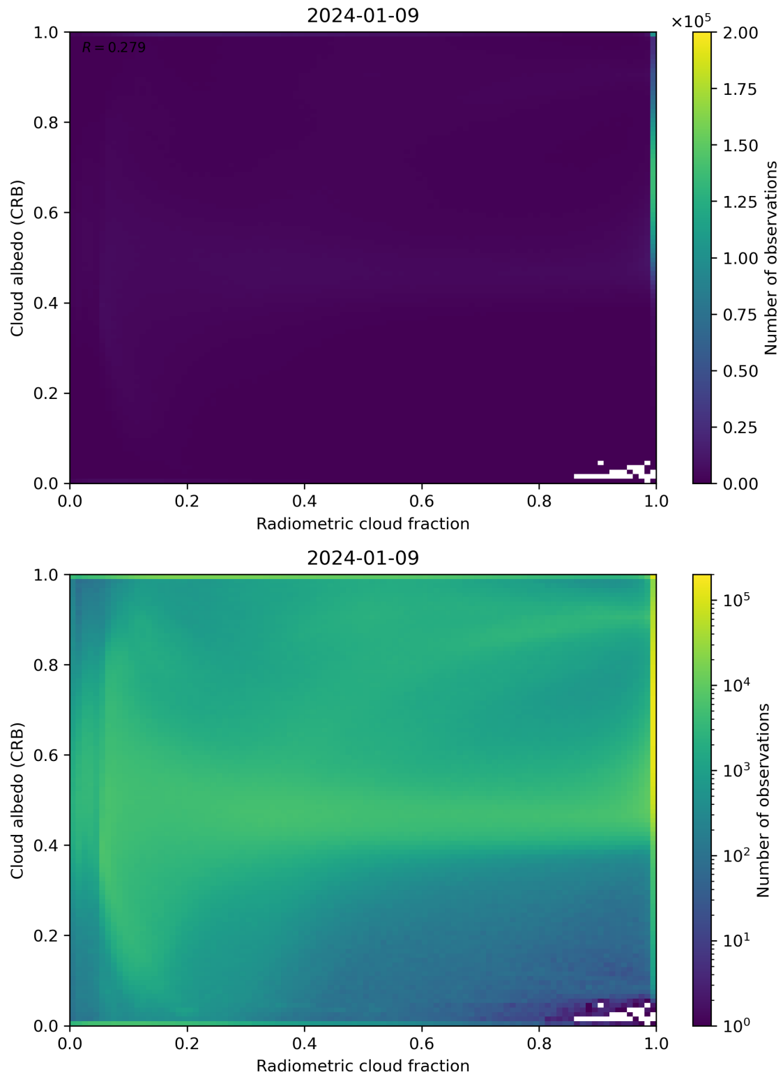
Figure 71: Scatter density plot of “Radiometric cloud fraction” against “Cloud albedo (CRB)” for 2024-01-08 to 2024-01-10.
