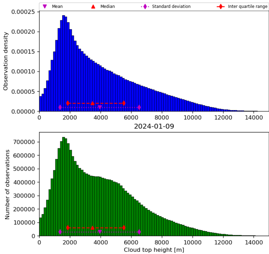
Figure 40: Histogram of “Cloud top height” for 2024-01-08 to 2024-01-10
