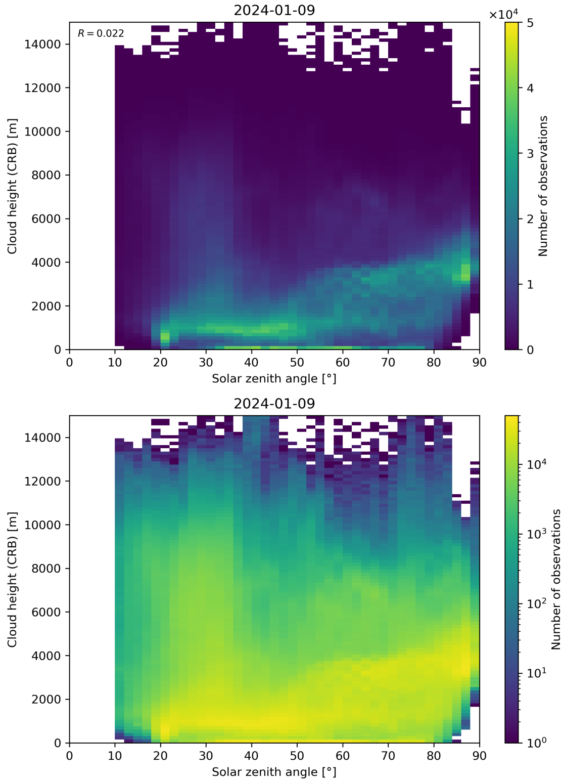
Figure 102: Scatter density plot of “Solar zenith angle” against “Cloud height (CRB)” for 2024-01-08 to 2024-01-10.
