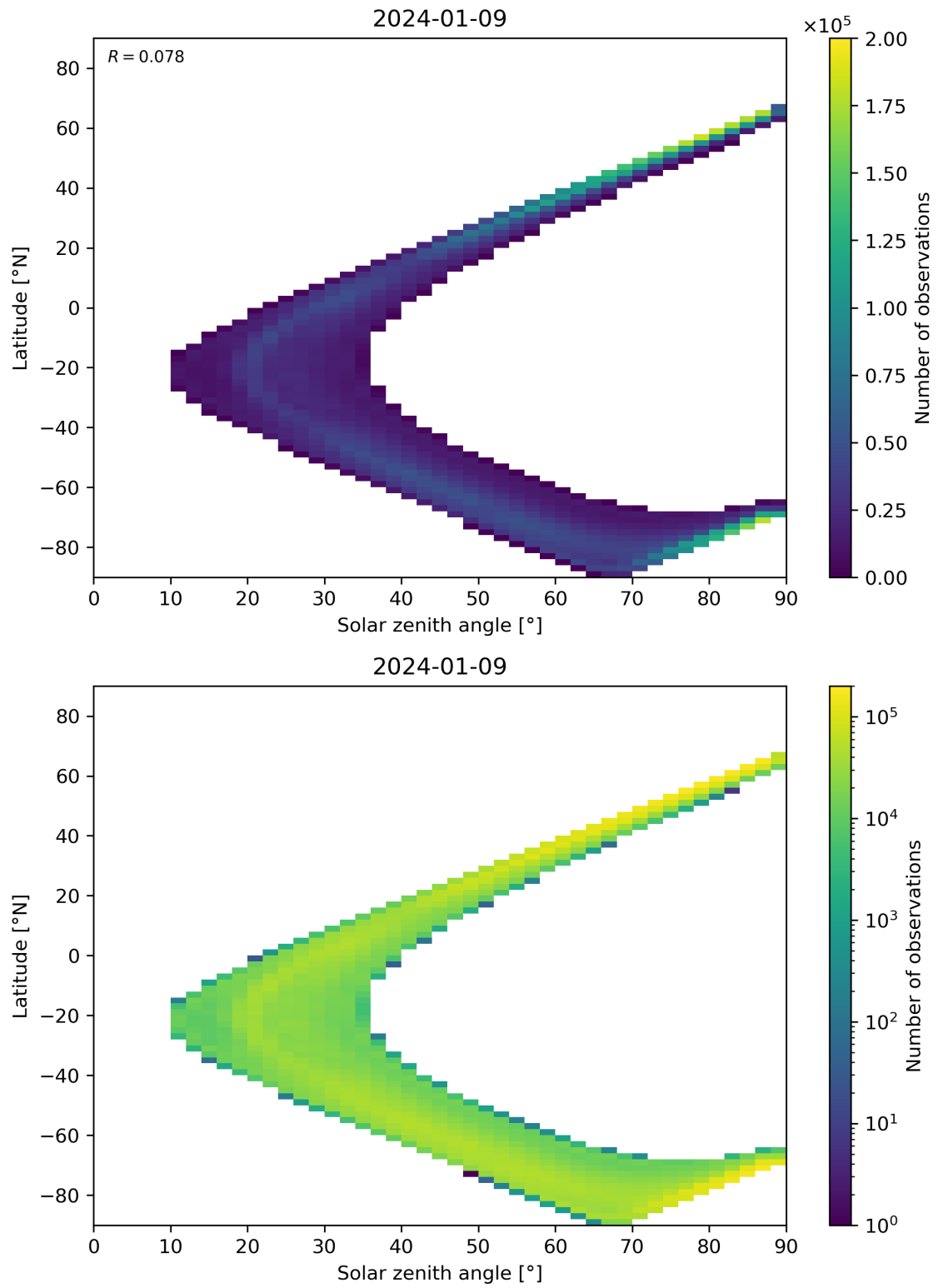
Figure 105: Scatter density plot of “Solar zenith angle” against “Latitude” for 2024-01-08 to 2024-01-10.
