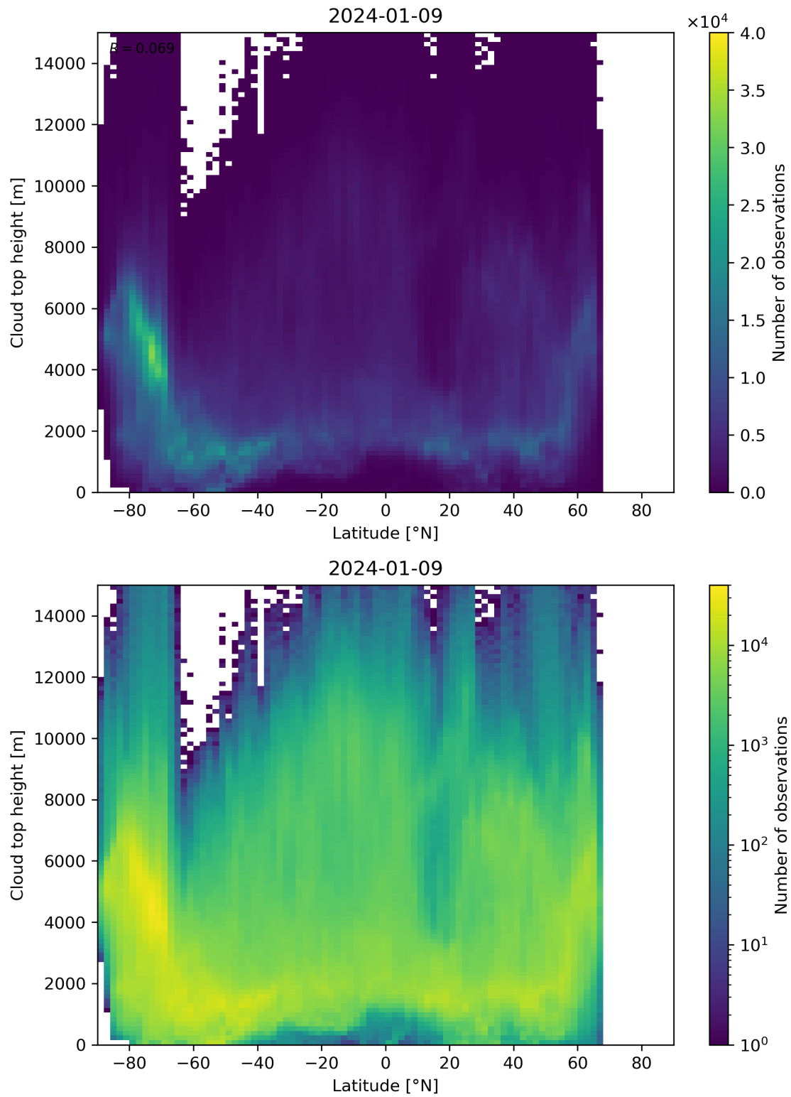
Figure 97: Scatter density plot of “Latitude” against “Cloud top height” for 2024-01-08 to 2024-01-10.
