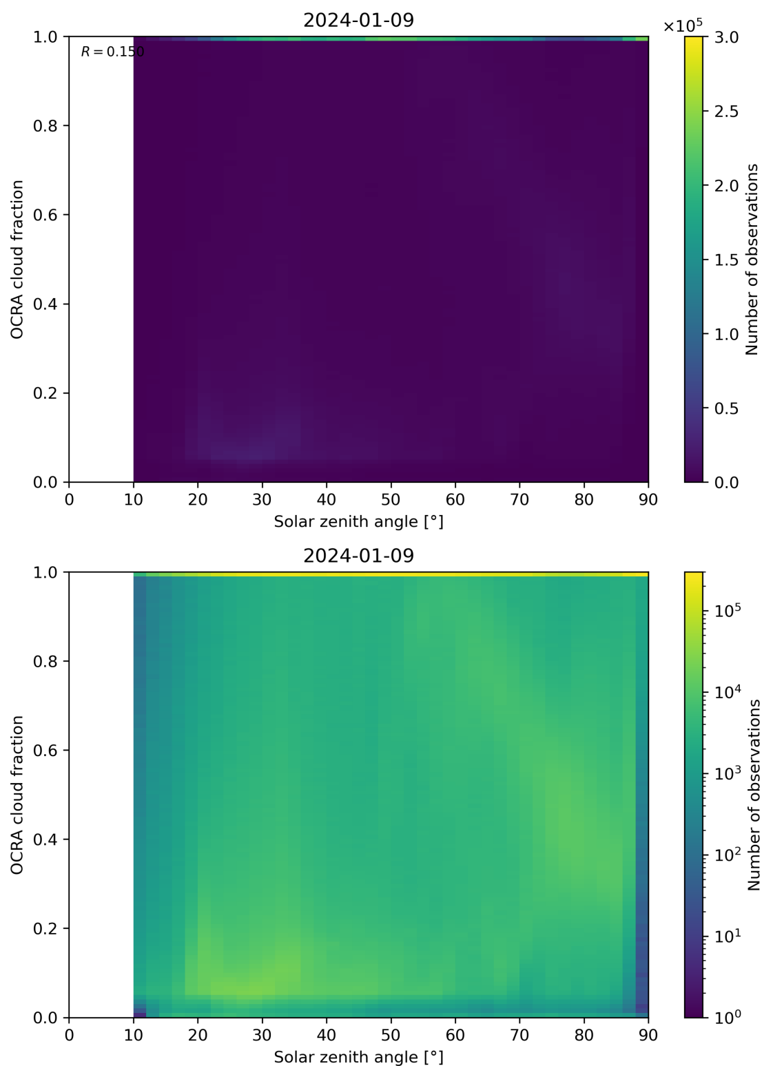
Figure 100: Scatter density plot of “Solar zenith angle” against “OCRA cloud fraction” for 2024-01-08 to 2024-01-10.
