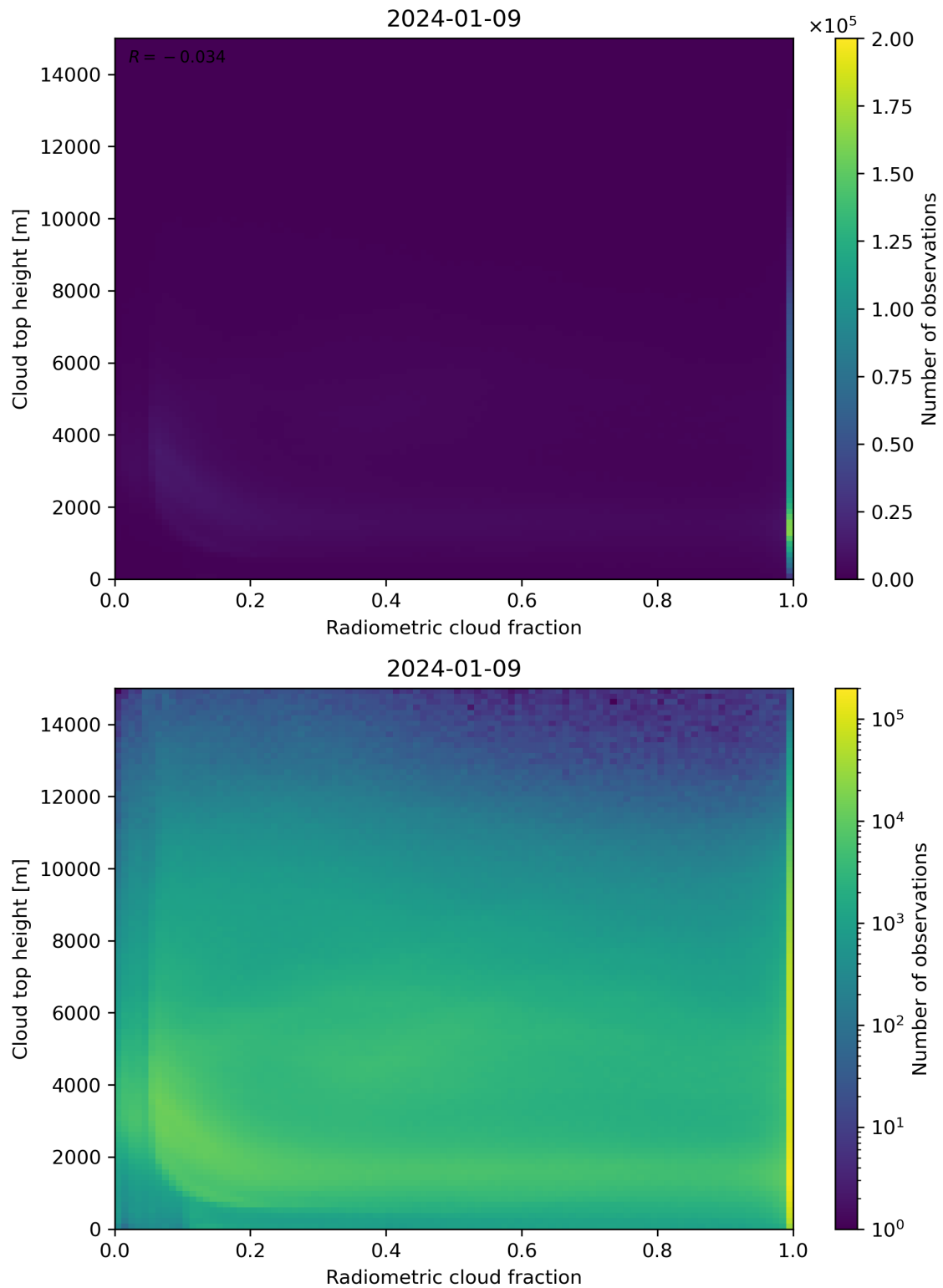
Figure 76: Scatter density plot of “Radiometric cloud fraction” against “Cloud top height” for 2024-01-08 to 2024-01-10.
