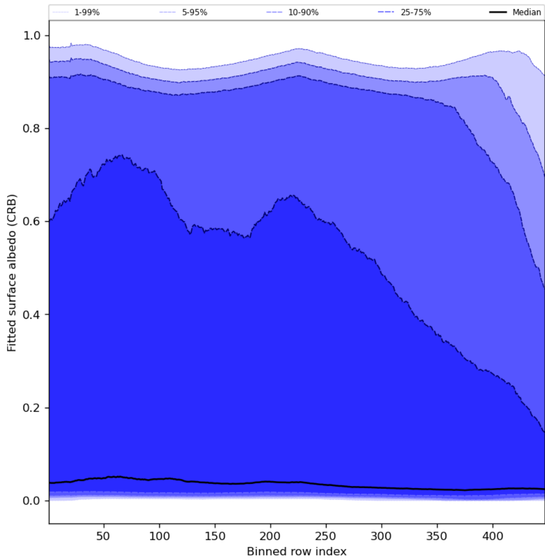
Figure 62: Along track statistics of “Fitted surface albedo (CRB)” for 2024-01-08 to 2024-01-10
