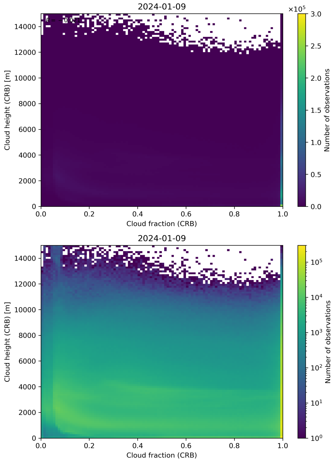
Figure 79: Scatter density plot of “Cloud fraction (CRB)” against “Cloud height (CRB)” for 2024-01-08 to 2024-01-10.
