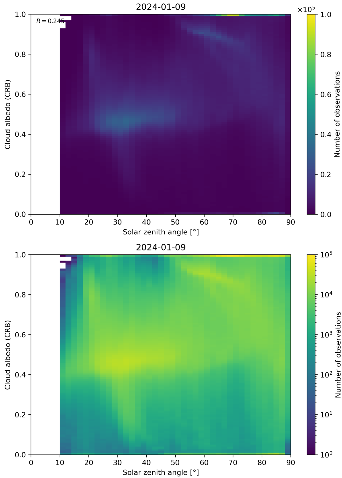
Figure 98: Scatter density plot of “Solar zenith angle” against “Cloud albedo (CRB)” for 2024-01-08 to 2024-01-10.
