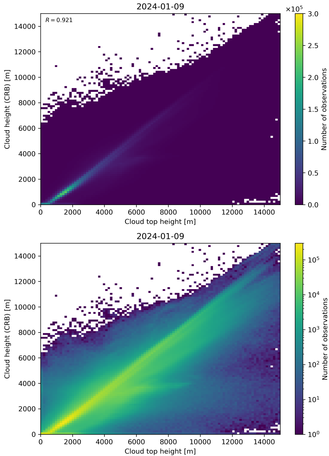
Figure 89: Scatter density plot of “Cloud top height” against “Cloud height (CRB)” for 2024-01-08 to 2024-01-10.
