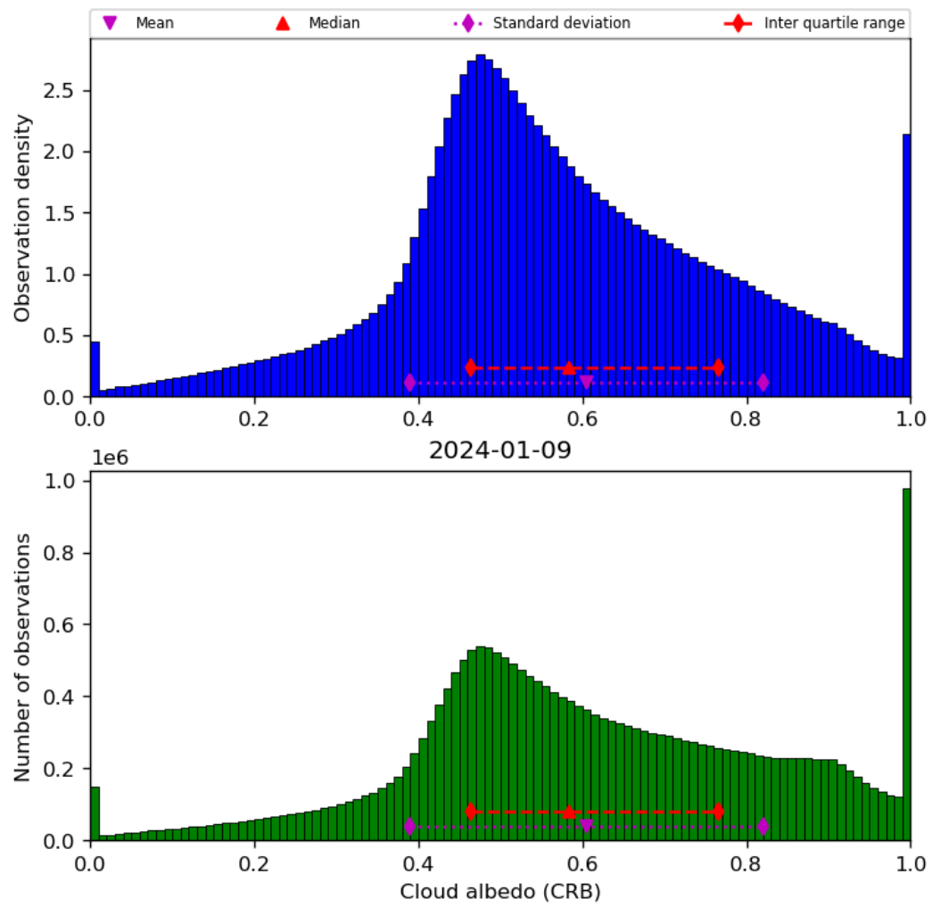
Figure 44: Histogram of “Cloud albedo (CRB)” for 2024-01-08 to 2024-01-10
