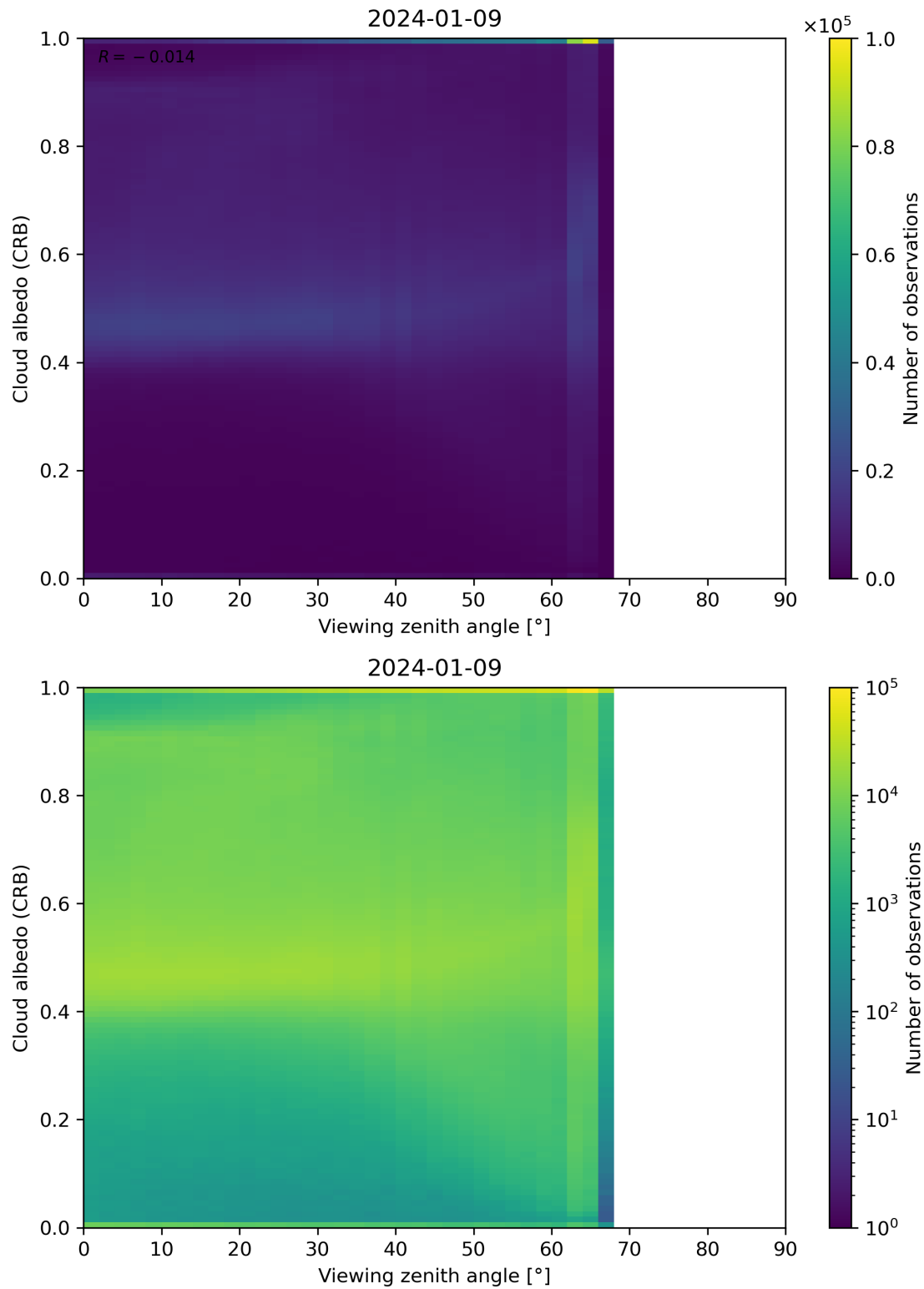
Figure 106: Scatter density plot of “Viewing zenith angle” against “Cloud albedo (CRB)” for 2024-01-08 to 2024-01-10.
