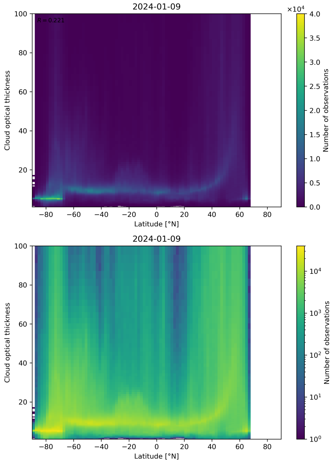
Figure 96: Scatter density plot of “Latitude” against “Cloud optical thickness” for 2024-01-08 to 2024-01-10.
