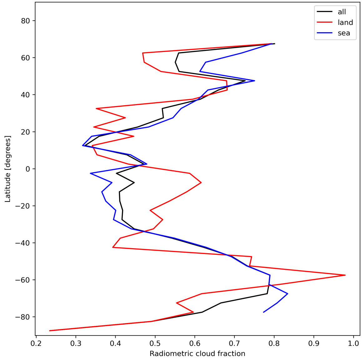
Figure 23: Zonal average of “Radiometric cloud fraction” for 2024-01-08 to 2024-01-10.
