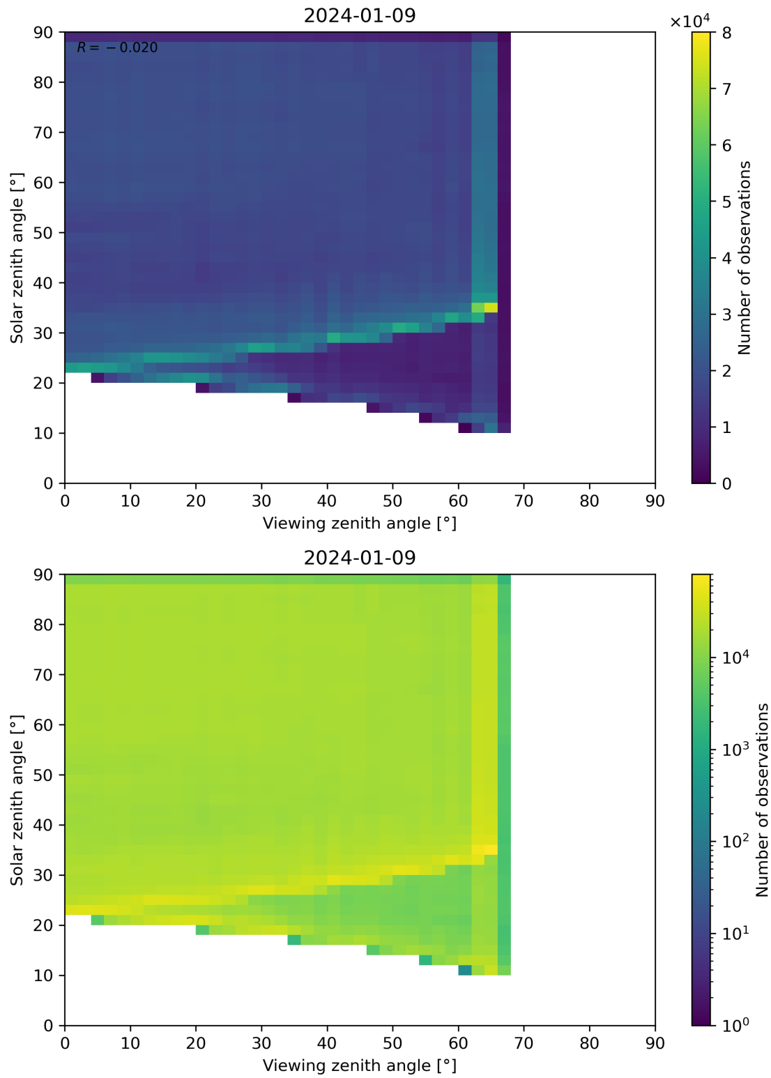
Figure 114: Scatter density plot of “Viewing zenith angle” against “Solar zenith angle” for 2024-01-08 to 2024-01-10.
