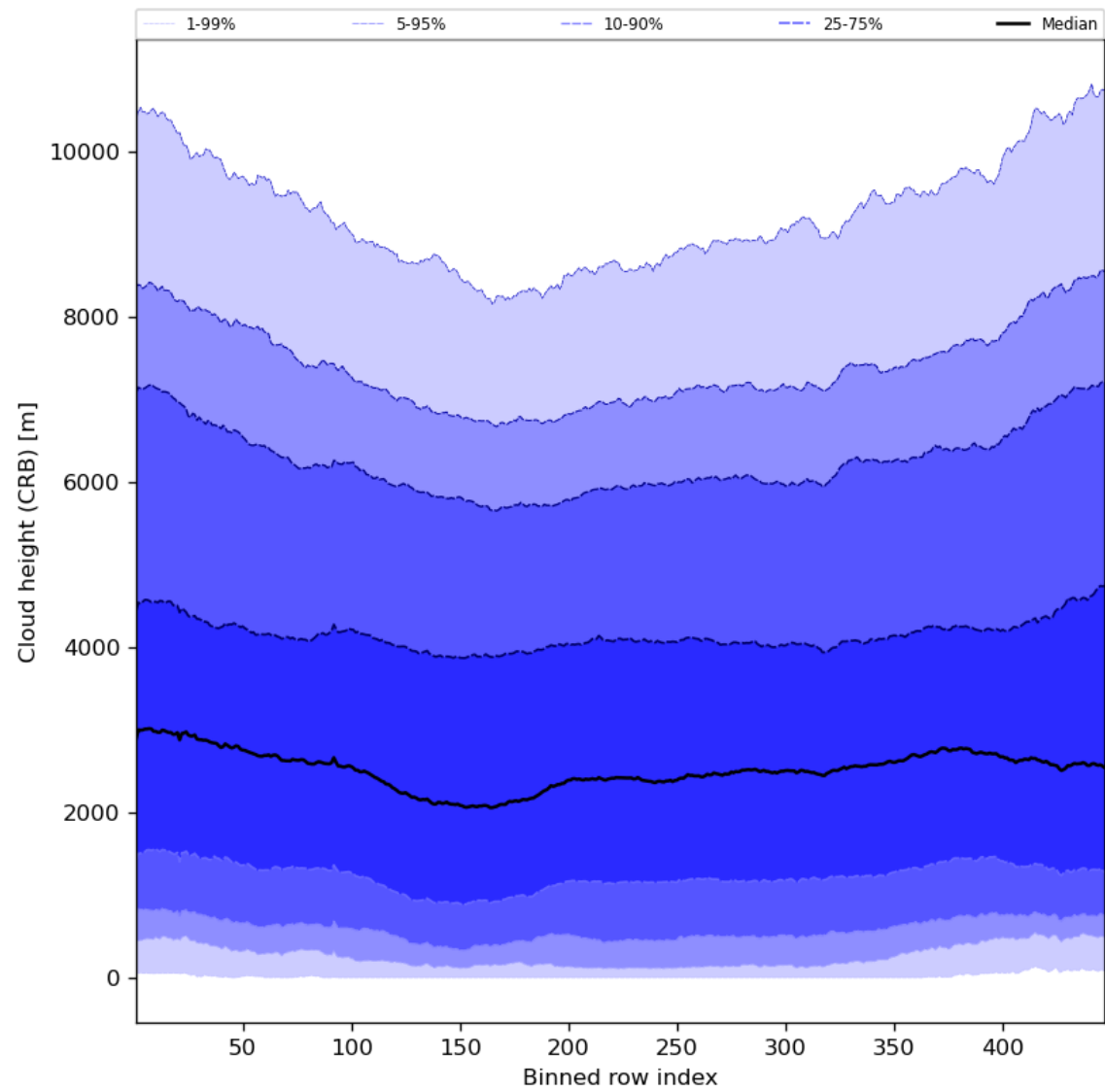
Figure 59: Along track statistics of “Cloud height (CRB)” for 2024-01-08 to 2024-01-10
