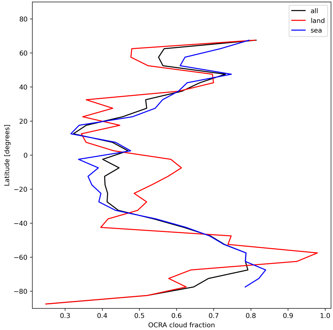
Figure 34: Zonal average of “OCRA cloud fraction” for 2024-01-08 to 2024-01-10.
