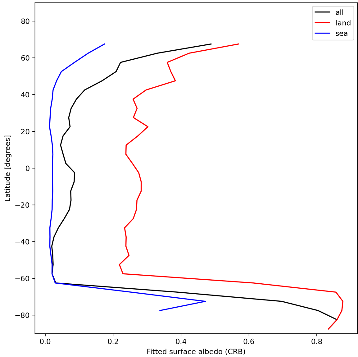
Figure 30: Zonal average of “Fitted surface albedo (CRB)” for 2024-01-08 to 2024-01-10.
