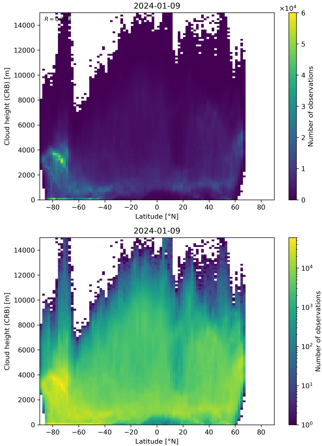
Figure 95: Scatter density plot of “Latitude” against “Cloud height (CRB)” for 2024-01-08 to 2024-01-10.
