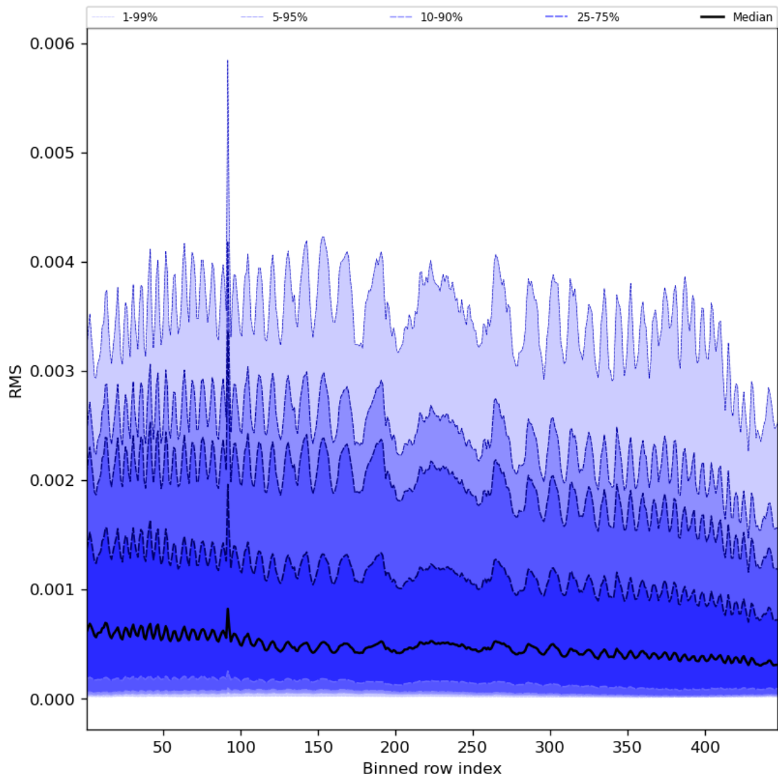
Figure 63: Along track statistics of “RMS” for 2024-01-10 to 2024-01-11
