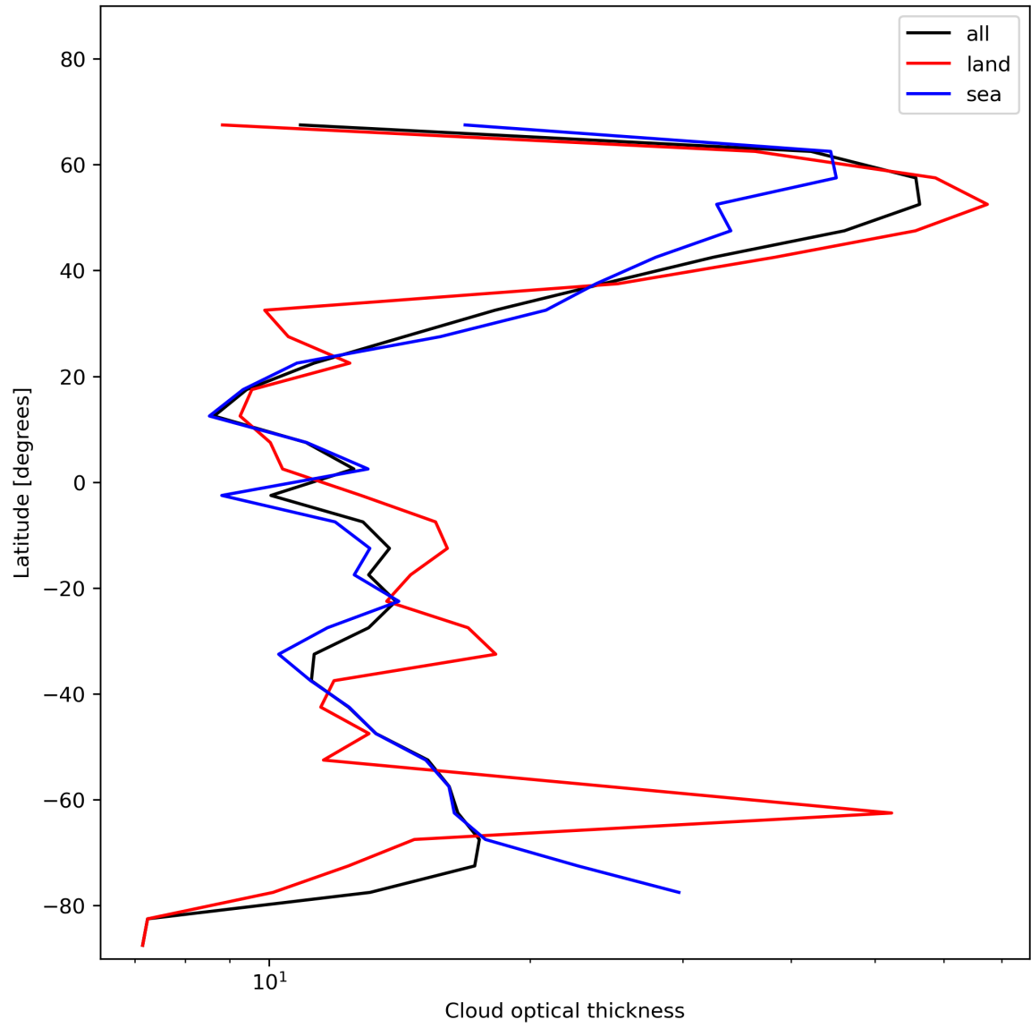
Figure 25: Zonal average of “Cloud optical thickness” for 2024-01-10 to 2024-01-11.
