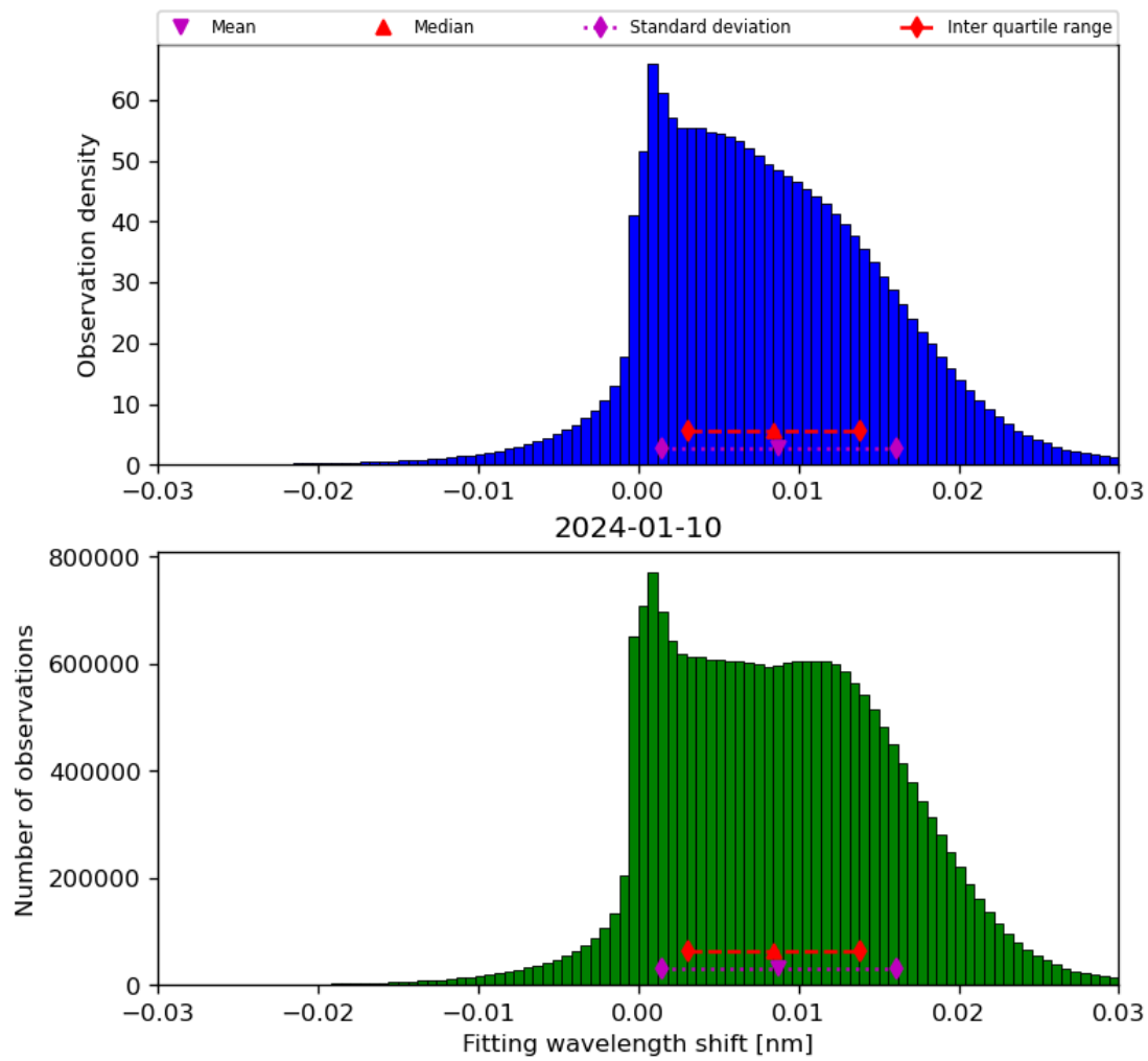
Figure 49: Histogram of “Fitting wavelength shift” for 2024-01-10 to 2024-01-11
