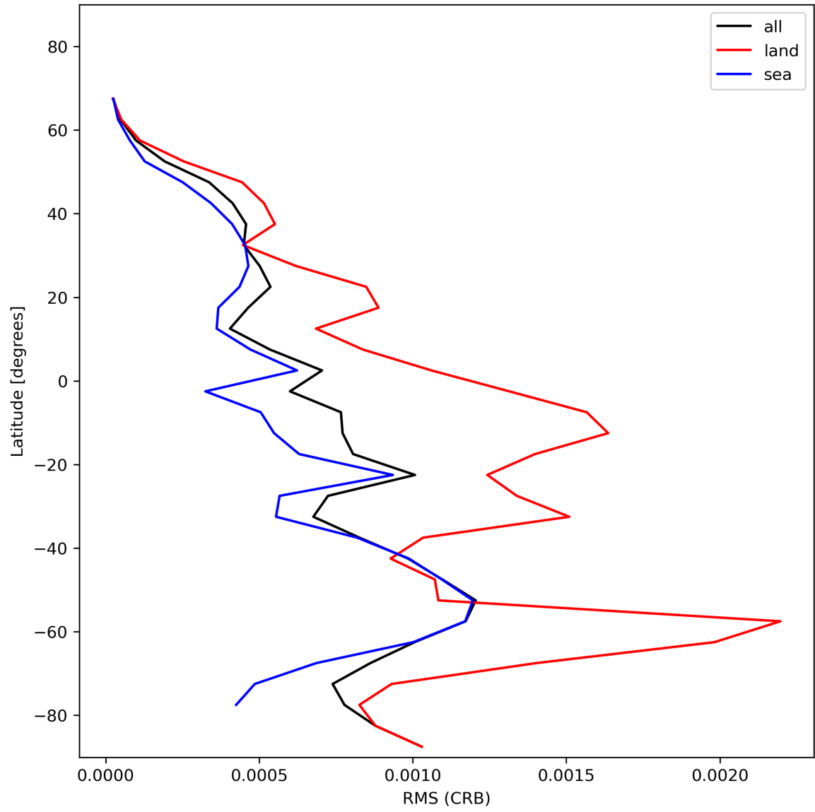
Figure 32: Zonal average of “RMS (CRB)” for 2024-01-10 to 2024-01-11.
