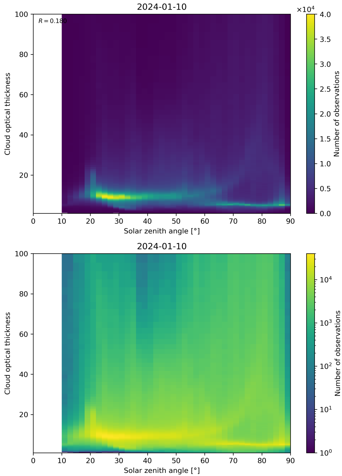
Figure 103: Scatter density plot of “Solar zenith angle” against “Cloud optical thickness” for 2024-01-10 to 2024-01-11.
