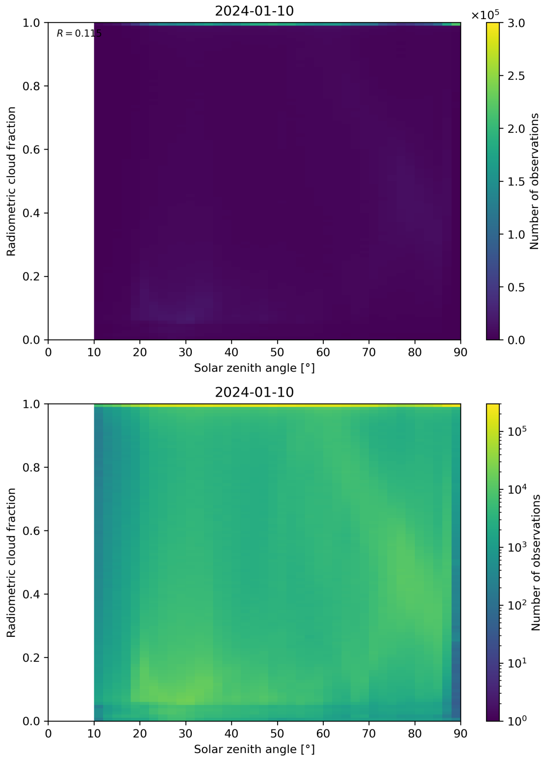
Figure 99: Scatter density plot of “Solar zenith angle” against “Radiometric cloud fraction” for 2024-01-10 to 2024-01-11.
