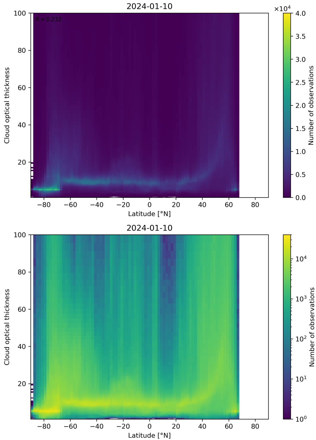
Figure 96: Scatter density plot of “Latitude” against “Cloud optical thickness” for 2024-01-10 to 2024-01-11.
