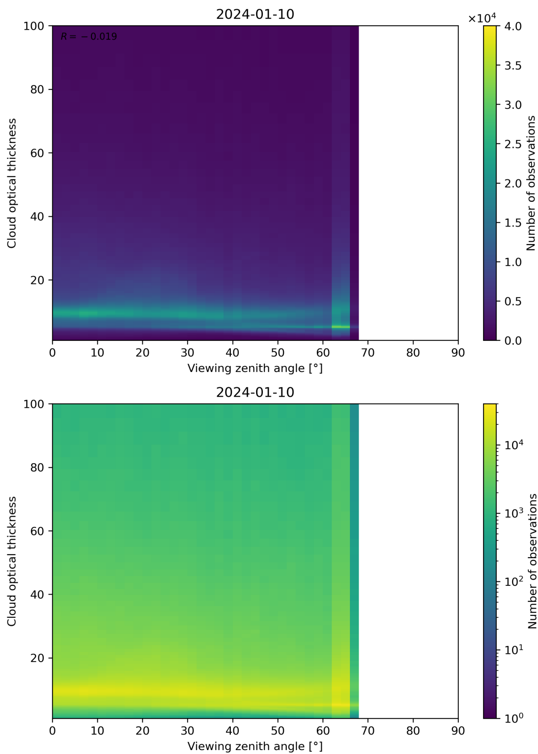
Figure 111: Scatter density plot of “Viewing zenith angle” against “Cloud optical thickness” for 2024-01-10 to 2024-01-11.
