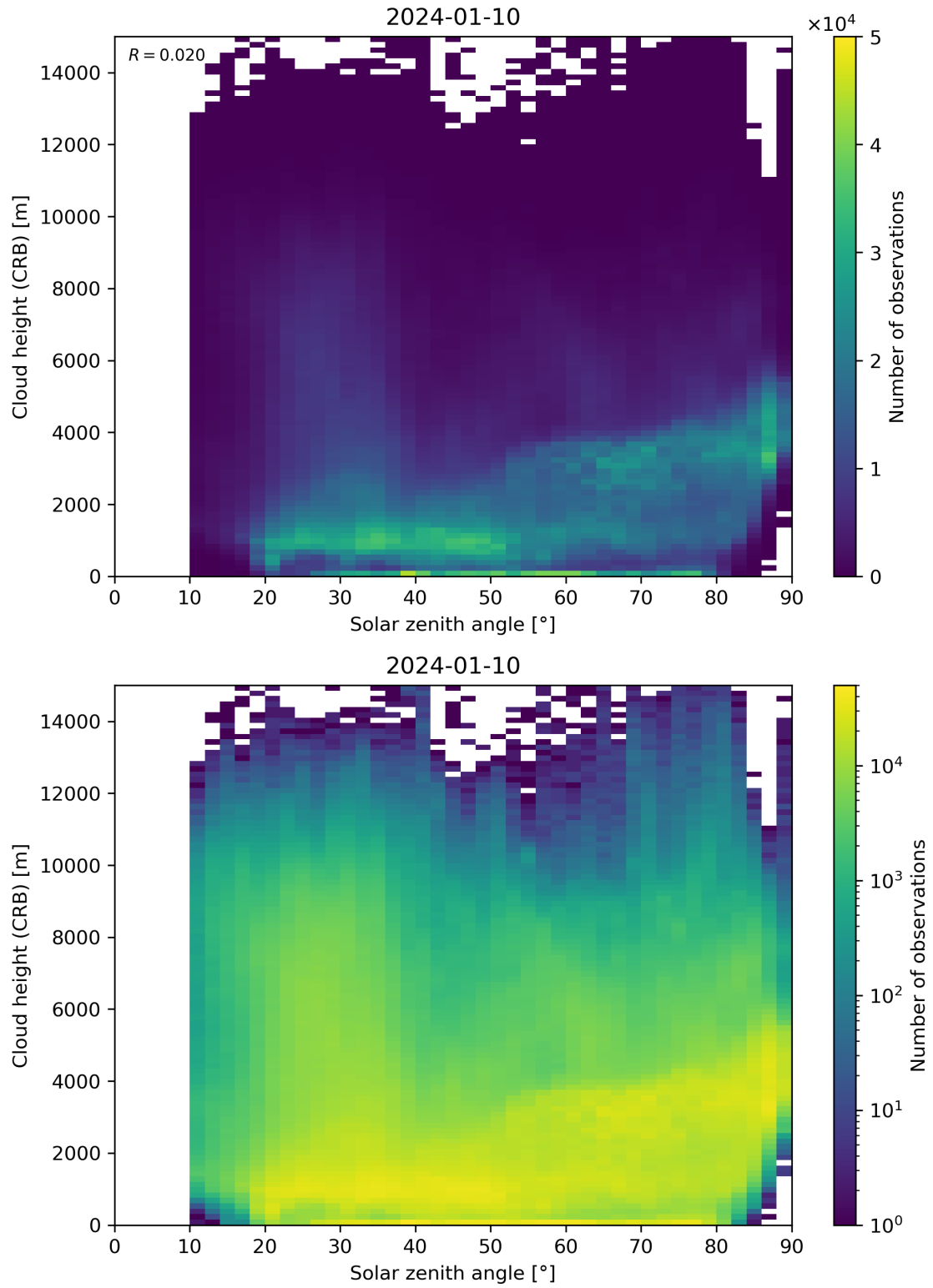
Figure 102: Scatter density plot of “Solar zenith angle” against “Cloud height (CRB)” for 2024-01-10 to 2024-01-11.
