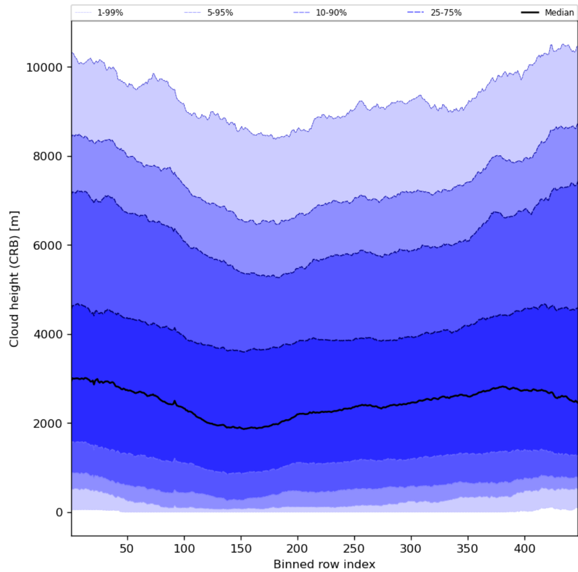
Figure 59: Along track statistics of “Cloud height (CRB)” for 2024-01-10 to 2024-01-11
