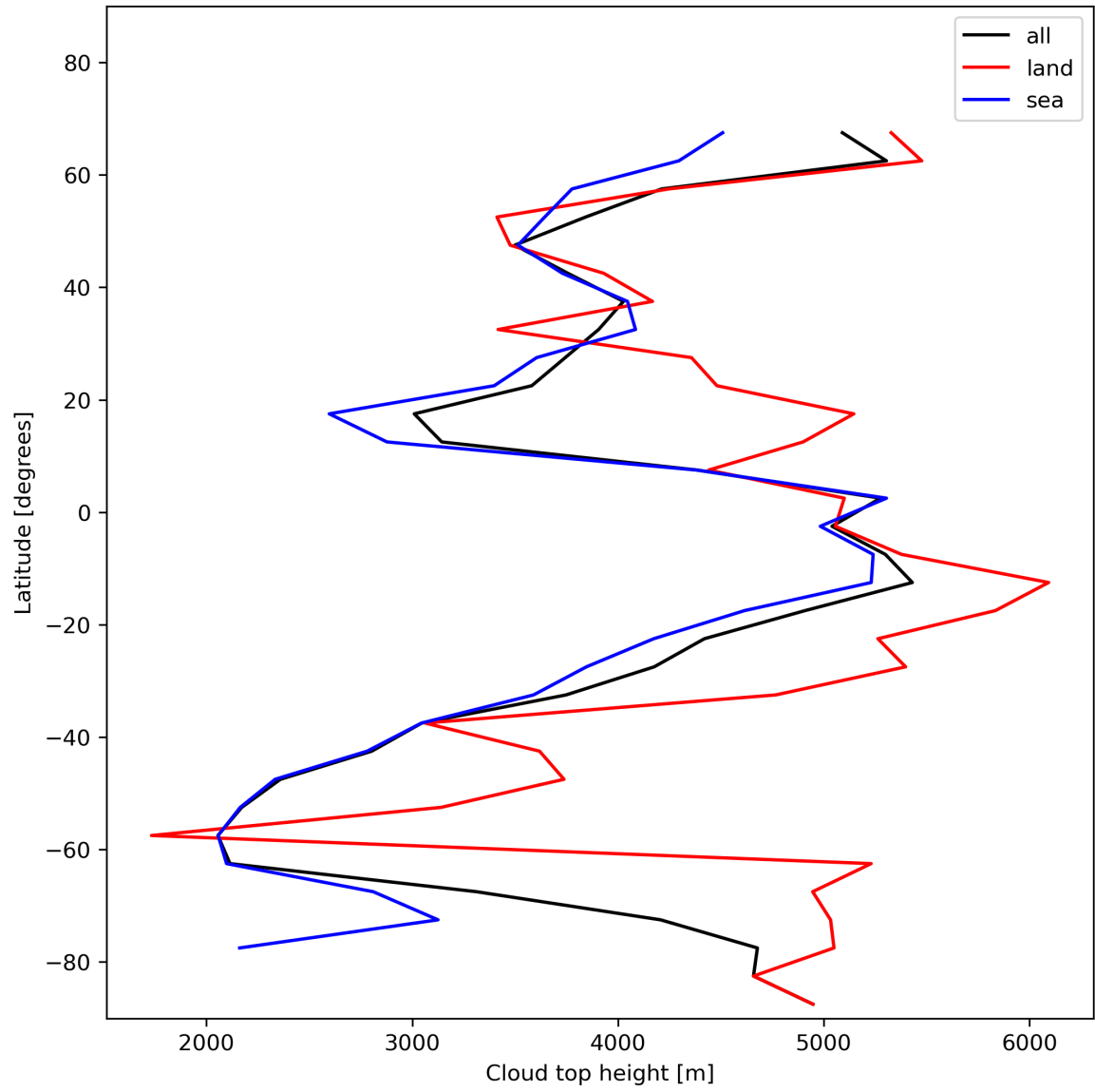
Figure 24: Zonal average of “Cloud top height” for 2024-01-10 to 2024-01-11.
