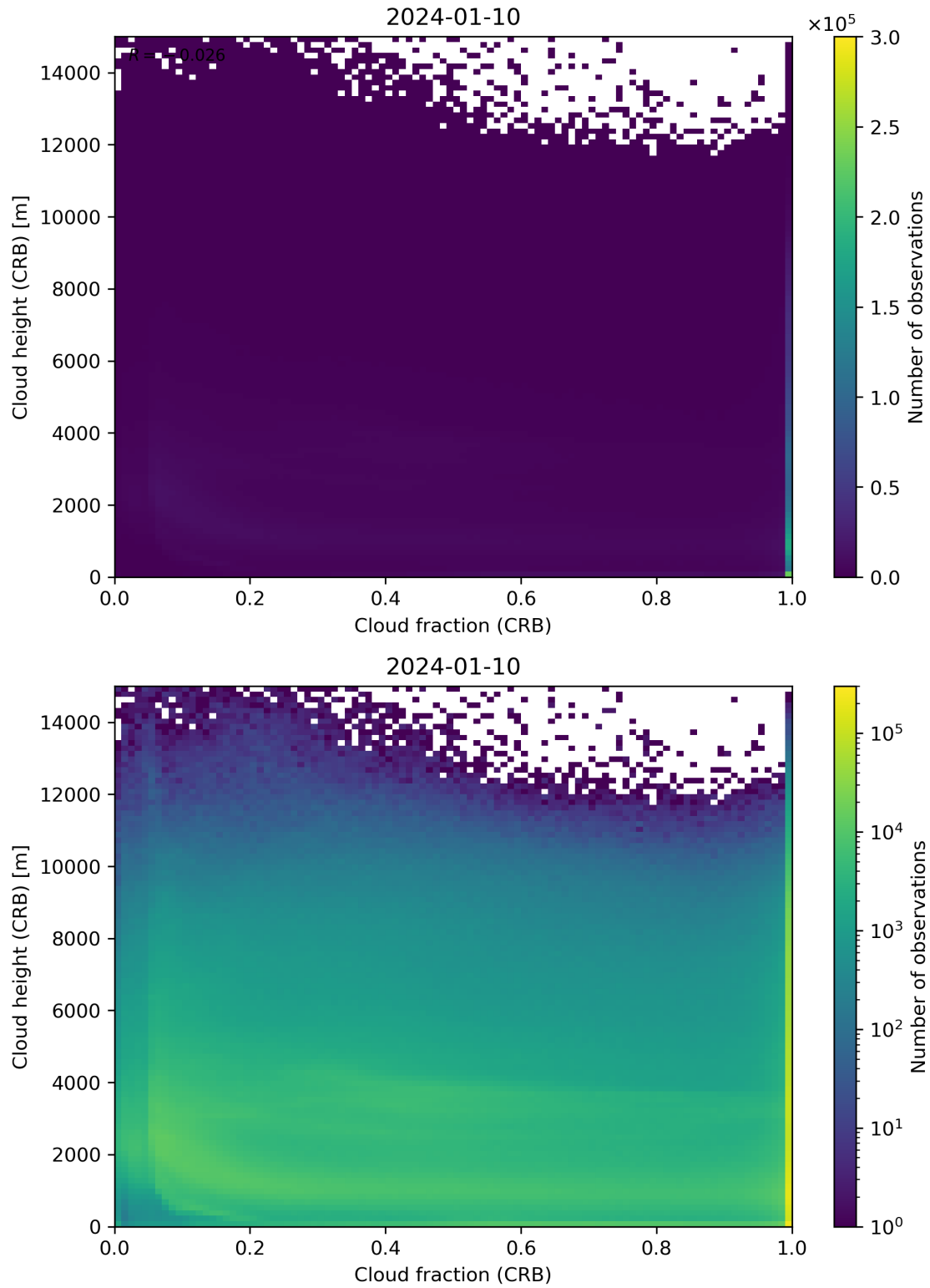
Figure 79: Scatter density plot of “Cloud fraction (CRB)” against “Cloud height (CRB)” for 2024-01-10 to 2024-01-11.
