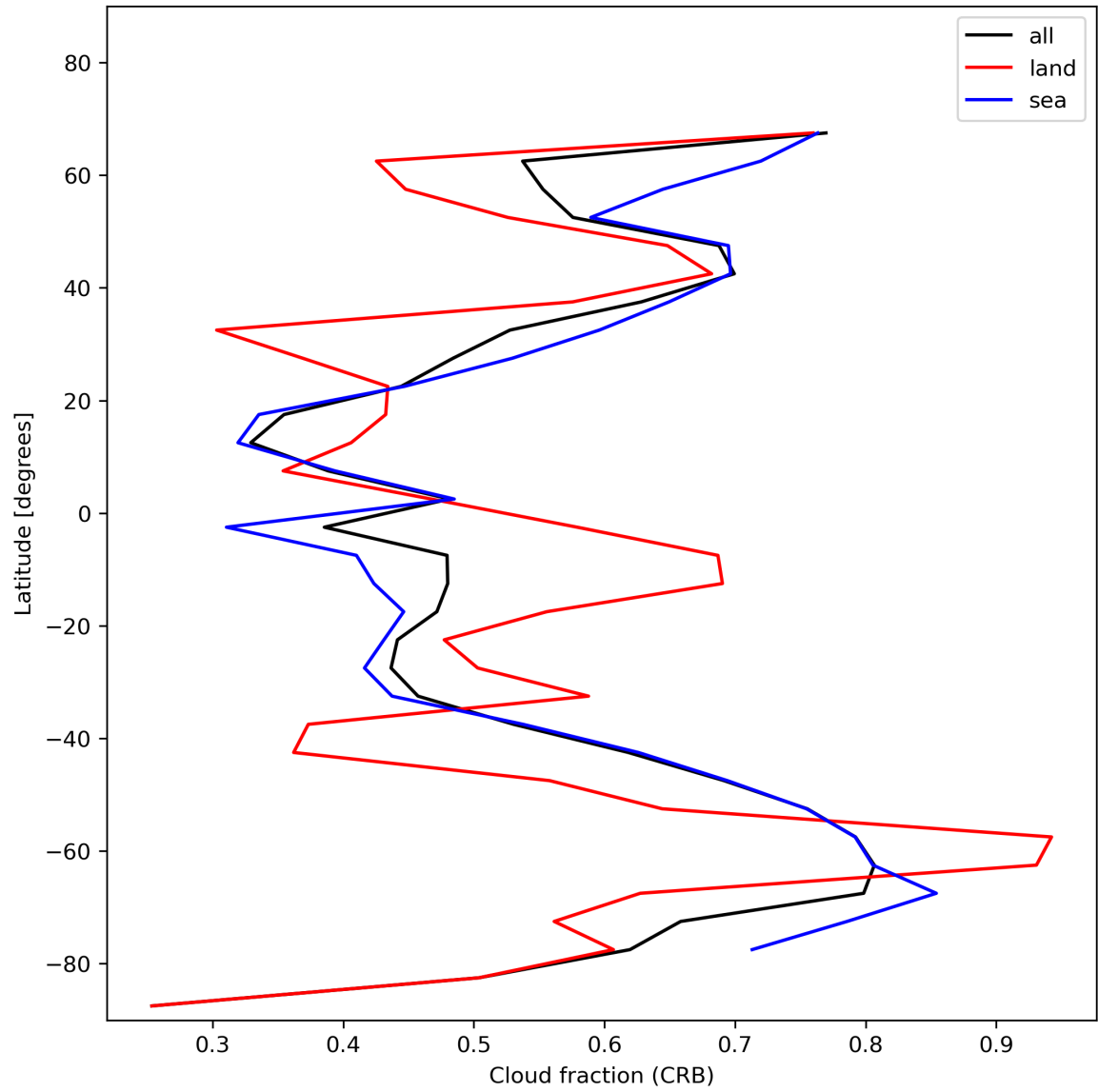
Figure 26: Zonal average of “Cloud fraction (CRB)” for 2024-01-10 to 2024-01-11.
