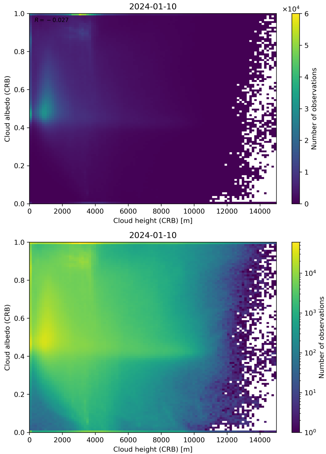
Figure 80: Scatter density plot of “Cloud height (CRB)” against “Cloud albedo (CRB)” for 2024-01-10 to 2024-01-11.
