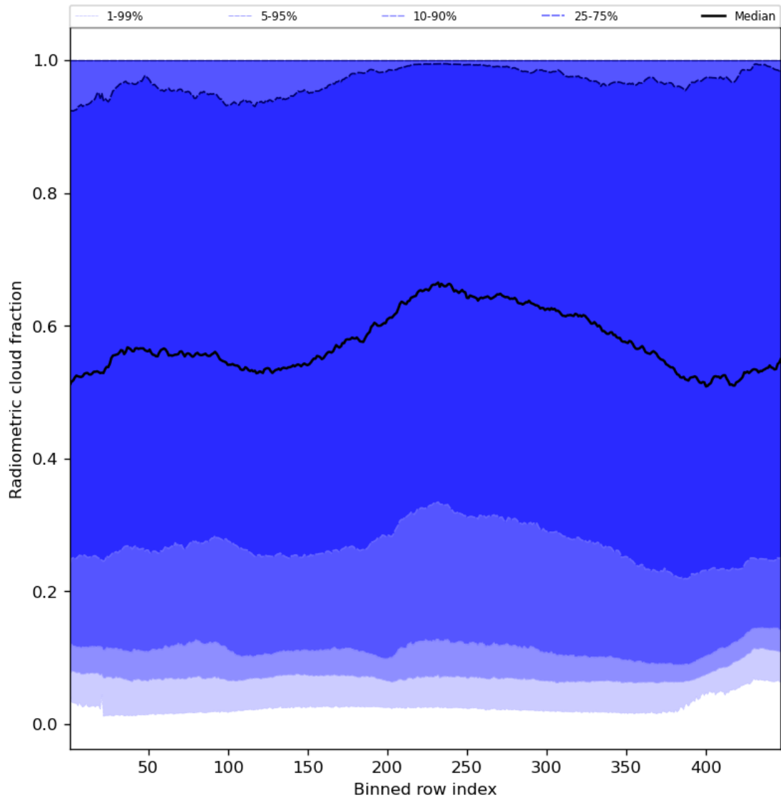
Figure 55: Along track statistics of “Radiometric cloud fraction” for 2024-01-10 to 2024-01-11
