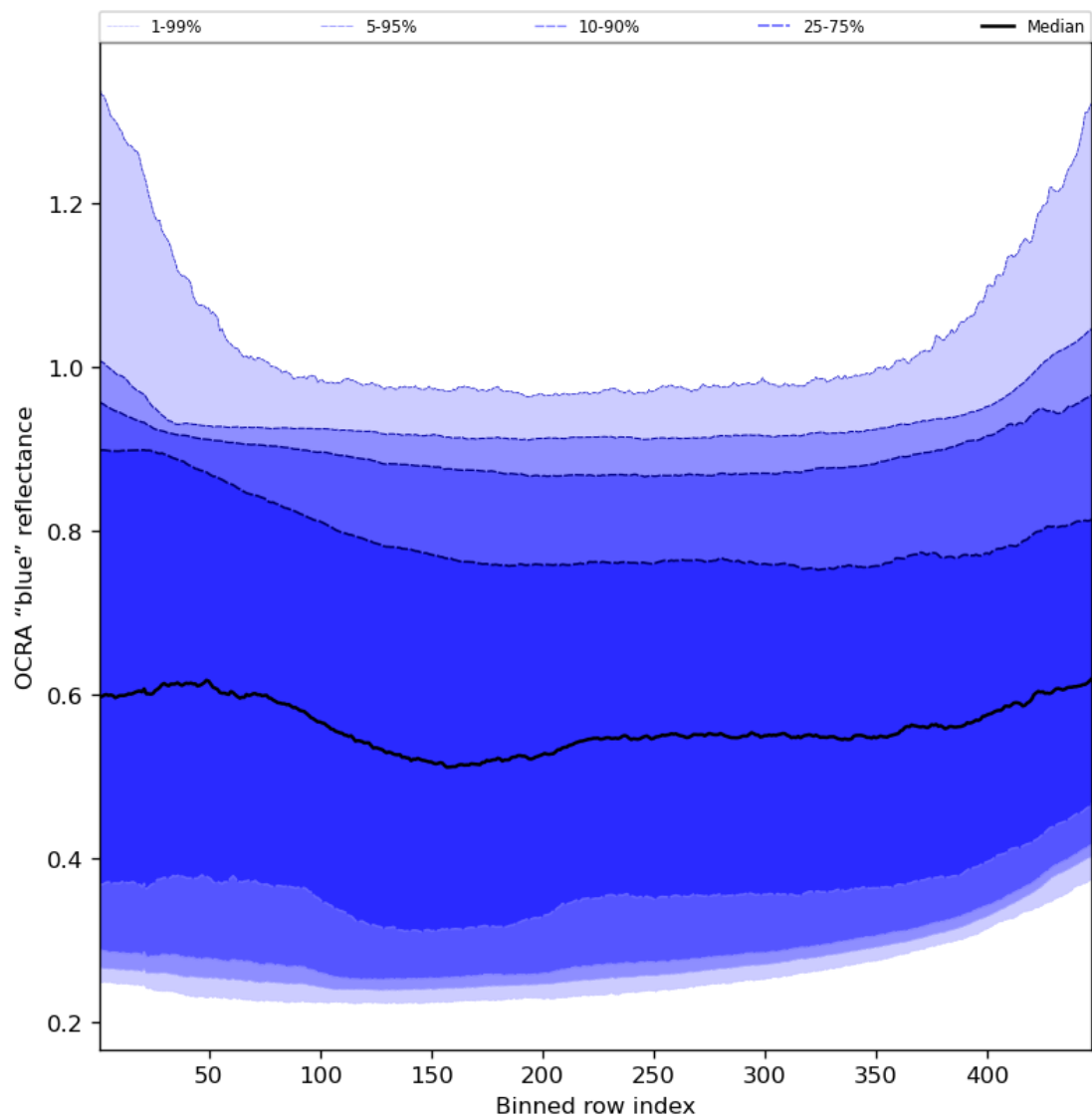
Figure 67: Along track statistics of “OCRA “blue” reflectance” for 2024-01-10 to 2024-01-11
