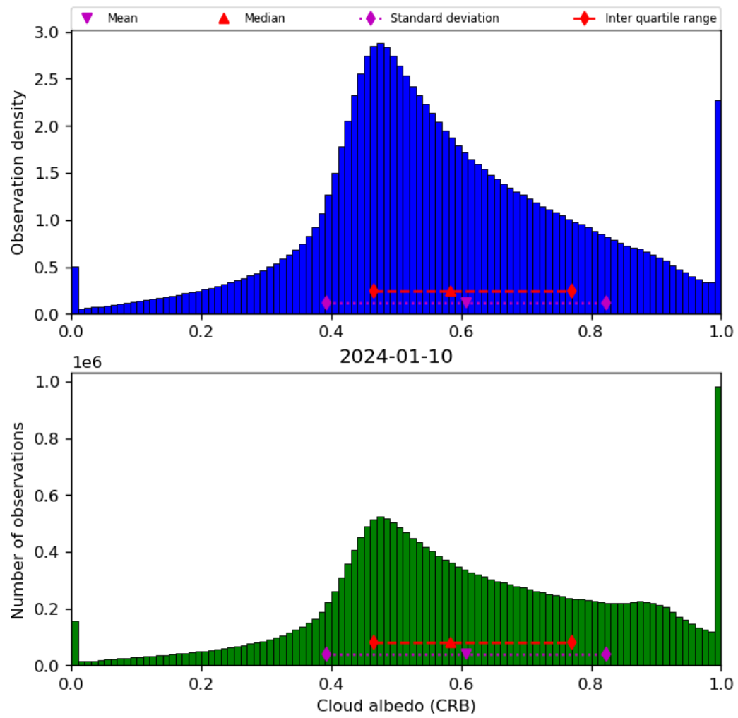
Figure 44: Histogram of “Cloud albedo (CRB)” for 2024-01-10 to 2024-01-11
