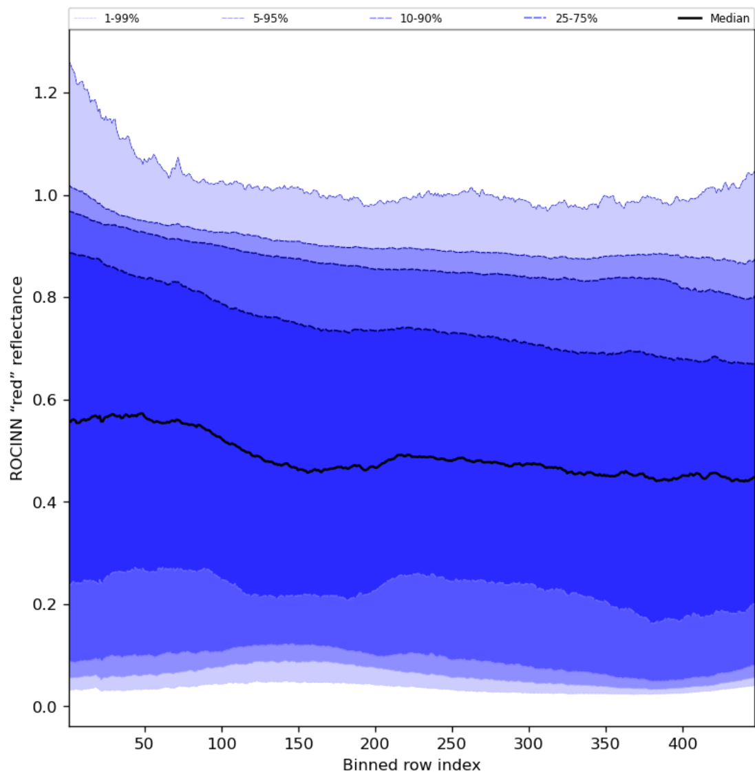
Figure 69: Along track statistics of “ROCINN “red” reflectance” for 2024-01-10 to 2024-01-11
