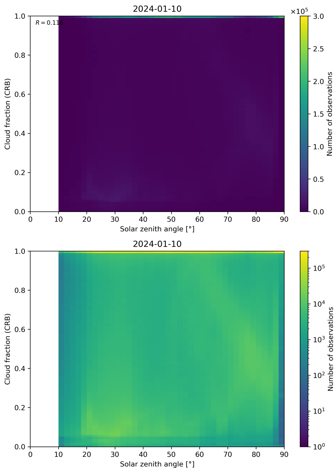
Figure 101: Scatter density plot of “Solar zenith angle” against “Cloud fraction (CRB)” for 2024-01-10 to 2024-01-11.
