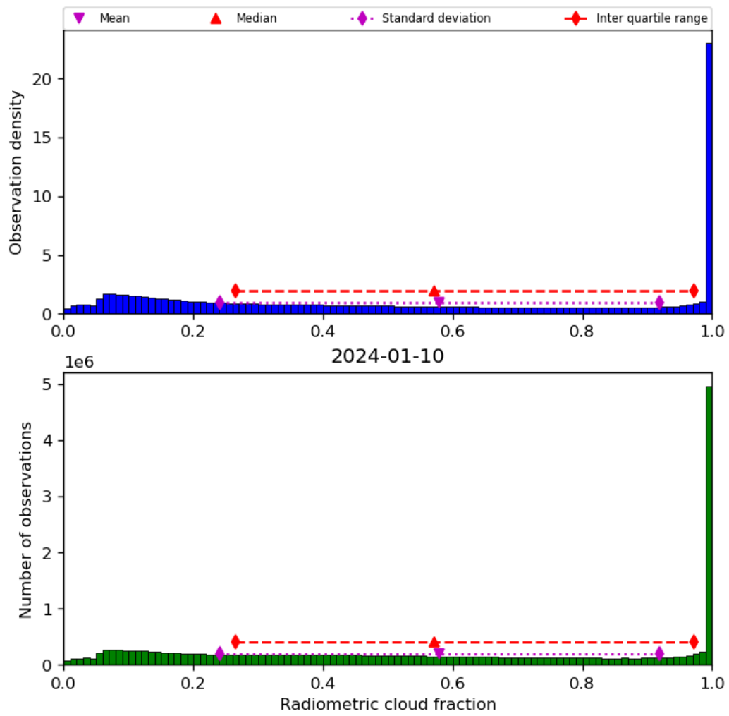
Figure 39: Histogram of “Radiometric cloud fraction” for 2024-01-10 to 2024-01-11
