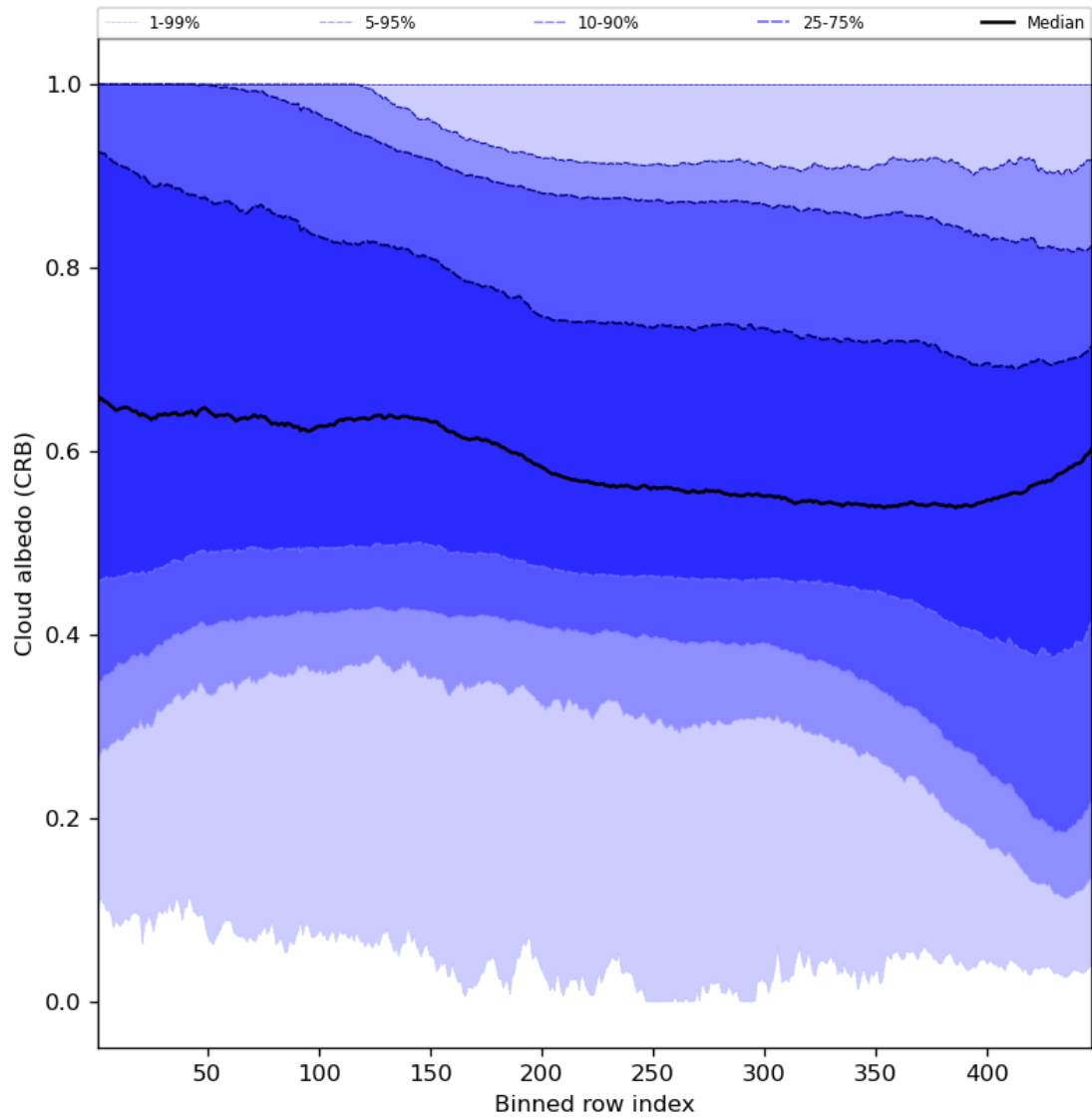
Figure 60: Along track statistics of “Cloud albedo (CRB)” for 2024-01-10 to 2024-01-11
