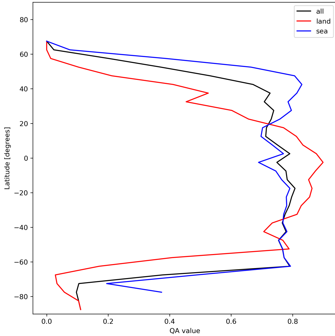
Figure 22: Zonal average of “QA value” for 2024-01-10 to 2024-01-11.
