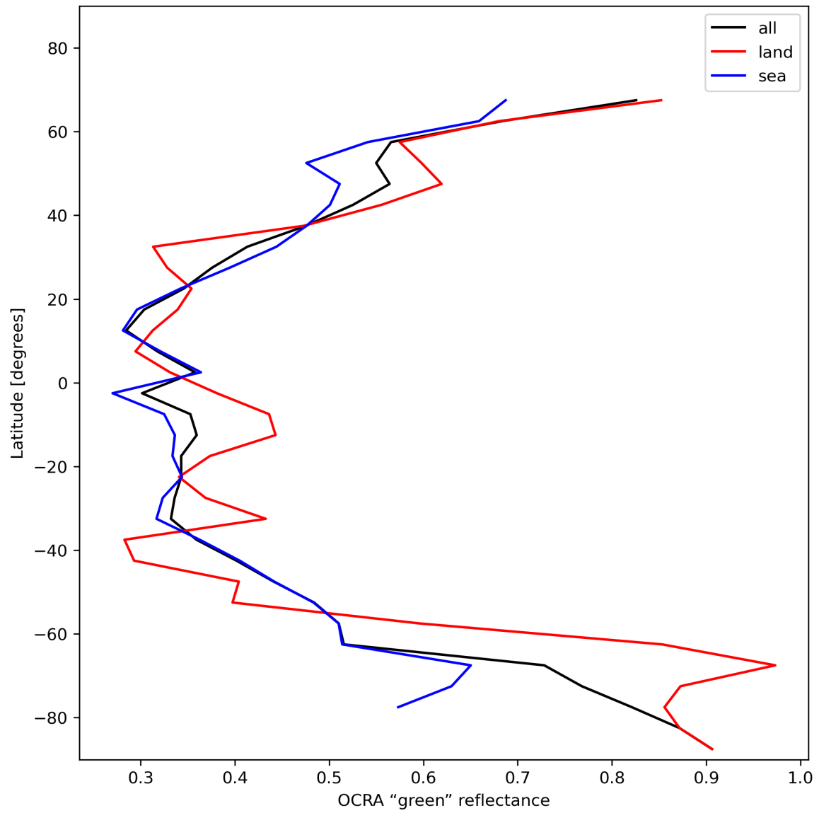
Figure 36: Zonal average of “OCRA “green” reflectance” for 2024-01-10 to 2024-01-11.
