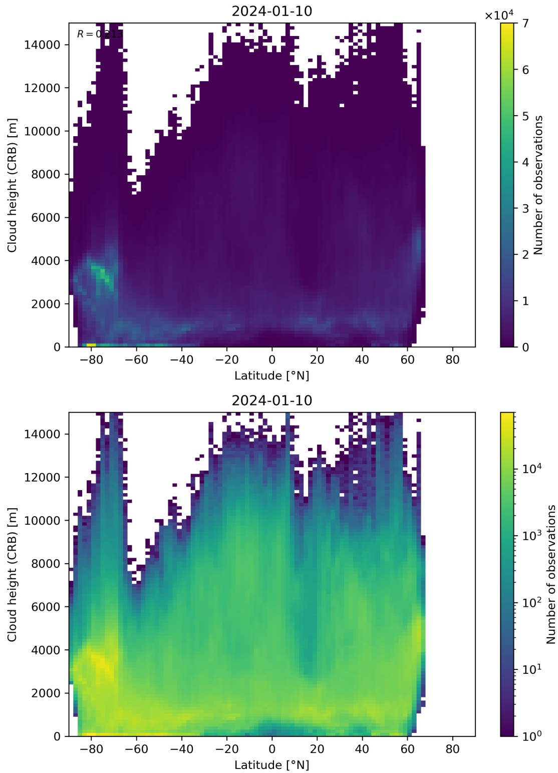
Figure 95: Scatter density plot of “Latitude” against “Cloud height (CRB)” for 2024-01-10 to 2024-01-11.
