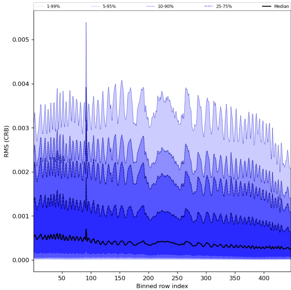
Figure 64: Along track statistics of “RMS (CRB)” for 2024-01-10 to 2024-01-11
