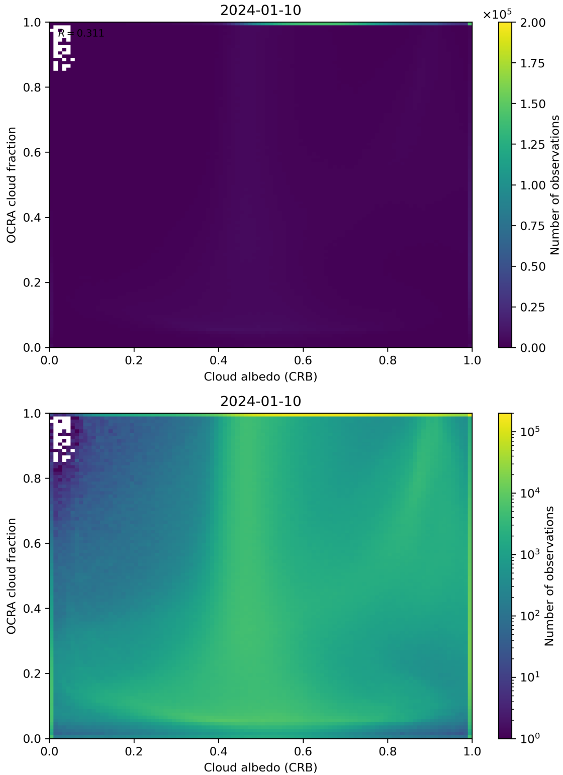
Figure 70: Scatter density plot of “Cloud albedo (CRB)” against “OCRA cloud fraction” for 2024-01-10 to 2024-01-11.
