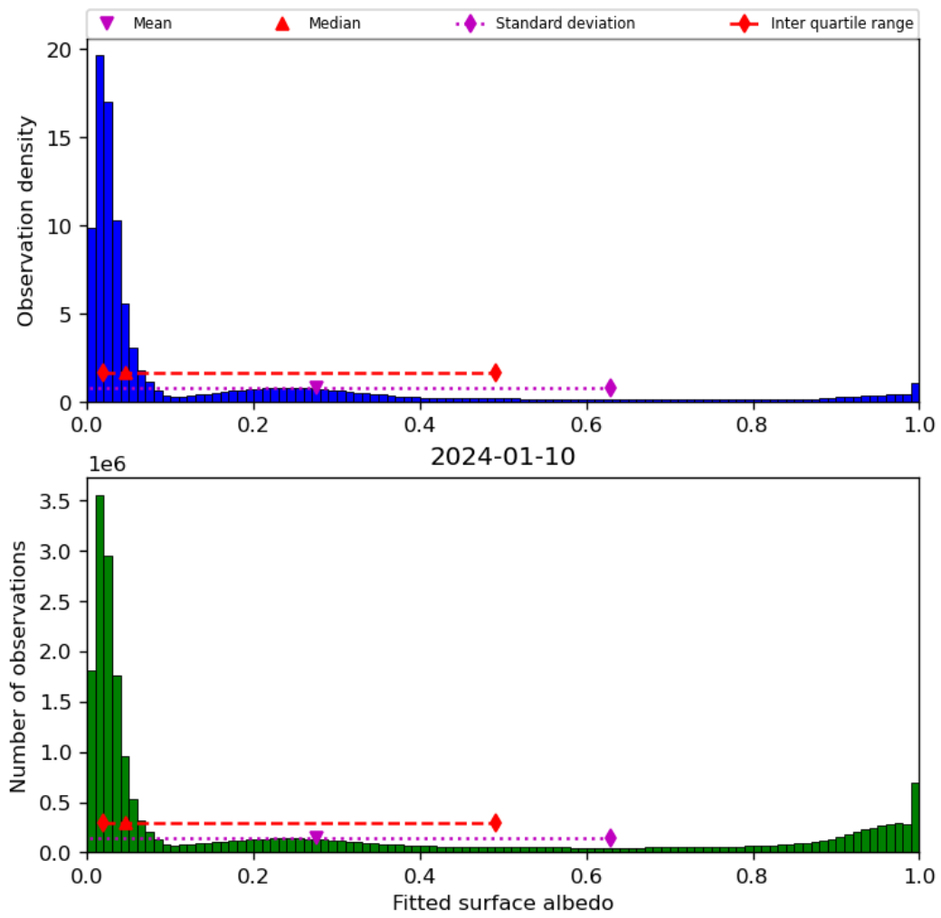
Figure 45: Histogram of “Fitted surface albedo” for 2024-01-10 to 2024-01-11
