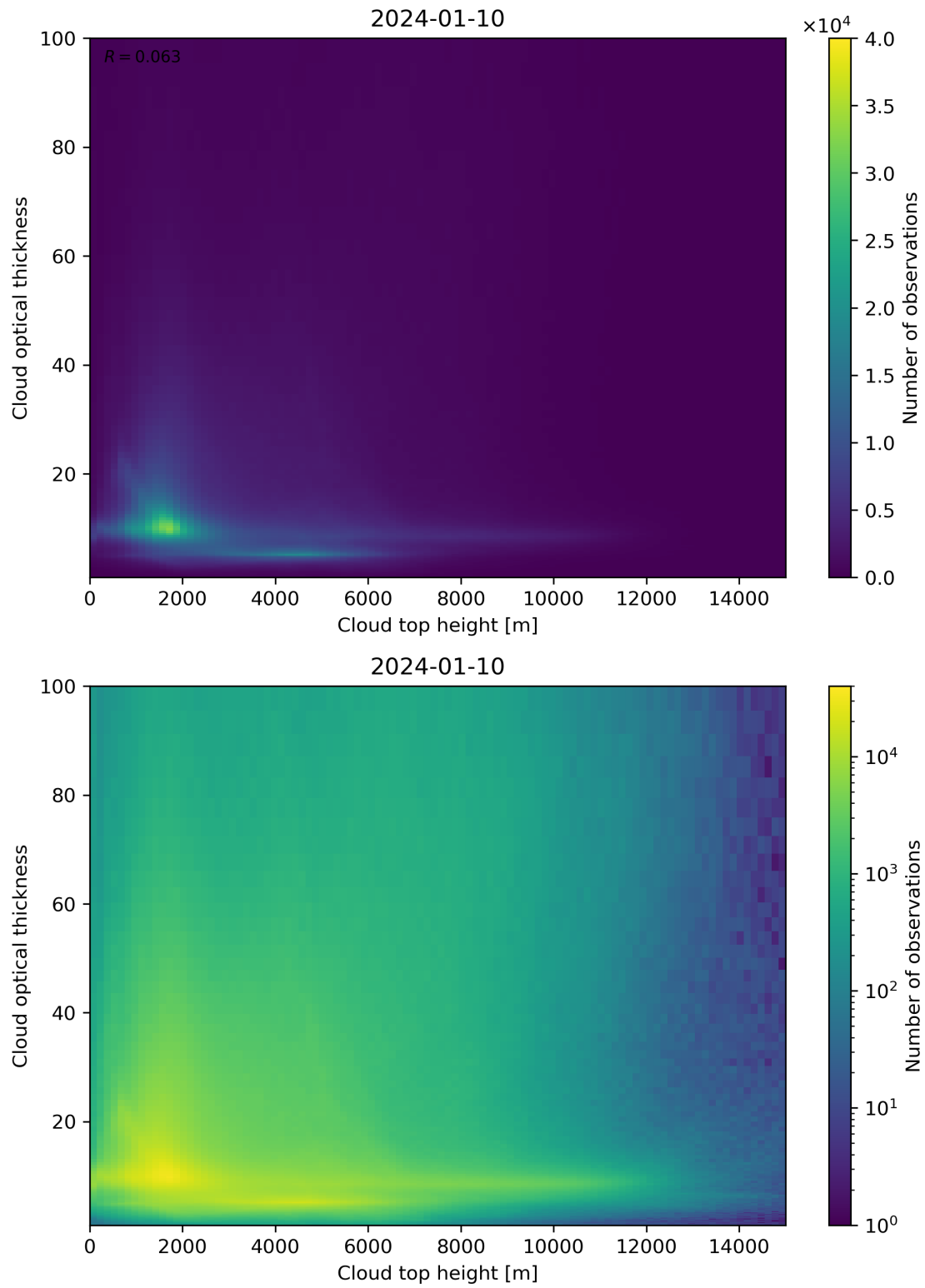
Figure 90: Scatter density plot of “Cloud top height” against “Cloud optical thickness” for 2024-01-10 to 2024-01-11.
