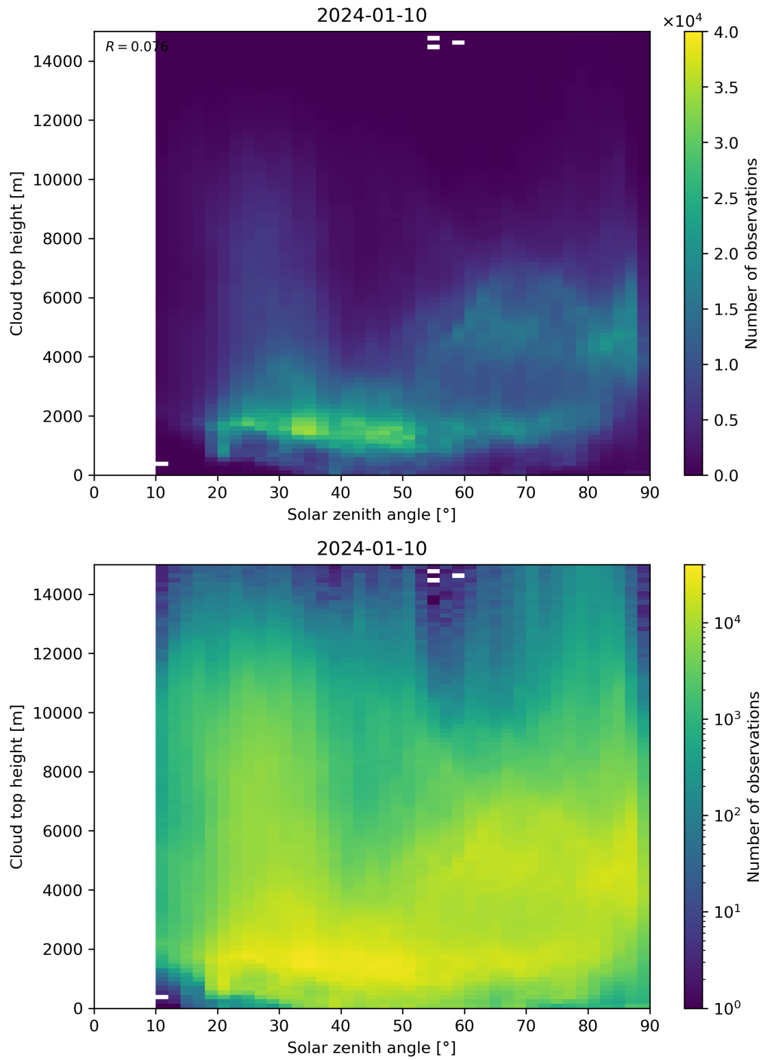
Figure 104: Scatter density plot of “Solar zenith angle” against “Cloud top height” for 2024-01-10 to 2024-01-11.
