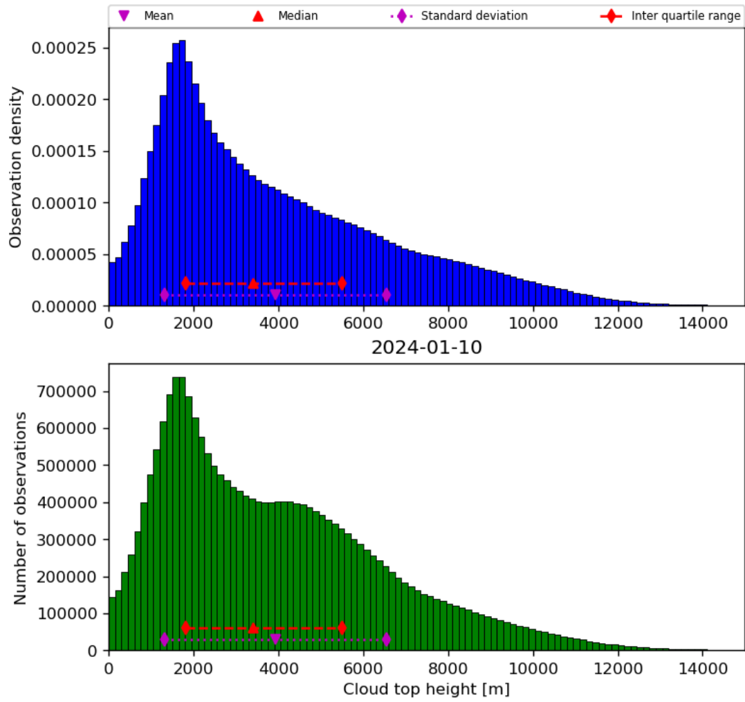
Figure 40: Histogram of “Cloud top height” for 2024-01-10 to 2024-01-11
