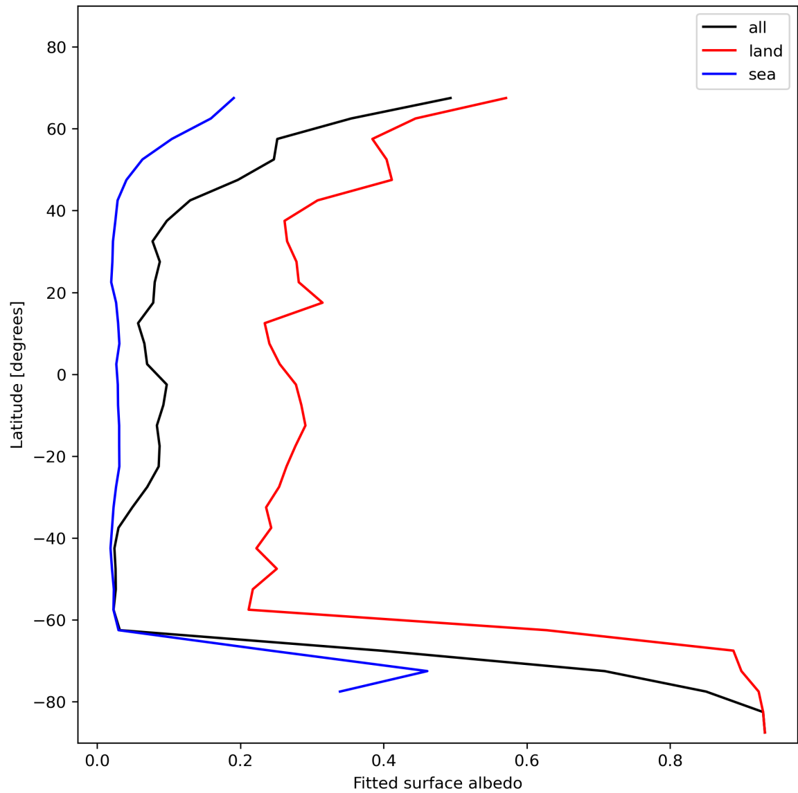
Figure 29: Zonal average of “Fitted surface albedo” for 2024-01-10 to 2024-01-11.
