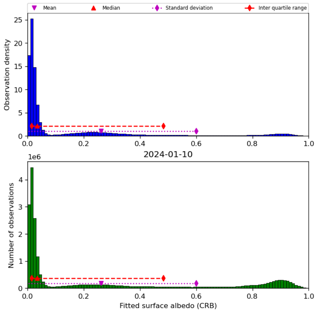
Figure 46: Histogram of “Fitted surface albedo (CRB)” for 2024-01-10 to 2024-01-11
