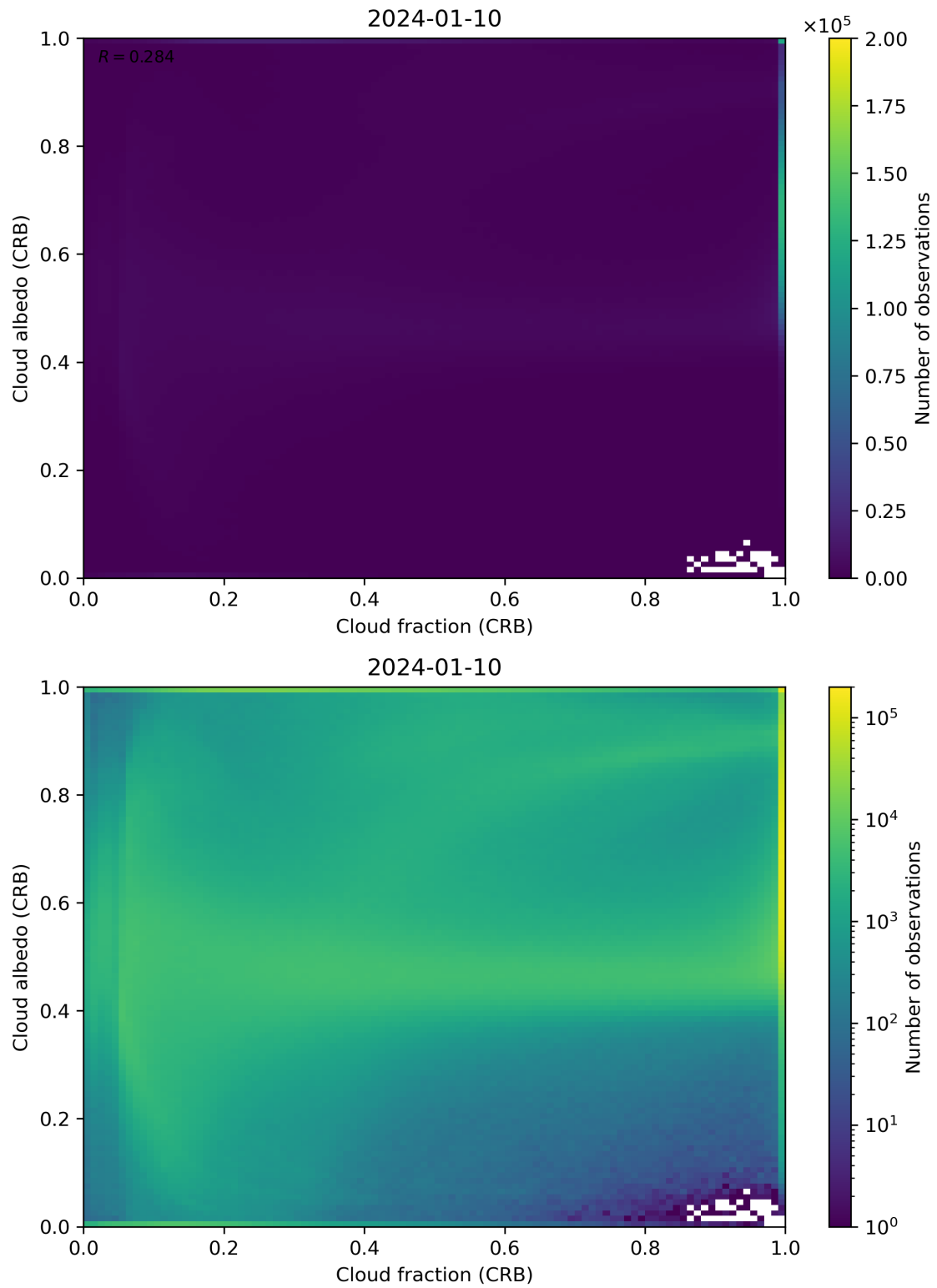
Figure 77: Scatter density plot of “Cloud fraction (CRB)” against “Cloud albedo (CRB)” for 2024-01-10 to 2024-01-11.
