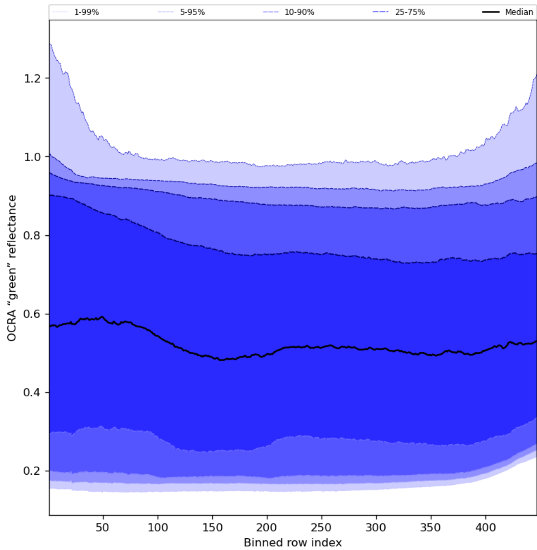
Figure 68: Along track statistics of “OCRA “green” reflectance” for 2024-01-10 to 2024-01-11
