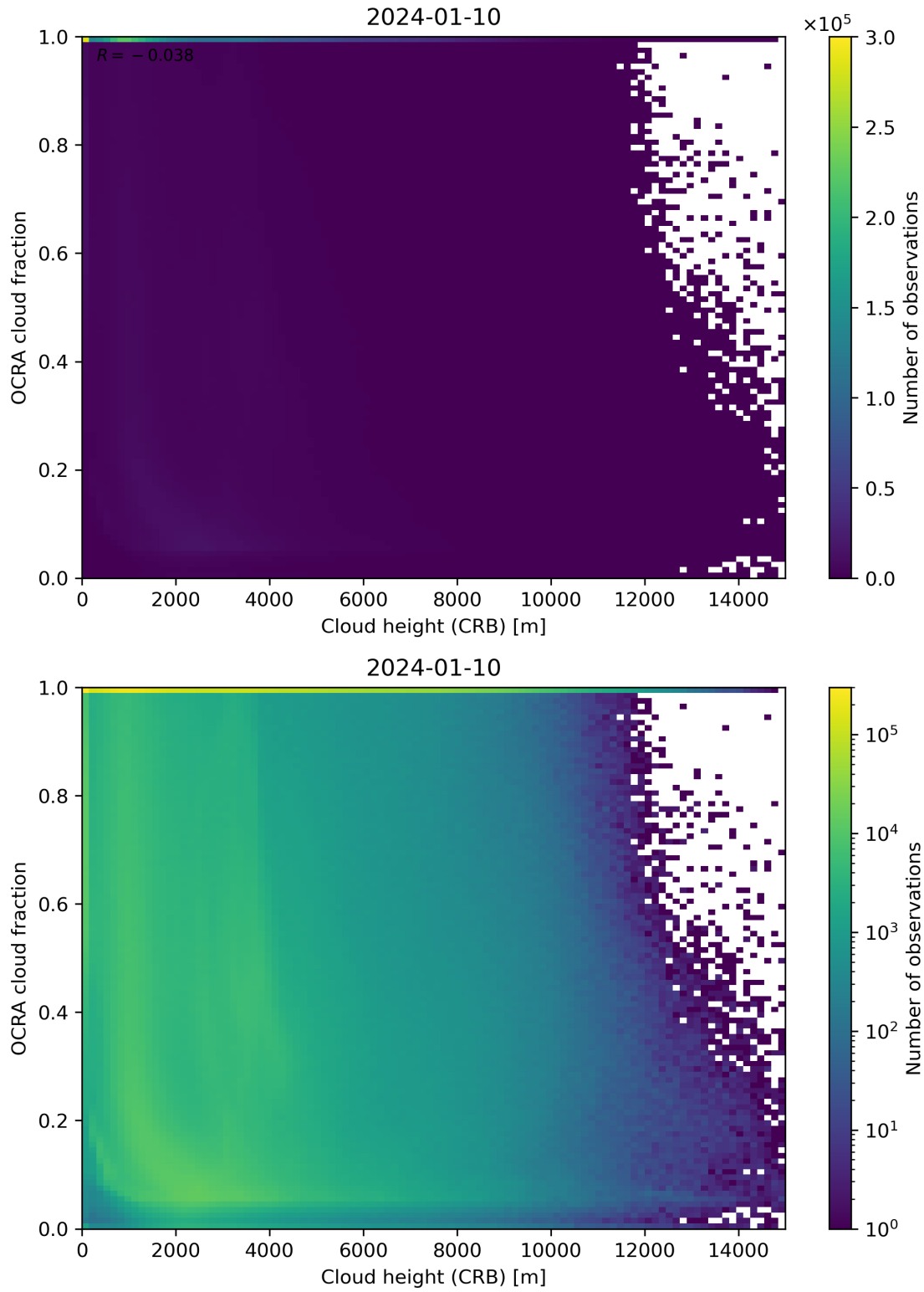
Figure 81: Scatter density plot of “Cloud height (CRB)” against “OCRA cloud fraction” for 2024-01-10 to 2024-01-11.
