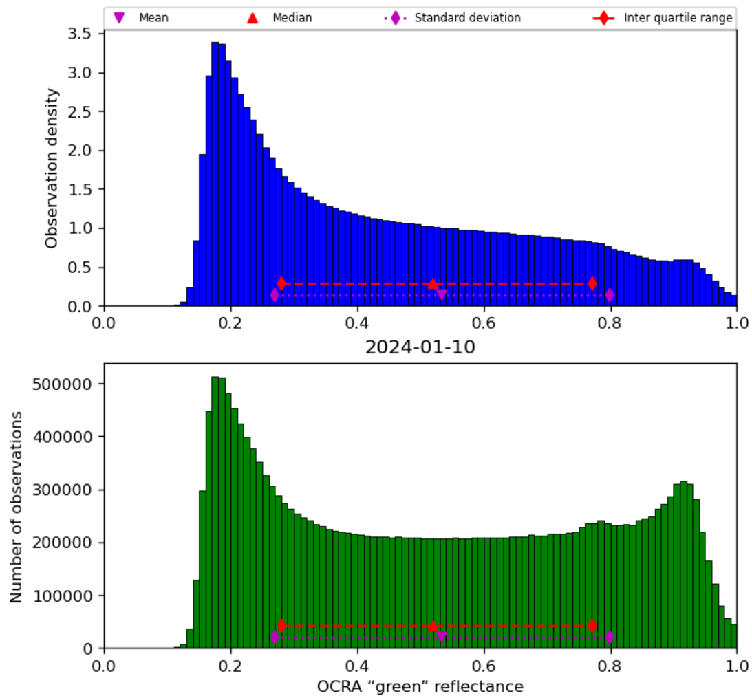
Figure 52: Histogram of “OCRA “green” reflectance” for 2024-01-10 to 2024-01-11
