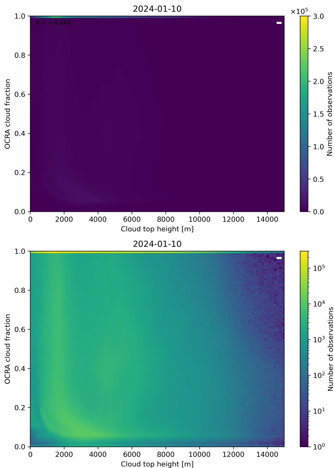
Figure 87: Scatter density plot of “Cloud top height” against “OCRA cloud fraction” for 2024-01-10 to 2024-01-11.
