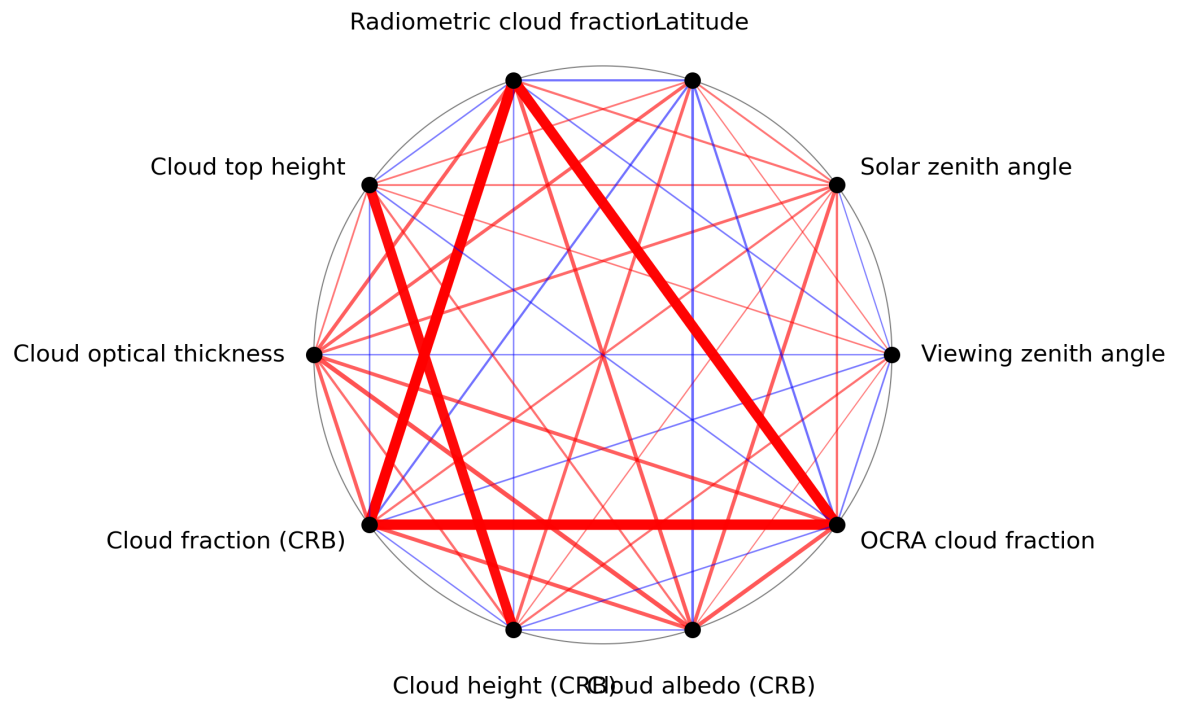
Figure 1: Map of correlation graph for 2024-01-10 to 2024-01-11.
