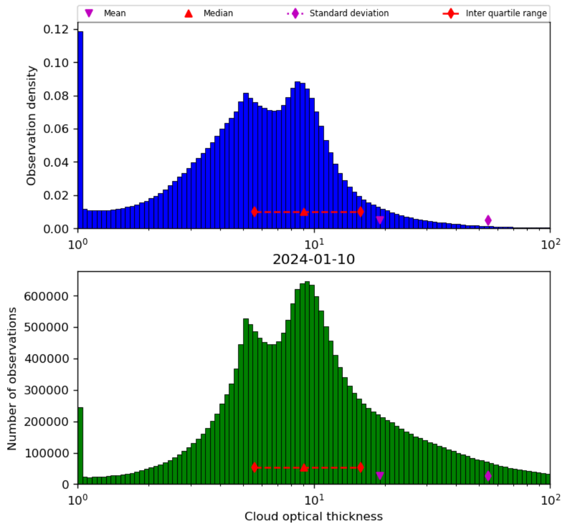
Figure 41: Histogram of “Cloud optical thickness” for 2024-01-10 to 2024-01-11
