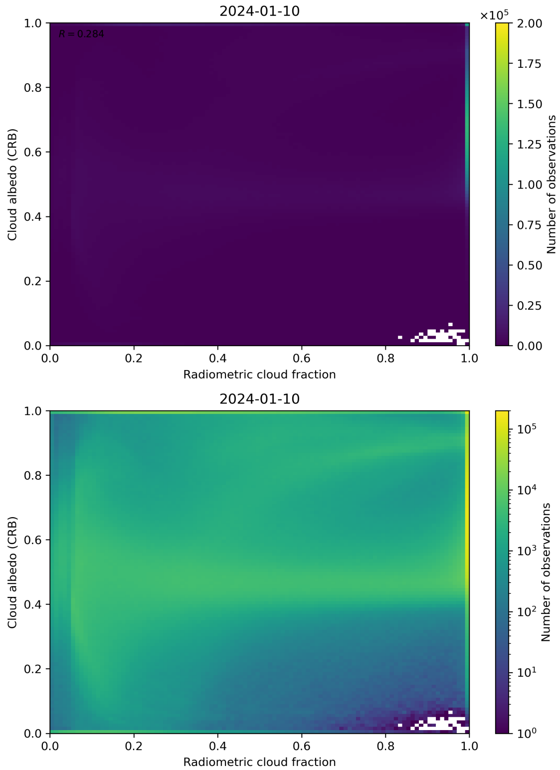
Figure 71: Scatter density plot of “Radiometric cloud fraction” against “Cloud albedo (CRB)” for 2024-01-10 to 2024-01-11.
