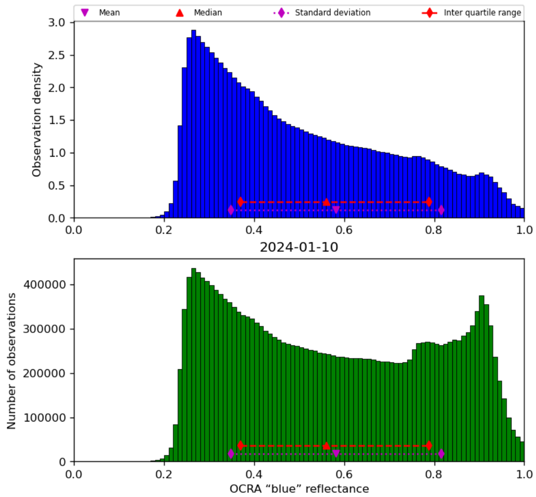
Figure 51: Histogram of “OCRA “blue” reflectance” for 2024-01-10 to 2024-01-11
