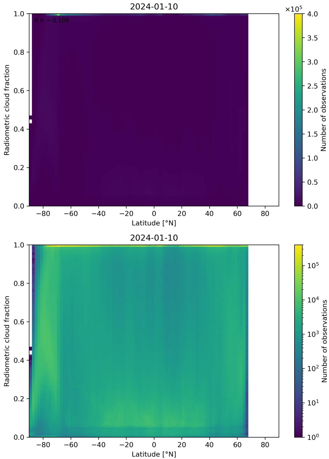
Figure 92: Scatter density plot of “Latitude” against “Radiometric cloud fraction” for 2024-01-10 to 2024-01-11.
