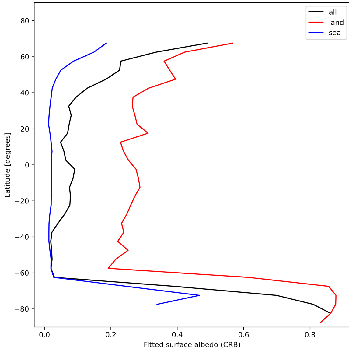
Figure 30: Zonal average of “Fitted surface albedo (CRB)” for 2024-01-10 to 2024-01-11.
