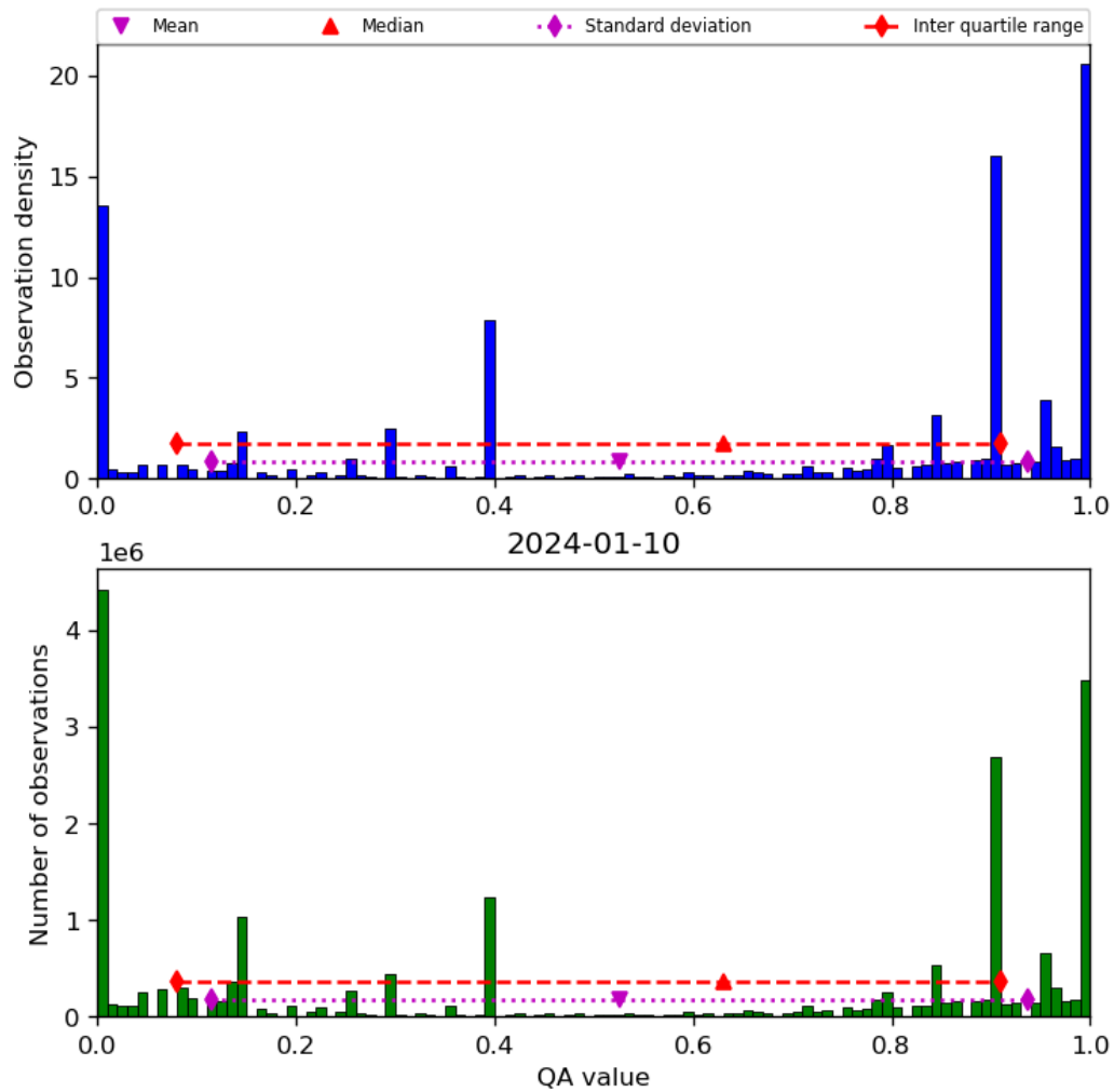
Figure 38: Histogram of “QA value” for 2024-01-10 to 2024-01-11
