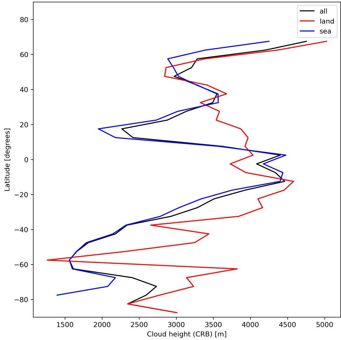
Figure 27: Zonal average of “Cloud height (CRB)” for 2024-01-10 to 2024-01-11.
