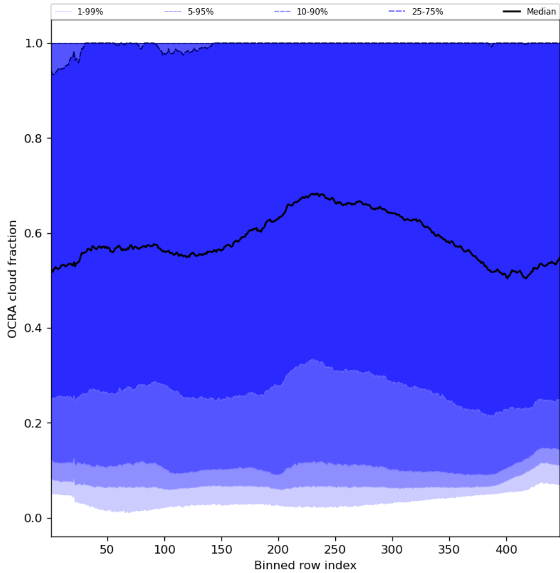
Figure 66: Along track statistics of “OCRA cloud fraction” for 2024-01-10 to 2024-01-11
