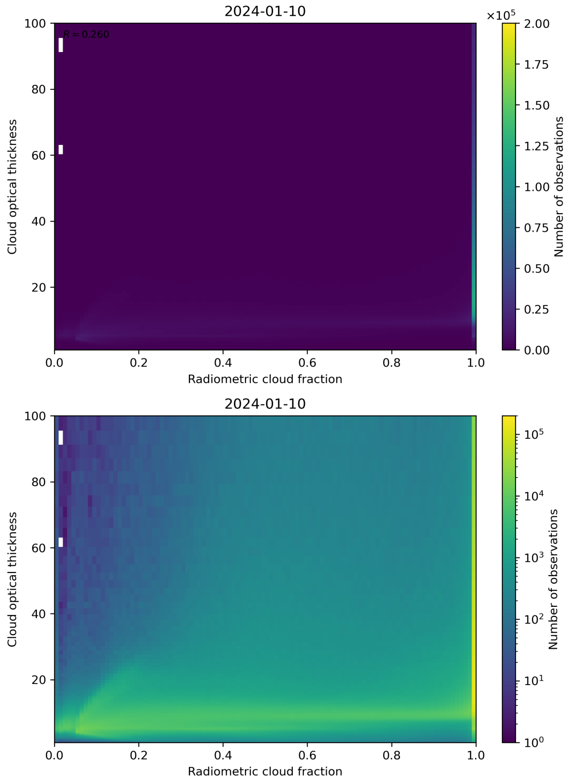
Figure 75: Scatter density plot of “Radiometric cloud fraction” against “Cloud optical thickness” for 2024-01-10 to 2024-01-11.
