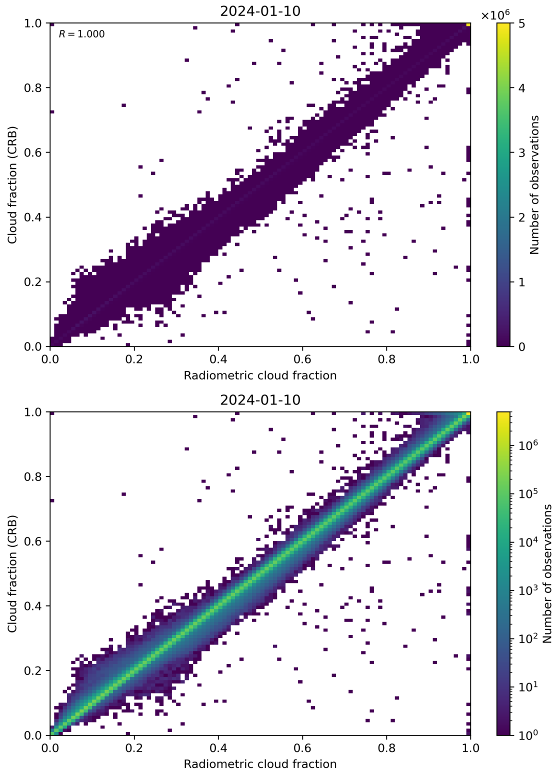
Figure 73: Scatter density plot of “Radiometric cloud fraction” against “Cloud fraction (CRB)” for 2024-01-10 to 2024-01-11.
