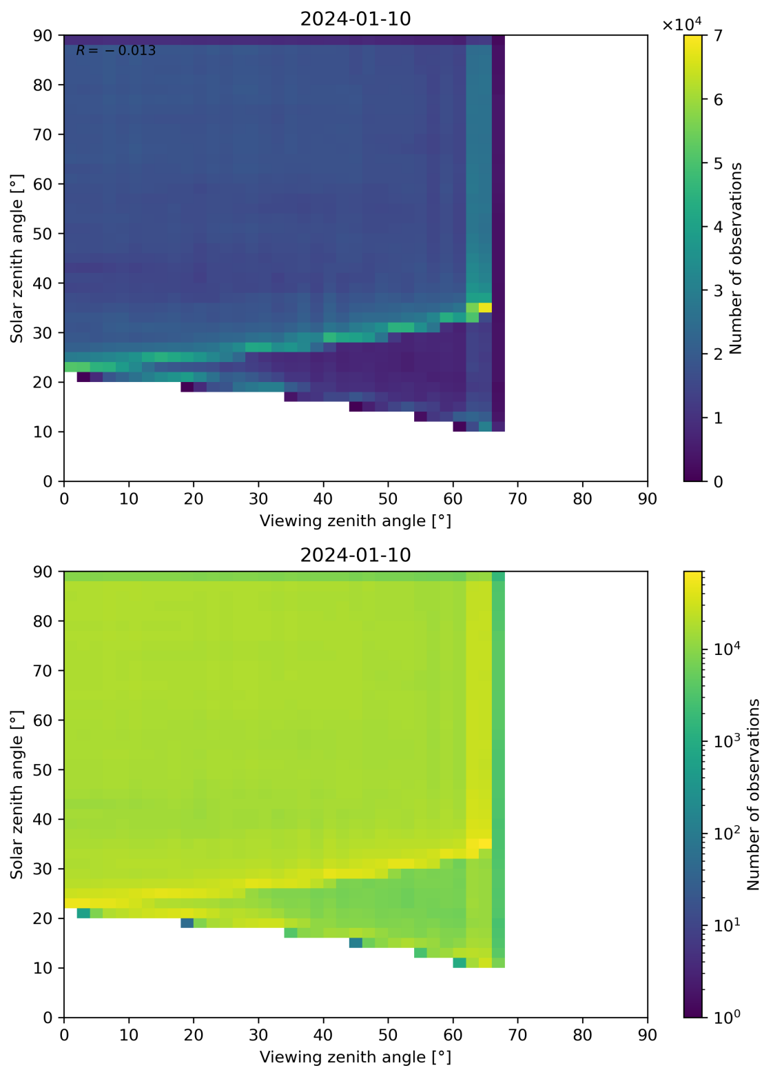
Figure 114: Scatter density plot of “Viewing zenith angle” against “Solar zenith angle” for 2024-01-10 to 2024-01-11.
