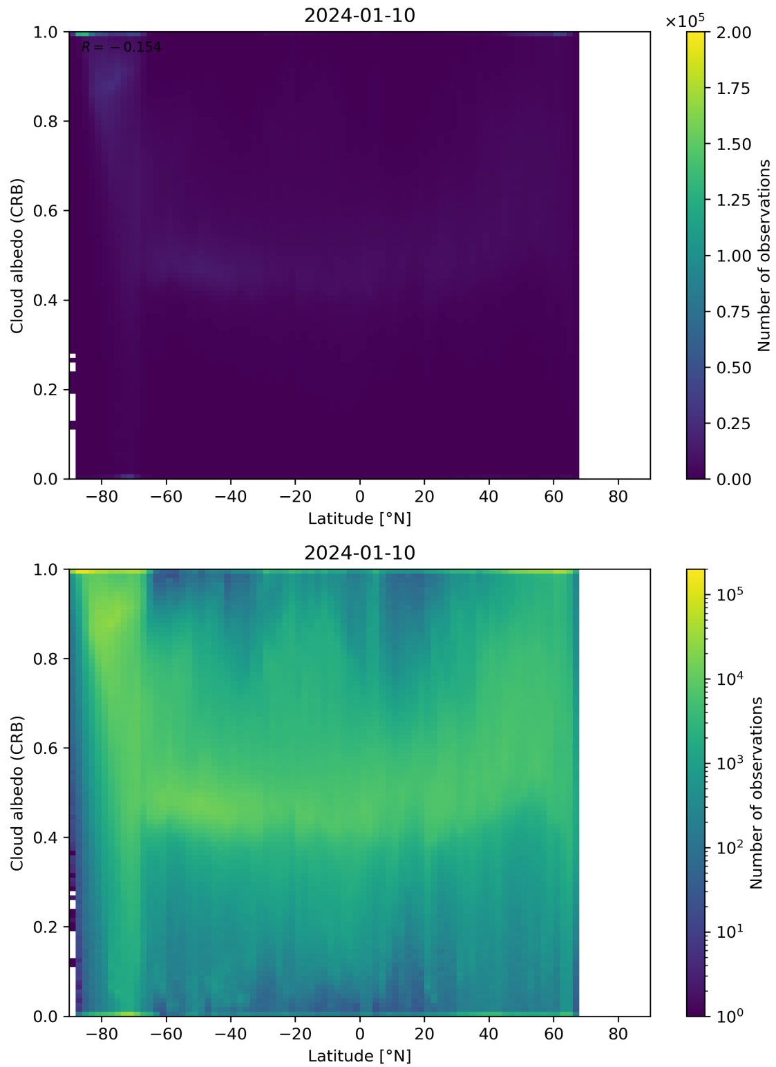
Figure 91: Scatter density plot of “Latitude” against “Cloud albedo (CRB)” for 2024-01-10 to 2024-01-11.
