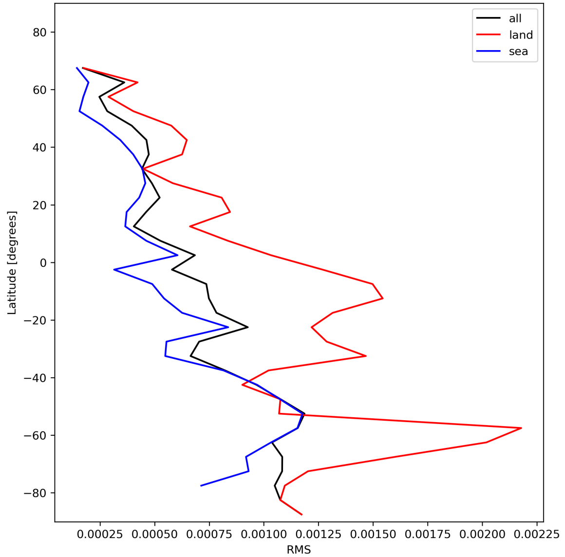
Figure 31: Zonal average of “RMS” for 2024-01-10 to 2024-01-11.
