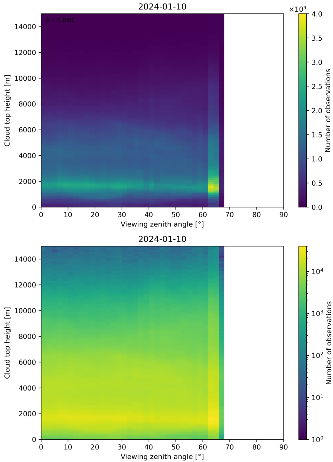
Figure 112: Scatter density plot of “Viewing zenith angle” against “Cloud top height” for 2024-01-10 to 2024-01-11.
