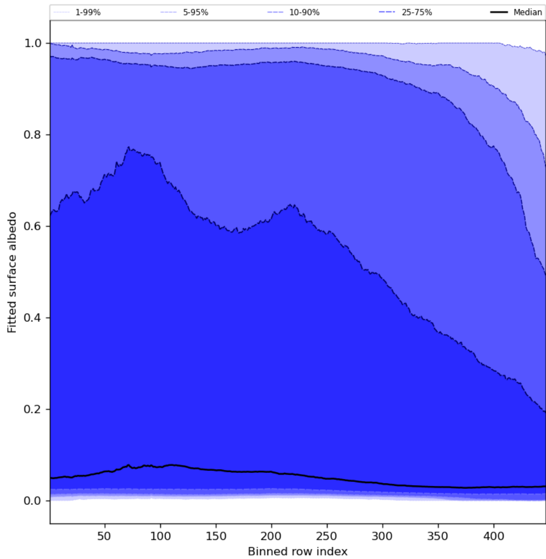
Figure 61: Along track statistics of “Fitted surface albedo” for 2024-01-10 to 2024-01-11
