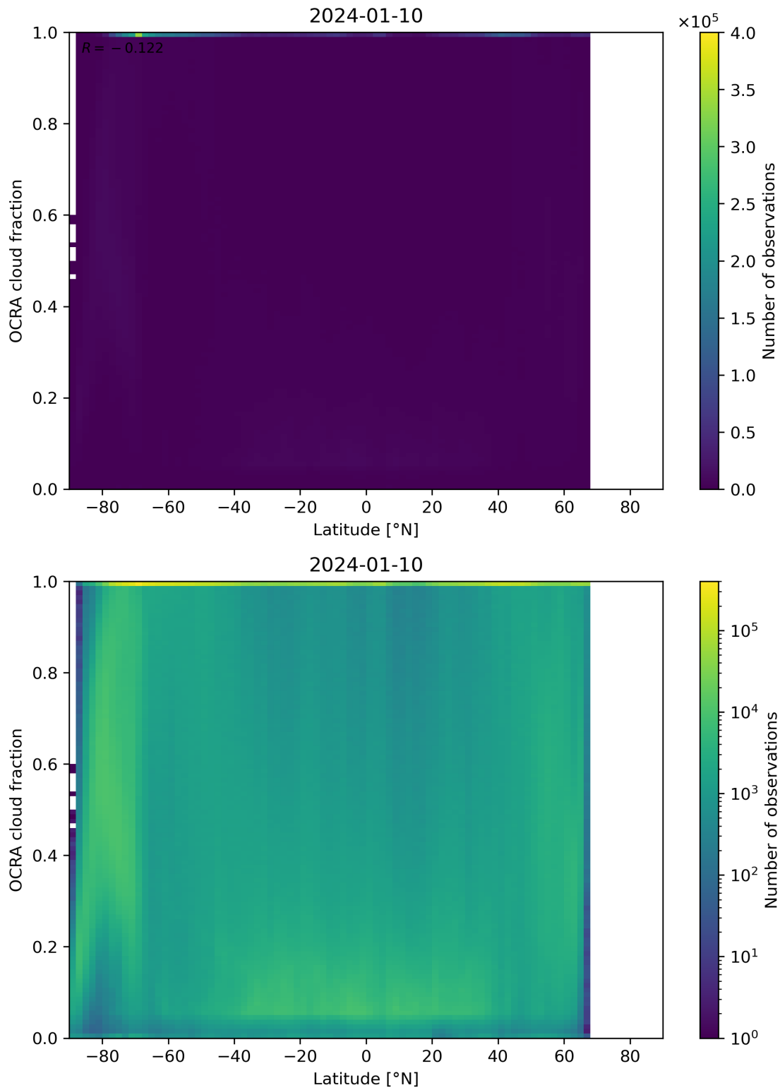
Figure 93: Scatter density plot of “Latitude” against “OCRA cloud fraction” for 2024-01-10 to 2024-01-11.
