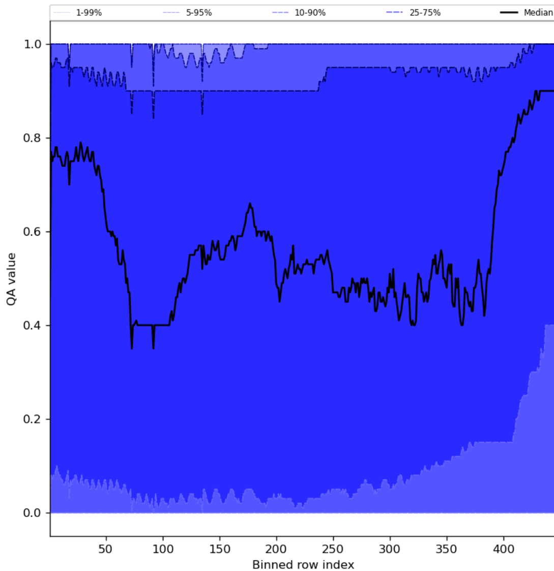
Figure 54: Along track statistics of “QA value” for 2024-01-10 to 2024-01-11
