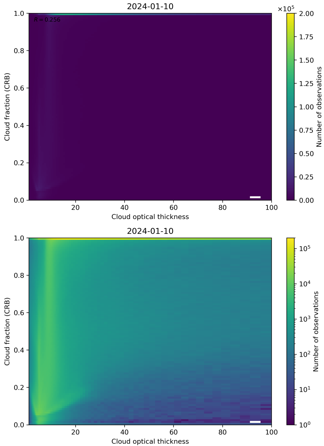
Figure 84: Scatter density plot of “Cloud optical thickness” against “Cloud fraction (CRB)” for 2024-01-10 to 2024-01-11.
