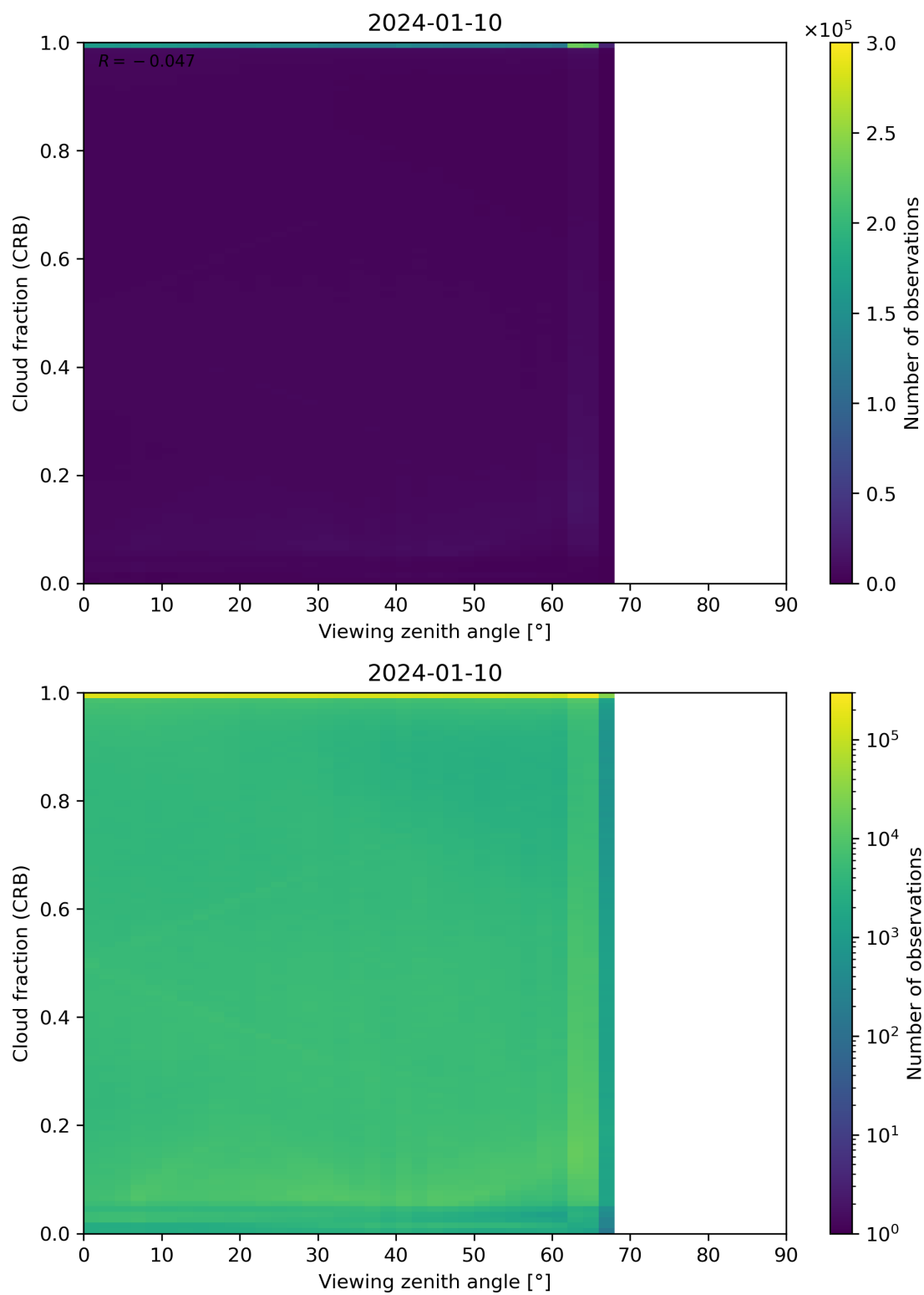
Figure 109: Scatter density plot of “Viewing zenith angle” against “Cloud fraction (CRB)” for 2024-01-10 to 2024-01-11.
