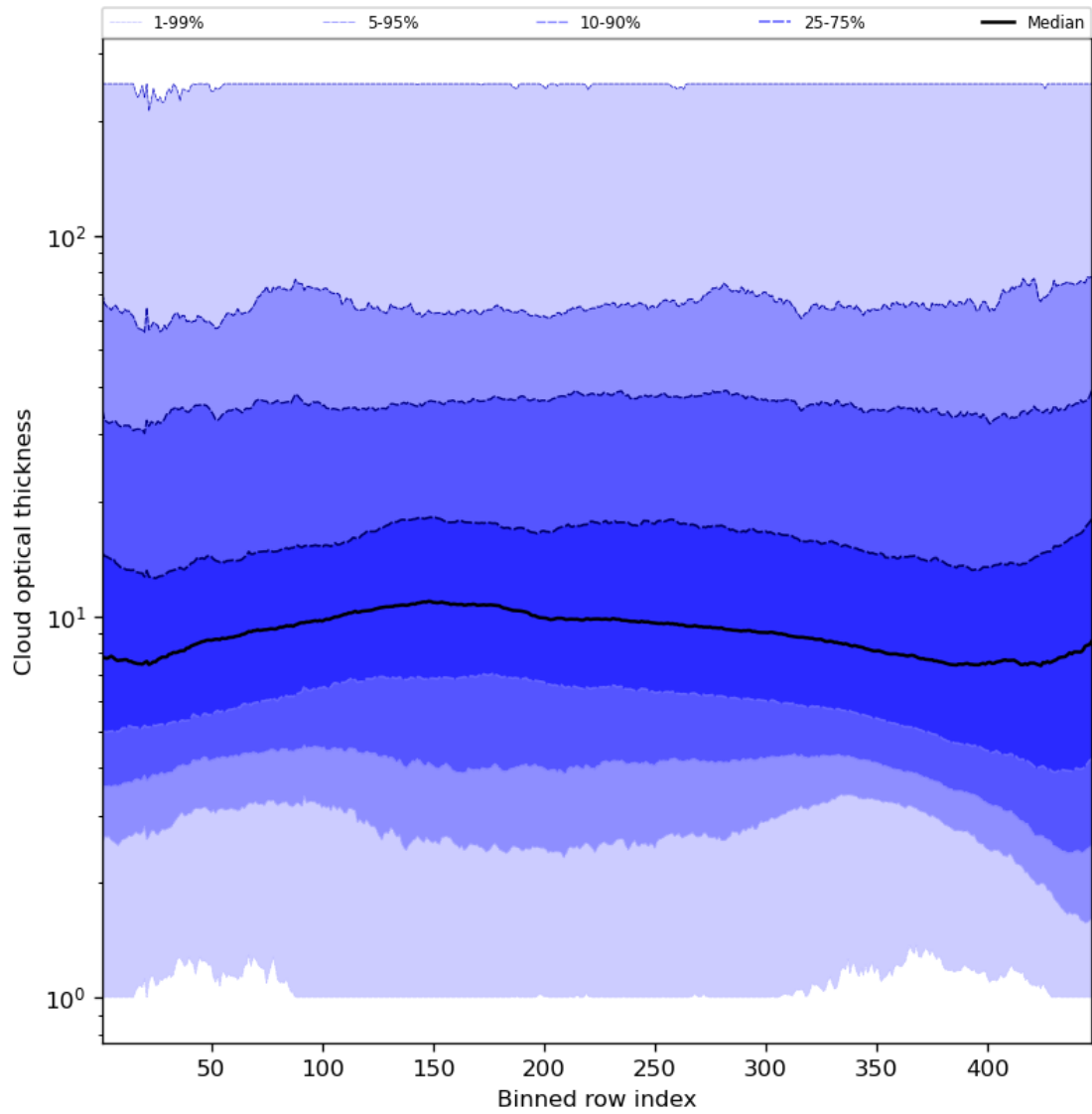
Figure 57: Along track statistics of “Cloud optical thickness” for 2024-01-10 to 2024-01-11
