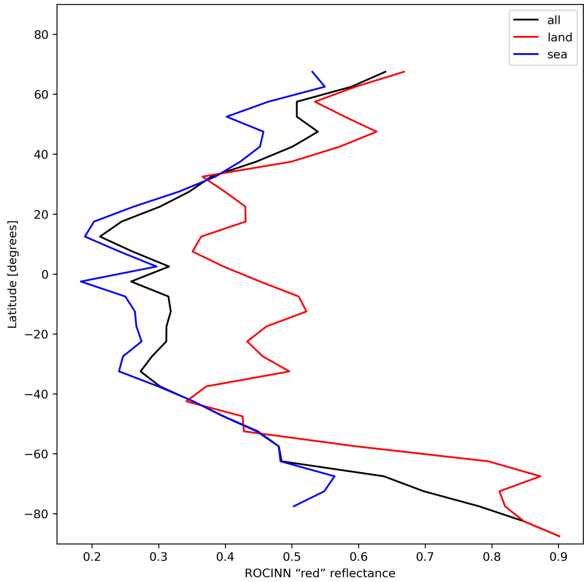
Figure 37: Zonal average of “ROCINN “red” reflectance” for 2024-01-10 to 2024-01-11.
