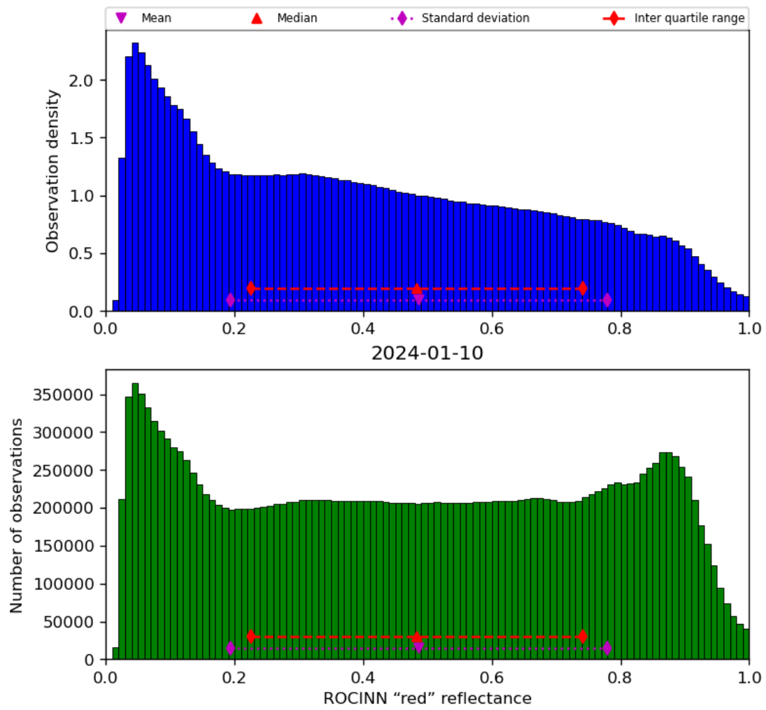
Figure 53: Histogram of “ROCINN “red” reflectance” for 2024-01-10 to 2024-01-11
