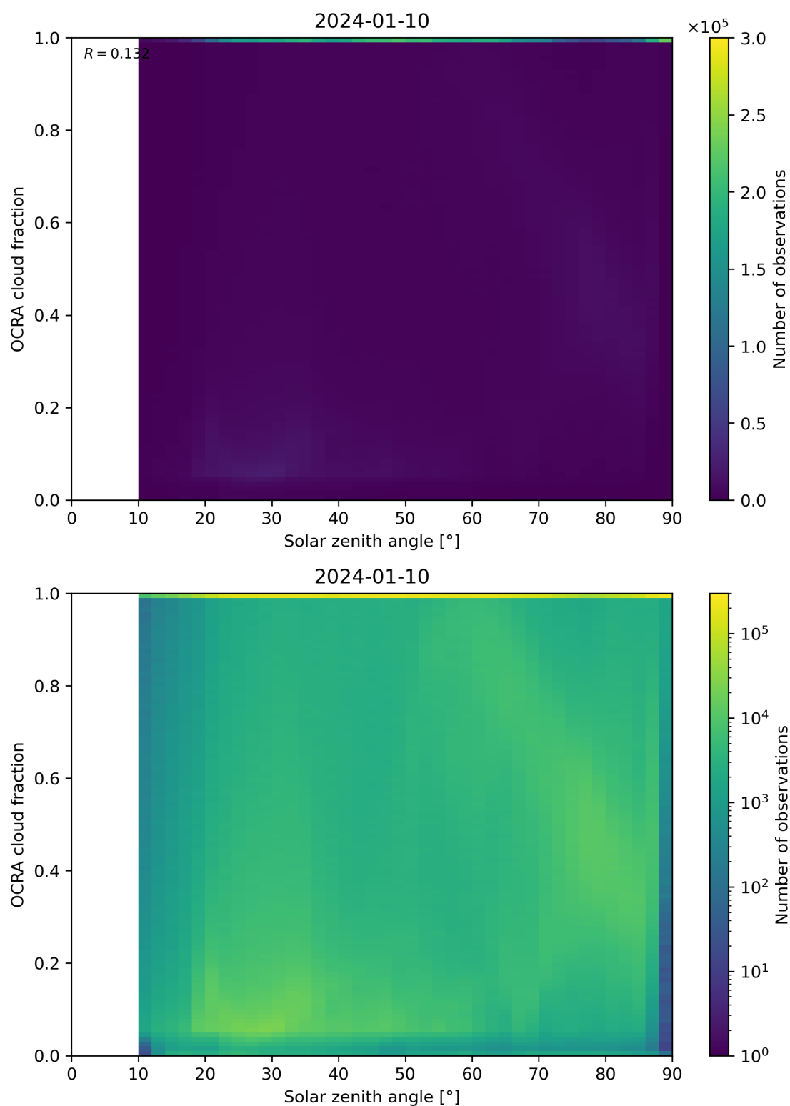
Figure 100: Scatter density plot of “Solar zenith angle” against “OCRA cloud fraction” for 2024-01-10 to 2024-01-11.
