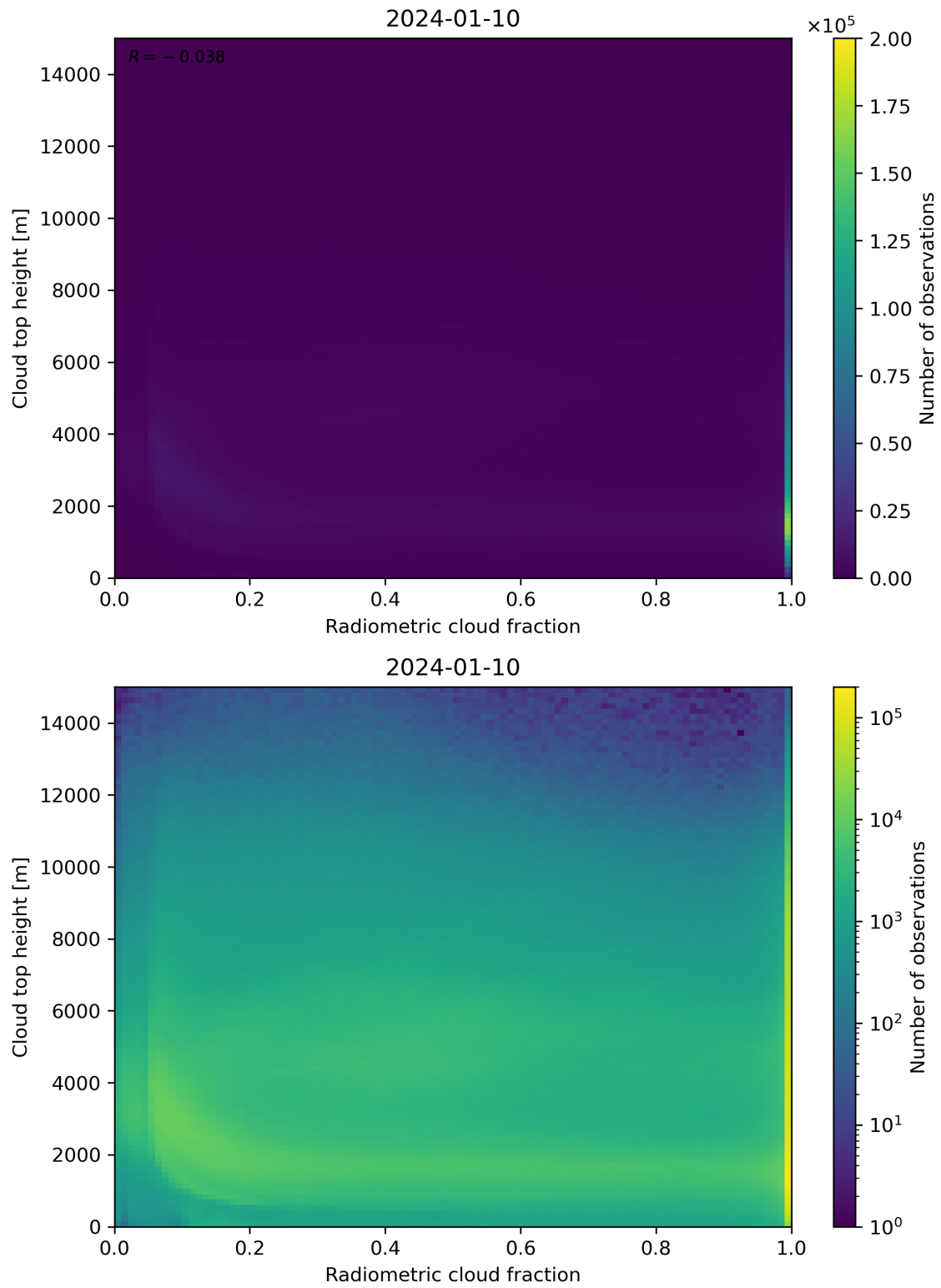
Figure 76: Scatter density plot of “Radiometric cloud fraction” against “Cloud top height” for 2024-01-10 to 2024-01-11.
