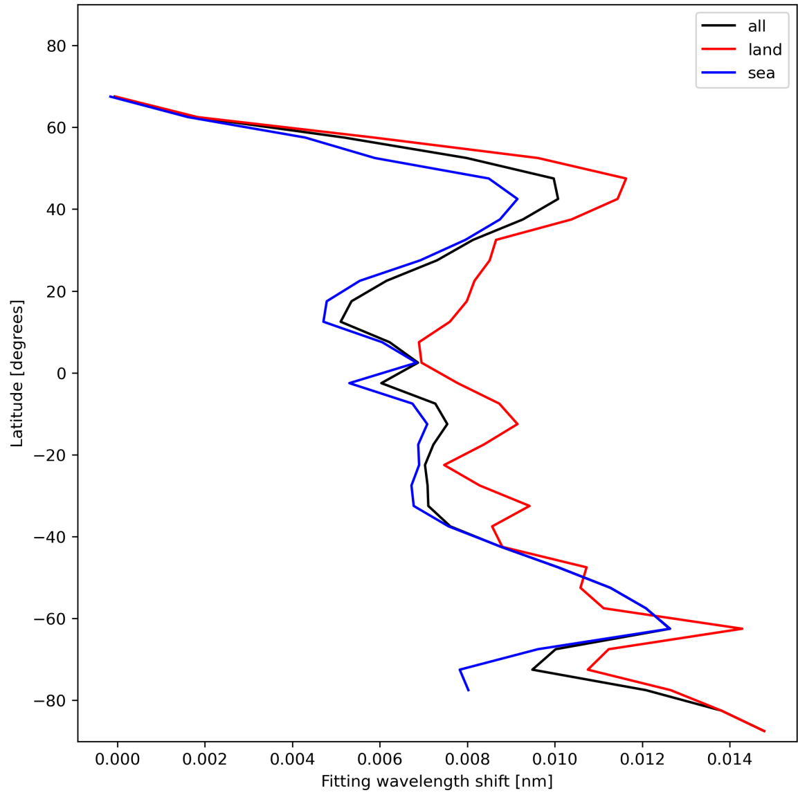
Figure 33: Zonal average of “Fitting wavelength shift” for 2024-01-10 to 2024-01-11.
