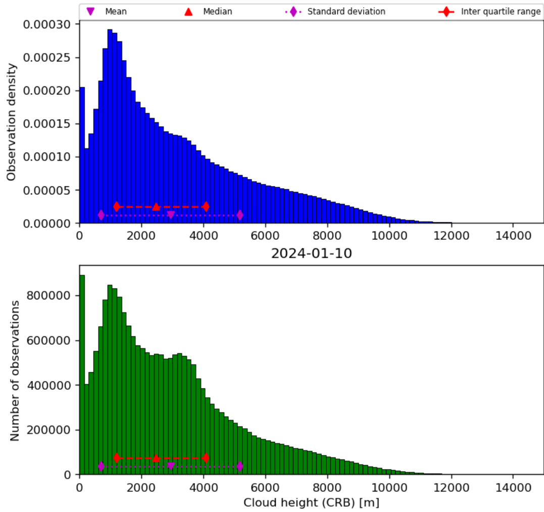
Figure 43: Histogram of “Cloud height (CRB)” for 2024-01-10 to 2024-01-11
