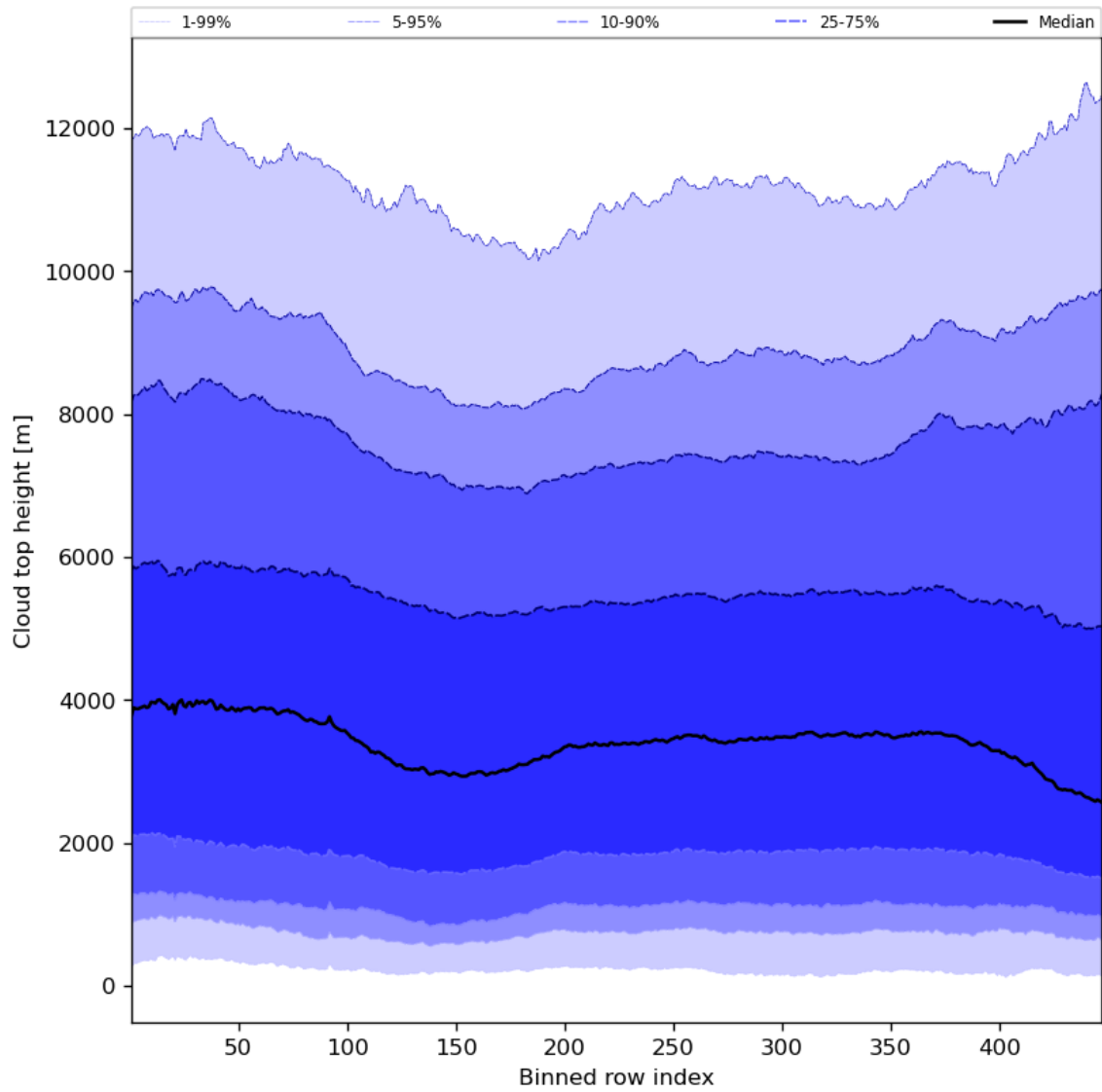
Figure 56: Along track statistics of “Cloud top height” for 2024-01-10 to 2024-01-11
