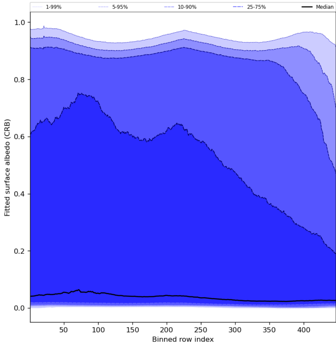
Figure 62: Along track statistics of “Fitted surface albedo (CRB)” for 2024-01-10 to 2024-01-11
