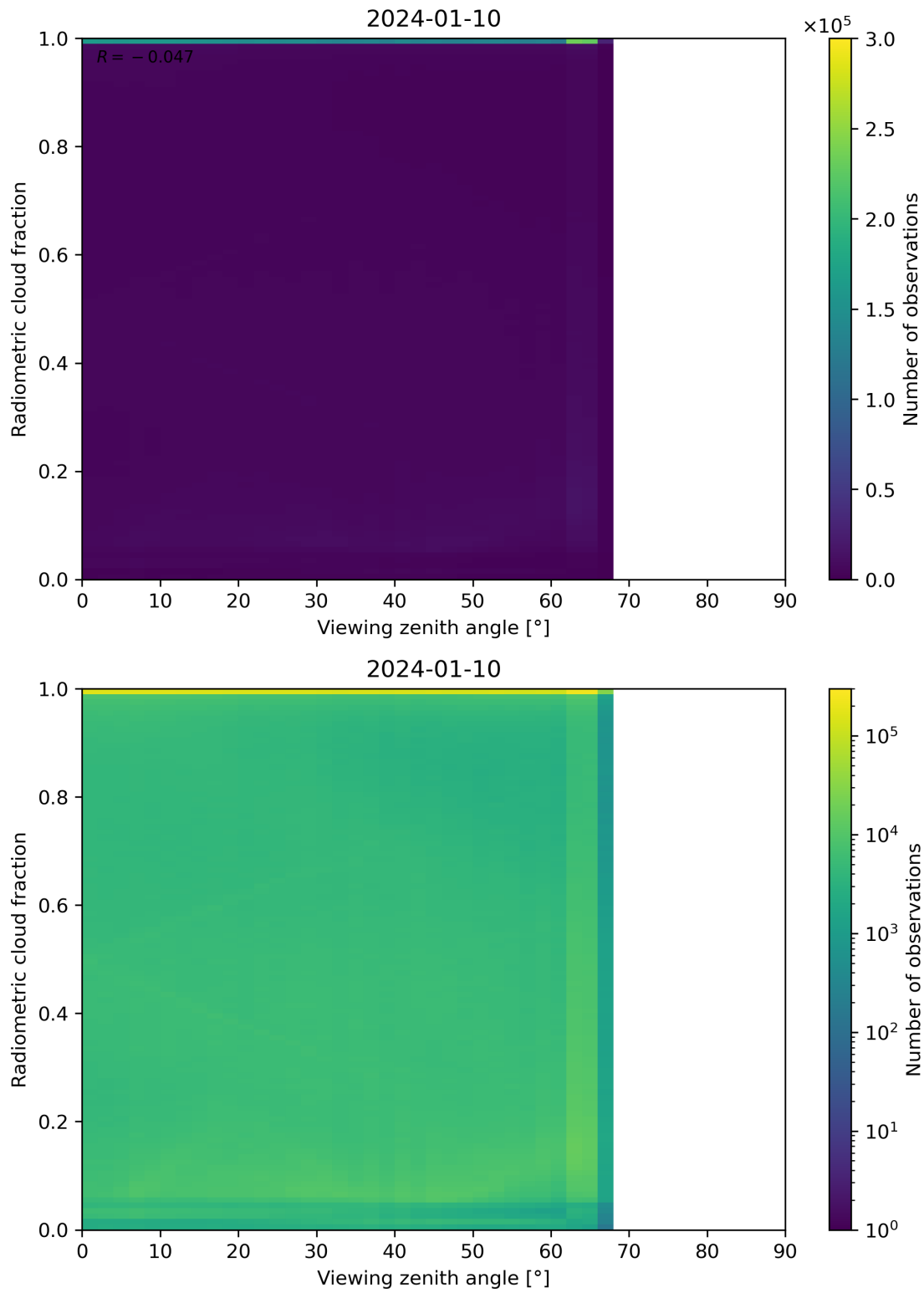
Figure 107: Scatter density plot of “Viewing zenith angle” against “Radiometric cloud fraction” for 2024-01-10 to 2024-01-11.
