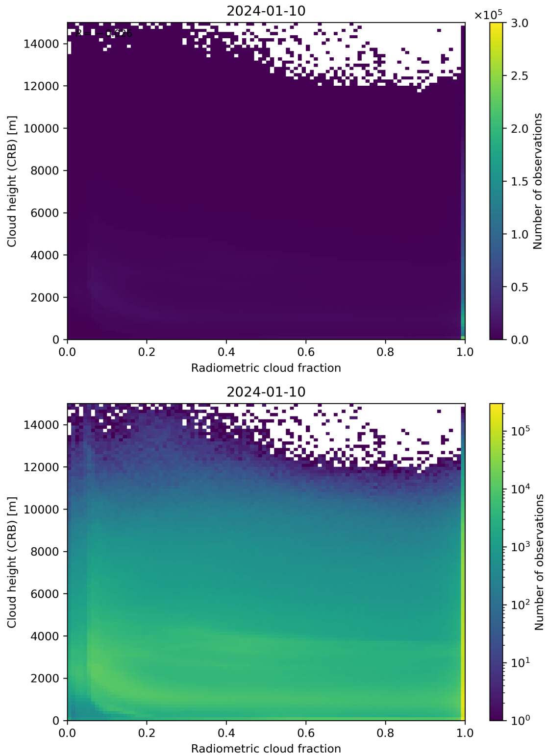
Figure 74: Scatter density plot of “Radiometric cloud fraction” against “Cloud height (CRB)” for 2024-01-10 to 2024-01-11.
