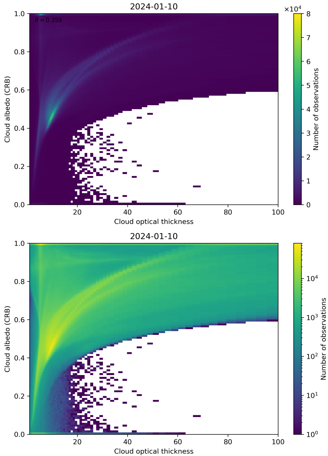
Figure 82: Scatter density plot of “Cloud optical thickness” against “Cloud albedo (CRB)” for 2024-01-10 to 2024-01-11.
