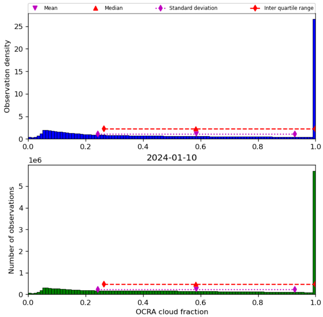
Figure 50: Histogram of “OCRA cloud fraction” for 2024-01-10 to 2024-01-11
