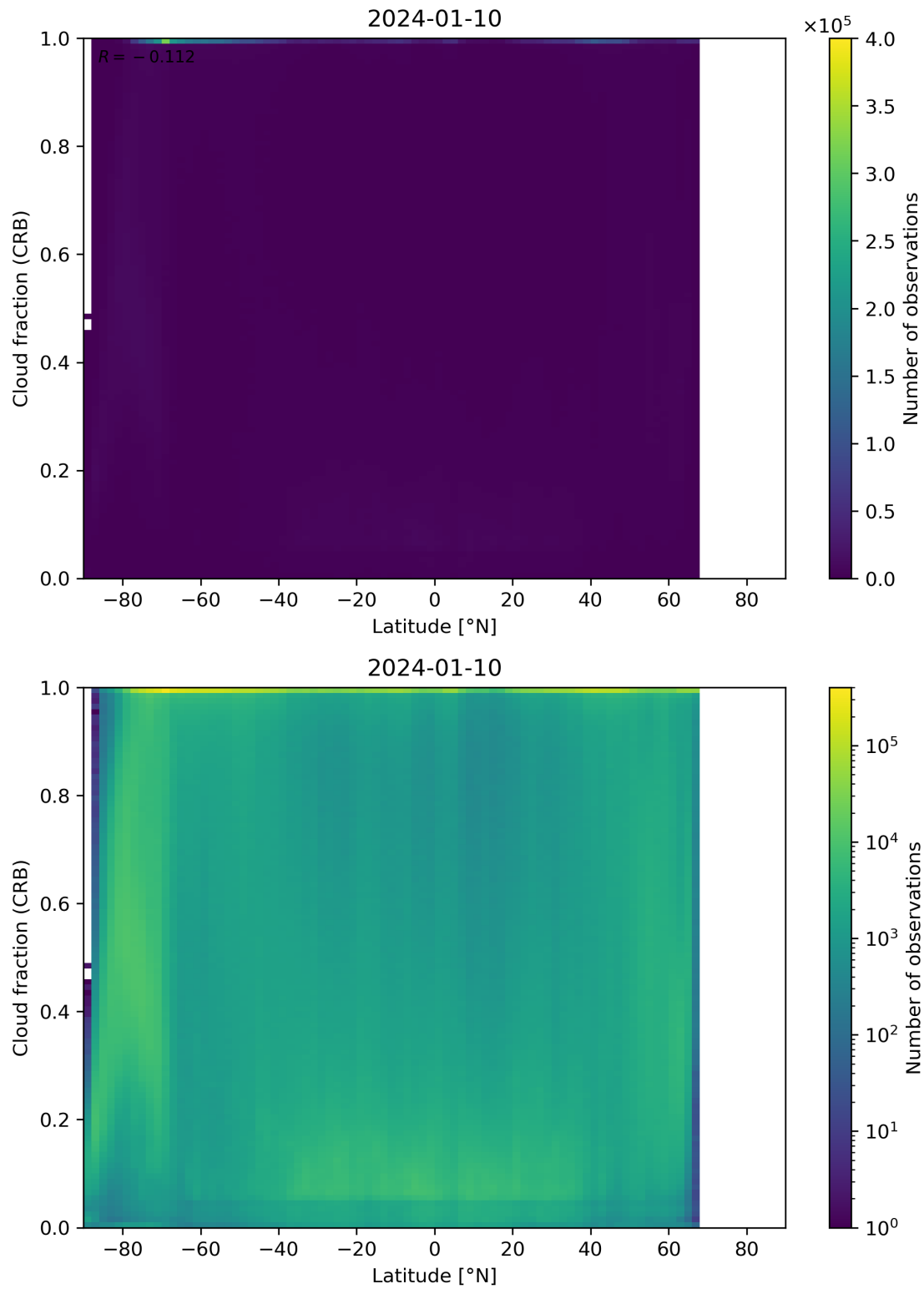
Figure 94: Scatter density plot of “Latitude” against “Cloud fraction (CRB)” for 2024-01-10 to 2024-01-11.
