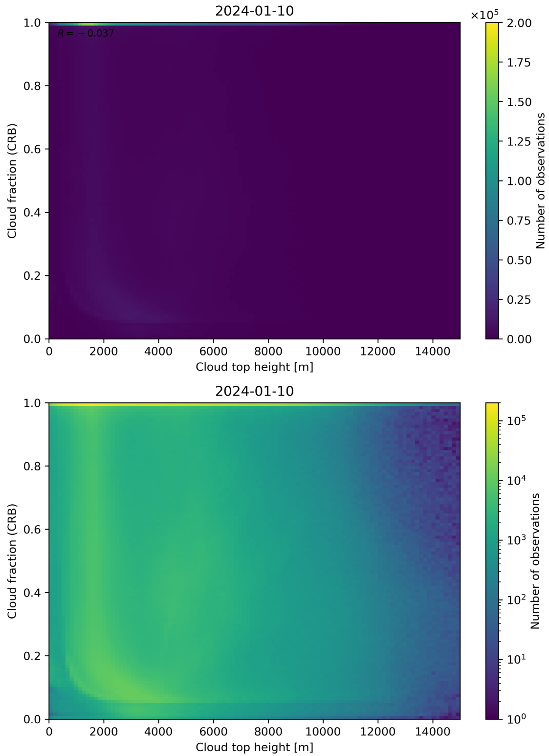
Figure 88: Scatter density plot of “Cloud top height” against “Cloud fraction (CRB)” for 2024-01-10 to 2024-01-11.
