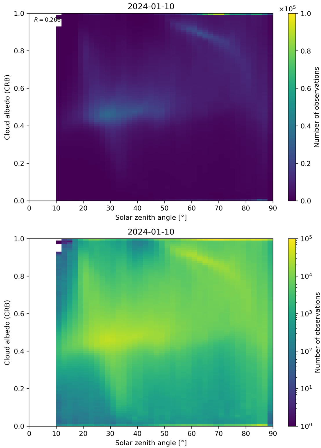
Figure 98: Scatter density plot of “Solar zenith angle” against “Cloud albedo (CRB)” for 2024-01-10 to 2024-01-11.
