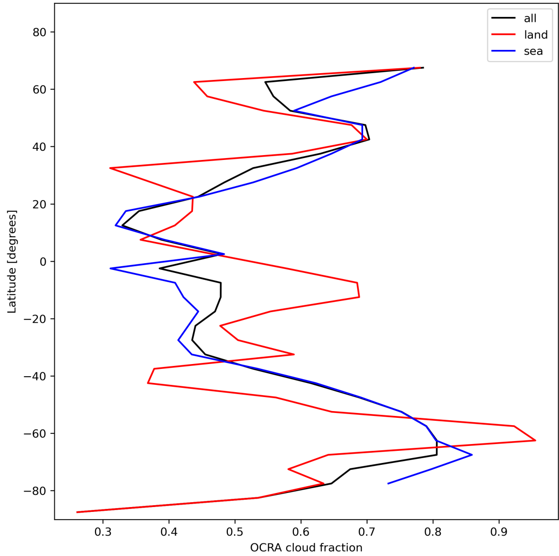
Figure 34: Zonal average of “OCRA cloud fraction” for 2024-01-10 to 2024-01-11.
