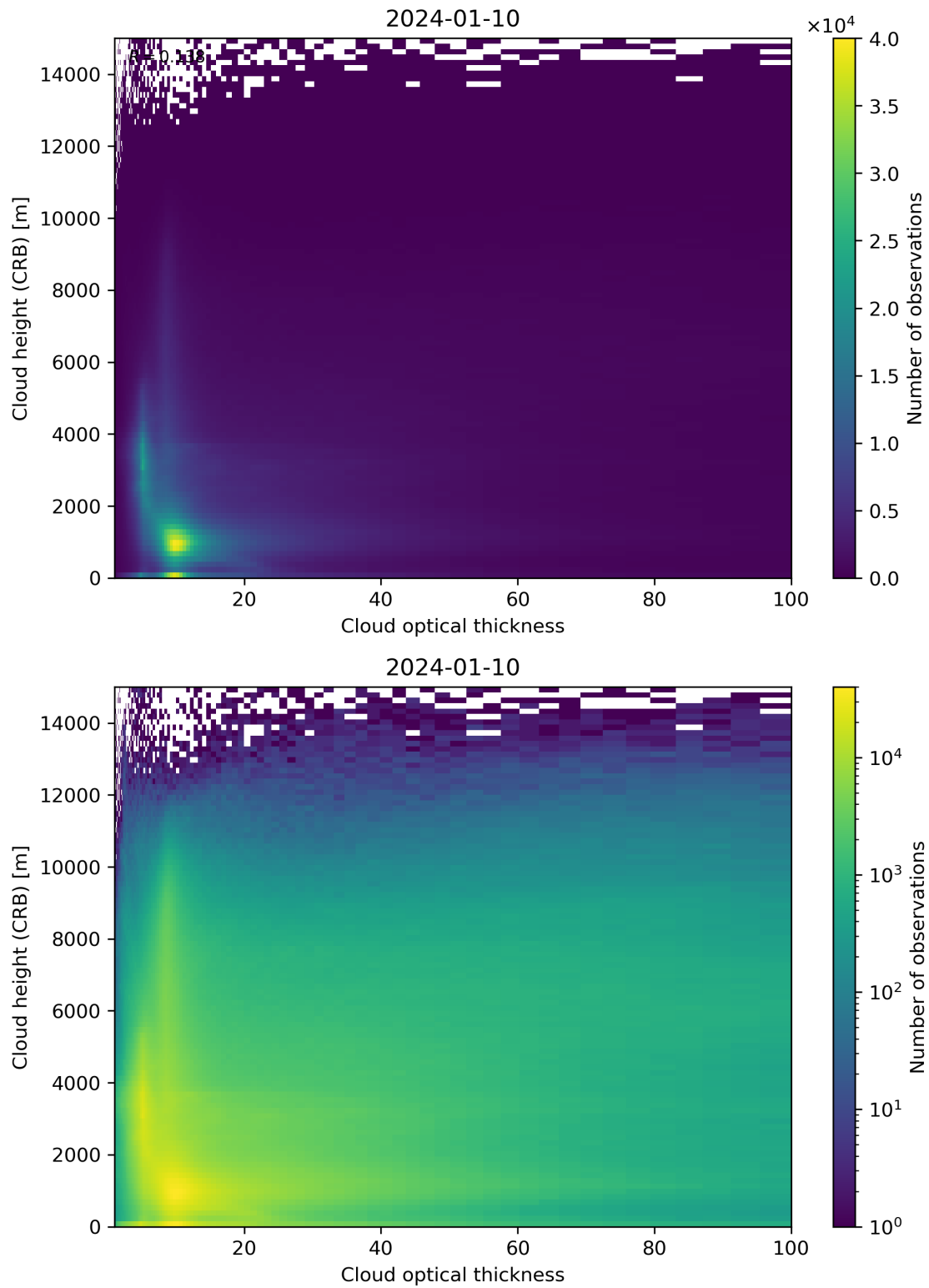
Figure 85: Scatter density plot of “Cloud optical thickness” against “Cloud height (CRB)” for 2024-01-10 to 2024-01-11.
