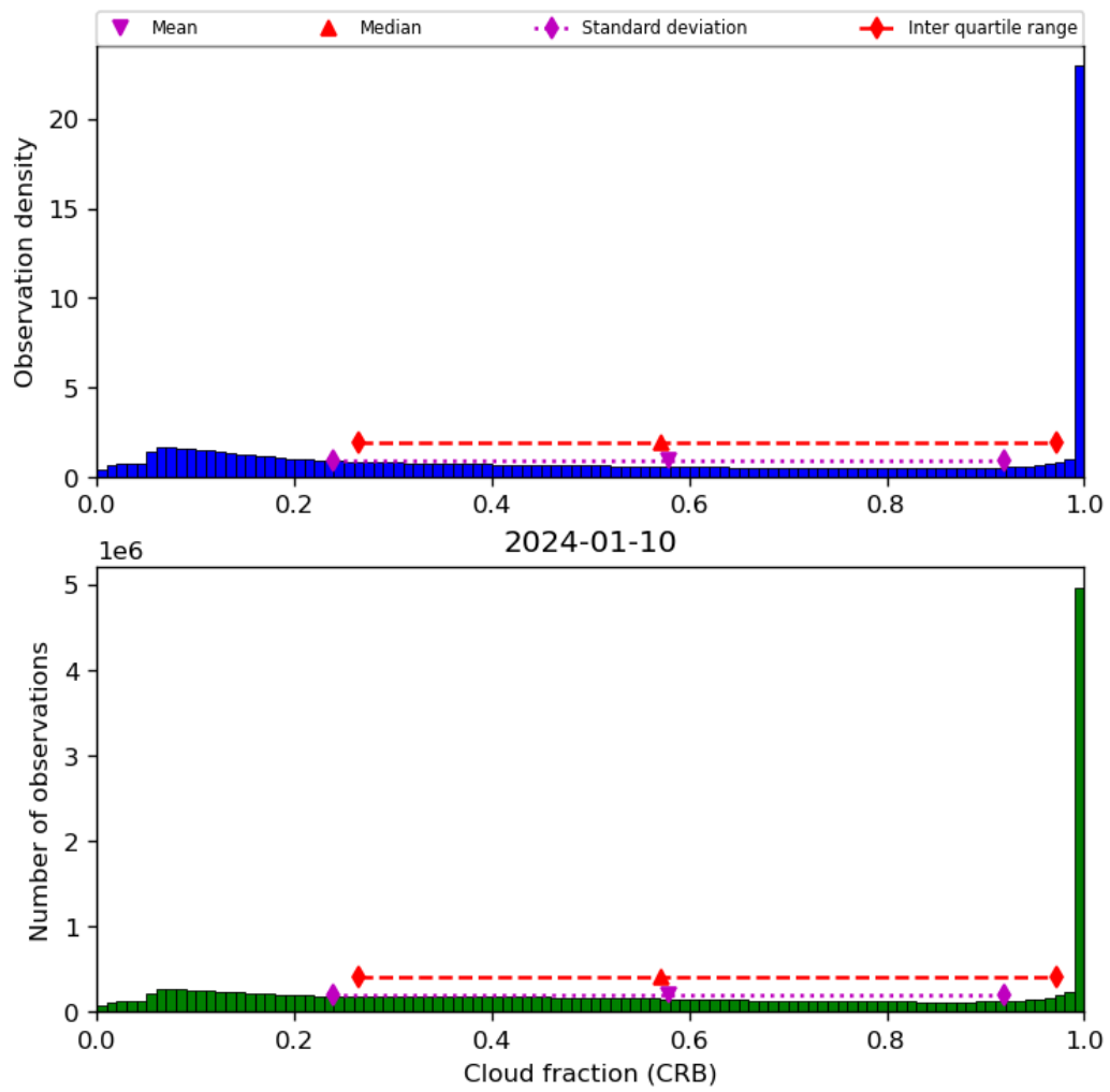
Figure 42: Histogram of “Cloud fraction (CRB)” for 2024-01-10 to 2024-01-11
