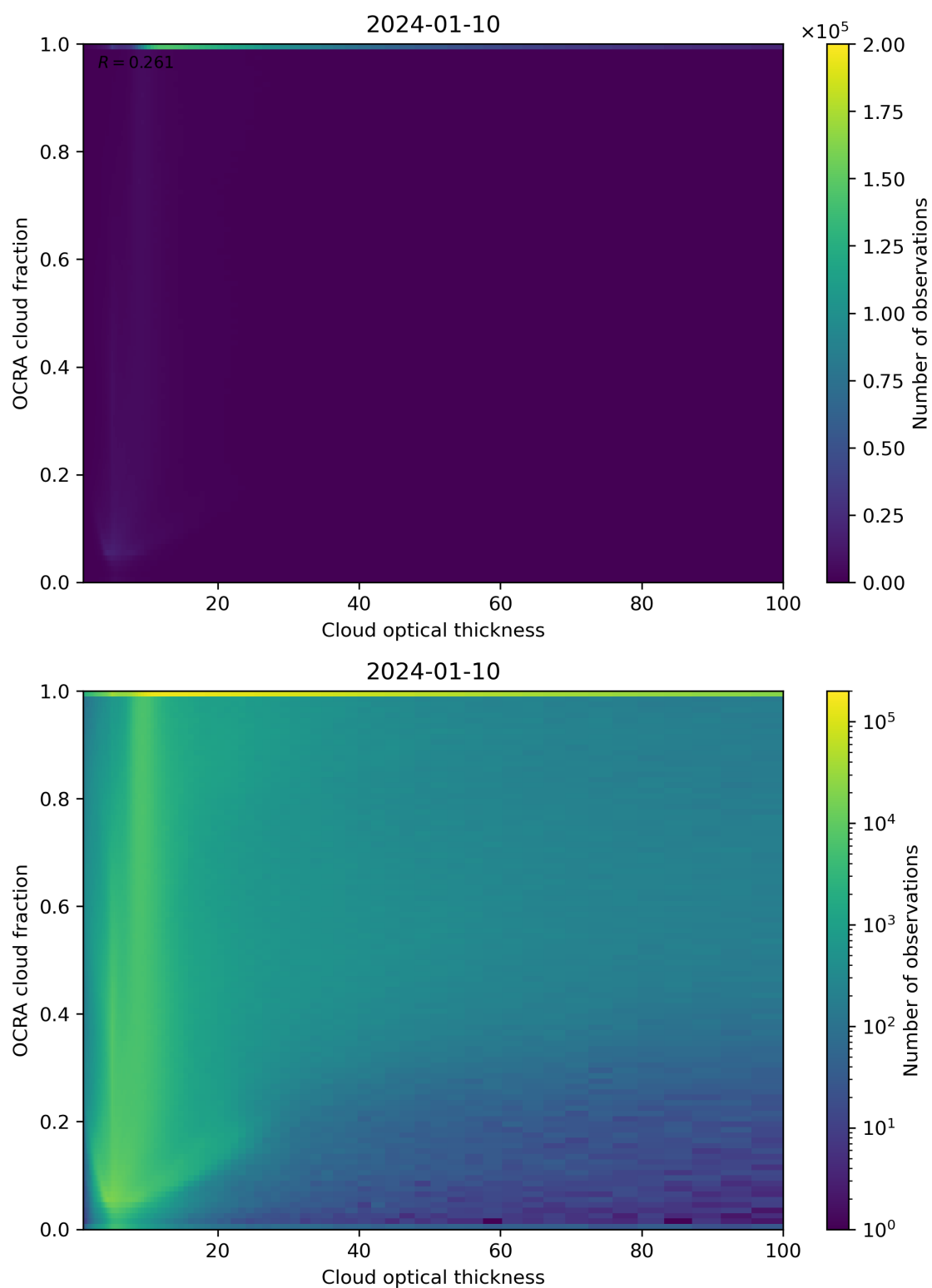
Figure 83: Scatter density plot of “Cloud optical thickness” against “OCRA cloud fraction” for 2024-01-10 to 2024-01-11.
