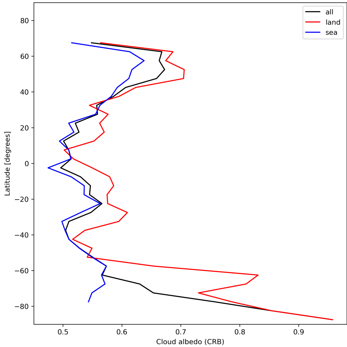
Figure 28: Zonal average of “Cloud albedo (CRB)” for 2024-01-10 to 2024-01-11.
