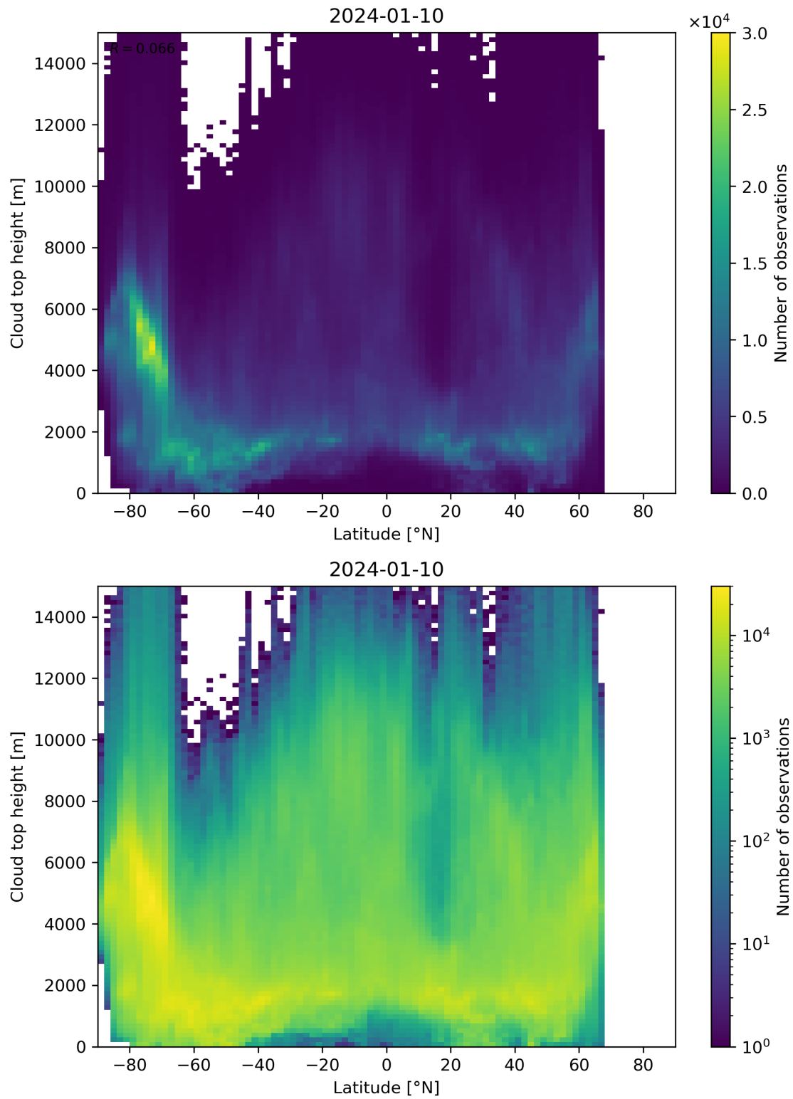
Figure 97: Scatter density plot of “Latitude” against “Cloud top height” for 2024-01-10 to 2024-01-11.
