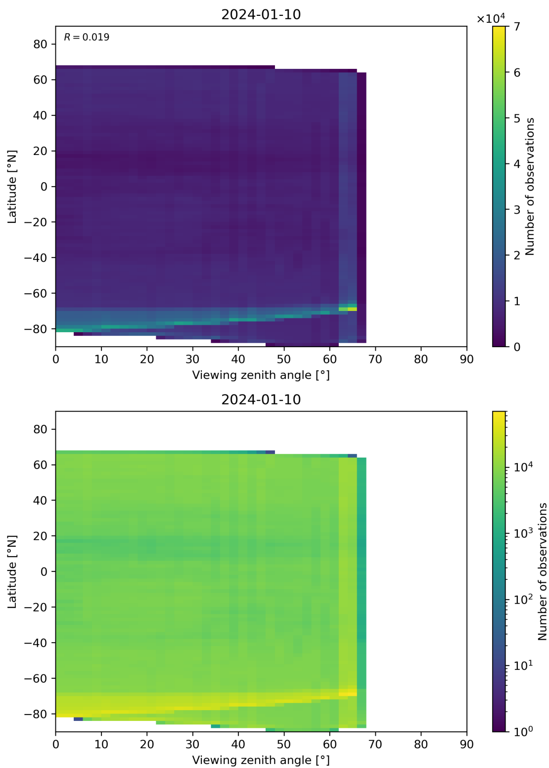
Figure 113: Scatter density plot of “Viewing zenith angle” against “Latitude” for 2024-01-10 to 2024-01-11.
