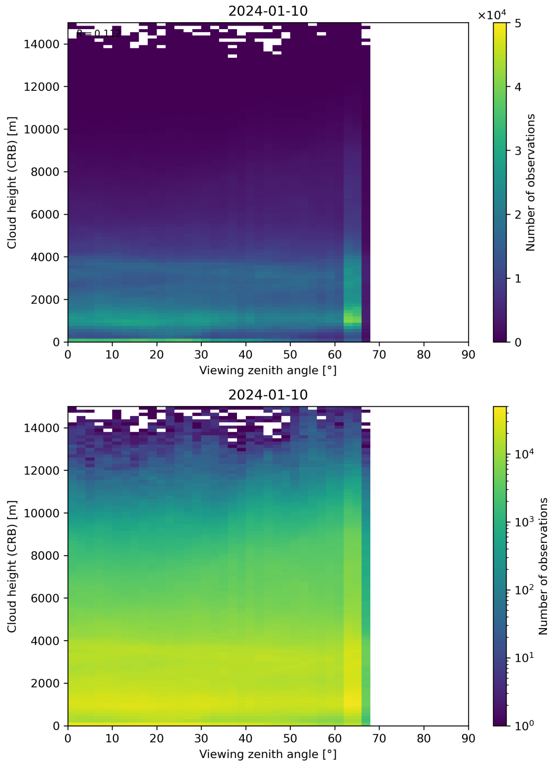
Figure 110: Scatter density plot of “Viewing zenith angle” against “Cloud height (CRB)” for 2024-01-10 to 2024-01-11.
