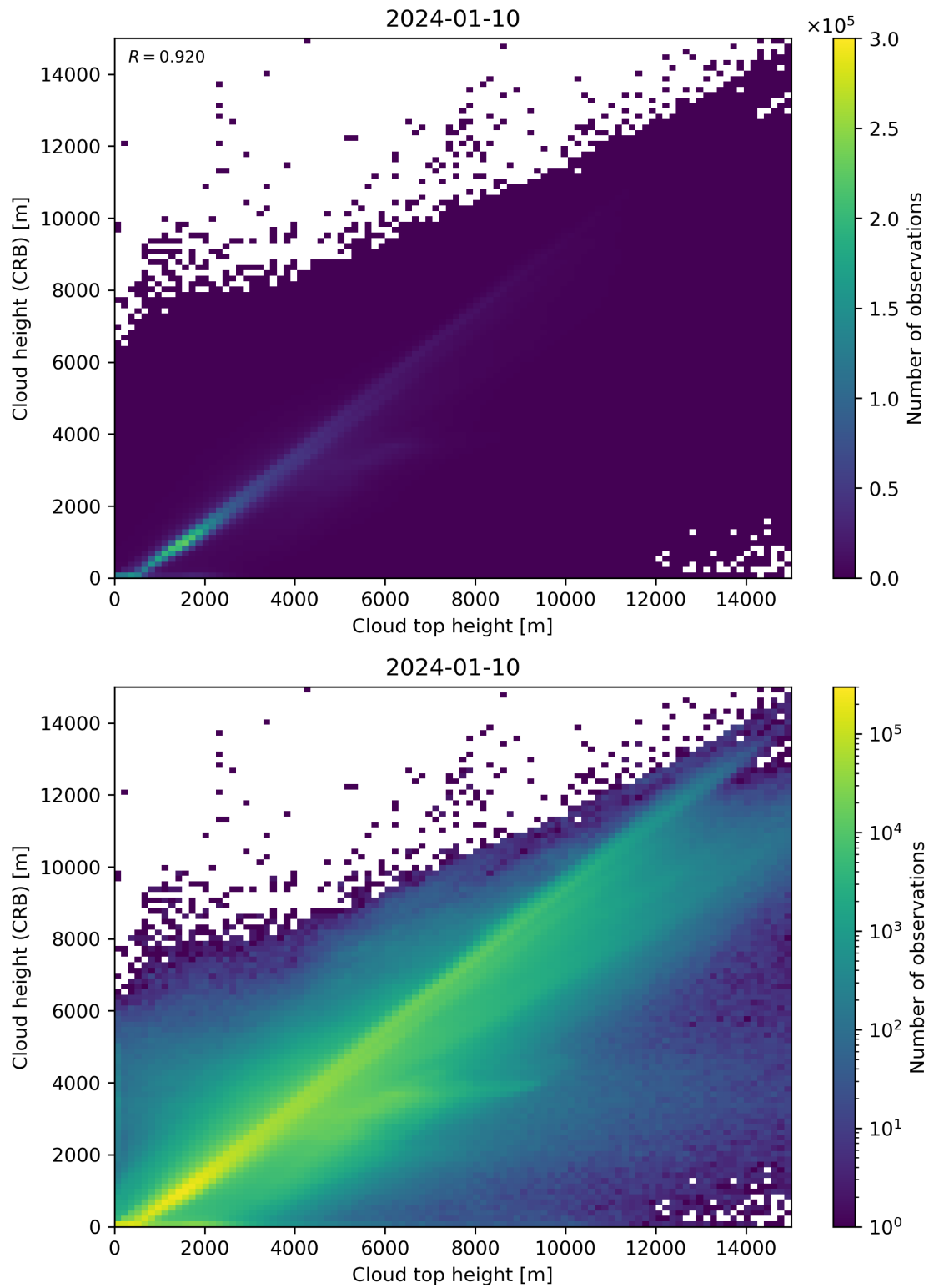
Figure 89: Scatter density plot of “Cloud top height” against “Cloud height (CRB)” for 2024-01-10 to 2024-01-11.
