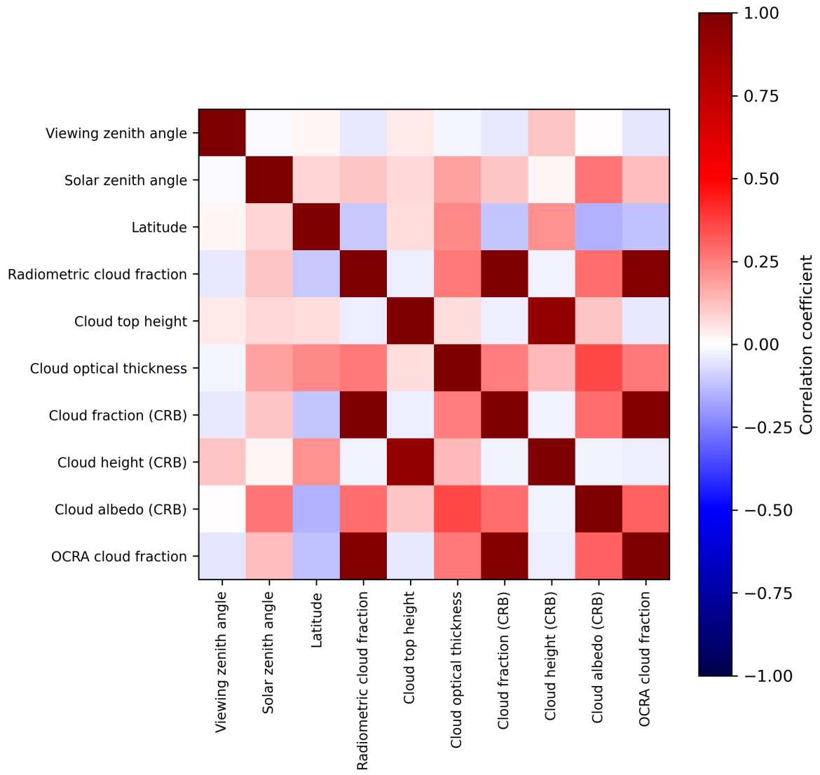
Figure 2: Map of correlation matrix for 2024-01-10 to 2024-01-11.
