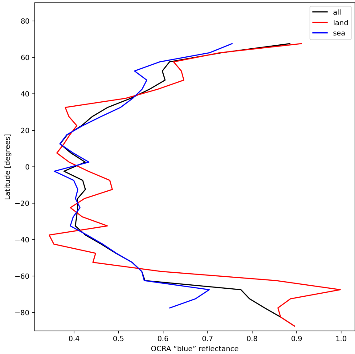
Figure 35: Zonal average of “OCRA “blue” reflectance” for 2024-01-10 to 2024-01-11.
