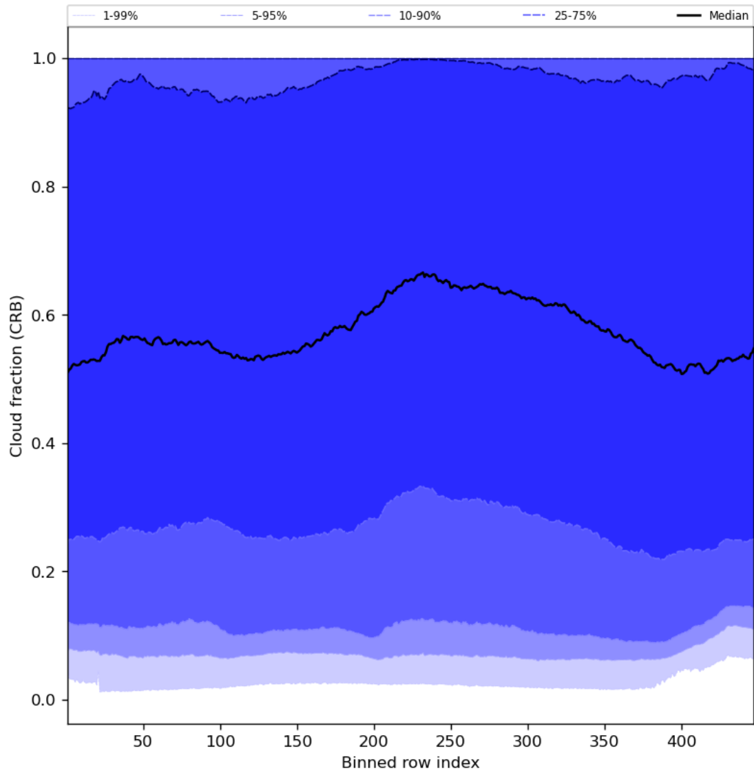
Figure 58: Along track statistics of “Cloud fraction (CRB)” for 2024-01-10 to 2024-01-11
