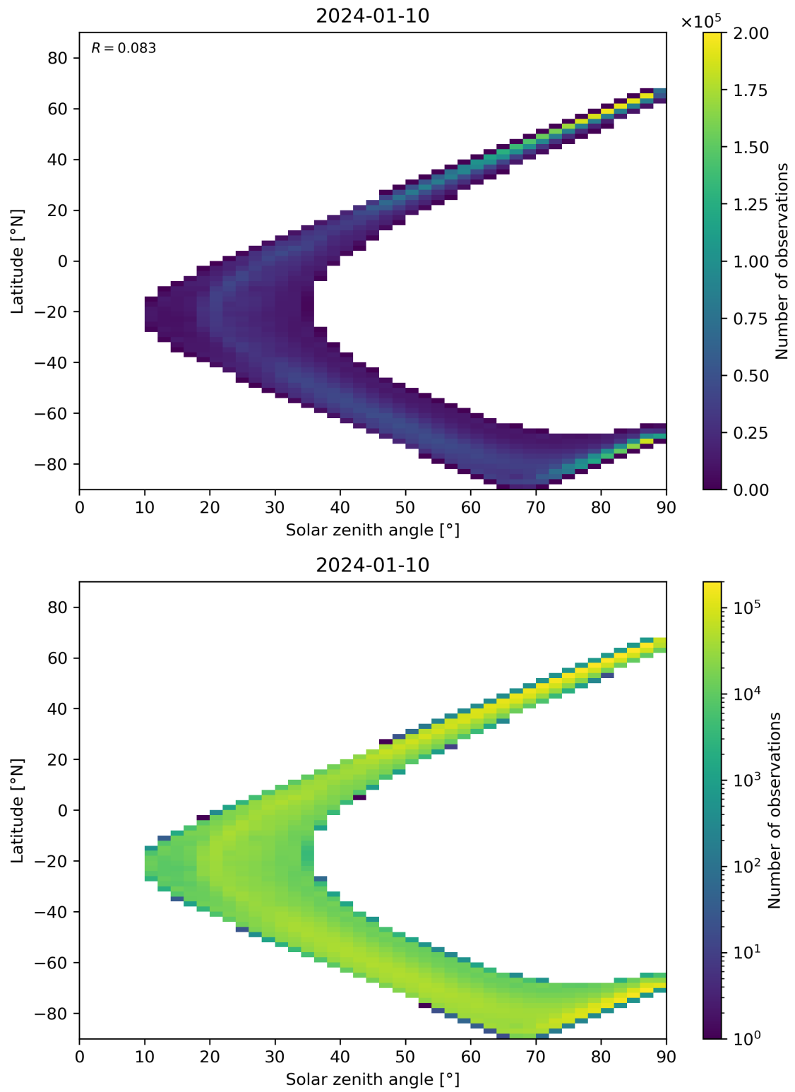
Figure 105: Scatter density plot of “Solar zenith angle” against “Latitude” for 2024-01-10 to 2024-01-11.
