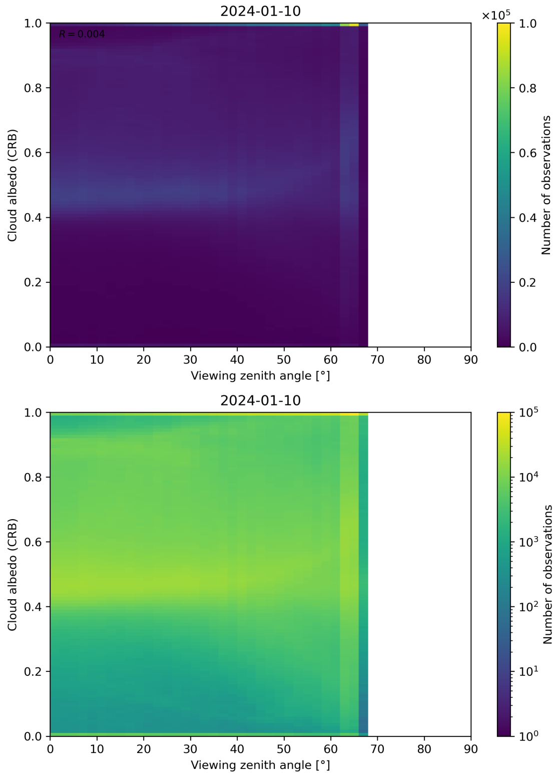
Figure 106: Scatter density plot of “Viewing zenith angle” against “Cloud albedo (CRB)” for 2024-01-10 to 2024-01-11.
