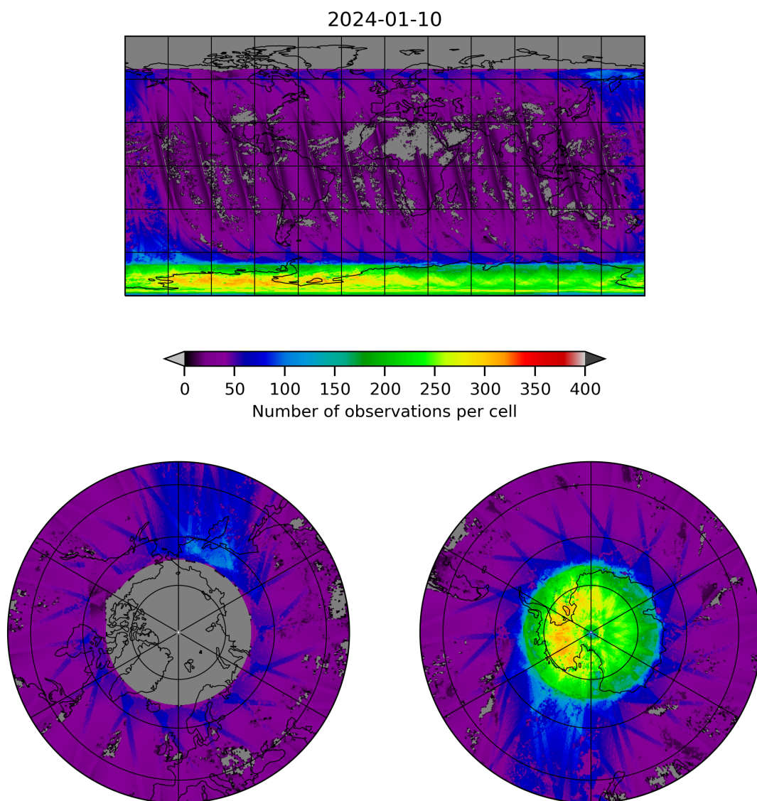
Figure 21: Map of the number of observations for 2024-01-10 to 2024-01-11
