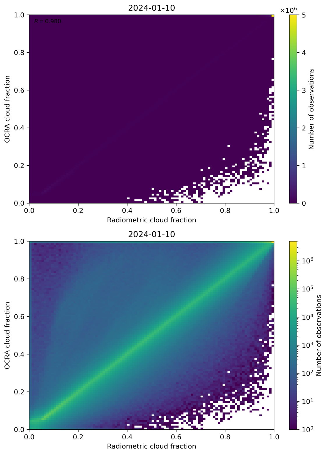
Figure 72: Scatter density plot of “Radiometric cloud fraction” against “OCRA cloud fraction” for 2024-01-10 to 2024-01-11.
