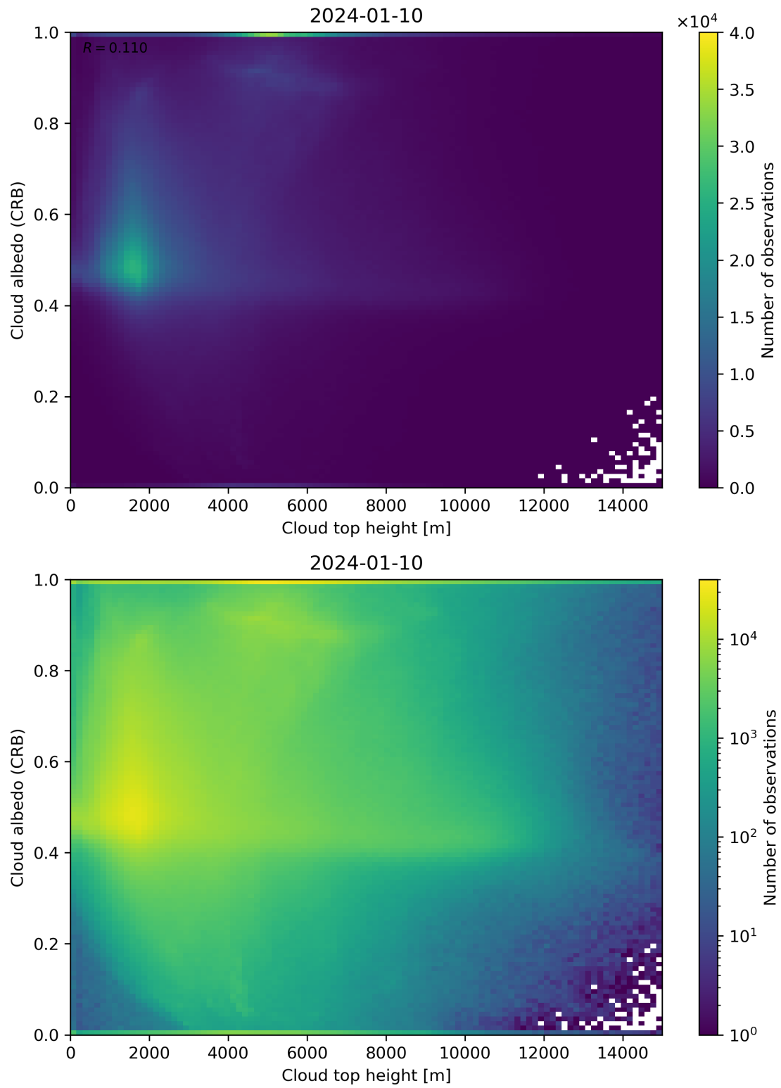
Figure 86: Scatter density plot of “Cloud top height” against “Cloud albedo (CRB)” for 2024-01-10 to 2024-01-11.
