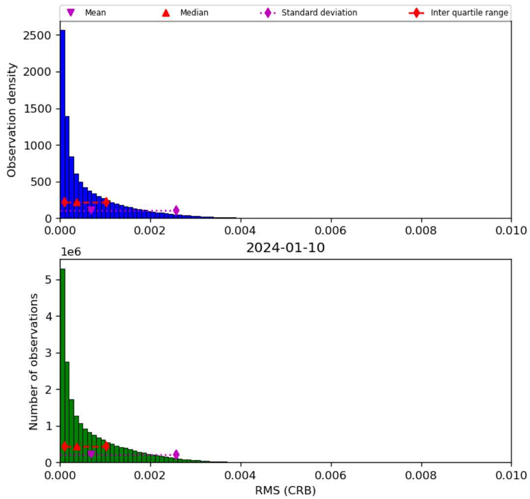
Figure 48: Histogram of “RMS (CRB)” for 2024-01-10 to 2024-01-11
