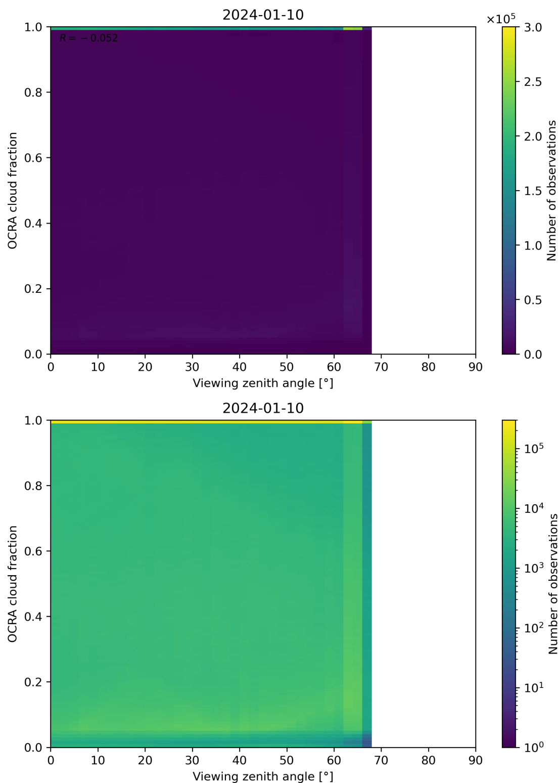
Figure 108: Scatter density plot of “Viewing zenith angle” against “OCRA cloud fraction” for 2024-01-10 to 2024-01-11.
