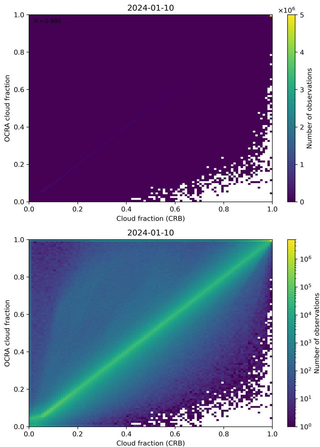
Figure 78: Scatter density plot of “Cloud fraction (CRB)” against “OCRA cloud fraction” for 2024-01-10 to 2024-01-11.
