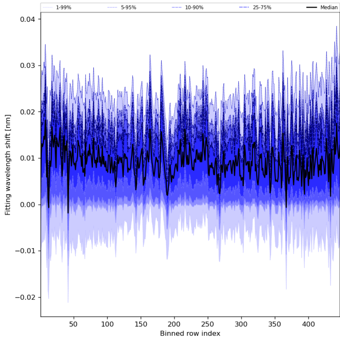
Figure 65: Along track statistics of “Fitting wavelength shift” for 2024-01-10 to 2024-01-11
