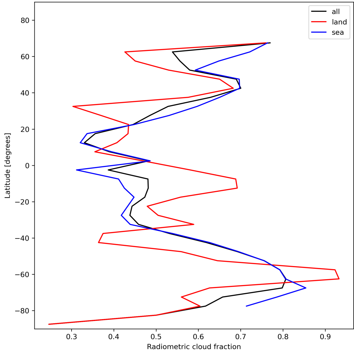
Figure 23: Zonal average of “Radiometric cloud fraction” for 2024-01-10 to 2024-01-11.
