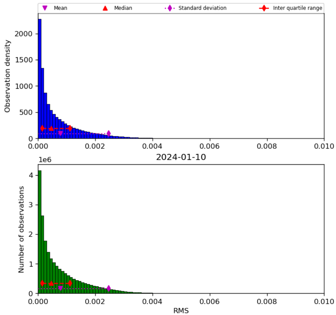
Figure 47: Histogram of “RMS” for 2024-01-10 to 2024-01-11
