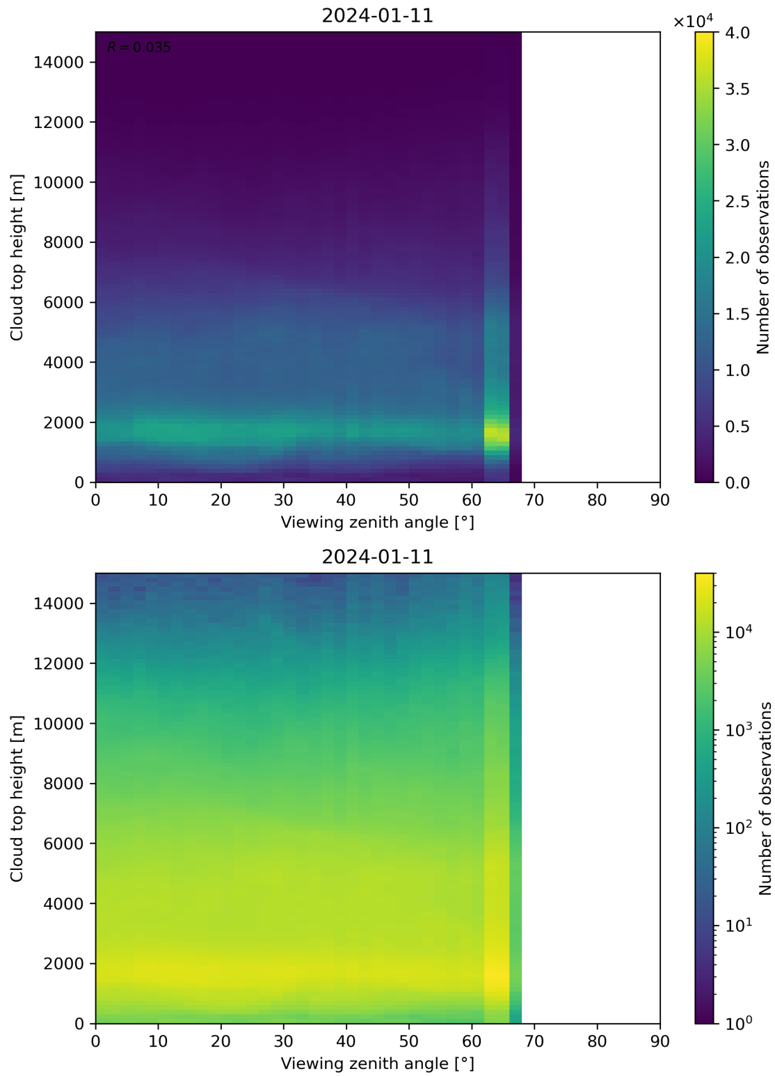
Figure 112: Scatter density plot of “Viewing zenith angle” against “Cloud top height” for 2024-01-10 to 2024-01-12.
