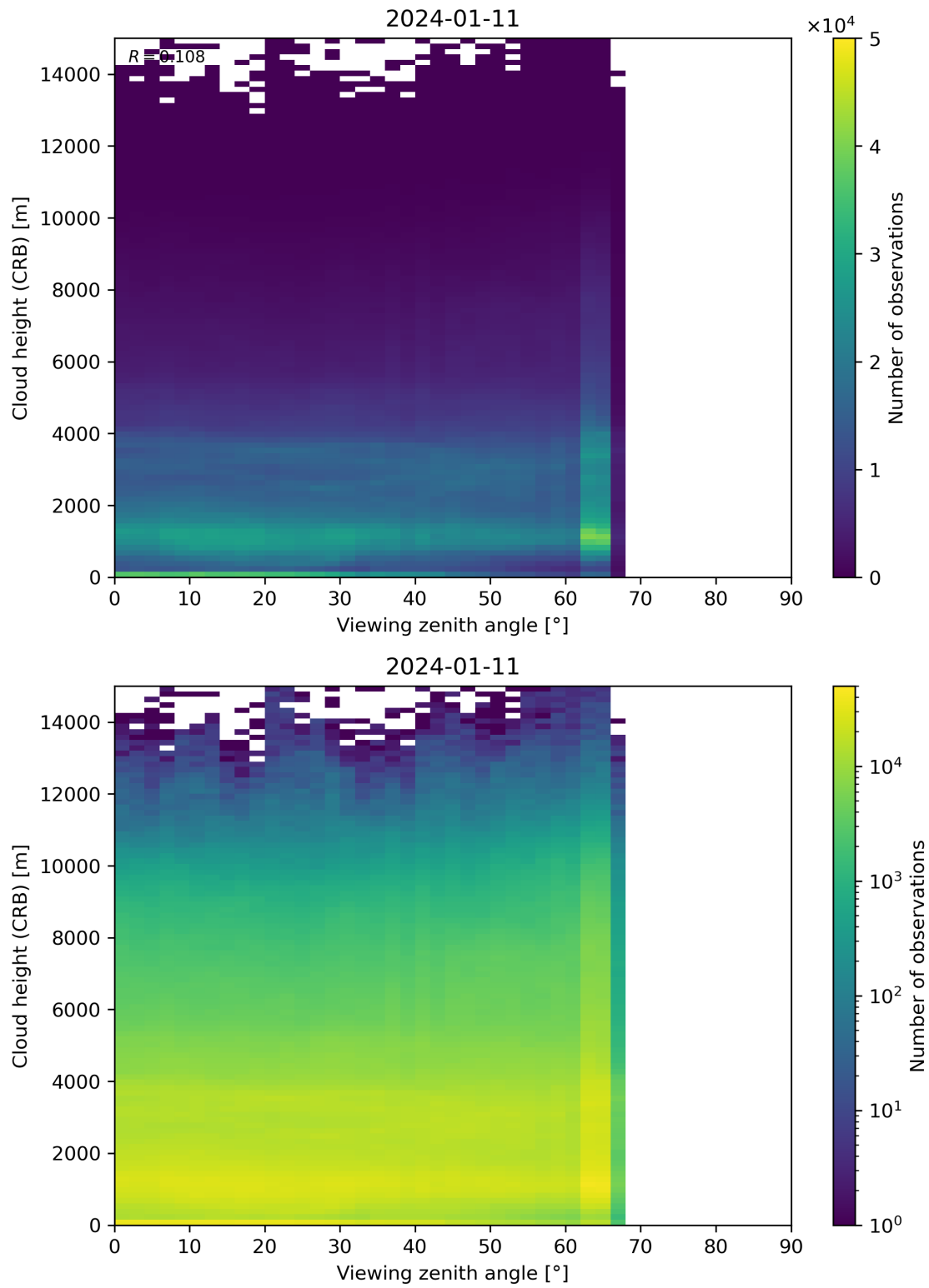
Figure 110: Scatter density plot of “Viewing zenith angle” against “Cloud height (CRB)” for 2024-01-10 to 2024-01-12.
