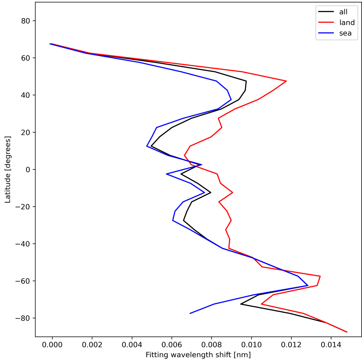
Figure 33: Zonal average of “Fitting wavelength shift” for 2024-01-10 to 2024-01-12.
