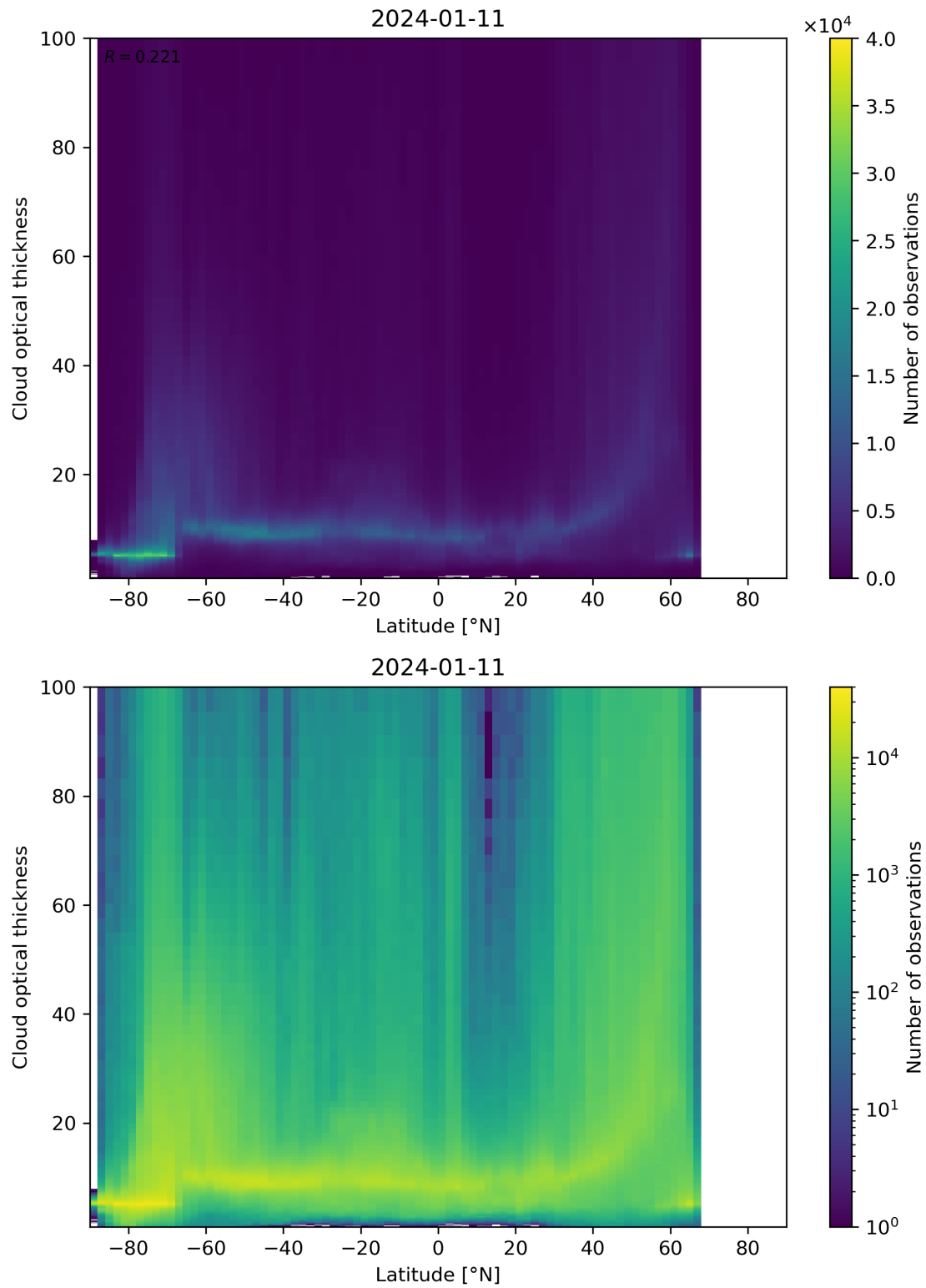
Figure 96: Scatter density plot of “Latitude” against “Cloud optical thickness” for 2024-01-10 to 2024-01-12.
