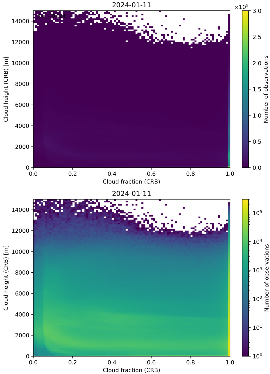
Figure 79: Scatter density plot of “Cloud fraction (CRB)” against “Cloud height (CRB)” for 2024-01-10 to 2024-01-12.
