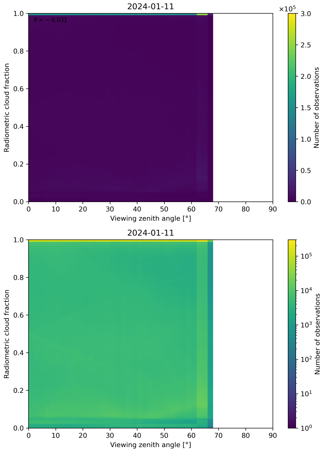
Figure 107: Scatter density plot of “Viewing zenith angle” against “Radiometric cloud fraction” for 2024-01-10 to 2024-01-12.
