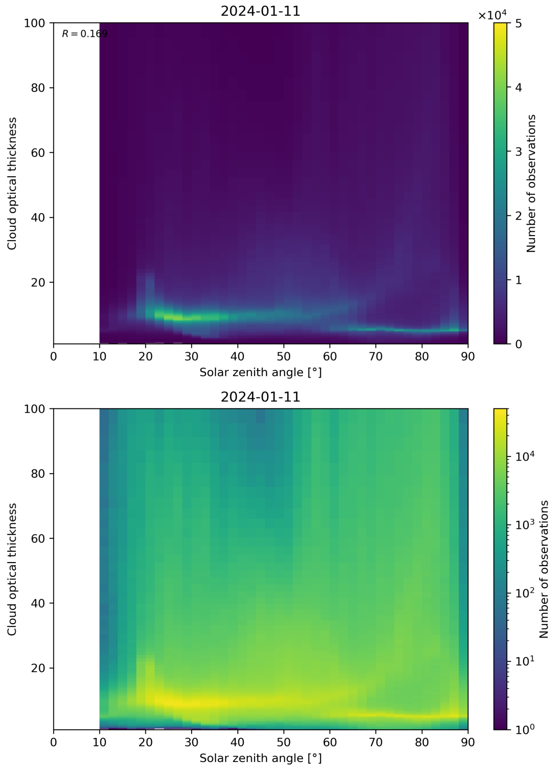
Figure 103: Scatter density plot of “Solar zenith angle” against “Cloud optical thickness” for 2024-01-10 to 2024-01-12.
