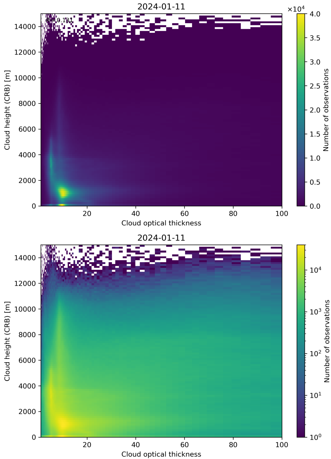
Figure 85: Scatter density plot of “Cloud optical thickness” against “Cloud height (CRB)” for 2024-01-10 to 2024-01-12.
