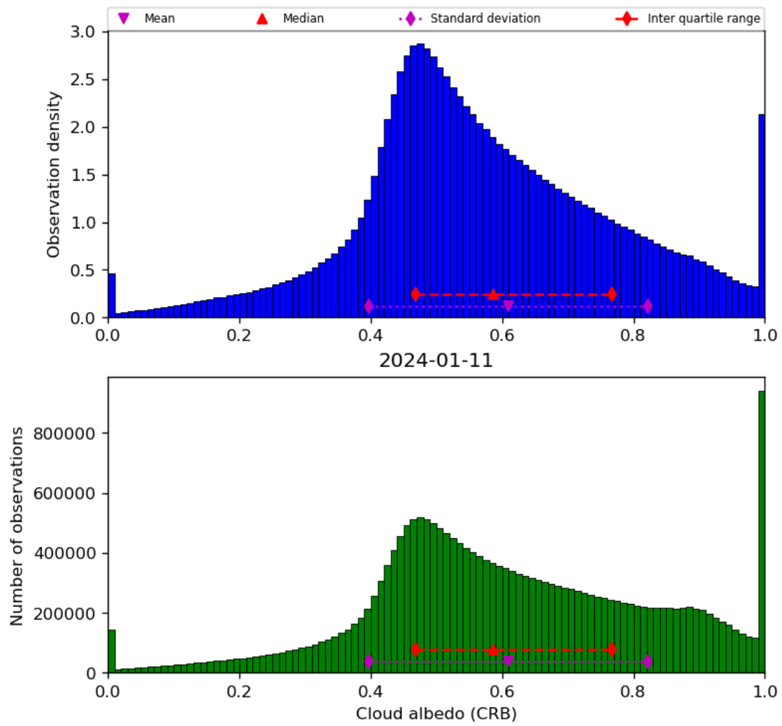
Figure 44: Histogram of “Cloud albedo (CRB)” for 2024-01-10 to 2024-01-12
