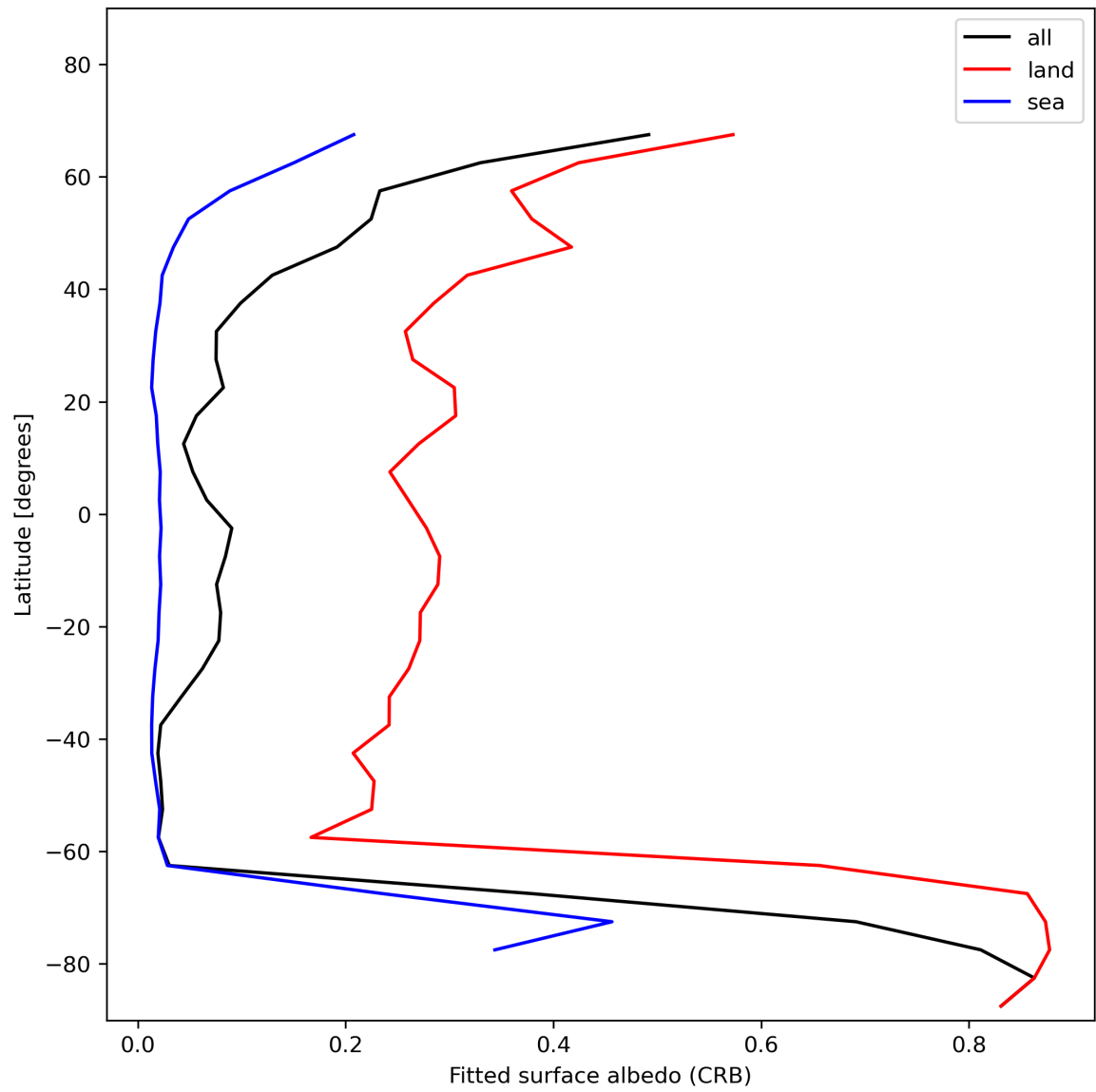
Figure 30: Zonal average of “Fitted surface albedo (CRB)” for 2024-01-10 to 2024-01-12.
