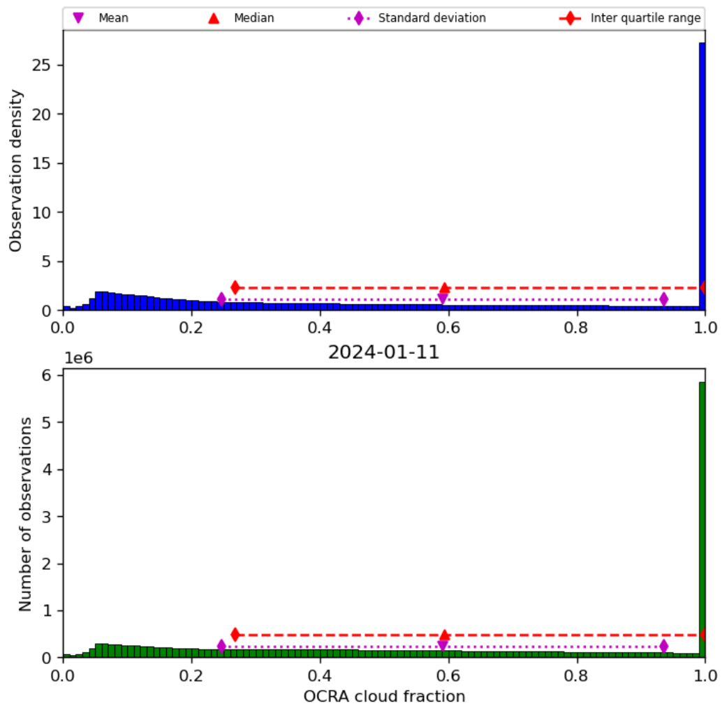
Figure 50: Histogram of “OCRA cloud fraction” for 2024-01-10 to 2024-01-12
