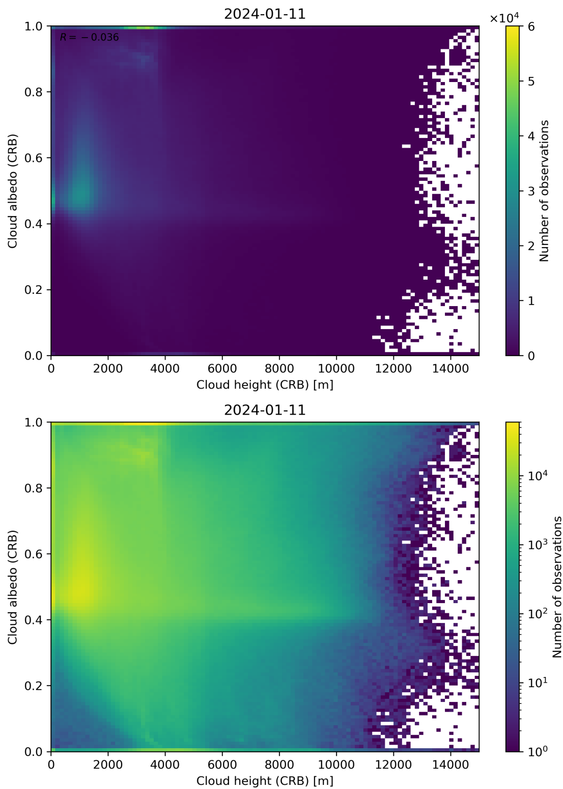
Figure 80: Scatter density plot of “Cloud height (CRB)” against “Cloud albedo (CRB)” for 2024-01-10 to 2024-01-12.
