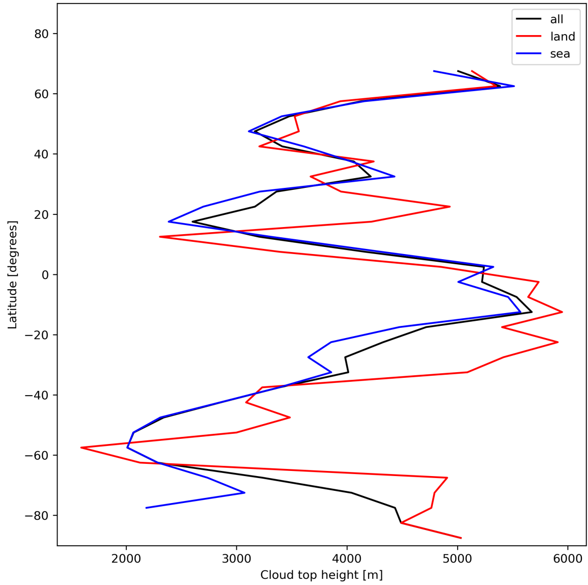
Figure 24: Zonal average of “Cloud top height” for 2024-01-10 to 2024-01-12.
