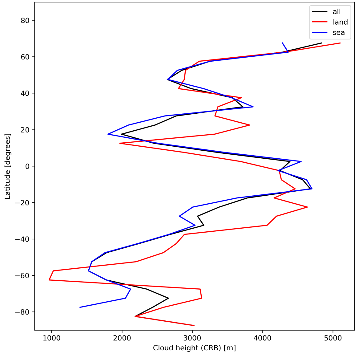
Figure 27: Zonal average of “Cloud height (CRB)” for 2024-01-10 to 2024-01-12.
