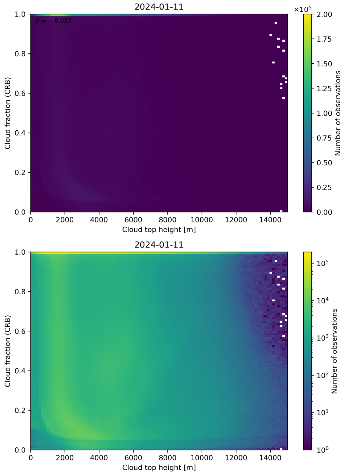
Figure 88: Scatter density plot of “Cloud top height” against “Cloud fraction (CRB)” for 2024-01-10 to 2024-01-12.
