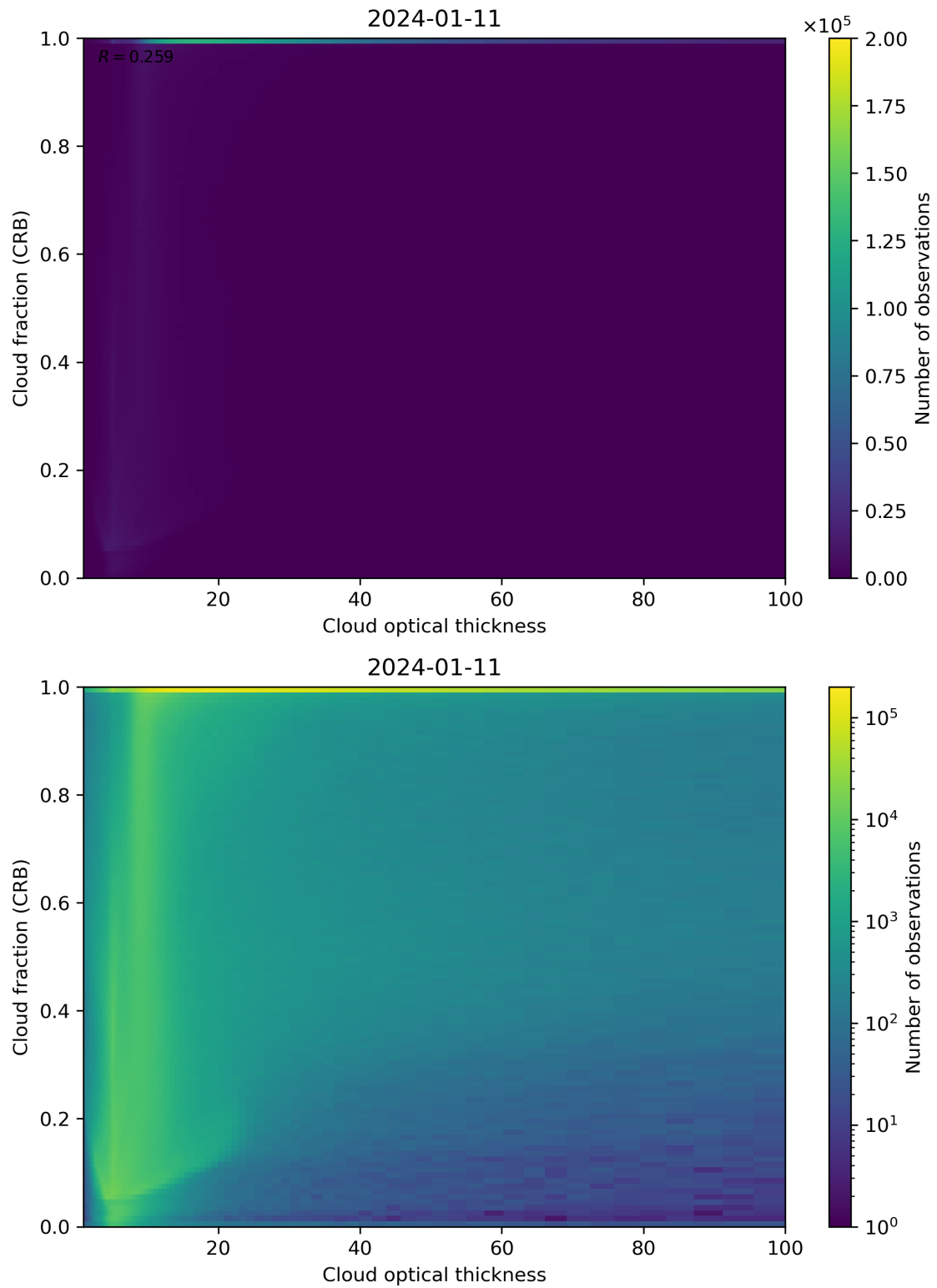
Figure 84: Scatter density plot of “Cloud optical thickness” against “Cloud fraction (CRB)” for 2024-01-10 to 2024-01-12.
