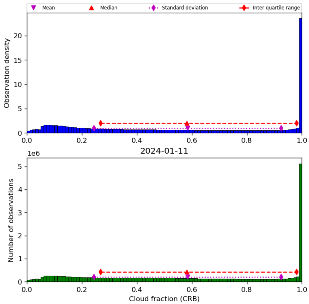
Figure 42: Histogram of “Cloud fraction (CRB)” for 2024-01-10 to 2024-01-12
