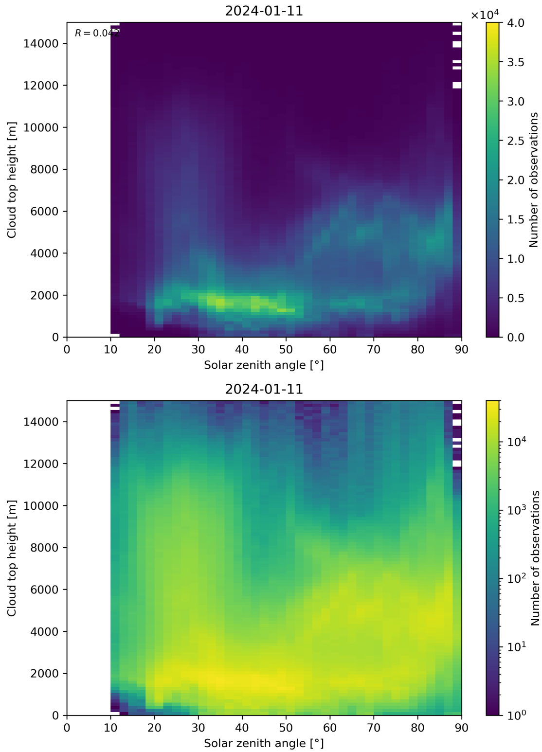
Figure 104: Scatter density plot of “Solar zenith angle” against “Cloud top height” for 2024-01-10 to 2024-01-12.
