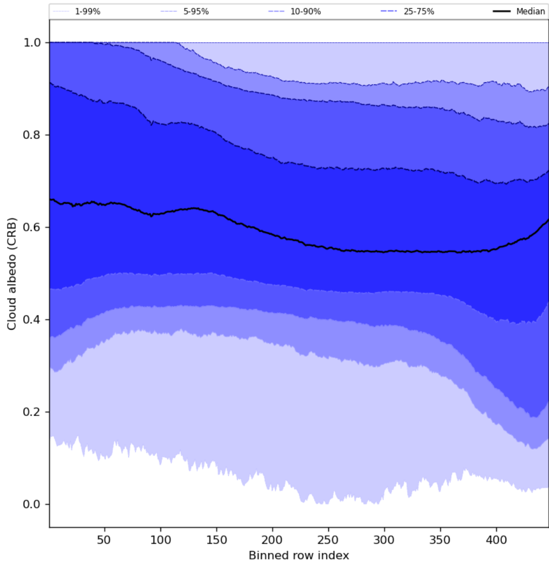
Figure 60: Along track statistics of “Cloud albedo (CRB)” for 2024-01-10 to 2024-01-12
