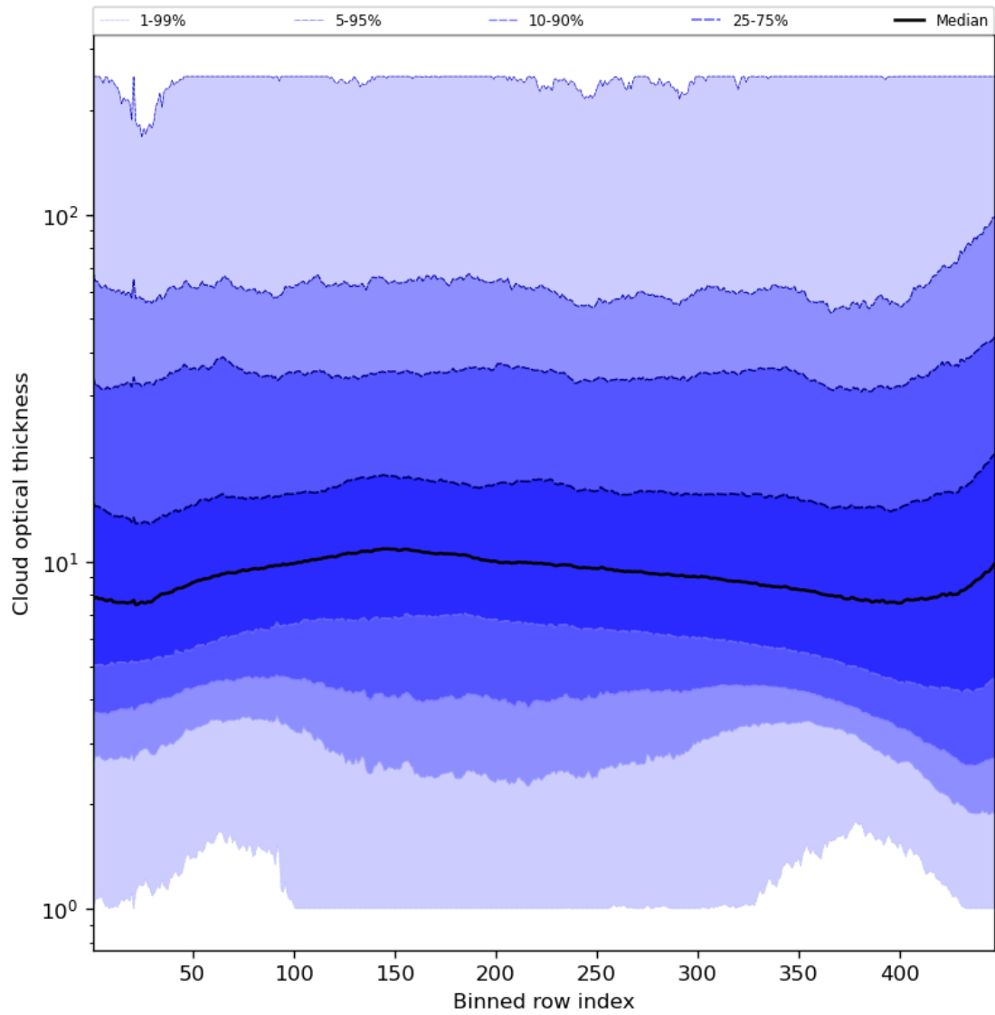
Figure 57: Along track statistics of “Cloud optical thickness” for 2024-01-10 to 2024-01-12
