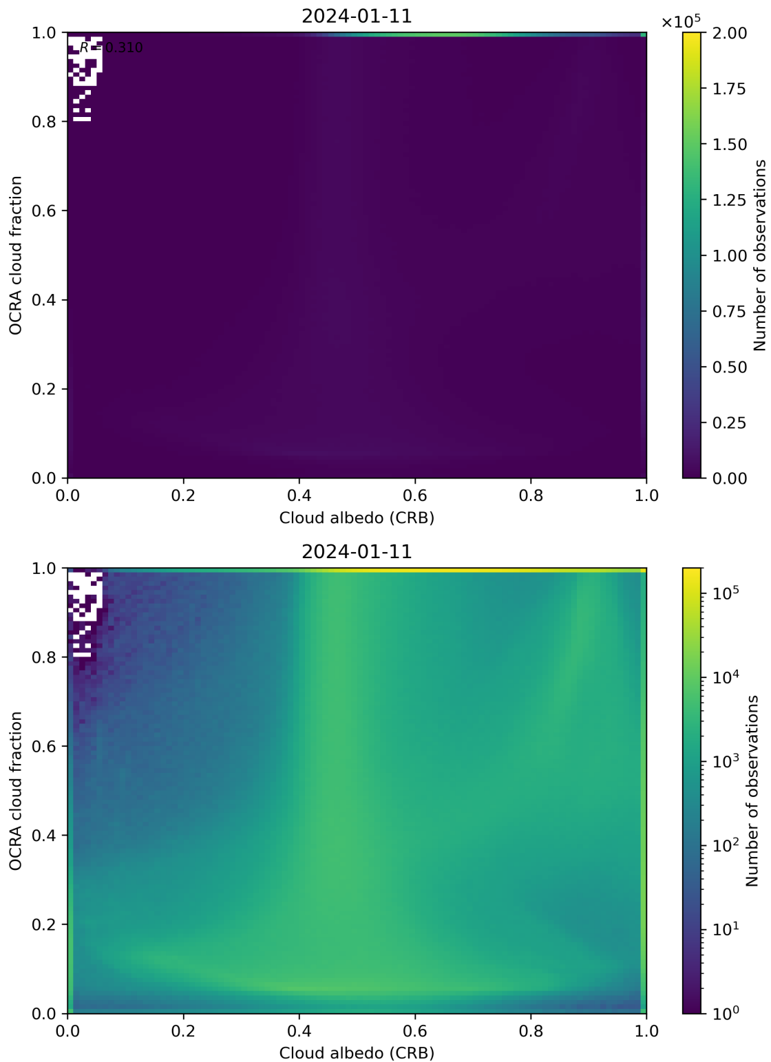
Figure 70: Scatter density plot of “Cloud albedo (CRB)” against “OCRA cloud fraction” for 2024-01-10 to 2024-01-12.
