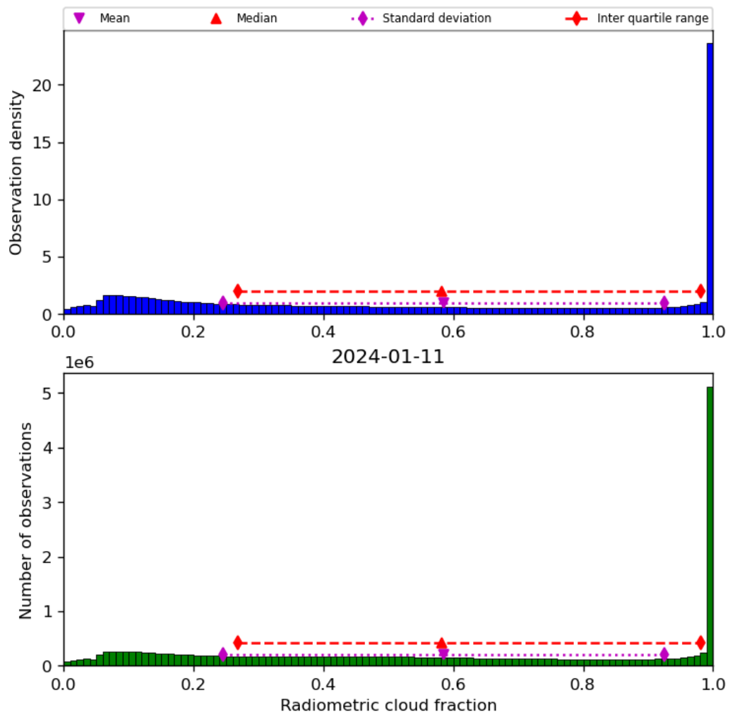
Figure 39: Histogram of “Radiometric cloud fraction” for 2024-01-10 to 2024-01-12
