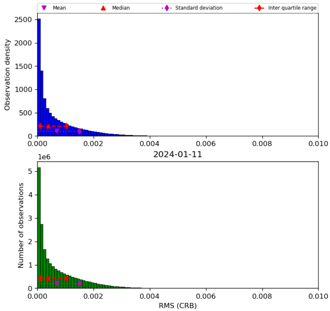
Figure 48: Histogram of “RMS (CRB)” for 2024-01-10 to 2024-01-12
