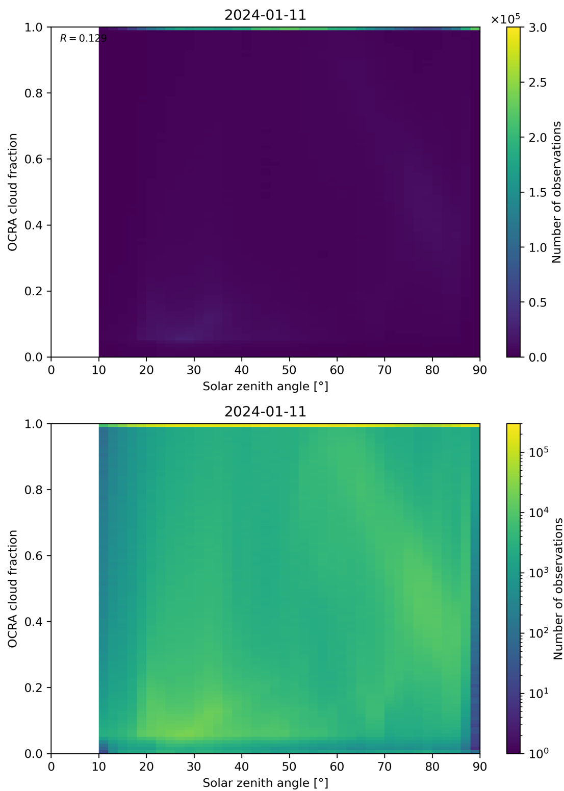
Figure 100: Scatter density plot of “Solar zenith angle” against “OCRA cloud fraction” for 2024-01-10 to 2024-01-12.
