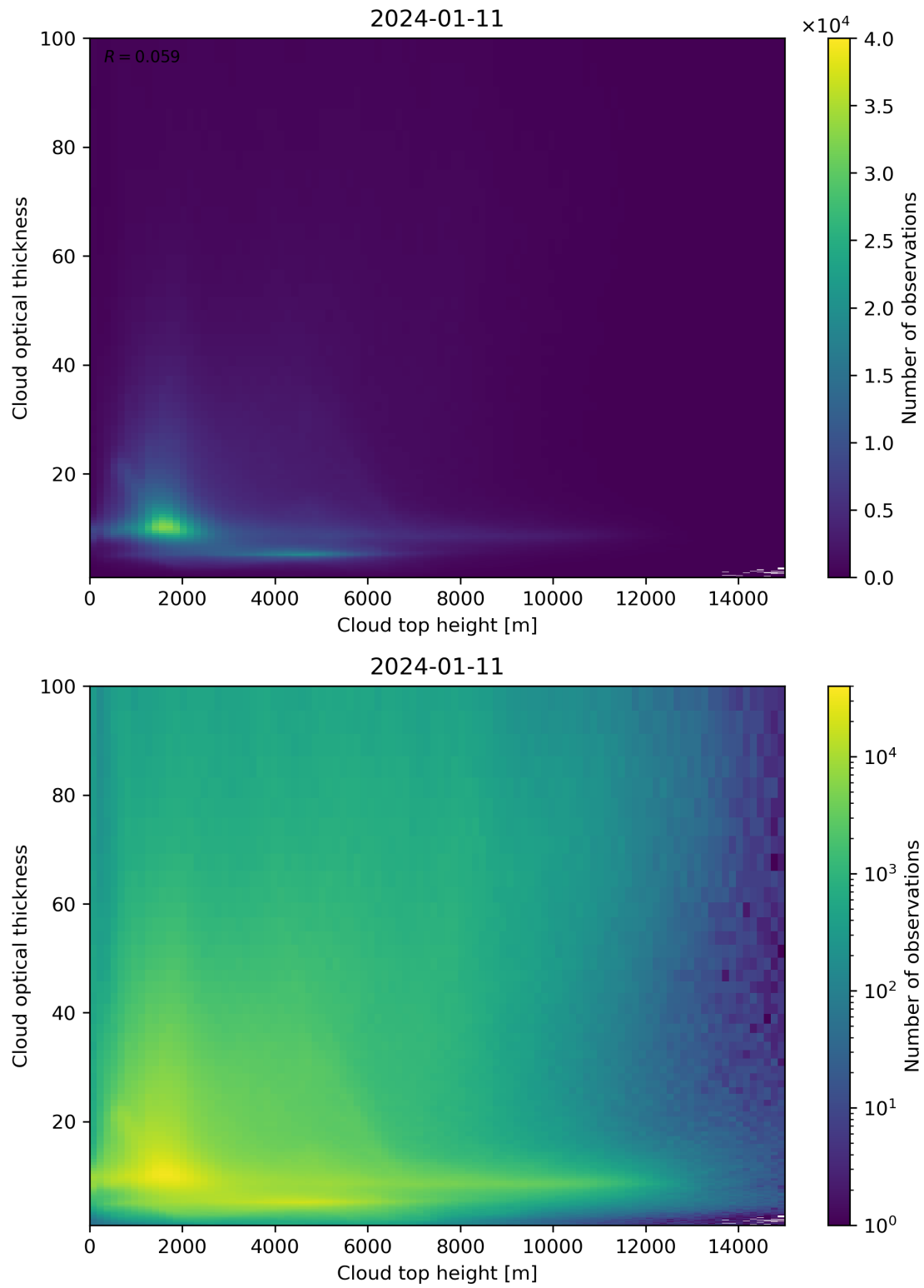
Figure 90: Scatter density plot of “Cloud top height” against “Cloud optical thickness” for 2024-01-10 to 2024-01-12.
