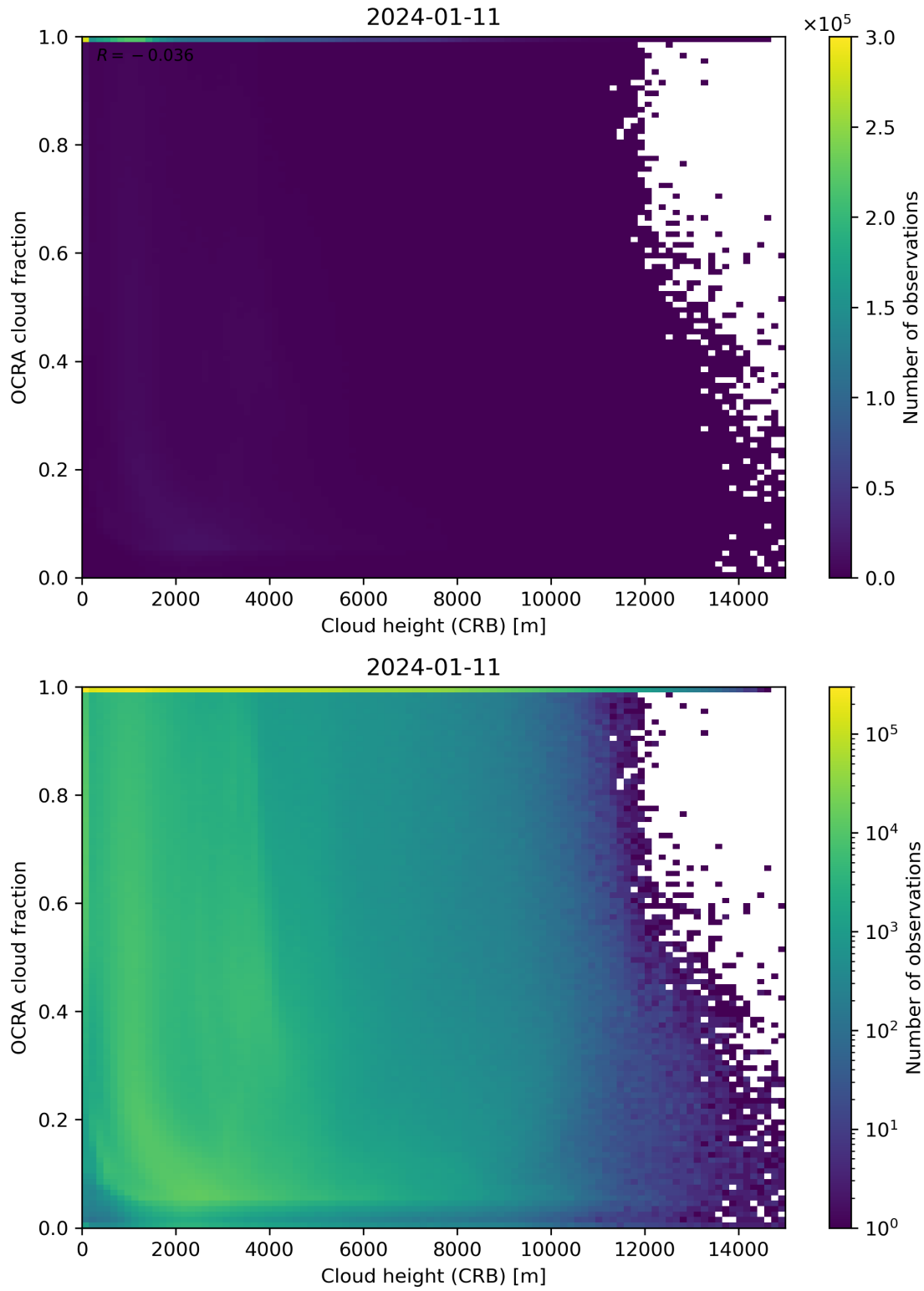
Figure 81: Scatter density plot of “Cloud height (CRB)” against “OCRA cloud fraction” for 2024-01-10 to 2024-01-12.
