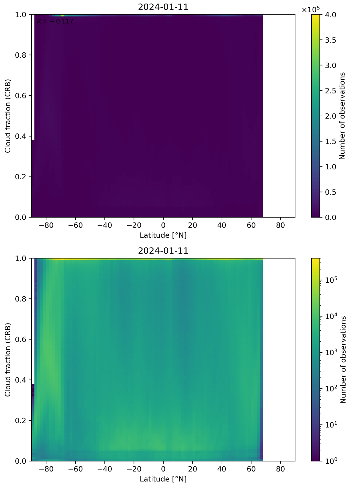
Figure 94: Scatter density plot of “Latitude” against “Cloud fraction (CRB)” for 2024-01-10 to 2024-01-12.
