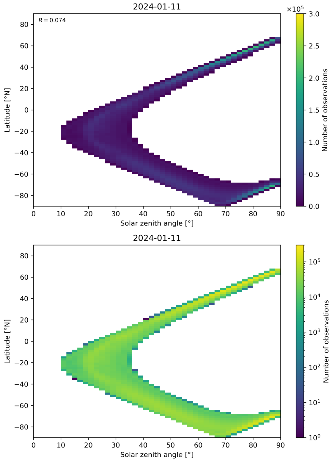
Figure 105: Scatter density plot of “Solar zenith angle” against “Latitude” for 2024-01-10 to 2024-01-12.
