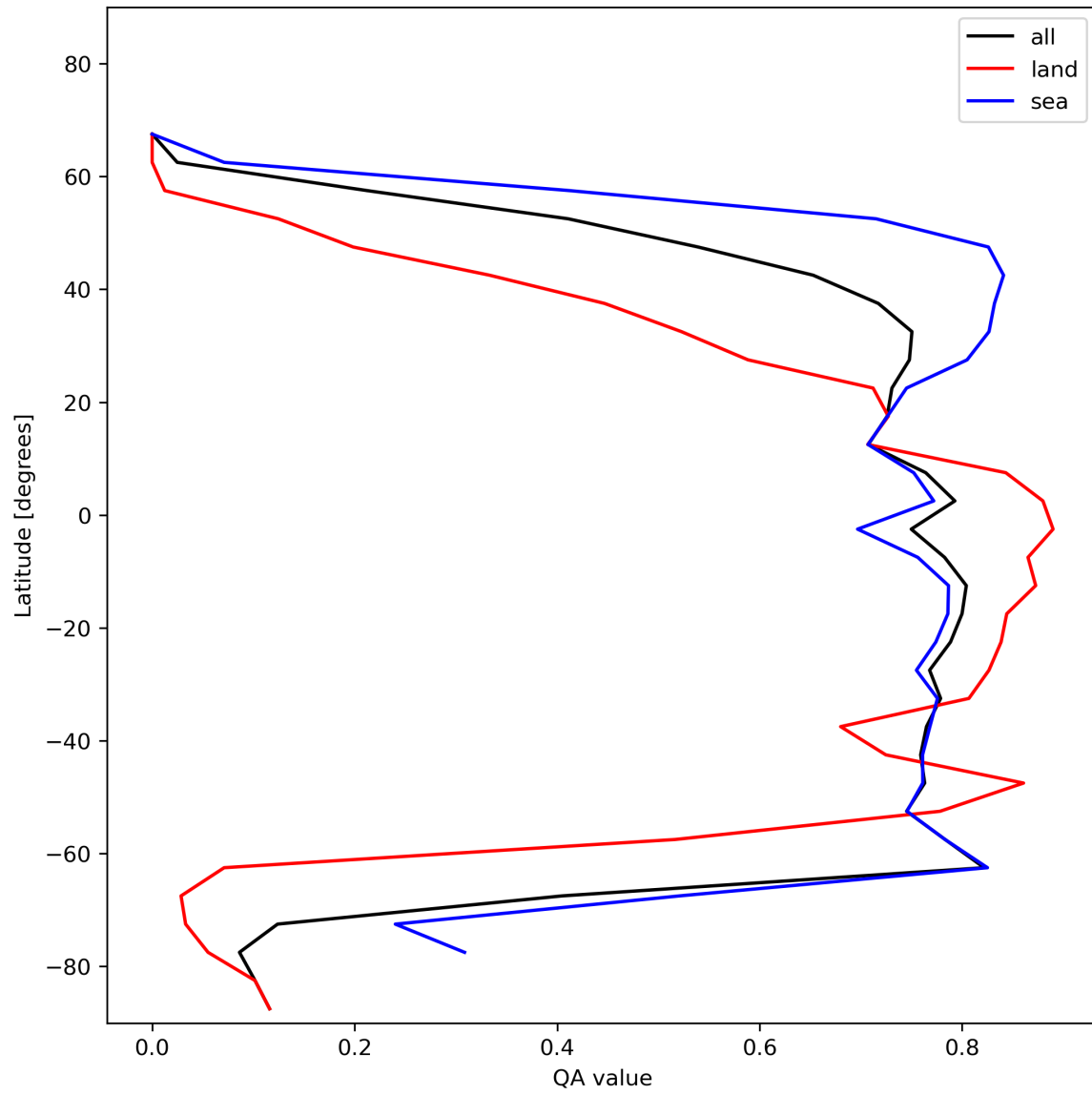
Figure 22: Zonal average of “QA value” for 2024-01-10 to 2024-01-12.
