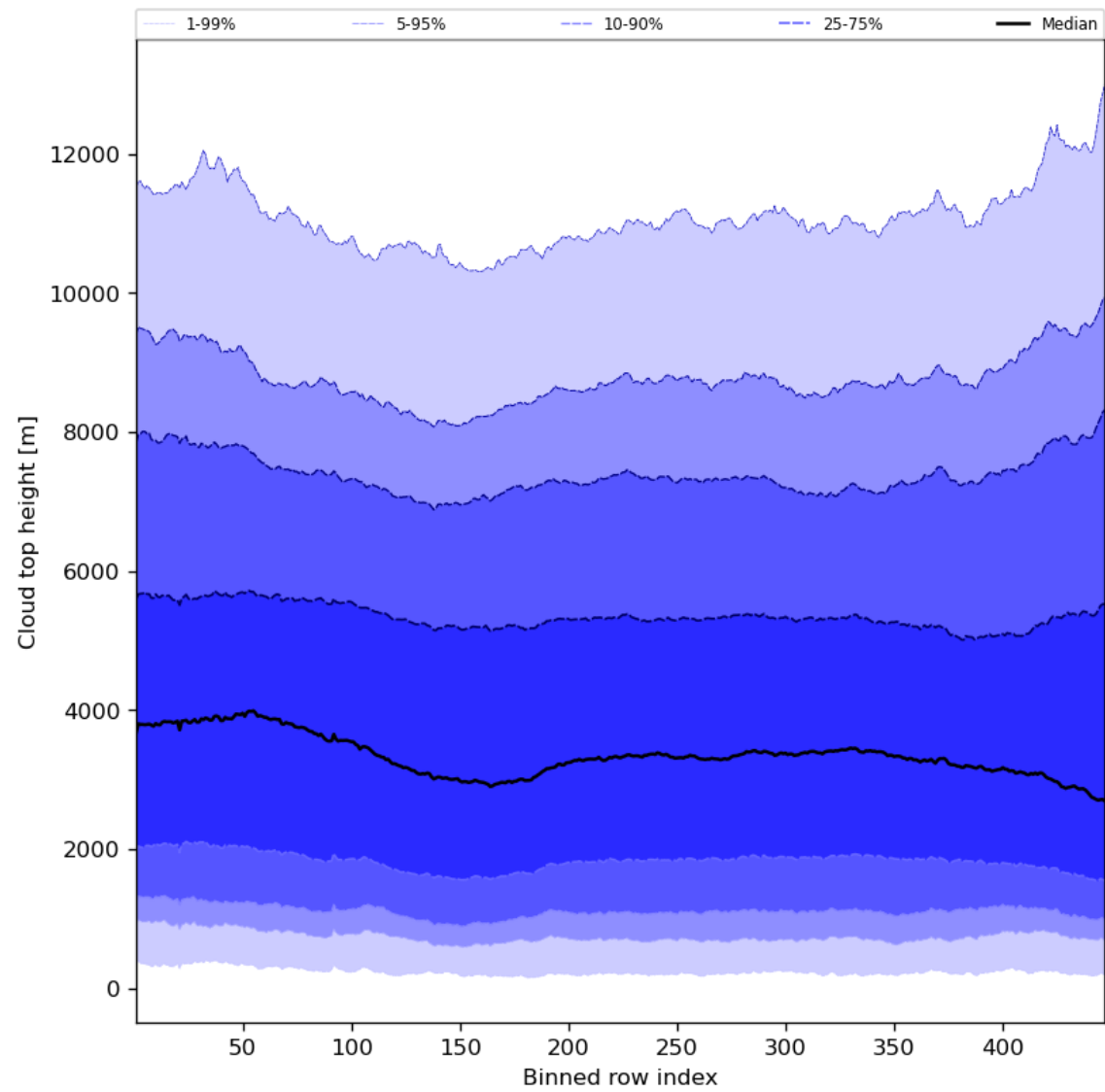
Figure 56: Along track statistics of “Cloud top height” for 2024-01-10 to 2024-01-12
