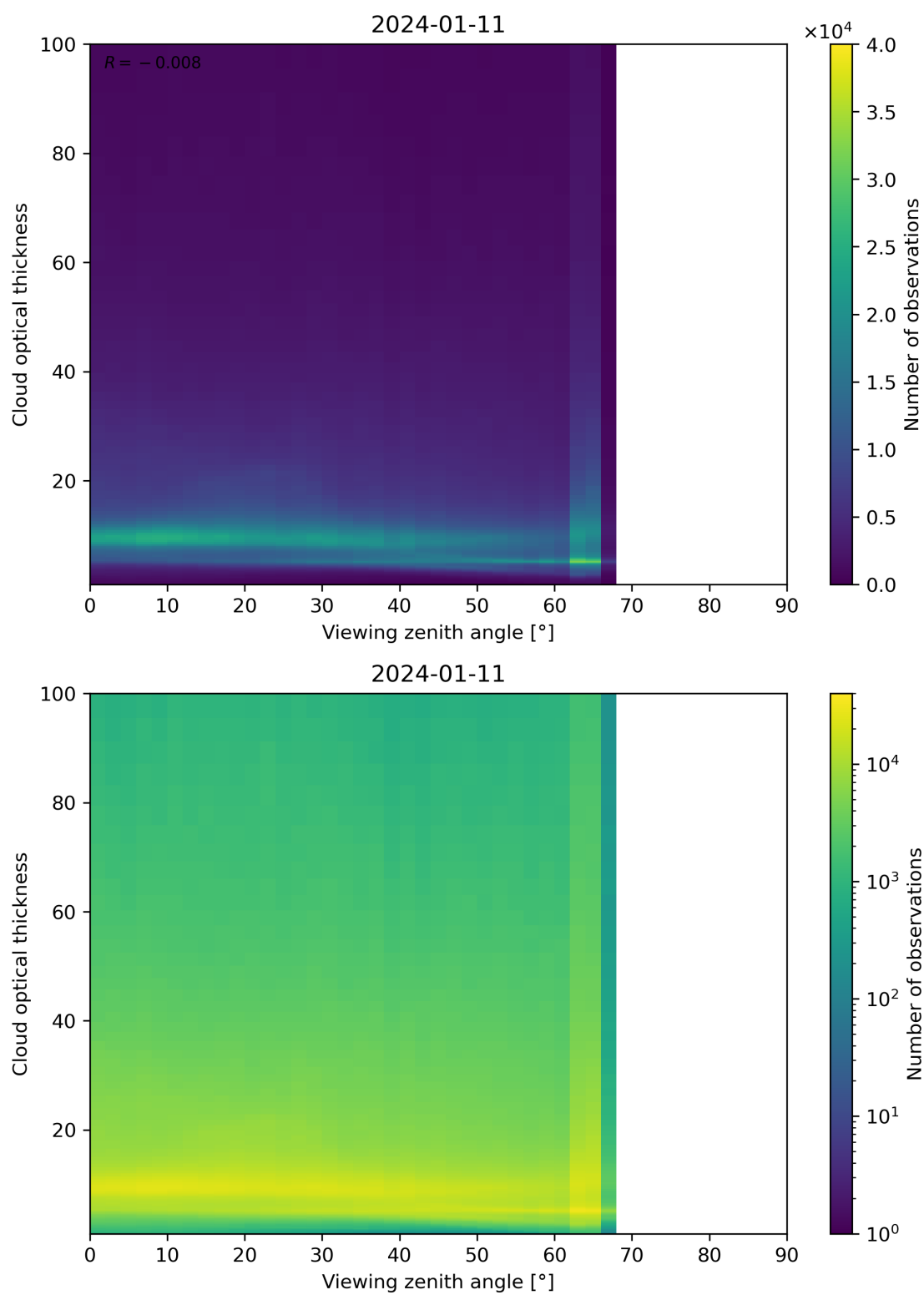
Figure 111: Scatter density plot of “Viewing zenith angle” against “Cloud optical thickness” for 2024-01-10 to 2024-01-12.
