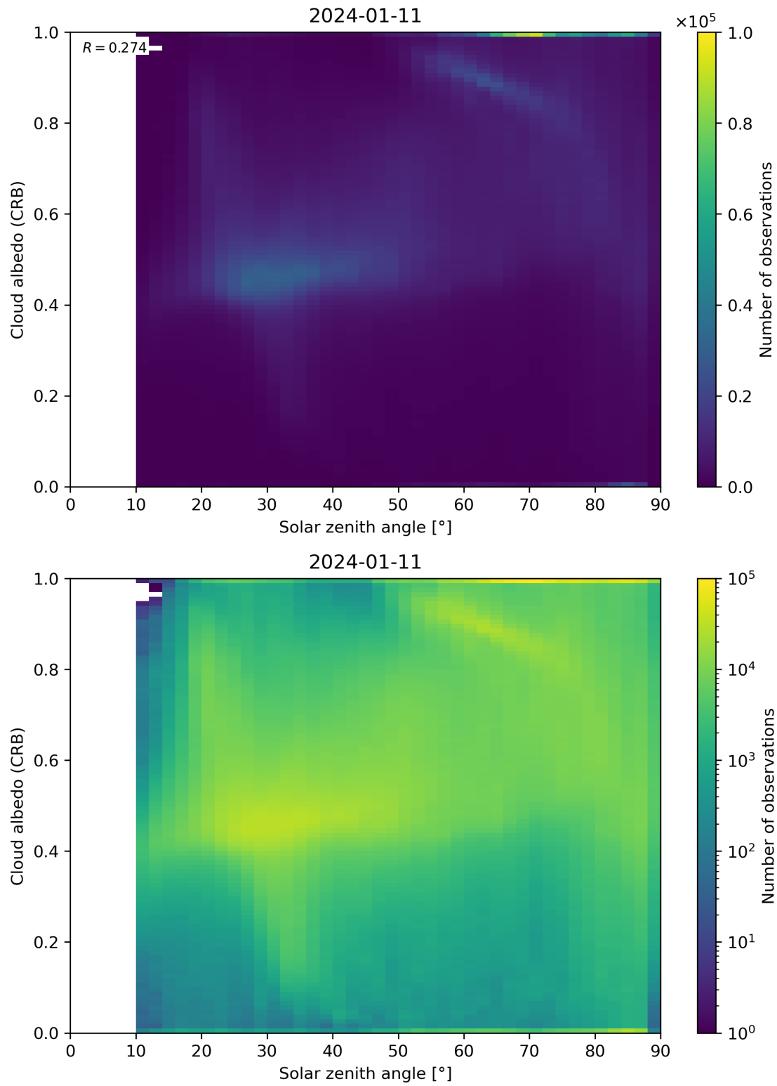
Figure 98: Scatter density plot of “Solar zenith angle” against “Cloud albedo (CRB)” for 2024-01-10 to 2024-01-12.
