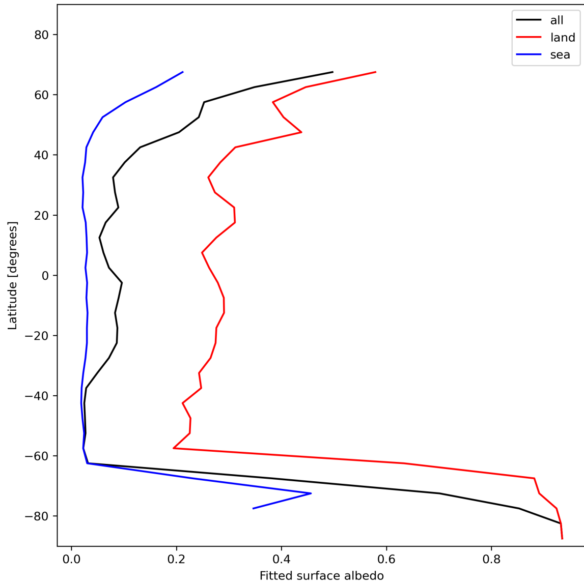
Figure 29: Zonal average of “Fitted surface albedo” for 2024-01-10 to 2024-01-12.
