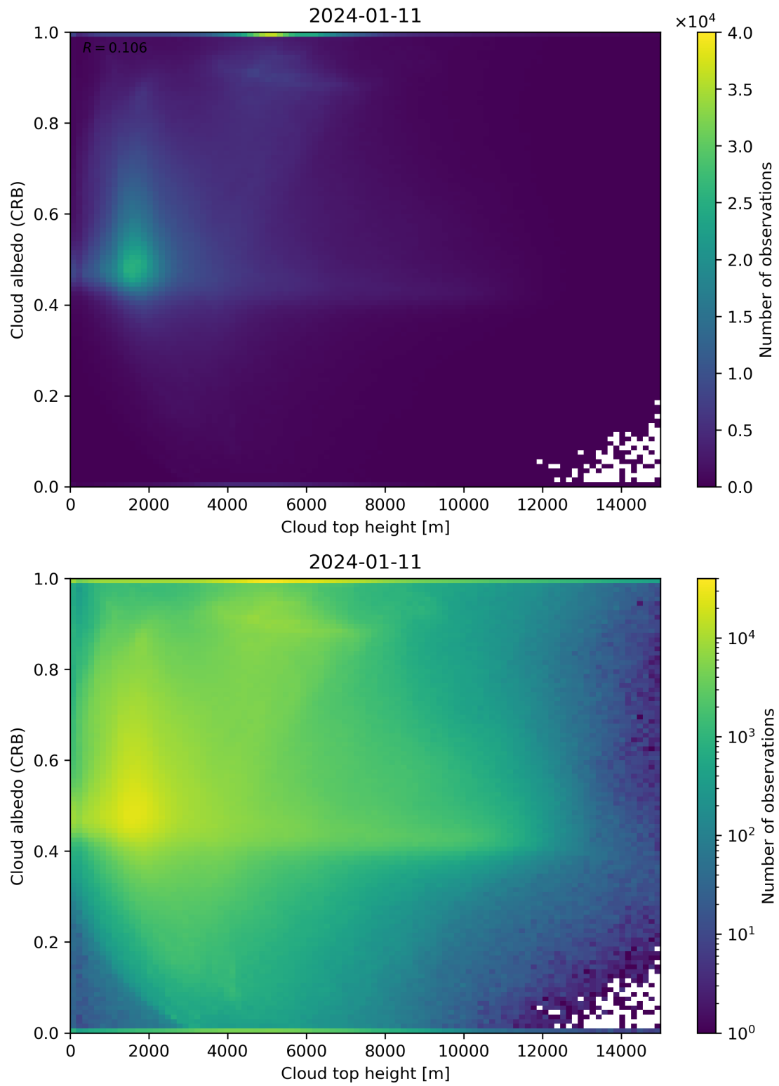
Figure 86: Scatter density plot of “Cloud top height” against “Cloud albedo (CRB)” for 2024-01-10 to 2024-01-12.
