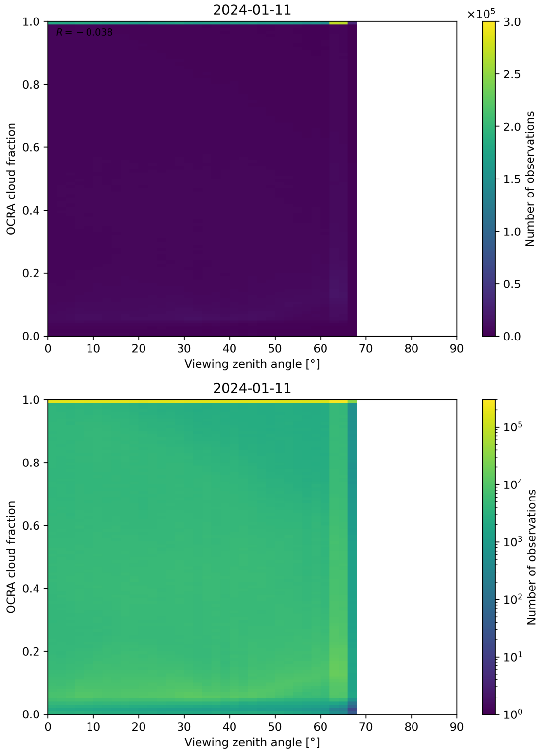
Figure 108: Scatter density plot of “Viewing zenith angle” against “OCRA cloud fraction” for 2024-01-10 to 2024-01-12.
