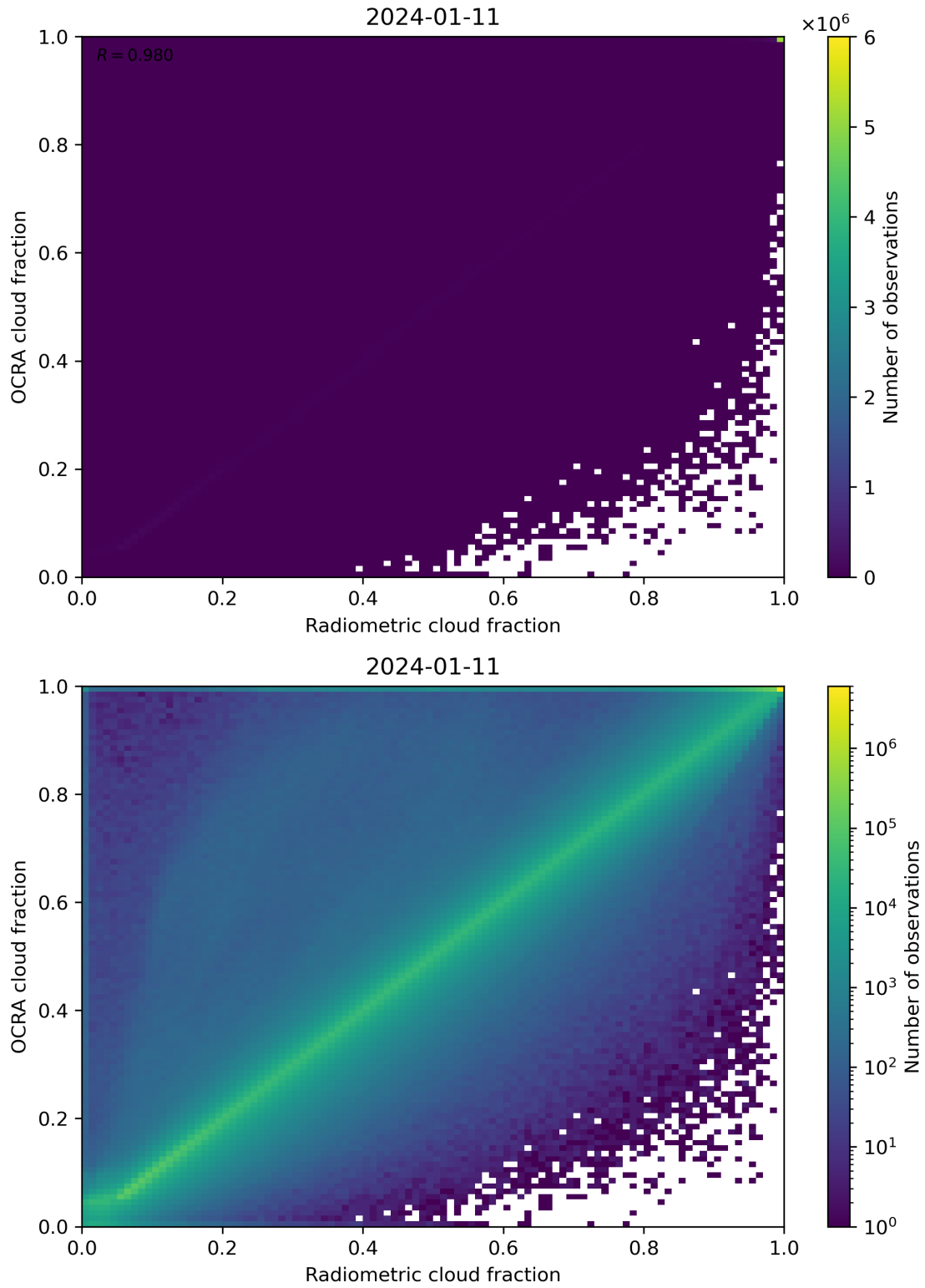
Figure 72: Scatter density plot of “Radiometric cloud fraction” against “OCRA cloud fraction” for 2024-01-10 to 2024-01-12.
