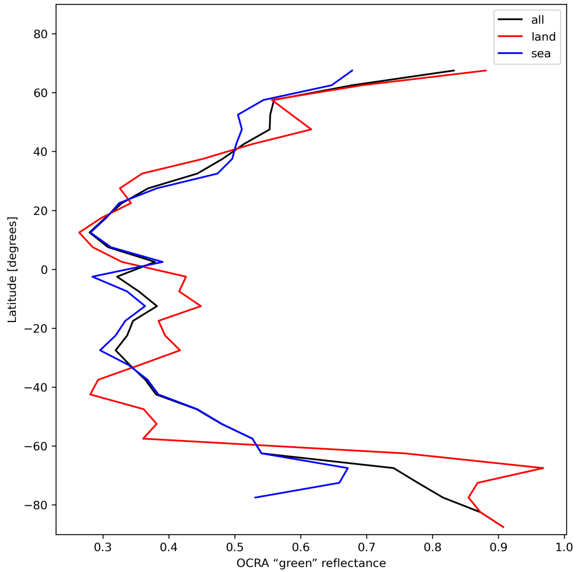
Figure 36: Zonal average of “OCRA “green” reflectance” for 2024-01-10 to 2024-01-12.
