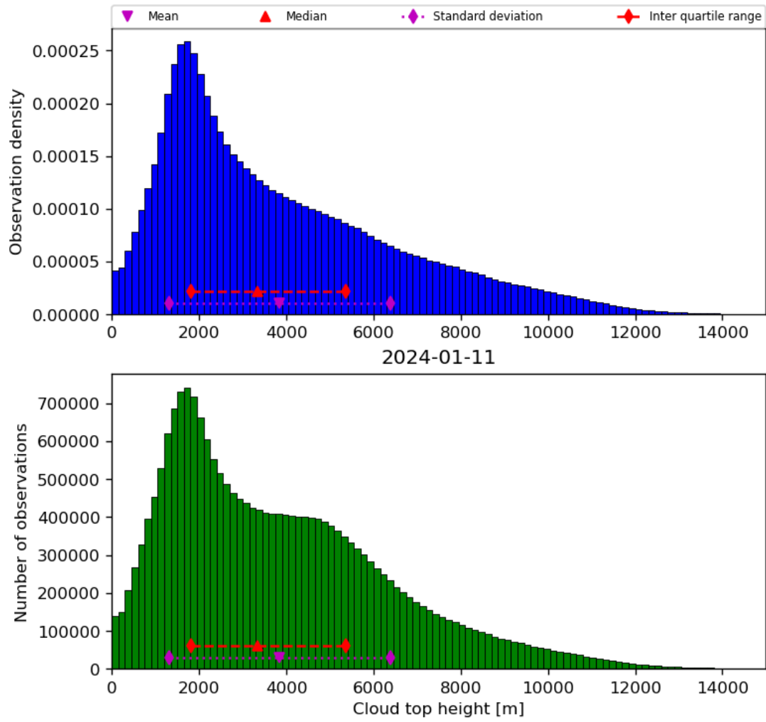
Figure 40: Histogram of “Cloud top height” for 2024-01-10 to 2024-01-12
