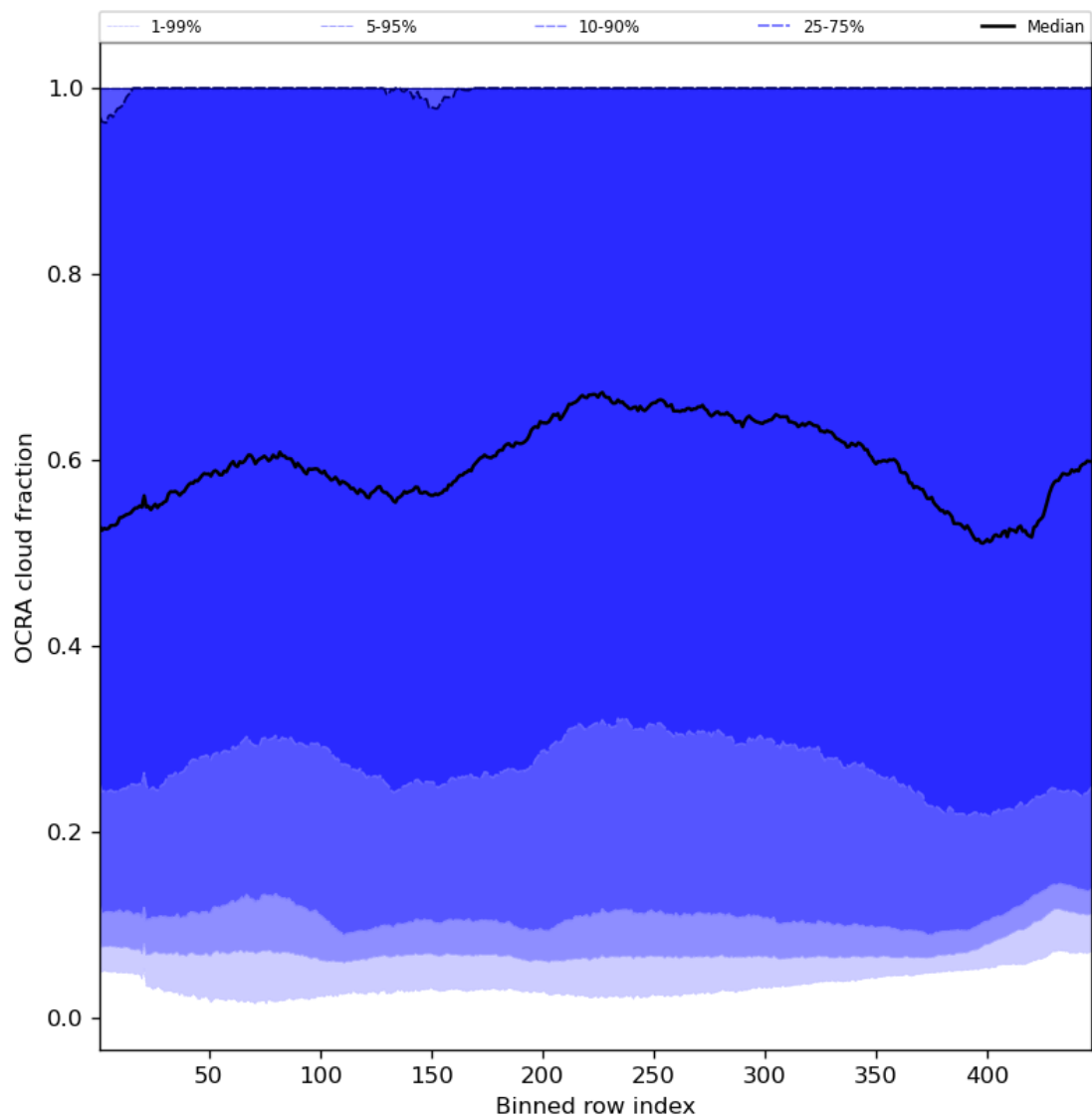
Figure 66: Along track statistics of “OCRA cloud fraction” for 2024-01-10 to 2024-01-12
