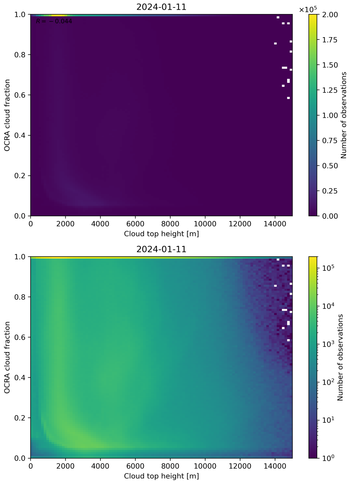
Figure 87: Scatter density plot of “Cloud top height” against “OCRA cloud fraction” for 2024-01-10 to 2024-01-12.
