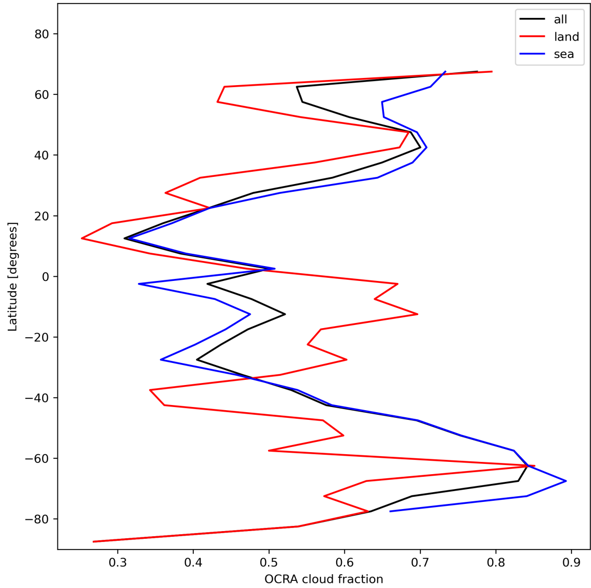
Figure 34: Zonal average of “OCRA cloud fraction” for 2024-01-10 to 2024-01-12.
