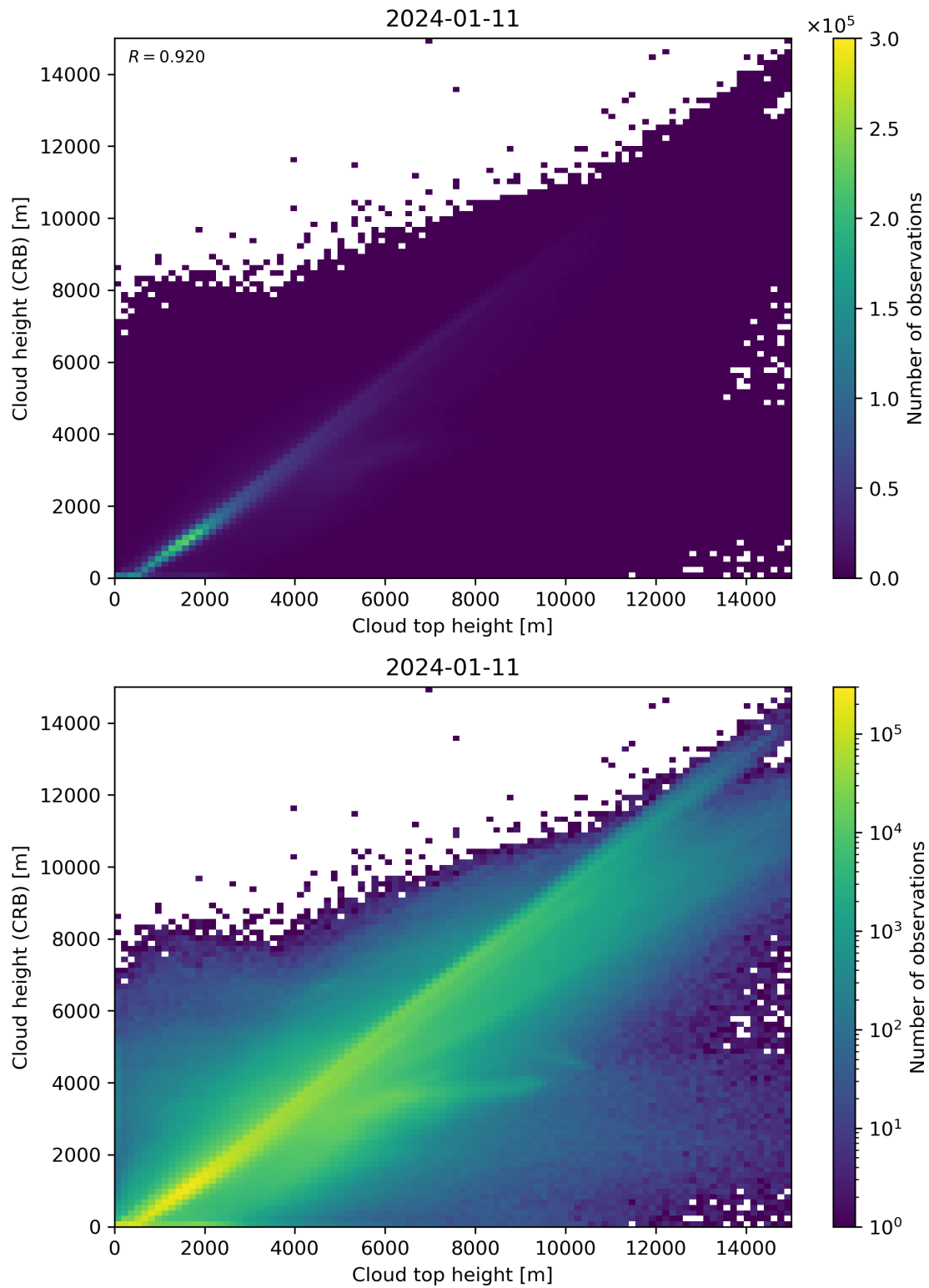
Figure 89: Scatter density plot of “Cloud top height” against “Cloud height (CRB)” for 2024-01-10 to 2024-01-12.
