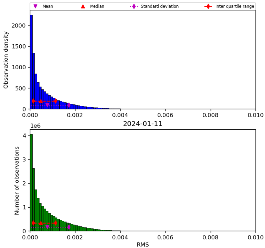
Figure 47: Histogram of “RMS” for 2024-01-10 to 2024-01-12
