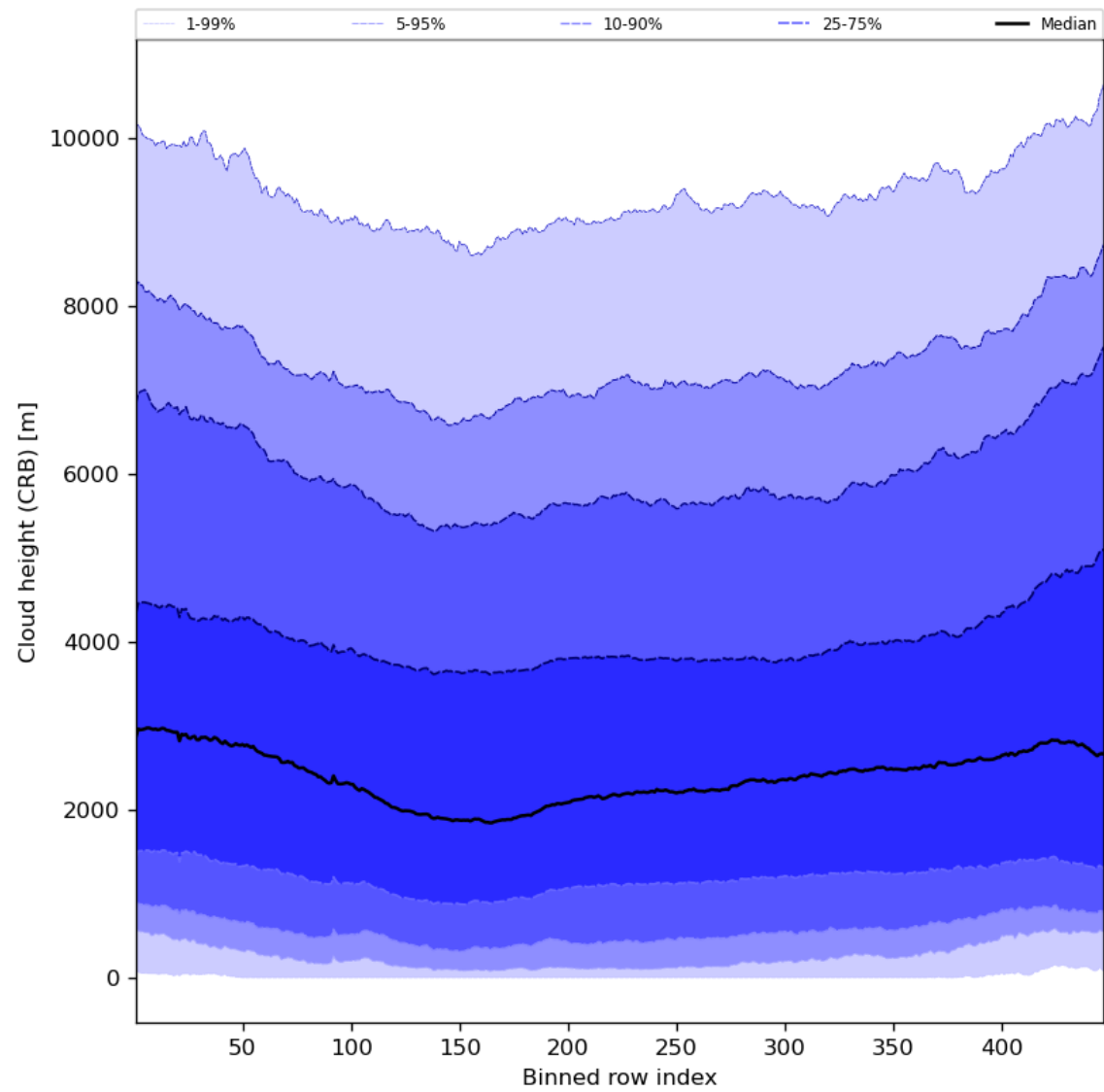
Figure 59: Along track statistics of “Cloud height (CRB)” for 2024-01-10 to 2024-01-12
