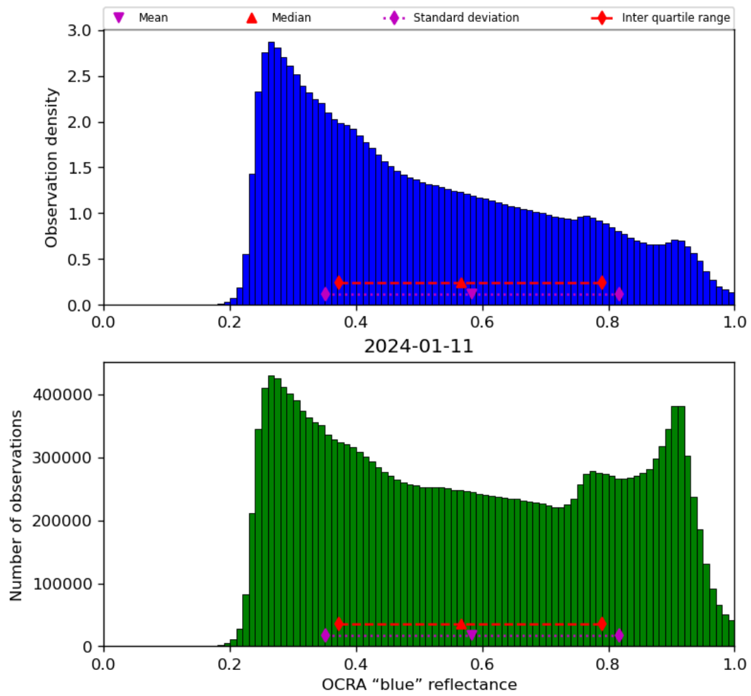
Figure 51: Histogram of “OCRA “blue” reflectance” for 2024-01-10 to 2024-01-12
