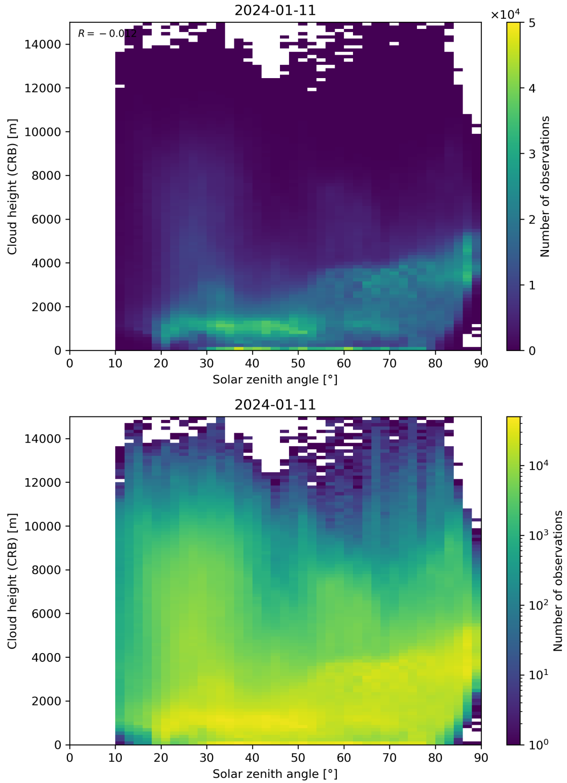
Figure 102: Scatter density plot of “Solar zenith angle” against “Cloud height (CRB)” for 2024-01-10 to 2024-01-12.
