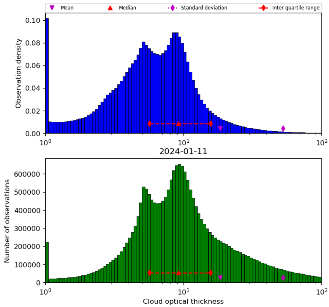
Figure 41: Histogram of “Cloud optical thickness” for 2024-01-10 to 2024-01-12
