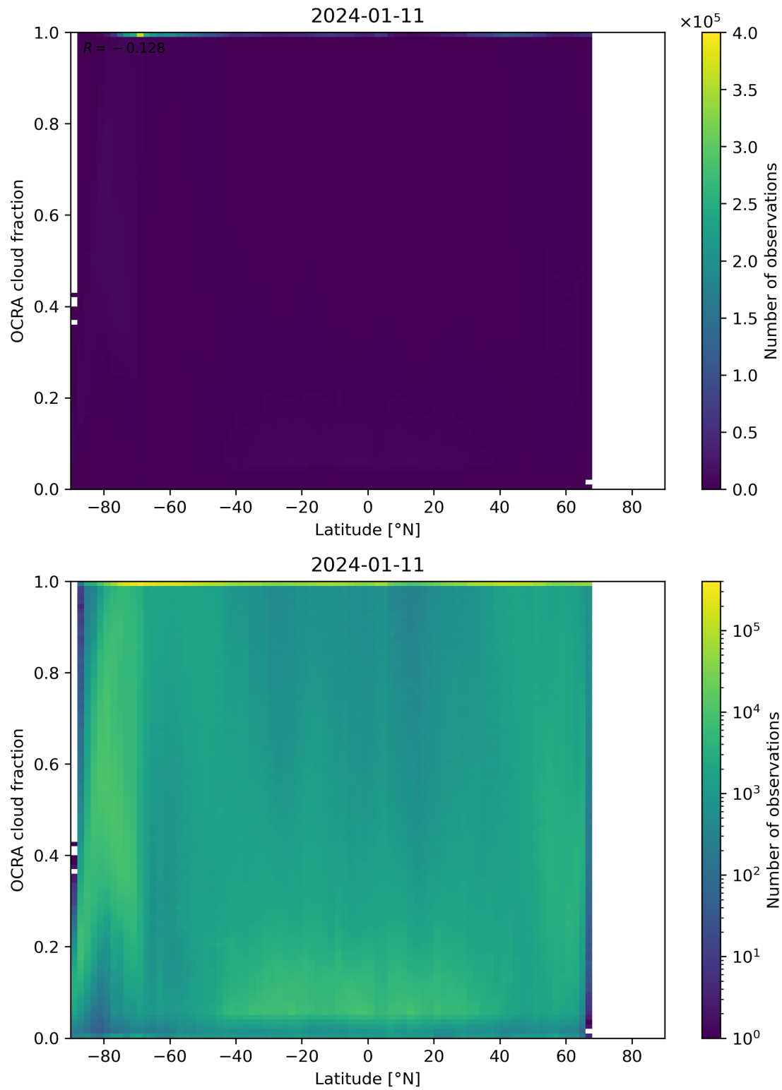
Figure 93: Scatter density plot of “Latitude” against “OCRA cloud fraction” for 2024-01-10 to 2024-01-12.
