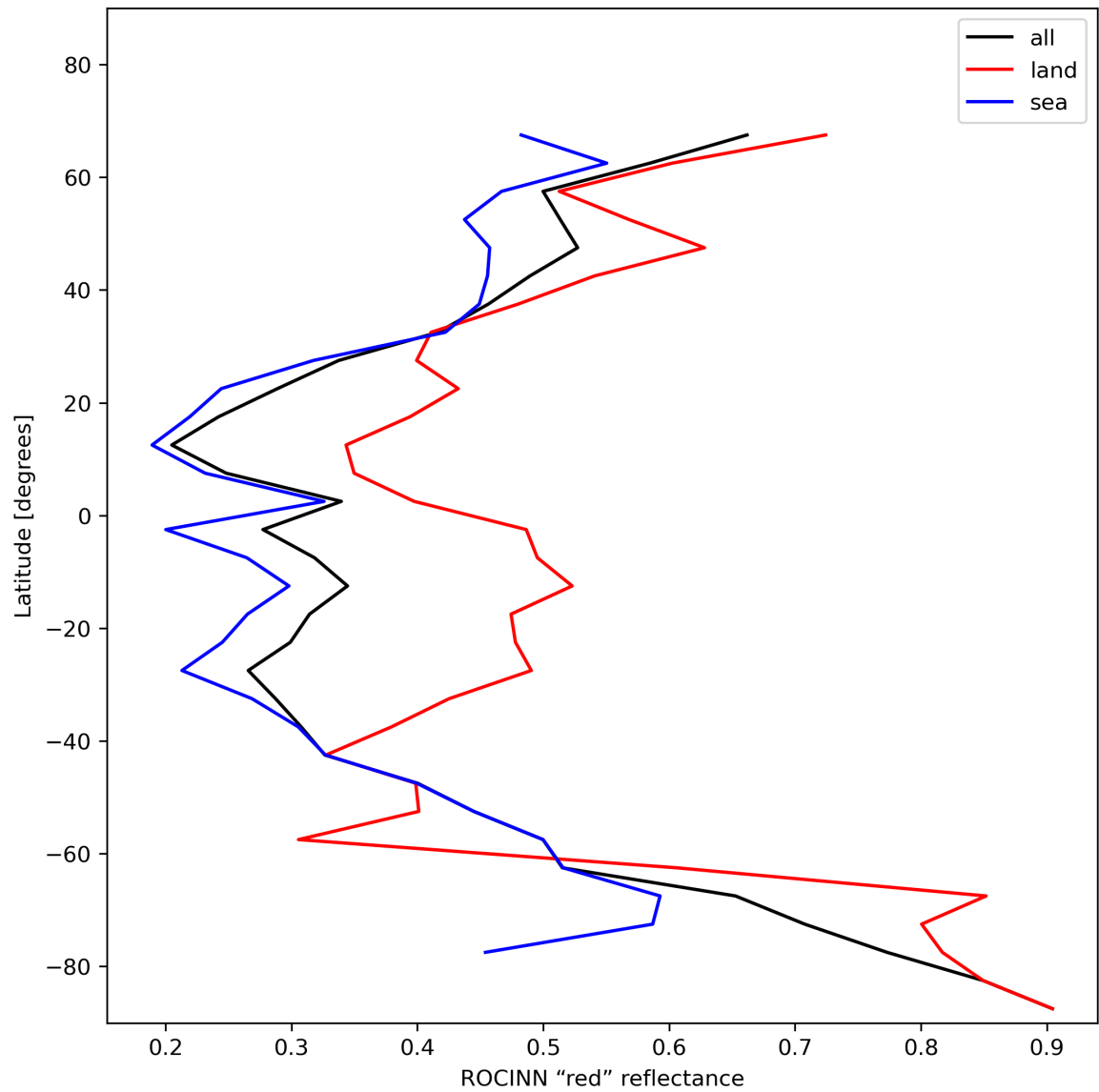
Figure 37: Zonal average of “ROCINN “red” reflectance” for 2024-01-10 to 2024-01-12.
