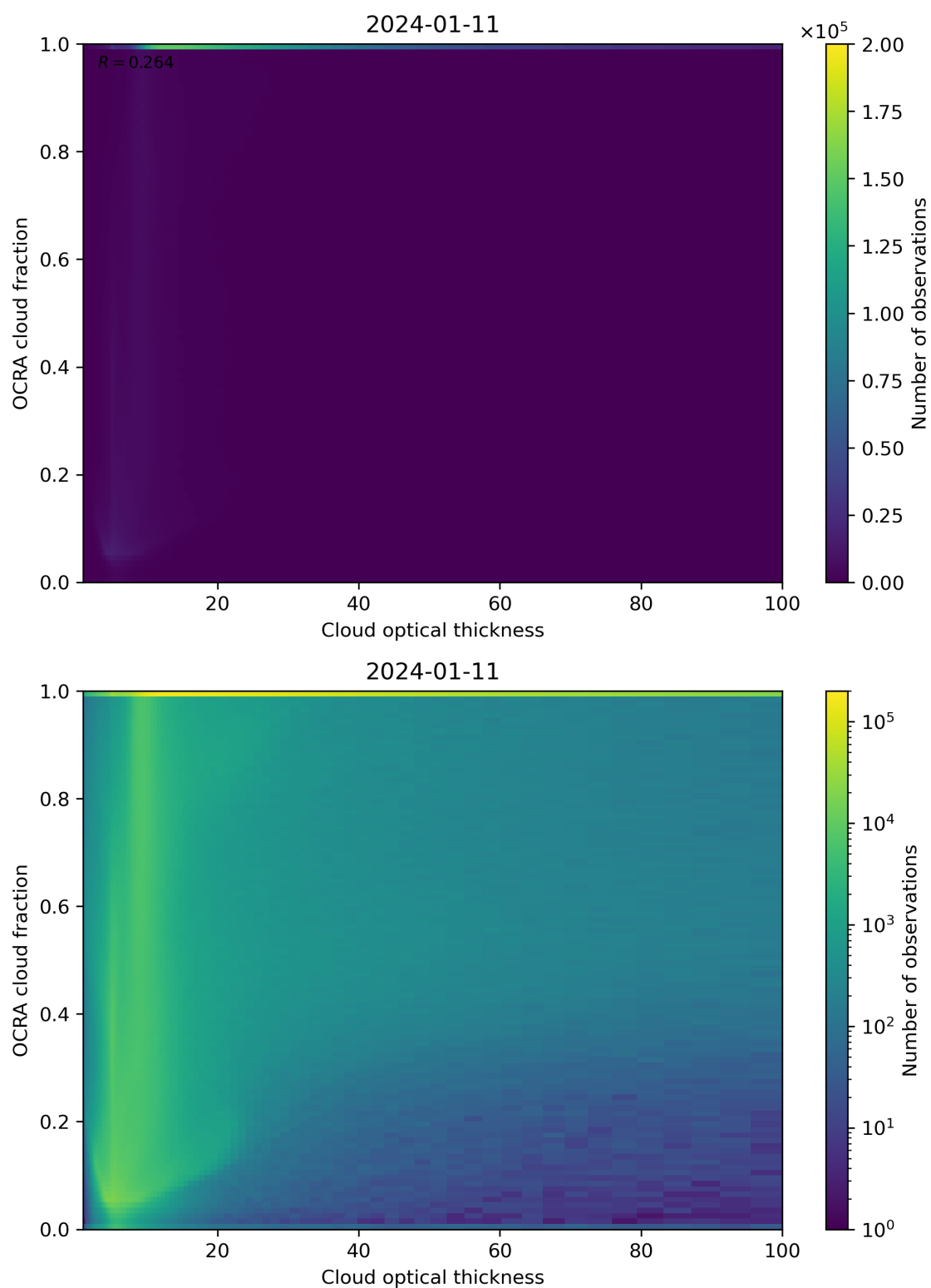
Figure 83: Scatter density plot of “Cloud optical thickness” against “OCRA cloud fraction” for 2024-01-10 to 2024-01-12.
