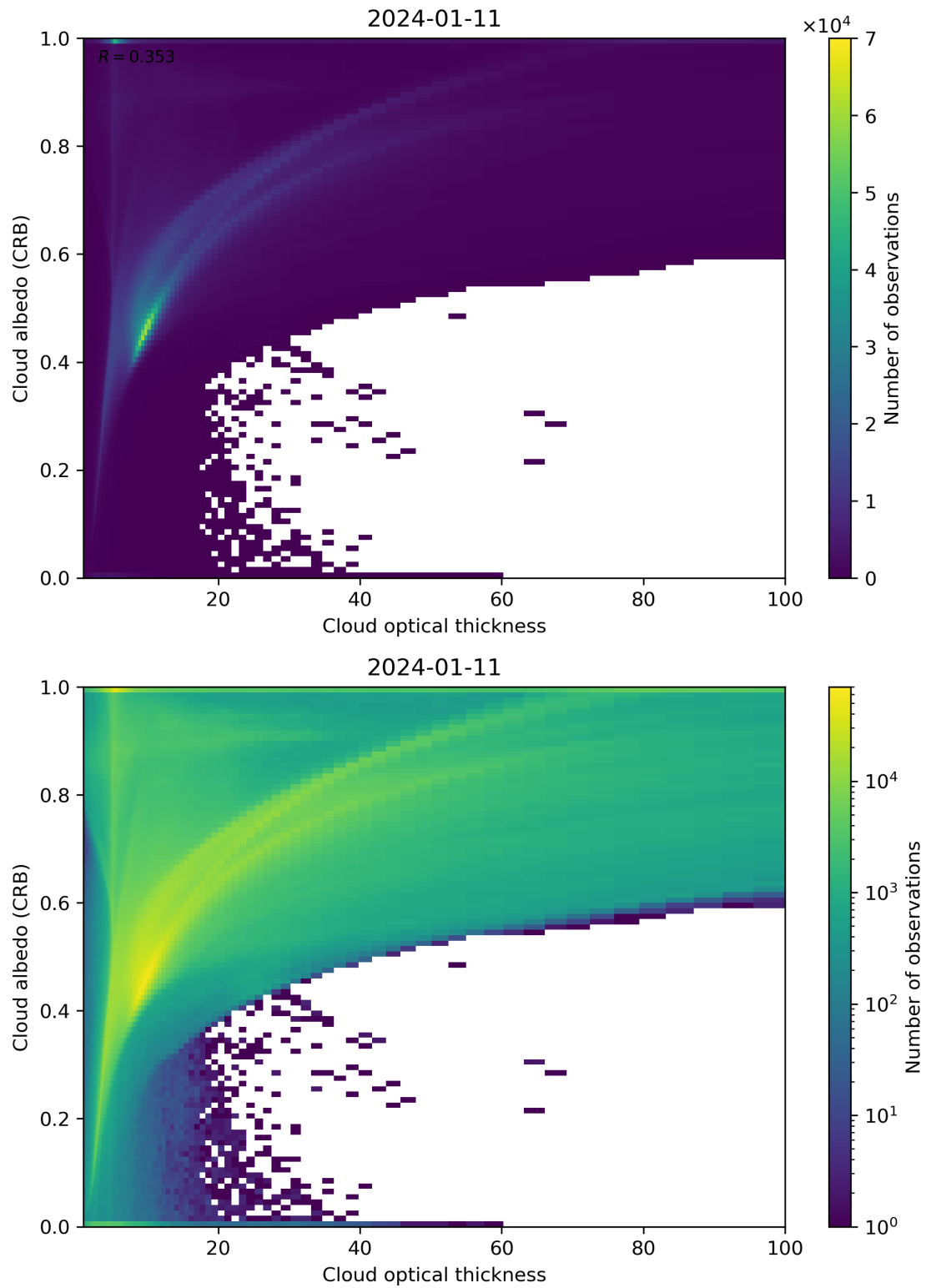
Figure 82: Scatter density plot of “Cloud optical thickness” against “Cloud albedo (CRB)” for 2024-01-10 to 2024-01-12.
