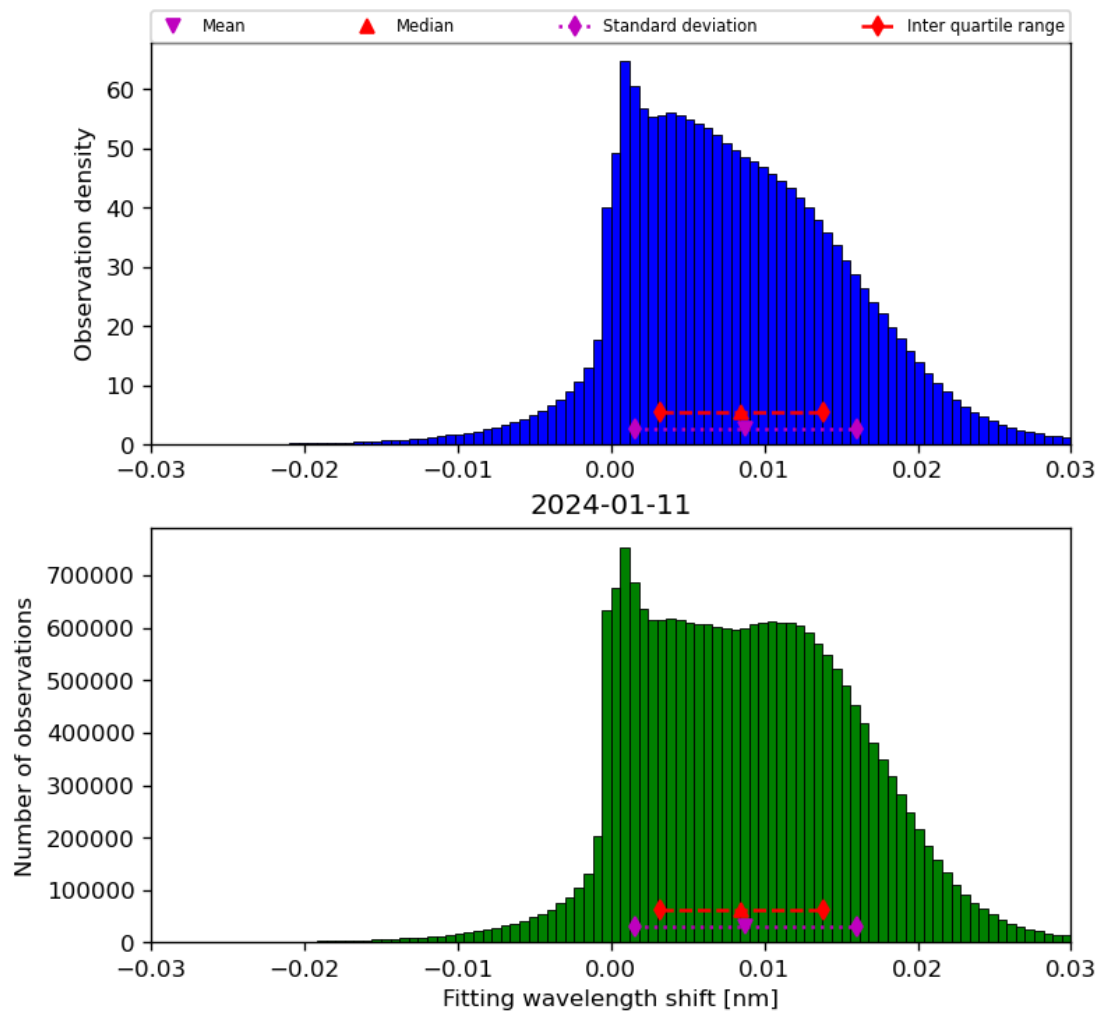
Figure 49: Histogram of “Fitting wavelength shift” for 2024-01-10 to 2024-01-12
