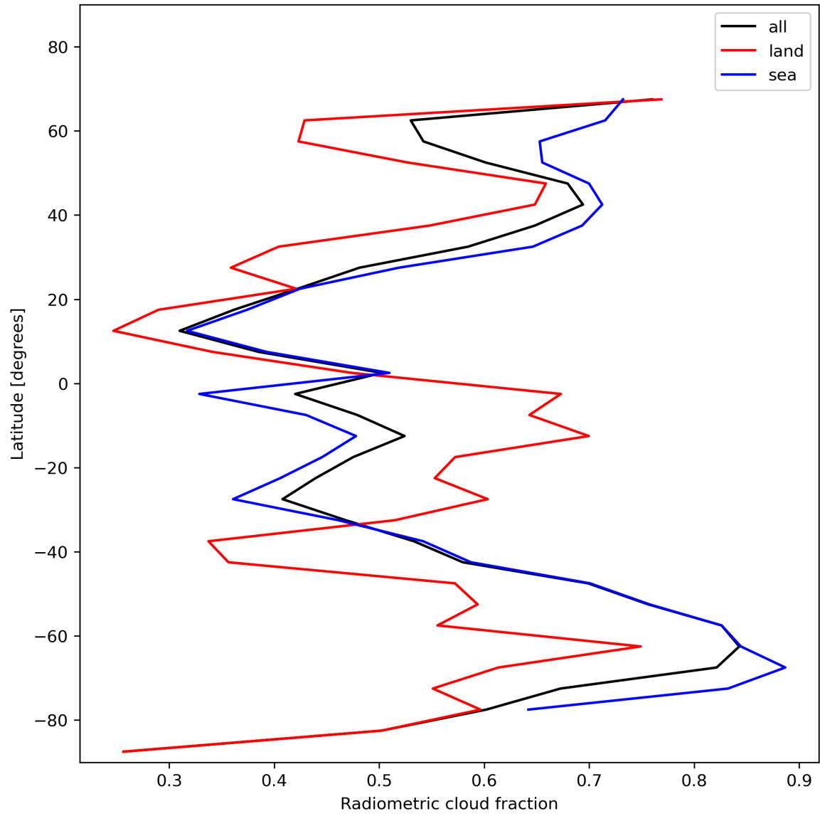
Figure 23: Zonal average of “Radiometric cloud fraction” for 2024-01-10 to 2024-01-12.
