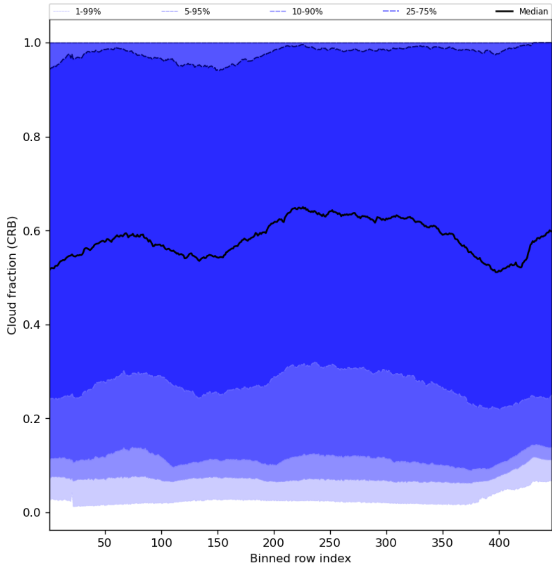
Figure 58: Along track statistics of “Cloud fraction (CRB)” for 2024-01-10 to 2024-01-12
