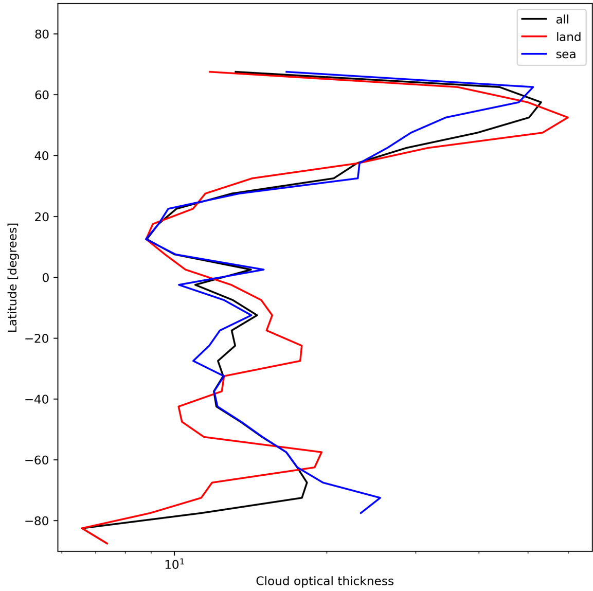
Figure 25: Zonal average of “Cloud optical thickness” for 2024-01-10 to 2024-01-12.
