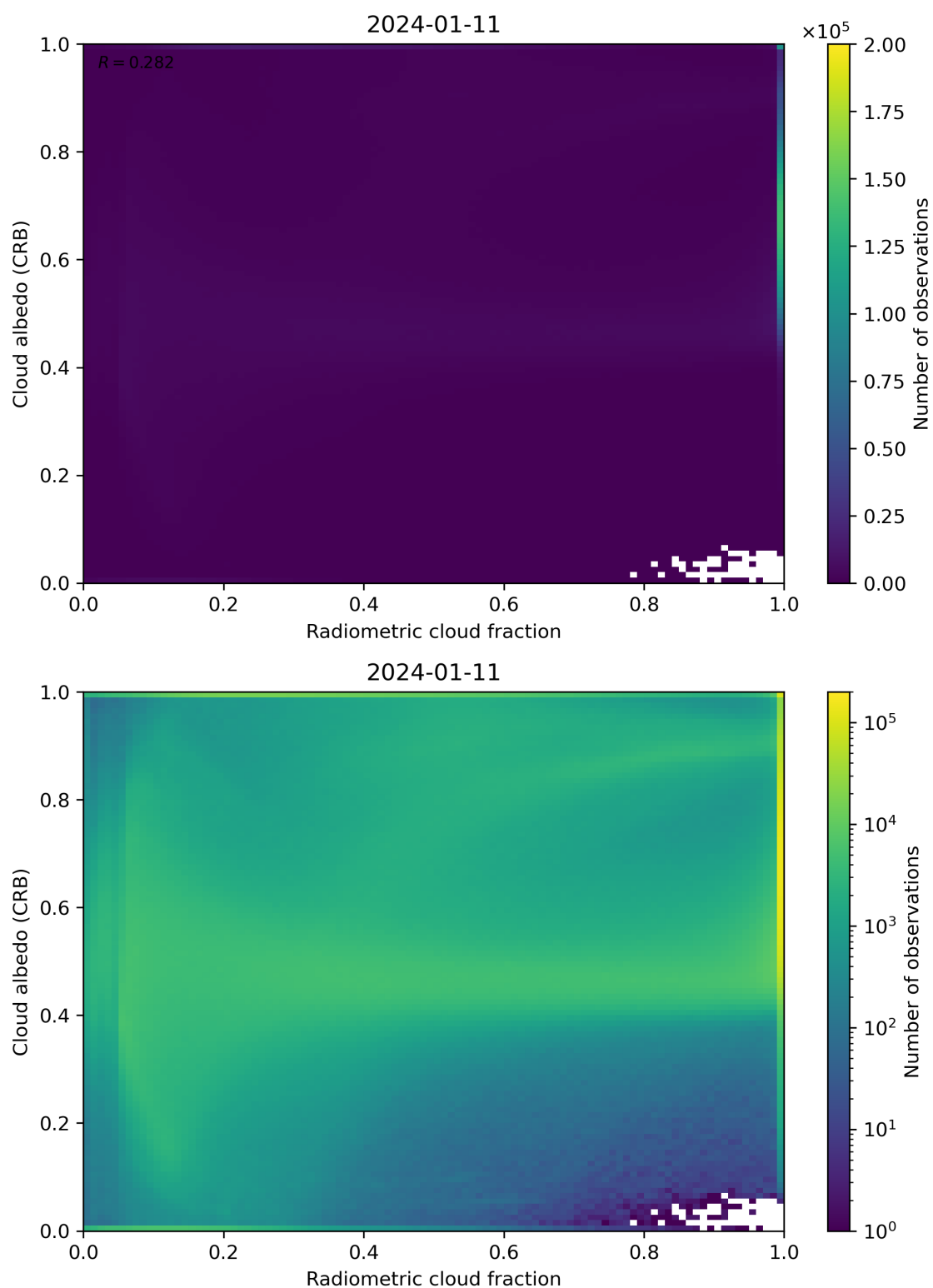
Figure 71: Scatter density plot of “Radiometric cloud fraction” against “Cloud albedo (CRB)” for 2024-01-10 to 2024-01-12.
