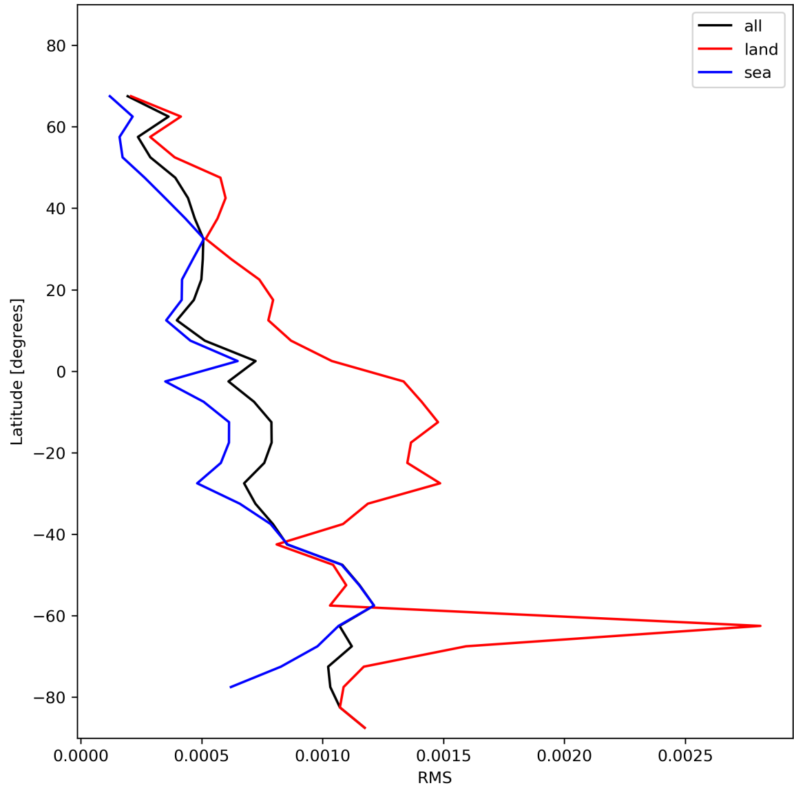
Figure 31: Zonal average of “RMS” for 2024-01-10 to 2024-01-12.
