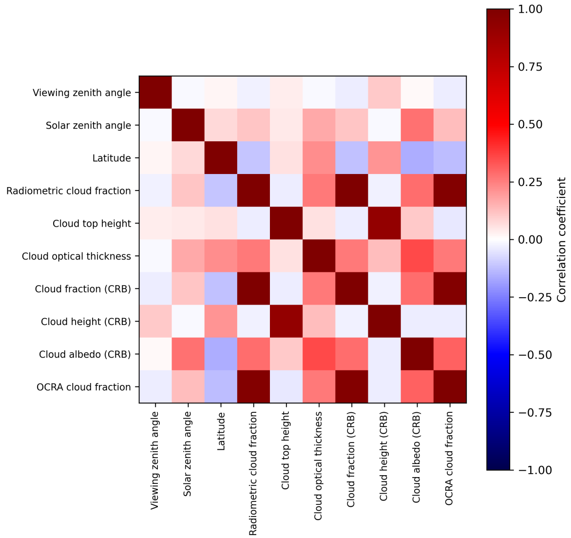
Figure 2: Map of correlation matrix for 2024-01-10 to 2024-01-12.
