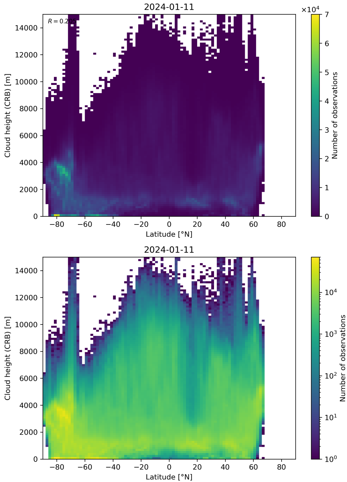
Figure 95: Scatter density plot of “Latitude” against “Cloud height (CRB)” for 2024-01-10 to 2024-01-12.
