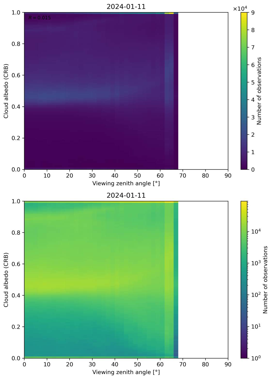
Figure 106: Scatter density plot of “Viewing zenith angle” against “Cloud albedo (CRB)” for 2024-01-10 to 2024-01-12.
