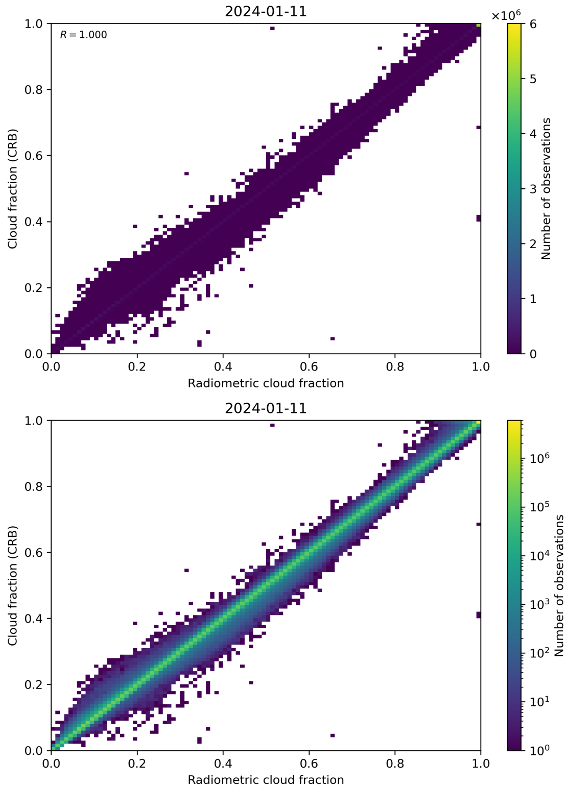
Figure 73: Scatter density plot of “Radiometric cloud fraction” against “Cloud fraction (CRB)” for 2024-01-10 to 2024-01-12.
