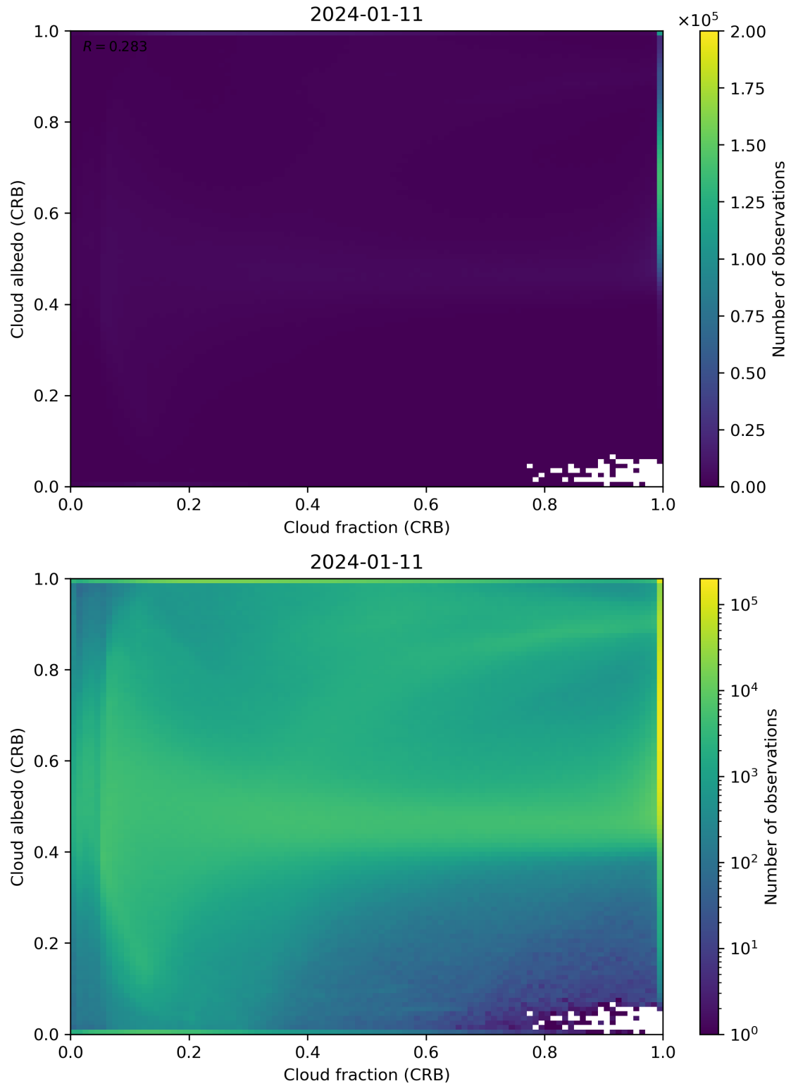
Figure 77: Scatter density plot of “Cloud fraction (CRB)” against “Cloud albedo (CRB)” for 2024-01-10 to 2024-01-12.
