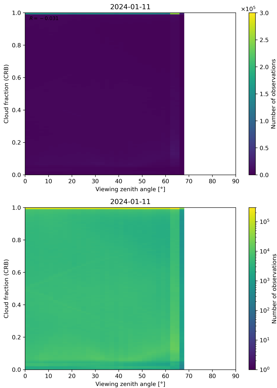
Figure 109: Scatter density plot of “Viewing zenith angle” against “Cloud fraction (CRB)” for 2024-01-10 to 2024-01-12.
