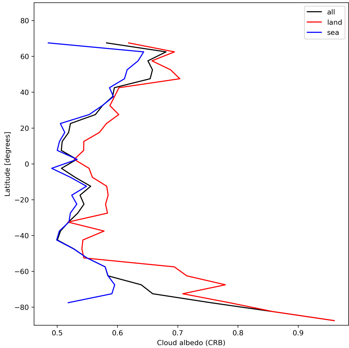
Figure 28: Zonal average of “Cloud albedo (CRB)” for 2024-01-10 to 2024-01-12.
