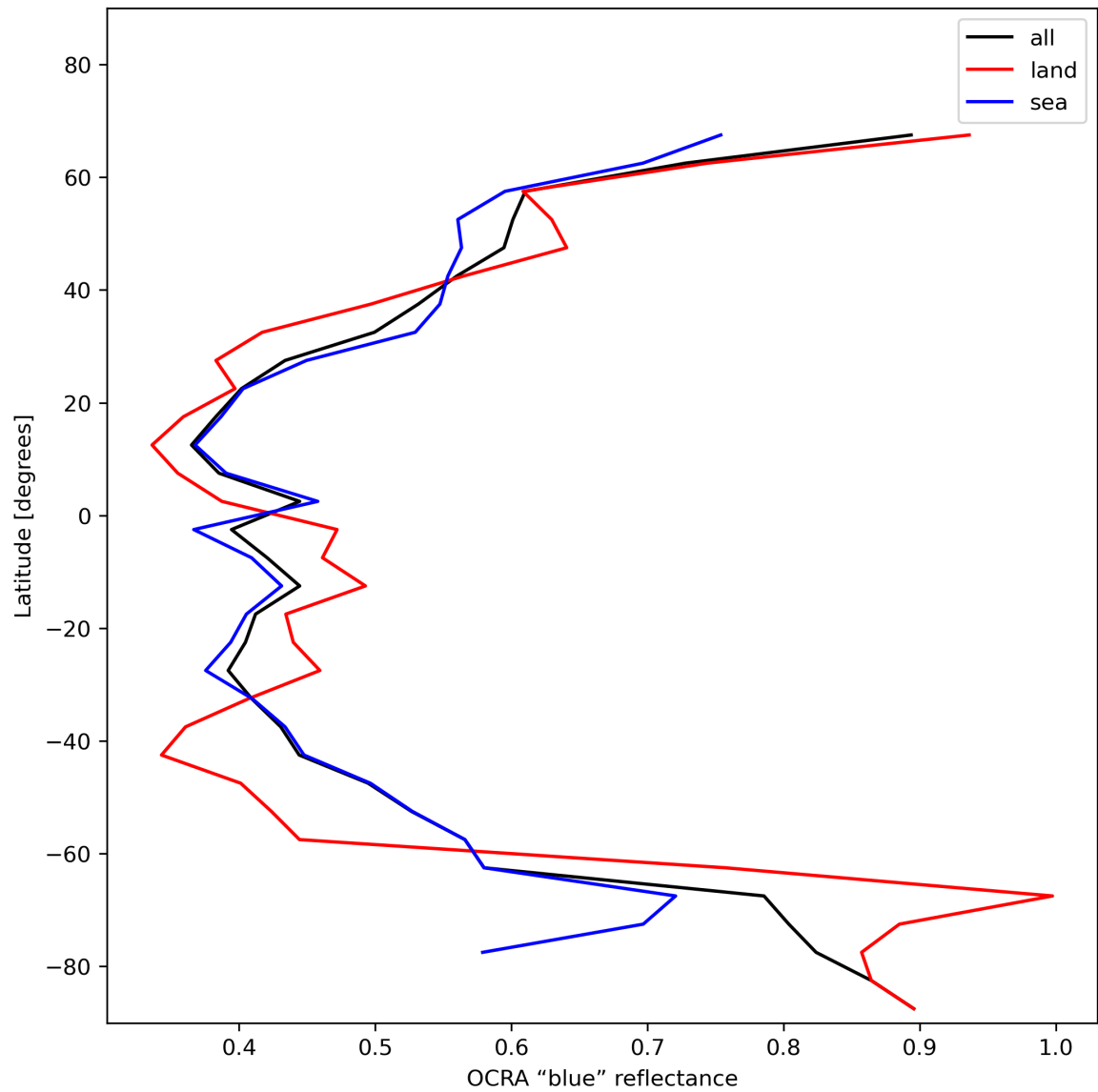
Figure 35: Zonal average of “OCRA “blue” reflectance” for 2024-01-10 to 2024-01-12.
