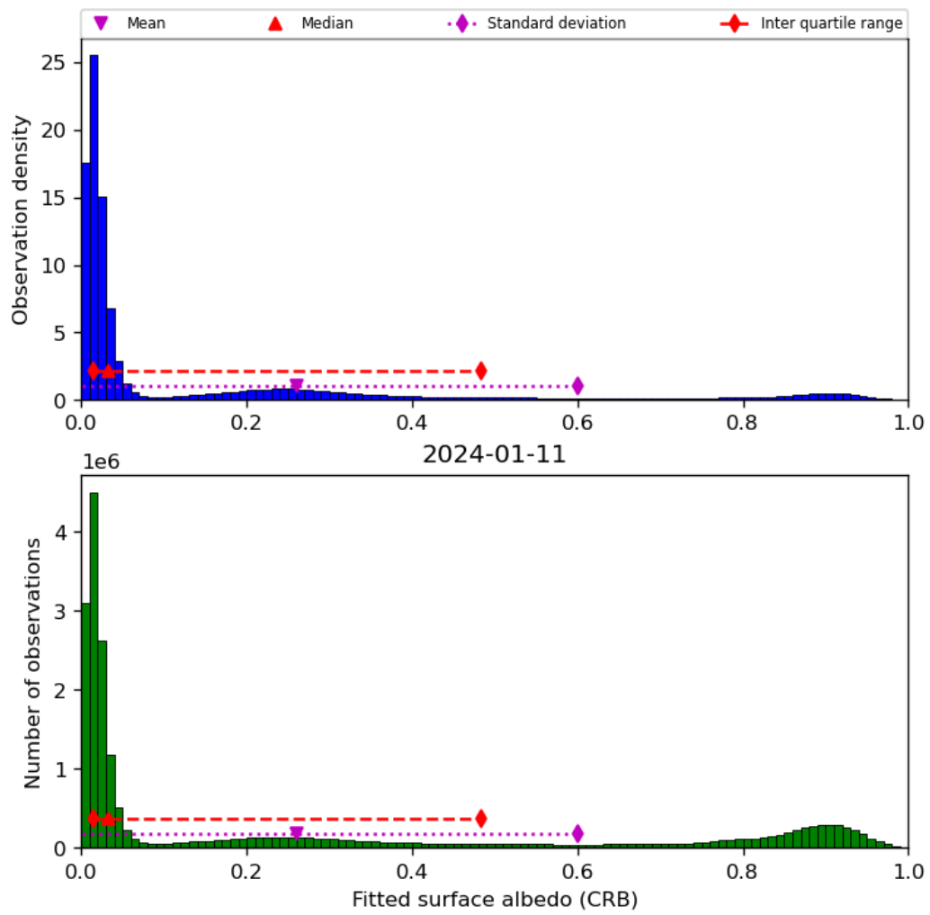
Figure 46: Histogram of “Fitted surface albedo (CRB)” for 2024-01-10 to 2024-01-12
