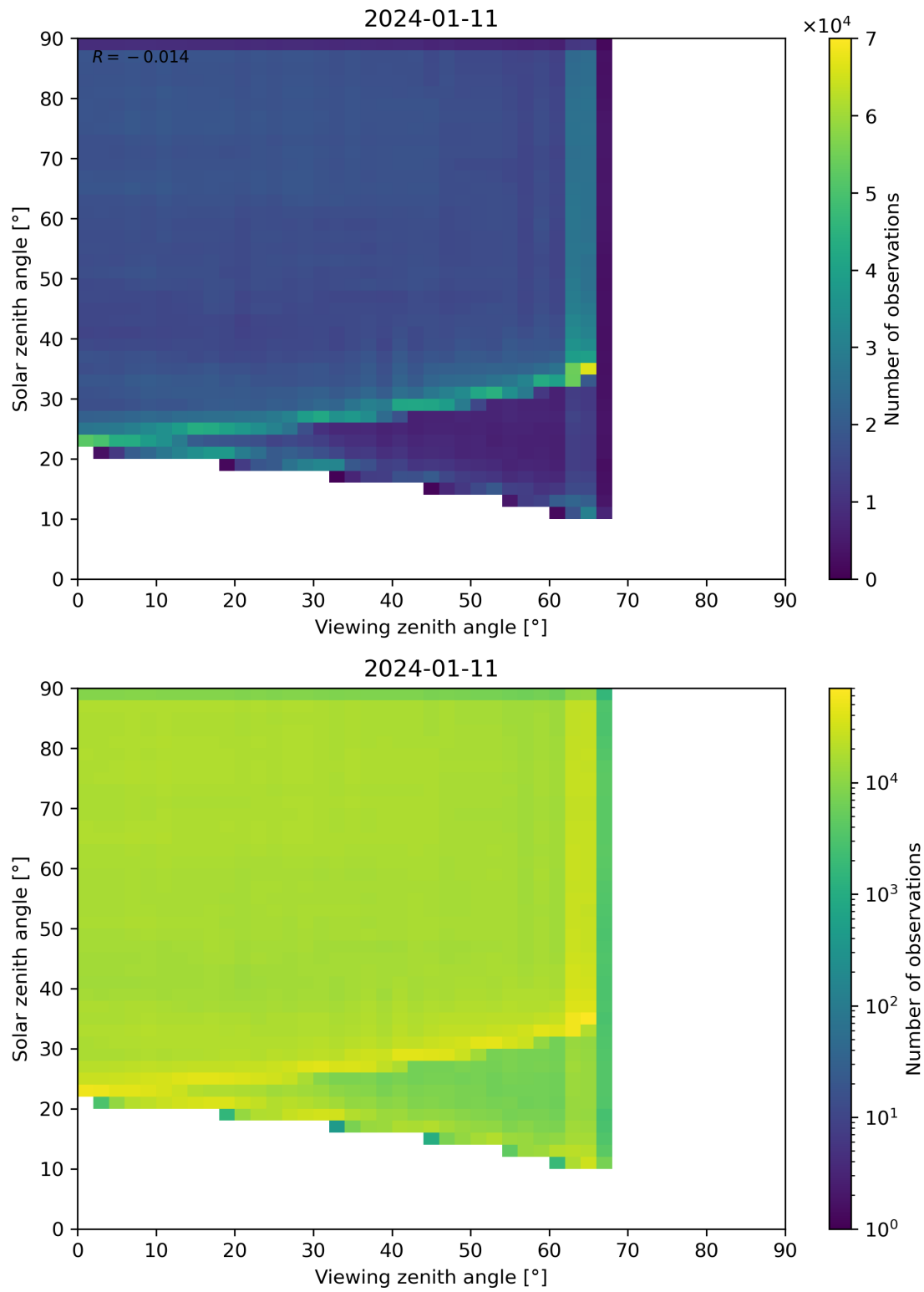
Figure 114: Scatter density plot of “Viewing zenith angle” against “Solar zenith angle” for 2024-01-10 to 2024-01-12.
