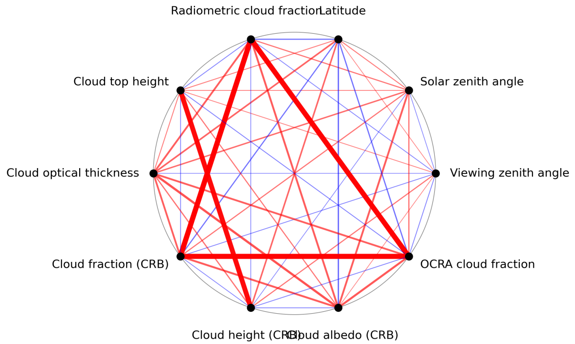
Figure 1: Map of correlation graph for 2024-01-10 to 2024-01-12.
