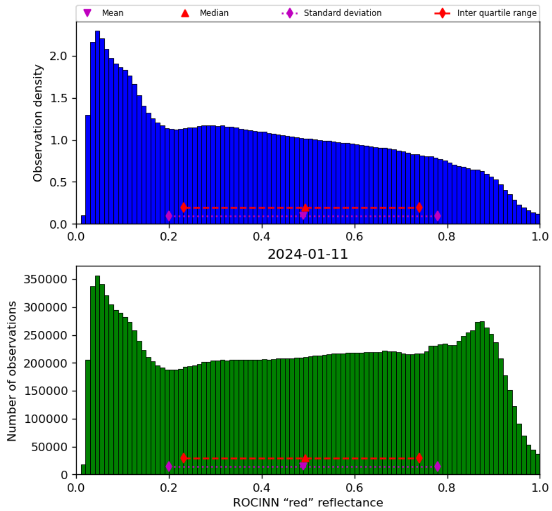
Figure 53: Histogram of “ROCINN “red” reflectance” for 2024-01-10 to 2024-01-12
