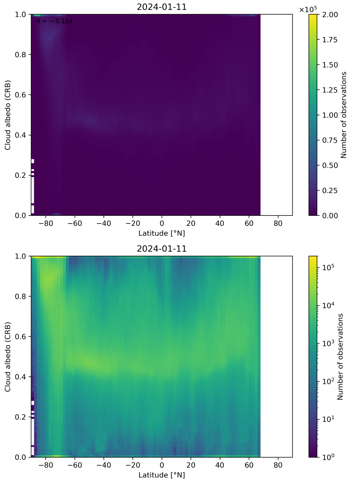
Figure 91: Scatter density plot of “Latitude” against “Cloud albedo (CRB)” for 2024-01-10 to 2024-01-12.
