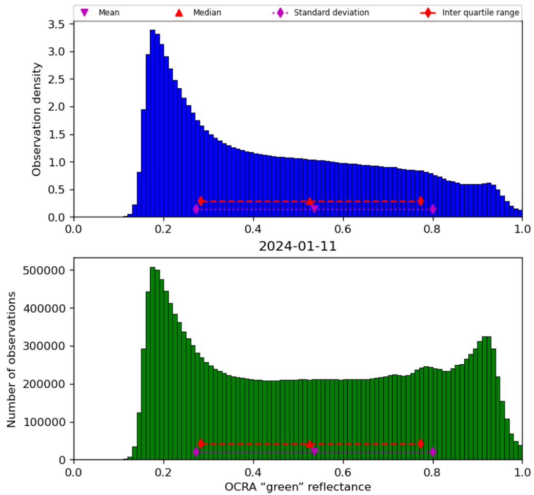
Figure 52: Histogram of “OCRA “green” reflectance” for 2024-01-10 to 2024-01-12
