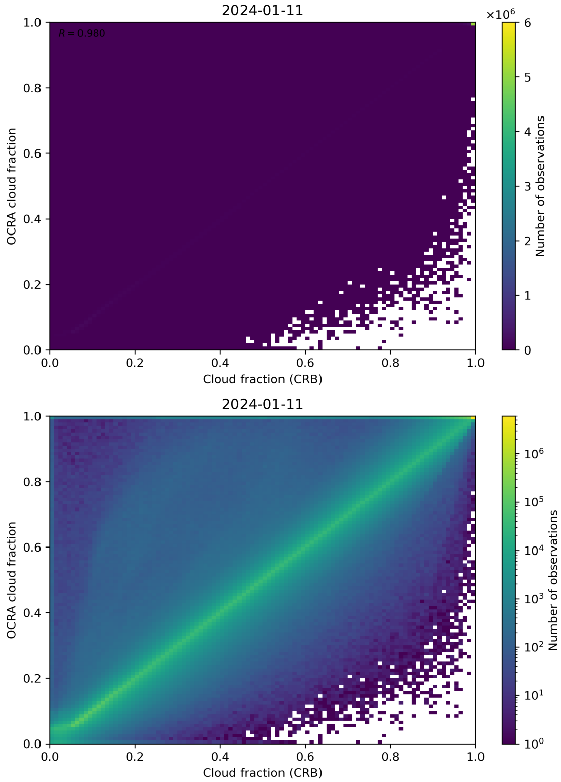
Figure 78: Scatter density plot of “Cloud fraction (CRB)” against “OCRA cloud fraction” for 2024-01-10 to 2024-01-12.
