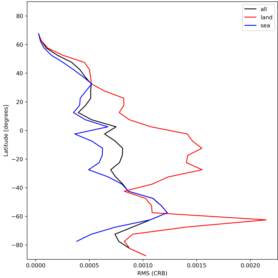
Figure 32: Zonal average of “RMS (CRB)” for 2024-01-10 to 2024-01-12.
