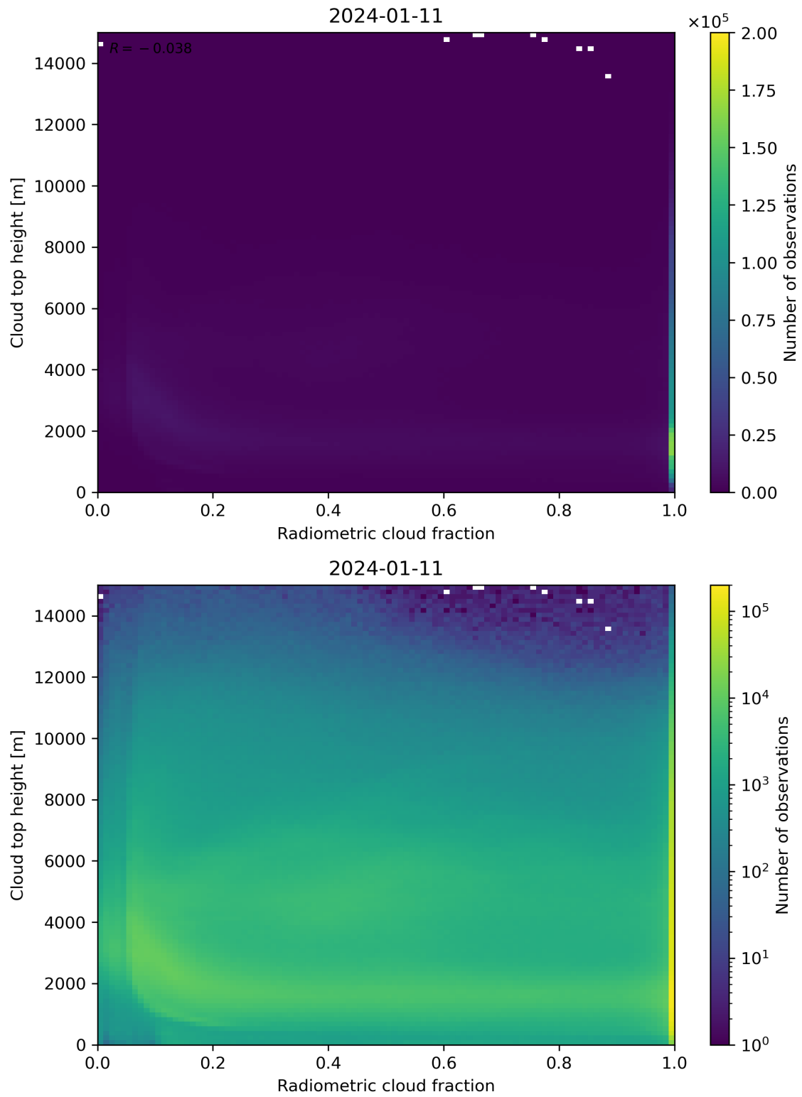
Figure 76: Scatter density plot of “Radiometric cloud fraction” against “Cloud top height” for 2024-01-10 to 2024-01-12.
