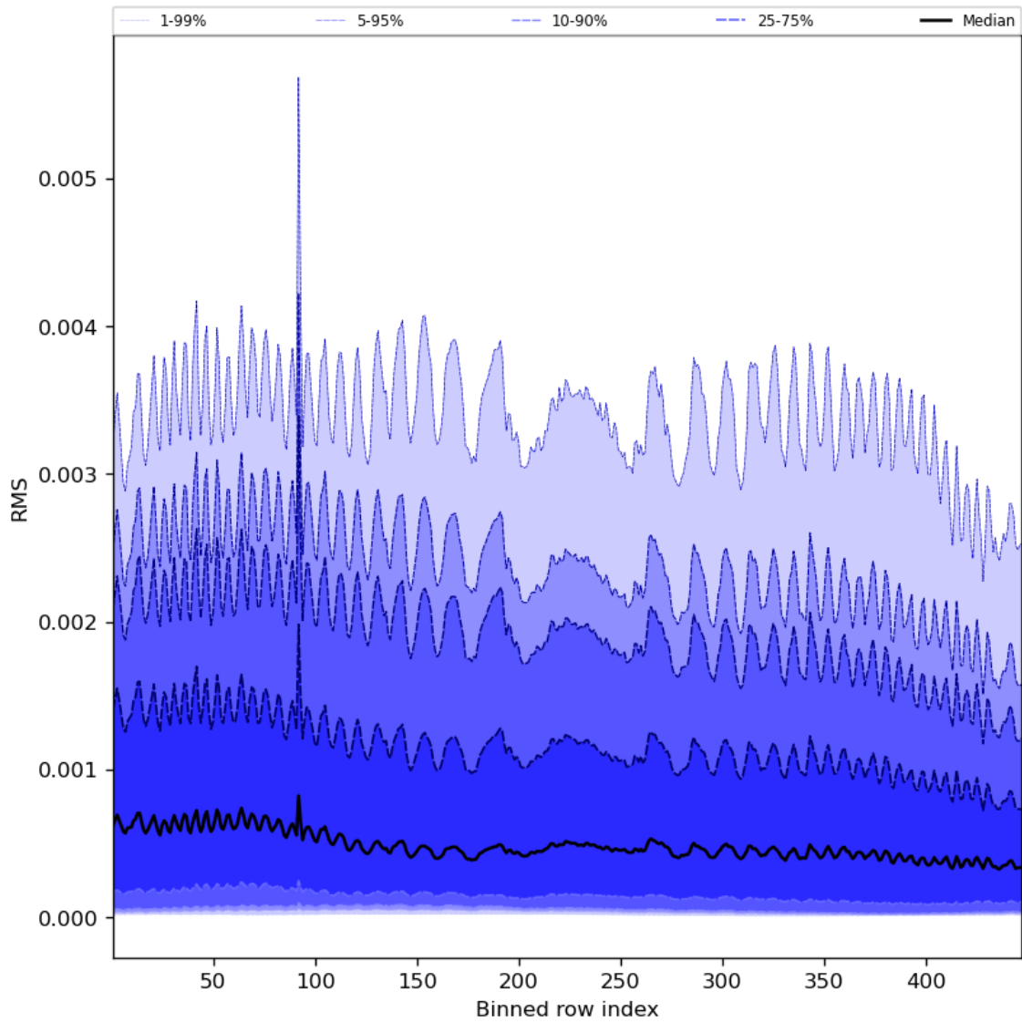
Figure 63: Along track statistics of “RMS” for 2024-01-10 to 2024-01-12
