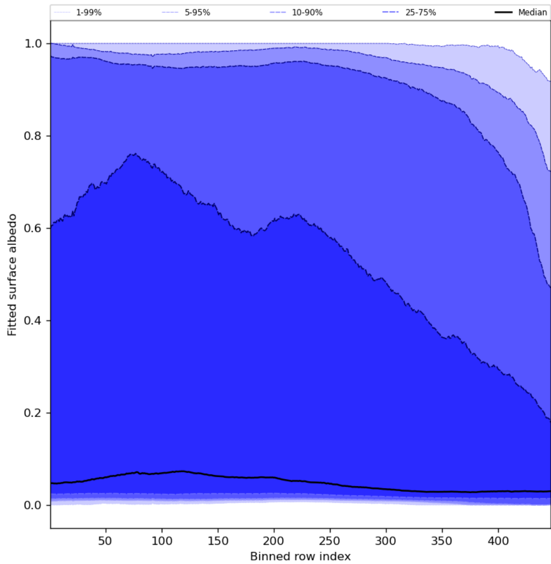
Figure 61: Along track statistics of “Fitted surface albedo” for 2024-01-10 to 2024-01-12
