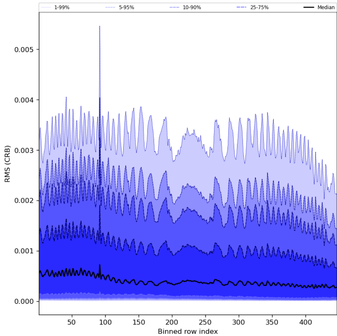
Figure 64: Along track statistics of “RMS (CRB)” for 2024-01-10 to 2024-01-12
