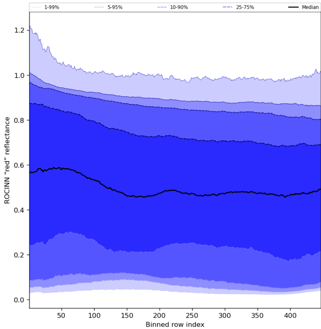
Figure 69: Along track statistics of "ROCINN "red" reflectance" for 2024-01-10 to 2024-01-12
