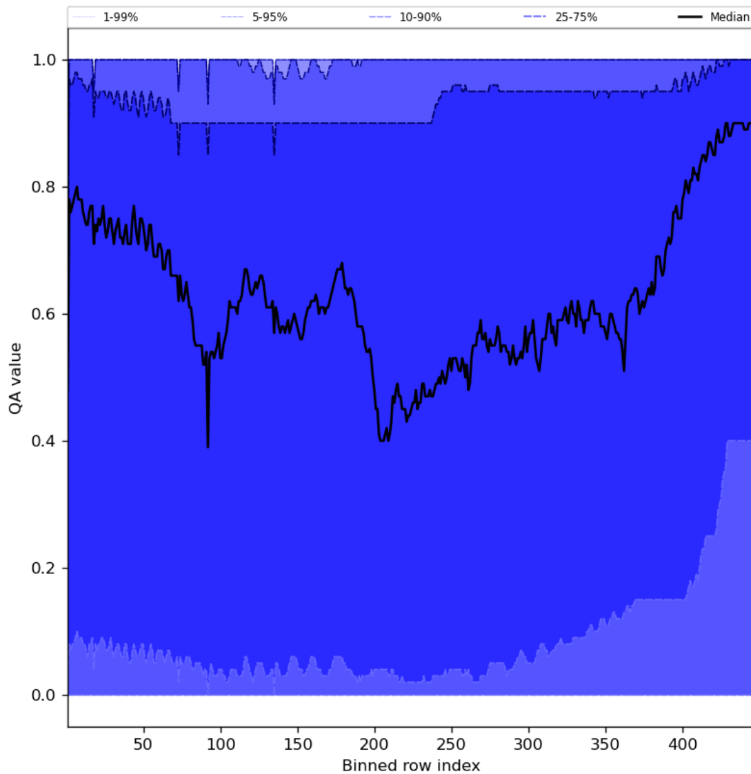
Figure 54: Along track statistics of “QA value” for 2024-01-10 to 2024-01-12
