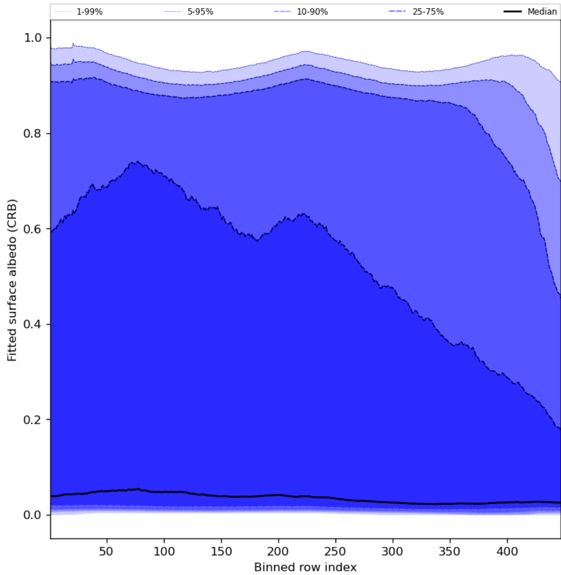
Figure 62: Along track statistics of “Fitted surface albedo (CRB)” for 2024-01-10 to 2024-01-12
