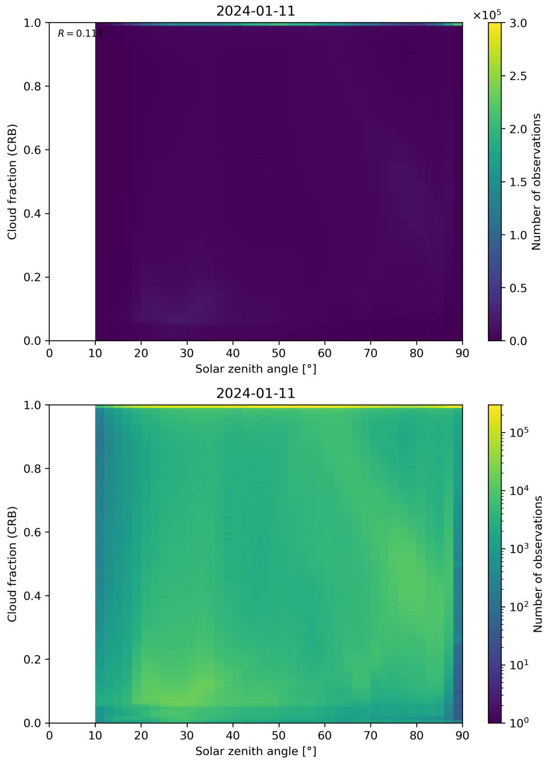
Figure 101: Scatter density plot of “Solar zenith angle” against “Cloud fraction (CRB)” for 2024-01-10 to 2024-01-12.
