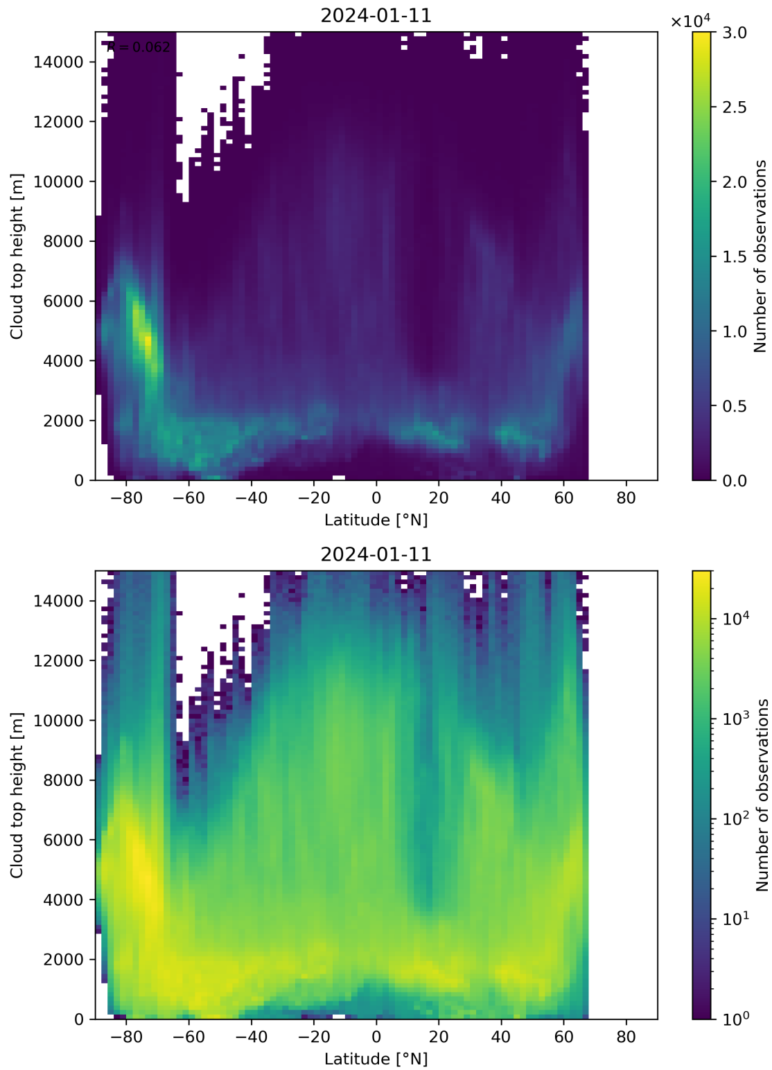
Figure 97: Scatter density plot of “Latitude” against “Cloud top height” for 2024-01-10 to 2024-01-12.
