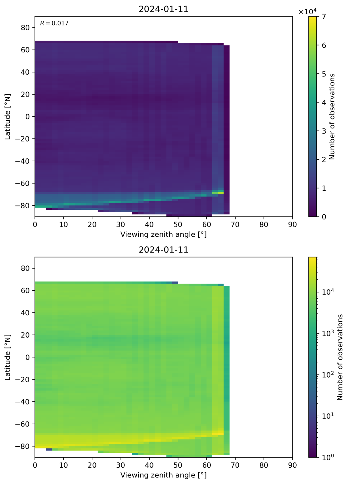
Figure 113: Scatter density plot of “Viewing zenith angle” against “Latitude” for 2024-01-10 to 2024-01-12.
