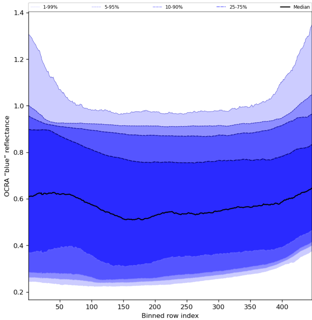
Figure 67: Along track statistics of “OCRA “blue” reflectance” for 2024-01-10 to 2024-01-12
