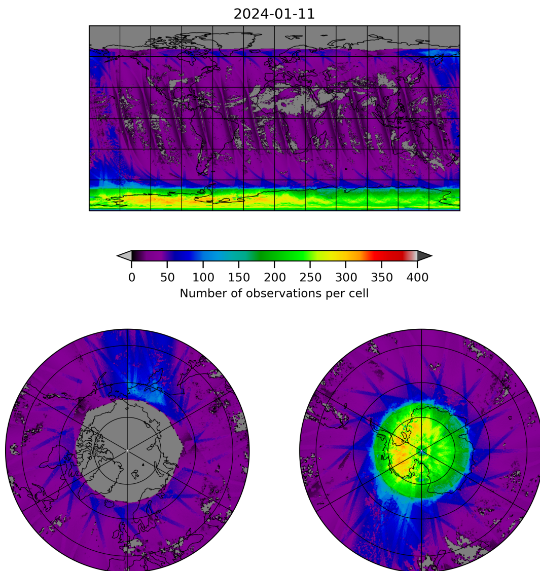
Figure 21: Map of the number of observations for 2024-01-10 to 2024-01-12
