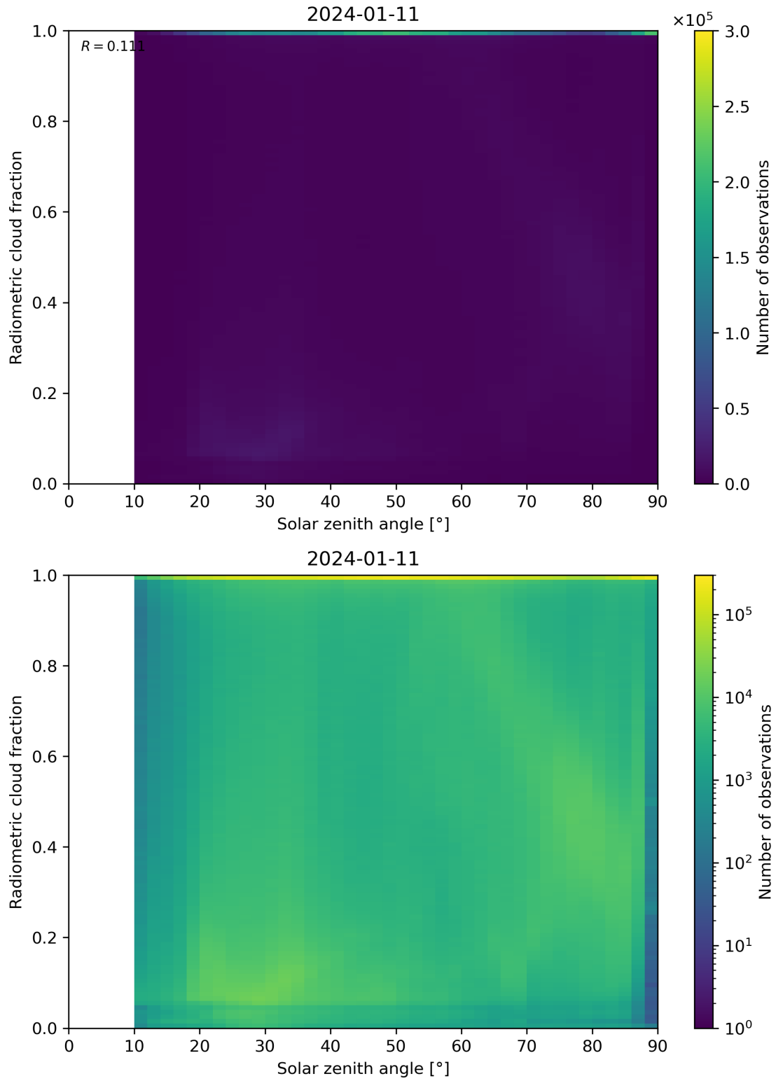
Figure 99: Scatter density plot of “Solar zenith angle” against “Radiometric cloud fraction” for 2024-01-10 to 2024-01-12.
