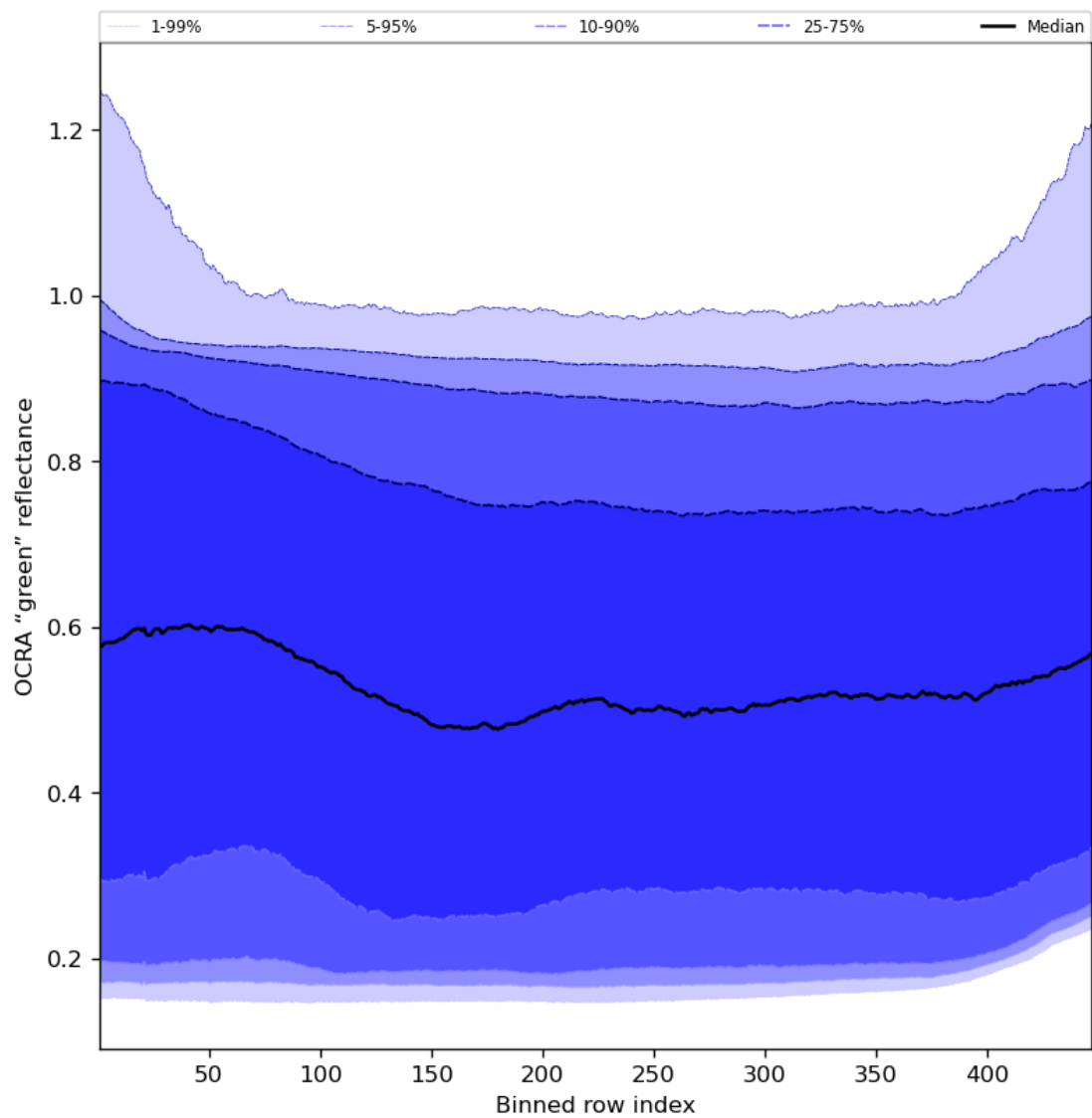
Figure 68: Along track statistics of “OCRA “green” reflectance” for 2024-01-10 to 2024-01-12
