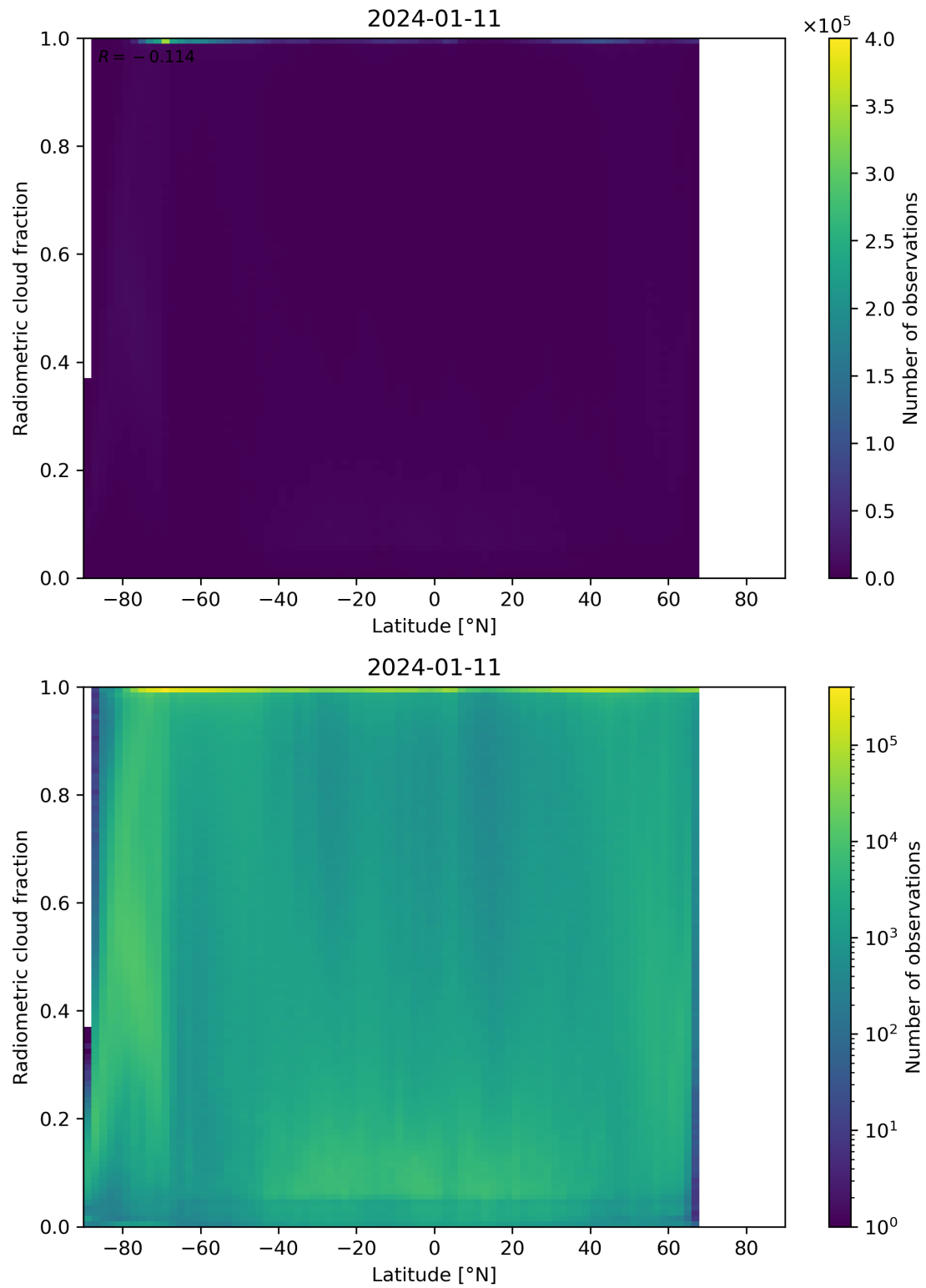
Figure 92: Scatter density plot of “Latitude” against “Radiometric cloud fraction” for 2024-01-10 to 2024-01-12.
