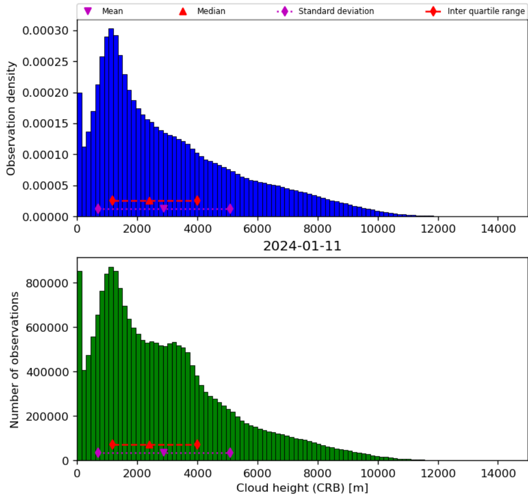
Figure 43: Histogram of “Cloud height (CRB)” for 2024-01-10 to 2024-01-12
