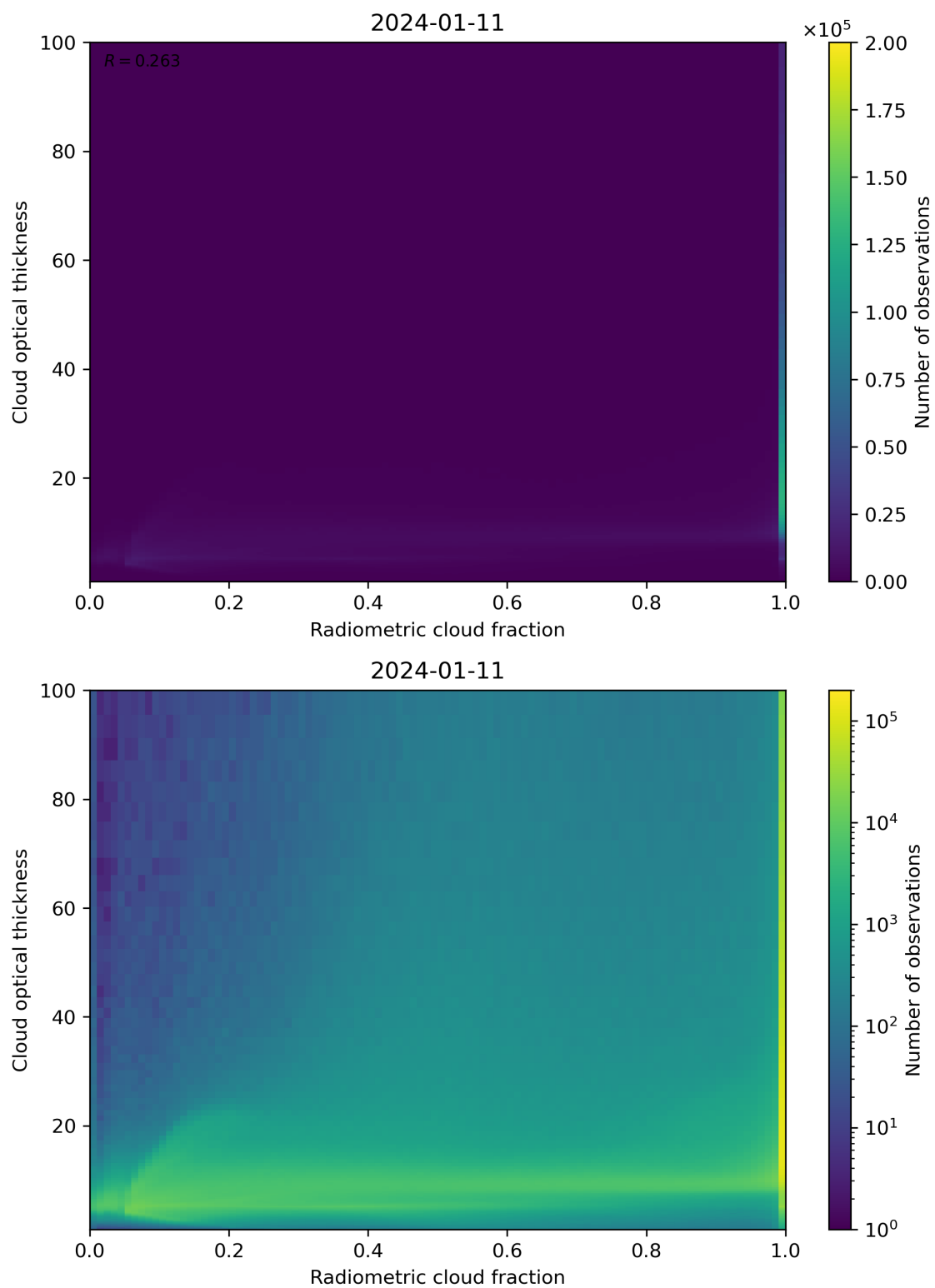
Figure 75: Scatter density plot of “Radiometric cloud fraction” against “Cloud optical thickness” for 2024-01-10 to 2024-01-12.
