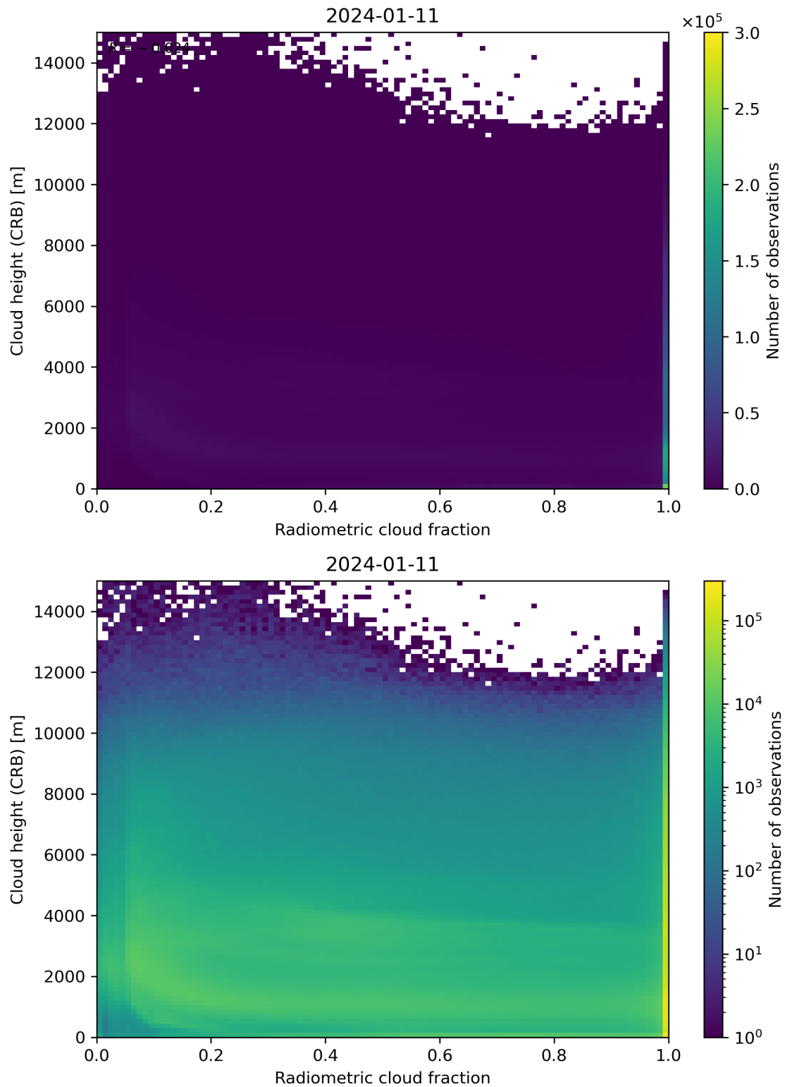
Figure 74: Scatter density plot of “Radiometric cloud fraction” against “Cloud height (CRB)” for 2024-01-10 to 2024-01-12.
