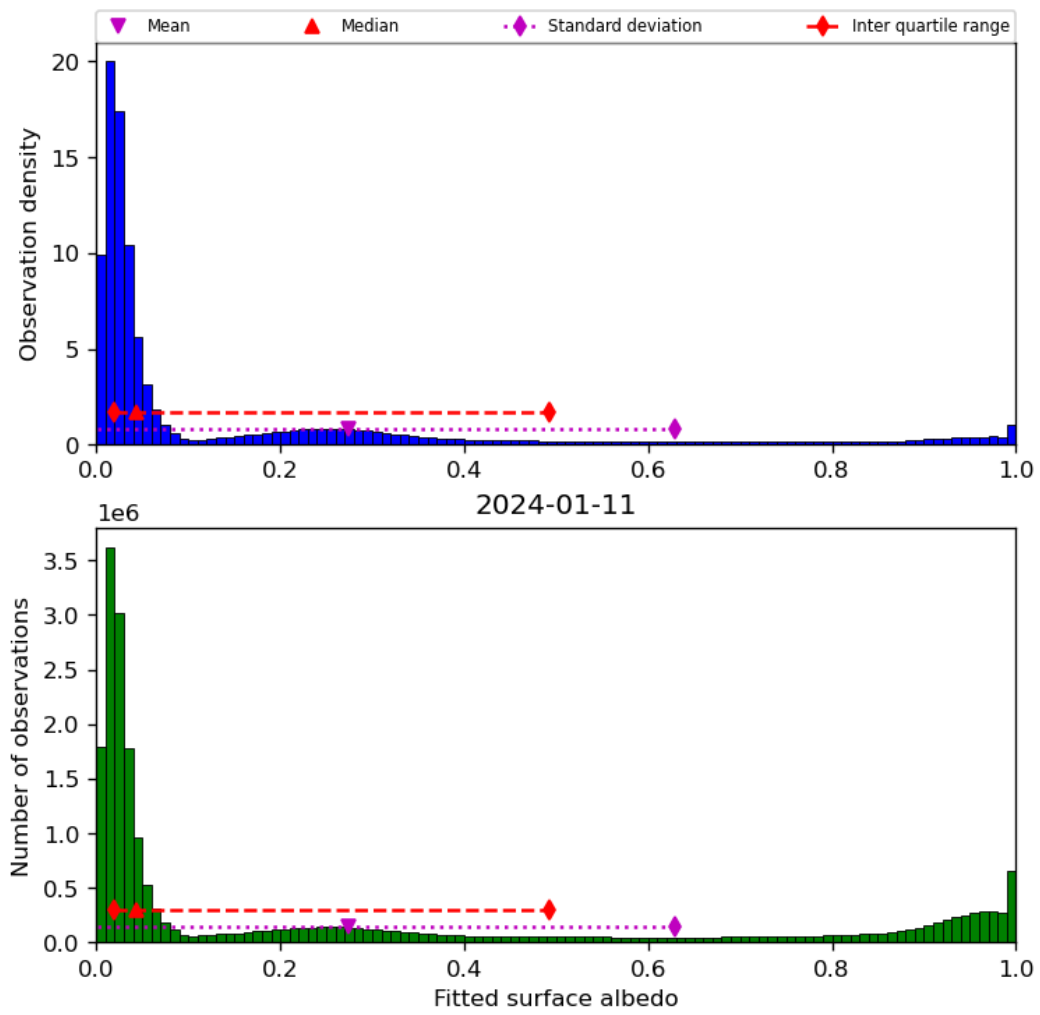
Figure 45: Histogram of “Fitted surface albedo” for 2024-01-10 to 2024-01-12
