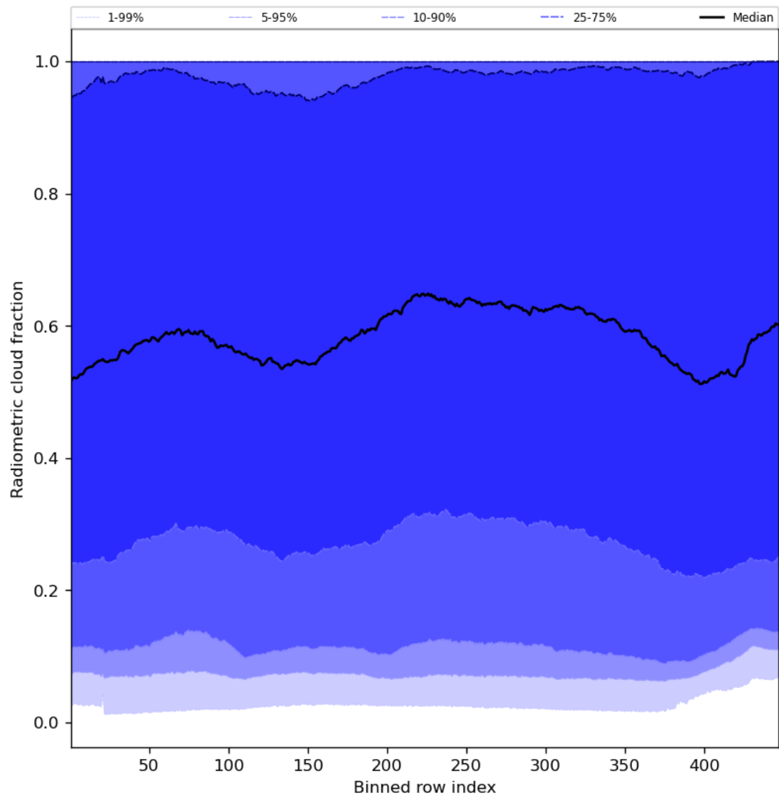
Figure 55: Along track statistics of “Radiometric cloud fraction” for 2024-01-10 to 2024-01-12
