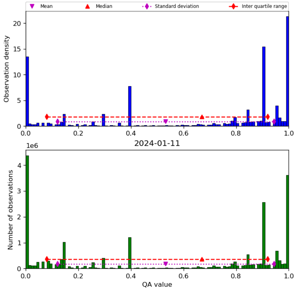
Figure 38: Histogram of “QA value” for 2024-01-10 to 2024-01-12
