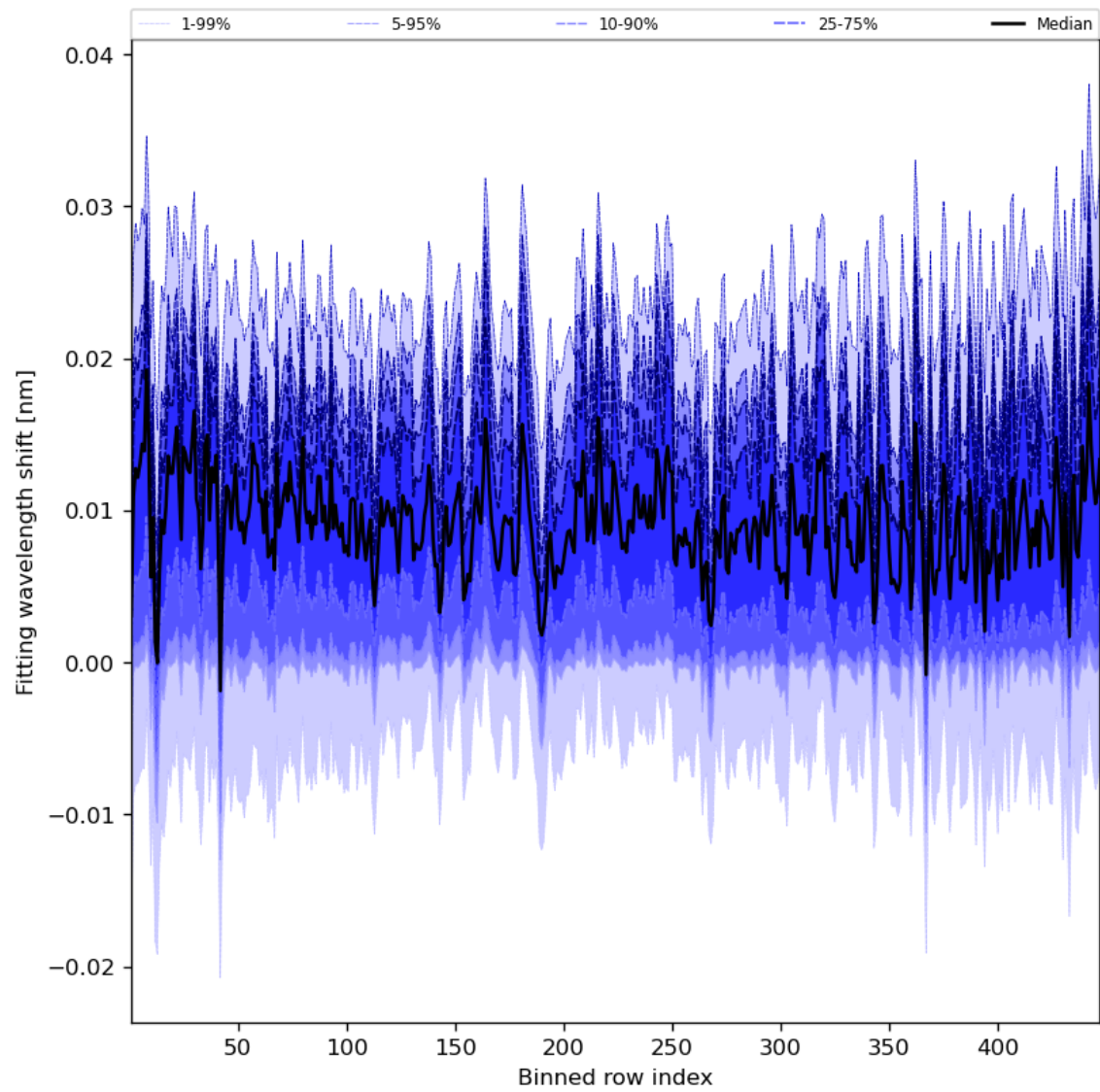
Figure 65: Along track statistics of “Fitting wavelength shift” for 2024-01-10 to 2024-01-12
