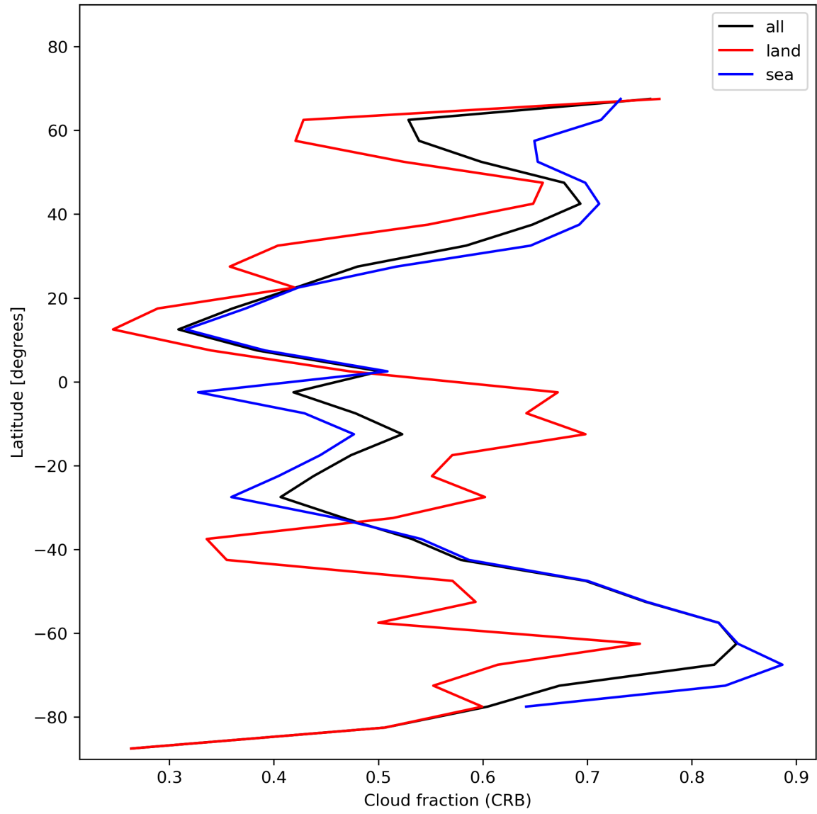
Figure 26: Zonal average of “Cloud fraction (CRB)” for 2024-01-10 to 2024-01-12.
