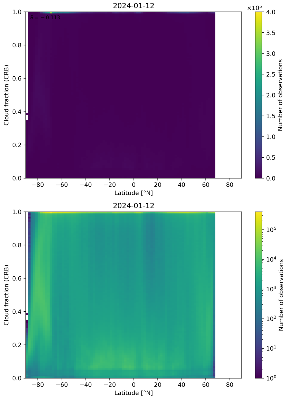
Figure 94: Scatter density plot of “Latitude” against “Cloud fraction (CRB)” for 2024-01-11 to 2024-01-13.
