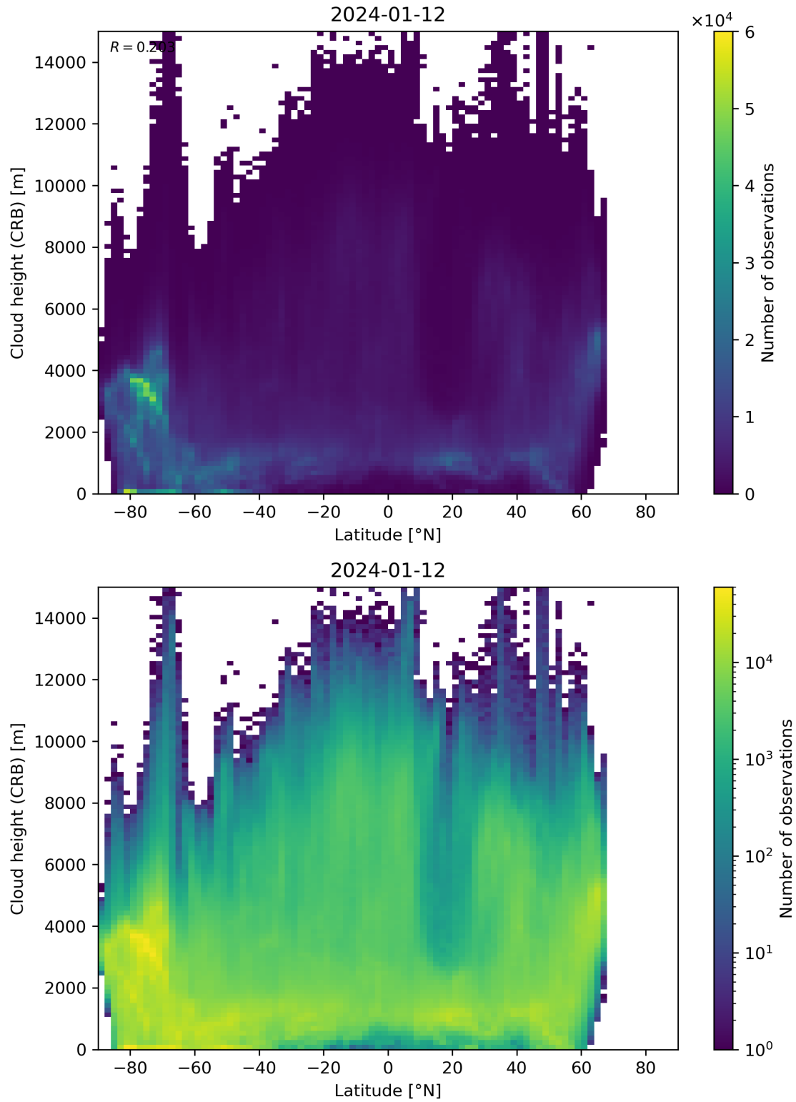
Figure 95: Scatter density plot of “Latitude” against “Cloud height (CRB)” for 2024-01-11 to 2024-01-13.
