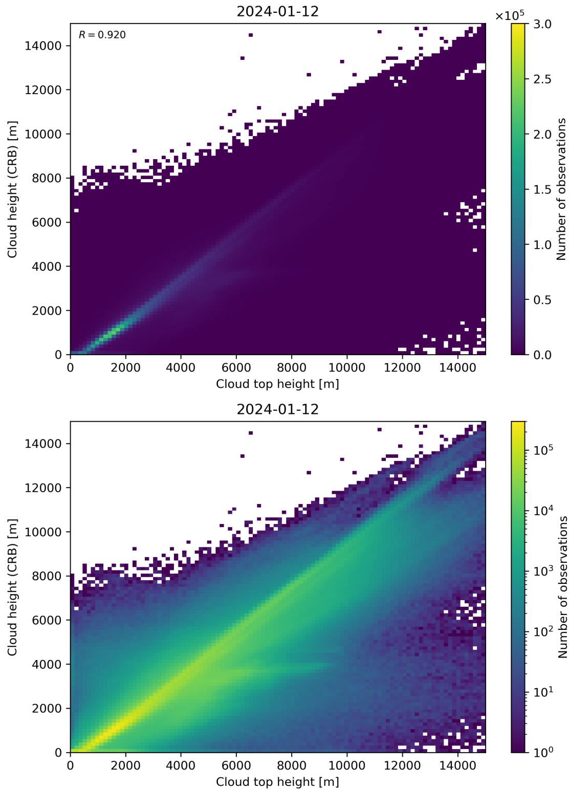
Figure 89: Scatter density plot of “Cloud top height” against “Cloud height (CRB)” for 2024-01-11 to 2024-01-13.
