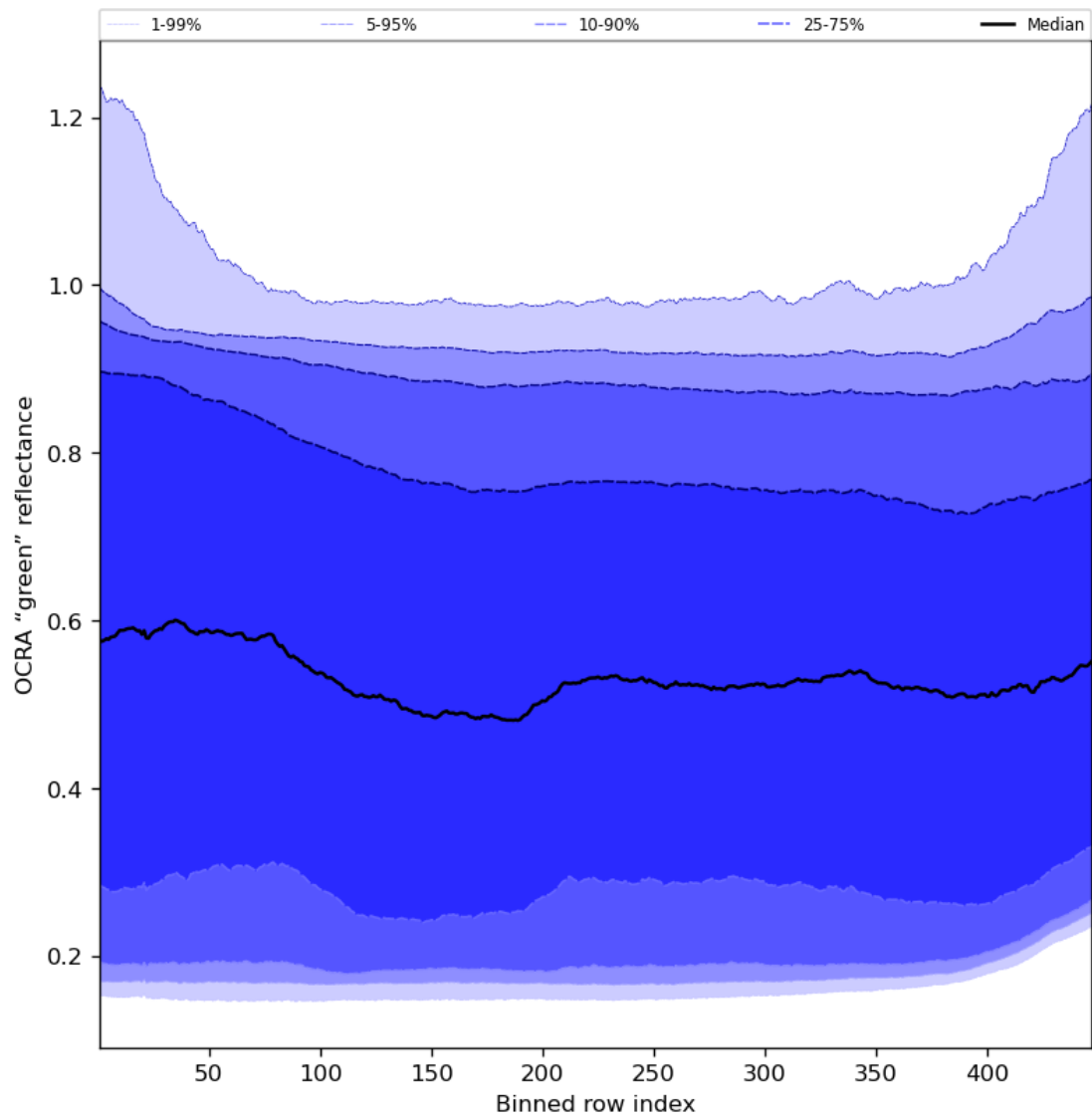
Figure 68: Along track statistics of "OCRA "green" reflectance" for 2024-01-11 to 2024-01-13
