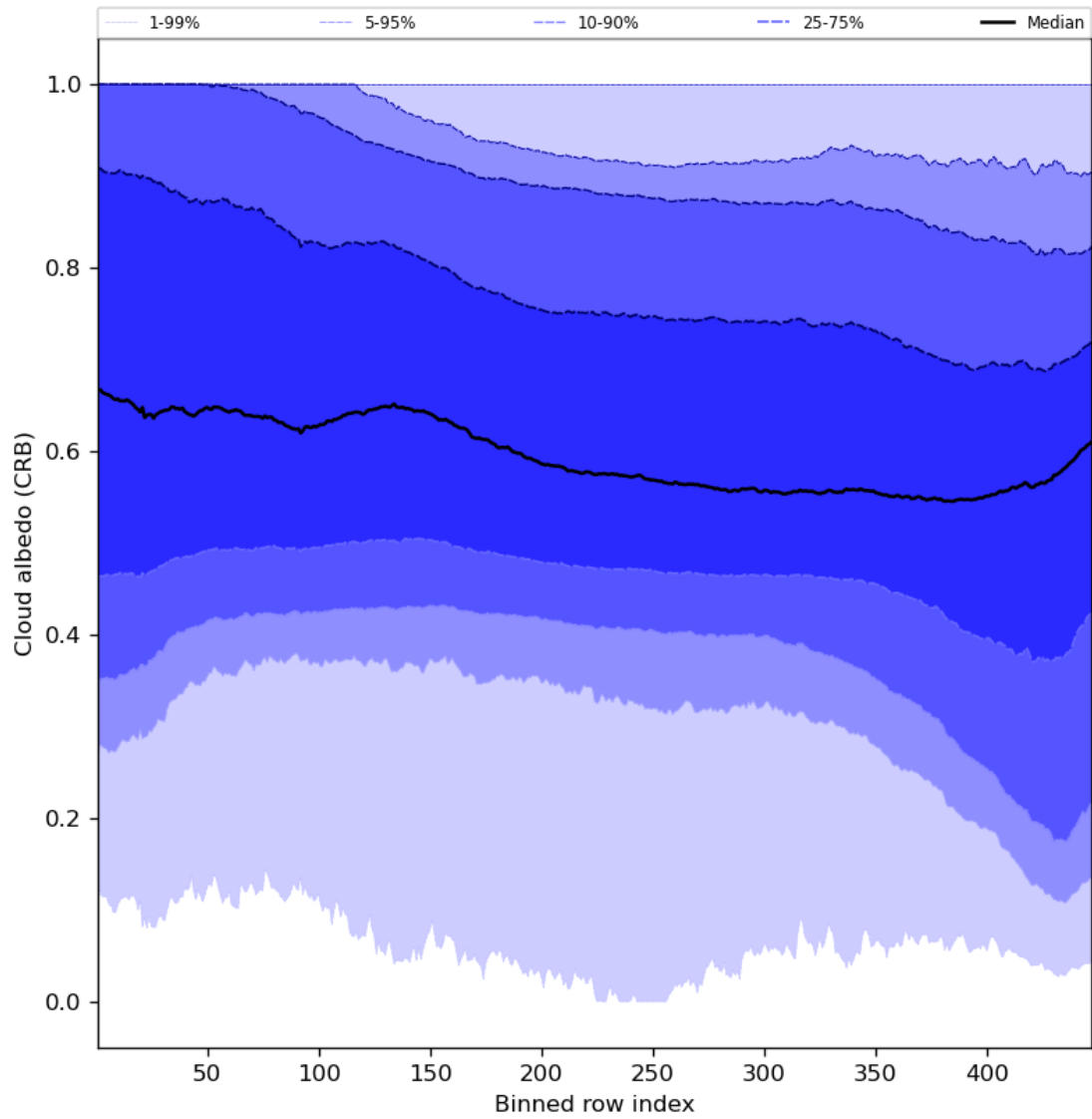
Figure 60: Along track statistics of “Cloud albedo (CRB)” for 2024-01-11 to 2024-01-13
