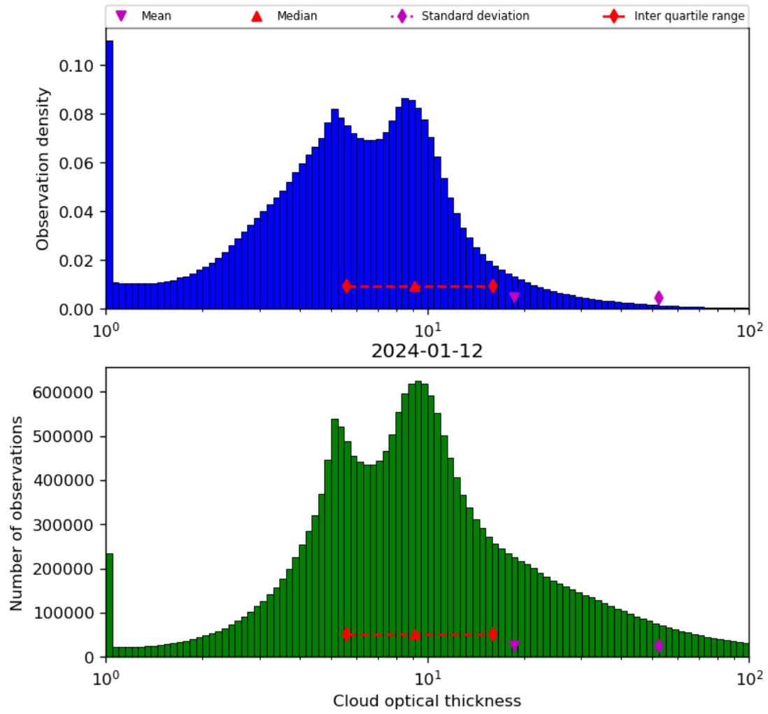
Figure 41: Histogram of “Cloud optical thickness” for 2024-01-11 to 2024-01-13
