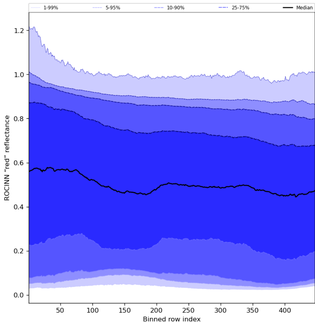
Figure 69: Along track statistics of “ROCINN “red” reflectance” for 2024-01-11 to 2024-01-13
