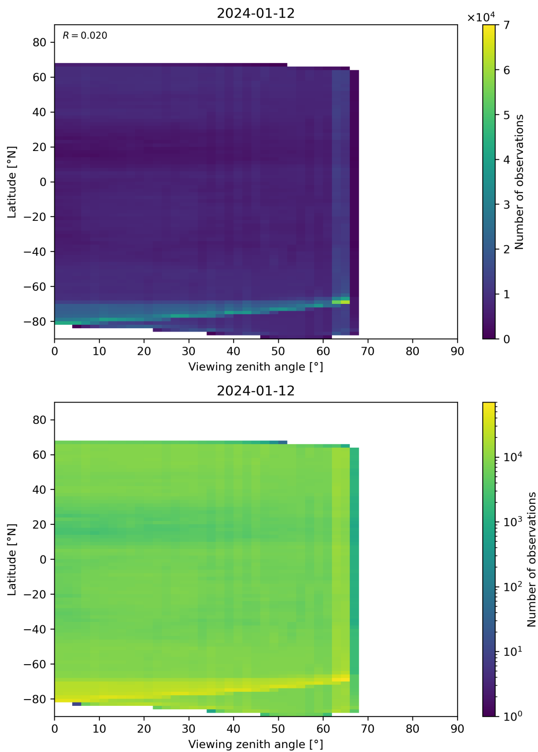
Figure 113: Scatter density plot of “Viewing zenith angle” against “Latitude” for 2024-01-11 to 2024-01-13.
