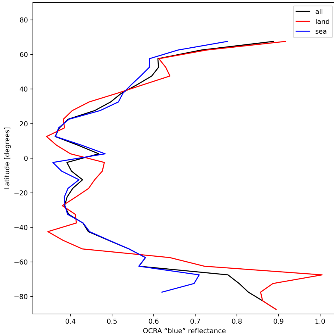
Figure 35: Zonal average of “OCRA “blue” reflectance” for 2024-01-11 to 2024-01-13.
