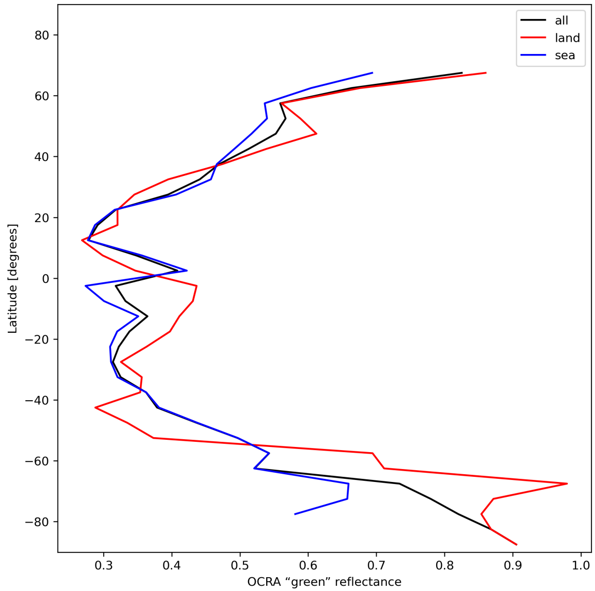
Figure 36: Zonal average of “OCRA “green” reflectance” for 2024-01-11 to 2024-01-13.
