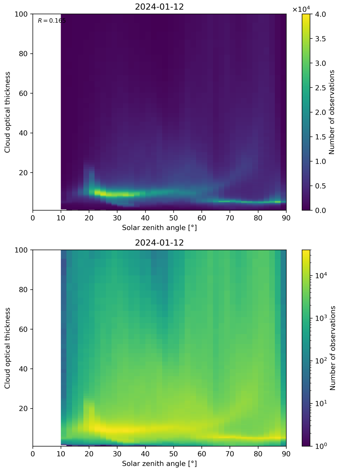
Figure 103: Scatter density plot of “Solar zenith angle” against “Cloud optical thickness” for 2024-01-11 to 2024-01-13.
