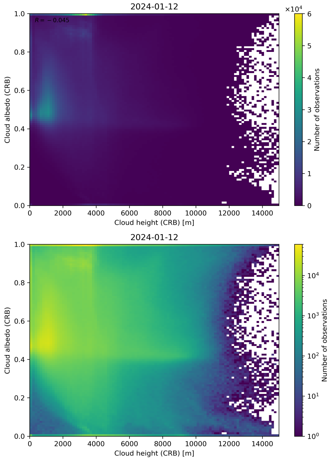
Figure 80: Scatter density plot of “Cloud height (CRB)” against “Cloud albedo (CRB)” for 2024-01-11 to 2024-01-13.
