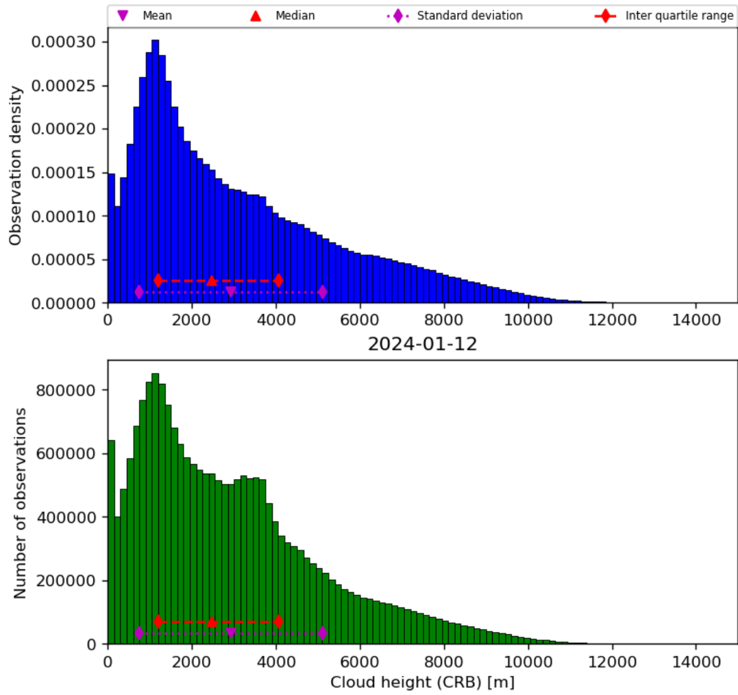
Figure 43: Histogram of “Cloud height (CRB)” for 2024-01-11 to 2024-01-13
