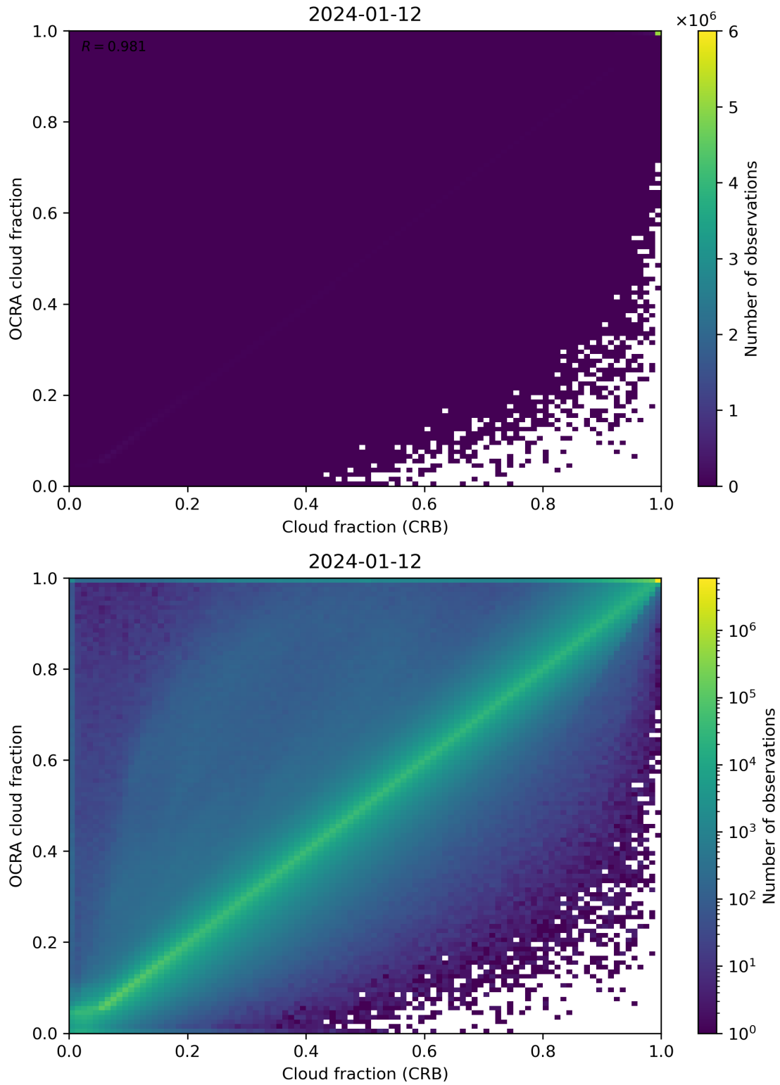
Figure 78: Scatter density plot of “Cloud fraction (CRB)” against “OCRA cloud fraction” for 2024-01-11 to 2024-01-13.
