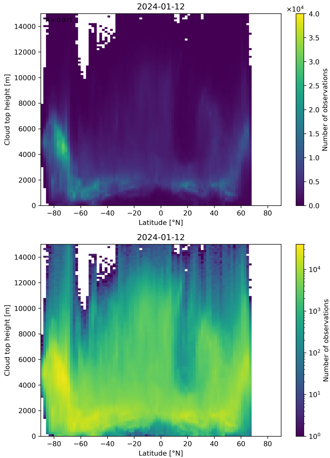
Figure 97: Scatter density plot of “Latitude” against “Cloud top height” for 2024-01-11 to 2024-01-13.
