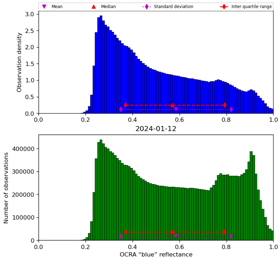
Figure 51: Histogram of “OCRA “blue” reflectance” for 2024-01-11 to 2024-01-13
