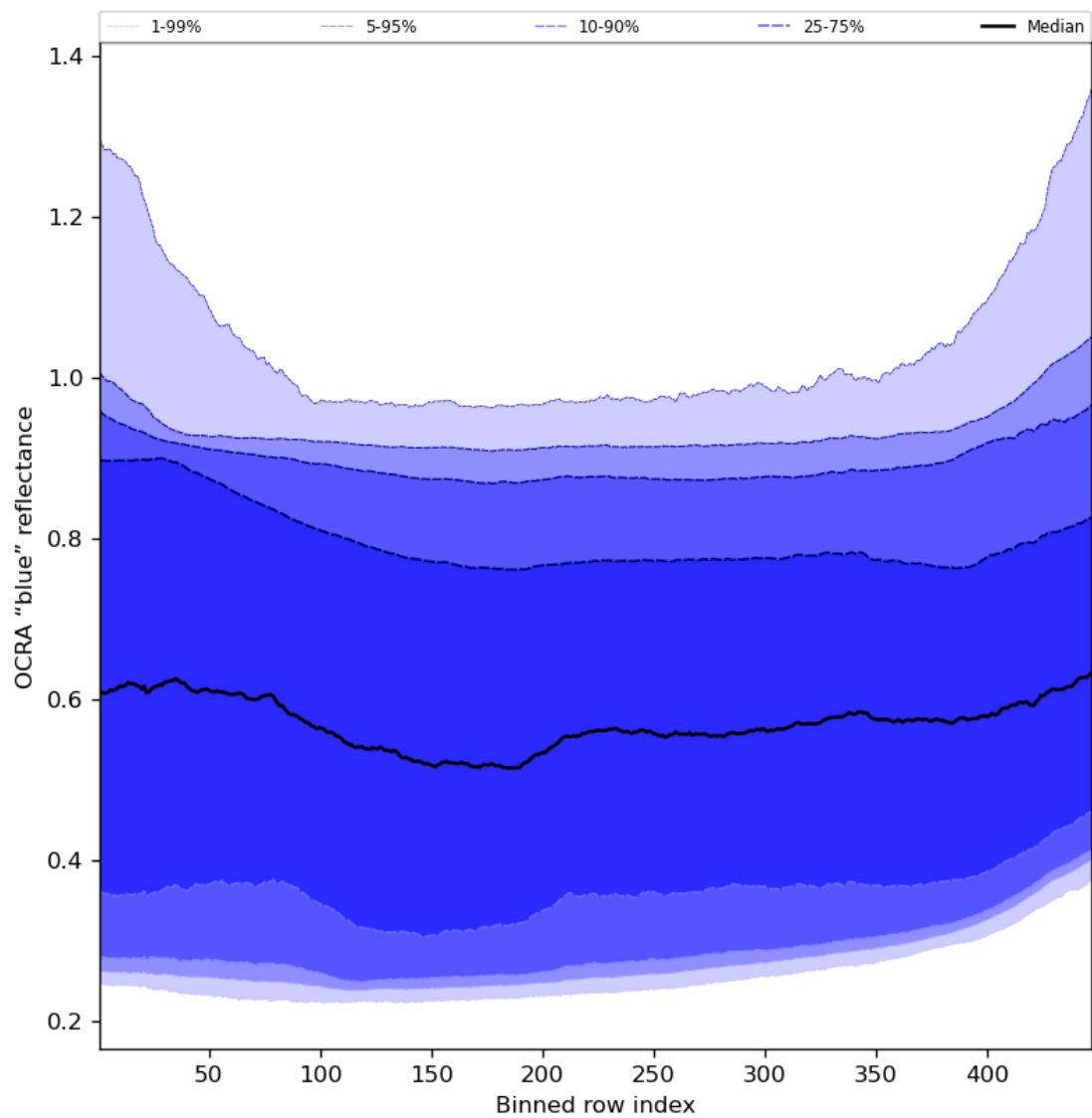
Figure 67: Along track statistics of “OCRA “blue” reflectance” for 2024-01-11 to 2024-01-13
