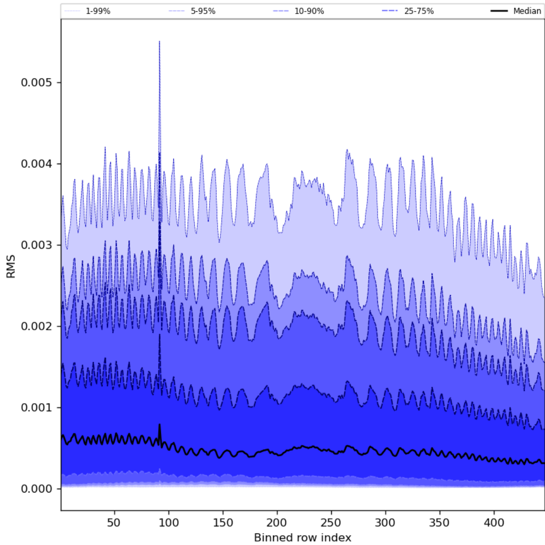
Figure 63: Along track statistics of “RMS” for 2024-01-11 to 2024-01-13
