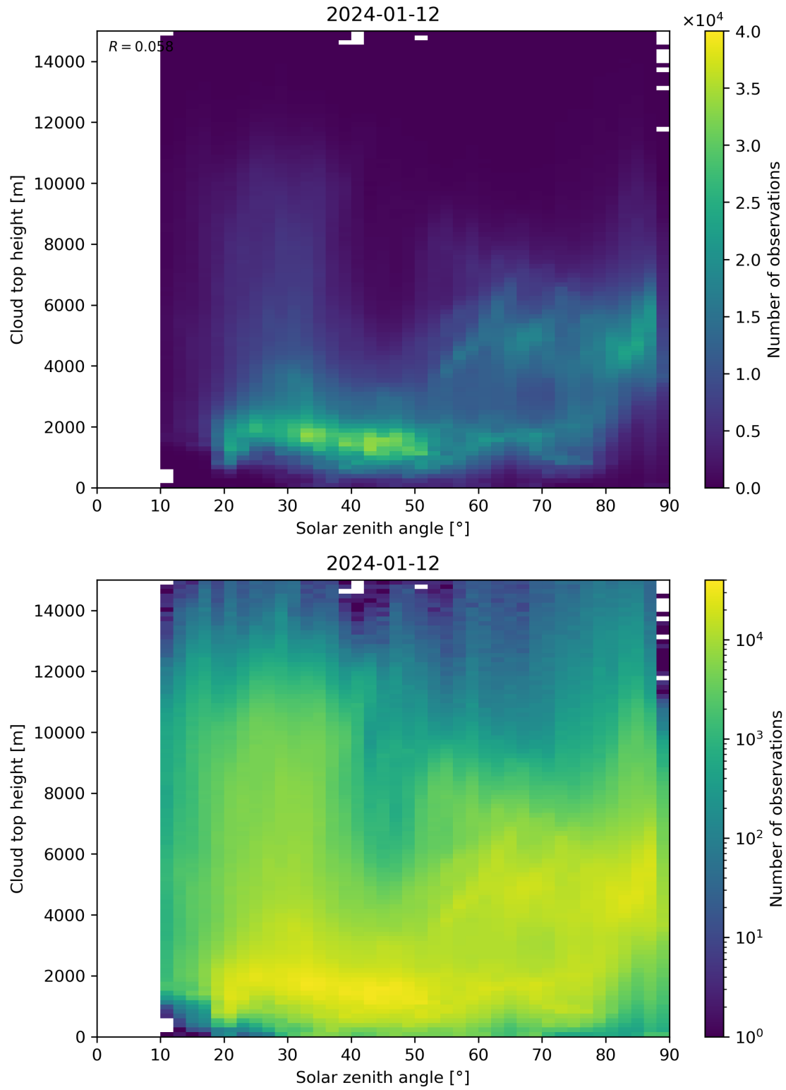
Figure 104: Scatter density plot of “Solar zenith angle” against “Cloud top height” for 2024-01-11 to 2024-01-13.
