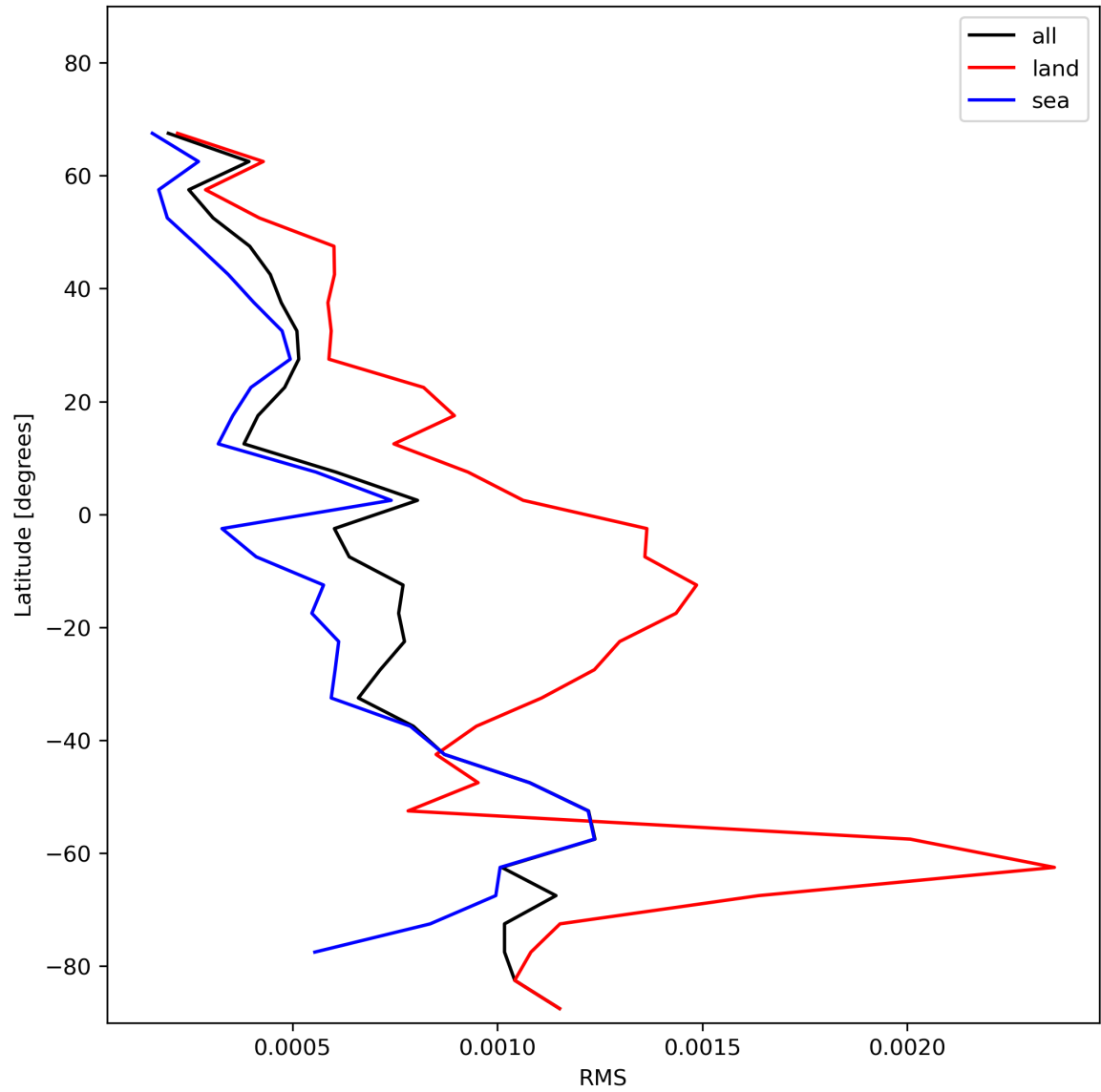
Figure 31: Zonal average of “RMS” for 2024-01-11 to 2024-01-13.
