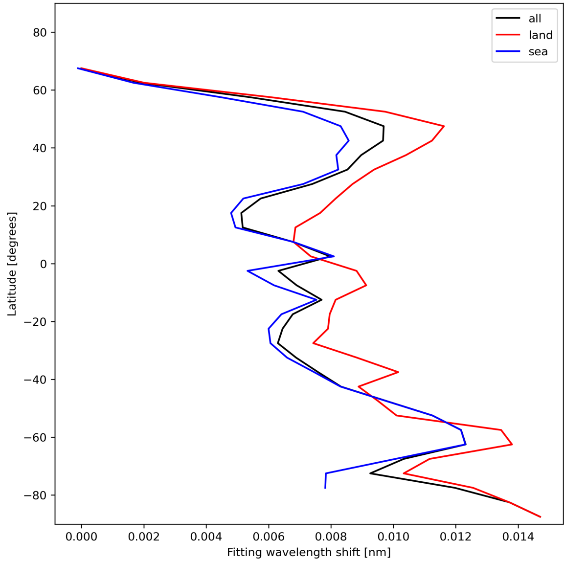
Figure 33: Zonal average of “Fitting wavelength shift” for 2024-01-11 to 2024-01-13.
