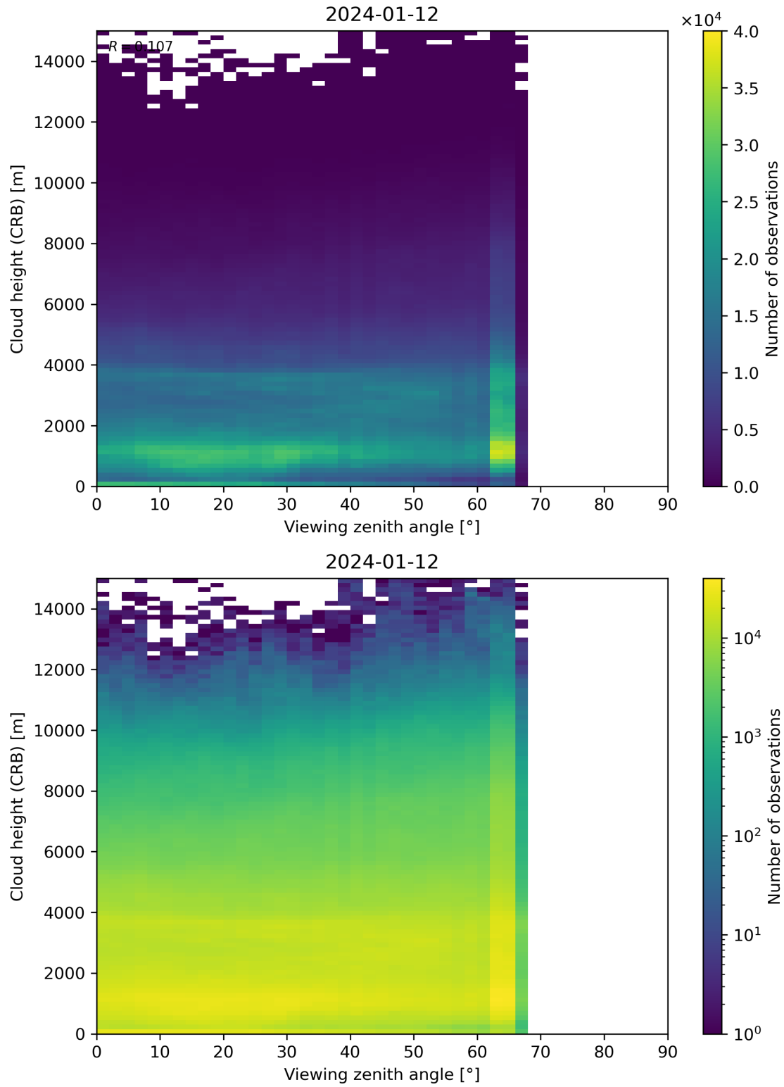
Figure 110: Scatter density plot of “Viewing zenith angle” against “Cloud height (CRB)” for 2024-01-11 to 2024-01-13.
