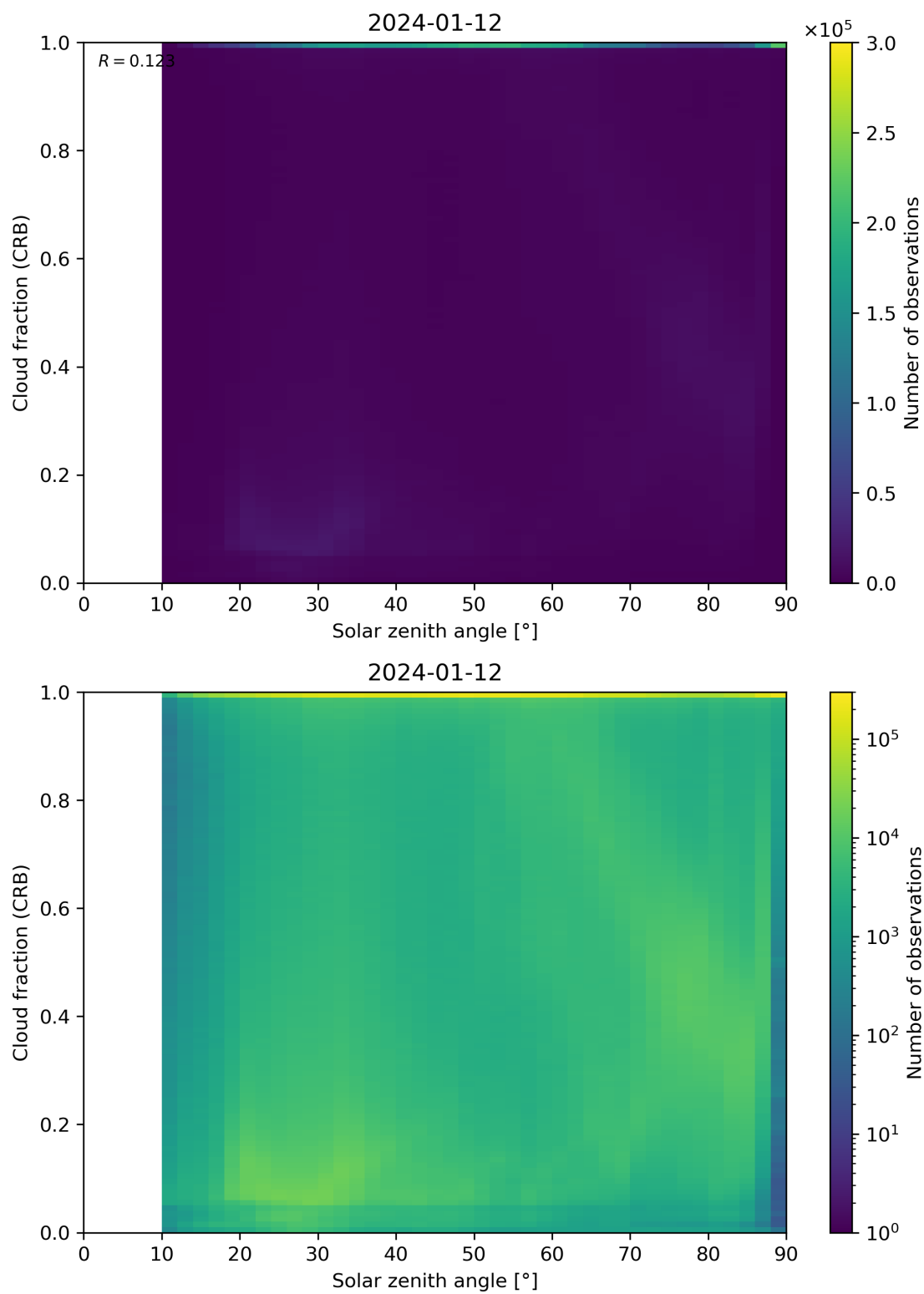
Figure 101: Scatter density plot of “Solar zenith angle” against “Cloud fraction (CRB)” for 2024-01-11 to 2024-01-13.
