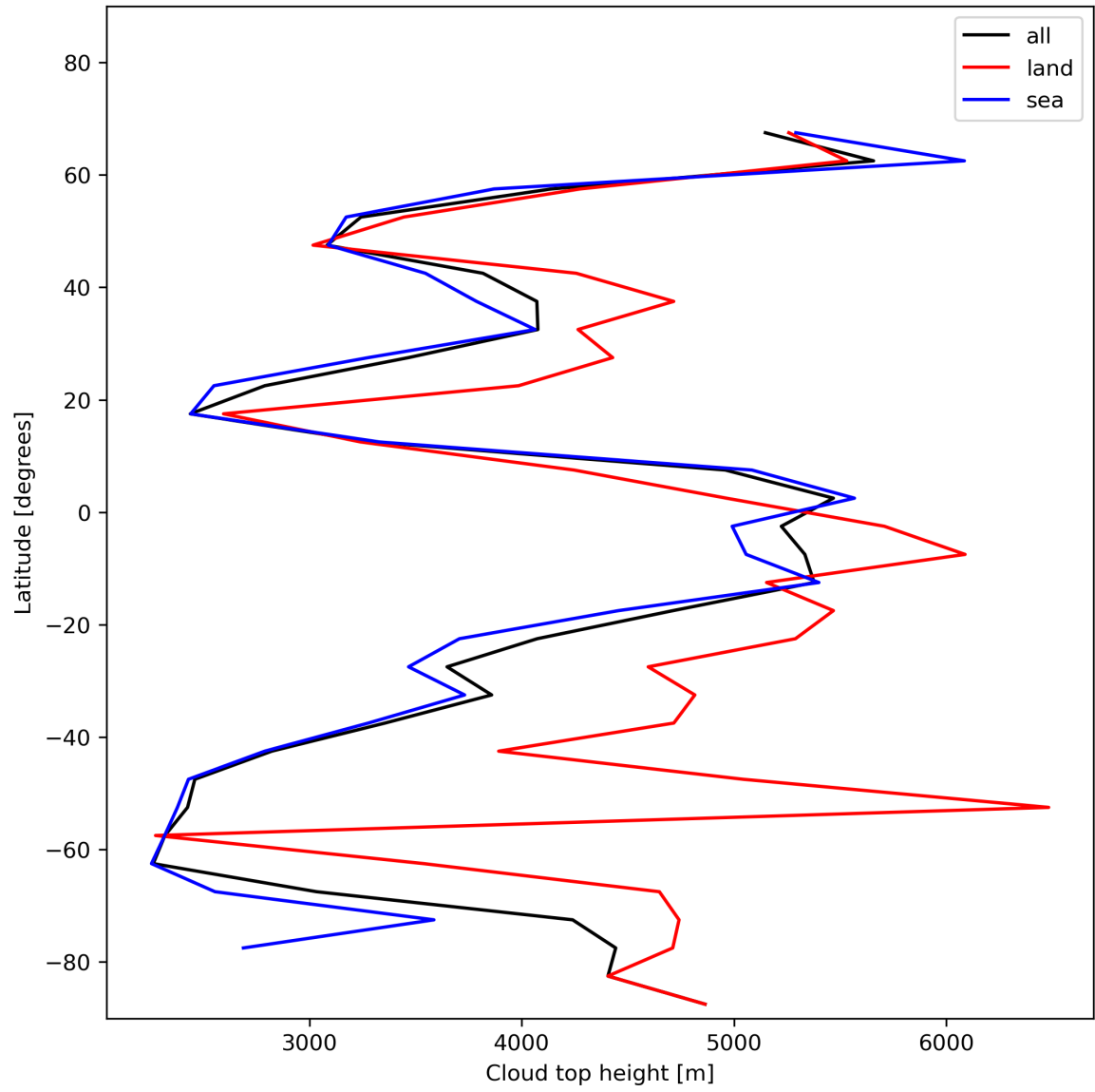
Figure 24: Zonal average of “Cloud top height” for 2024-01-11 to 2024-01-13.
