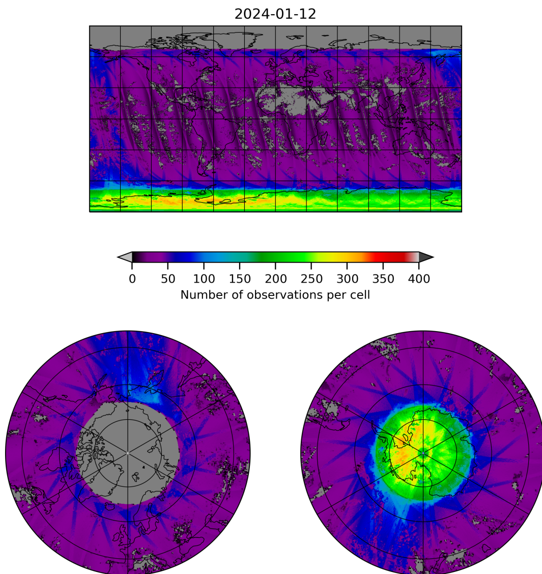
Figure 21: Map of the number of observations for 2024-01-11 to 2024-01-13
