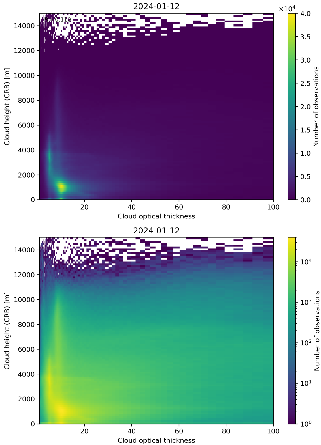
Figure 85: Scatter density plot of “Cloud optical thickness” against “Cloud height (CRB)” for 2024-01-11 to 2024-01-13.
