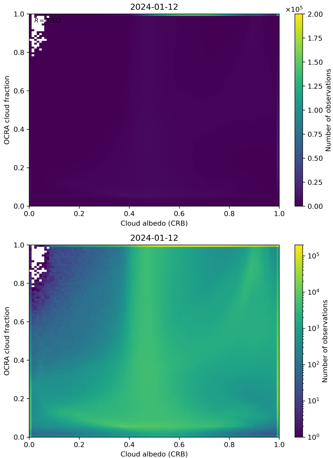
Figure 70: Scatter density plot of “Cloud albedo (CRB)” against “OCRA cloud fraction” for 2024-01-11 to 2024-01-13.
