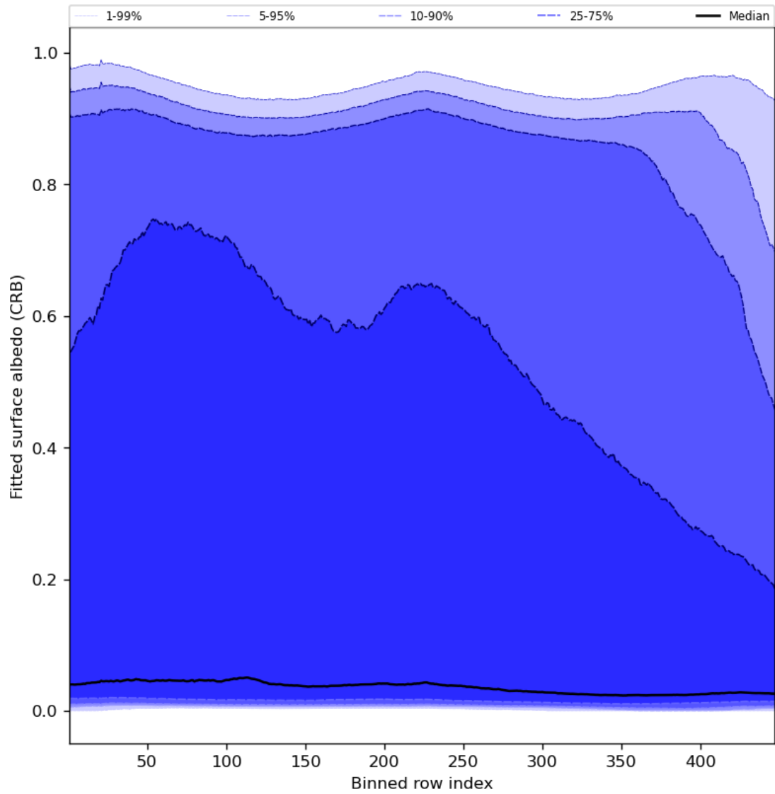
Figure 62: Along track statistics of “Fitted surface albedo (CRB)” for 2024-01-11 to 2024-01-13
