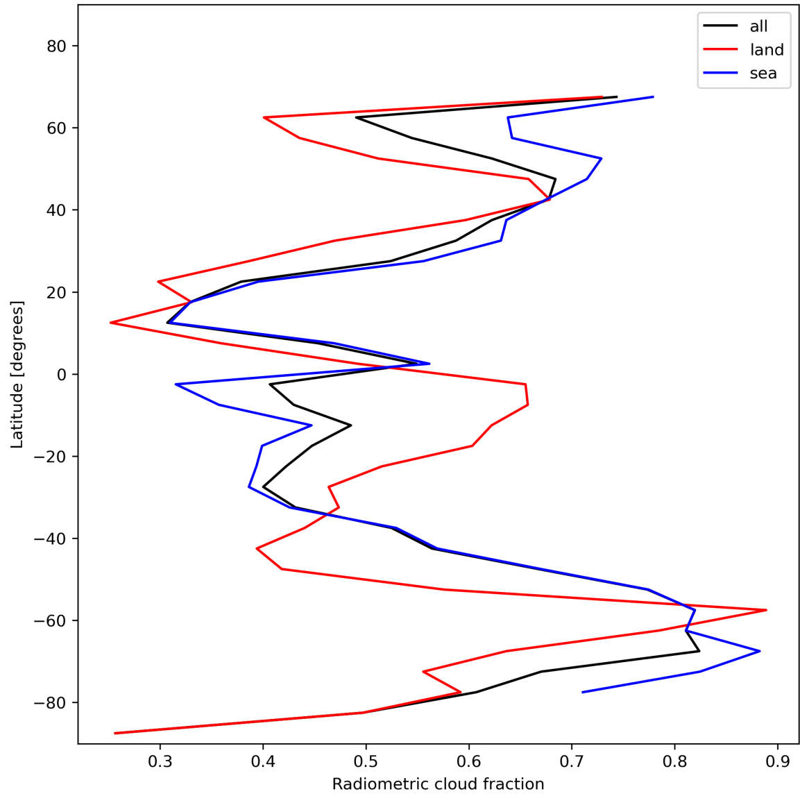
Figure 23: Zonal average of “Radiometric cloud fraction” for 2024-01-11 to 2024-01-13.
