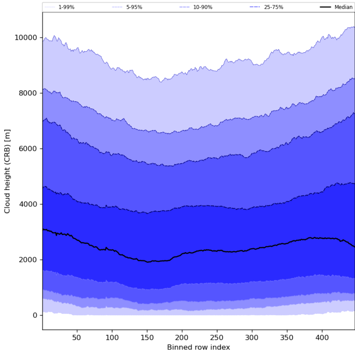
Figure 59: Along track statistics of “Cloud height (CRB)” for 2024-01-11 to 2024-01-13
