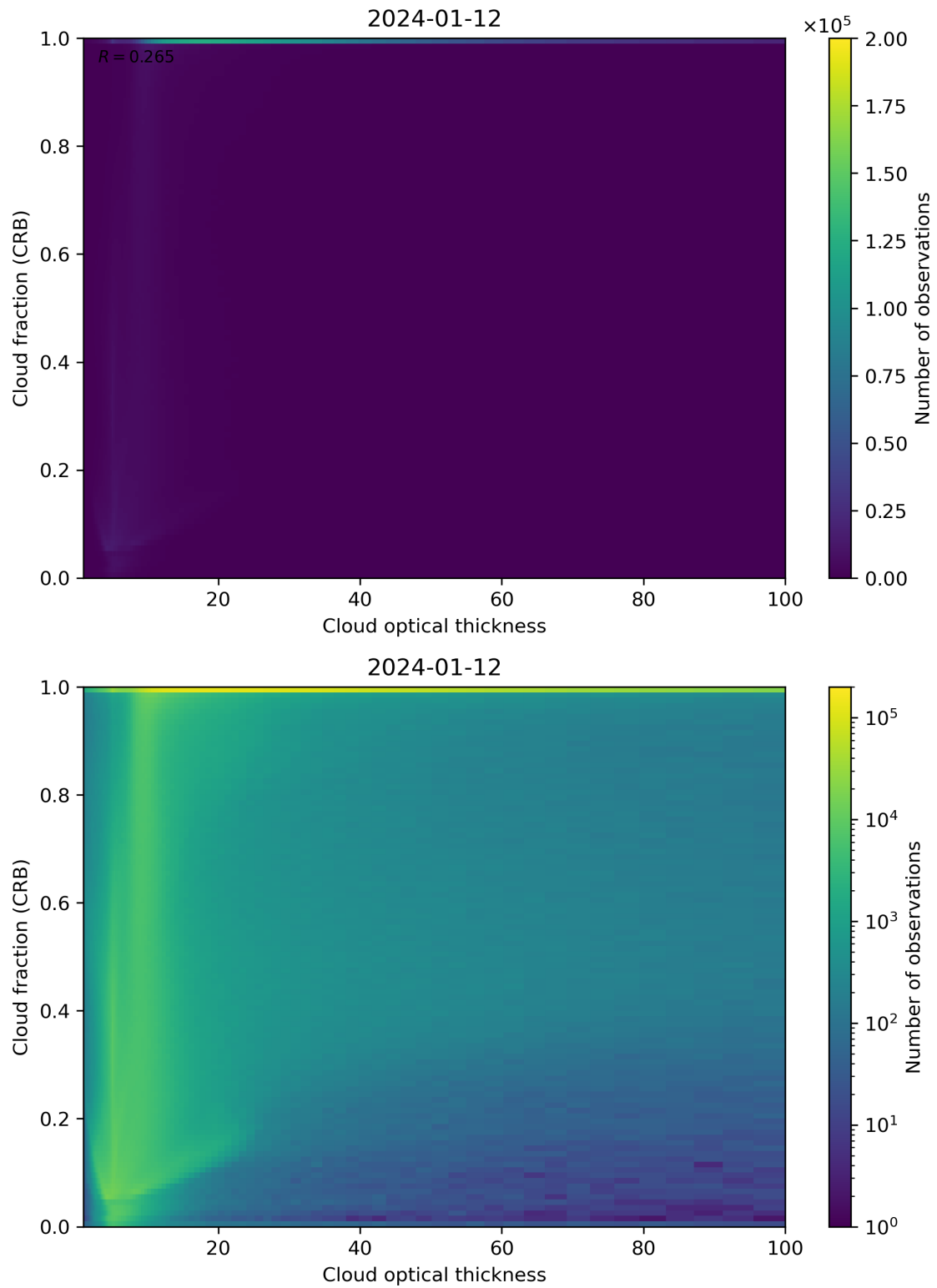
Figure 84: Scatter density plot of “Cloud optical thickness” against “Cloud fraction (CRB)” for 2024-01-11 to 2024-01-13.
