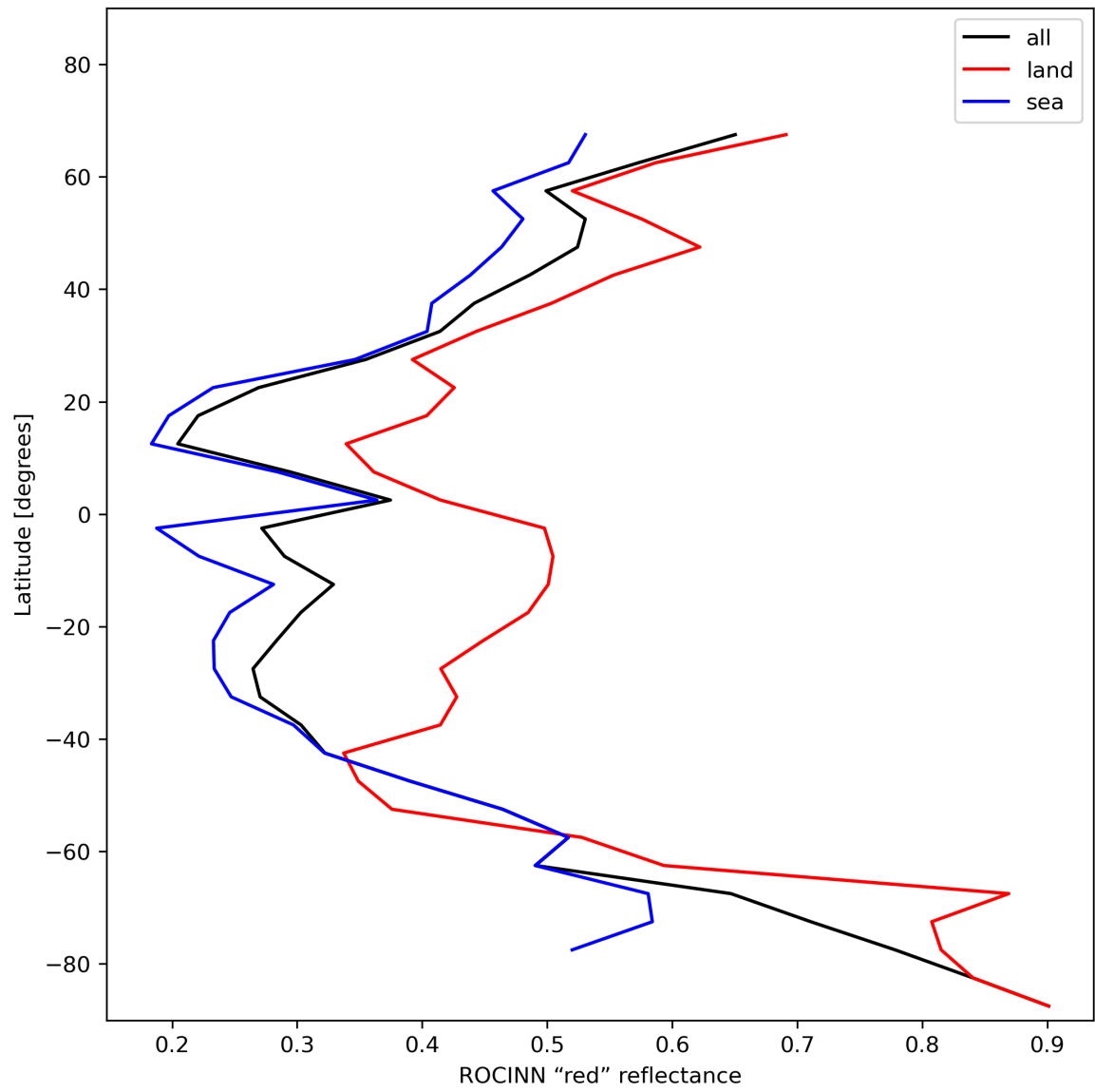
Figure 37: Zonal average of “ROCINN “red” reflectance” for 2024-01-11 to 2024-01-13.
