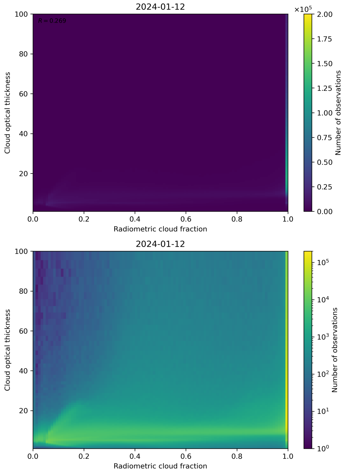
Figure 75: Scatter density plot of “Radiometric cloud fraction” against “Cloud optical thickness” for 2024-01-11 to 2024-01-13.
