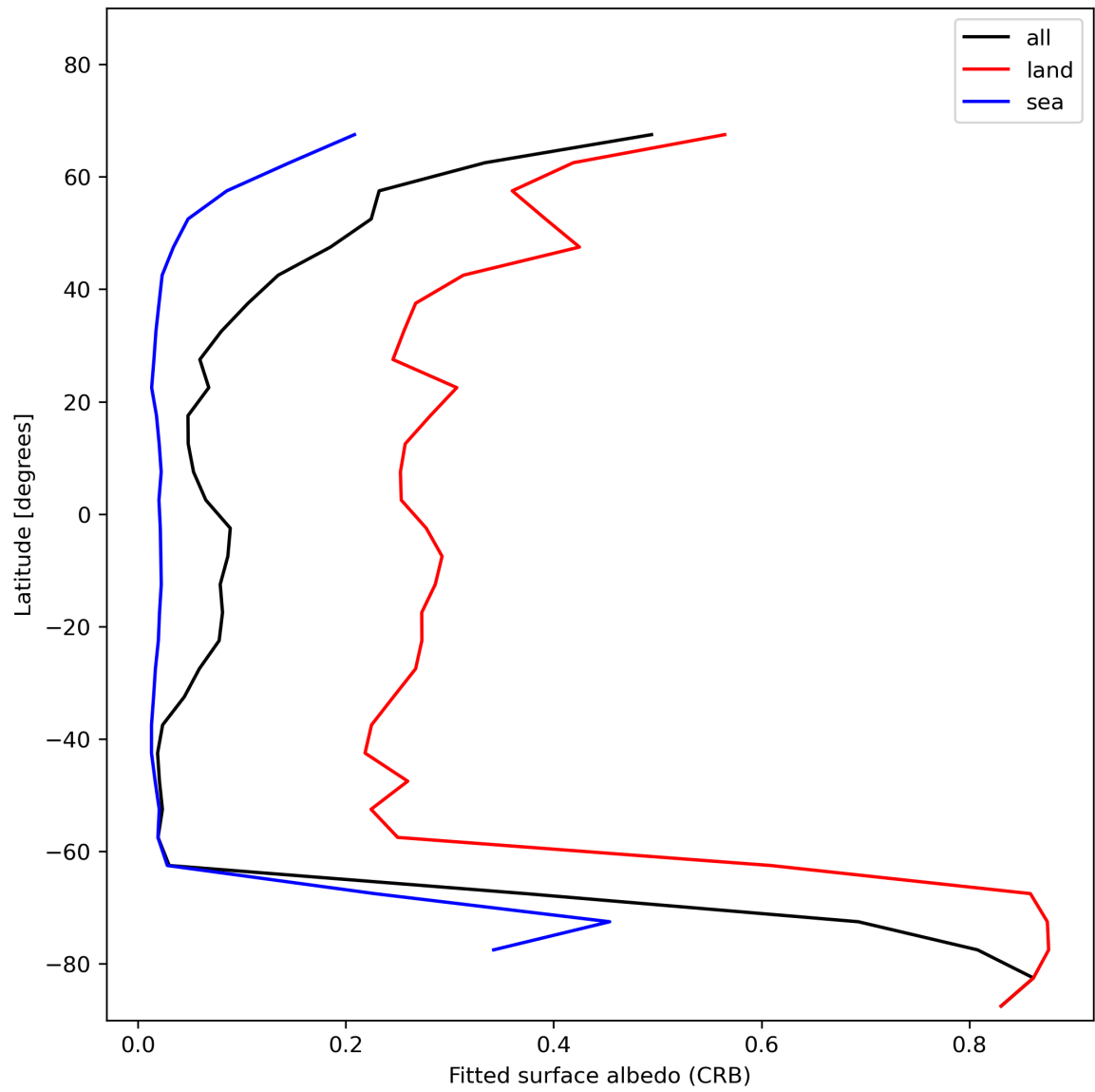
Figure 30: Zonal average of “Fitted surface albedo (CRB)” for 2024-01-11 to 2024-01-13.
