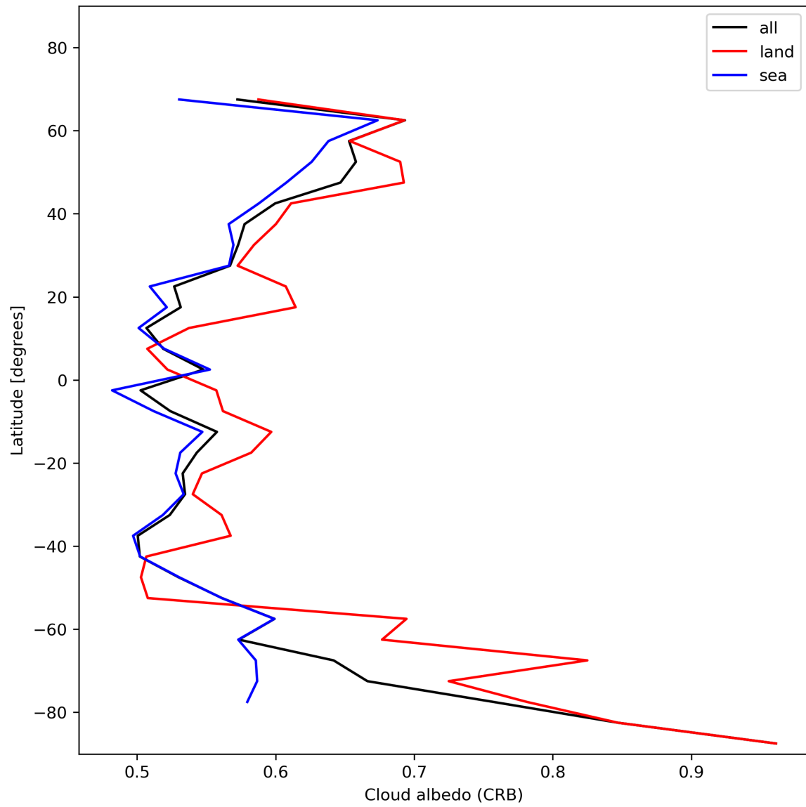
Figure 28: Zonal average of “Cloud albedo (CRB)” for 2024-01-11 to 2024-01-13.
