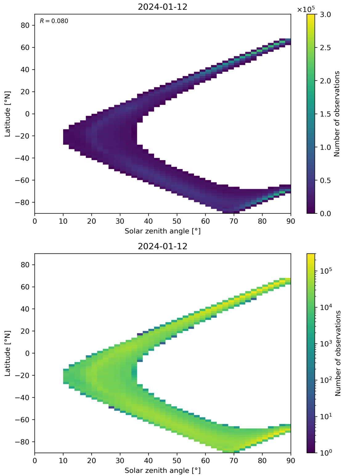
Figure 105: Scatter density plot of “Solar zenith angle” against “Latitude” for 2024-01-11 to 2024-01-13.
