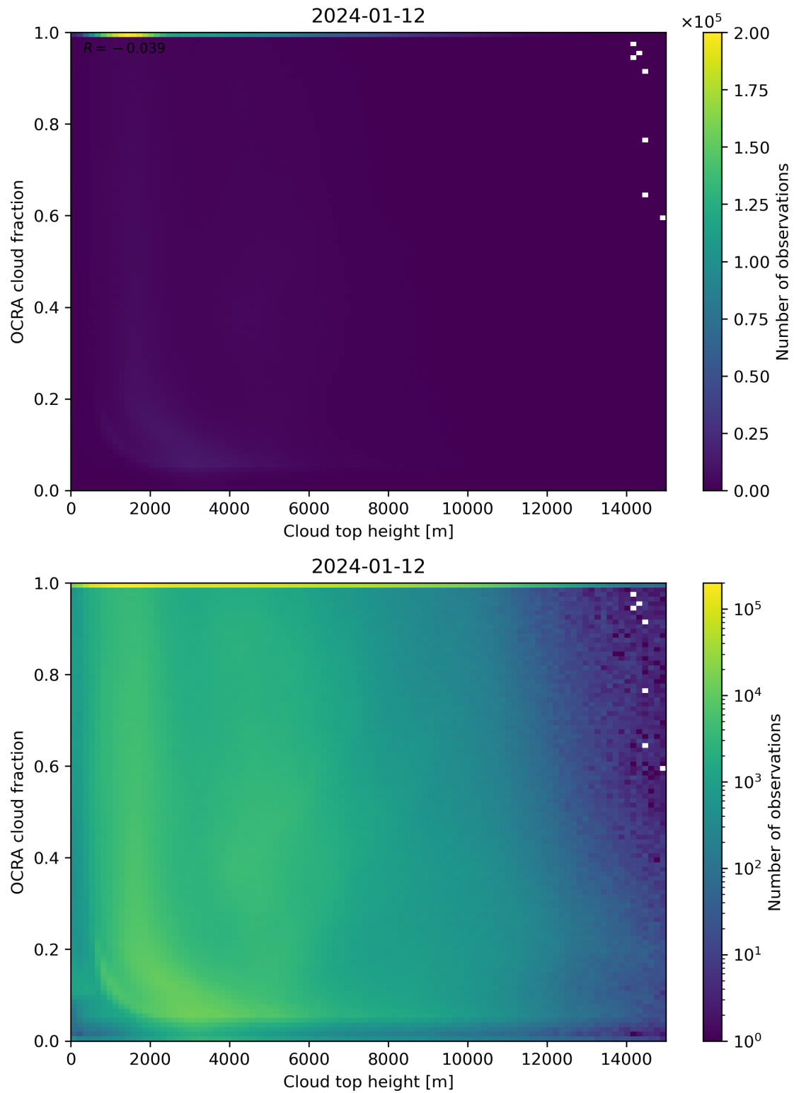
Figure 87: Scatter density plot of “Cloud top height” against “OCRA cloud fraction” for 2024-01-11 to 2024-01-13.
