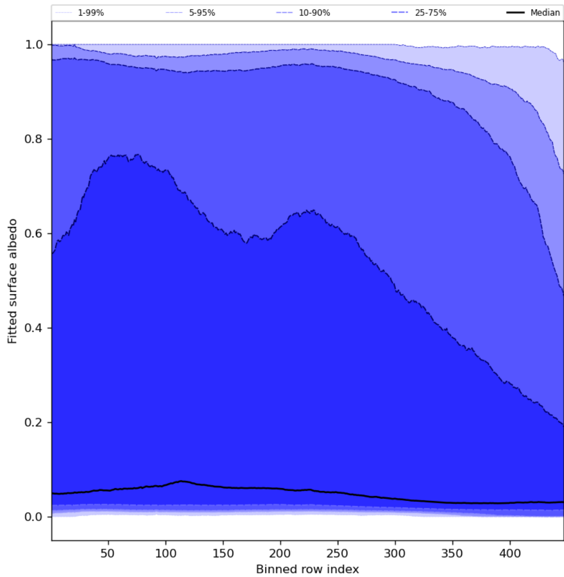
Figure 61: Along track statistics of “Fitted surface albedo” for 2024-01-11 to 2024-01-13
