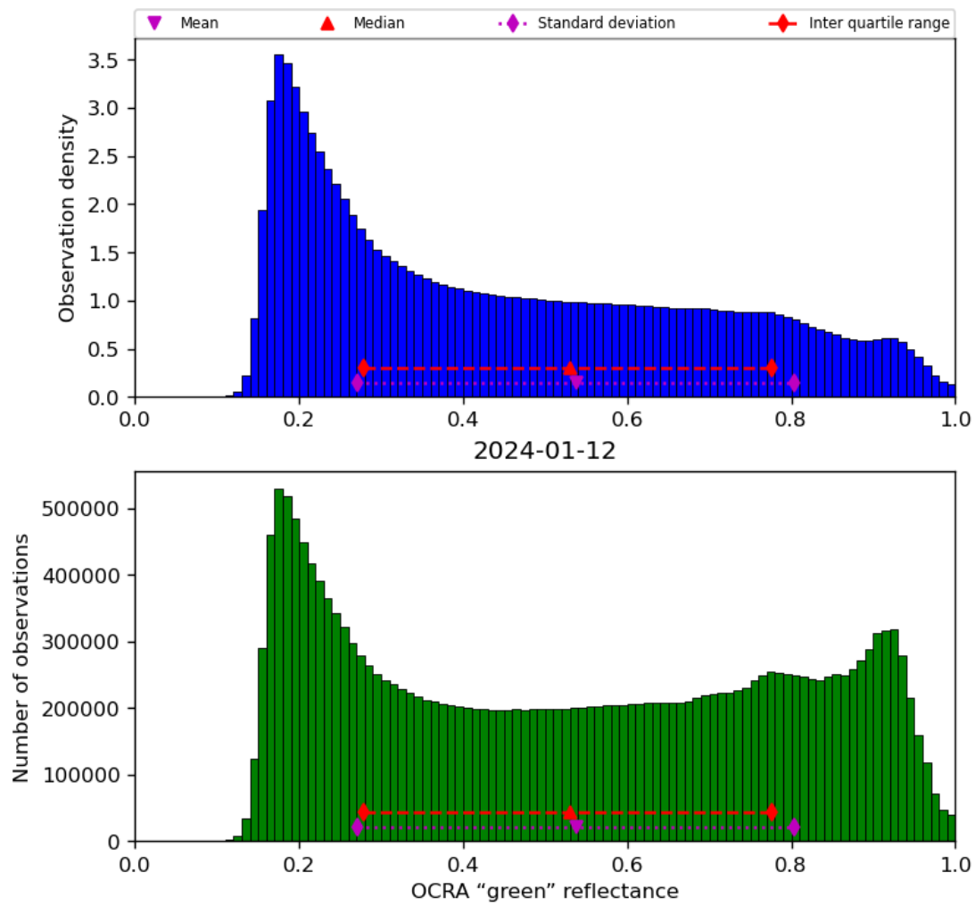
Figure 52: Histogram of “OCRA “green” reflectance” for 2024-01-11 to 2024-01-13
