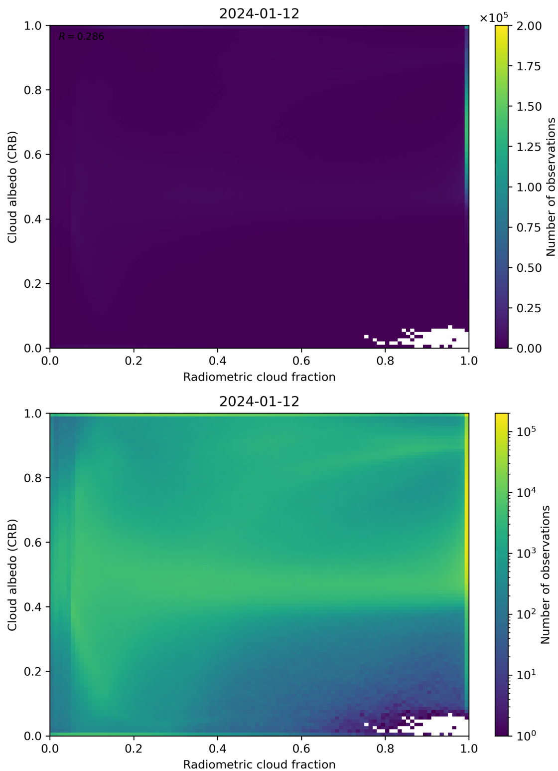
Figure 71: Scatter density plot of “Radiometric cloud fraction” against “Cloud albedo (CRB)” for 2024-01-11 to 2024-01-13.
