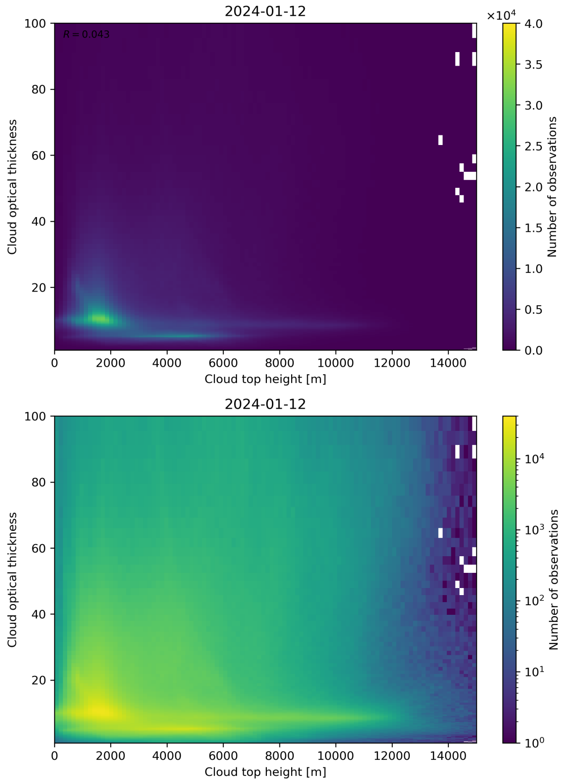
Figure 90: Scatter density plot of “Cloud top height” against “Cloud optical thickness” for 2024-01-11 to 2024-01-13.
