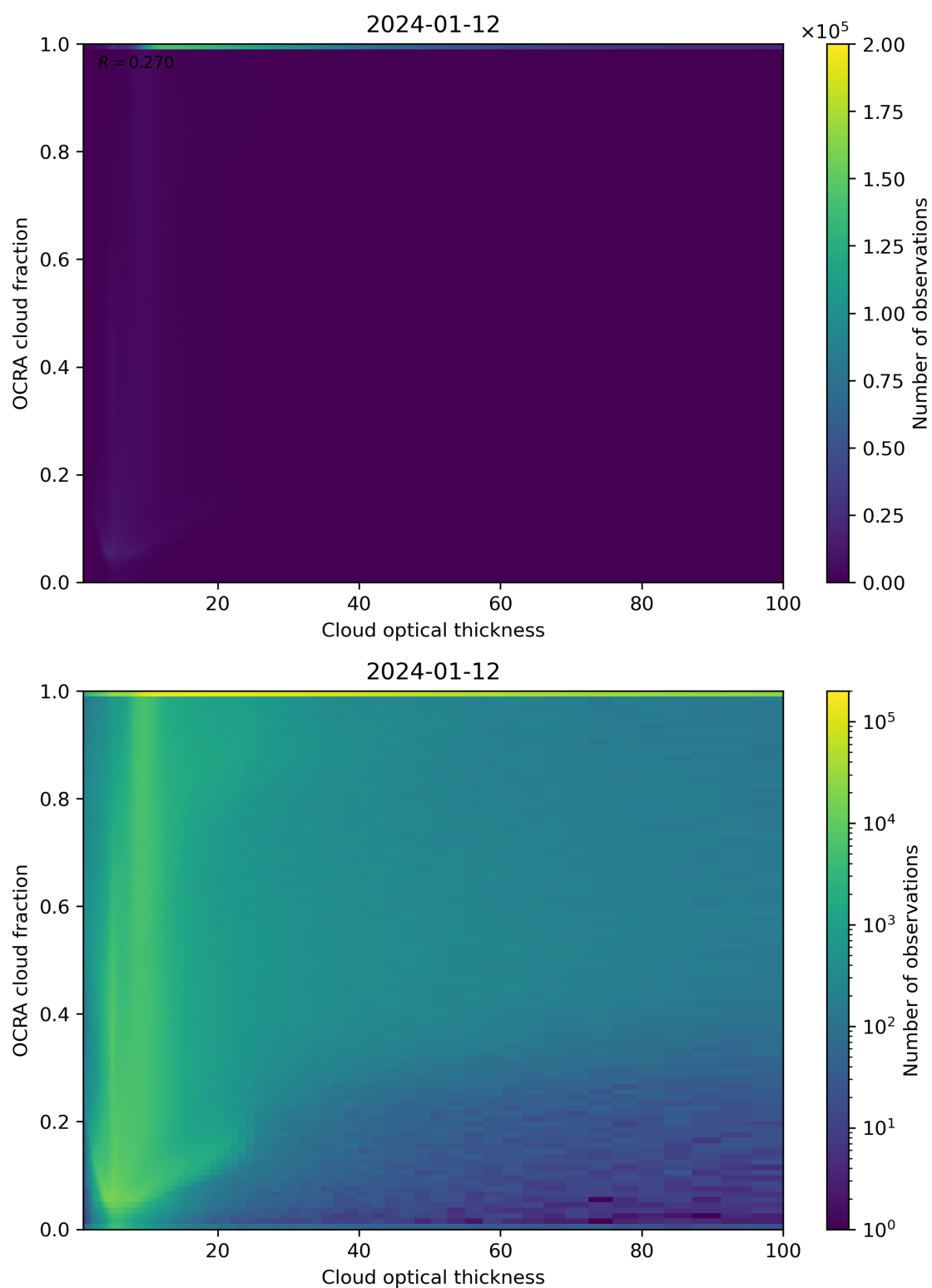
Figure 83: Scatter density plot of “Cloud optical thickness” against “OCRA cloud fraction” for 2024-01-11 to 2024-01-13.
