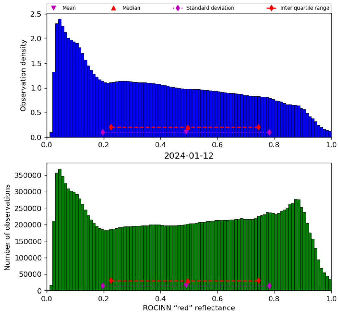
Figure 53: Histogram of “ROCINN “red” reflectance” for 2024-01-11 to 2024-01-13
