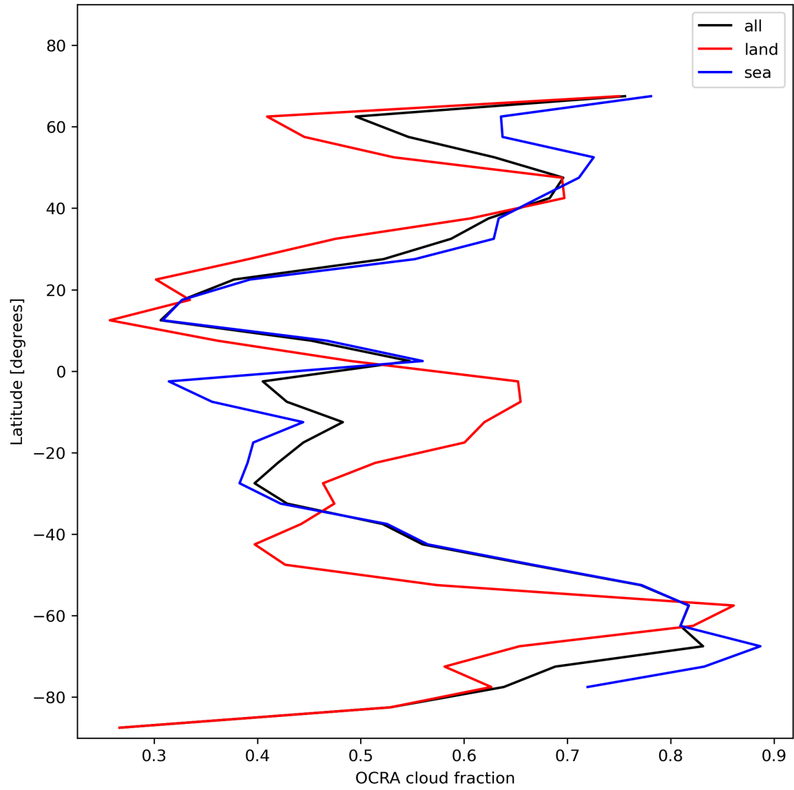
Figure 34: Zonal average of “OCRA cloud fraction” for 2024-01-11 to 2024-01-13.
