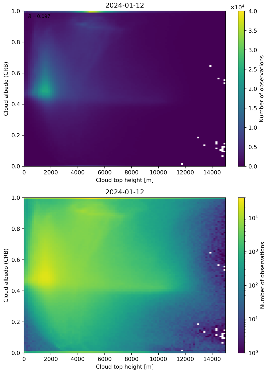
Figure 86: Scatter density plot of “Cloud top height” against “Cloud albedo (CRB)” for 2024-01-11 to 2024-01-13.
