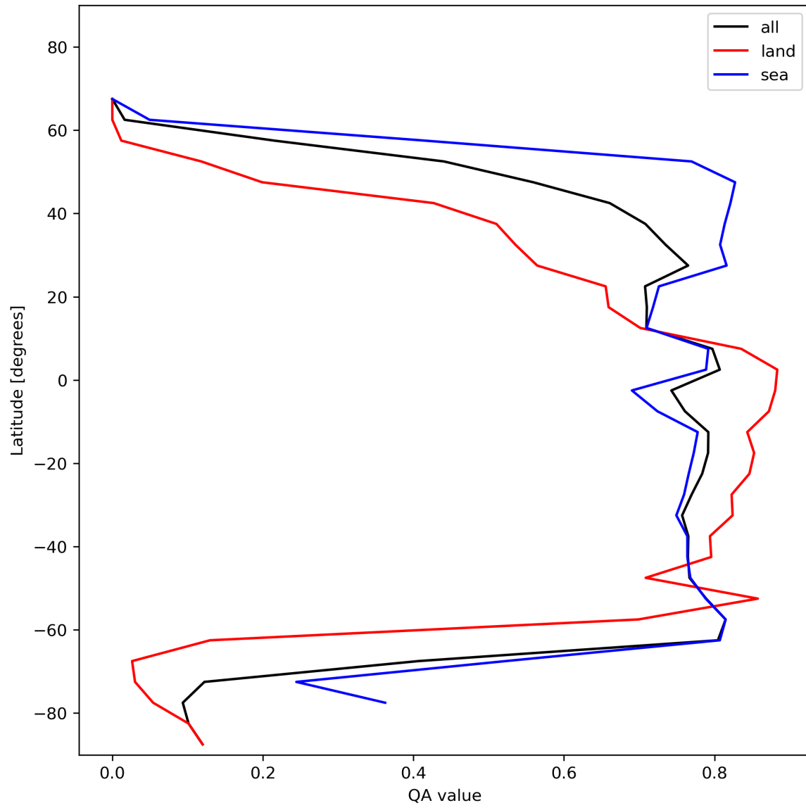
Figure 22: Zonal average of “QA value” for 2024-01-11 to 2024-01-13.
