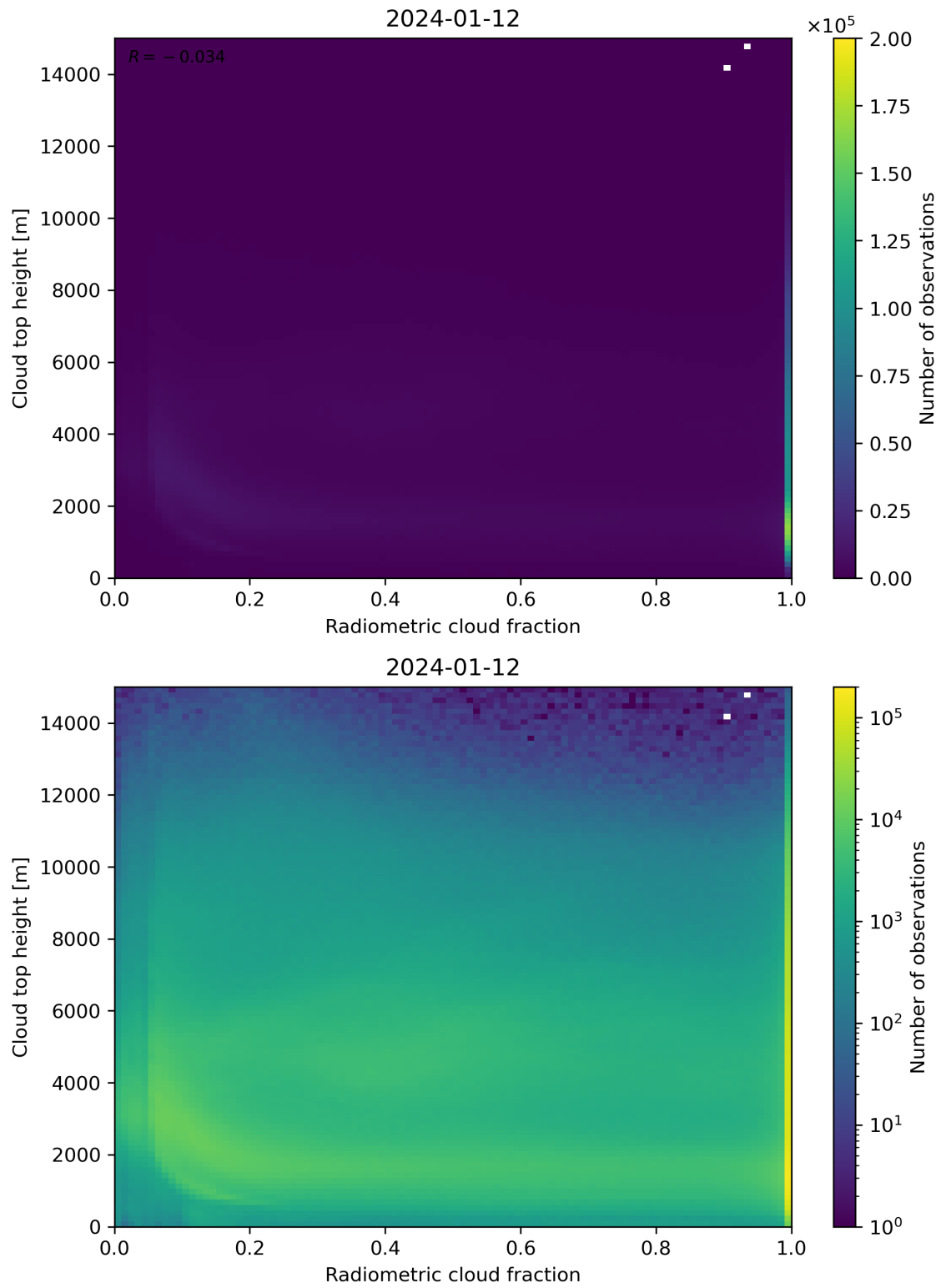
Figure 76: Scatter density plot of “Radiometric cloud fraction” against “Cloud top height” for 2024-01-11 to 2024-01-13.
