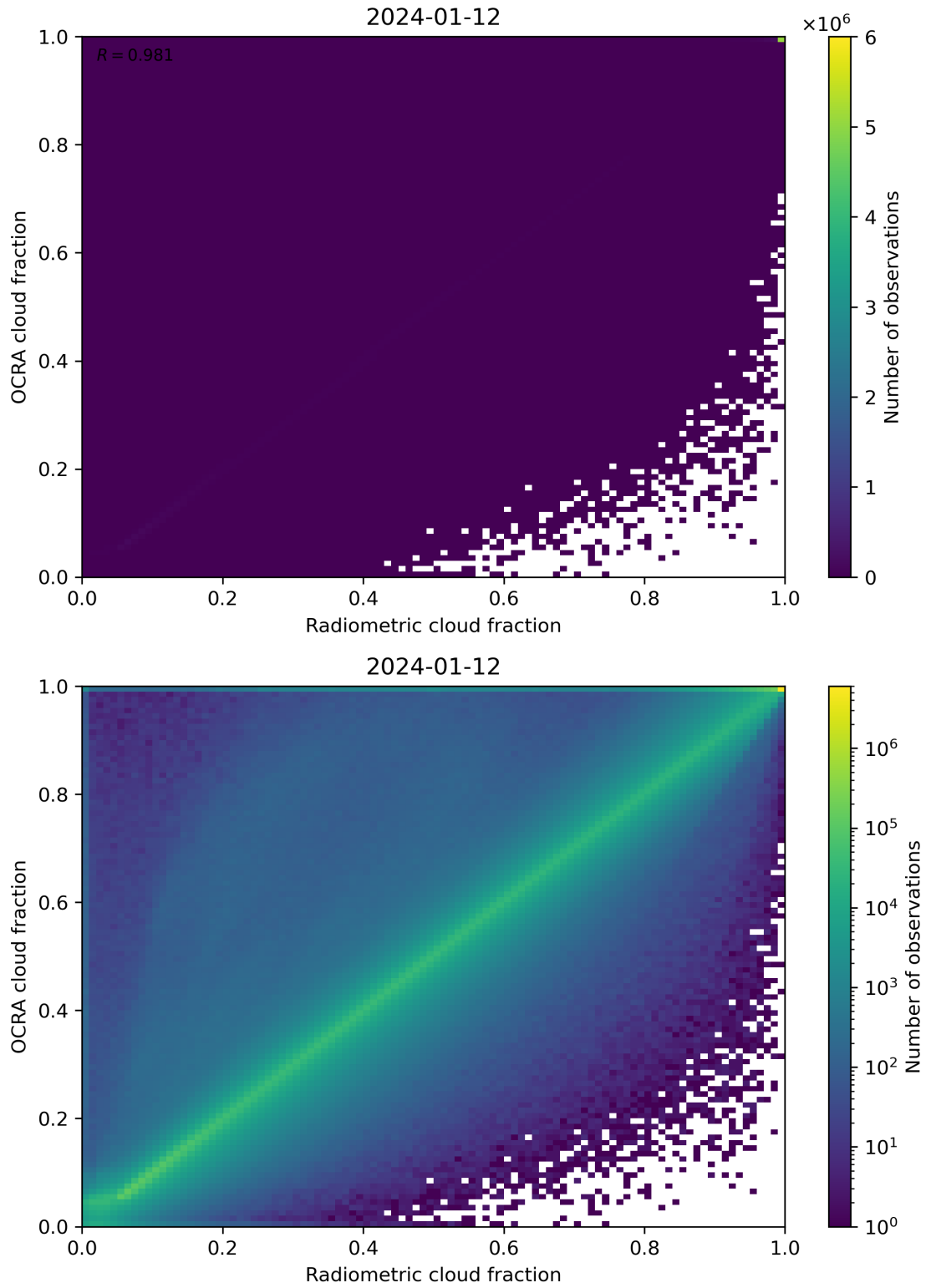
Figure 72: Scatter density plot of “Radiometric cloud fraction” against “OCRA cloud fraction” for 2024-01-11 to 2024-01-13.
