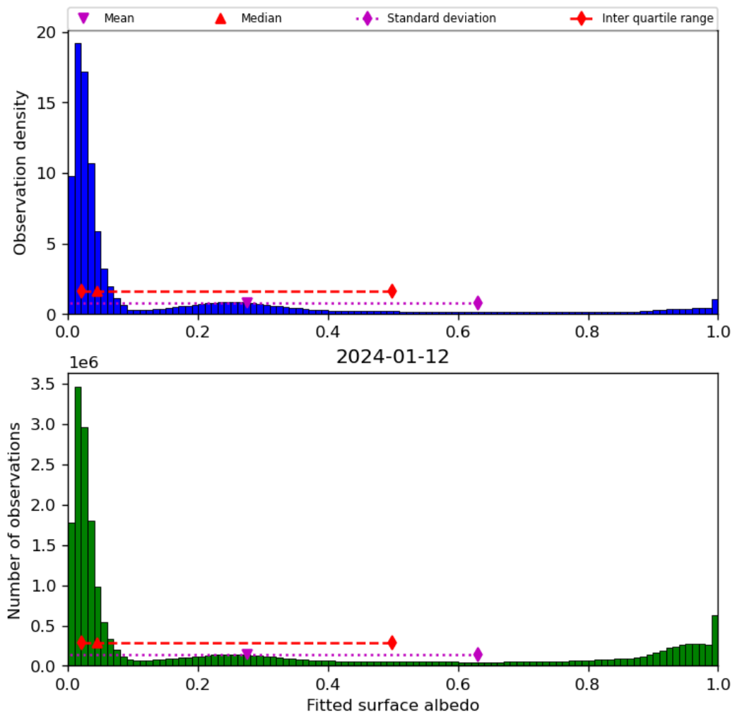
Figure 45: Histogram of “Fitted surface albedo” for 2024-01-11 to 2024-01-13
