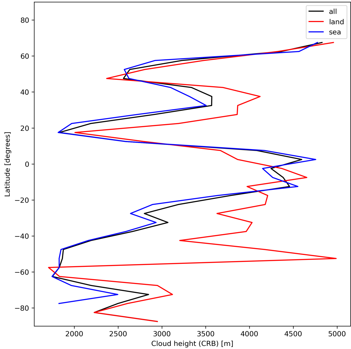
Figure 27: Zonal average of “Cloud height (CRB)” for 2024-01-11 to 2024-01-13.
