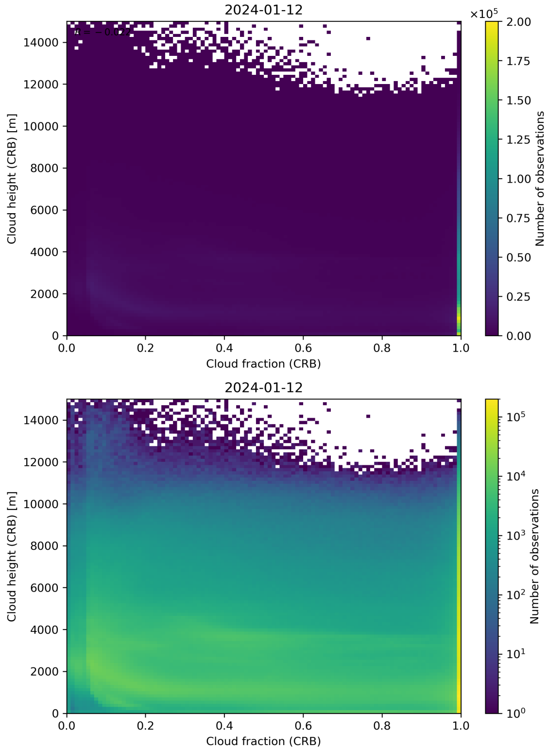
Figure 79: Scatter density plot of “Cloud fraction (CRB)” against “Cloud height (CRB)” for 2024-01-11 to 2024-01-13.
