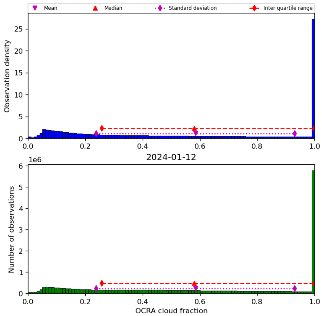
Figure 50: Histogram of “OCRA cloud fraction” for 2024-01-11 to 2024-01-13
