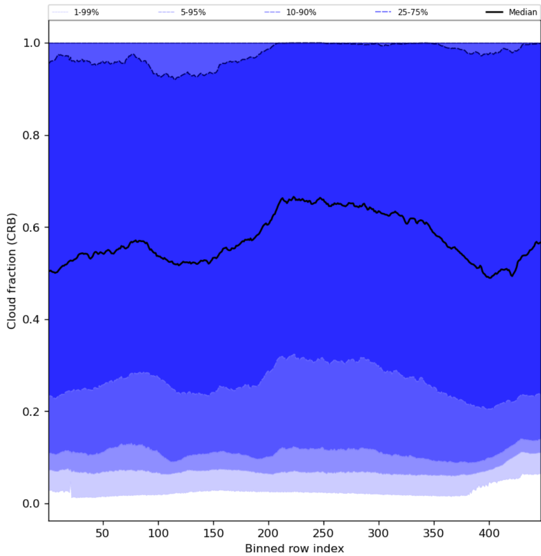
Figure 58: Along track statistics of “Cloud fraction (CRB)” for 2024-01-11 to 2024-01-13
