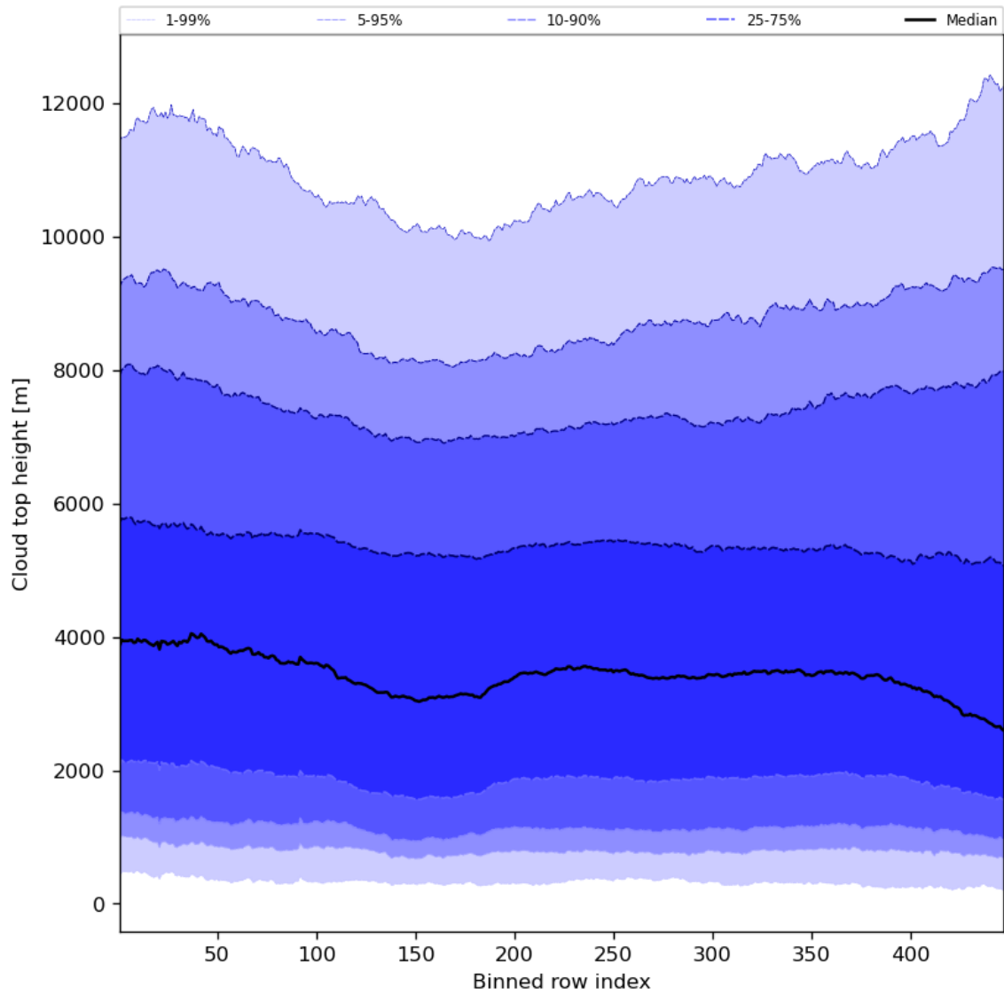
Figure 56: Along track statistics of “Cloud top height” for 2024-01-11 to 2024-01-13
