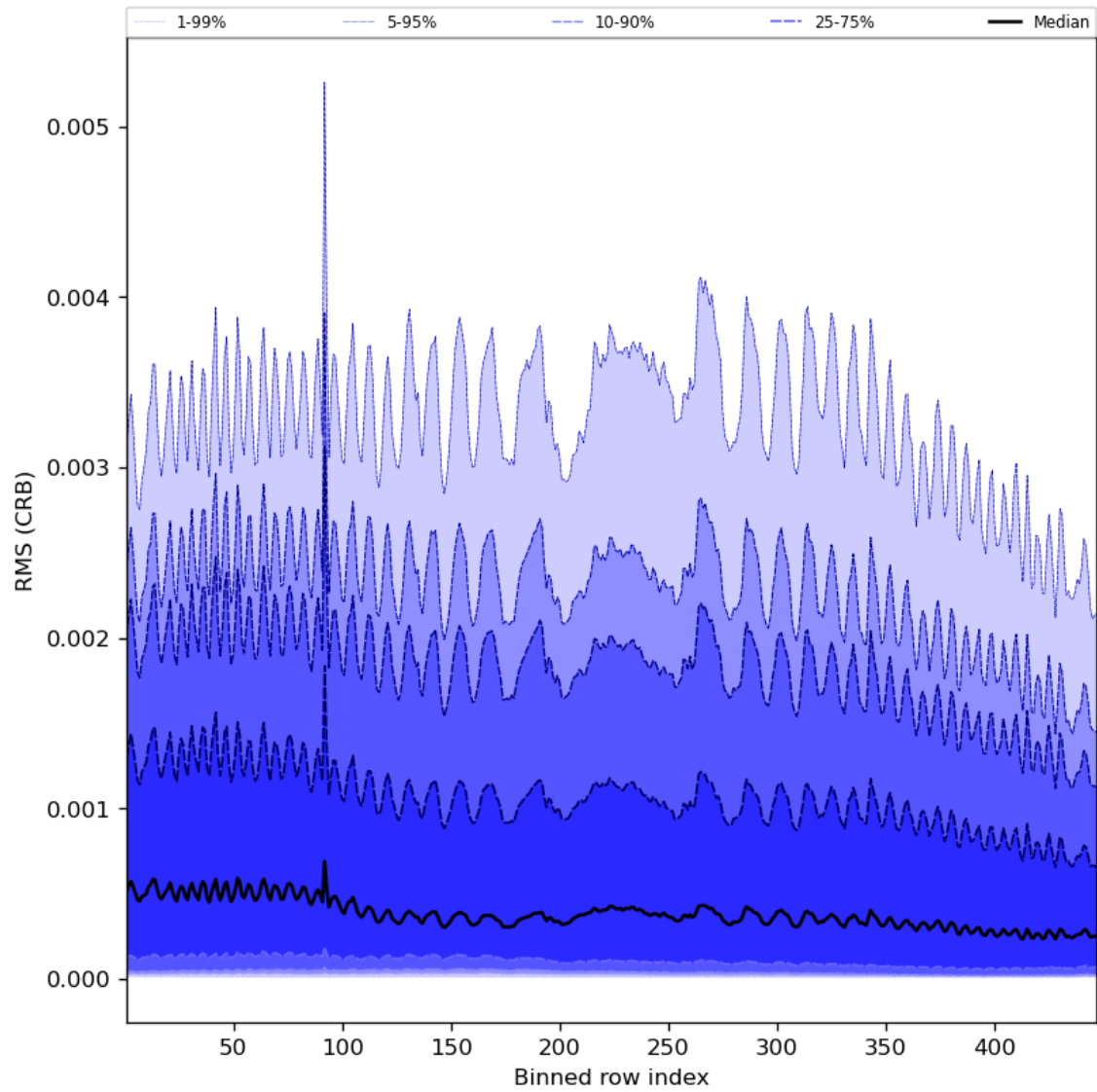
Figure 64: Along track statistics of “RMS (CRB)” for 2024-01-11 to 2024-01-13
