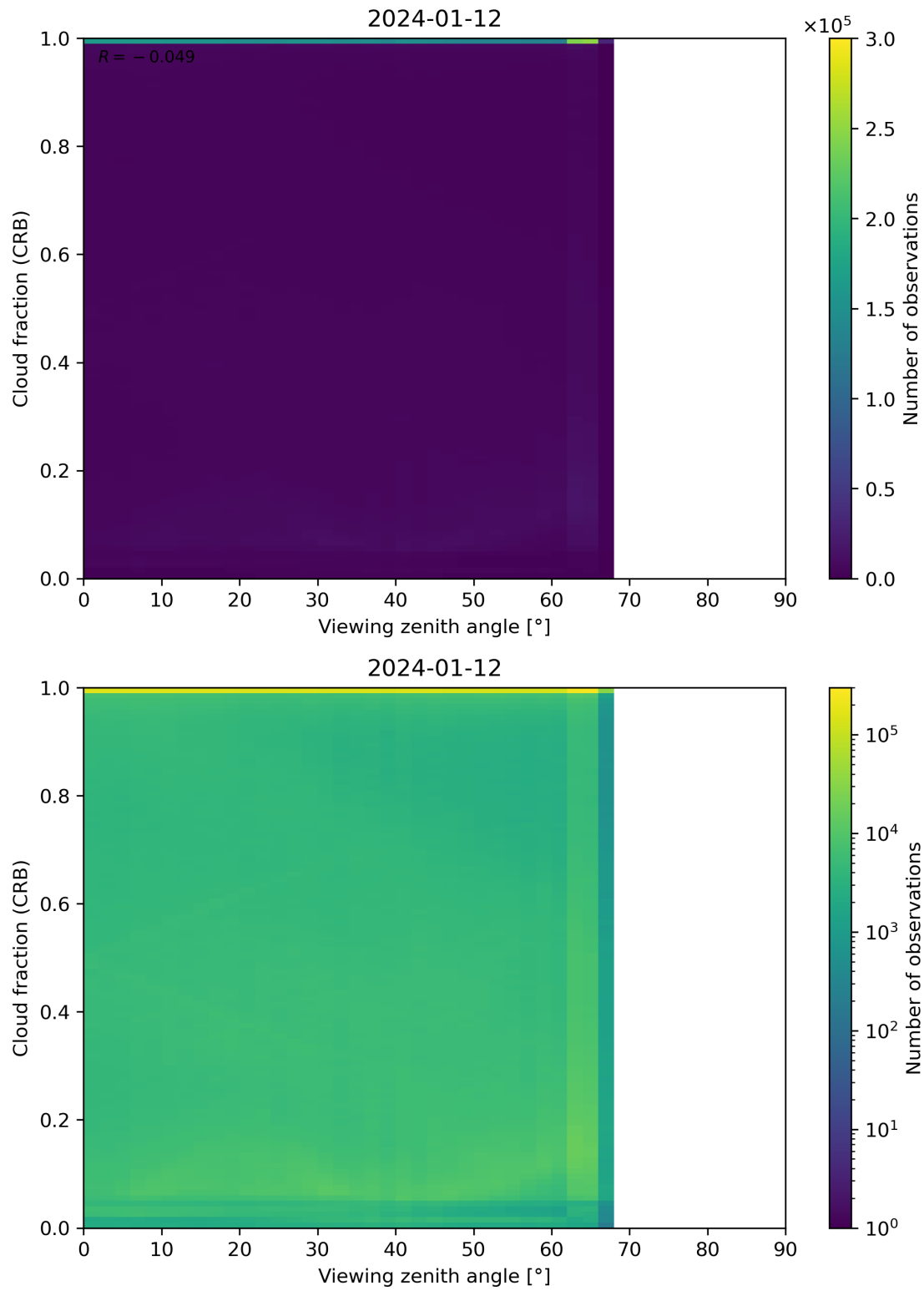
Figure 109: Scatter density plot of “Viewing zenith angle” against “Cloud fraction (CRB)” for 2024-01-11 to 2024-01-13.
