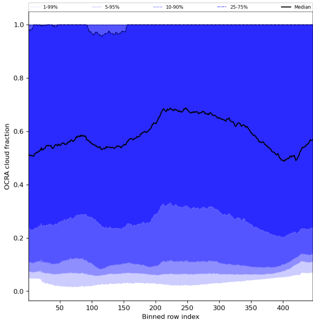
Figure 66: Along track statistics of “OCRA cloud fraction” for 2024-01-11 to 2024-01-13
