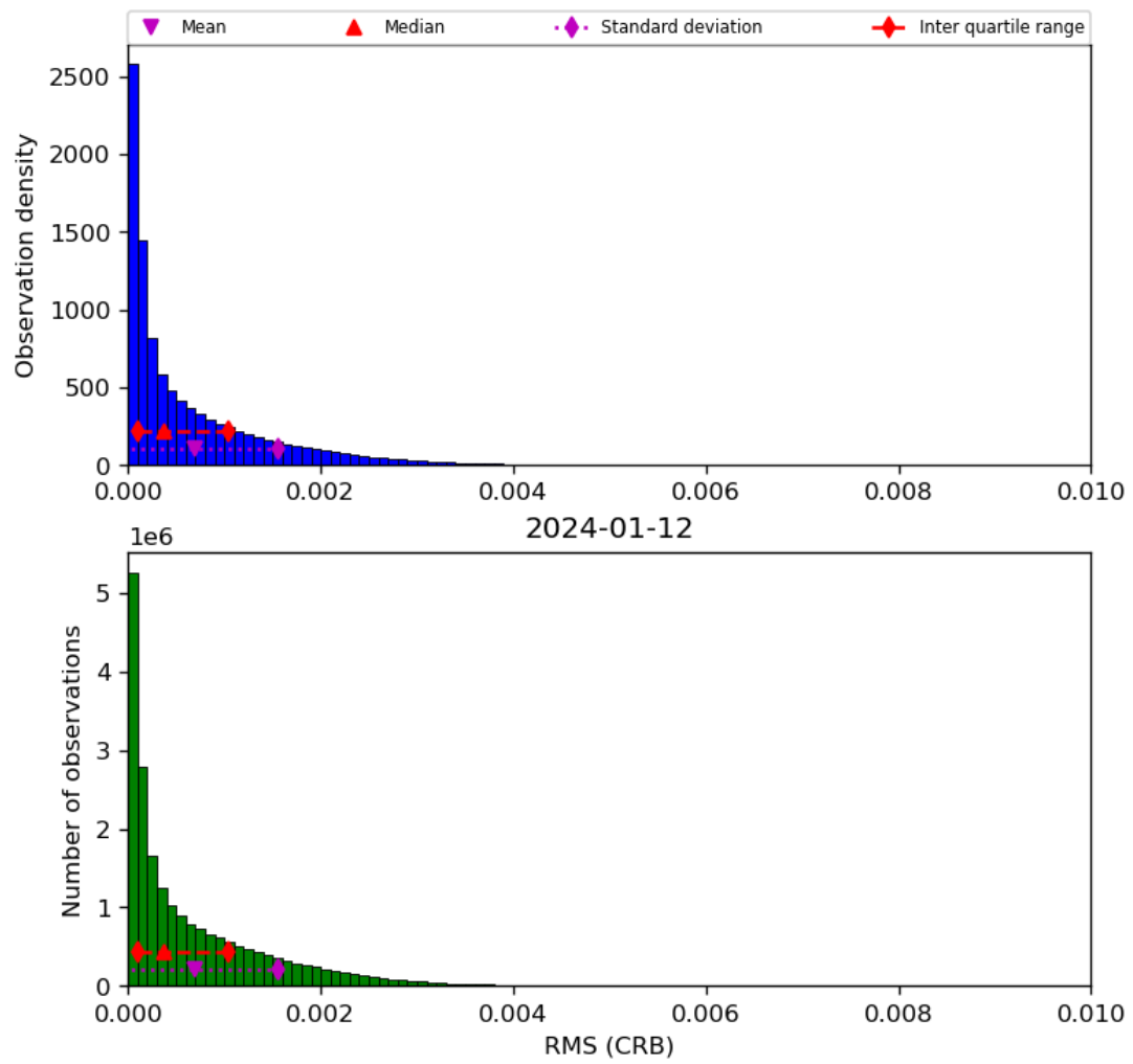
Figure 48: Histogram of “RMS (CRB)” for 2024-01-11 to 2024-01-13
