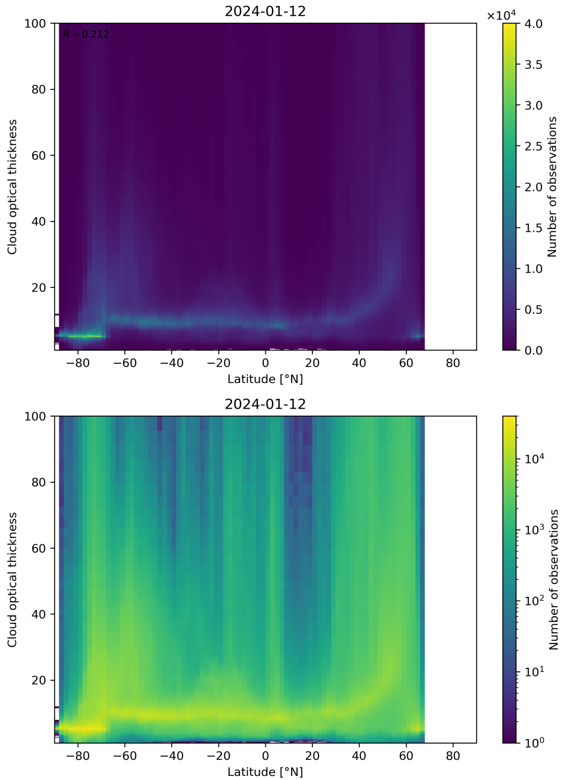
Figure 96: Scatter density plot of “Latitude” against “Cloud optical thickness” for 2024-01-11 to 2024-01-13.
