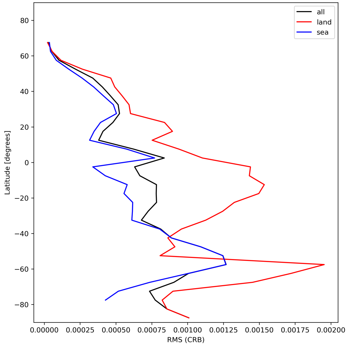
Figure 32: Zonal average of “RMS (CRB)” for 2024-01-11 to 2024-01-13.
