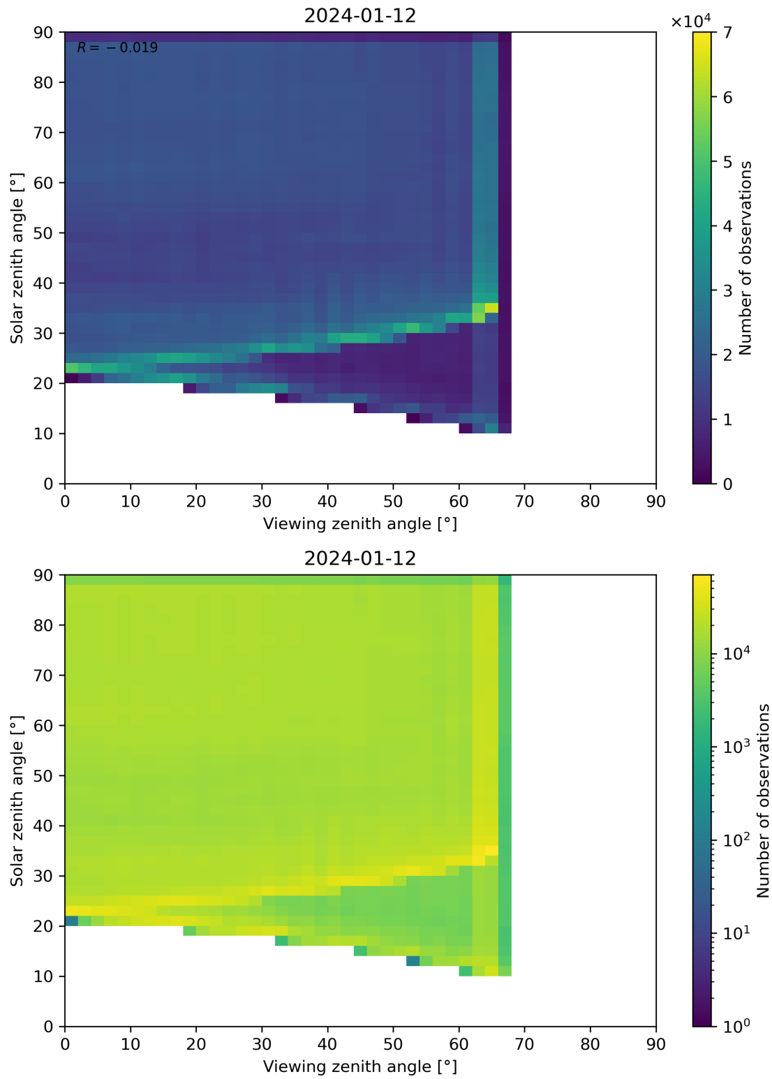
Figure 114: Scatter density plot of “Viewing zenith angle” against “Solar zenith angle” for 2024-01-11 to 2024-01-13.
