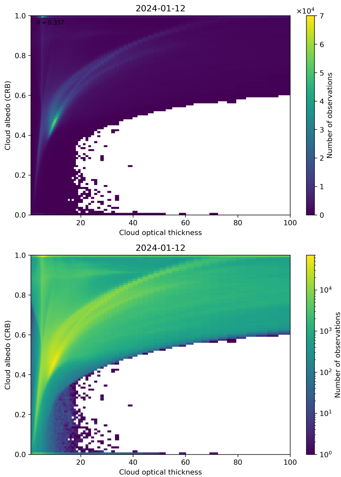
Figure 82: Scatter density plot of “Cloud optical thickness” against “Cloud albedo (CRB)” for 2024-01-11 to 2024-01-13.
