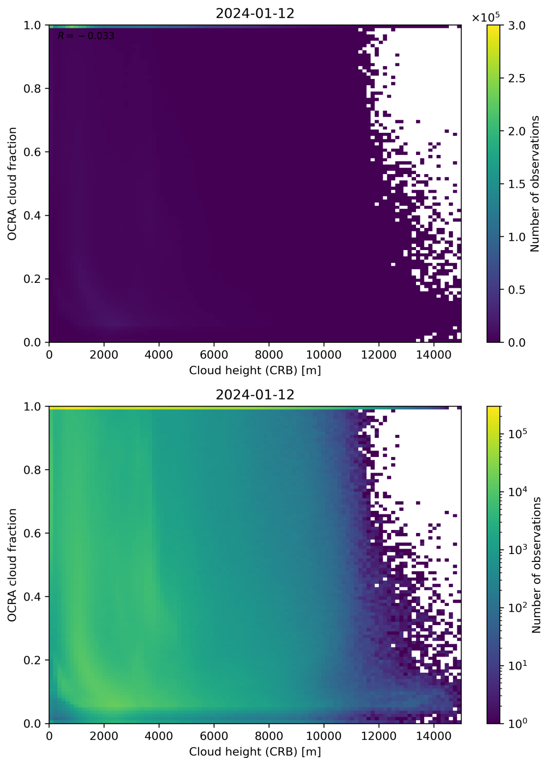
Figure 81: Scatter density plot of “Cloud height (CRB)” against “OCRA cloud fraction” for 2024-01-11 to 2024-01-13.
