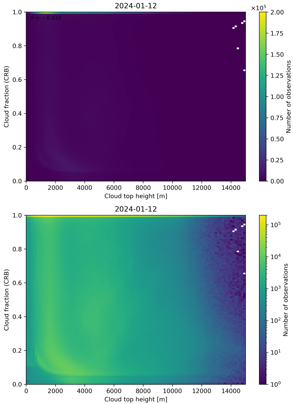
Figure 88: Scatter density plot of “Cloud top height” against “Cloud fraction (CRB)” for 2024-01-11 to 2024-01-13.
