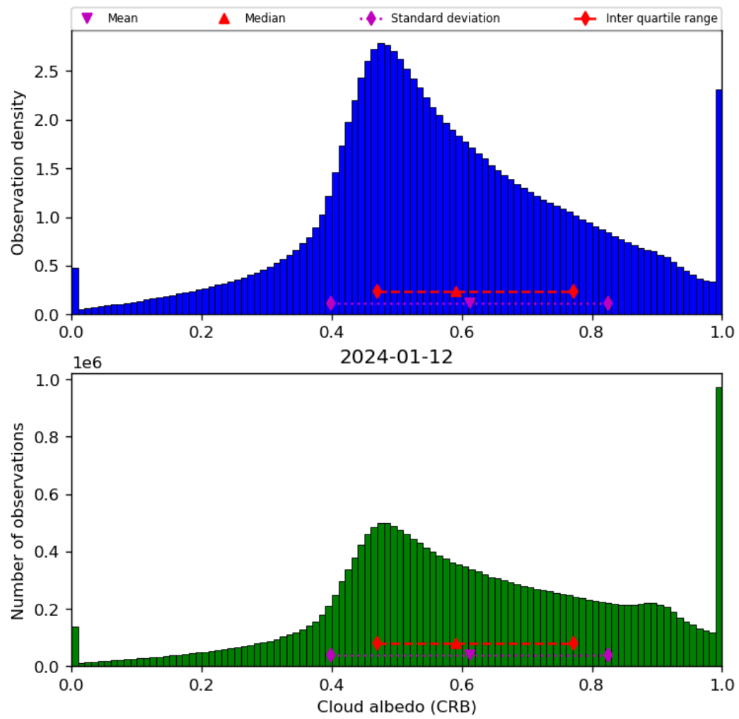
Figure 44: Histogram of “Cloud albedo (CRB)” for 2024-01-11 to 2024-01-13
