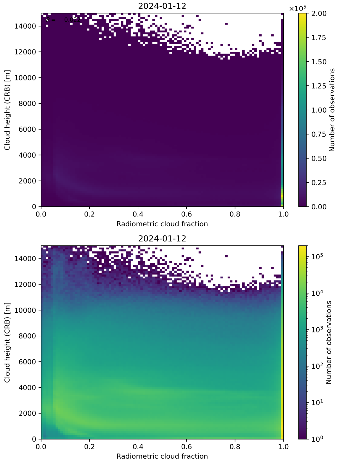
Figure 74: Scatter density plot of “Radiometric cloud fraction” against “Cloud height (CRB)” for 2024-01-11 to 2024-01-13.
