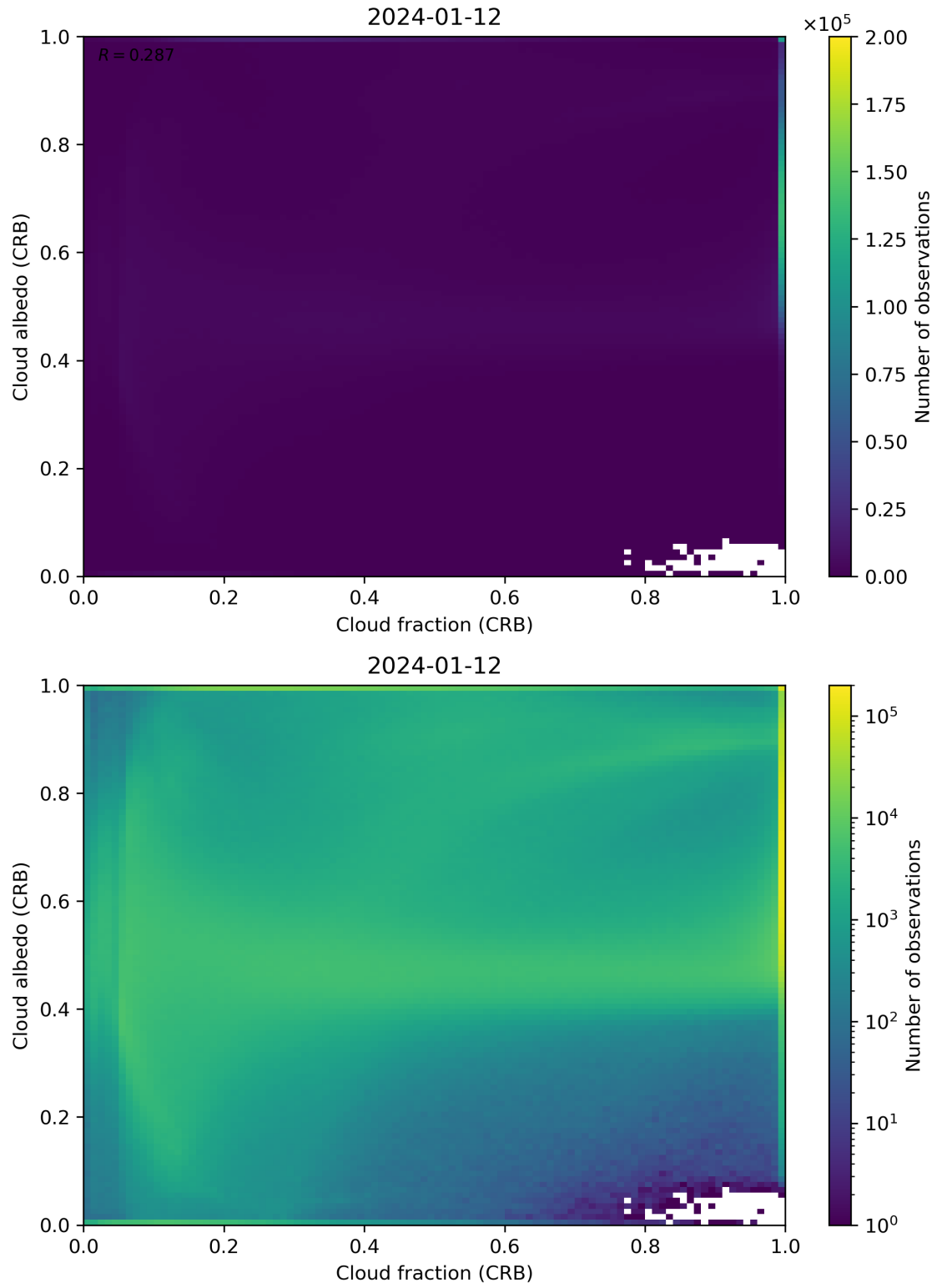
Figure 77: Scatter density plot of “Cloud fraction (CRB)” against “Cloud albedo (CRB)” for 2024-01-11 to 2024-01-13.
