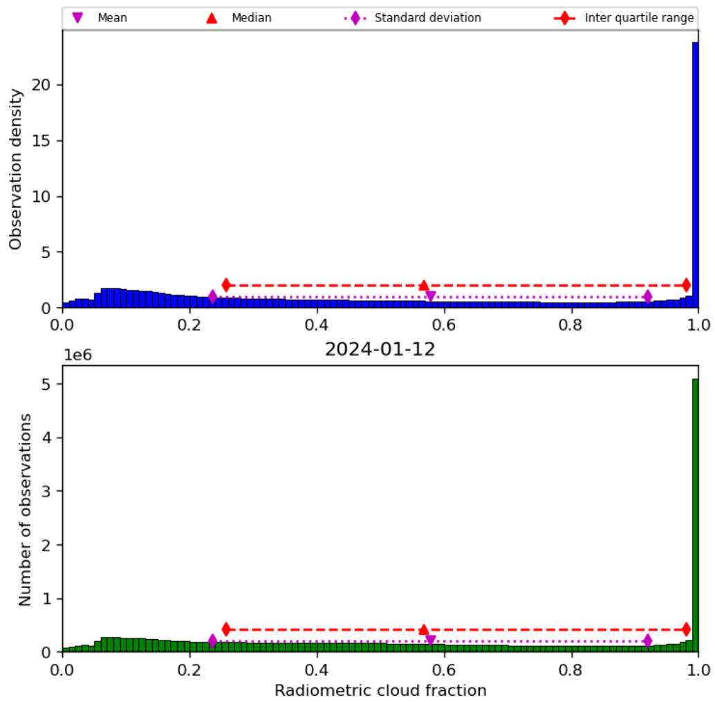
Figure 39: Histogram of “Radiometric cloud fraction” for 2024-01-11 to 2024-01-13
