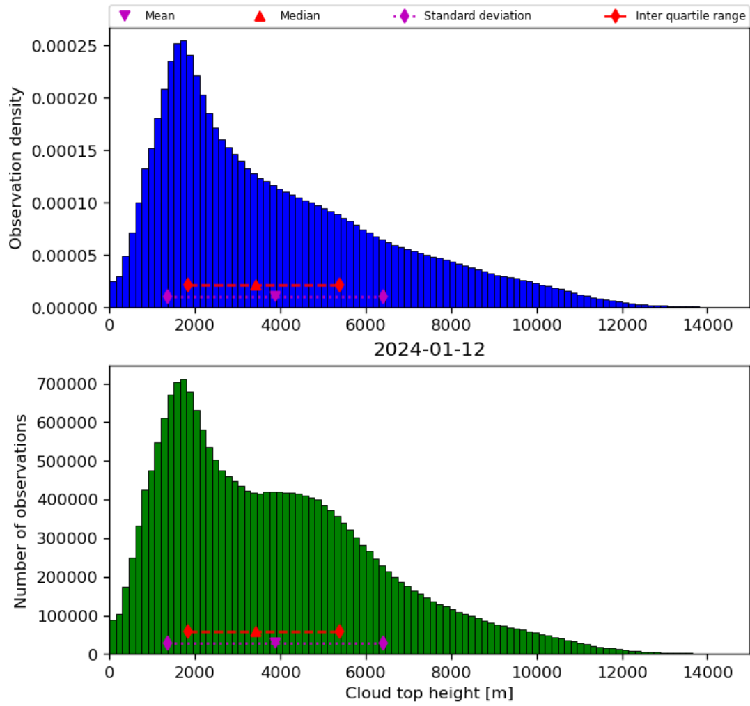
Figure 40: Histogram of “Cloud top height” for 2024-01-11 to 2024-01-13
