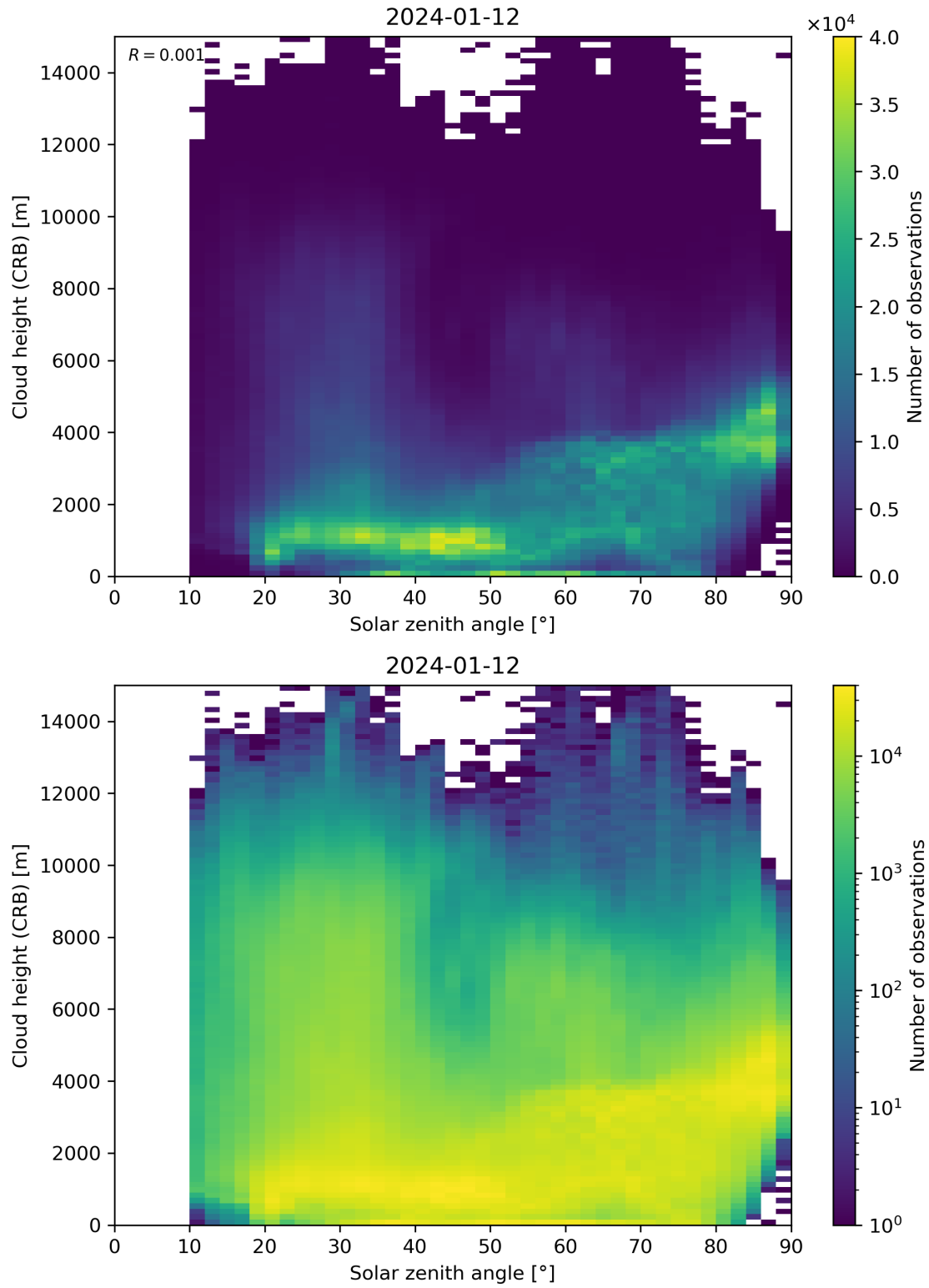
Figure 102: Scatter density plot of “Solar zenith angle” against “Cloud height (CRB)” for 2024-01-11 to 2024-01-13.
