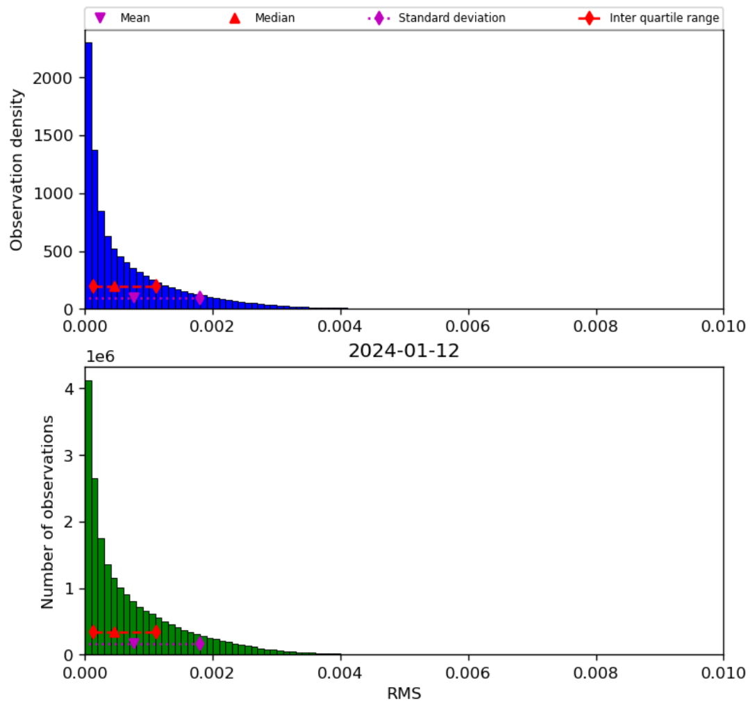
Figure 47: Histogram of “RMS” for 2024-01-11 to 2024-01-13
