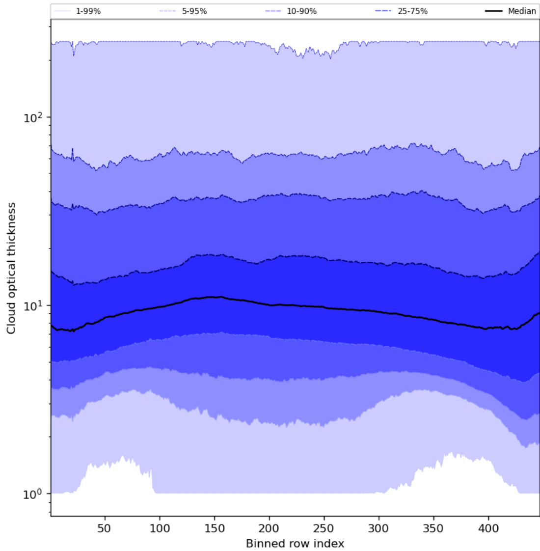
Figure 57: Along track statistics of “Cloud optical thickness” for 2024-01-11 to 2024-01-13
