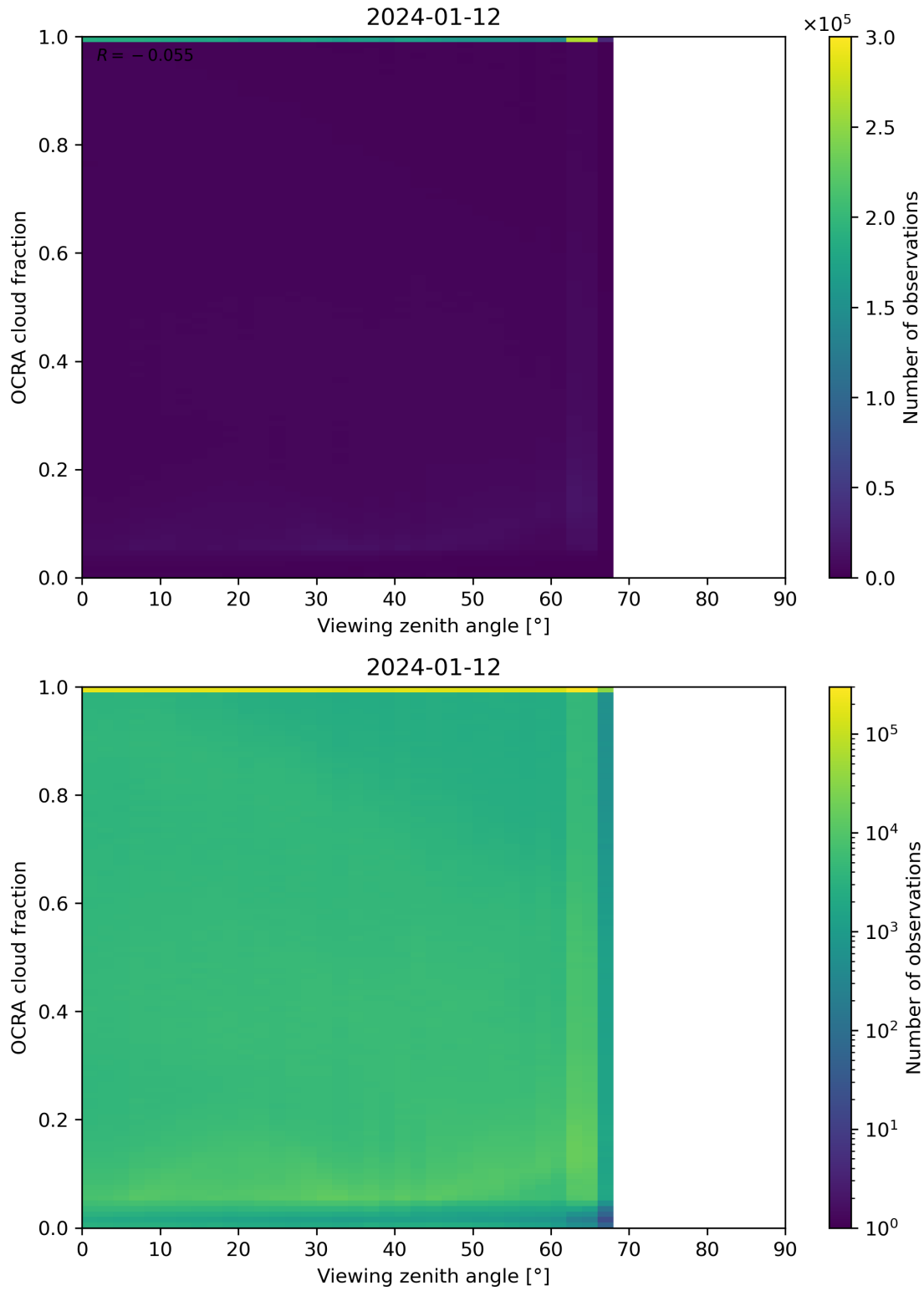
Figure 108: Scatter density plot of “Viewing zenith angle” against “OCRA cloud fraction” for 2024-01-11 to 2024-01-13.
