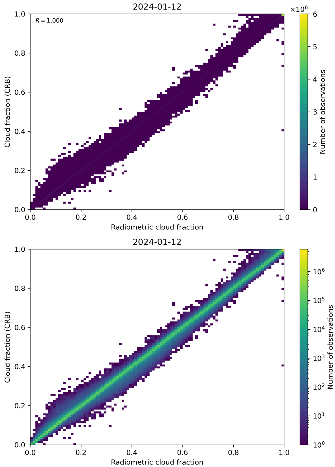
Figure 73: Scatter density plot of “Radiometric cloud fraction” against “Cloud fraction (CRB)” for 2024-01-11 to 2024-01-13.
