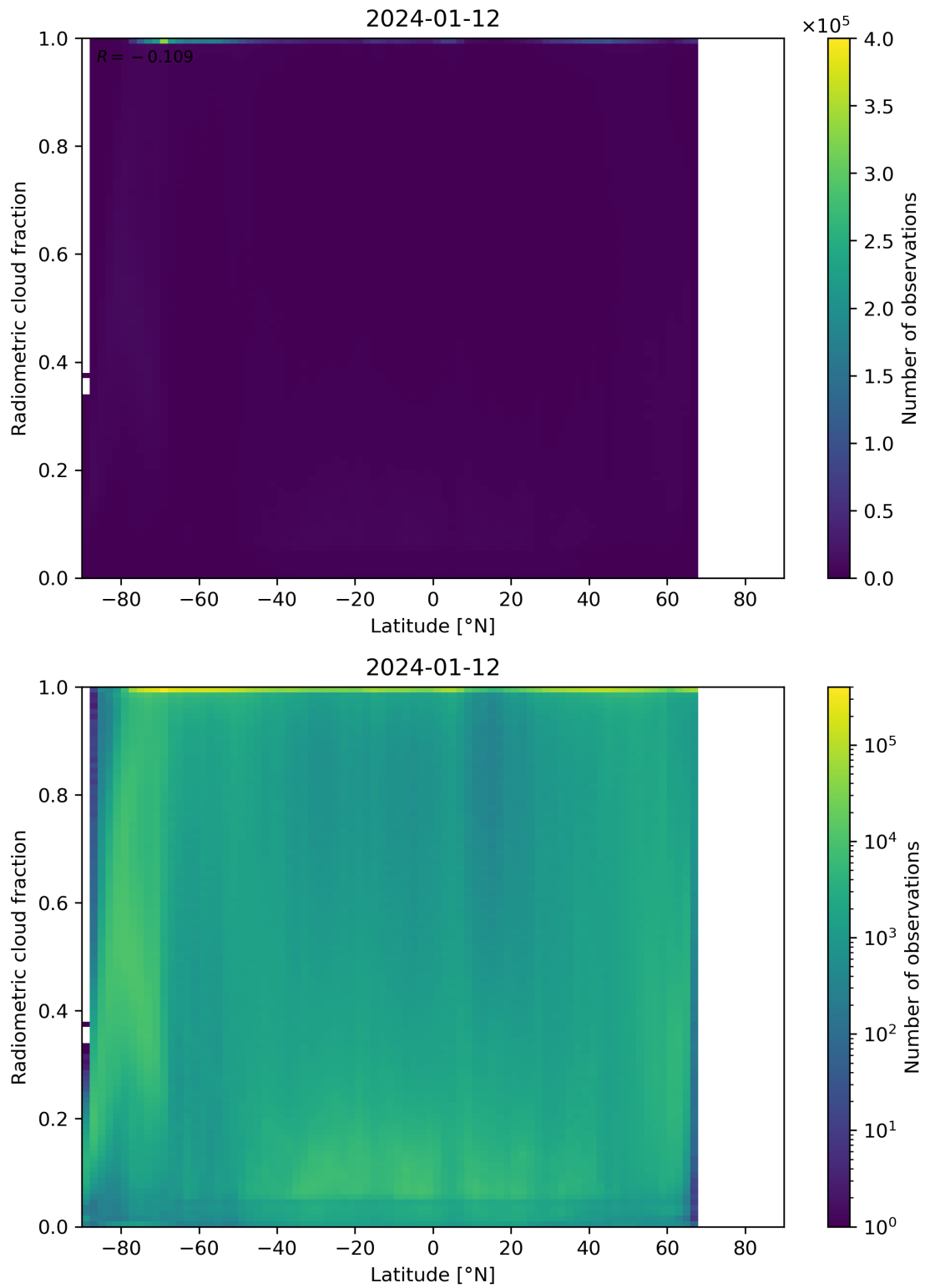
Figure 92: Scatter density plot of “Latitude” against “Radiometric cloud fraction” for 2024-01-11 to 2024-01-13.
