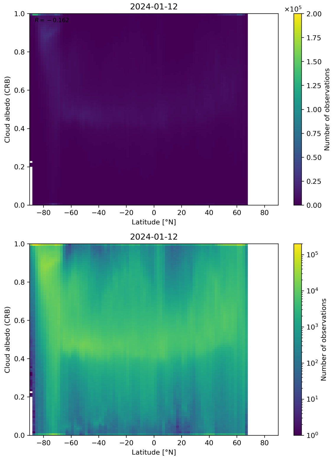
Figure 91: Scatter density plot of “Latitude” against “Cloud albedo (CRB)” for 2024-01-11 to 2024-01-13.
