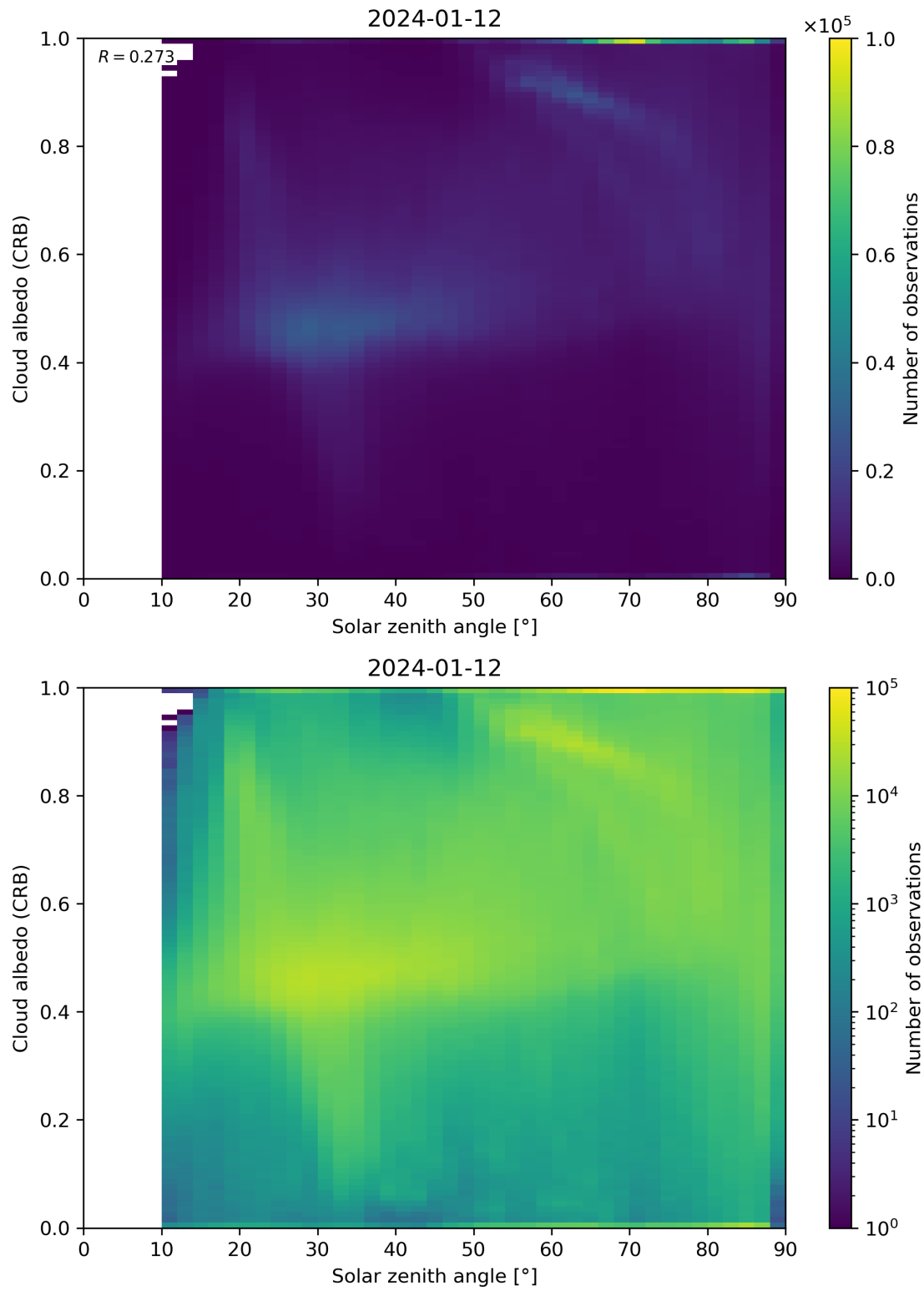
Figure 98: Scatter density plot of “Solar zenith angle” against “Cloud albedo (CRB)” for 2024-01-11 to 2024-01-13.
