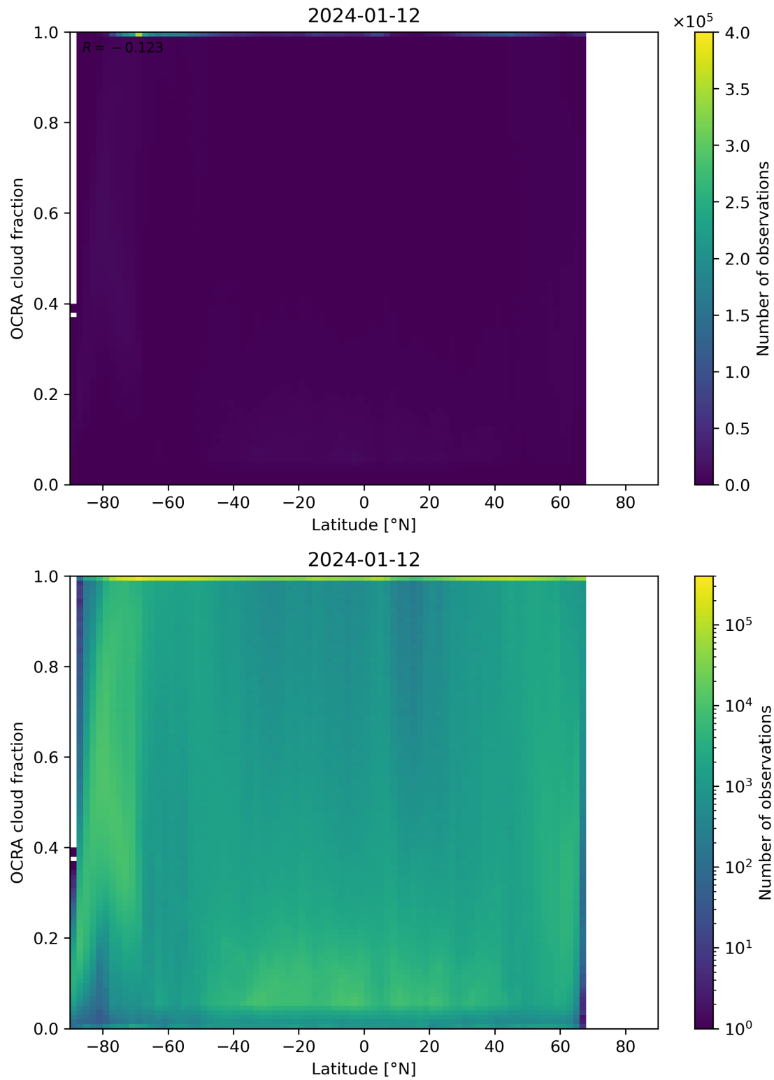
Figure 93: Scatter density plot of “Latitude” against “OCRA cloud fraction” for 2024-01-11 to 2024-01-13.
