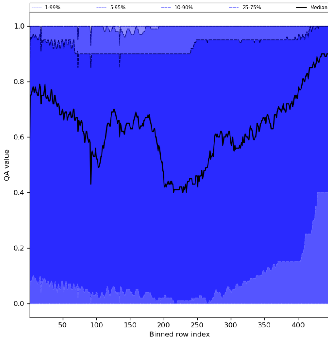
Figure 54: Along track statistics of “QA value” for 2024-01-11 to 2024-01-13
