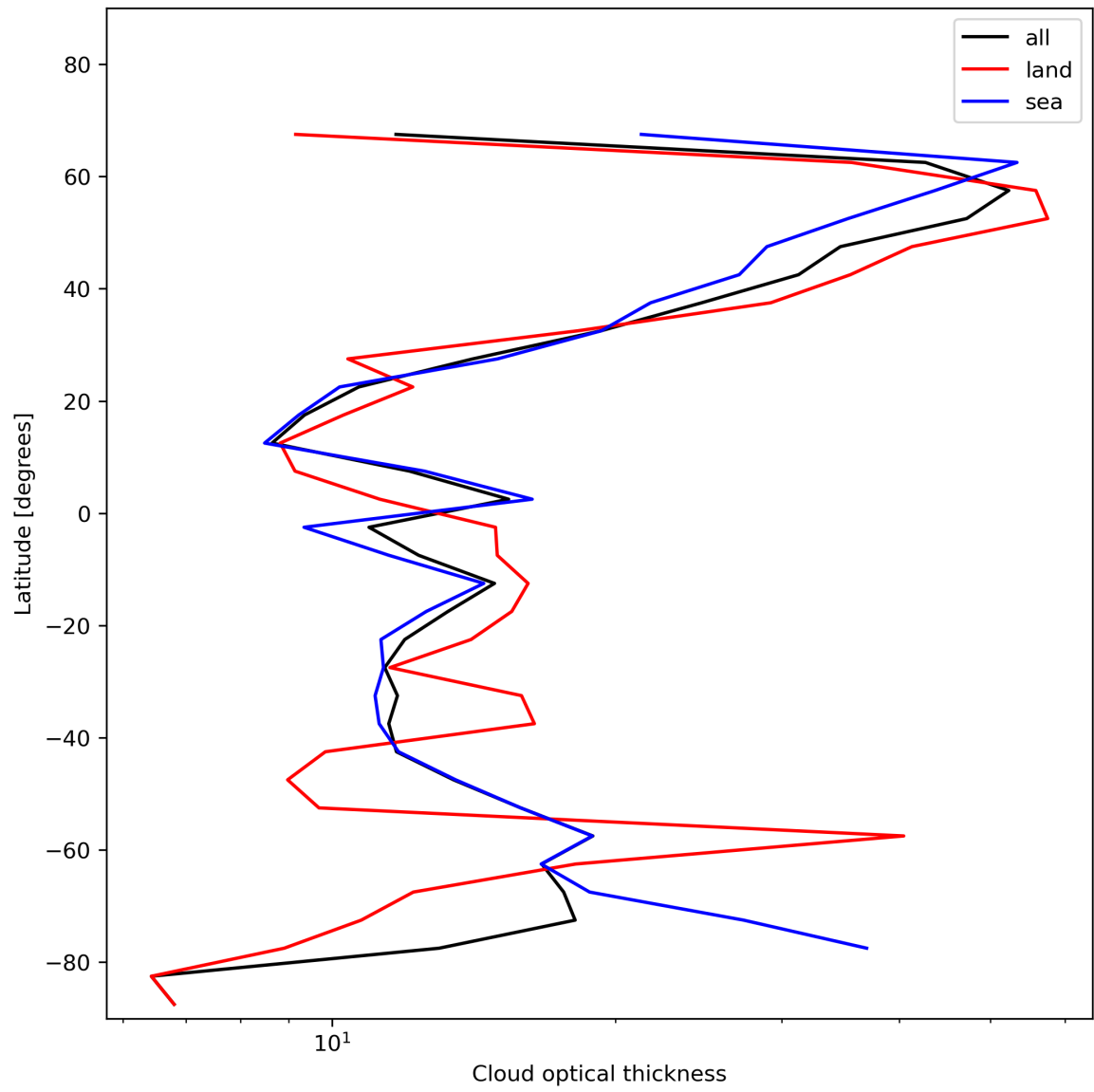
Figure 25: Zonal average of “Cloud optical thickness” for 2024-01-11 to 2024-01-13.
