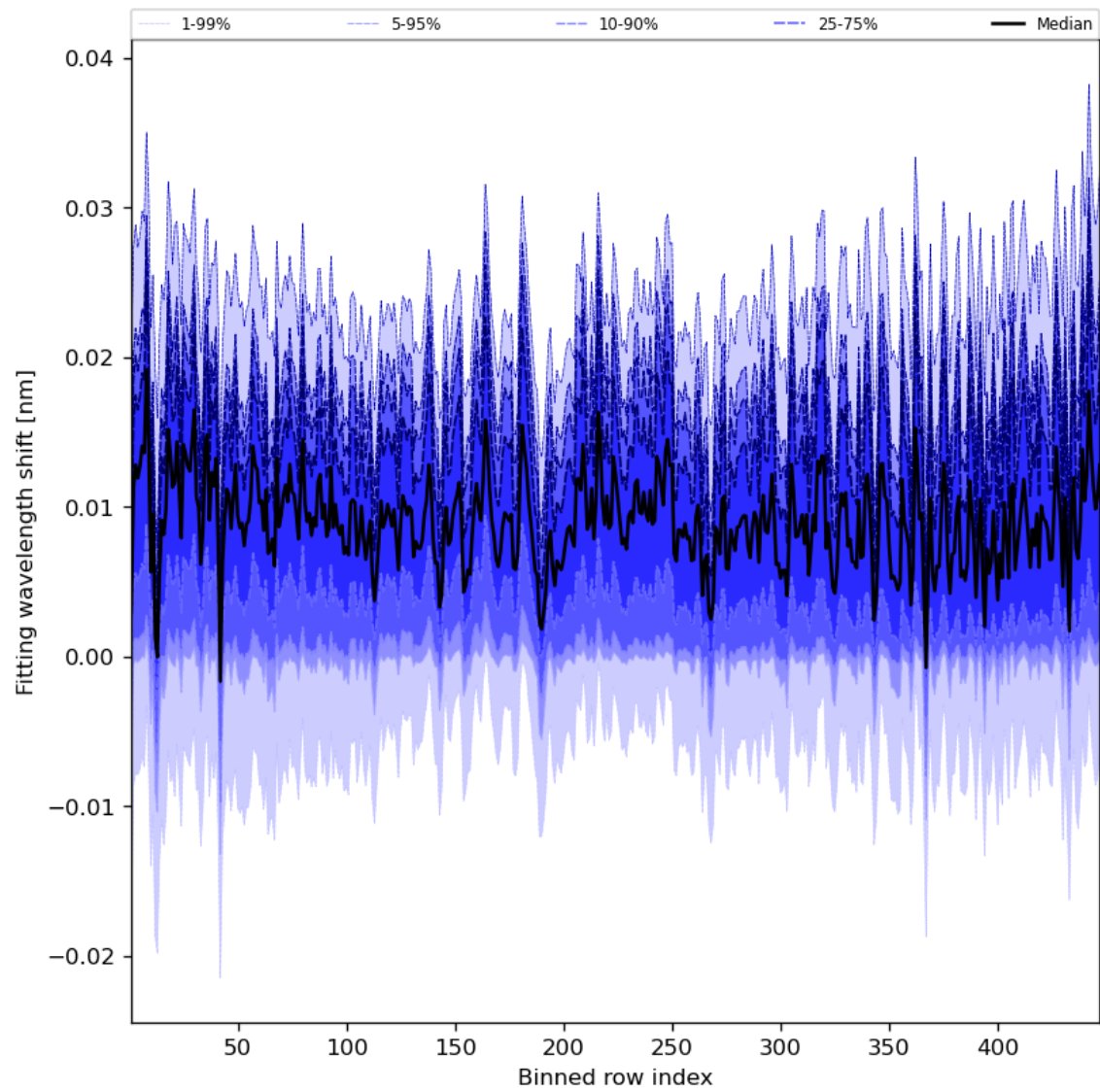
Figure 65: Along track statistics of “Fitting wavelength shift” for 2024-01-11 to 2024-01-13
