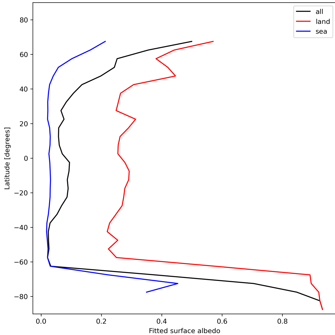
Figure 29: Zonal average of “Fitted surface albedo” for 2024-01-11 to 2024-01-13.
