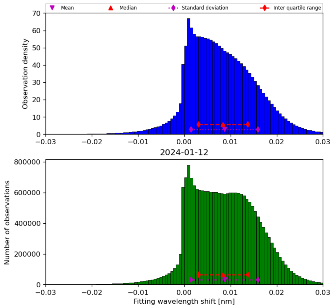
Figure 49: Histogram of “Fitting wavelength shift” for 2024-01-11 to 2024-01-13
