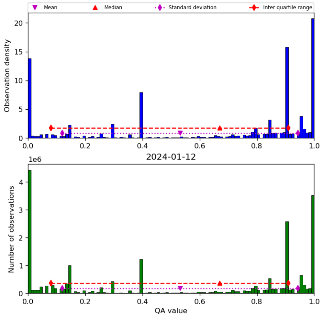
Figure 38: Histogram of “QA value” for 2024-01-11 to 2024-01-13
