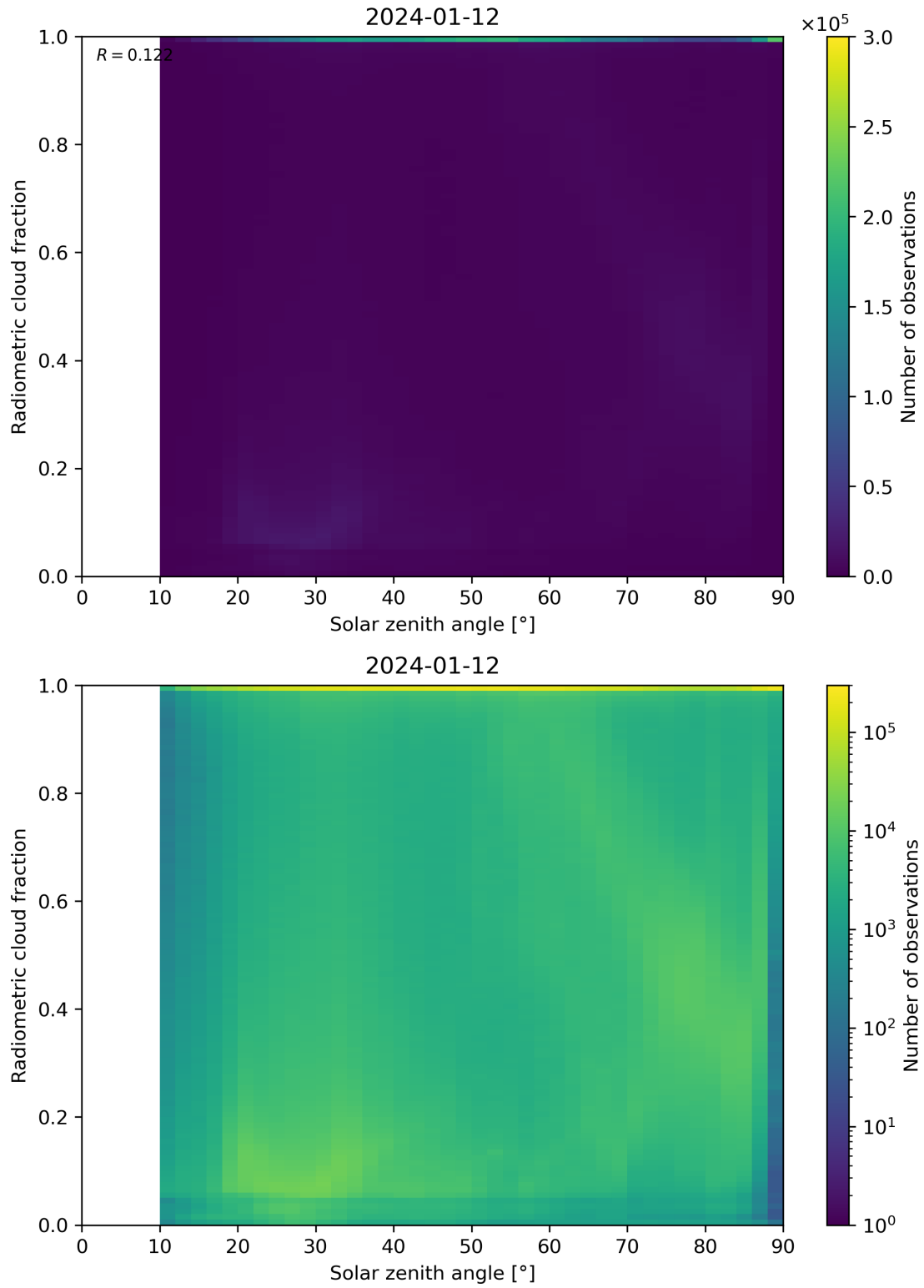
Figure 99: Scatter density plot of “Solar zenith angle” against “Radiometric cloud fraction” for 2024-01-11 to 2024-01-13.
