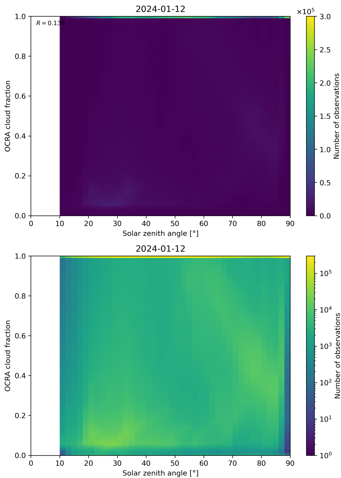
Figure 100: Scatter density plot of “Solar zenith angle” against “OCRA cloud fraction” for 2024-01-11 to 2024-01-13.
