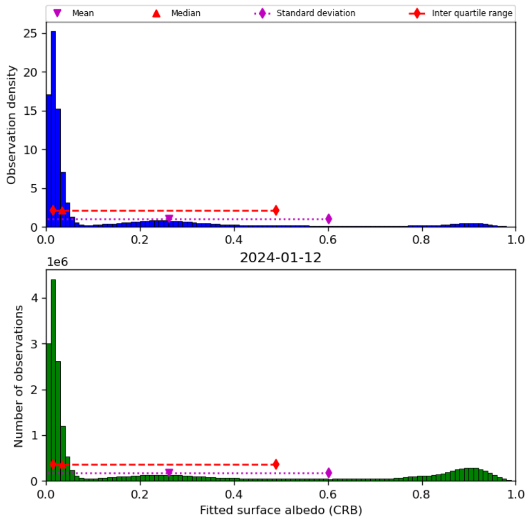
Figure 46: Histogram of “Fitted surface albedo (CRB)” for 2024-01-11 to 2024-01-13
