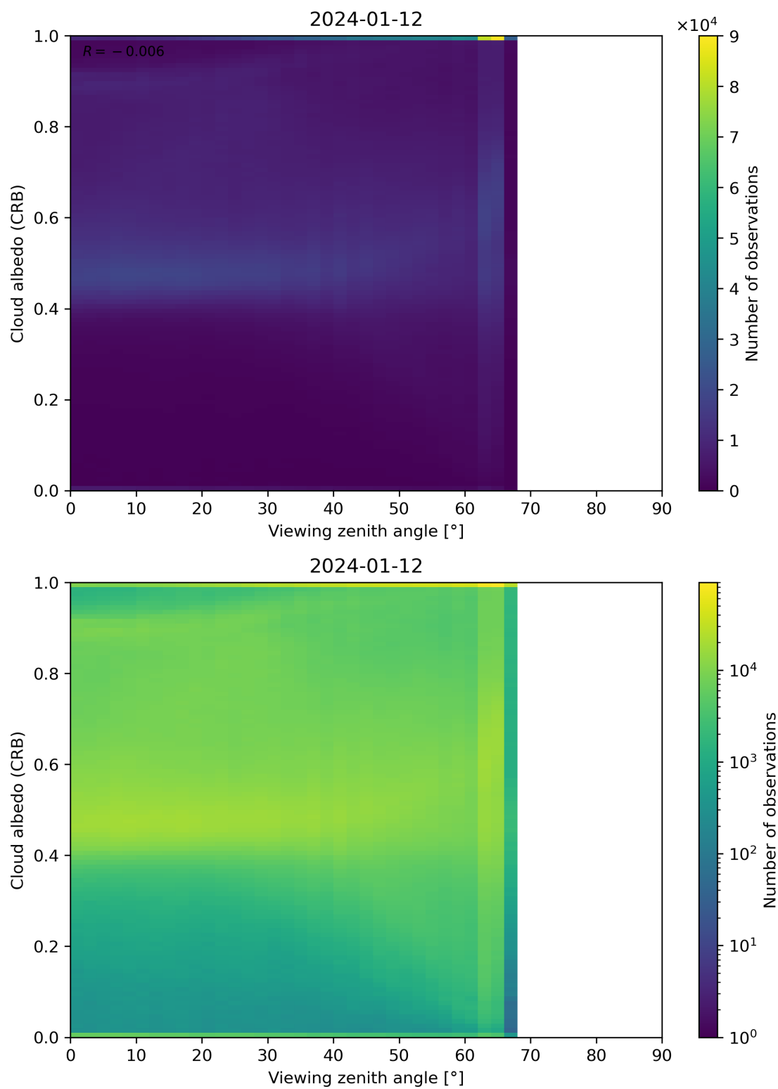
Figure 106: Scatter density plot of “Viewing zenith angle” against “Cloud albedo (CRB)” for 2024-01-11 to 2024-01-13.
