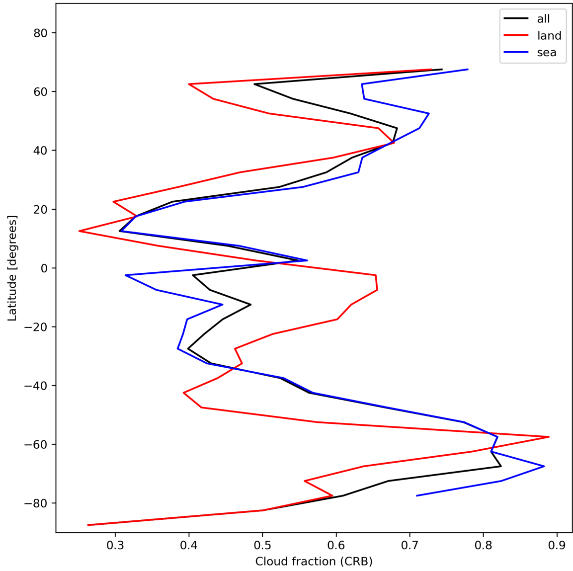
Figure 26: Zonal average of “Cloud fraction (CRB)” for 2024-01-11 to 2024-01-13.
