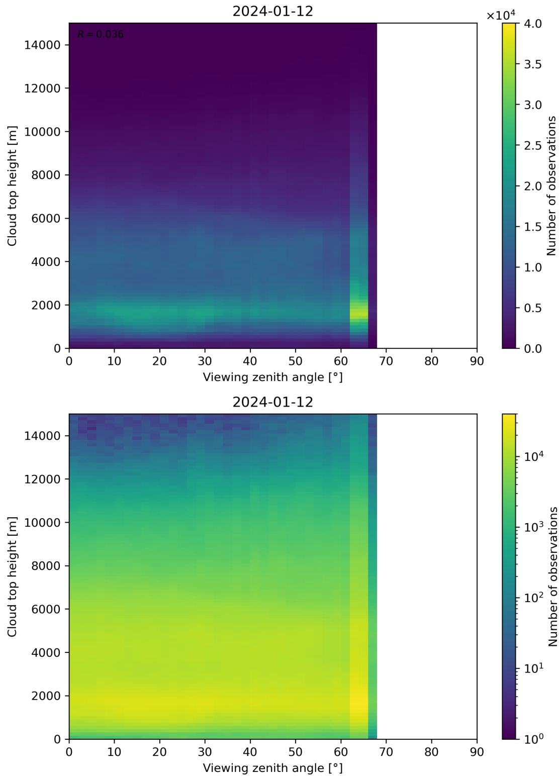
Figure 112: Scatter density plot of “Viewing zenith angle” against “Cloud top height” for 2024-01-11 to 2024-01-13.
