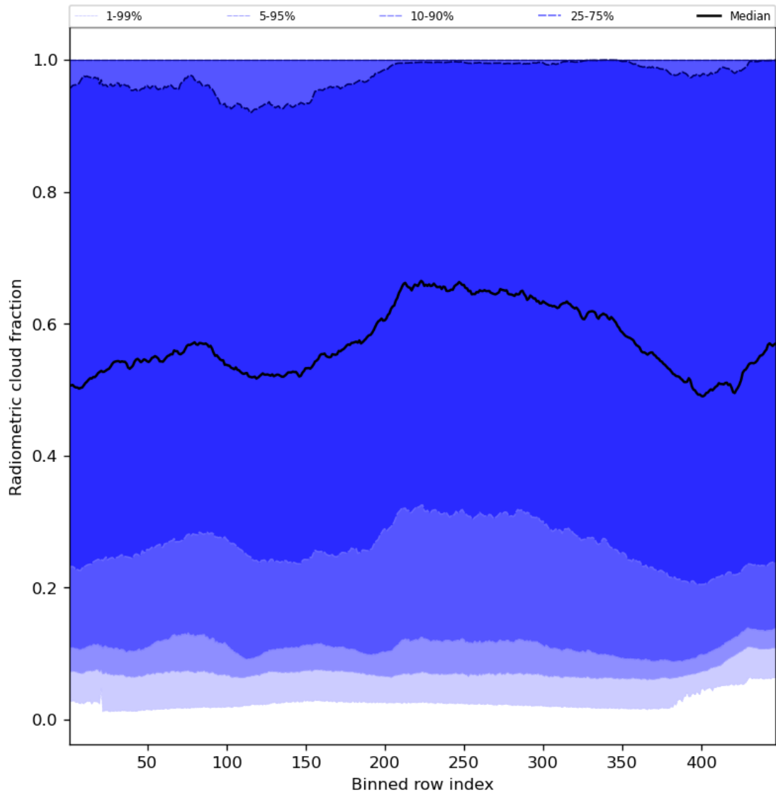
Figure 55: Along track statistics of “Radiometric cloud fraction” for 2024-01-11 to 2024-01-13
