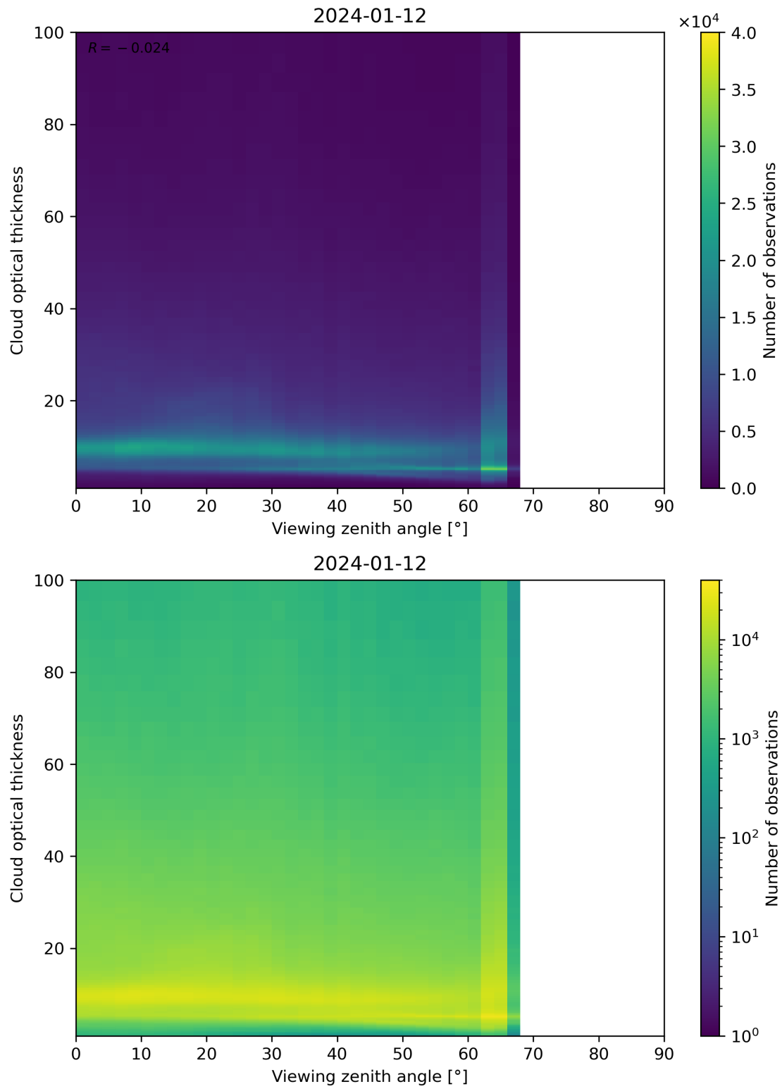
Figure 111: Scatter density plot of “Viewing zenith angle” against “Cloud optical thickness” for 2024-01-11 to 2024-01-13.
