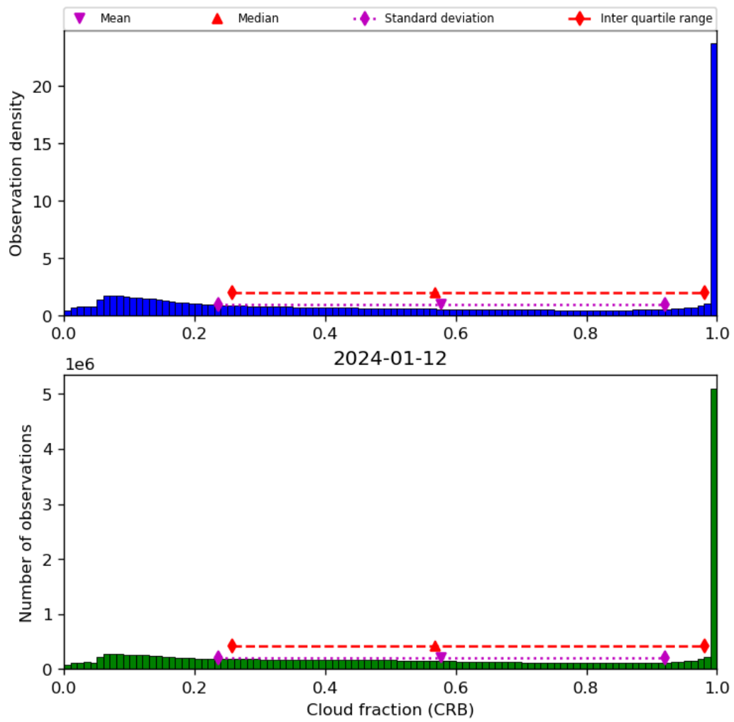
Figure 42: Histogram of “Cloud fraction (CRB)” for 2024-01-11 to 2024-01-13
