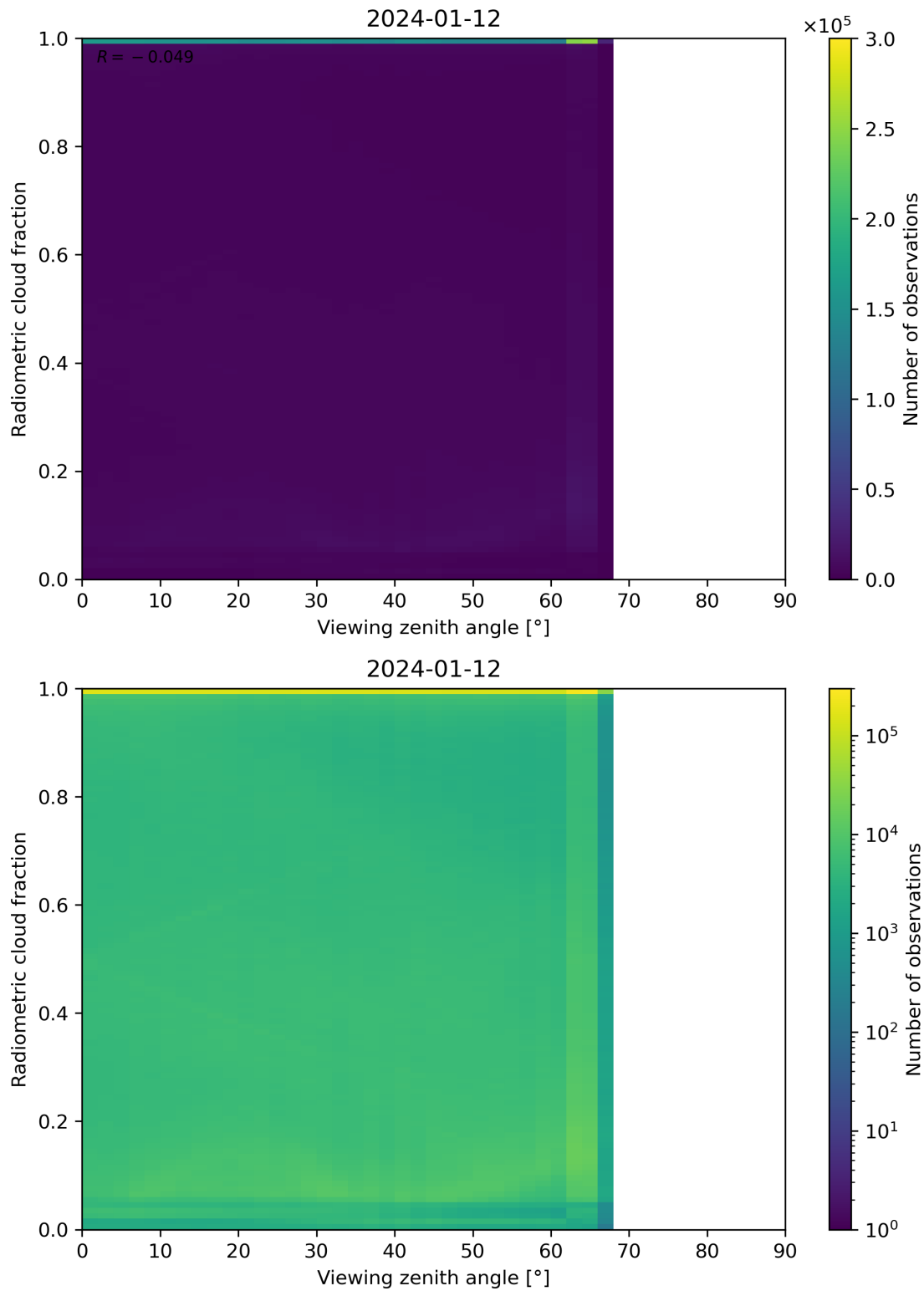
Figure 107: Scatter density plot of “Viewing zenith angle” against “Radiometric cloud fraction” for 2024-01-11 to 2024-01-13.
