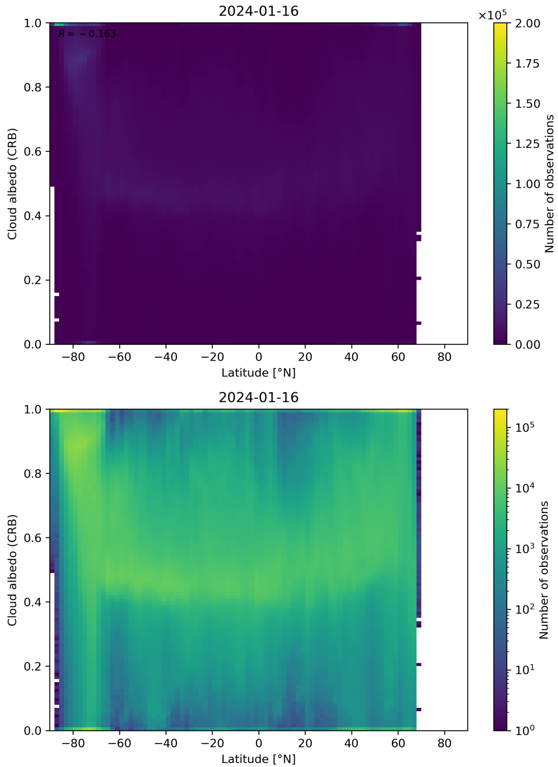
Figure 91: Scatter density plot of “Latitude” against “Cloud albedo (CRB)” for 2024-01-15 to 2024-01-17.
