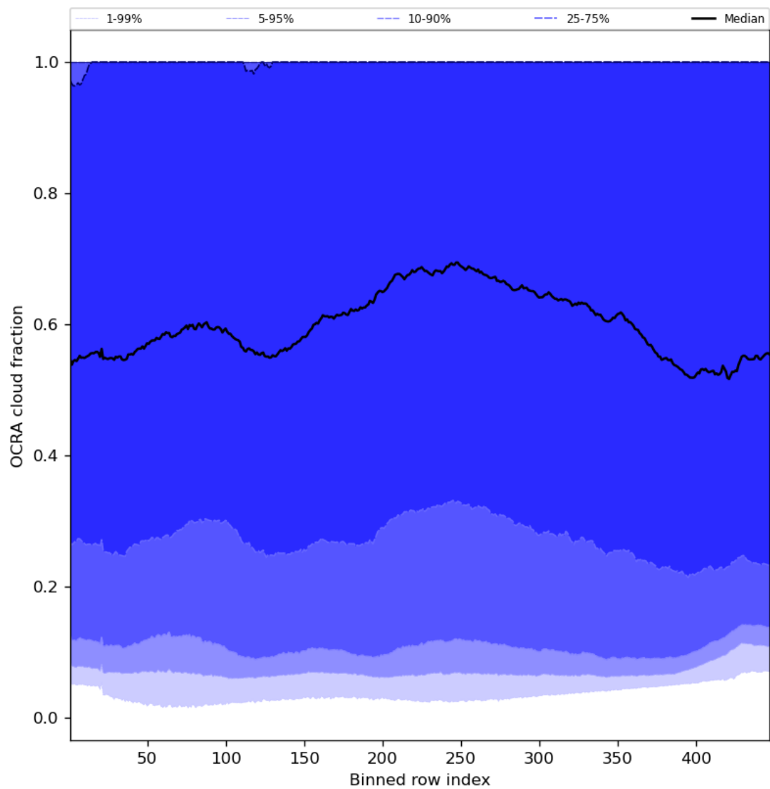
Figure 66: Along track statistics of “OCRA cloud fraction” for 2024-01-15 to 2024-01-17
