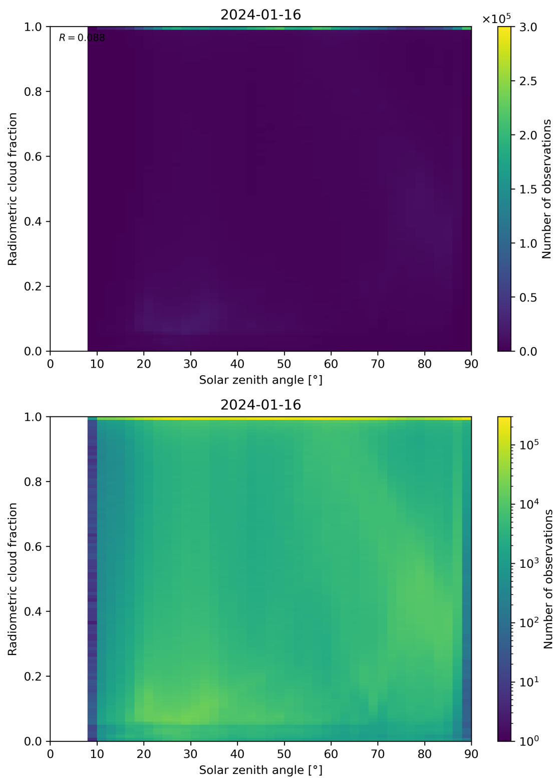
Figure 99: Scatter density plot of “Solar zenith angle” against “Radiometric cloud fraction” for 2024-01-15 to 2024-01-17.
