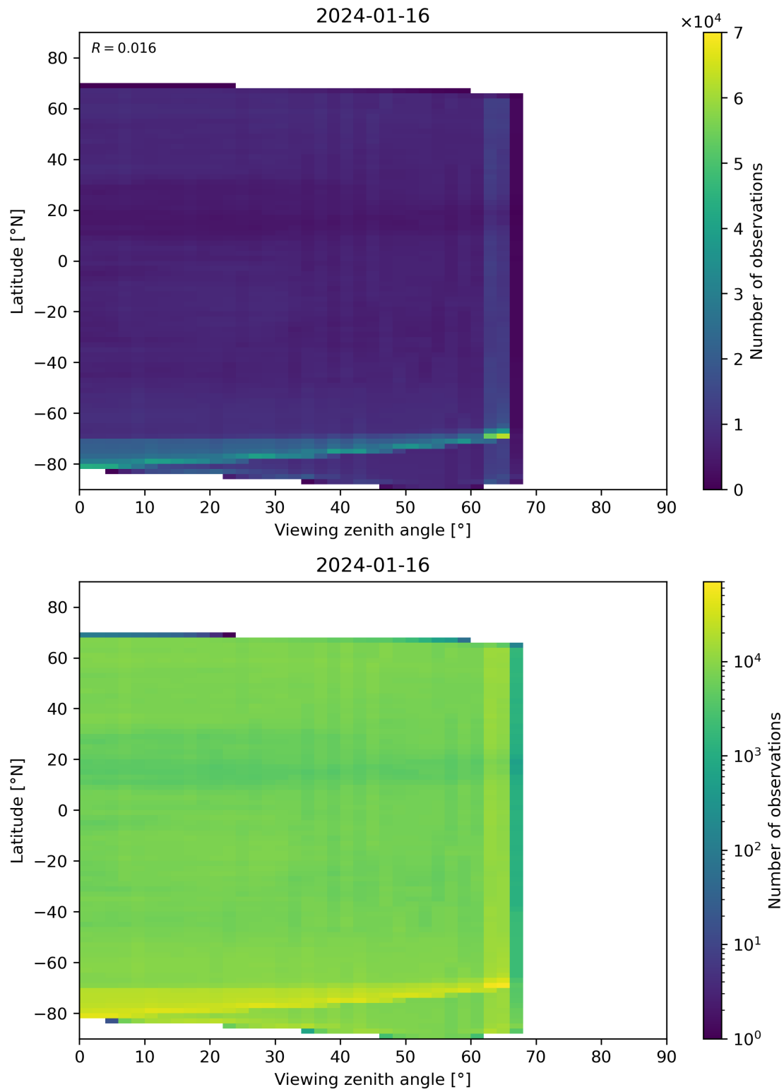
Figure 113: Scatter density plot of “Viewing zenith angle” against “Latitude” for 2024-01-15 to 2024-01-17.
