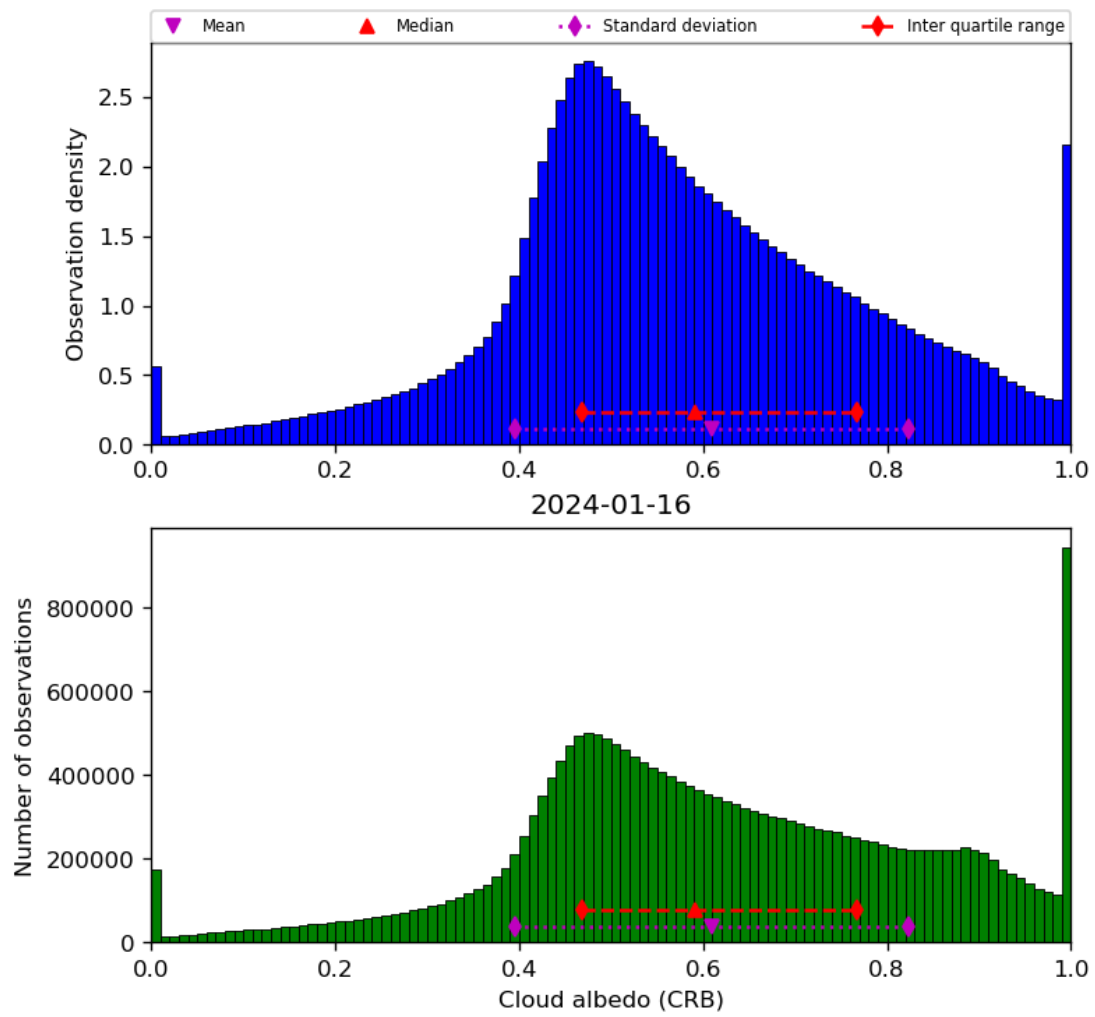
Figure 44: Histogram of “Cloud albedo (CRB)” for 2024-01-15 to 2024-01-17
