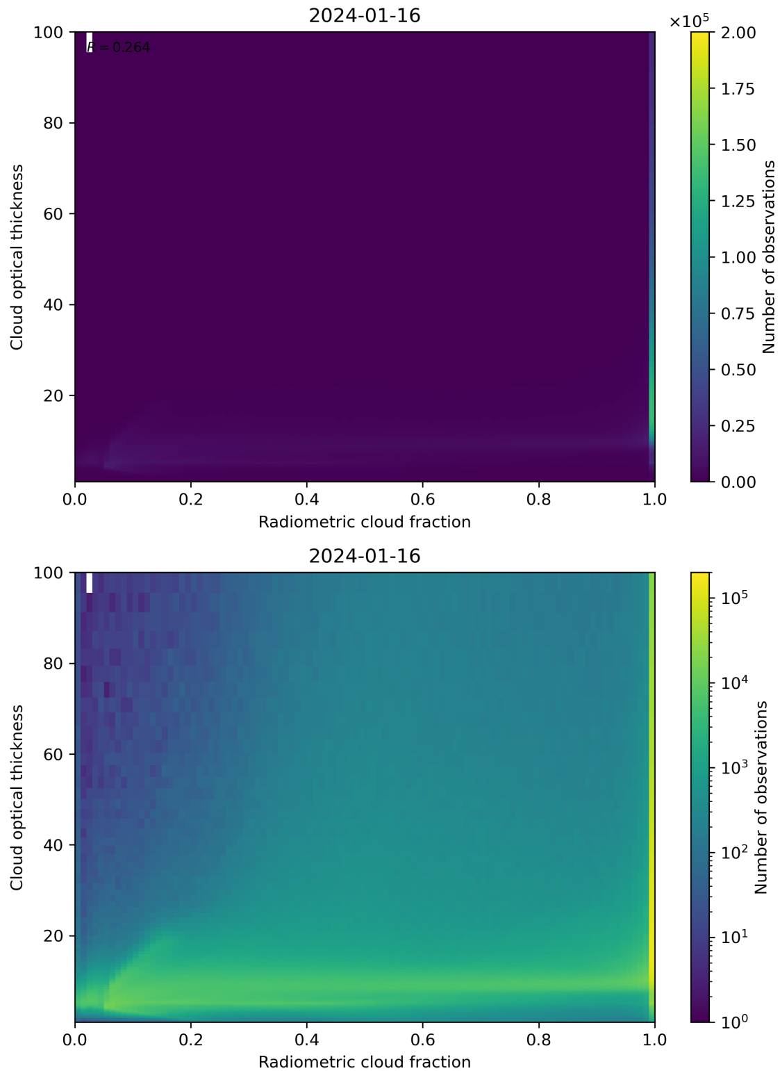
Figure 75: Scatter density plot of “Radiometric cloud fraction” against “Cloud optical thickness” for 2024-01-15 to 2024-01-17.
