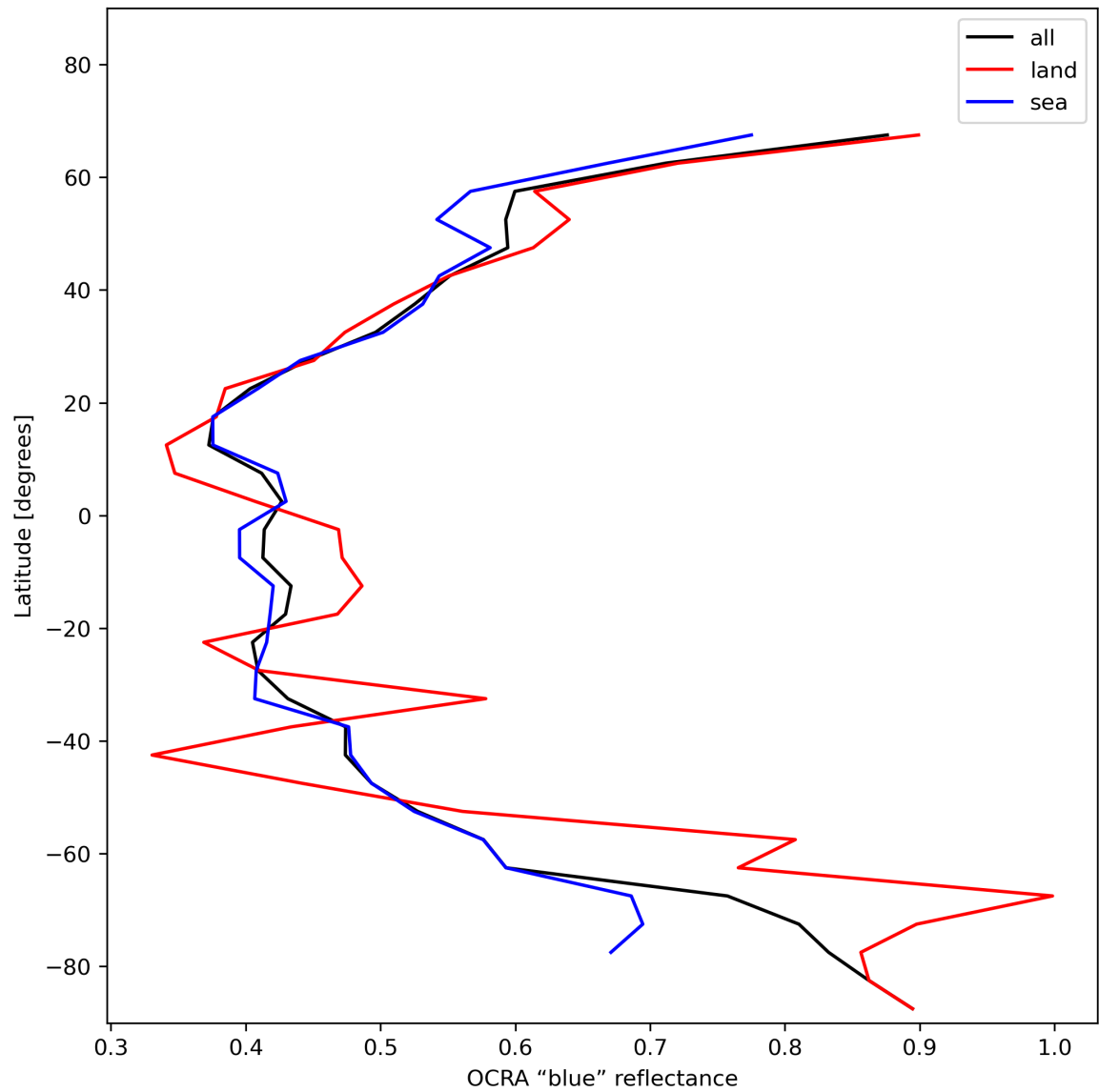
Figure 35: Zonal average of “OCRA “blue” reflectance” for 2024-01-15 to 2024-01-17.
