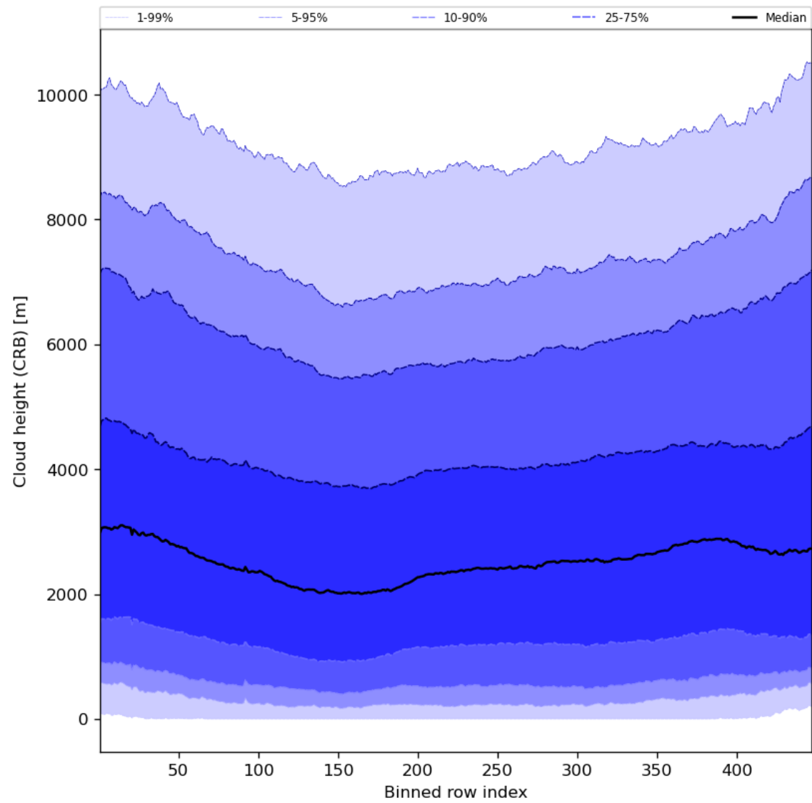
Figure 59: Along track statistics of “Cloud height (CRB)” for 2024-01-15 to 2024-01-17
