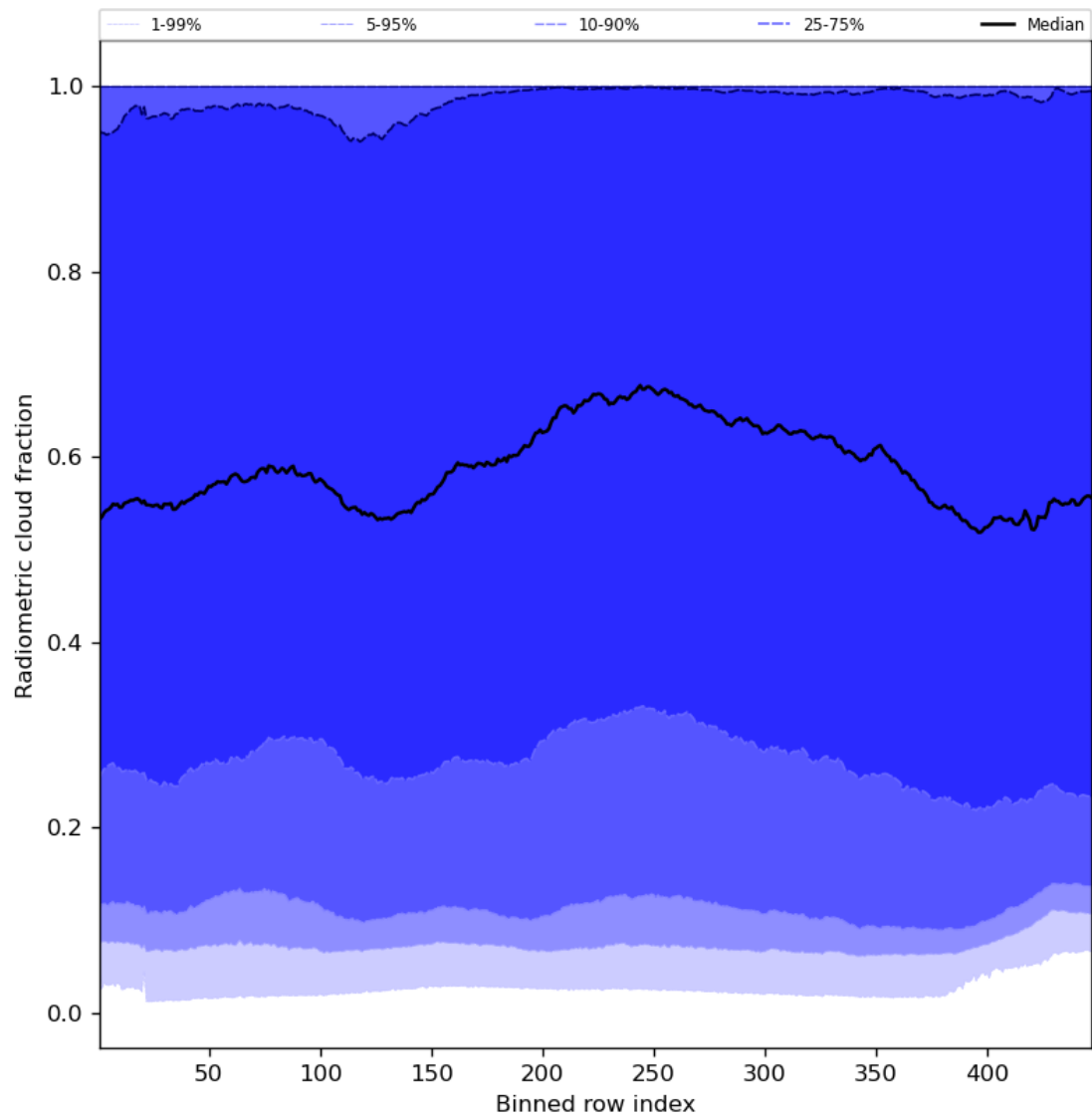
Figure 55: Along track statistics of “Radiometric cloud fraction” for 2024-01-15 to 2024-01-17
