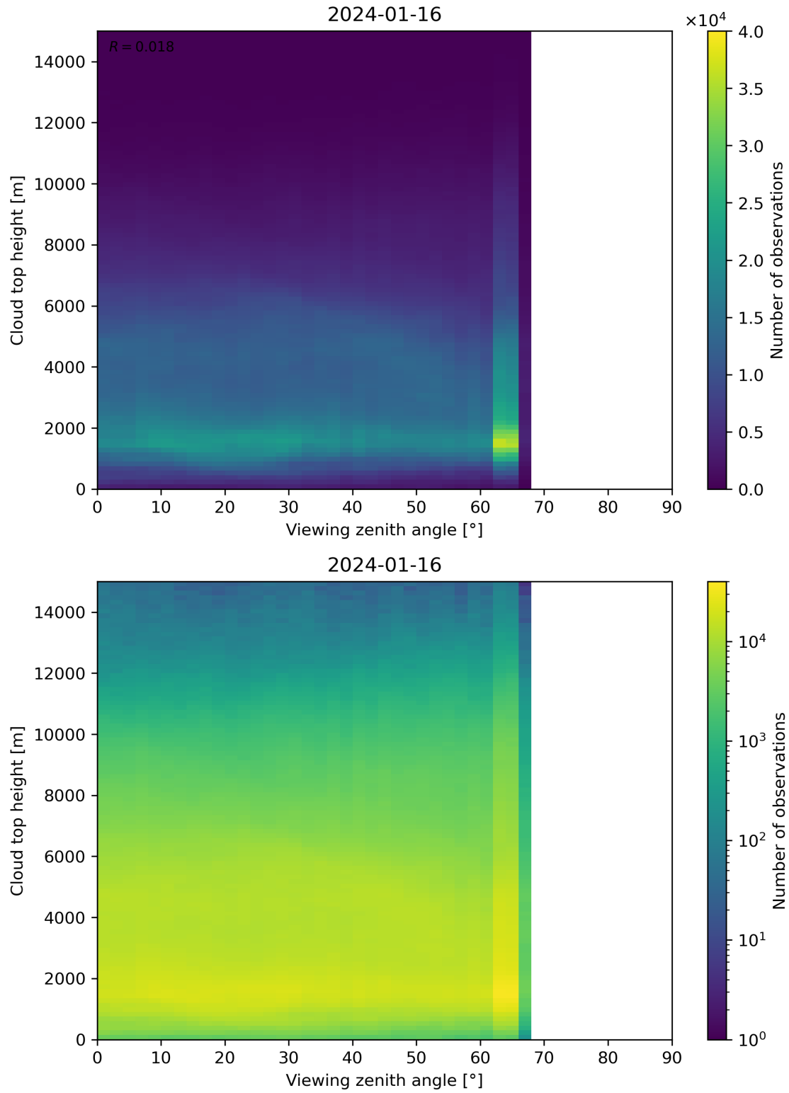
Figure 112: Scatter density plot of “Viewing zenith angle” against “Cloud top height” for 2024-01-15 to 2024-01-17.
