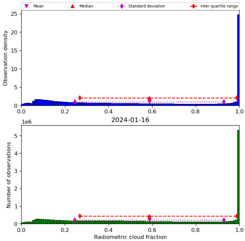
Figure 39: Histogram of “Radiometric cloud fraction” for 2024-01-15 to 2024-01-17
