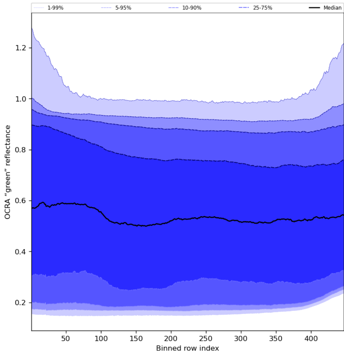
Figure 68: Along track statistics of “OCRA “green” reflectance” for 2024-01-15 to 2024-01-17
