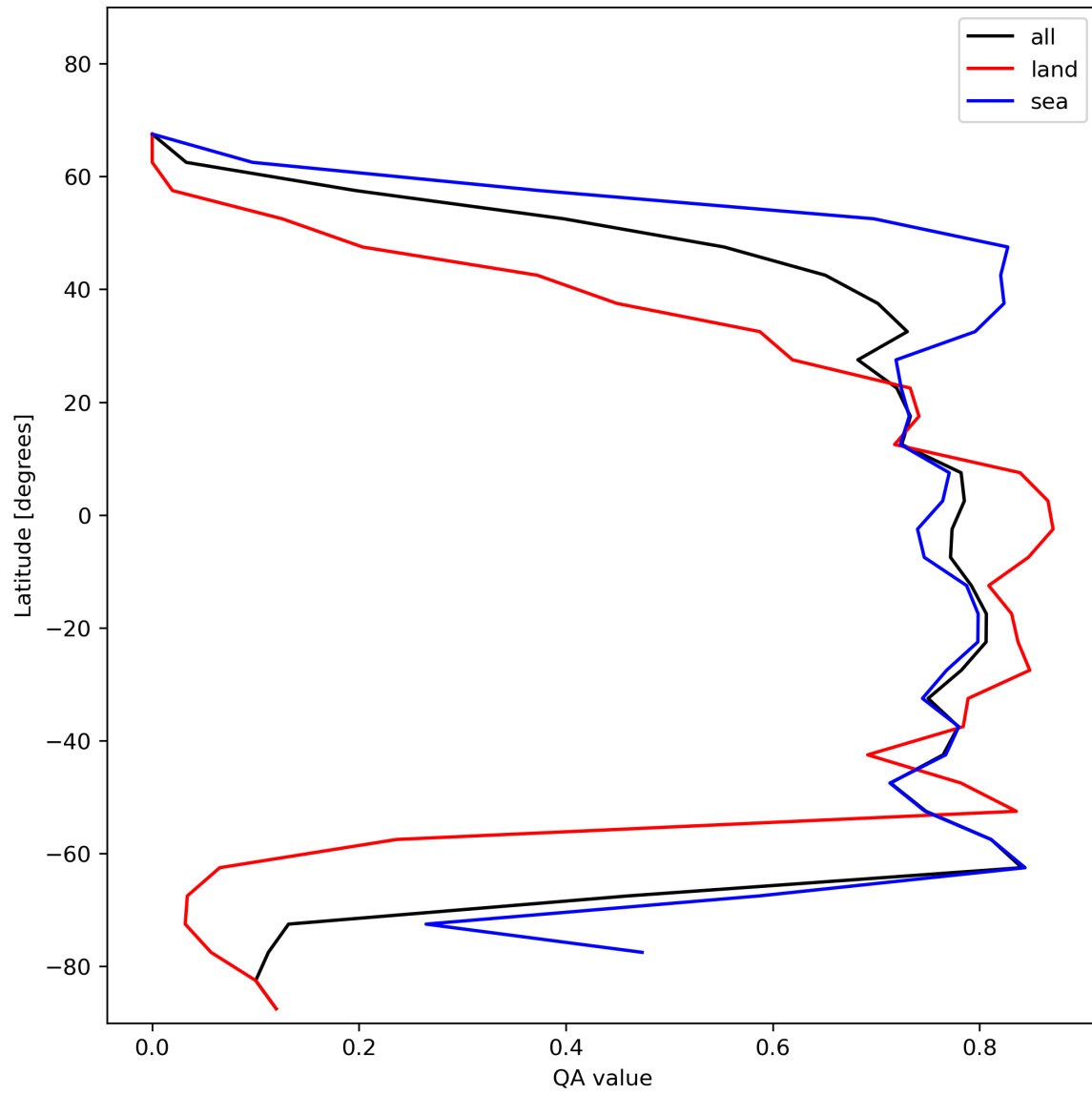
Figure 22: Zonal average of “QA value” for 2024-01-15 to 2024-01-17.
