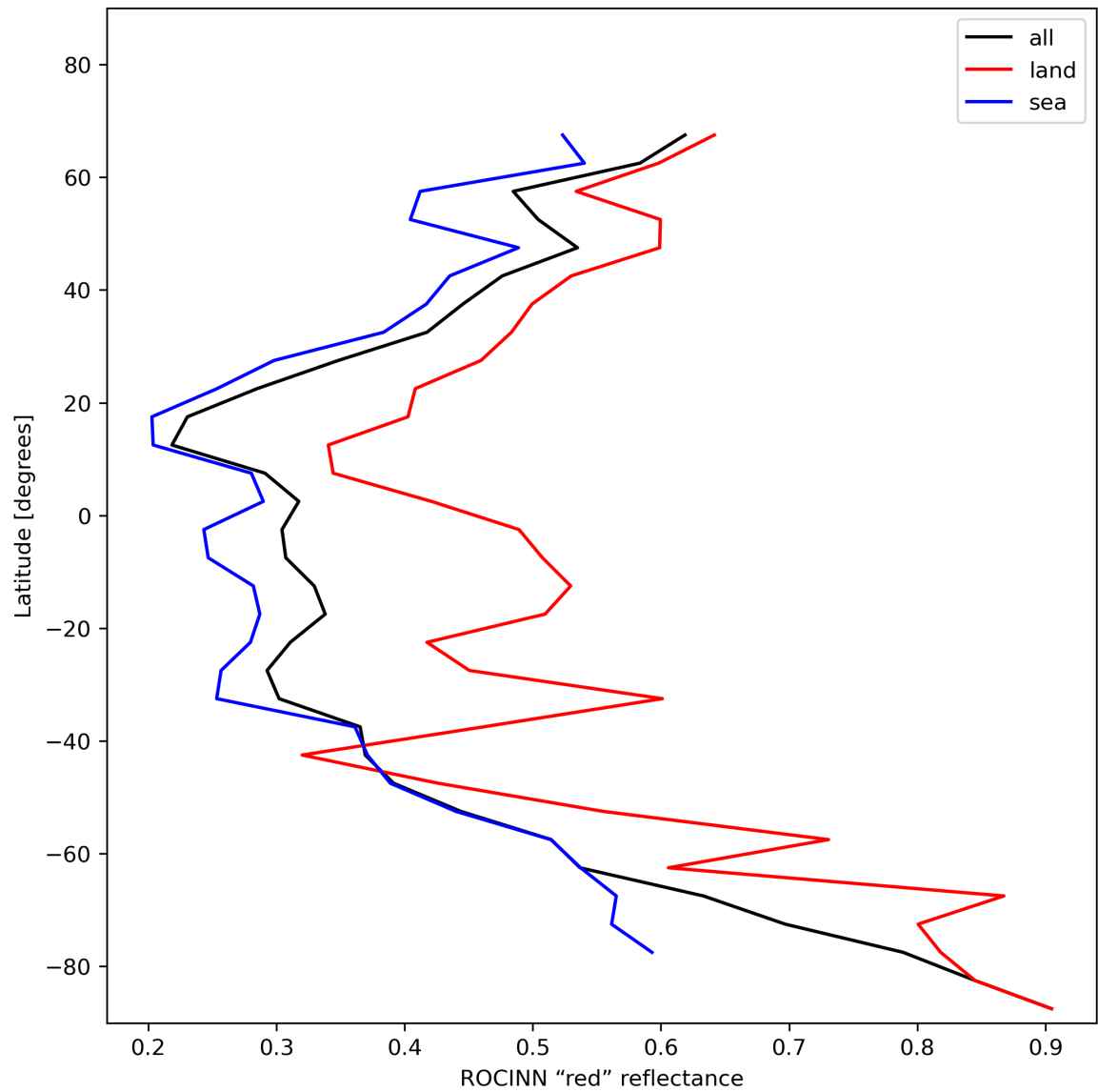
Figure 37: Zonal average of “ROCINN “red” reflectance” for 2024-01-15 to 2024-01-17.
