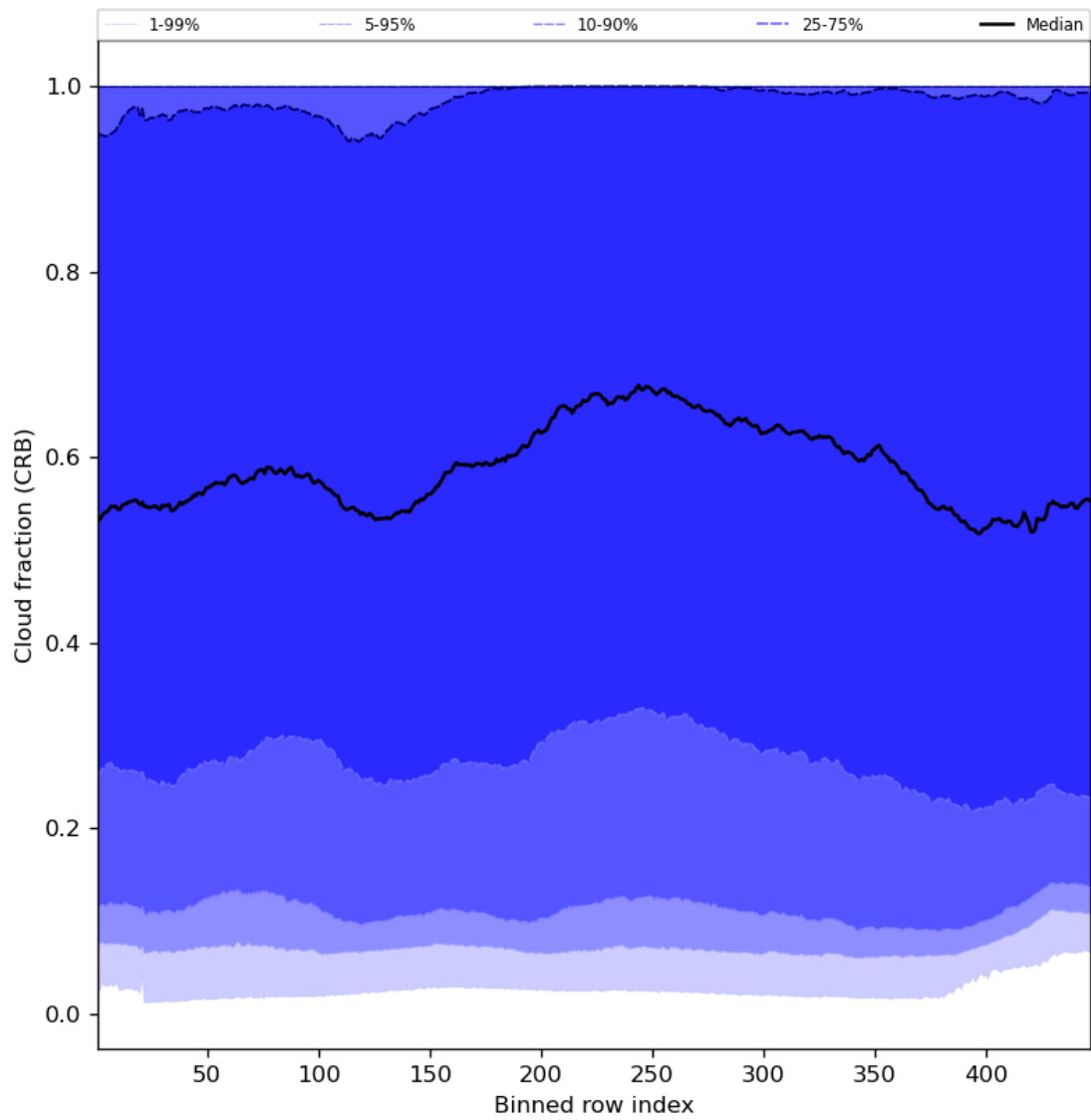
Figure 58: Along track statistics of “Cloud fraction (CRB)” for 2024-01-15 to 2024-01-17
