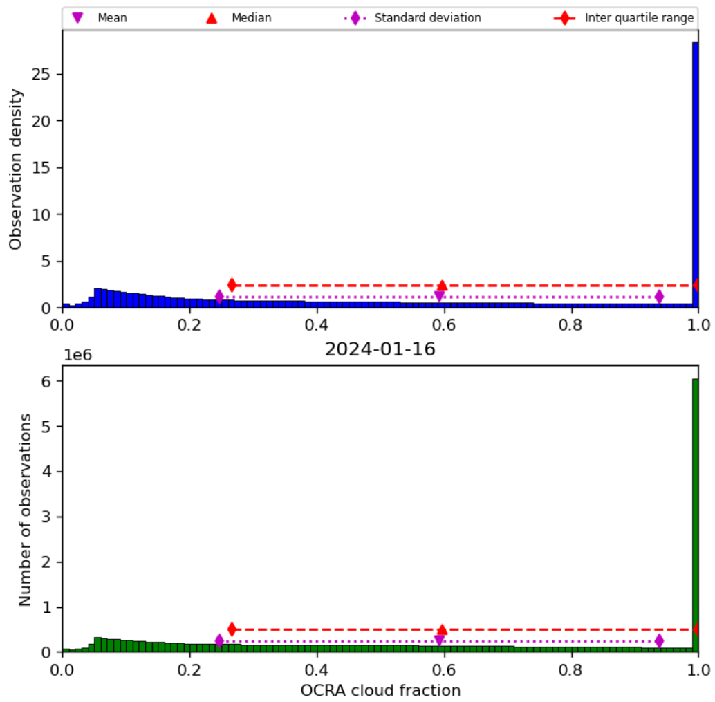
Figure 50: Histogram of “OCRA cloud fraction” for 2024-01-15 to 2024-01-17
