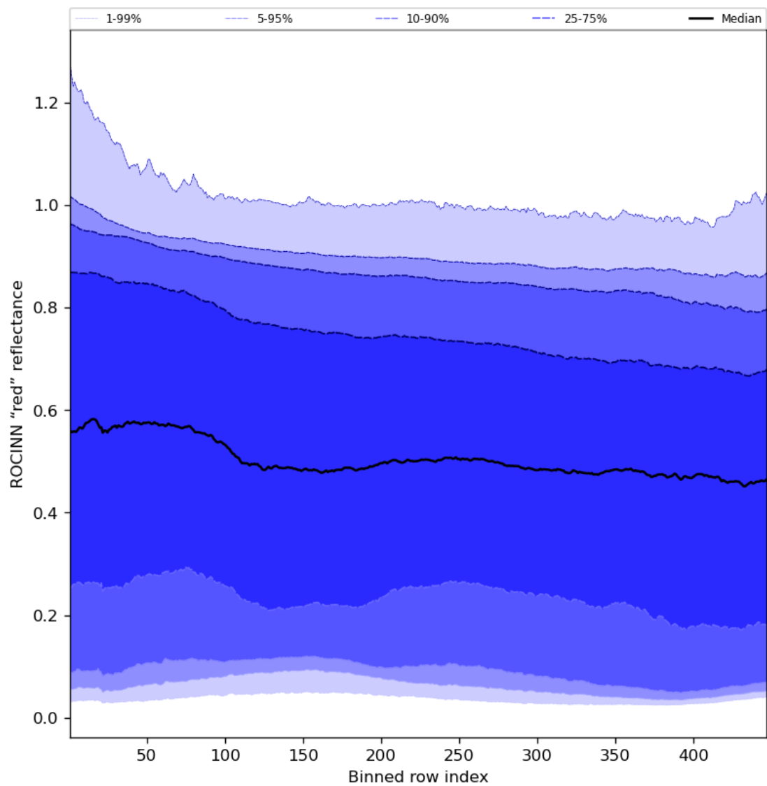
Figure 69: Along track statistics of “ROCINN “red” reflectance” for 2024-01-15 to 2024-01-17
