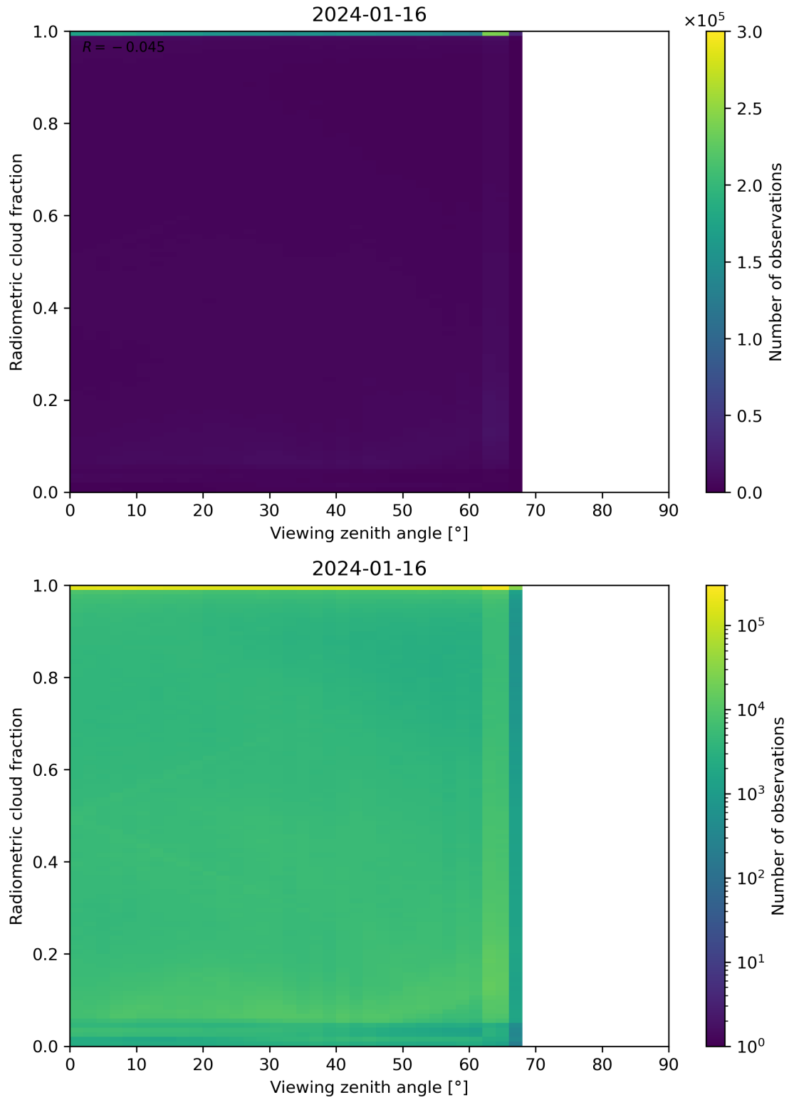
Figure 107: Scatter density plot of “Viewing zenith angle” against “Radiometric cloud fraction” for 2024-01-15 to 2024-01-17.
