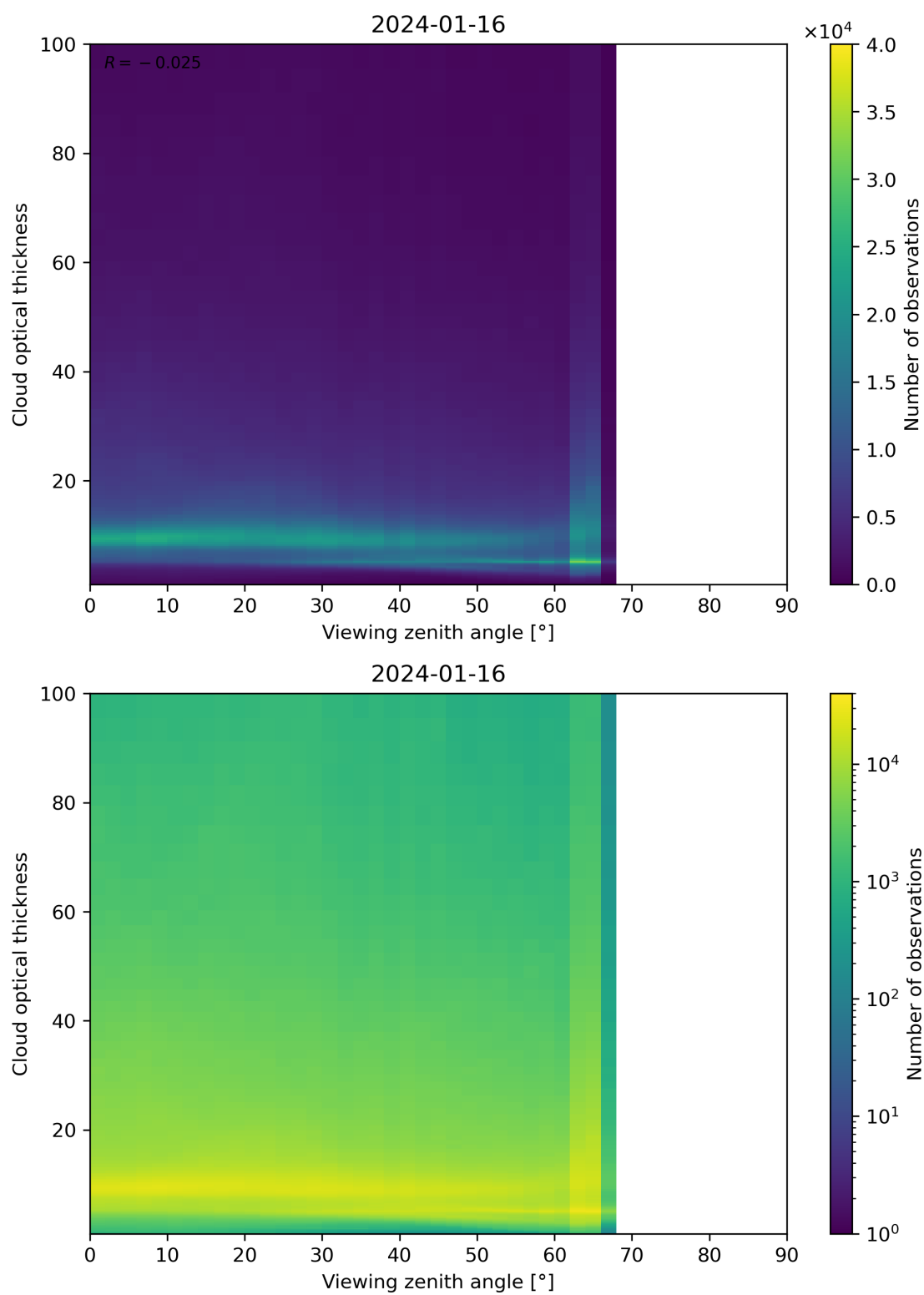
Figure 111: Scatter density plot of “Viewing zenith angle” against “Cloud optical thickness” for 2024-01-15 to 2024-01-17.
