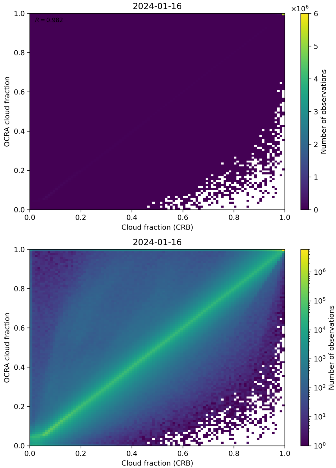
Figure 78: Scatter density plot of “Cloud fraction (CRB)” against “OCRA cloud fraction” for 2024-01-15 to 2024-01-17.
