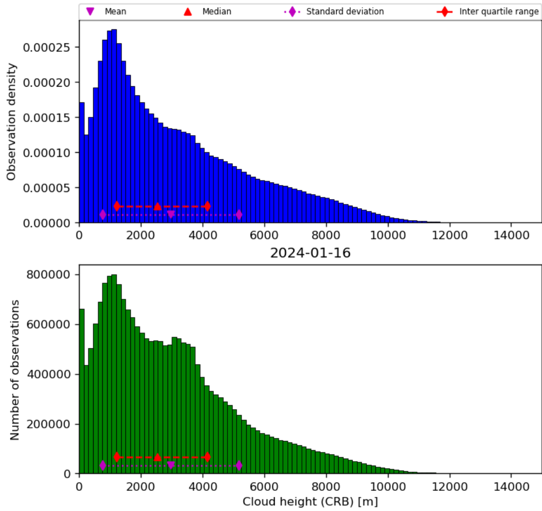
Figure 43: Histogram of “Cloud height (CRB)” for 2024-01-15 to 2024-01-17
