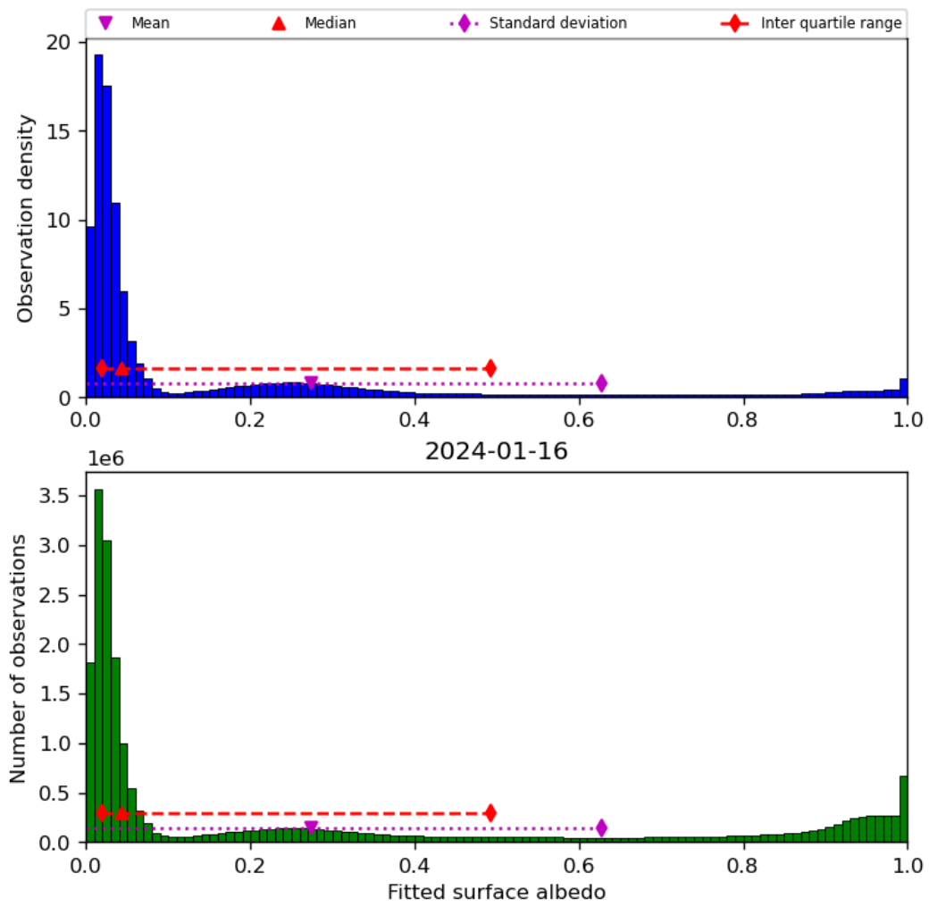
Figure 45: Histogram of “Fitted surface albedo” for 2024-01-15 to 2024-01-17
