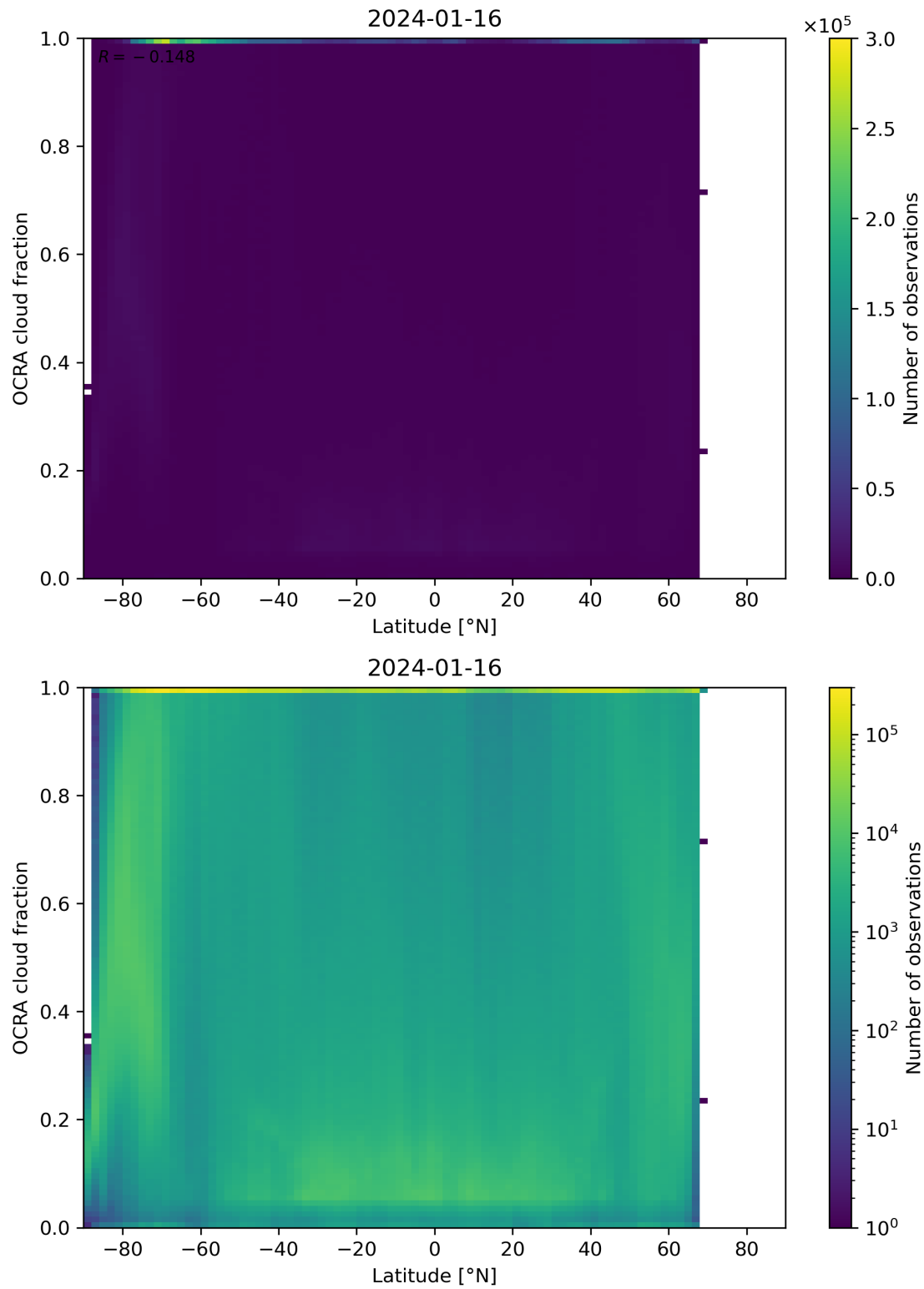
Figure 93: Scatter density plot of “Latitude” against “OCRA cloud fraction” for 2024-01-15 to 2024-01-17.
