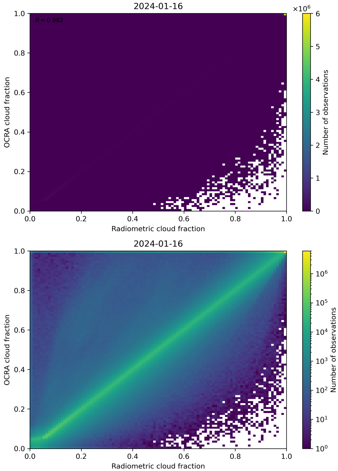
Figure 72: Scatter density plot of “Radiometric cloud fraction” against “OCRA cloud fraction” for 2024-01-15 to 2024-01-17.
