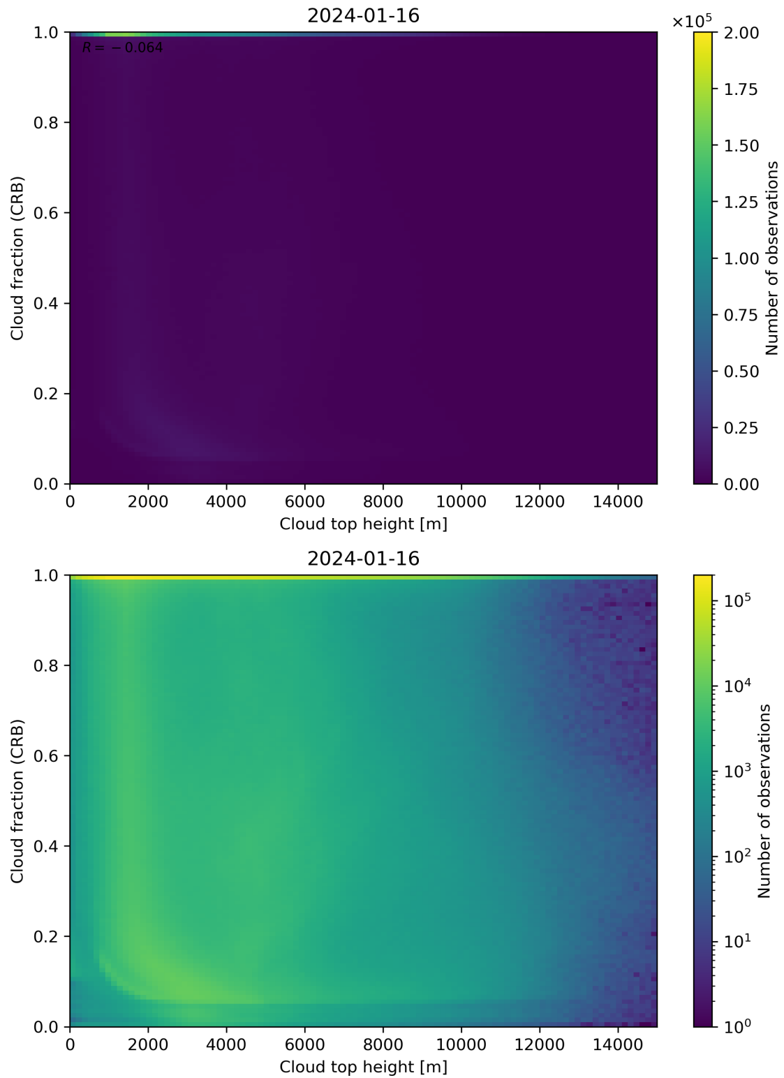
Figure 88: Scatter density plot of “Cloud top height” against “Cloud fraction (CRB)” for 2024-01-15 to 2024-01-17.
