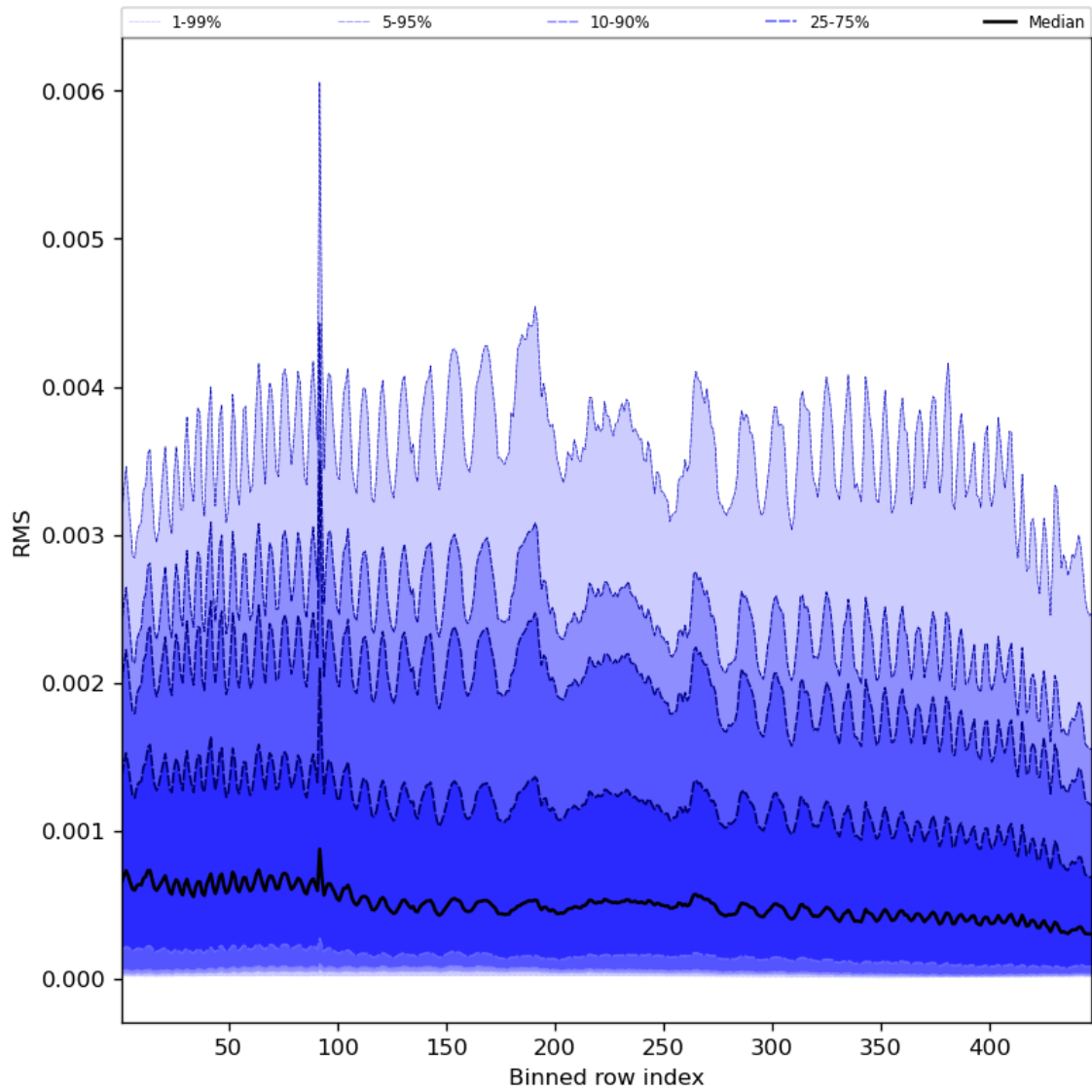
Figure 63: Along track statistics of “RMS” for 2024-01-15 to 2024-01-17
