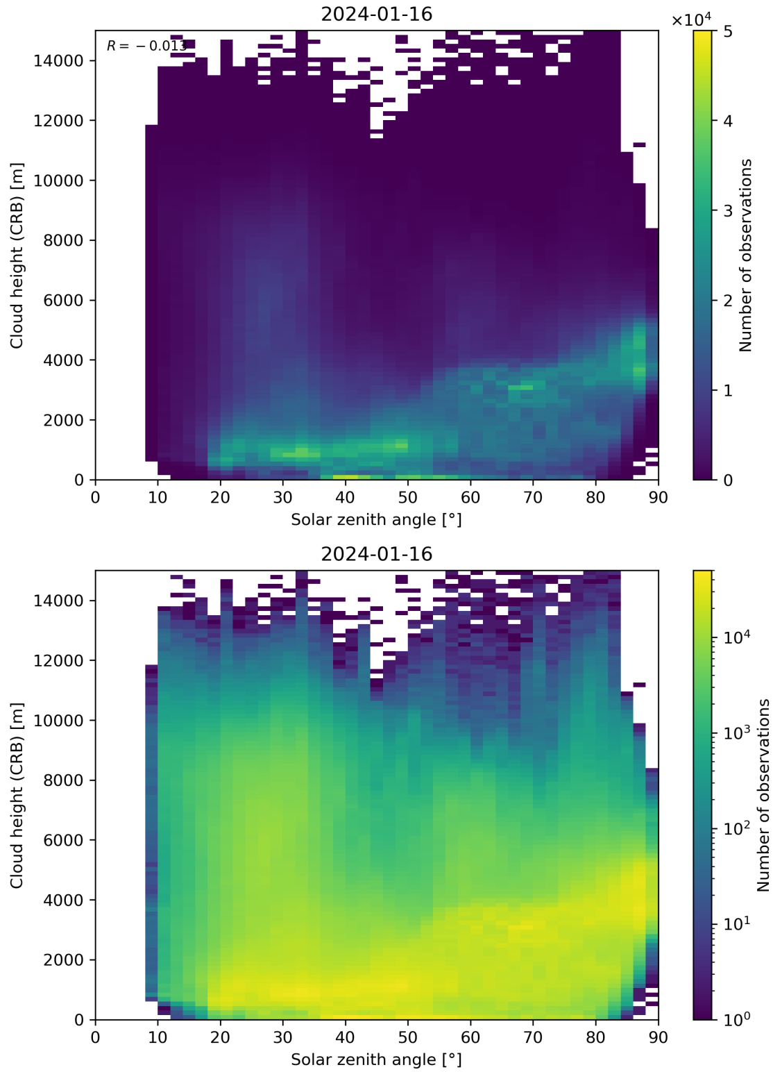
Figure 102: Scatter density plot of “Solar zenith angle” against “Cloud height (CRB)” for 2024-01-15 to 2024-01-17.
