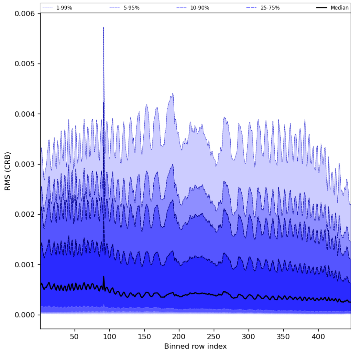
Figure 64: Along track statistics of “RMS (CRB)” for 2024-01-15 to 2024-01-17
