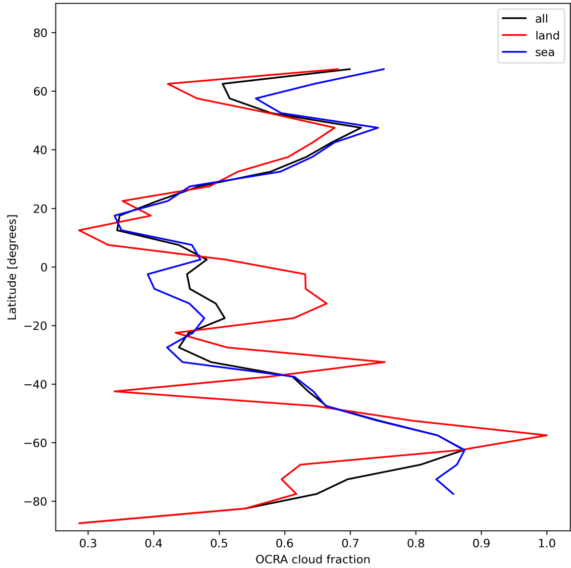
Figure 34: Zonal average of “OCRA cloud fraction” for 2024-01-15 to 2024-01-17.
