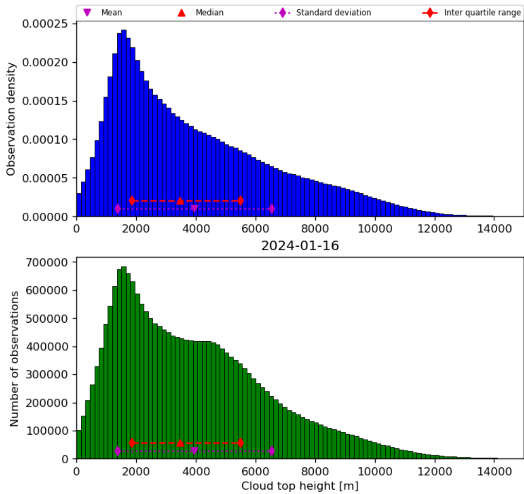
Figure 40: Histogram of “Cloud top height” for 2024-01-15 to 2024-01-17
