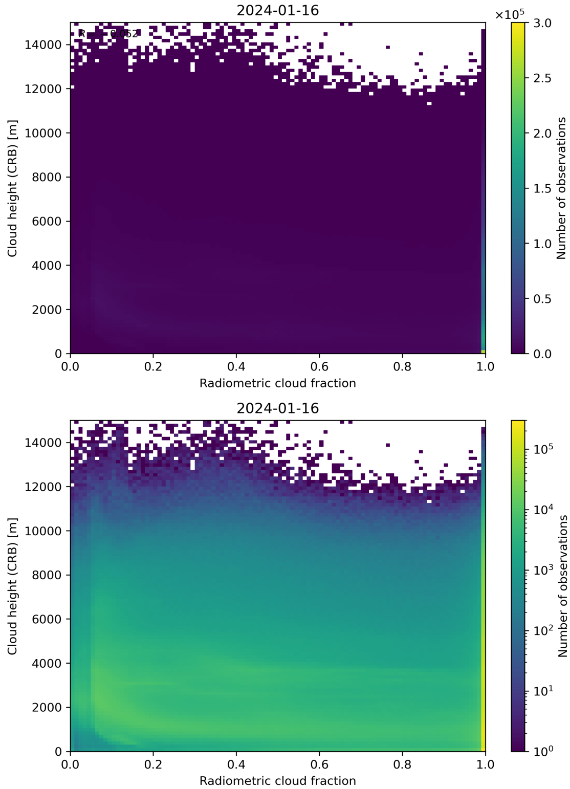
Figure 74: Scatter density plot of “Radiometric cloud fraction” against “Cloud height (CRB)” for 2024-01-15 to 2024-01-17.
