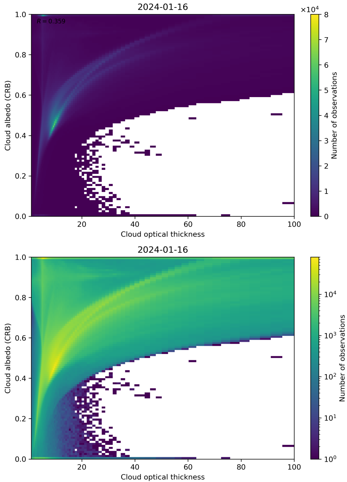
Figure 82: Scatter density plot of “Cloud optical thickness” against “Cloud albedo (CRB)” for 2024-01-15 to 2024-01-17.
