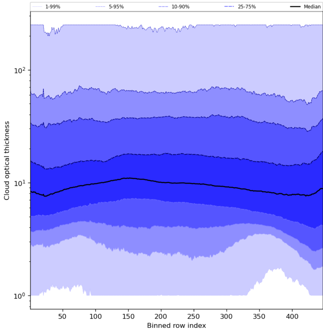
Figure 57: Along track statistics of “Cloud optical thickness” for 2024-01-15 to 2024-01-17
