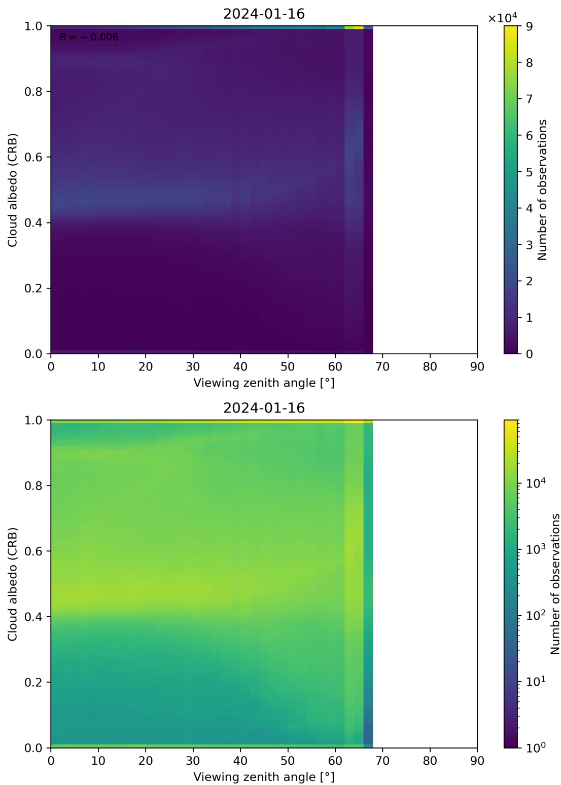
Figure 106: Scatter density plot of “Viewing zenith angle” against “Cloud albedo (CRB)” for 2024-01-15 to 2024-01-17.
