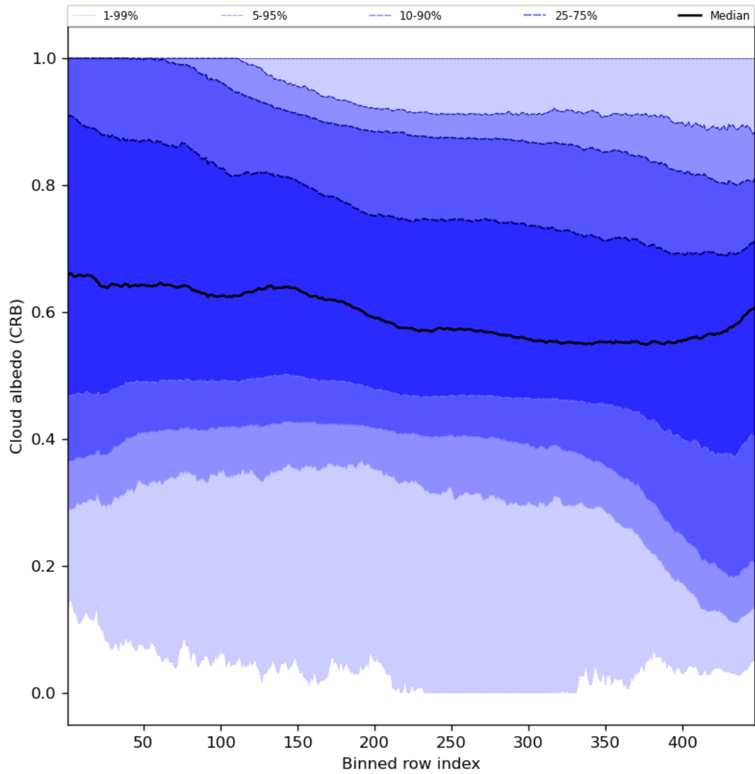
Figure 60: Along track statistics of “Cloud albedo (CRB)” for 2024-01-15 to 2024-01-17
