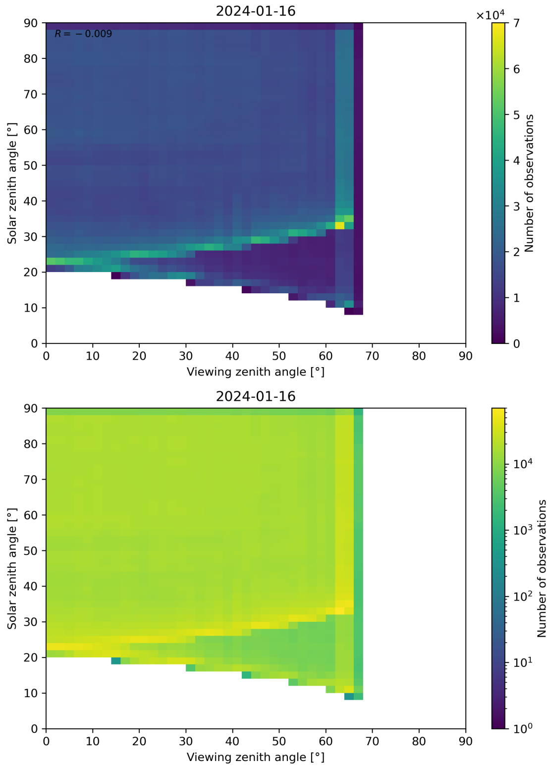
Figure 114: Scatter density plot of “Viewing zenith angle” against “Solar zenith angle” for 2024-01-15 to 2024-01-17.
