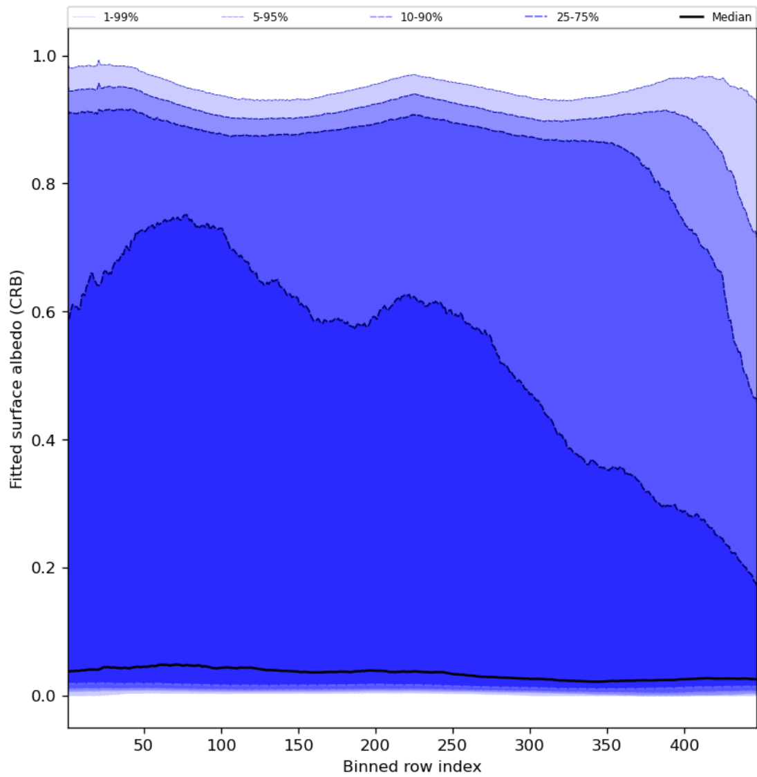
Figure 62: Along track statistics of “Fitted surface albedo (CRB)” for 2024-01-15 to 2024-01-17
