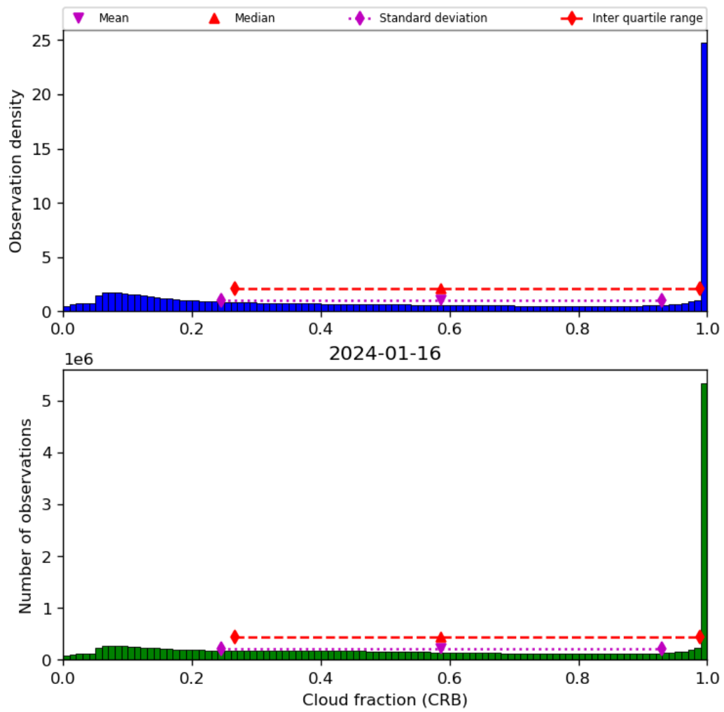
Figure 42: Histogram of “Cloud fraction (CRB)” for 2024-01-15 to 2024-01-17
