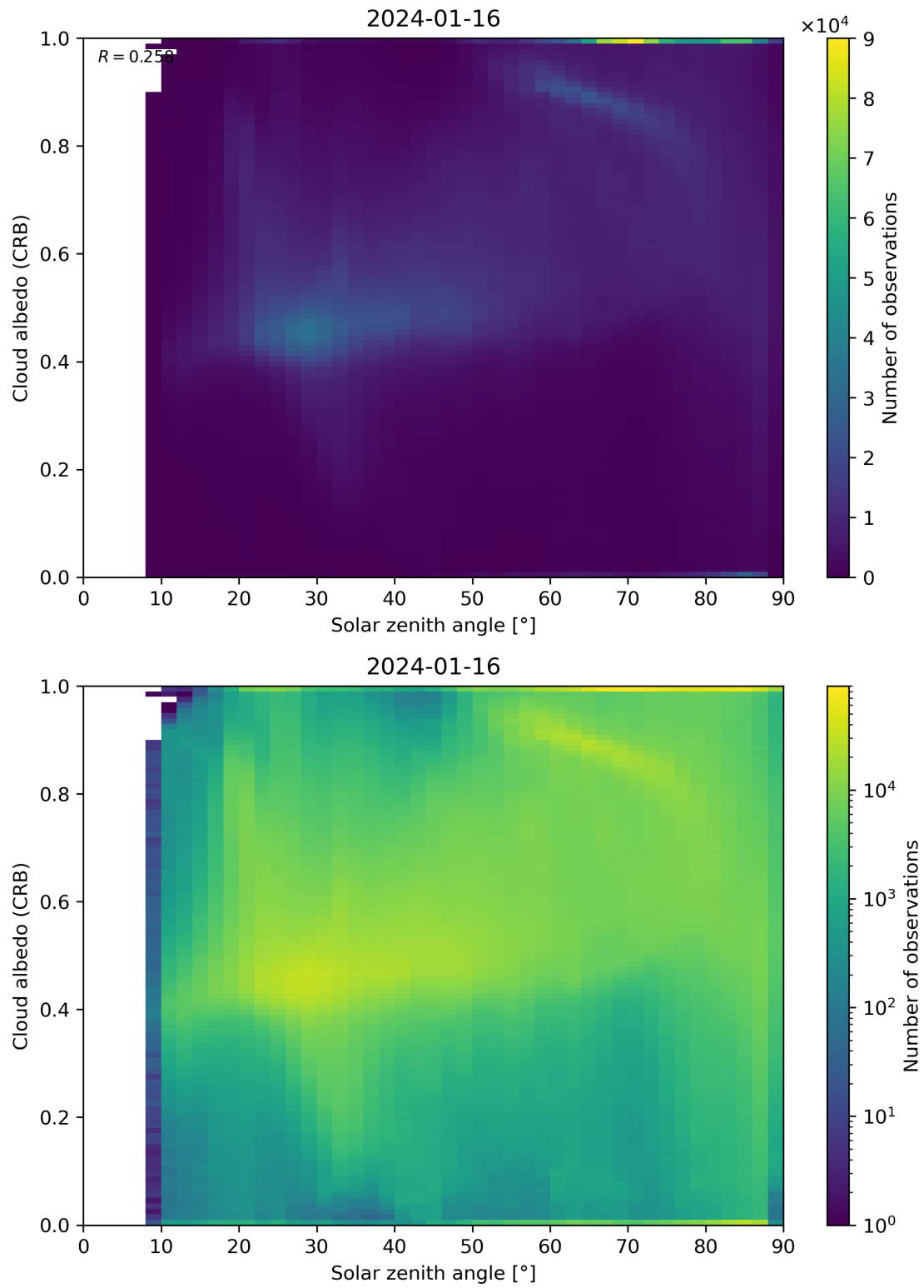
Figure 98: Scatter density plot of “Solar zenith angle” against “Cloud albedo (CRB)” for 2024-01-15 to 2024-01-17.
