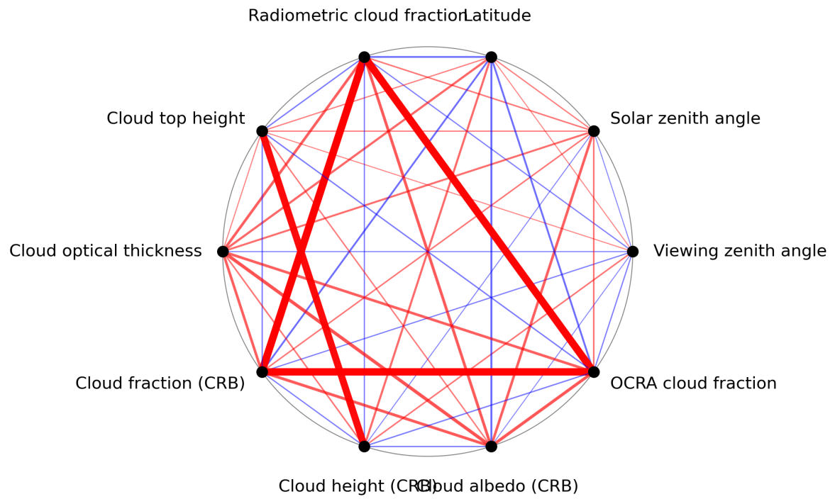
Figure 1: Map of correlation graph for 2024-01-15 to 2024-01-17.
