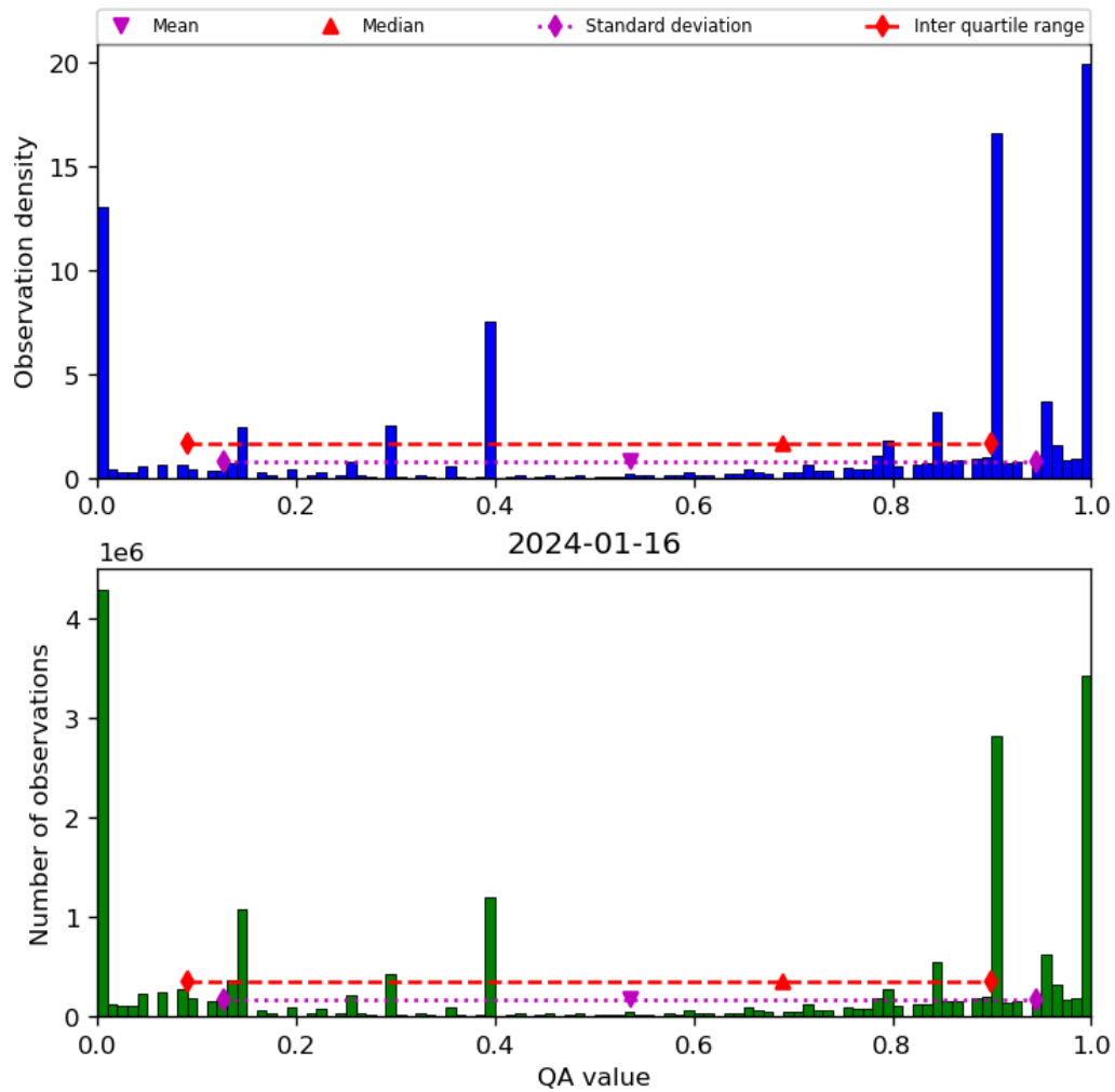
Figure 38: Histogram of “QA value” for 2024-01-15 to 2024-01-17
