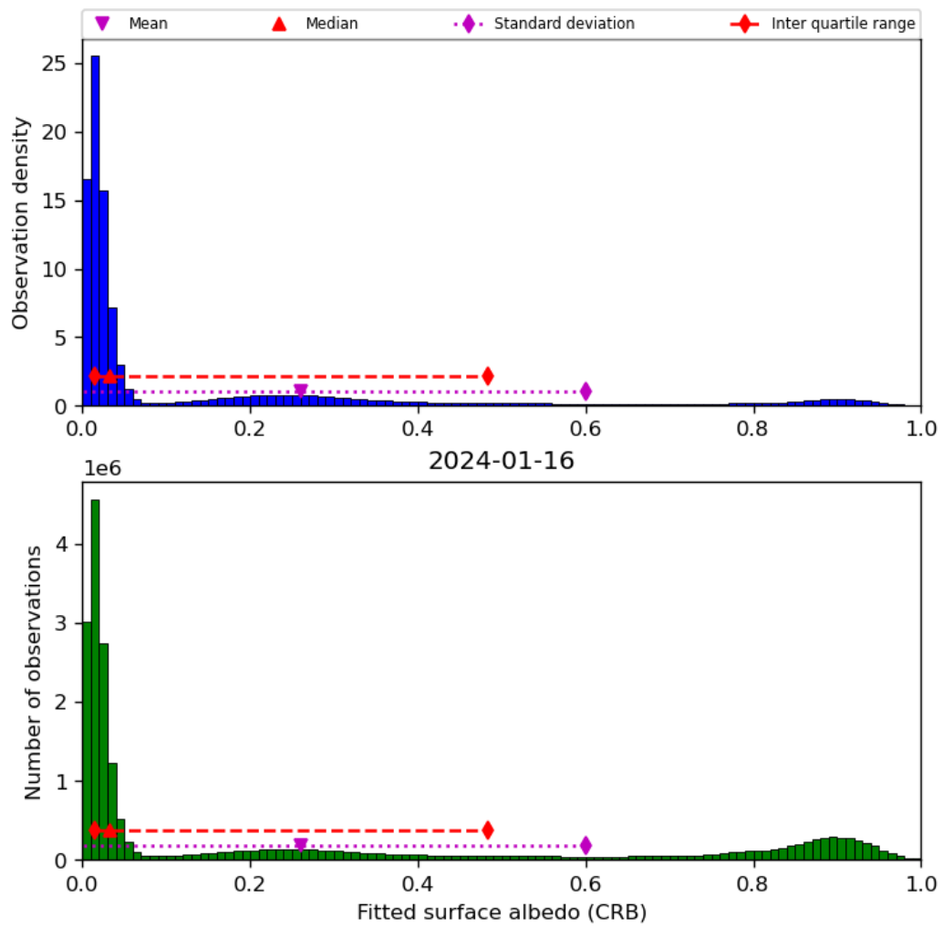
Figure 46: Histogram of “Fitted surface albedo (CRB)” for 2024-01-15 to 2024-01-17
