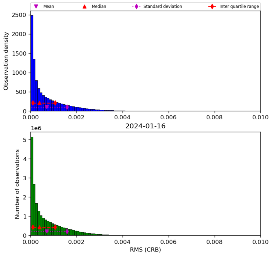
Figure 48: Histogram of “RMS (CRB)” for 2024-01-15 to 2024-01-17
