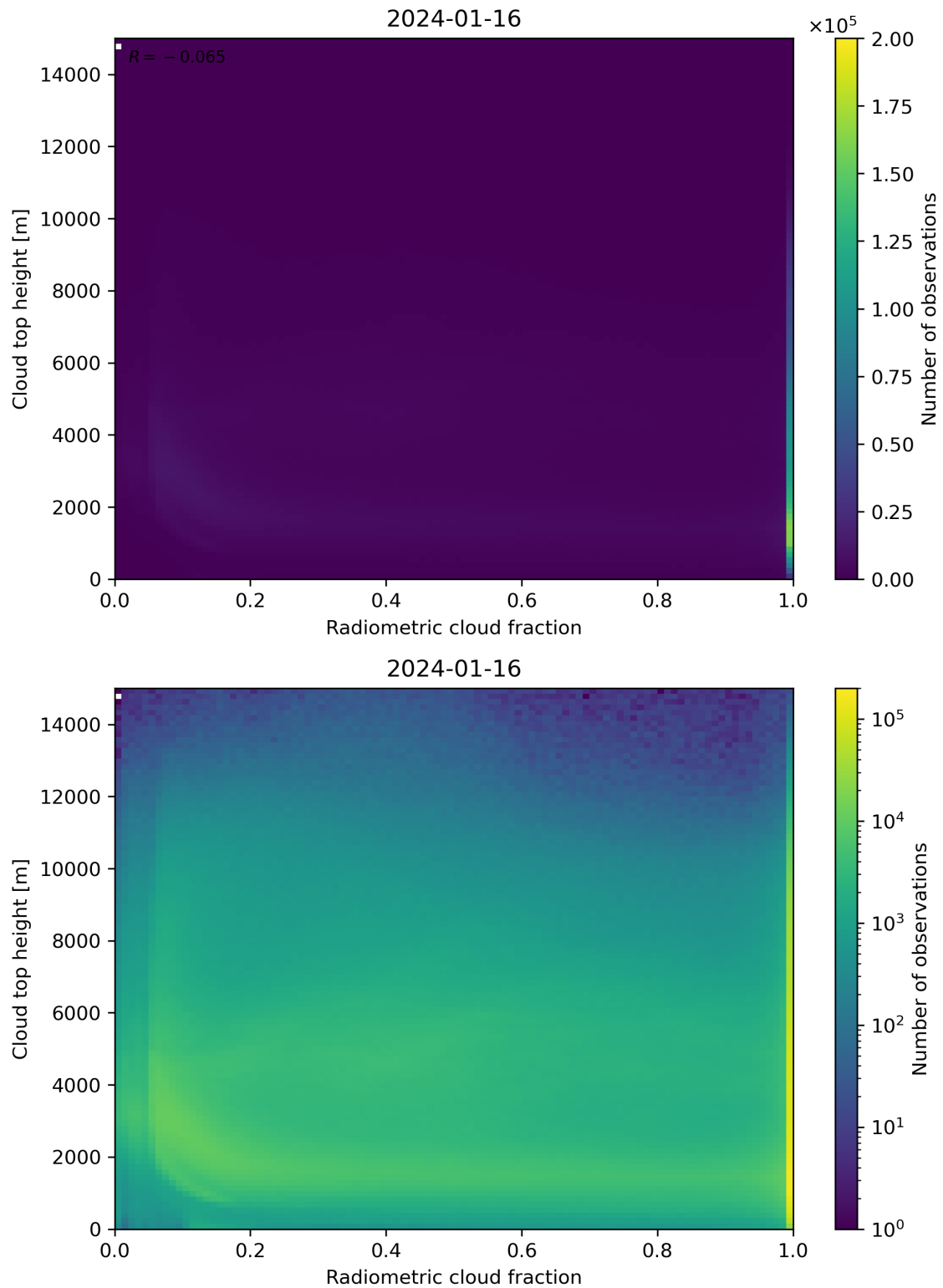
Figure 76: Scatter density plot of “Radiometric cloud fraction” against “Cloud top height” for 2024-01-15 to 2024-01-17.
