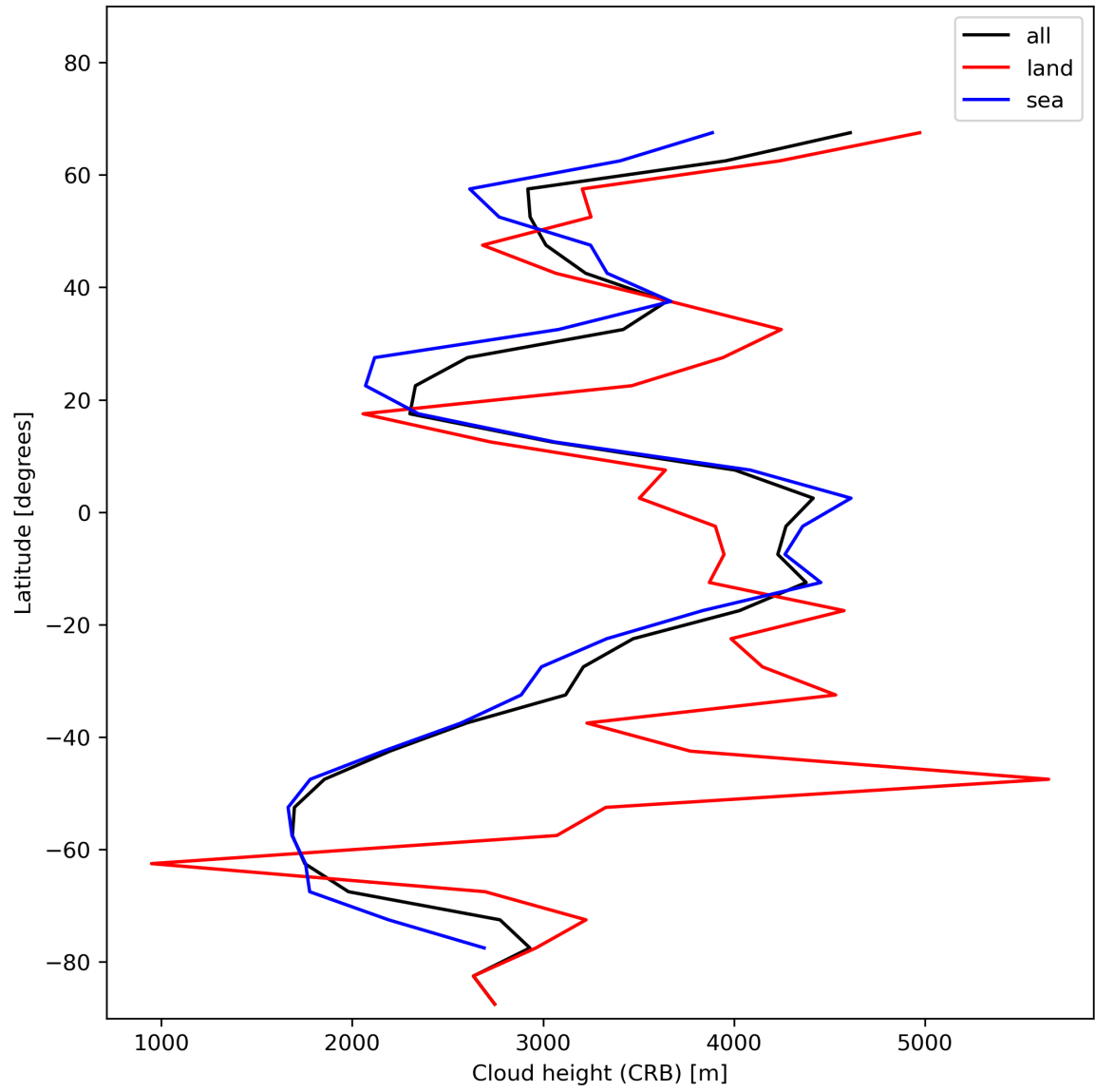
Figure 27: Zonal average of “Cloud height (CRB)” for 2024-01-15 to 2024-01-17.
