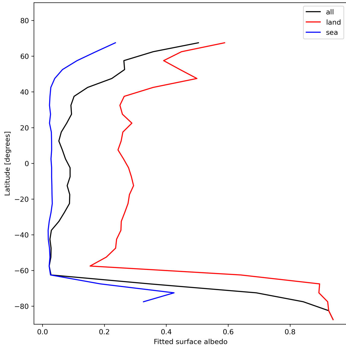
Figure 29: Zonal average of “Fitted surface albedo” for 2024-01-15 to 2024-01-17.
