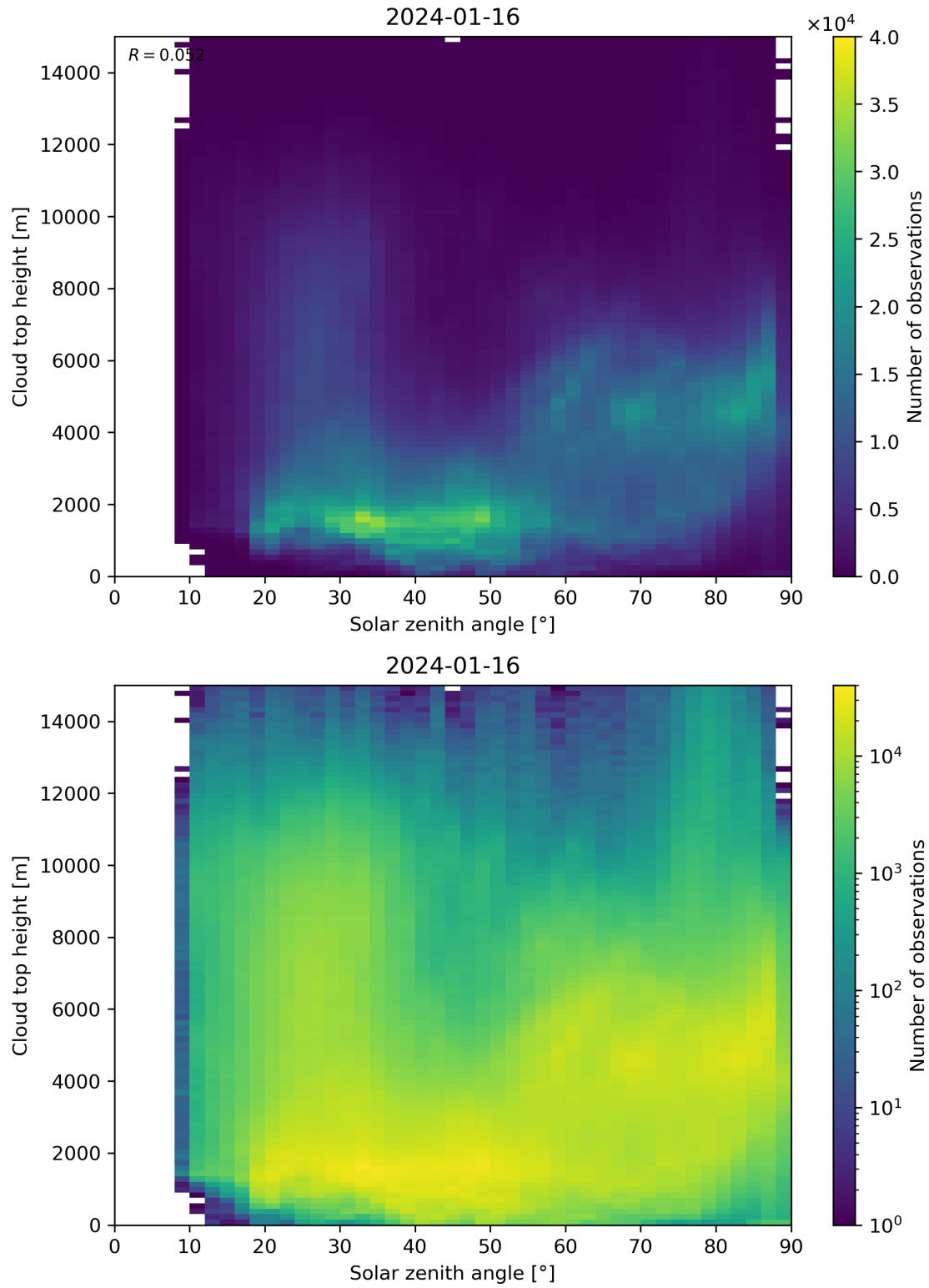
Figure 104: Scatter density plot of “Solar zenith angle” against “Cloud top height” for 2024-01-15 to 2024-01-17.
