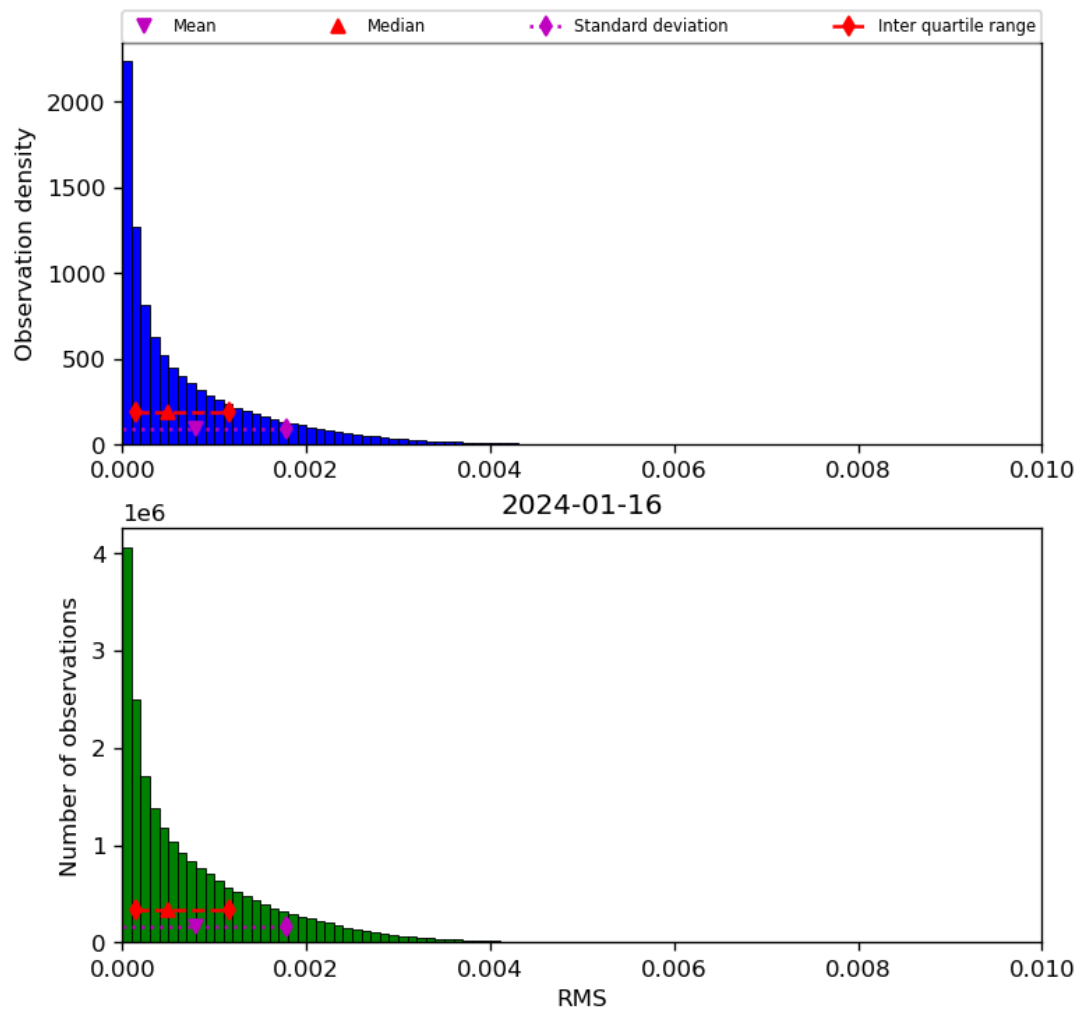
Figure 47: Histogram of “RMS” for 2024-01-15 to 2024-01-17
