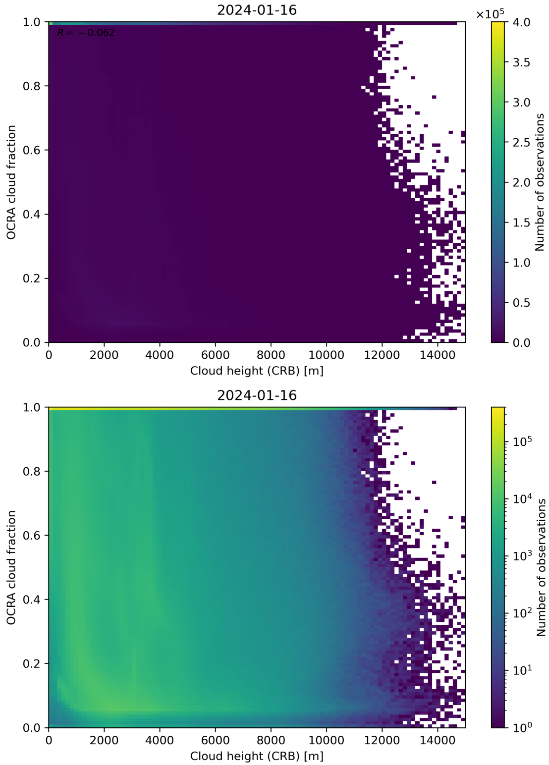
Figure 81: Scatter density plot of “Cloud height (CRB)” against “OCRA cloud fraction” for 2024-01-15 to 2024-01-17.
