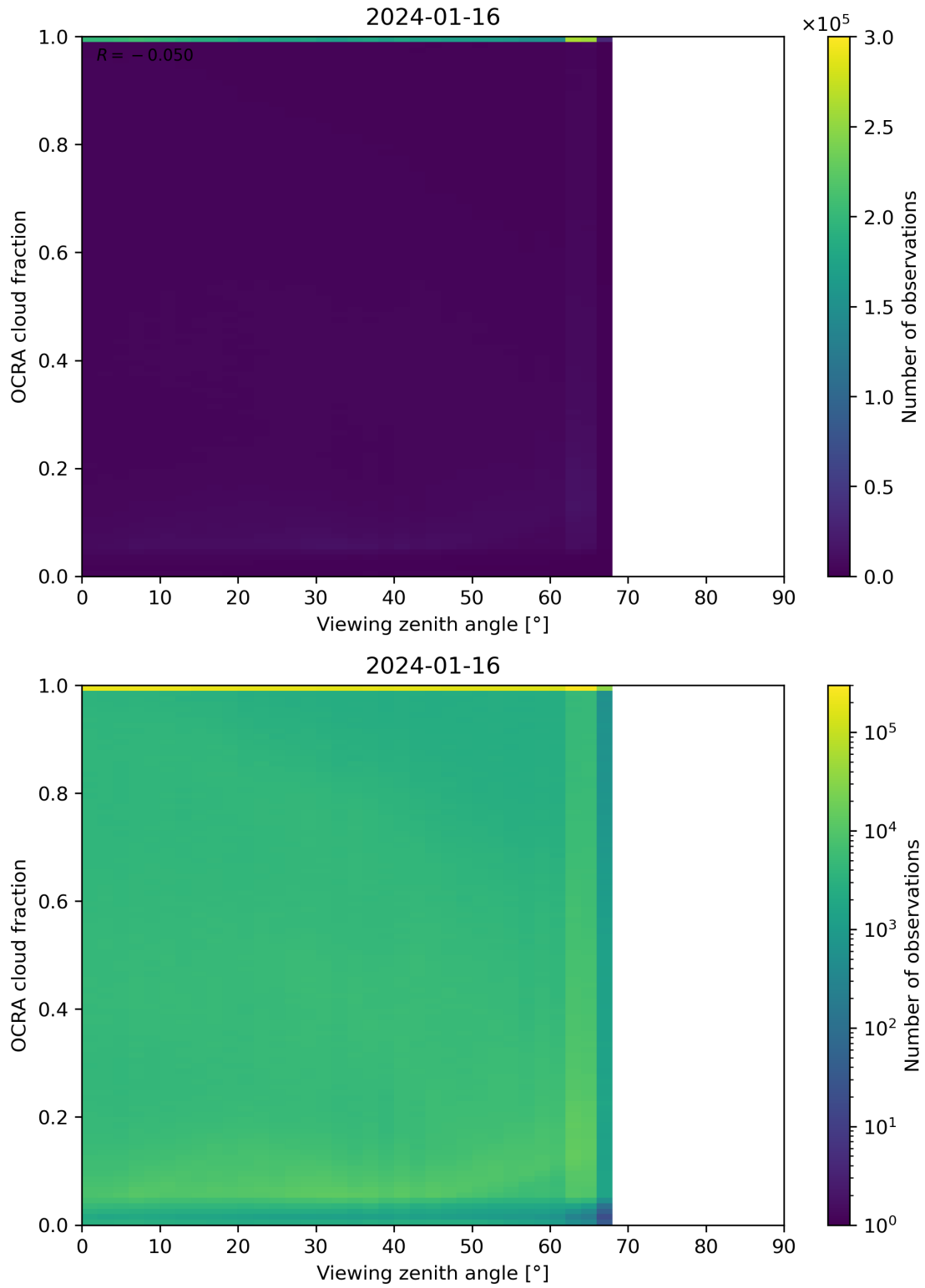
Figure 108: Scatter density plot of “Viewing zenith angle” against “OCRA cloud fraction” for 2024-01-15 to 2024-01-17.
