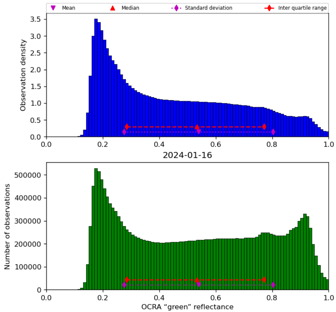
Figure 52: Histogram of “OCRA “green” reflectance” for 2024-01-15 to 2024-01-17
