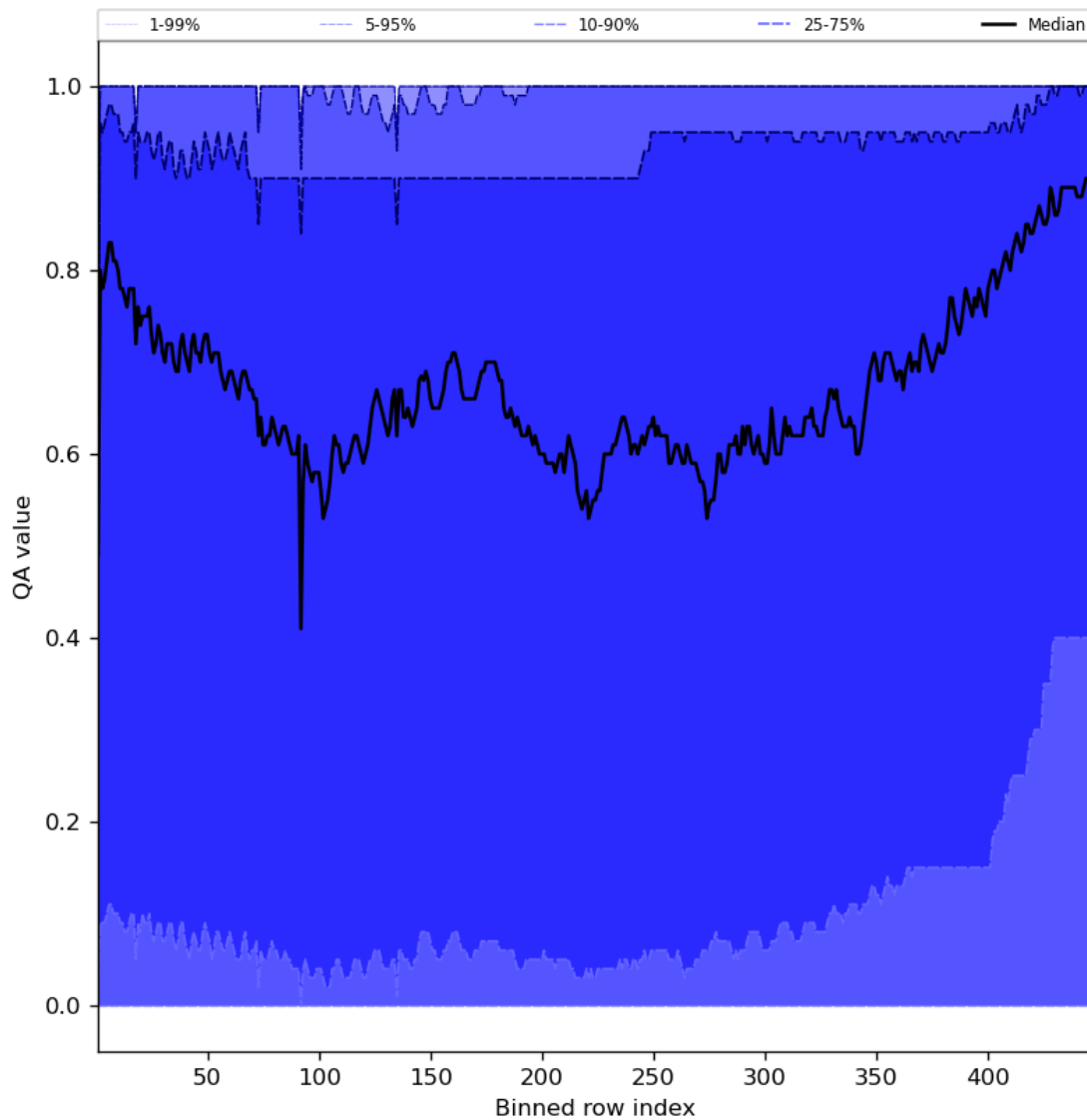
Figure 54: Along track statistics of “QA value” for 2024-01-15 to 2024-01-17
