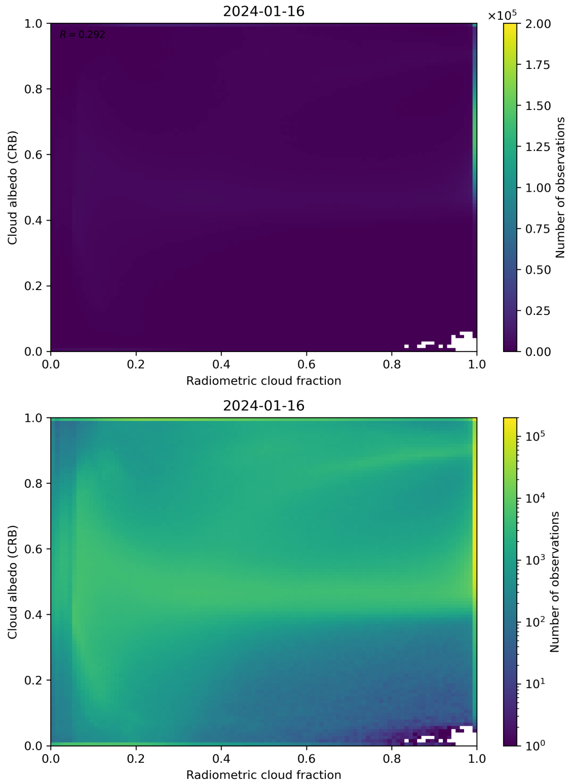
Figure 71: Scatter density plot of “Radiometric cloud fraction” against “Cloud albedo (CRB)” for 2024-01-15 to 2024-01-17.
