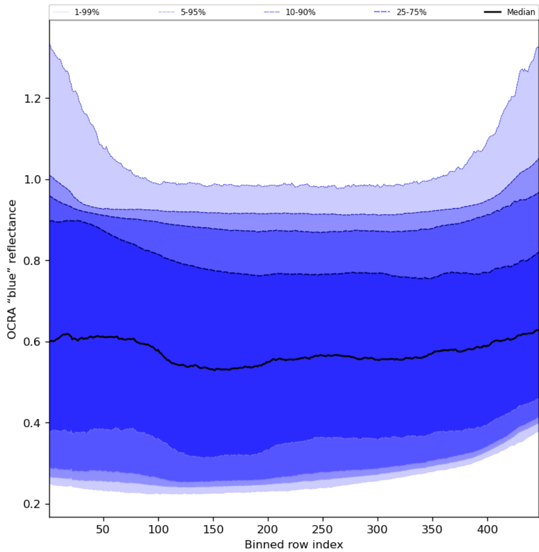
Figure 67: Along track statistics of “OCRA “blue” reflectance” for 2024-01-15 to 2024-01-17
