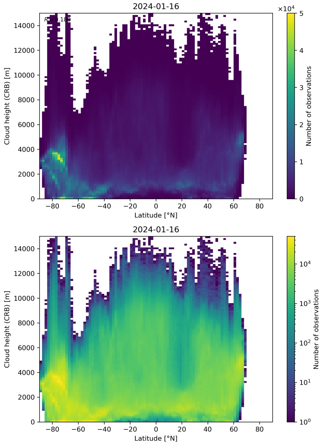
Figure 95: Scatter density plot of “Latitude” against “Cloud height (CRB)” for 2024-01-15 to 2024-01-17.
