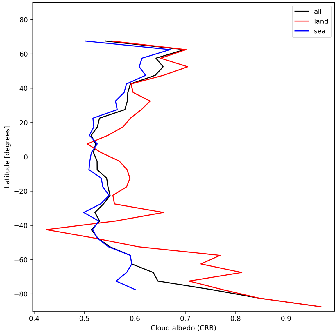
Figure 28: Zonal average of “Cloud albedo (CRB)” for 2024-01-15 to 2024-01-17.
