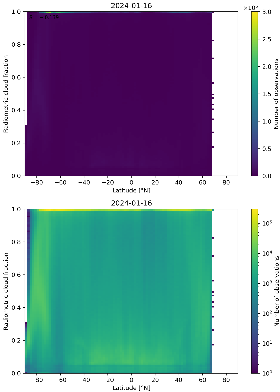
Figure 92: Scatter density plot of “Latitude” against “Radiometric cloud fraction” for 2024-01-15 to 2024-01-17.
