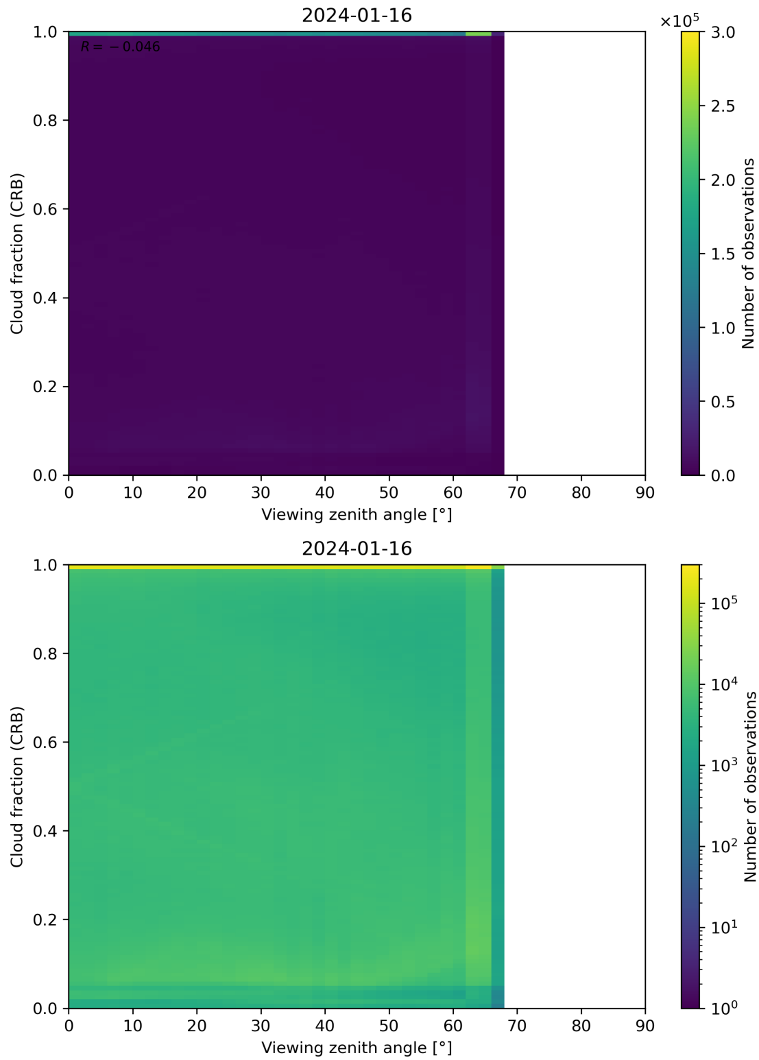
Figure 109: Scatter density plot of “Viewing zenith angle” against “Cloud fraction (CRB)” for 2024-01-15 to 2024-01-17.
