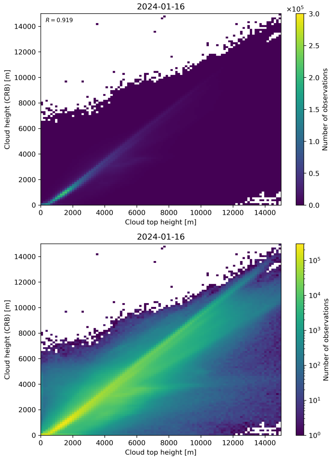
Figure 89: Scatter density plot of “Cloud top height” against “Cloud height (CRB)” for 2024-01-15 to 2024-01-17.
