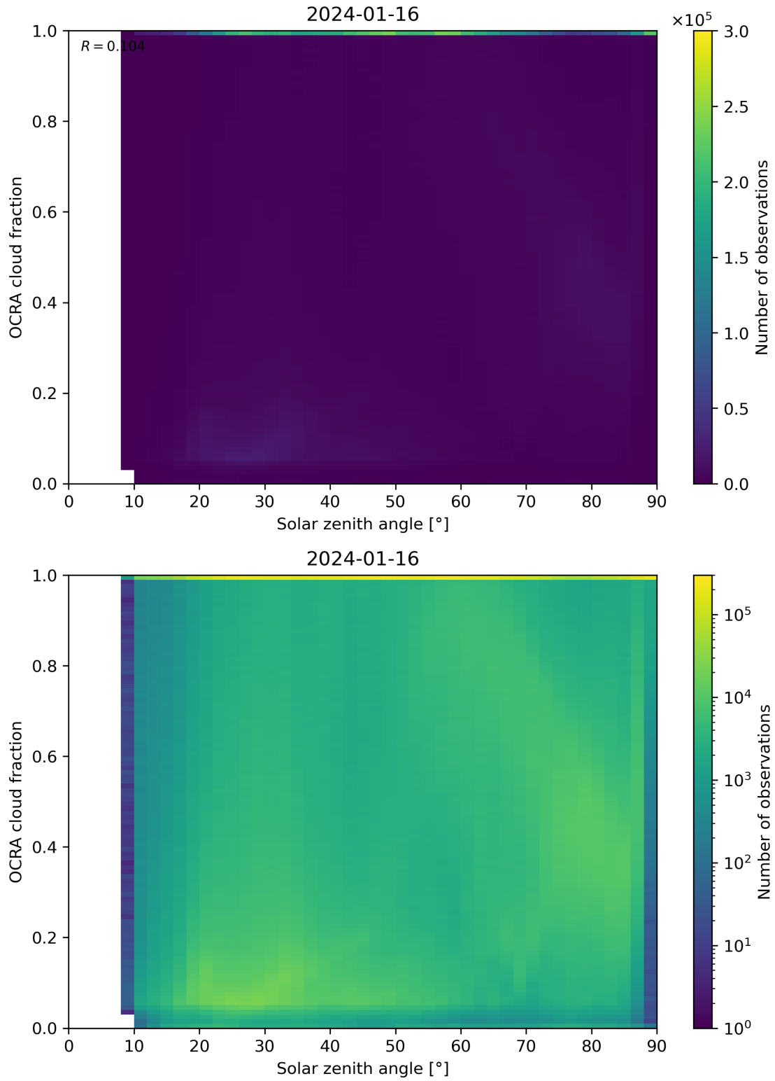
Figure 100: Scatter density plot of “Solar zenith angle” against “OCRA cloud fraction” for 2024-01-15 to 2024-01-17.
