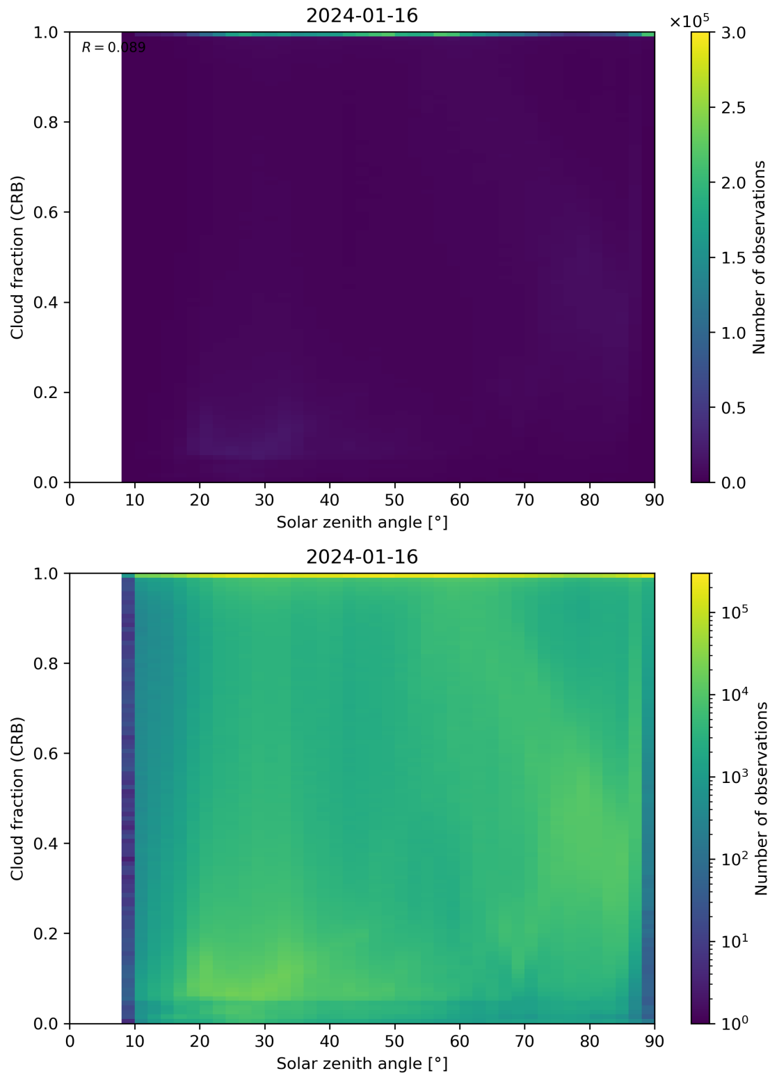
Figure 101: Scatter density plot of “Solar zenith angle” against “Cloud fraction (CRB)” for 2024-01-15 to 2024-01-17.
