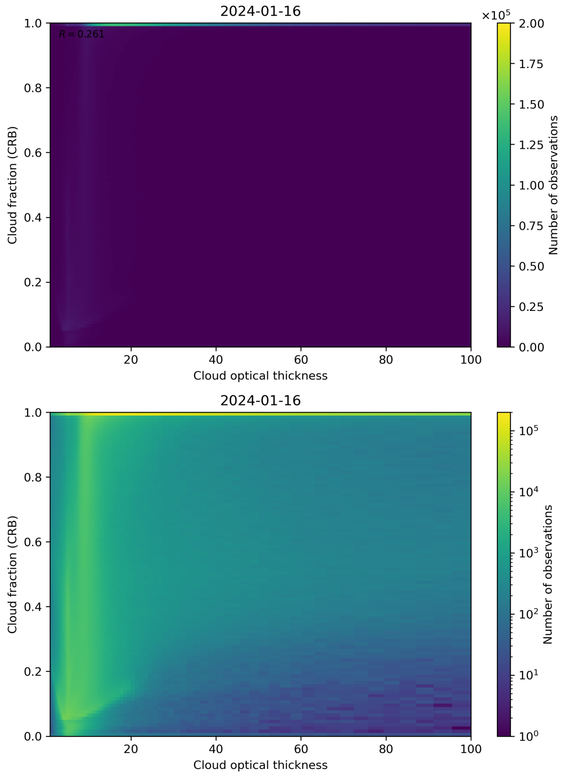
Figure 84: Scatter density plot of “Cloud optical thickness” against “Cloud fraction (CRB)” for 2024-01-15 to 2024-01-17.
