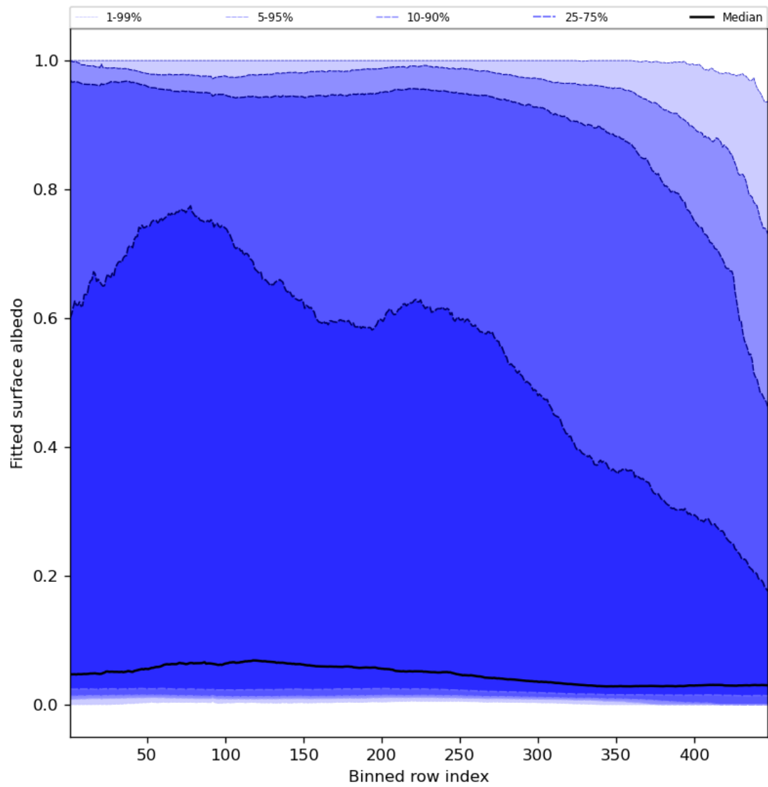
Figure 61: Along track statistics of “Fitted surface albedo” for 2024-01-15 to 2024-01-17
