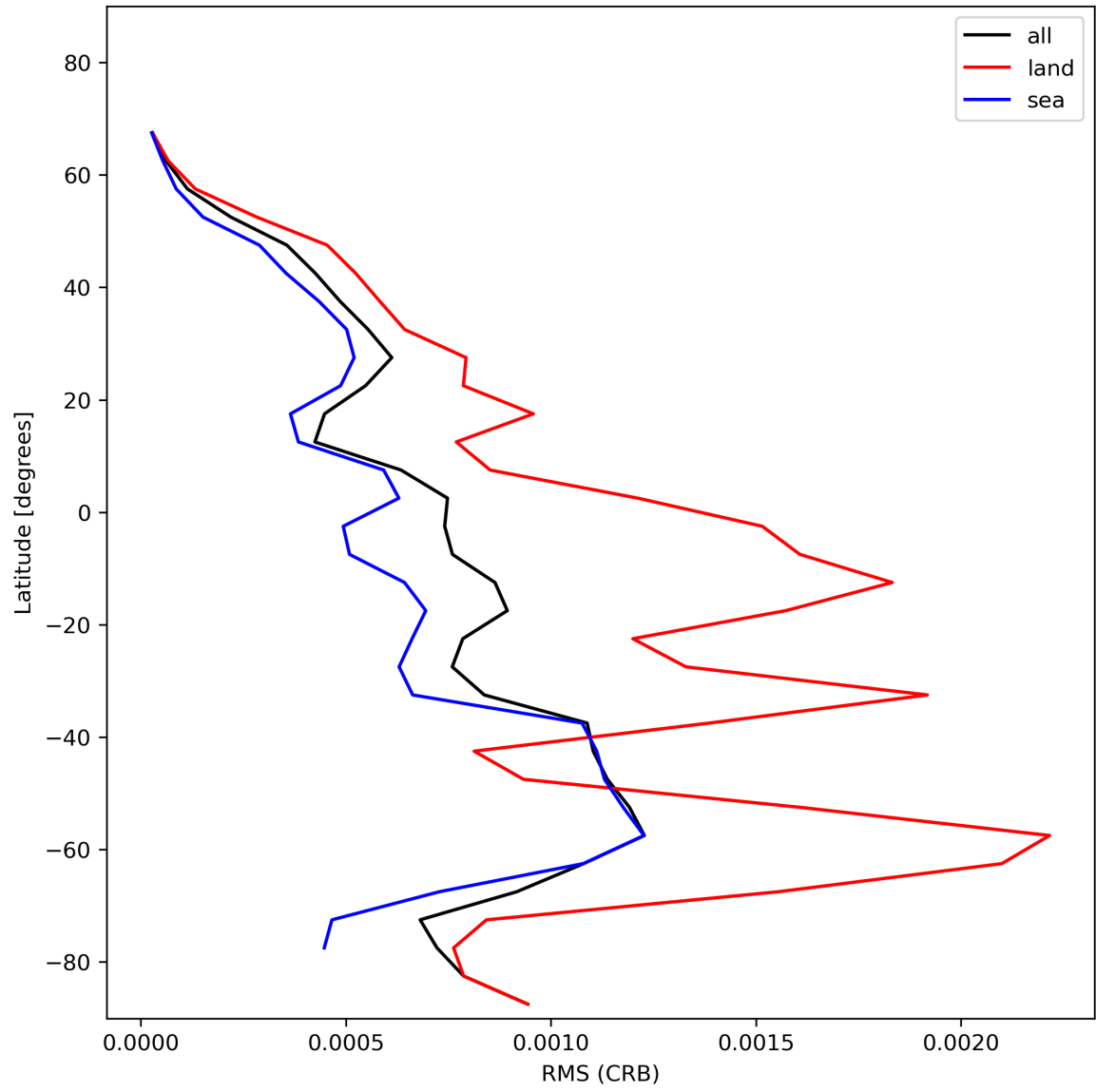
Figure 32: Zonal average of “RMS (CRB)” for 2024-01-15 to 2024-01-17.
