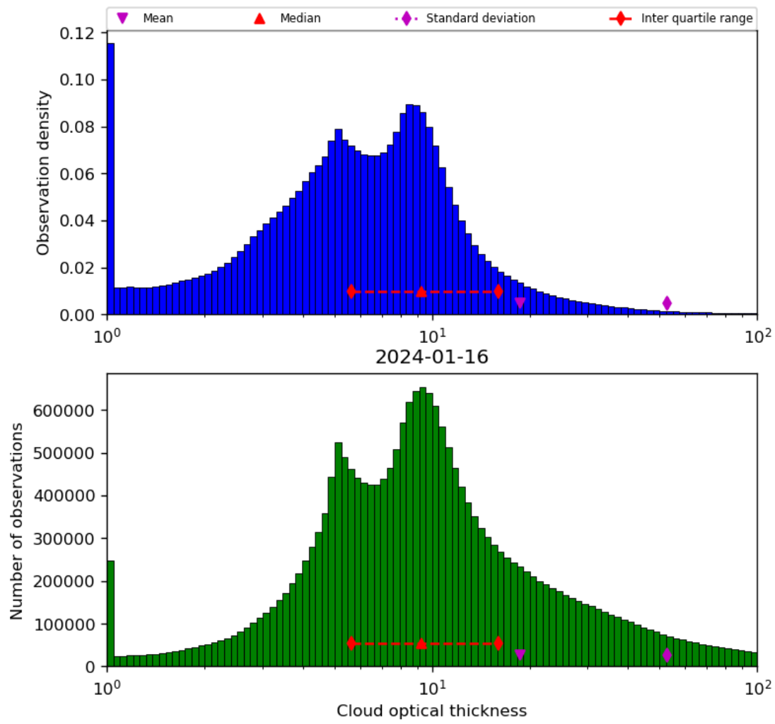
Figure 41: Histogram of “Cloud optical thickness” for 2024-01-15 to 2024-01-17
