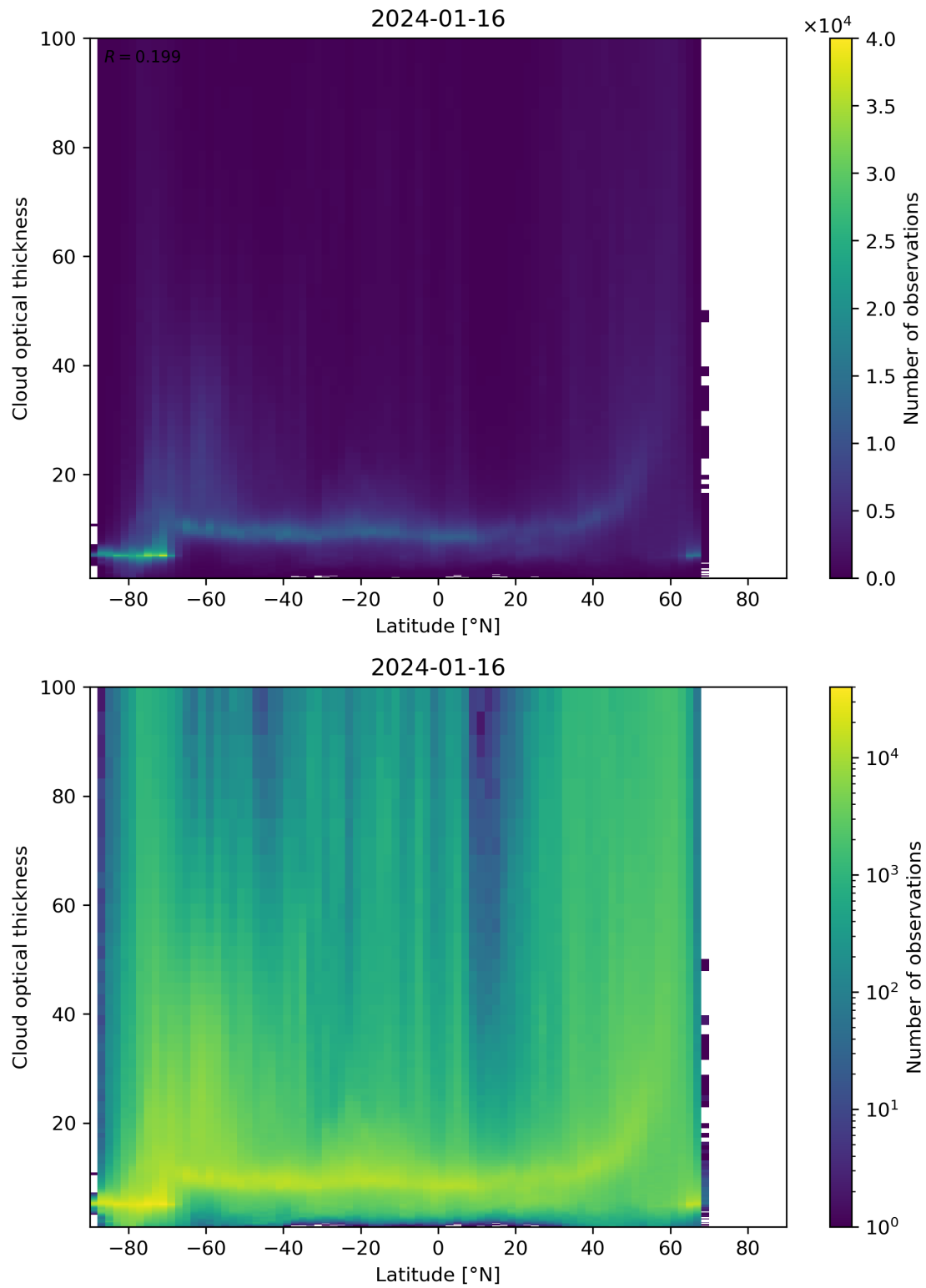
Figure 96: Scatter density plot of “Latitude” against “Cloud optical thickness” for 2024-01-15 to 2024-01-17.
