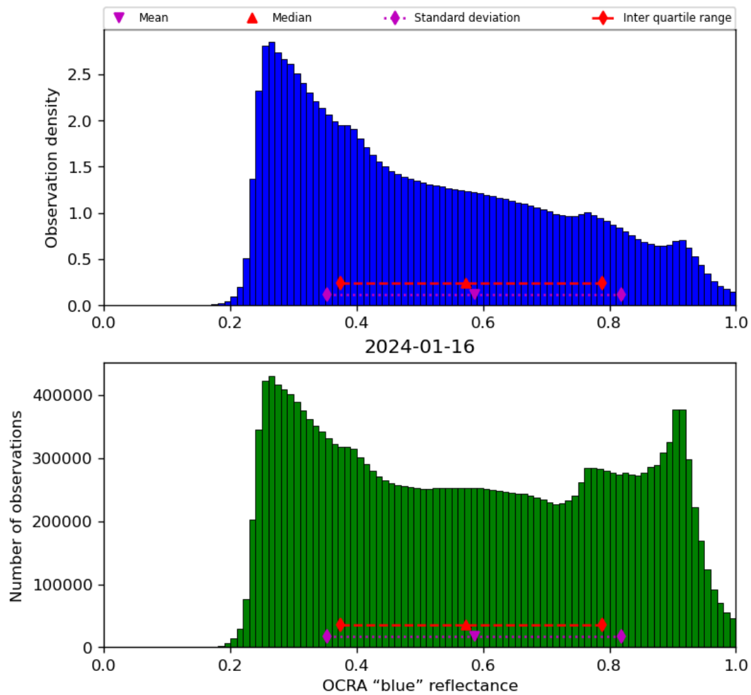
Figure 51: Histogram of “OCRA “blue” reflectance” for 2024-01-15 to 2024-01-17
