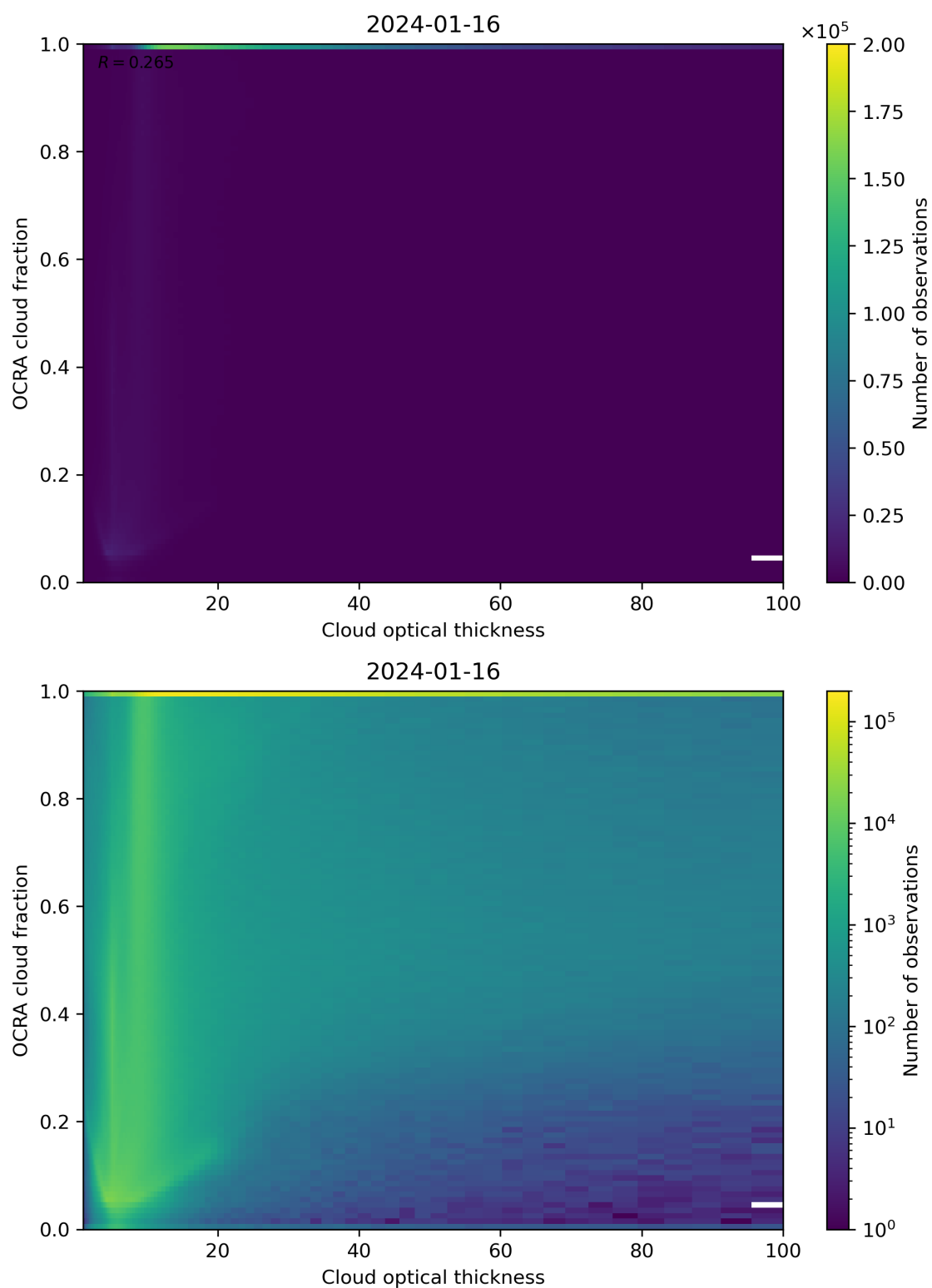
Figure 83: Scatter density plot of “Cloud optical thickness” against “OCRA cloud fraction” for 2024-01-15 to 2024-01-17.
