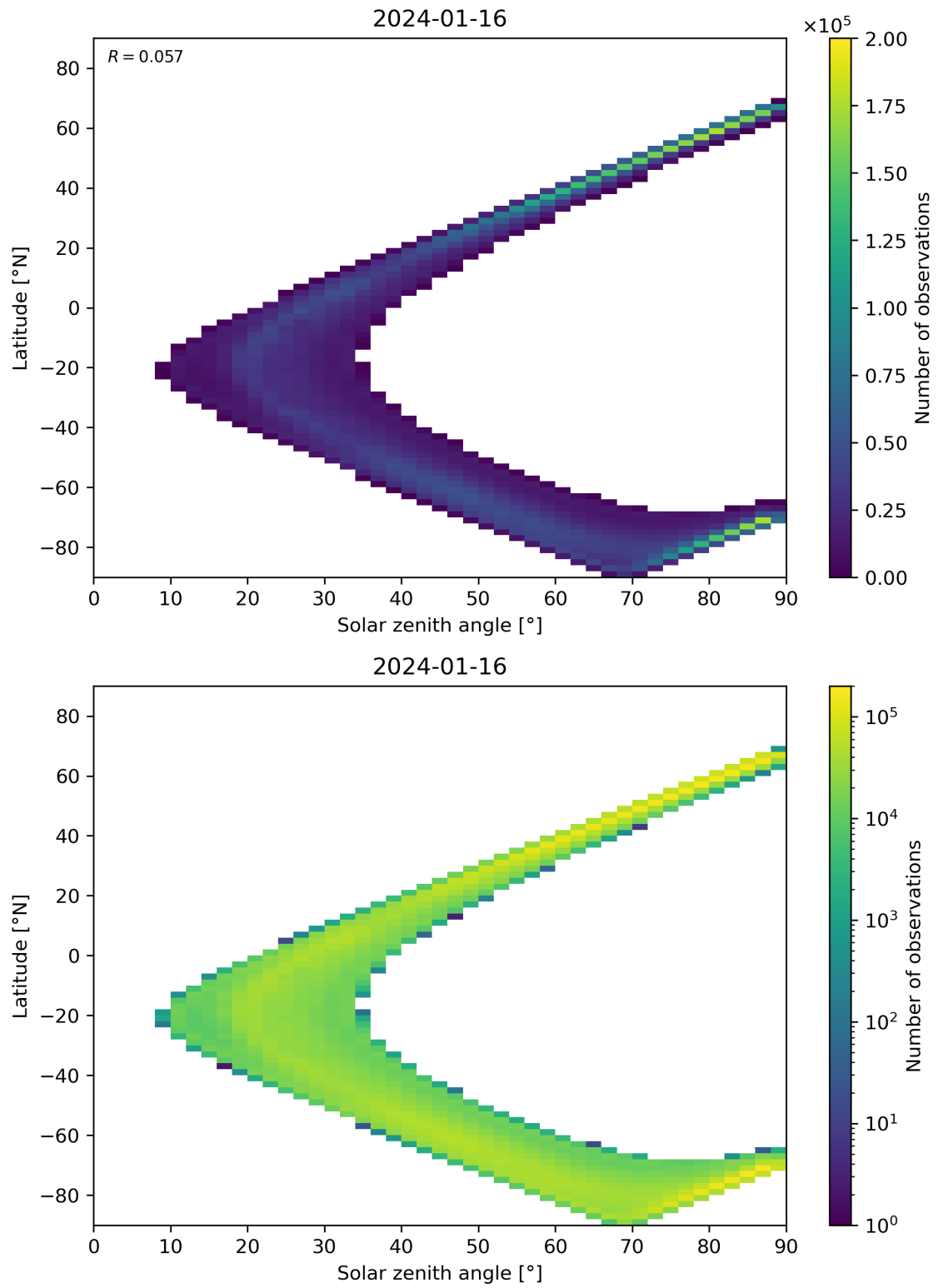
Figure 105: Scatter density plot of “Solar zenith angle” against “Latitude” for 2024-01-15 to 2024-01-17.
