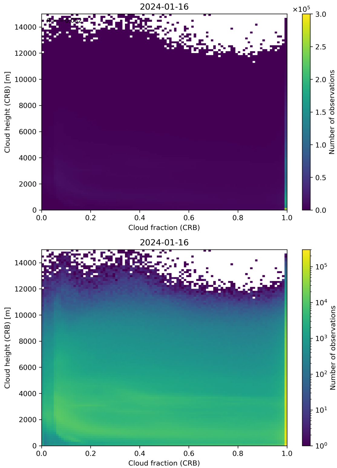
Figure 79: Scatter density plot of “Cloud fraction (CRB)” against “Cloud height (CRB)” for 2024-01-15 to 2024-01-17.
