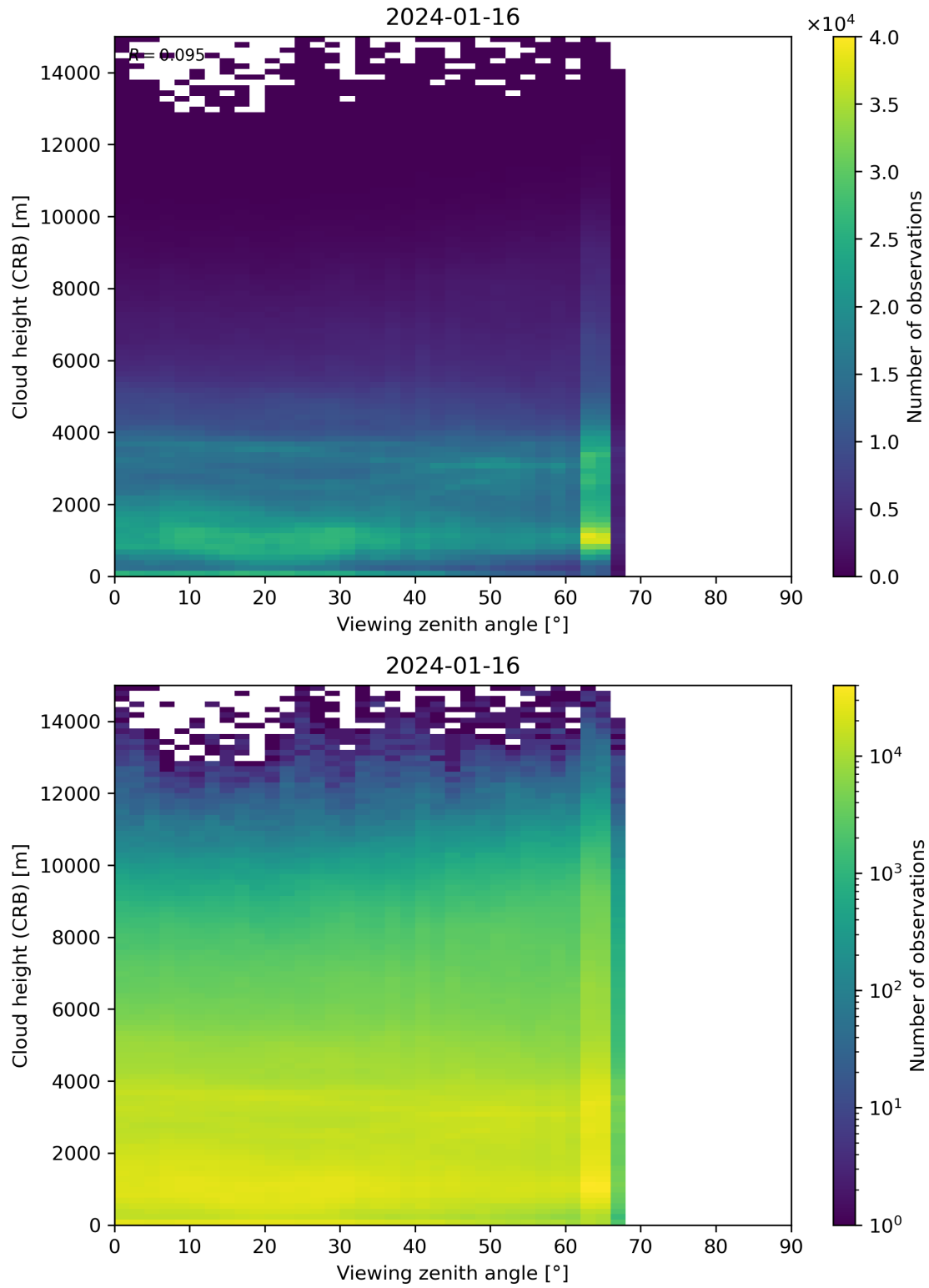
Figure 110: Scatter density plot of “Viewing zenith angle” against “Cloud height (CRB)” for 2024-01-15 to 2024-01-17.
