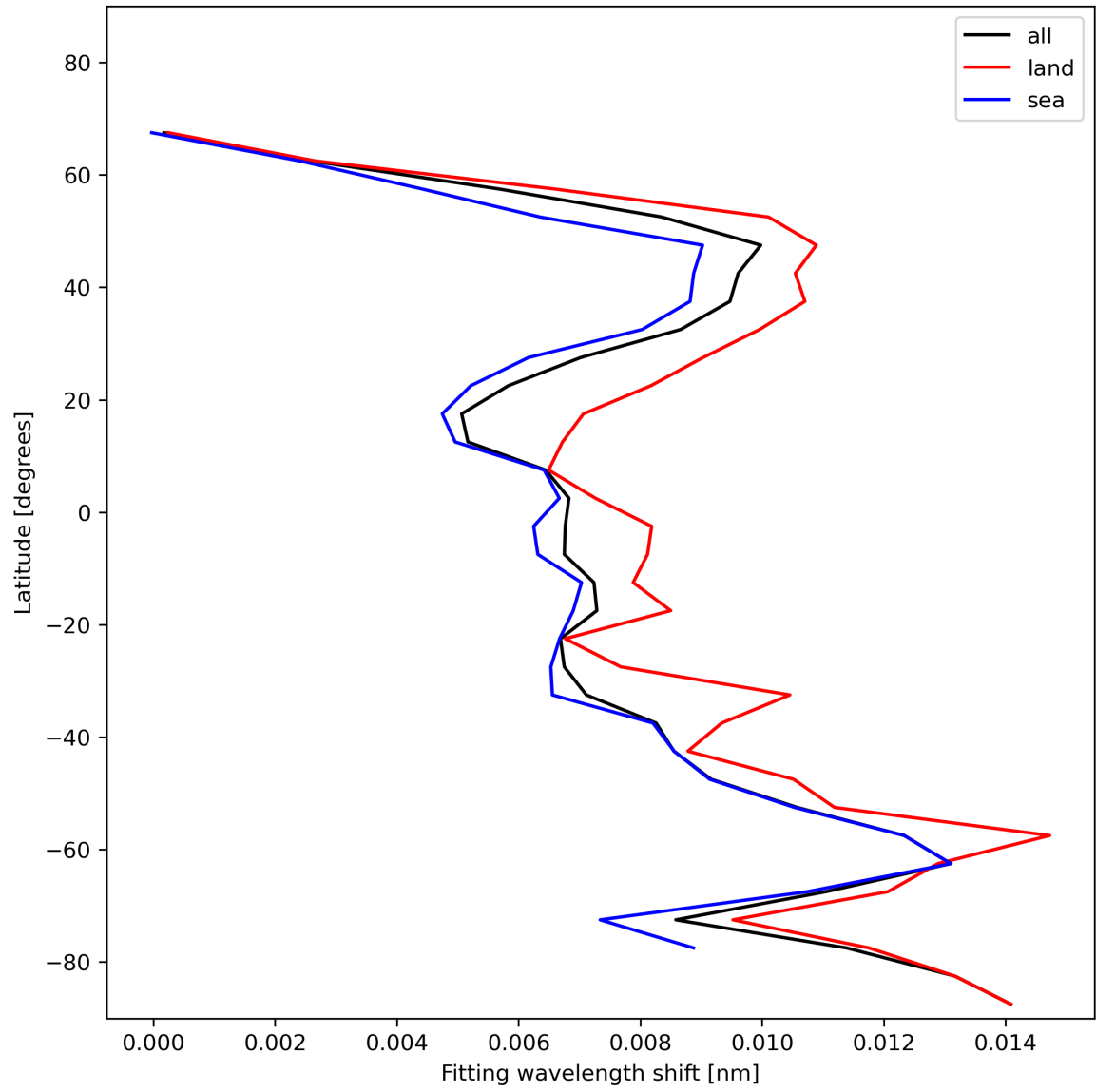
Figure 33: Zonal average of “Fitting wavelength shift” for 2024-01-15 to 2024-01-17.
