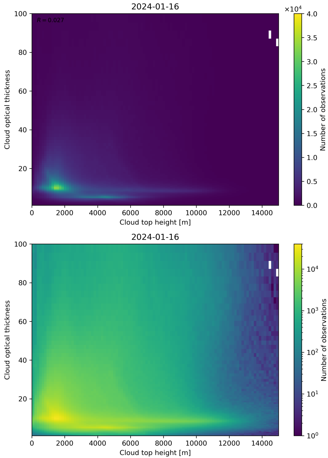
Figure 90: Scatter density plot of “Cloud top height” against “Cloud optical thickness” for 2024-01-15 to 2024-01-17.
