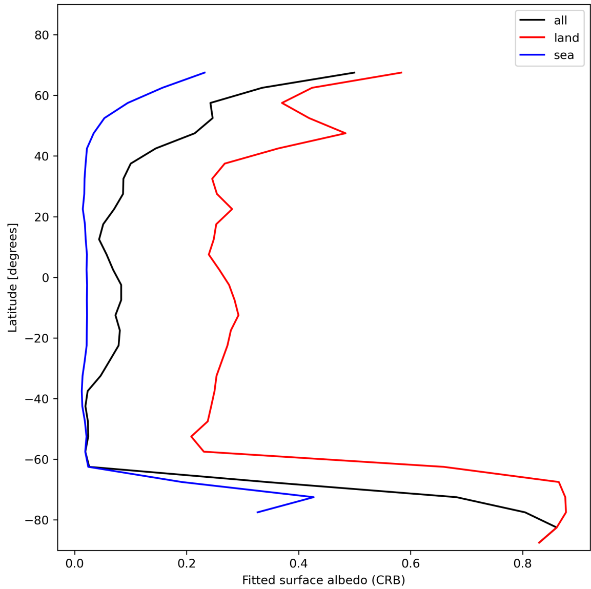
Figure 30: Zonal average of “Fitted surface albedo (CRB)” for 2024-01-15 to 2024-01-17.
