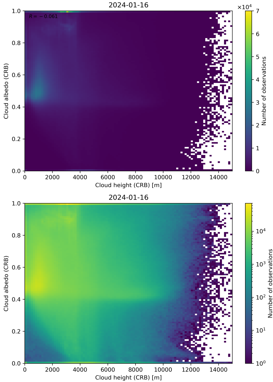
Figure 80: Scatter density plot of “Cloud height (CRB)” against “Cloud albedo (CRB)” for 2024-01-15 to 2024-01-17.
