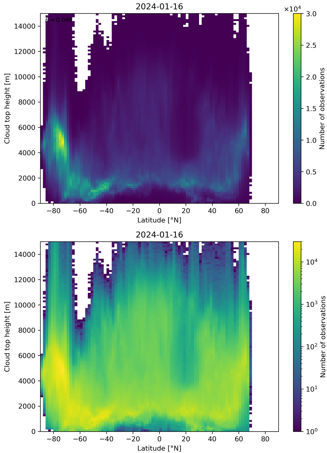
Figure 97: Scatter density plot of “Latitude” against “Cloud top height” for 2024-01-15 to 2024-01-17.
