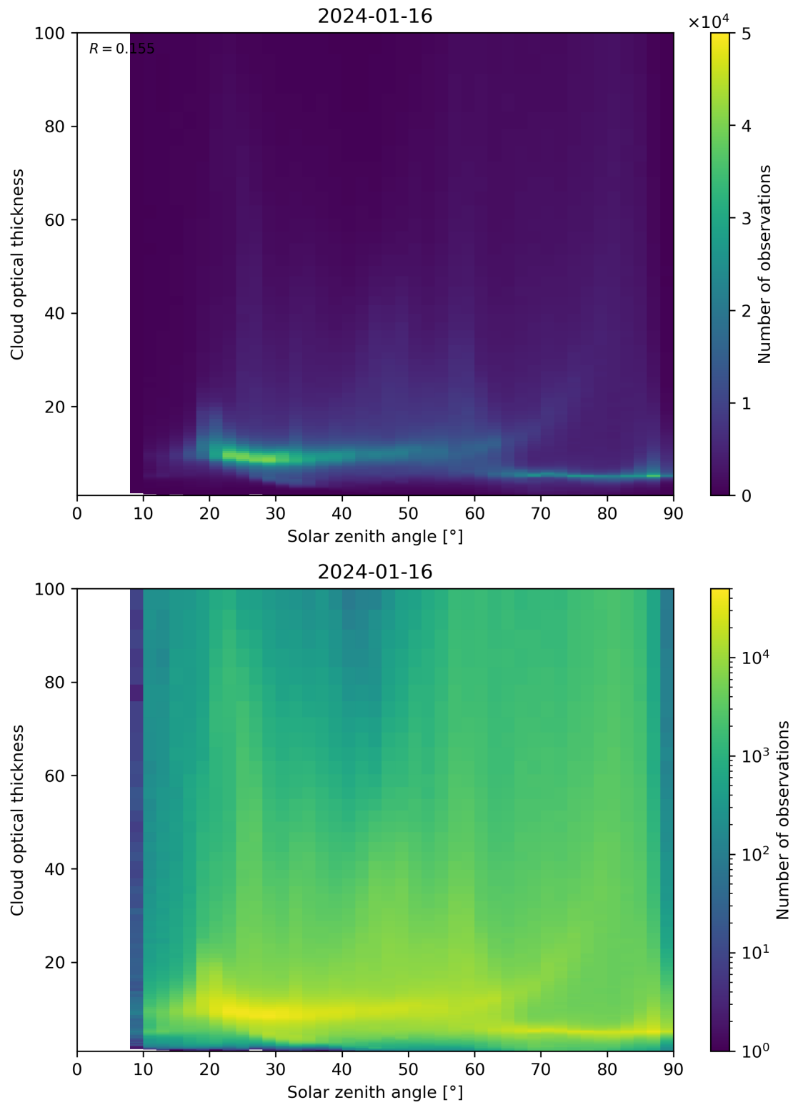
Figure 103: Scatter density plot of “Solar zenith angle” against “Cloud optical thickness” for 2024-01-15 to 2024-01-17.
