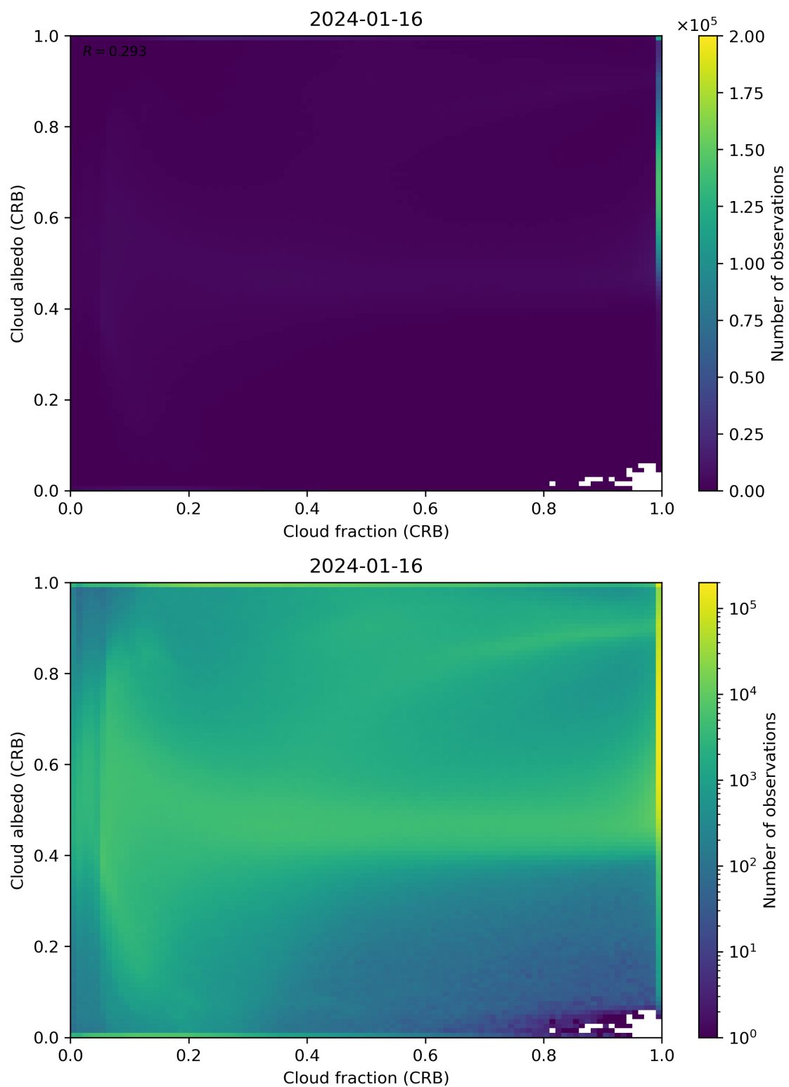
Figure 77: Scatter density plot of “Cloud fraction (CRB)” against “Cloud albedo (CRB)” for 2024-01-15 to 2024-01-17.
