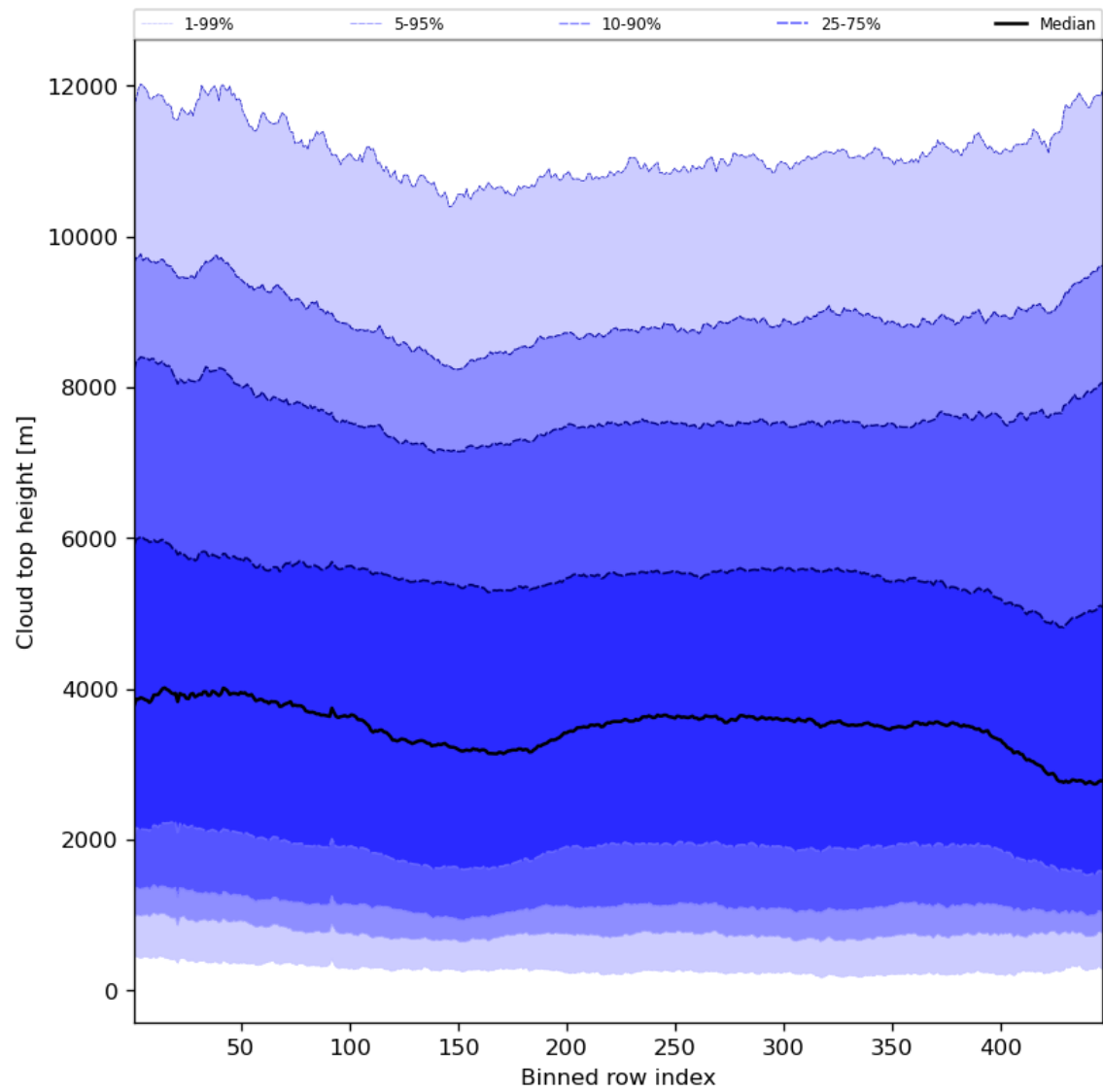
Figure 56: Along track statistics of “Cloud top height” for 2024-01-15 to 2024-01-17
