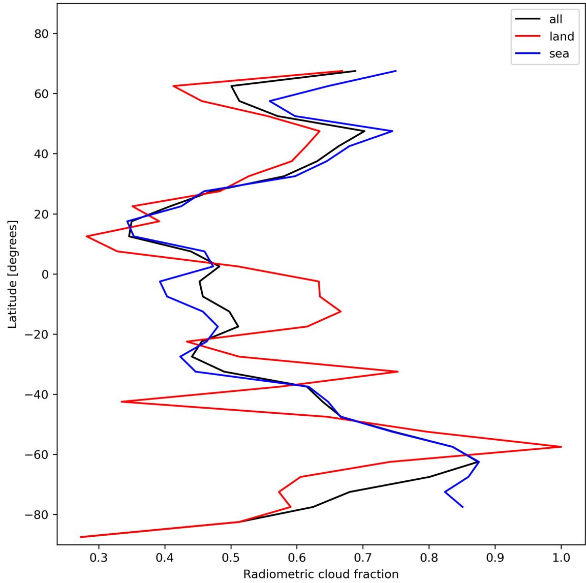
Figure 23: Zonal average of “Radiometric cloud fraction” for 2024-01-15 to 2024-01-17.
