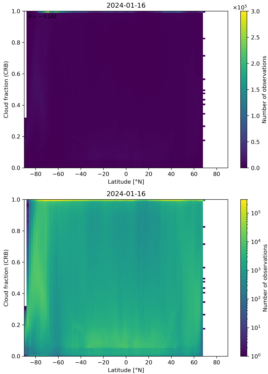
Figure 94: Scatter density plot of “Latitude” against “Cloud fraction (CRB)” for 2024-01-15 to 2024-01-17.
