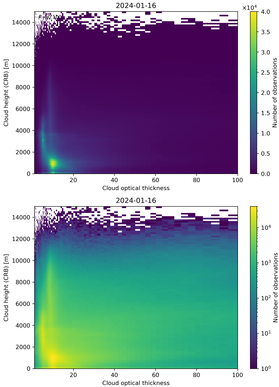
Figure 85: Scatter density plot of “Cloud optical thickness” against “Cloud height (CRB)” for 2024-01-15 to 2024-01-17.
