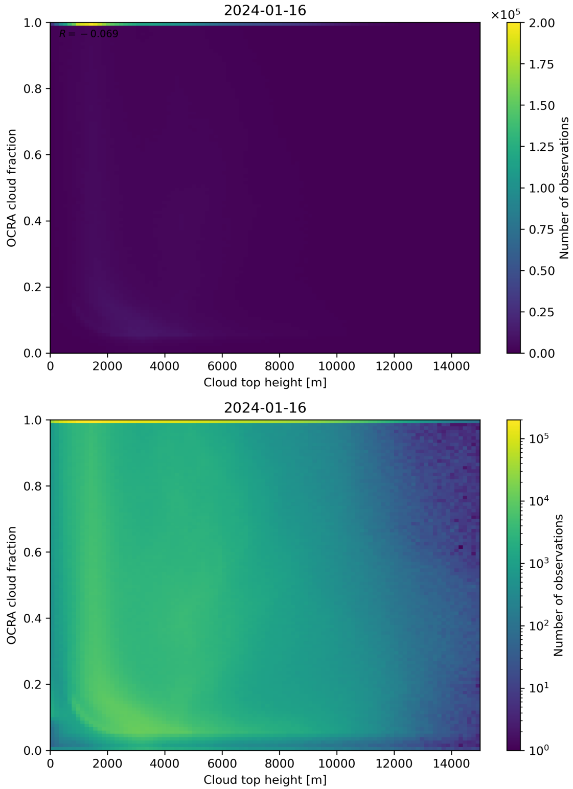
Figure 87: Scatter density plot of “Cloud top height” against “OCRA cloud fraction” for 2024-01-15 to 2024-01-17.
