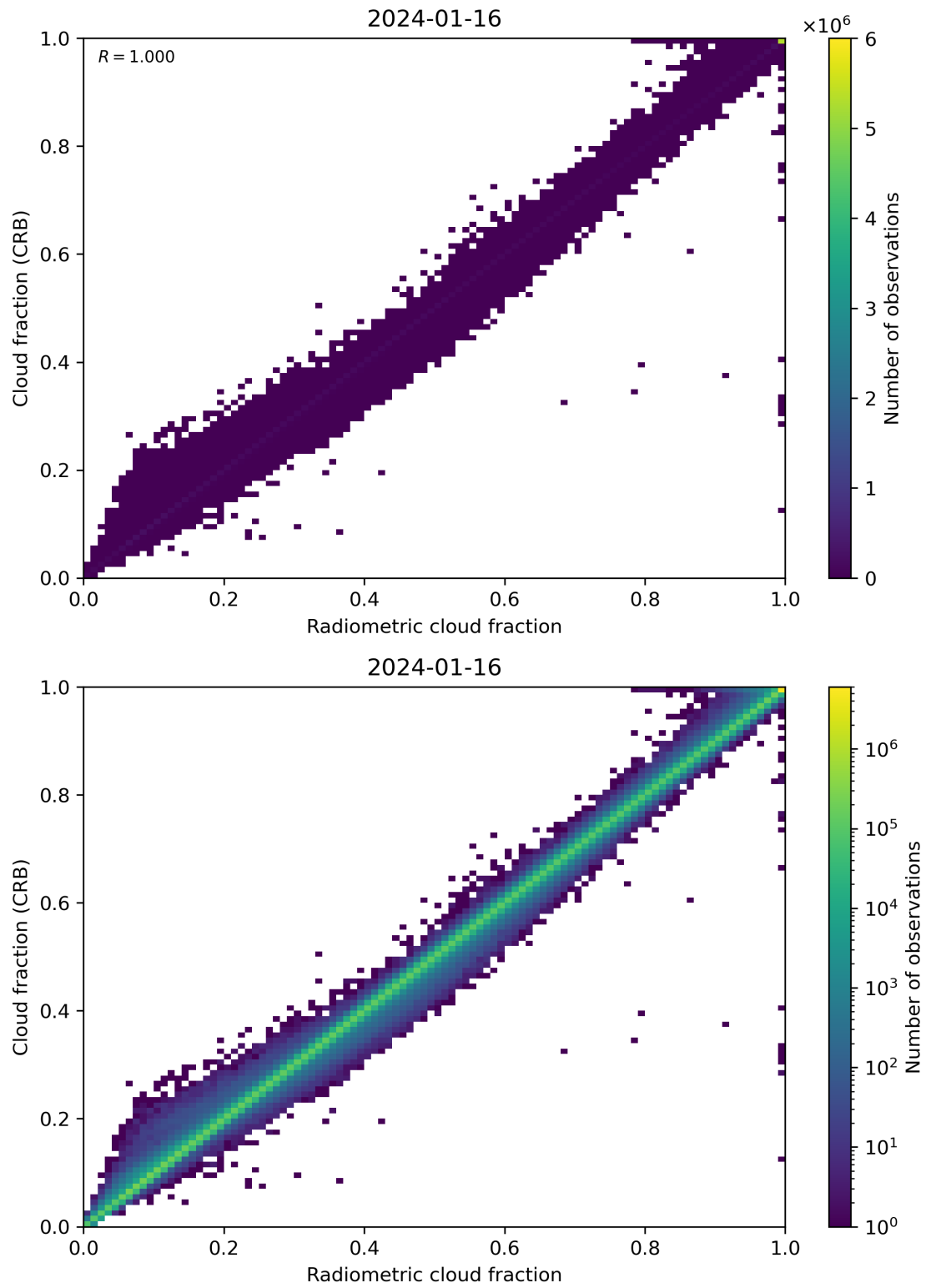
Figure 73: Scatter density plot of “Radiometric cloud fraction” against “Cloud fraction (CRB)” for 2024-01-15 to 2024-01-17.
