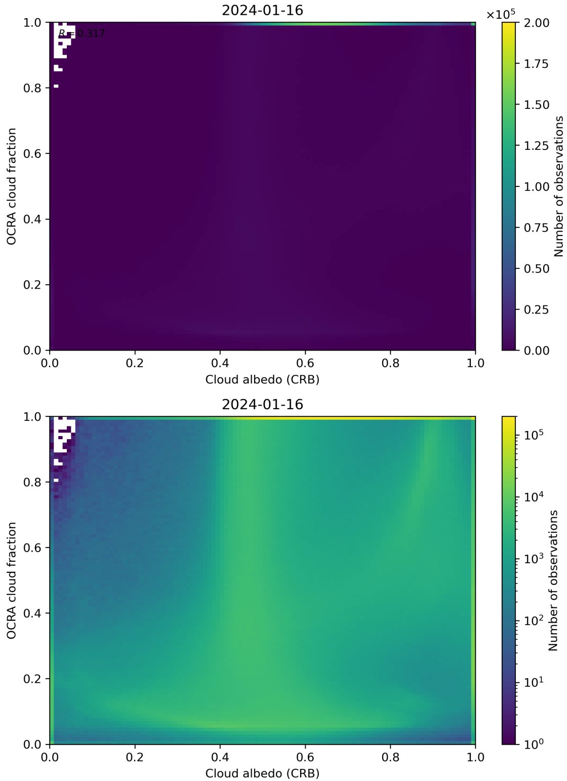
Figure 70: Scatter density plot of “Cloud albedo (CRB)” against “OCRA cloud fraction” for 2024-01-15 to 2024-01-17.
