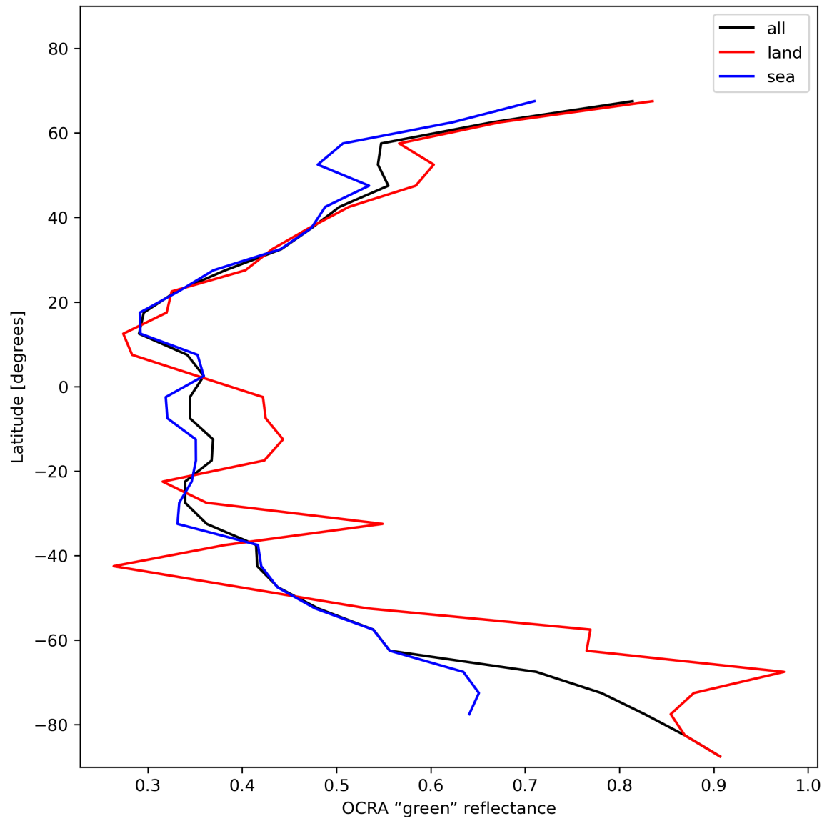
Figure 36: Zonal average of “OCRA “green” reflectance” for 2024-01-15 to 2024-01-17.
