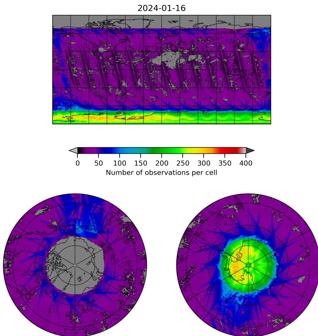
Figure 21: Map of the number of observations for 2024-01-15 to 2024-01-17
