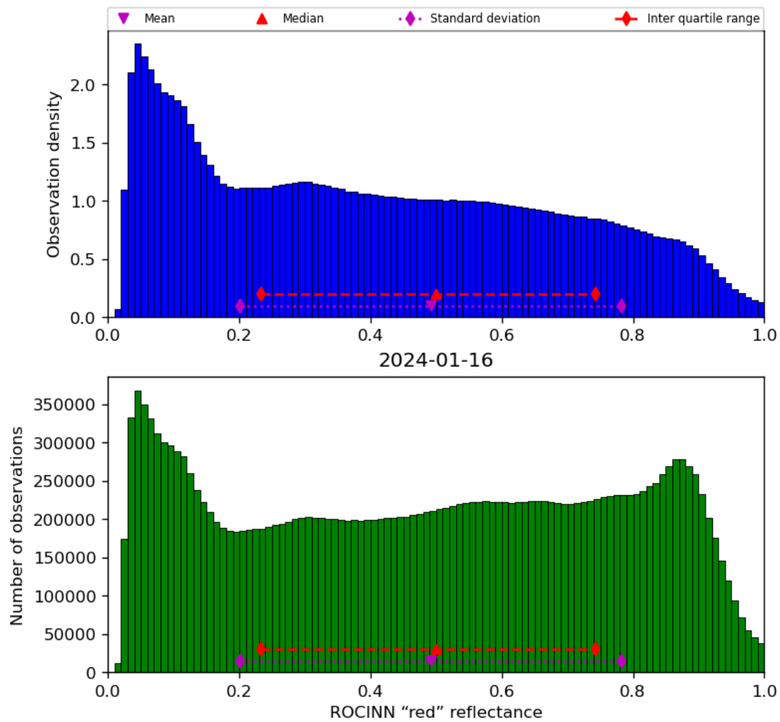
Figure 53: Histogram of “ROCINN “red” reflectance” for 2024-01-15 to 2024-01-17
