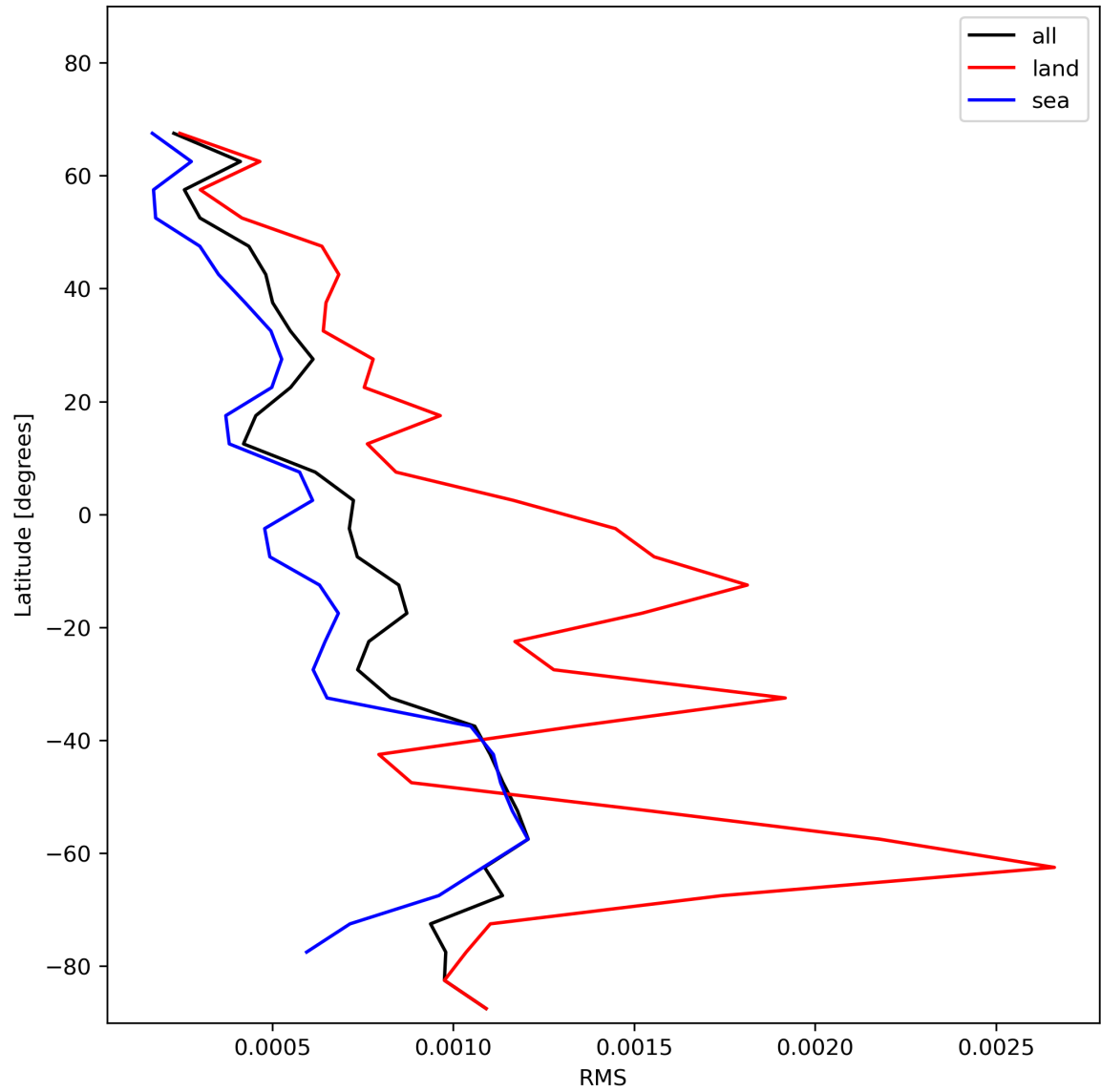
Figure 31: Zonal average of “RMS” for 2024-01-15 to 2024-01-17.
