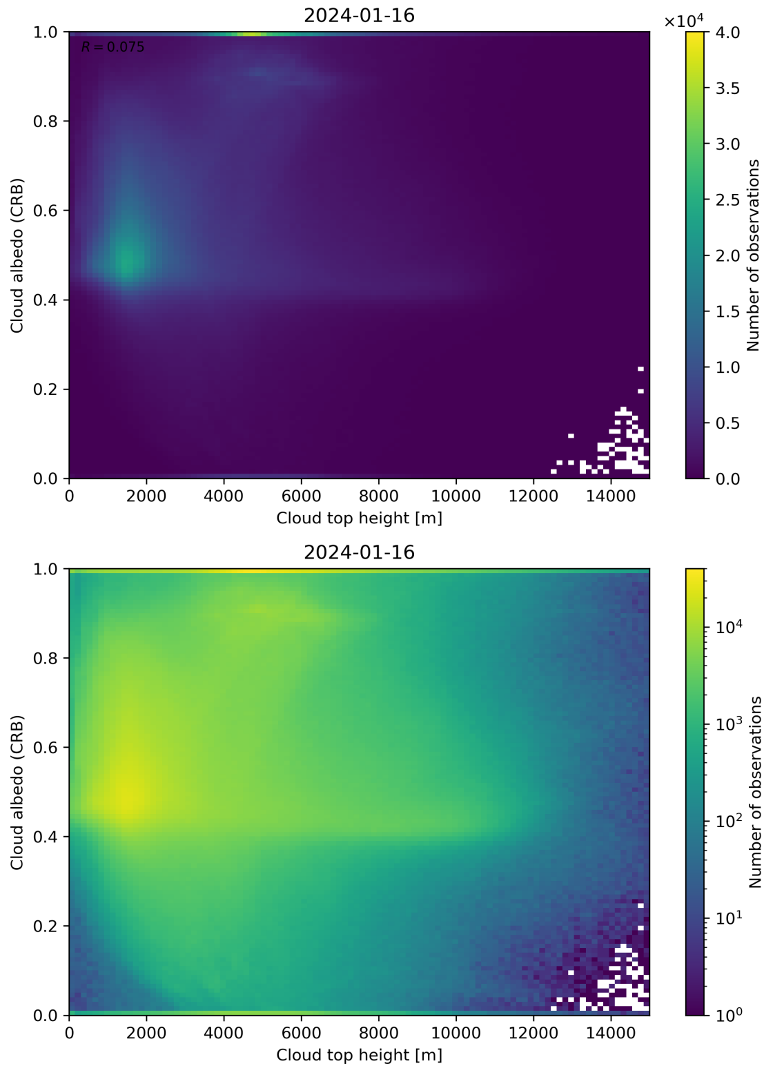
Figure 86: Scatter density plot of “Cloud top height” against “Cloud albedo (CRB)” for 2024-01-15 to 2024-01-17.
