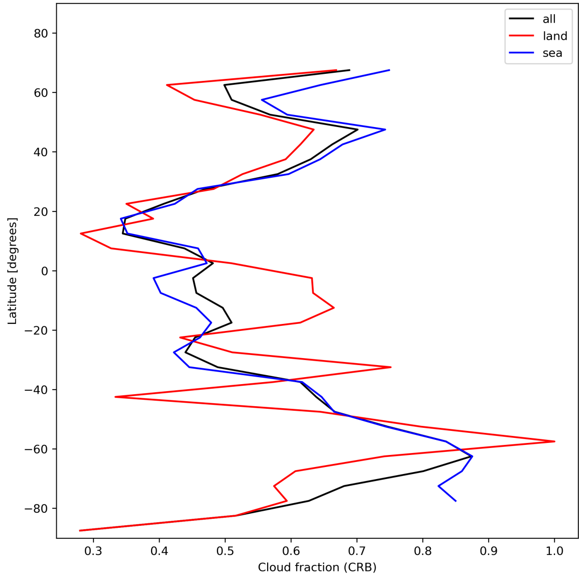
Figure 26: Zonal average of “Cloud fraction (CRB)” for 2024-01-15 to 2024-01-17.
