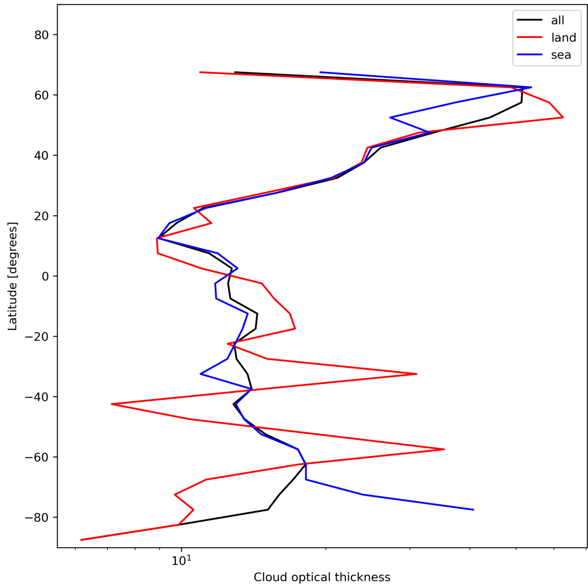
Figure 25: Zonal average of “Cloud optical thickness” for 2024-01-15 to 2024-01-17.
