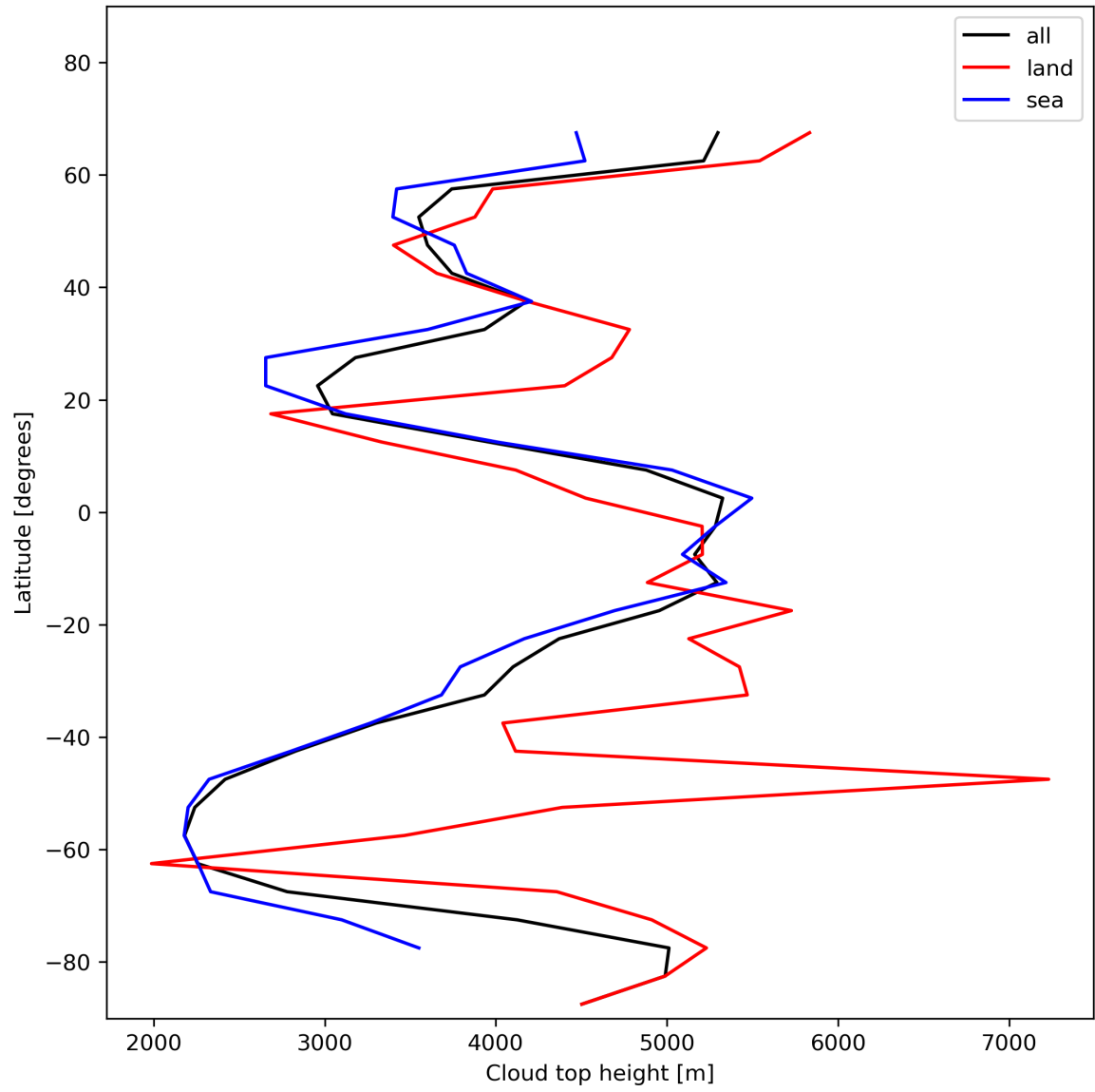
Figure 24: Zonal average of “Cloud top height” for 2024-01-15 to 2024-01-17.
