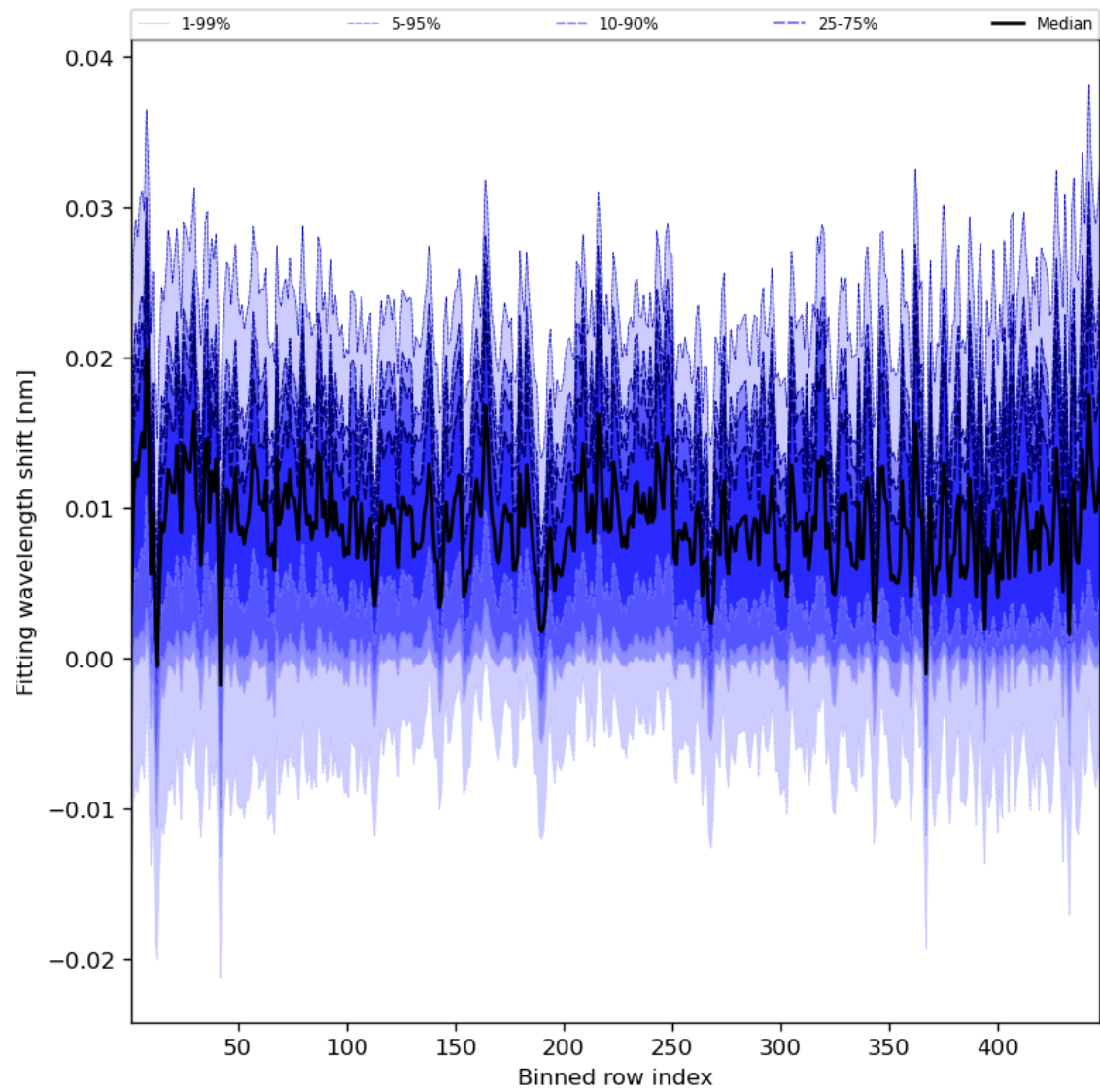
Figure 65: Along track statistics of “Fitting wavelength shift” for 2024-01-15 to 2024-01-17
