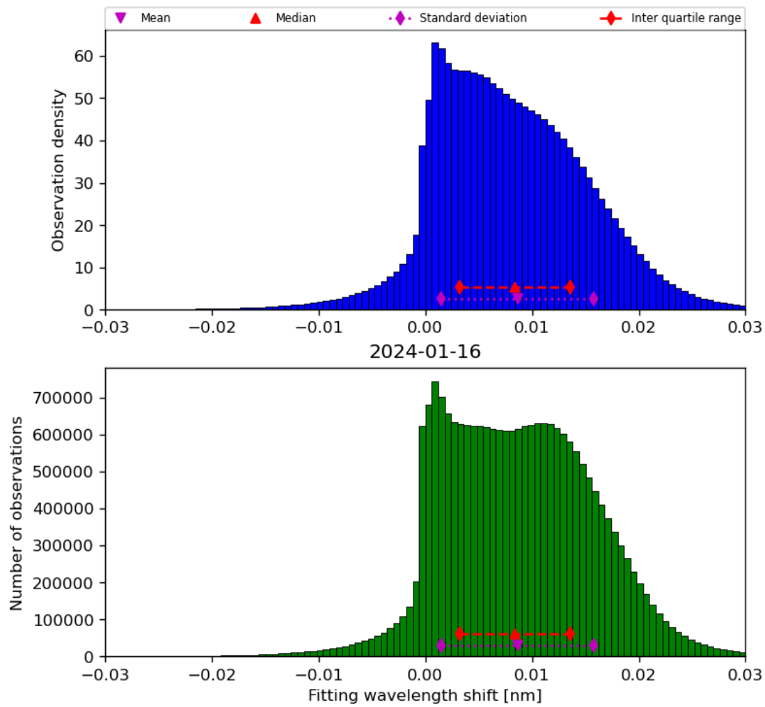
Figure 49: Histogram of “Fitting wavelength shift” for 2024-01-15 to 2024-01-17
