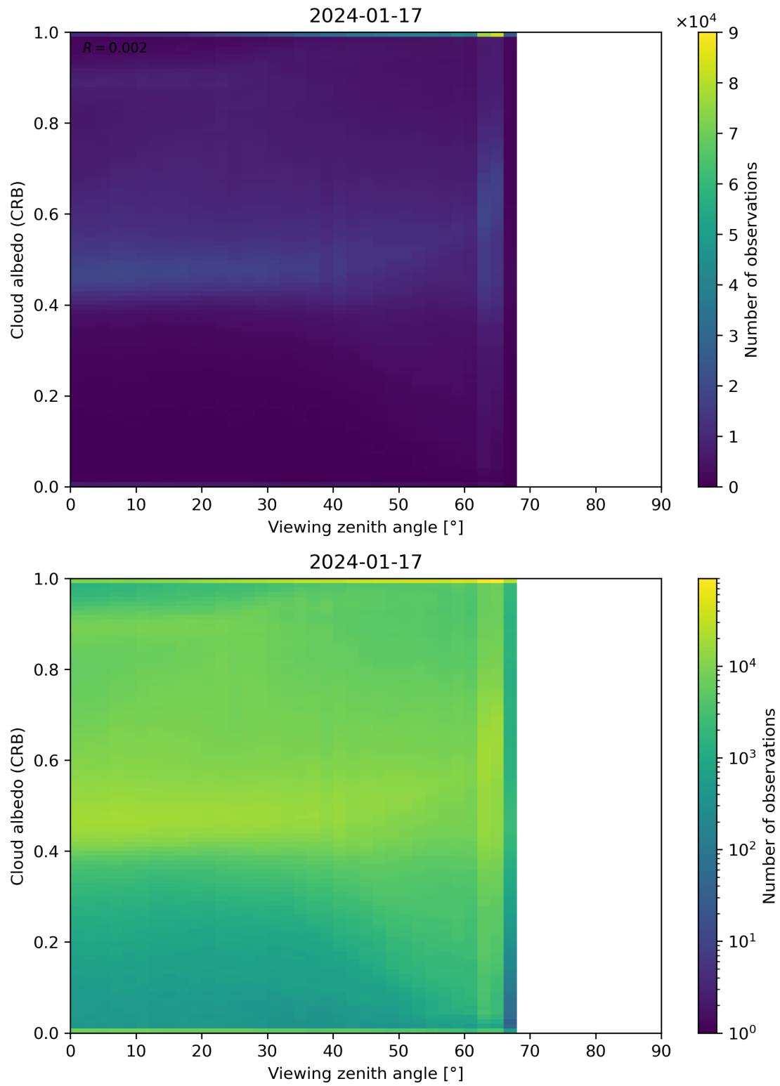
Figure 106: Scatter density plot of “Viewing zenith angle” against “Cloud albedo (CRB)” for 2024-01-16 to 2024-01-18.
