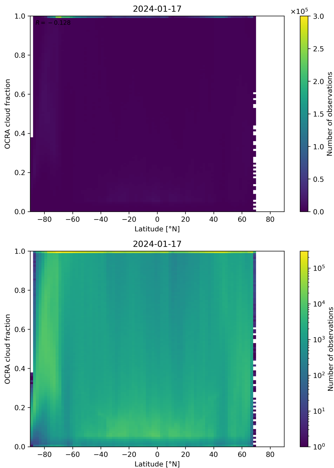
Figure 93: Scatter density plot of “Latitude” against “OCRA cloud fraction” for 2024-01-16 to 2024-01-18.
