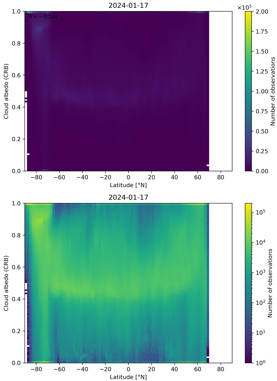
Figure 91: Scatter density plot of “Latitude” against “Cloud albedo (CRB)” for 2024-01-16 to 2024-01-18.
