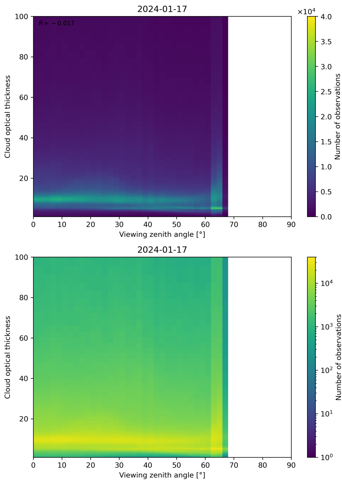
Figure 111: Scatter density plot of “Viewing zenith angle” against “Cloud optical thickness” for 2024-01-16 to 2024-01-18.
