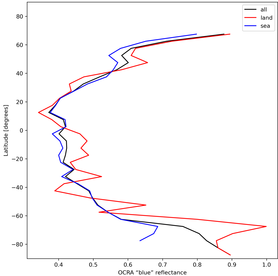
Figure 35: Zonal average of “OCRA “blue” reflectance” for 2024-01-16 to 2024-01-18.
