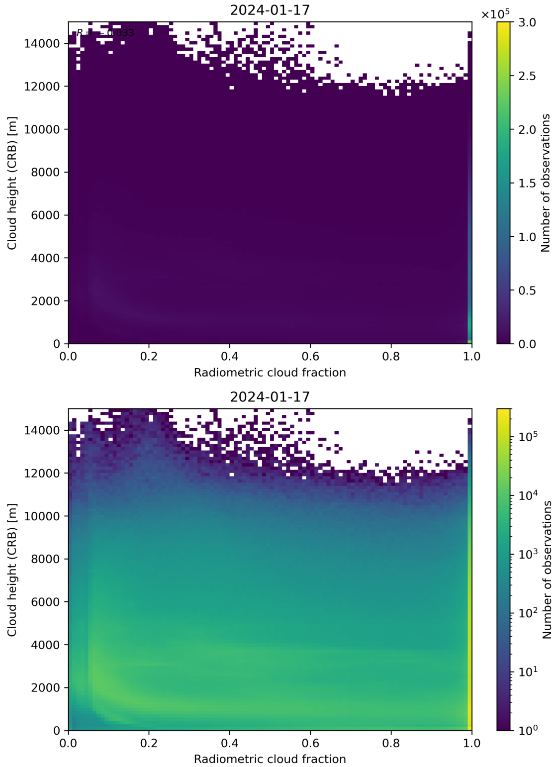
Figure 74: Scatter density plot of “Radiometric cloud fraction” against “Cloud height (CRB)” for 2024-01-16 to 2024-01-18.
