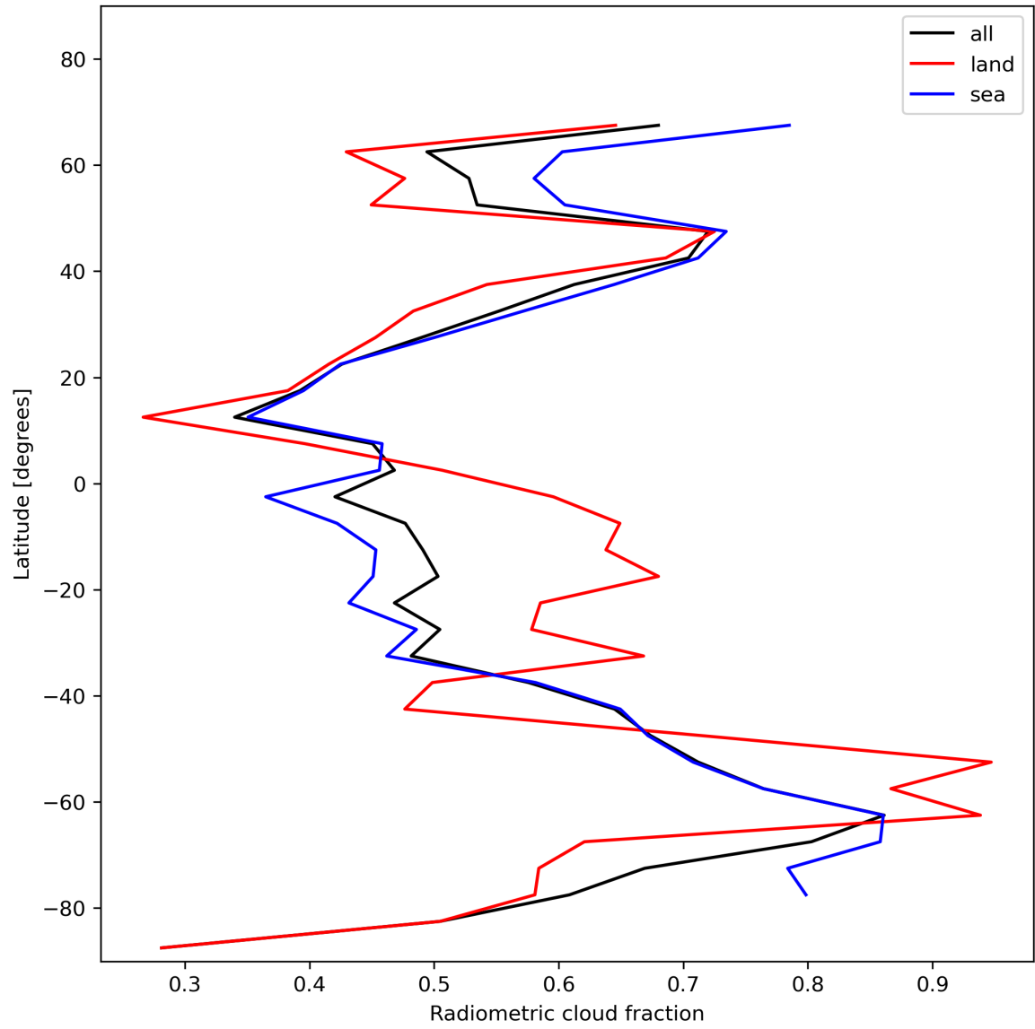
Figure 23: Zonal average of “Radiometric cloud fraction” for 2024-01-16 to 2024-01-18.
