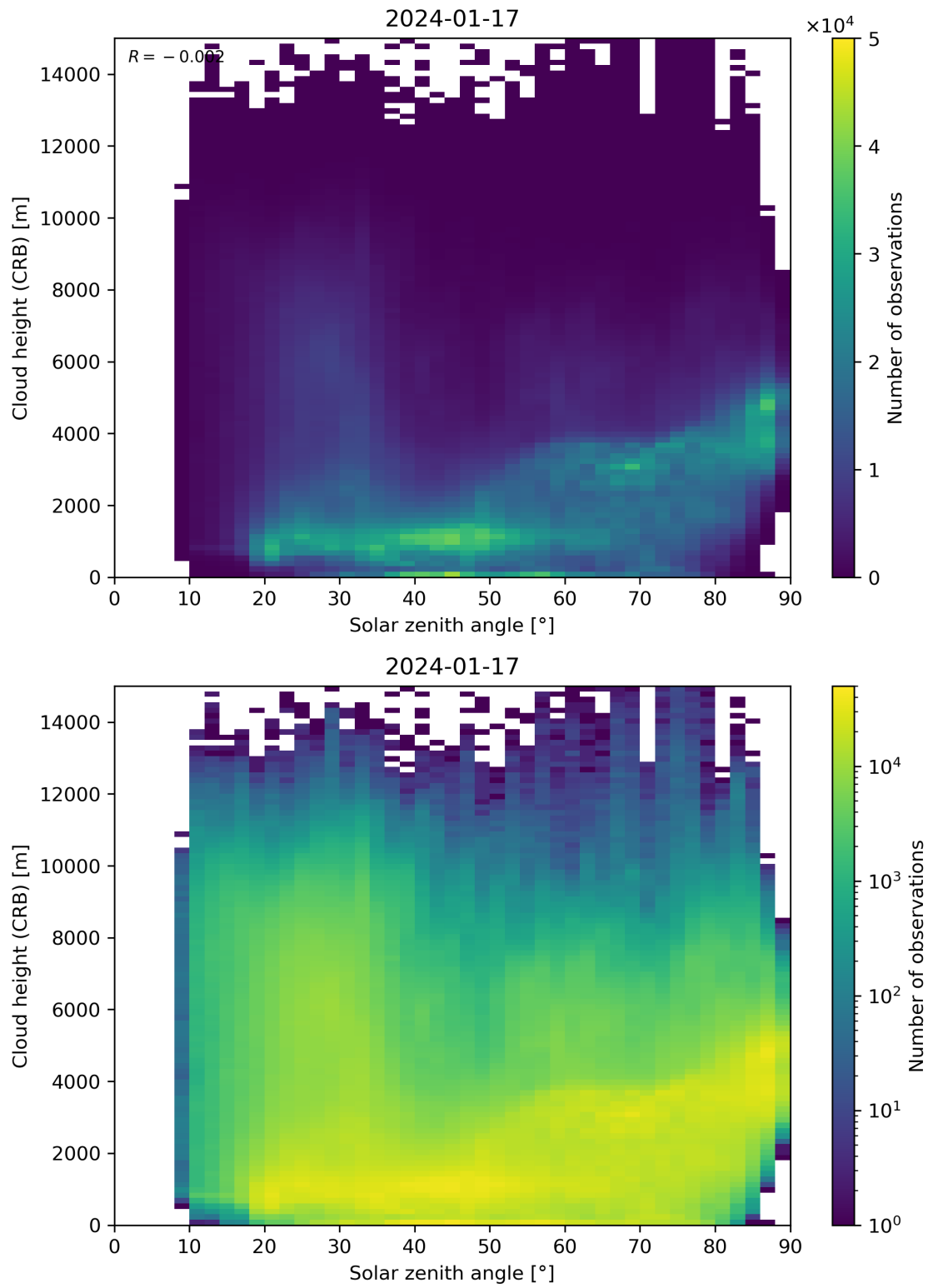
Figure 102: Scatter density plot of “Solar zenith angle” against “Cloud height (CRB)” for 2024-01-16 to 2024-01-18.
