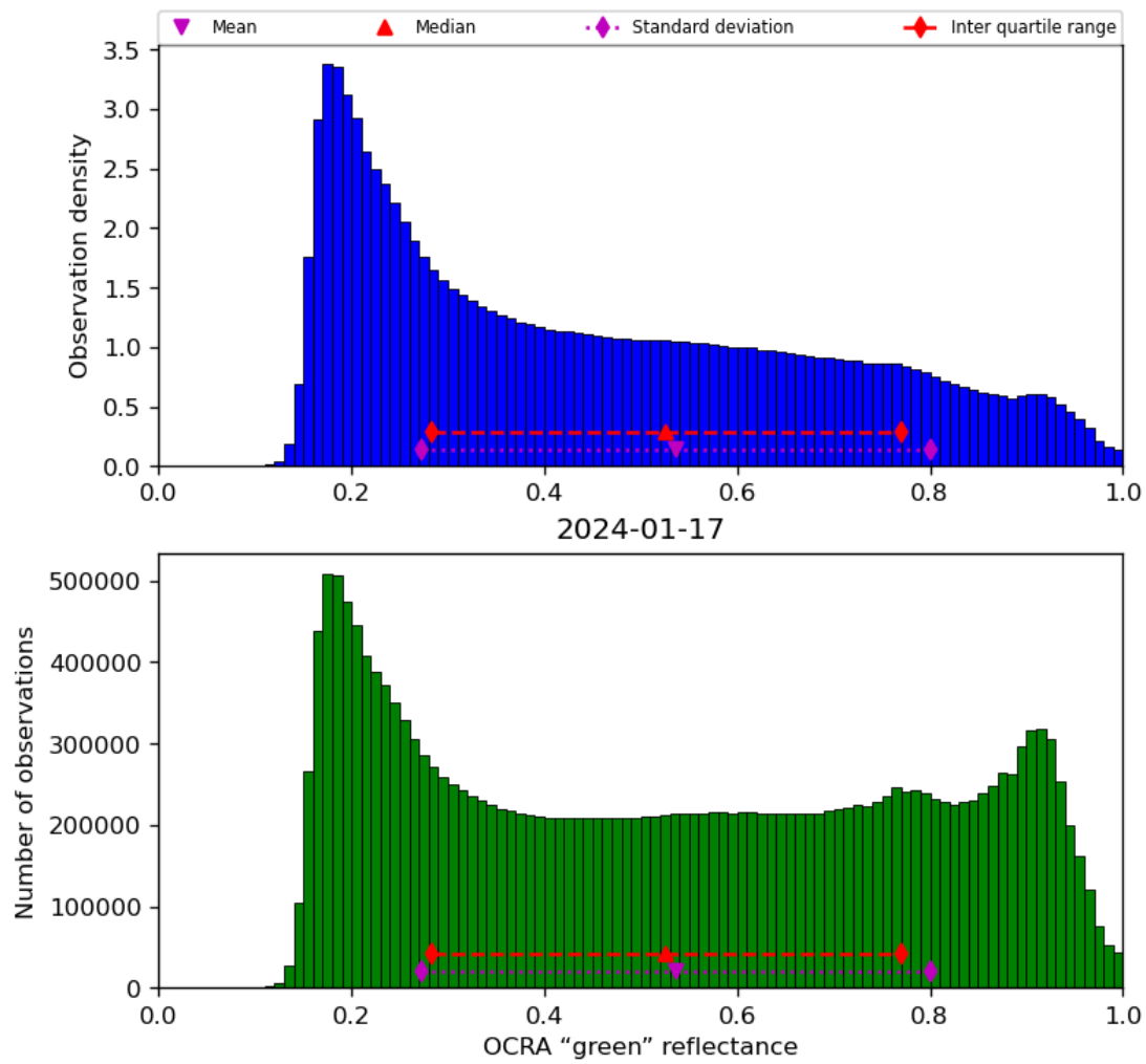
Figure 52: Histogram of “OCRA “green” reflectance” for 2024-01-16 to 2024-01-18
