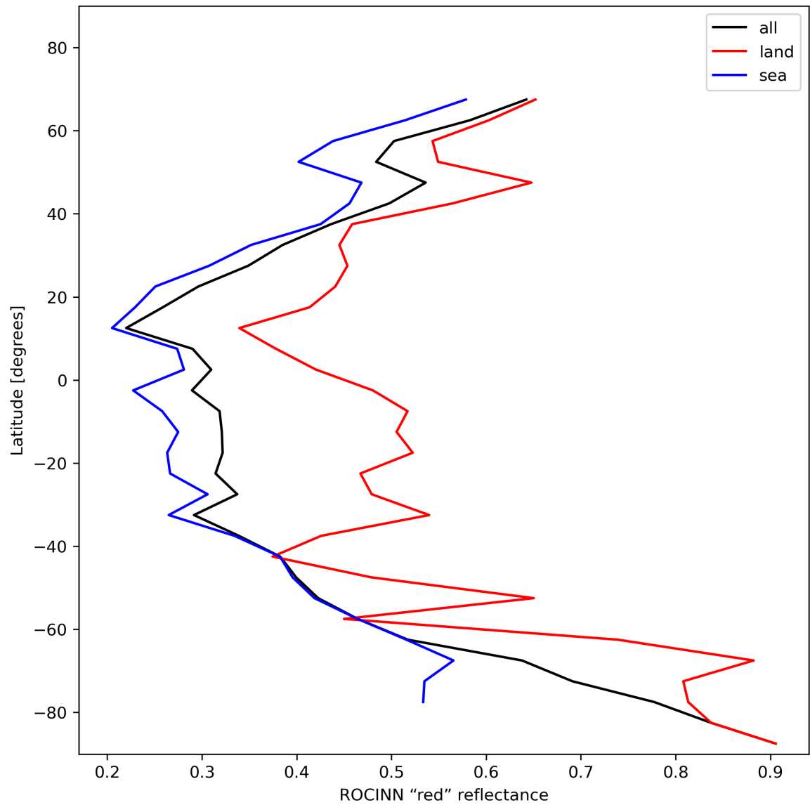
Figure 37: Zonal average of “ROCINN “red” reflectance” for 2024-01-16 to 2024-01-18.
