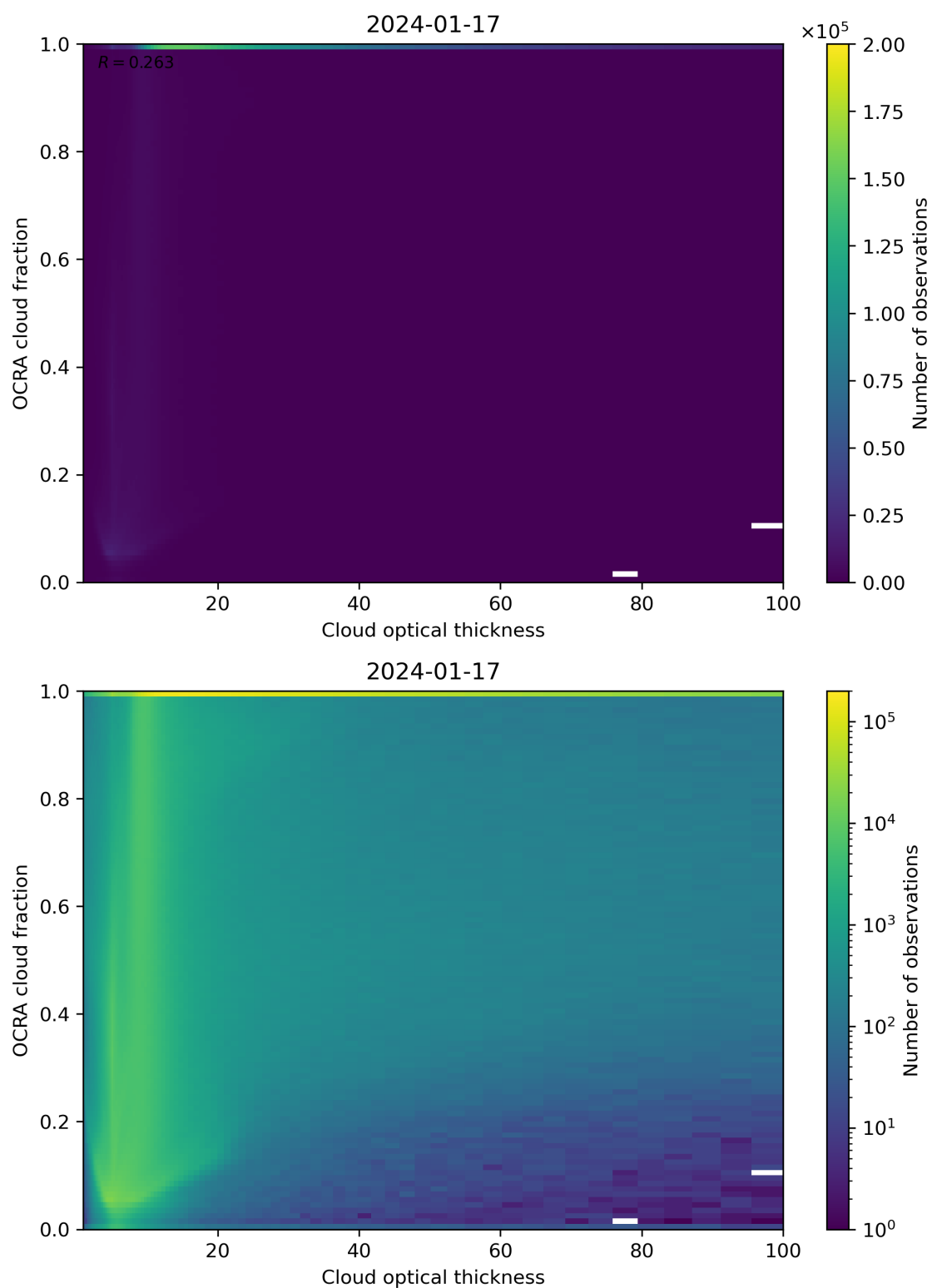
Figure 83: Scatter density plot of “Cloud optical thickness” against “OCRA cloud fraction” for 2024-01-16 to 2024-01-18.
