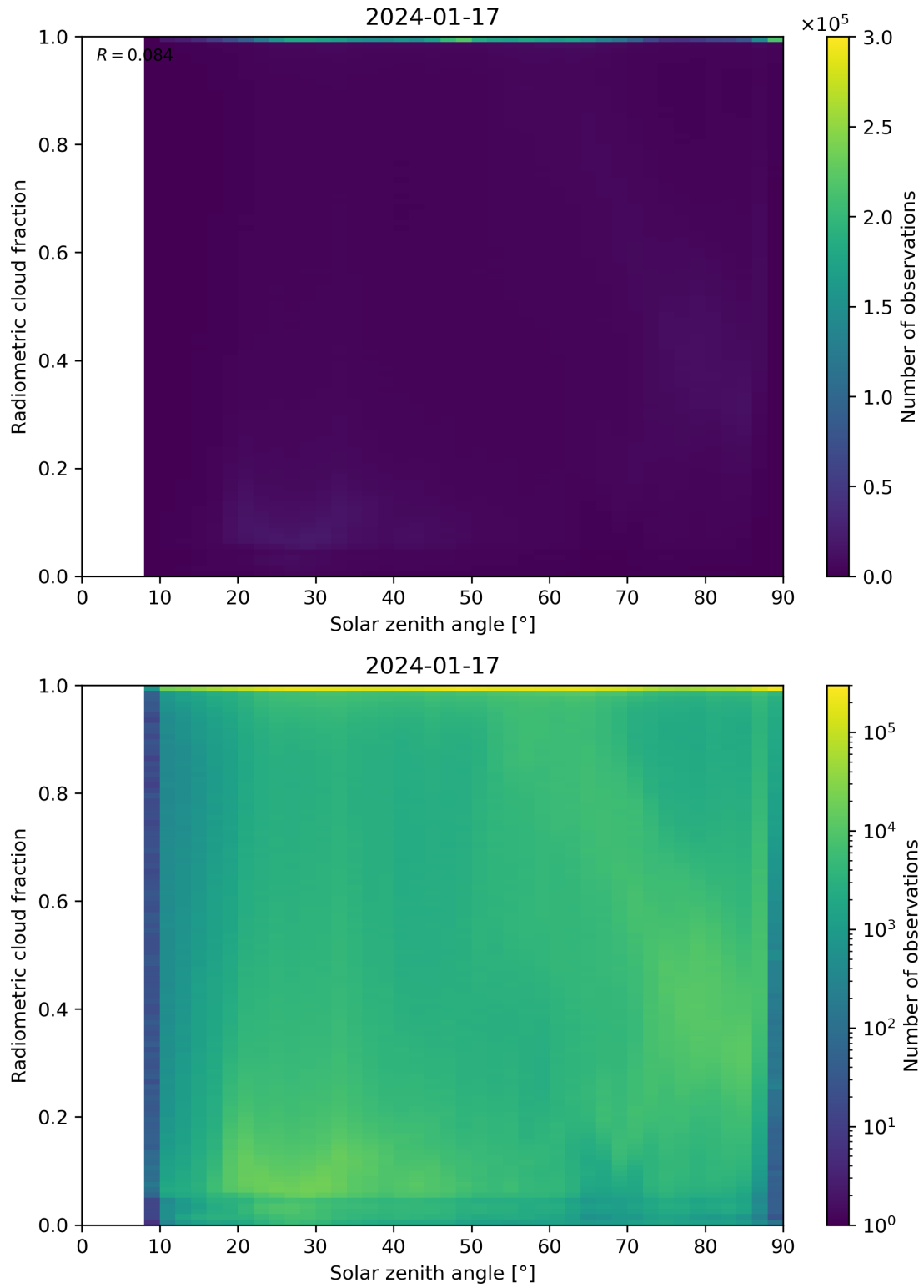
Figure 99: Scatter density plot of “Solar zenith angle” against “Radiometric cloud fraction” for 2024-01-16 to 2024-01-18.
