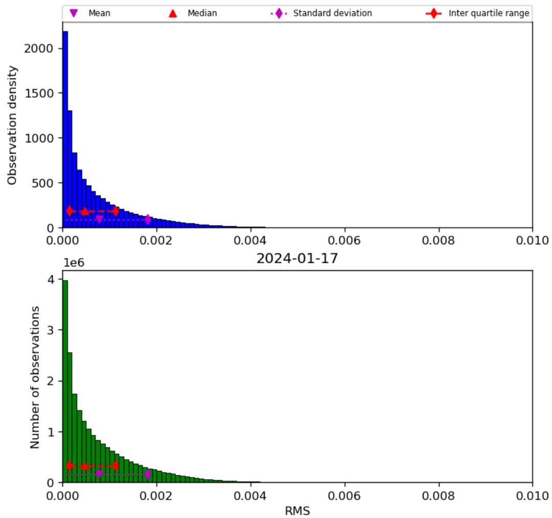
Figure 47: Histogram of “RMS” for 2024-01-16 to 2024-01-18
