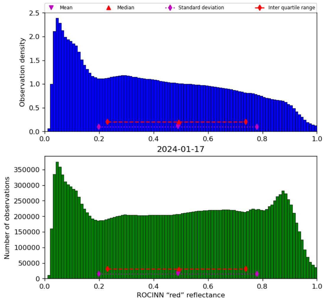
Figure 53: Histogram of “ROCINN “red” reflectance” for 2024-01-16 to 2024-01-18
