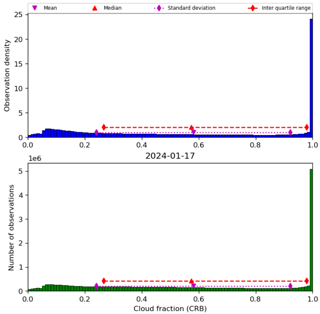
Figure 42: Histogram of “Cloud fraction (CRB)” for 2024-01-16 to 2024-01-18
