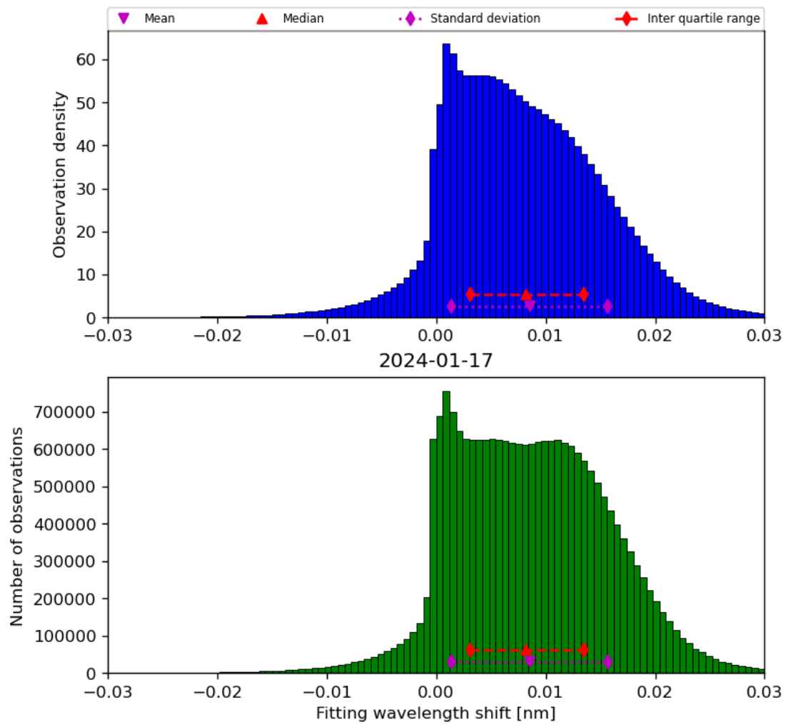
Figure 49: Histogram of “Fitting wavelength shift” for 2024-01-16 to 2024-01-18
