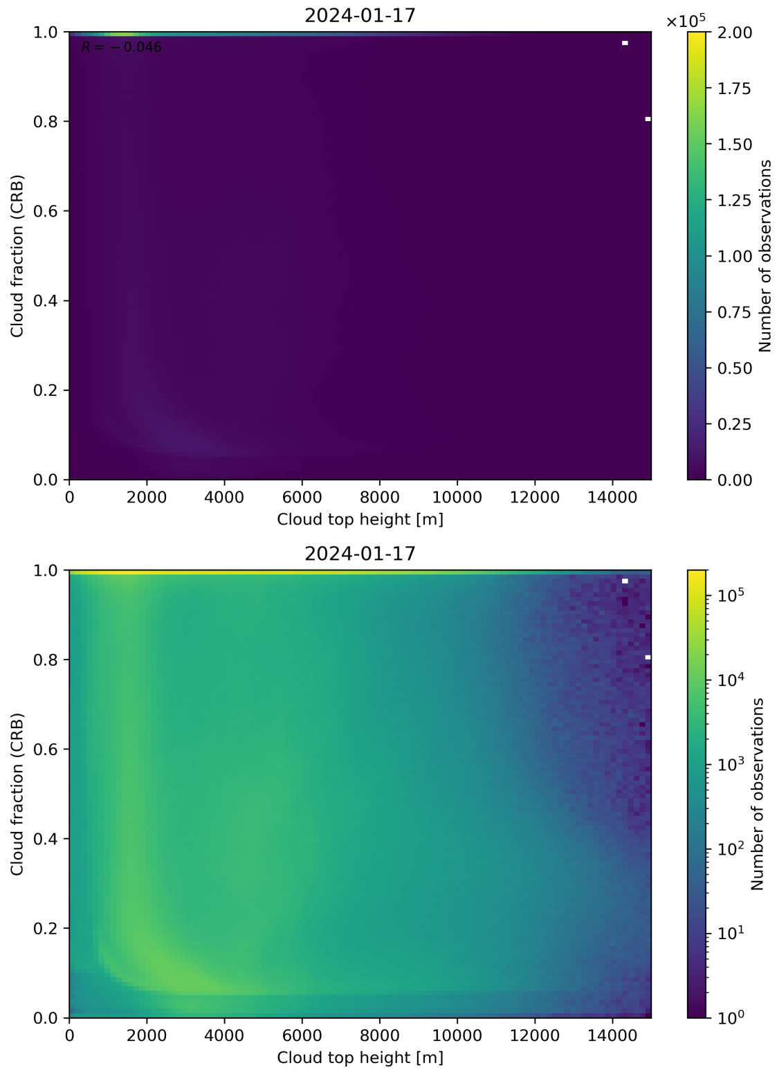
Figure 88: Scatter density plot of “Cloud top height” against “Cloud fraction (CRB)” for 2024-01-16 to 2024-01-18.
