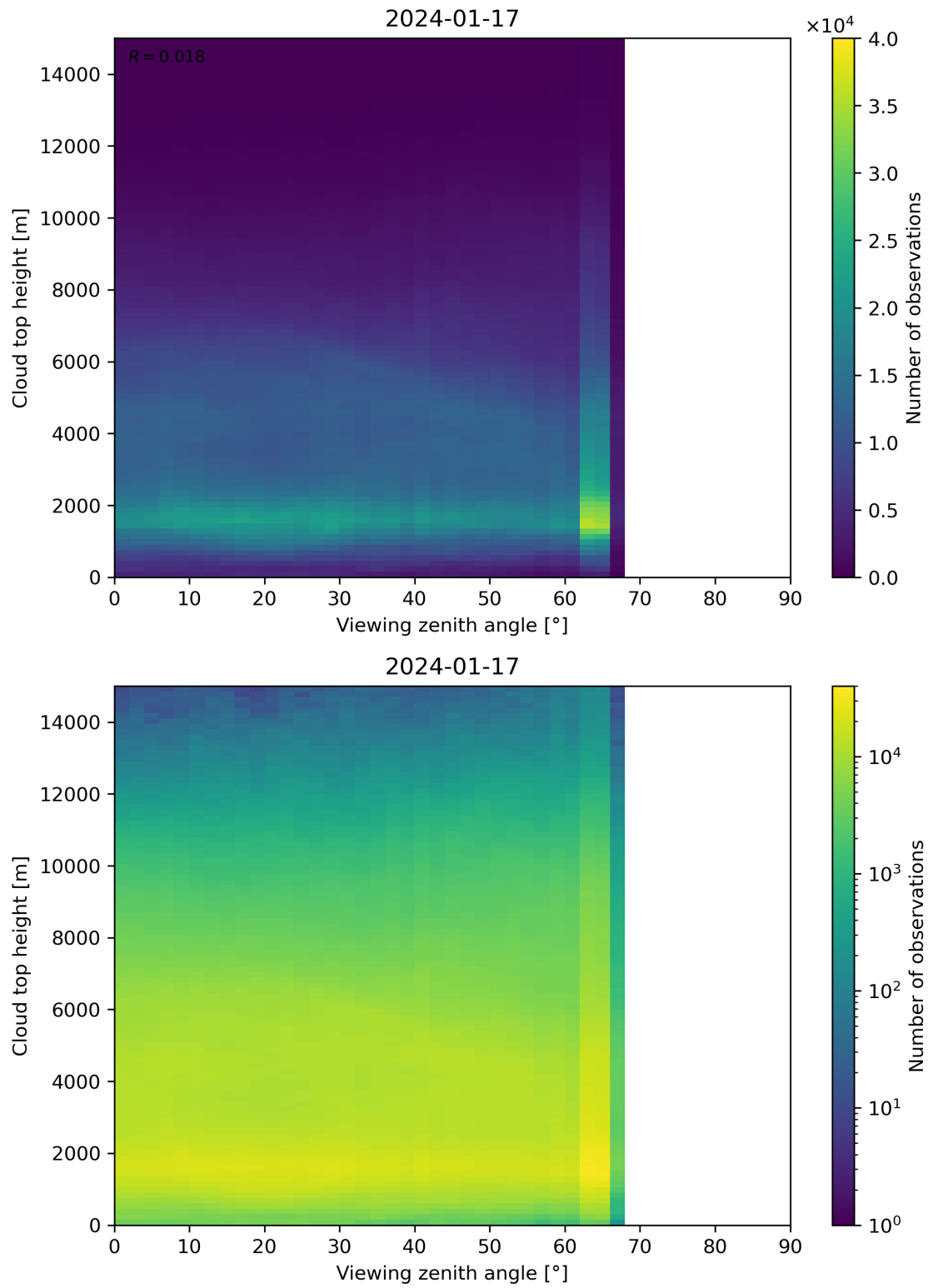
Figure 112: Scatter density plot of “Viewing zenith angle” against “Cloud top height” for 2024-01-16 to 2024-01-18.
