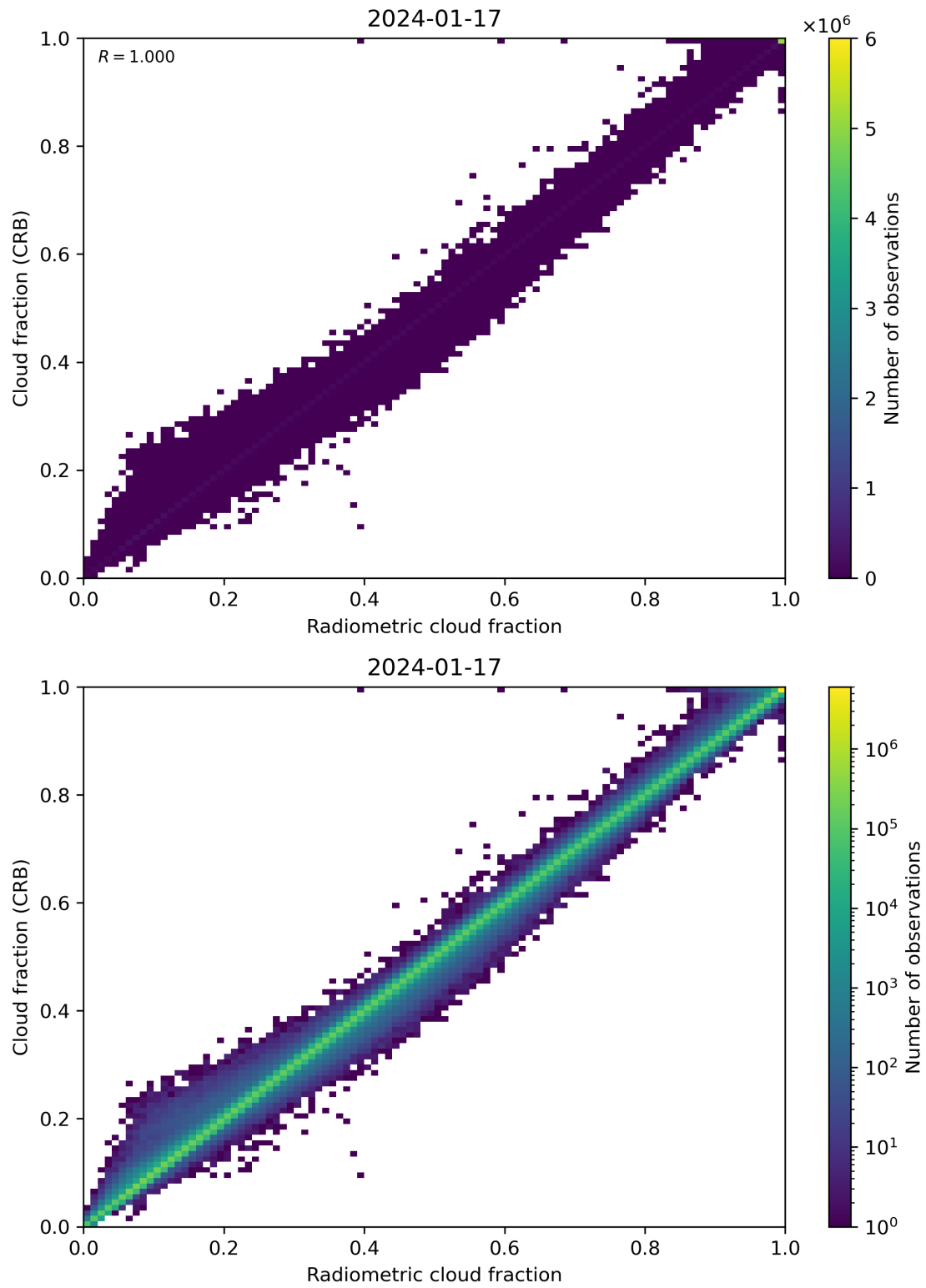
Figure 73: Scatter density plot of “Radiometric cloud fraction” against “Cloud fraction (CRB)” for 2024-01-16 to 2024-01-18.
