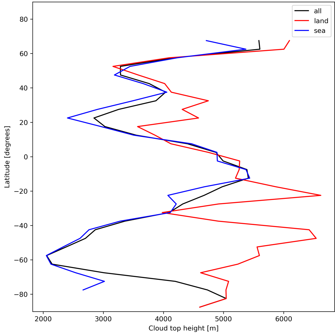
Figure 24: Zonal average of “Cloud top height” for 2024-01-16 to 2024-01-18.
