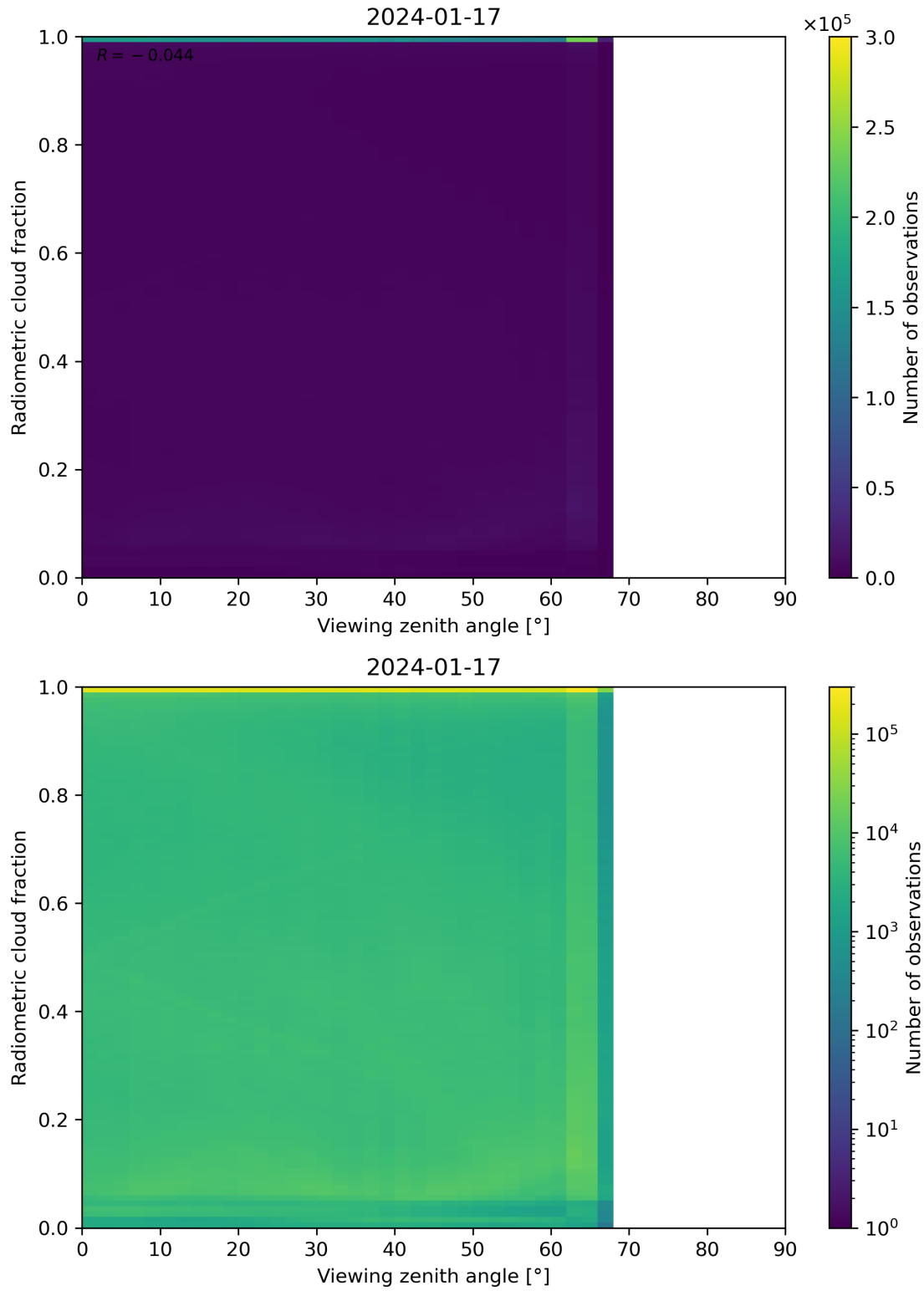
Figure 107: Scatter density plot of “Viewing zenith angle” against “Radiometric cloud fraction” for 2024-01-16 to 2024-01-18.
