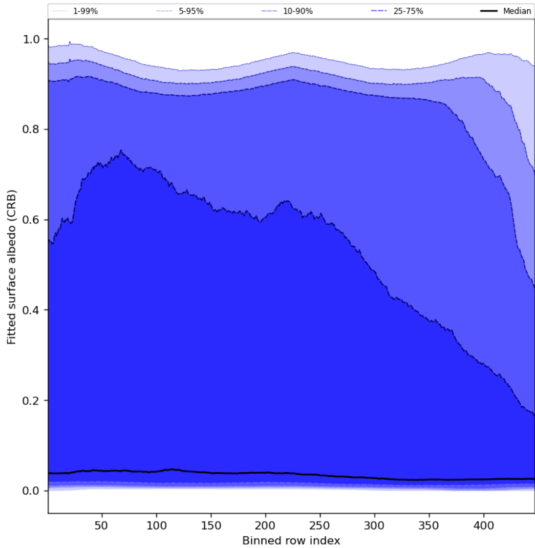
Figure 62: Along track statistics of “Fitted surface albedo (CRB)” for 2024-01-16 to 2024-01-18
