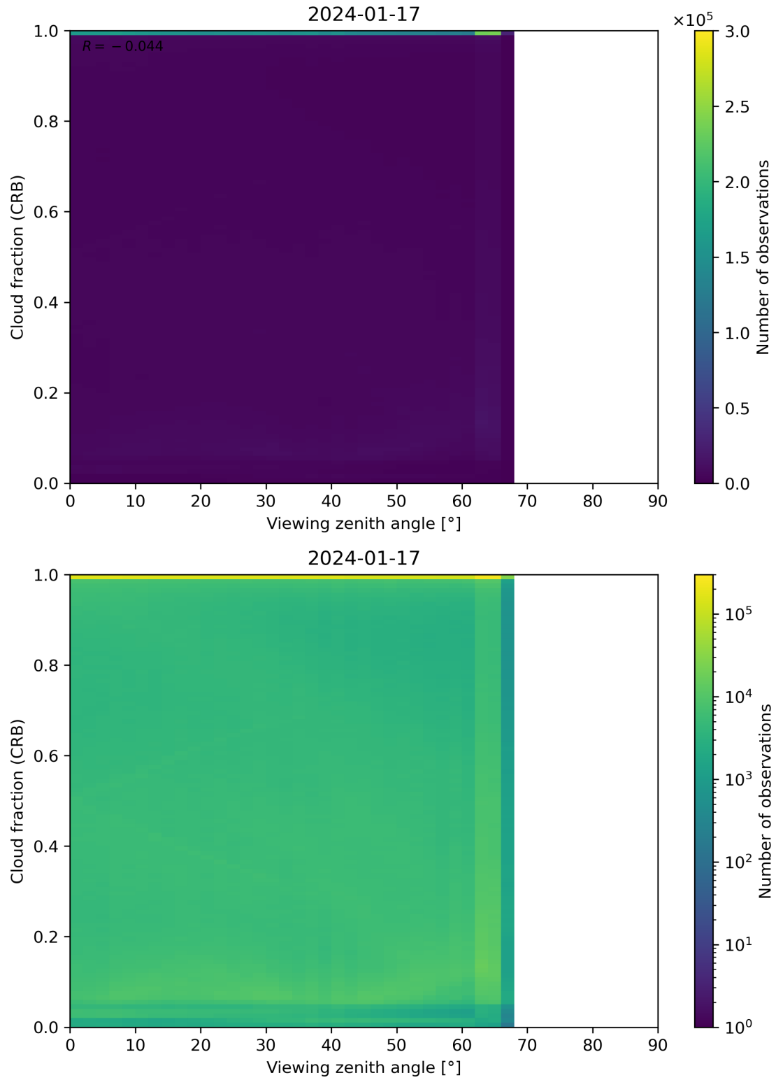
Figure 109: Scatter density plot of “Viewing zenith angle” against “Cloud fraction (CRB)” for 2024-01-16 to 2024-01-18.
