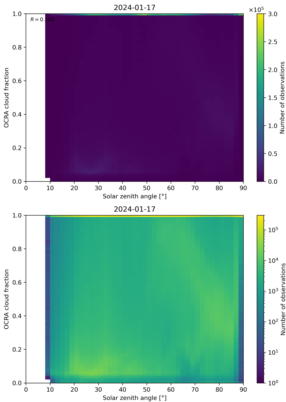
Figure 100: Scatter density plot of “Solar zenith angle” against “OCRA cloud fraction” for 2024-01-16 to 2024-01-18.
