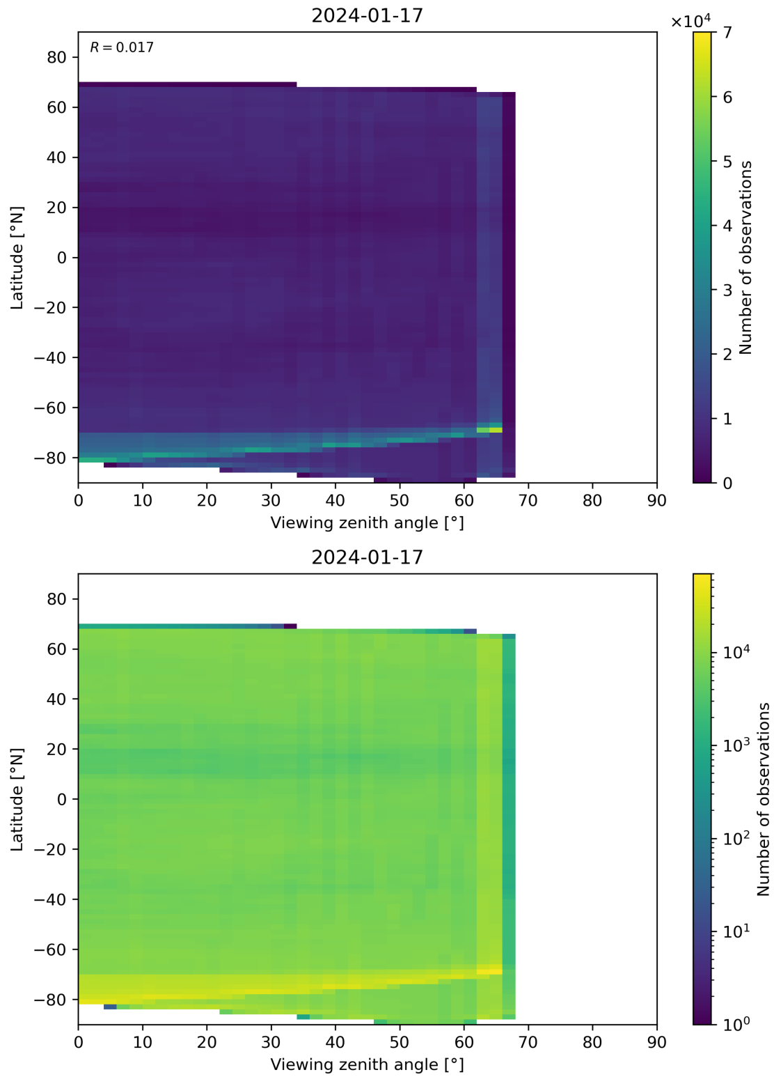
Figure 113: Scatter density plot of “Viewing zenith angle” against “Latitude” for 2024-01-16 to 2024-01-18.
