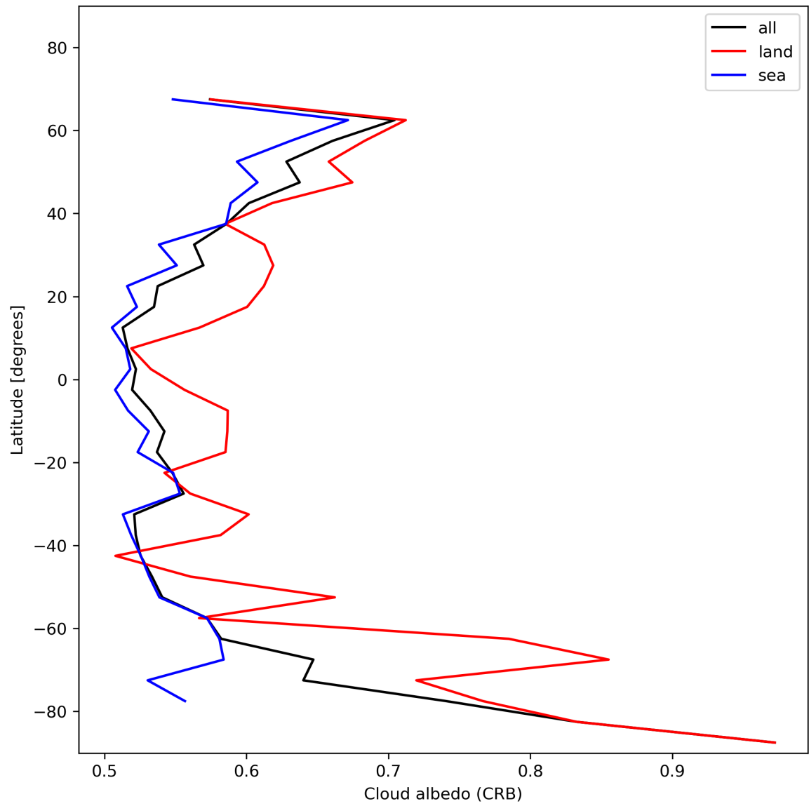
Figure 28: Zonal average of “Cloud albedo (CRB)” for 2024-01-16 to 2024-01-18.
