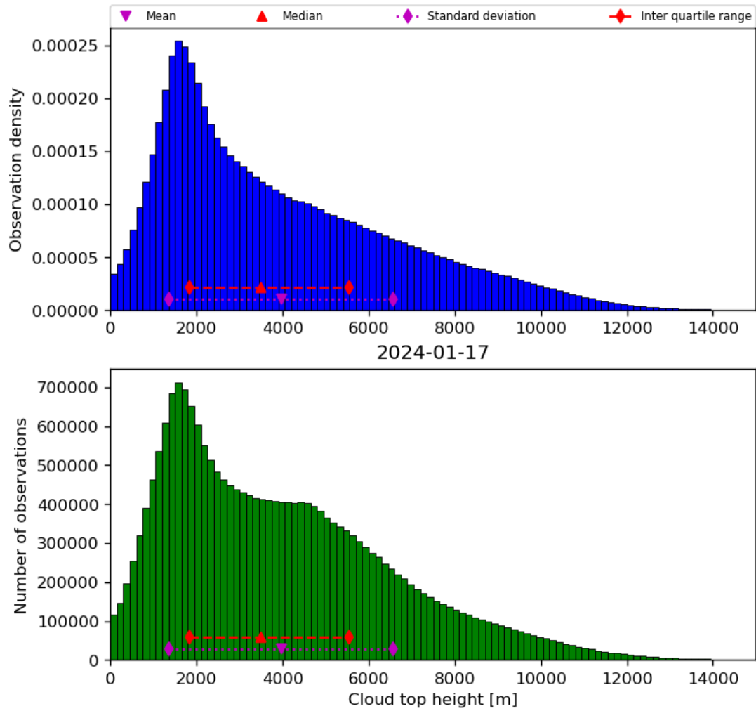
Figure 40: Histogram of “Cloud top height” for 2024-01-16 to 2024-01-18
