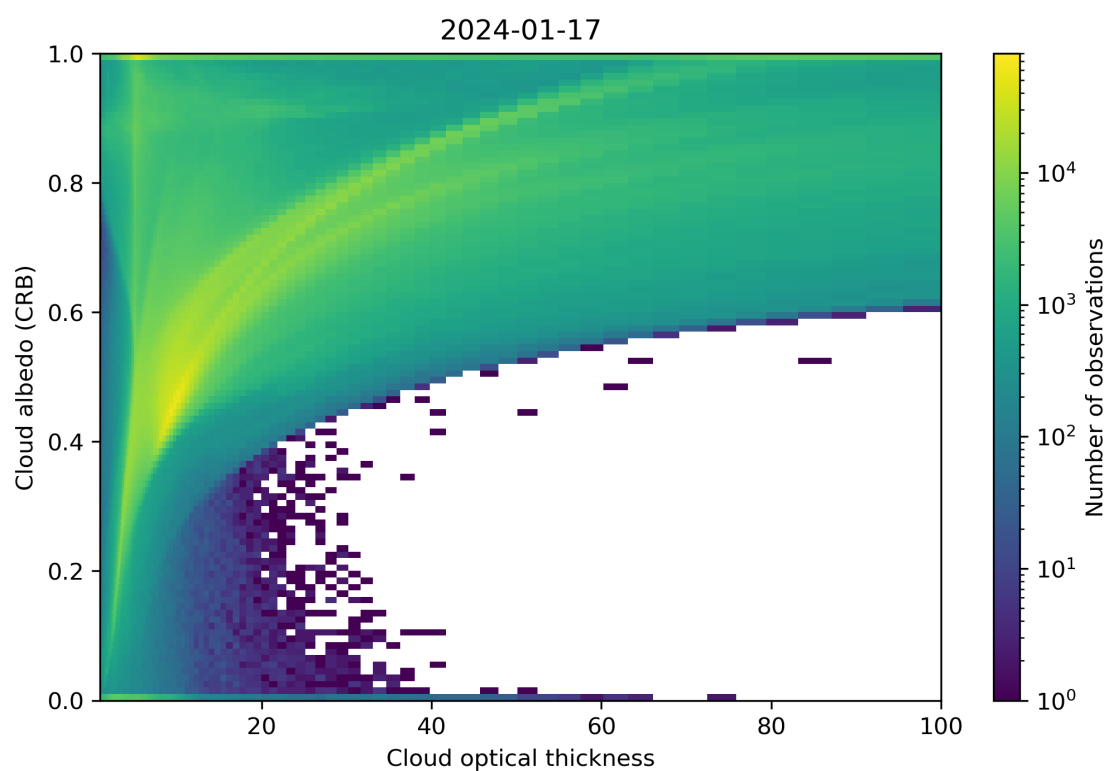
Figure 82: Scatter density plot of “Cloud optical thickness” against “Cloud albedo (CRB)” for 2024-01-16 to 2024-01-18.
