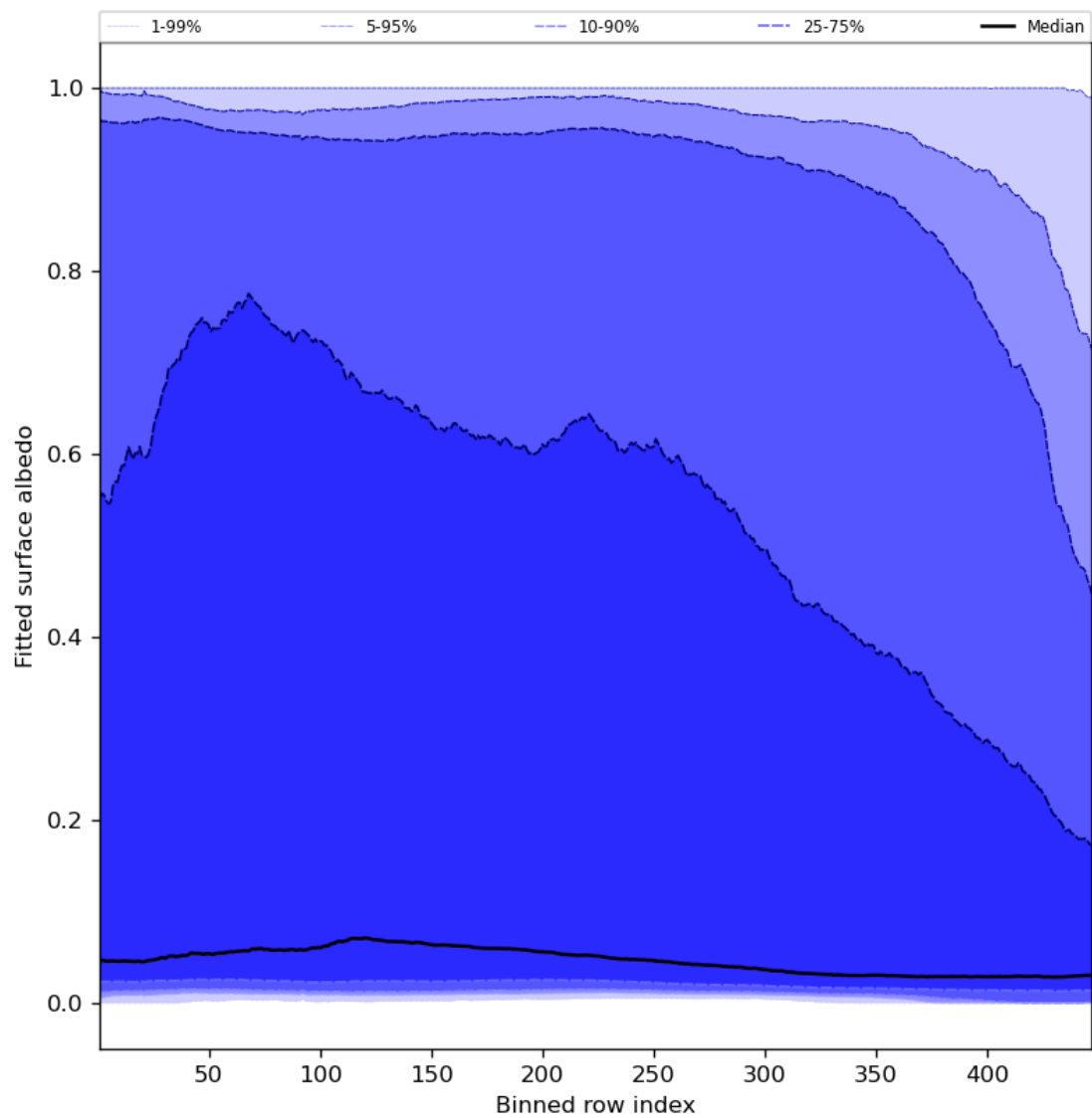
Figure 61: Along track statistics of “Fitted surface albedo” for 2024-01-16 to 2024-01-18
