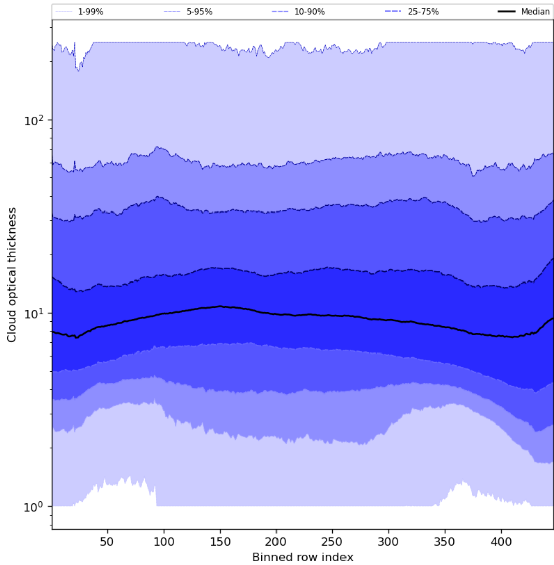
Figure 57: Along track statistics of “Cloud optical thickness” for 2024-01-16 to 2024-01-18
