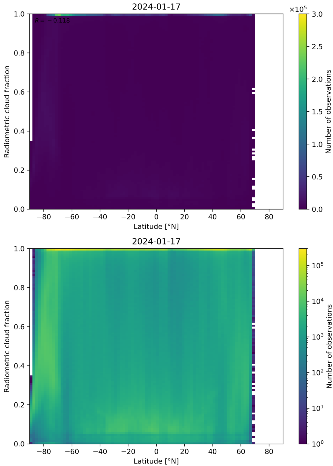
Figure 92: Scatter density plot of “Latitude” against “Radiometric cloud fraction” for 2024-01-16 to 2024-01-18.
