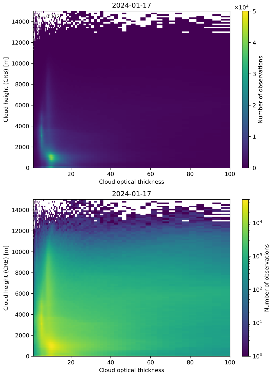
Figure 85: Scatter density plot of “Cloud optical thickness” against “Cloud height (CRB)” for 2024-01-16 to 2024-01-18.
