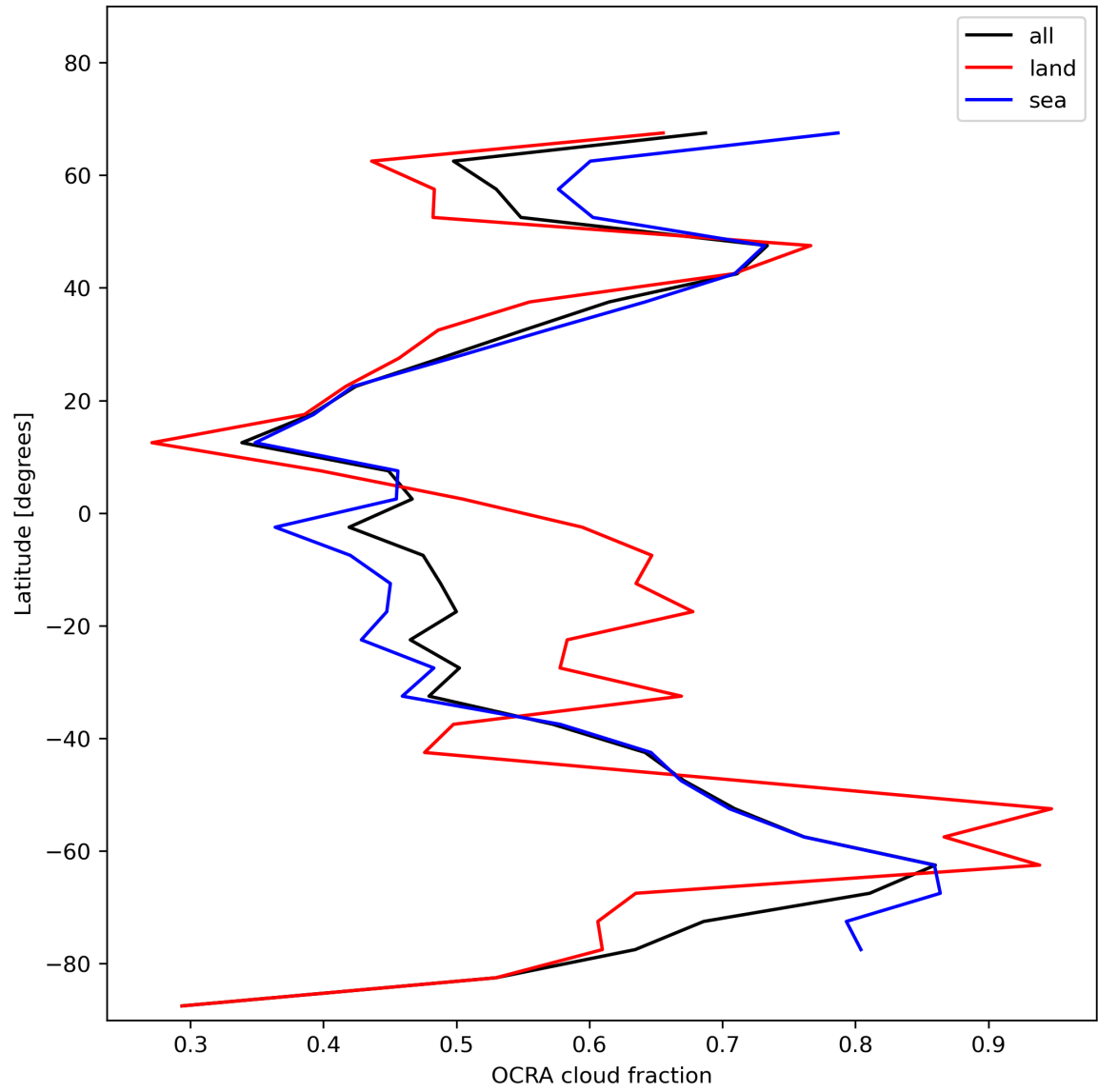
Figure 34: Zonal average of “OCRA cloud fraction” for 2024-01-16 to 2024-01-18.
