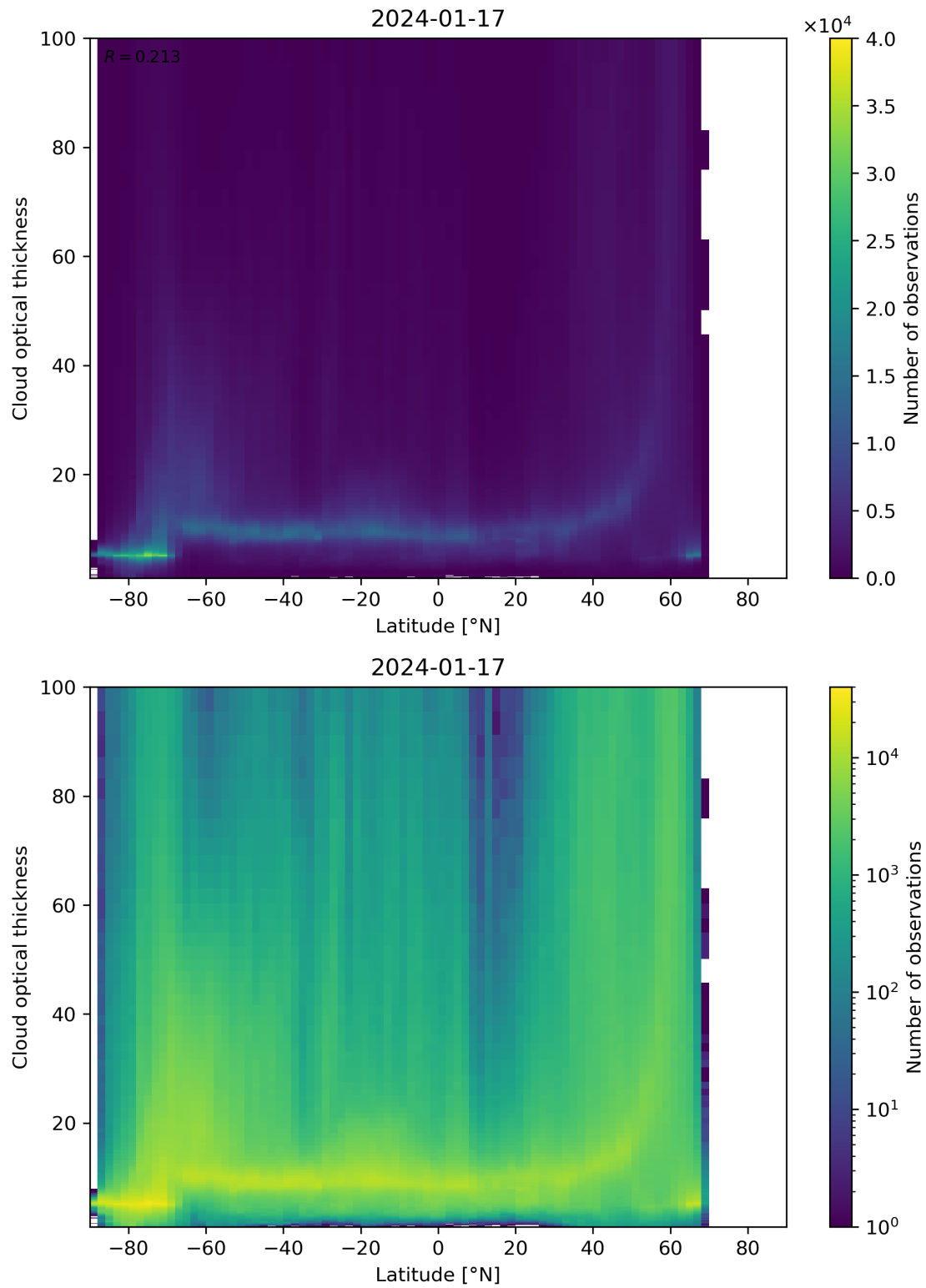
Figure 96: Scatter density plot of “Latitude” against “Cloud optical thickness” for 2024-01-16 to 2024-01-18.
