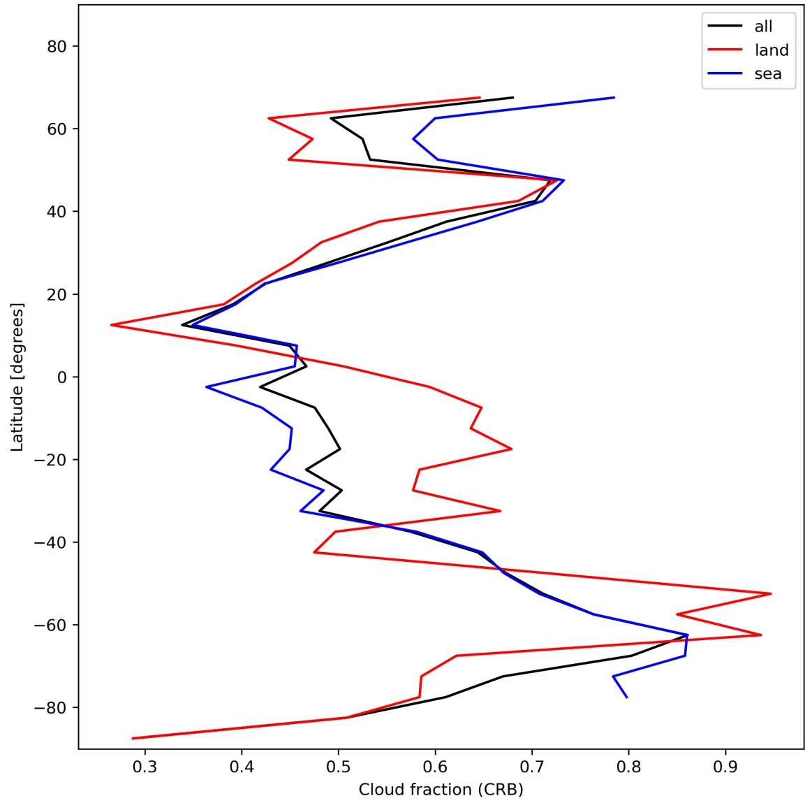
Figure 26: Zonal average of “Cloud fraction (CRB)” for 2024-01-16 to 2024-01-18.
