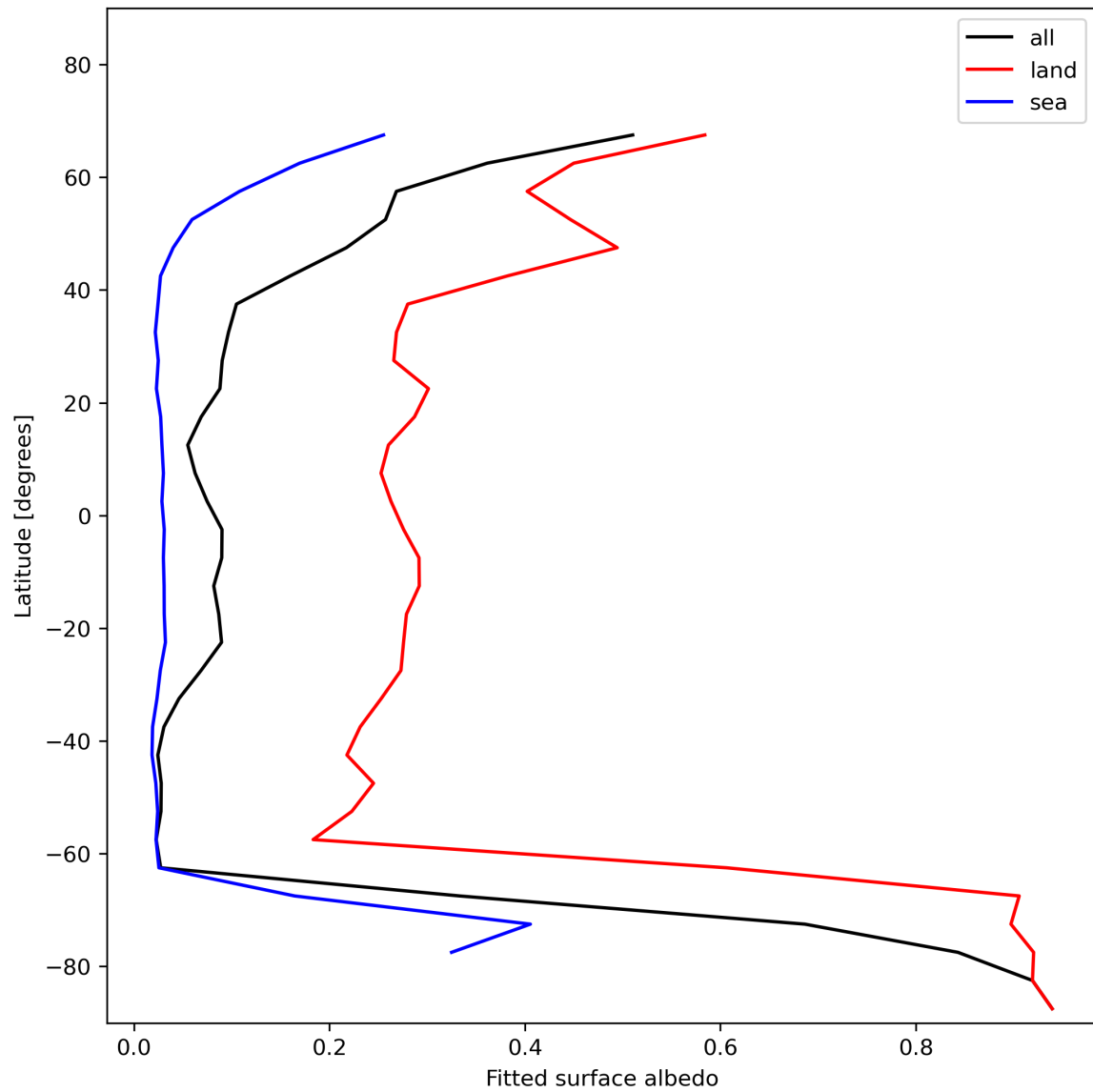
Figure 29: Zonal average of “Fitted surface albedo” for 2024-01-16 to 2024-01-18.
