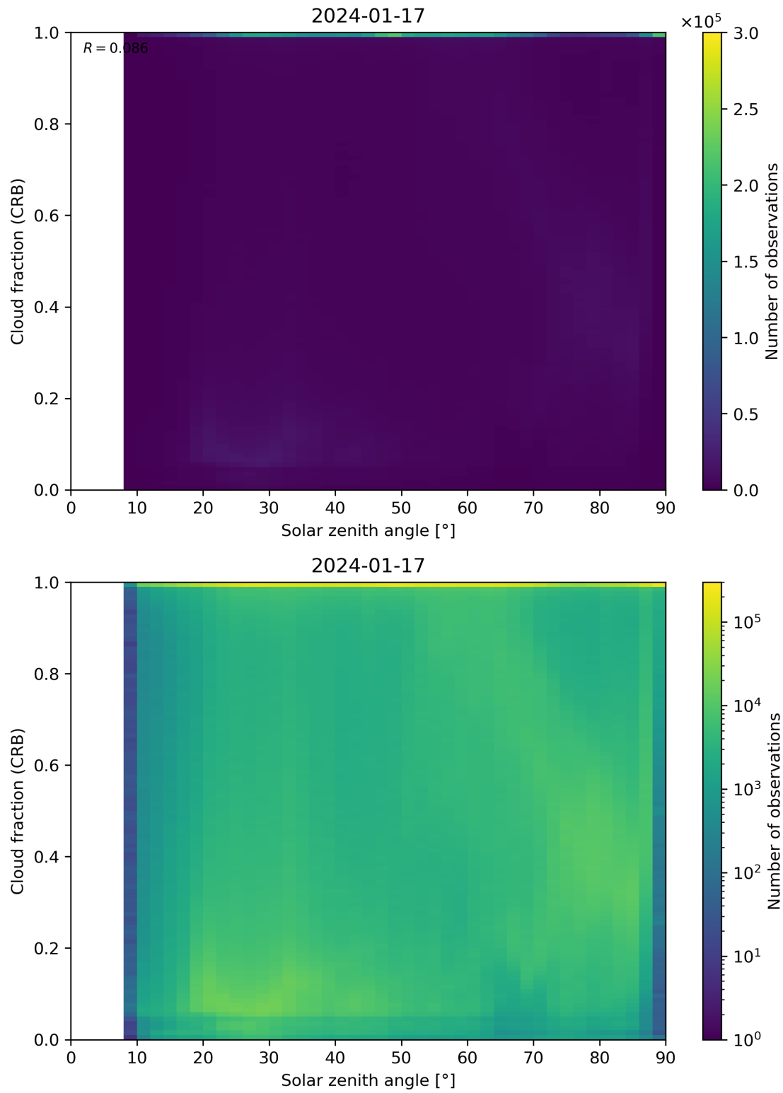
Figure 101: Scatter density plot of “Solar zenith angle” against “Cloud fraction (CRB)” for 2024-01-16 to 2024-01-18.
