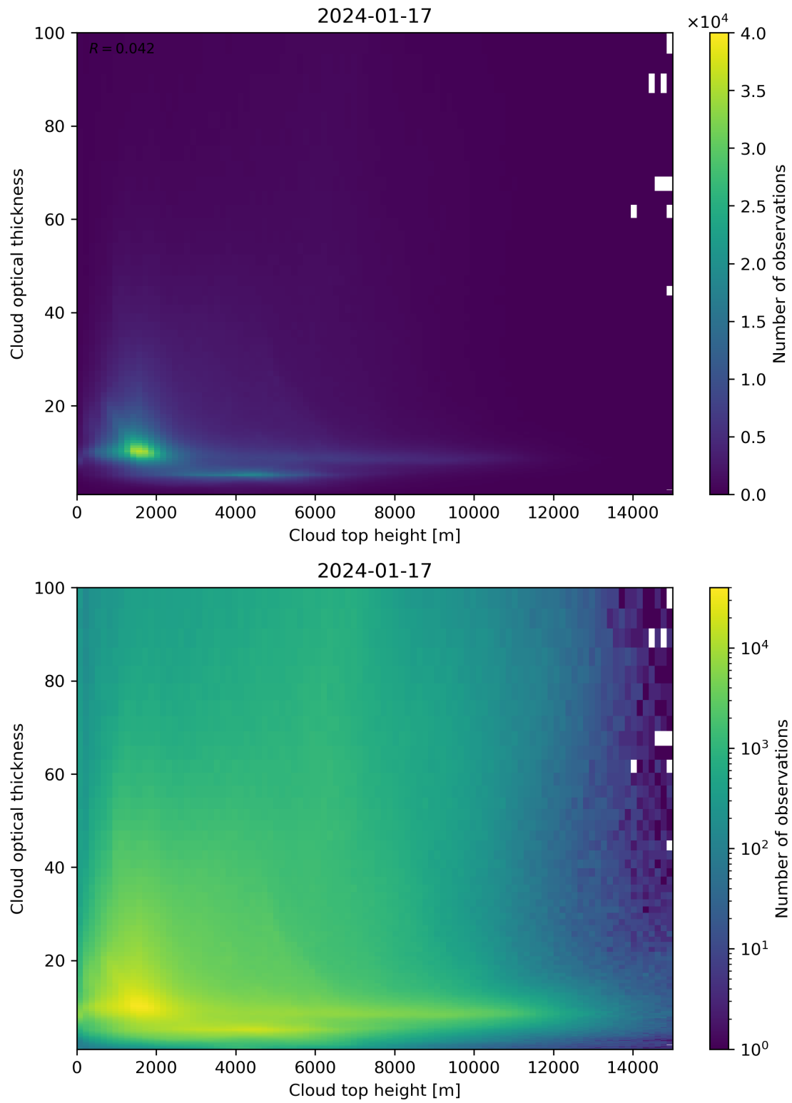
Figure 90: Scatter density plot of “Cloud top height” against “Cloud optical thickness” for 2024-01-16 to 2024-01-18.
