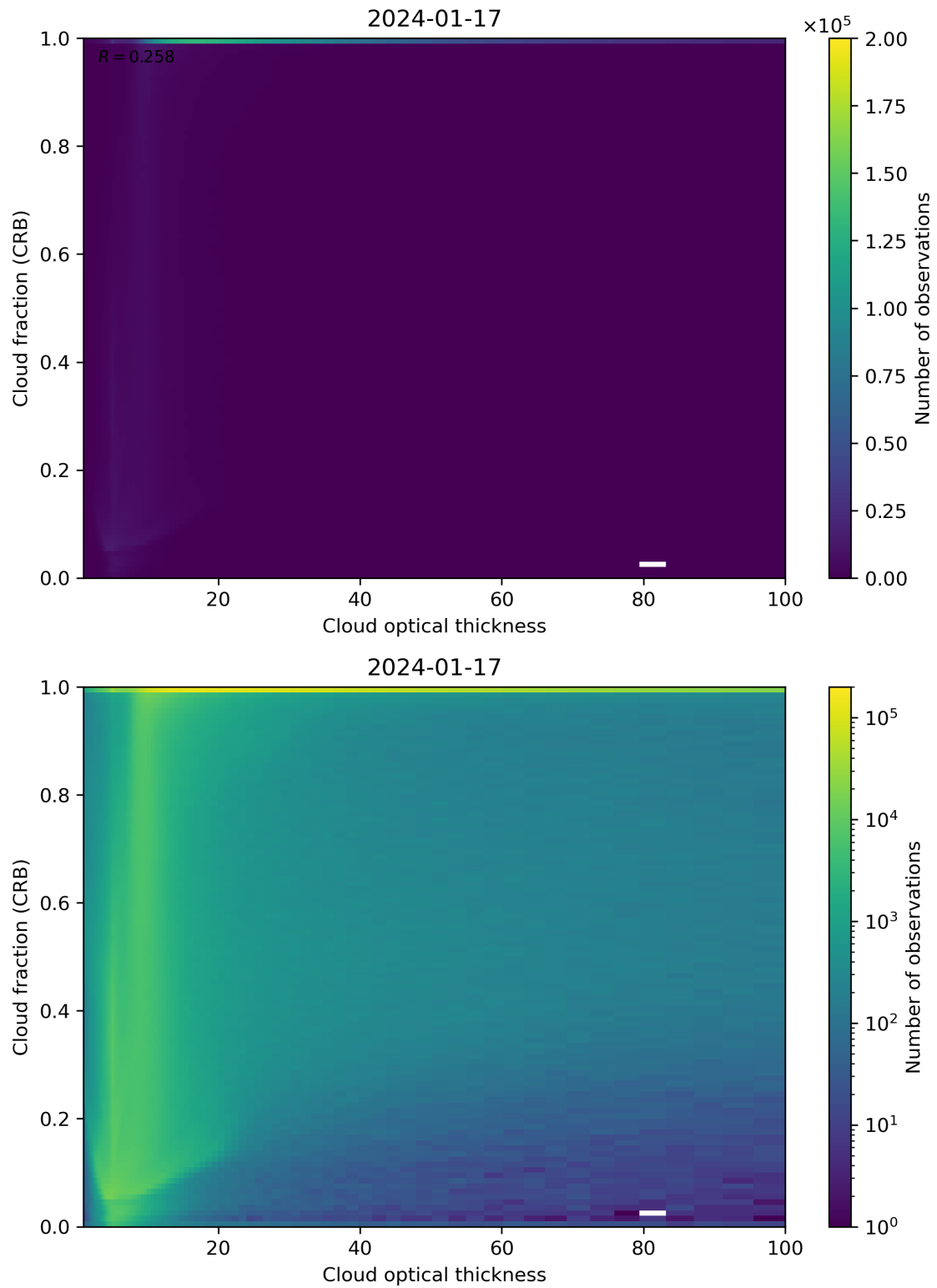
Figure 84: Scatter density plot of “Cloud optical thickness” against “Cloud fraction (CRB)” for 2024-01-16 to 2024-01-18.
