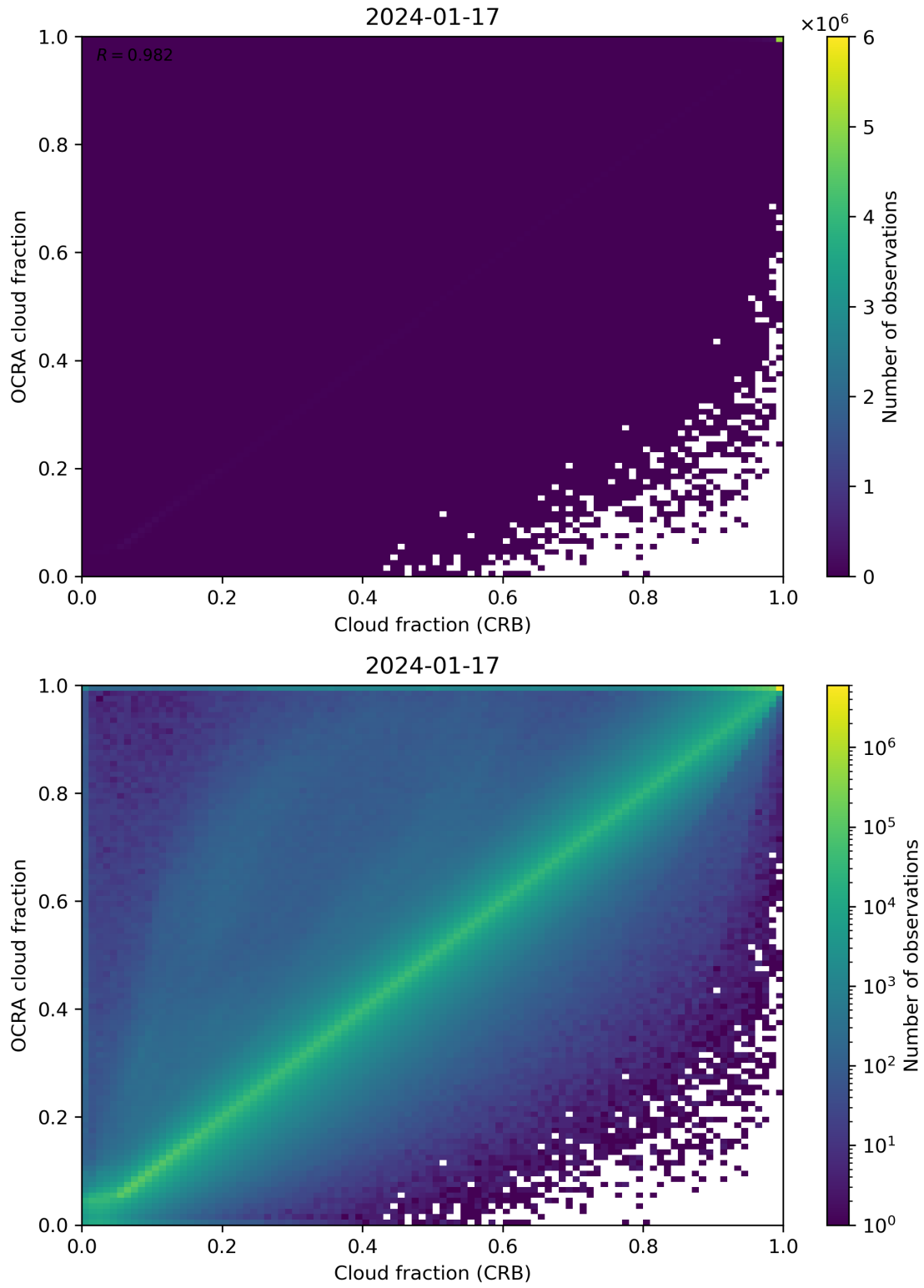
Figure 78: Scatter density plot of “Cloud fraction (CRB)” against “OCRA cloud fraction” for 2024-01-16 to 2024-01-18.
