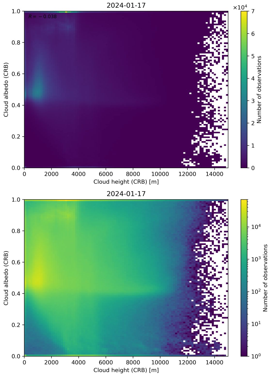
Figure 80: Scatter density plot of “Cloud height (CRB)” against “Cloud albedo (CRB)” for 2024-01-16 to 2024-01-18.
