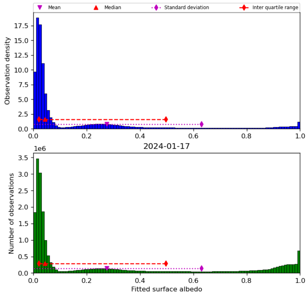
Figure 45: Histogram of “Fitted surface albedo” for 2024-01-16 to 2024-01-18
