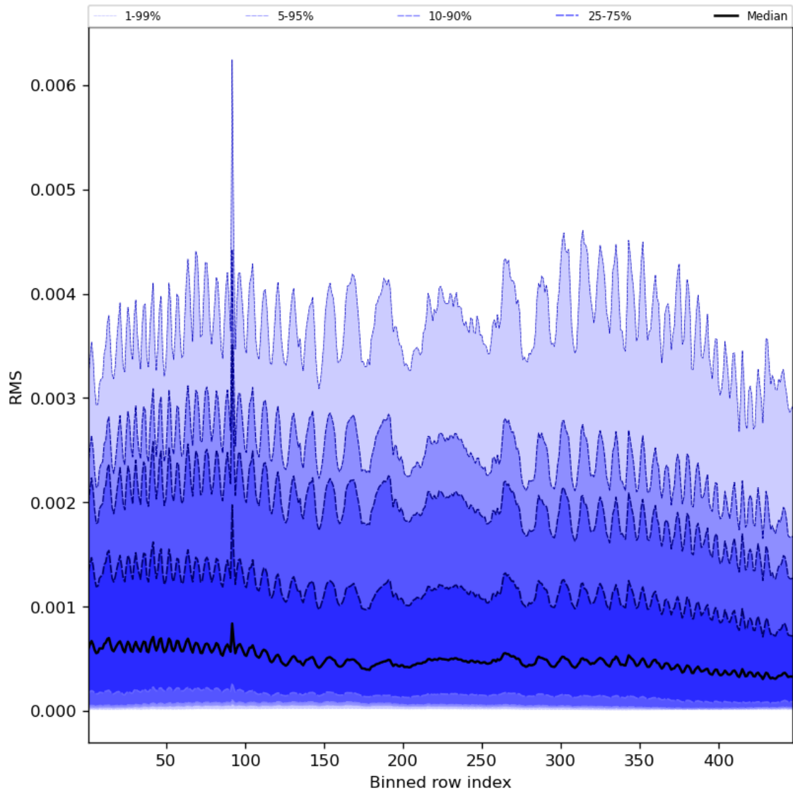
Figure 63: Along track statistics of “RMS” for 2024-01-16 to 2024-01-18
