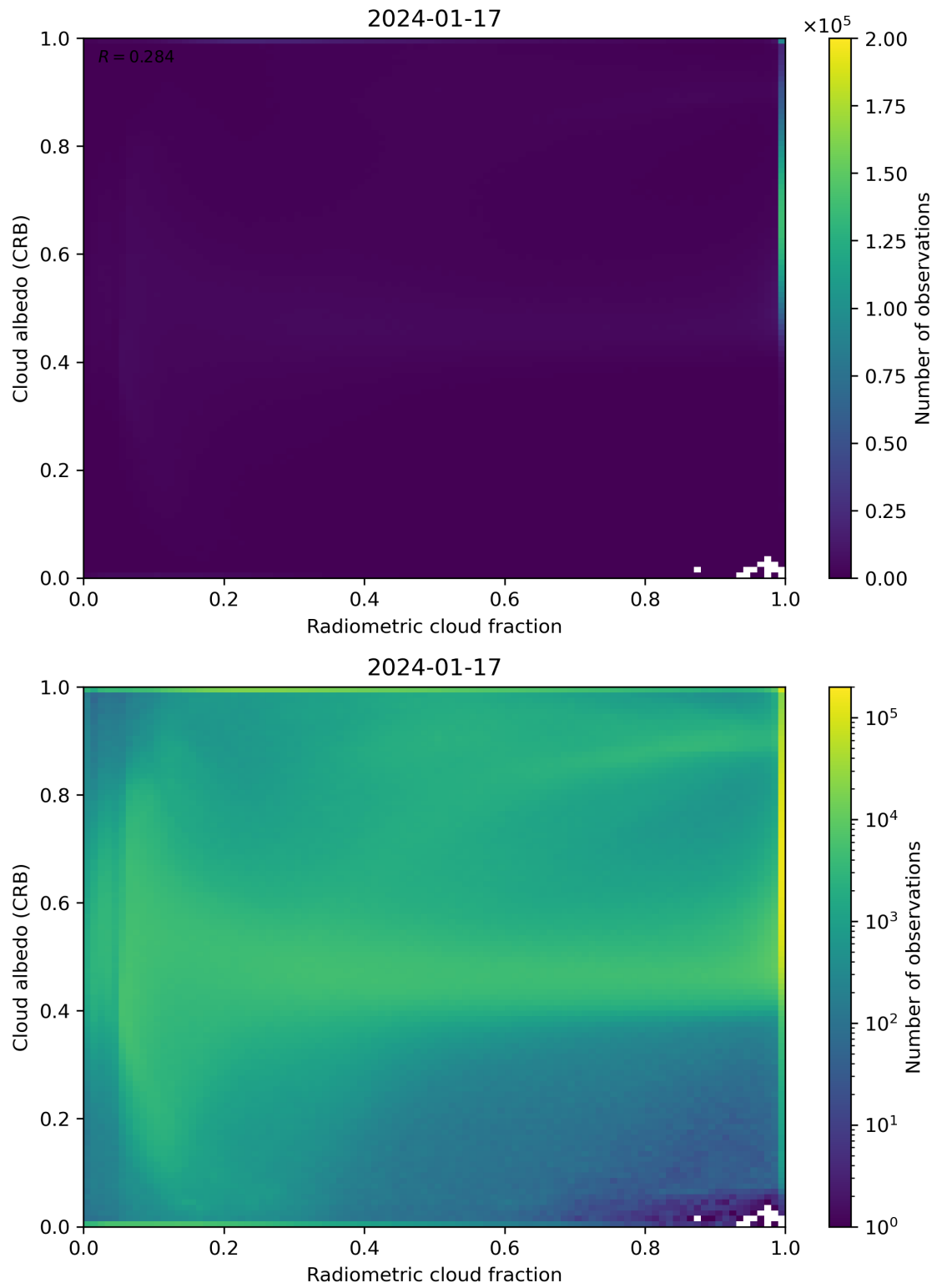
Figure 71: Scatter density plot of “Radiometric cloud fraction” against “Cloud albedo (CRB)” for 2024-01-16 to 2024-01-18.
