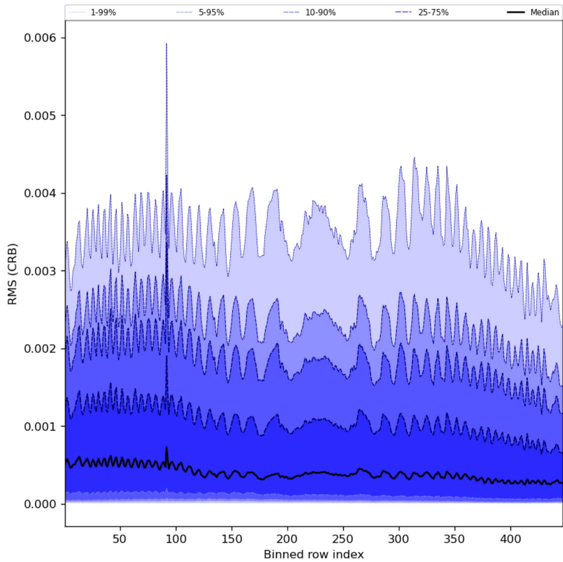
Figure 64: Along track statistics of “RMS (CRB)” for 2024-01-16 to 2024-01-18
