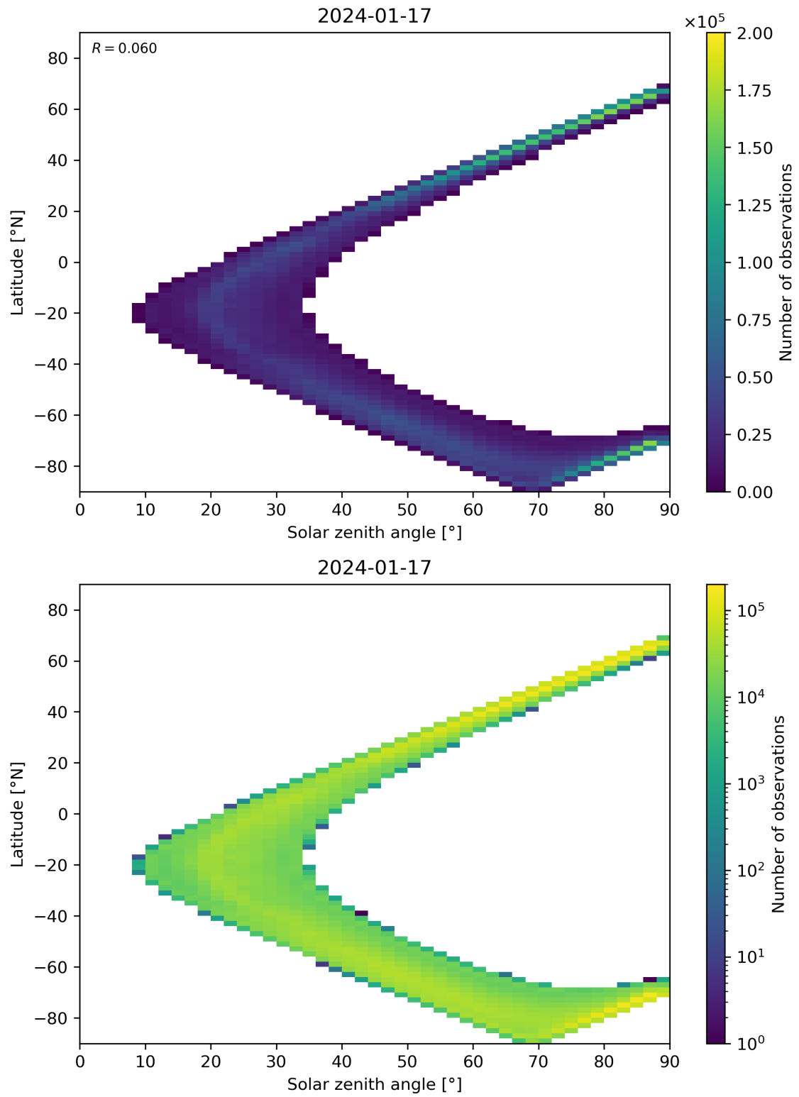
Figure 105: Scatter density plot of “Solar zenith angle” against “Latitude” for 2024-01-16 to 2024-01-18.
