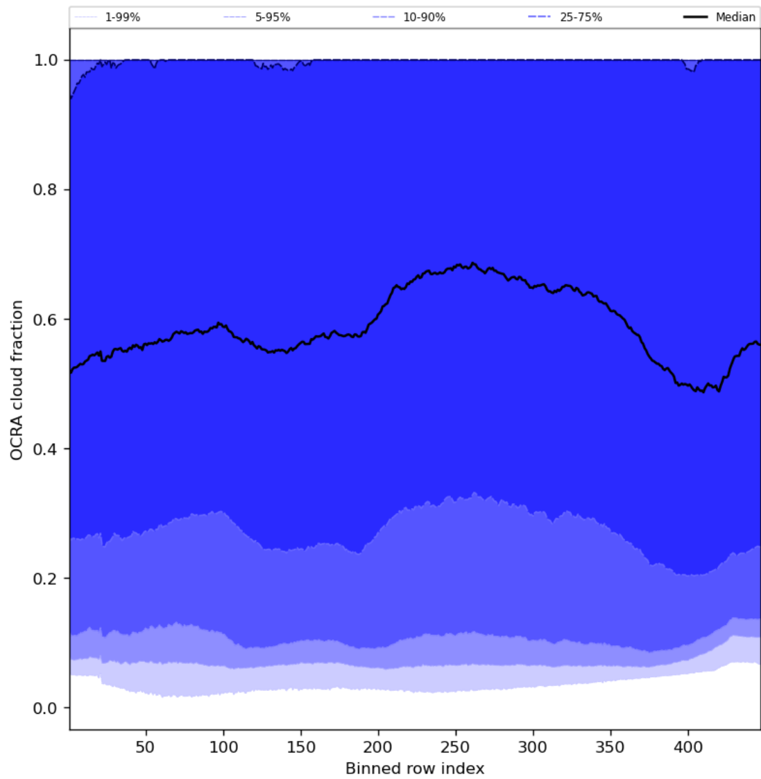
Figure 66: Along track statistics of “OCRA cloud fraction” for 2024-01-16 to 2024-01-18
