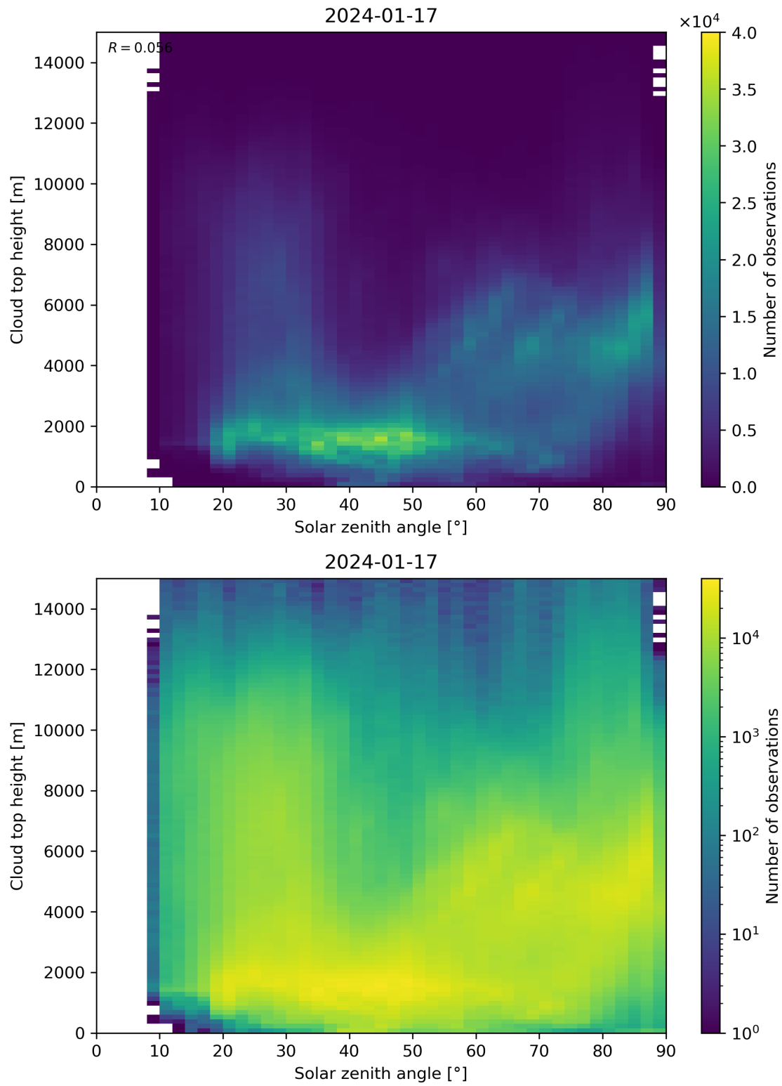
Figure 104: Scatter density plot of “Solar zenith angle” against “Cloud top height” for 2024-01-16 to 2024-01-18.
