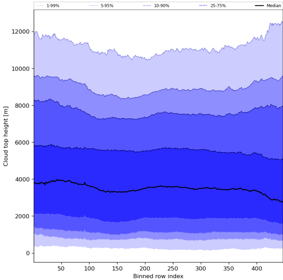
Figure 56: Along track statistics of “Cloud top height” for 2024-01-16 to 2024-01-18
