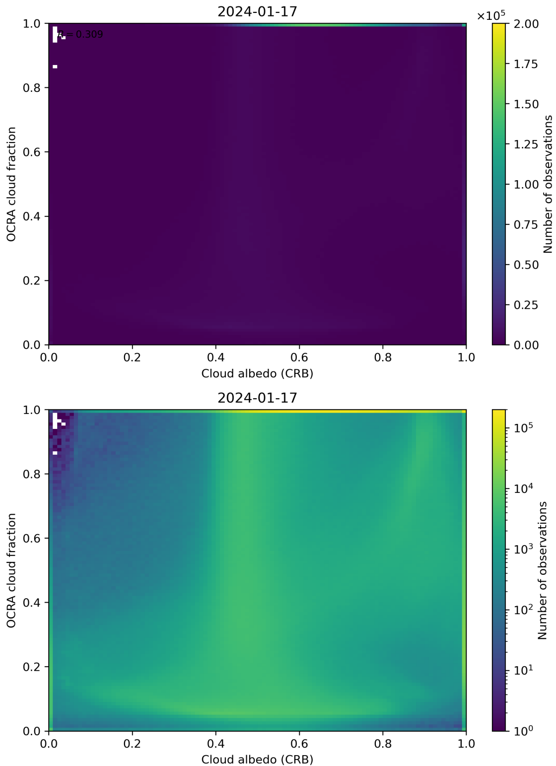
Figure 70: Scatter density plot of “Cloud albedo (CRB)” against “OCRA cloud fraction” for 2024-01-16 to 2024-01-18.
