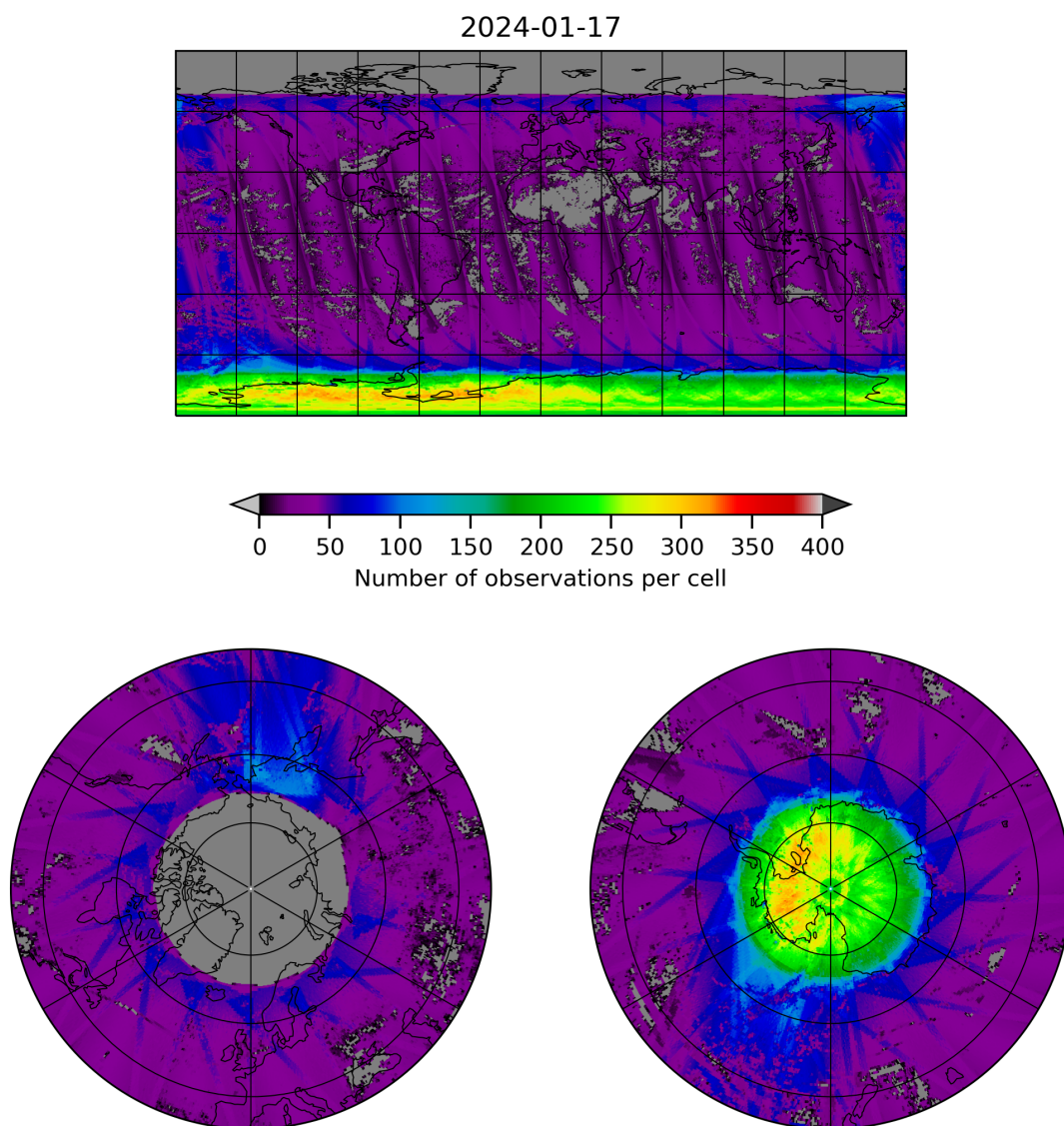
Figure 21: Map of the number of observations for 2024-01-16 to 2024-01-18
