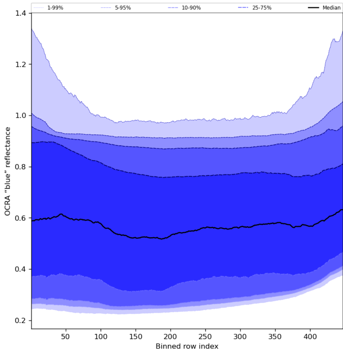
Figure 67: Along track statistics of "OCRA "blue" reflectance" for 2024-01-16 to 2024-01-18
