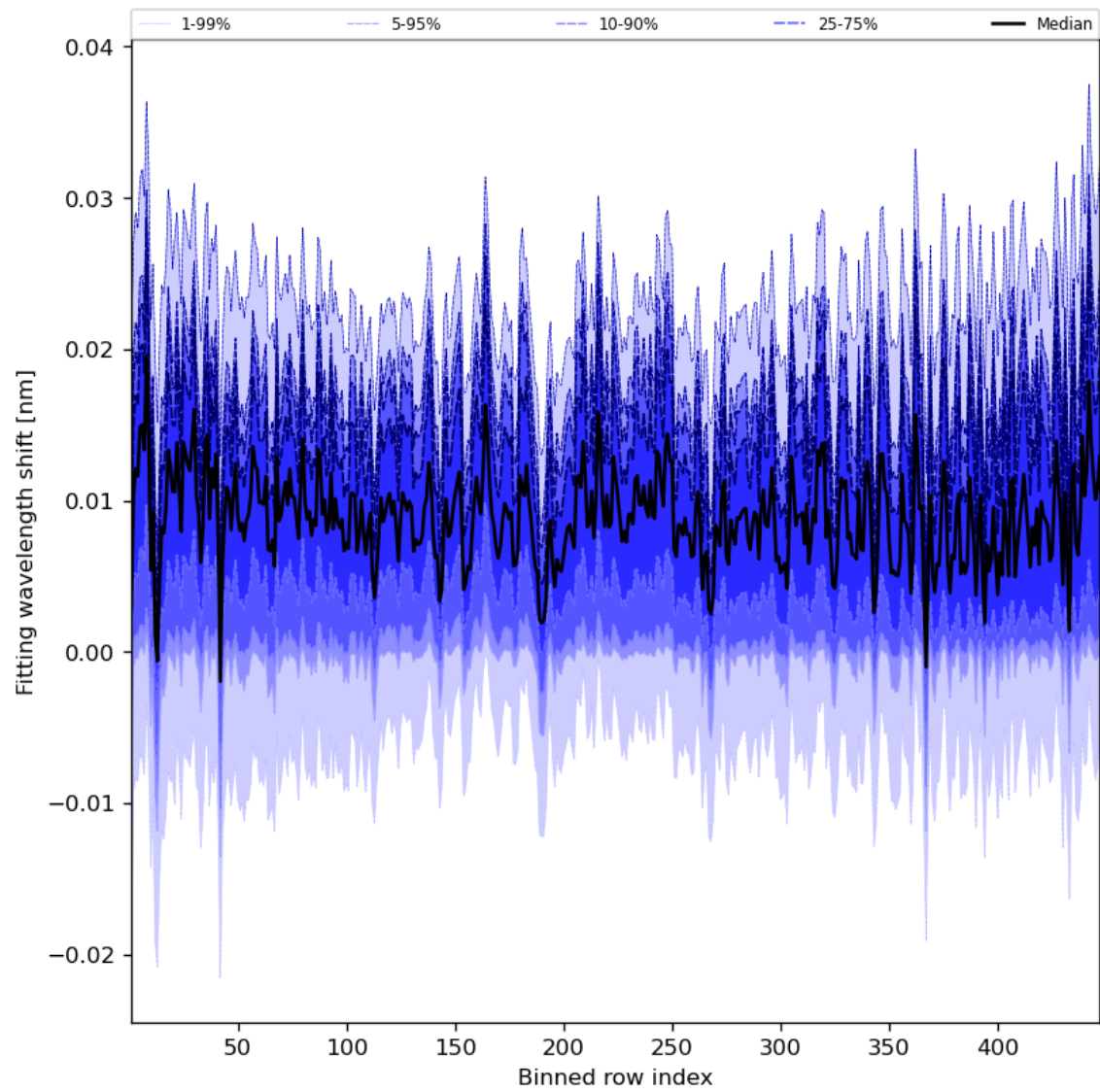
Figure 65: Along track statistics of “Fitting wavelength shift” for 2024-01-16 to 2024-01-18
