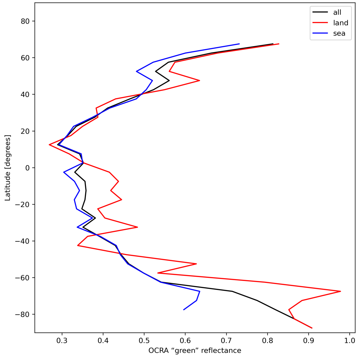
Figure 36: Zonal average of “OCRA “green” reflectance” for 2024-01-16 to 2024-01-18.
