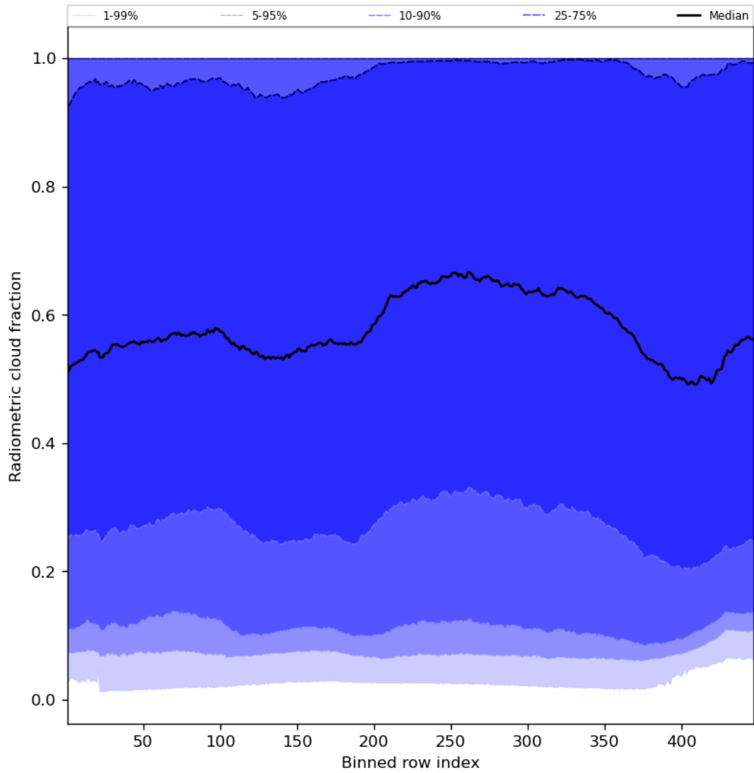
Figure 55: Along track statistics of “Radiometric cloud fraction” for 2024-01-16 to 2024-01-18
