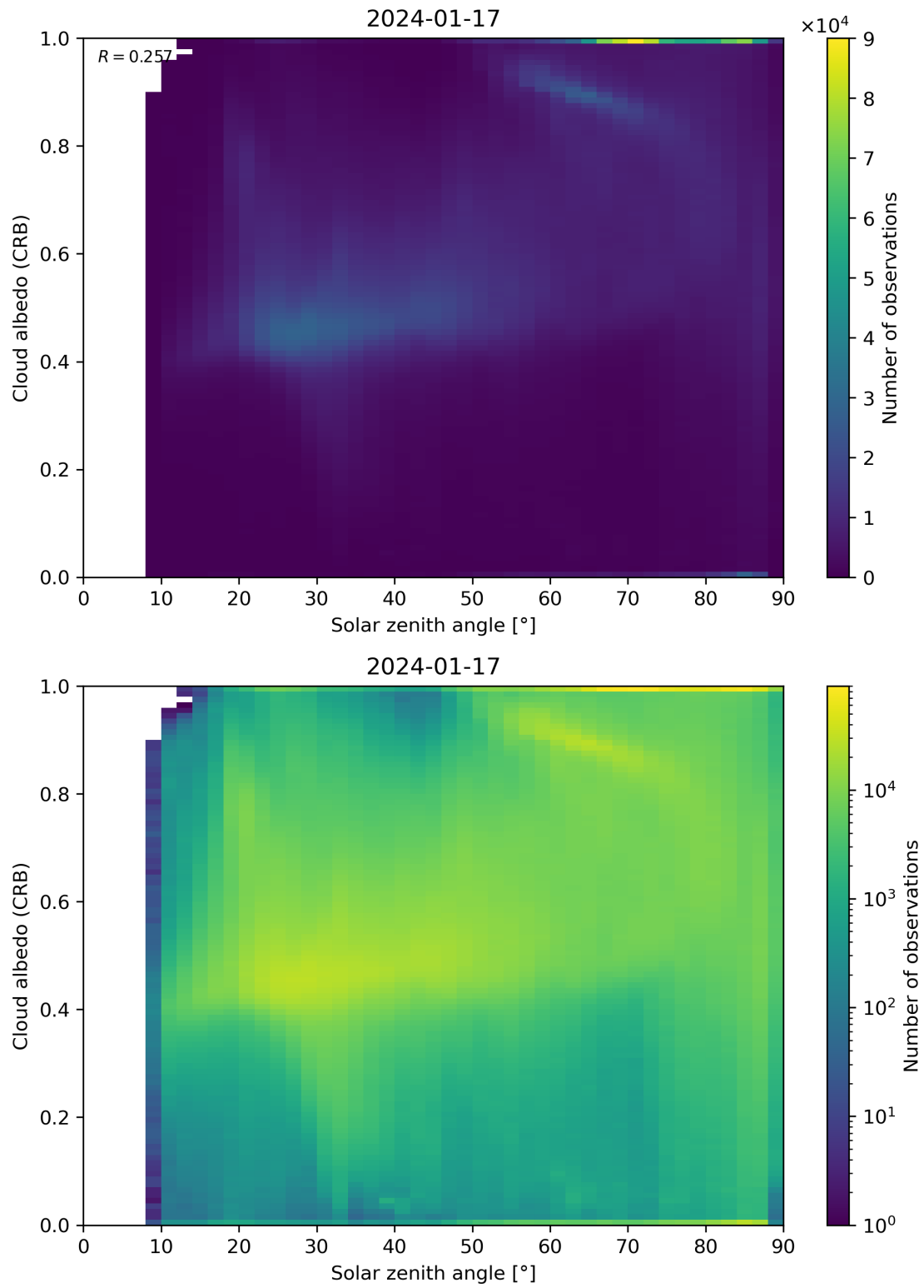
Figure 98: Scatter density plot of “Solar zenith angle” against “Cloud albedo (CRB)” for 2024-01-16 to 2024-01-18.
