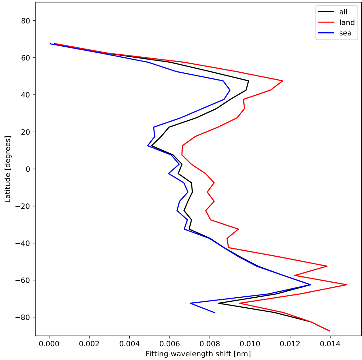
Figure 33: Zonal average of “Fitting wavelength shift” for 2024-01-16 to 2024-01-18.
