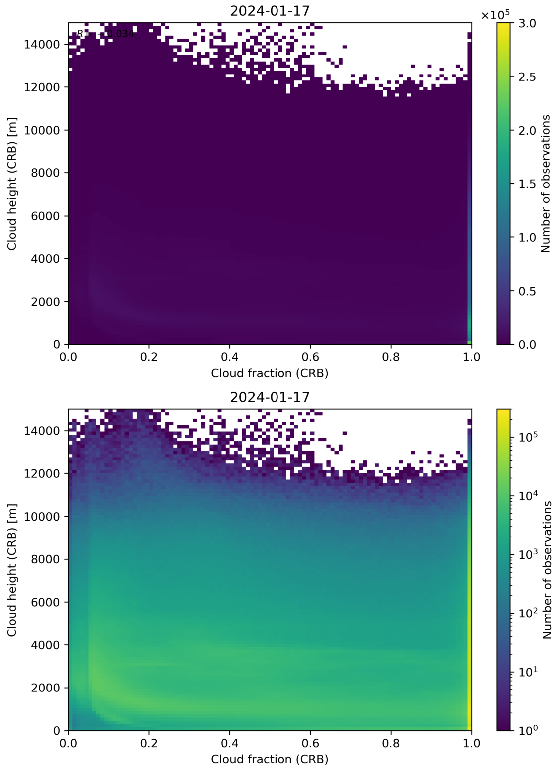
Figure 79: Scatter density plot of “Cloud fraction (CRB)” against “Cloud height (CRB)” for 2024-01-16 to 2024-01-18.
