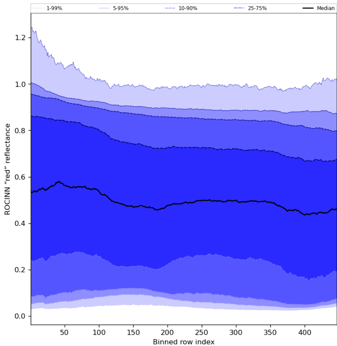
Figure 69: Along track statistics of “ROCINN “red” reflectance” for 2024-01-16 to 2024-01-18
