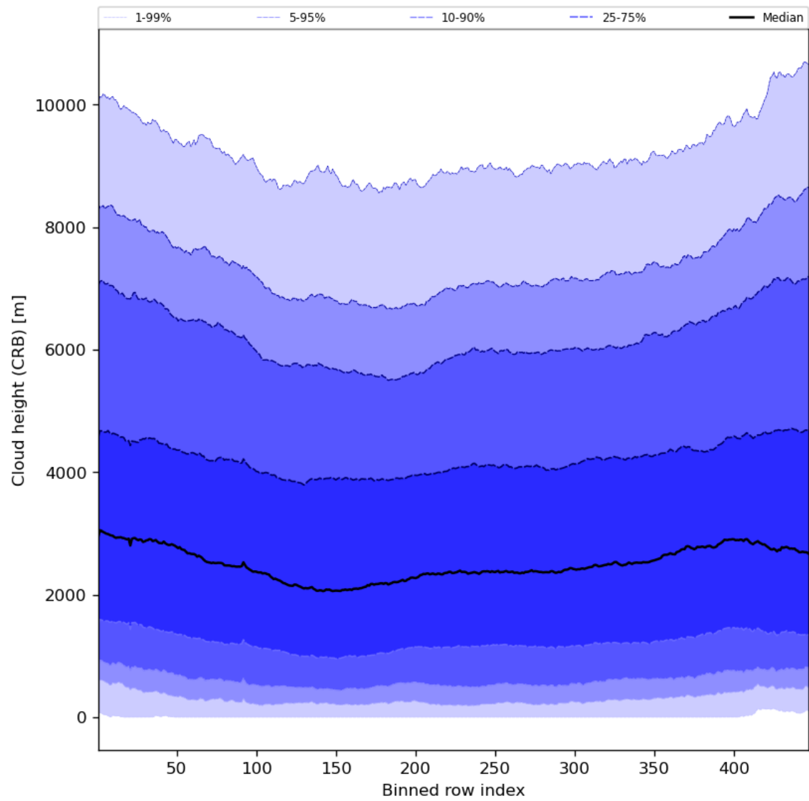
Figure 59: Along track statistics of “Cloud height (CRB)” for 2024-01-16 to 2024-01-18
