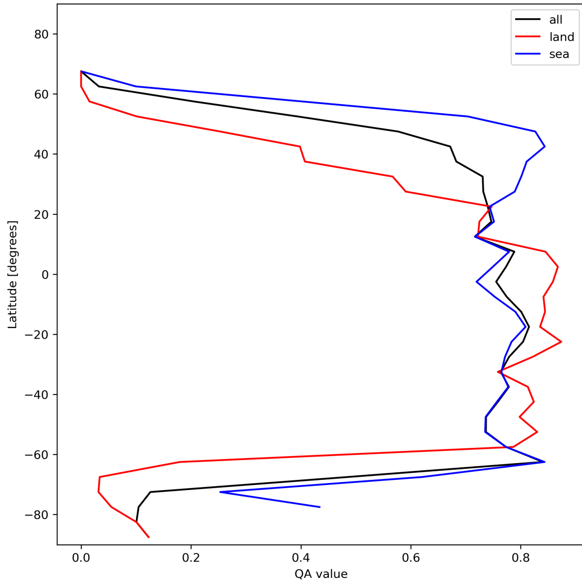
Figure 22: Zonal average of “QA value” for 2024-01-16 to 2024-01-18.
