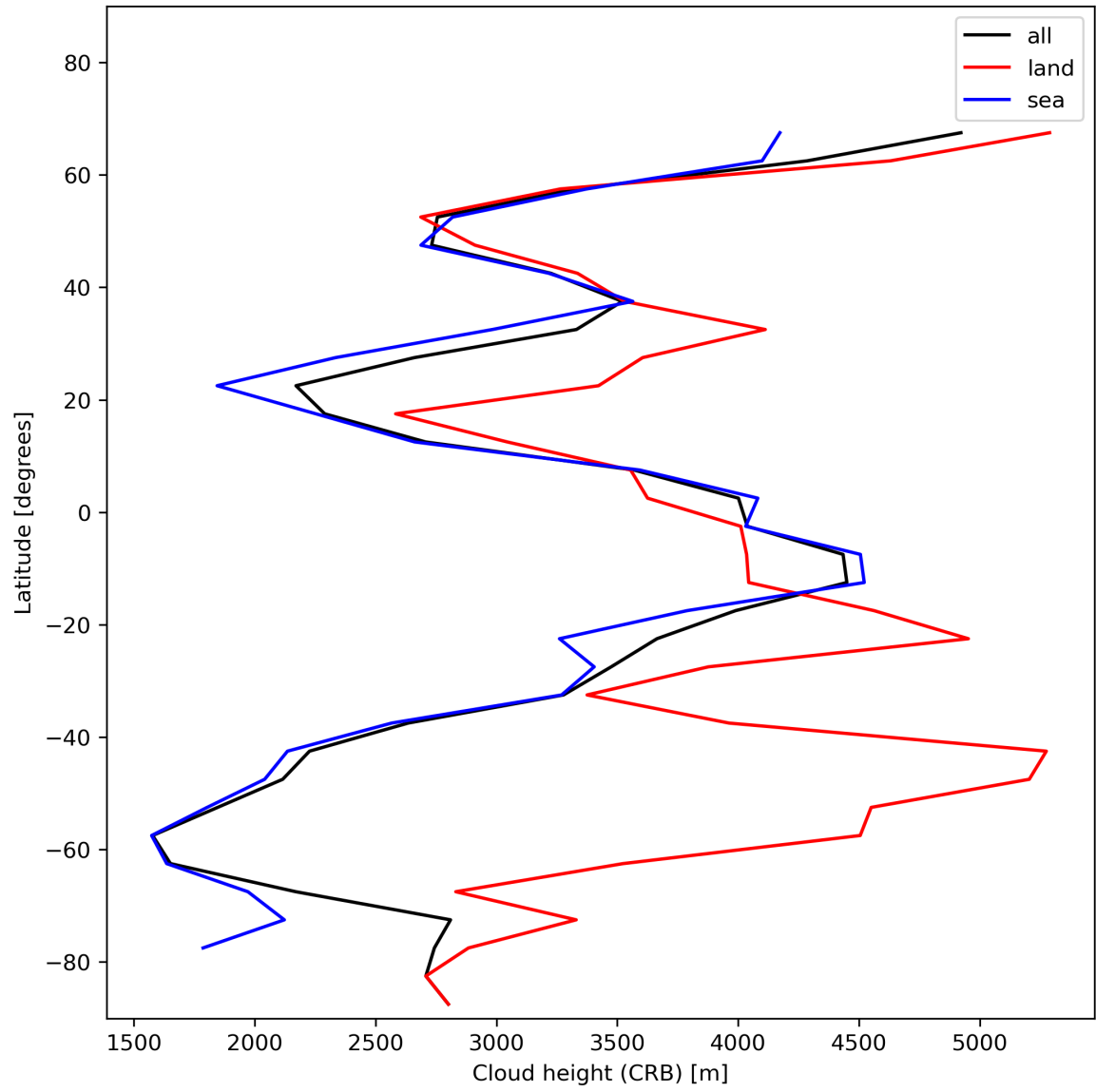
Figure 27: Zonal average of “Cloud height (CRB)” for 2024-01-16 to 2024-01-18.
