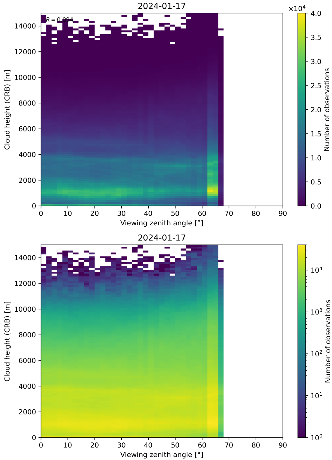
Figure 110: Scatter density plot of “Viewing zenith angle” against “Cloud height (CRB)” for 2024-01-16 to 2024-01-18.
