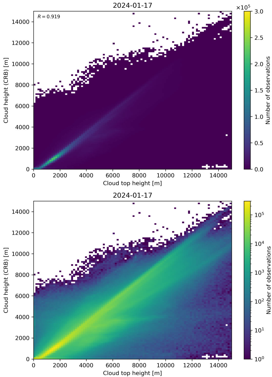
Figure 89: Scatter density plot of “Cloud top height” against “Cloud height (CRB)” for 2024-01-16 to 2024-01-18.
