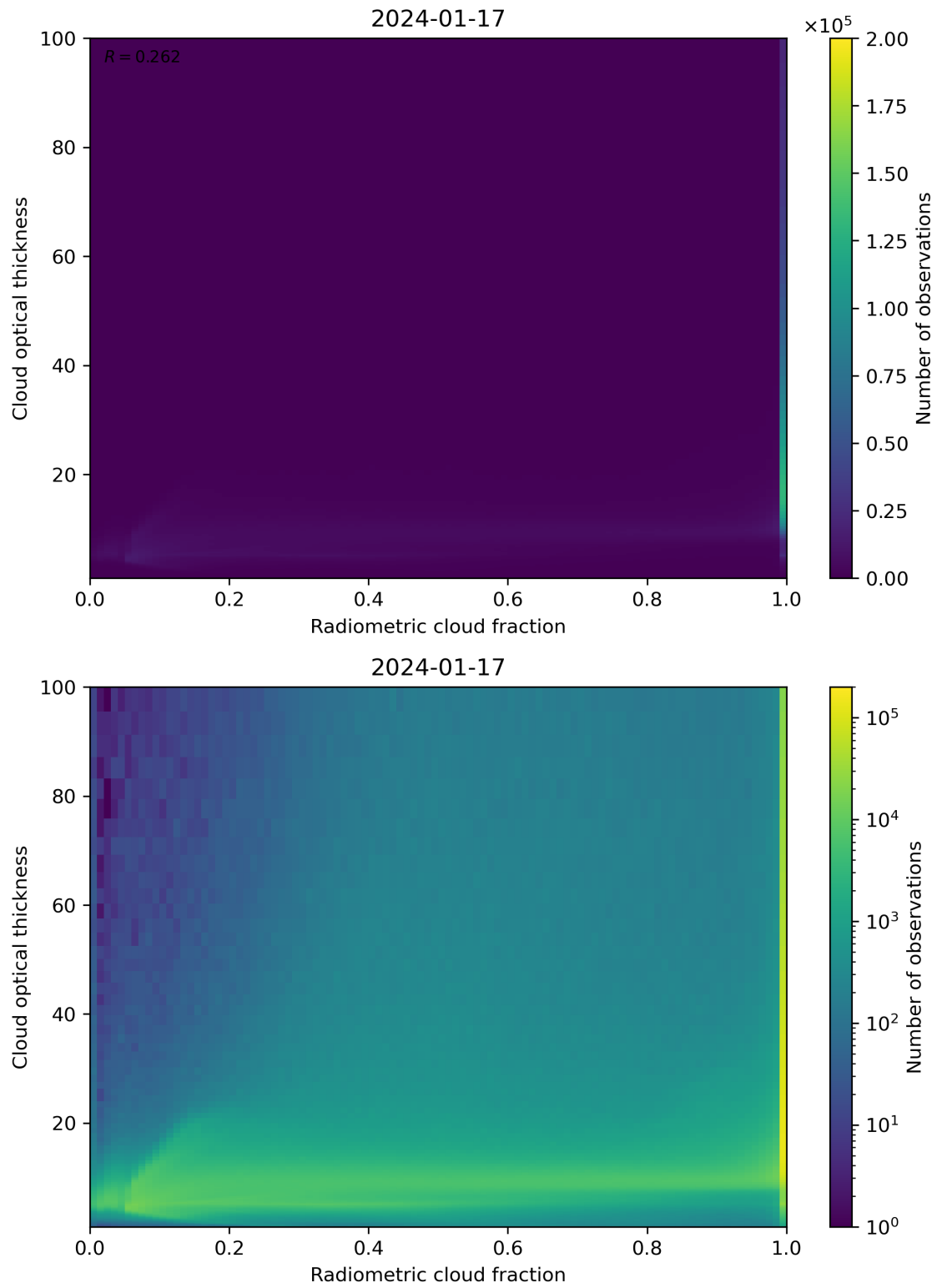
Figure 75: Scatter density plot of “Radiometric cloud fraction” against “Cloud optical thickness” for 2024-01-16 to 2024-01-18.
