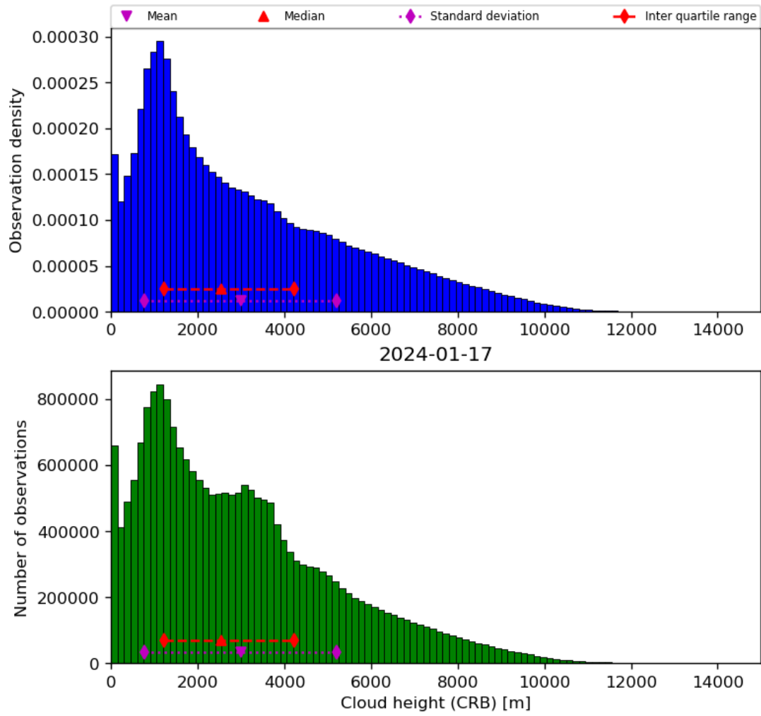
Figure 43: Histogram of “Cloud height (CRB)” for 2024-01-16 to 2024-01-18
