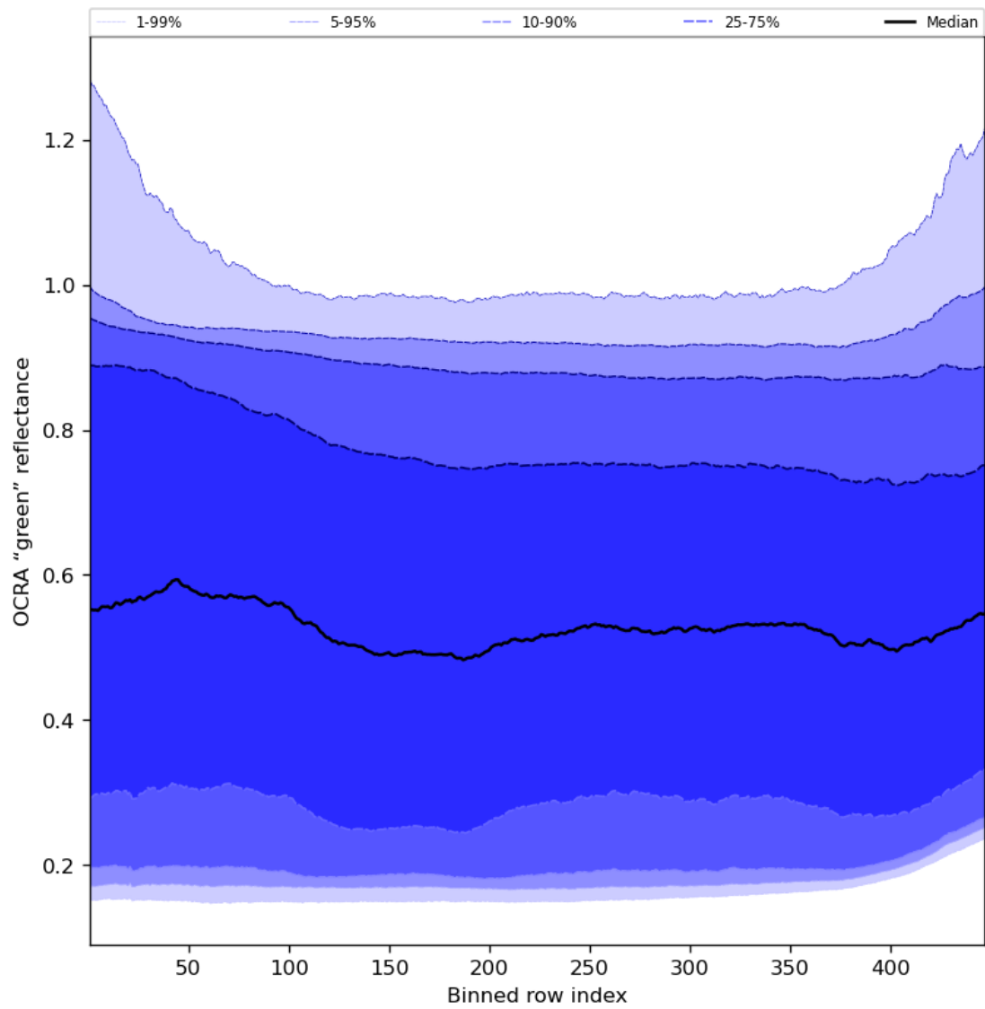
Figure 68: Along track statistics of “OCRA “green” reflectance” for 2024-01-16 to 2024-01-18
