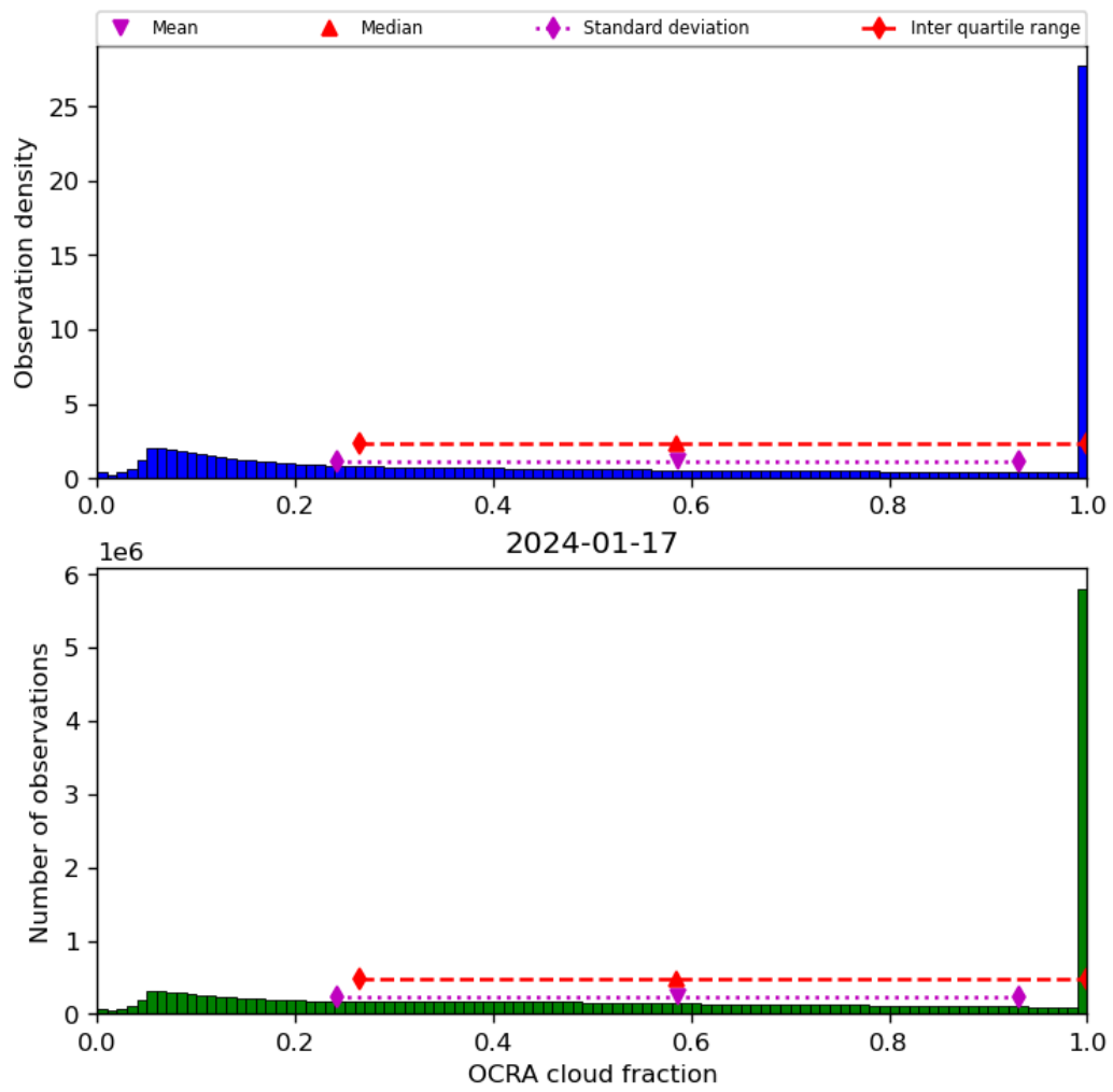
Figure 50: Histogram of “OCRA cloud fraction” for 2024-01-16 to 2024-01-18
