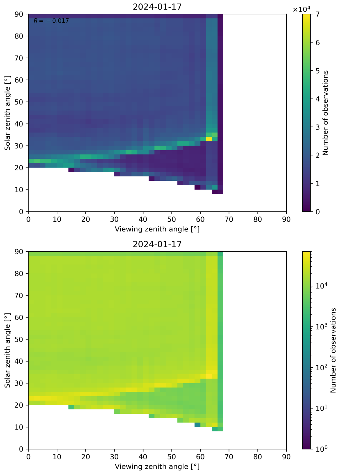
Figure 114: Scatter density plot of “Viewing zenith angle” against “Solar zenith angle” for 2024-01-16 to 2024-01-18.
