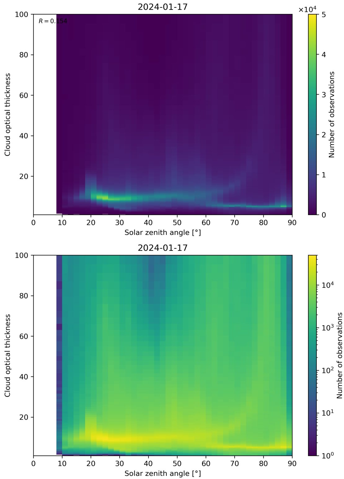
Figure 103: Scatter density plot of “Solar zenith angle” against “Cloud optical thickness” for 2024-01-16 to 2024-01-18.
