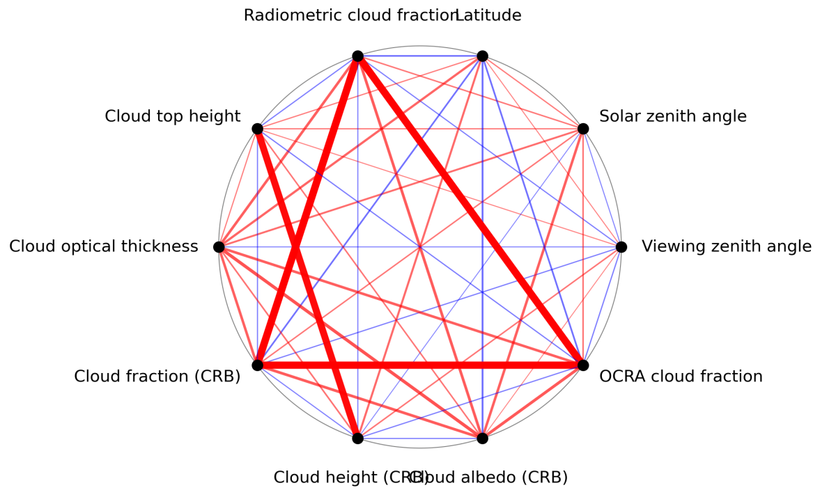
Figure 1: Map of correlation graph for 2024-01-16 to 2024-01-18.
