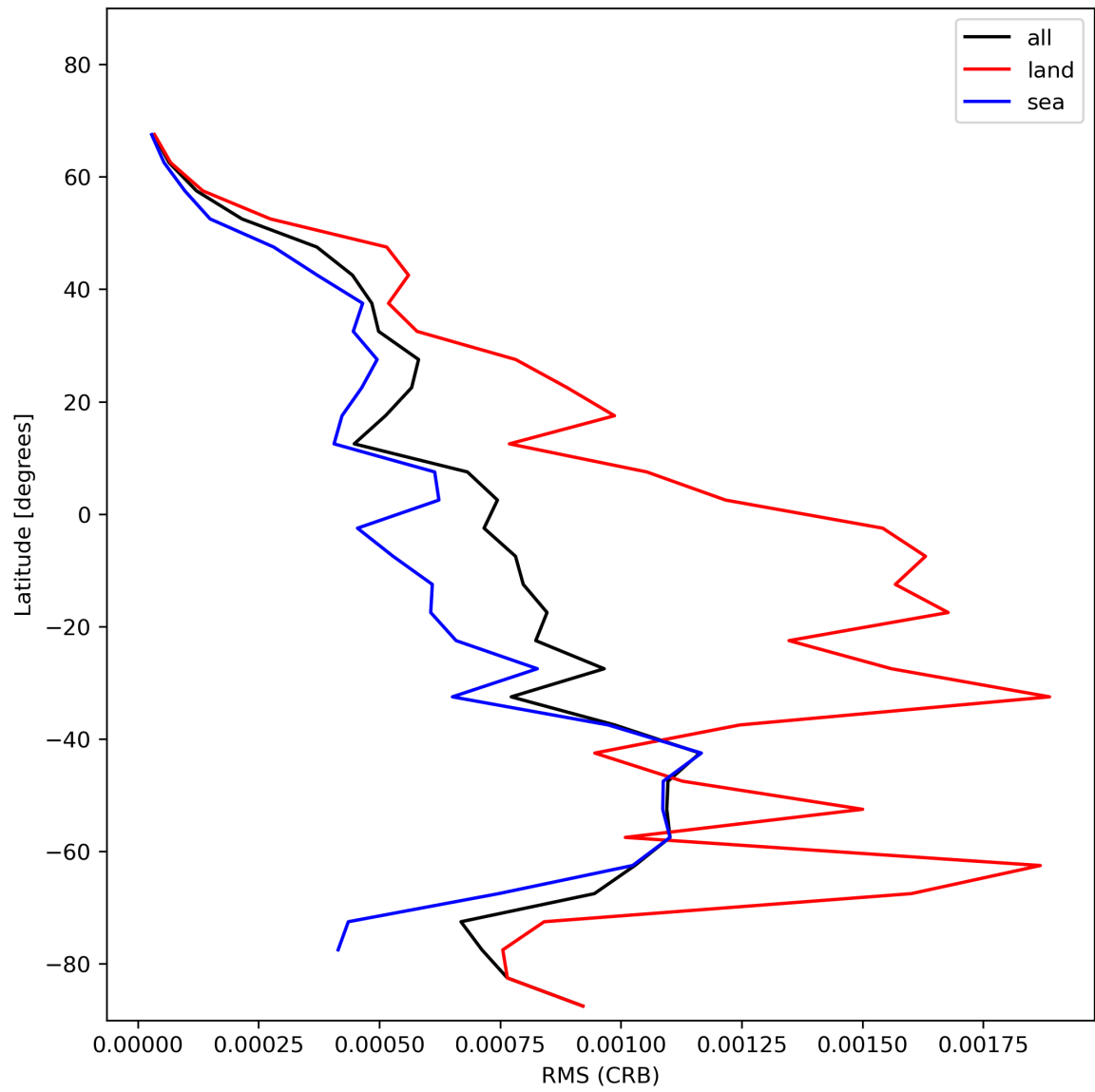
Figure 32: Zonal average of “RMS (CRB)” for 2024-01-16 to 2024-01-18.
