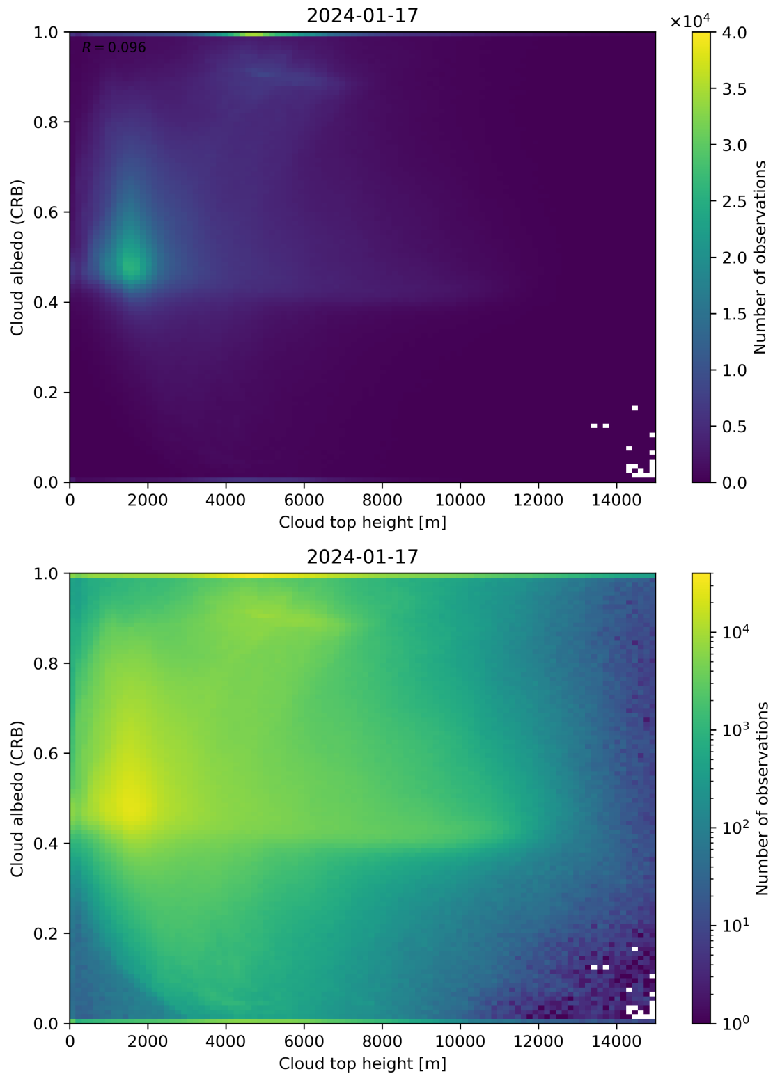
Figure 86: Scatter density plot of “Cloud top height” against “Cloud albedo (CRB)” for 2024-01-16 to 2024-01-18.
