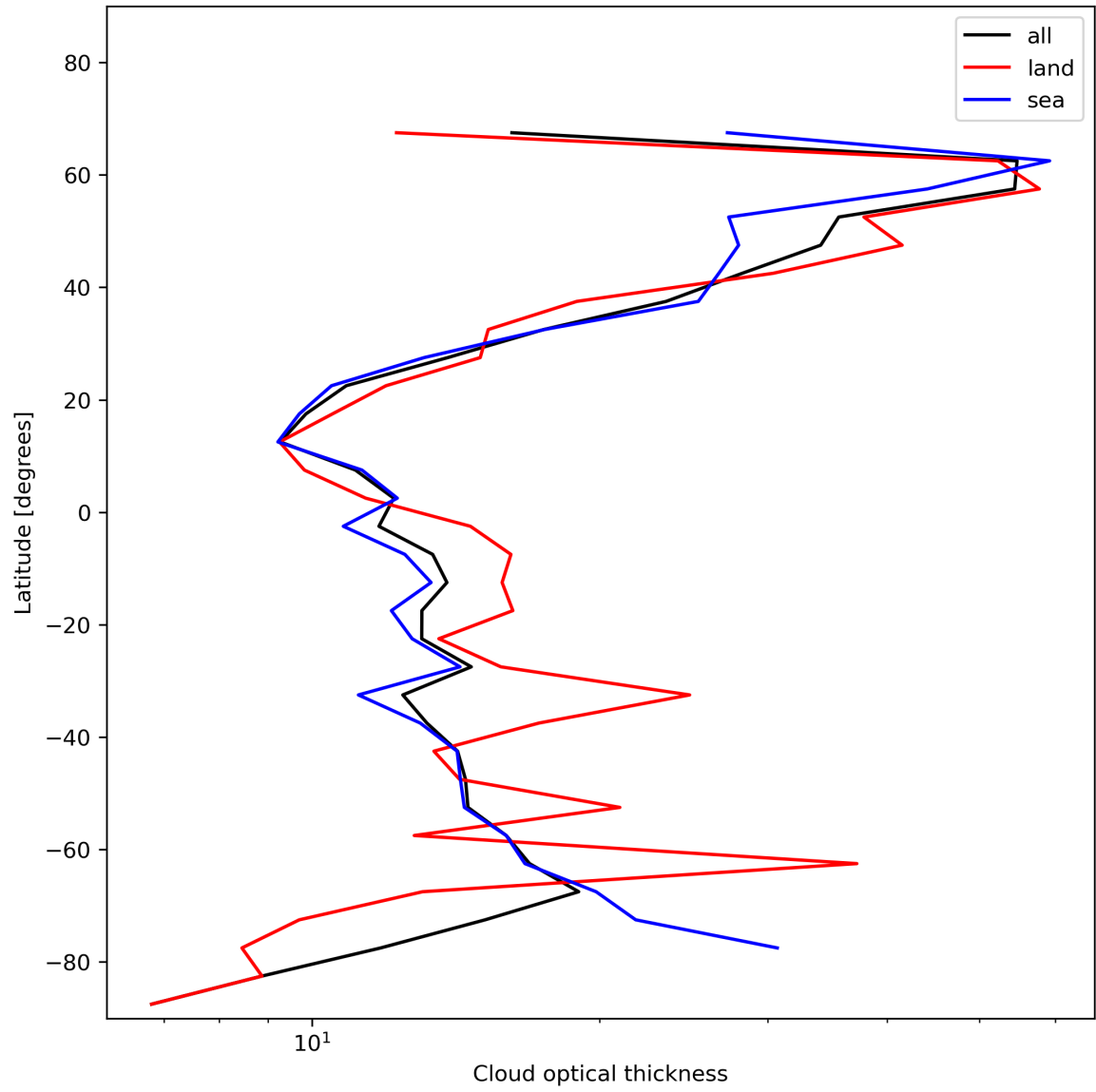
Figure 25: Zonal average of “Cloud optical thickness” for 2024-01-16 to 2024-01-18.
