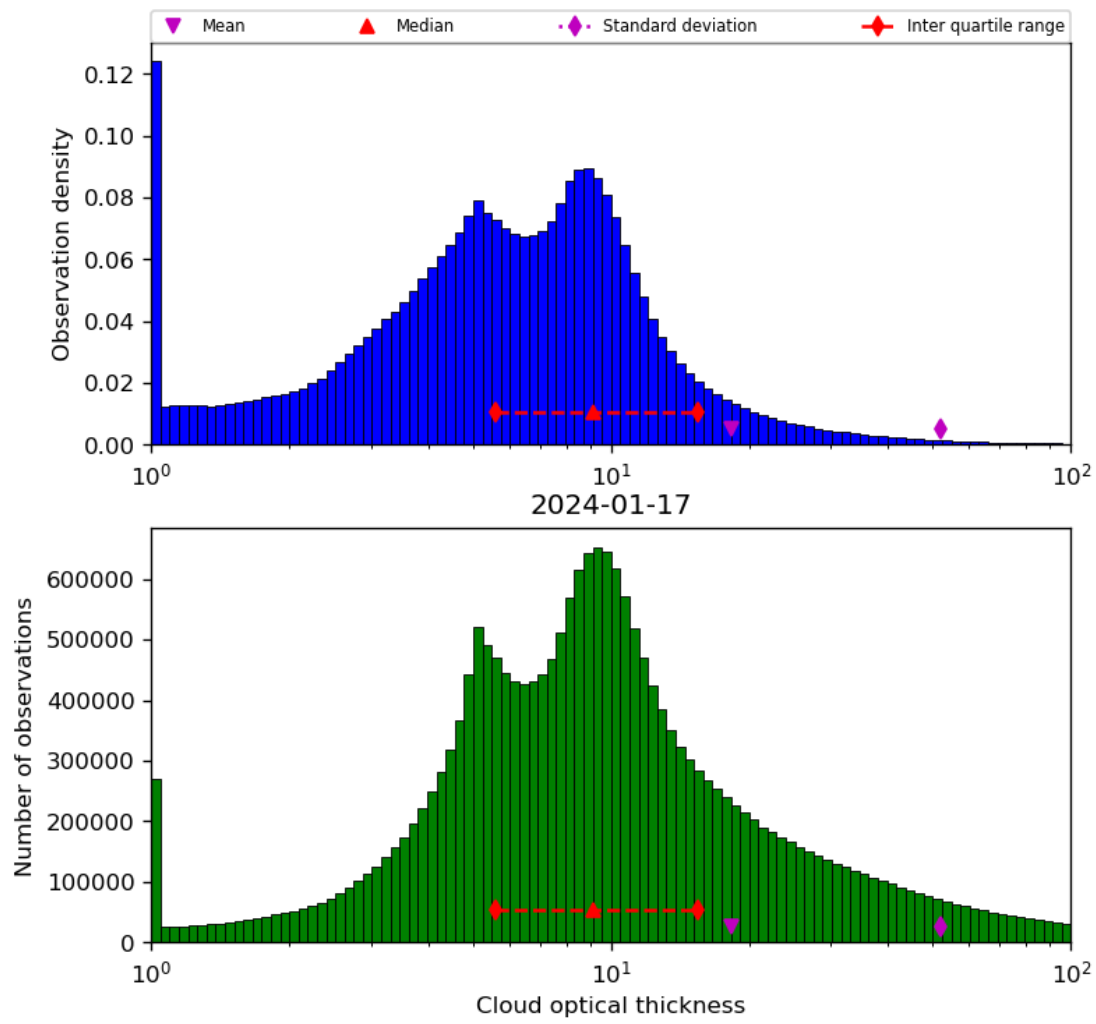
Figure 41: Histogram of “Cloud optical thickness” for 2024-01-16 to 2024-01-18
