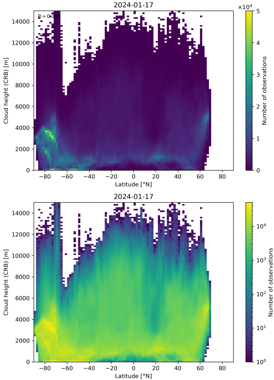
Figure 95: Scatter density plot of “Latitude” against “Cloud height (CRB)” for 2024-01-16 to 2024-01-18.
