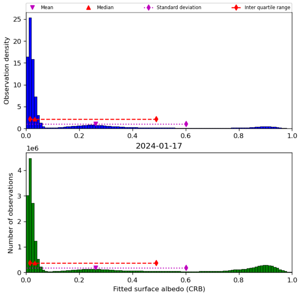
Figure 46: Histogram of “Fitted surface albedo (CRB)” for 2024-01-16 to 2024-01-18
