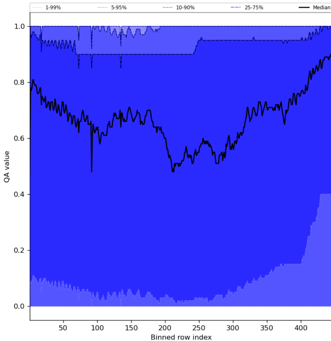
Figure 54: Along track statistics of “QA value” for 2024-01-16 to 2024-01-18
