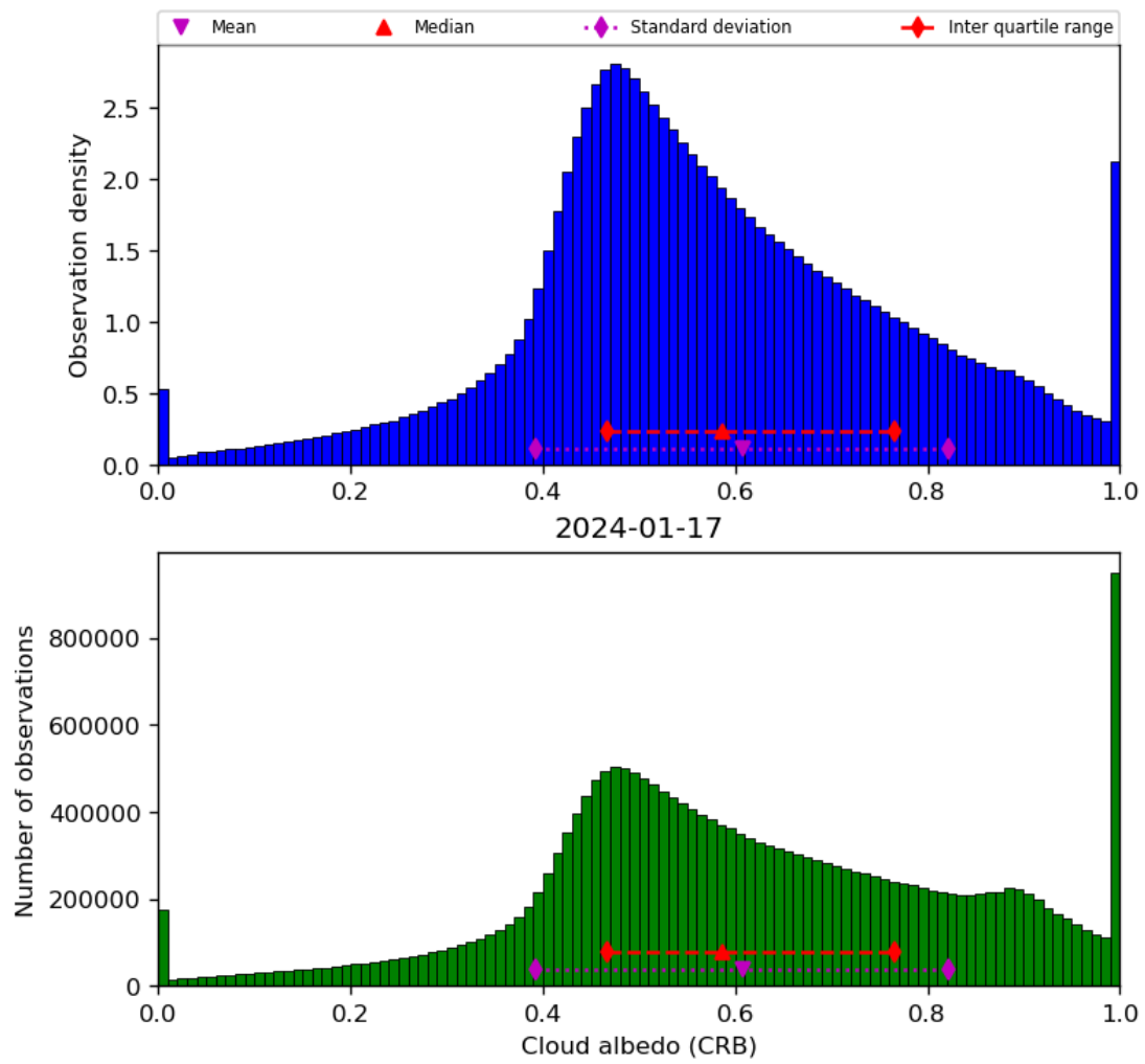
Figure 44: Histogram of “Cloud albedo (CRB)” for 2024-01-16 to 2024-01-18
