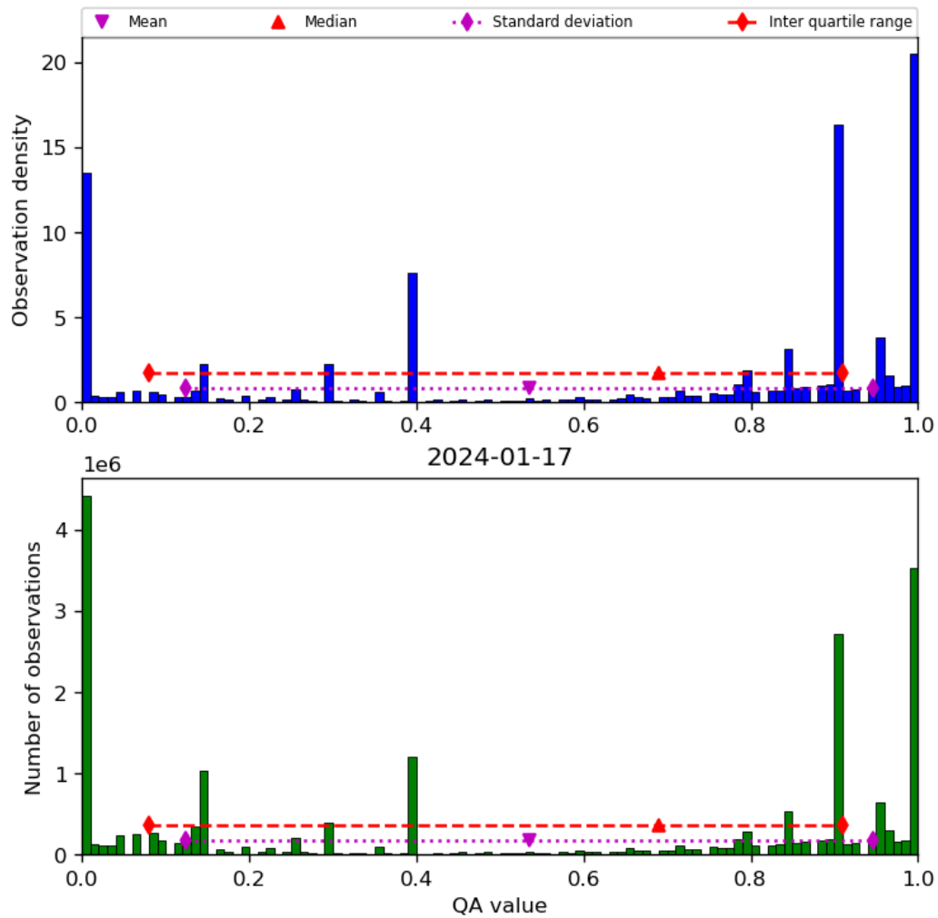
Figure 38: Histogram of “QA value” for 2024-01-16 to 2024-01-18
