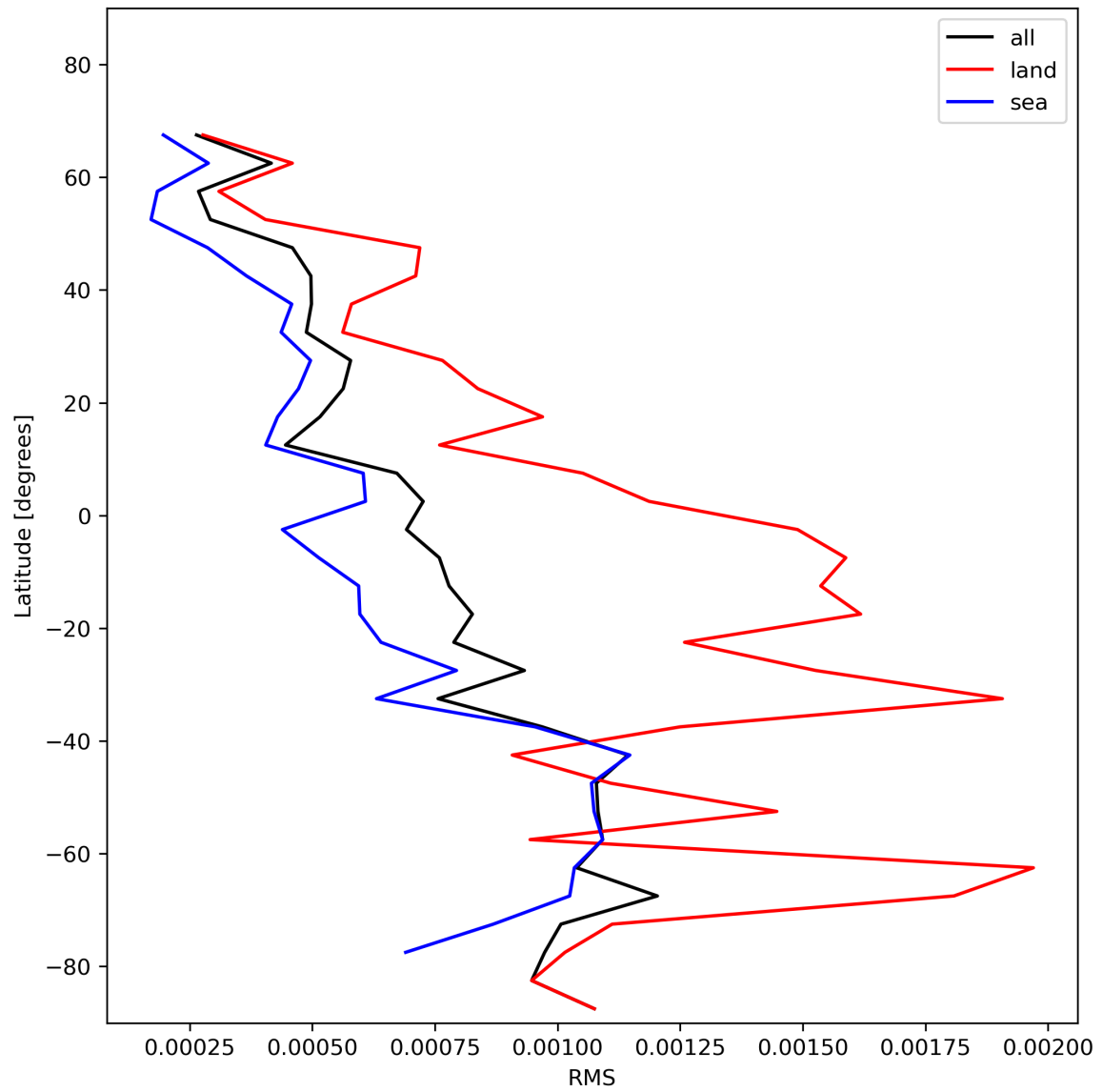
Figure 31: Zonal average of “RMS” for 2024-01-16 to 2024-01-18.
