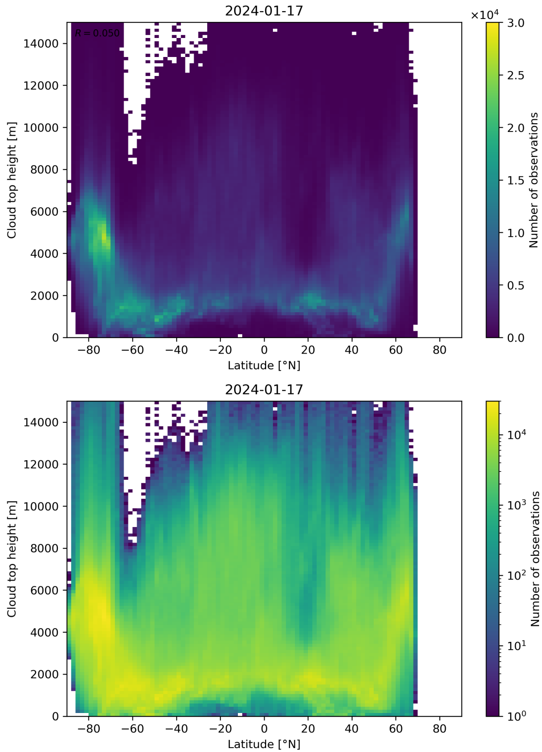
Figure 97: Scatter density plot of “Latitude” against “Cloud top height” for 2024-01-16 to 2024-01-18.
