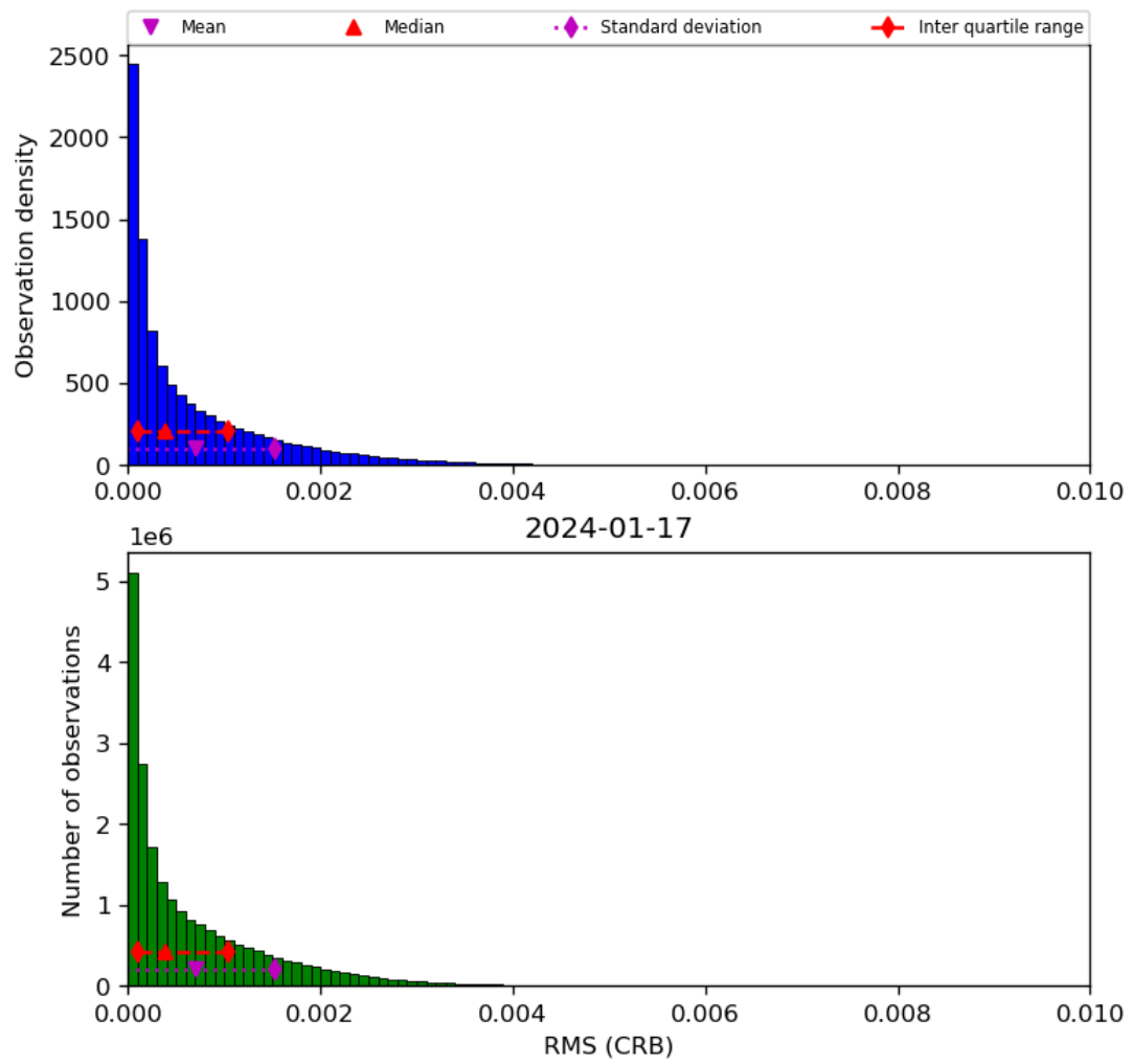
Figure 48: Histogram of “RMS (CRB)” for 2024-01-16 to 2024-01-18
