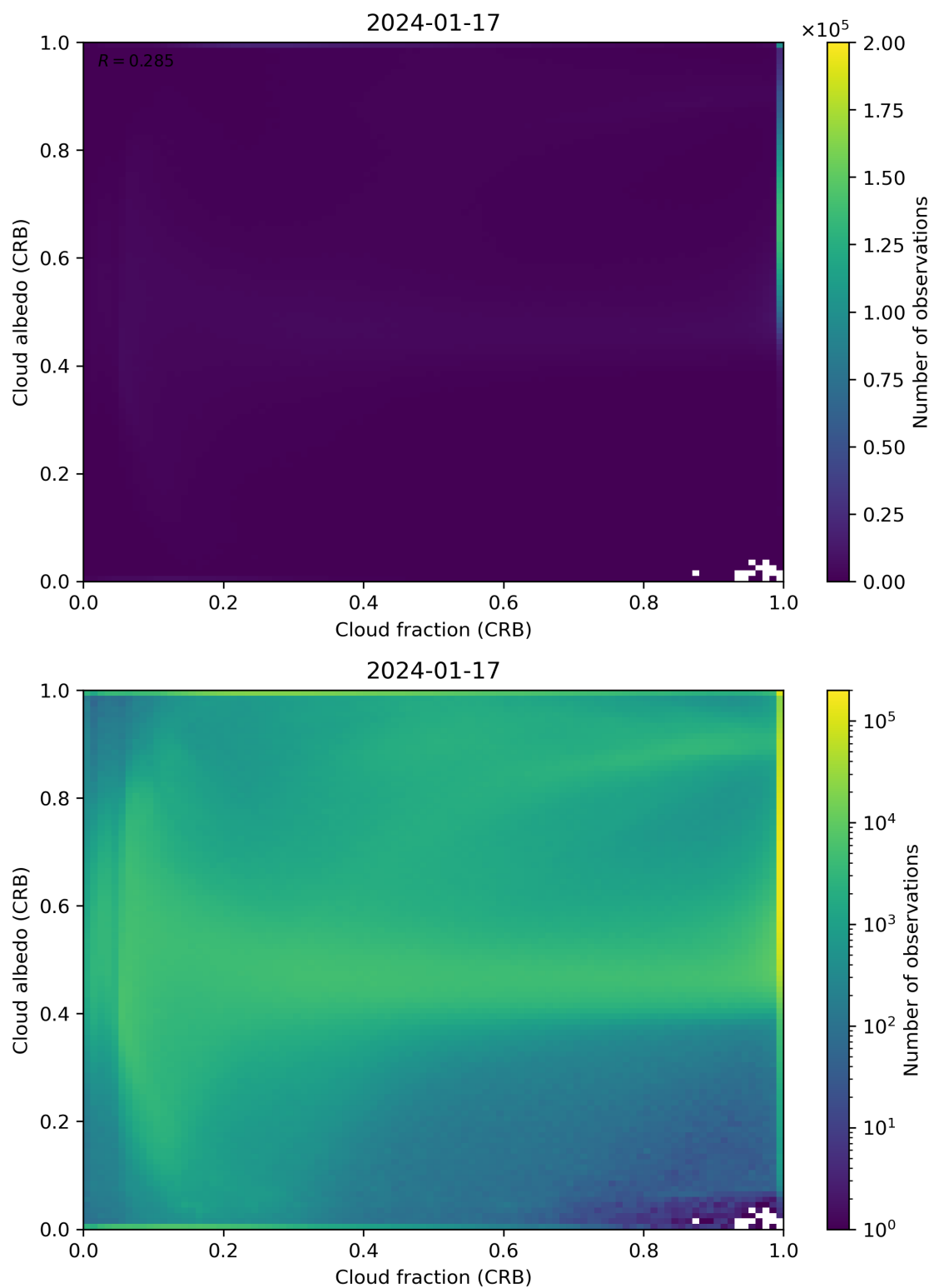
Figure 77: Scatter density plot of “Cloud fraction (CRB)” against “Cloud albedo (CRB)” for 2024-01-16 to 2024-01-18.
