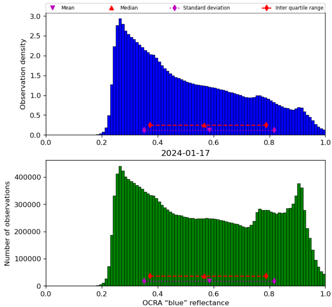
Figure 51: Histogram of “OCRA “blue” reflectance” for 2024-01-16 to 2024-01-18
