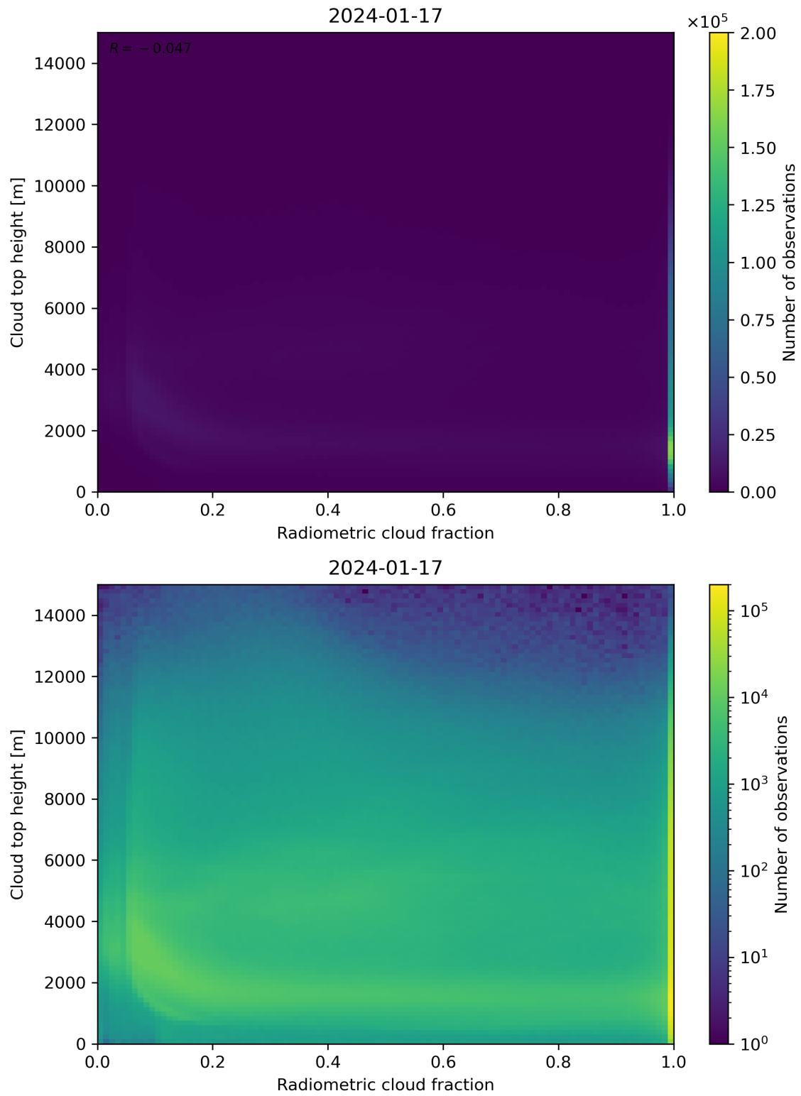
Figure 76: Scatter density plot of “Radiometric cloud fraction” against “Cloud top height” for 2024-01-16 to 2024-01-18.
