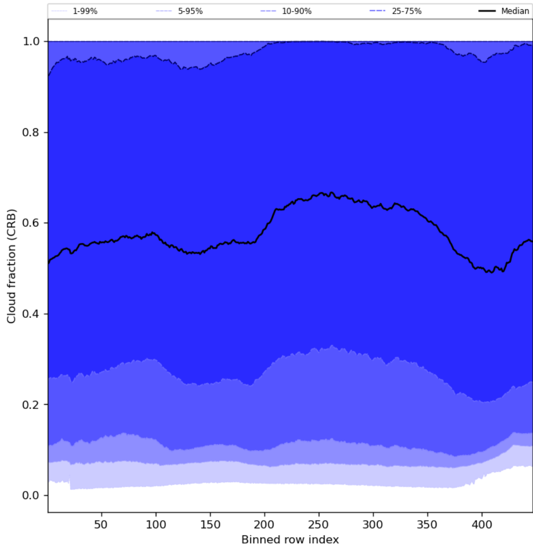
Figure 58: Along track statistics of “Cloud fraction (CRB)” for 2024-01-16 to 2024-01-18
