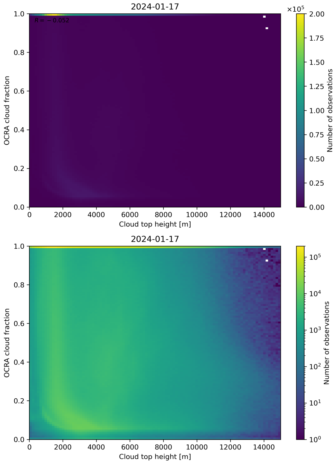
Figure 87: Scatter density plot of “Cloud top height” against “OCRA cloud fraction” for 2024-01-16 to 2024-01-18.
