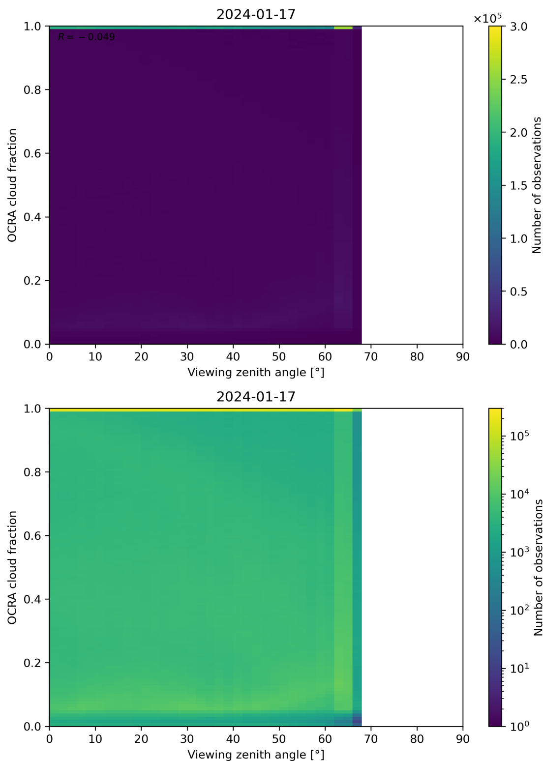
Figure 108: Scatter density plot of “Viewing zenith angle” against “OCRA cloud fraction” for 2024-01-16 to 2024-01-18.
