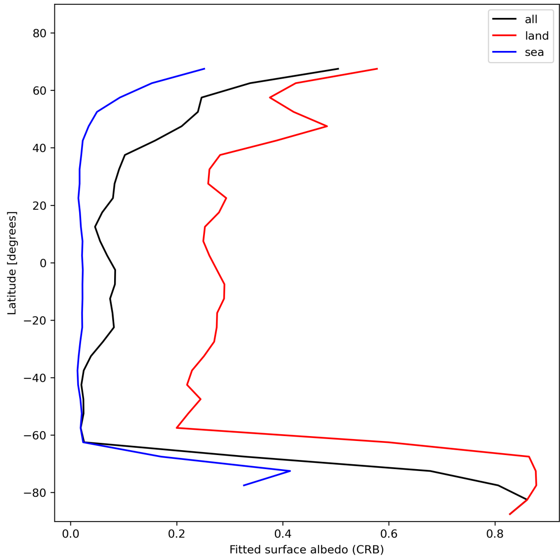
Figure 30: Zonal average of “Fitted surface albedo (CRB)” for 2024-01-16 to 2024-01-18.
