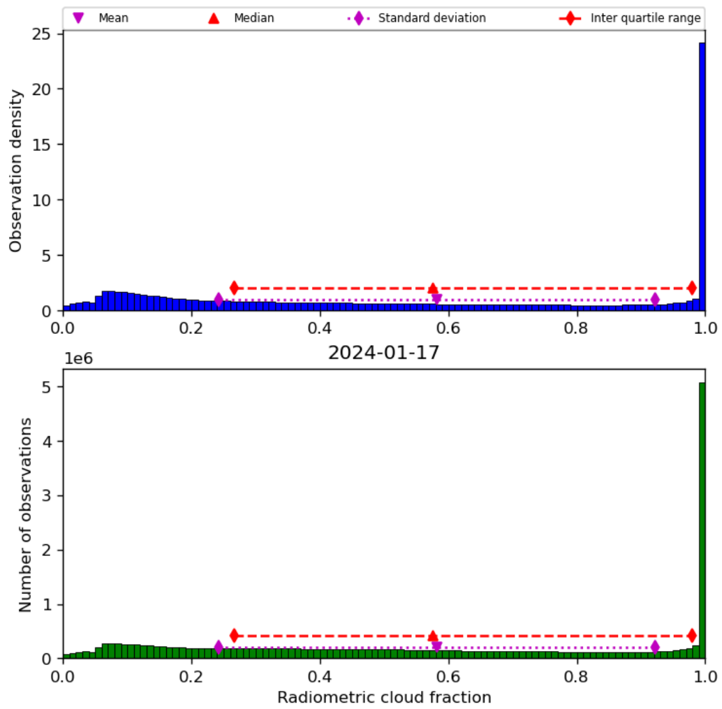
Figure 39: Histogram of “Radiometric cloud fraction” for 2024-01-16 to 2024-01-18
