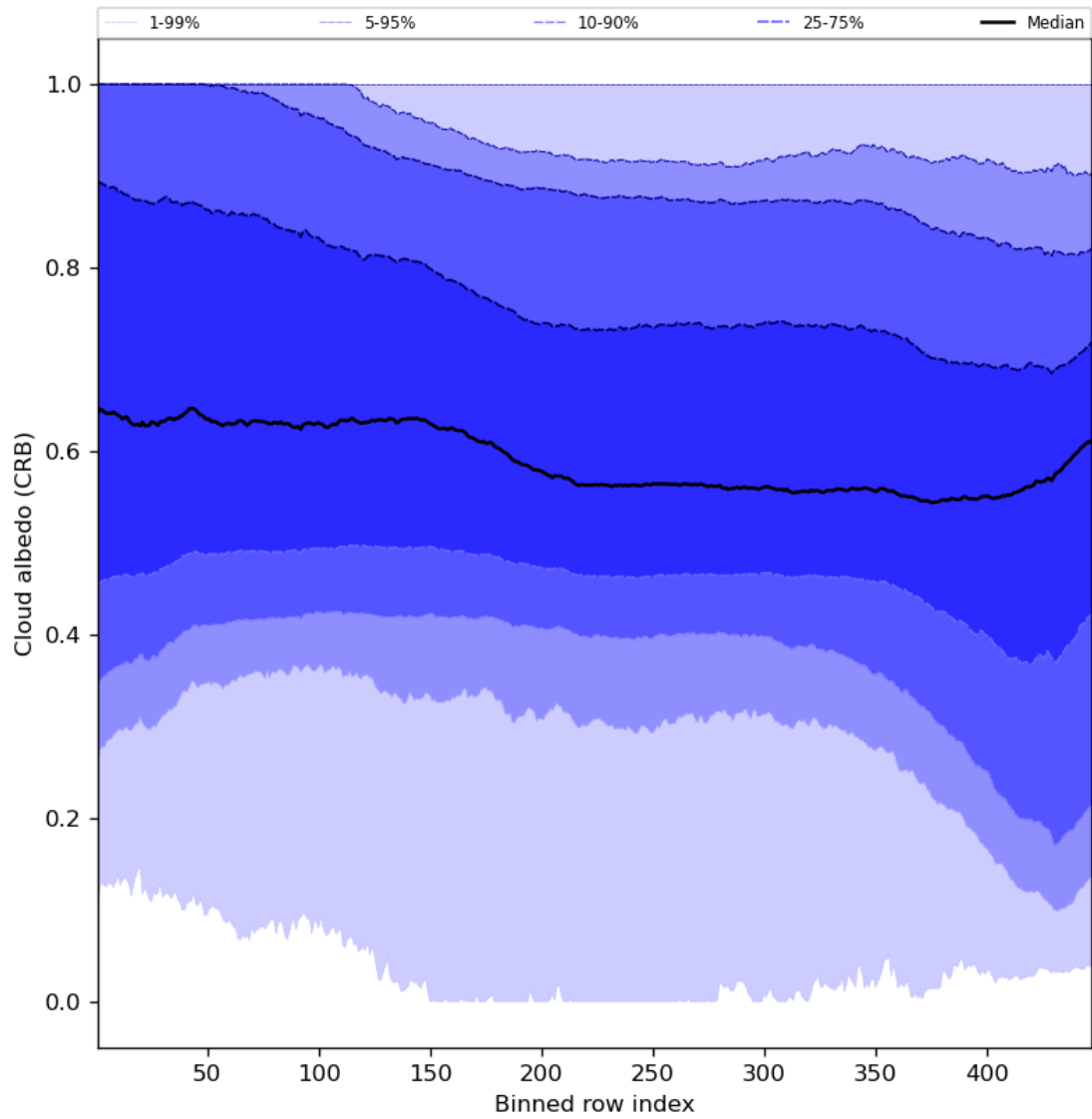
Figure 60: Along track statistics of “Cloud albedo (CRB)” for 2024-01-16 to 2024-01-18
