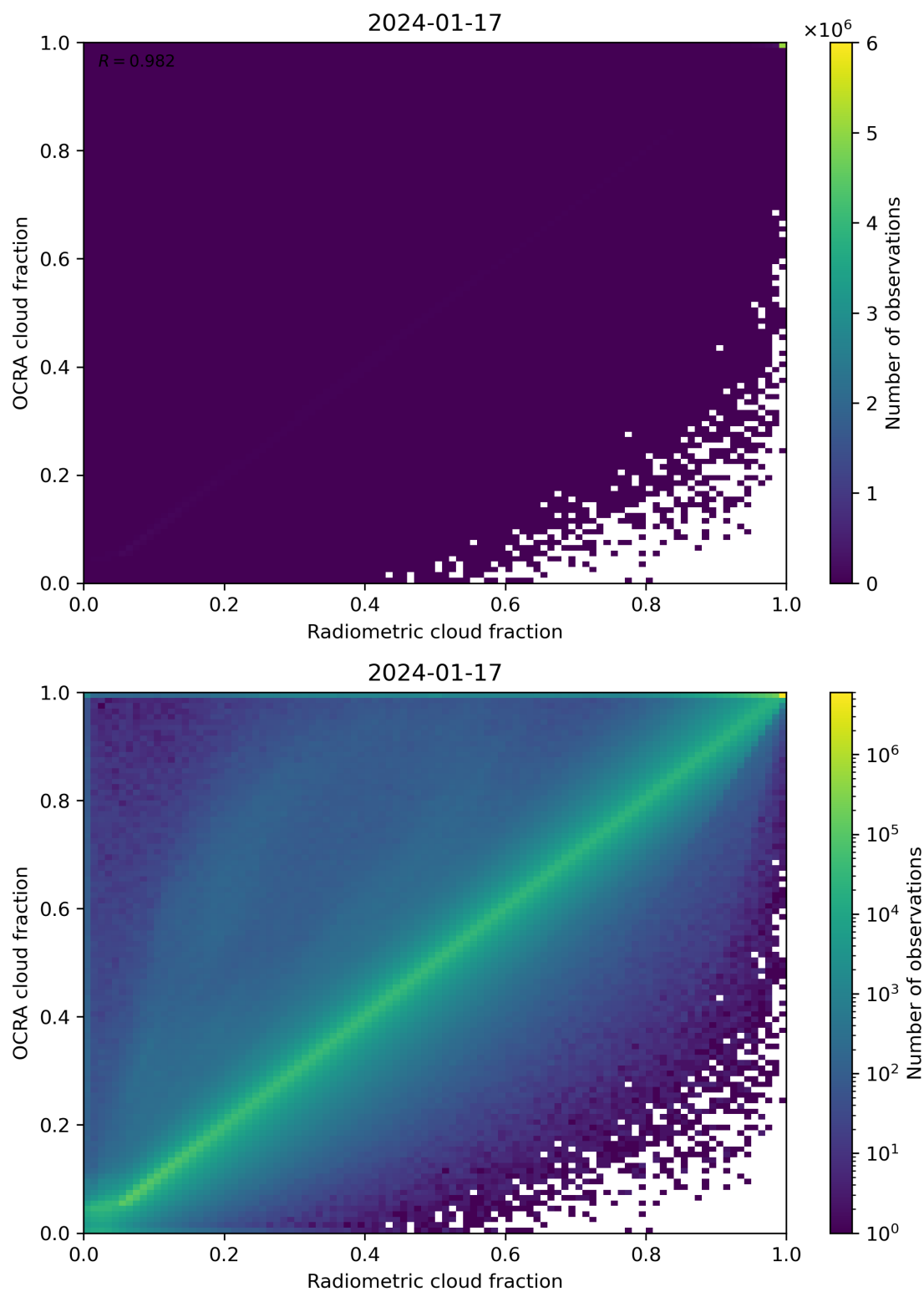
Figure 72: Scatter density plot of “Radiometric cloud fraction” against “OCRA cloud fraction” for 2024-01-16 to 2024-01-18.
