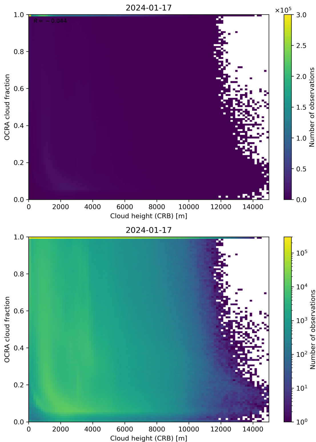
Figure 81: Scatter density plot of “Cloud height (CRB)” against “OCRA cloud fraction” for 2024-01-16 to 2024-01-18.
