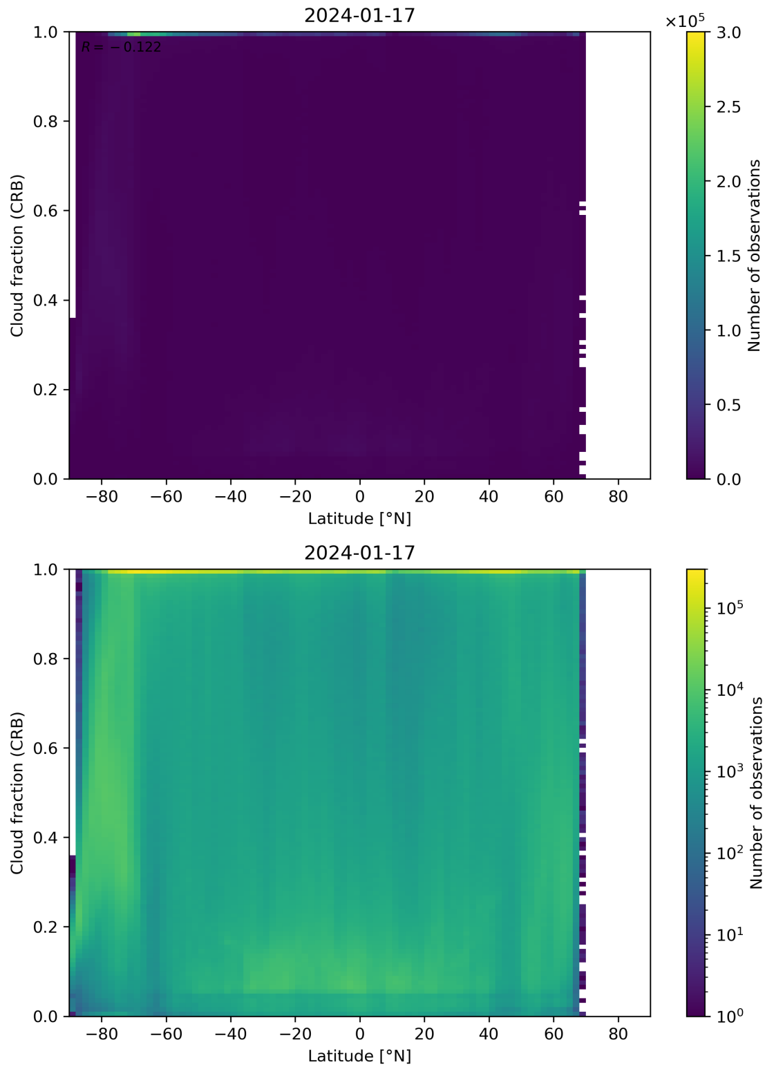
Figure 94: Scatter density plot of “Latitude” against “Cloud fraction (CRB)” for 2024-01-16 to 2024-01-18.
