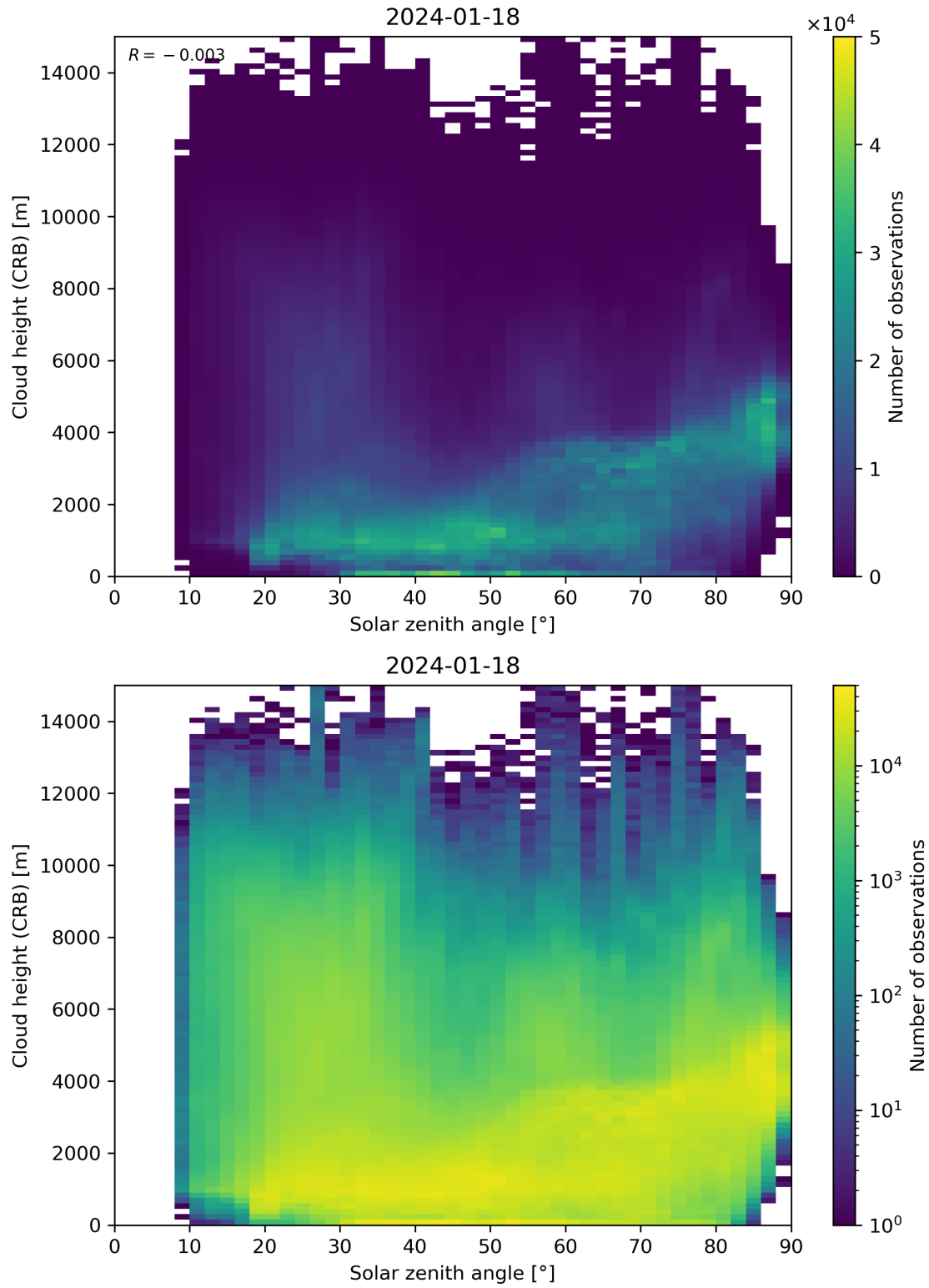
Figure 102: Scatter density plot of “Solar zenith angle” against “Cloud height (CRB)” for 2024-01-17 to 2024-01-19.
