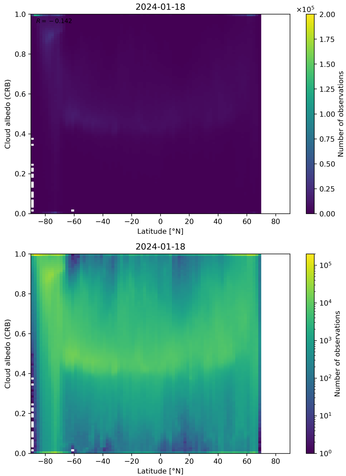
Figure 91: Scatter density plot of “Latitude” against “Cloud albedo (CRB)” for 2024-01-17 to 2024-01-19.
