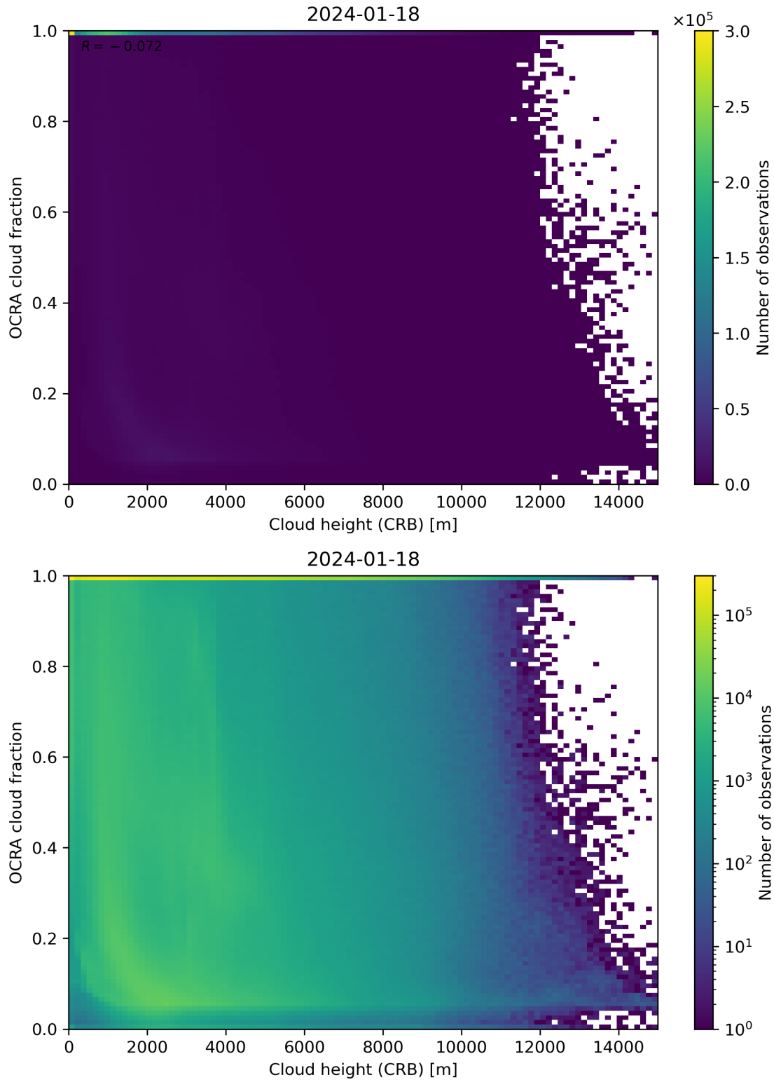
Figure 81: Scatter density plot of “Cloud height (CRB)” against “OCRA cloud fraction” for 2024-01-17 to 2024-01-19.
