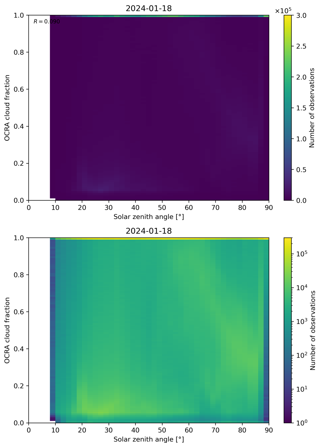
Figure 100: Scatter density plot of “Solar zenith angle” against “OCRA cloud fraction” for 2024-01-17 to 2024-01-19.
