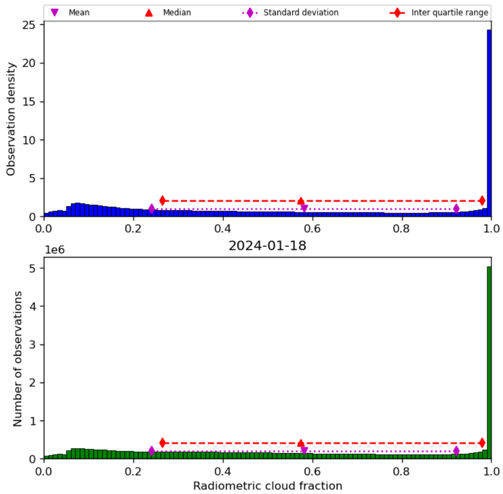
Figure 39: Histogram of “Radiometric cloud fraction” for 2024-01-17 to 2024-01-19
