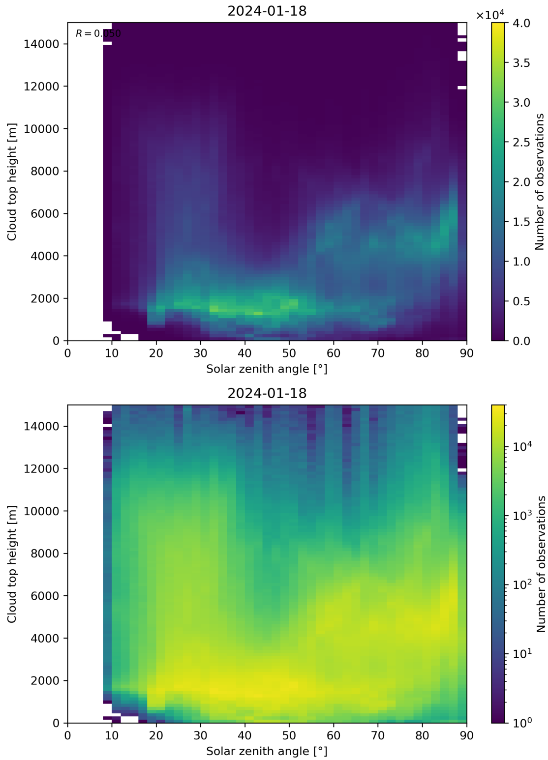
Figure 104: Scatter density plot of “Solar zenith angle” against “Cloud top height” for 2024-01-17 to 2024-01-19.
