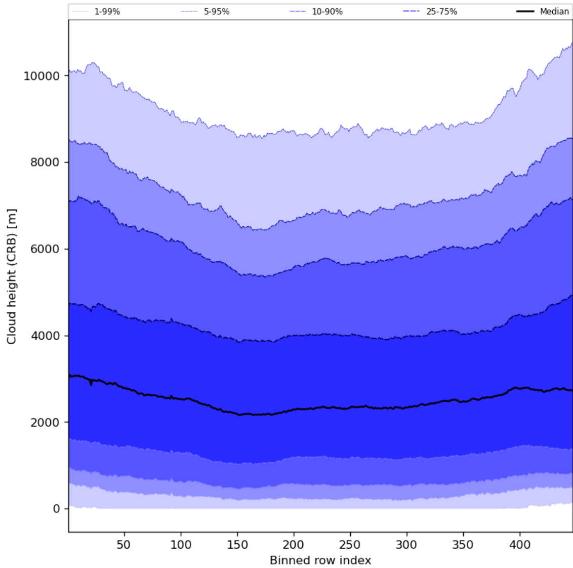
Figure 59: Along track statistics of “Cloud height (CRB)” for 2024-01-17 to 2024-01-19
