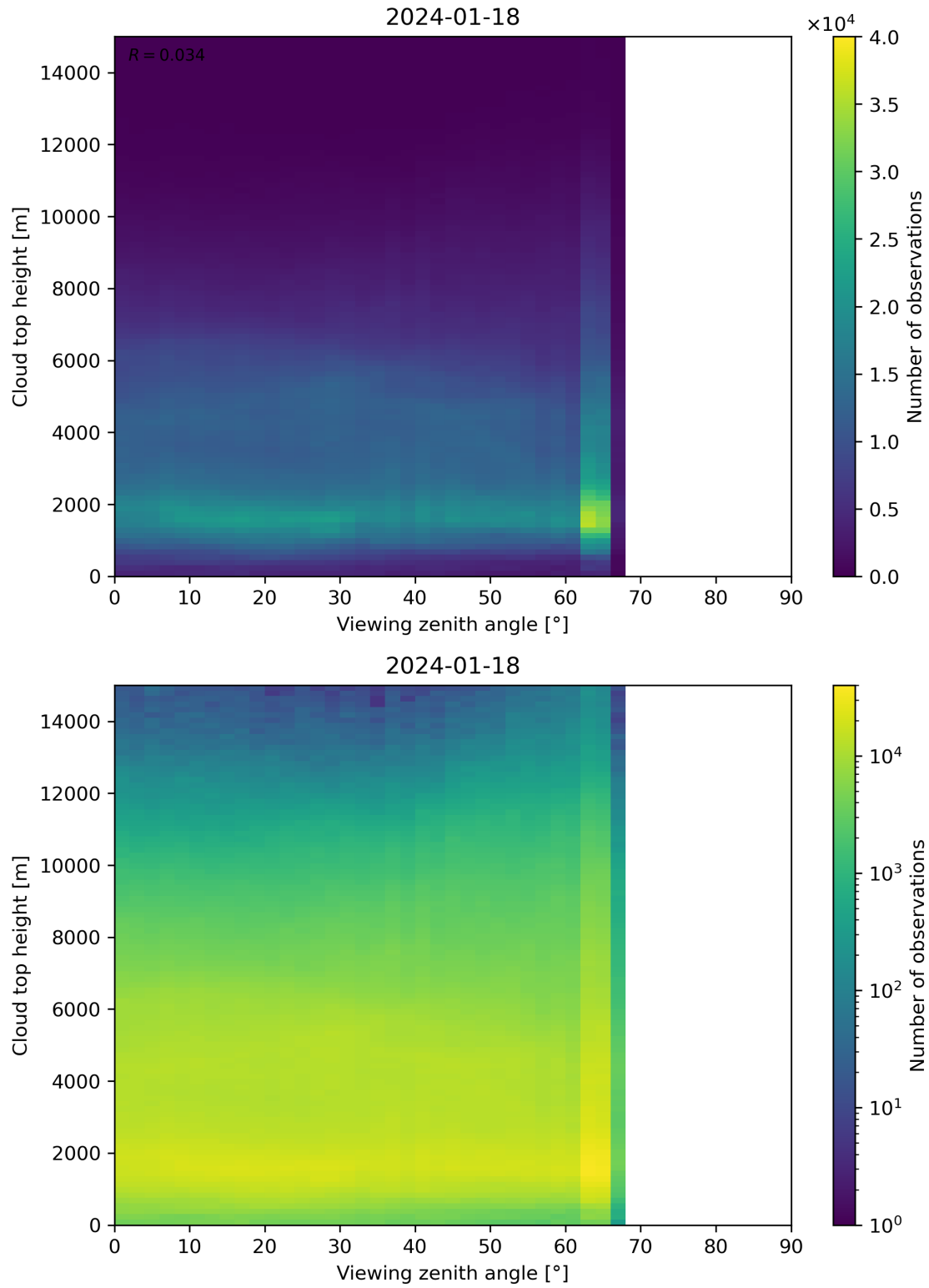
Figure 112: Scatter density plot of “Viewing zenith angle” against “Cloud top height” for 2024-01-17 to 2024-01-19.
