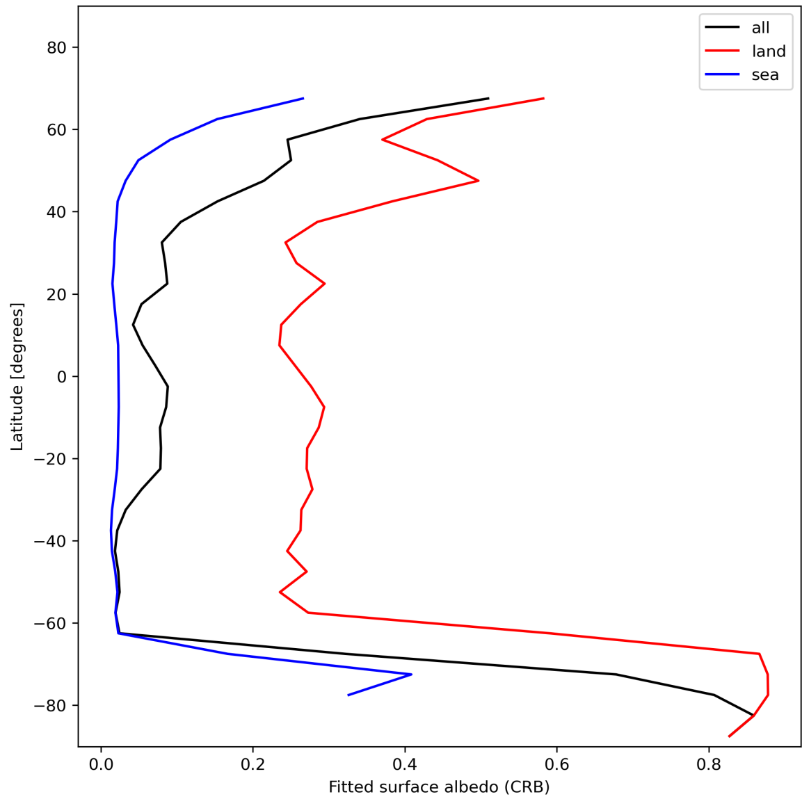
Figure 30: Zonal average of “Fitted surface albedo (CRB)” for 2024-01-17 to 2024-01-19.
