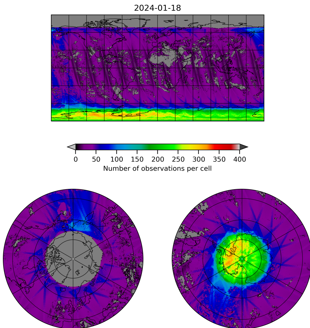
Figure 21: Map of the number of observations for 2024-01-17 to 2024-01-19
