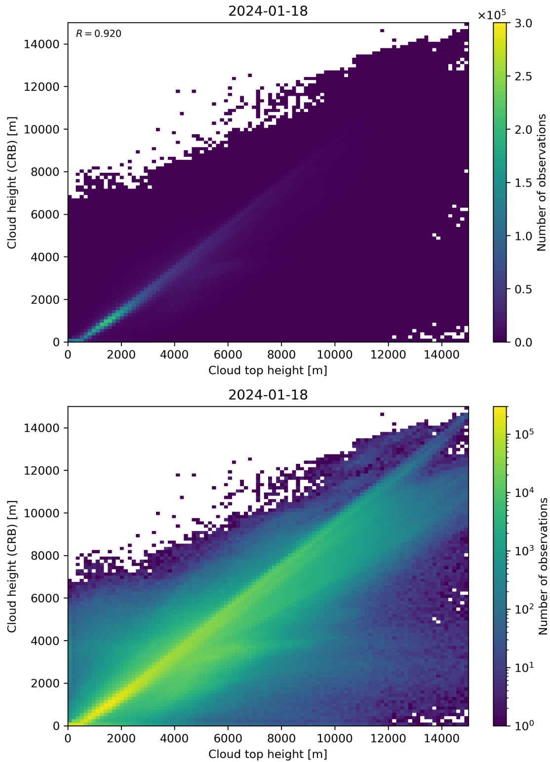
Figure 89: Scatter density plot of “Cloud top height” against “Cloud height (CRB)” for 2024-01-17 to 2024-01-19.
