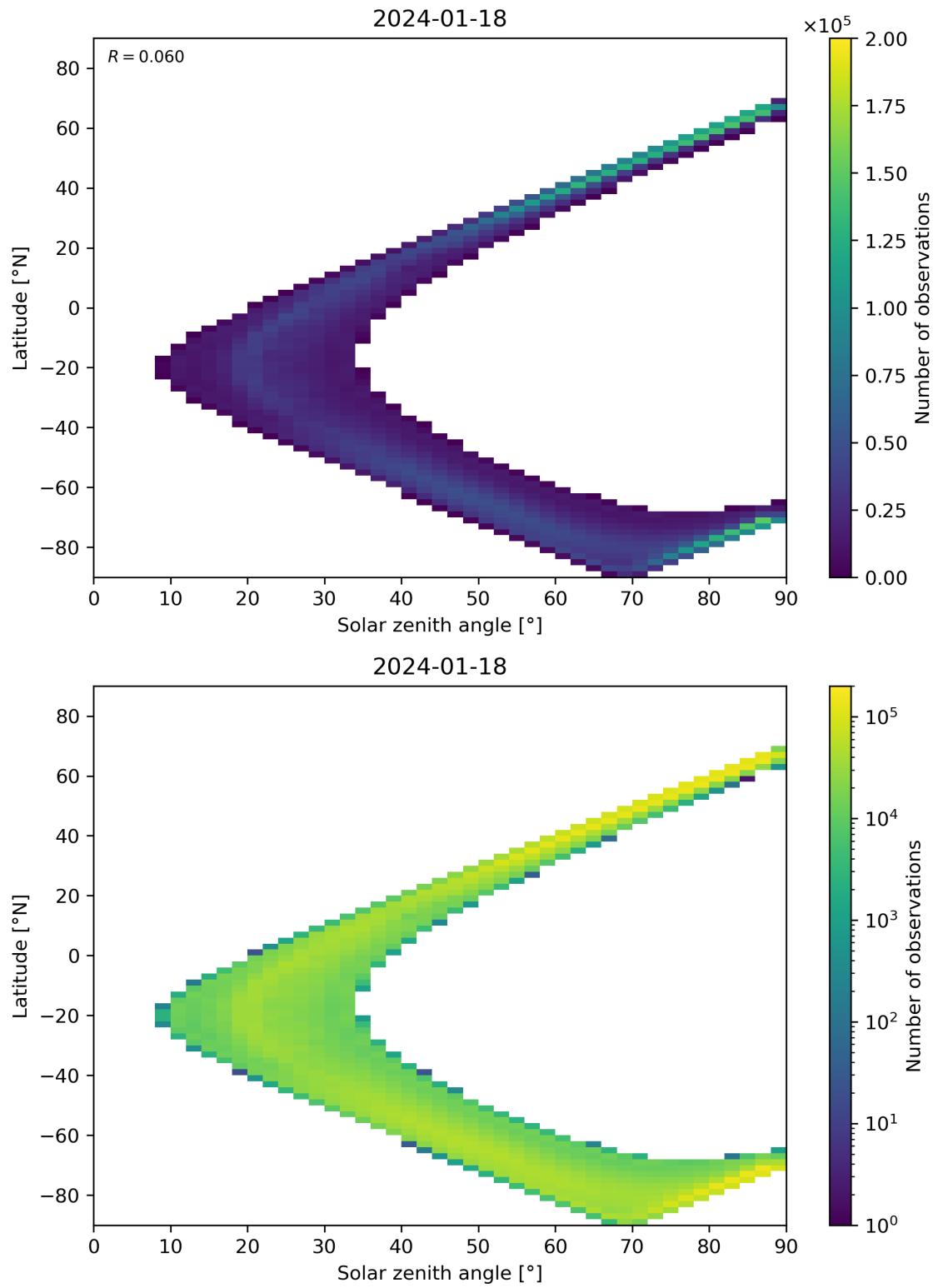
Figure 105: Scatter density plot of “Solar zenith angle” against “Latitude” for 2024-01-17 to 2024-01-19.
