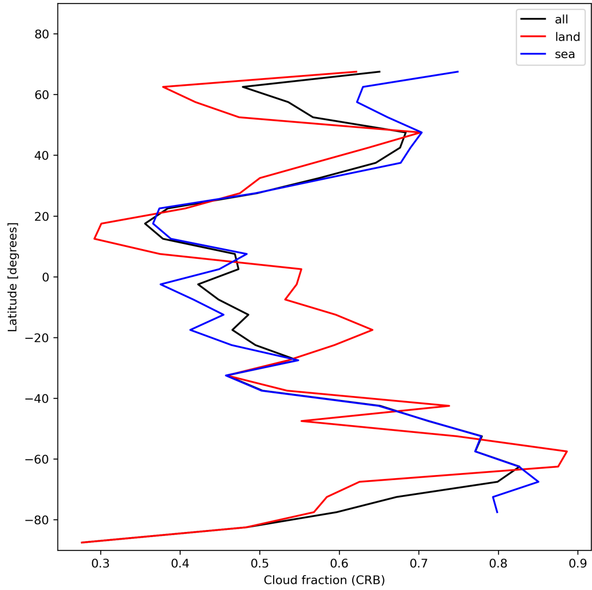
Figure 26: Zonal average of “Cloud fraction (CRB)” for 2024-01-17 to 2024-01-19.
