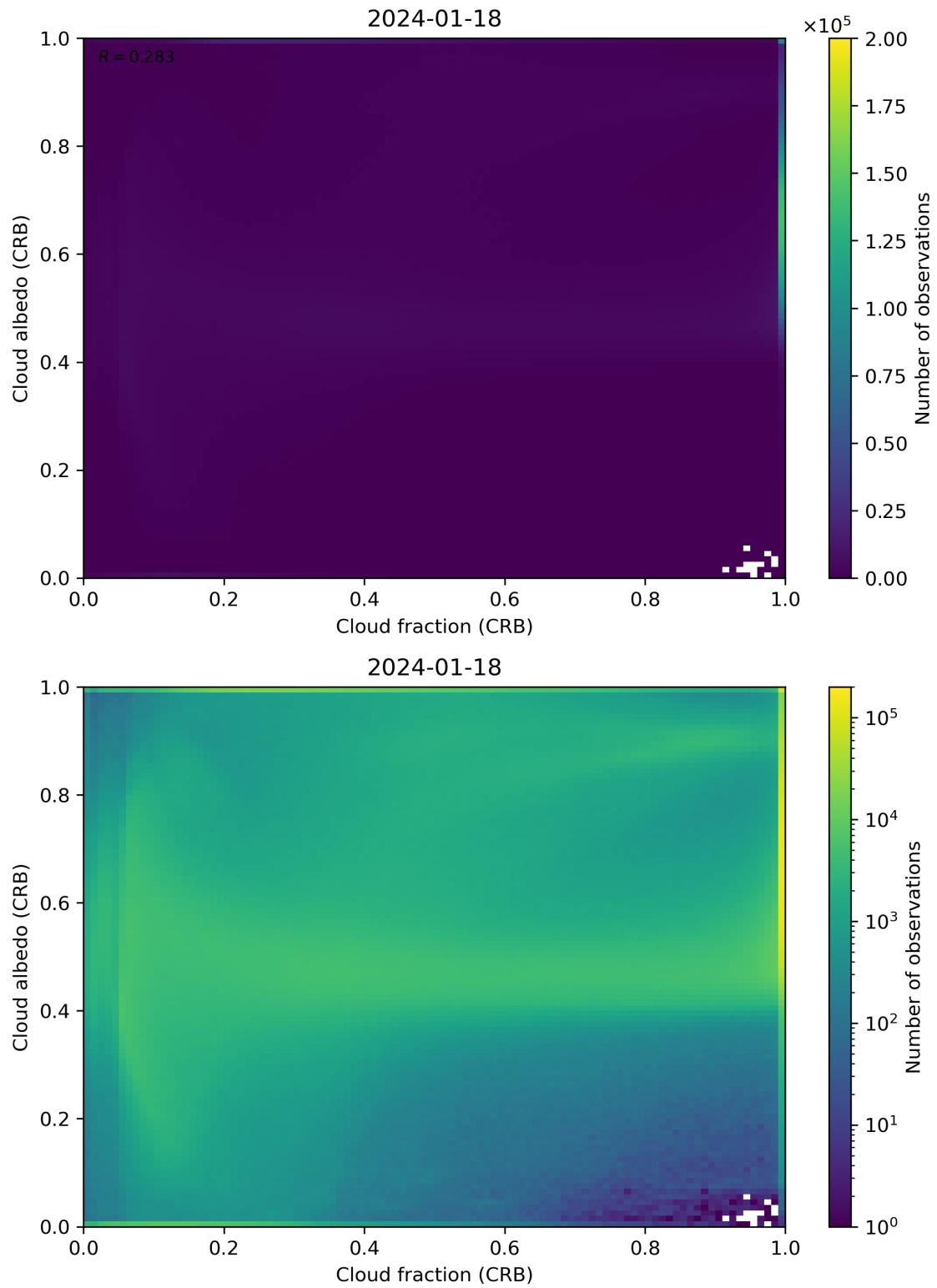
Figure 77: Scatter density plot of “Cloud fraction (CRB)” against “Cloud albedo (CRB)” for 2024-01-17 to 2024-01-19.
