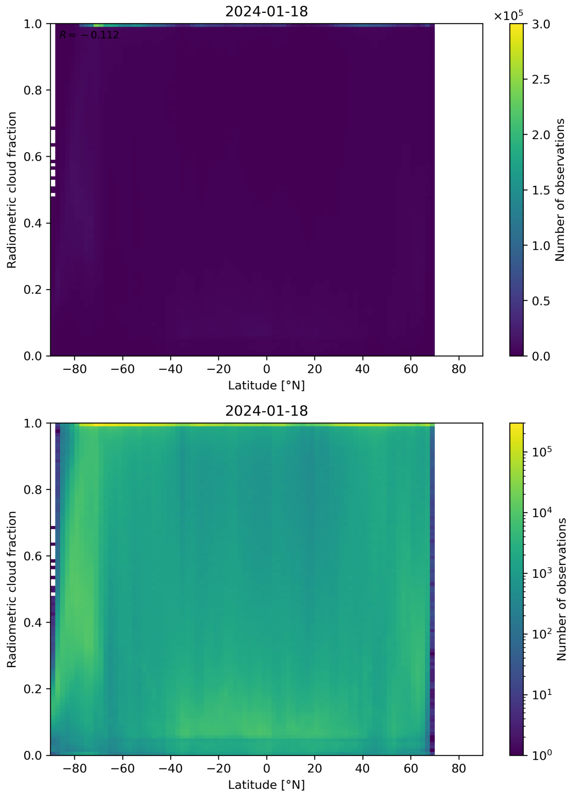
Figure 92: Scatter density plot of “Latitude” against “Radiometric cloud fraction” for 2024-01-17 to 2024-01-19.
