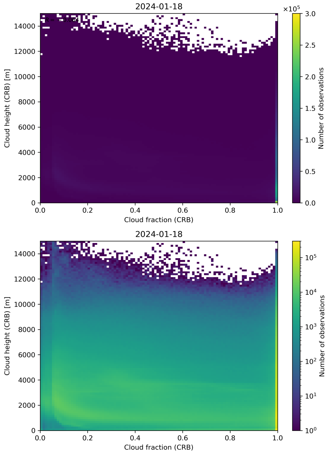
Figure 79: Scatter density plot of “Cloud fraction (CRB)” against “Cloud height (CRB)” for 2024-01-17 to 2024-01-19.
