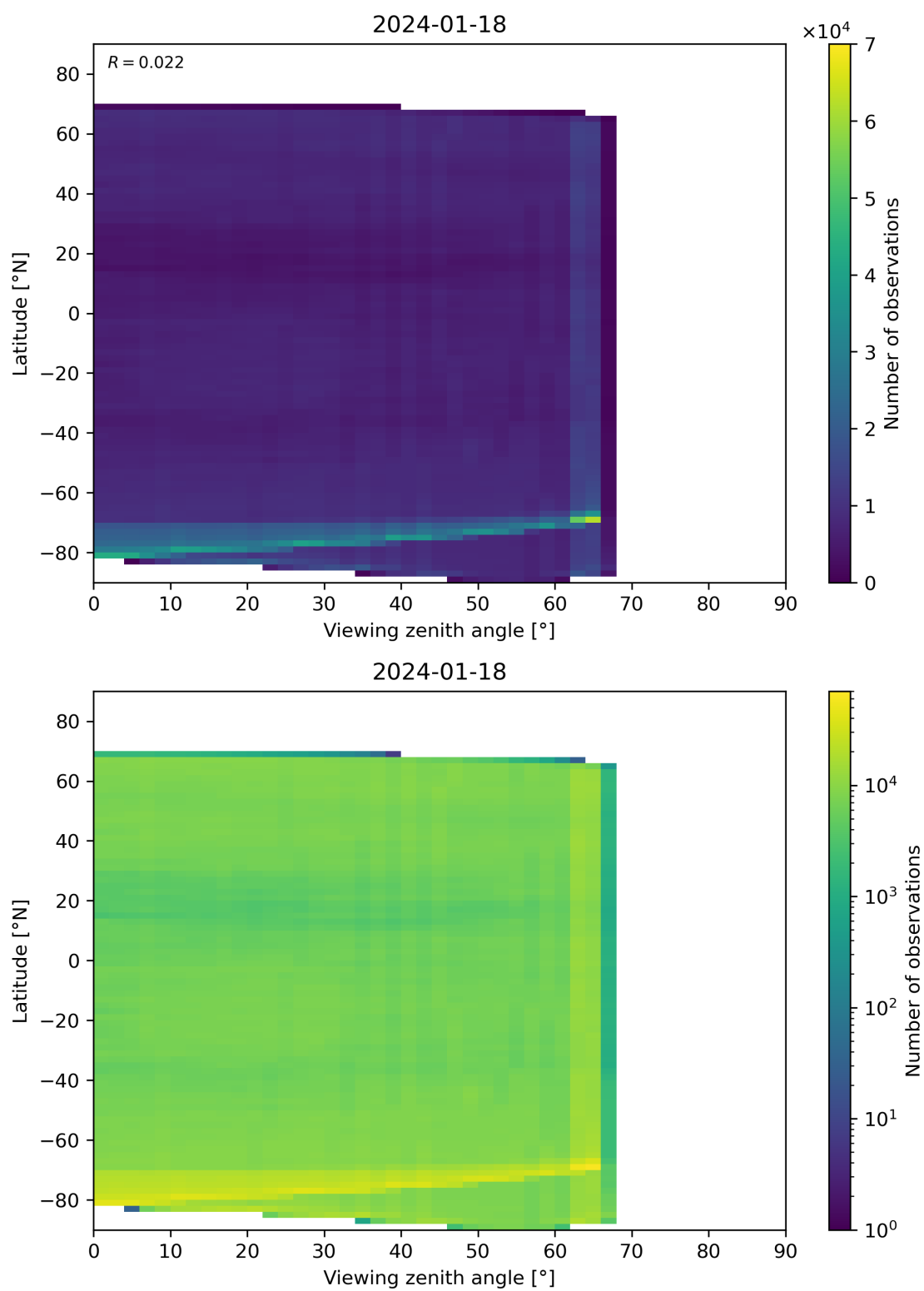
Figure 113: Scatter density plot of “Viewing zenith angle” against “Latitude” for 2024-01-17 to 2024-01-19.
