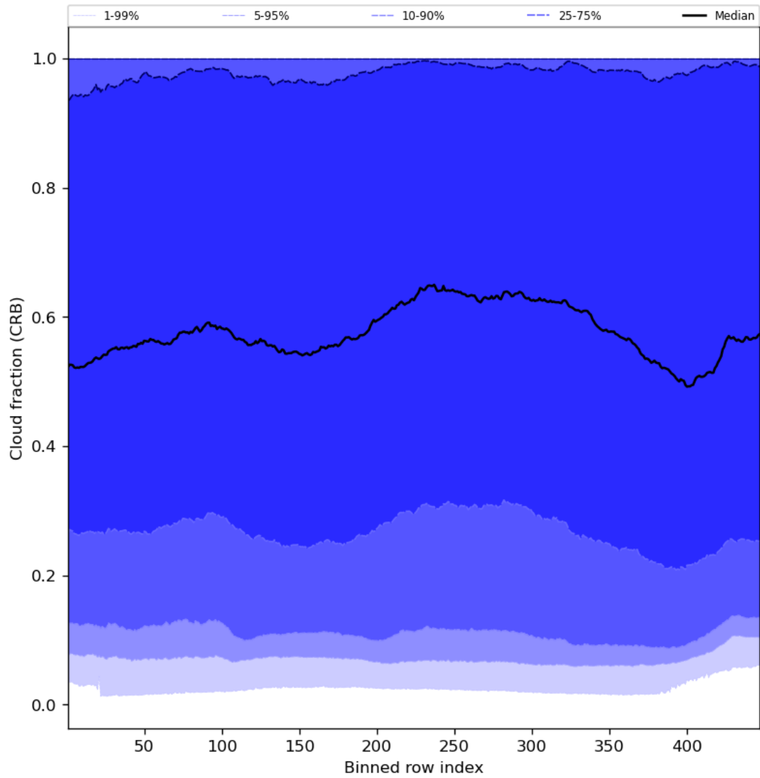
Figure 58: Along track statistics of “Cloud fraction (CRB)” for 2024-01-17 to 2024-01-19
