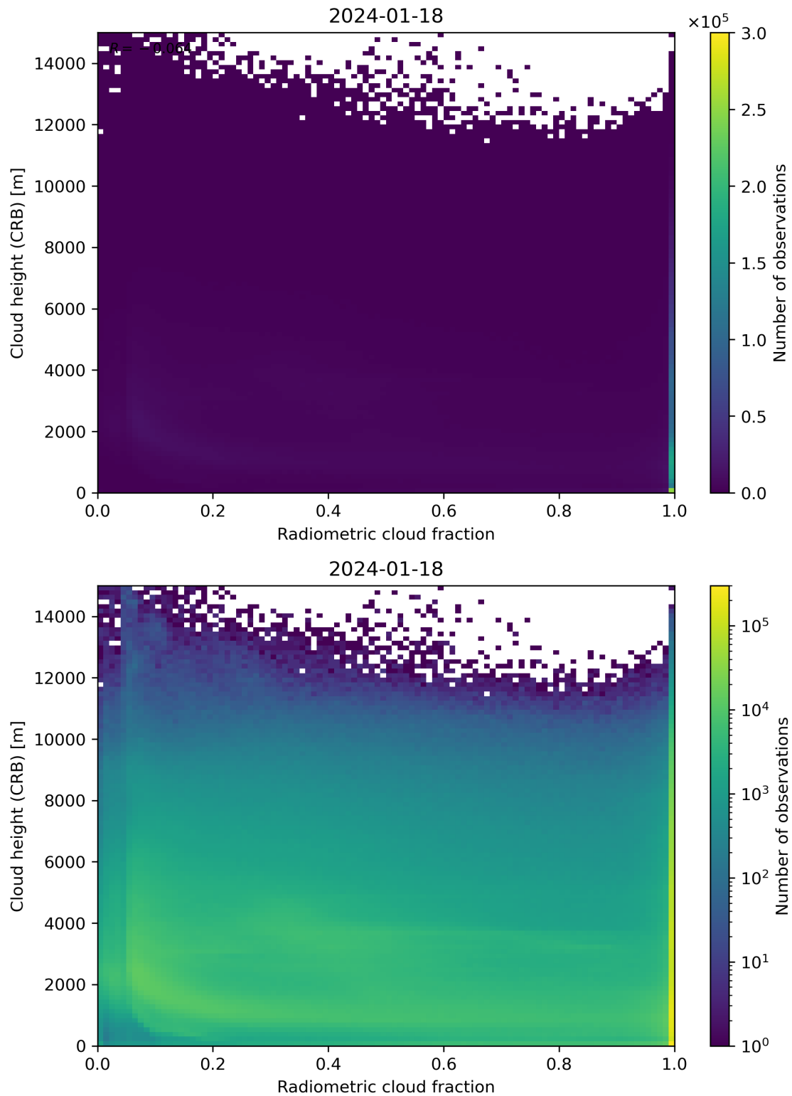
Figure 74: Scatter density plot of “Radiometric cloud fraction” against “Cloud height (CRB)” for 2024-01-17 to 2024-01-19.
