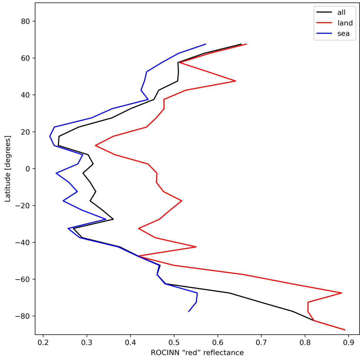
Figure 37: Zonal average of “ROCINN “red” reflectance” for 2024-01-17 to 2024-01-19.
