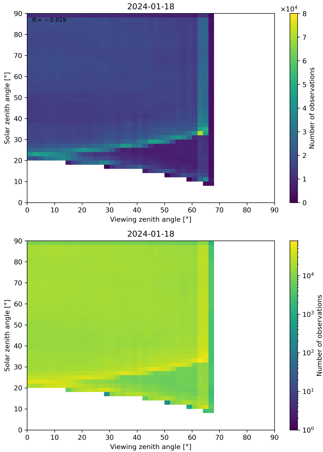
Figure 114: Scatter density plot of “Viewing zenith angle” against “Solar zenith angle” for 2024-01-17 to 2024-01-19.
