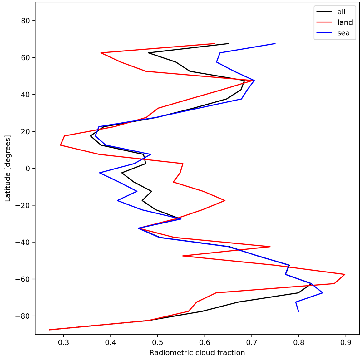
Figure 23: Zonal average of “Radiometric cloud fraction” for 2024-01-17 to 2024-01-19.
