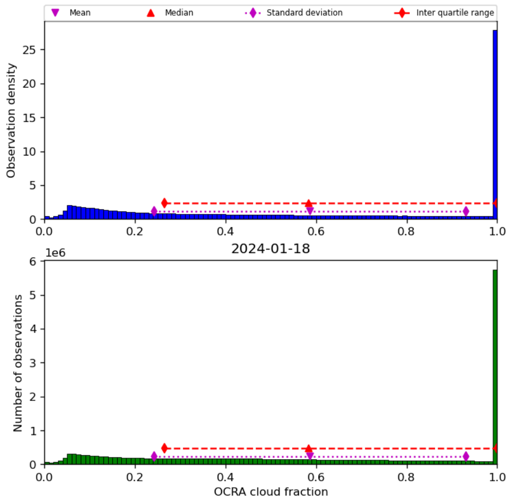
Figure 50: Histogram of “OCRA cloud fraction” for 2024-01-17 to 2024-01-19
