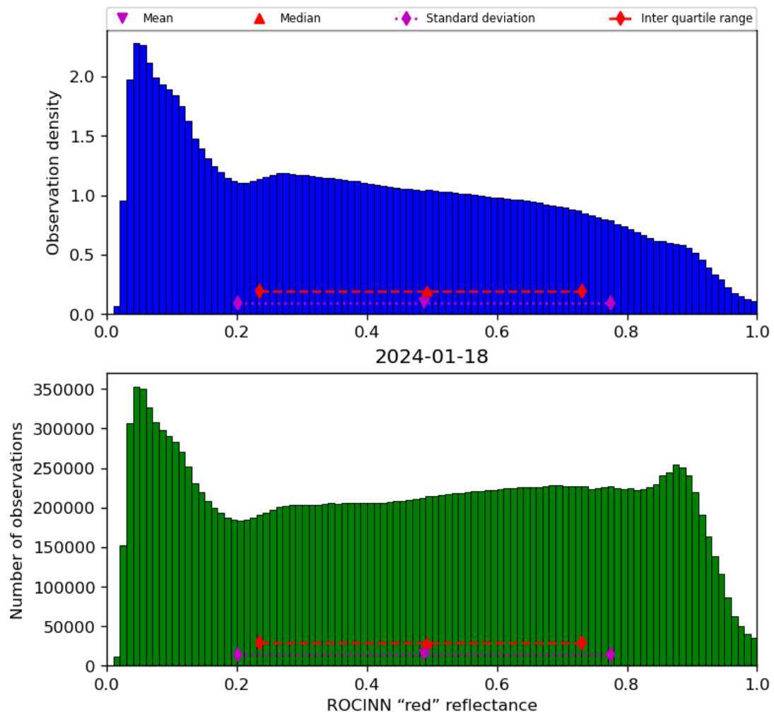
Figure 53: Histogram of “ROCINN “red” reflectance” for 2024-01-17 to 2024-01-19
