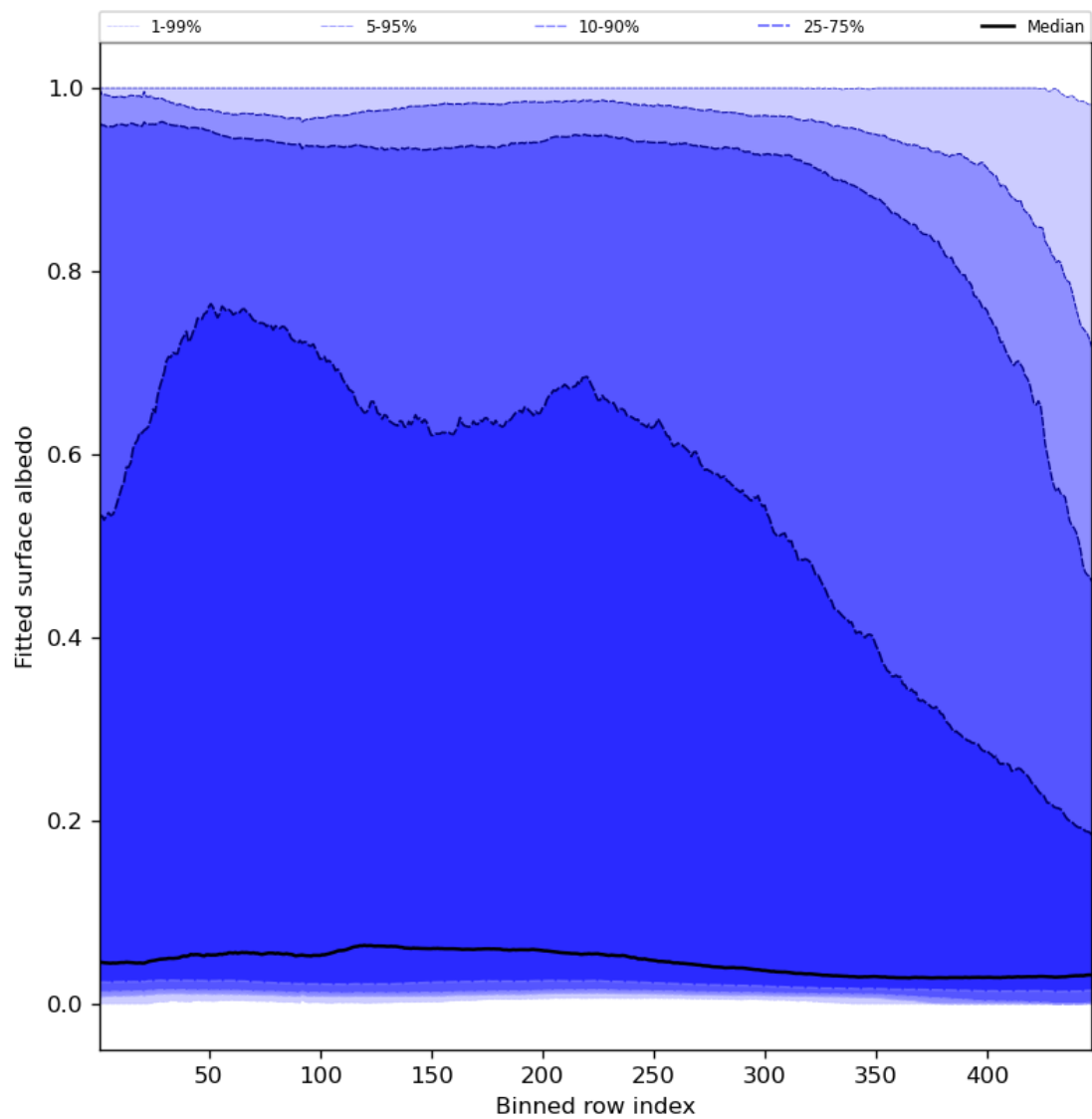
Figure 61: Along track statistics of “Fitted surface albedo” for 2024-01-17 to 2024-01-19
