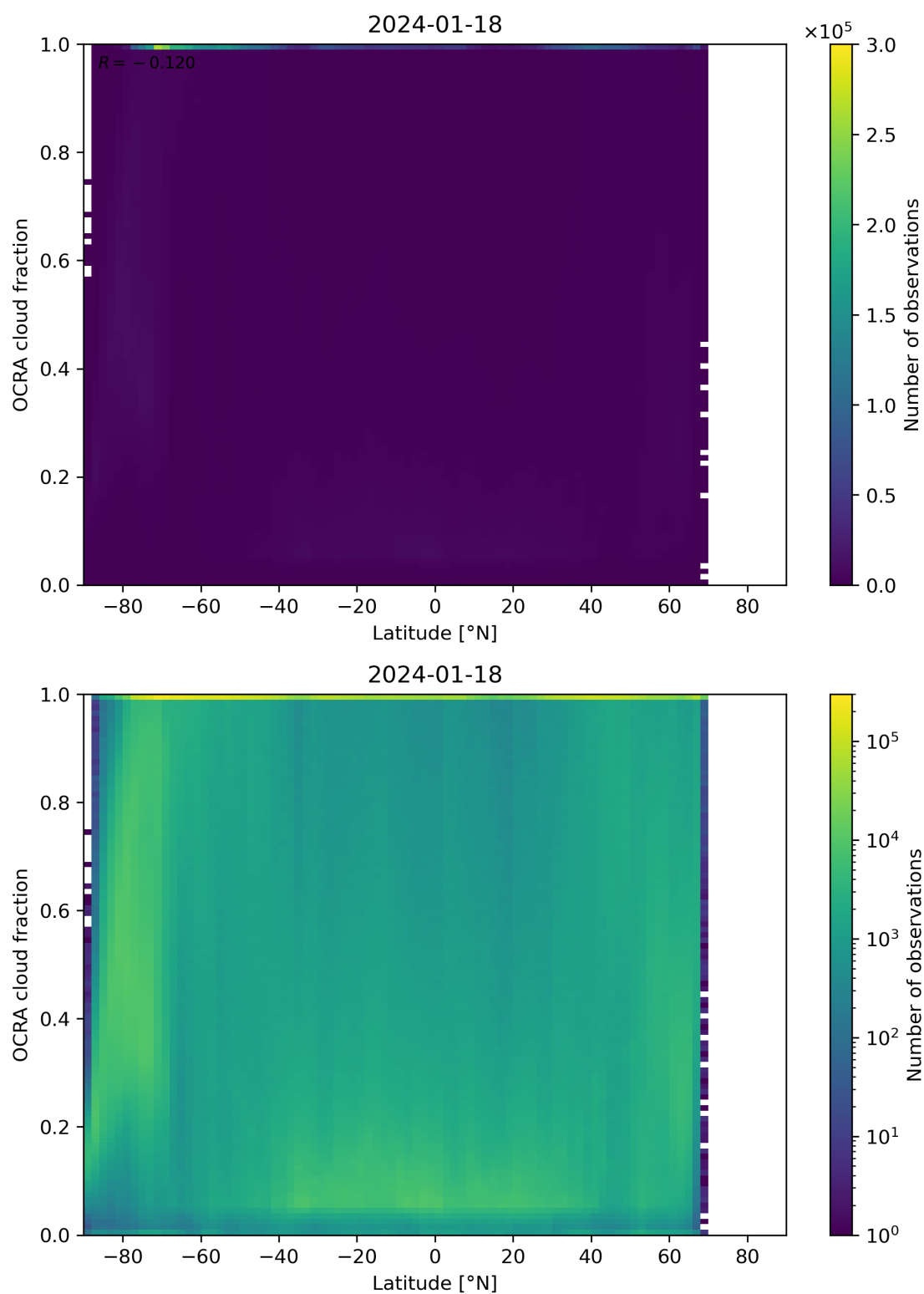
Figure 93: Scatter density plot of “Latitude” against “OCRA cloud fraction” for 2024-01-17 to 2024-01-19.
