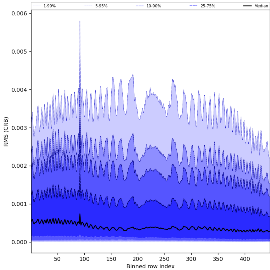
Figure 64: Along track statistics of “RMS (CRB)” for 2024-01-17 to 2024-01-19
