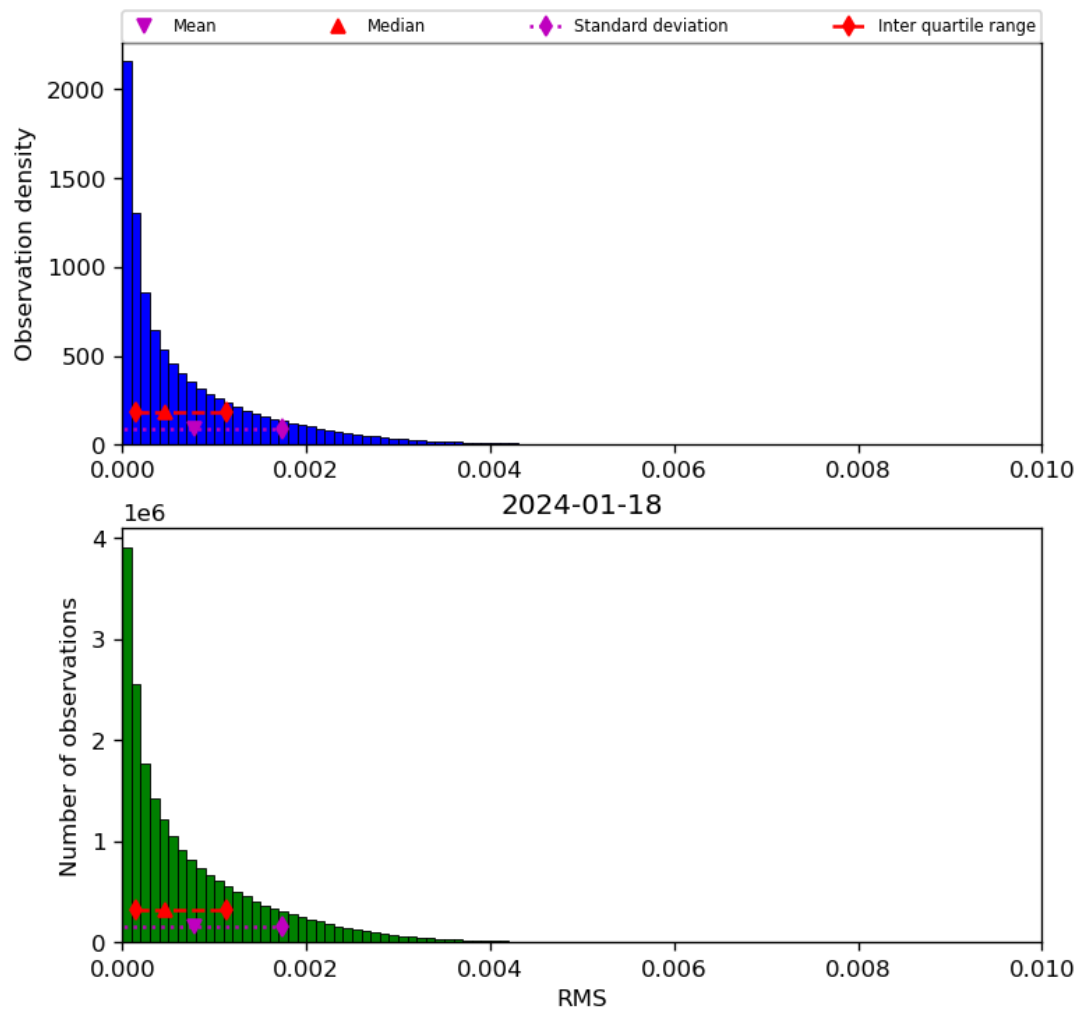
Figure 47: Histogram of “RMS” for 2024-01-17 to 2024-01-19
