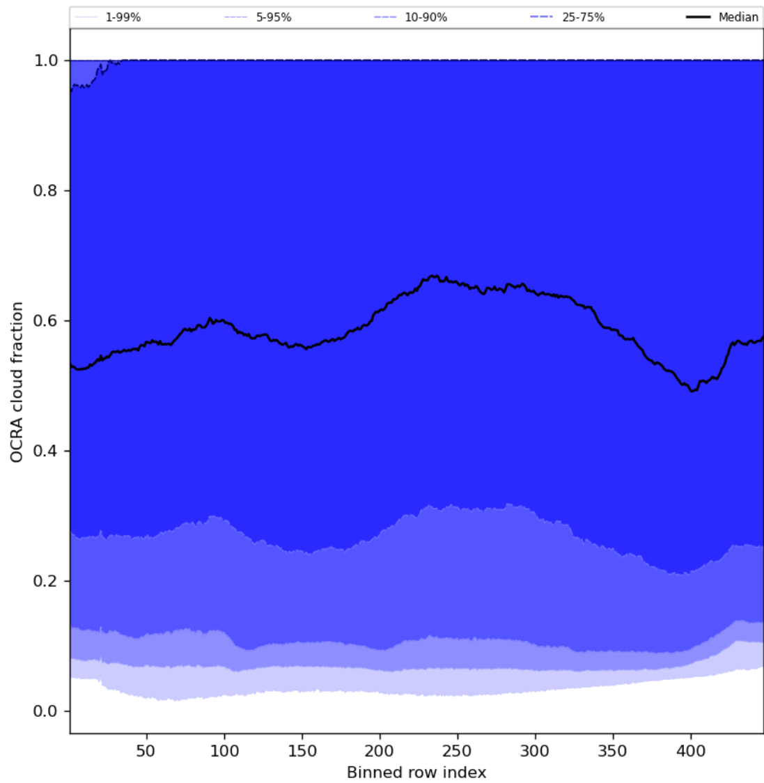
Figure 66: Along track statistics of “OCRA cloud fraction” for 2024-01-17 to 2024-01-19
