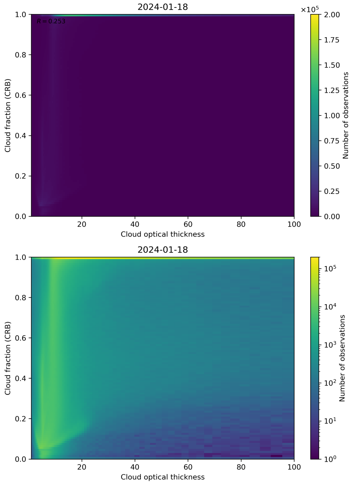
Figure 84: Scatter density plot of “Cloud optical thickness” against “Cloud fraction (CRB)” for 2024-01-17 to 2024-01-19.
