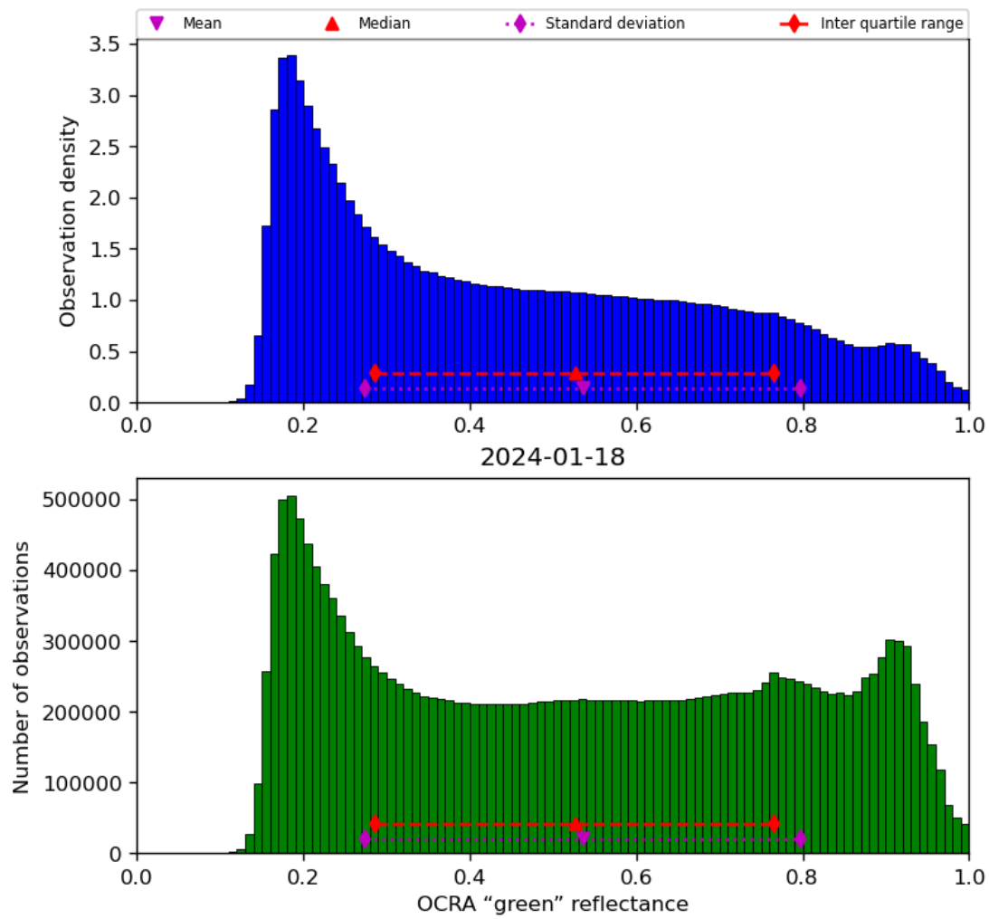
Figure 52: Histogram of “OCRA “green” reflectance” for 2024-01-17 to 2024-01-19
