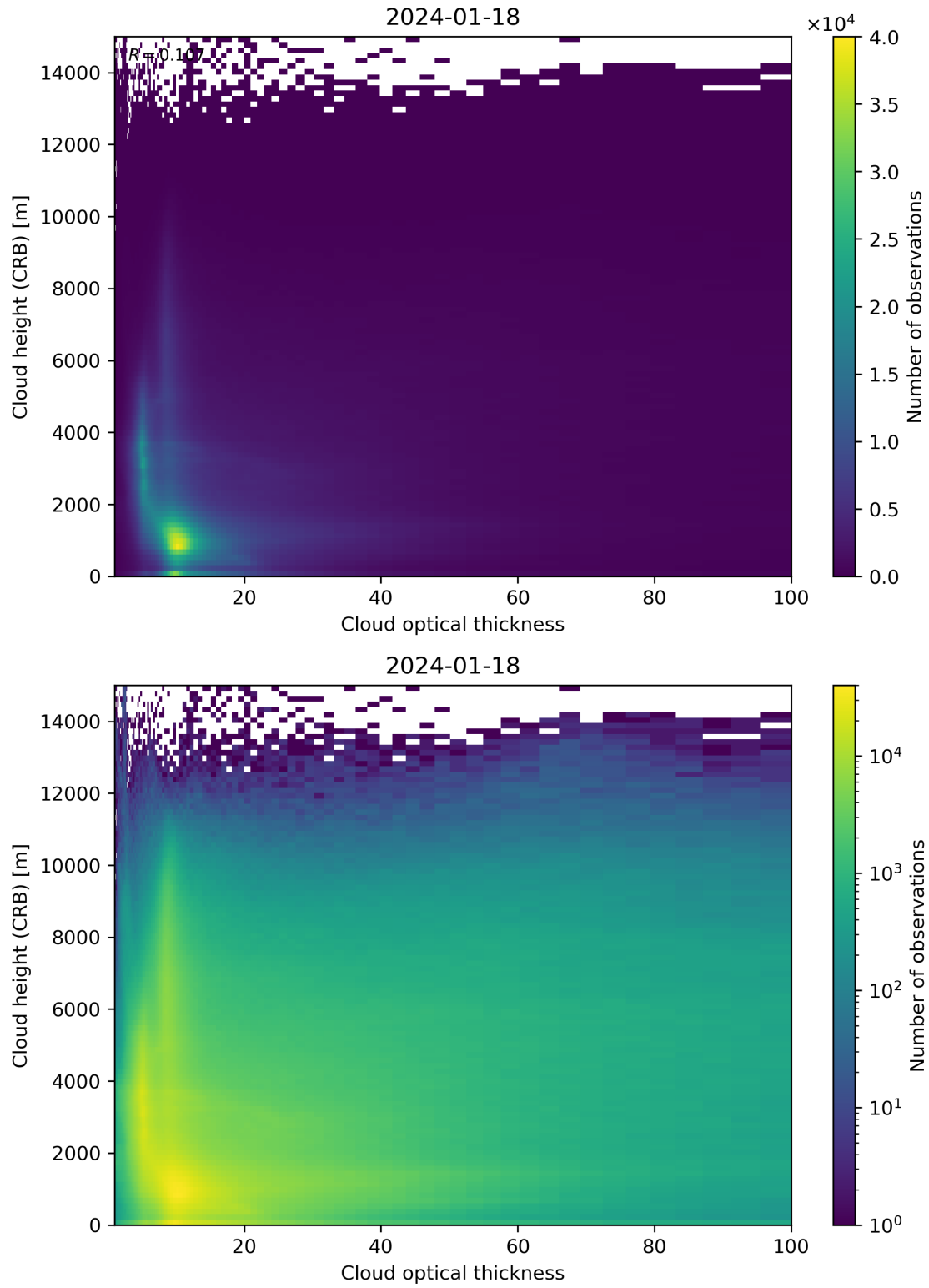
Figure 85: Scatter density plot of “Cloud optical thickness” against “Cloud height (CRB)” for 2024-01-17 to 2024-01-19.
