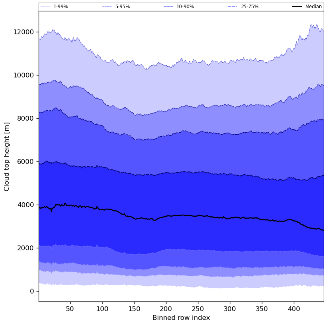
Figure 56: Along track statistics of “Cloud top height” for 2024-01-17 to 2024-01-19
