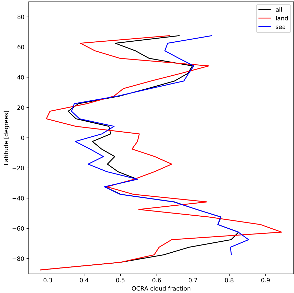
Figure 34: Zonal average of “OCRA cloud fraction” for 2024-01-17 to 2024-01-19.
