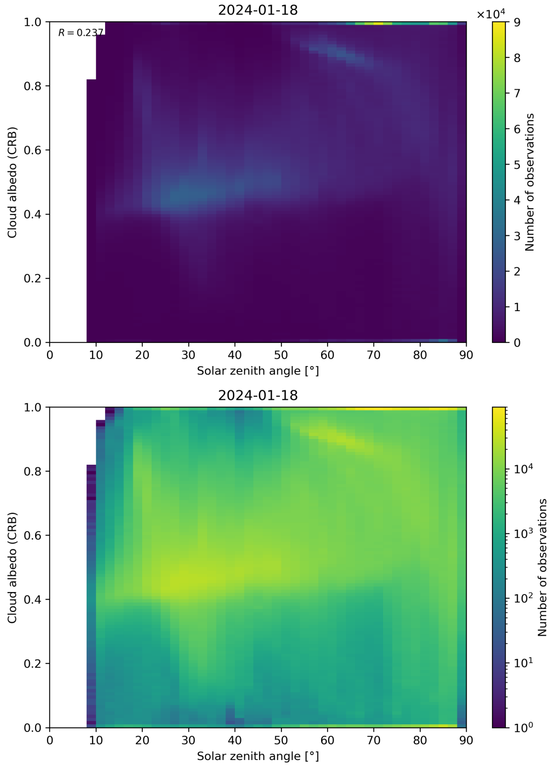
Figure 98: Scatter density plot of “Solar zenith angle” against “Cloud albedo (CRB)” for 2024-01-17 to 2024-01-19.
