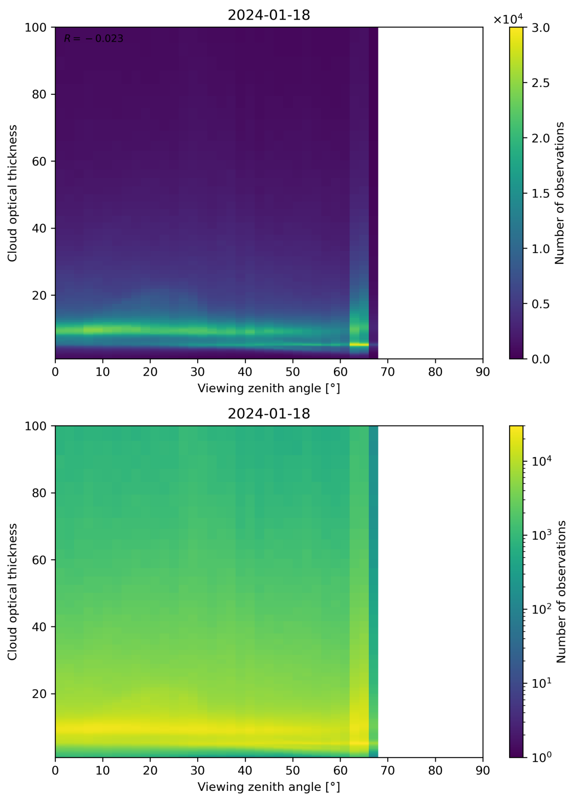
Figure 111: Scatter density plot of “Viewing zenith angle” against “Cloud optical thickness” for 2024-01-17 to 2024-01-19.
