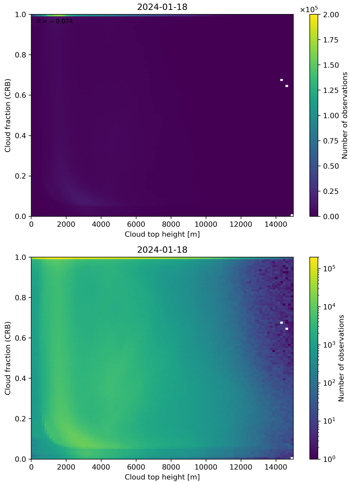
Figure 88: Scatter density plot of “Cloud top height” against “Cloud fraction (CRB)” for 2024-01-17 to 2024-01-19.
