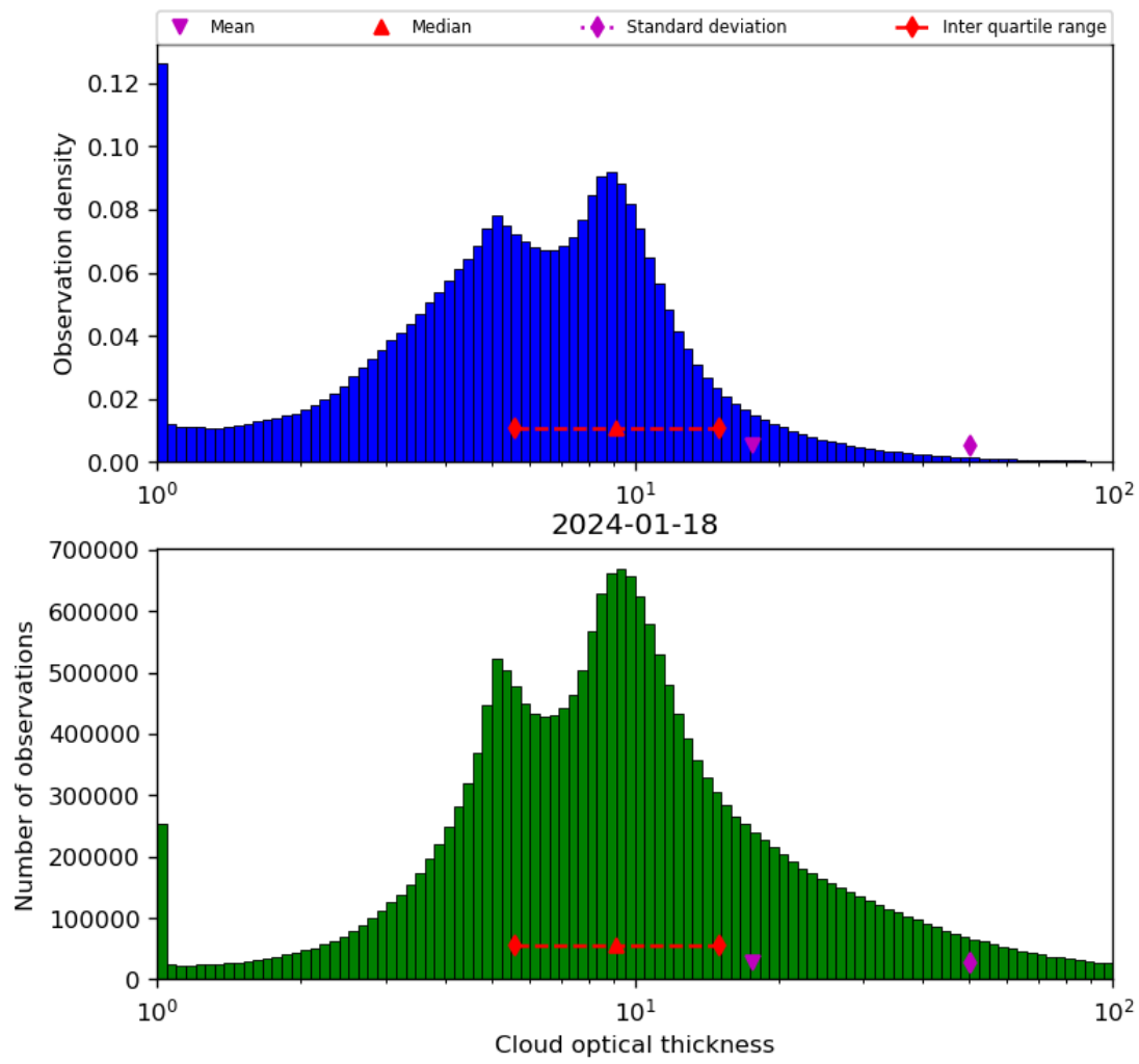
Figure 41: Histogram of “Cloud optical thickness” for 2024-01-17 to 2024-01-19
