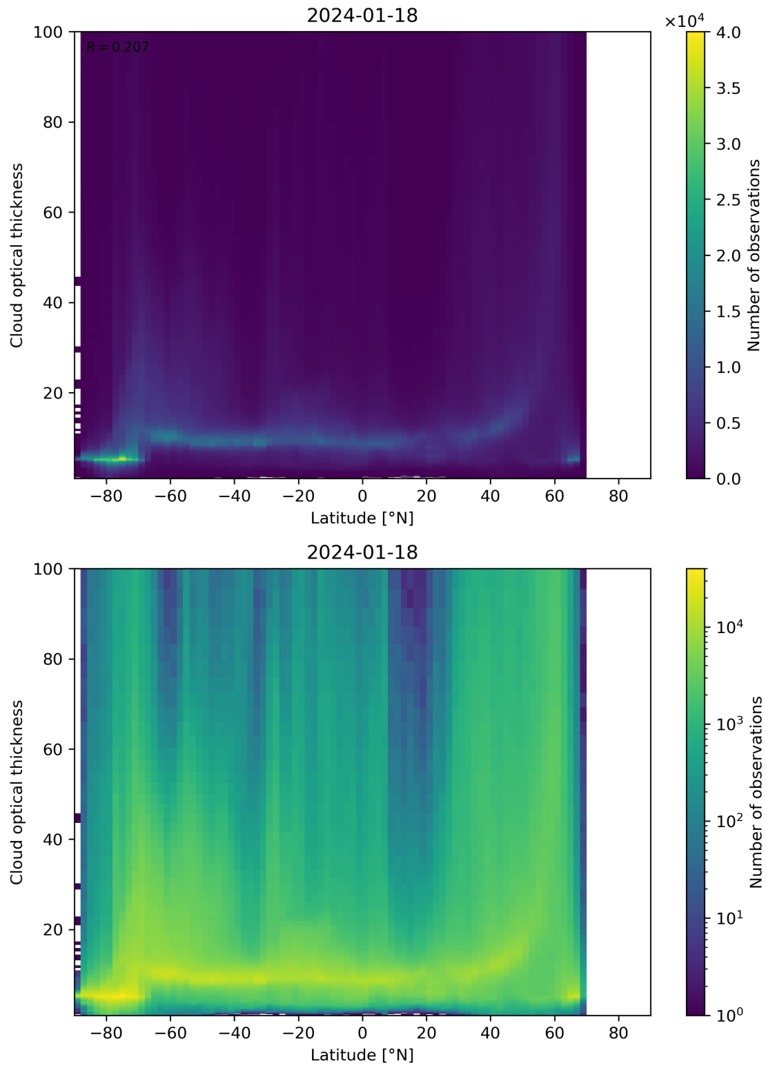
Figure 96: Scatter density plot of “Latitude” against “Cloud optical thickness” for 2024-01-17 to 2024-01-19.
