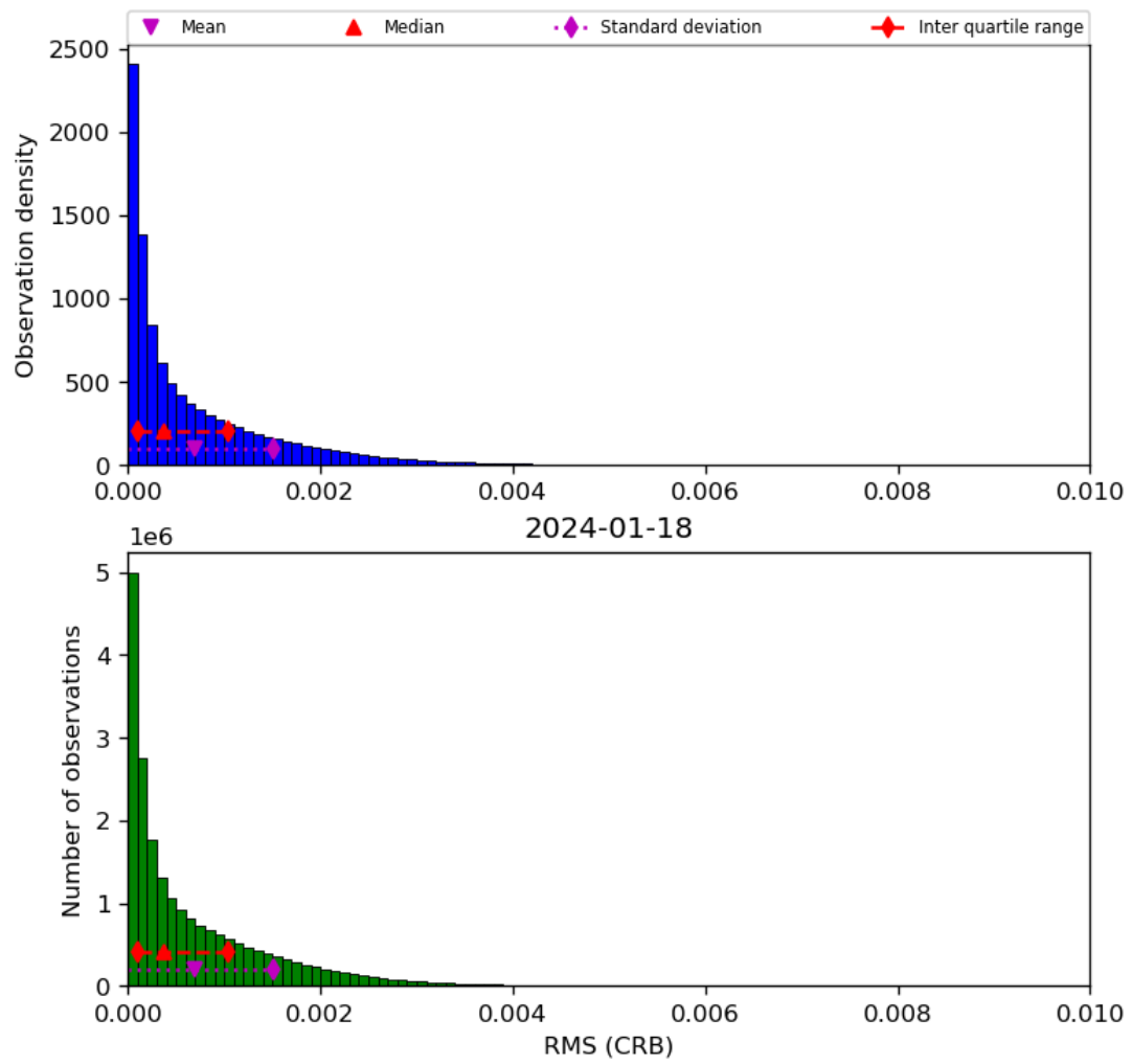
Figure 48: Histogram of “RMS (CRB)” for 2024-01-17 to 2024-01-19
