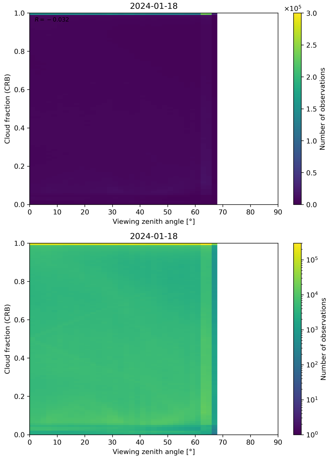
Figure 109: Scatter density plot of “Viewing zenith angle” against “Cloud fraction (CRB)” for 2024-01-17 to 2024-01-19.
