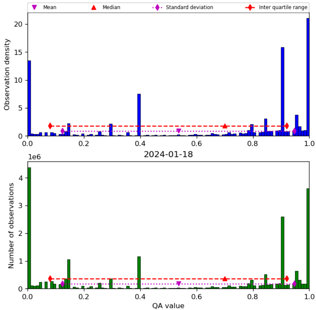
Figure 38: Histogram of “QA value” for 2024-01-17 to 2024-01-19
