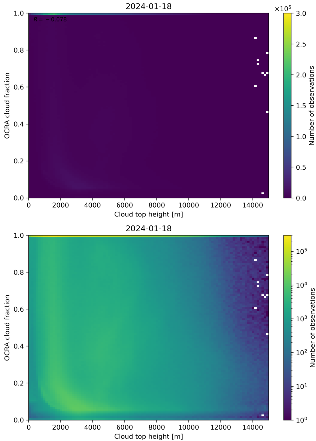
Figure 87: Scatter density plot of “Cloud top height” against “OCRA cloud fraction” for 2024-01-17 to 2024-01-19.
