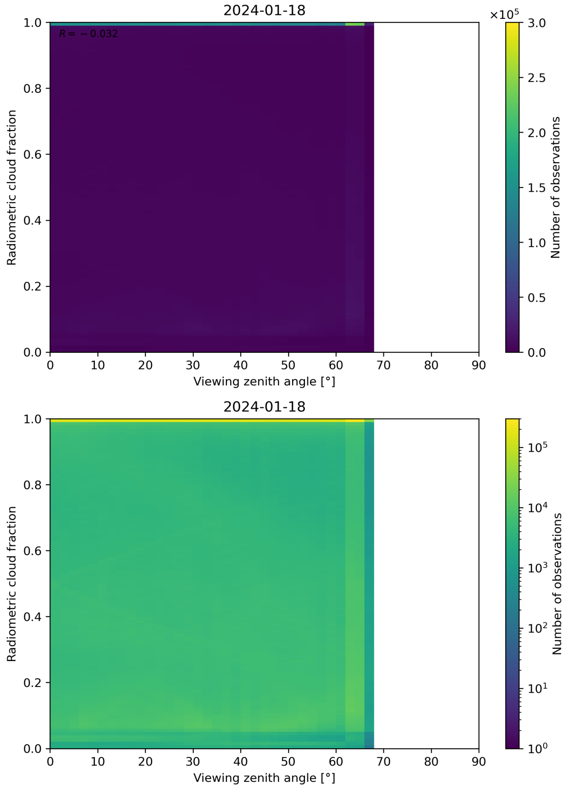
Figure 107: Scatter density plot of “Viewing zenith angle” against “Radiometric cloud fraction” for 2024-01-17 to 2024-01-19.
