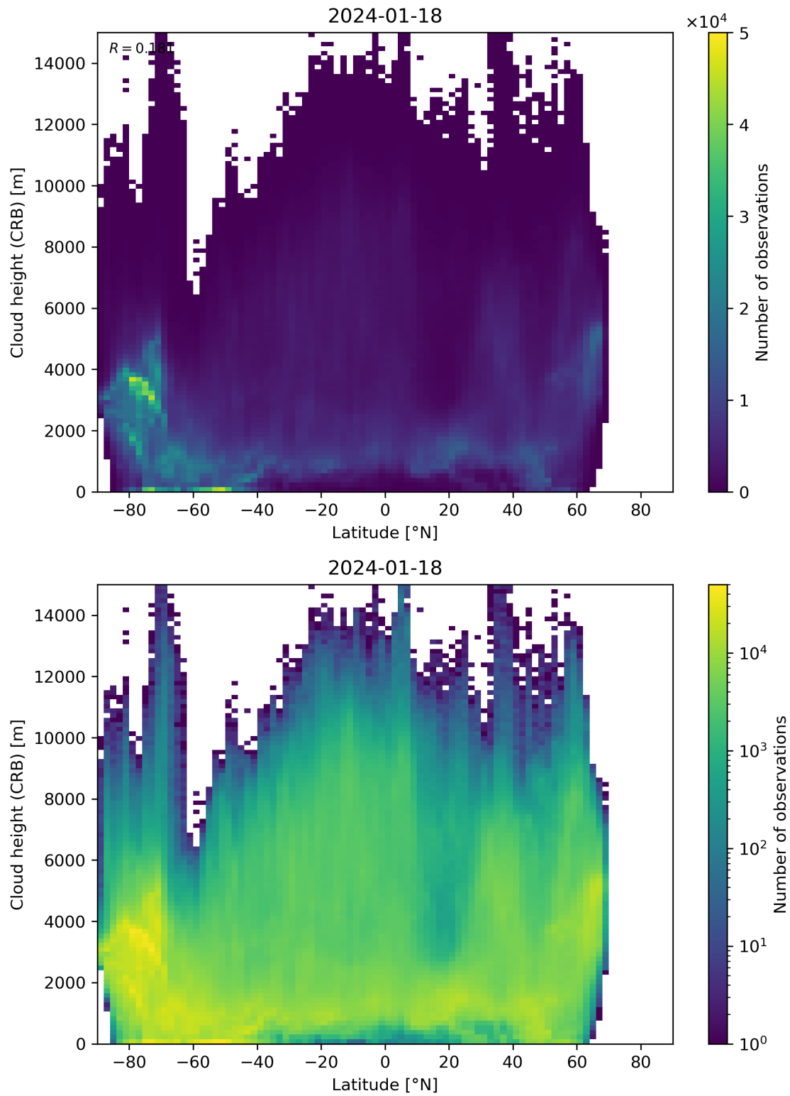
Figure 95: Scatter density plot of “Latitude” against “Cloud height (CRB)” for 2024-01-17 to 2024-01-19.
