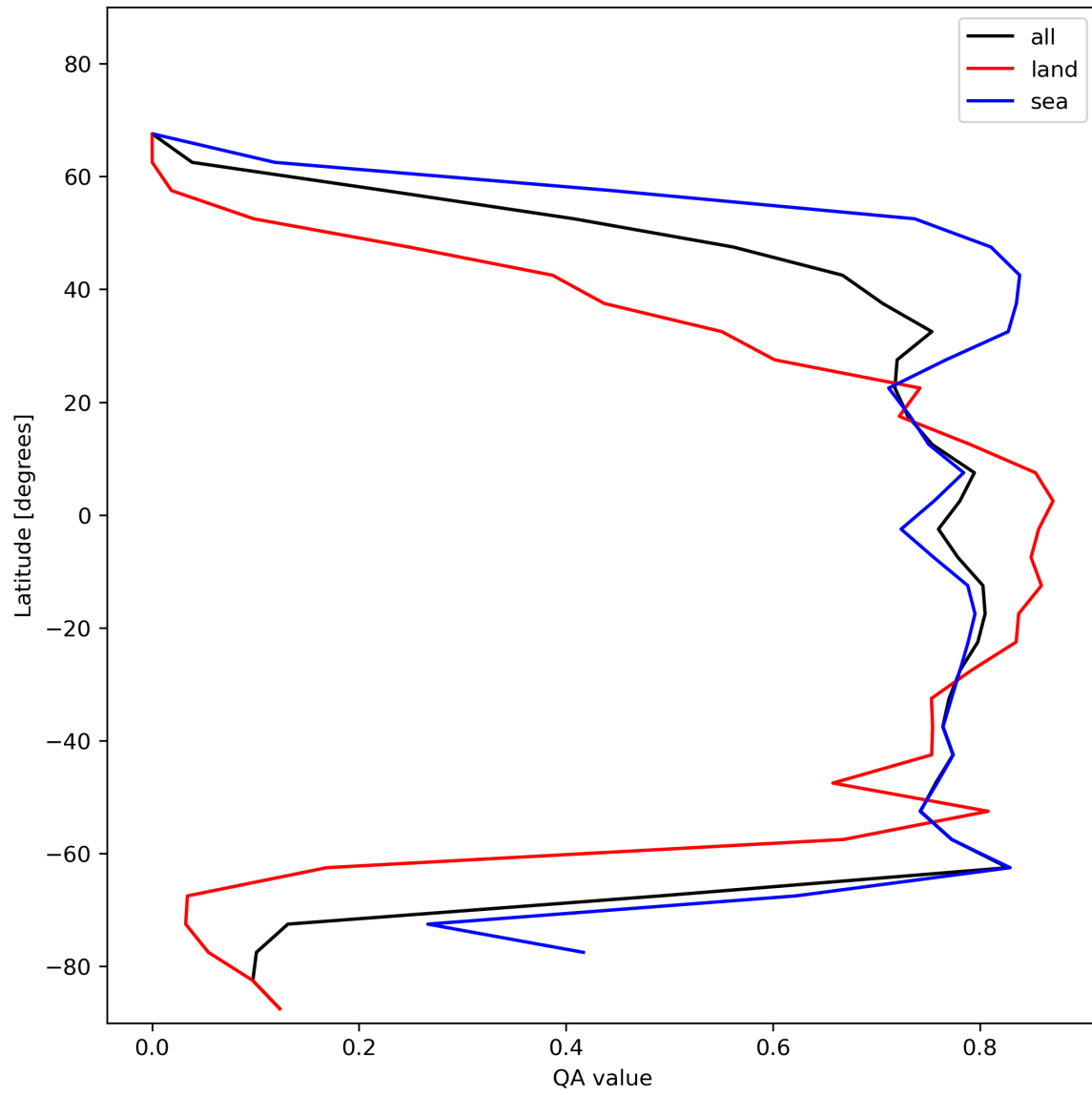
Figure 22: Zonal average of “QA value” for 2024-01-17 to 2024-01-19.
