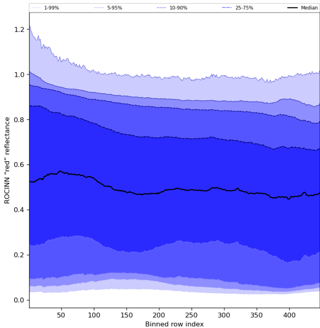
Figure 69: Along track statistics of “ROCINN “red” reflectance” for 2024-01-17 to 2024-01-19
