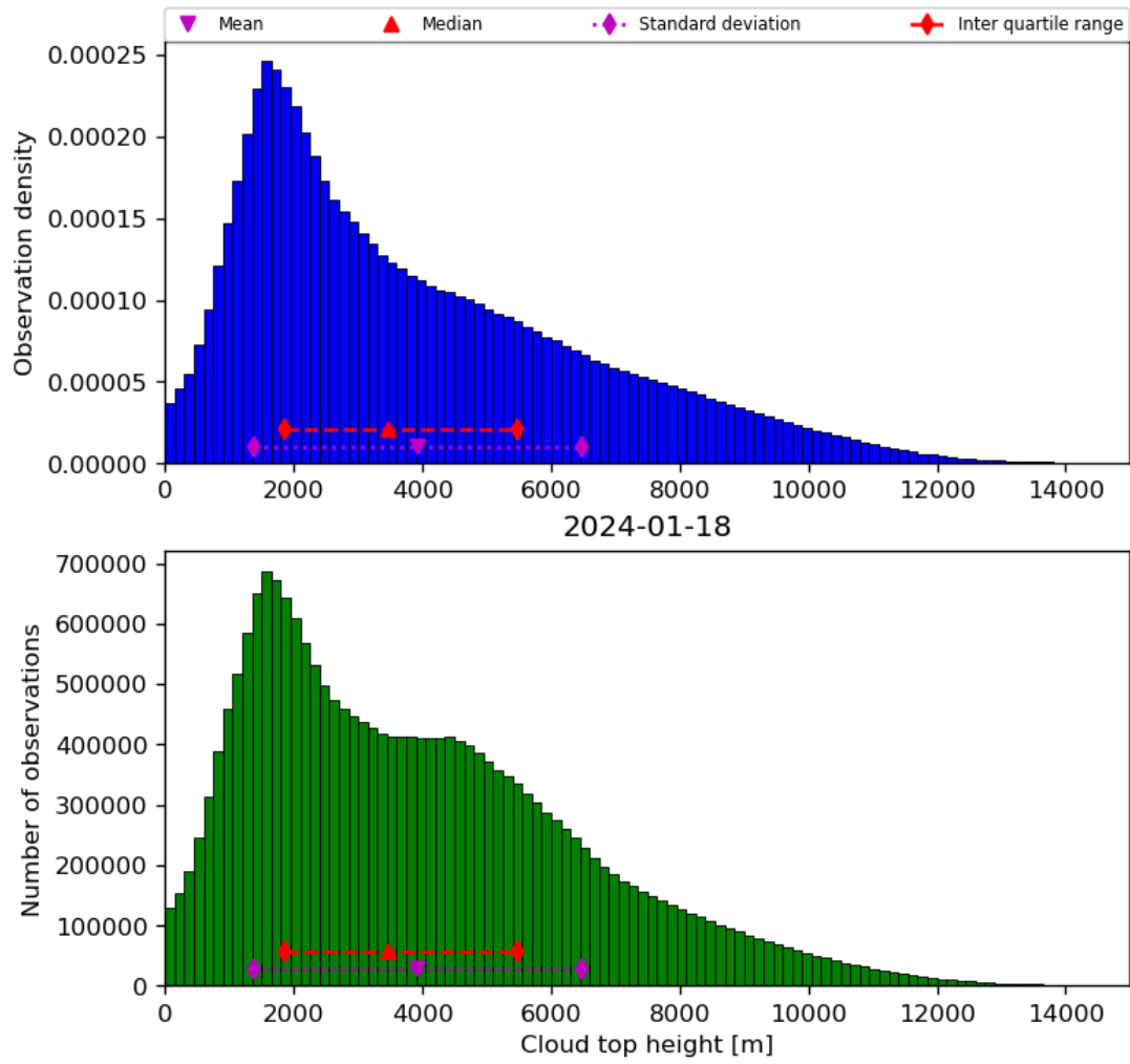
Figure 40: Histogram of “Cloud top height” for 2024-01-17 to 2024-01-19
