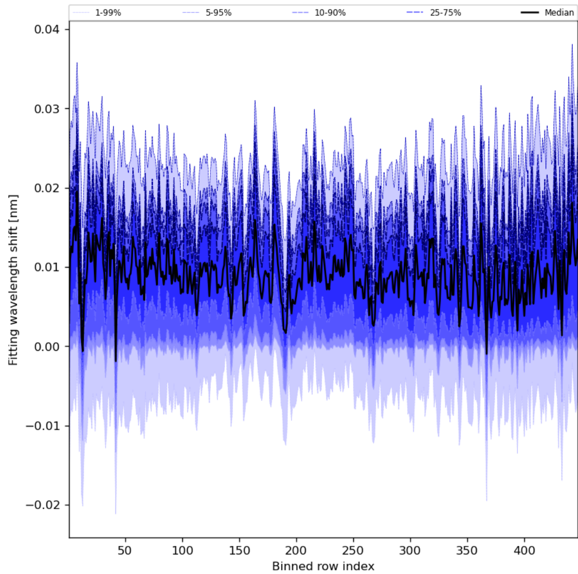
Figure 65: Along track statistics of “Fitting wavelength shift” for 2024-01-17 to 2024-01-19
