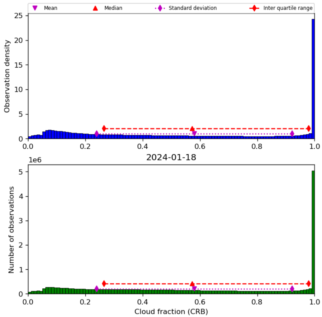
Figure 42: Histogram of “Cloud fraction (CRB)” for 2024-01-17 to 2024-01-19
