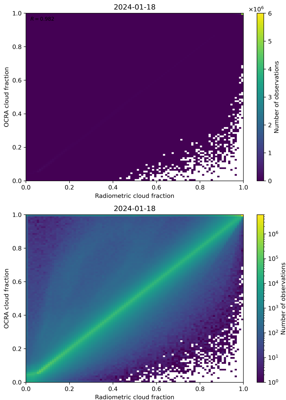
Figure 72: Scatter density plot of “Radiometric cloud fraction” against “OCRA cloud fraction” for 2024-01-17 to 2024-01-19.
