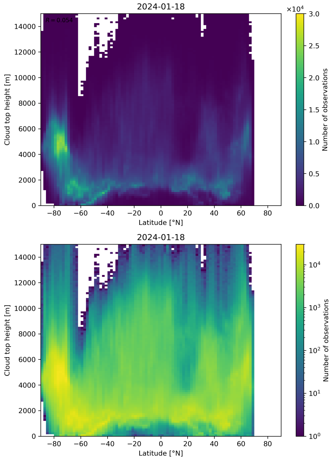
Figure 97: Scatter density plot of “Latitude” against “Cloud top height” for 2024-01-17 to 2024-01-19.
