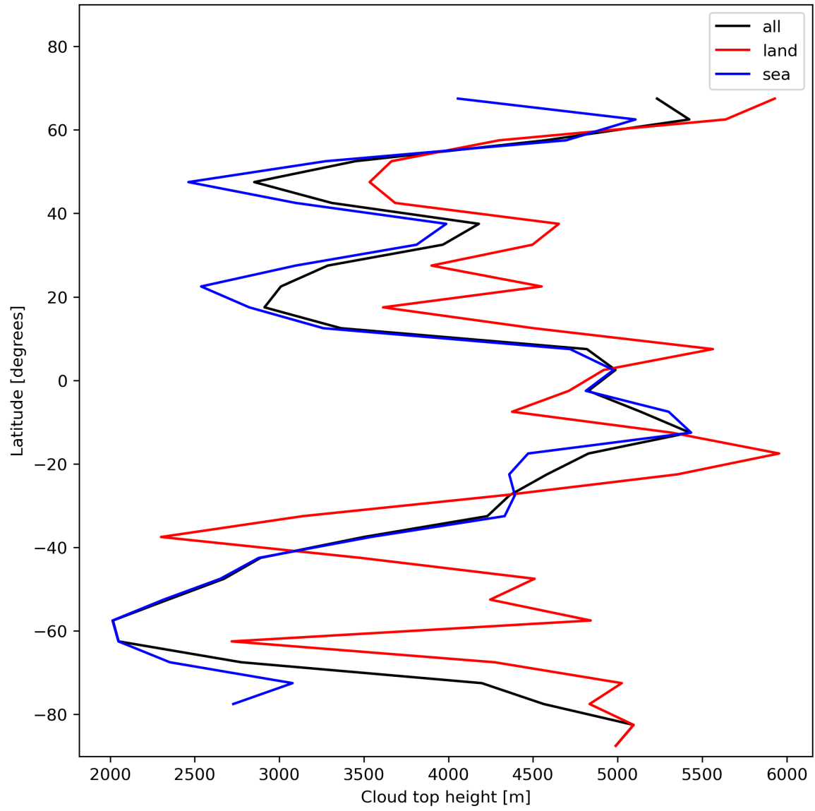
Figure 24: Zonal average of “Cloud top height” for 2024-01-17 to 2024-01-19.
