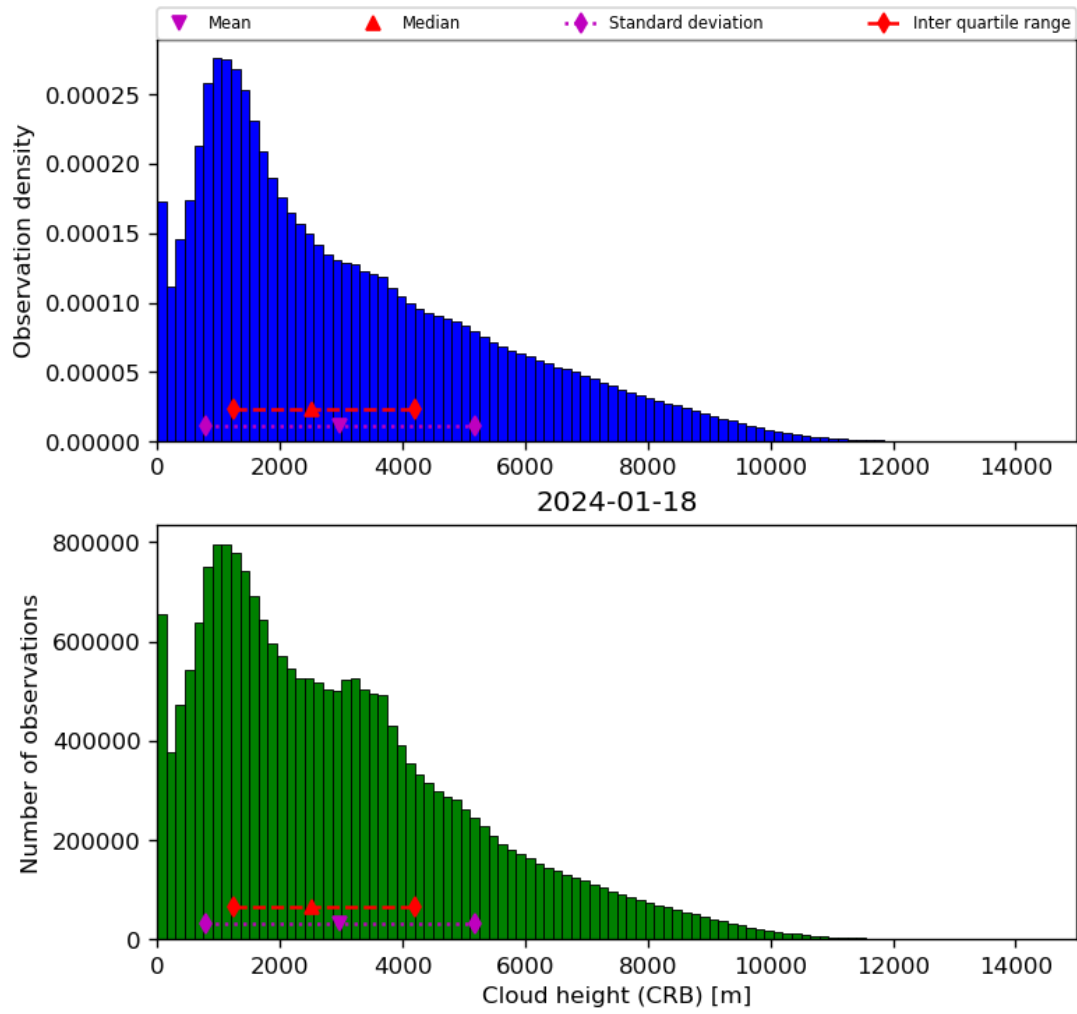
Figure 43: Histogram of “Cloud height (CRB)” for 2024-01-17 to 2024-01-19
