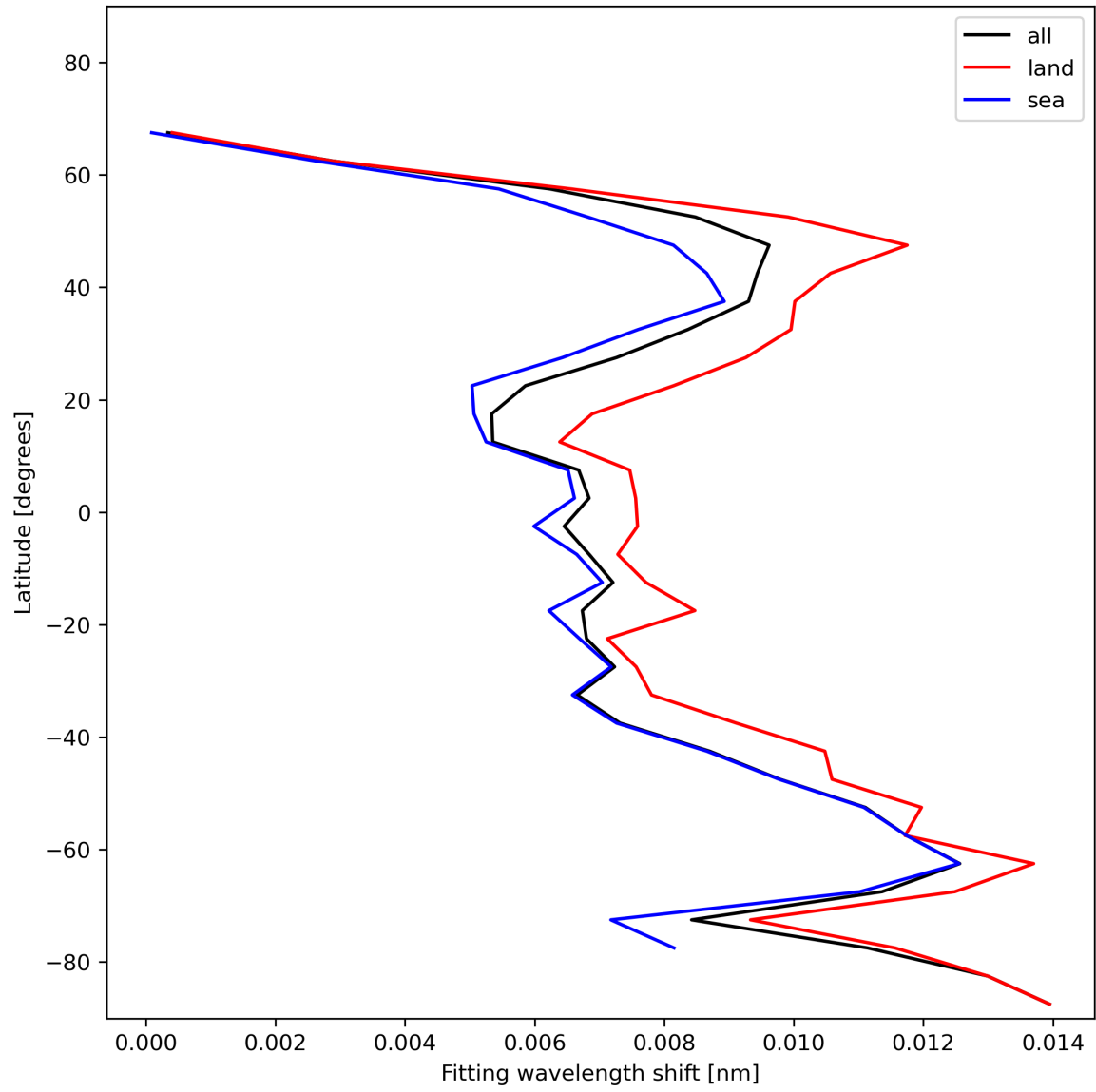
Figure 33: Zonal average of “Fitting wavelength shift” for 2024-01-17 to 2024-01-19.
