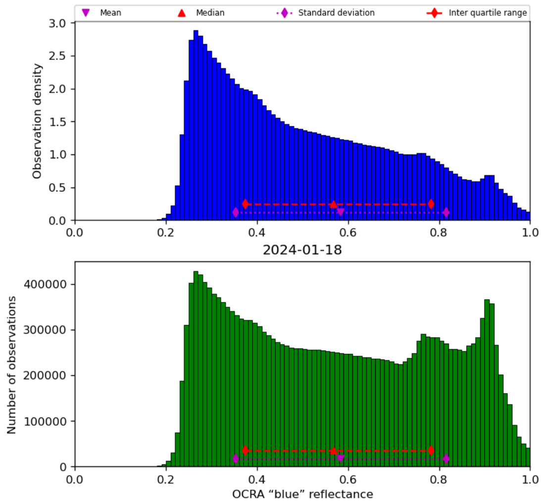
Figure 51: Histogram of “OCRA “blue” reflectance” for 2024-01-17 to 2024-01-19
