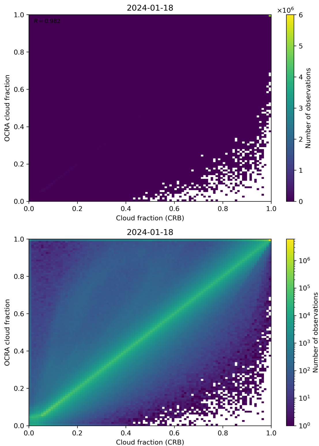
Figure 78: Scatter density plot of “Cloud fraction (CRB)” against “OCRA cloud fraction” for 2024-01-17 to 2024-01-19.
