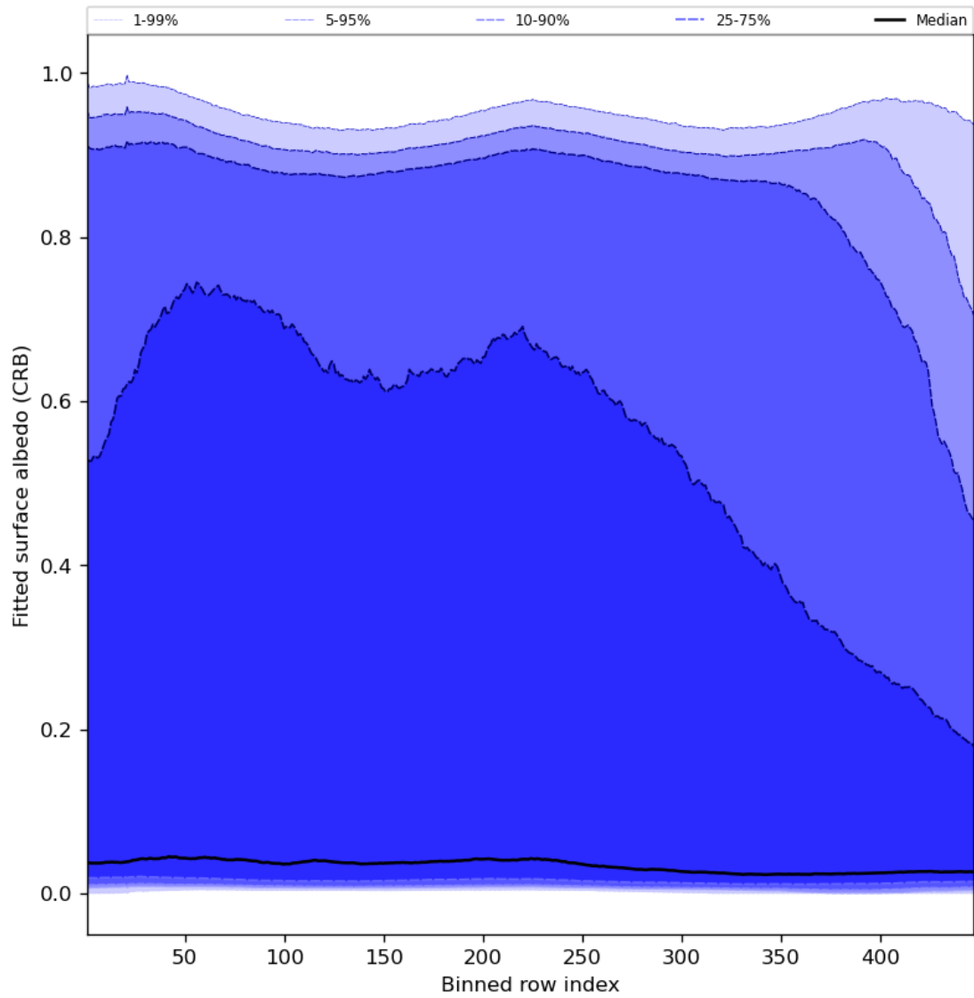
Figure 62: Along track statistics of “Fitted surface albedo (CRB)” for 2024-01-17 to 2024-01-19
