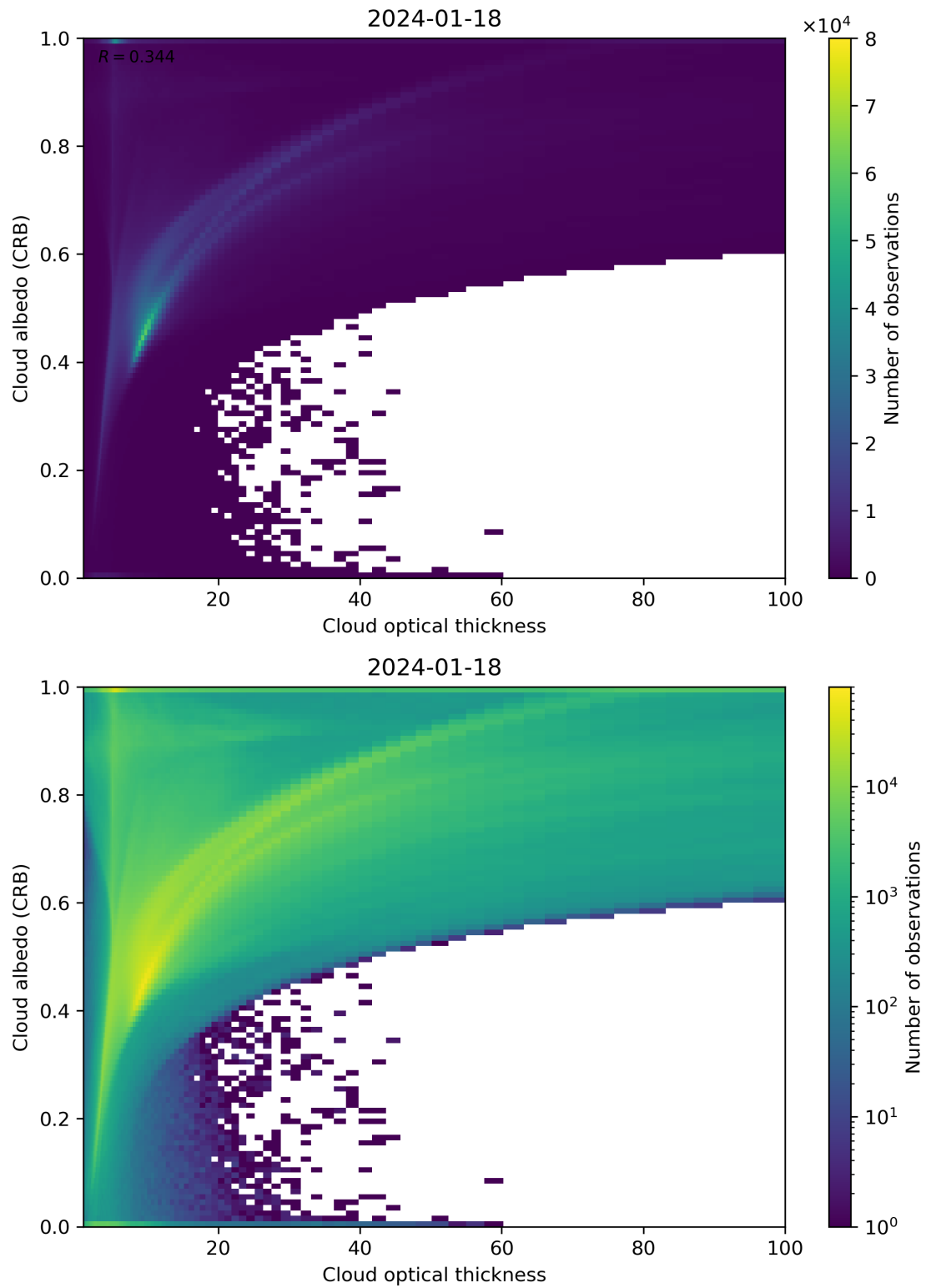
Figure 82: Scatter density plot of “Cloud optical thickness” against “Cloud albedo (CRB)” for 2024-01-17 to 2024-01-19.
