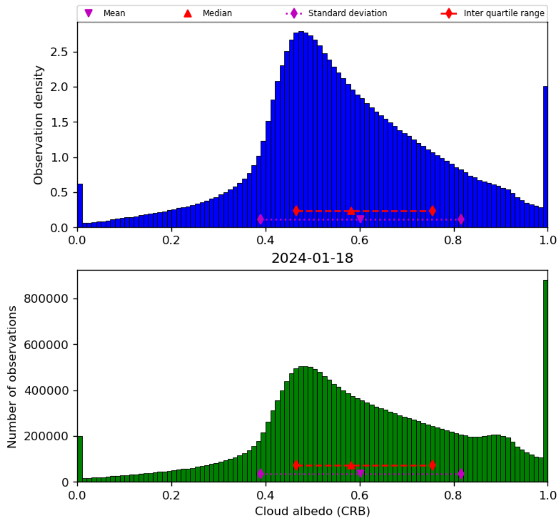
Figure 44: Histogram of “Cloud albedo (CRB)” for 2024-01-17 to 2024-01-19
