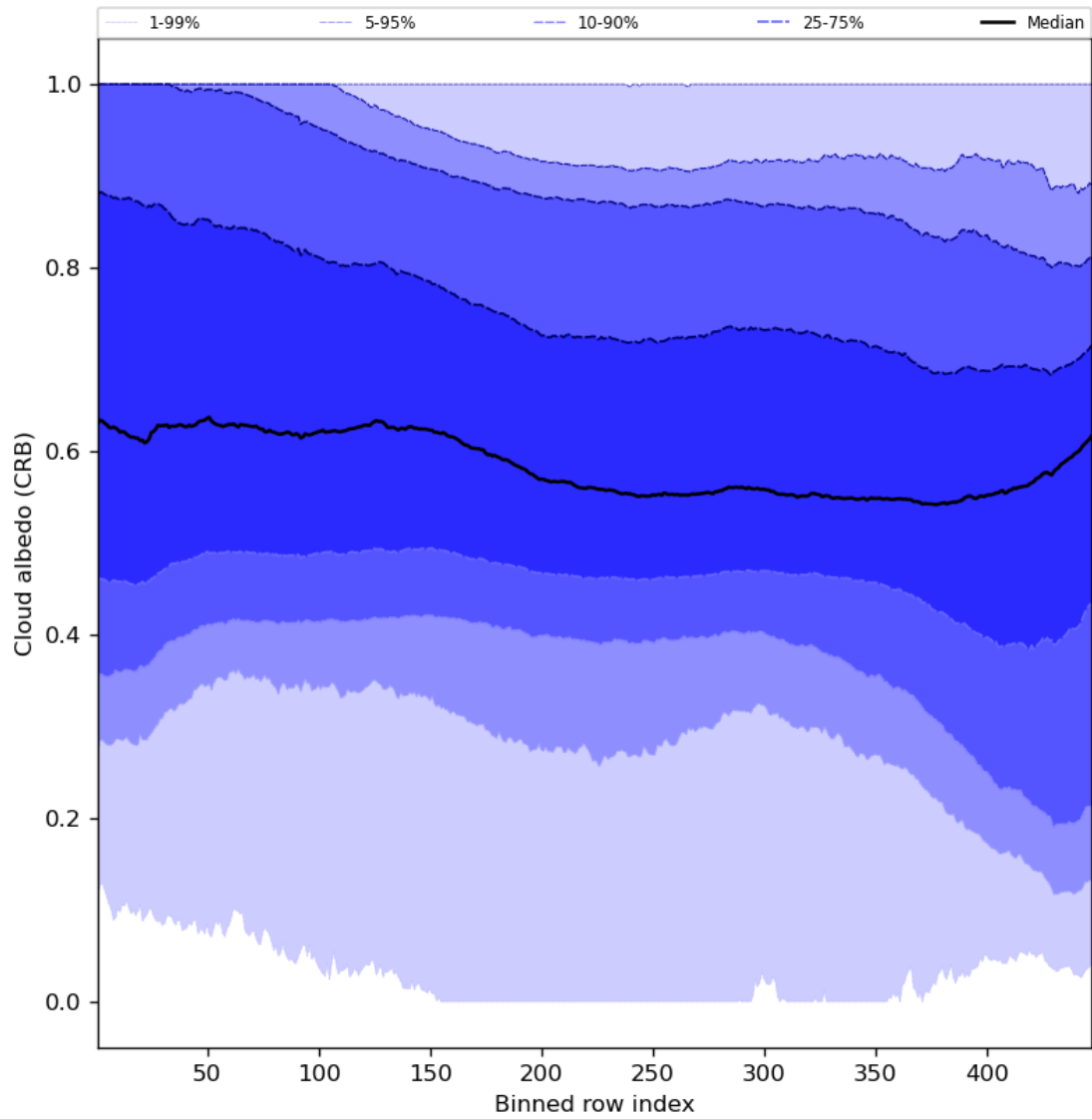
Figure 60: Along track statistics of “Cloud albedo (CRB)” for 2024-01-17 to 2024-01-19
