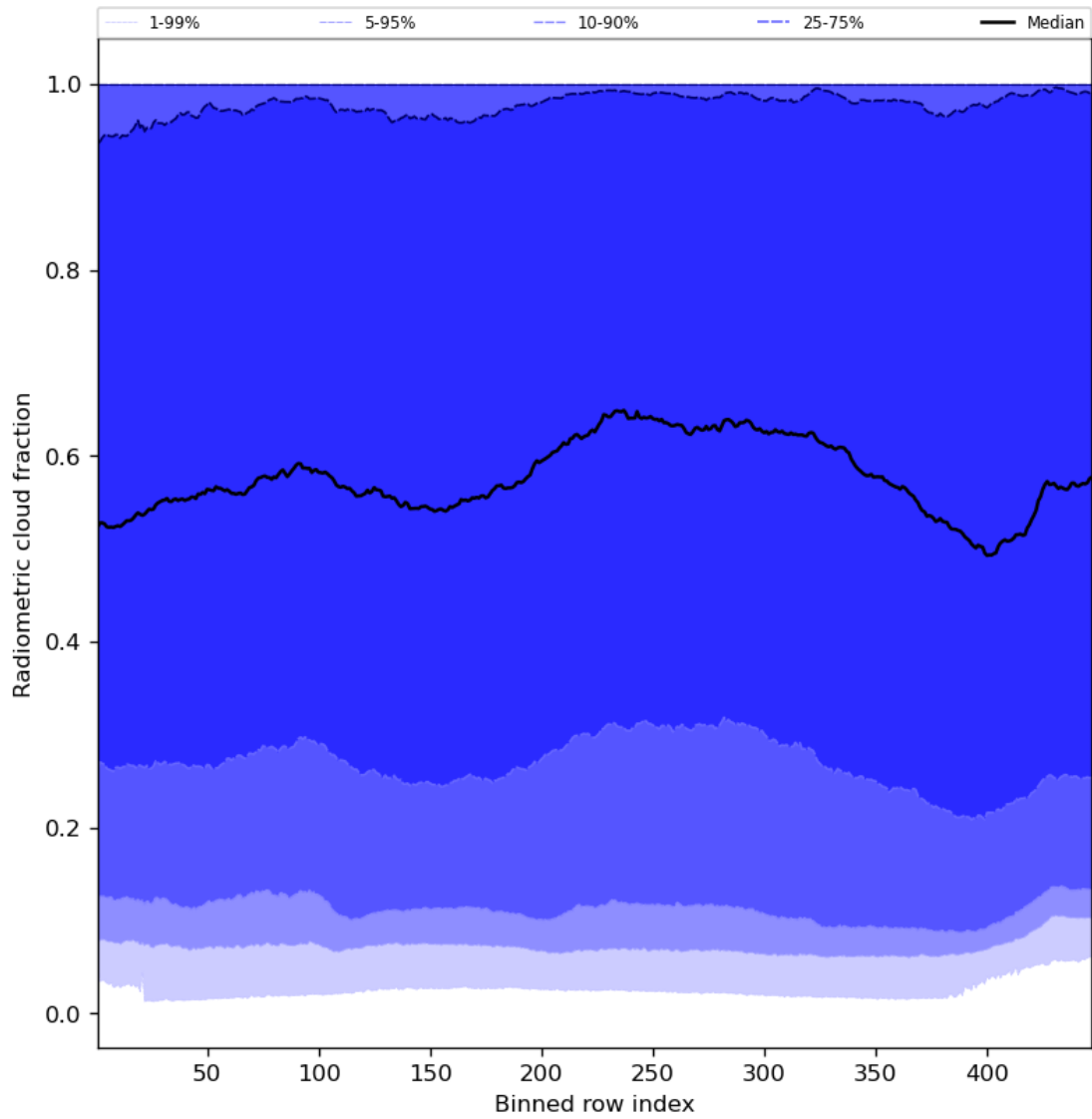
Figure 55: Along track statistics of “Radiometric cloud fraction” for 2024-01-17 to 2024-01-19
