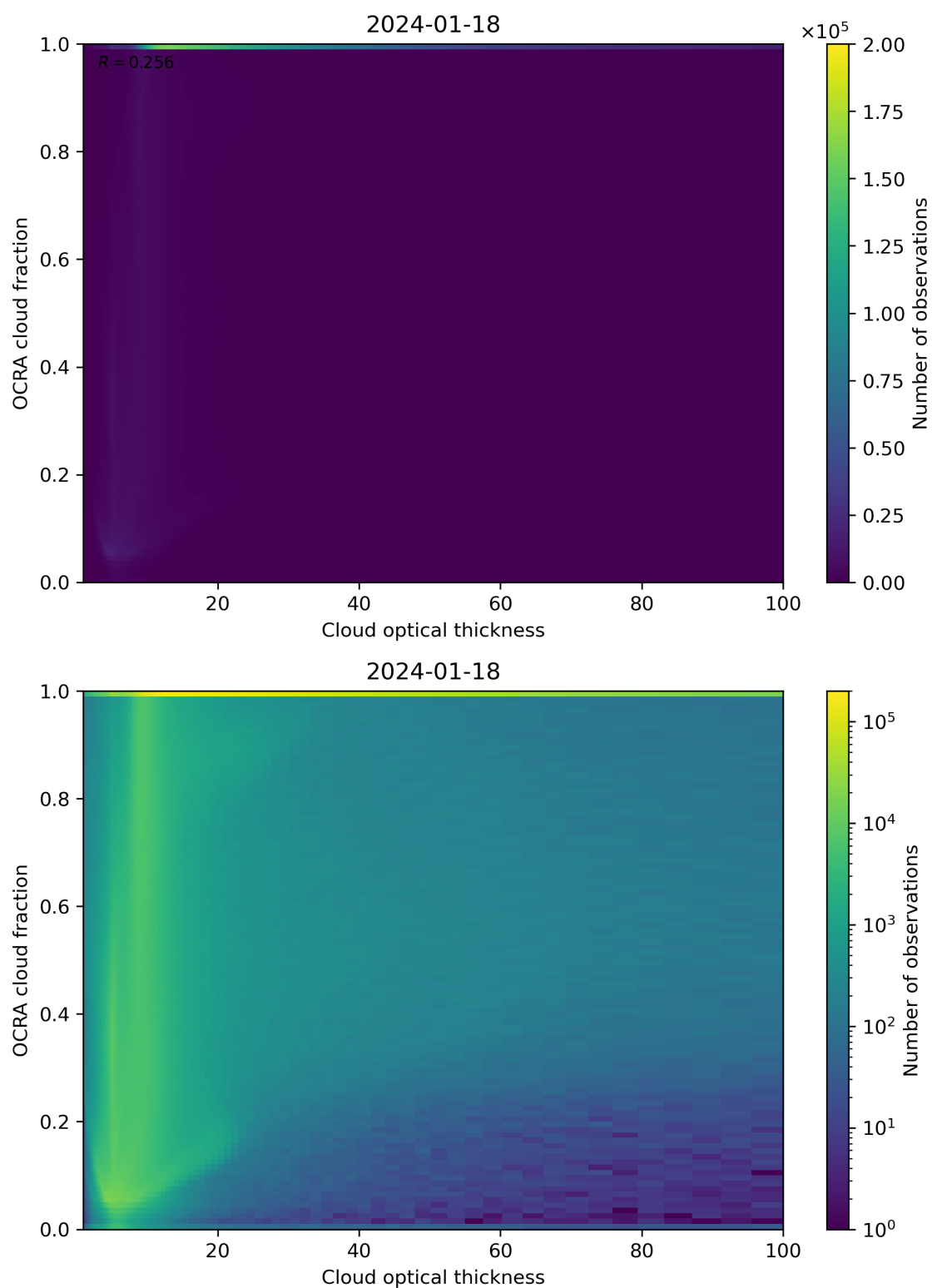
Figure 83: Scatter density plot of “Cloud optical thickness” against “OCRA cloud fraction” for 2024-01-17 to 2024-01-19.
