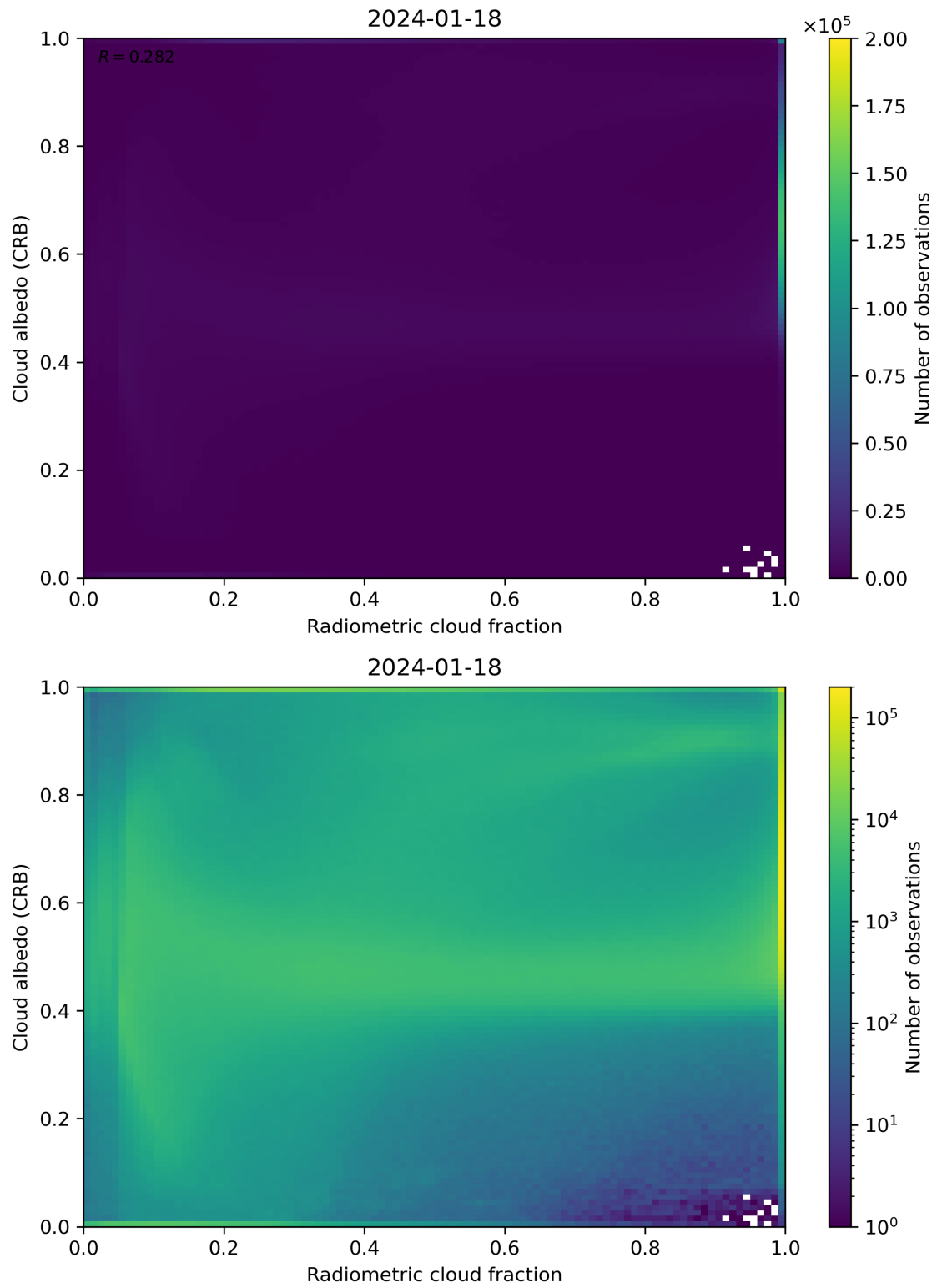
Figure 71: Scatter density plot of “Radiometric cloud fraction” against “Cloud albedo (CRB)” for 2024-01-17 to 2024-01-19.
