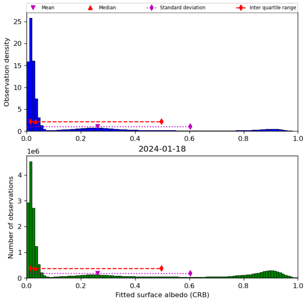
Figure 46: Histogram of “Fitted surface albedo (CRB)” for 2024-01-17 to 2024-01-19
