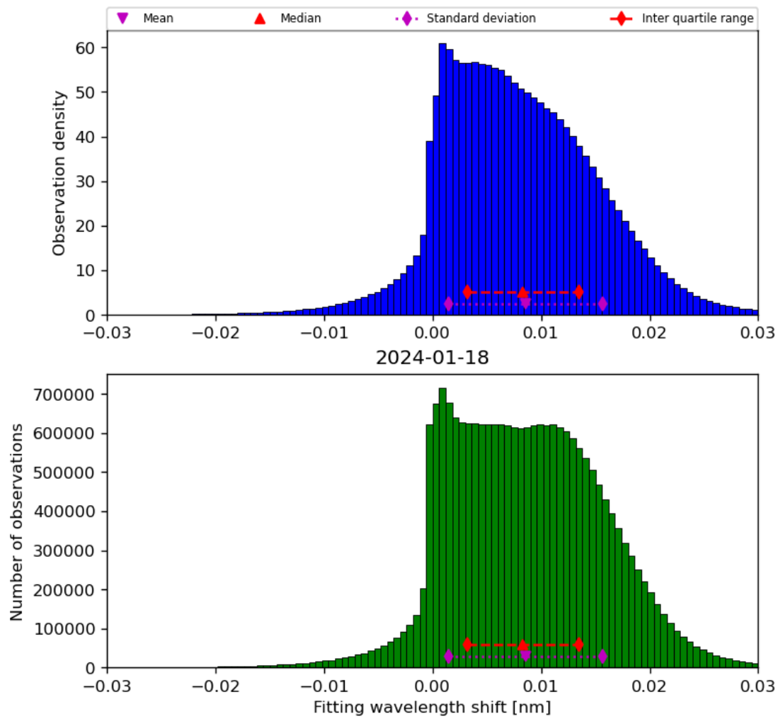
Figure 49: Histogram of “Fitting wavelength shift” for 2024-01-17 to 2024-01-19
