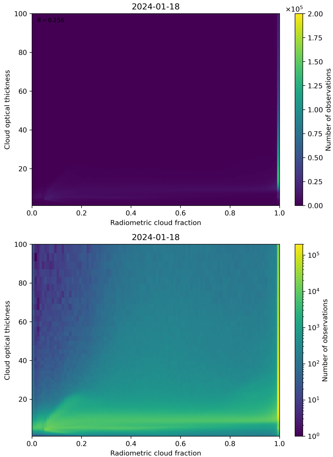
Figure 75: Scatter density plot of “Radiometric cloud fraction” against “Cloud optical thickness” for 2024-01-17 to 2024-01-19.
