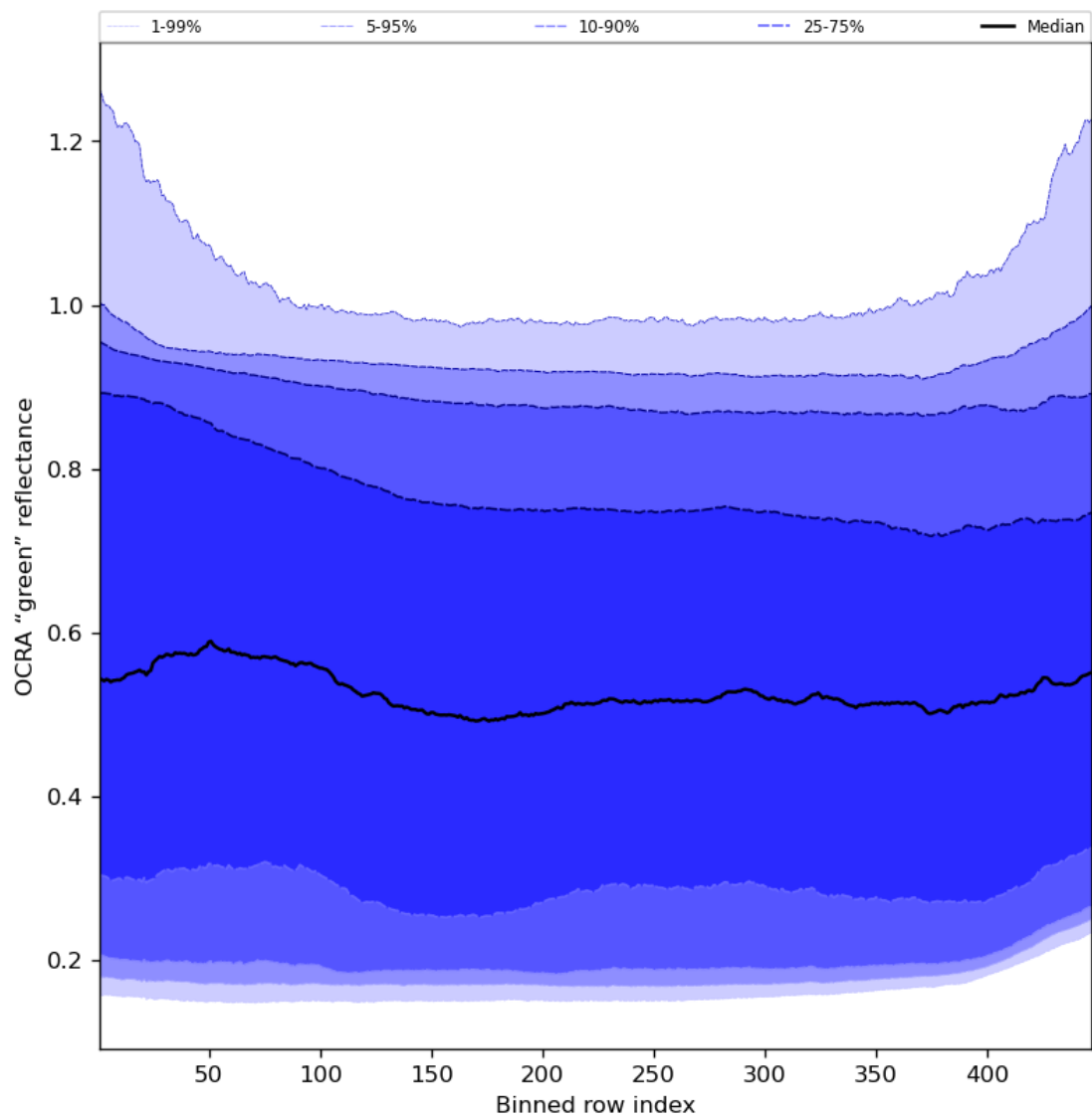
Figure 68: Along track statistics of "OCRA "green" reflectance" for 2024-01-17 to 2024-01-19
