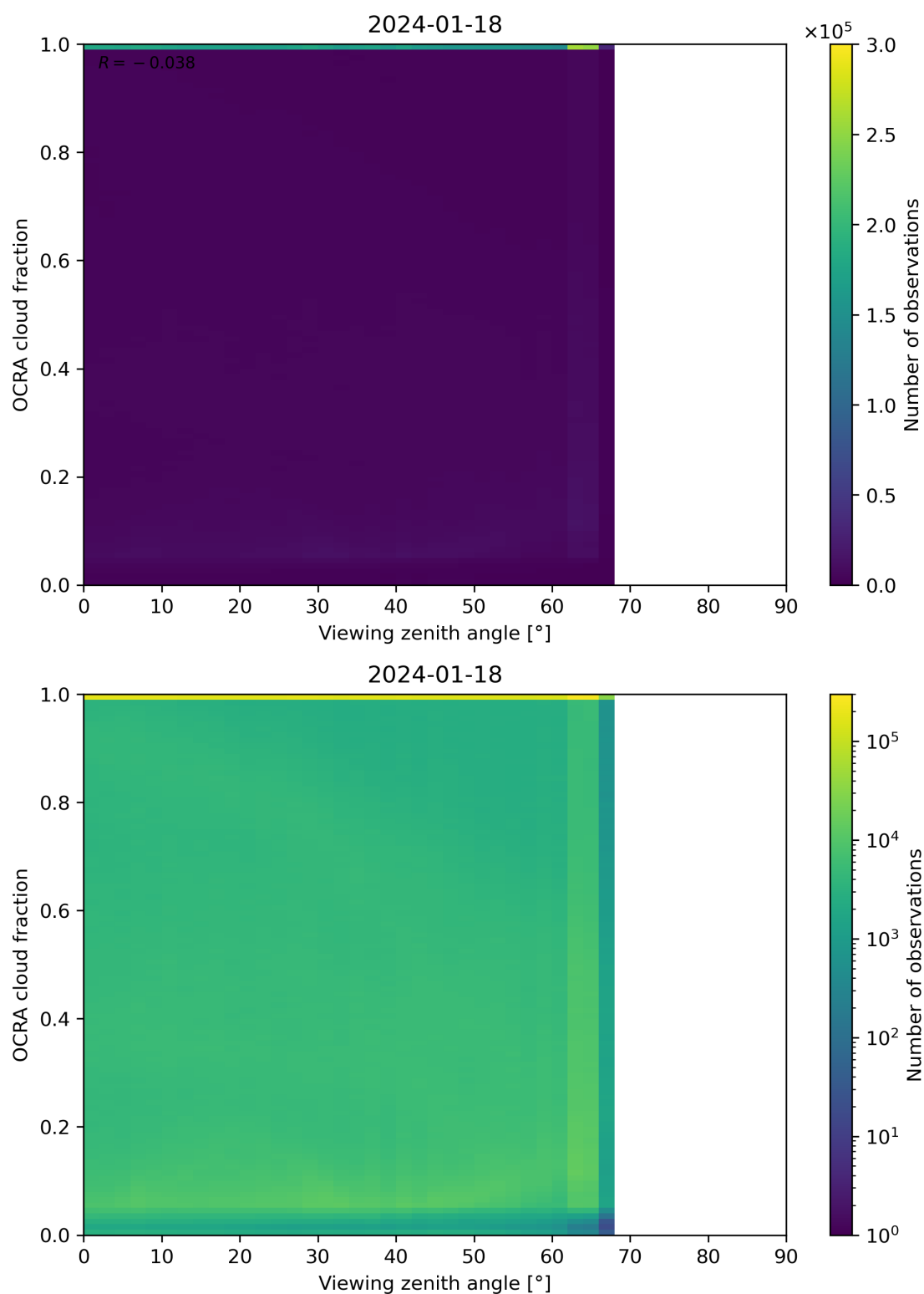
Figure 108: Scatter density plot of “Viewing zenith angle” against “OCRA cloud fraction” for 2024-01-17 to 2024-01-19.
