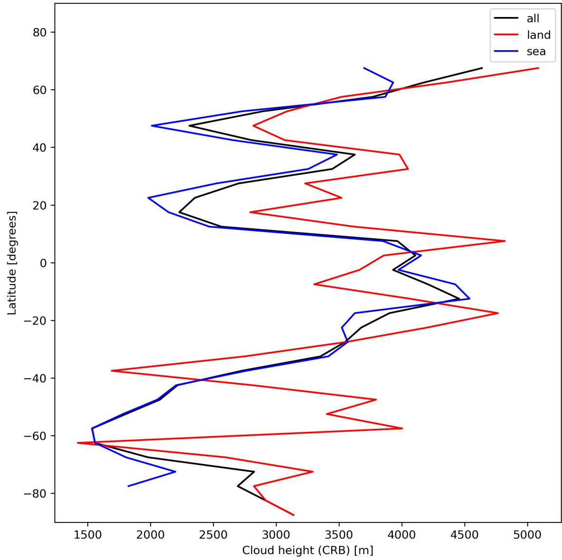
Figure 27: Zonal average of “Cloud height (CRB)” for 2024-01-17 to 2024-01-19.
