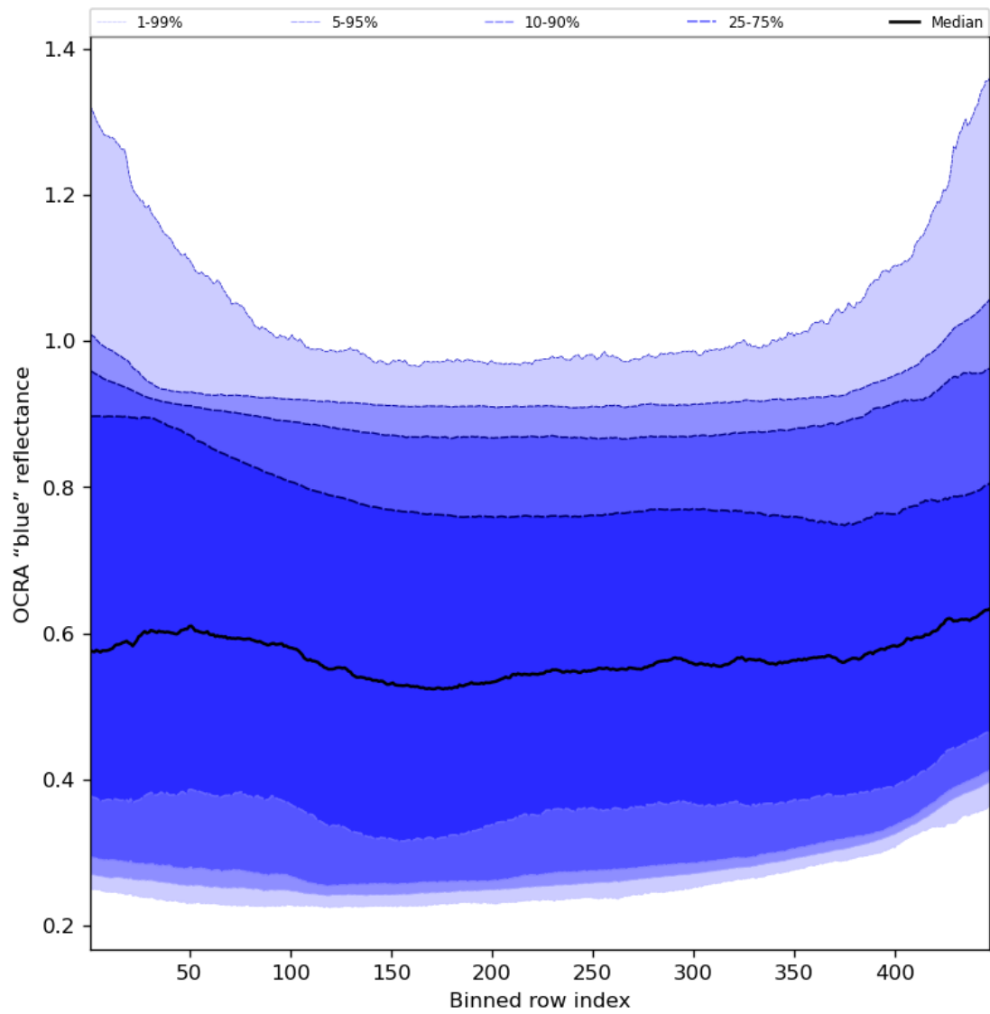
Figure 67: Along track statistics of “OCRA “blue” reflectance” for 2024-01-17 to 2024-01-19
