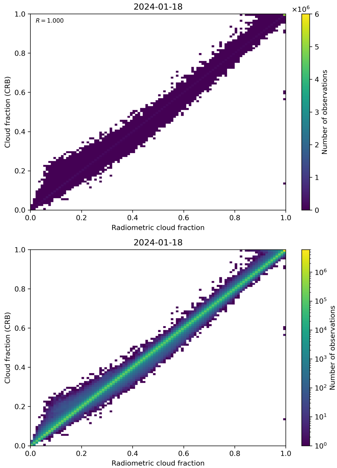
Figure 73: Scatter density plot of “Radiometric cloud fraction” against “Cloud fraction (CRB)” for 2024-01-17 to 2024-01-19.
