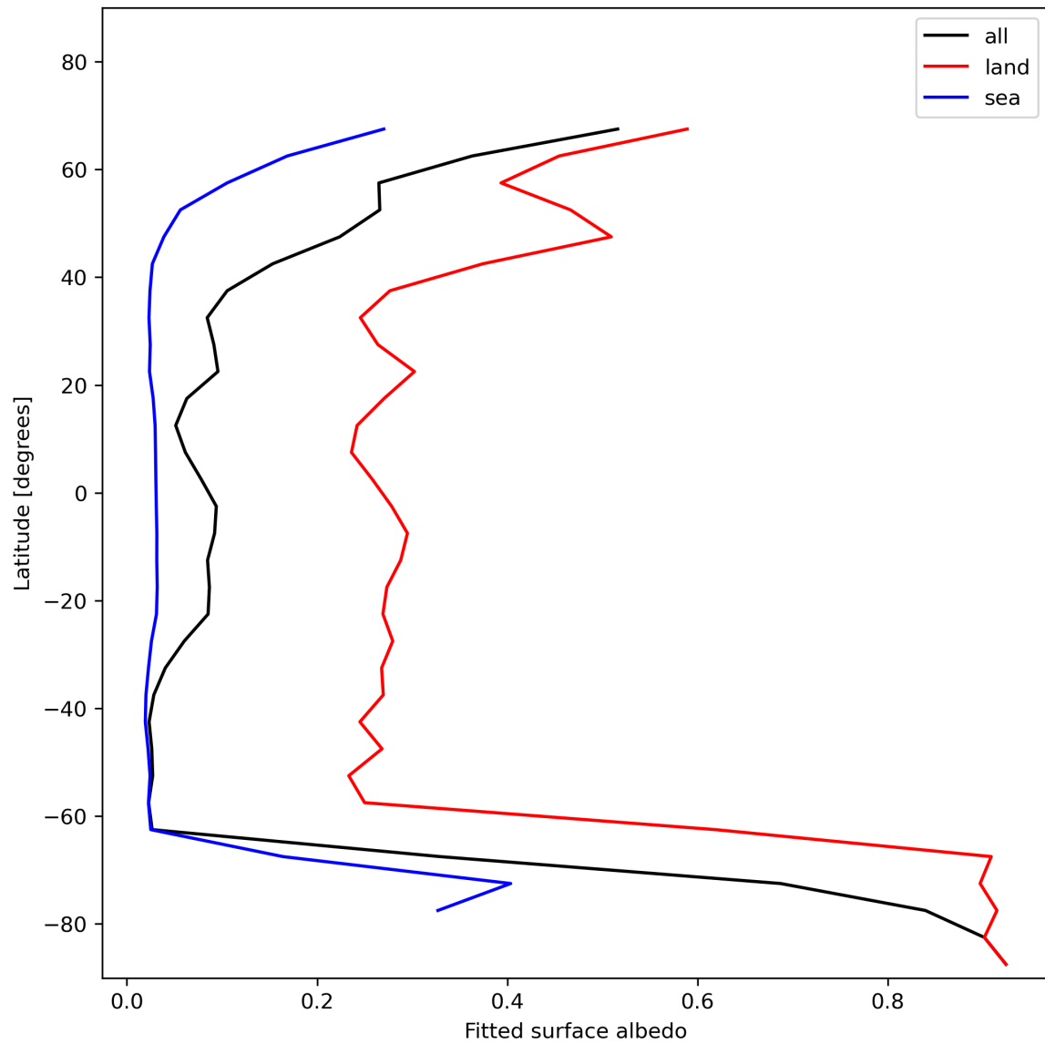
Figure 29: Zonal average of “Fitted surface albedo” for 2024-01-17 to 2024-01-19.
