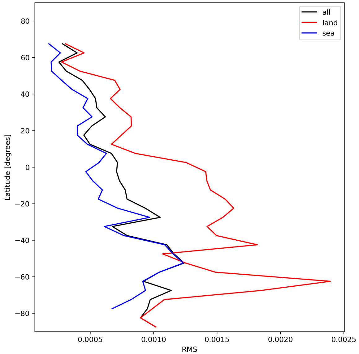
Figure 31: Zonal average of “RMS” for 2024-01-17 to 2024-01-19.
