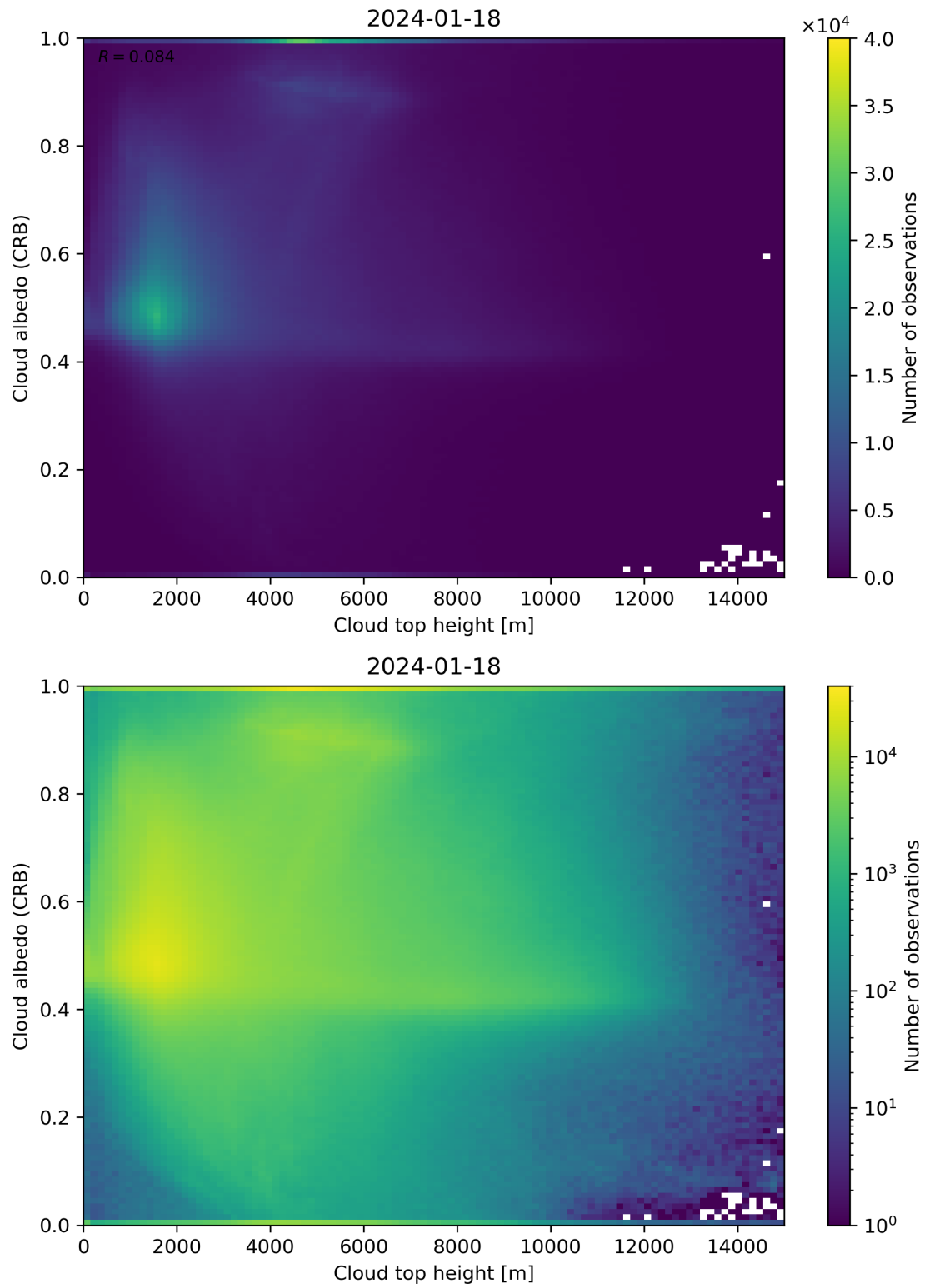
Figure 86: Scatter density plot of “Cloud top height” against “Cloud albedo (CRB)” for 2024-01-17 to 2024-01-19.
