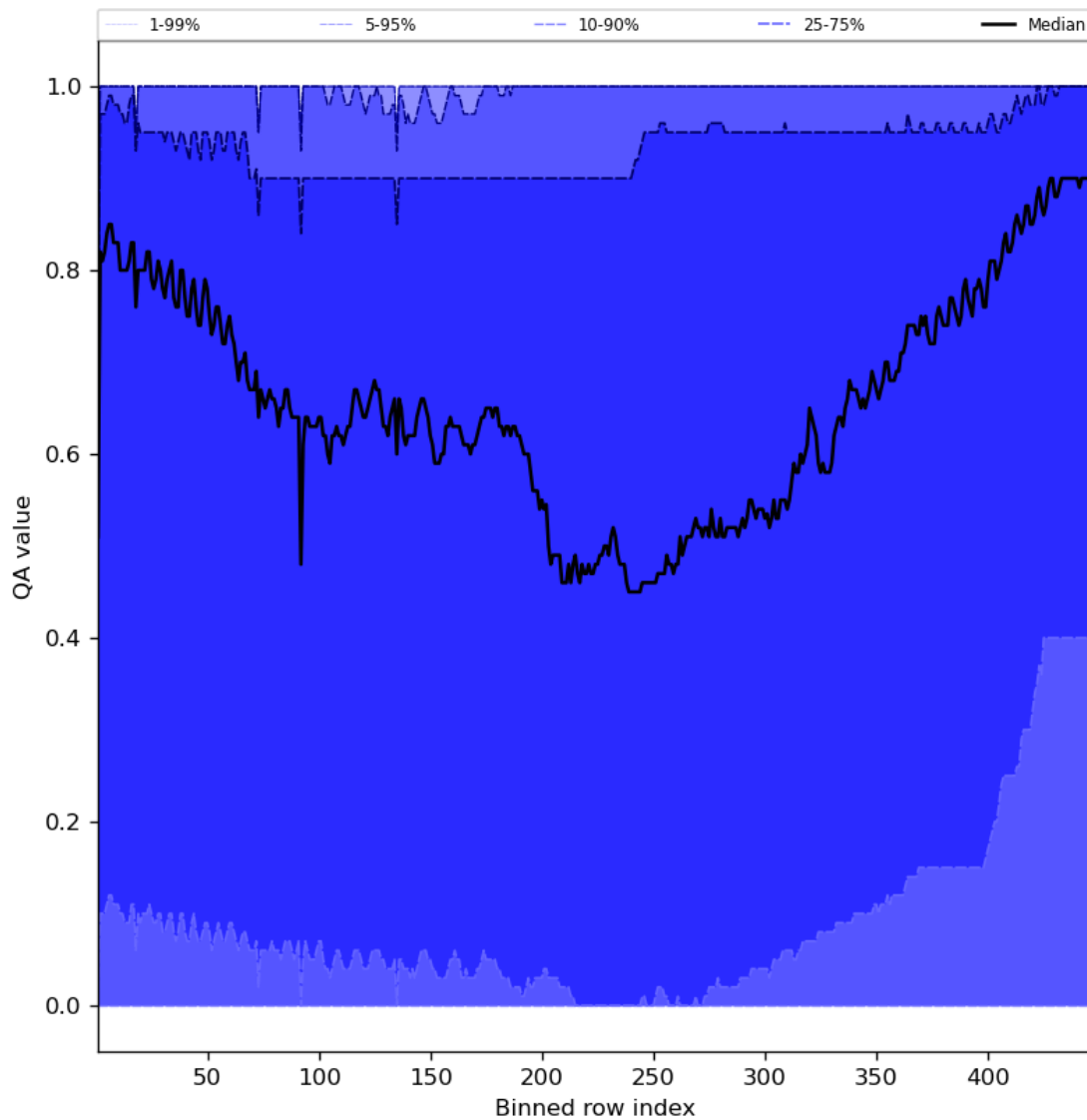
Figure 54: Along track statistics of “QA value” for 2024-01-17 to 2024-01-19
