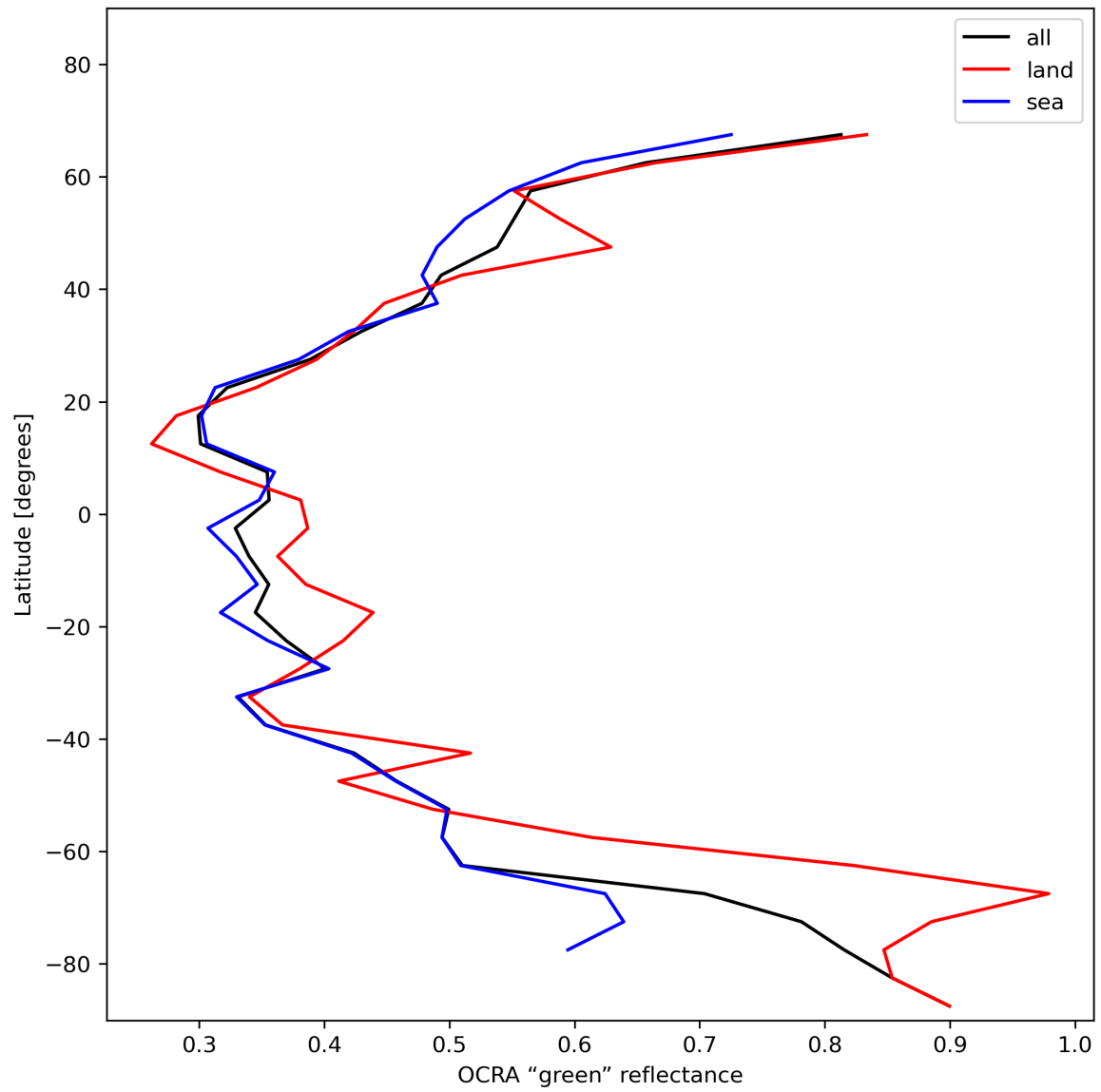
Figure 36: Zonal average of “OCRA “green” reflectance” for 2024-01-17 to 2024-01-19.
