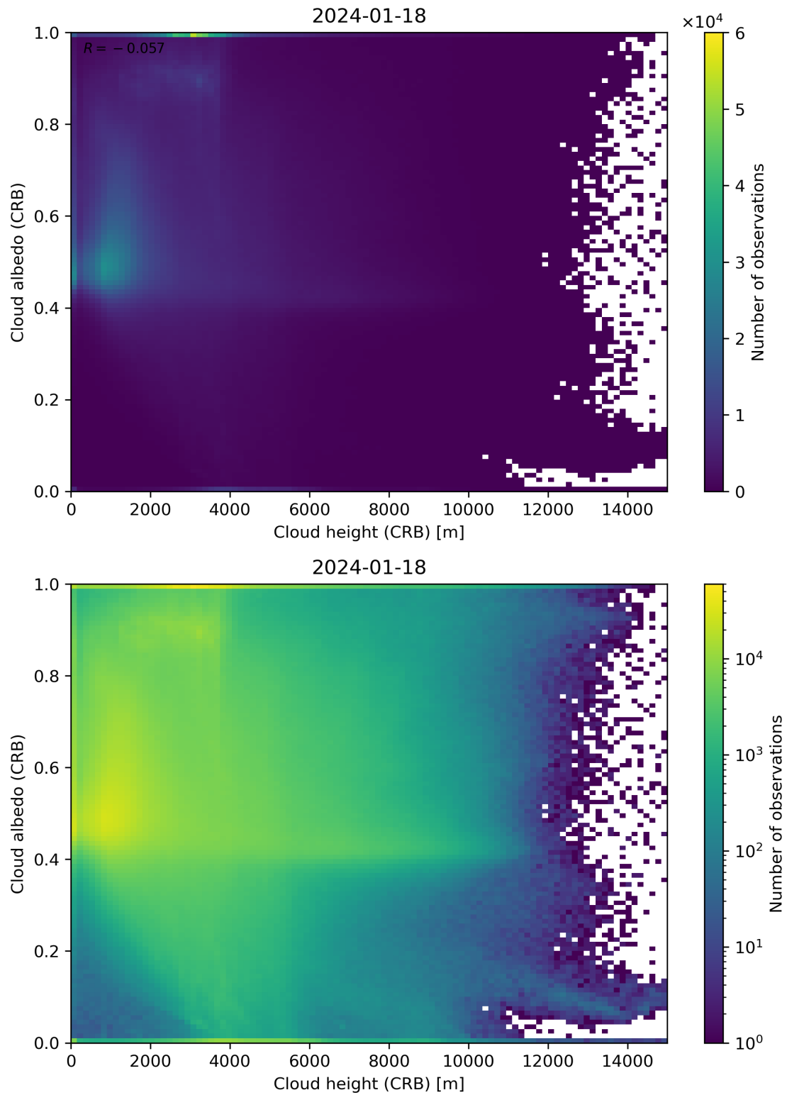
Figure 80: Scatter density plot of “Cloud height (CRB)” against “Cloud albedo (CRB)” for 2024-01-17 to 2024-01-19.
