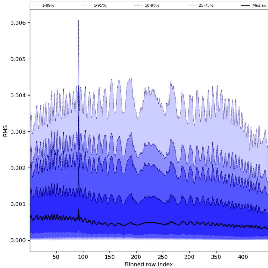
Figure 63: Along track statistics of “RMS” for 2024-01-17 to 2024-01-19
