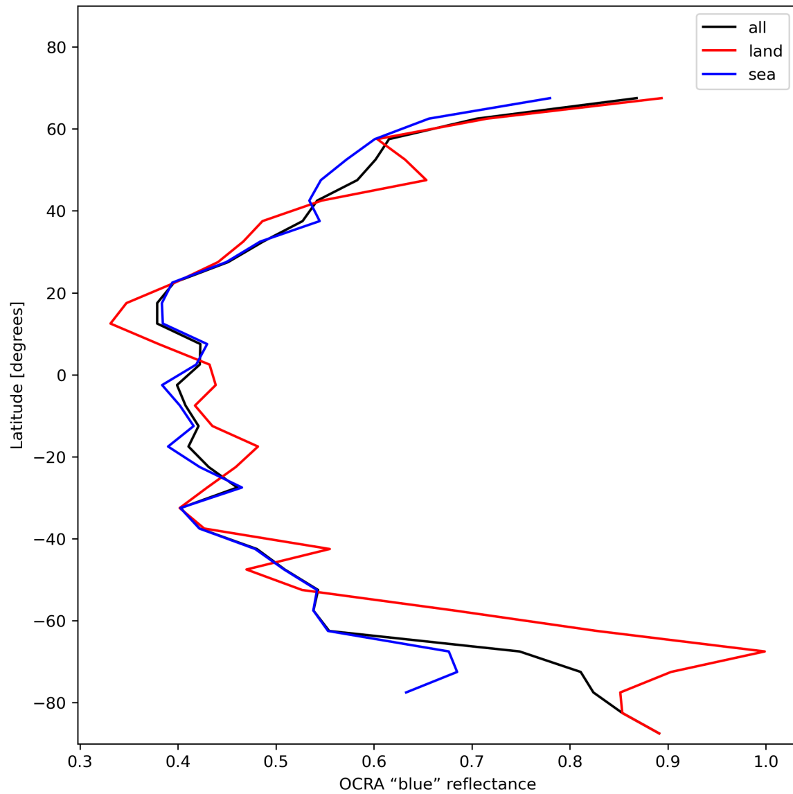
Figure 35: Zonal average of “OCRA “blue” reflectance” for 2024-01-17 to 2024-01-19.
