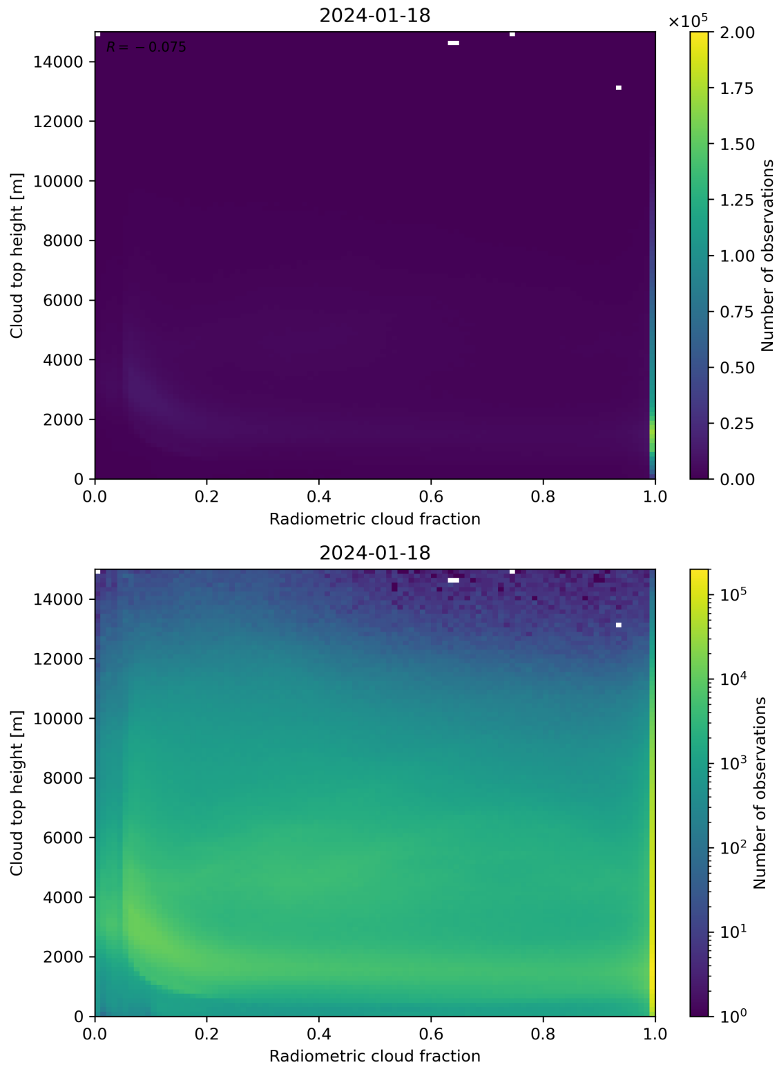
Figure 76: Scatter density plot of “Radiometric cloud fraction” against “Cloud top height” for 2024-01-17 to 2024-01-19.
