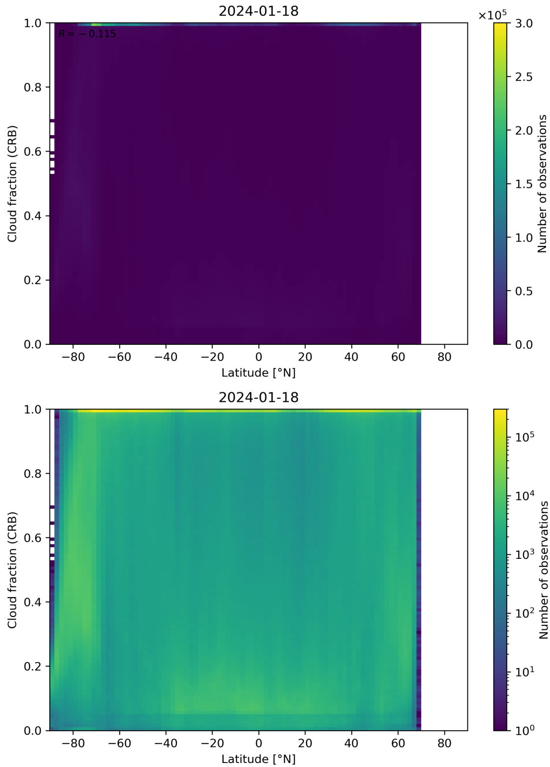
Figure 94: Scatter density plot of “Latitude” against “Cloud fraction (CRB)” for 2024-01-17 to 2024-01-19.
