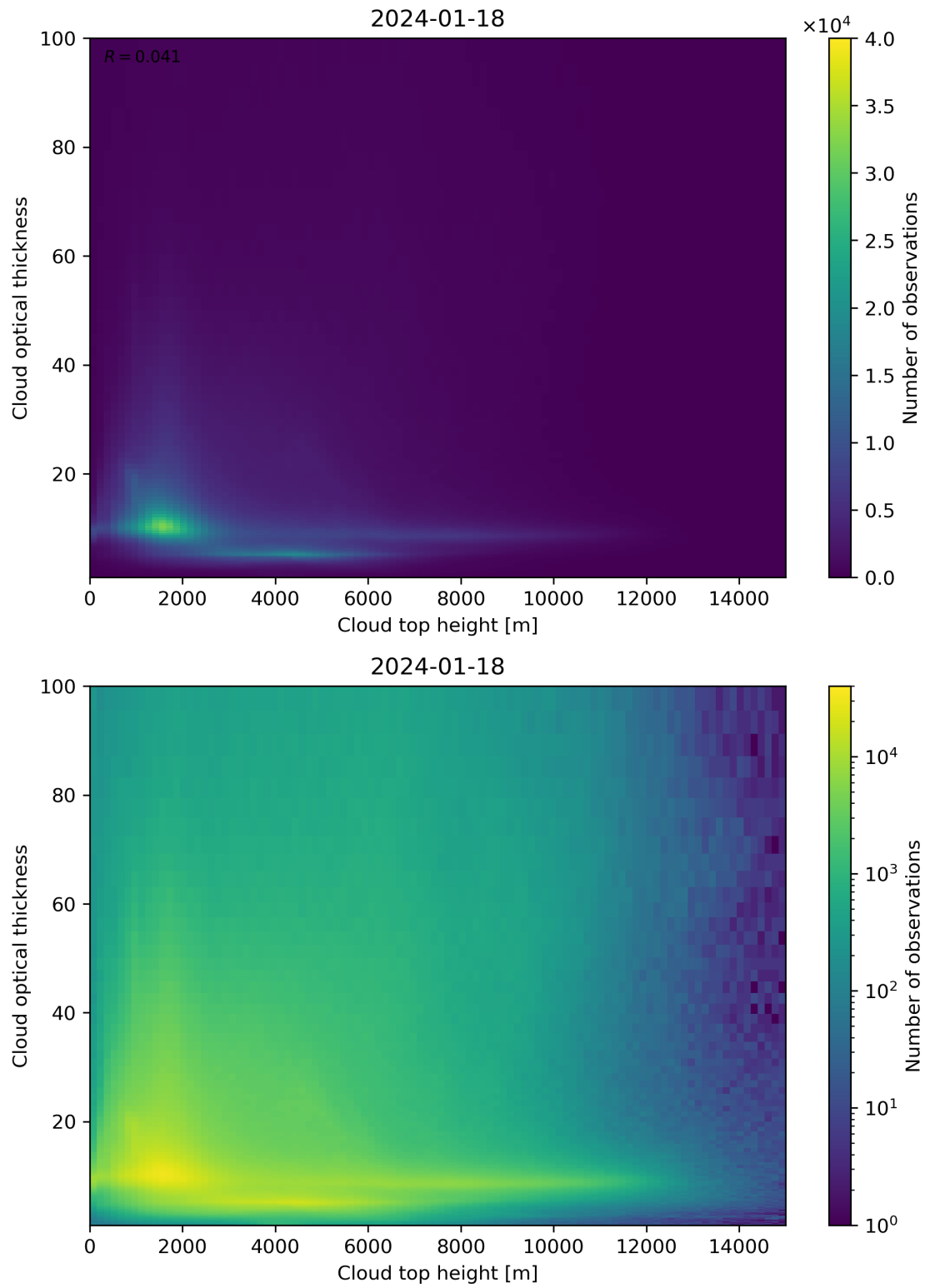
Figure 90: Scatter density plot of “Cloud top height” against “Cloud optical thickness” for 2024-01-17 to 2024-01-19.
