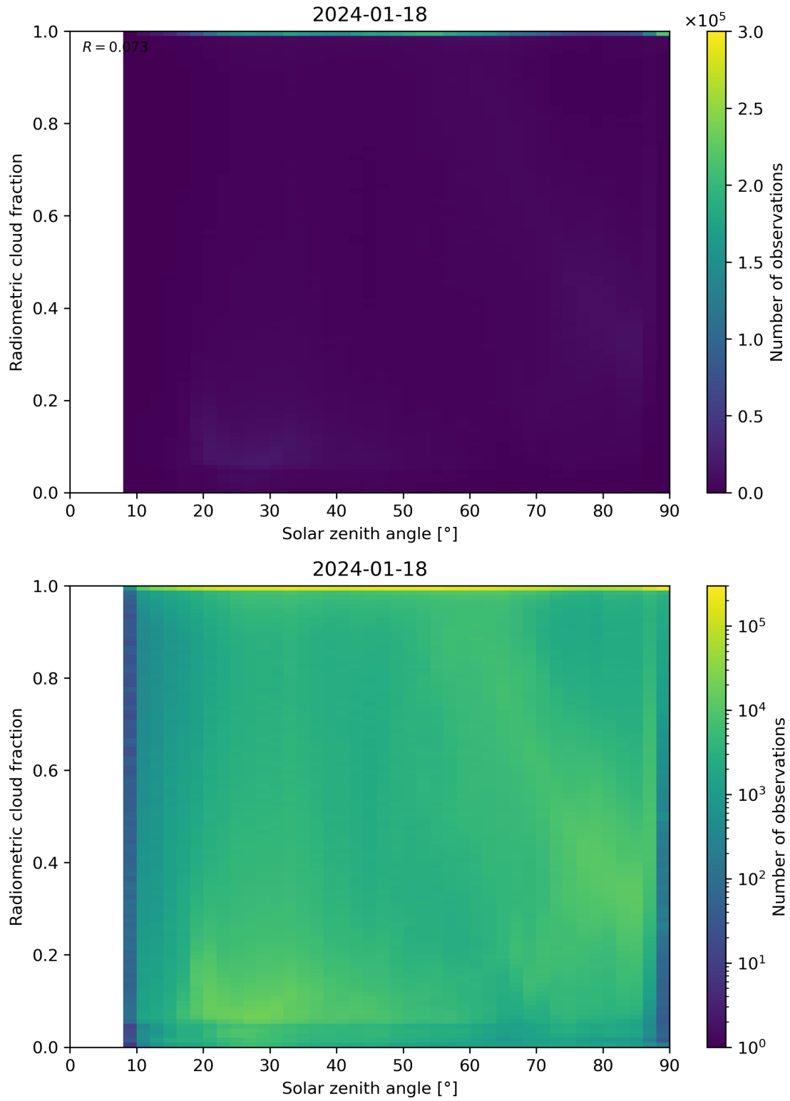
Figure 99: Scatter density plot of “Solar zenith angle” against “Radiometric cloud fraction” for 2024-01-17 to 2024-01-19.
