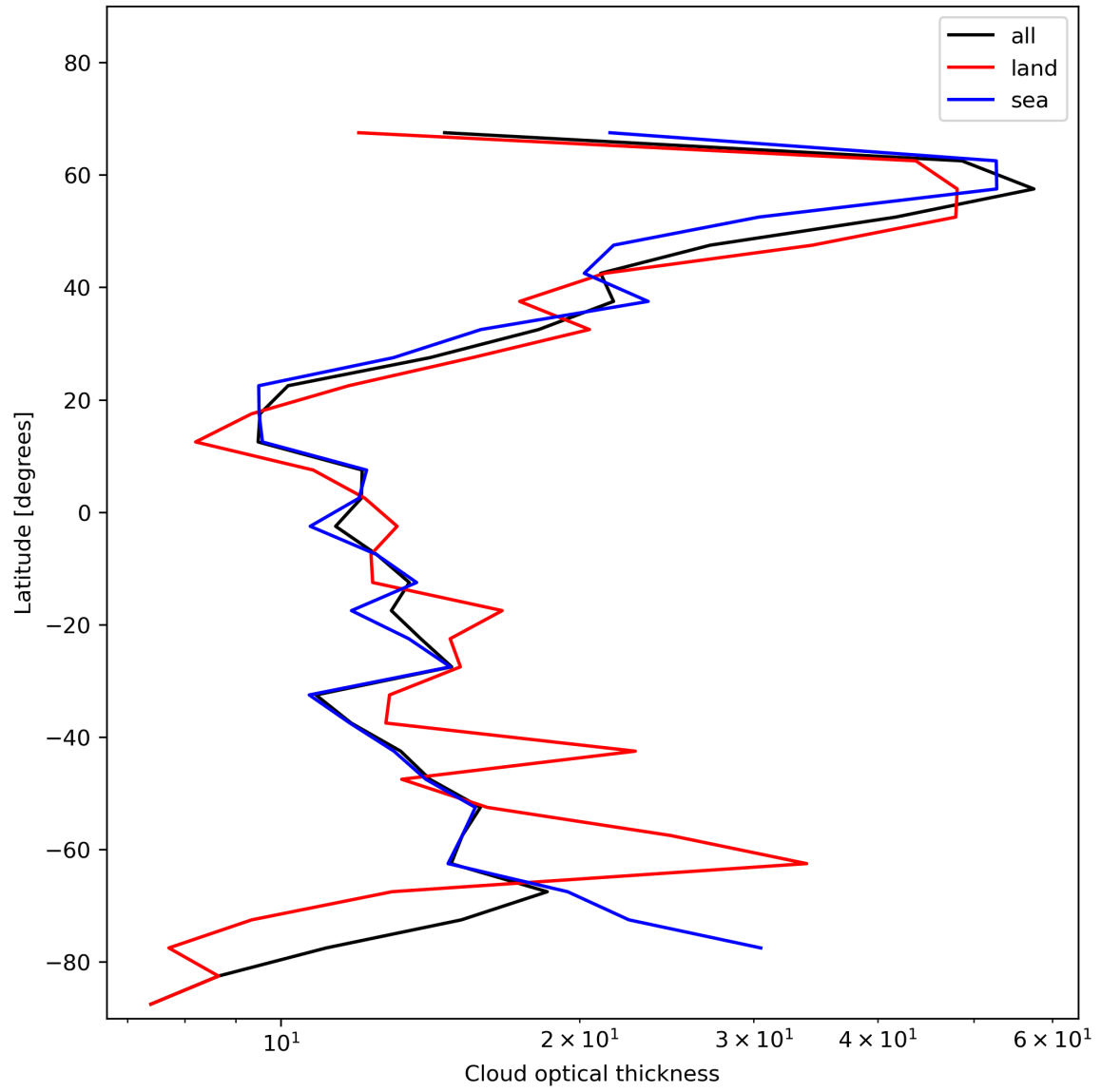
Figure 25: Zonal average of “Cloud optical thickness” for 2024-01-17 to 2024-01-19.
