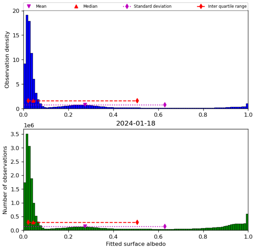
Figure 45: Histogram of “Fitted surface albedo” for 2024-01-17 to 2024-01-19
