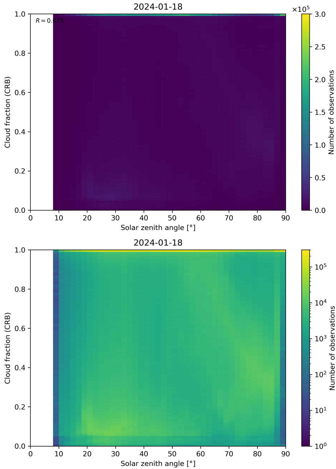
Figure 101: Scatter density plot of “Solar zenith angle” against “Cloud fraction (CRB)” for 2024-01-17 to 2024-01-19.
