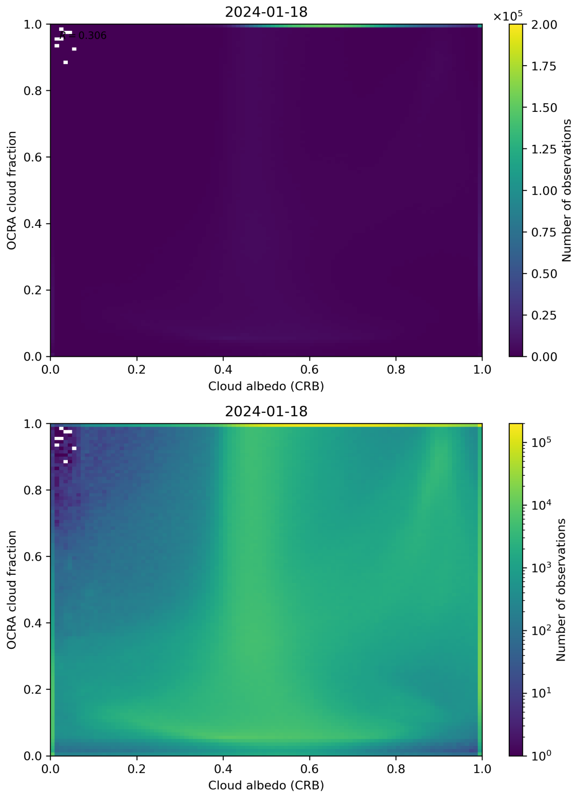
Figure 70: Scatter density plot of “Cloud albedo (CRB)” against “OCRA cloud fraction” for 2024-01-17 to 2024-01-19.
