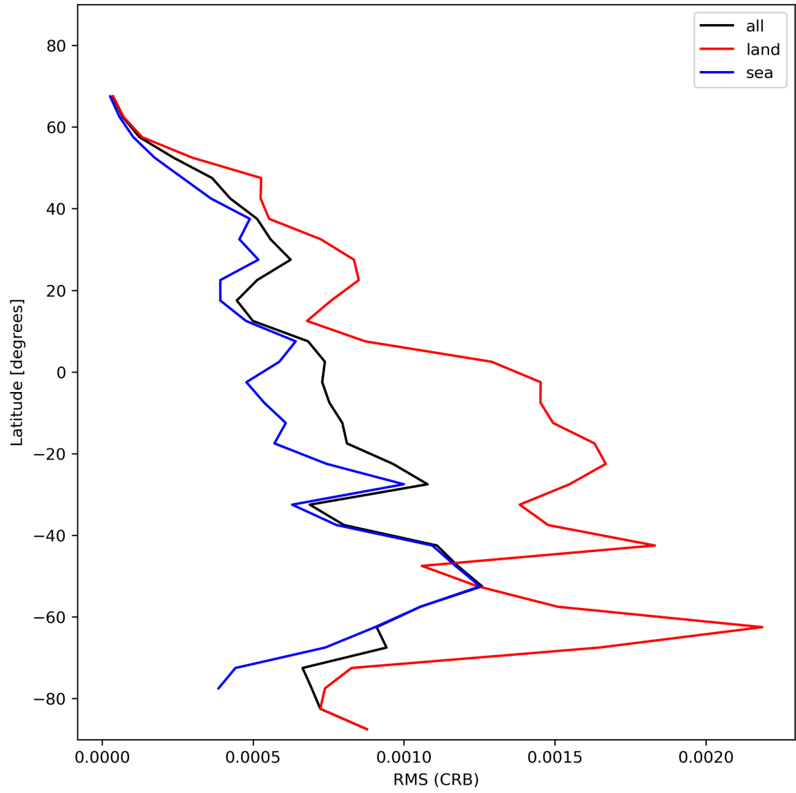
Figure 32: Zonal average of “RMS (CRB)” for 2024-01-17 to 2024-01-19.
