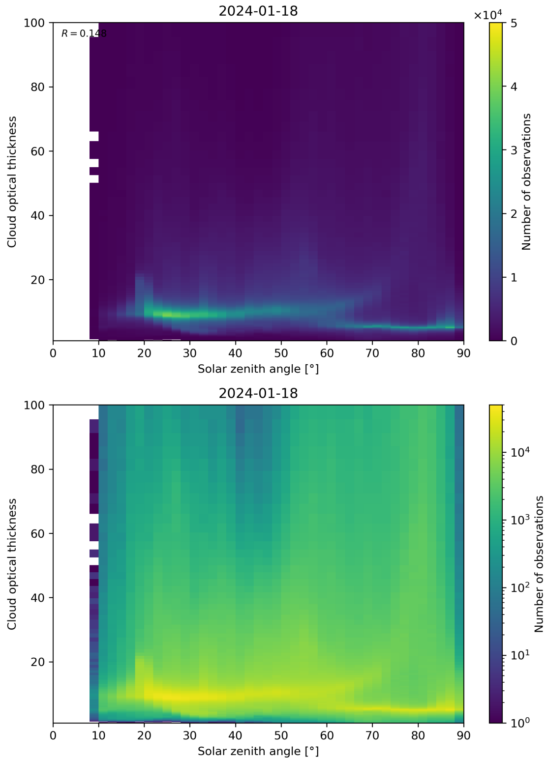
Figure 103: Scatter density plot of “Solar zenith angle” against “Cloud optical thickness” for 2024-01-17 to 2024-01-19.
