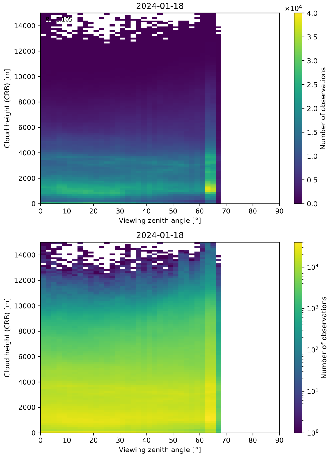
Figure 110: Scatter density plot of “Viewing zenith angle” against “Cloud height (CRB)” for 2024-01-17 to 2024-01-19.
