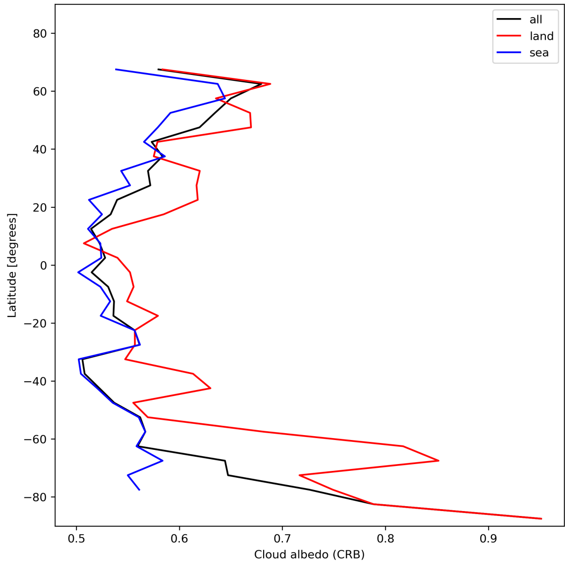
Figure 28: Zonal average of “Cloud albedo (CRB)” for 2024-01-17 to 2024-01-19.
