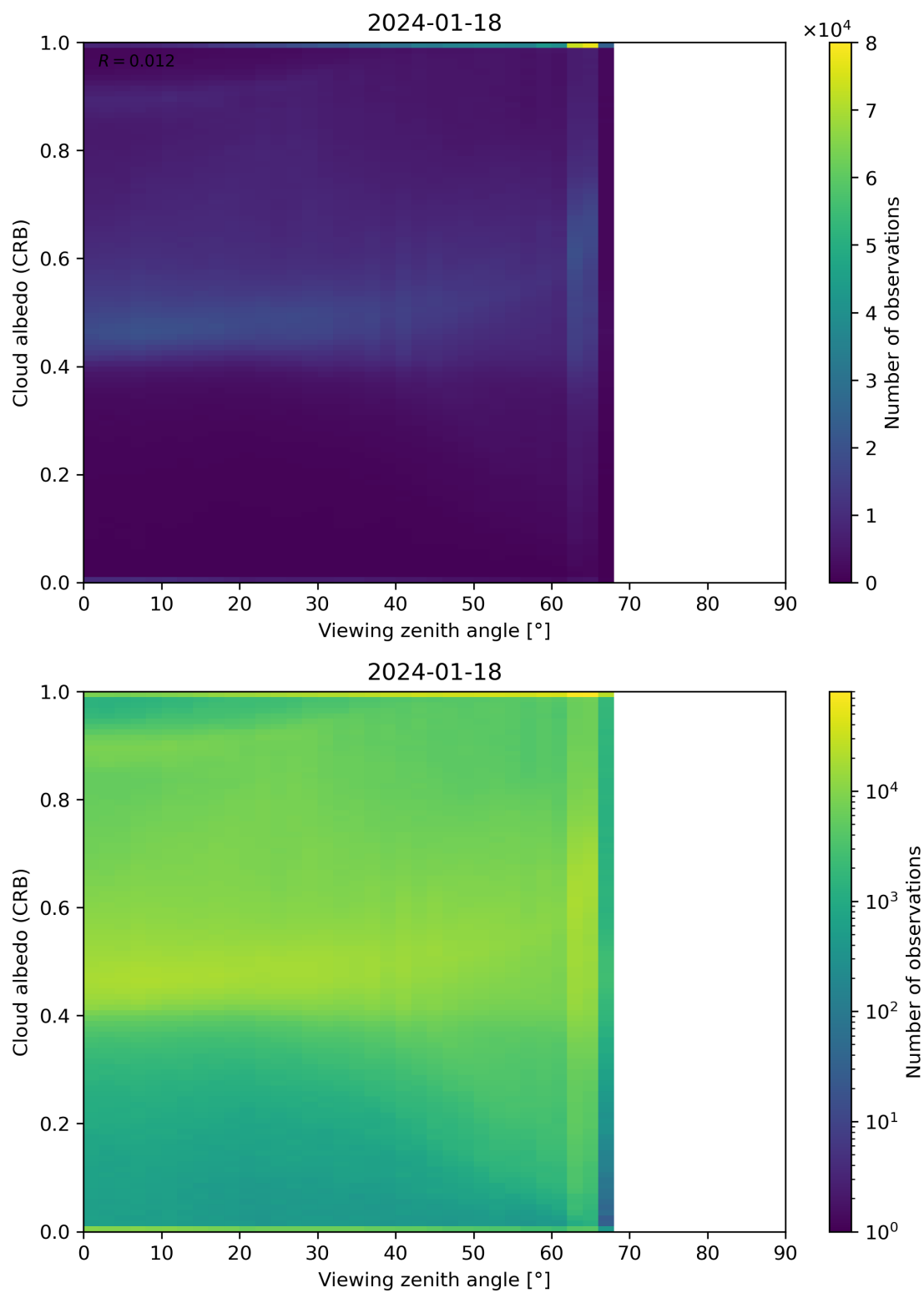
Figure 106: Scatter density plot of “Viewing zenith angle” against “Cloud albedo (CRB)” for 2024-01-17 to 2024-01-19.
