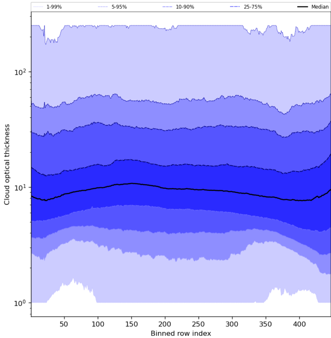
Figure 57: Along track statistics of “Cloud optical thickness” for 2024-01-17 to 2024-01-19
