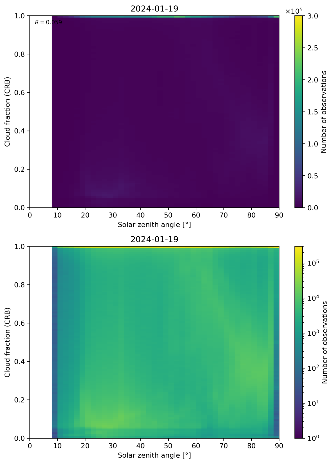
Figure 101: Scatter density plot of “Solar zenith angle” against “Cloud fraction (CRB)” for 2024-01-18 to 2024-01-20.
