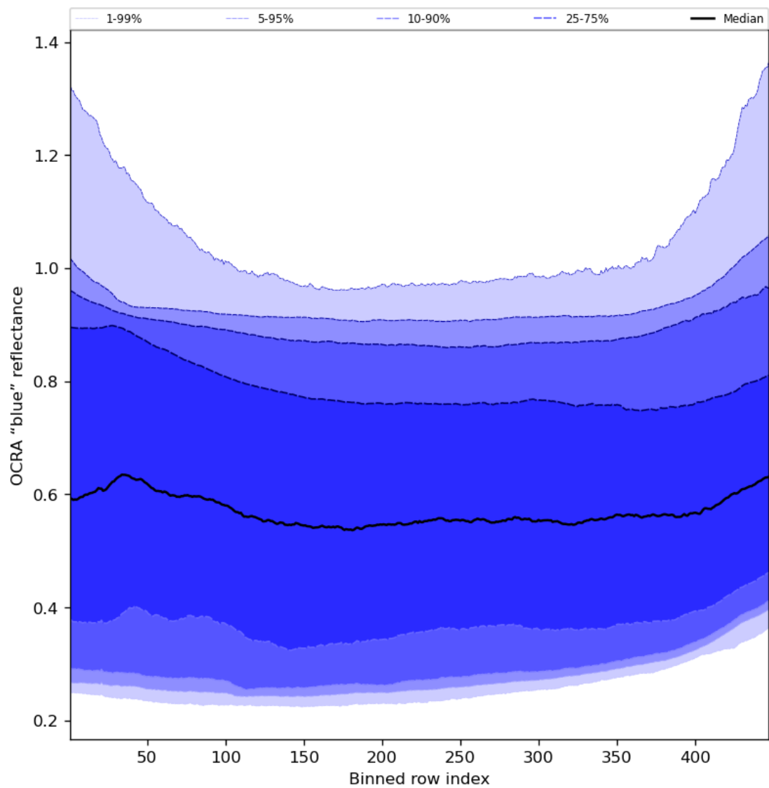
Figure 67: Along track statistics of “OCRA “blue” reflectance” for 2024-01-18 to 2024-01-20
