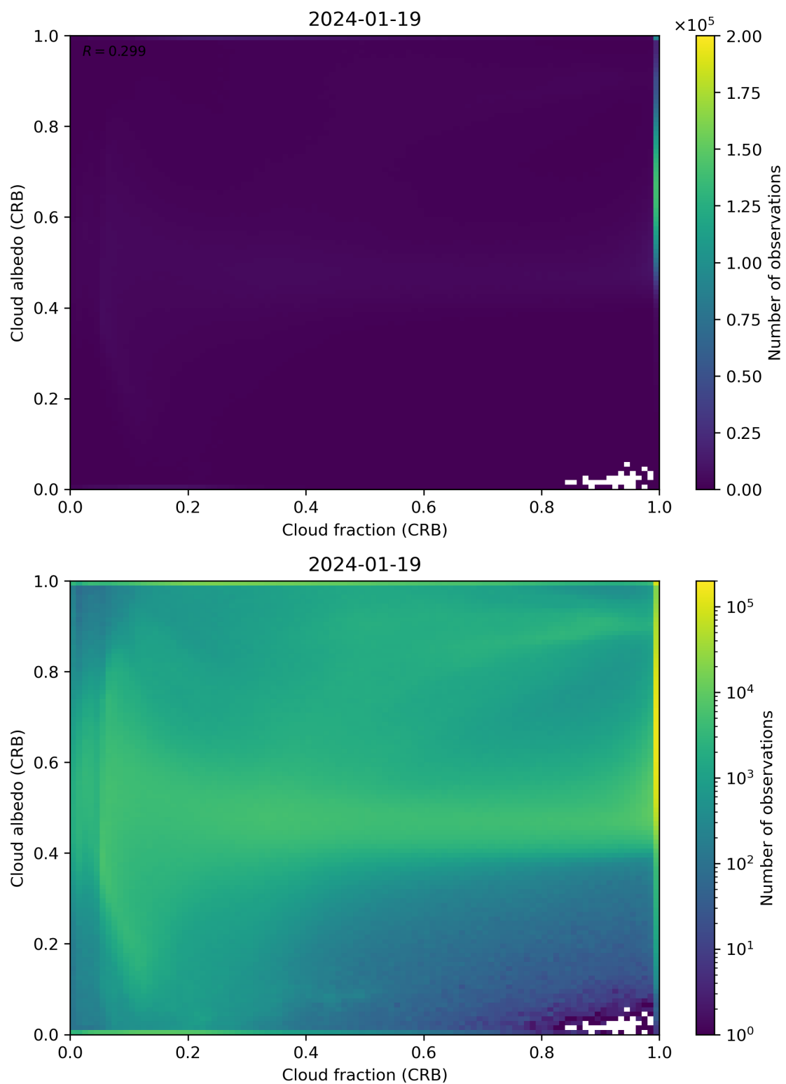
Figure 77: Scatter density plot of “Cloud fraction (CRB)” against “Cloud albedo (CRB)” for 2024-01-18 to 2024-01-20.
