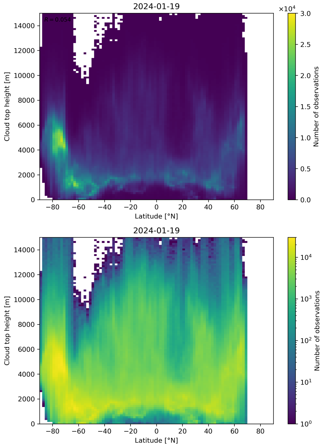
Figure 97: Scatter density plot of “Latitude” against “Cloud top height” for 2024-01-18 to 2024-01-20.
