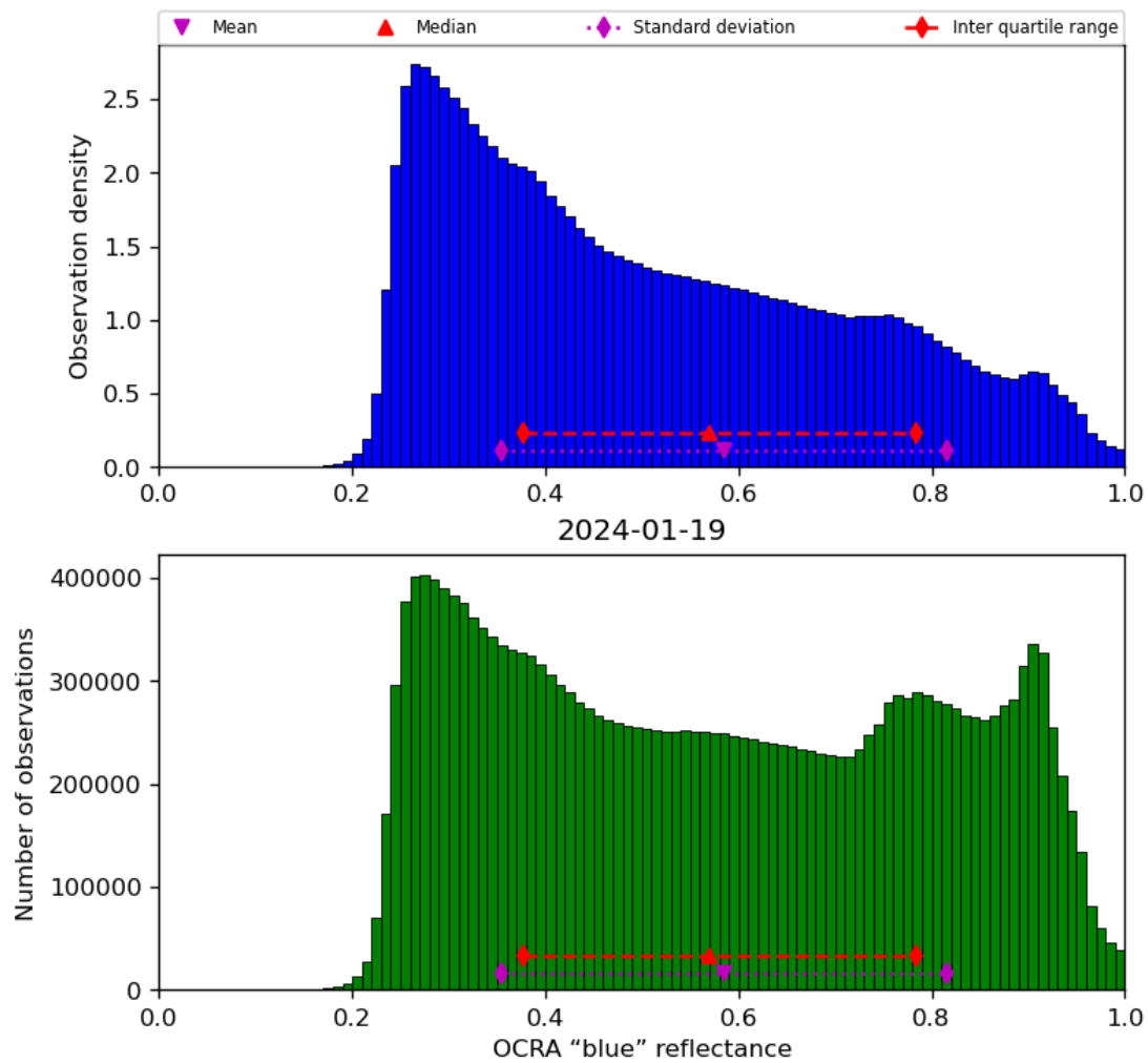
Figure 51: Histogram of “OCRA “blue” reflectance” for 2024-01-18 to 2024-01-20
