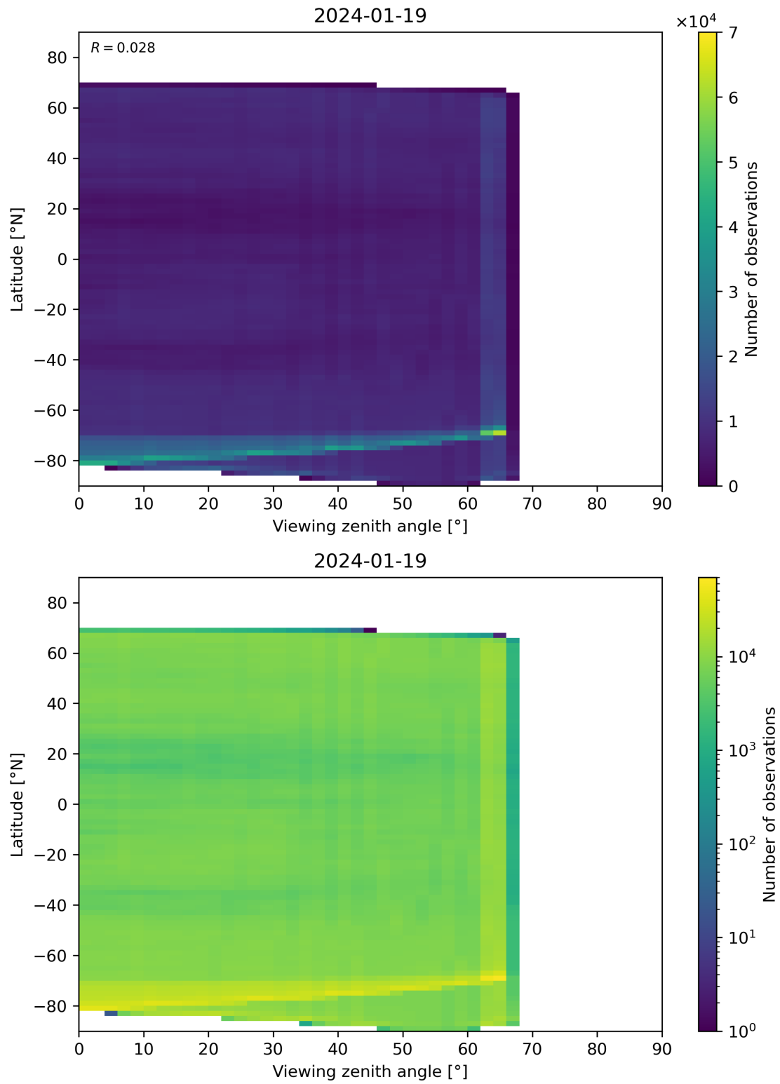
Figure 113: Scatter density plot of “Viewing zenith angle” against “Latitude” for 2024-01-18 to 2024-01-20.
