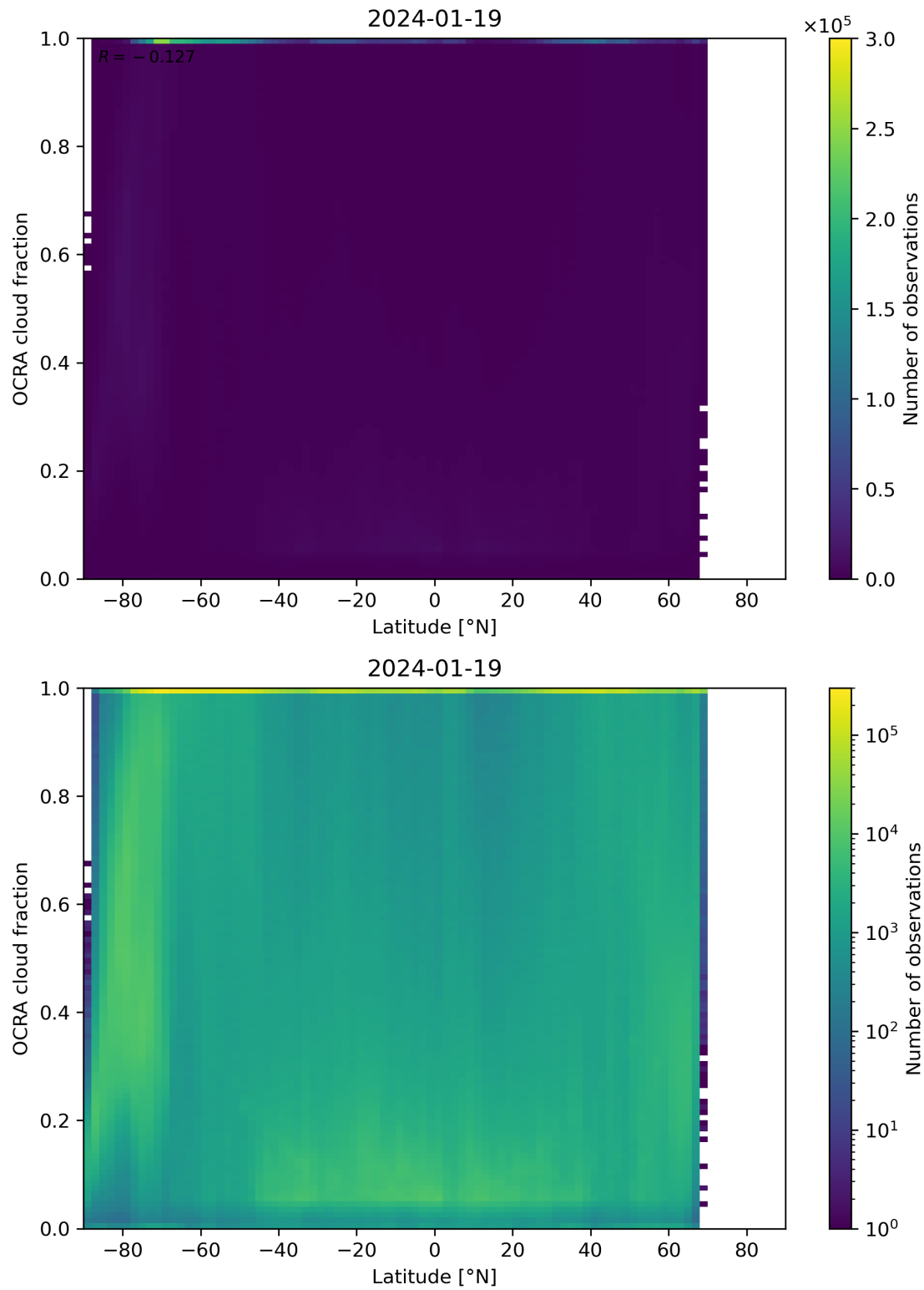
Figure 93: Scatter density plot of “Latitude” against “OCRA cloud fraction” for 2024-01-18 to 2024-01-20.
