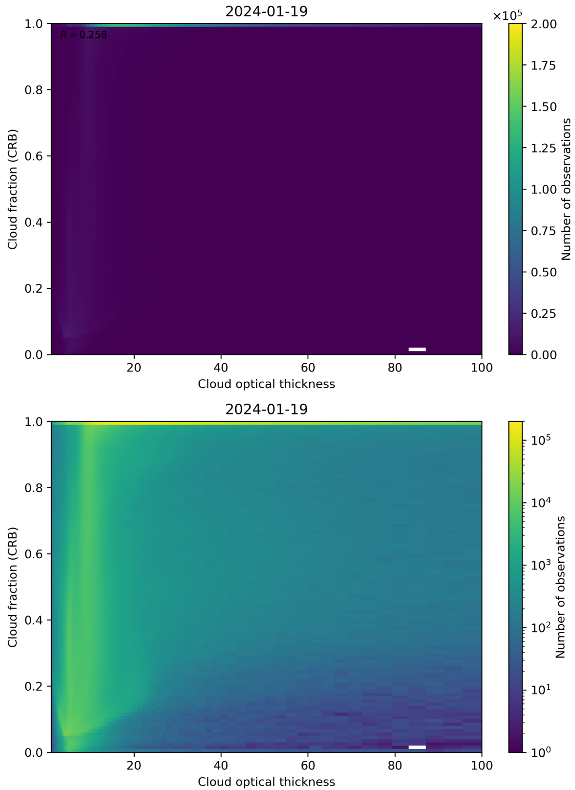
Figure 84: Scatter density plot of “Cloud optical thickness” against “Cloud fraction (CRB)” for 2024-01-18 to 2024-01-20.
