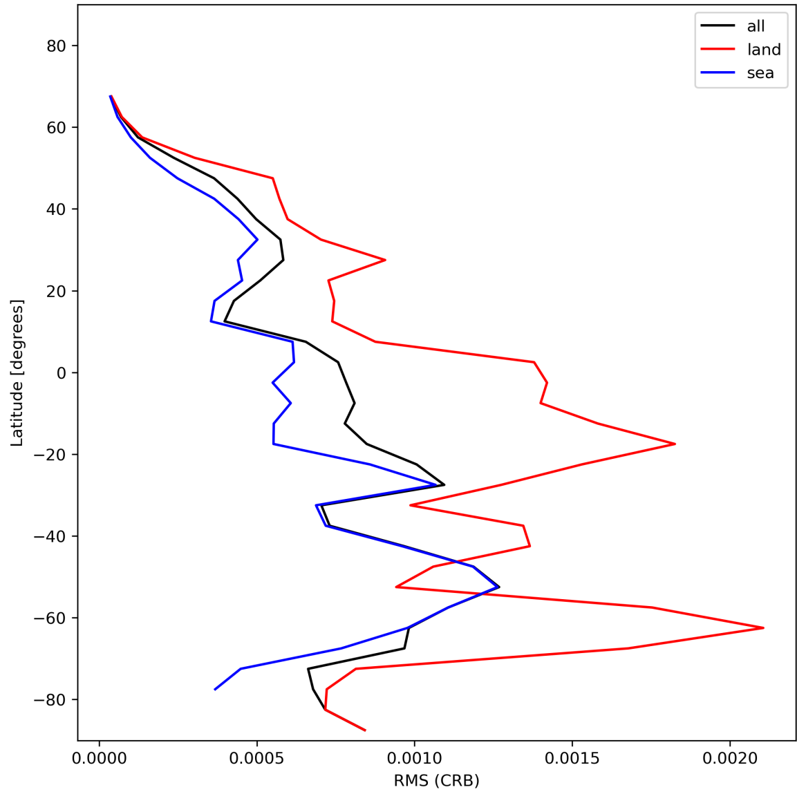
Figure 32: Zonal average of “RMS (CRB)” for 2024-01-18 to 2024-01-20.
