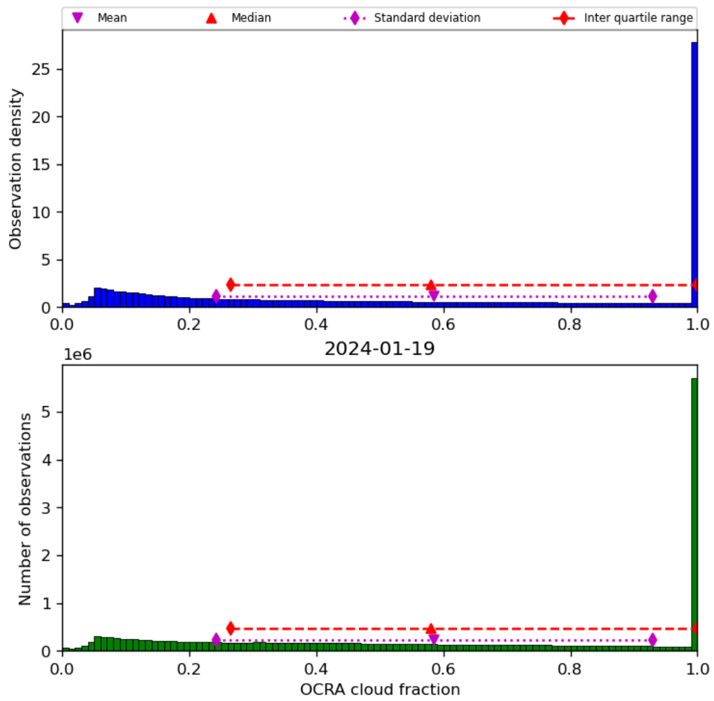
Figure 50: Histogram of “OCRA cloud fraction” for 2024-01-18 to 2024-01-20
