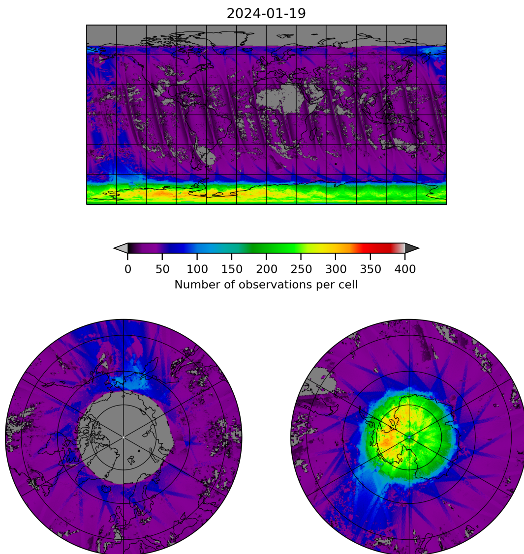
Figure 21: Map of the number of observations for 2024-01-18 to 2024-01-20
