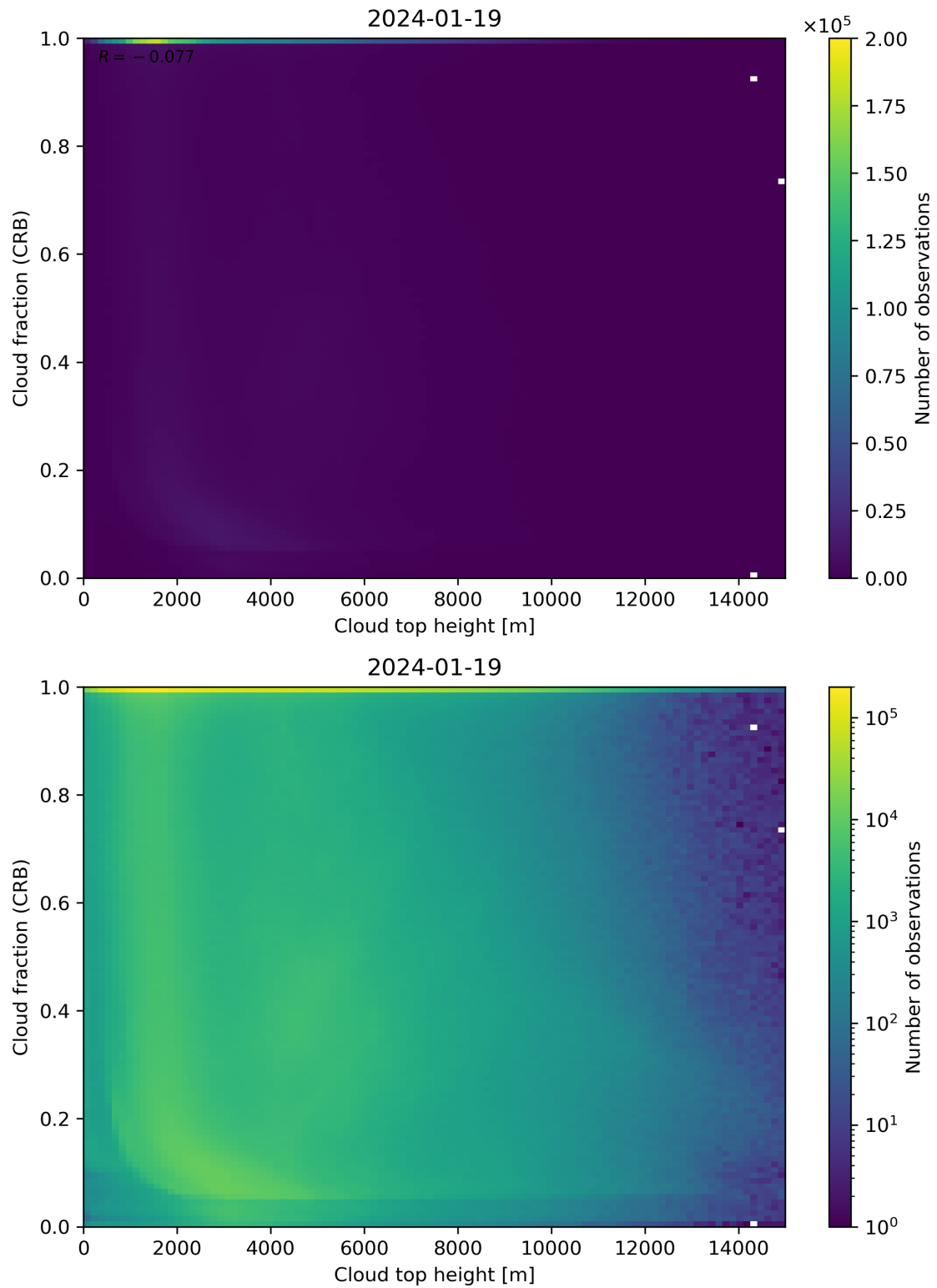
Figure 88: Scatter density plot of “Cloud top height” against “Cloud fraction (CRB)” for 2024-01-18 to 2024-01-20.
