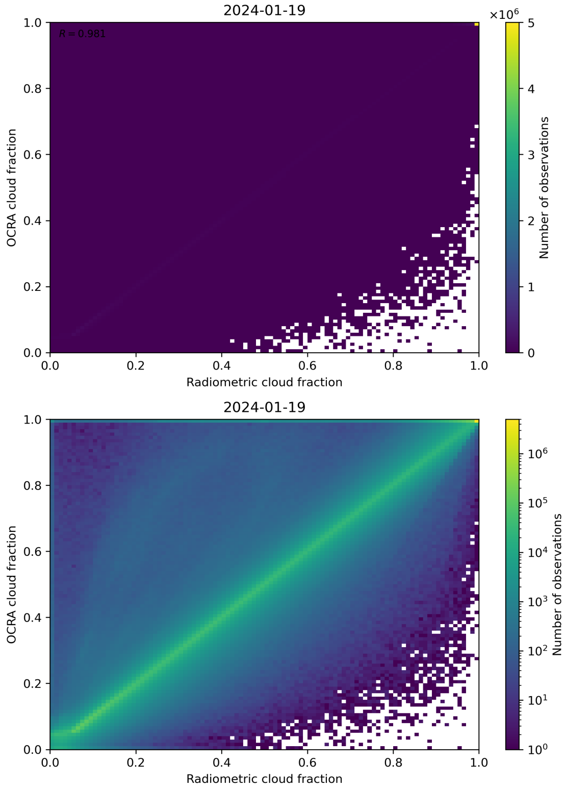
Figure 72: Scatter density plot of “Radiometric cloud fraction” against “OCRA cloud fraction” for 2024-01-18 to 2024-01-20.
