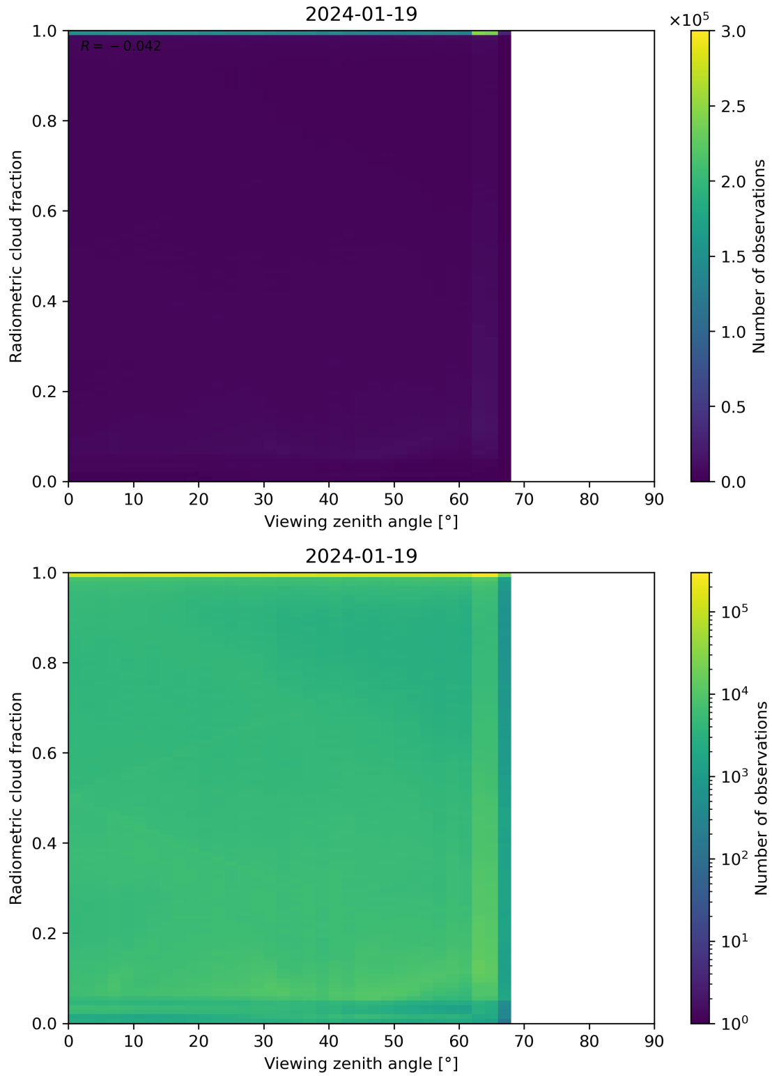
Figure 107: Scatter density plot of “Viewing zenith angle” against “Radiometric cloud fraction” for 2024-01-18 to 2024-01-20.
