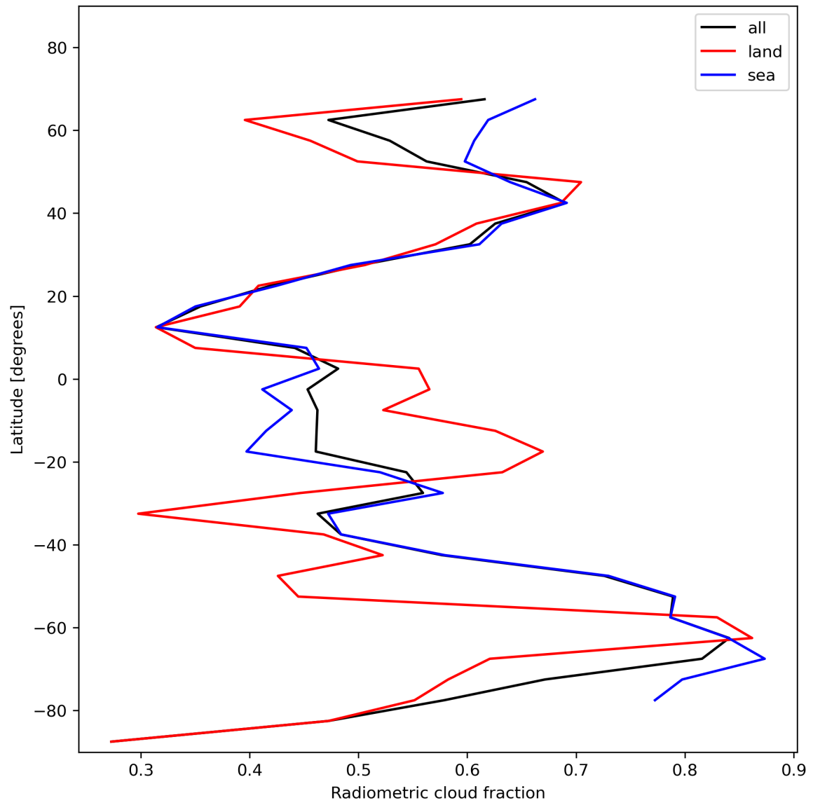
Figure 23: Zonal average of “Radiometric cloud fraction” for 2024-01-18 to 2024-01-20.
