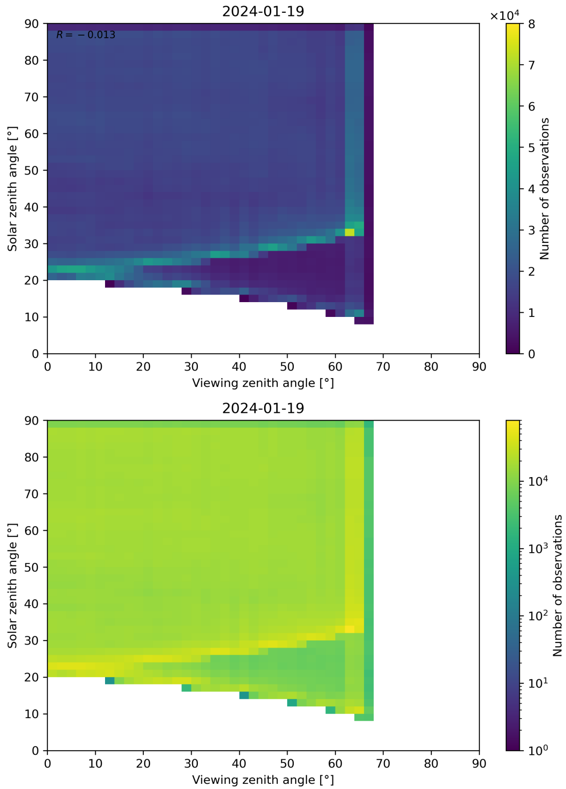
Figure 114: Scatter density plot of “Viewing zenith angle” against “Solar zenith angle” for 2024-01-18 to 2024-01-20.
