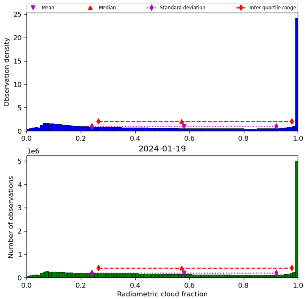
Figure 39: Histogram of “Radiometric cloud fraction” for 2024-01-18 to 2024-01-20
