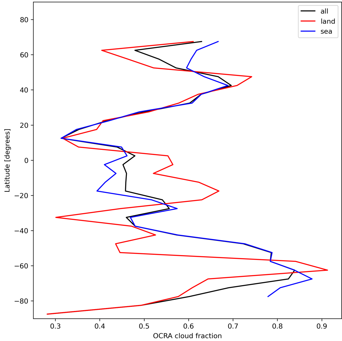
Figure 34: Zonal average of “OCRA cloud fraction” for 2024-01-18 to 2024-01-20.
