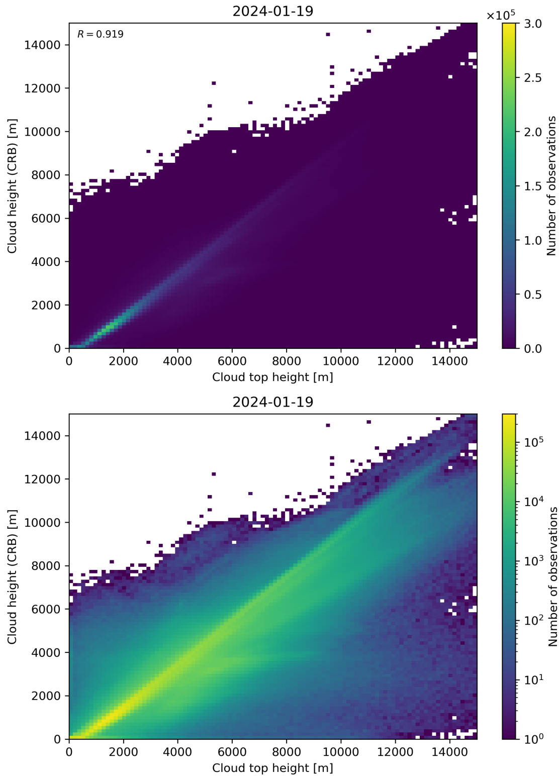
Figure 89: Scatter density plot of “Cloud top height” against “Cloud height (CRB)” for 2024-01-18 to 2024-01-20.
