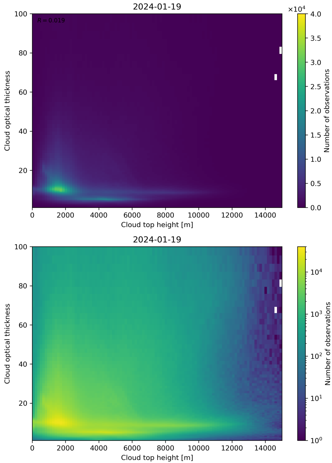
Figure 90: Scatter density plot of “Cloud top height” against “Cloud optical thickness” for 2024-01-18 to 2024-01-20.
