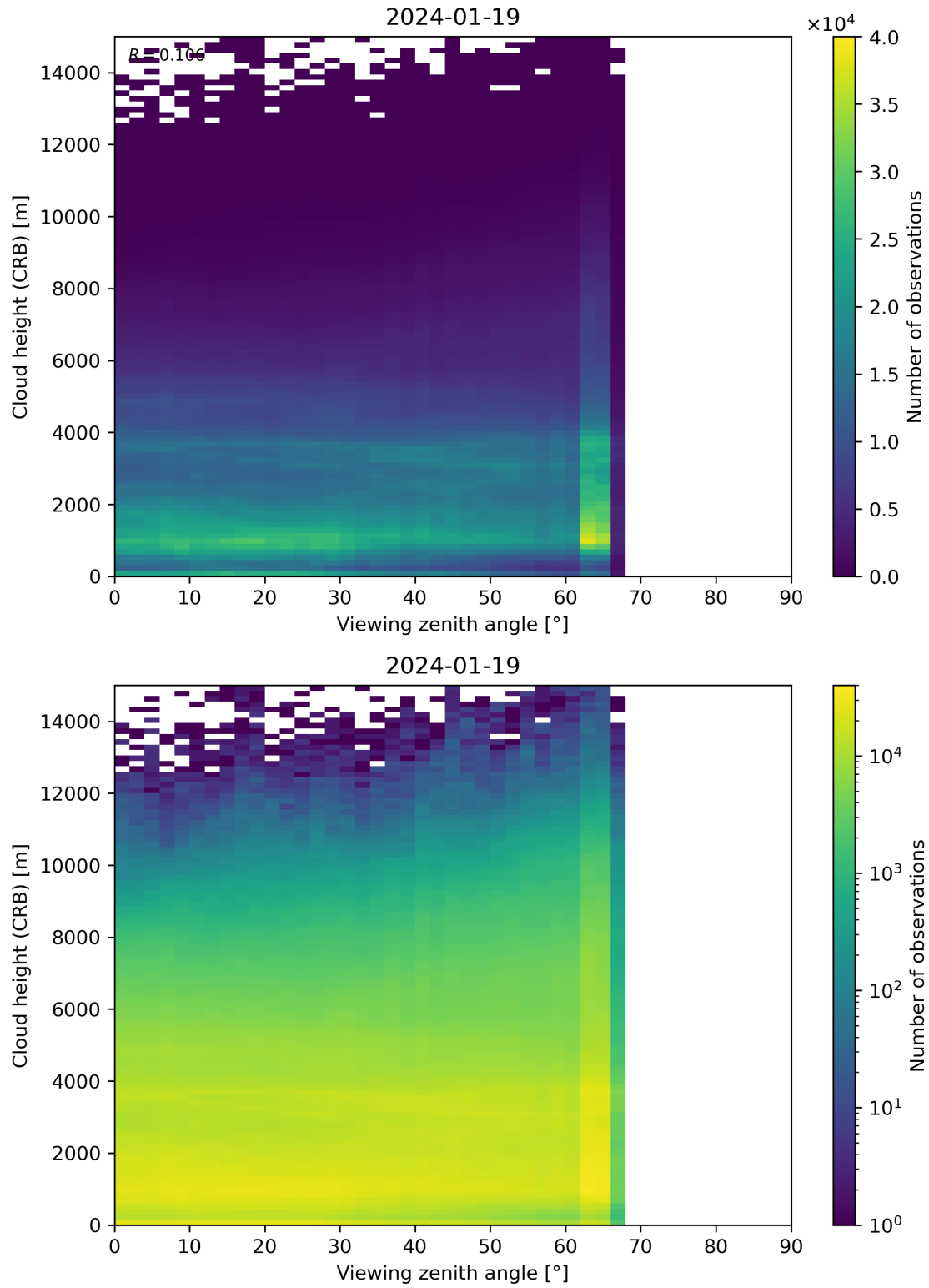
Figure 110: Scatter density plot of “Viewing zenith angle” against “Cloud height (CRB)” for 2024-01-18 to 2024-01-20.
