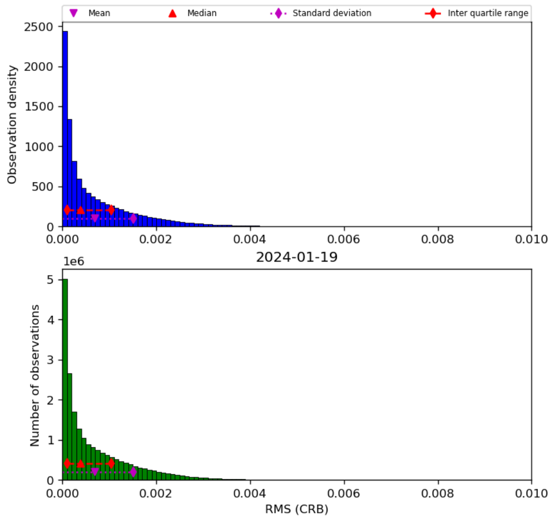
Figure 48: Histogram of “RMS (CRB)” for 2024-01-18 to 2024-01-20
