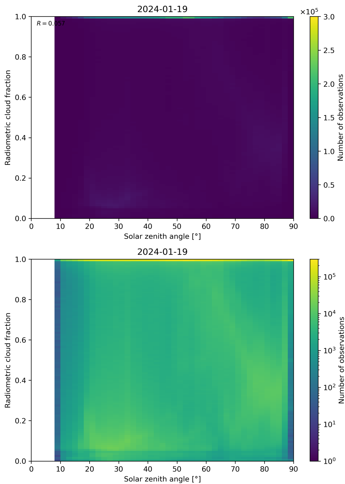
Figure 99: Scatter density plot of “Solar zenith angle” against “Radiometric cloud fraction” for 2024-01-18 to 2024-01-20.
