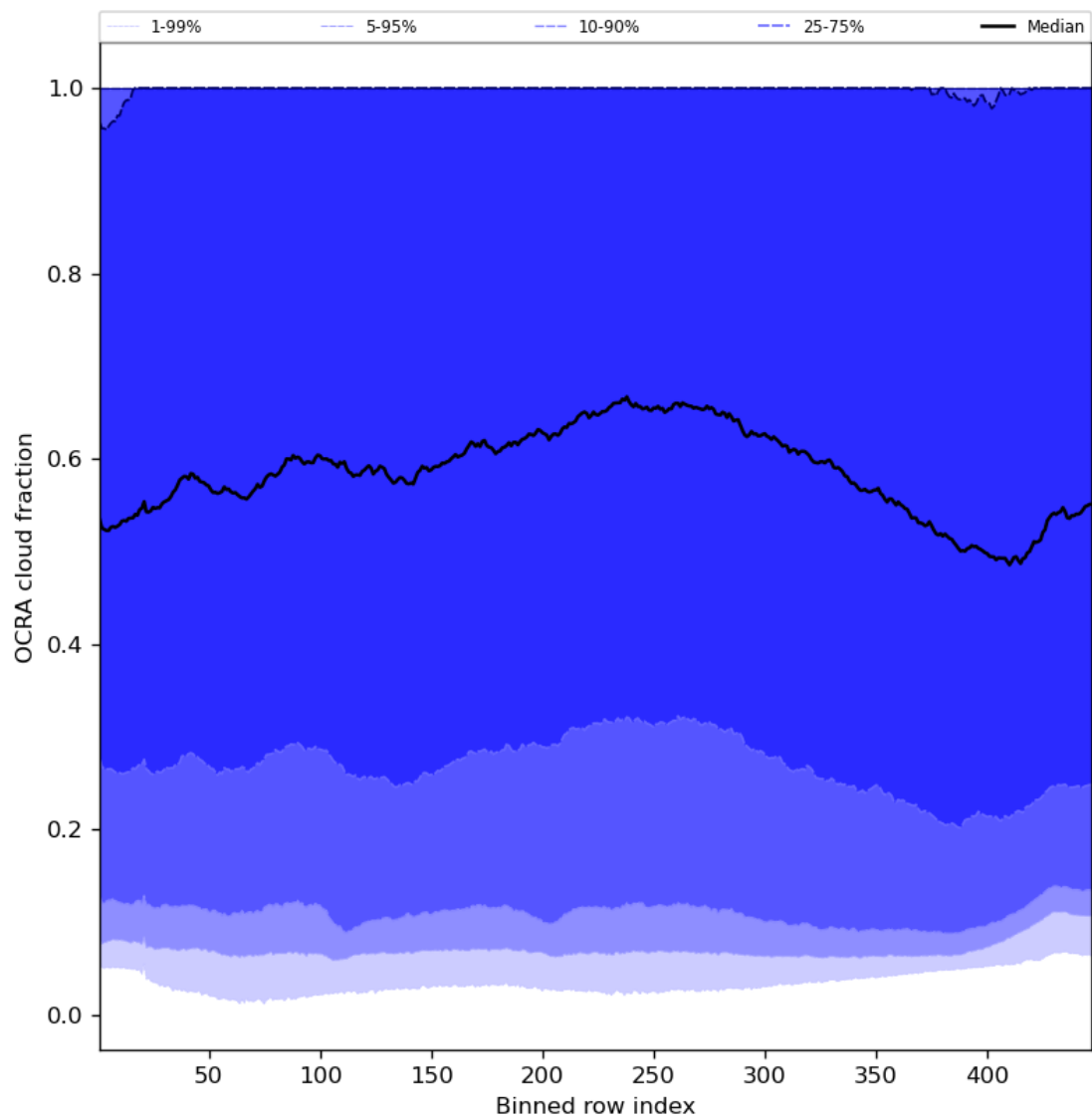
Figure 66: Along track statistics of “OCRA cloud fraction” for 2024-01-18 to 2024-01-20
