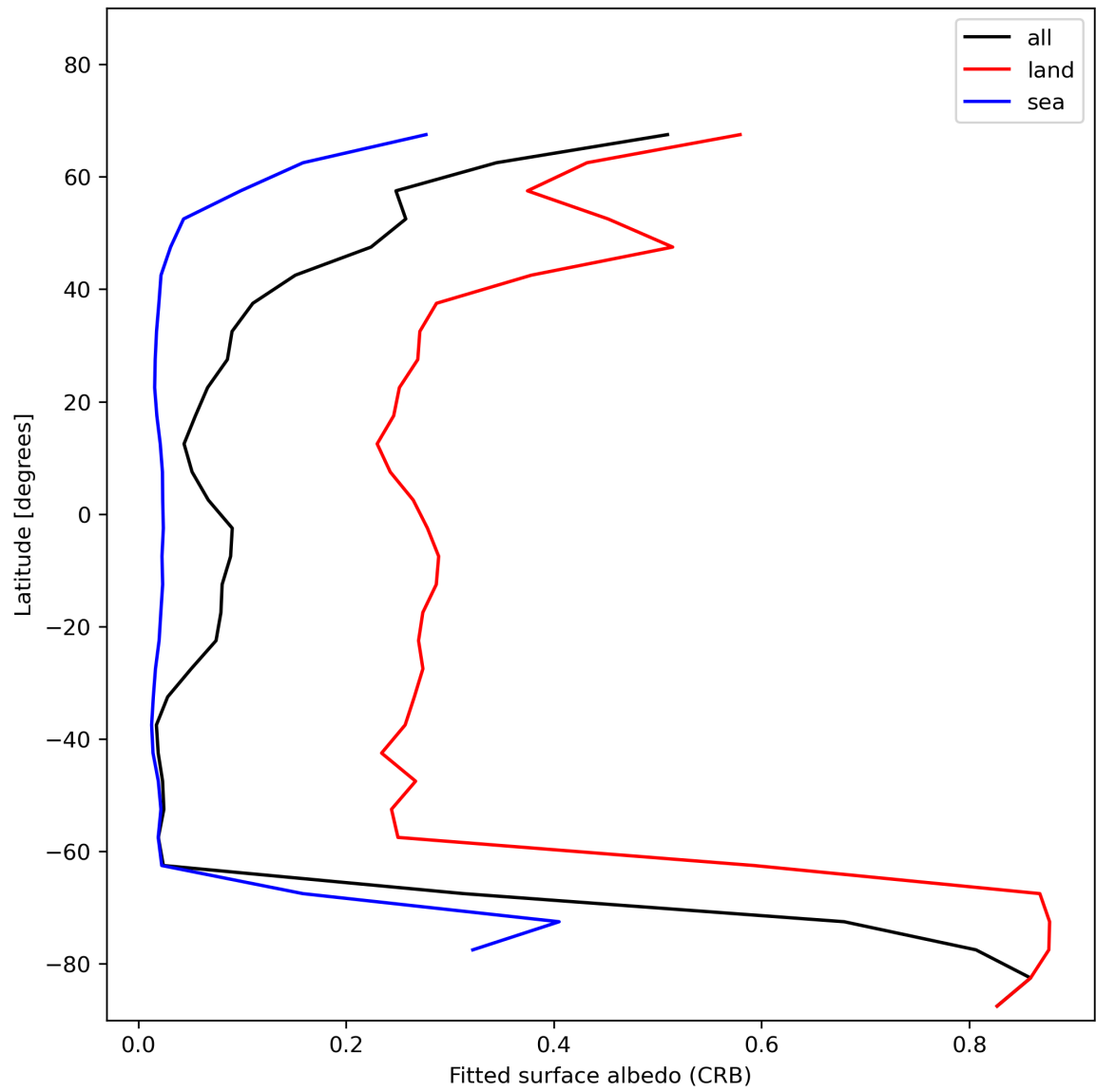
Figure 30: Zonal average of “Fitted surface albedo (CRB)” for 2024-01-18 to 2024-01-20.
