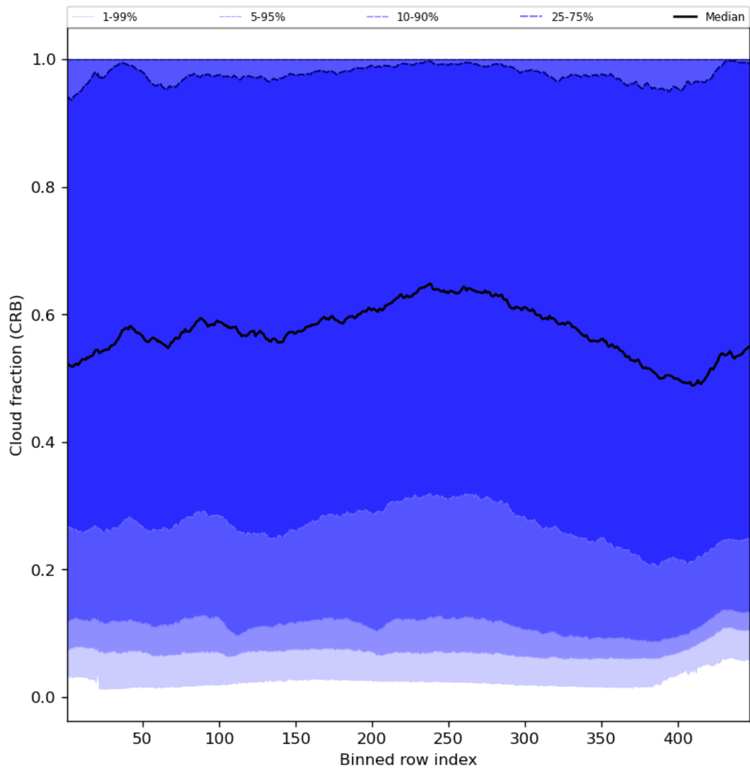
Figure 58: Along track statistics of “Cloud fraction (CRB)” for 2024-01-18 to 2024-01-20
