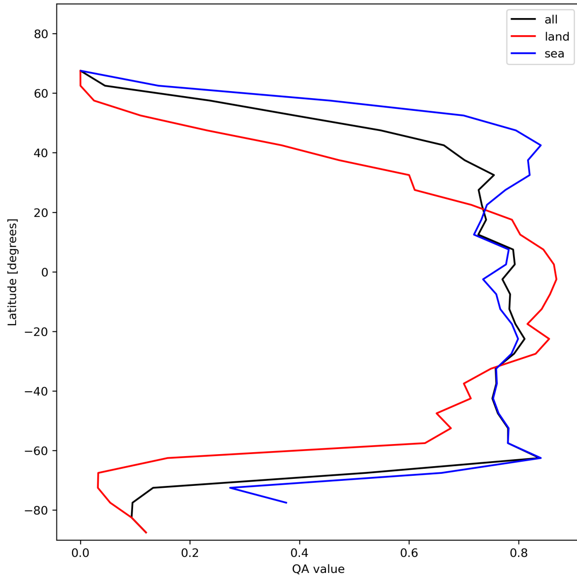
Figure 22: Zonal average of “QA value” for 2024-01-18 to 2024-01-20.
