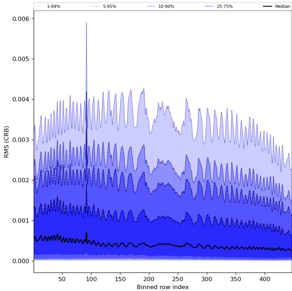
Figure 64: Along track statistics of “RMS (CRB)” for 2024-01-18 to 2024-01-20
