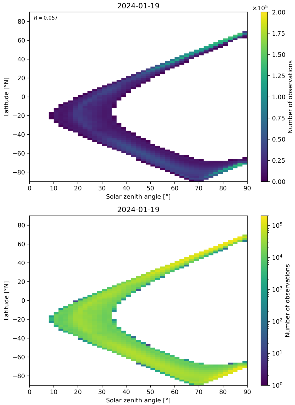
Figure 105: Scatter density plot of “Solar zenith angle” against “Latitude” for 2024-01-18 to 2024-01-20.
