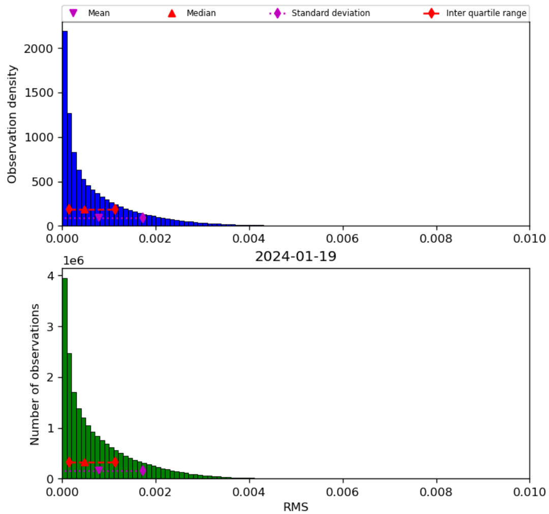
Figure 47: Histogram of “RMS” for 2024-01-18 to 2024-01-20
