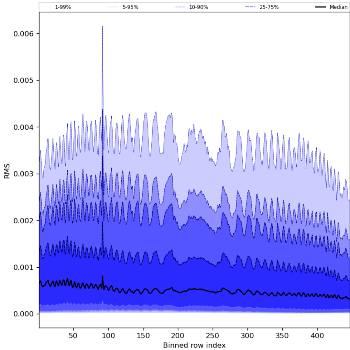
Figure 63: Along track statistics of “RMS” for 2024-01-18 to 2024-01-20
