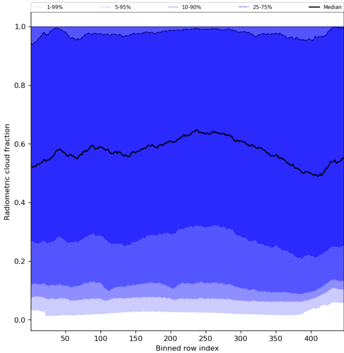
Figure 55: Along track statistics of “Radiometric cloud fraction” for 2024-01-18 to 2024-01-20
