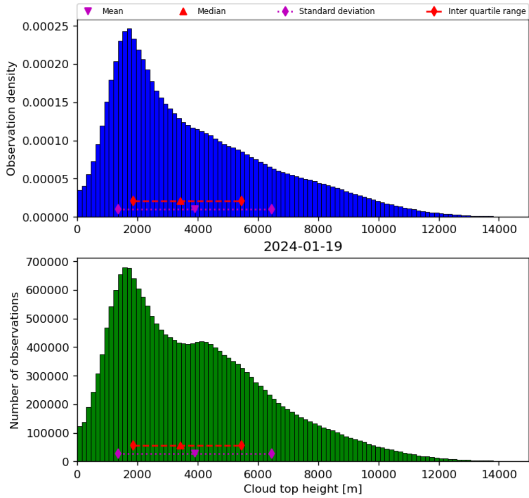
Figure 40: Histogram of “Cloud top height” for 2024-01-18 to 2024-01-20
