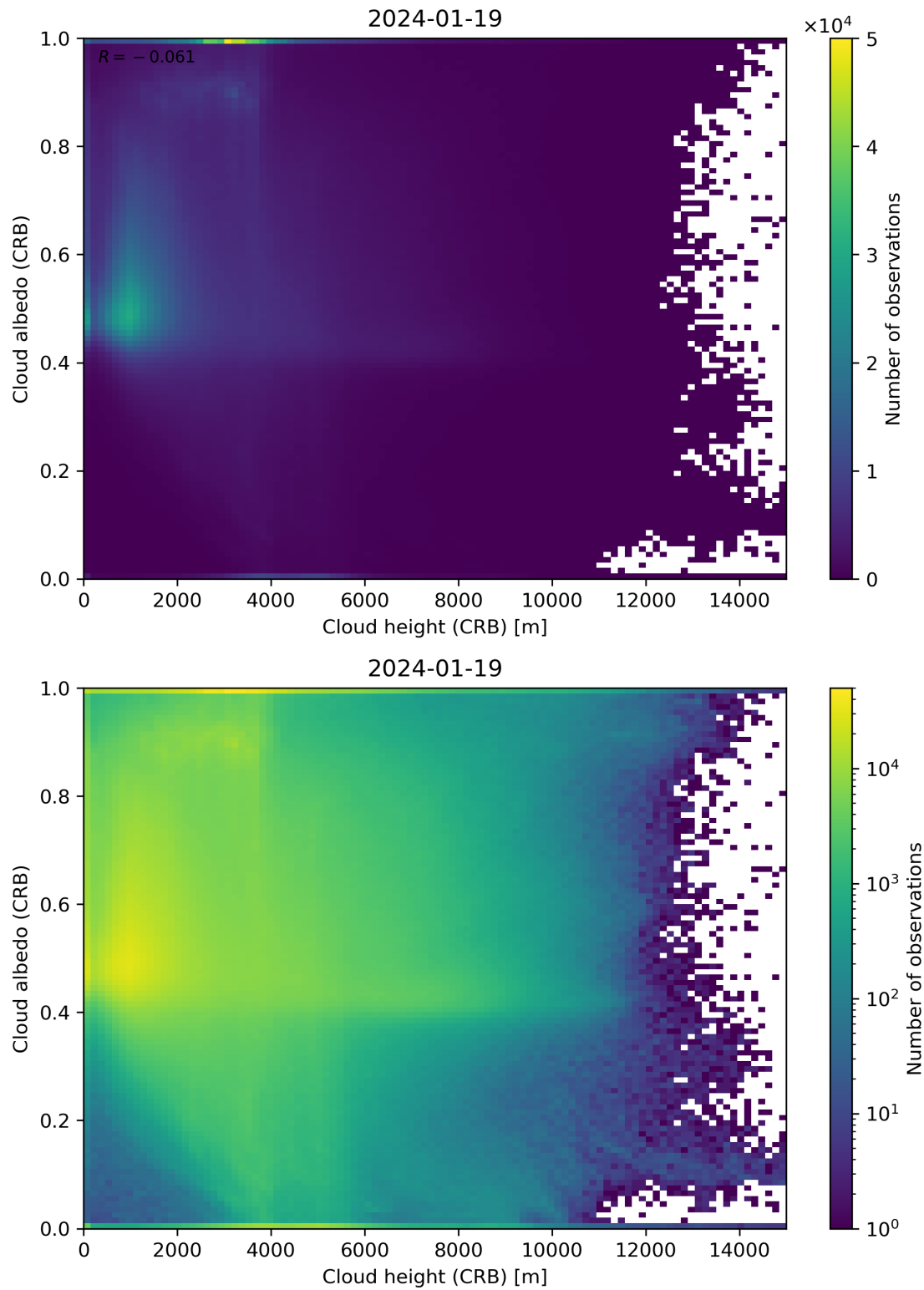
Figure 80: Scatter density plot of “Cloud height (CRB)” against “Cloud albedo (CRB)” for 2024-01-18 to 2024-01-20.
