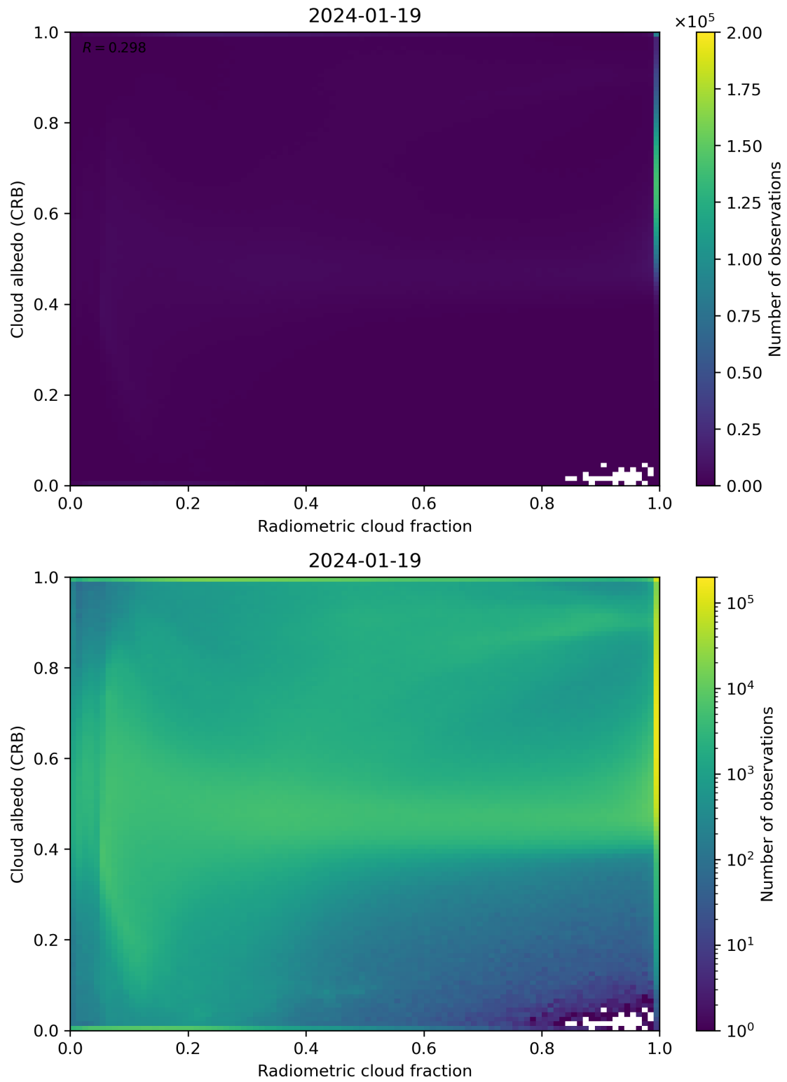
Figure 71: Scatter density plot of “Radiometric cloud fraction” against “Cloud albedo (CRB)” for 2024-01-18 to 2024-01-20.
