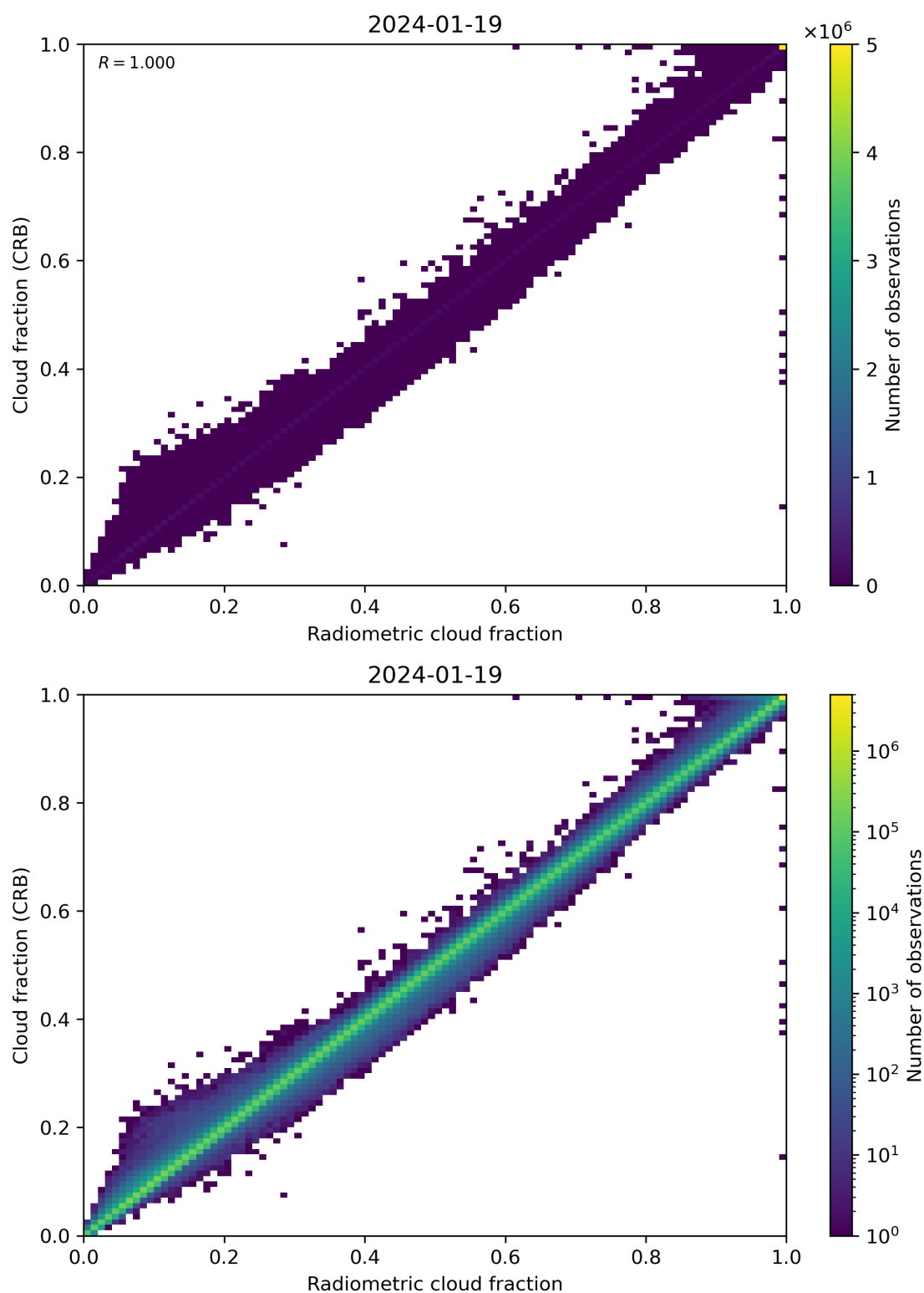
Figure 73: Scatter density plot of “Radiometric cloud fraction” against “Cloud fraction (CRB)” for 2024-01-18 to 2024-01-20.
