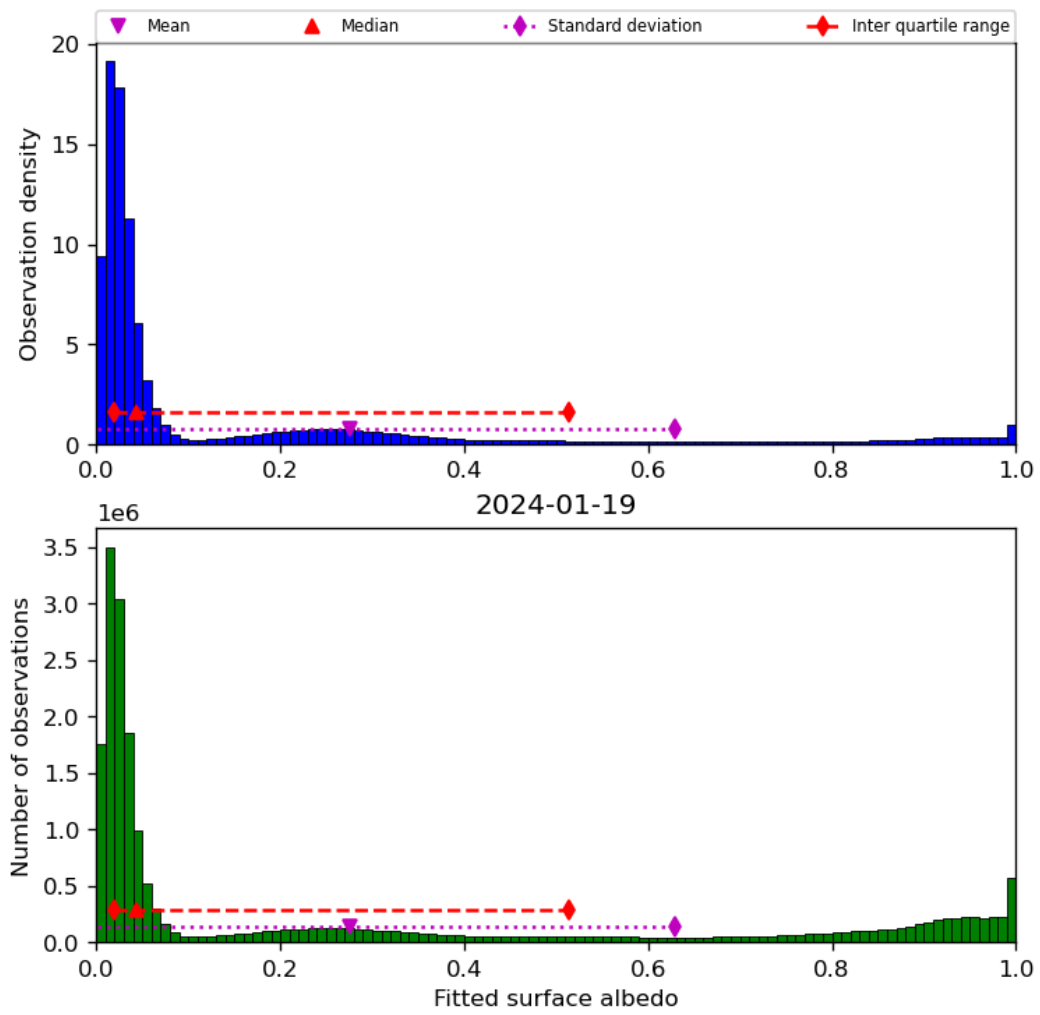
Figure 45: Histogram of “Fitted surface albedo” for 2024-01-18 to 2024-01-20
