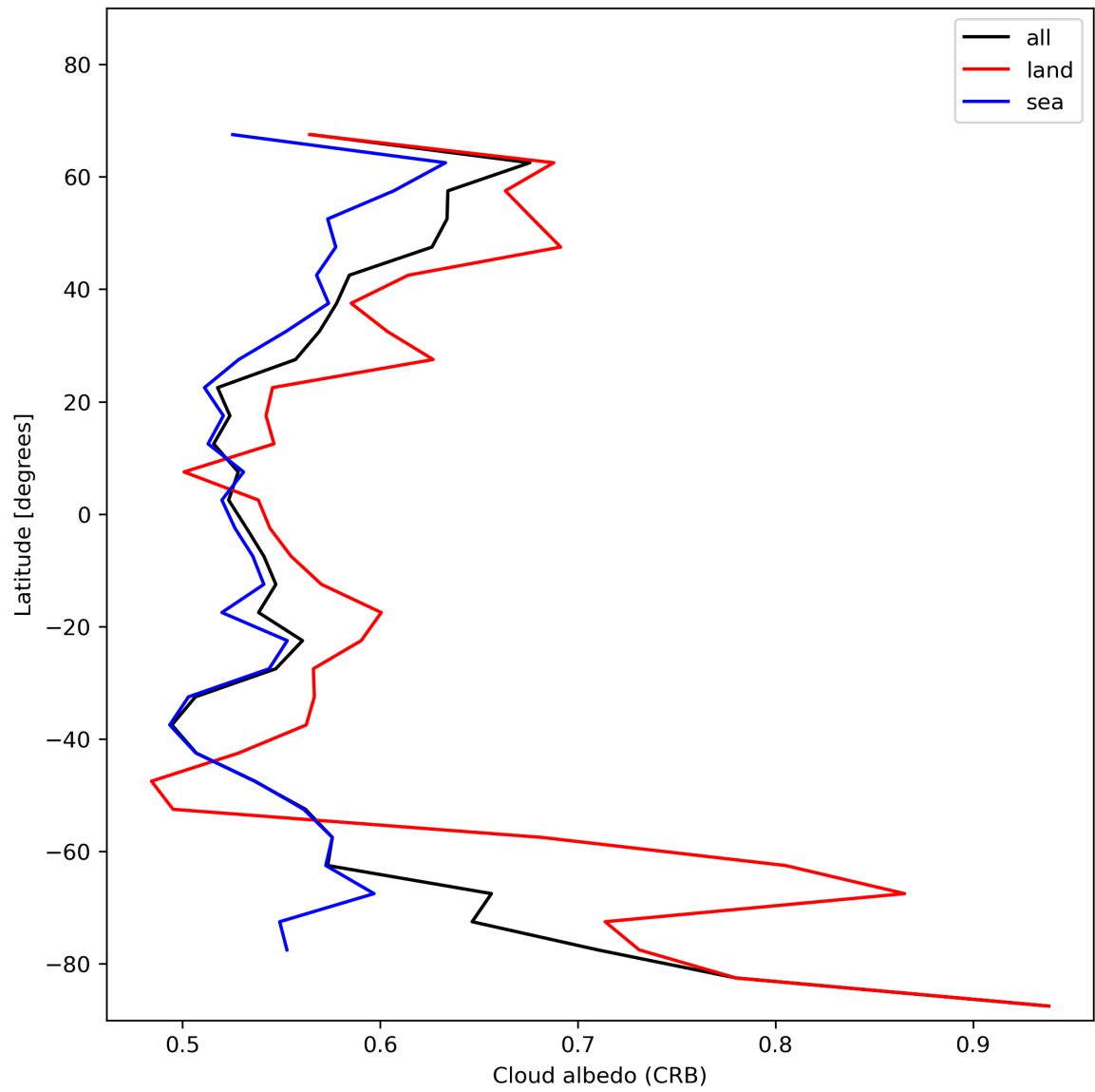
Figure 28: Zonal average of “Cloud albedo (CRB)” for 2024-01-18 to 2024-01-20.
