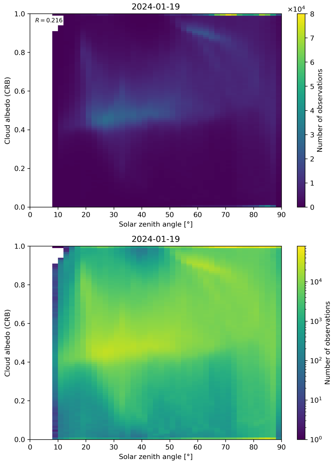
Figure 98: Scatter density plot of “Solar zenith angle” against “Cloud albedo (CRB)” for 2024-01-18 to 2024-01-20.
