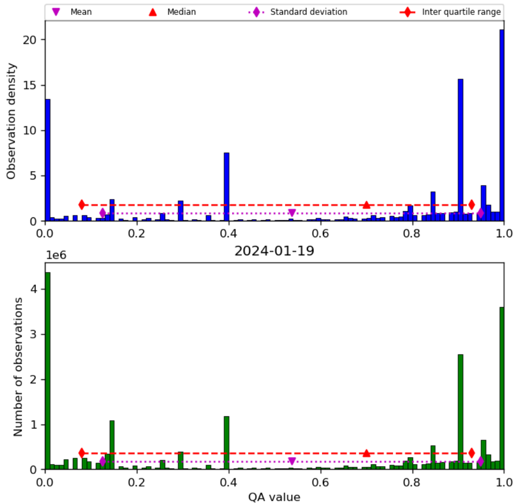
Figure 38: Histogram of “QA value” for 2024-01-18 to 2024-01-20
