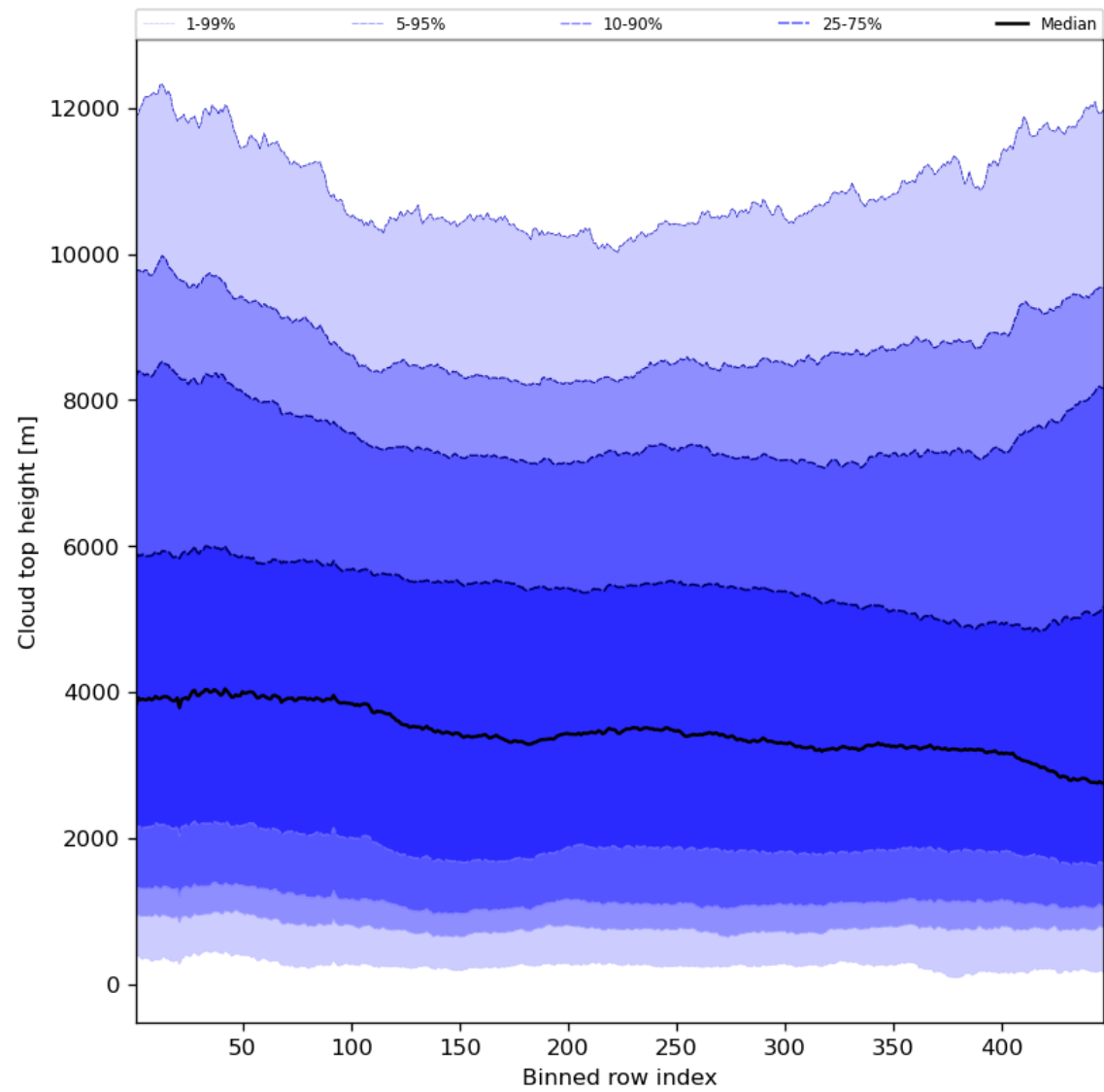
Figure 56: Along track statistics of “Cloud top height” for 2024-01-18 to 2024-01-20
