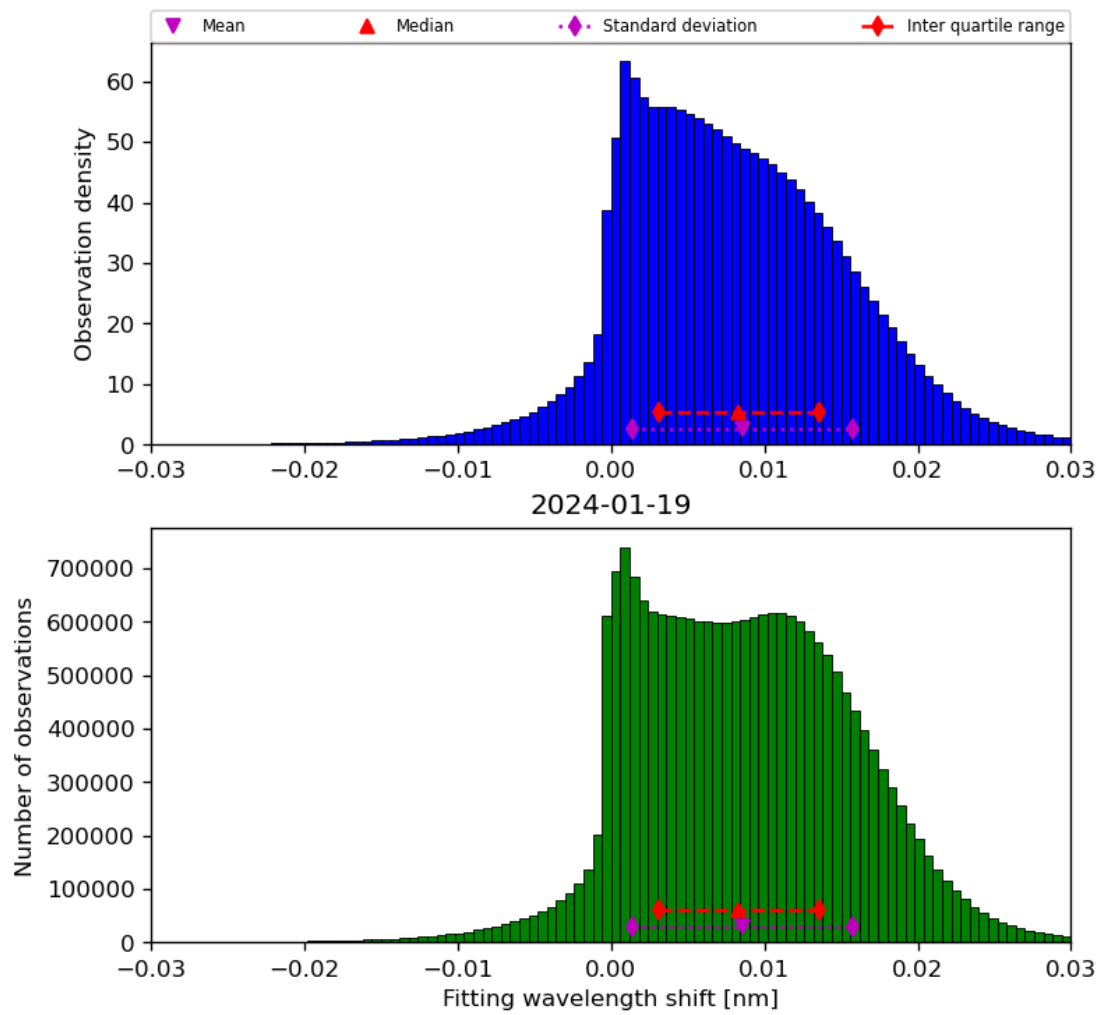
Figure 49: Histogram of “Fitting wavelength shift” for 2024-01-18 to 2024-01-20
