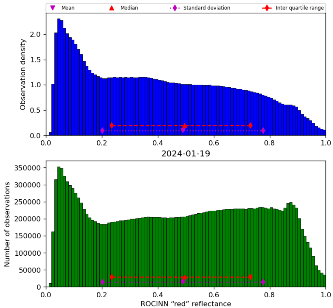
Figure 53: Histogram of “ROCINN “red” reflectance” for 2024-01-18 to 2024-01-20
