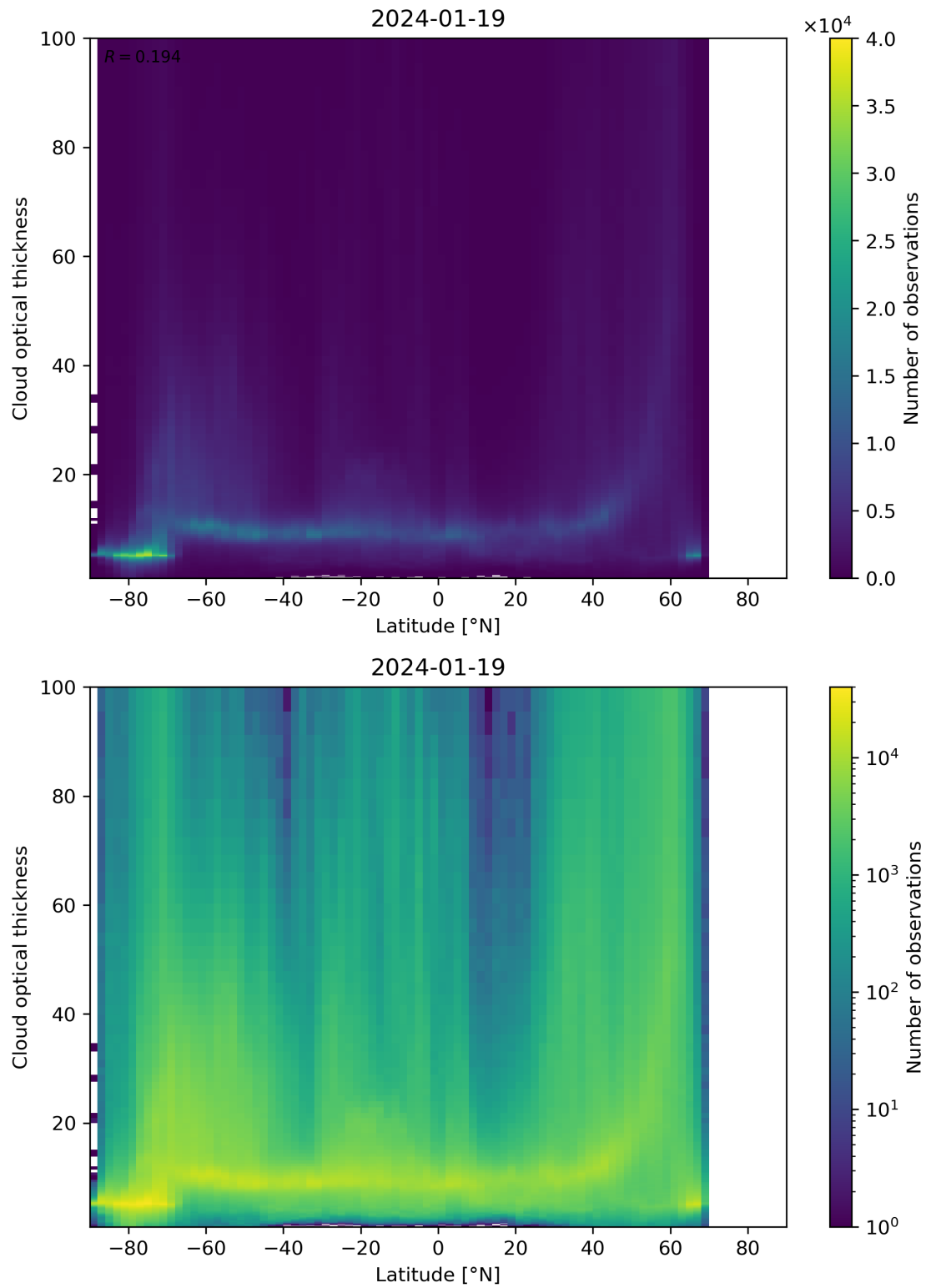
Figure 96: Scatter density plot of “Latitude” against “Cloud optical thickness” for 2024-01-18 to 2024-01-20.
