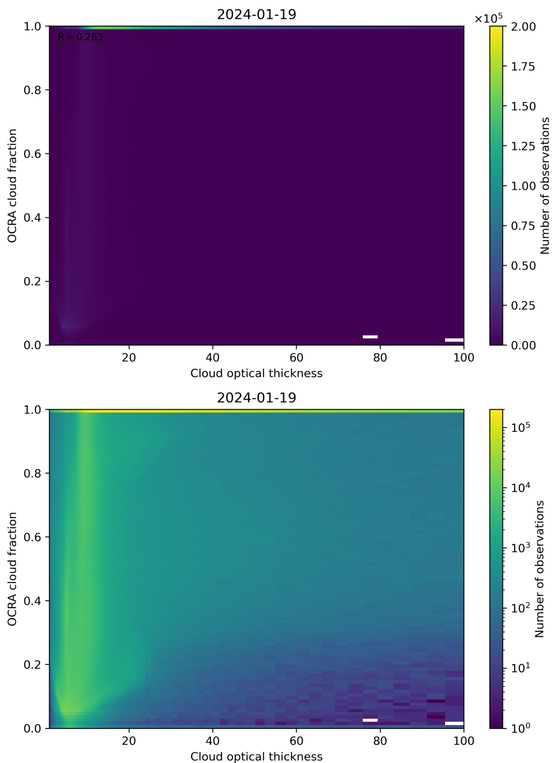
Figure 83: Scatter density plot of “Cloud optical thickness” against “OCRA cloud fraction” for 2024-01-18 to 2024-01-20.
