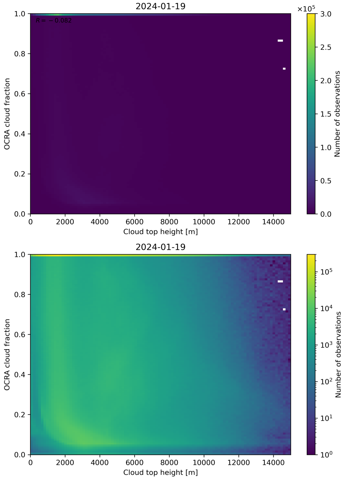
Figure 87: Scatter density plot of “Cloud top height” against “OCRA cloud fraction” for 2024-01-18 to 2024-01-20.
