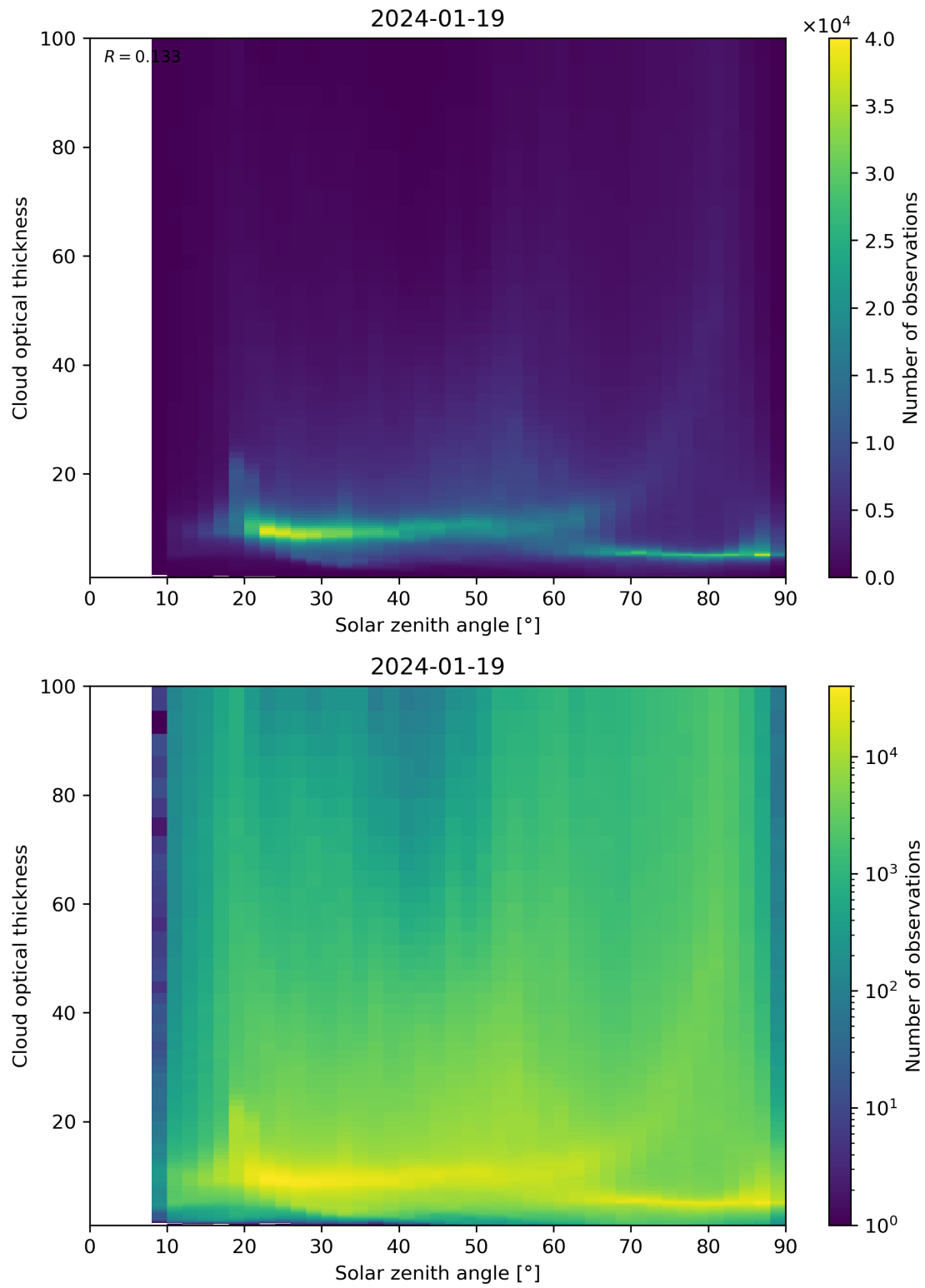
Figure 103: Scatter density plot of “Solar zenith angle” against “Cloud optical thickness” for 2024-01-18 to 2024-01-20.
