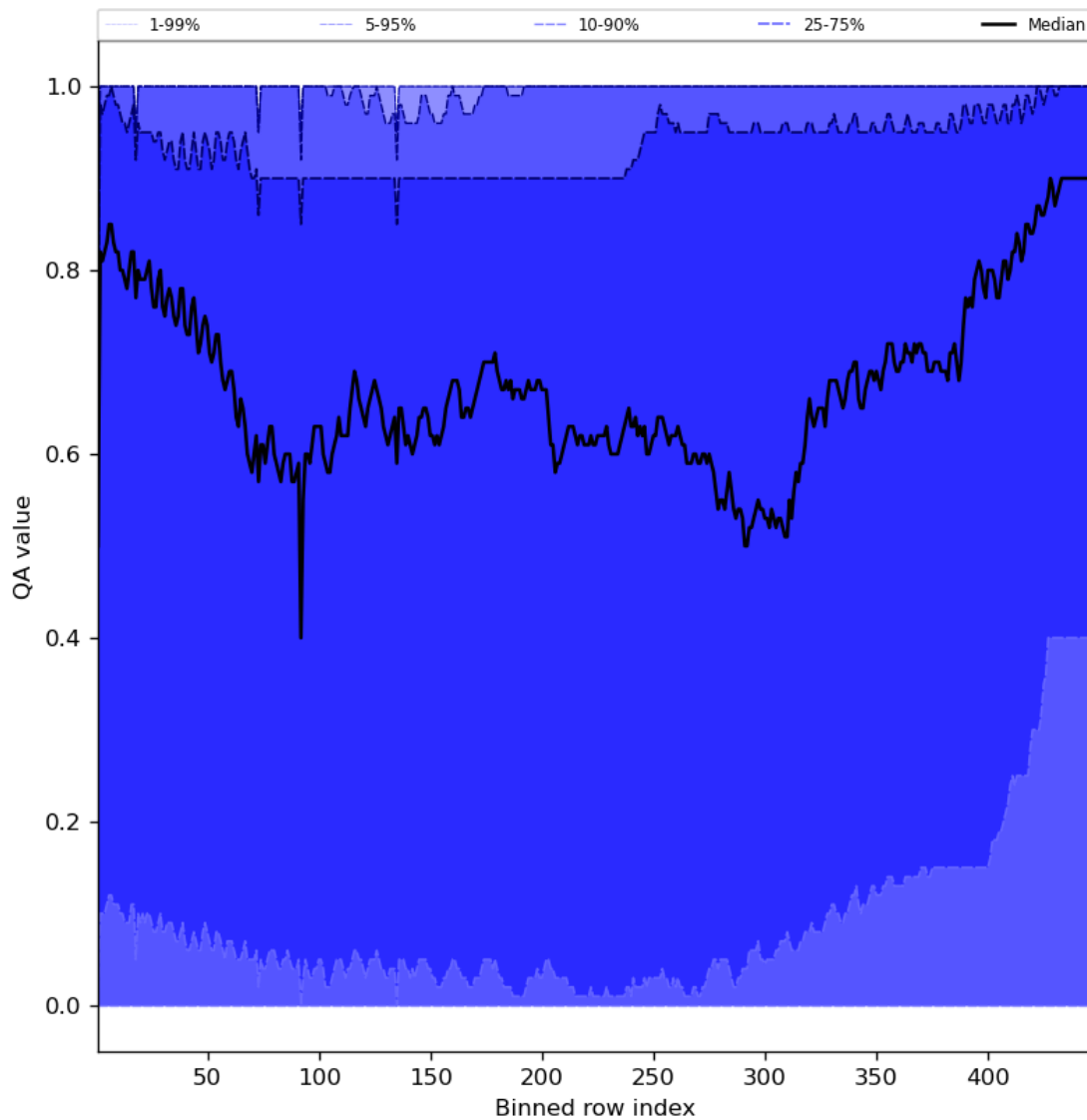
Figure 54: Along track statistics of “QA value” for 2024-01-18 to 2024-01-20
