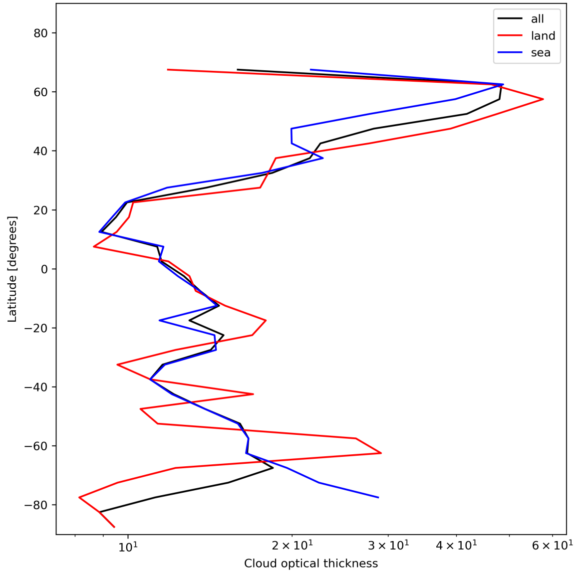
Figure 25: Zonal average of “Cloud optical thickness” for 2024-01-18 to 2024-01-20.
