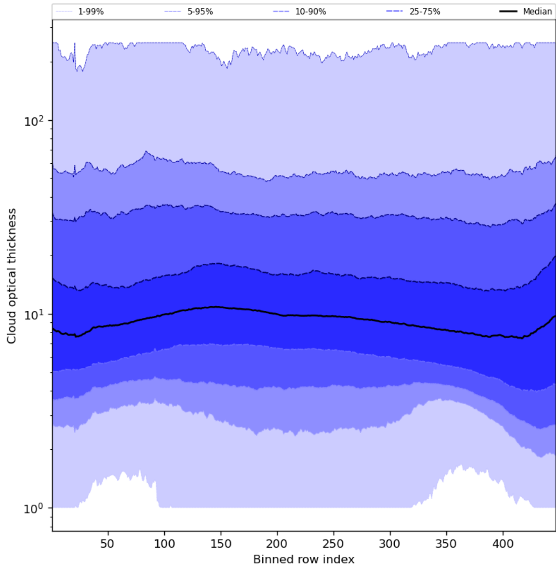
Figure 57: Along track statistics of “Cloud optical thickness” for 2024-01-18 to 2024-01-20
