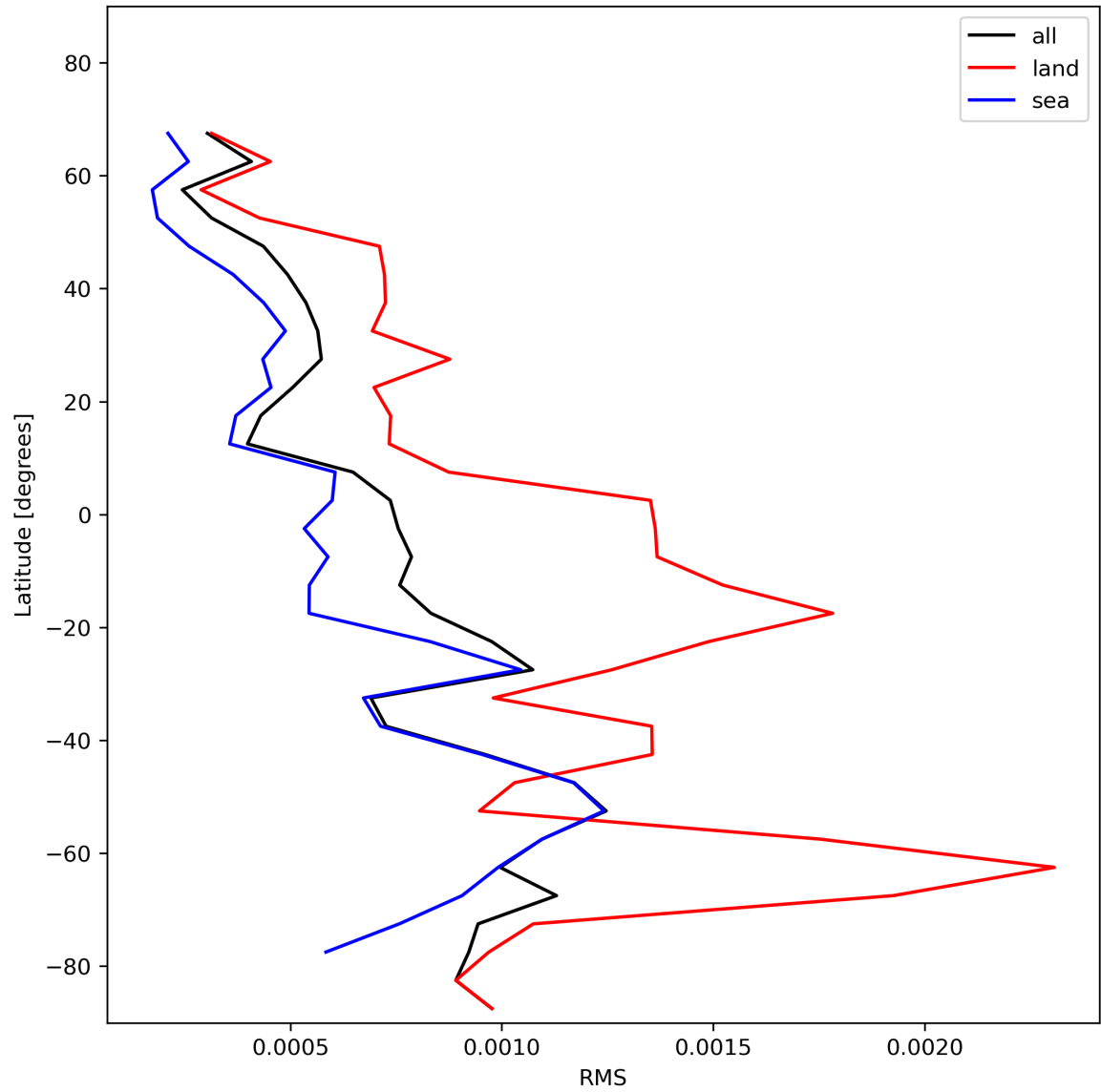
Figure 31: Zonal average of “RMS” for 2024-01-18 to 2024-01-20.
