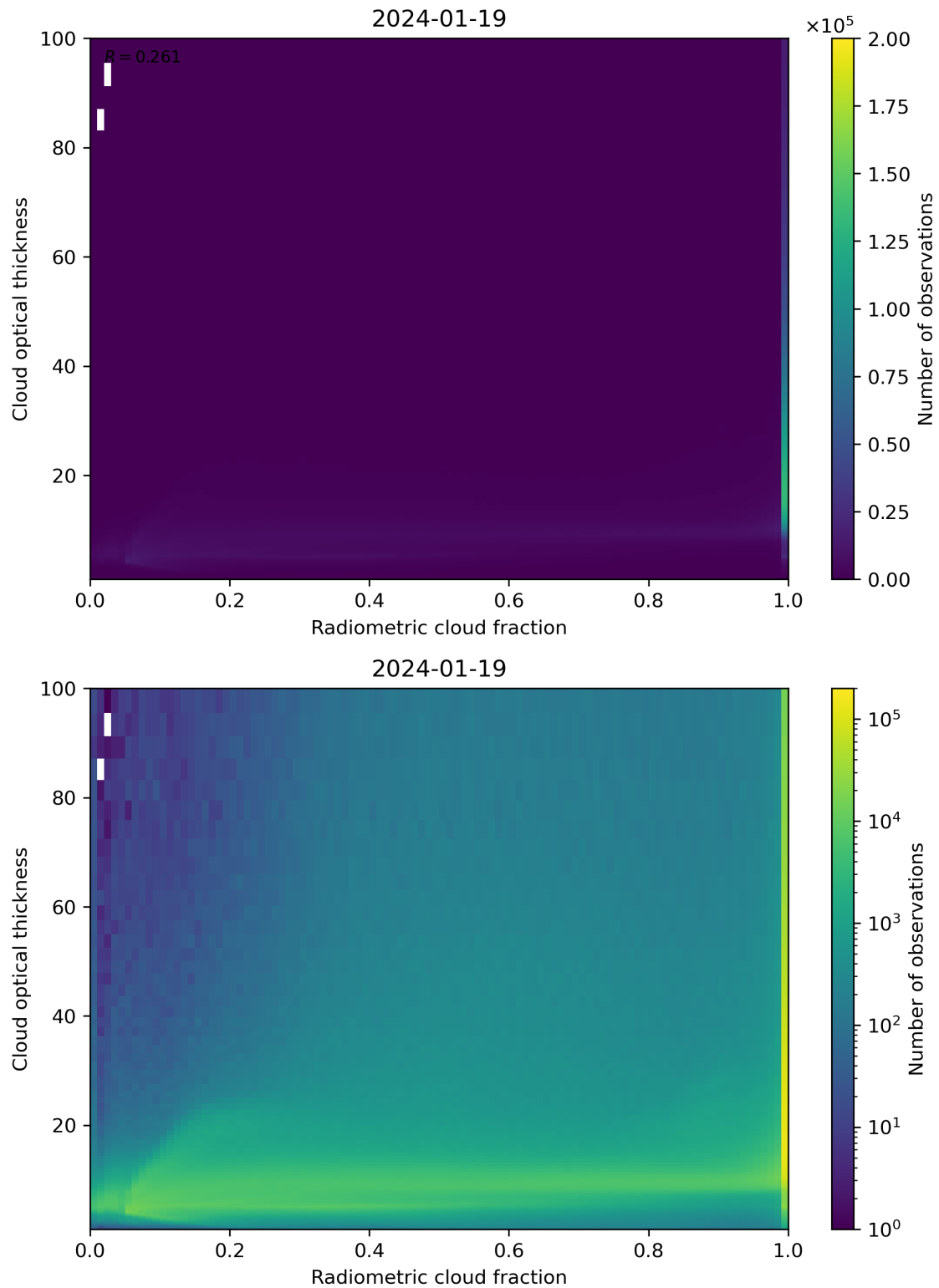
Figure 75: Scatter density plot of “Radiometric cloud fraction” against “Cloud optical thickness” for 2024-01-18 to 2024-01-20.
