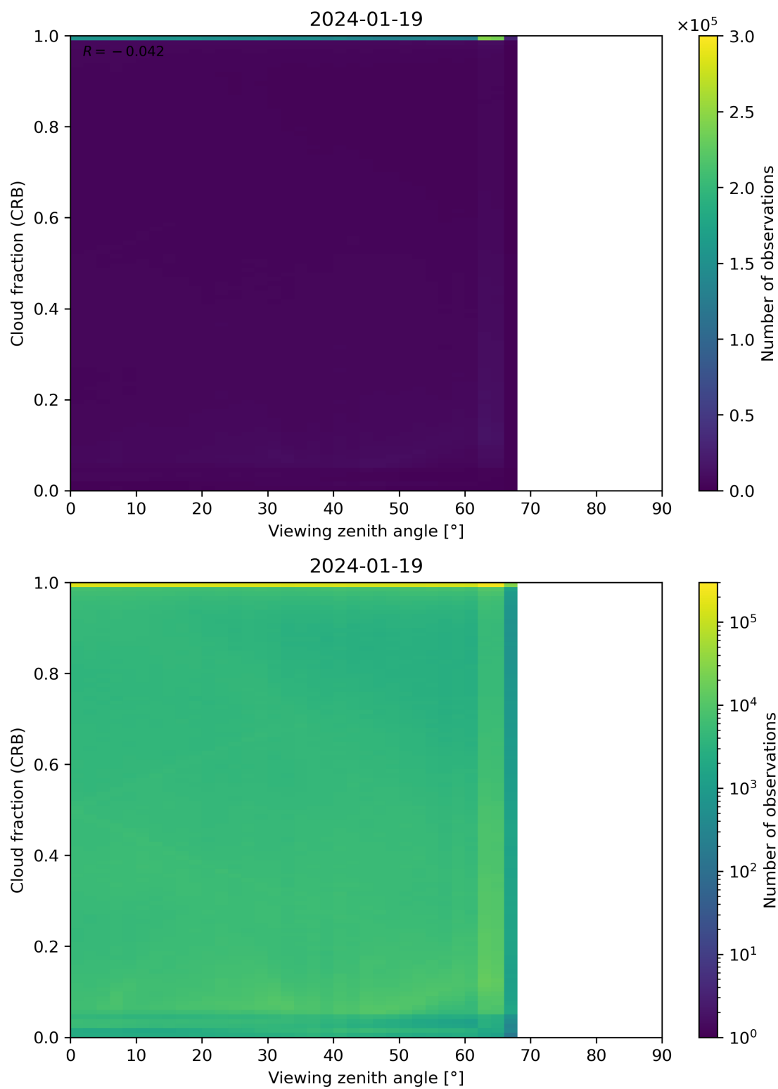
Figure 109: Scatter density plot of “Viewing zenith angle” against “Cloud fraction (CRB)” for 2024-01-18 to 2024-01-20.
