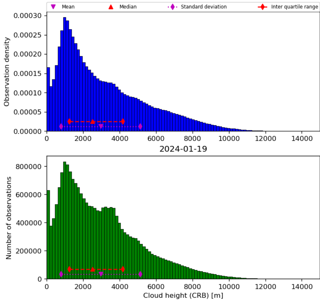
Figure 43: Histogram of “Cloud height (CRB)” for 2024-01-18 to 2024-01-20
