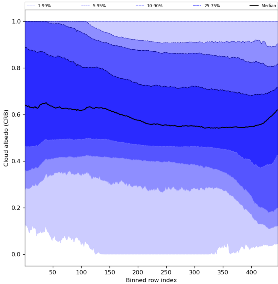
Figure 60: Along track statistics of “Cloud albedo (CRB)” for 2024-01-18 to 2024-01-20
