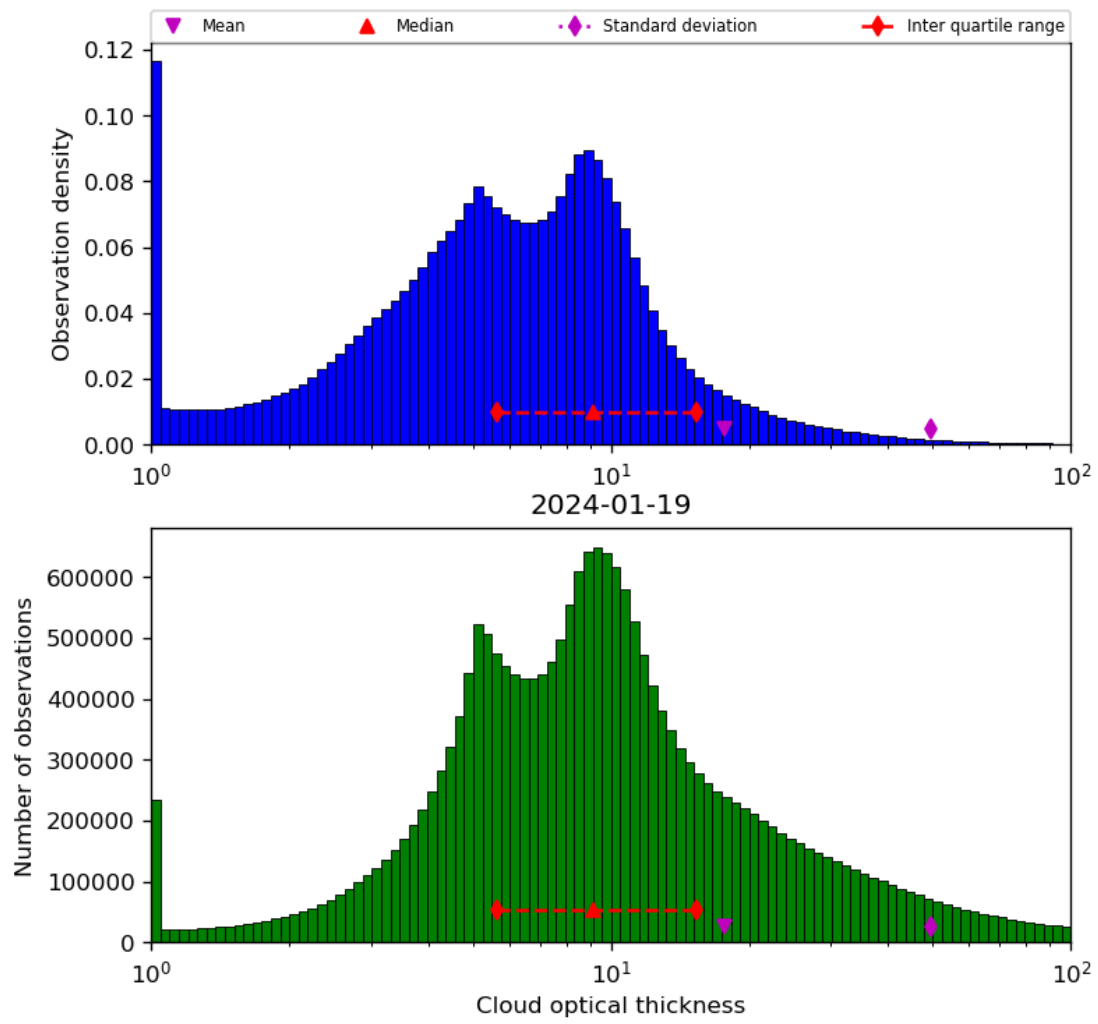
Figure 41: Histogram of “Cloud optical thickness” for 2024-01-18 to 2024-01-20
