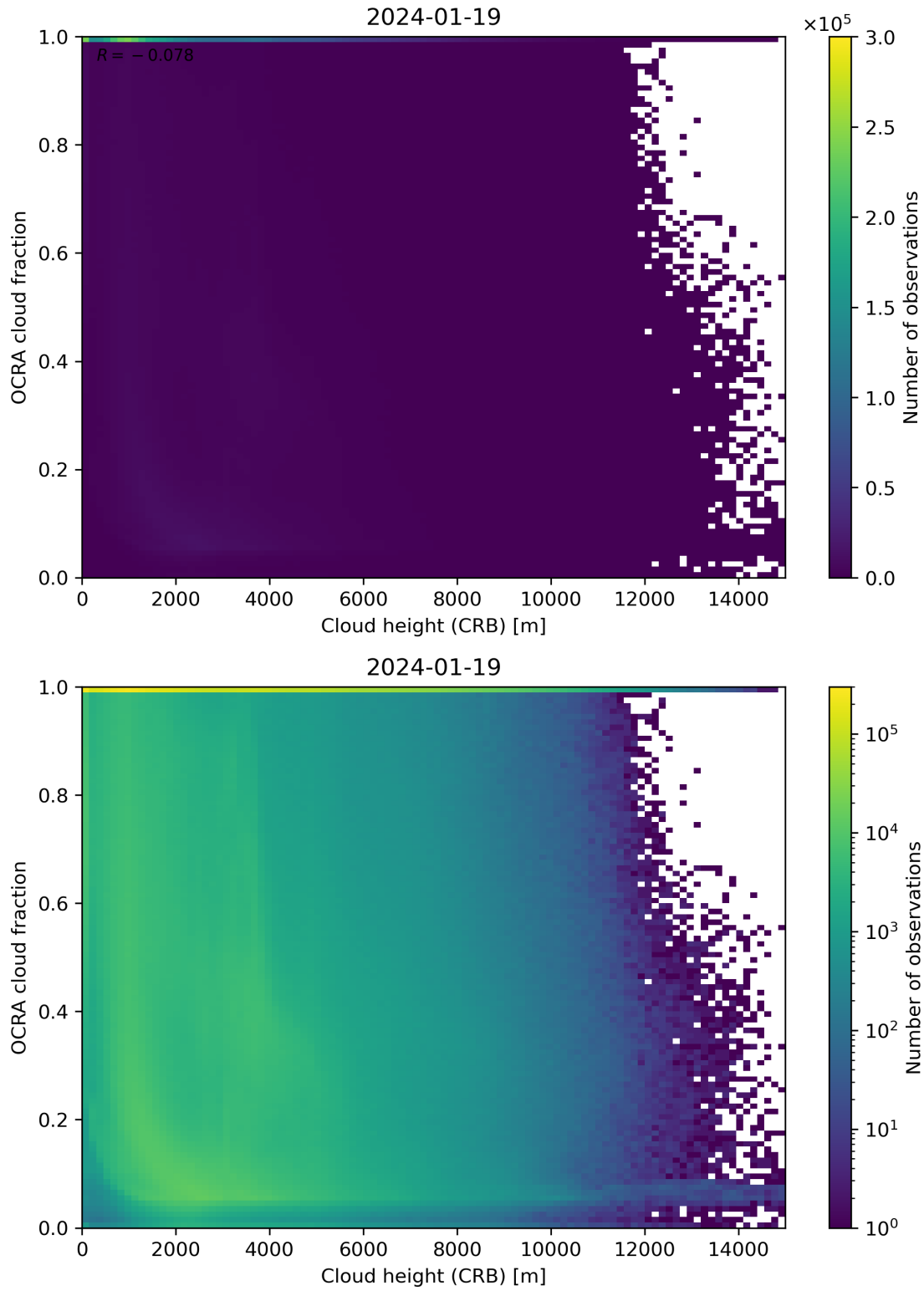
Figure 81: Scatter density plot of “Cloud height (CRB)” against “OCRA cloud fraction” for 2024-01-18 to 2024-01-20.
