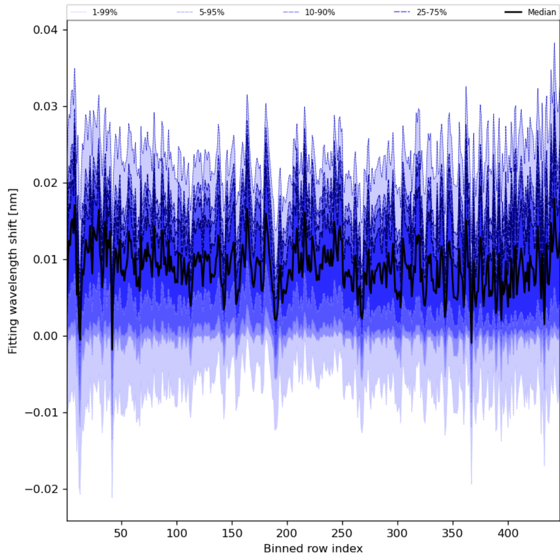
Figure 65: Along track statistics of “Fitting wavelength shift” for 2024-01-18 to 2024-01-20
