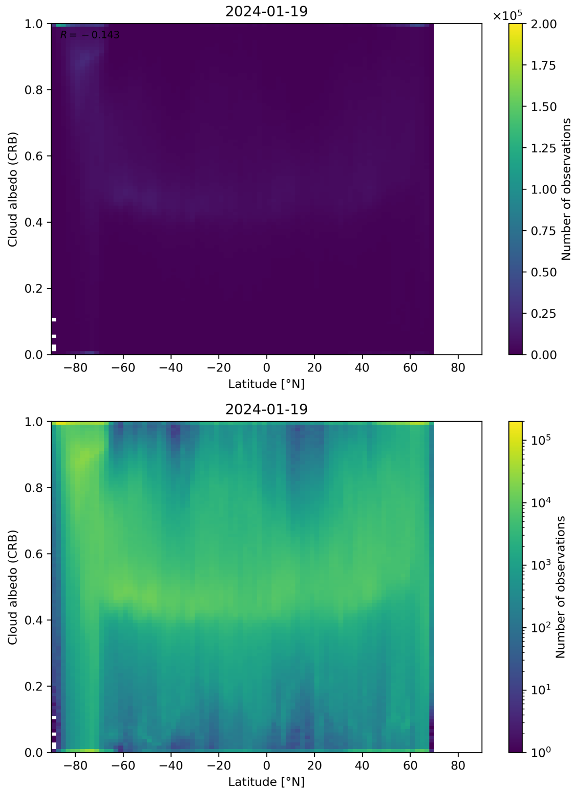
Figure 91: Scatter density plot of “Latitude” against “Cloud albedo (CRB)” for 2024-01-18 to 2024-01-20.
