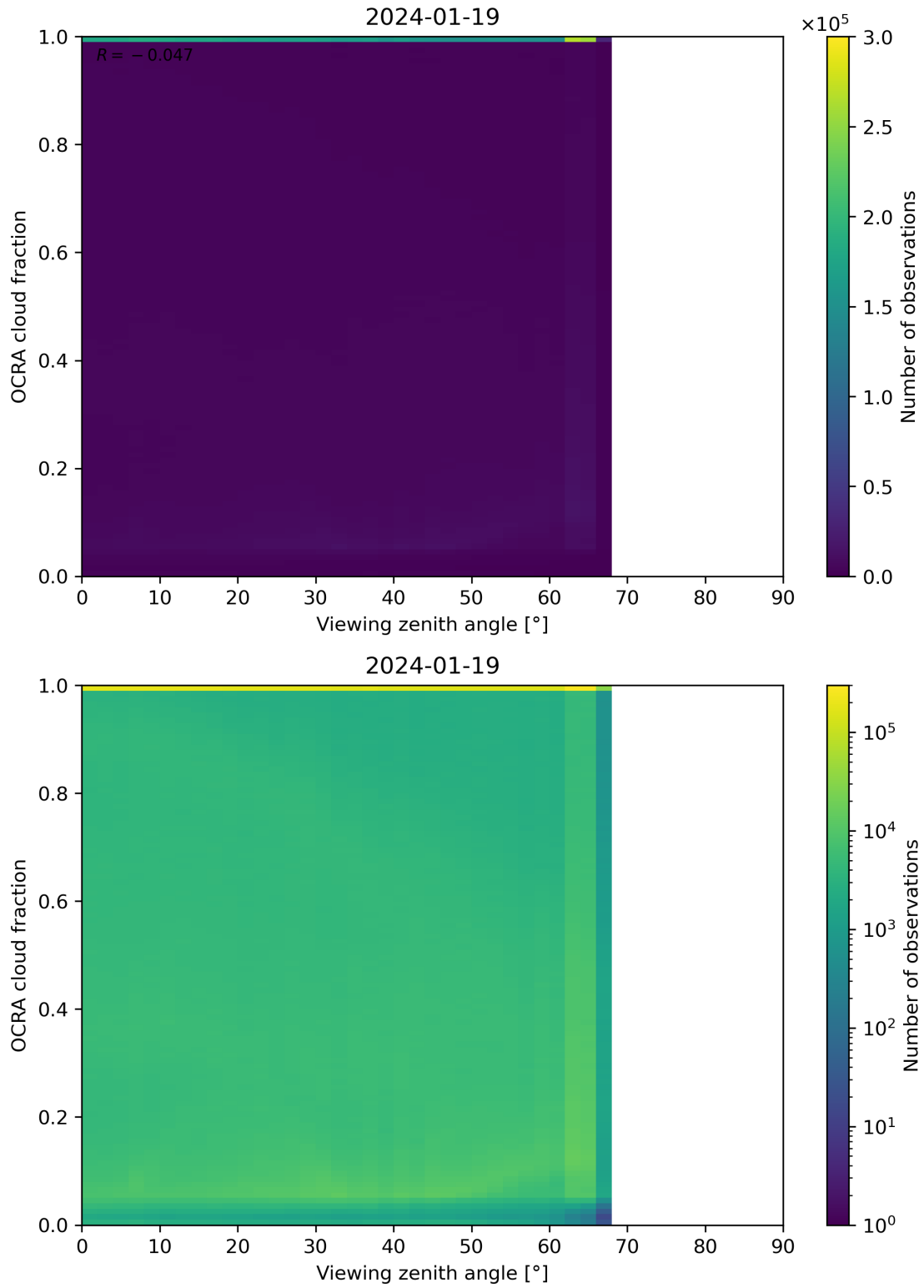
Figure 108: Scatter density plot of “Viewing zenith angle” against “OCRA cloud fraction” for 2024-01-18 to 2024-01-20.
