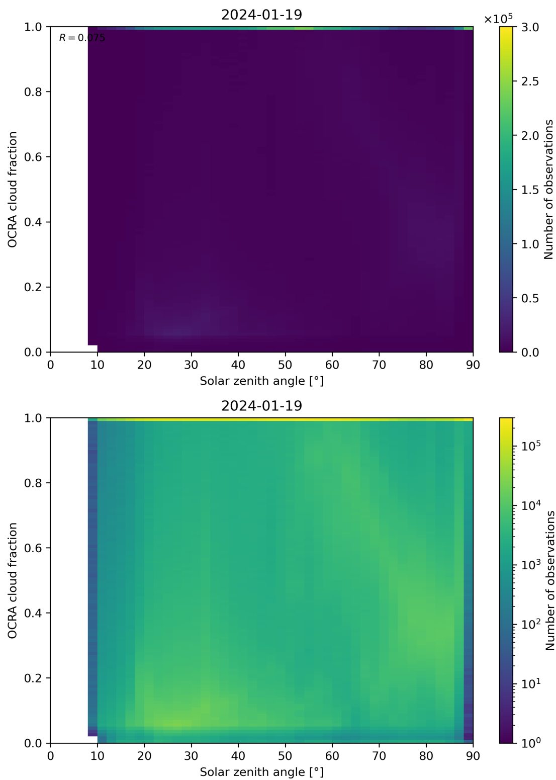
Figure 100: Scatter density plot of “Solar zenith angle” against “OCRA cloud fraction” for 2024-01-18 to 2024-01-20.
