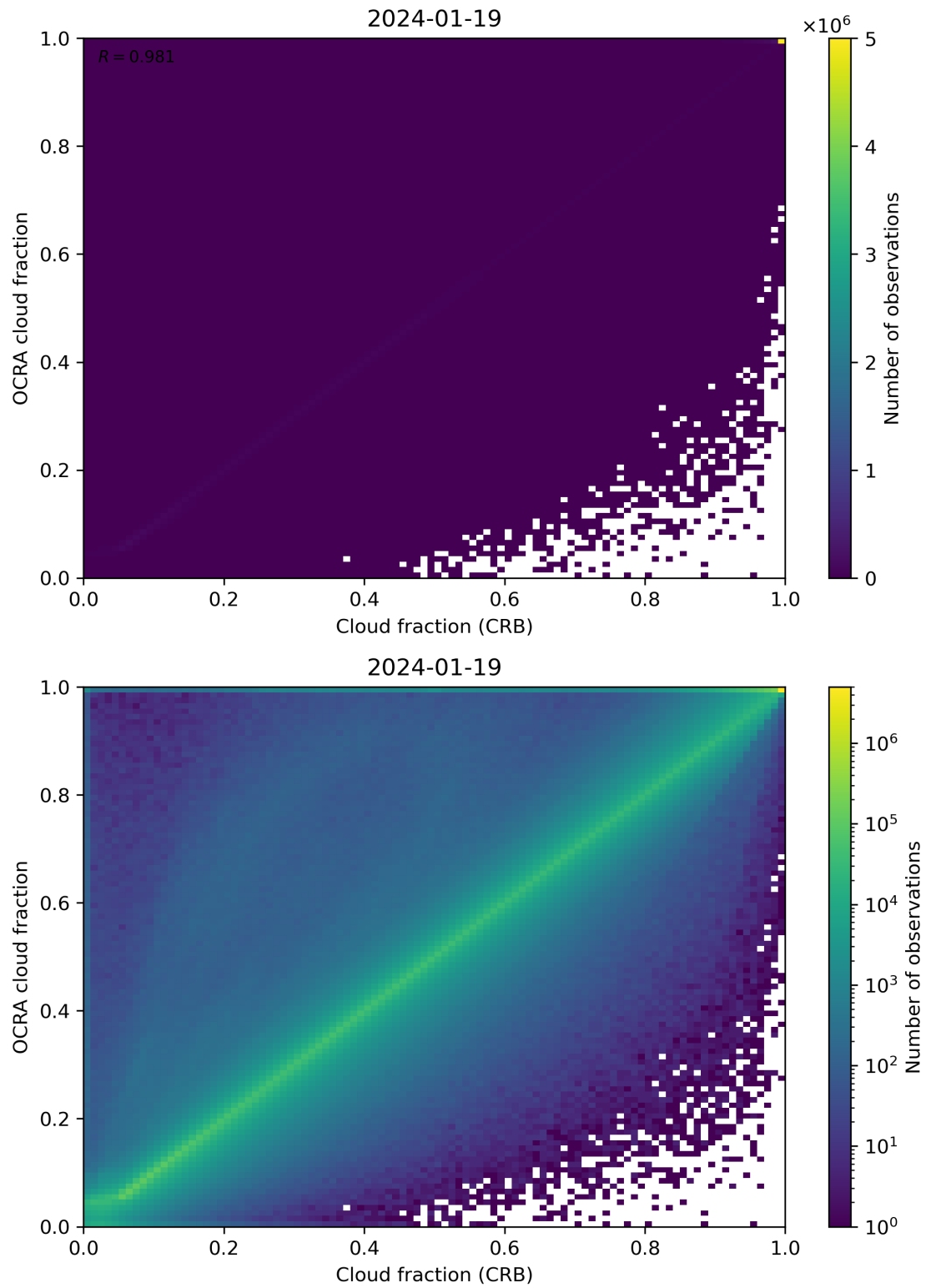
Figure 78: Scatter density plot of “Cloud fraction (CRB)” against “OCRA cloud fraction” for 2024-01-18 to 2024-01-20.
