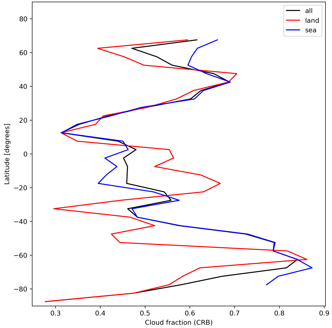
Figure 26: Zonal average of “Cloud fraction (CRB)” for 2024-01-18 to 2024-01-20.
