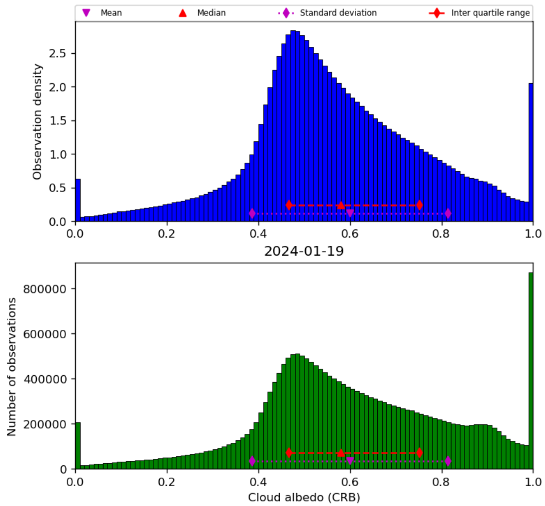
Figure 44: Histogram of “Cloud albedo (CRB)” for 2024-01-18 to 2024-01-20
