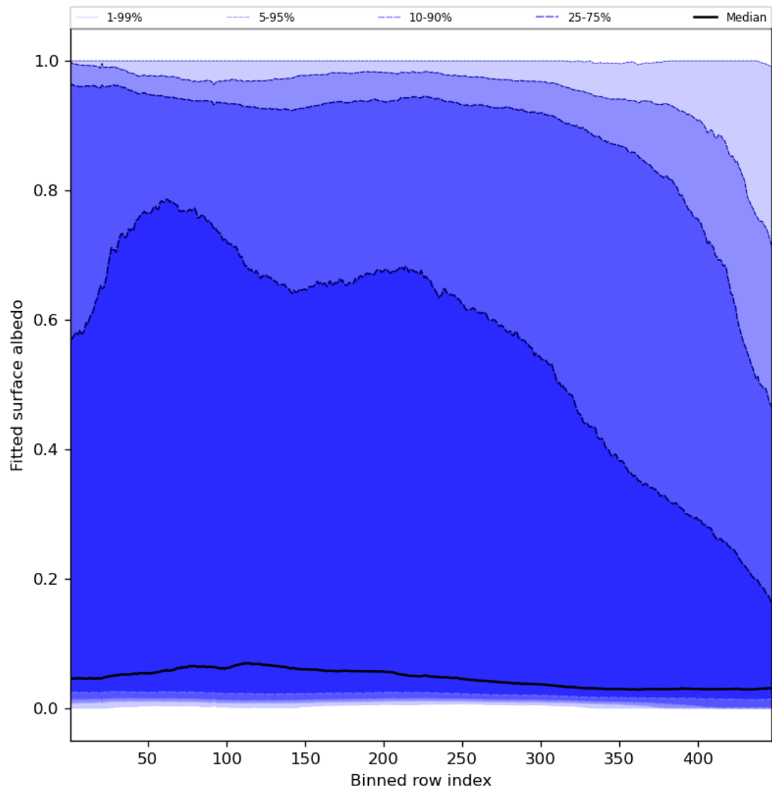
Figure 61: Along track statistics of “Fitted surface albedo” for 2024-01-18 to 2024-01-20
