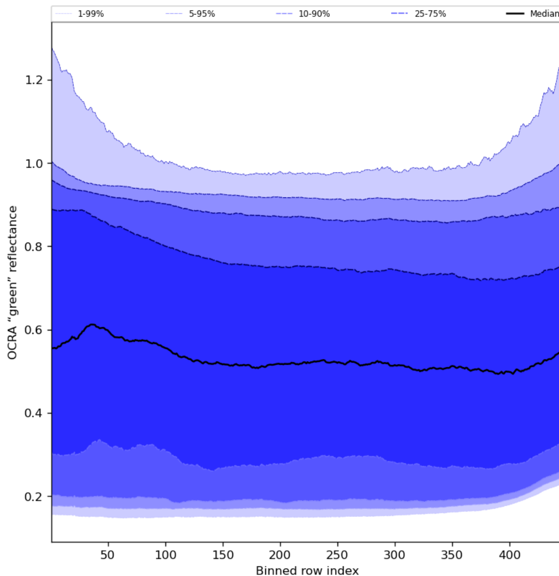
Figure 68: Along track statistics of "OCRA "green" reflectance" for 2024-01-18 to 2024-01-20
