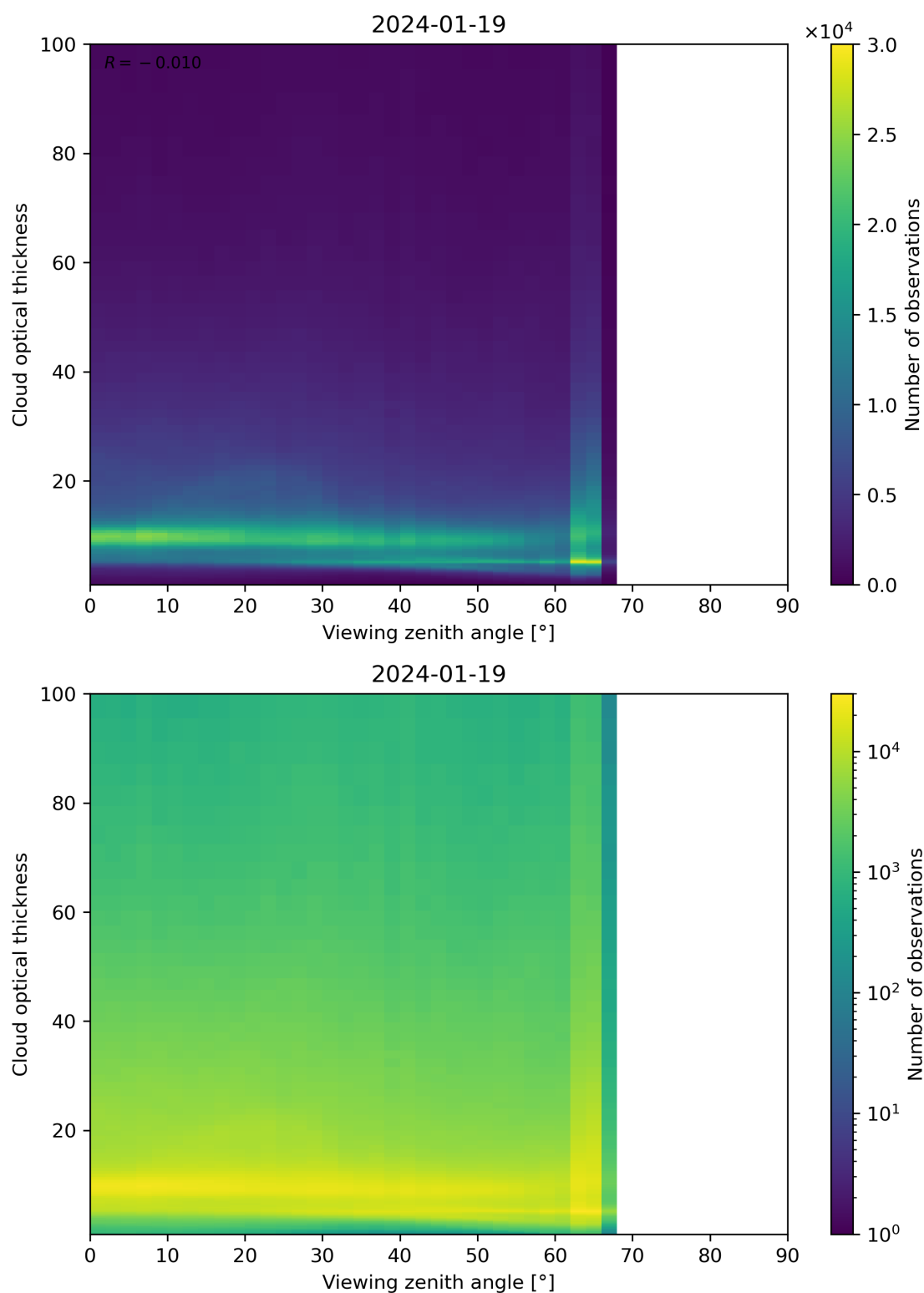
Figure 111: Scatter density plot of “Viewing zenith angle” against “Cloud optical thickness” for 2024-01-18 to 2024-01-20.
