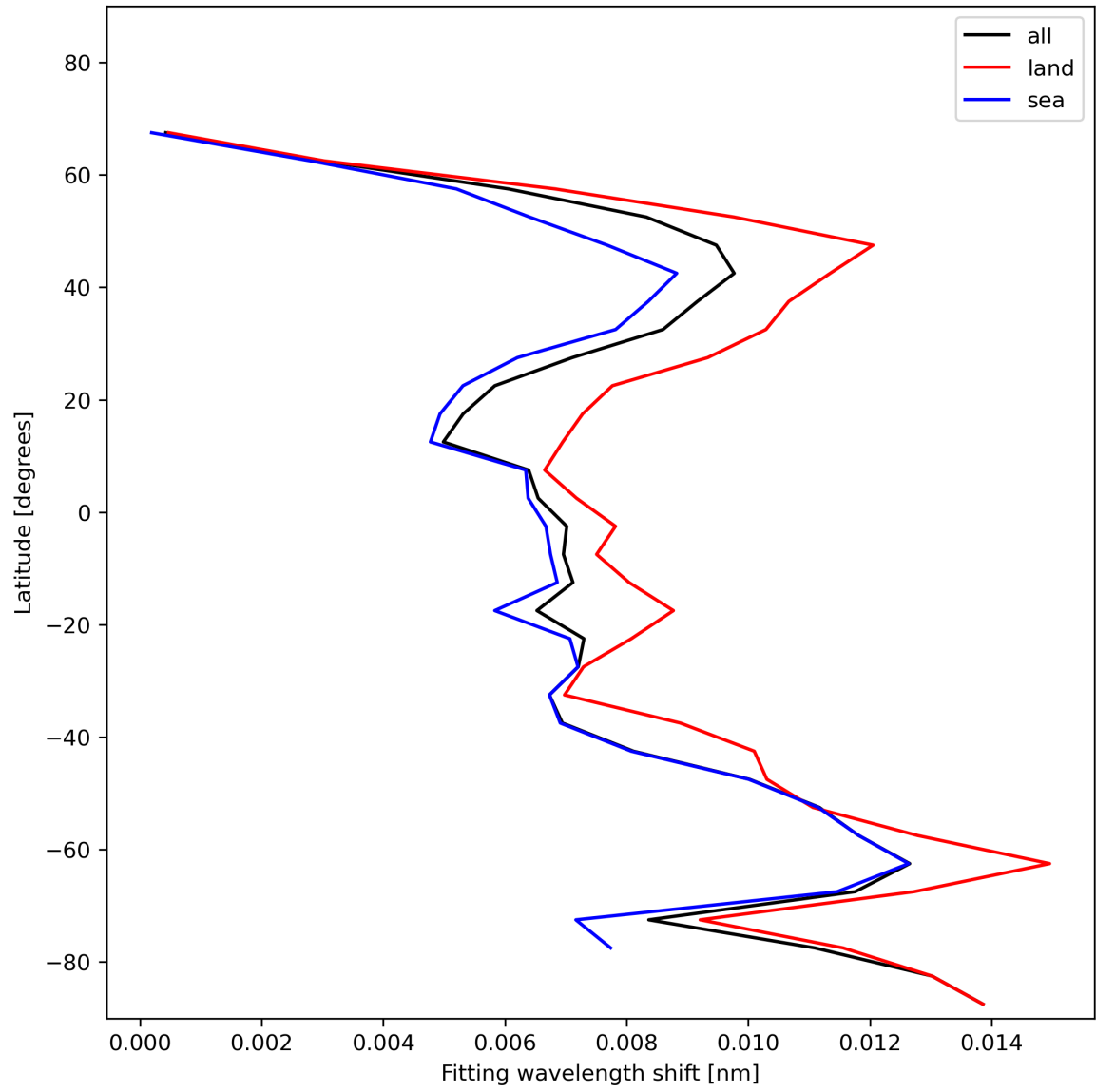
Figure 33: Zonal average of “Fitting wavelength shift” for 2024-01-18 to 2024-01-20.
