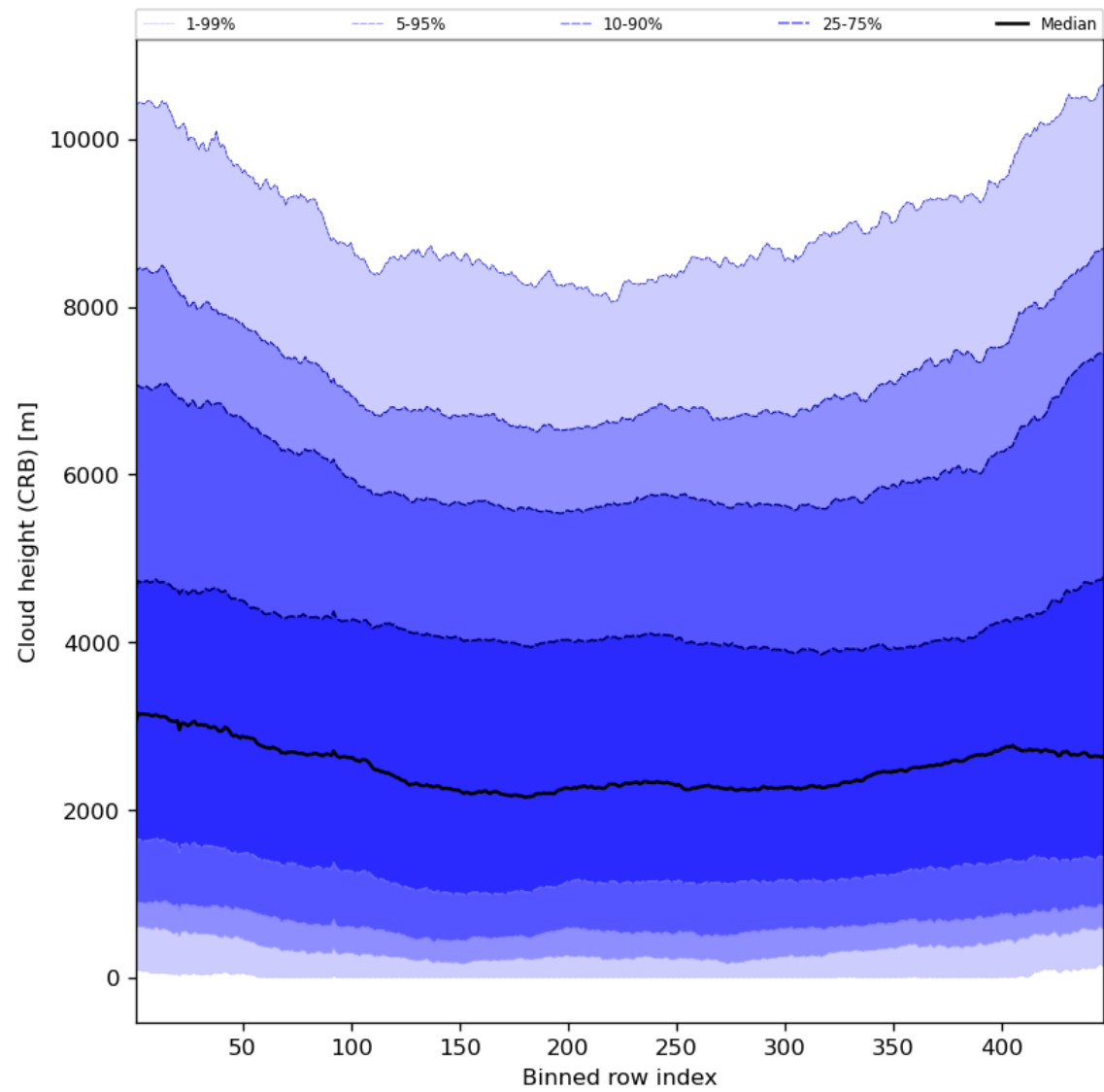
Figure 59: Along track statistics of “Cloud height (CRB)” for 2024-01-18 to 2024-01-20
