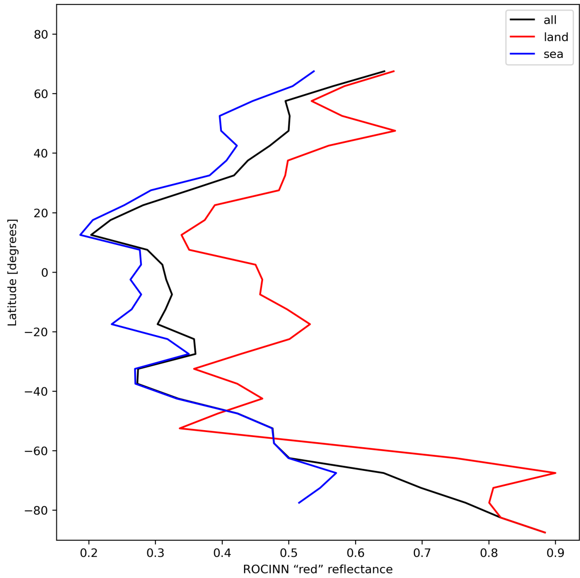
Figure 37: Zonal average of “ROCINN “red” reflectance” for 2024-01-18 to 2024-01-20.
