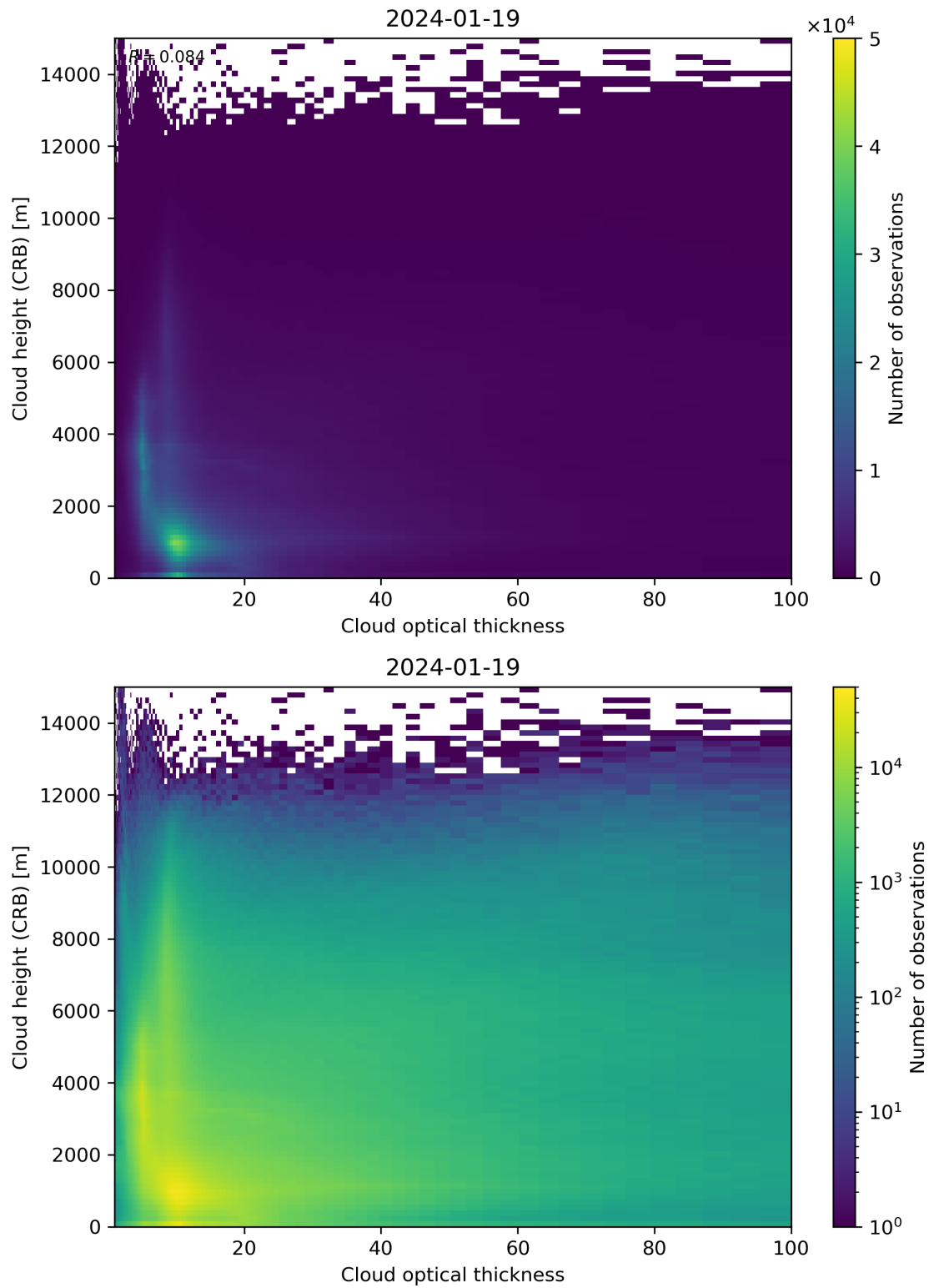
Figure 85: Scatter density plot of “Cloud optical thickness” against “Cloud height (CRB)” for 2024-01-18 to 2024-01-20.
