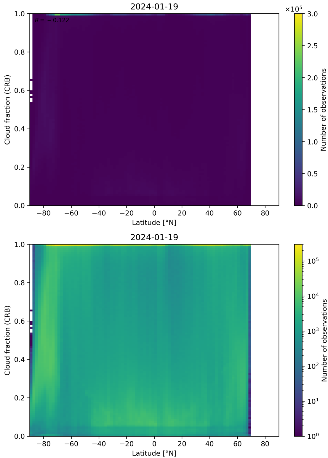
Figure 94: Scatter density plot of “Latitude” against “Cloud fraction (CRB)” for 2024-01-18 to 2024-01-20.
