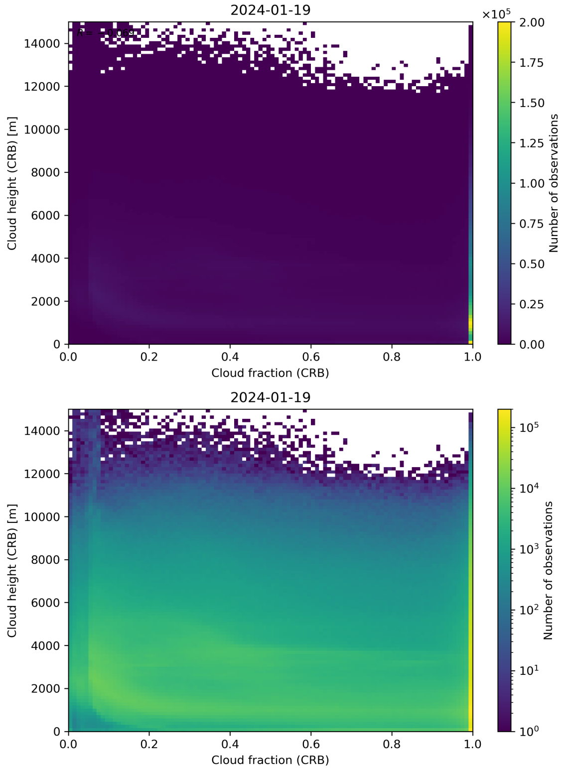
Figure 79: Scatter density plot of “Cloud fraction (CRB)” against “Cloud height (CRB)” for 2024-01-18 to 2024-01-20.
