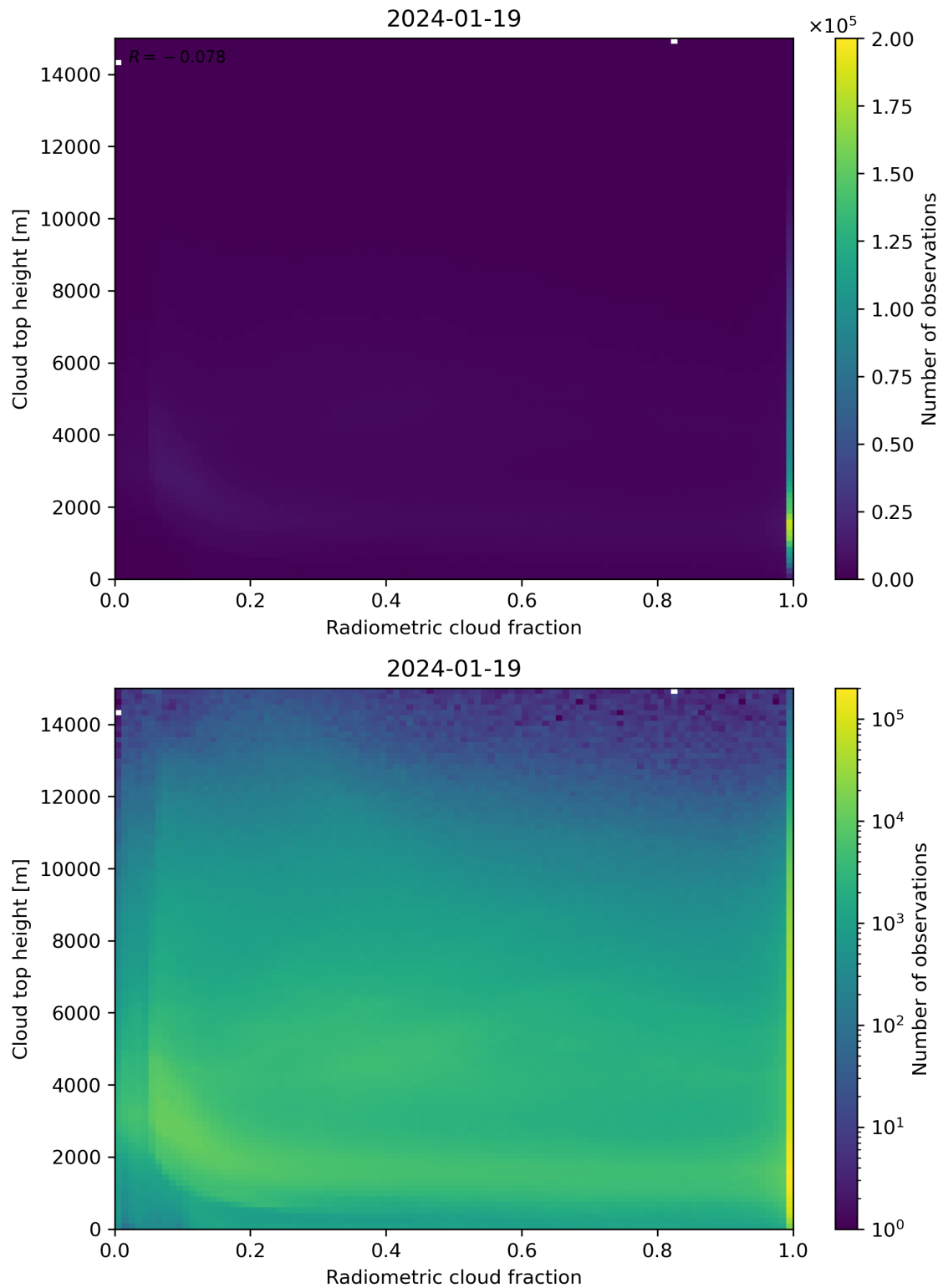
Figure 76: Scatter density plot of “Radiometric cloud fraction” against “Cloud top height” for 2024-01-18 to 2024-01-20.
