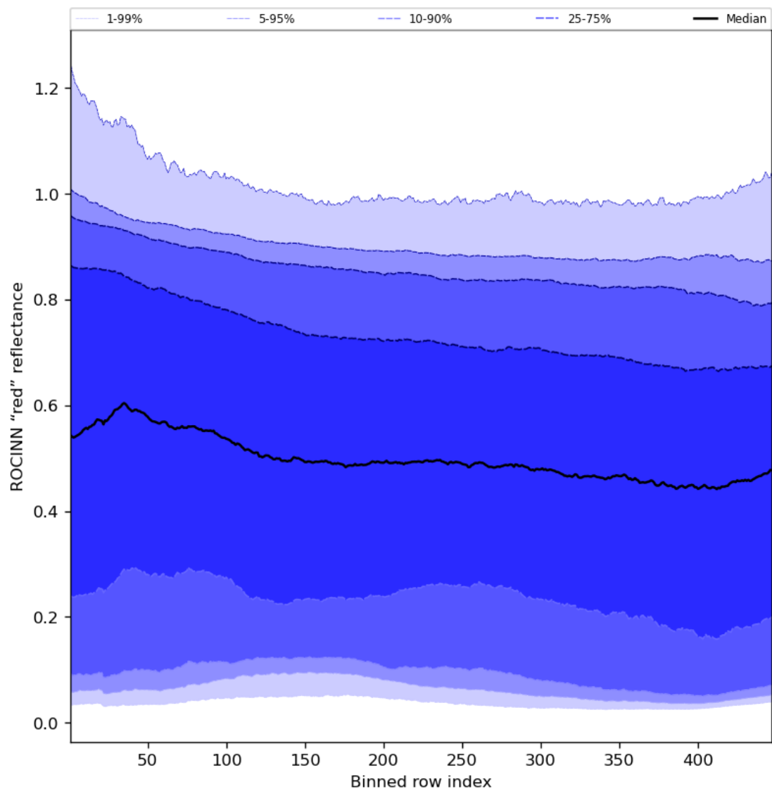
Figure 69: Along track statistics of “ROCINN “red” reflectance” for 2024-01-18 to 2024-01-20
