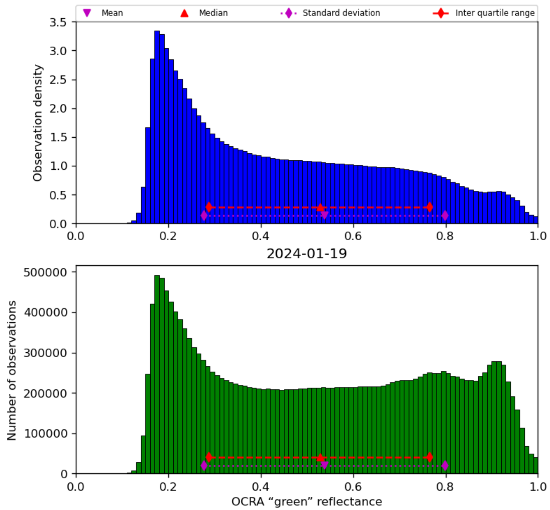
Figure 52: Histogram of “OCRA “green” reflectance” for 2024-01-18 to 2024-01-20
