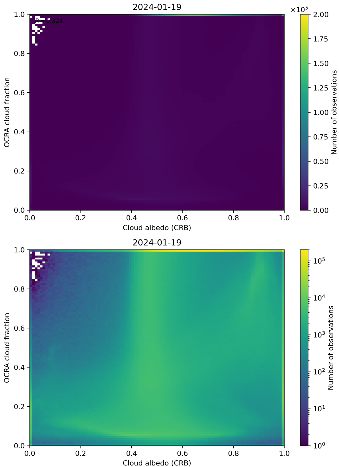
Figure 70: Scatter density plot of “Cloud albedo (CRB)” against “OCRA cloud fraction” for 2024-01-18 to 2024-01-20.
