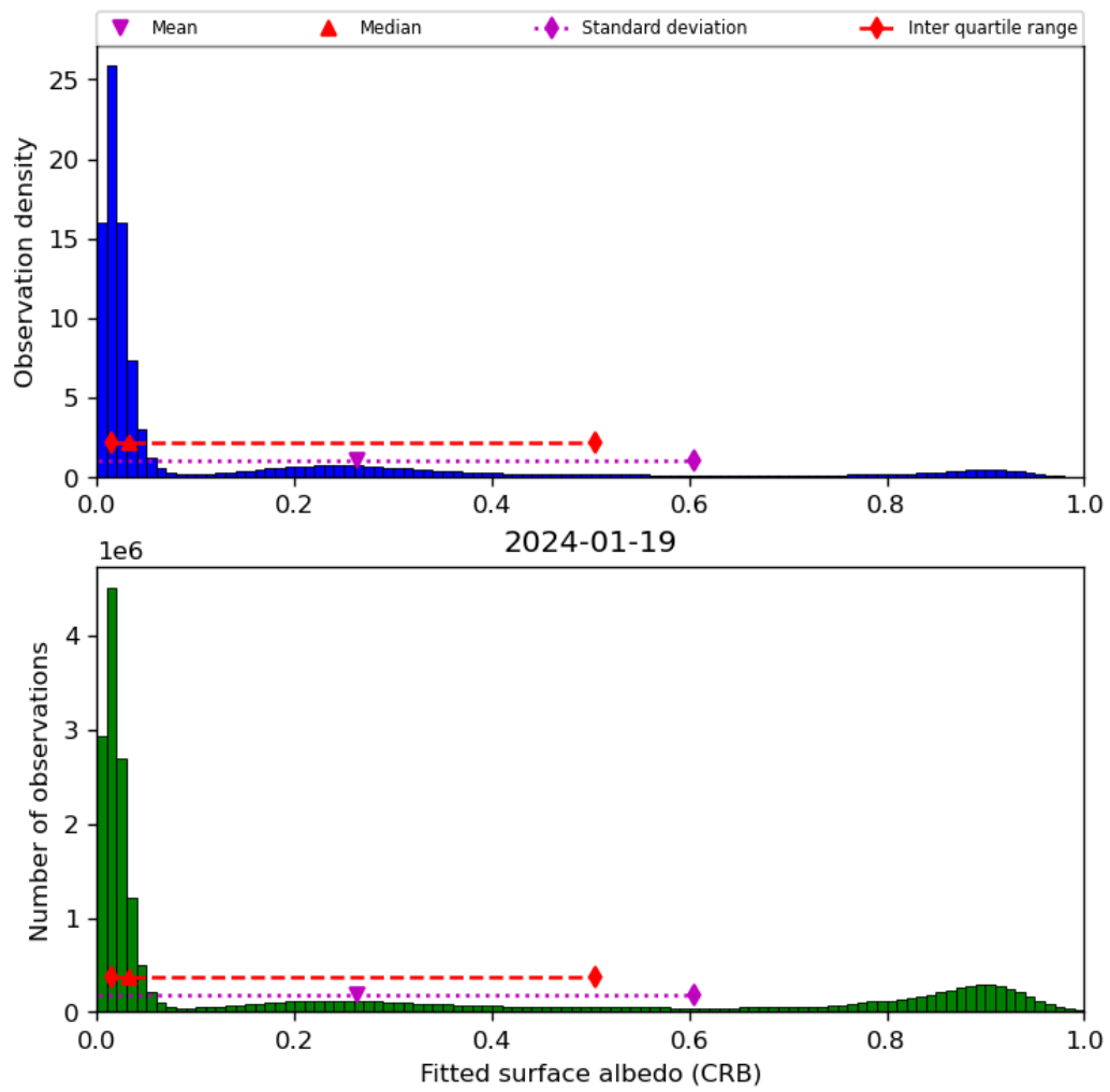
Figure 46: Histogram of “Fitted surface albedo (CRB)” for 2024-01-18 to 2024-01-20
