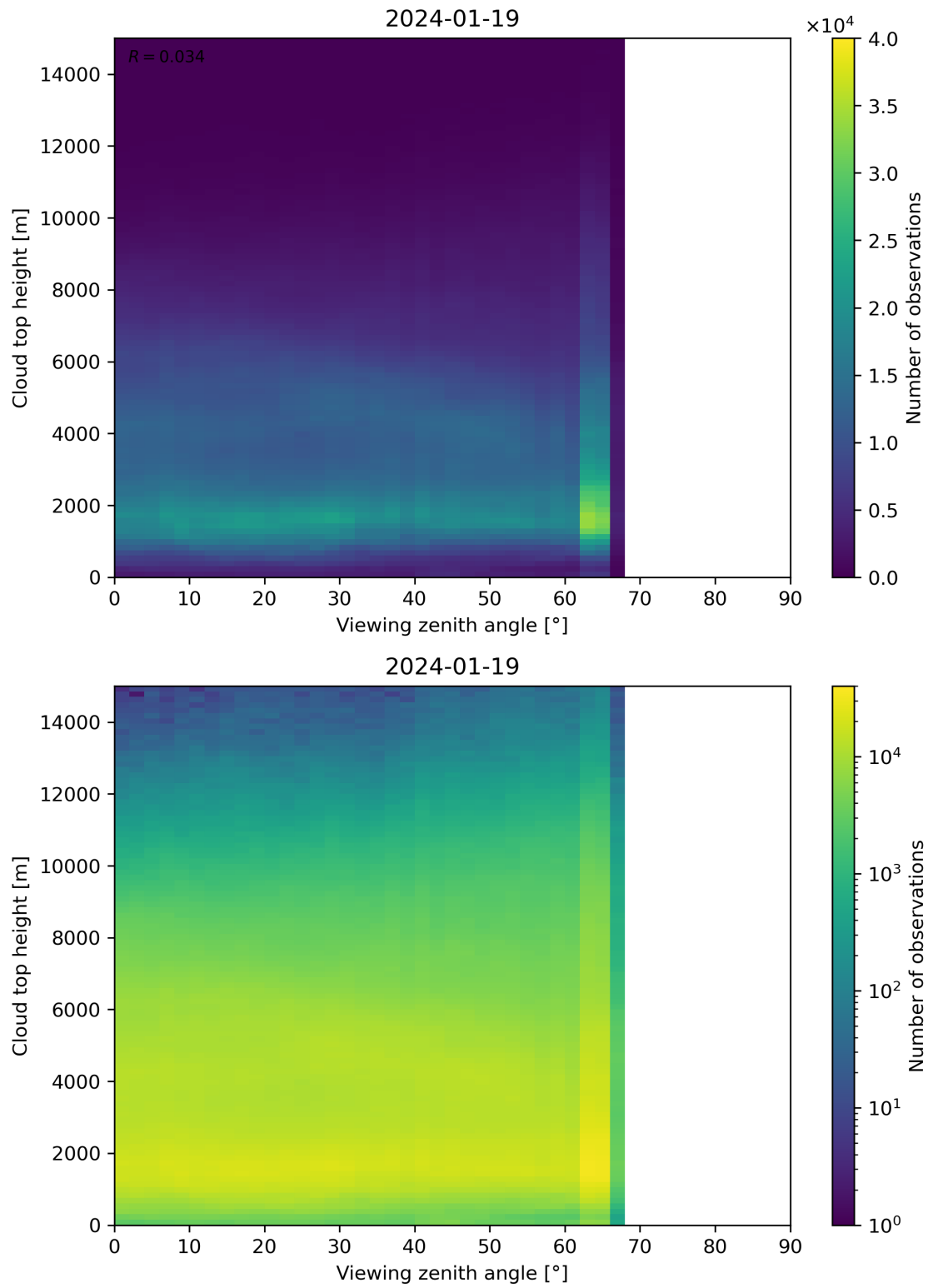
Figure 112: Scatter density plot of “Viewing zenith angle” against “Cloud top height” for 2024-01-18 to 2024-01-20.
