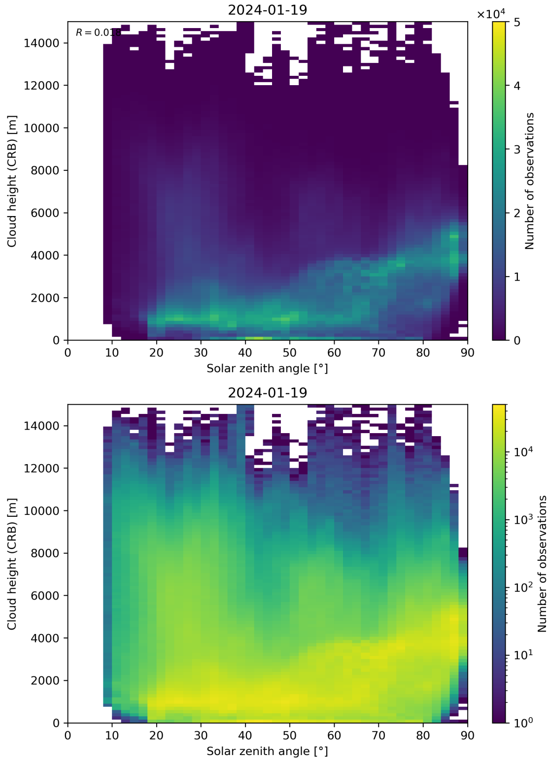
Figure 102: Scatter density plot of “Solar zenith angle” against “Cloud height (CRB)” for 2024-01-18 to 2024-01-20.
