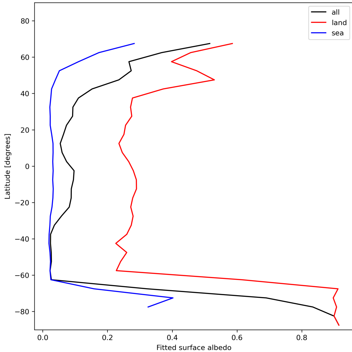
Figure 29: Zonal average of “Fitted surface albedo” for 2024-01-18 to 2024-01-20.
