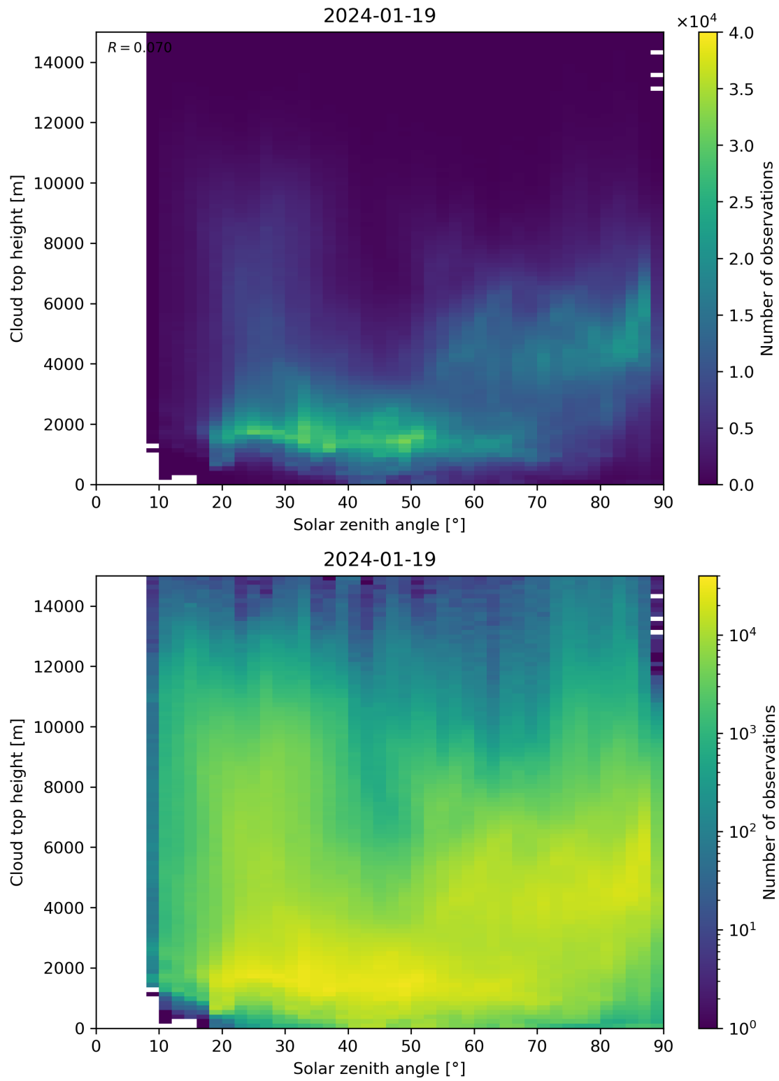
Figure 104: Scatter density plot of “Solar zenith angle” against “Cloud top height” for 2024-01-18 to 2024-01-20.
