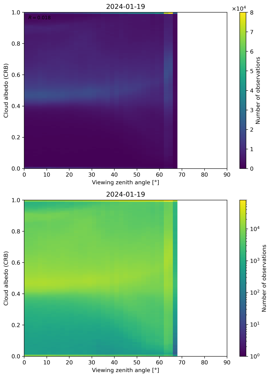
Figure 106: Scatter density plot of “Viewing zenith angle” against “Cloud albedo (CRB)” for 2024-01-18 to 2024-01-20.
