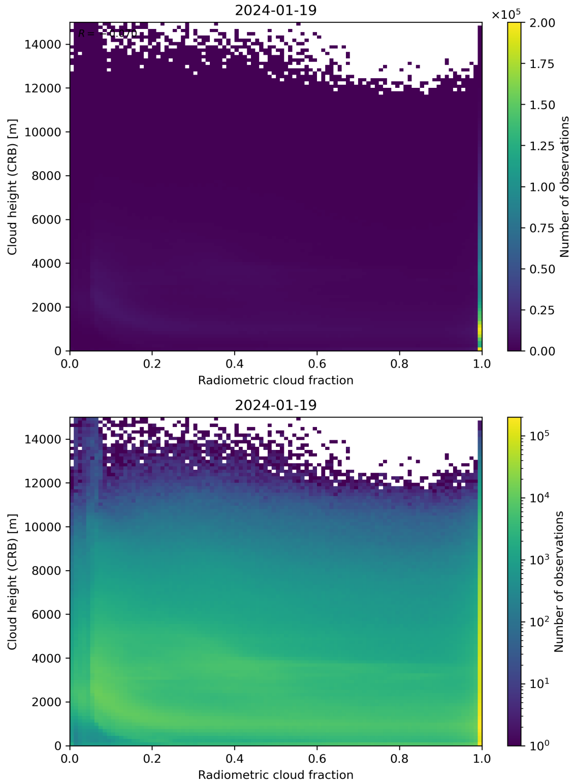
Figure 74: Scatter density plot of “Radiometric cloud fraction” against “Cloud height (CRB)” for 2024-01-18 to 2024-01-20.
