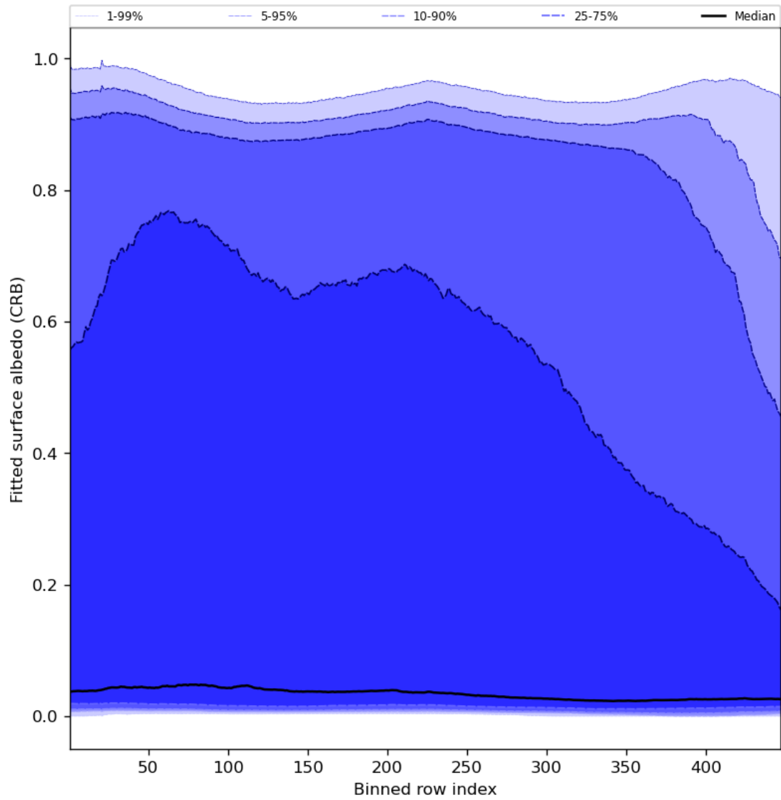
Figure 62: Along track statistics of “Fitted surface albedo (CRB)” for 2024-01-18 to 2024-01-20
