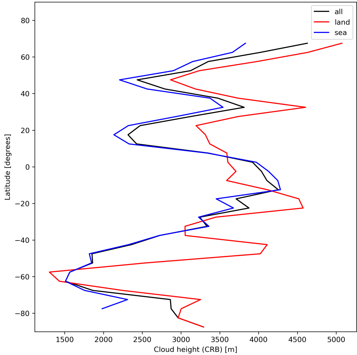
Figure 27: Zonal average of “Cloud height (CRB)” for 2024-01-18 to 2024-01-20.
