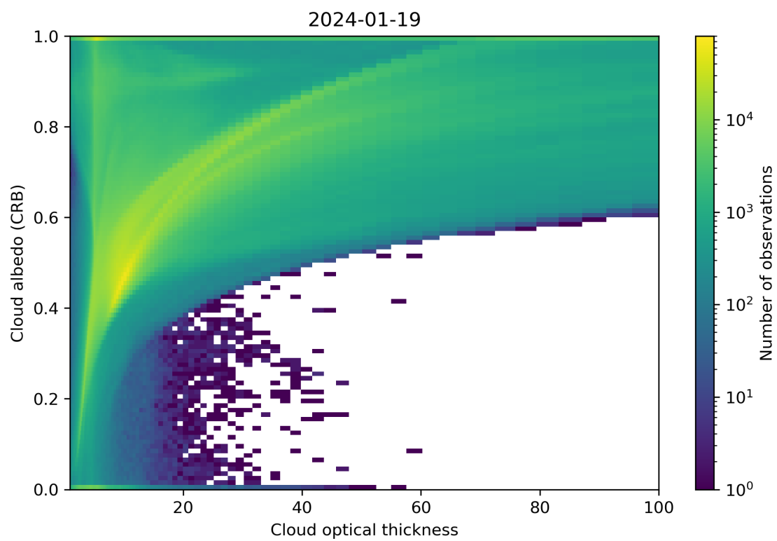
Figure 82: Scatter density plot of “Cloud optical thickness” against “Cloud albedo (CRB)” for 2024-01-18 to 2024-01-20.
