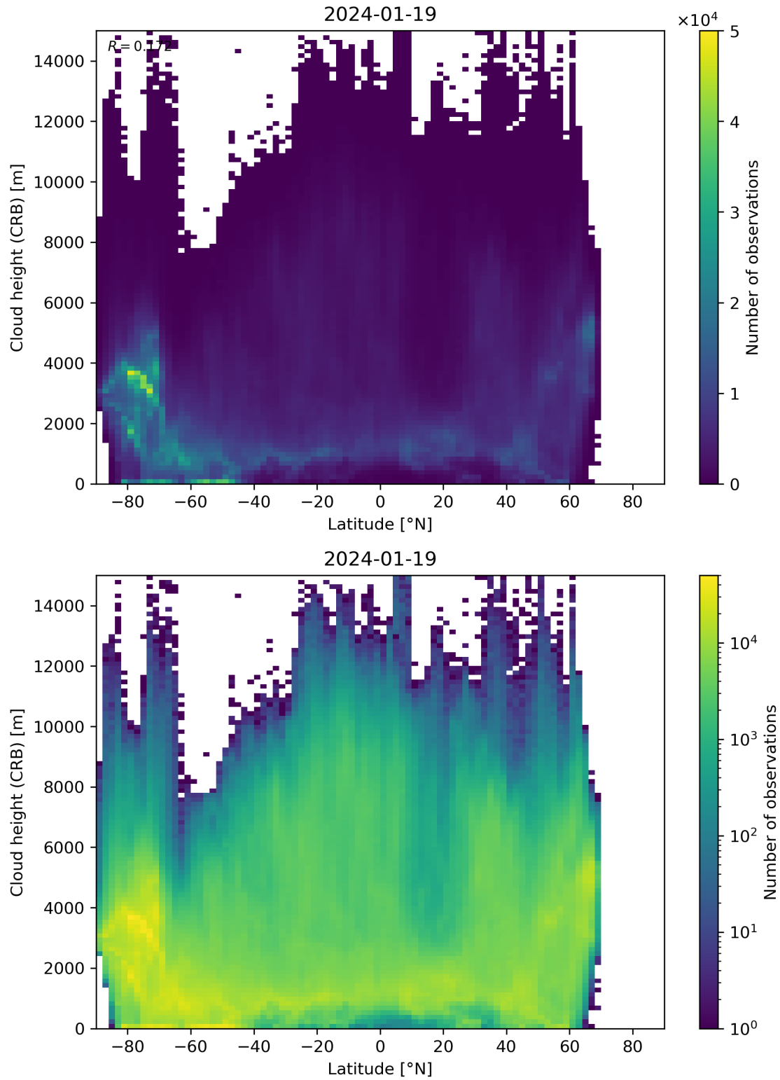
Figure 95: Scatter density plot of “Latitude” against “Cloud height (CRB)” for 2024-01-18 to 2024-01-20.
