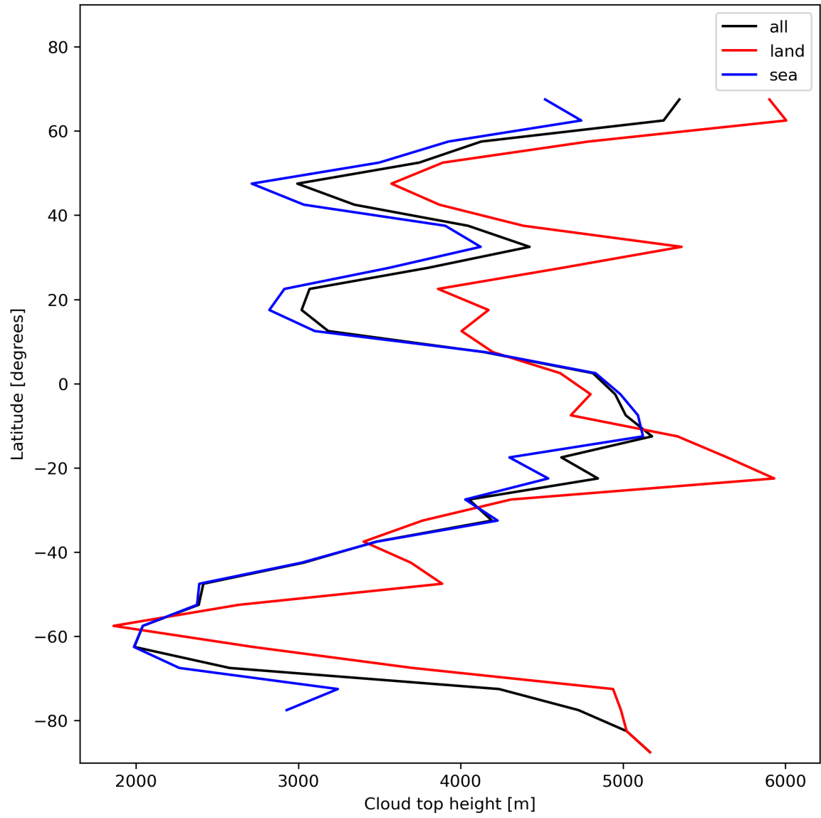
Figure 24: Zonal average of “Cloud top height” for 2024-01-18 to 2024-01-20.
