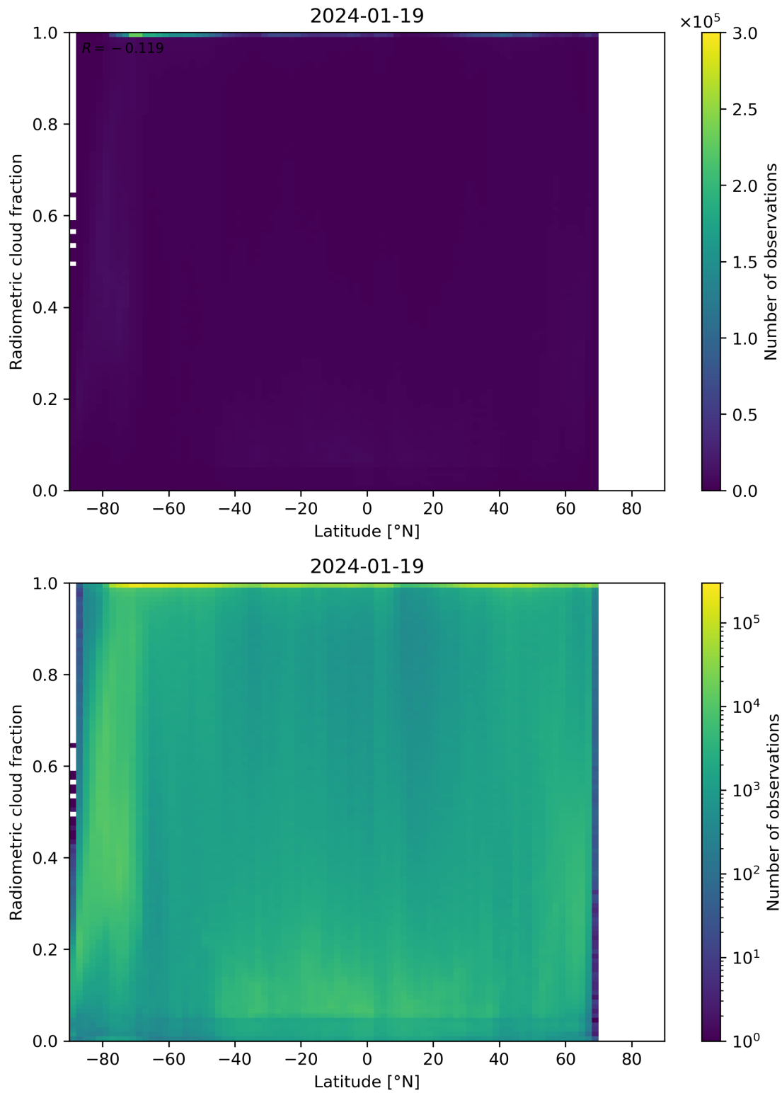
Figure 92: Scatter density plot of “Latitude” against “Radiometric cloud fraction” for 2024-01-18 to 2024-01-20.
