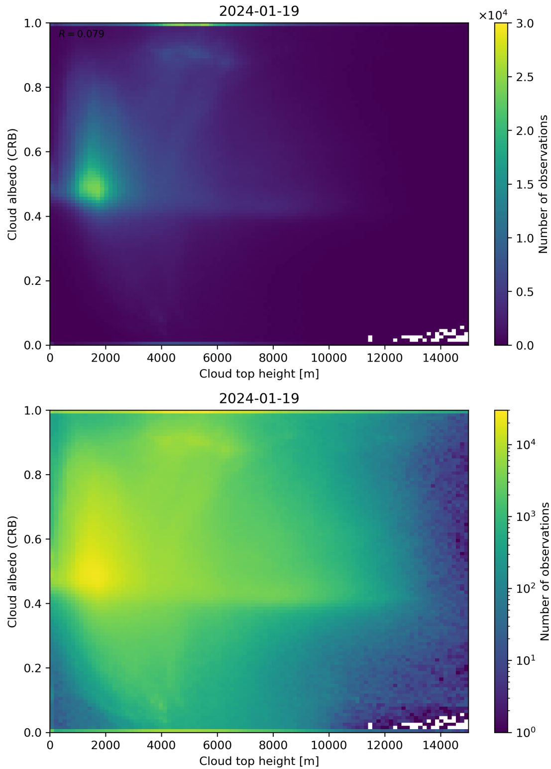
Figure 86: Scatter density plot of “Cloud top height” against “Cloud albedo (CRB)” for 2024-01-18 to 2024-01-20.
