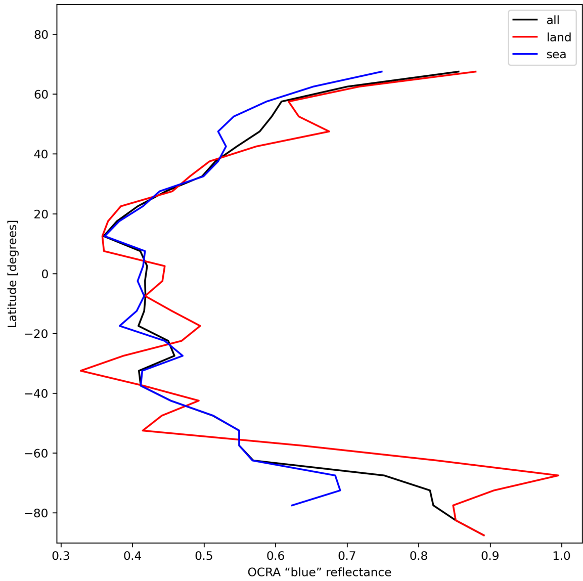
Figure 35: Zonal average of “OCRA “blue” reflectance” for 2024-01-18 to 2024-01-20.
