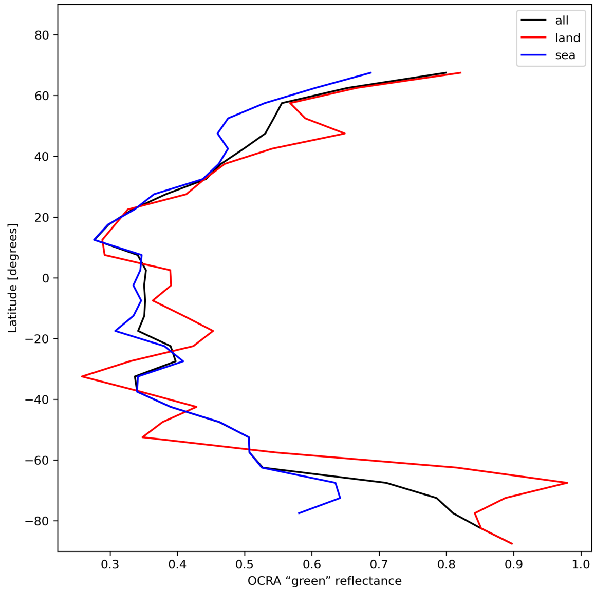
Figure 36: Zonal average of “OCRA “green” reflectance” for 2024-01-18 to 2024-01-20.
