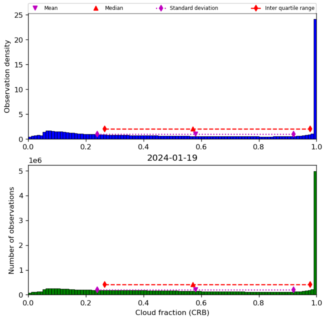
Figure 42: Histogram of “Cloud fraction (CRB)” for 2024-01-18 to 2024-01-20
