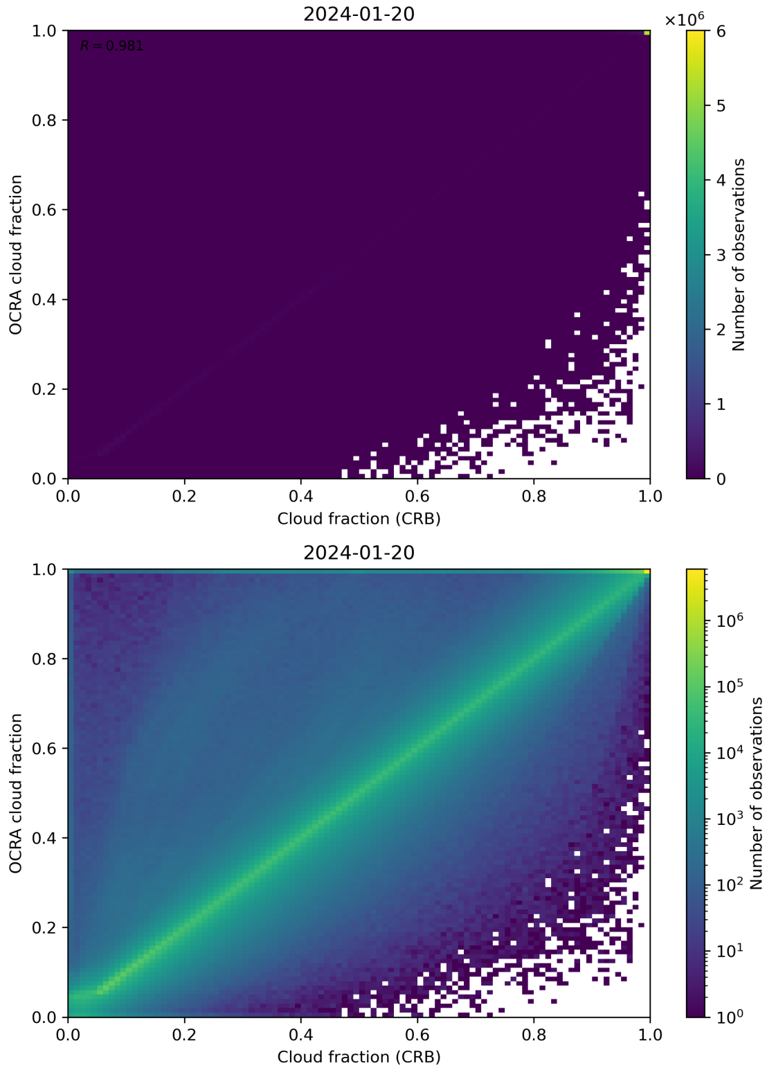
Figure 78: Scatter density plot of “Cloud fraction (CRB)” against “OCRA cloud fraction” for 2024-01-19 to 2024-01-21.
