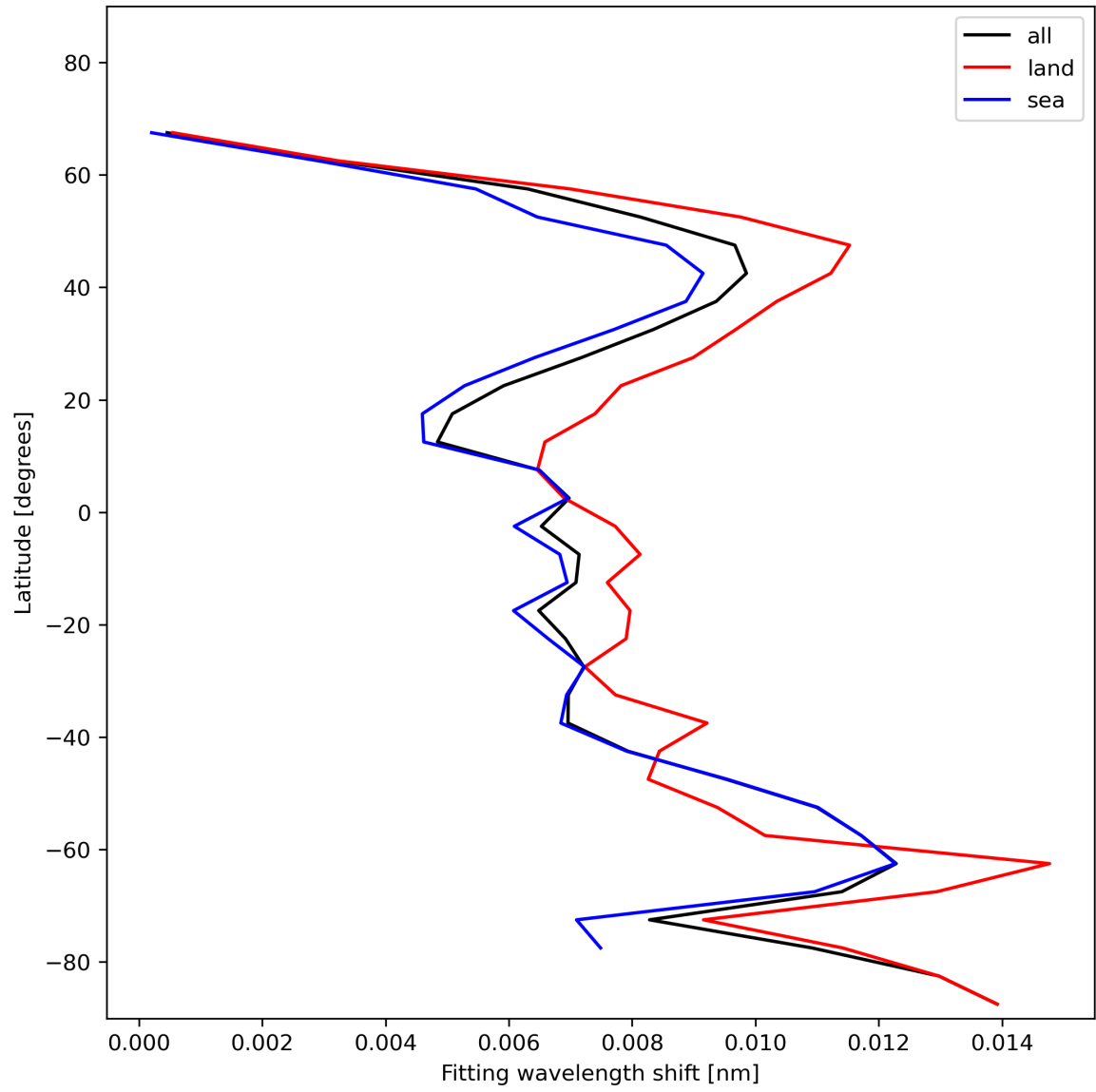
Figure 33: Zonal average of “Fitting wavelength shift” for 2024-01-19 to 2024-01-21.
