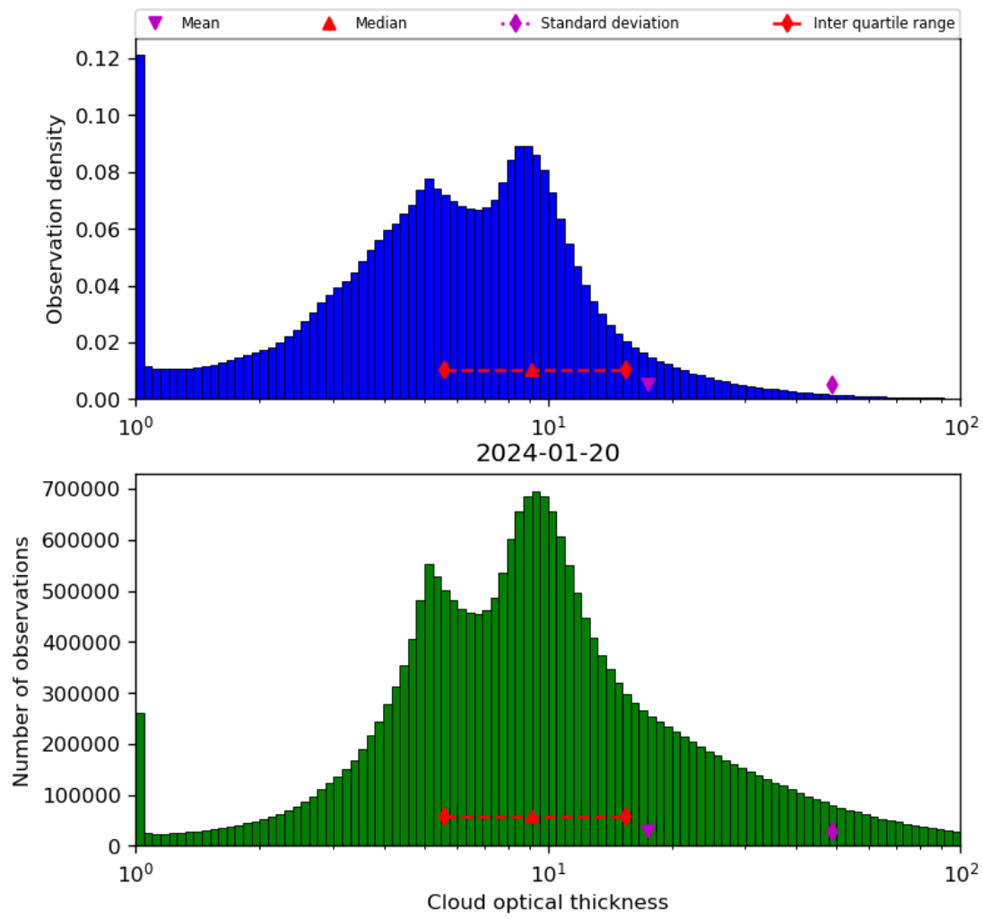
Figure 41: Histogram of “Cloud optical thickness” for 2024-01-19 to 2024-01-21
