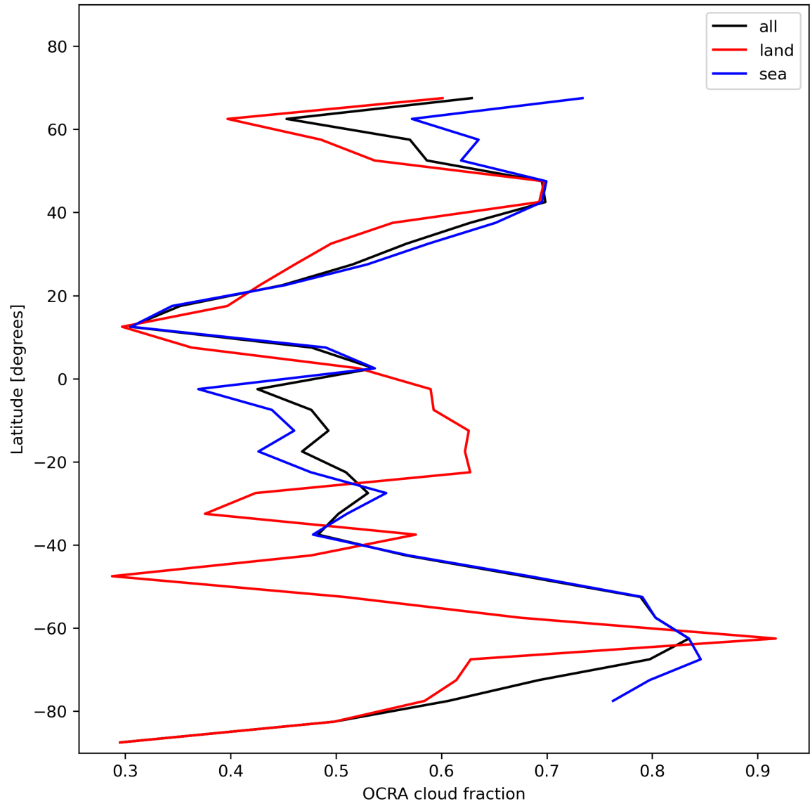
Figure 34: Zonal average of “OCRA cloud fraction” for 2024-01-19 to 2024-01-21.
