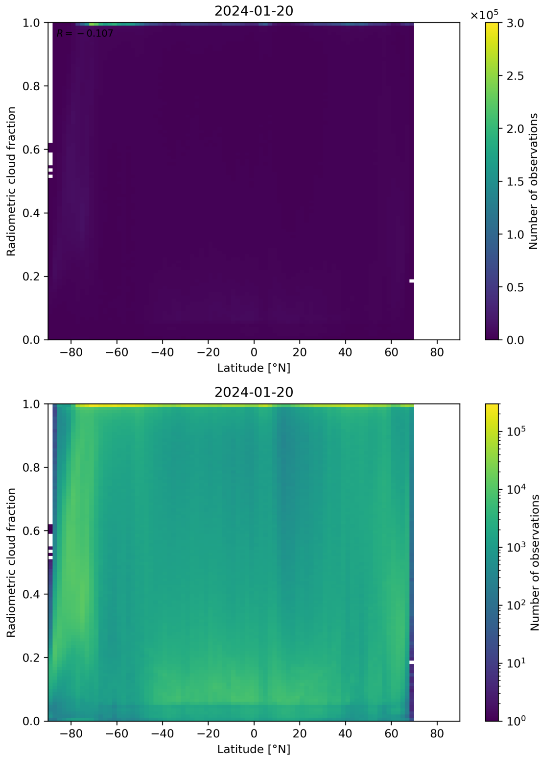
Figure 92: Scatter density plot of “Latitude” against “Radiometric cloud fraction” for 2024-01-19 to 2024-01-21.
