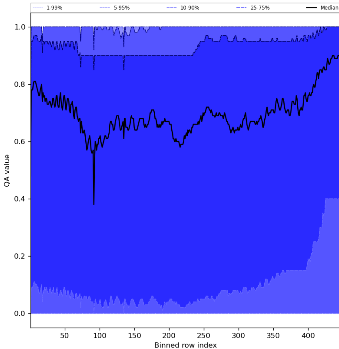
Figure 54: Along track statistics of “QA value” for 2024-01-19 to 2024-01-21
