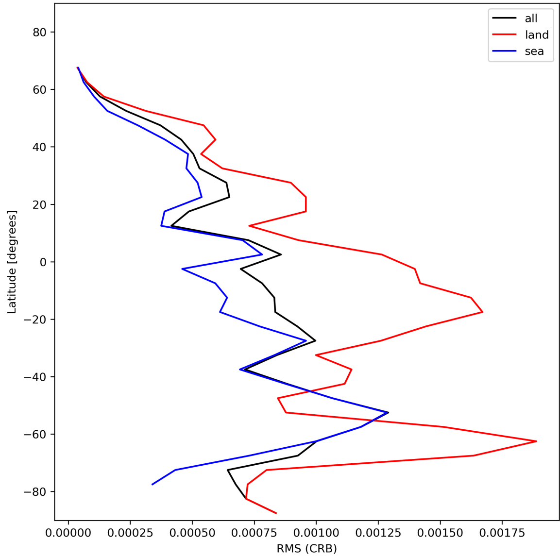
Figure 32: Zonal average of “RMS (CRB)” for 2024-01-19 to 2024-01-21.
