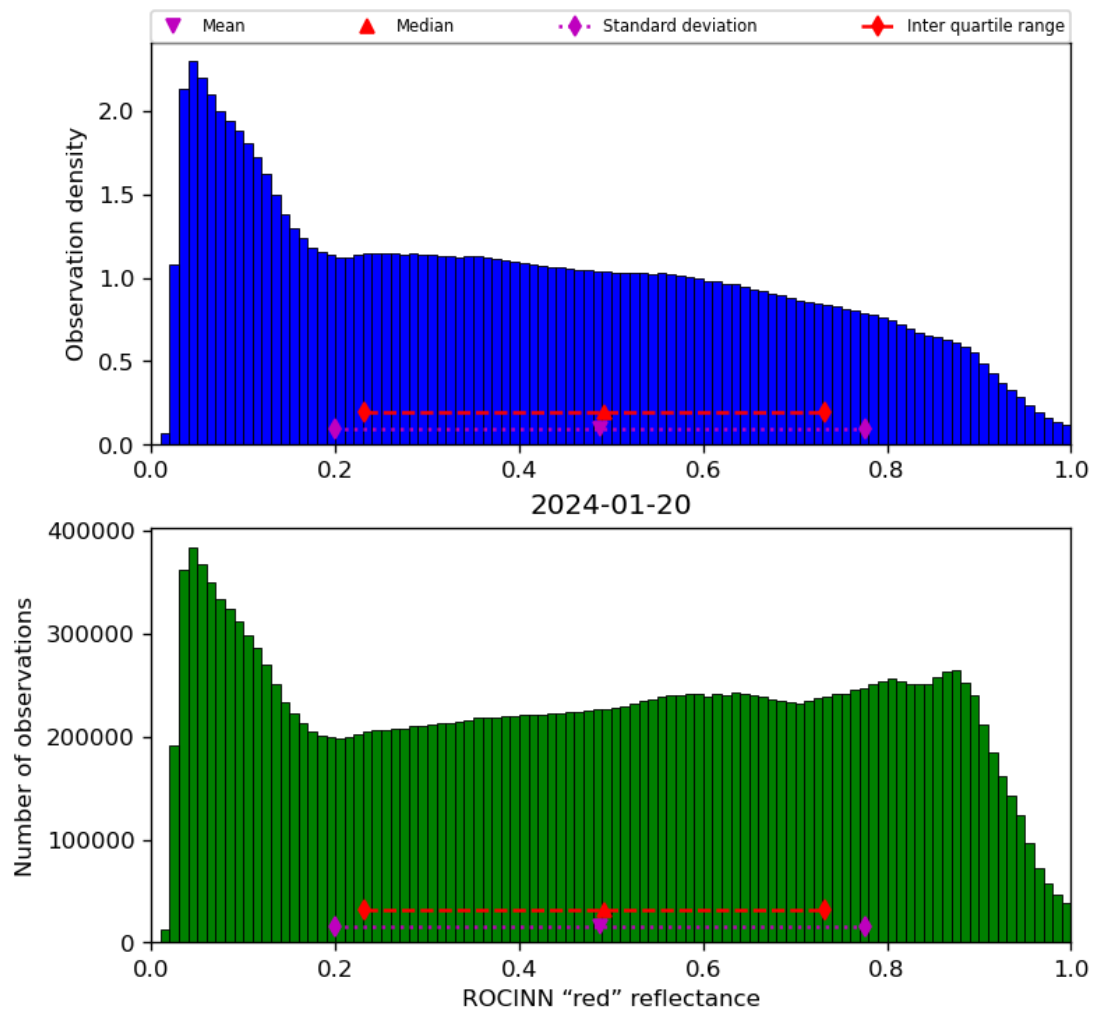
Figure 53: Histogram of “ROCINN “red” reflectance” for 2024-01-19 to 2024-01-21
