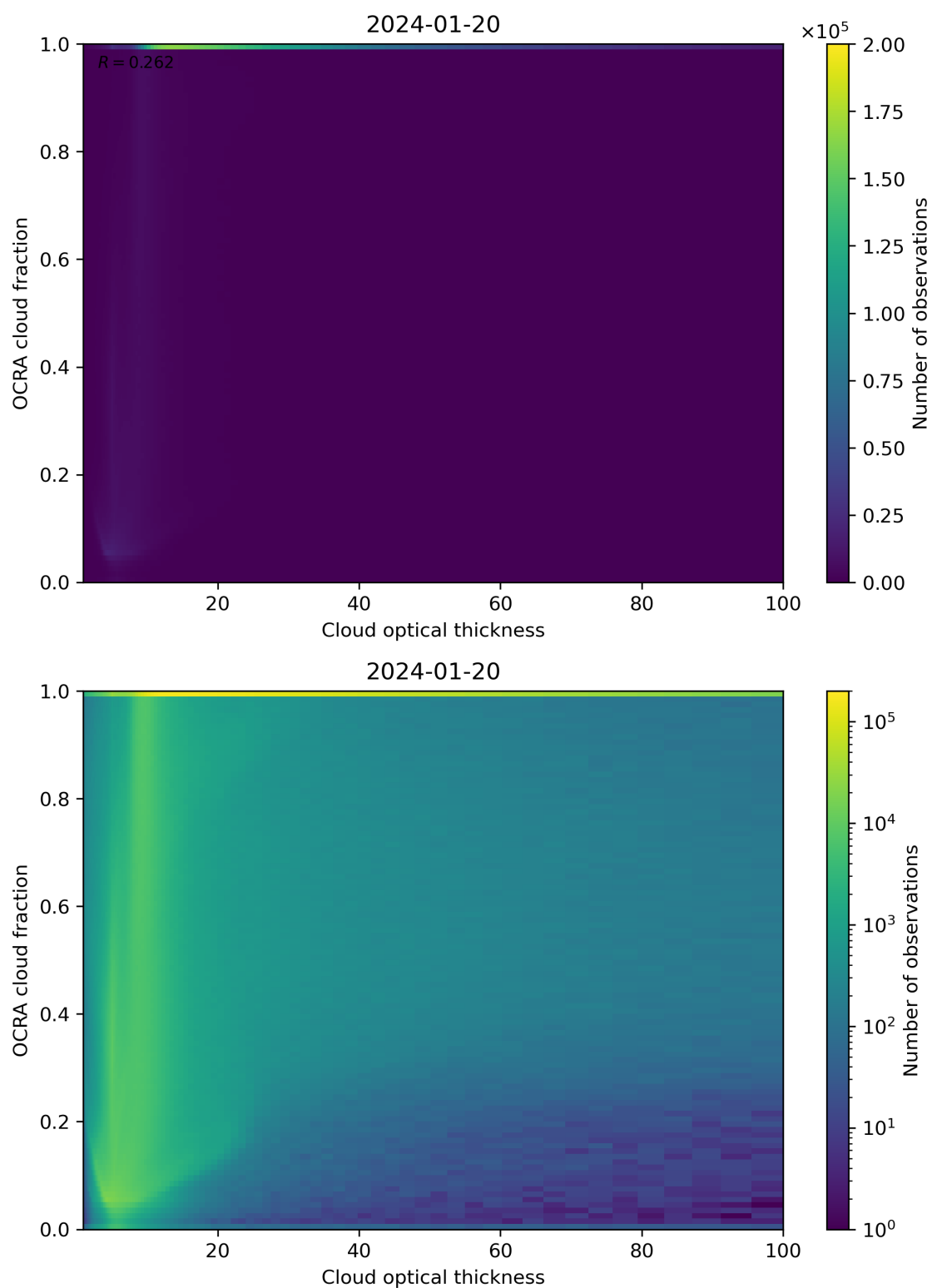
Figure 83: Scatter density plot of “Cloud optical thickness” against “OCRA cloud fraction” for 2024-01-19 to 2024-01-21.
