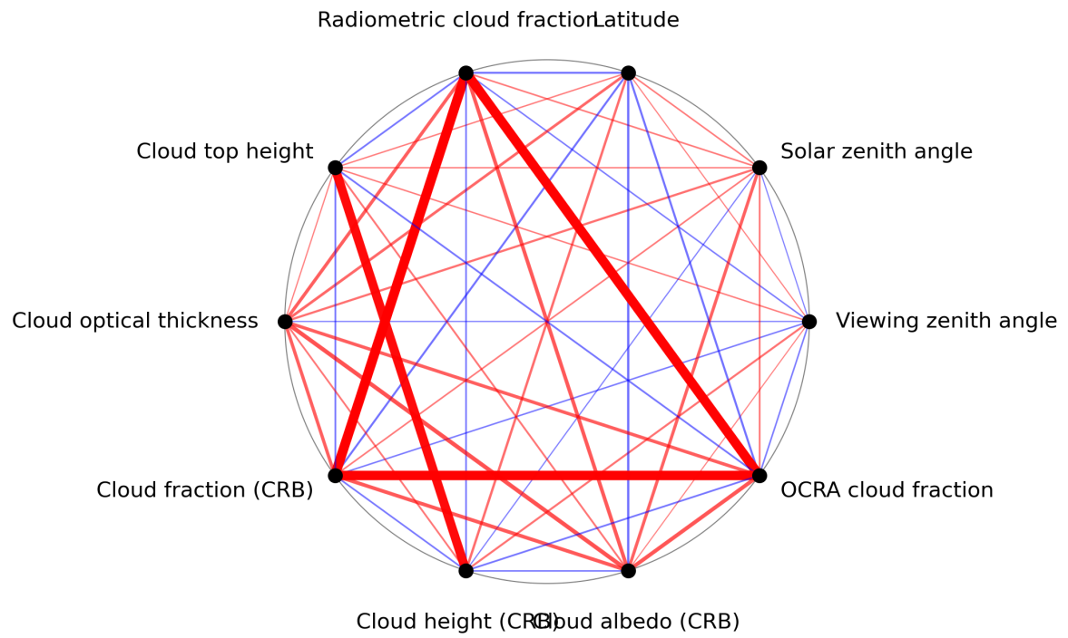
Figure 1: Map of correlation graph for 2024-01-19 to 2024-01-21.
