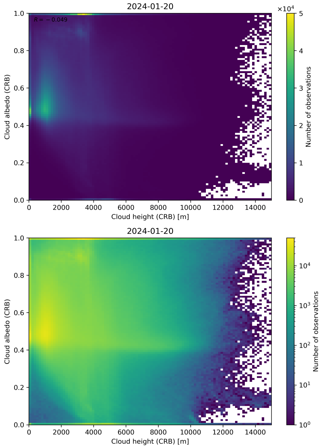
Figure 80: Scatter density plot of “Cloud height (CRB)” against “Cloud albedo (CRB)” for 2024-01-19 to 2024-01-21.
