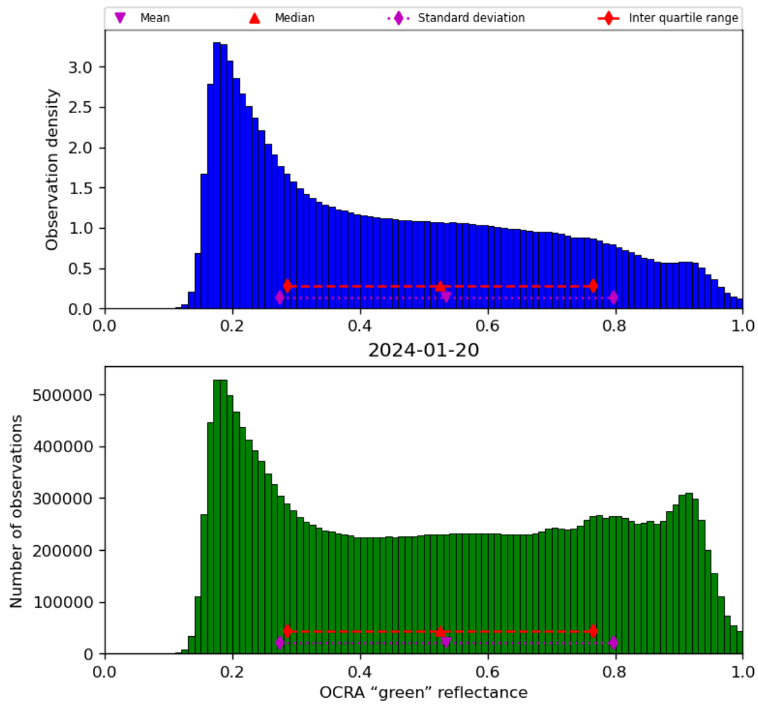
Figure 52: Histogram of “OCRA “green” reflectance” for 2024-01-19 to 2024-01-21
