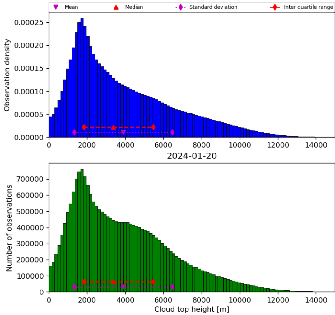
Figure 40: Histogram of “Cloud top height” for 2024-01-19 to 2024-01-21
