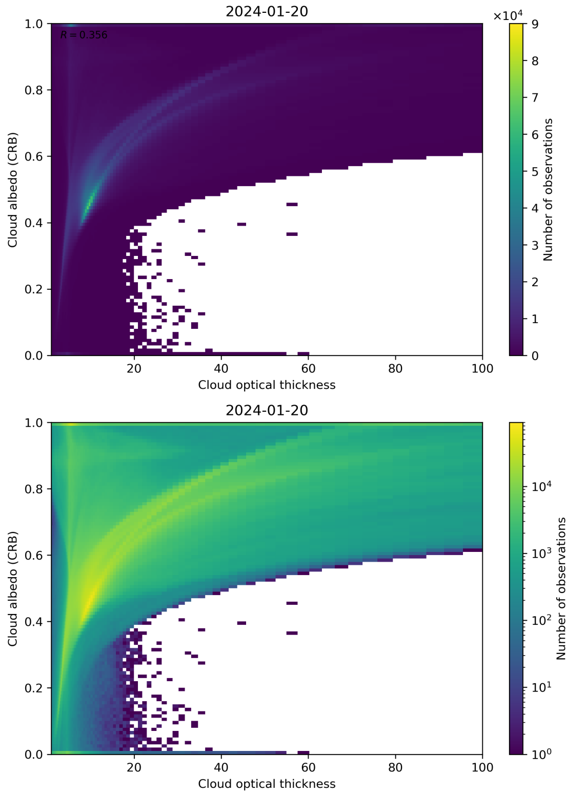
Figure 82: Scatter density plot of “Cloud optical thickness” against “Cloud albedo (CRB)” for 2024-01-19 to 2024-01-21.
