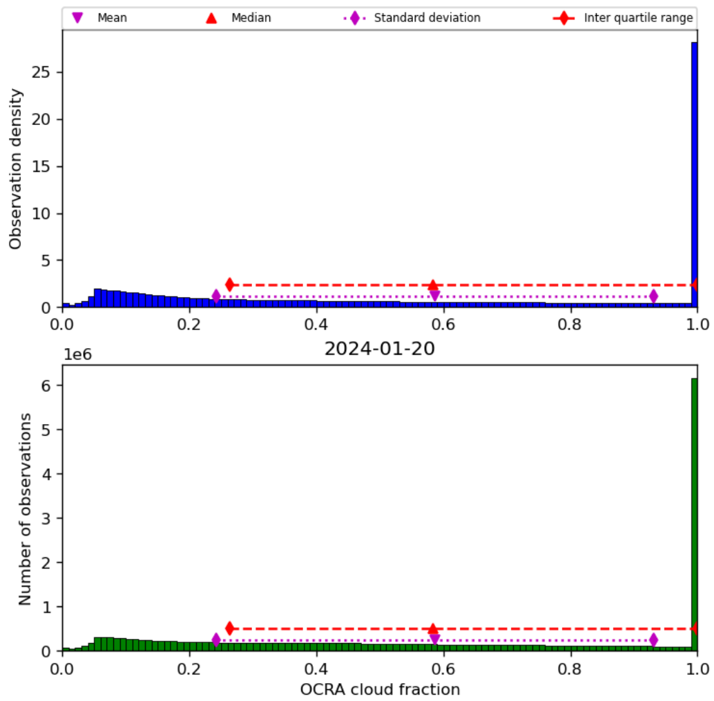
Figure 50: Histogram of “OCRA cloud fraction” for 2024-01-19 to 2024-01-21
