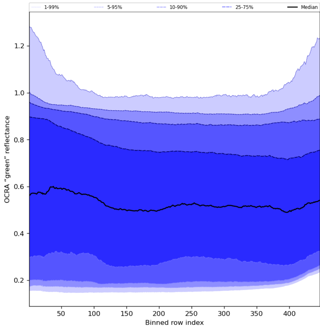
Figure 68: Along track statistics of "OCRA "green" reflectance" for 2024-01-19 to 2024-01-21
