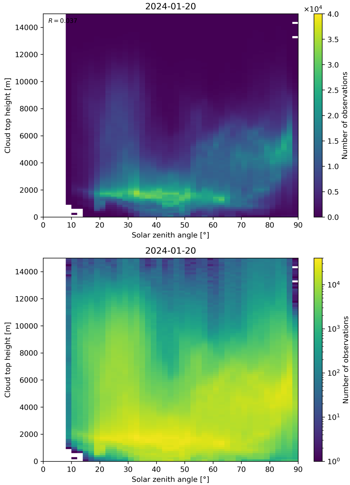
Figure 104: Scatter density plot of “Solar zenith angle” against “Cloud top height” for 2024-01-19 to 2024-01-21.
