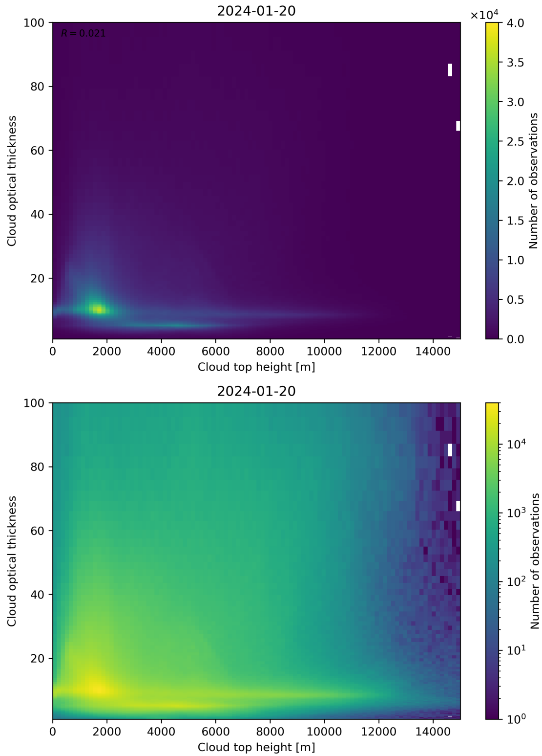
Figure 90: Scatter density plot of “Cloud top height” against “Cloud optical thickness” for 2024-01-19 to 2024-01-21.
