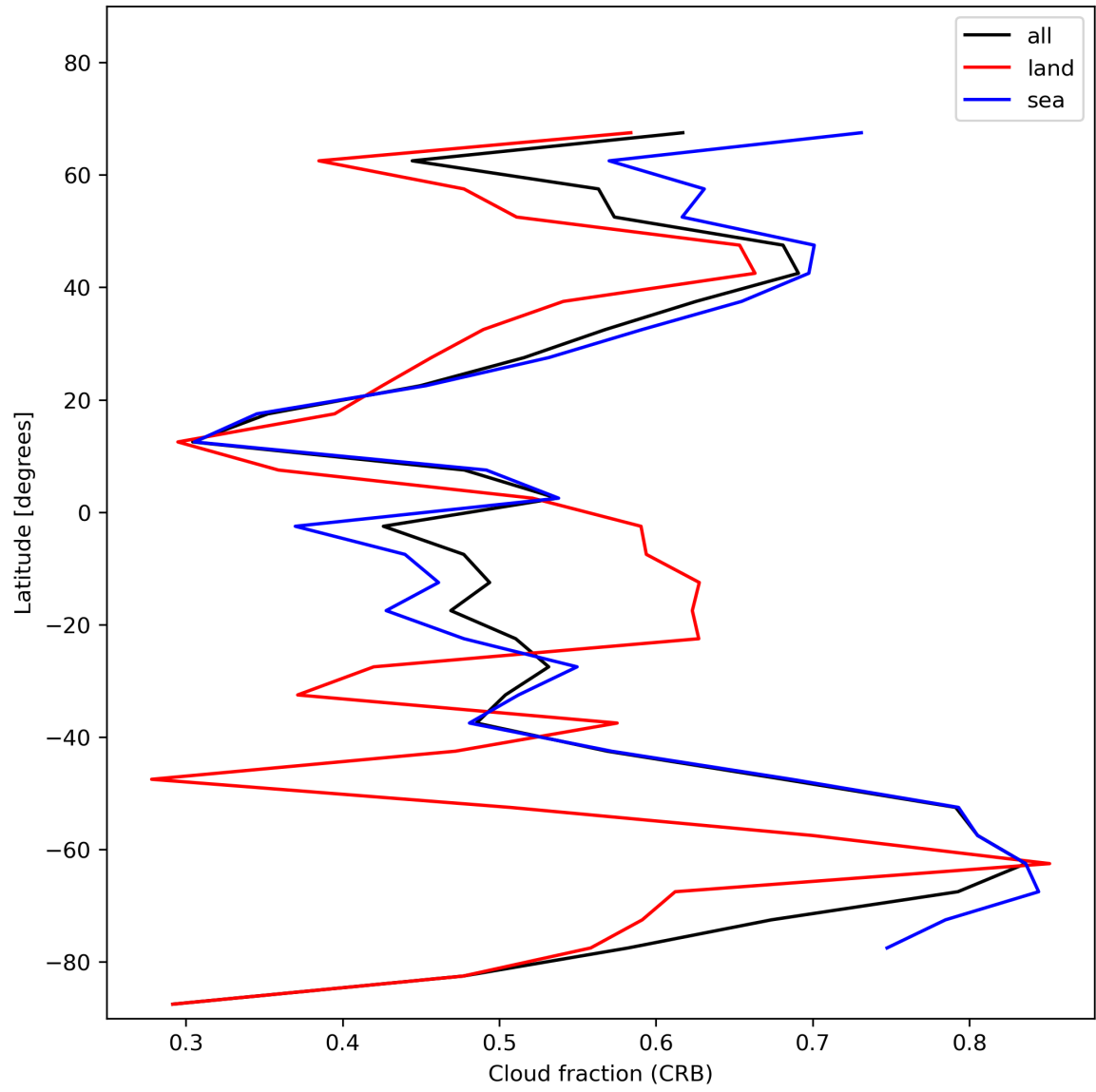
Figure 26: Zonal average of “Cloud fraction (CRB)” for 2024-01-19 to 2024-01-21.
