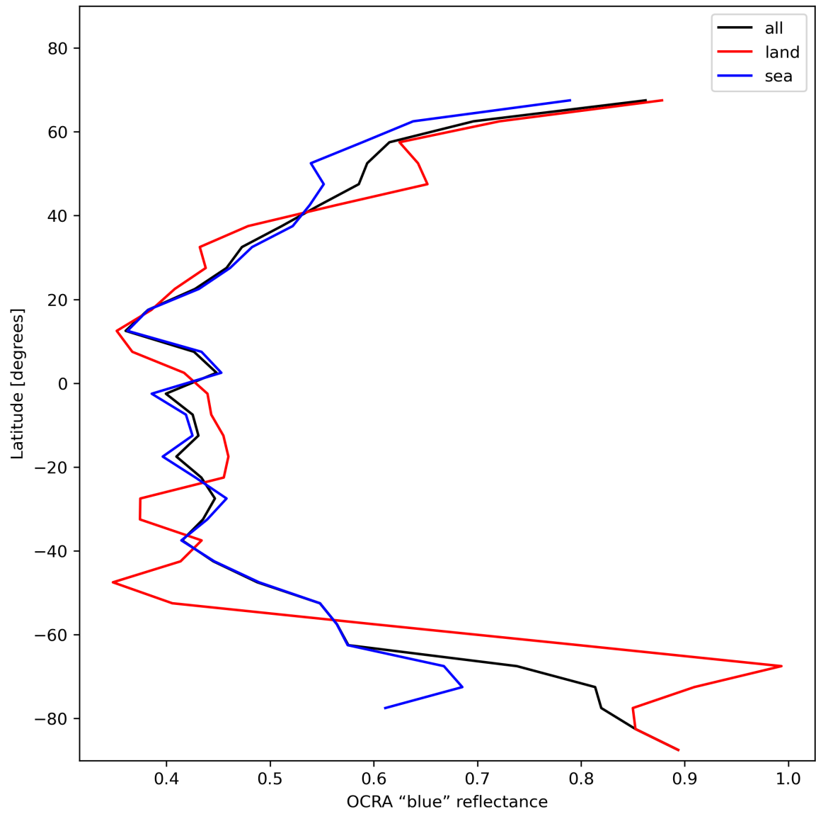
Figure 35: Zonal average of “OCRA “blue” reflectance” for 2024-01-19 to 2024-01-21.
