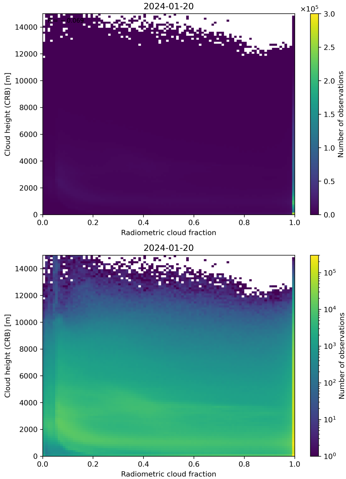
Figure 74: Scatter density plot of “Radiometric cloud fraction” against “Cloud height (CRB)” for 2024-01-19 to 2024-01-21.
