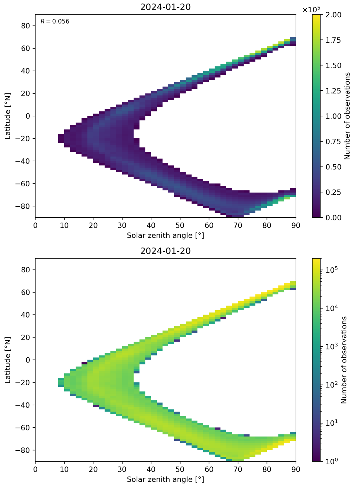
Figure 105: Scatter density plot of “Solar zenith angle” against “Latitude” for 2024-01-19 to 2024-01-21.
