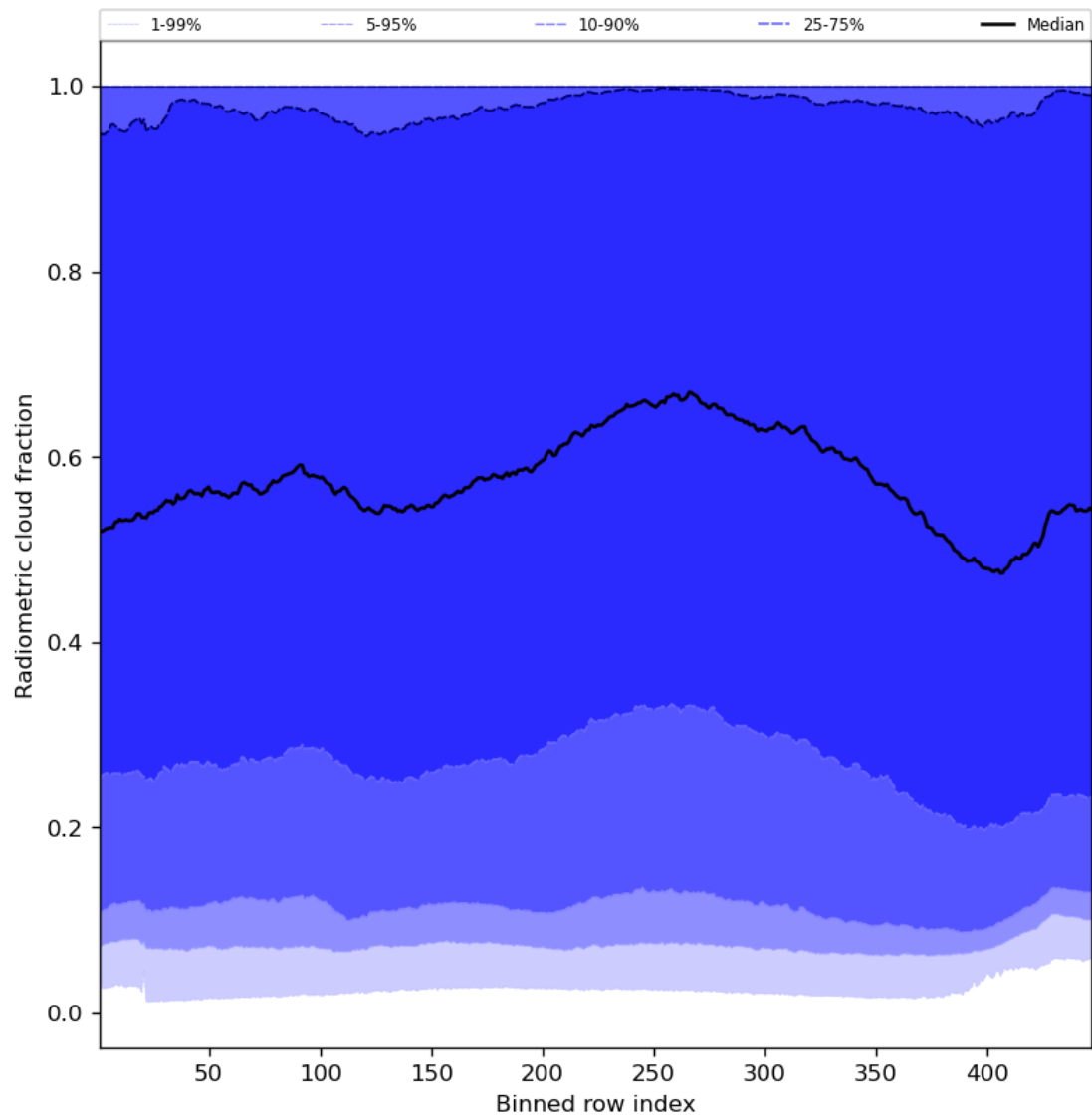
Figure 55: Along track statistics of “Radiometric cloud fraction” for 2024-01-19 to 2024-01-21
