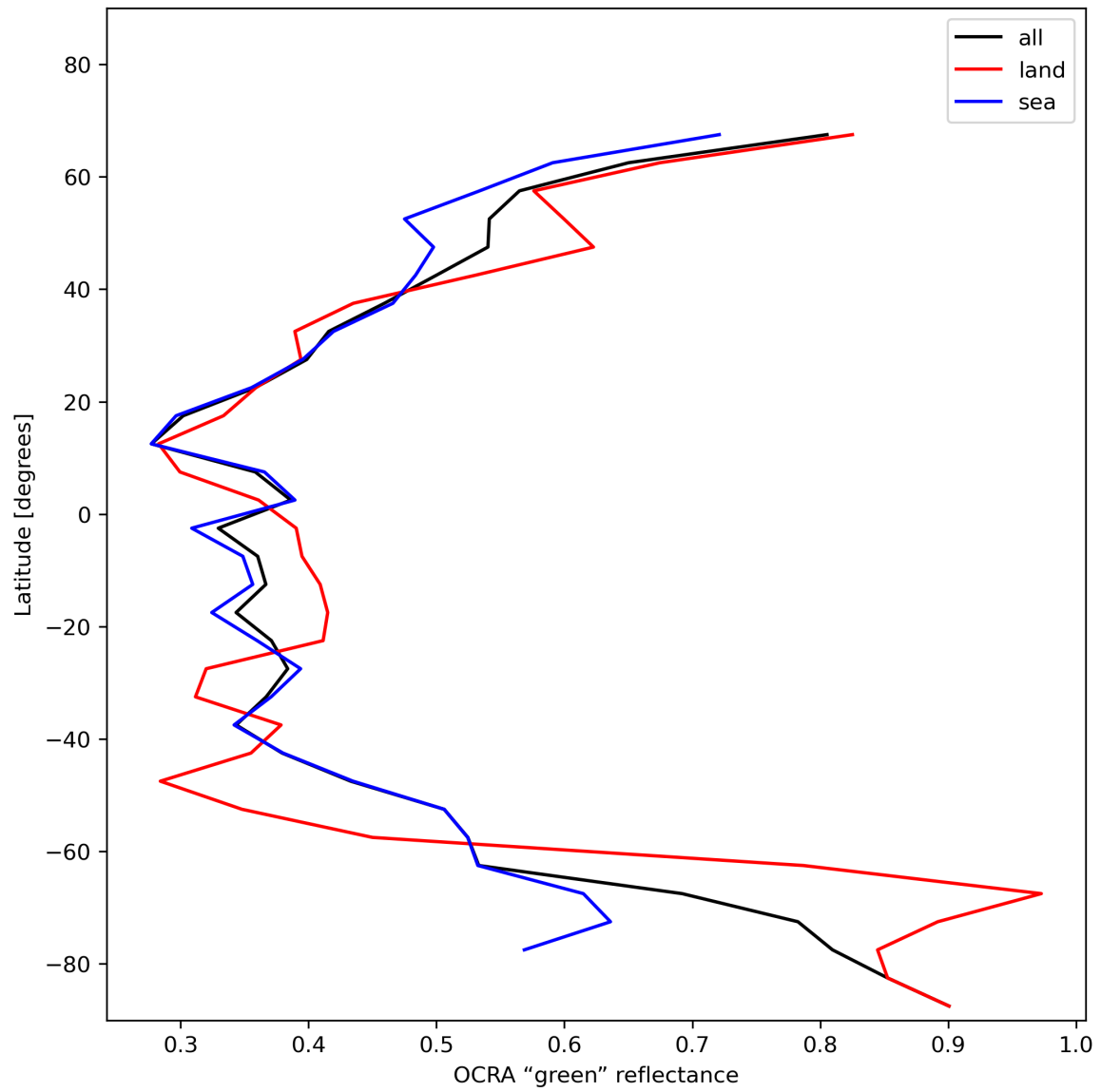
Figure 36: Zonal average of “OCRA “green” reflectance” for 2024-01-19 to 2024-01-21.
