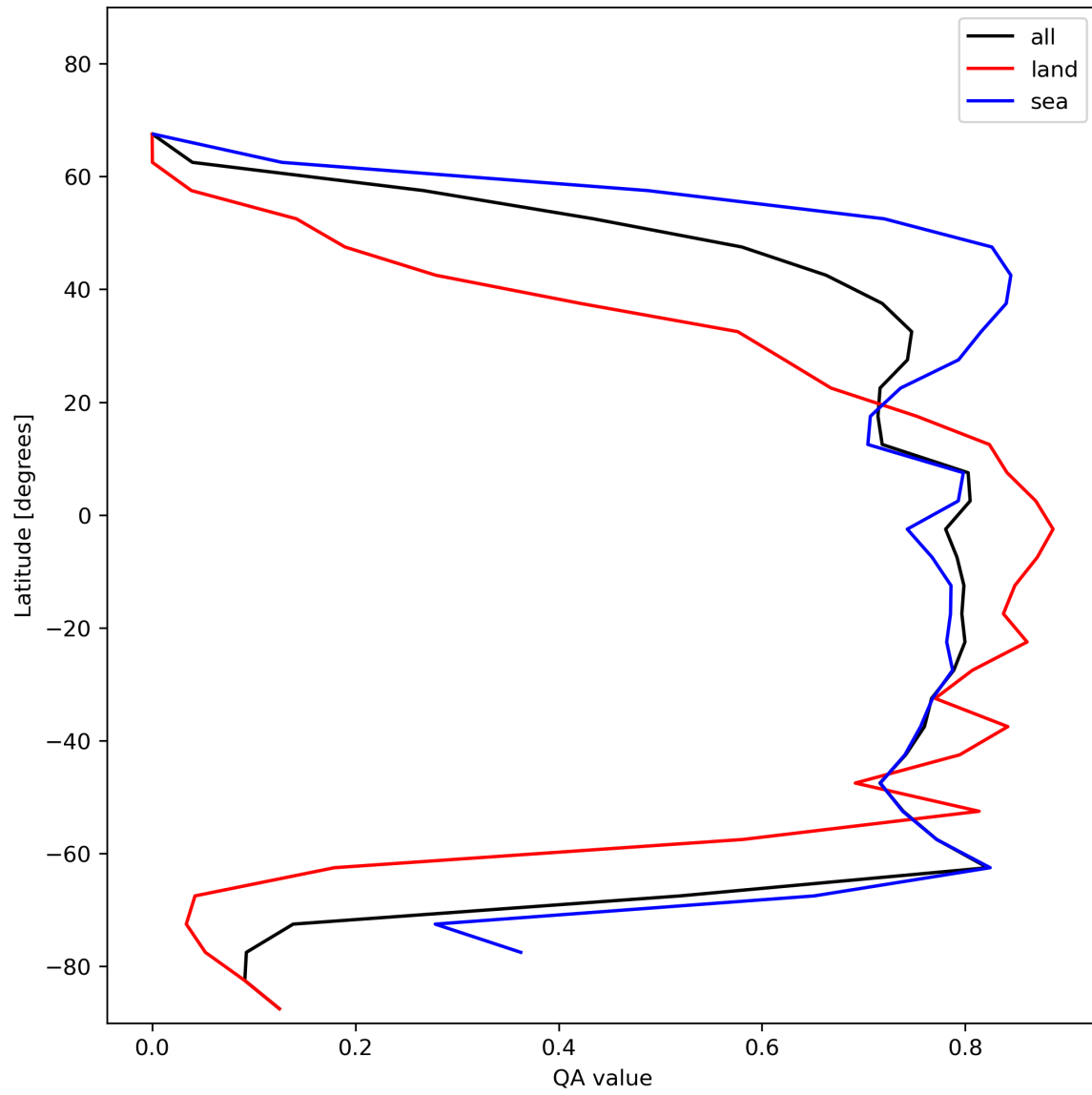
Figure 22: Zonal average of “QA value” for 2024-01-19 to 2024-01-21.
