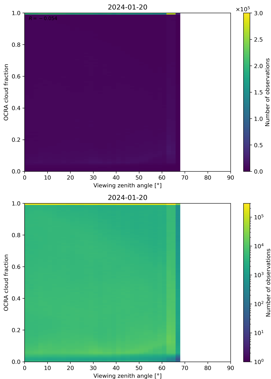
Figure 108: Scatter density plot of “Viewing zenith angle” against “OCRA cloud fraction” for 2024-01-19 to 2024-01-21.
