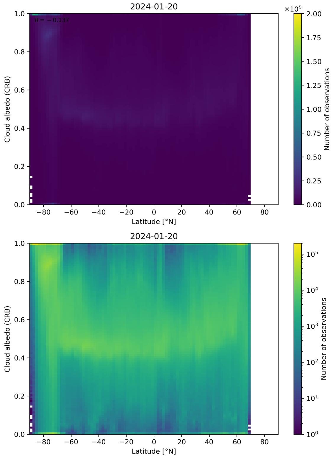
Figure 91: Scatter density plot of “Latitude” against “Cloud albedo (CRB)” for 2024-01-19 to 2024-01-21.
