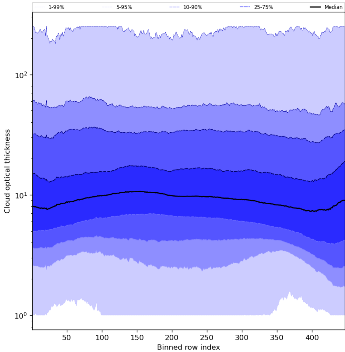
Figure 57: Along track statistics of “Cloud optical thickness” for 2024-01-19 to 2024-01-21
