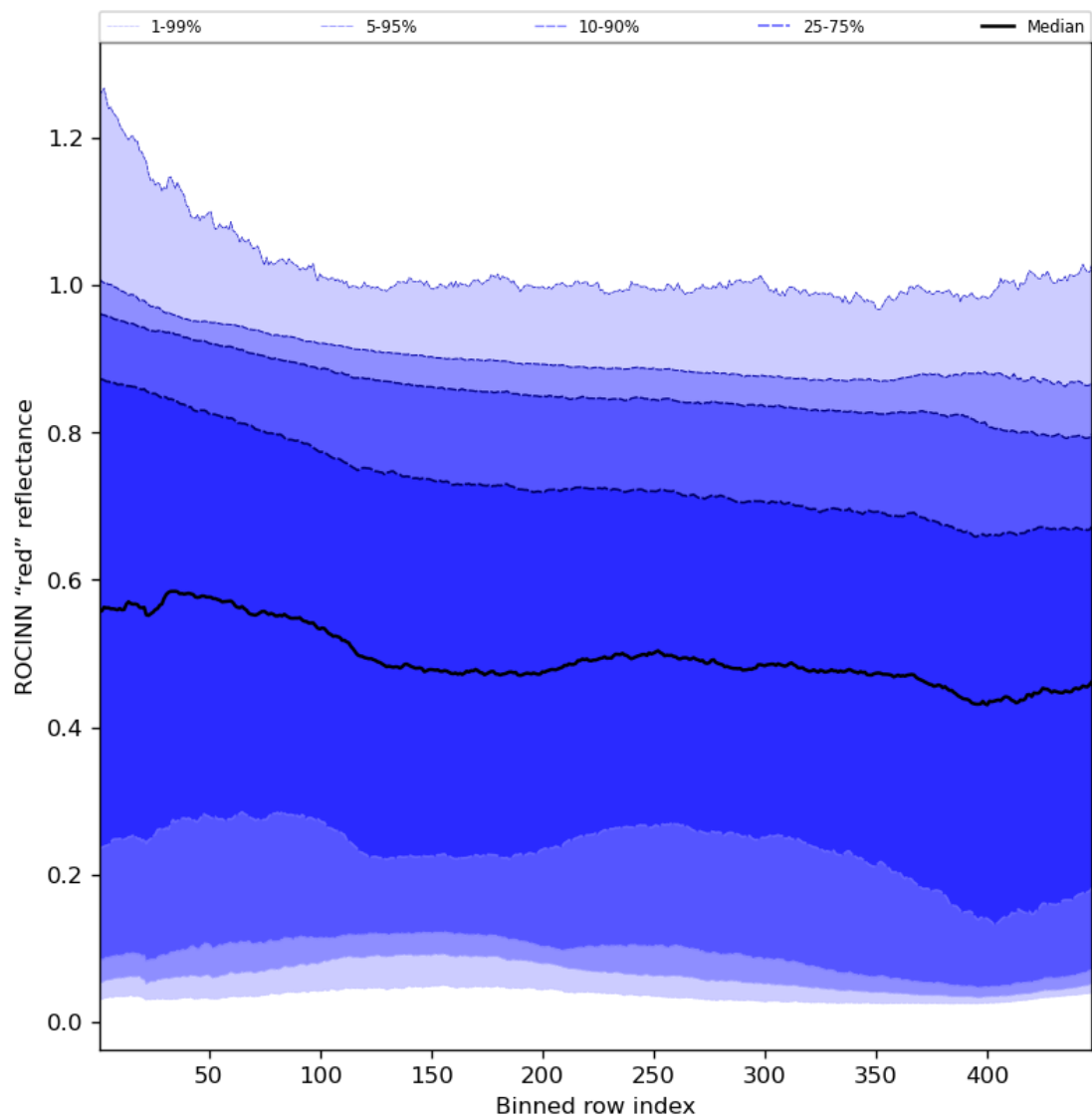
Figure 69: Along track statistics of “ROCINN “red” reflectance” for 2024-01-19 to 2024-01-21
