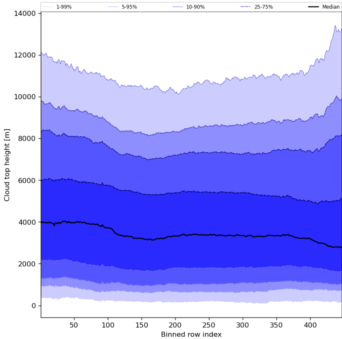
Figure 56: Along track statistics of “Cloud top height” for 2024-01-19 to 2024-01-21
