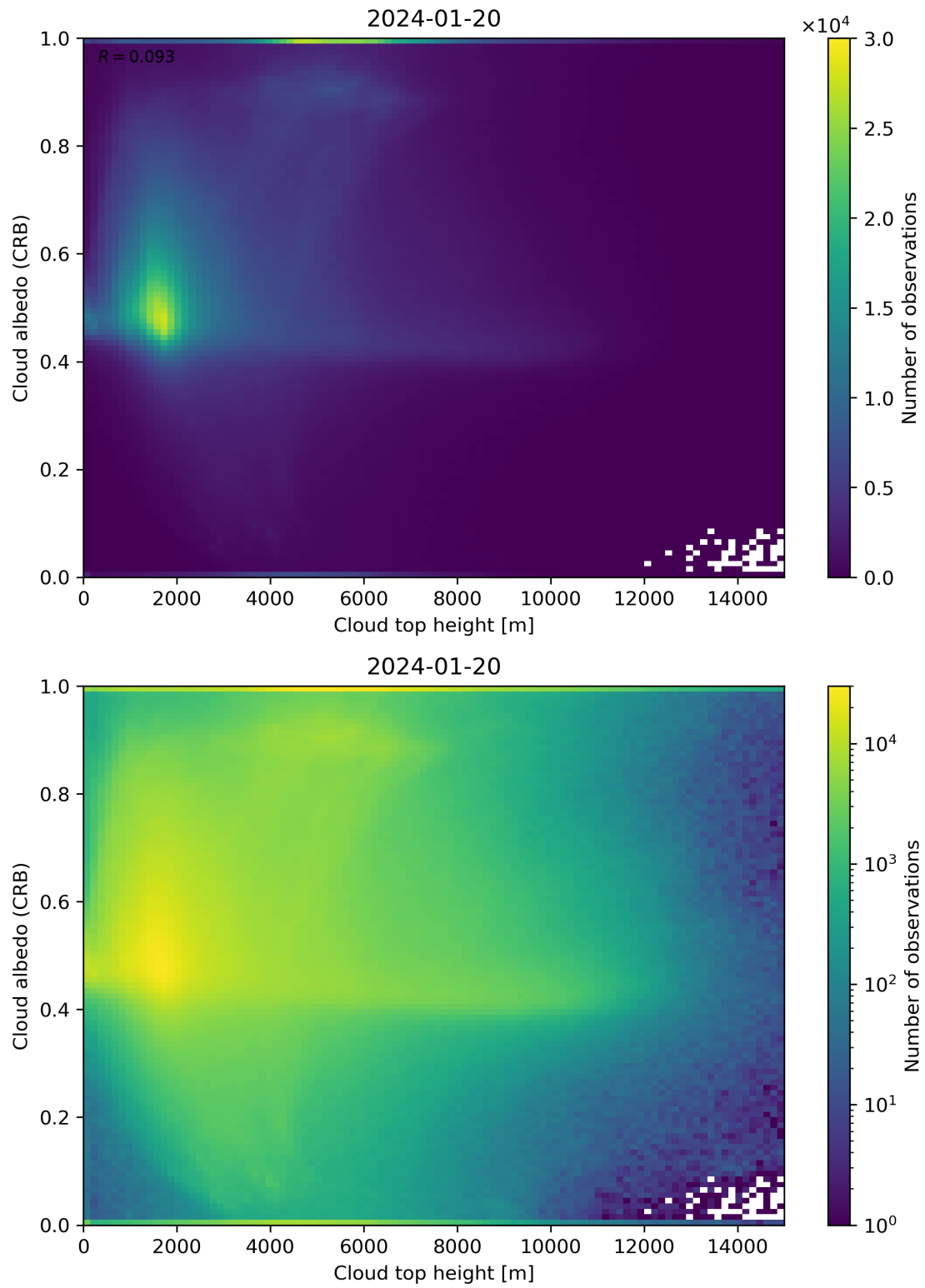
Figure 86: Scatter density plot of “Cloud top height” against “Cloud albedo (CRB)” for 2024-01-19 to 2024-01-21.
