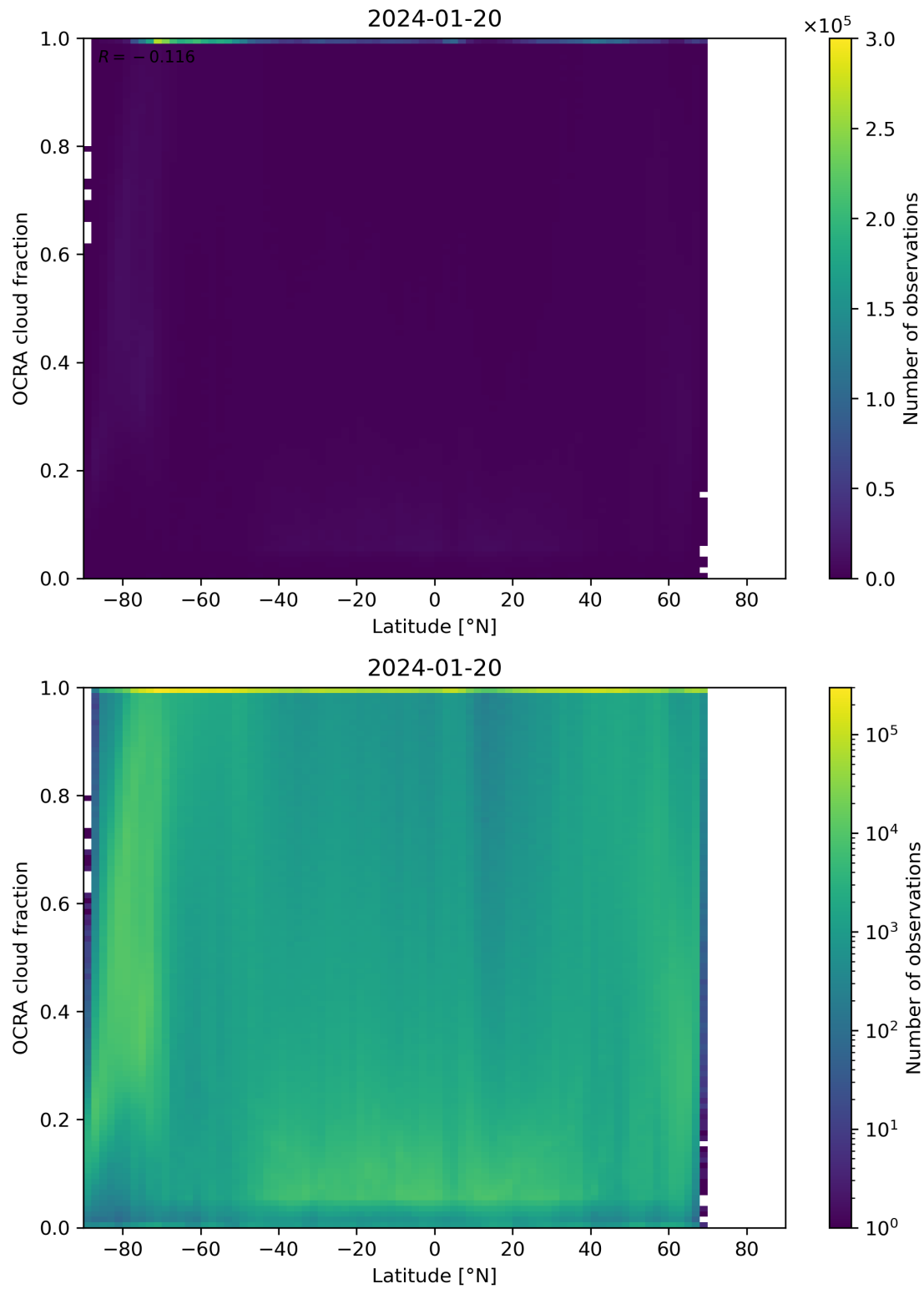
Figure 93: Scatter density plot of “Latitude” against “OCRA cloud fraction” for 2024-01-19 to 2024-01-21.
