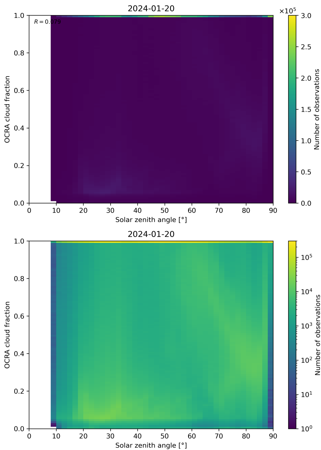
Figure 100: Scatter density plot of “Solar zenith angle” against “OCRA cloud fraction” for 2024-01-19 to 2024-01-21.
