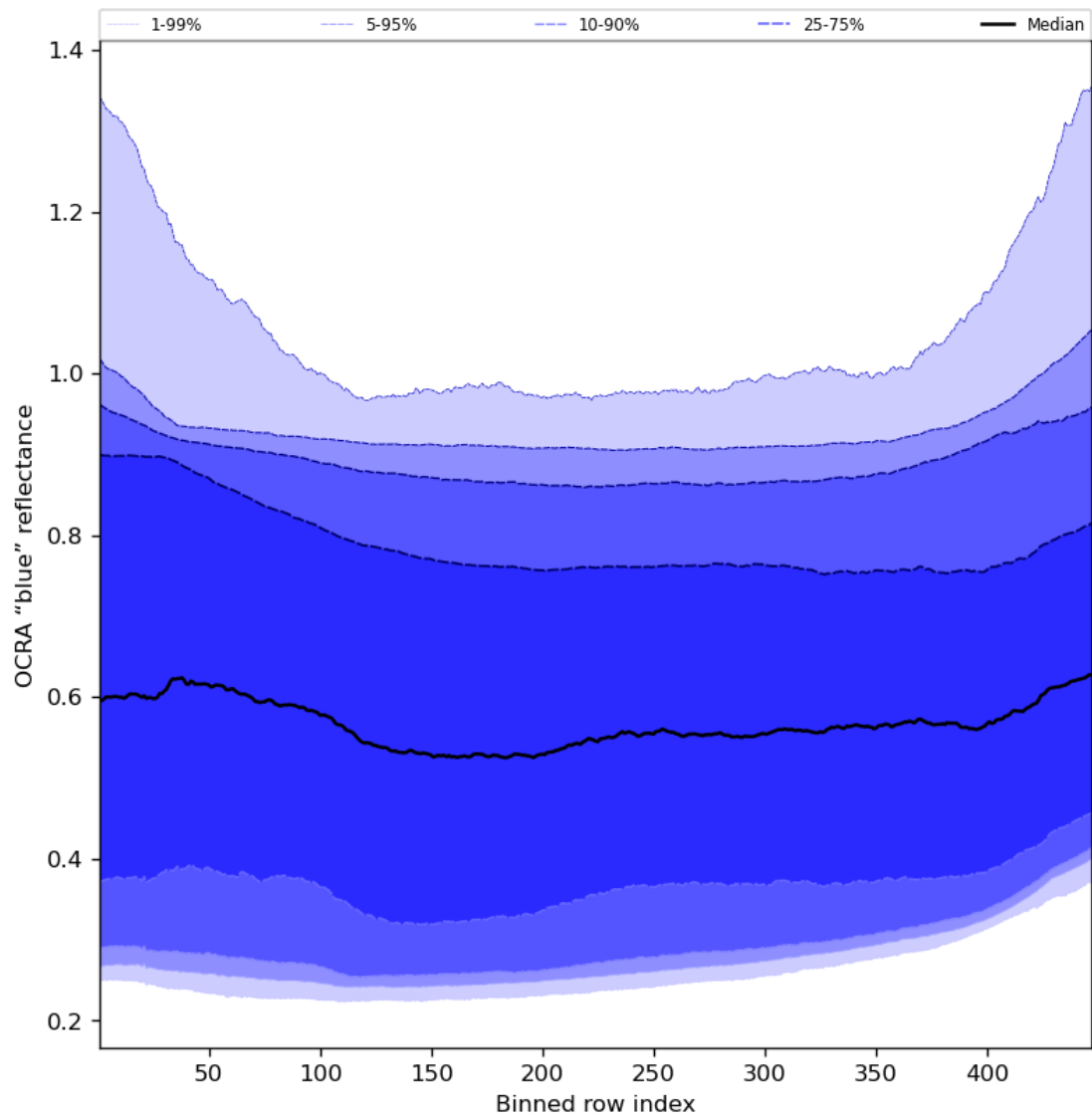
Figure 67: Along track statistics of “OCRA “blue” reflectance” for 2024-01-19 to 2024-01-21
