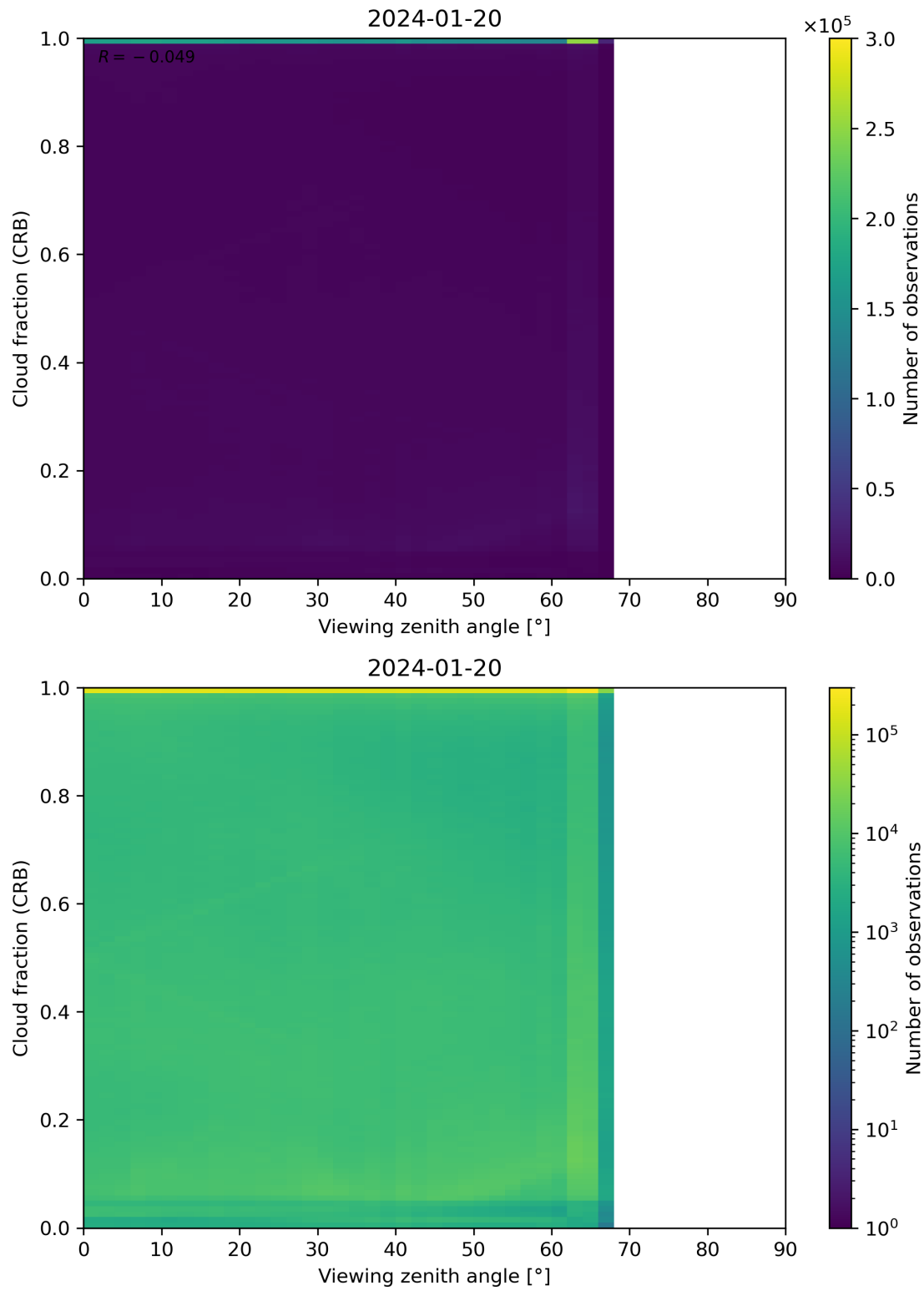
Figure 109: Scatter density plot of “Viewing zenith angle” against “Cloud fraction (CRB)” for 2024-01-19 to 2024-01-21.
