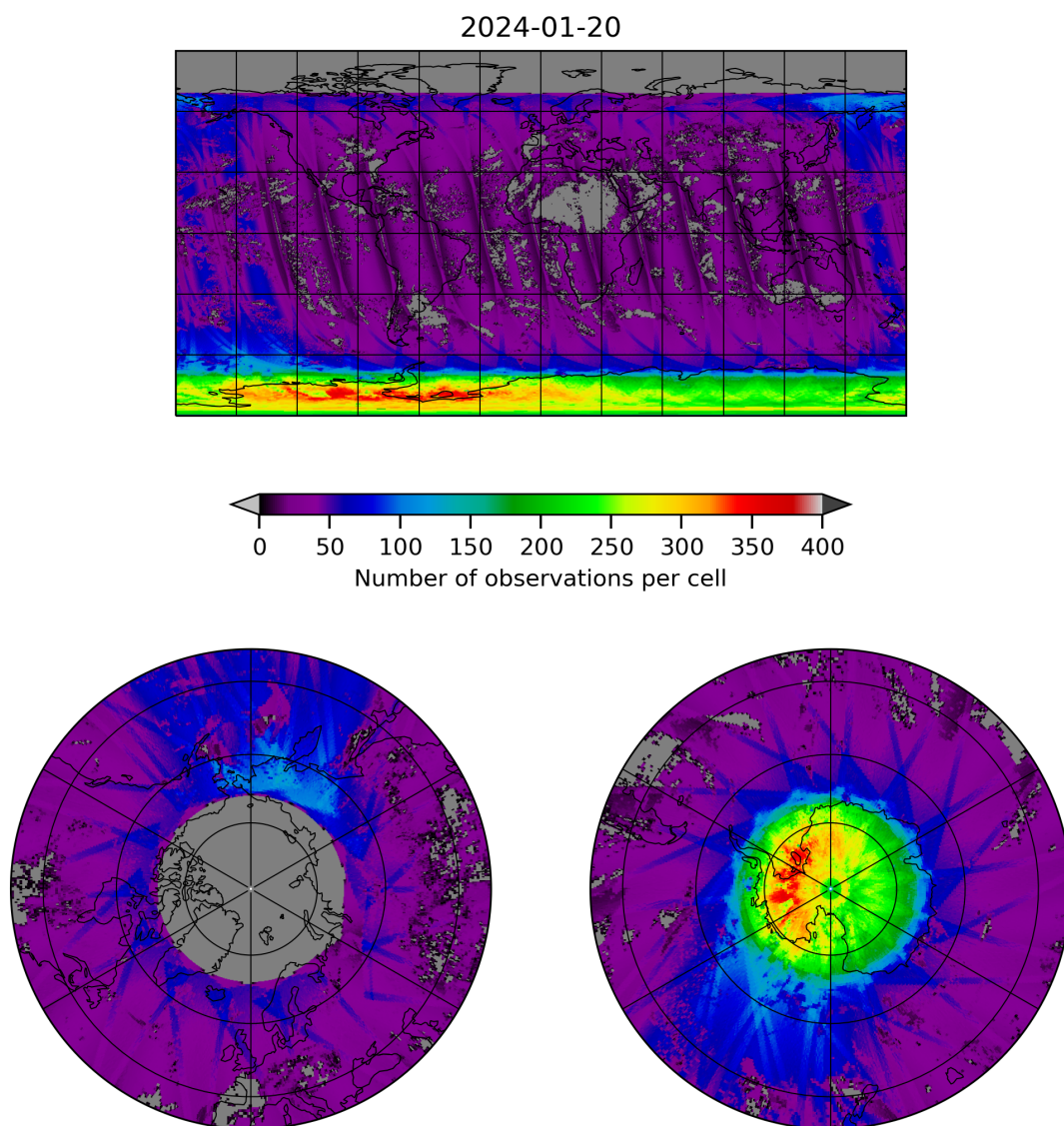
Figure 21: Map of the number of observations for 2024-01-19 to 2024-01-21
