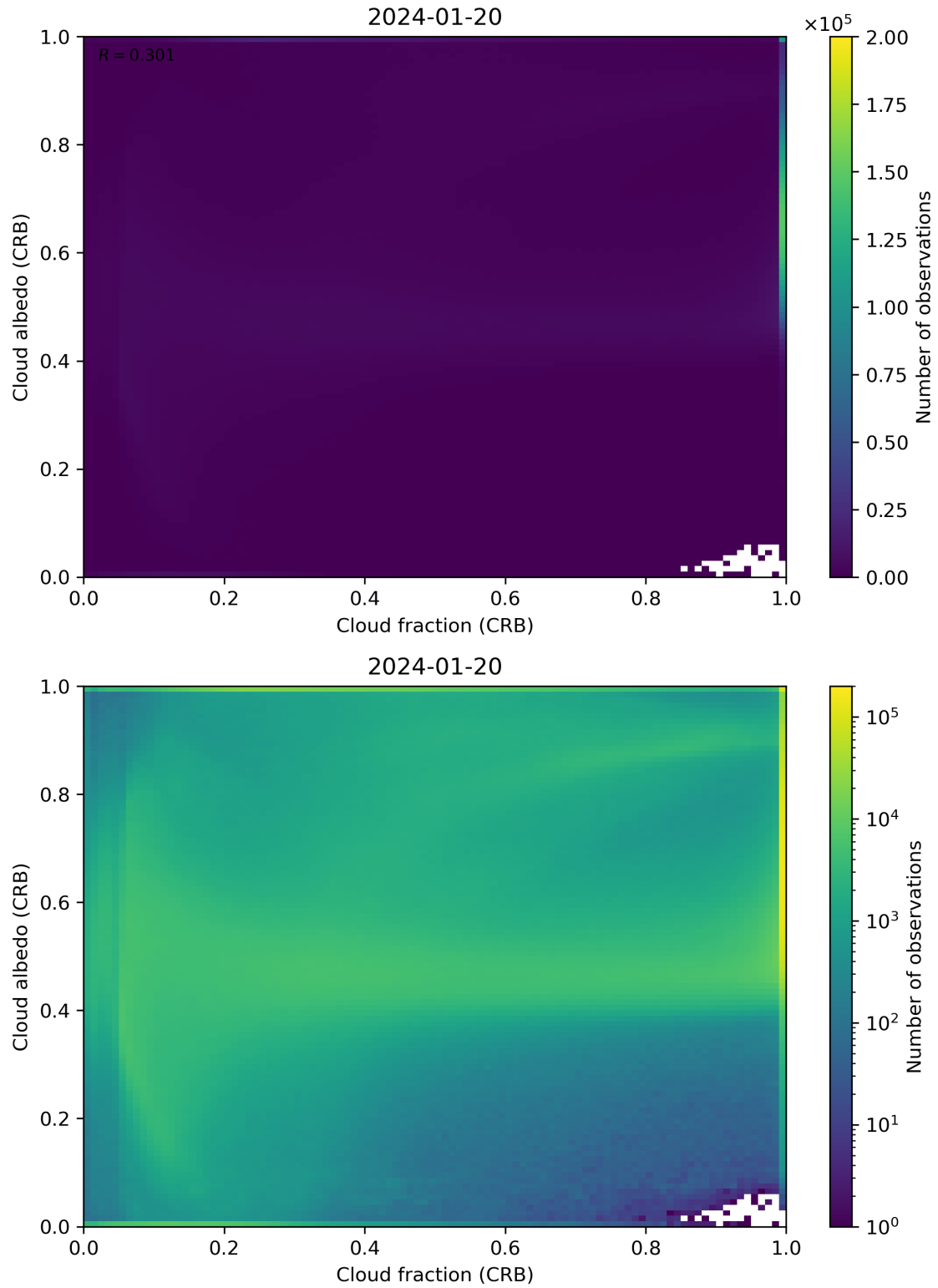
Figure 77: Scatter density plot of “Cloud fraction (CRB)” against “Cloud albedo (CRB)” for 2024-01-19 to 2024-01-21.
