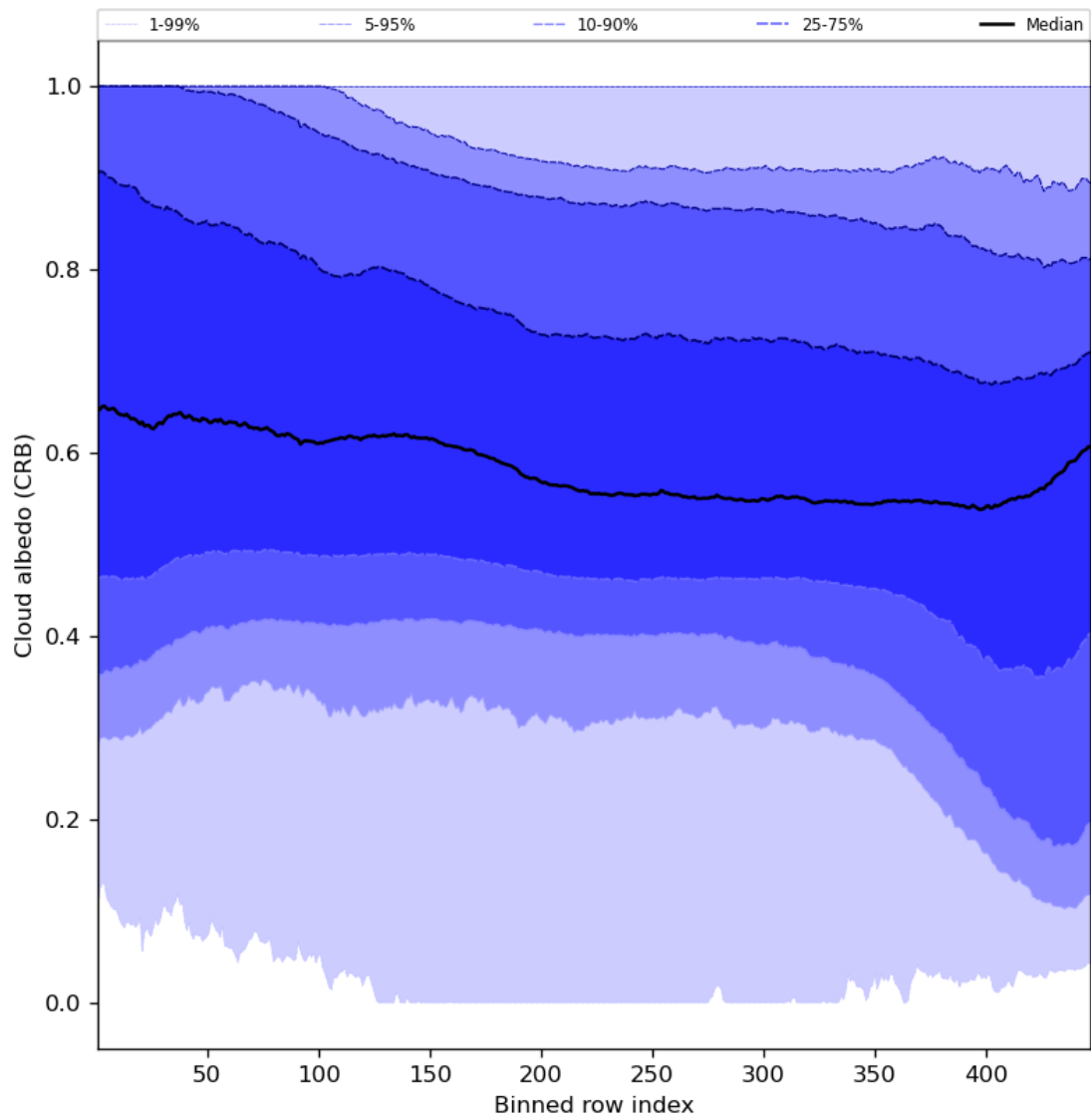
Figure 60: Along track statistics of “Cloud albedo (CRB)” for 2024-01-19 to 2024-01-21
