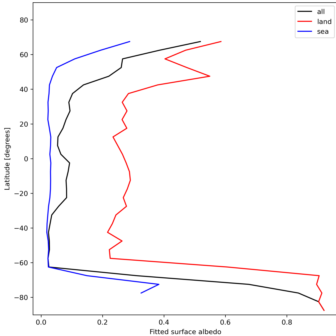
Figure 29: Zonal average of “Fitted surface albedo” for 2024-01-19 to 2024-01-21.
