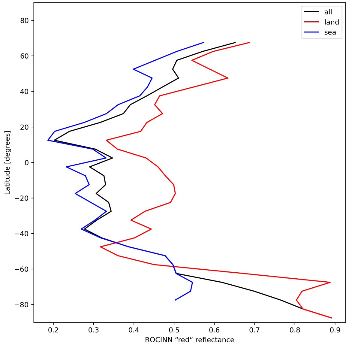
Figure 37: Zonal average of “ROCINN “red” reflectance” for 2024-01-19 to 2024-01-21.
