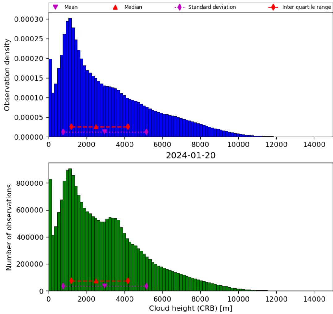
Figure 43: Histogram of “Cloud height (CRB)” for 2024-01-19 to 2024-01-21
