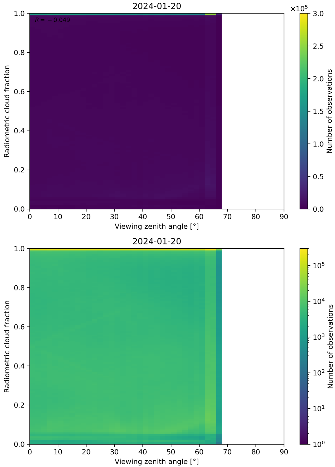
Figure 107: Scatter density plot of “Viewing zenith angle” against “Radiometric cloud fraction” for 2024-01-19 to 2024-01-21.
