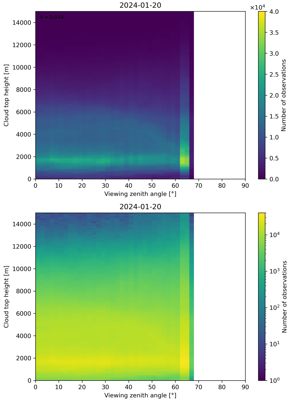
Figure 112: Scatter density plot of “Viewing zenith angle” against “Cloud top height” for 2024-01-19 to 2024-01-21.
