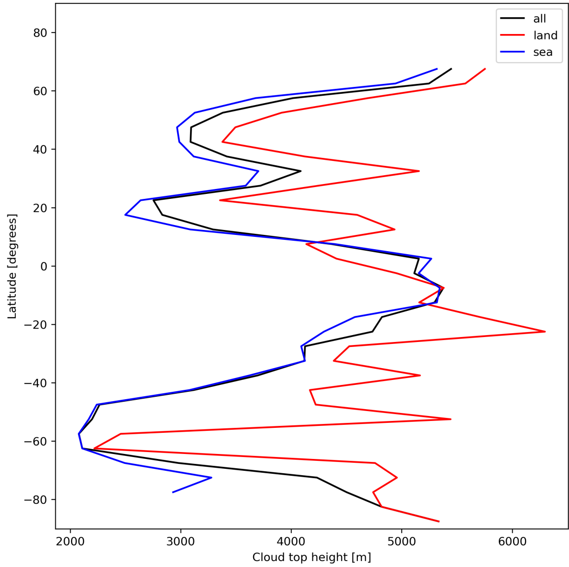
Figure 24: Zonal average of “Cloud top height” for 2024-01-19 to 2024-01-21.
