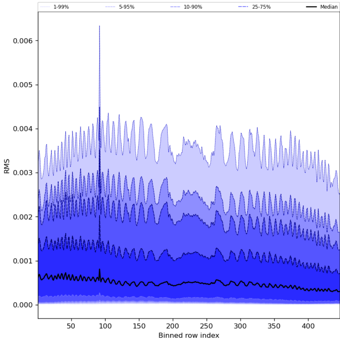
Figure 63: Along track statistics of “RMS” for 2024-01-19 to 2024-01-21
