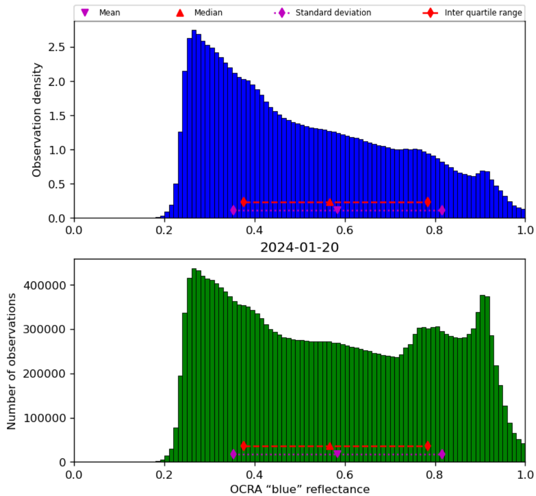
Figure 51: Histogram of “OCRA “blue” reflectance” for 2024-01-19 to 2024-01-21
