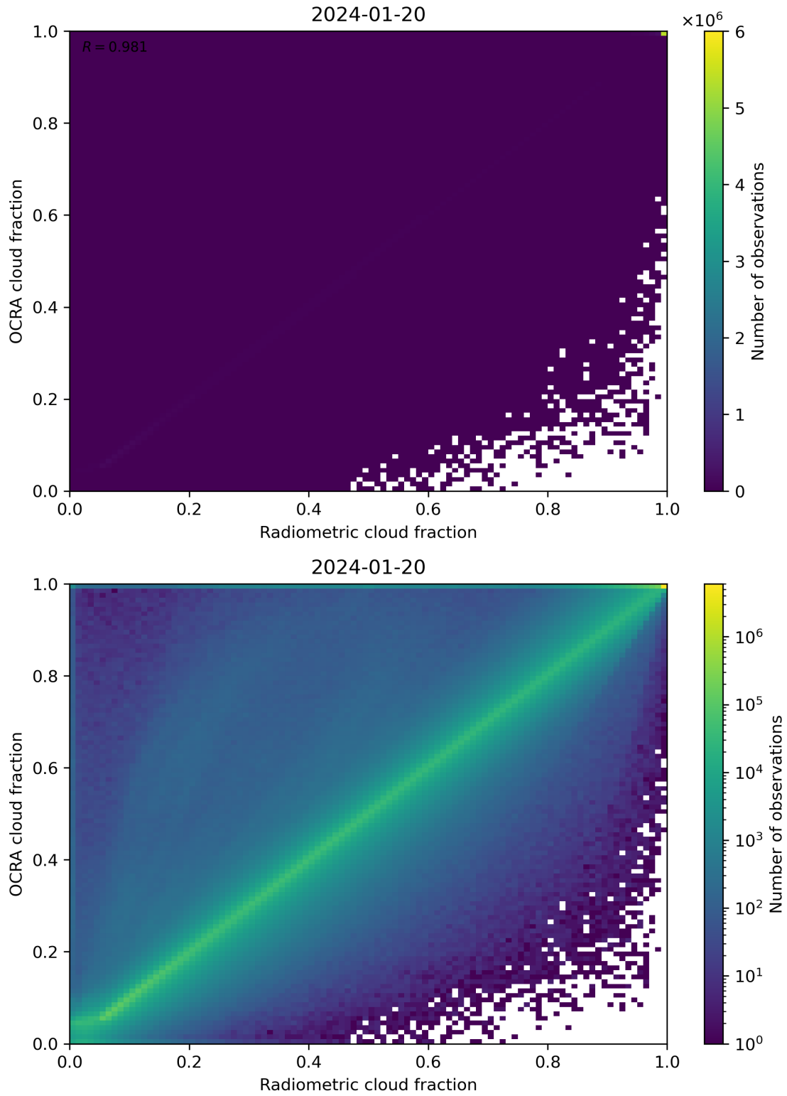
Figure 72: Scatter density plot of “Radiometric cloud fraction” against “OCRA cloud fraction” for 2024-01-19 to 2024-01-21.
