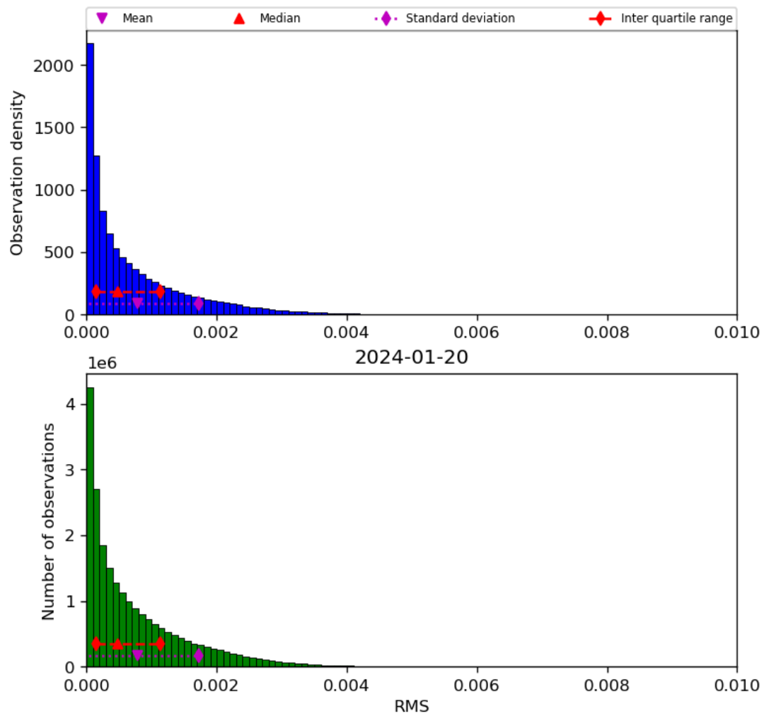
Figure 47: Histogram of “RMS” for 2024-01-19 to 2024-01-21
