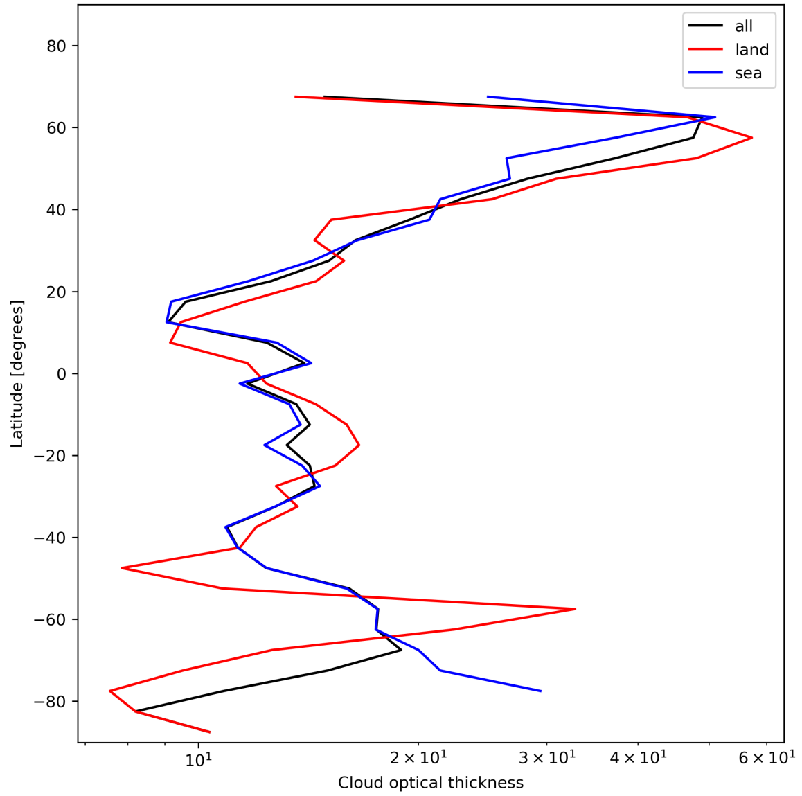
Figure 25: Zonal average of “Cloud optical thickness” for 2024-01-19 to 2024-01-21.
