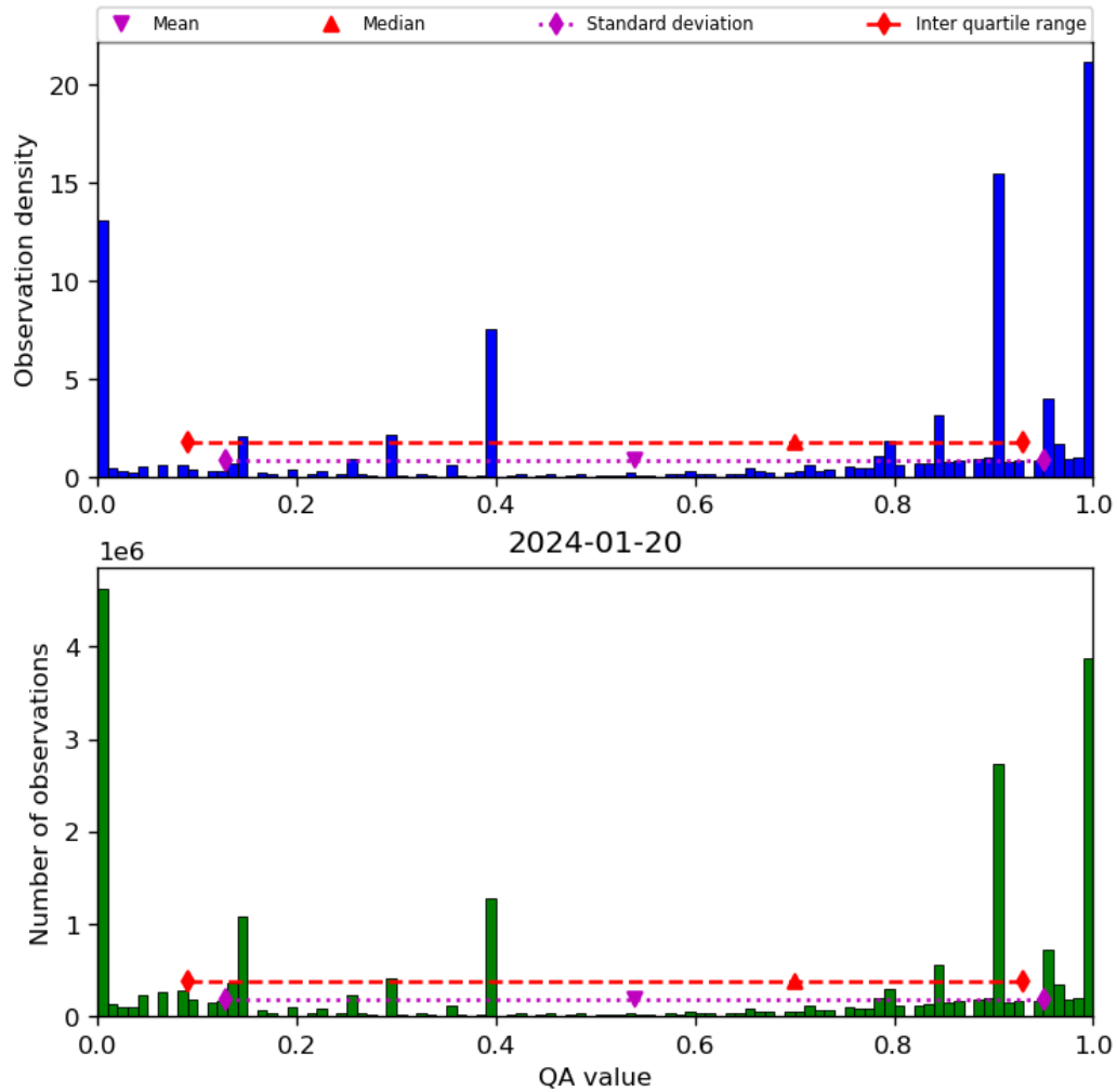
Figure 38: Histogram of “QA value” for 2024-01-19 to 2024-01-21
