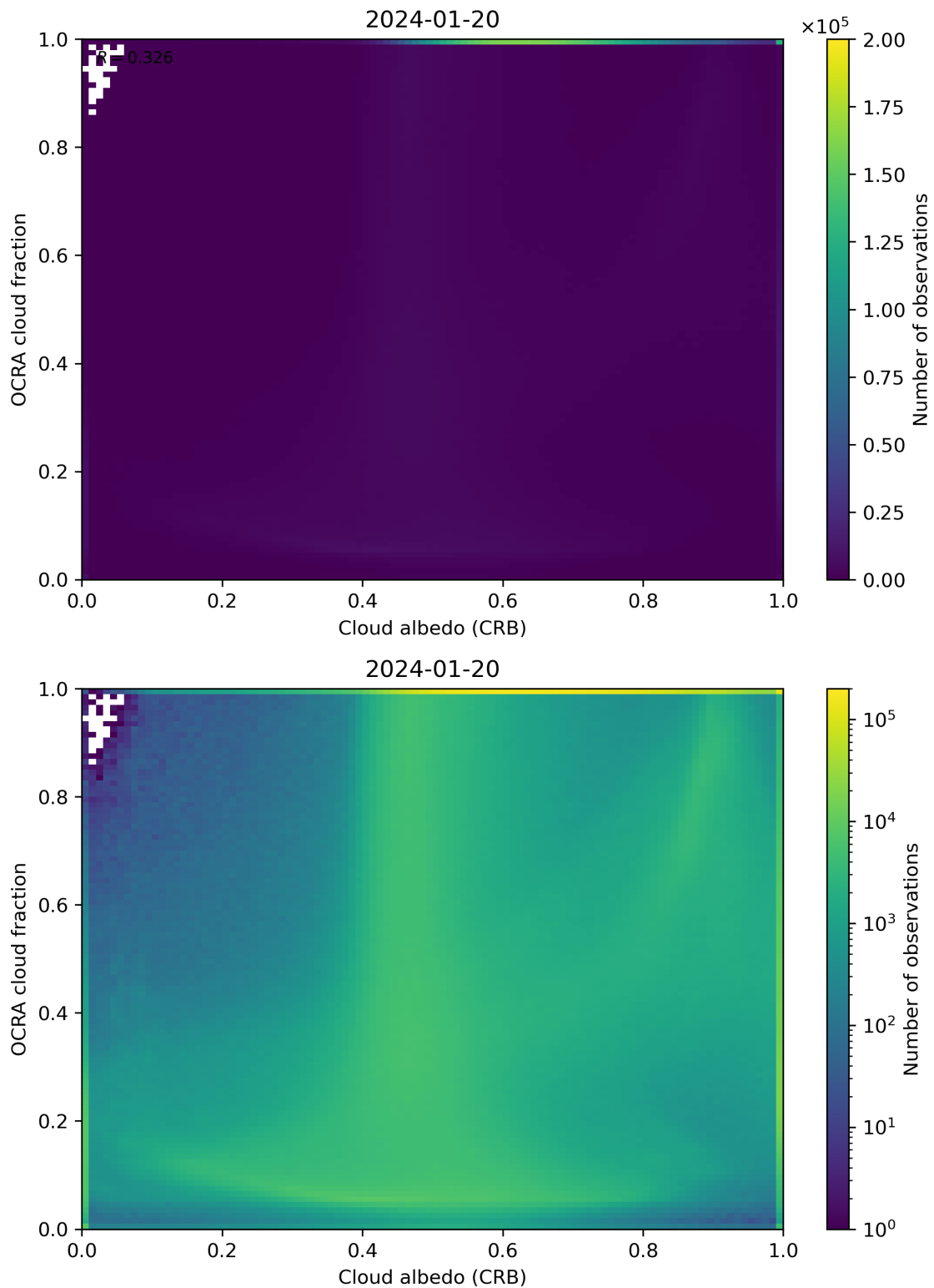
Figure 70: Scatter density plot of “Cloud albedo (CRB)” against “OCRA cloud fraction” for 2024-01-19 to 2024-01-21.
