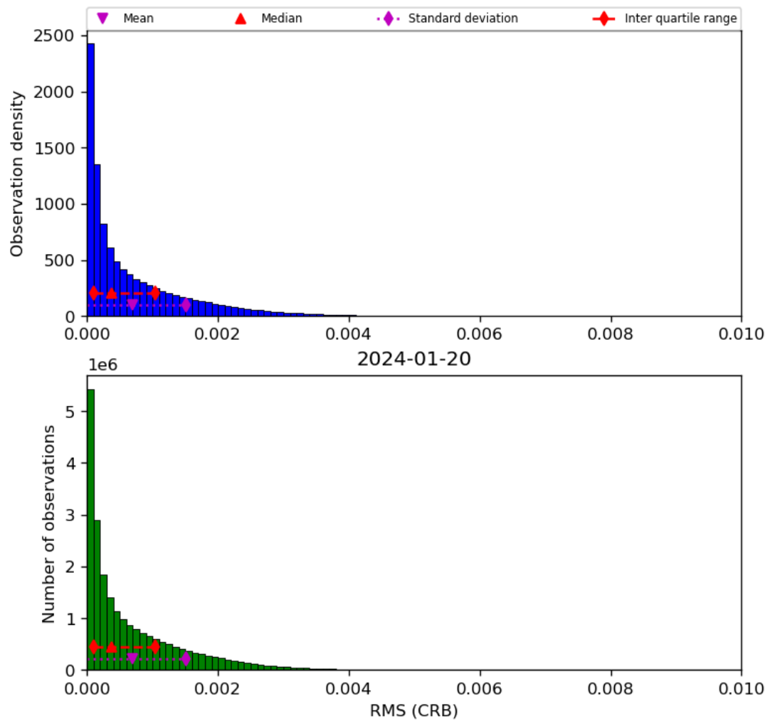
Figure 48: Histogram of “RMS (CRB)” for 2024-01-19 to 2024-01-21
