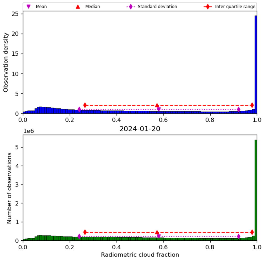
Figure 39: Histogram of “Radiometric cloud fraction” for 2024-01-19 to 2024-01-21
