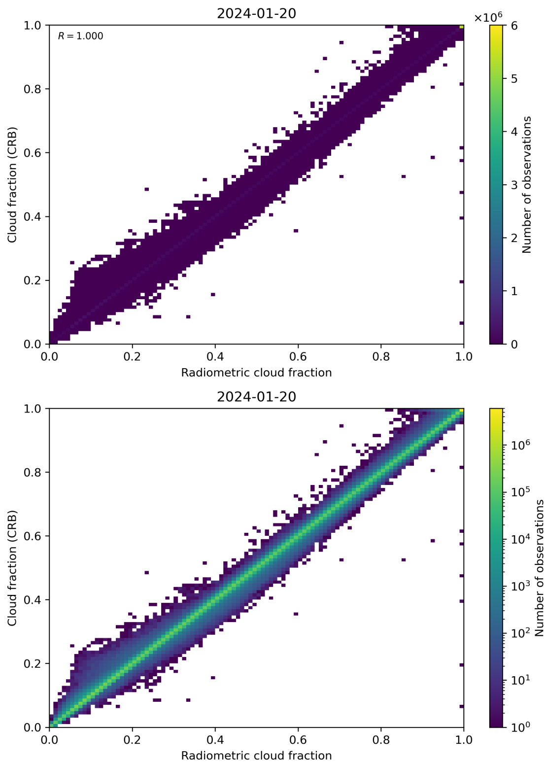
Figure 73: Scatter density plot of “Radiometric cloud fraction” against “Cloud fraction (CRB)” for 2024-01-19 to 2024-01-21.
