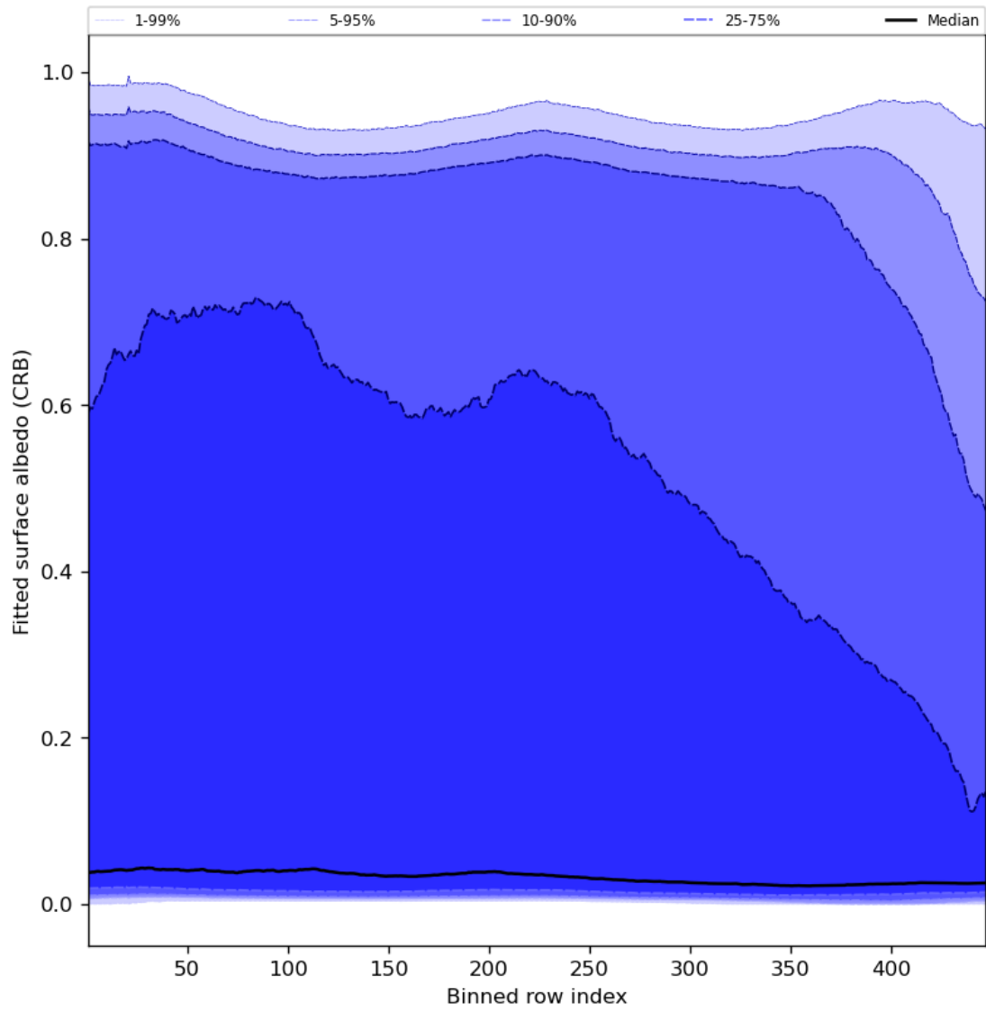
Figure 62: Along track statistics of “Fitted surface albedo (CRB)” for 2024-01-19 to 2024-01-21
