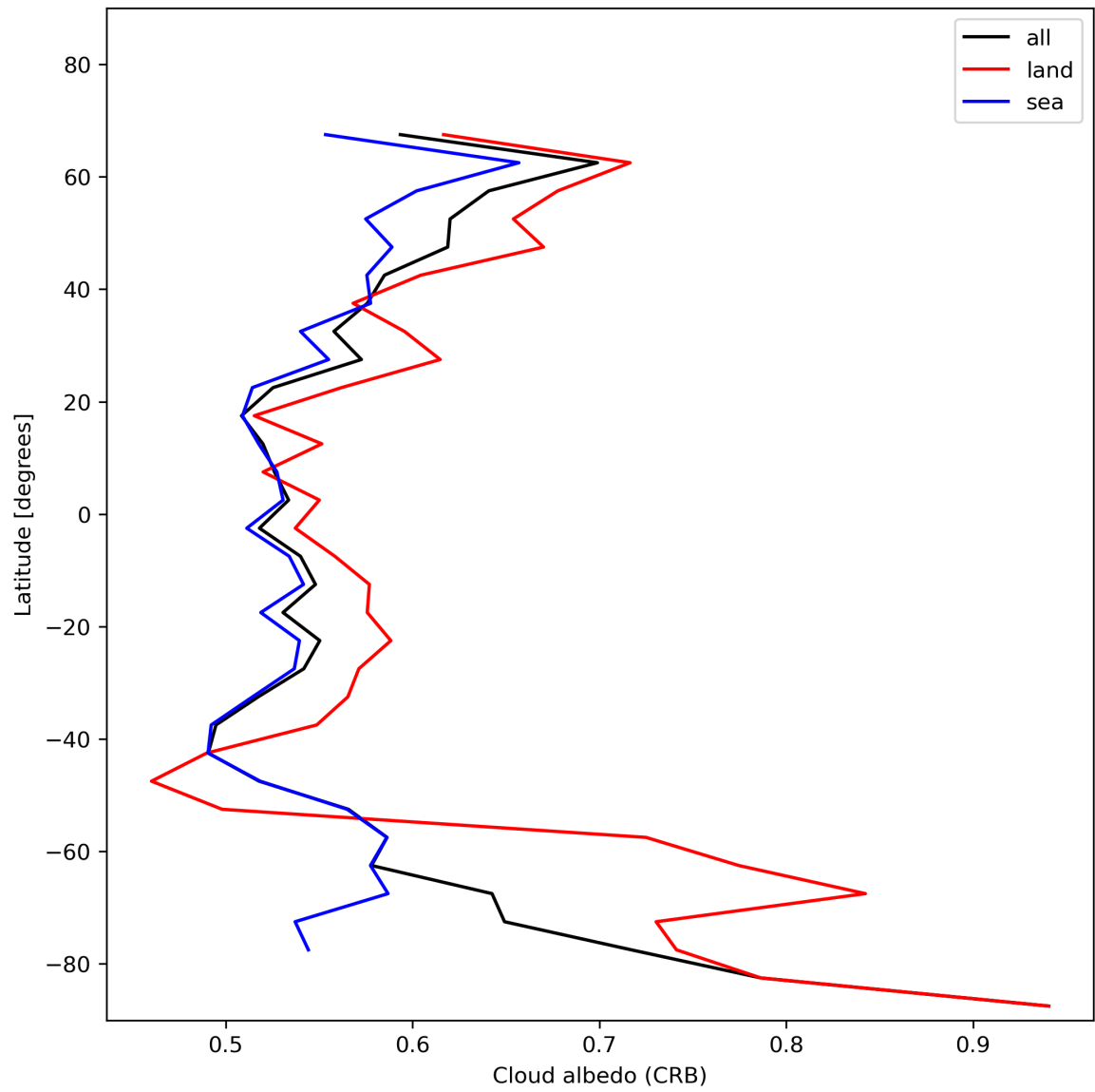
Figure 28: Zonal average of “Cloud albedo (CRB)” for 2024-01-19 to 2024-01-21.
