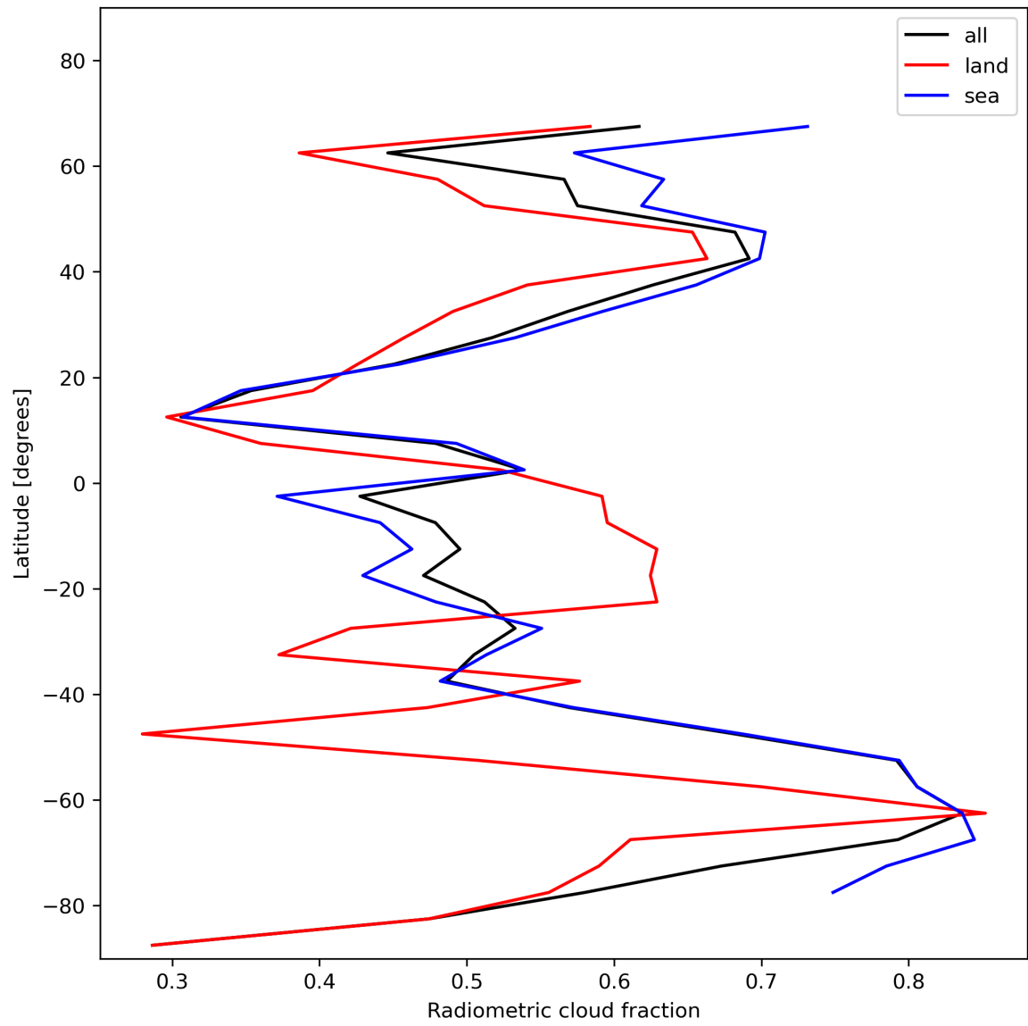
Figure 23: Zonal average of “Radiometric cloud fraction” for 2024-01-19 to 2024-01-21.
