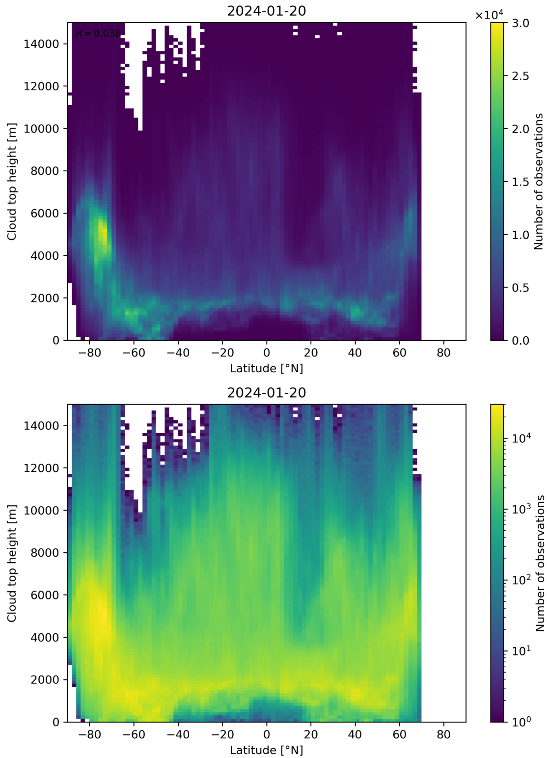
Figure 97: Scatter density plot of “Latitude” against “Cloud top height” for 2024-01-19 to 2024-01-21.
