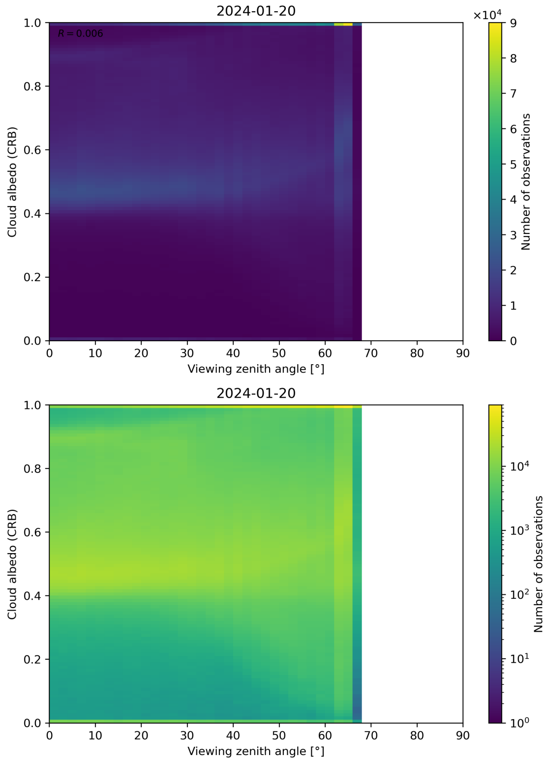
Figure 106: Scatter density plot of “Viewing zenith angle” against “Cloud albedo (CRB)” for 2024-01-19 to 2024-01-21.
