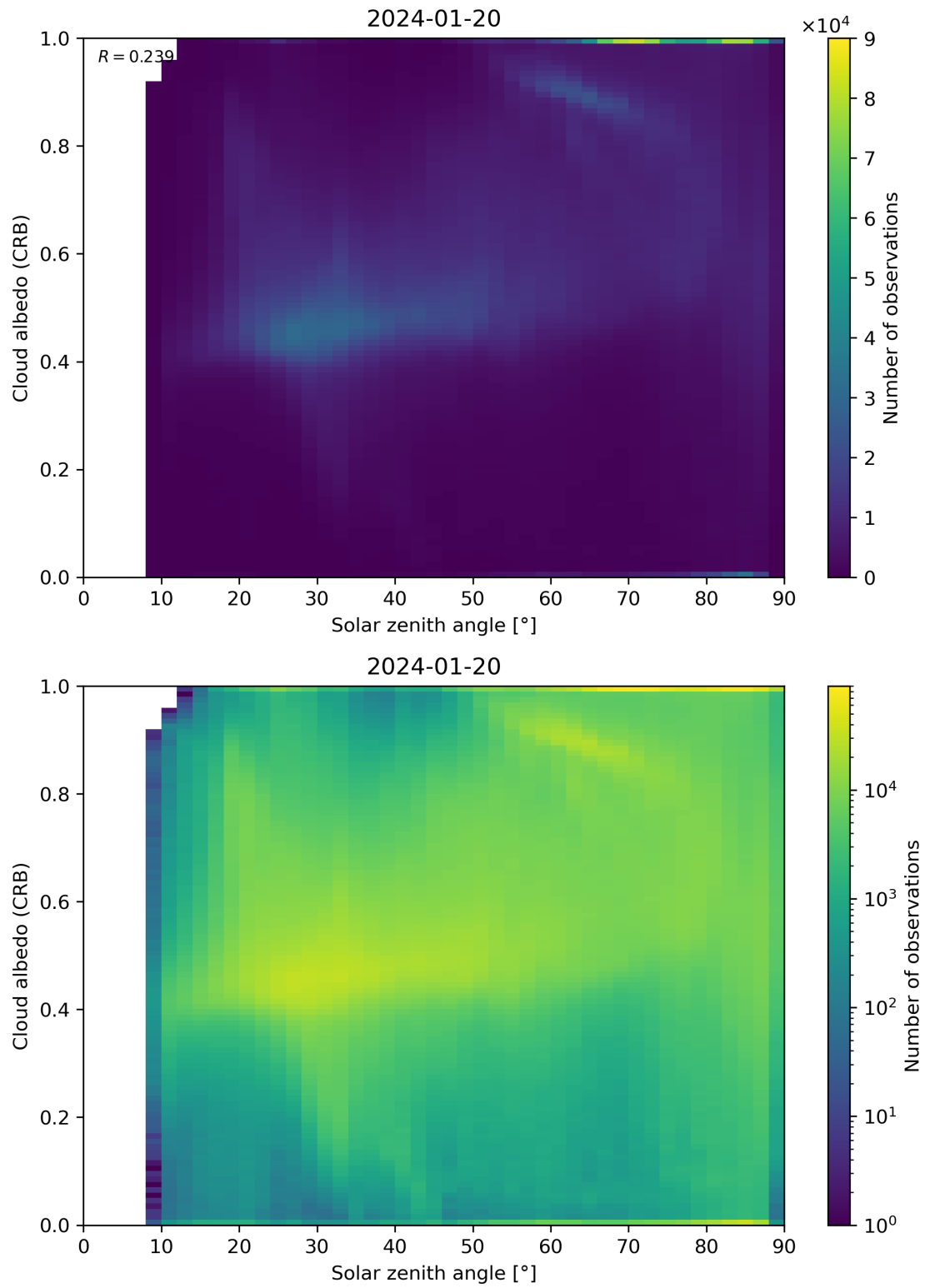
Figure 98: Scatter density plot of “Solar zenith angle” against “Cloud albedo (CRB)” for 2024-01-19 to 2024-01-21.
