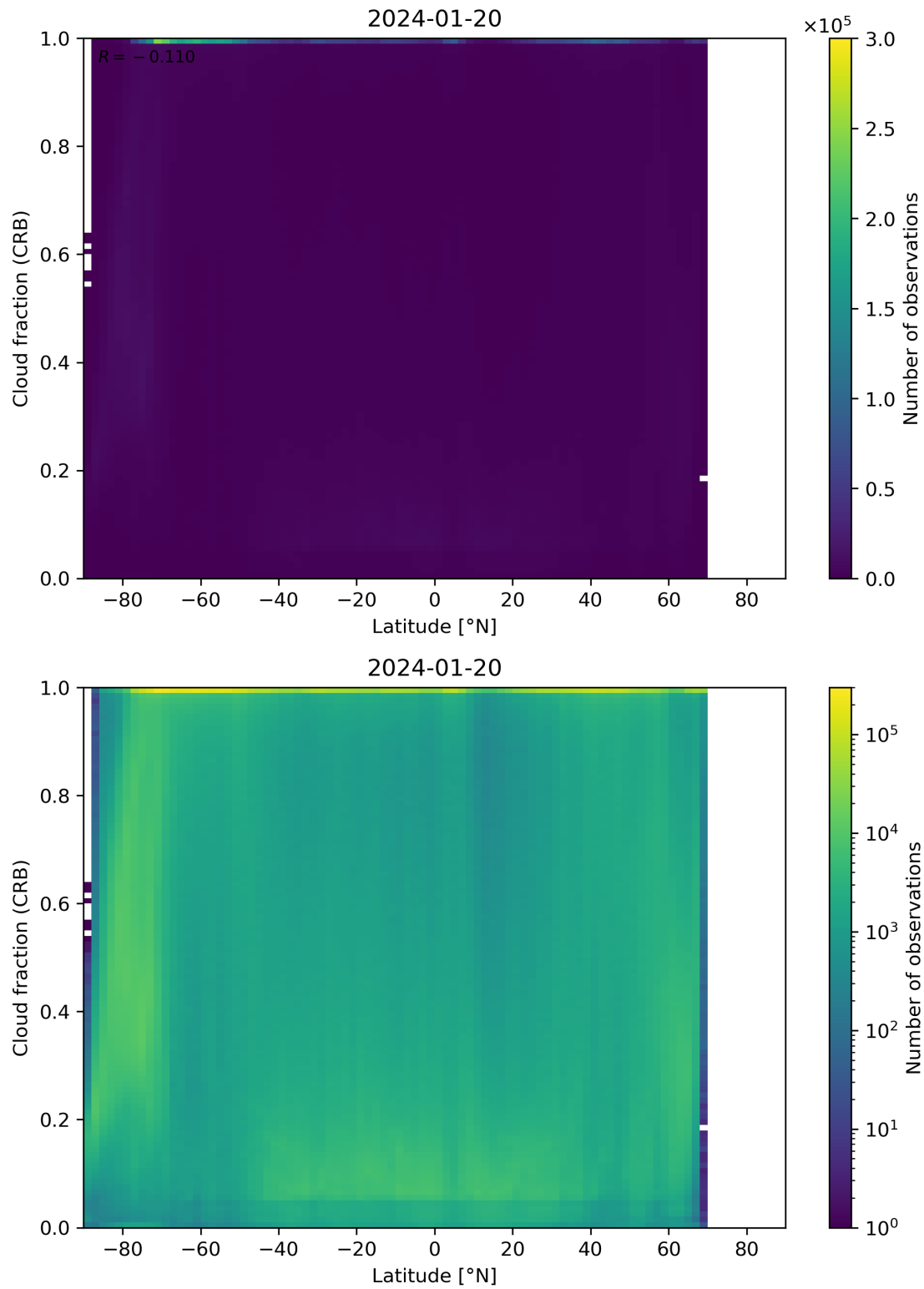
Figure 94: Scatter density plot of “Latitude” against “Cloud fraction (CRB)” for 2024-01-19 to 2024-01-21.
