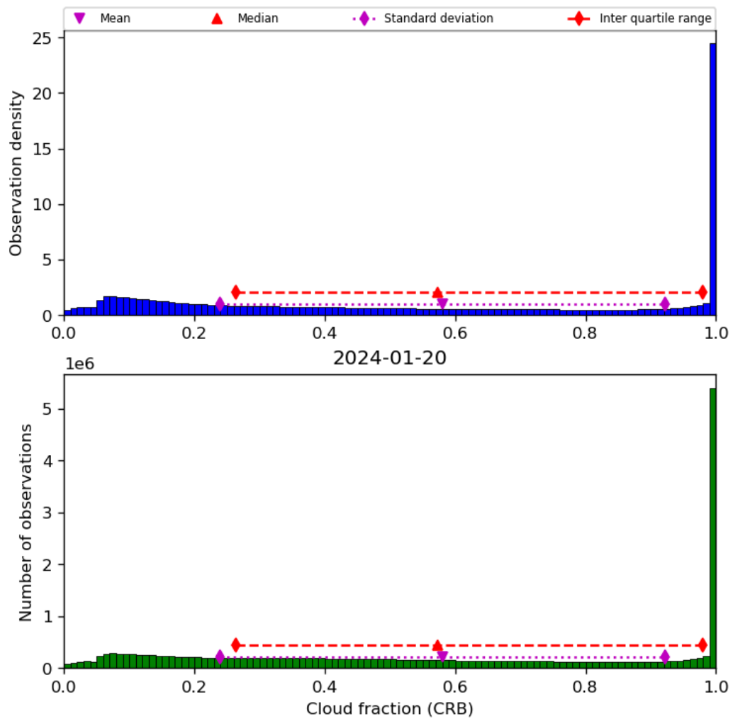
Figure 42: Histogram of “Cloud fraction (CRB)” for 2024-01-19 to 2024-01-21
