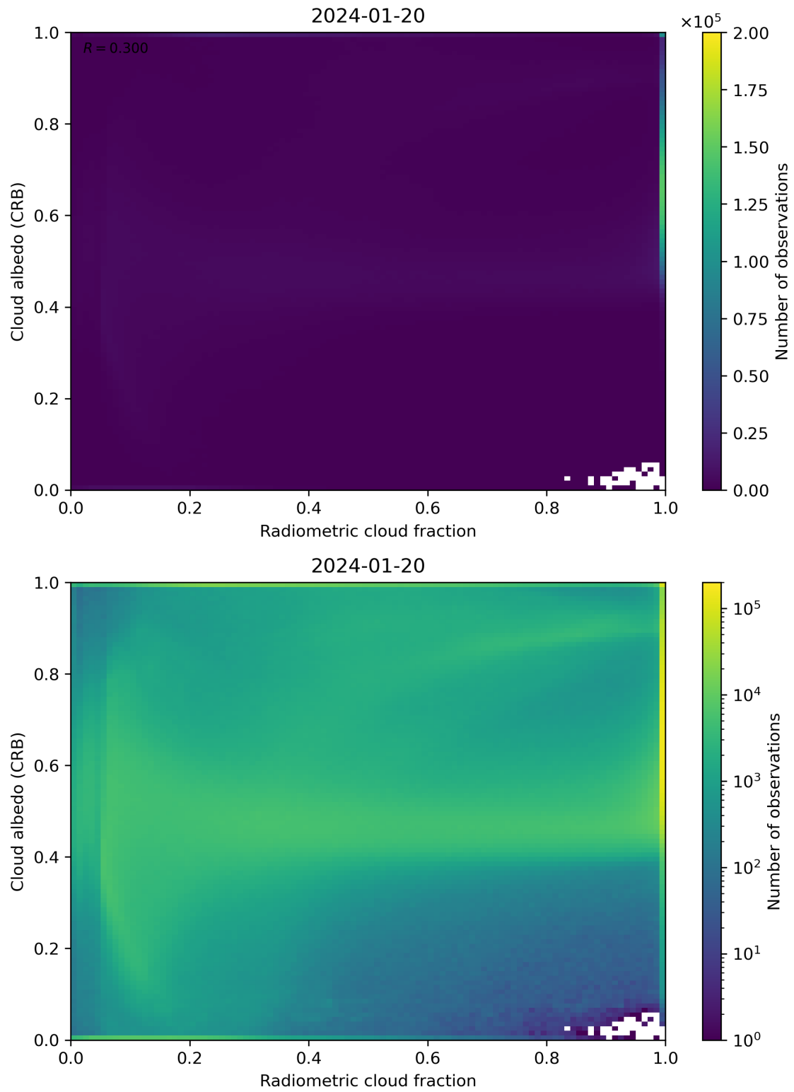
Figure 71: Scatter density plot of “Radiometric cloud fraction” against “Cloud albedo (CRB)” for 2024-01-19 to 2024-01-21.
