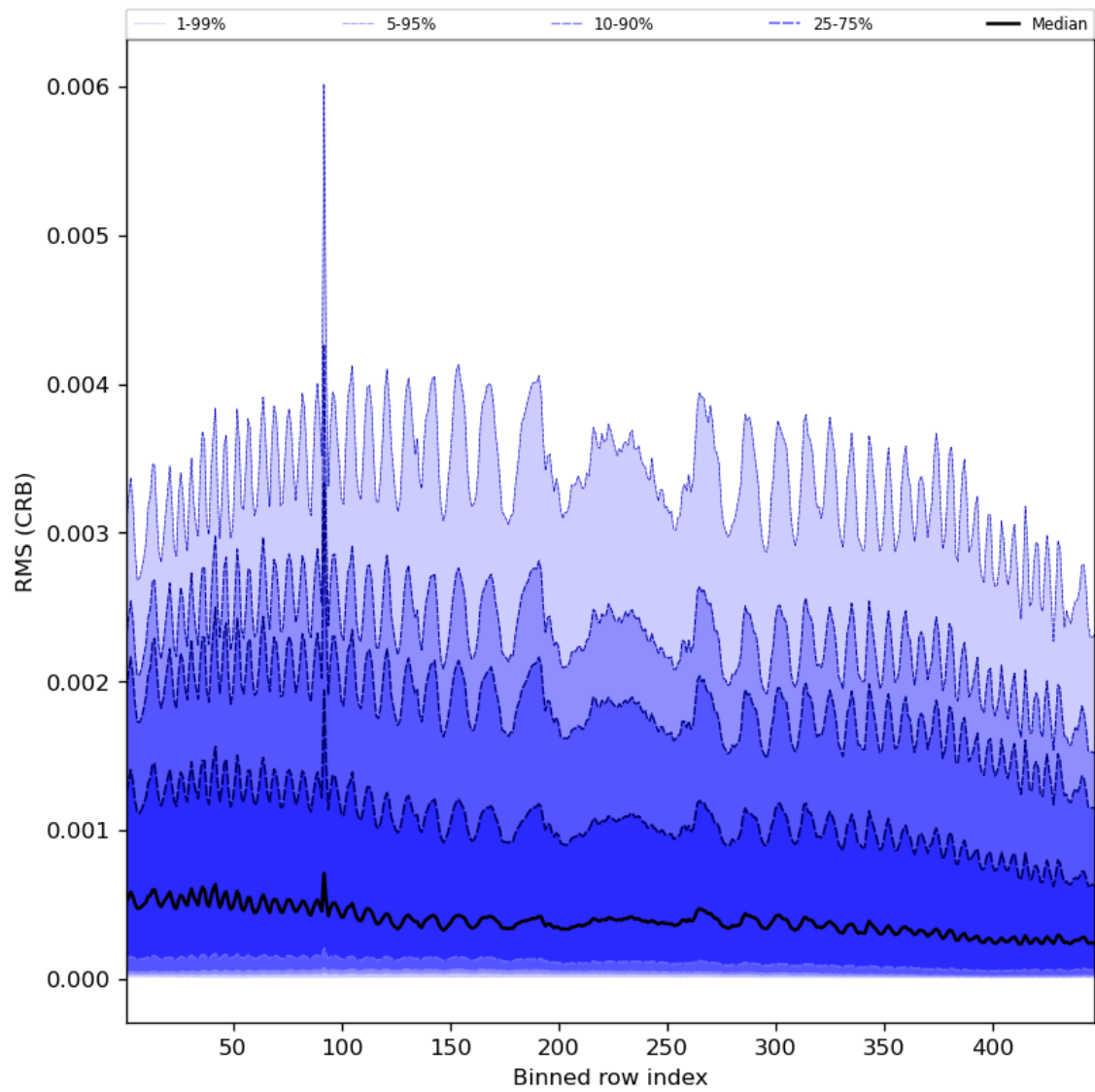
Figure 64: Along track statistics of “RMS (CRB)” for 2024-01-19 to 2024-01-21
