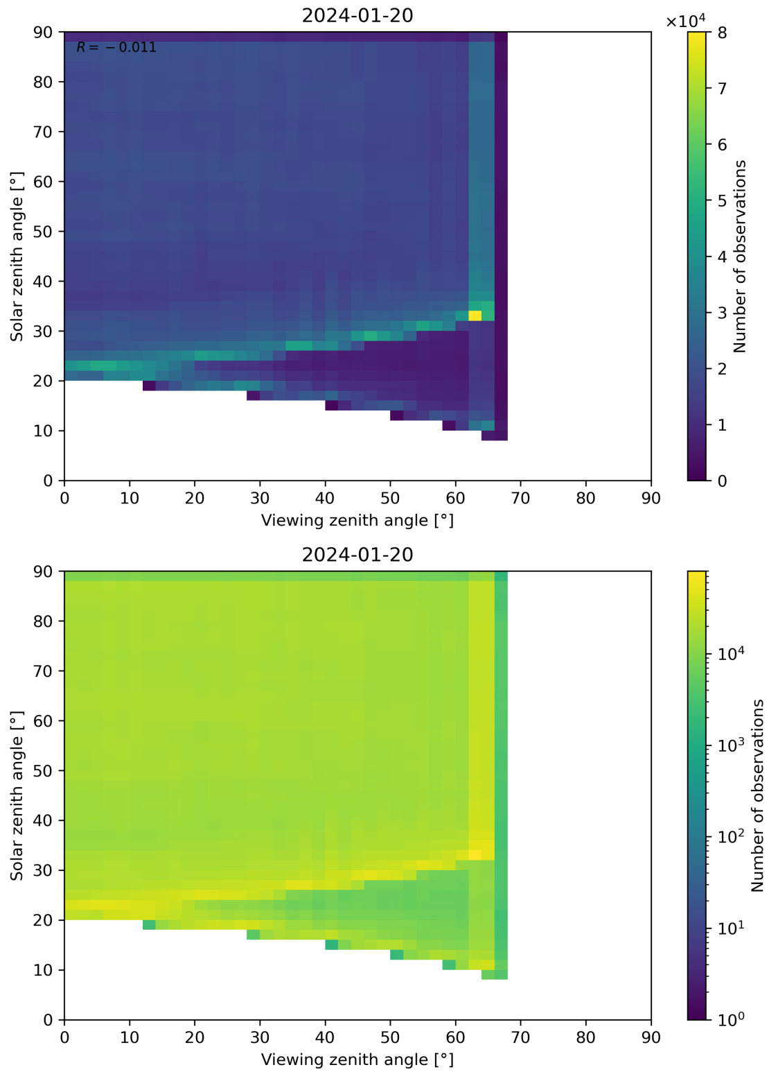
Figure 114: Scatter density plot of “Viewing zenith angle” against “Solar zenith angle” for 2024-01-19 to 2024-01-21.
