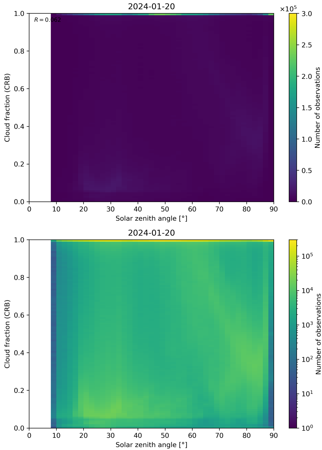
Figure 101: Scatter density plot of “Solar zenith angle” against “Cloud fraction (CRB)” for 2024-01-19 to 2024-01-21.
