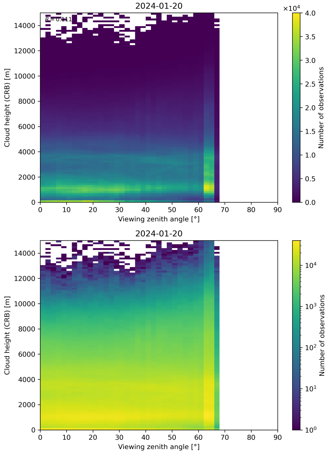
Figure 110: Scatter density plot of “Viewing zenith angle” against “Cloud height (CRB)” for 2024-01-19 to 2024-01-21.
