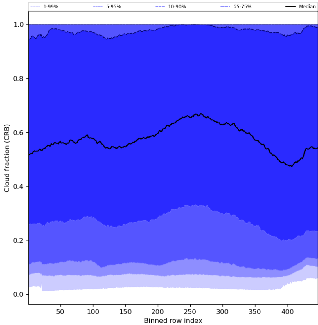
Figure 58: Along track statistics of “Cloud fraction (CRB)” for 2024-01-19 to 2024-01-21
