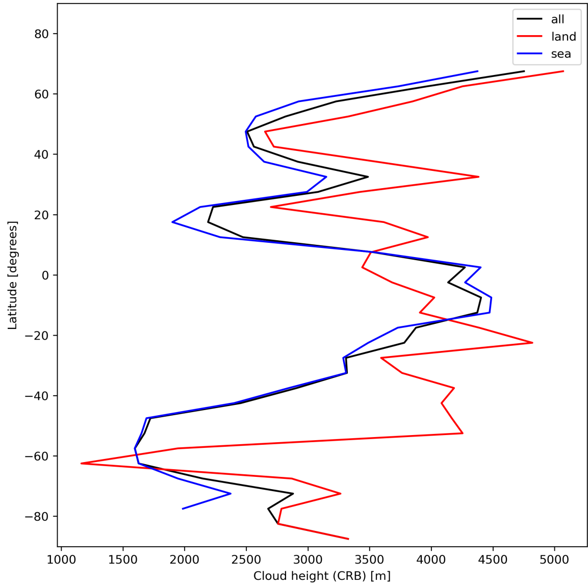
Figure 27: Zonal average of “Cloud height (CRB)” for 2024-01-19 to 2024-01-21.
