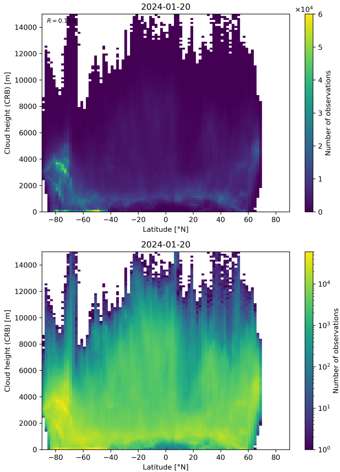
Figure 95: Scatter density plot of “Latitude” against “Cloud height (CRB)” for 2024-01-19 to 2024-01-21.
