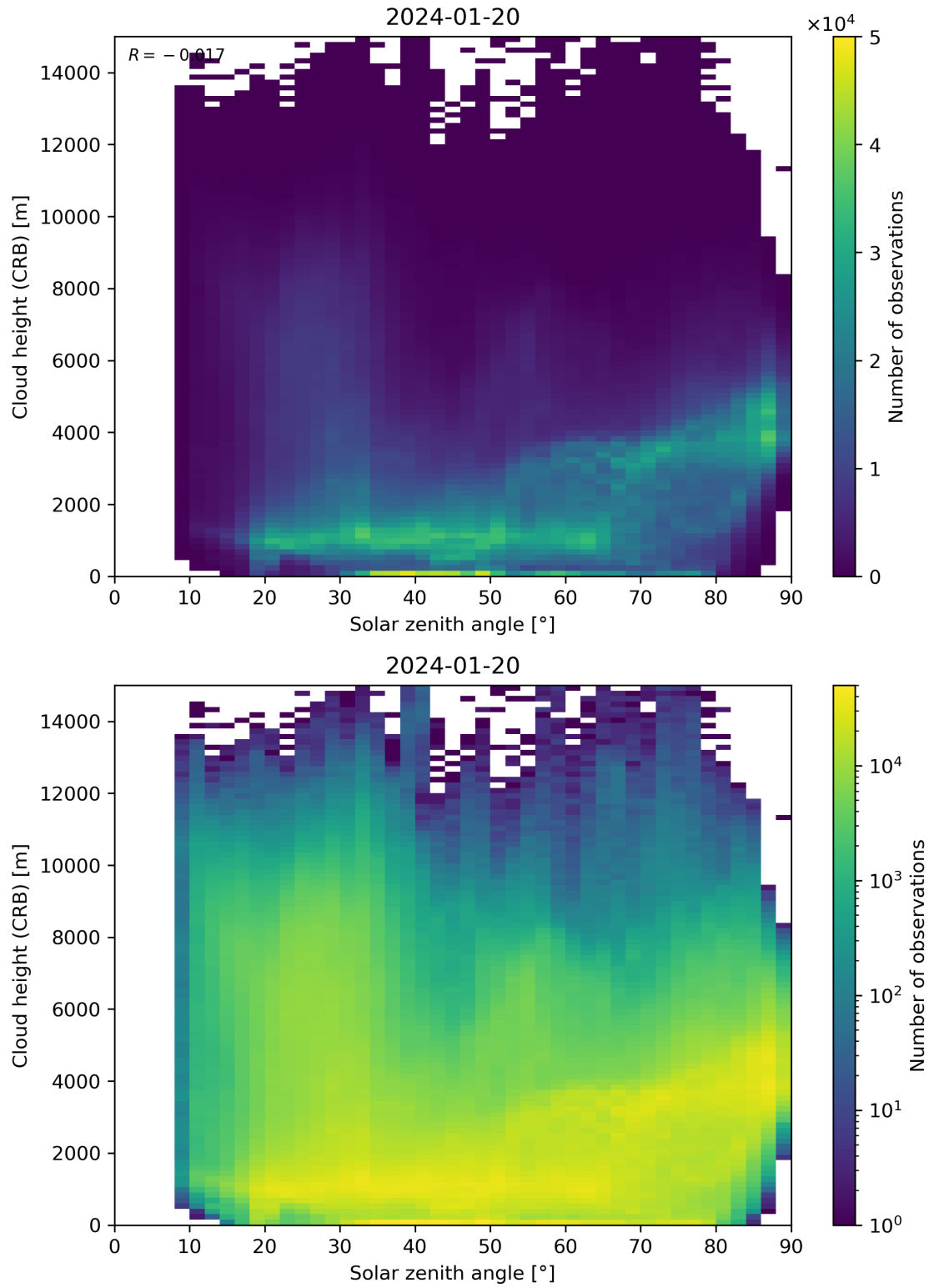
Figure 102: Scatter density plot of “Solar zenith angle” against “Cloud height (CRB)” for 2024-01-19 to 2024-01-21.
