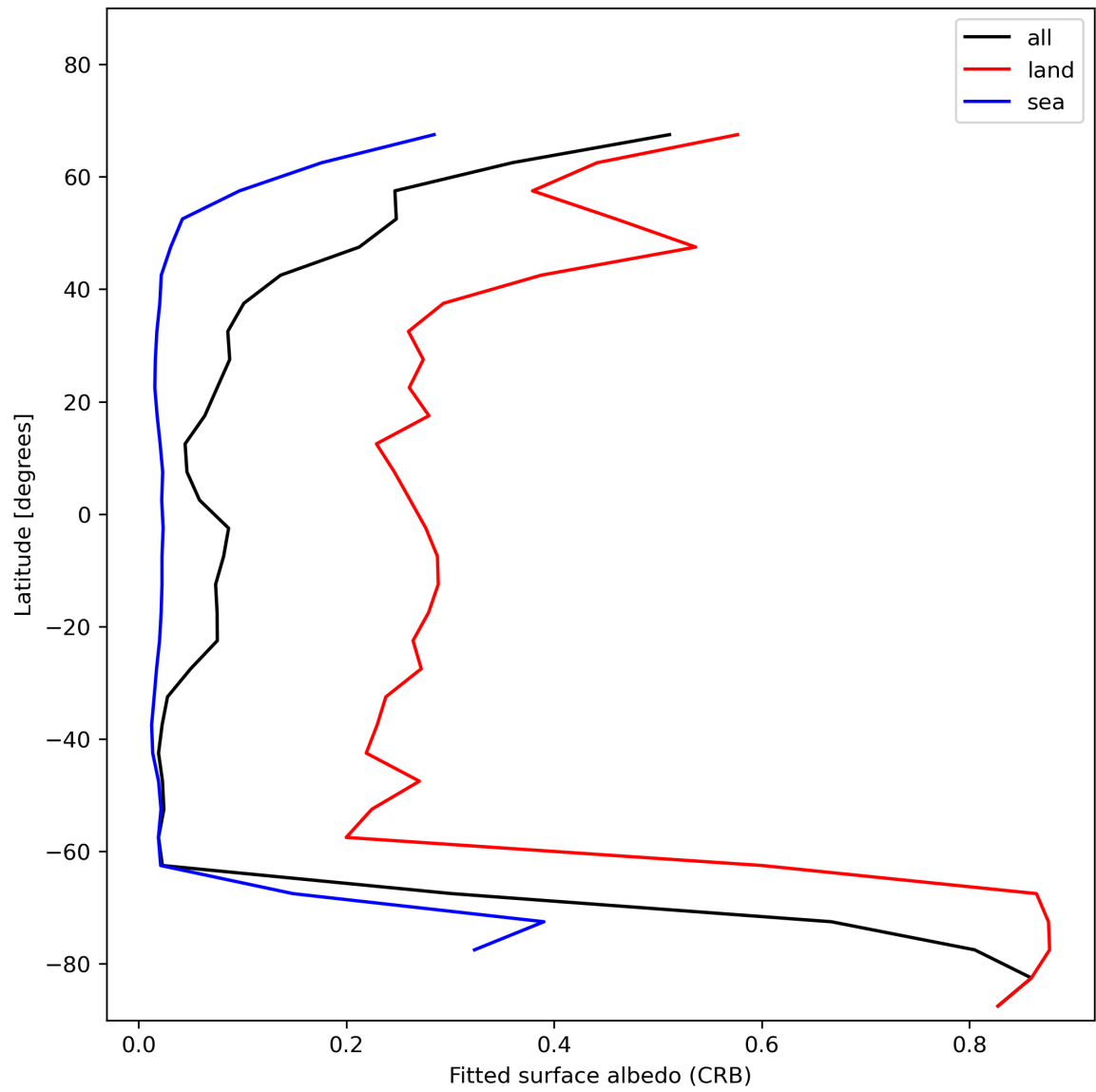
Figure 30: Zonal average of “Fitted surface albedo (CRB)” for 2024-01-19 to 2024-01-21.
