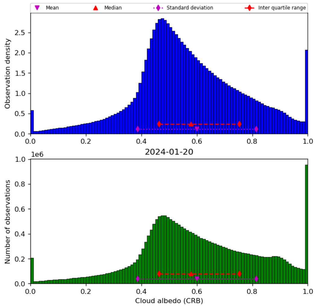
Figure 44: Histogram of “Cloud albedo (CRB)” for 2024-01-19 to 2024-01-21
