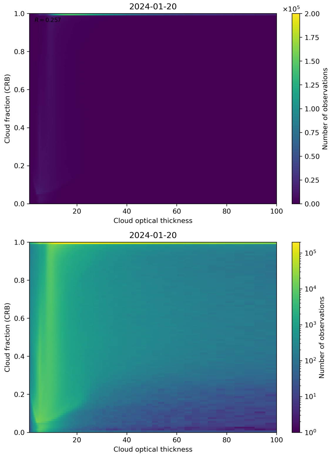
Figure 84: Scatter density plot of “Cloud optical thickness” against “Cloud fraction (CRB)” for 2024-01-19 to 2024-01-21.
