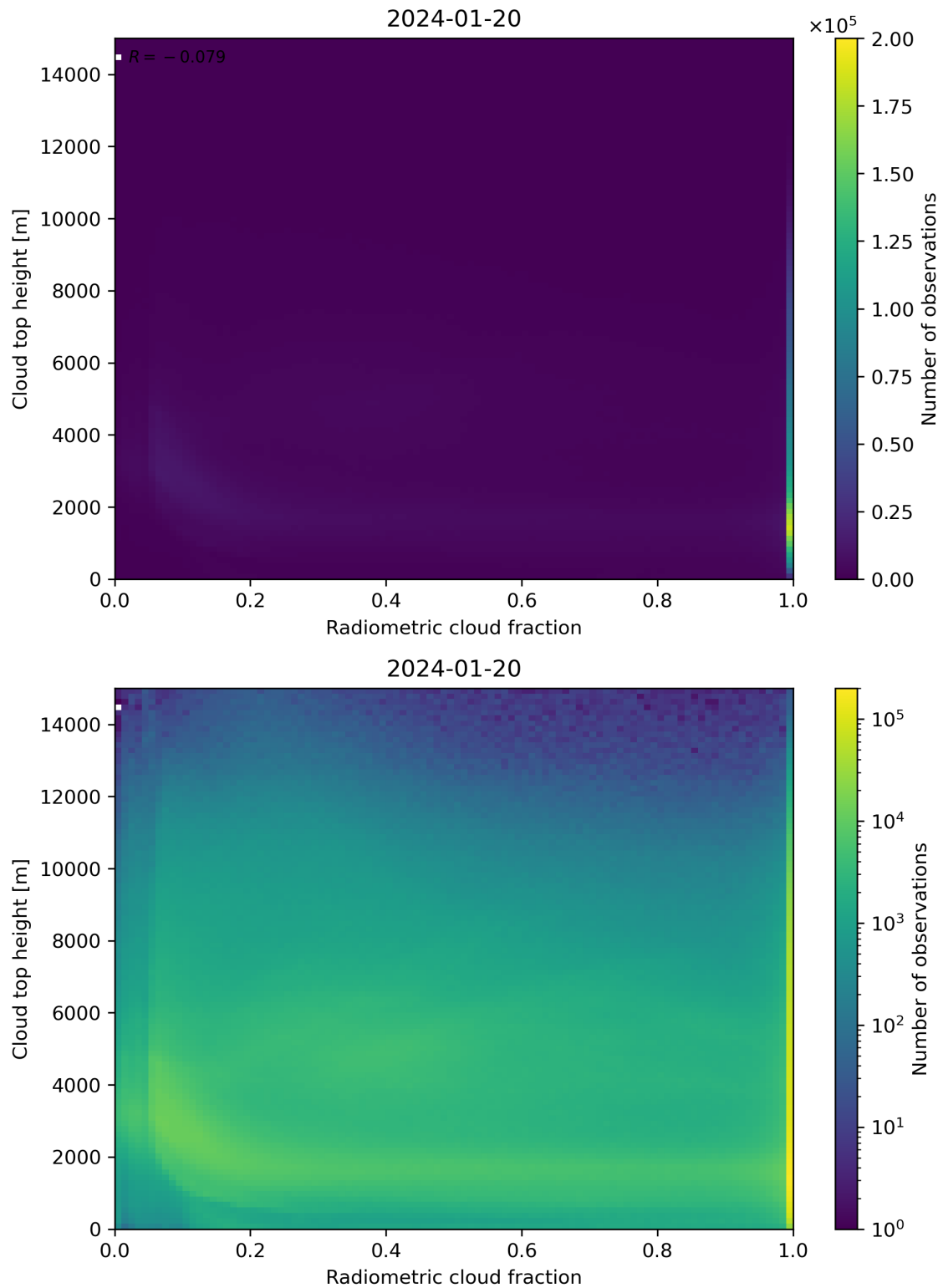
Figure 76: Scatter density plot of “Radiometric cloud fraction” against “Cloud top height” for 2024-01-19 to 2024-01-21.
