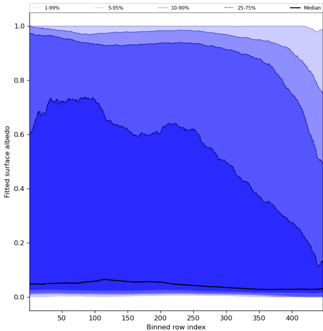
Figure 61: Along track statistics of “Fitted surface albedo” for 2024-01-19 to 2024-01-21
