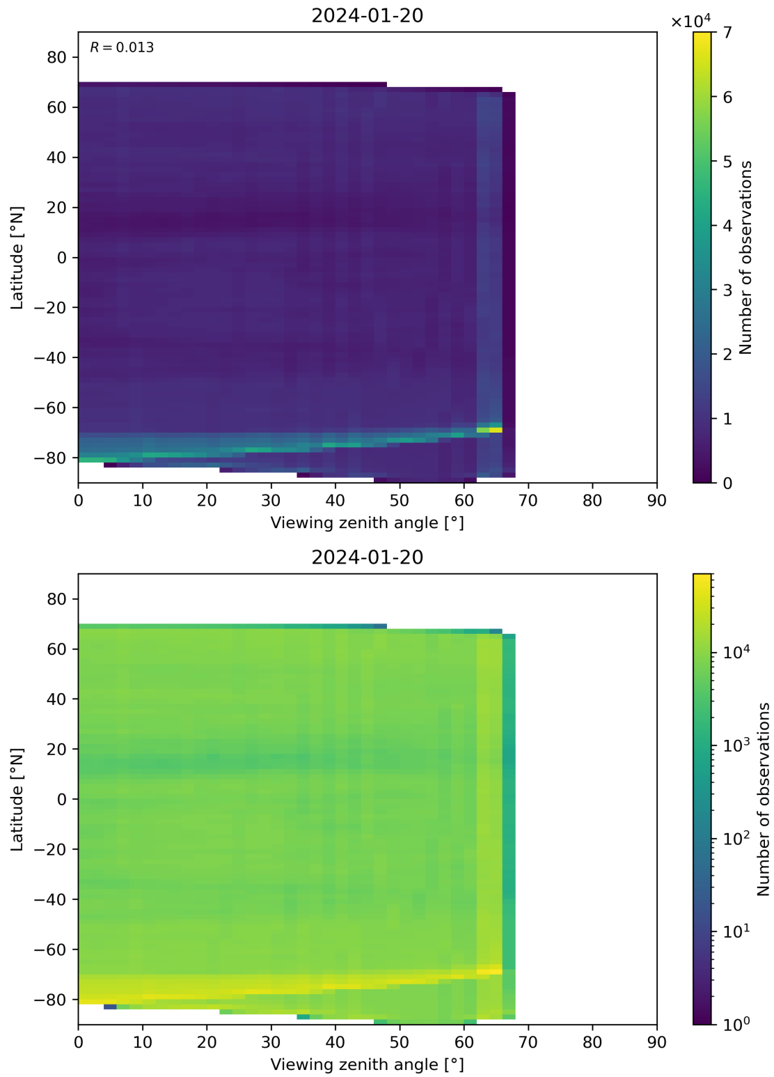
Figure 113: Scatter density plot of “Viewing zenith angle” against “Latitude” for 2024-01-19 to 2024-01-21.
