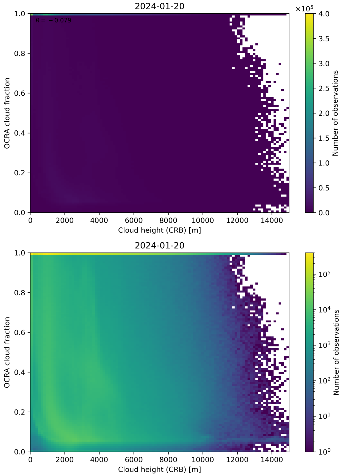
Figure 81: Scatter density plot of “Cloud height (CRB)” against “OCRA cloud fraction” for 2024-01-19 to 2024-01-21.
