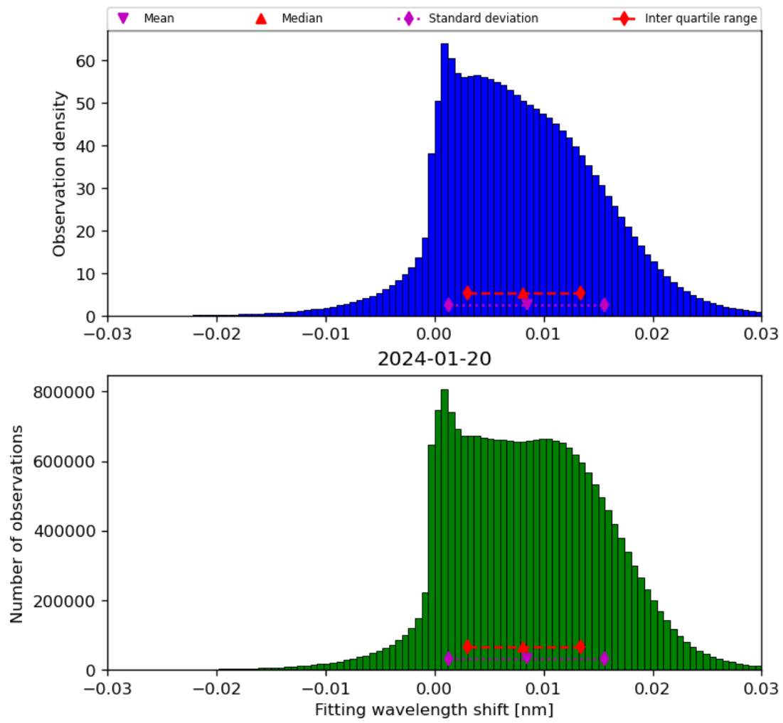
Figure 49: Histogram of “Fitting wavelength shift” for 2024-01-19 to 2024-01-21
