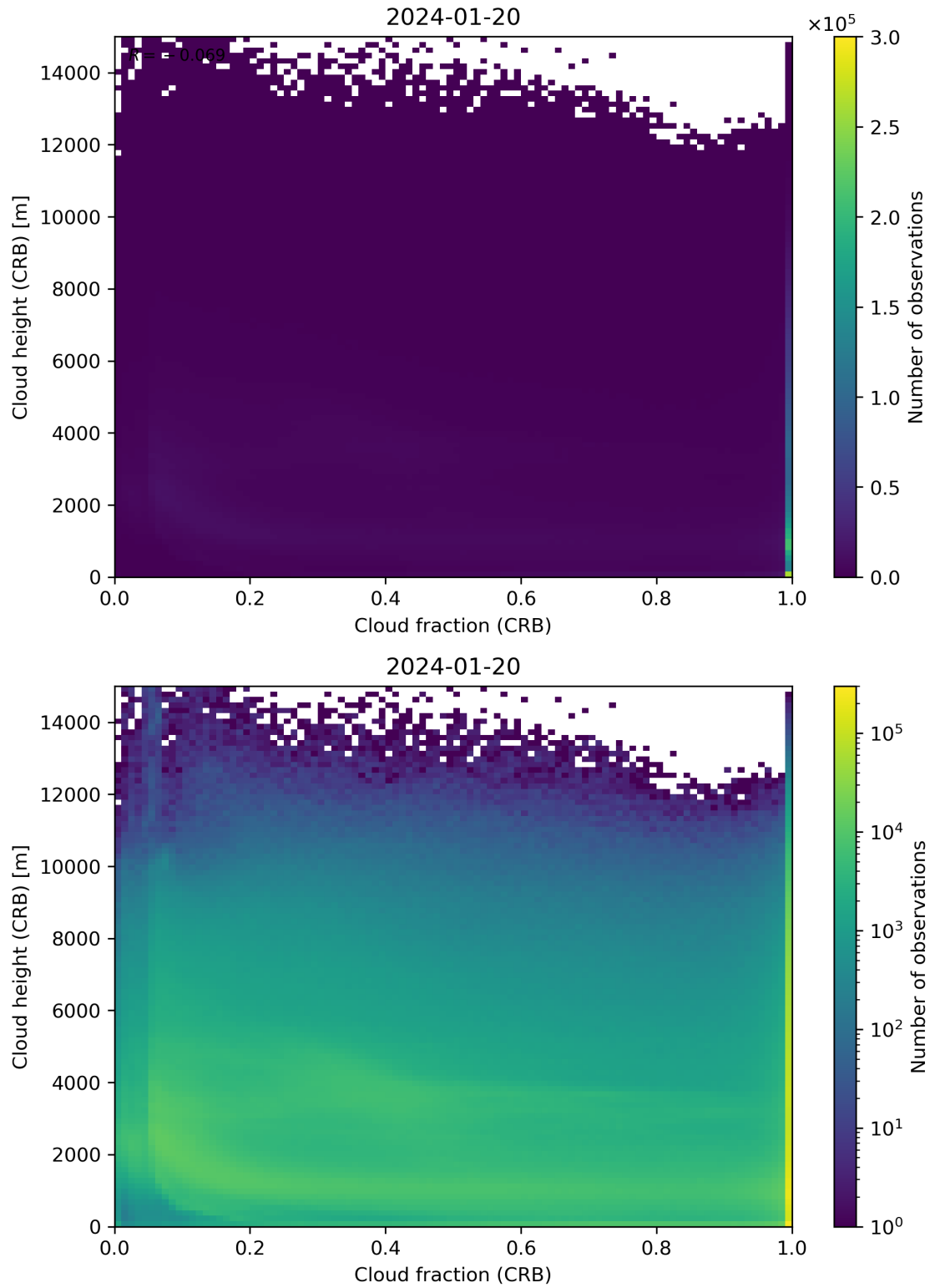
Figure 79: Scatter density plot of “Cloud fraction (CRB)” against “Cloud height (CRB)” for 2024-01-19 to 2024-01-21.
