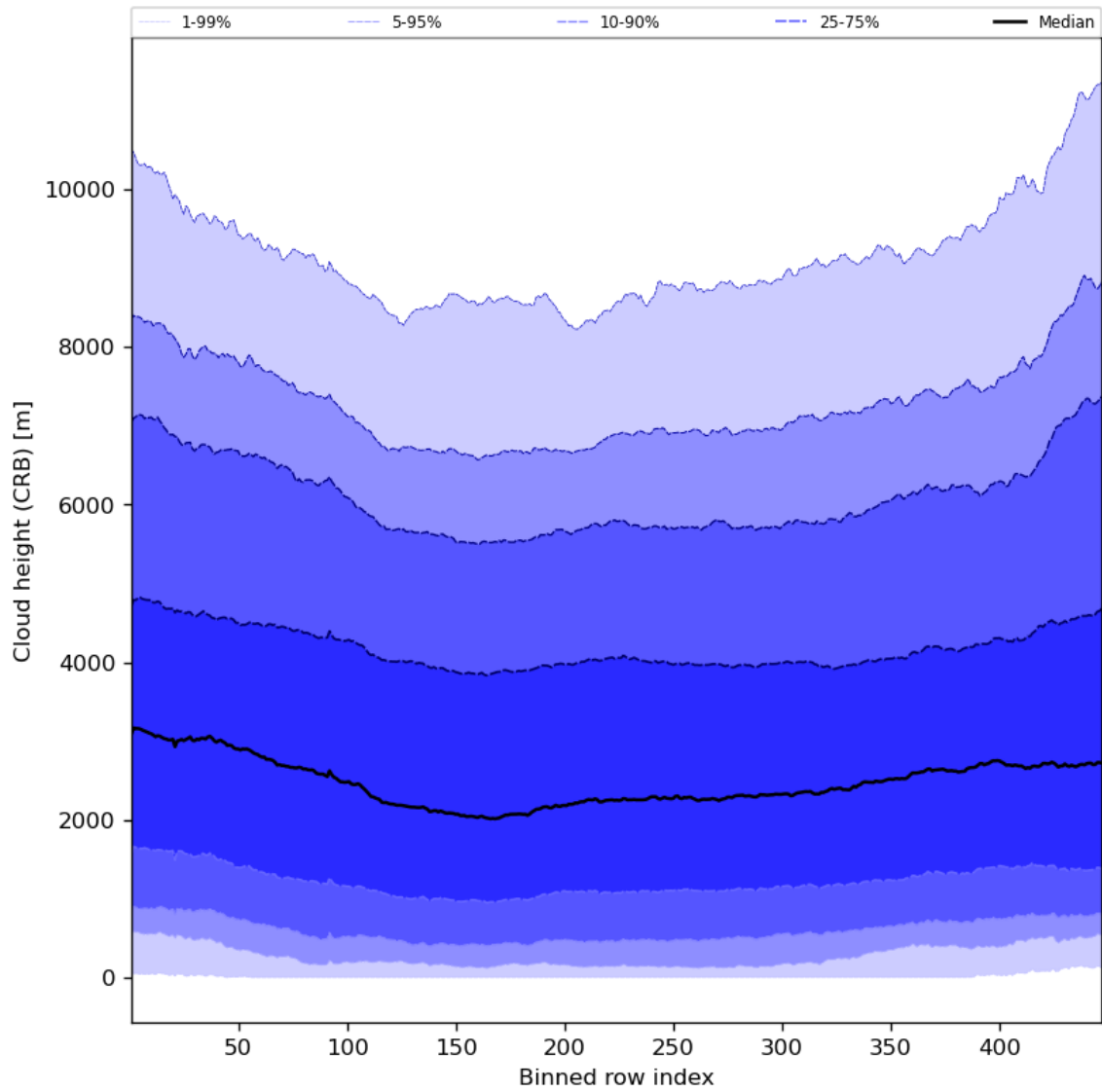
Figure 59: Along track statistics of “Cloud height (CRB)” for 2024-01-19 to 2024-01-21
