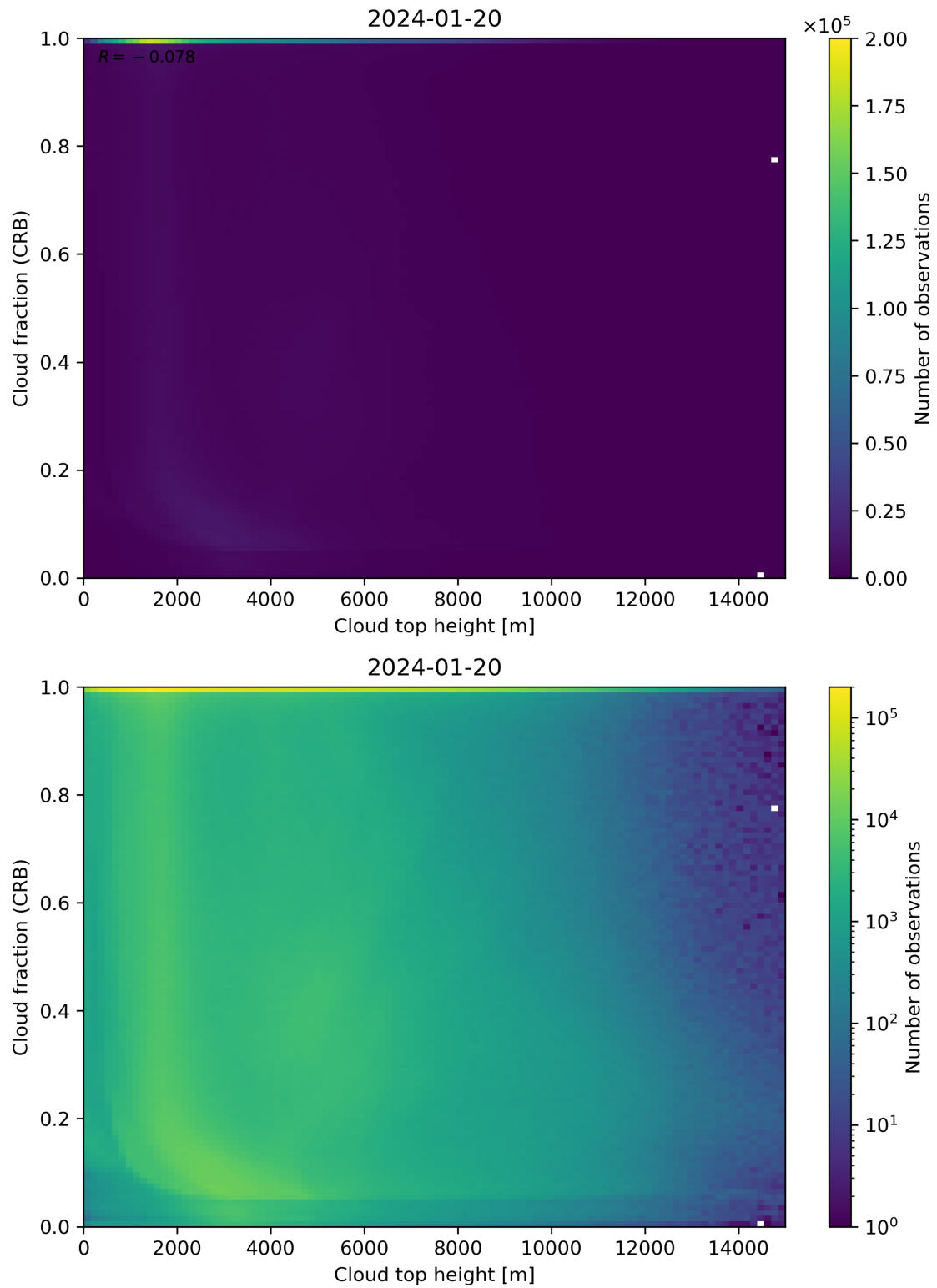
Figure 88: Scatter density plot of “Cloud top height” against “Cloud fraction (CRB)” for 2024-01-19 to 2024-01-21.
