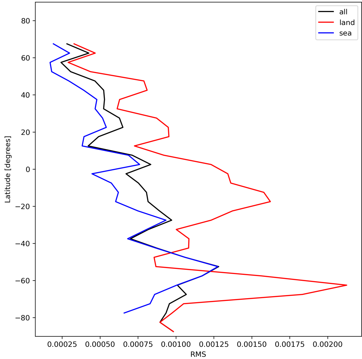
Figure 31: Zonal average of “RMS” for 2024-01-19 to 2024-01-21.
