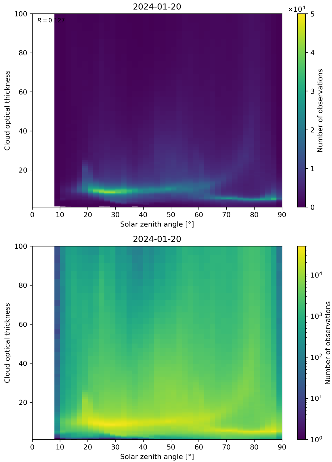
Figure 103: Scatter density plot of “Solar zenith angle” against “Cloud optical thickness” for 2024-01-19 to 2024-01-21.
