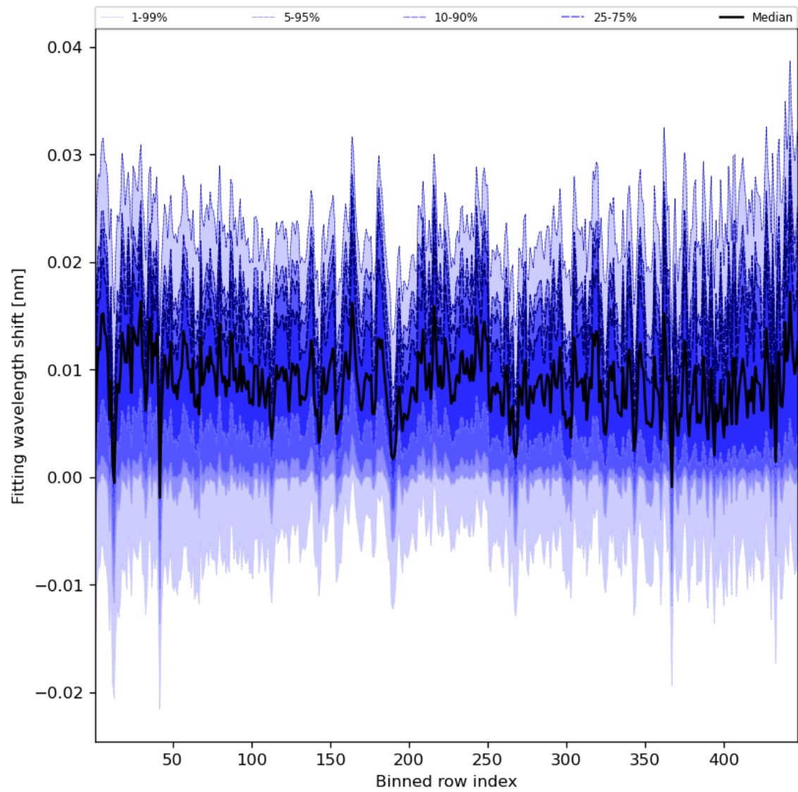
Figure 65: Along track statistics of “Fitting wavelength shift” for 2024-01-19 to 2024-01-21
