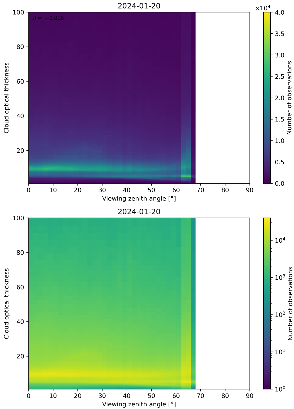
Figure 111: Scatter density plot of “Viewing zenith angle” against “Cloud optical thickness” for 2024-01-19 to 2024-01-21.
