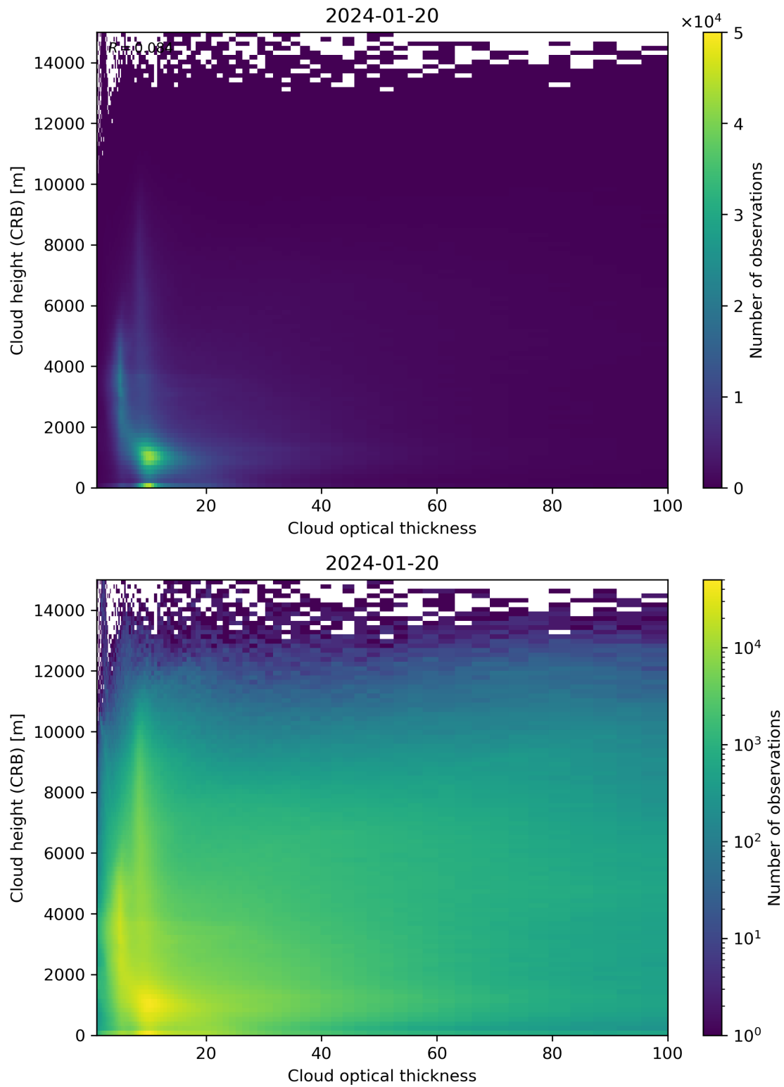
Figure 85: Scatter density plot of “Cloud optical thickness” against “Cloud height (CRB)” for 2024-01-19 to 2024-01-21.
