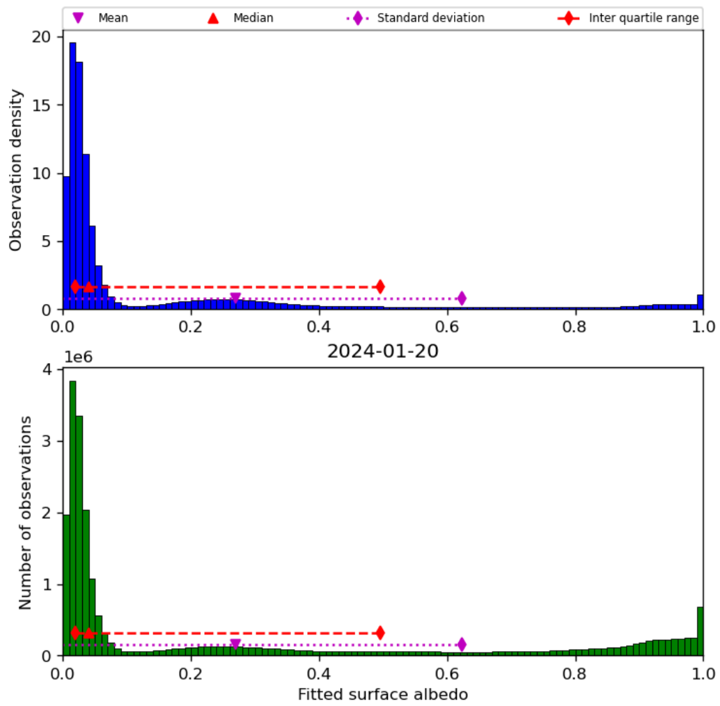
Figure 45: Histogram of “Fitted surface albedo” for 2024-01-19 to 2024-01-21
