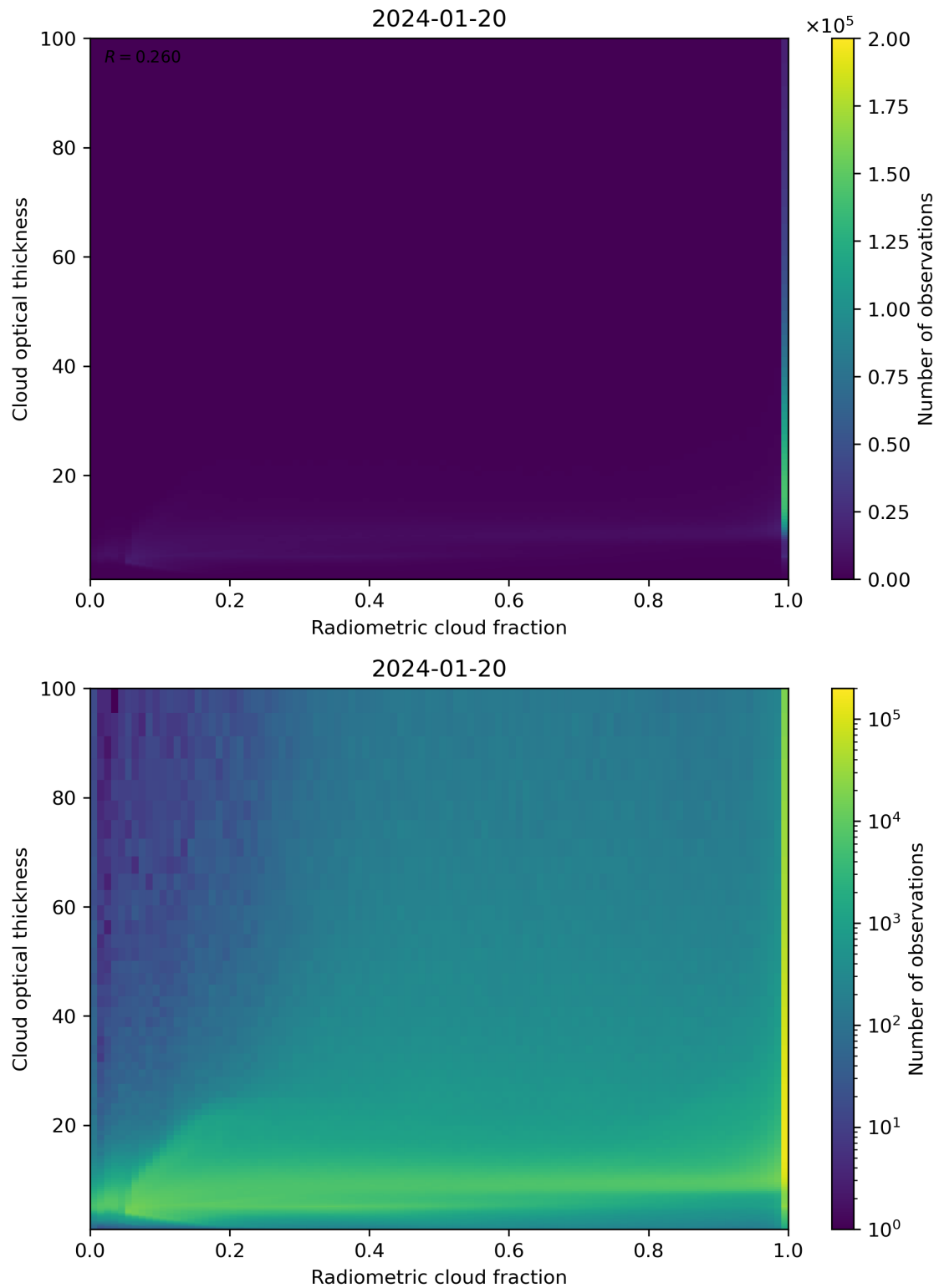
Figure 75: Scatter density plot of “Radiometric cloud fraction” against “Cloud optical thickness” for 2024-01-19 to 2024-01-21.
