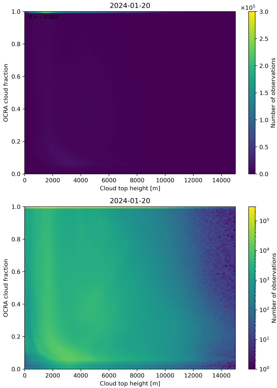
Figure 87: Scatter density plot of “Cloud top height” against “OCRA cloud fraction” for 2024-01-19 to 2024-01-21.
