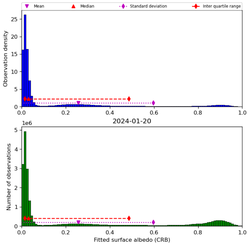
Figure 46: Histogram of “Fitted surface albedo (CRB)” for 2024-01-19 to 2024-01-21
