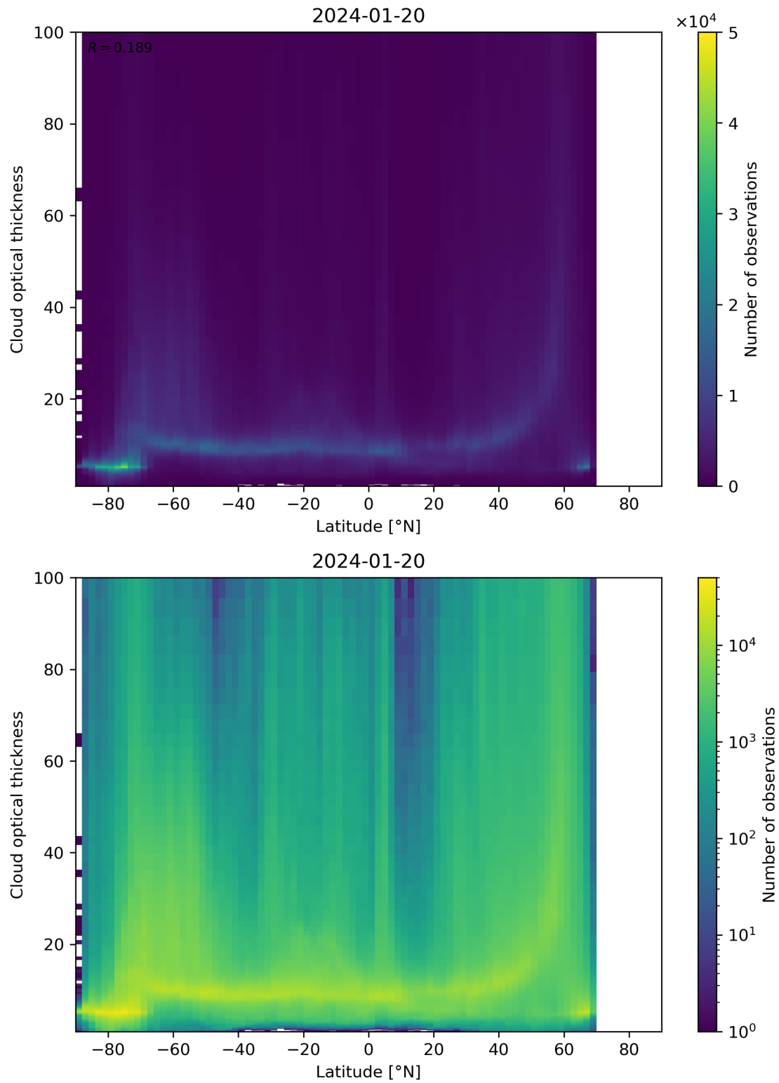
Figure 96: Scatter density plot of “Latitude” against “Cloud optical thickness” for 2024-01-19 to 2024-01-21.
