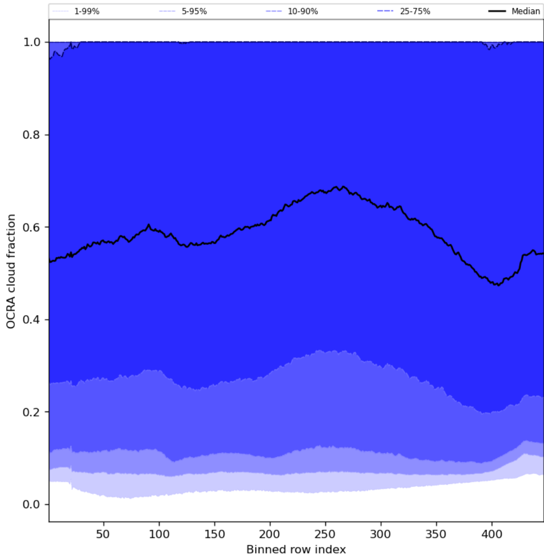
Figure 66: Along track statistics of “OCRA cloud fraction” for 2024-01-19 to 2024-01-21
