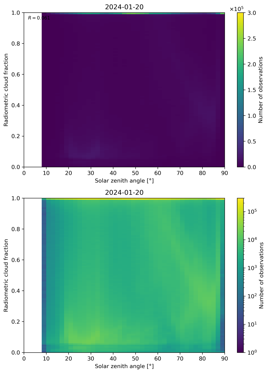
Figure 99: Scatter density plot of “Solar zenith angle” against “Radiometric cloud fraction” for 2024-01-19 to 2024-01-21.
