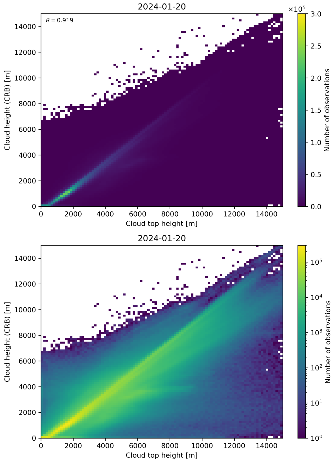
Figure 89: Scatter density plot of “Cloud top height” against “Cloud height (CRB)” for 2024-01-19 to 2024-01-21.
