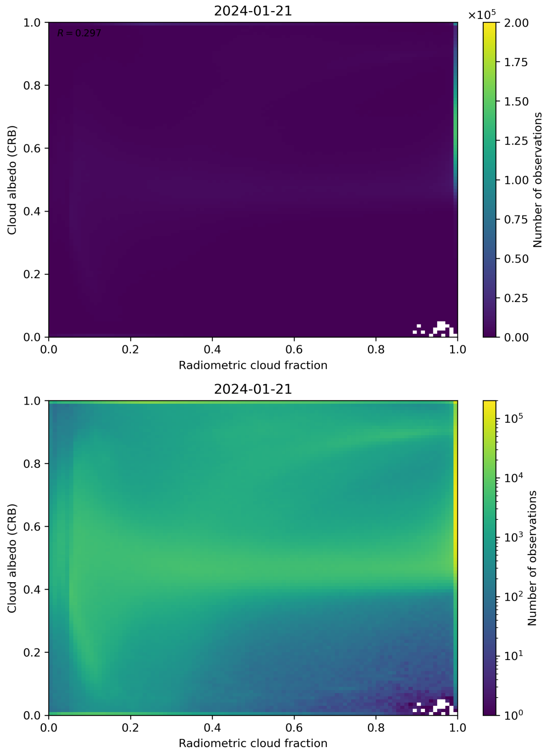
Figure 71: Scatter density plot of “Radiometric cloud fraction” against “Cloud albedo (CRB)” for 2024-01-21 to 2024-01-22.
