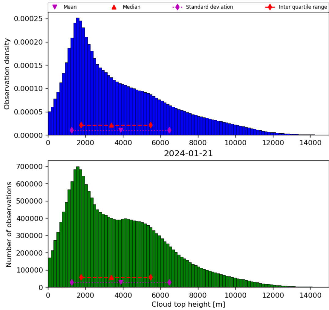
Figure 40: Histogram of “Cloud top height” for 2024-01-21 to 2024-01-22
