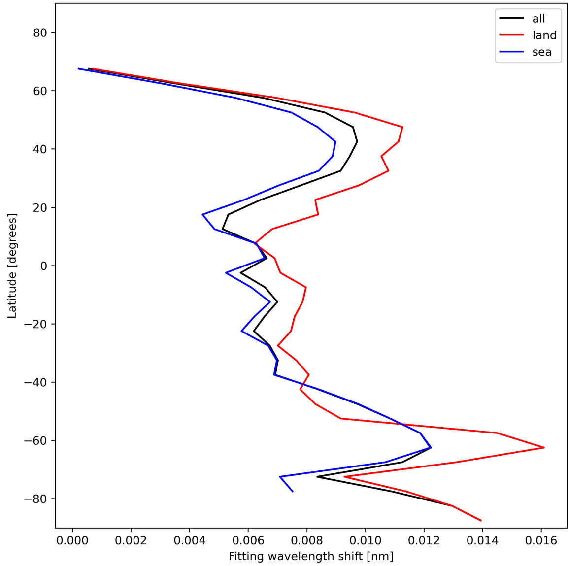
Figure 33: Zonal average of “Fitting wavelength shift” for 2024-01-21 to 2024-01-22.
