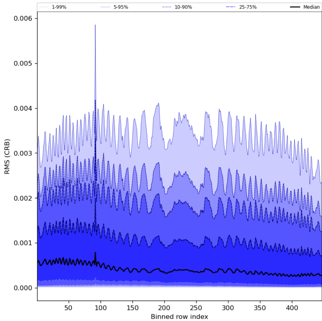
Figure 64: Along track statistics of “RMS (CRB)” for 2024-01-21 to 2024-01-22
