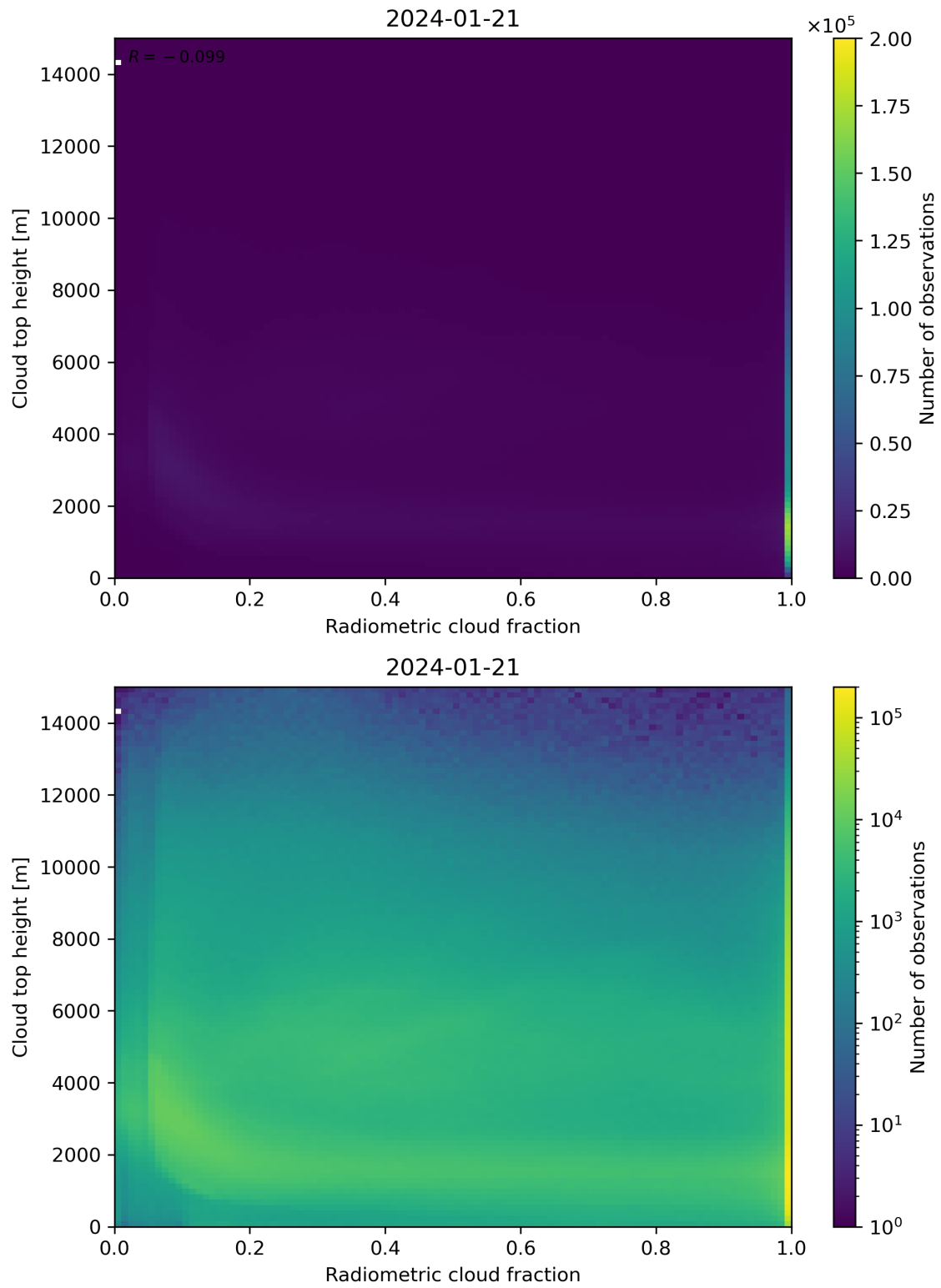
Figure 76: Scatter density plot of “Radiometric cloud fraction” against “Cloud top height” for 2024-01-21 to 2024-01-22.
