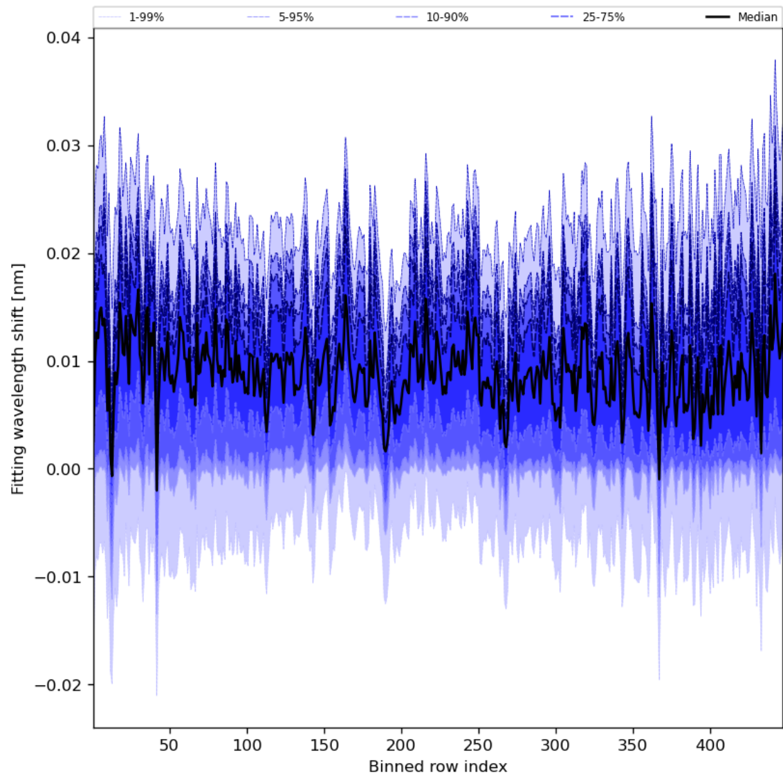
Figure 65: Along track statistics of “Fitting wavelength shift” for 2024-01-21 to 2024-01-22
