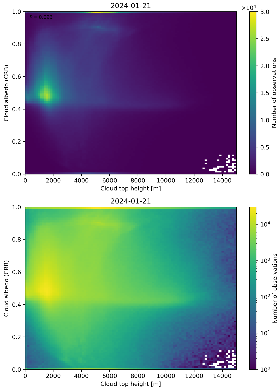
Figure 86: Scatter density plot of “Cloud top height” against “Cloud albedo (CRB)” for 2024-01-21 to 2024-01-22.
