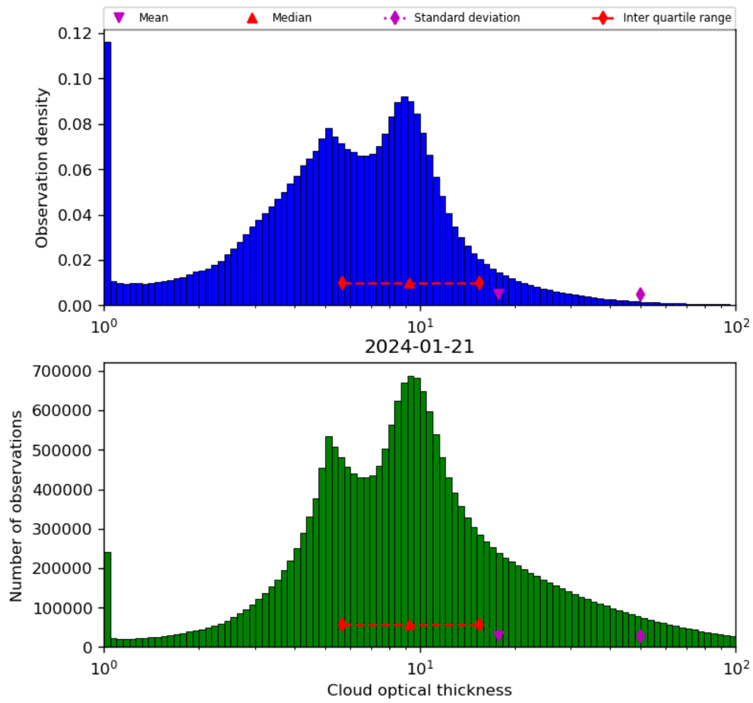
Figure 41: Histogram of “Cloud optical thickness” for 2024-01-21 to 2024-01-22
