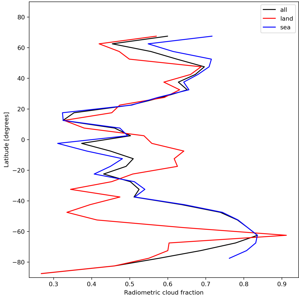
Figure 23: Zonal average of “Radiometric cloud fraction” for 2024-01-21 to 2024-01-22.
