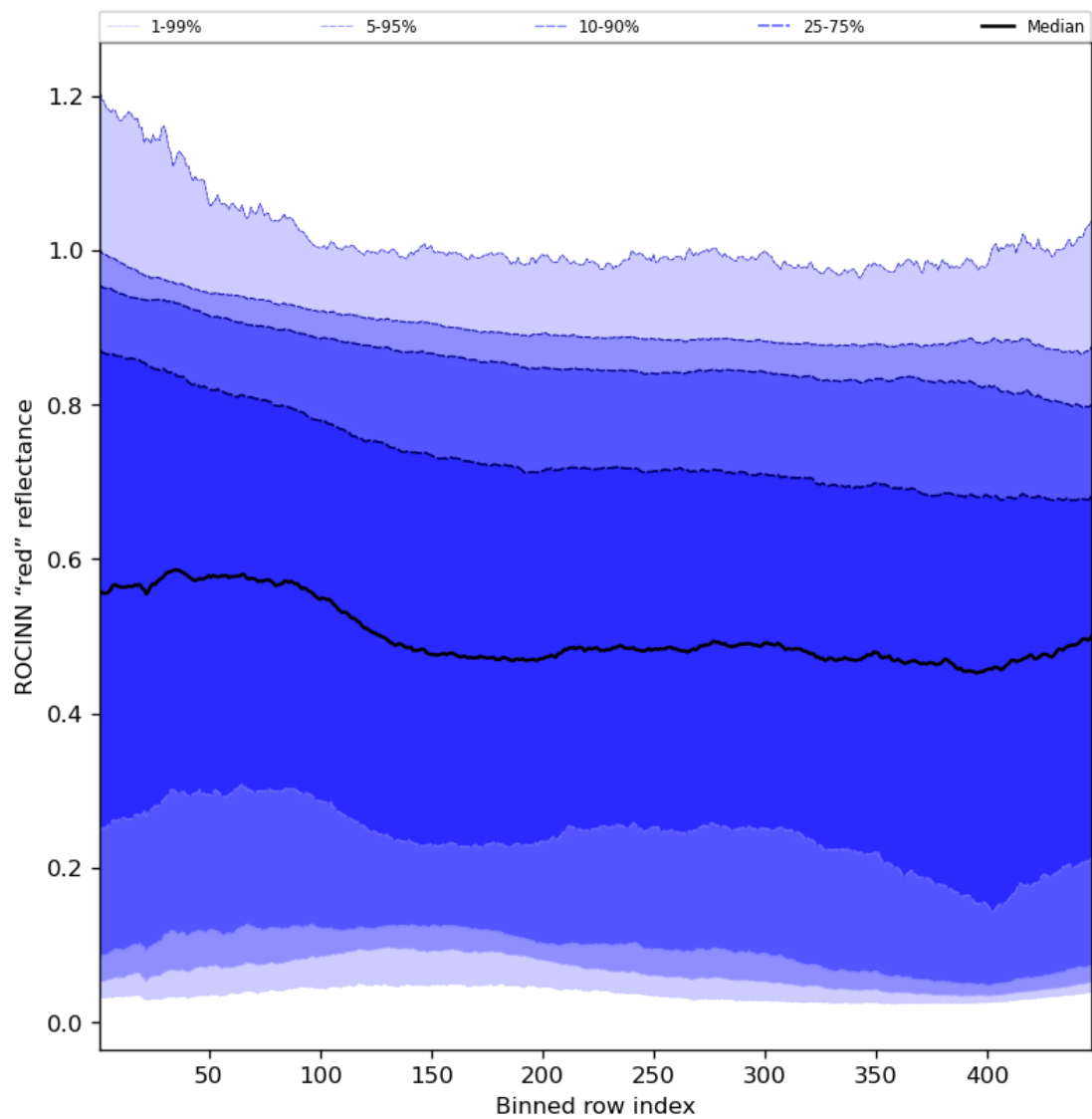
Figure 69: Along track statistics of “ROCINN “red” reflectance” for 2024-01-21 to 2024-01-22
