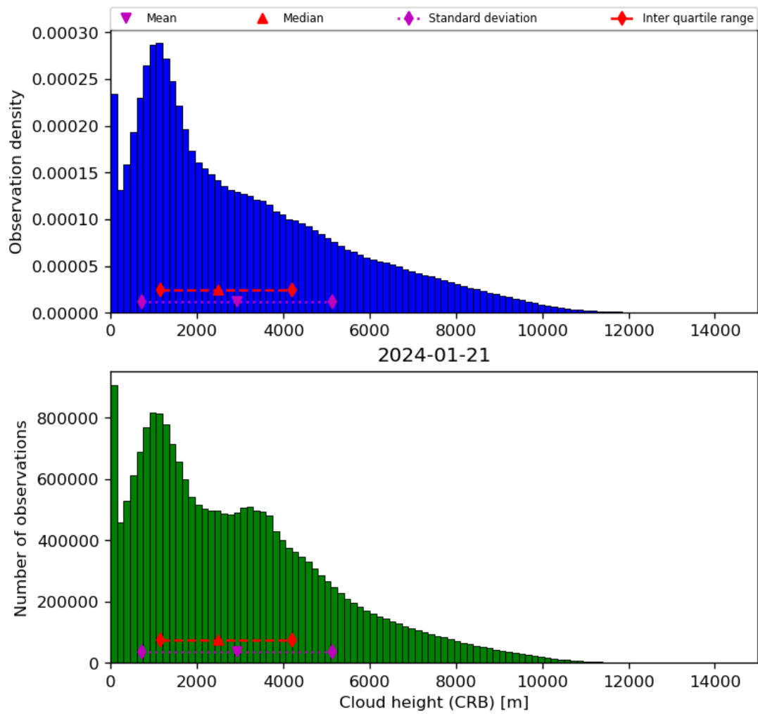
Figure 43: Histogram of “Cloud height (CRB)” for 2024-01-21 to 2024-01-22
