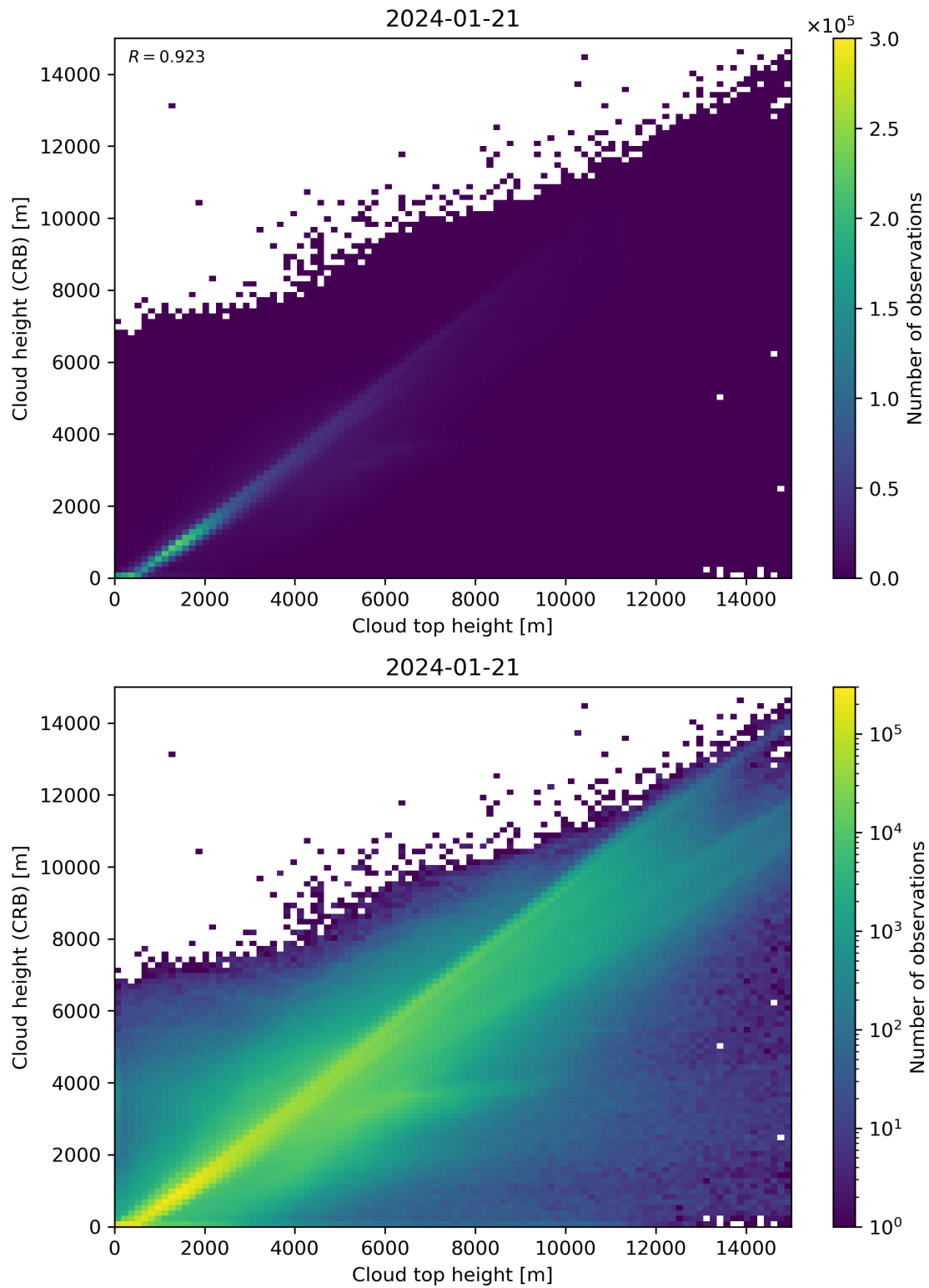
Figure 89: Scatter density plot of “Cloud top height” against “Cloud height (CRB)” for 2024-01-21 to 2024-01-22.
