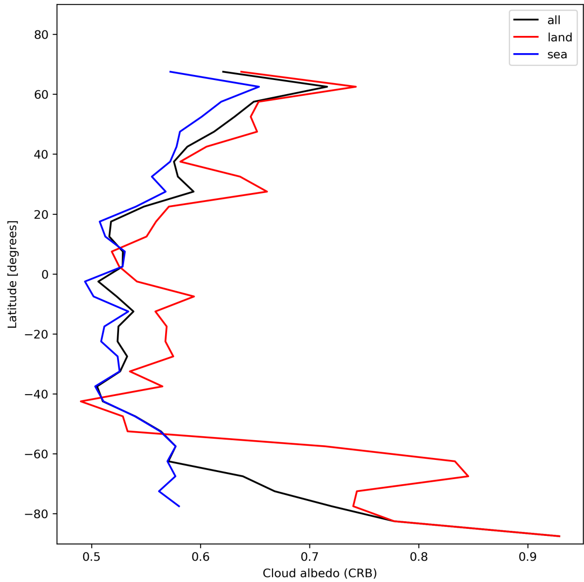
Figure 28: Zonal average of “Cloud albedo (CRB)” for 2024-01-21 to 2024-01-22.
