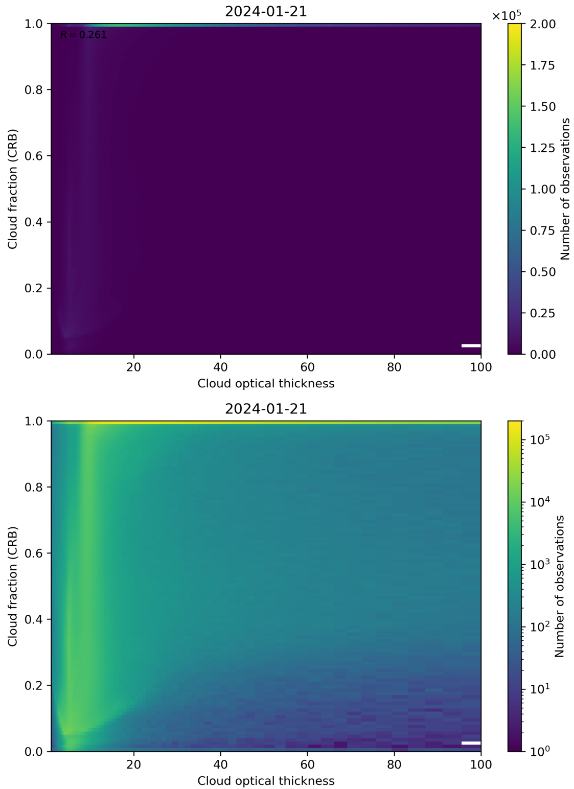
Figure 84: Scatter density plot of “Cloud optical thickness” against “Cloud fraction (CRB)” for 2024-01-21 to 2024-01-22.
