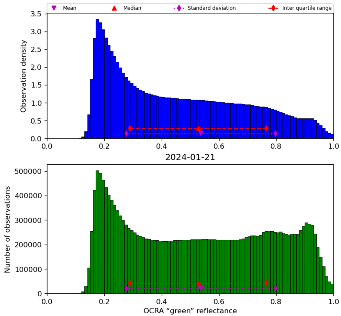
Figure 52: Histogram of “OCRA “green” reflectance” for 2024-01-21 to 2024-01-22
