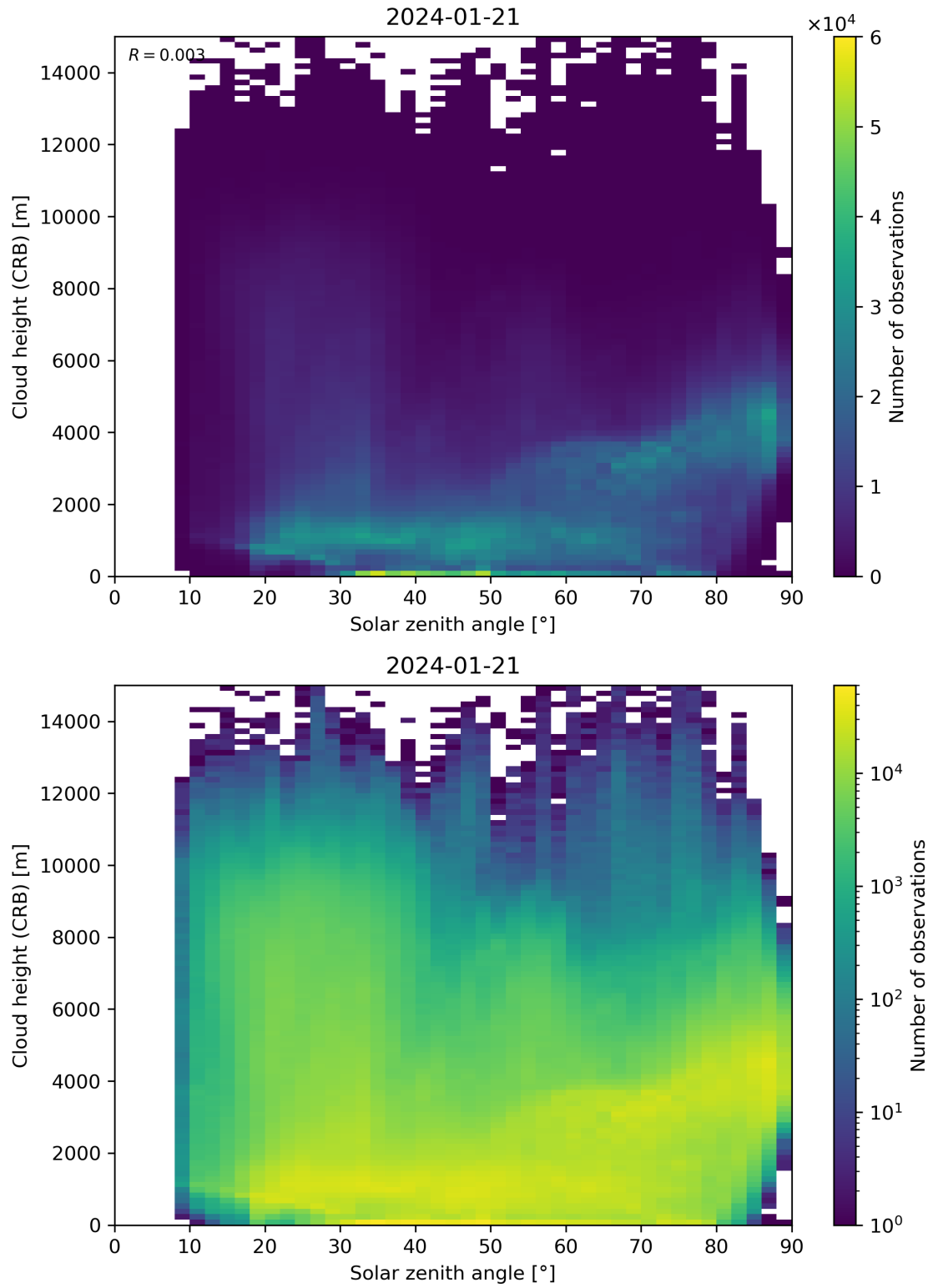
Figure 102: Scatter density plot of “Solar zenith angle” against “Cloud height (CRB)” for 2024-01-21 to 2024-01-22.
