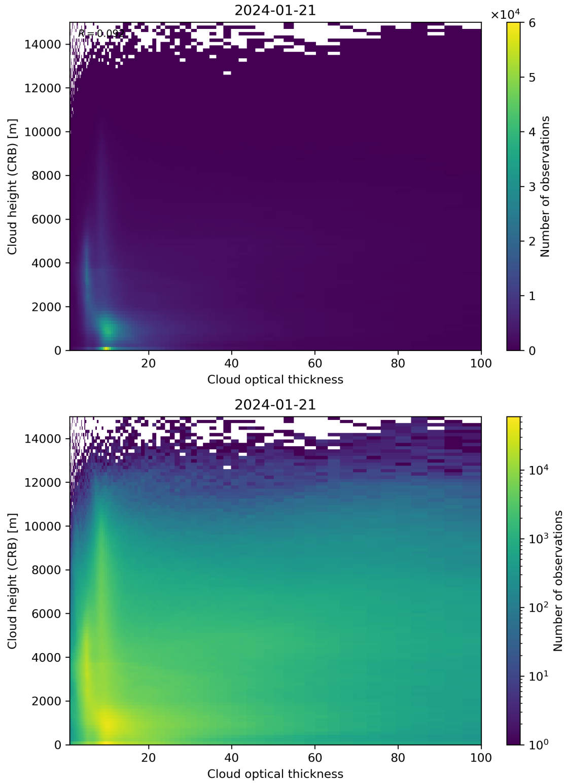
Figure 85: Scatter density plot of “Cloud optical thickness” against “Cloud height (CRB)” for 2024-01-21 to 2024-01-22.
