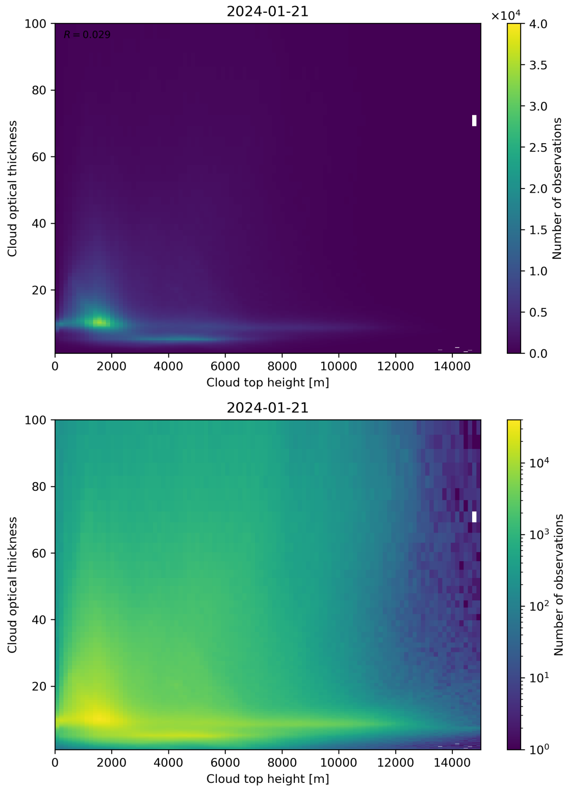
Figure 90: Scatter density plot of “Cloud top height” against “Cloud optical thickness” for 2024-01-21 to 2024-01-22.
