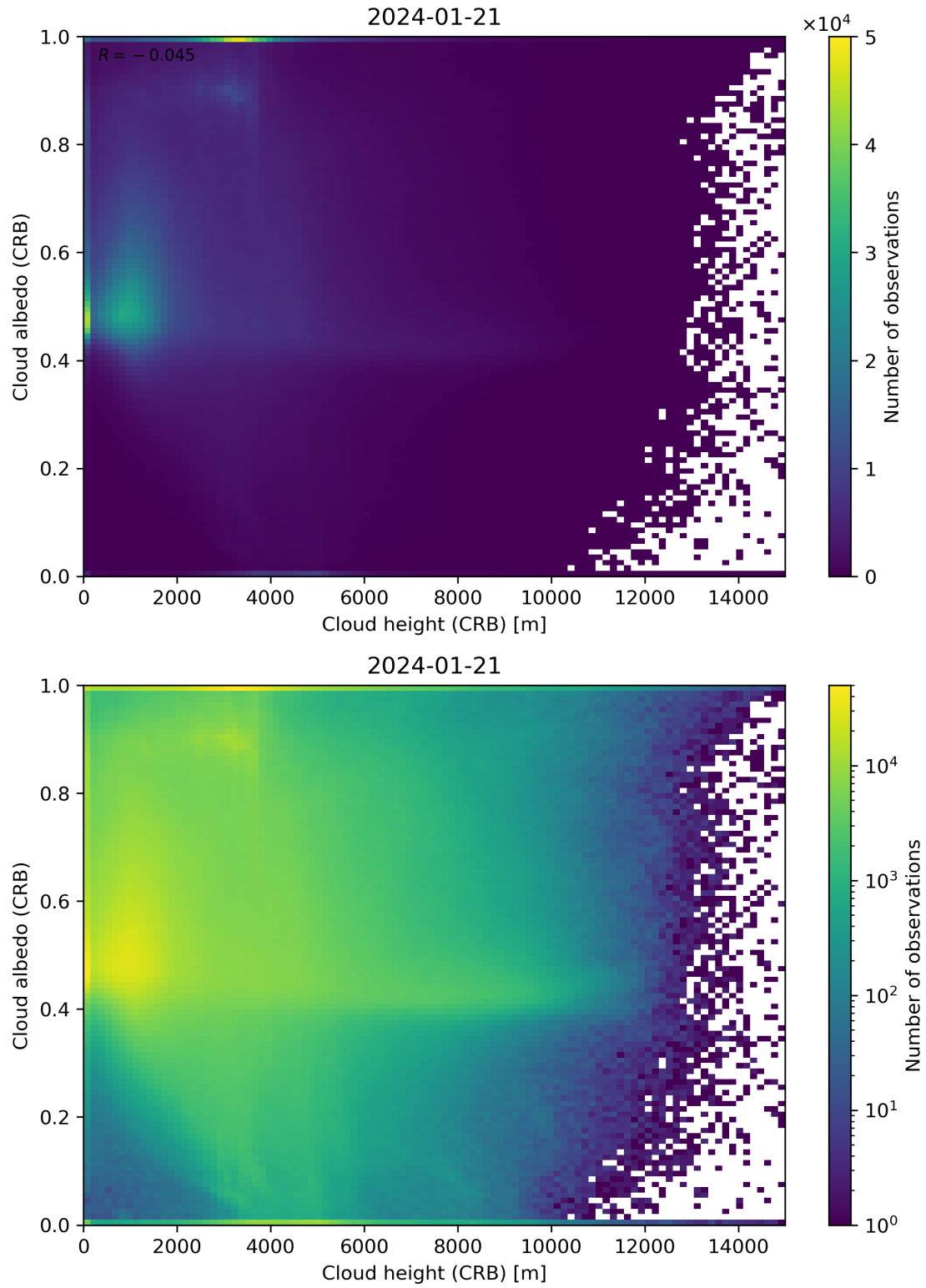
Figure 80: Scatter density plot of “Cloud height (CRB)” against “Cloud albedo (CRB)” for 2024-01-21 to 2024-01-22.
