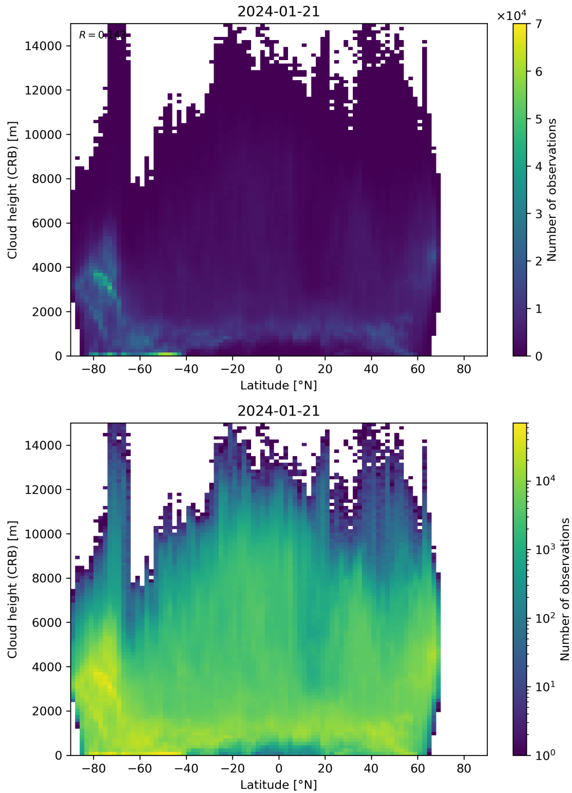
Figure 95: Scatter density plot of “Latitude” against “Cloud height (CRB)” for 2024-01-21 to 2024-01-22.
