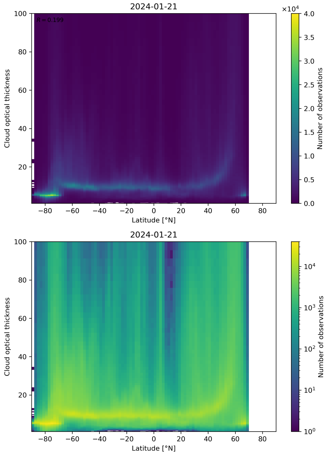
Figure 96: Scatter density plot of “Latitude” against “Cloud optical thickness” for 2024-01-21 to 2024-01-22.
