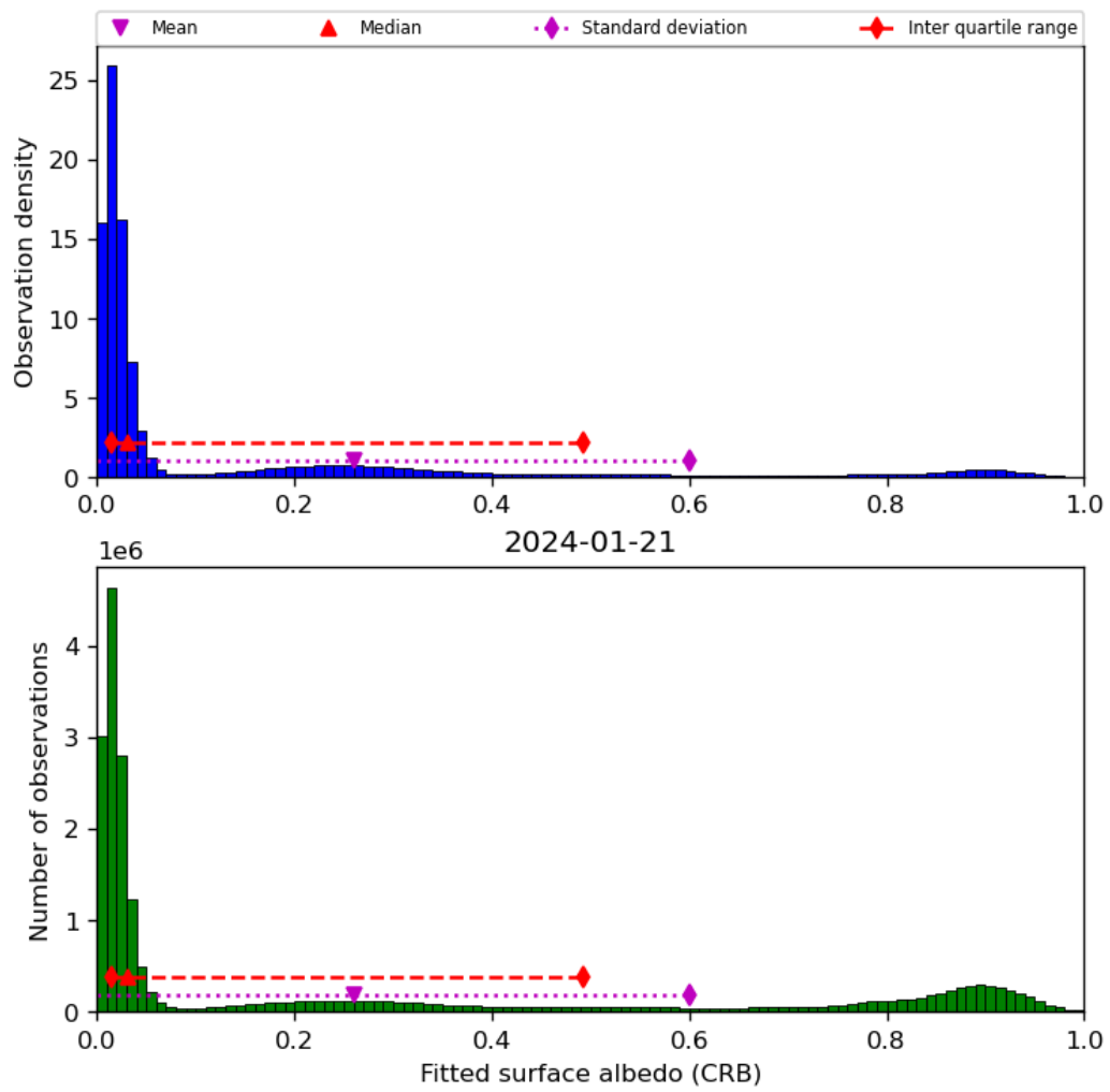
Figure 46: Histogram of “Fitted surface albedo (CRB)” for 2024-01-21 to 2024-01-22
