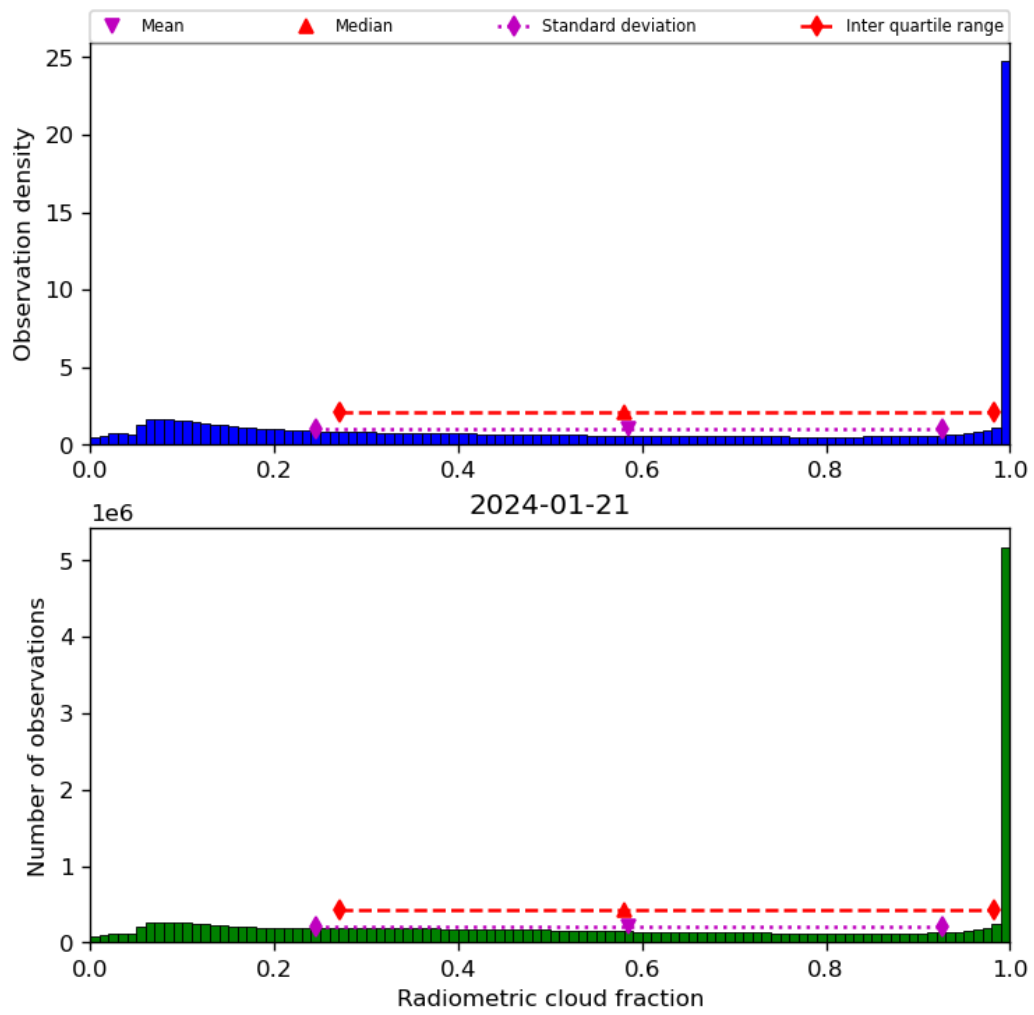
Figure 39: Histogram of “Radiometric cloud fraction” for 2024-01-21 to 2024-01-22
