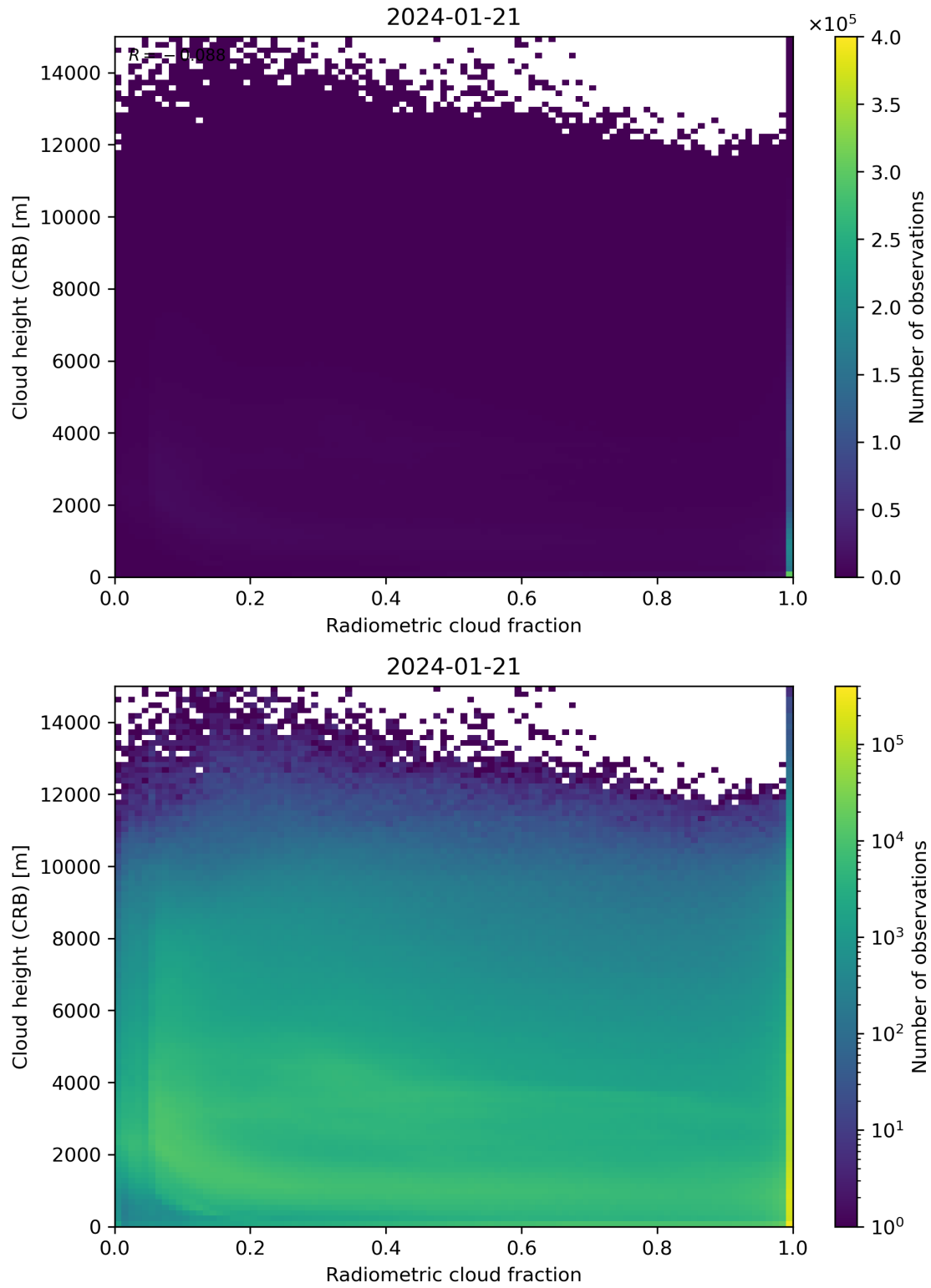
Figure 74: Scatter density plot of “Radiometric cloud fraction” against “Cloud height (CRB)” for 2024-01-21 to 2024-01-22.
