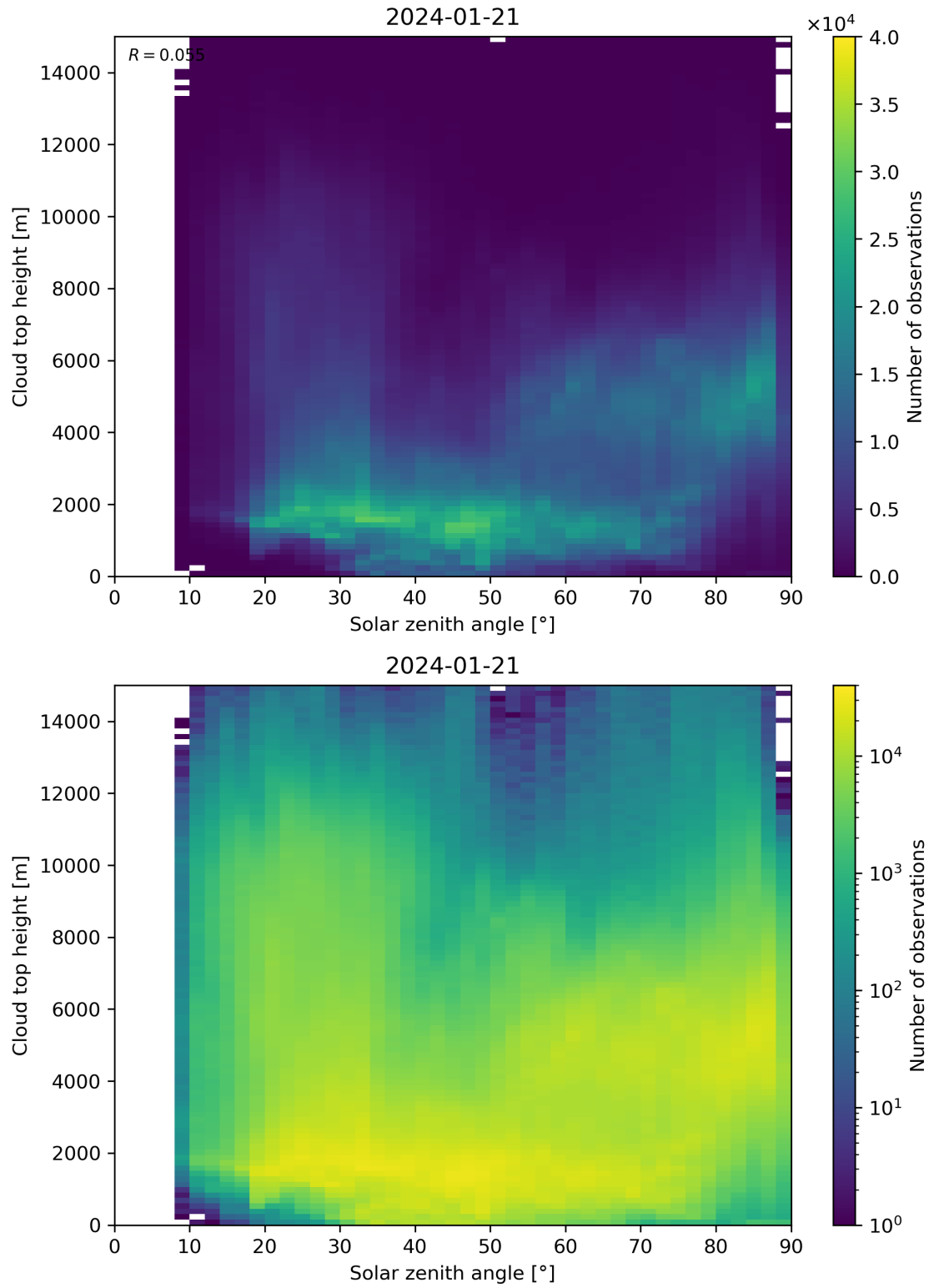
Figure 104: Scatter density plot of “Solar zenith angle” against “Cloud top height” for 2024-01-21 to 2024-01-22.
