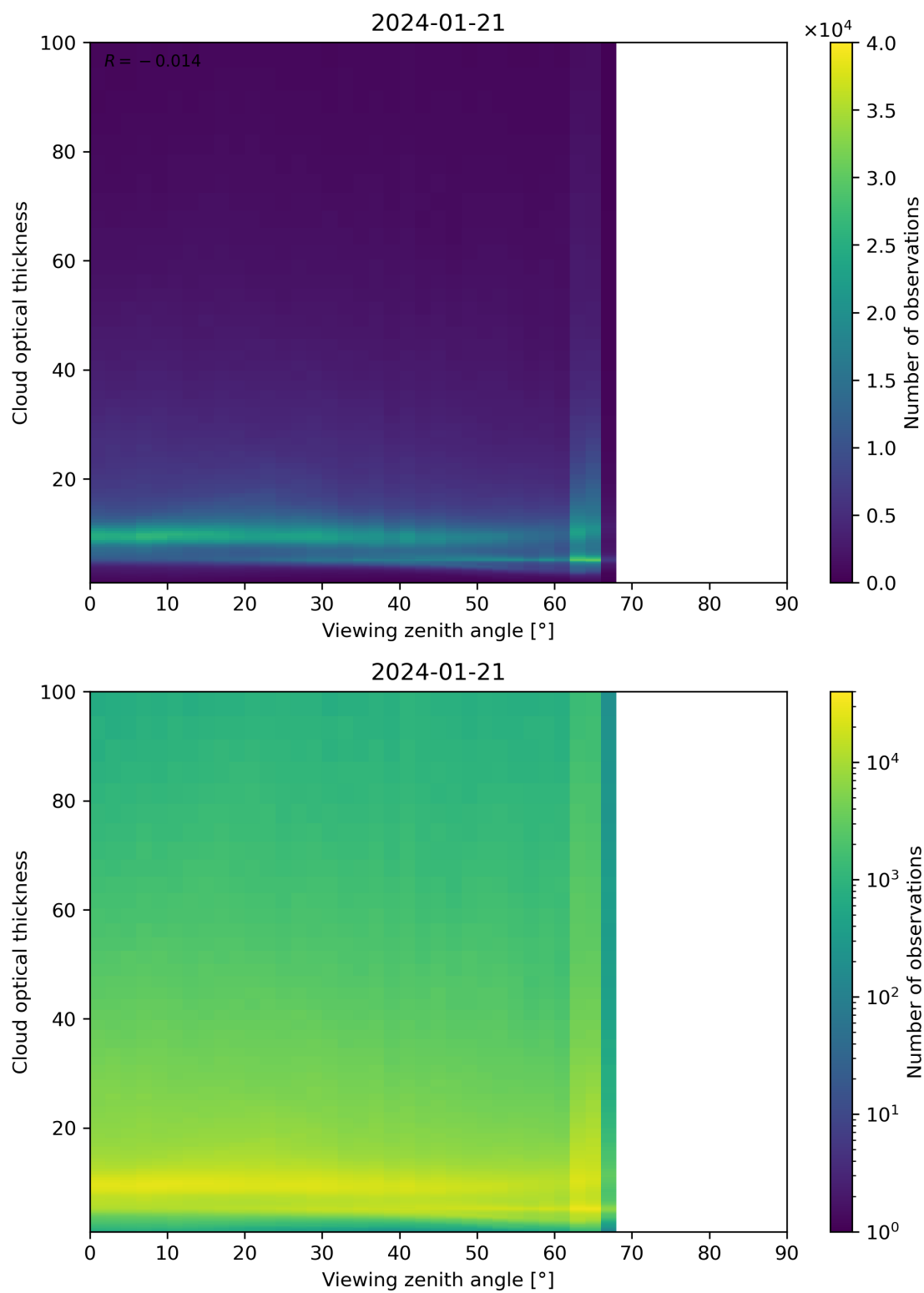
Figure 111: Scatter density plot of “Viewing zenith angle” against “Cloud optical thickness” for 2024-01-21 to 2024-01-22.
