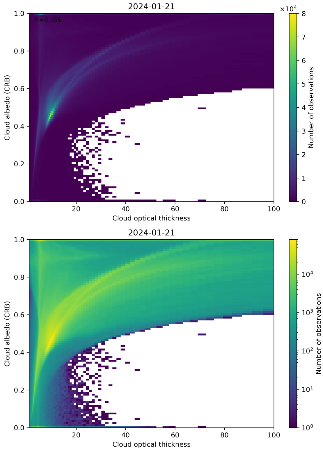
Figure 82: Scatter density plot of “Cloud optical thickness” against “Cloud albedo (CRB)” for 2024-01-21 to 2024-01-22.
