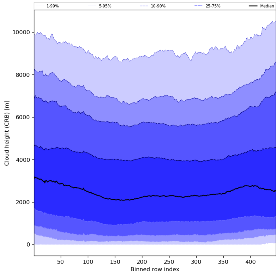
Figure 59: Along track statistics of “Cloud height (CRB)” for 2024-01-21 to 2024-01-22
