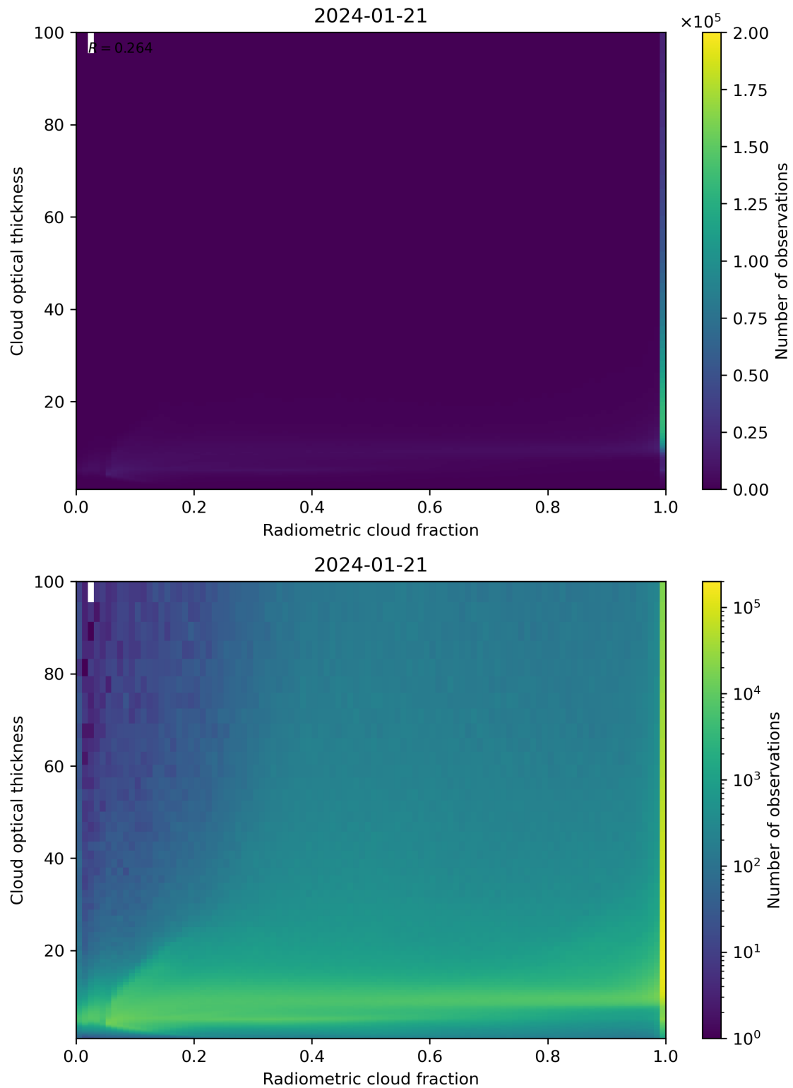
Figure 75: Scatter density plot of “Radiometric cloud fraction” against “Cloud optical thickness” for 2024-01-21 to 2024-01-22.
