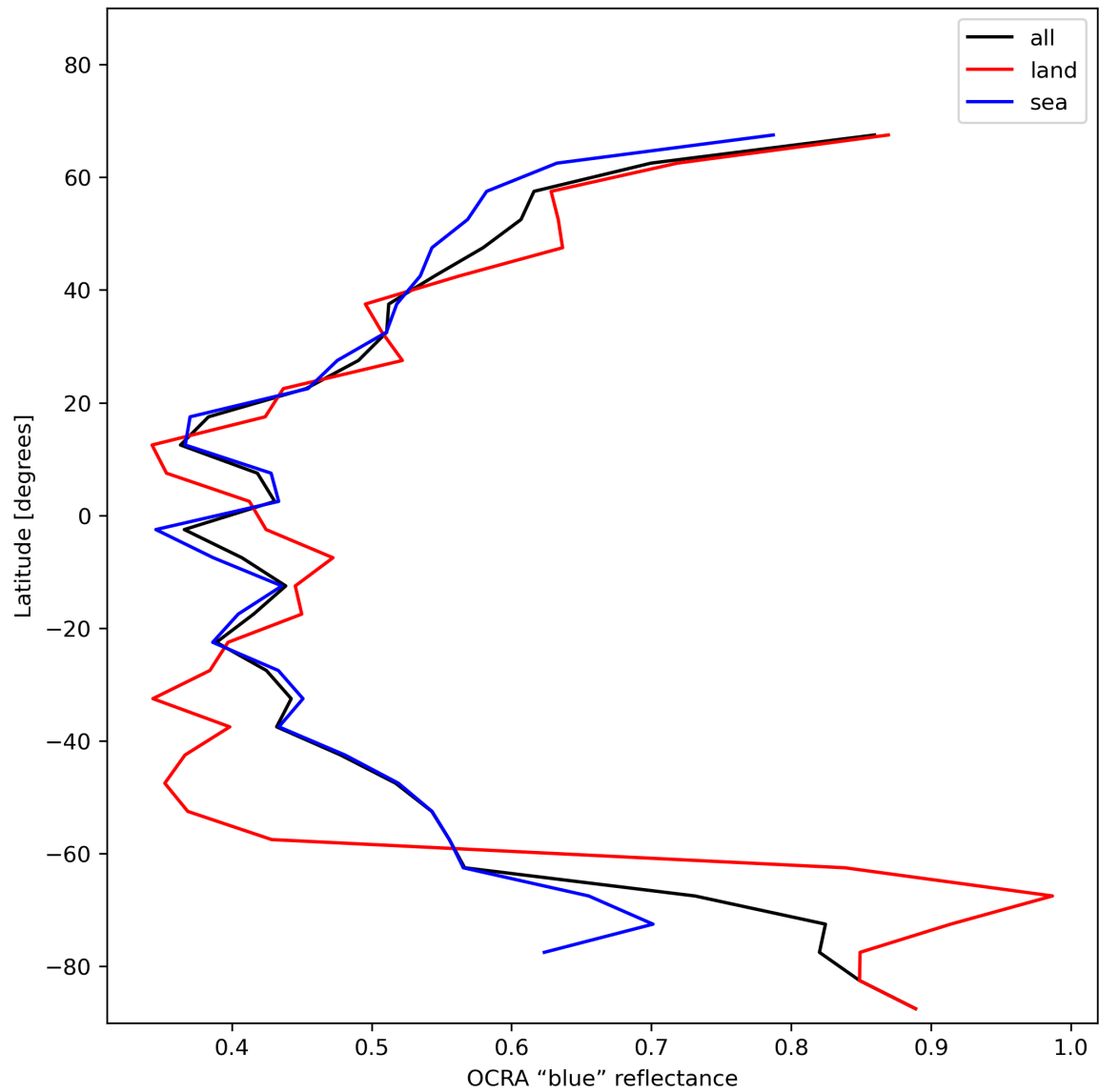
Figure 35: Zonal average of “OCRA “blue” reflectance” for 2024-01-21 to 2024-01-22.
