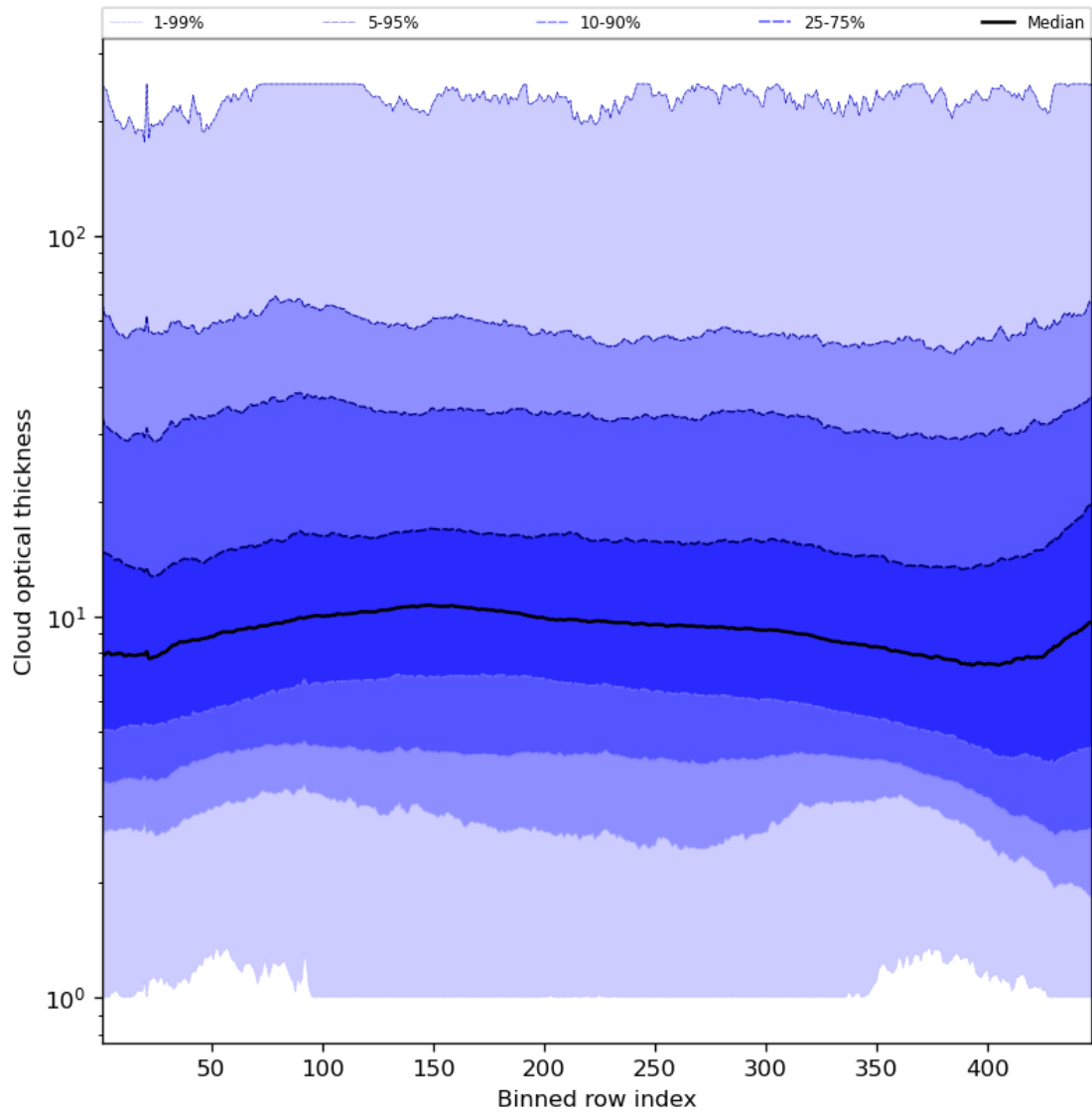
Figure 57: Along track statistics of “Cloud optical thickness” for 2024-01-21 to 2024-01-22
