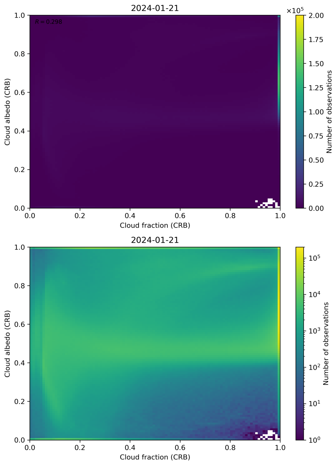
Figure 77: Scatter density plot of “Cloud fraction (CRB)” against “Cloud albedo (CRB)” for 2024-01-21 to 2024-01-22.
