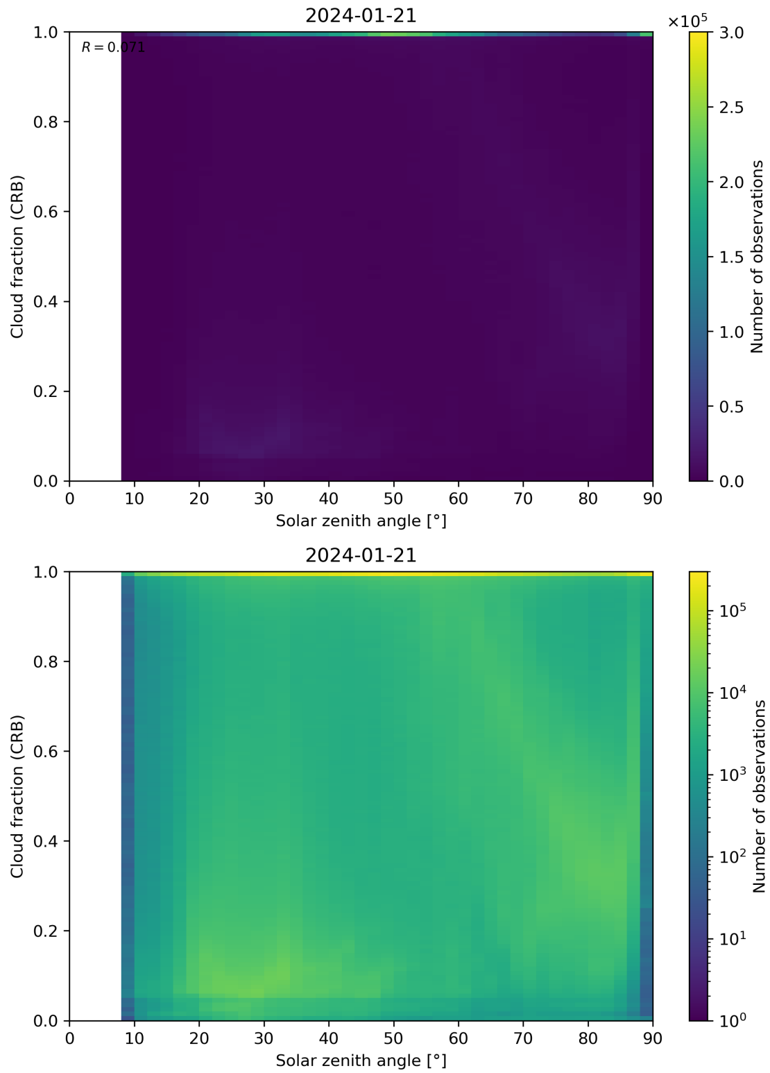
Figure 101: Scatter density plot of “Solar zenith angle” against “Cloud fraction (CRB)” for 2024-01-21 to 2024-01-22.
