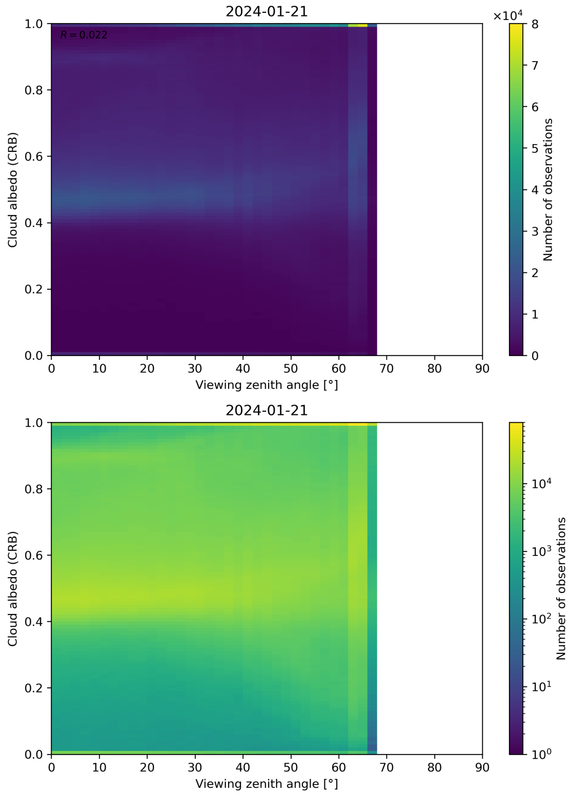
Figure 106: Scatter density plot of “Viewing zenith angle” against “Cloud albedo (CRB)” for 2024-01-21 to 2024-01-22.
