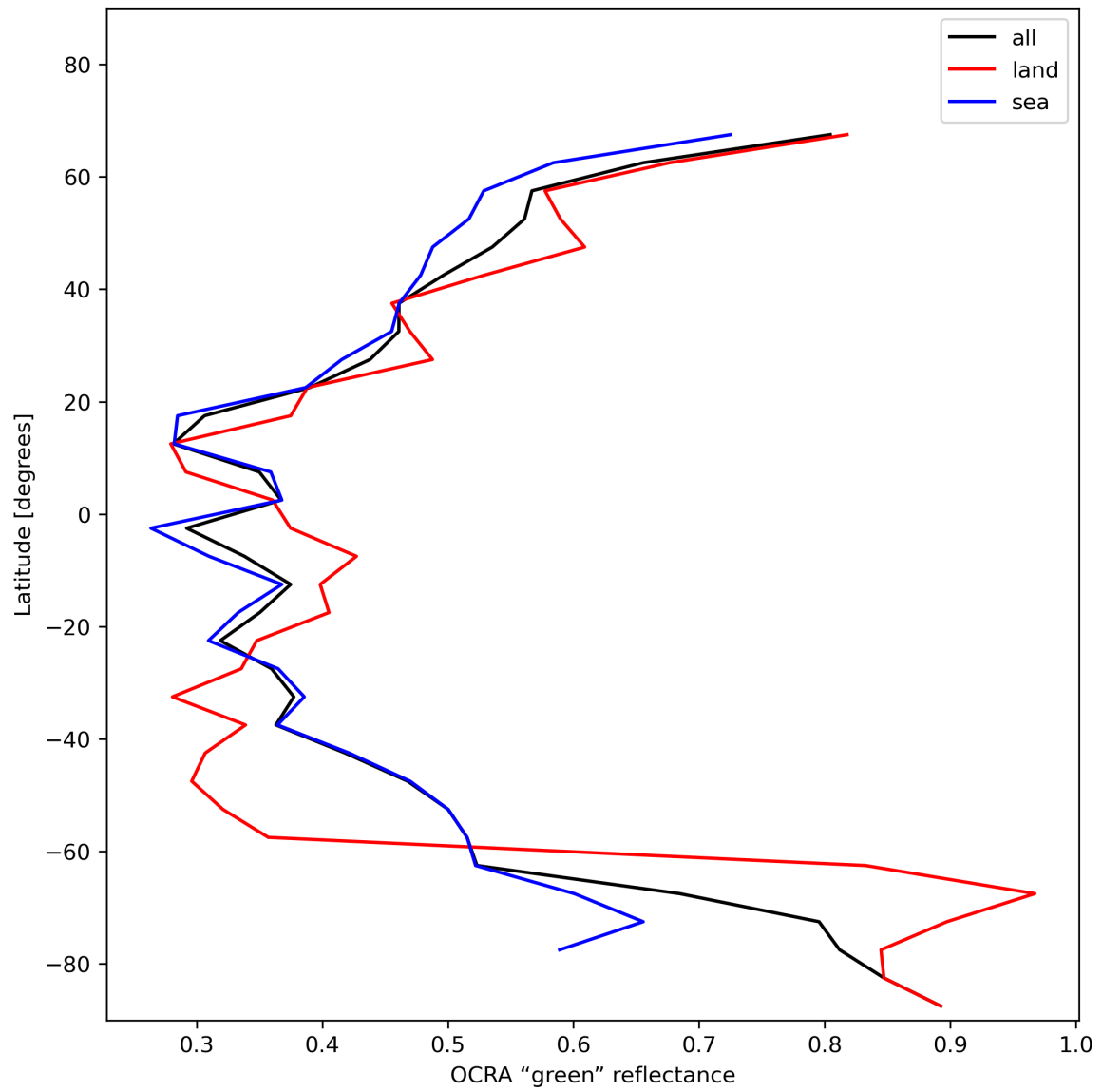
Figure 36: Zonal average of “OCRA “green” reflectance” for 2024-01-21 to 2024-01-22.
