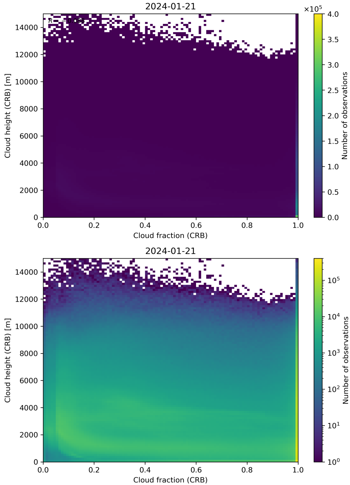
Figure 79: Scatter density plot of “Cloud fraction (CRB)” against “Cloud height (CRB)” for 2024-01-21 to 2024-01-22.
