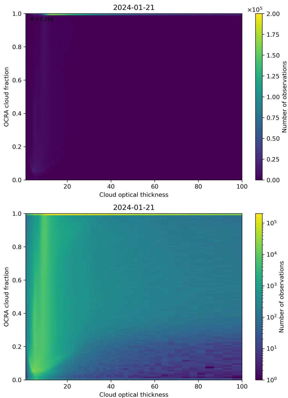
Figure 83: Scatter density plot of “Cloud optical thickness” against “OCRA cloud fraction” for 2024-01-21 to 2024-01-22.
