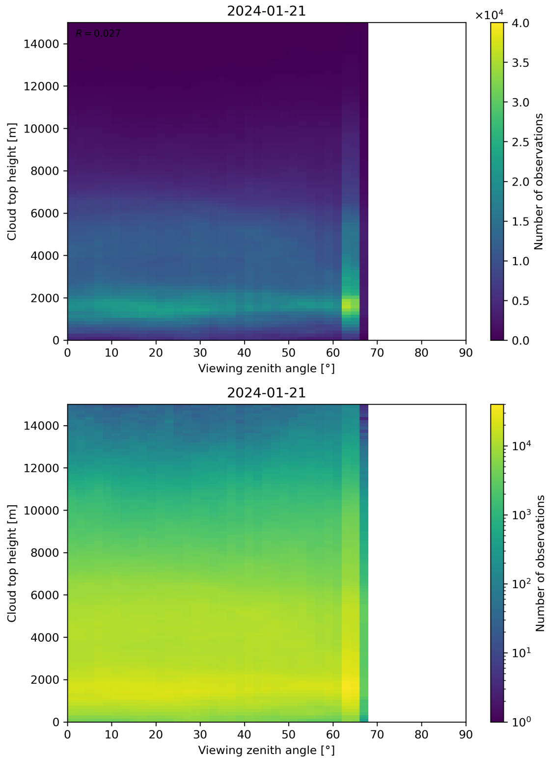
Figure 112: Scatter density plot of “Viewing zenith angle” against “Cloud top height” for 2024-01-21 to 2024-01-22.
