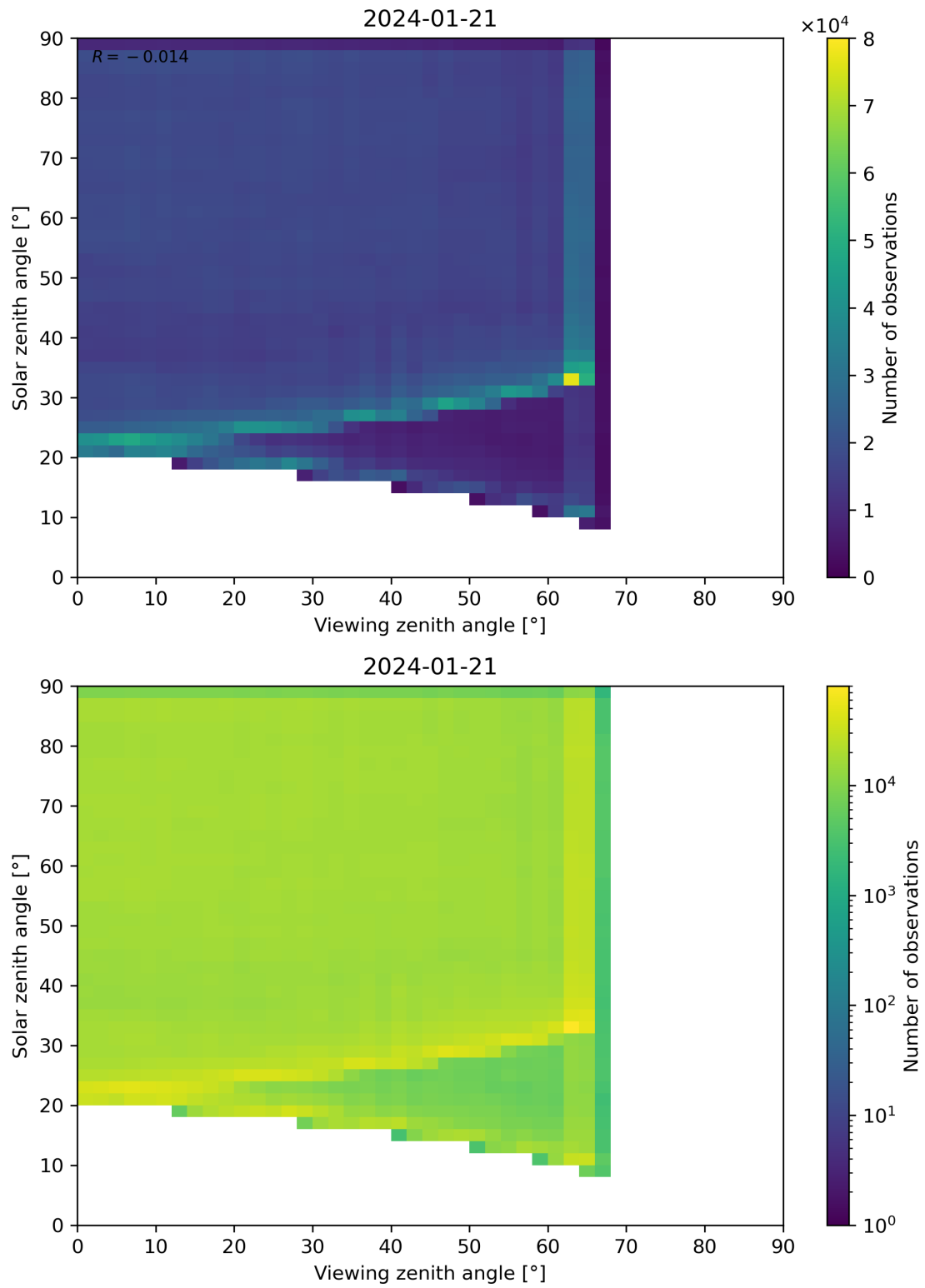
Figure 114: Scatter density plot of “Viewing zenith angle” against “Solar zenith angle” for 2024-01-21 to 2024-01-22.
