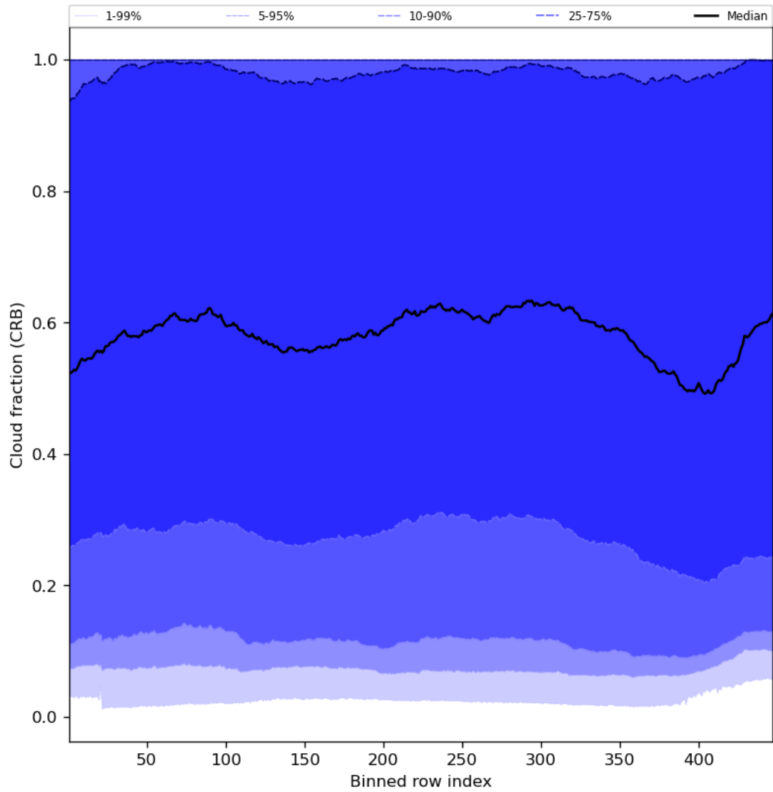
Figure 58: Along track statistics of “Cloud fraction (CRB)” for 2024-01-21 to 2024-01-22
