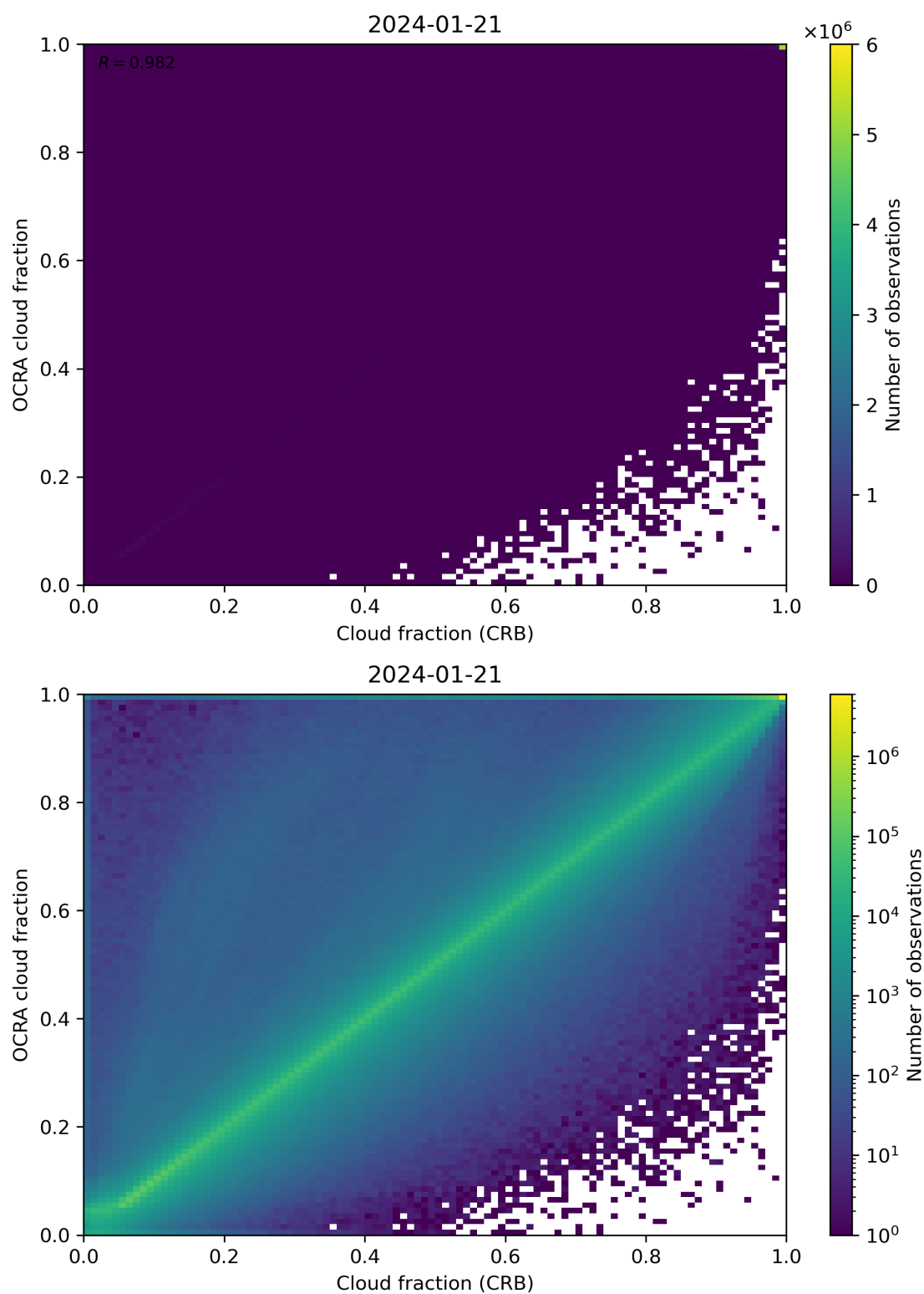
Figure 78: Scatter density plot of “Cloud fraction (CRB)” against “OCRA cloud fraction” for 2024-01-21 to 2024-01-22.
