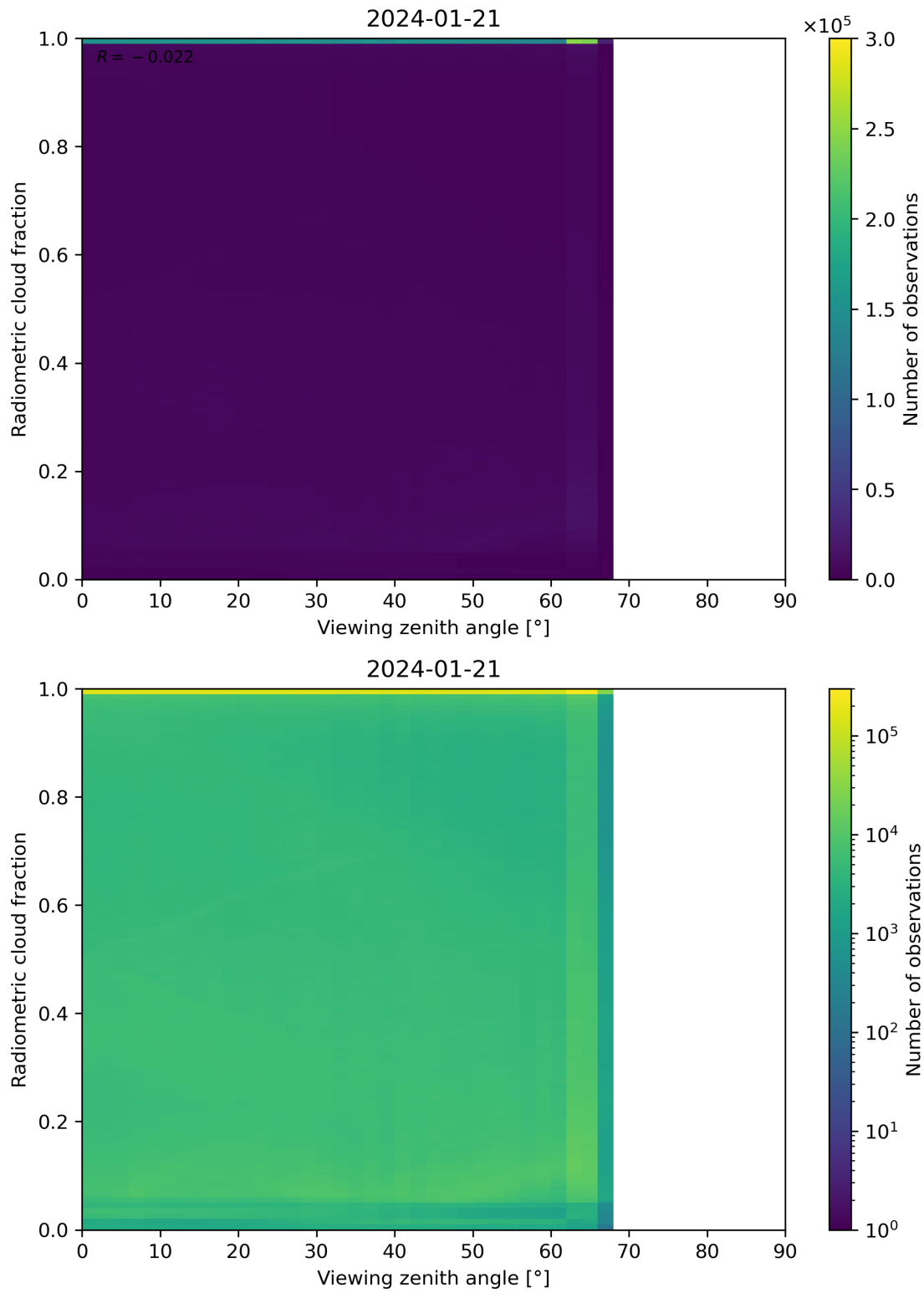
Figure 107: Scatter density plot of “Viewing zenith angle” against “Radiometric cloud fraction” for 2024-01-21 to 2024-01-22.
