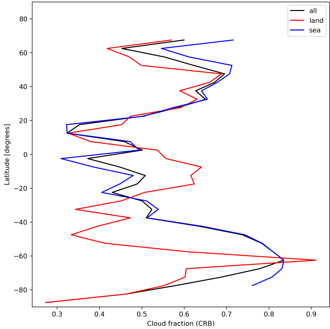
Figure 26: Zonal average of “Cloud fraction (CRB)” for 2024-01-21 to 2024-01-22.
