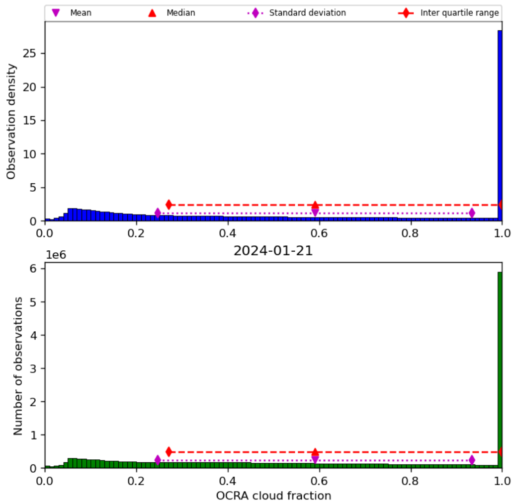
Figure 50: Histogram of “OCRA cloud fraction” for 2024-01-21 to 2024-01-22
