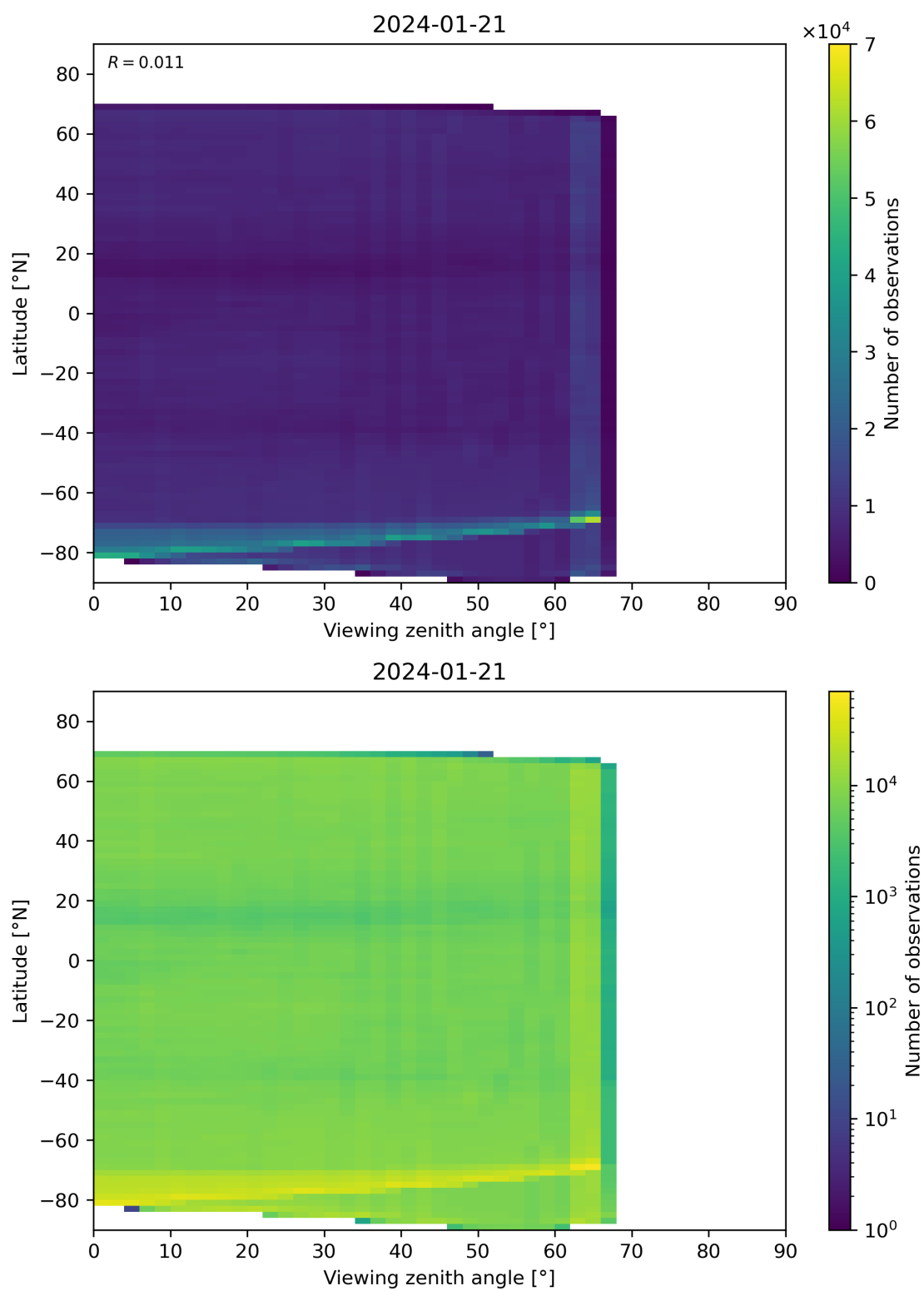
Figure 113: Scatter density plot of “Viewing zenith angle” against “Latitude” for 2024-01-21 to 2024-01-22.
