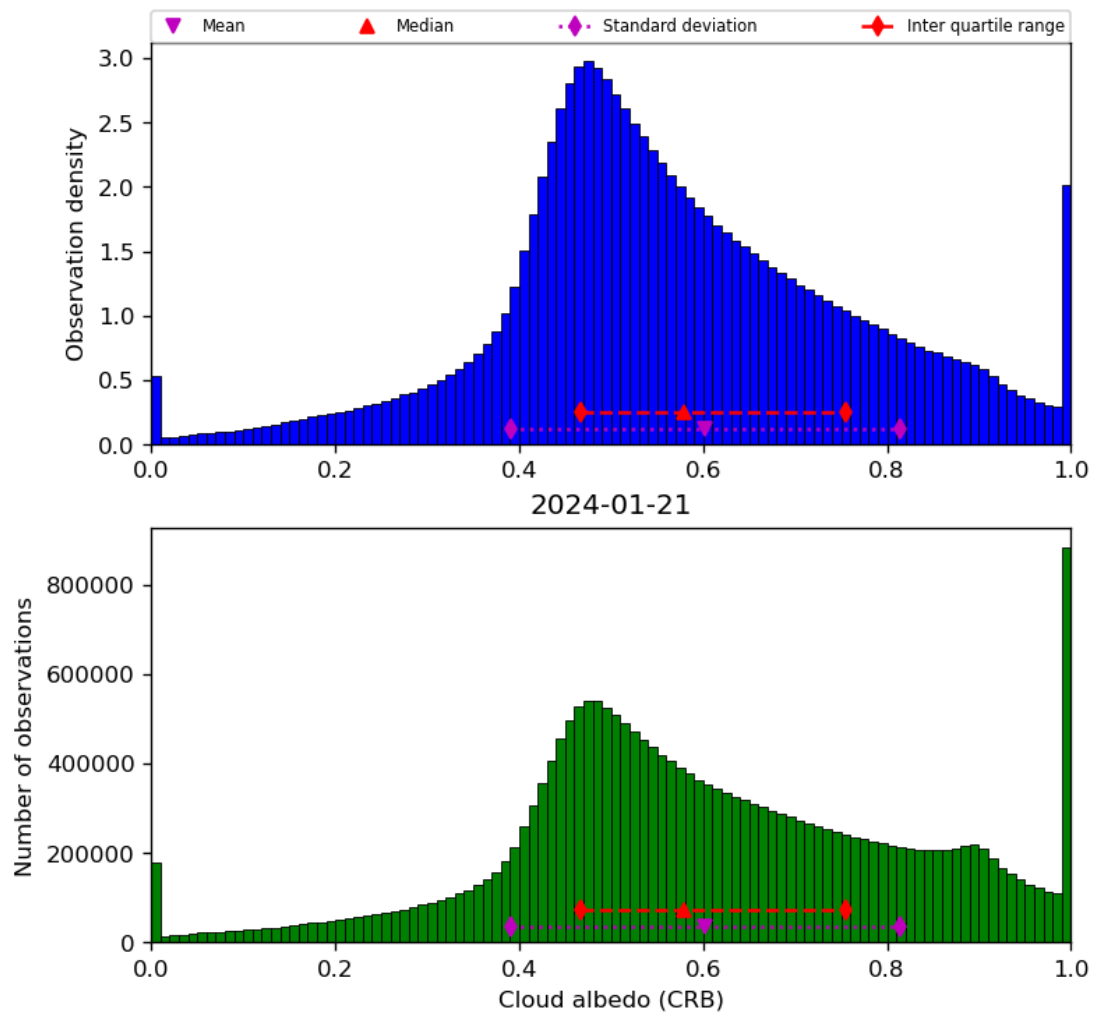
Figure 44: Histogram of “Cloud albedo (CRB)” for 2024-01-21 to 2024-01-22
