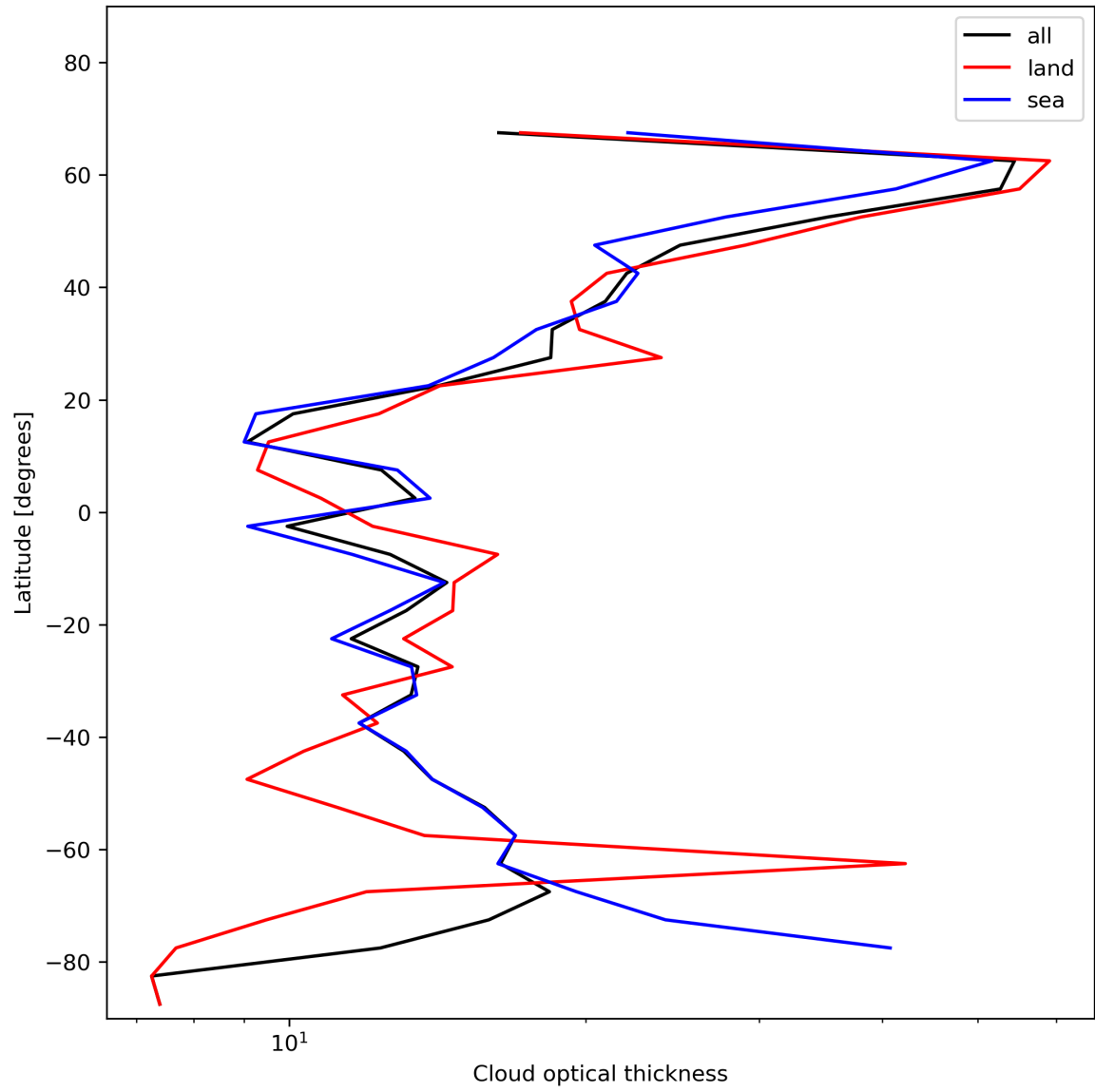
Figure 25: Zonal average of “Cloud optical thickness” for 2024-01-21 to 2024-01-22.
