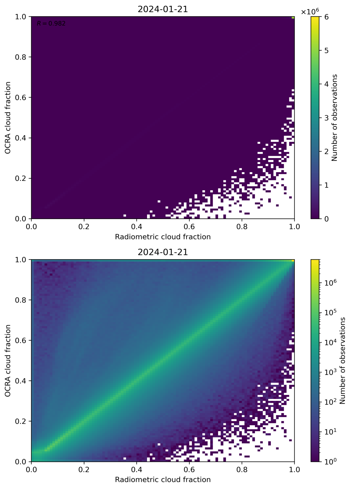
Figure 72: Scatter density plot of “Radiometric cloud fraction” against “OCRA cloud fraction” for 2024-01-21 to 2024-01-22.
