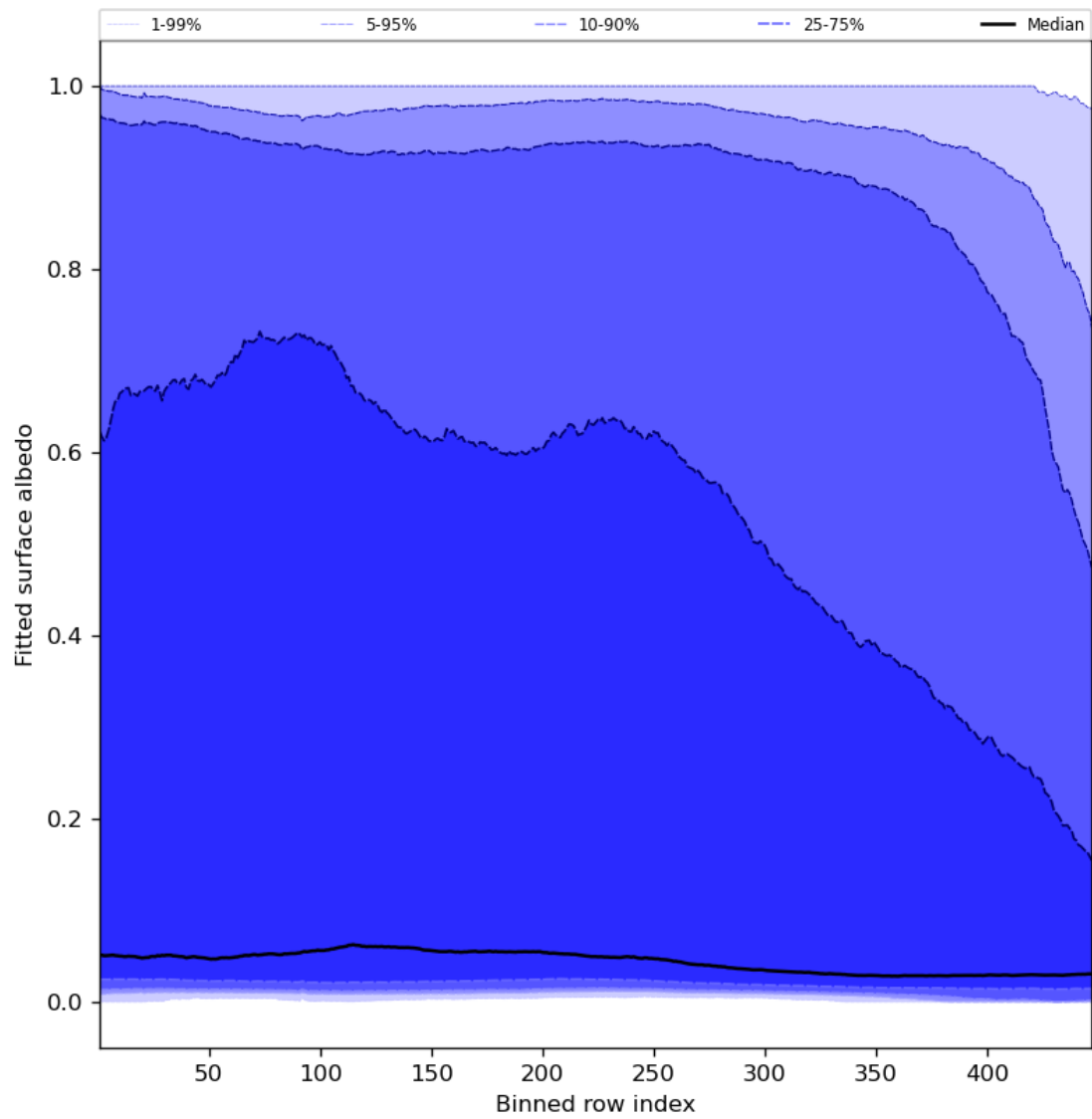
Figure 61: Along track statistics of “Fitted surface albedo” for 2024-01-21 to 2024-01-22
