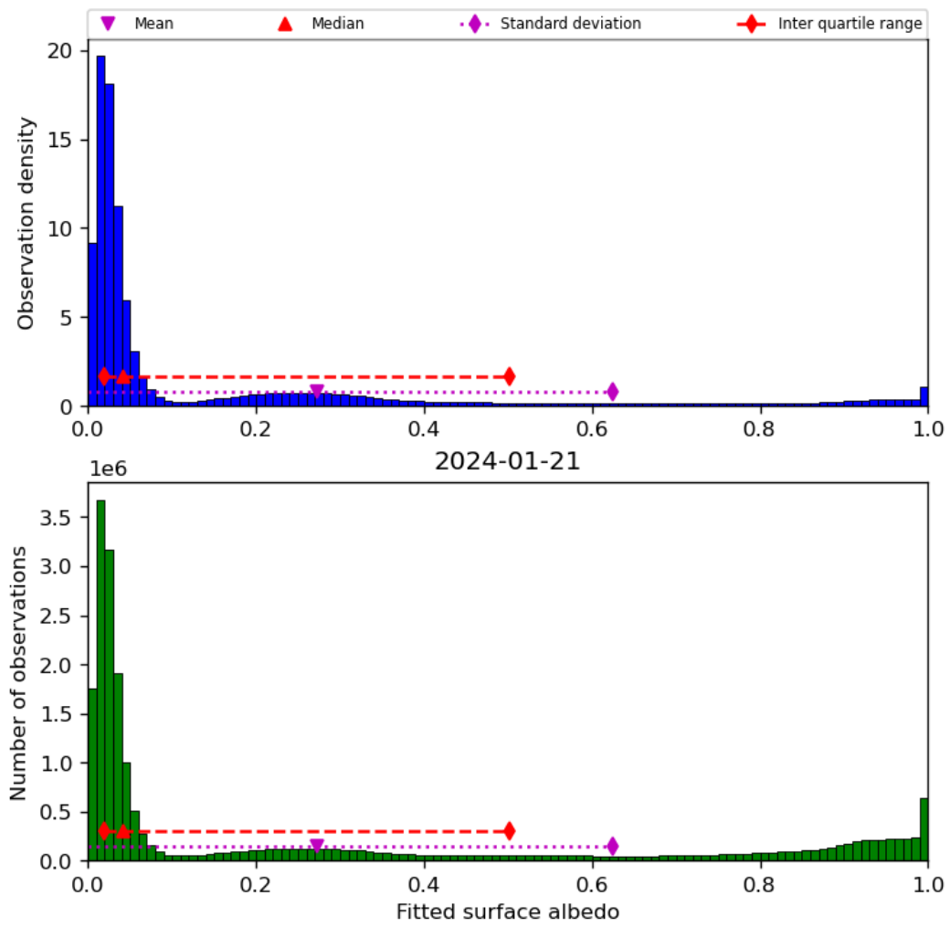
Figure 45: Histogram of “Fitted surface albedo” for 2024-01-21 to 2024-01-22
