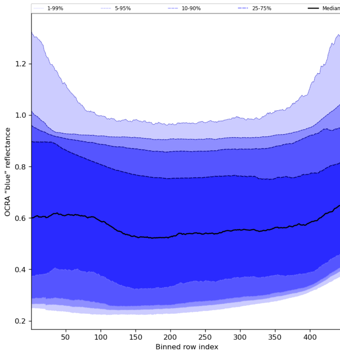
Figure 67: Along track statistics of “OCRA “blue” reflectance” for 2024-01-21 to 2024-01-22
