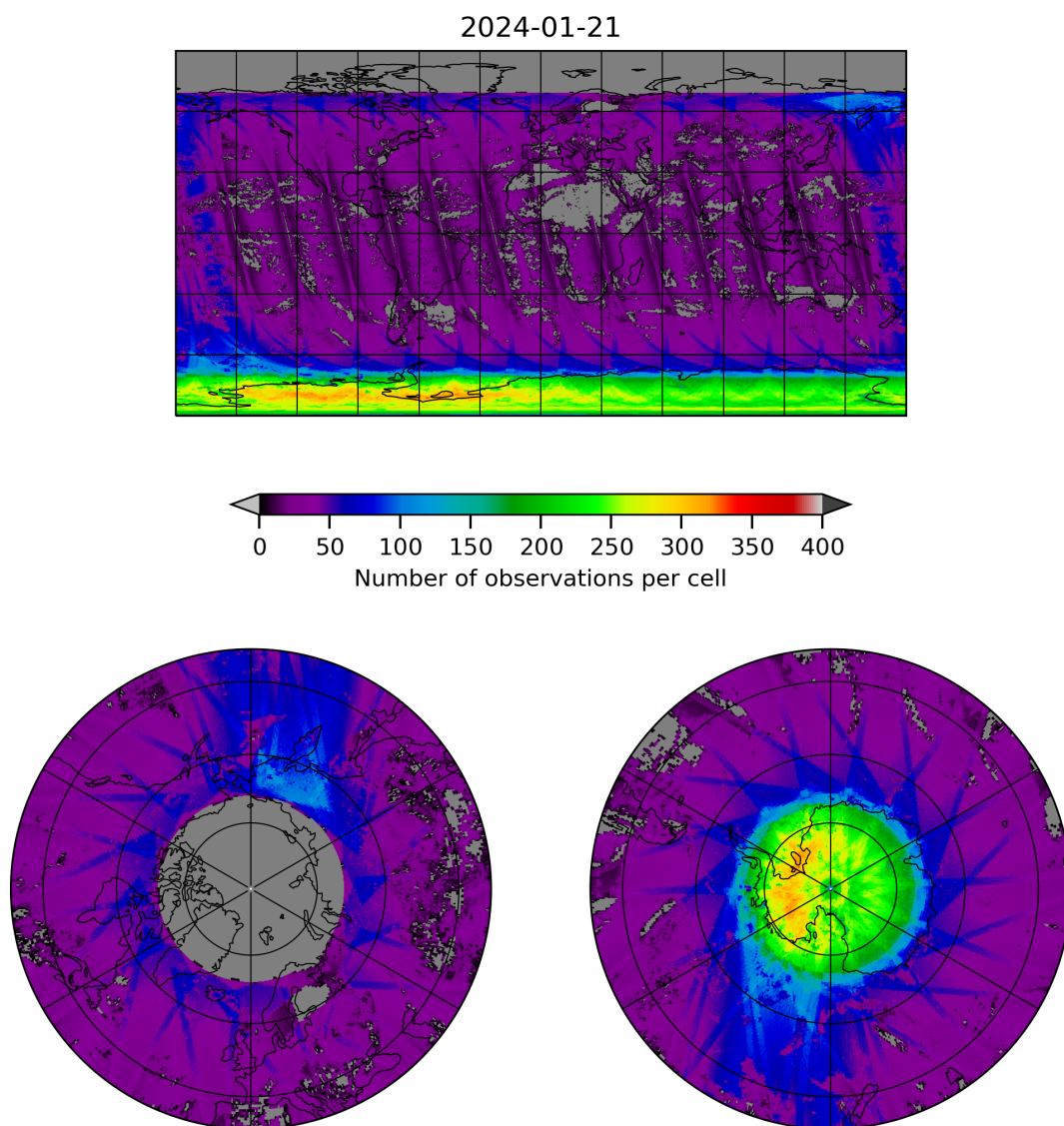
Figure 21: Map of the number of observations for 2024-01-21 to 2024-01-22
