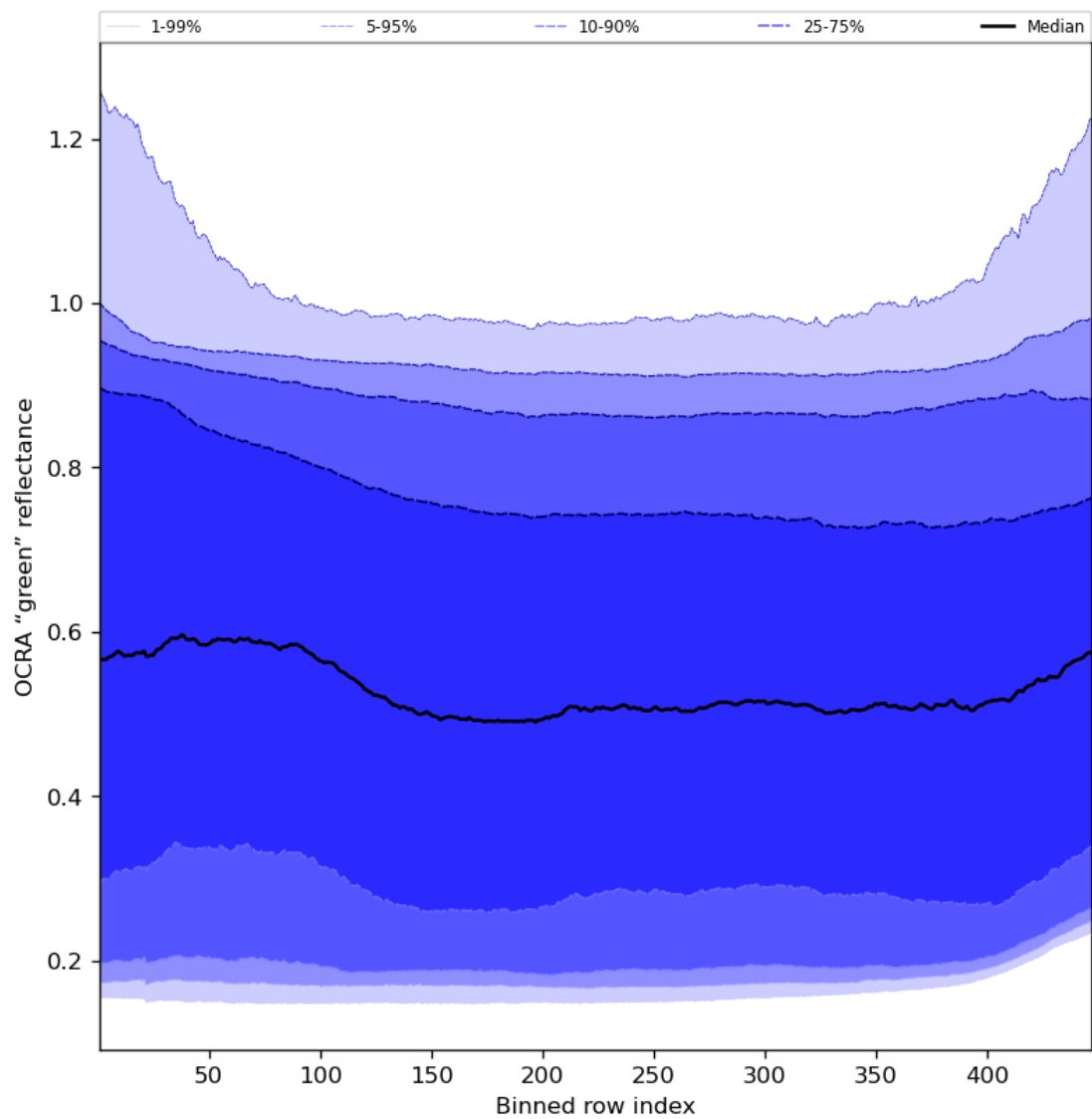
Figure 68: Along track statistics of “OCRA “green” reflectance” for 2024-01-21 to 2024-01-22
