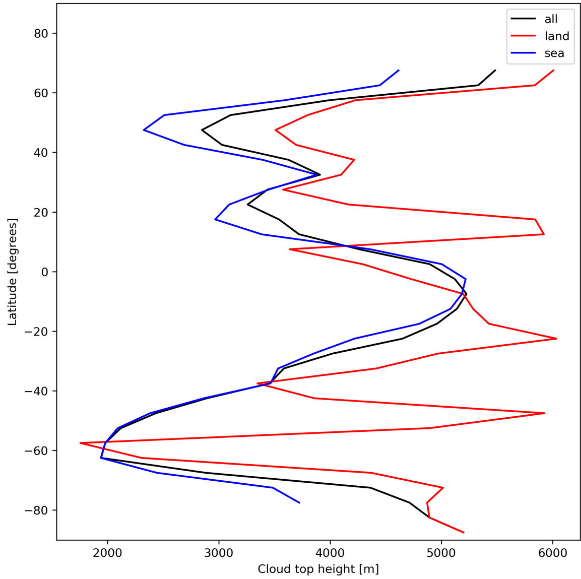
Figure 24: Zonal average of “Cloud top height” for 2024-01-21 to 2024-01-22.
