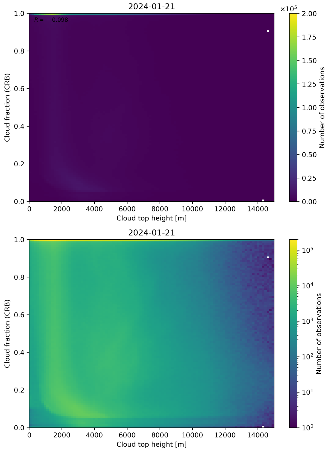
Figure 88: Scatter density plot of “Cloud top height” against “Cloud fraction (CRB)” for 2024-01-21 to 2024-01-22.
