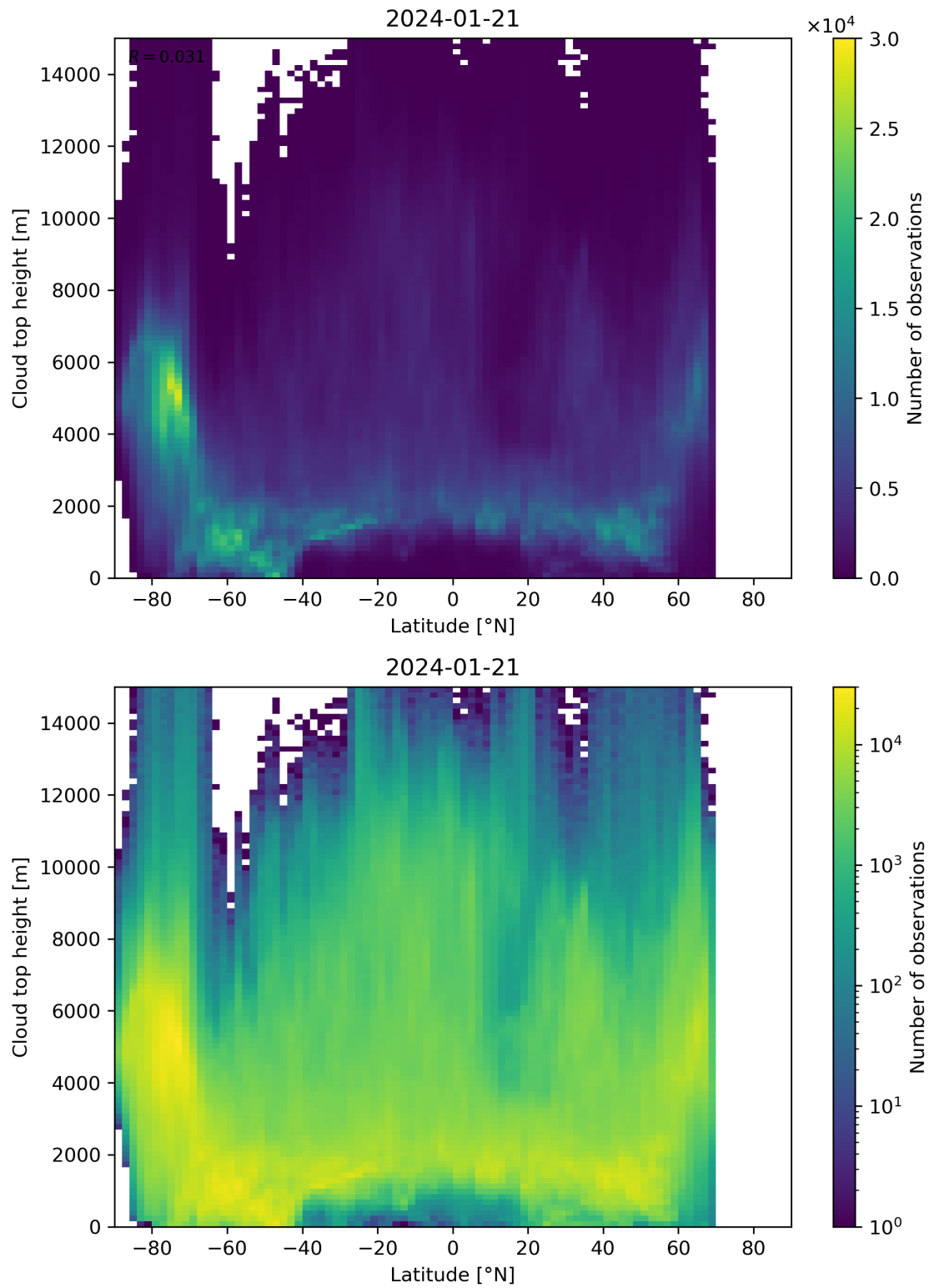
Figure 97: Scatter density plot of “Latitude” against “Cloud top height” for 2024-01-21 to 2024-01-22.
