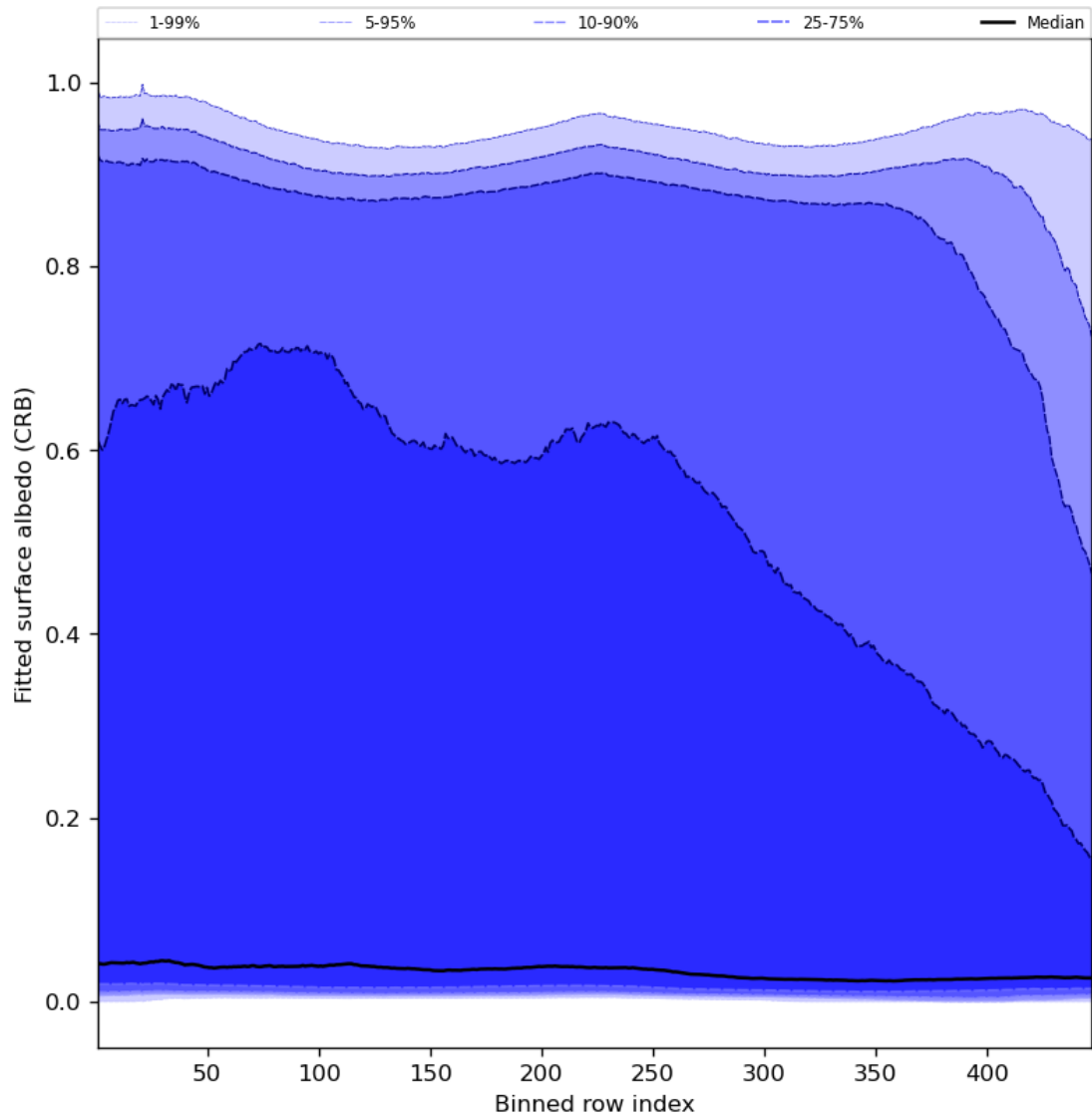
Figure 62: Along track statistics of “Fitted surface albedo (CRB)” for 2024-01-21 to 2024-01-22
