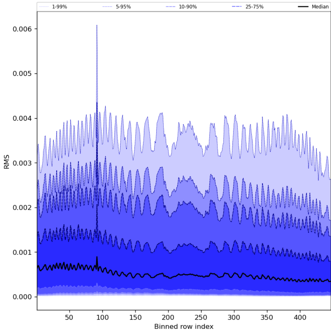
Figure 63: Along track statistics of “RMS” for 2024-01-21 to 2024-01-22
