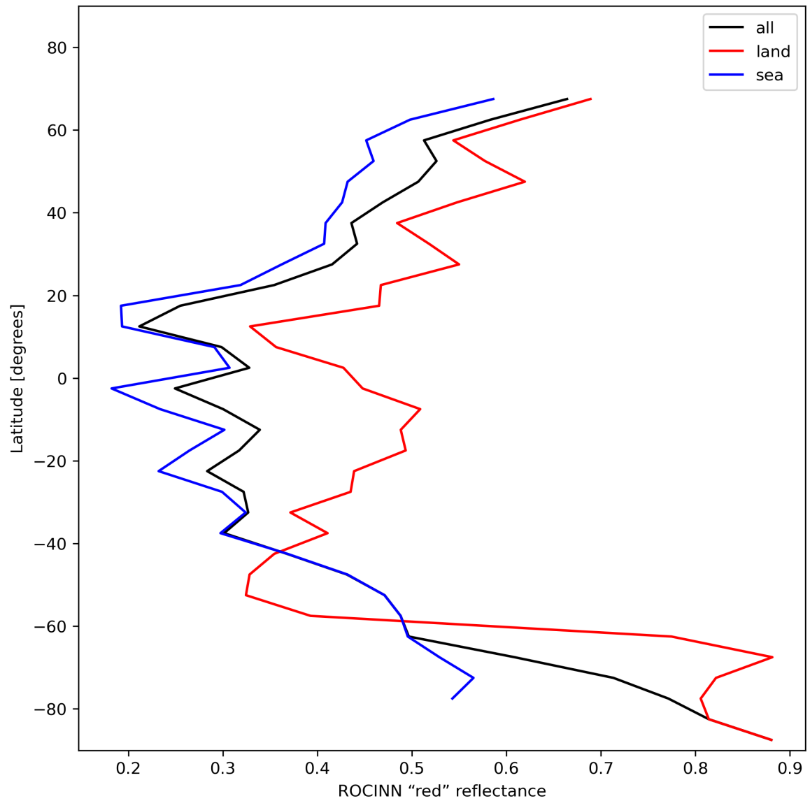
Figure 37: Zonal average of “ROCINN “red” reflectance” for 2024-01-21 to 2024-01-22.
