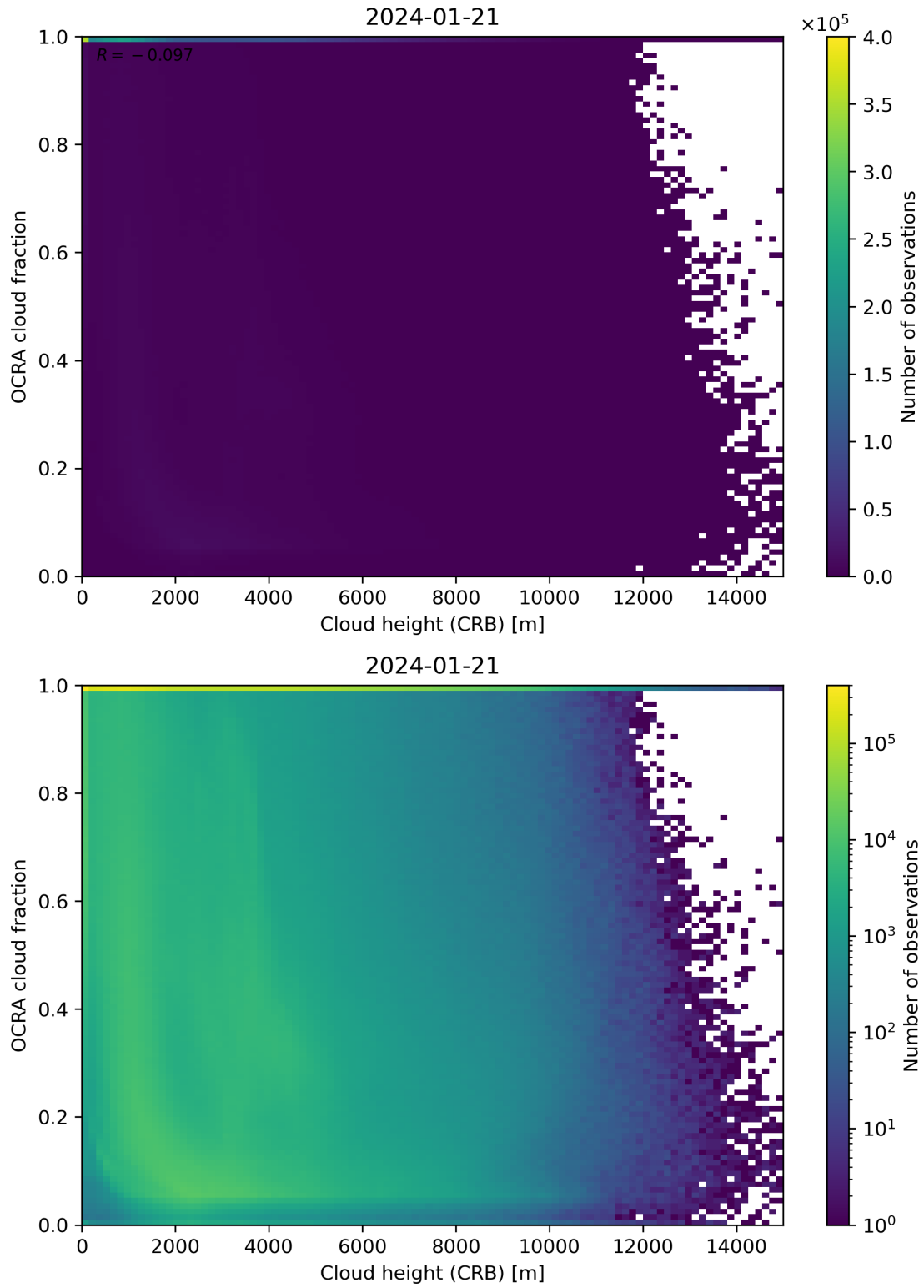
Figure 81: Scatter density plot of “Cloud height (CRB)” against “OCRA cloud fraction” for 2024-01-21 to 2024-01-22.
