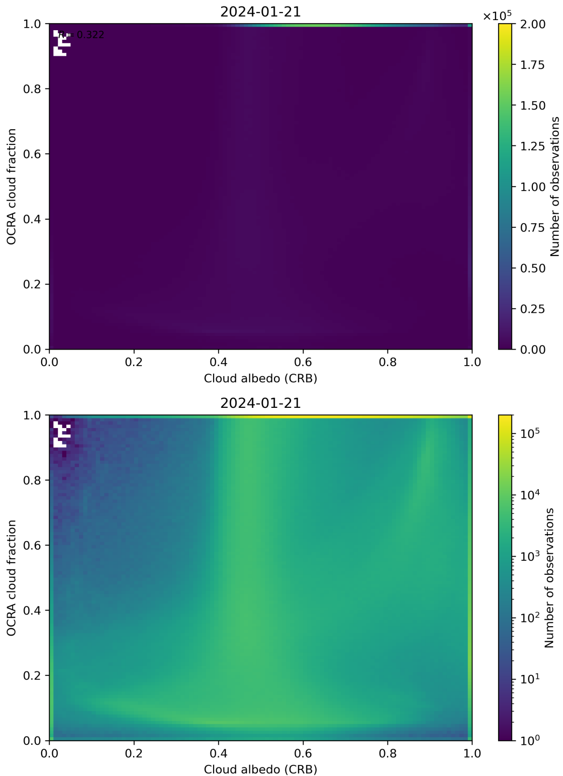
Figure 70: Scatter density plot of “Cloud albedo (CRB)” against “OCRA cloud fraction” for 2024-01-21 to 2024-01-22.
