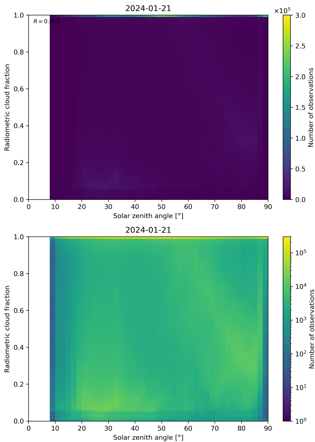
Figure 99: Scatter density plot of “Solar zenith angle” against “Radiometric cloud fraction” for 2024-01-21 to 2024-01-22.
