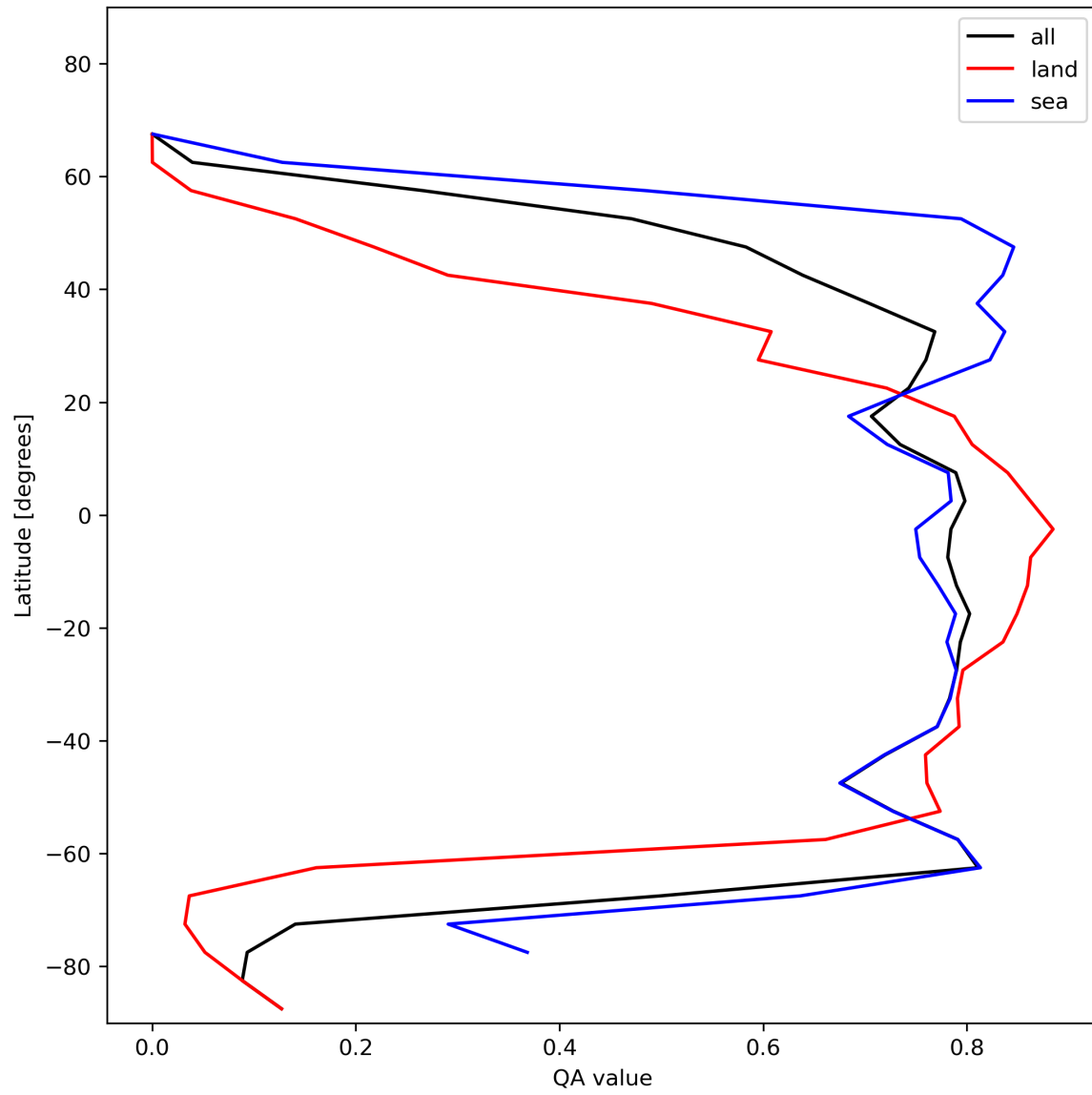
Figure 22: Zonal average of “QA value” for 2024-01-21 to 2024-01-22.
