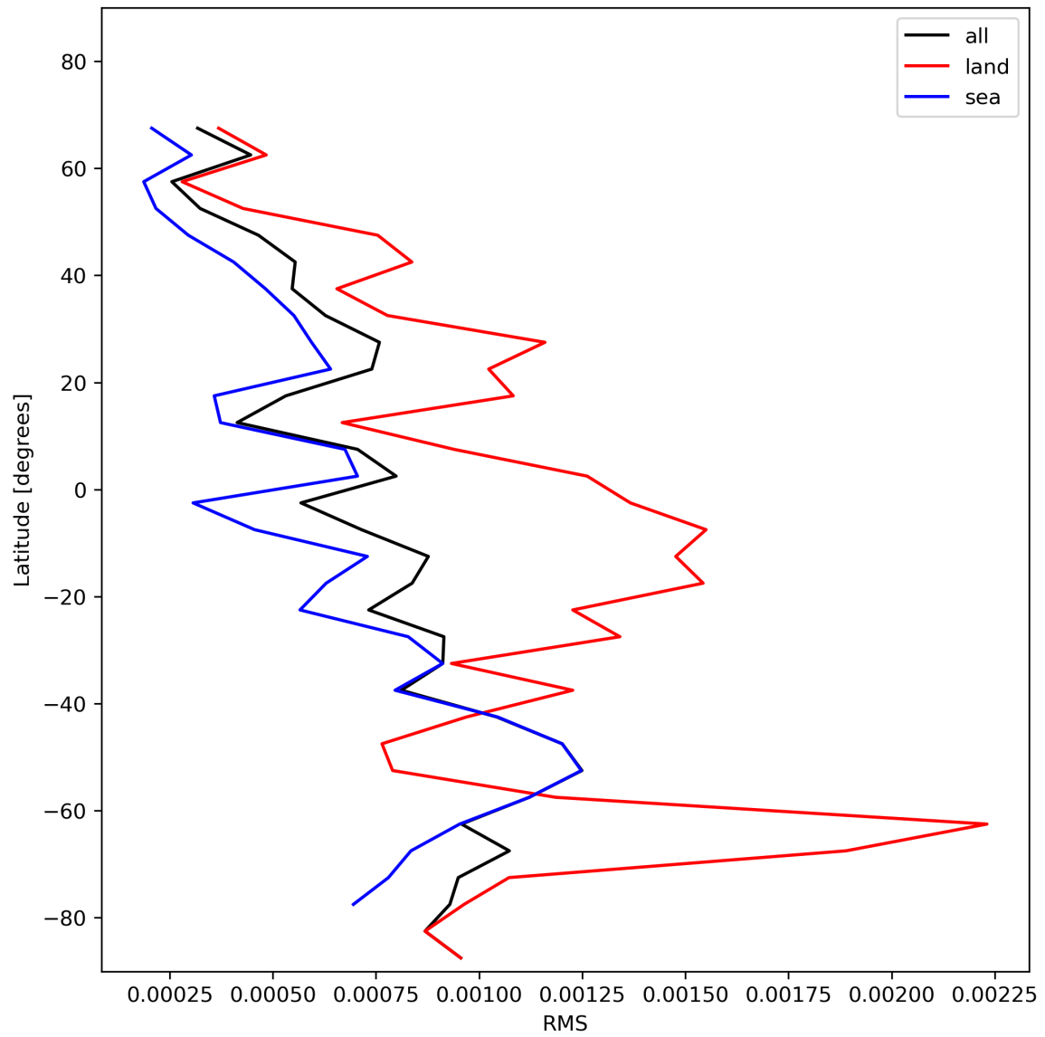
Figure 31: Zonal average of “RMS” for 2024-01-21 to 2024-01-22.
