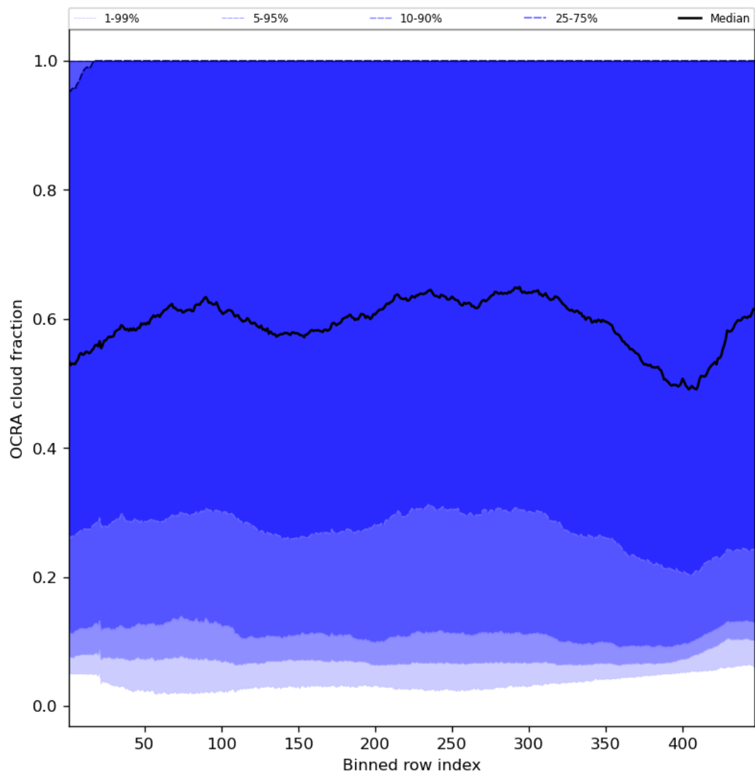
Figure 66: Along track statistics of “OCRA cloud fraction” for 2024-01-21 to 2024-01-22
