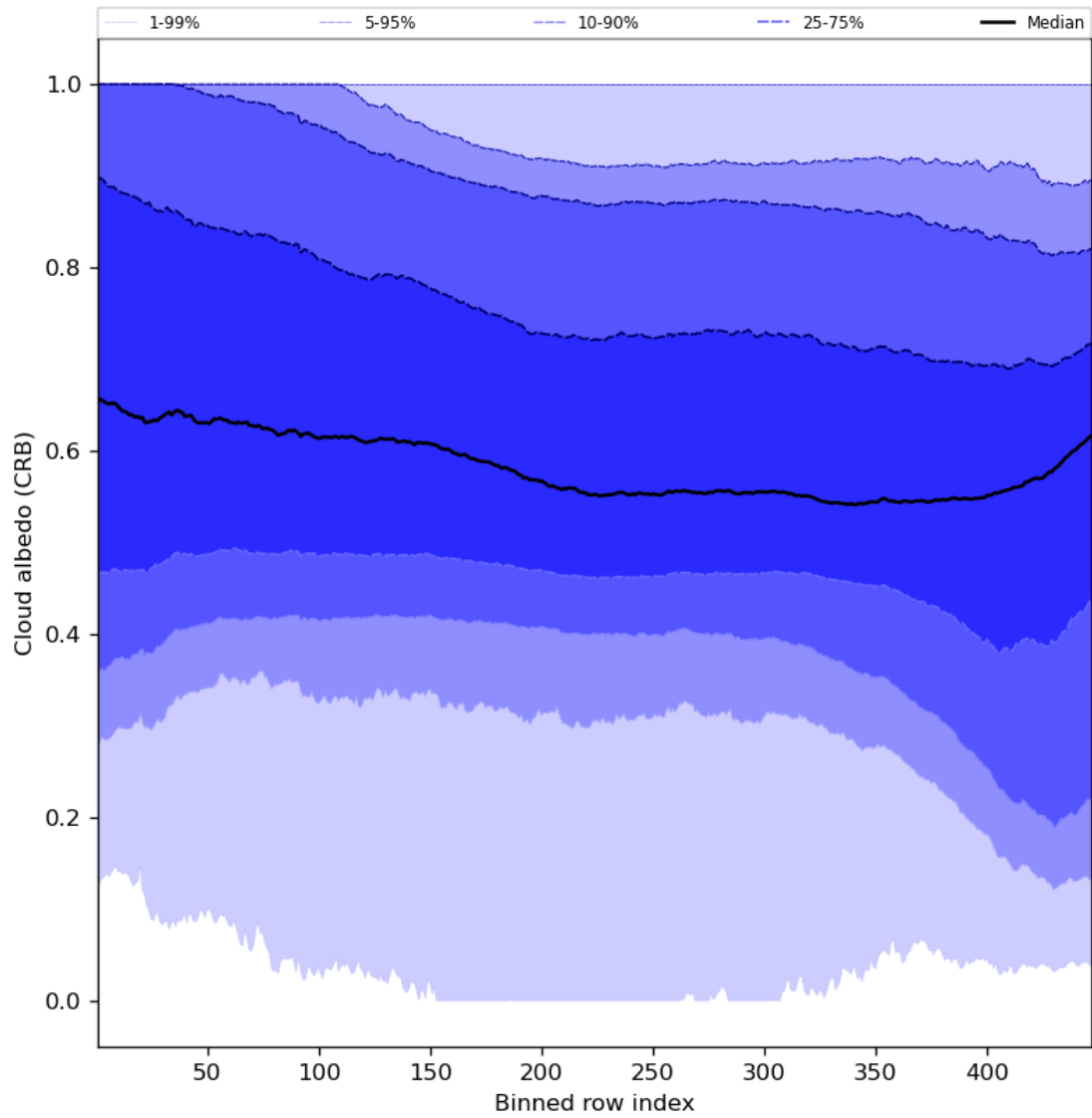
Figure 60: Along track statistics of “Cloud albedo (CRB)” for 2024-01-21 to 2024-01-22
