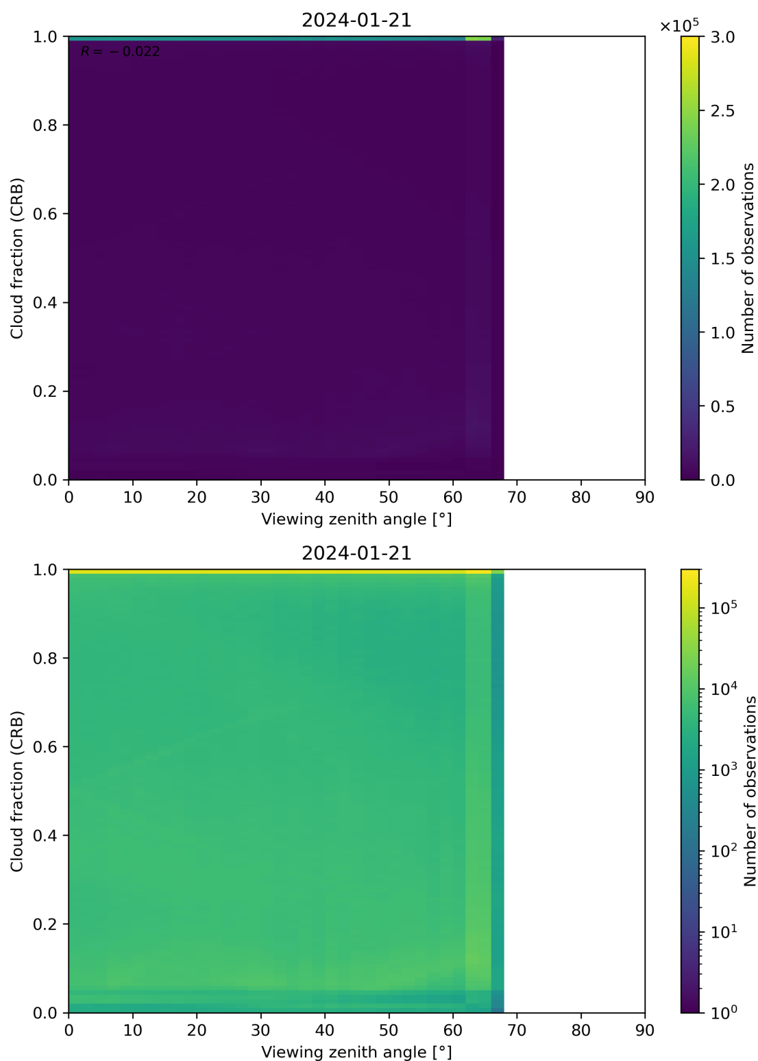
Figure 109: Scatter density plot of “Viewing zenith angle” against “Cloud fraction (CRB)” for 2024-01-21 to 2024-01-22.
