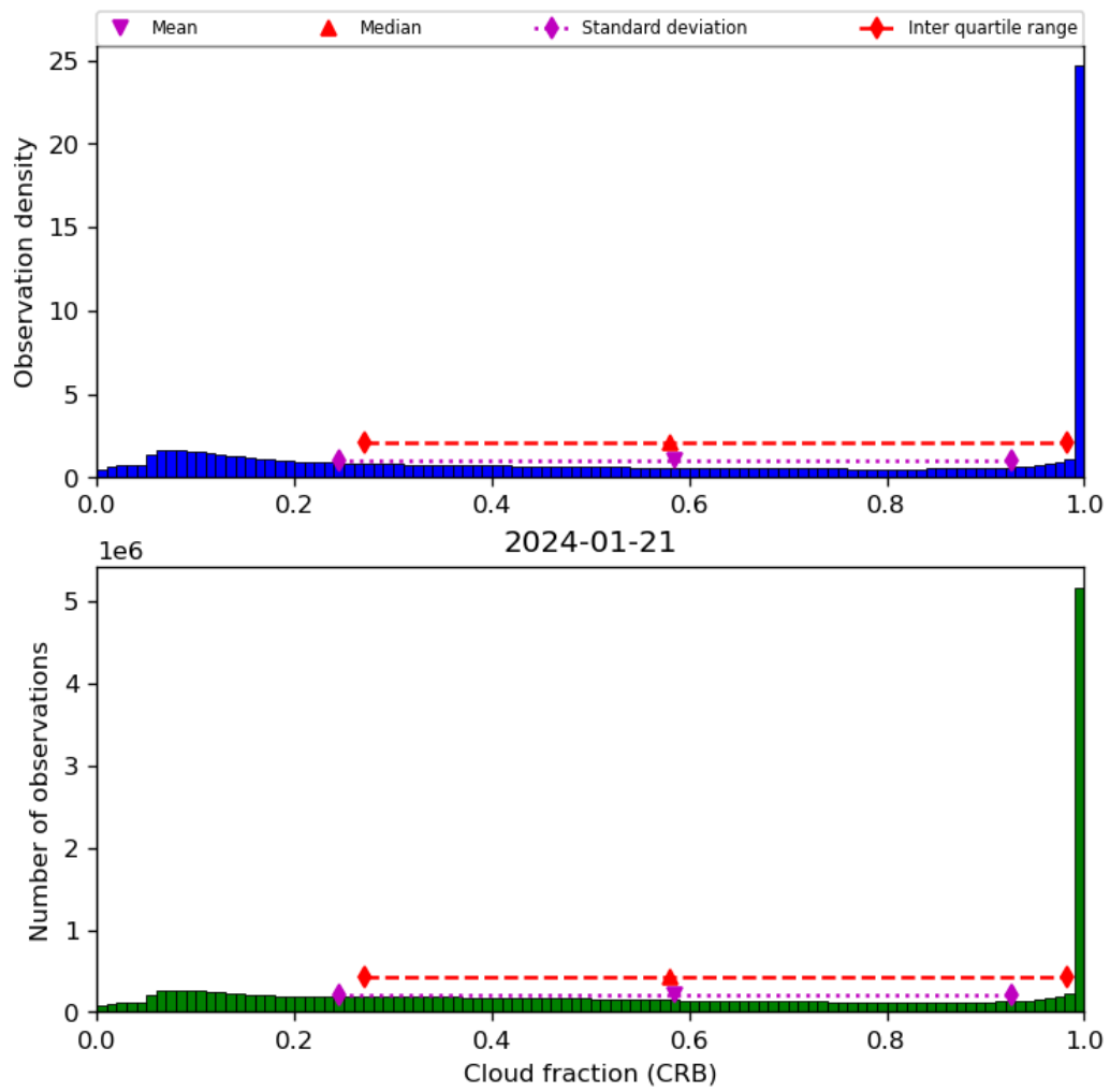
Figure 42: Histogram of “Cloud fraction (CRB)” for 2024-01-21 to 2024-01-22
