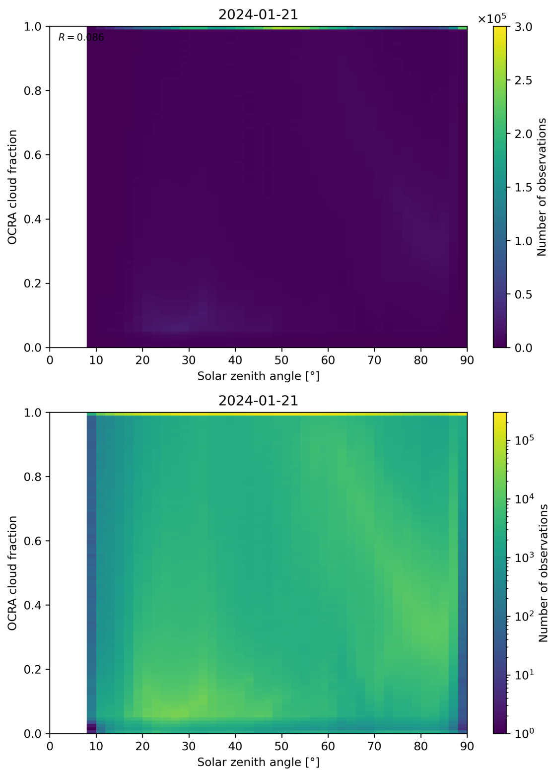
Figure 100: Scatter density plot of “Solar zenith angle” against “OCRA cloud fraction” for 2024-01-21 to 2024-01-22.
