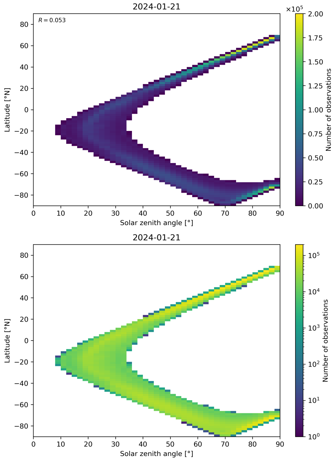
Figure 105: Scatter density plot of “Solar zenith angle” against “Latitude” for 2024-01-21 to 2024-01-22.
