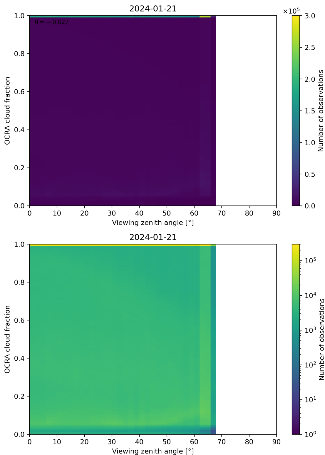
Figure 108: Scatter density plot of “Viewing zenith angle” against “OCRA cloud fraction” for 2024-01-21 to 2024-01-22.
