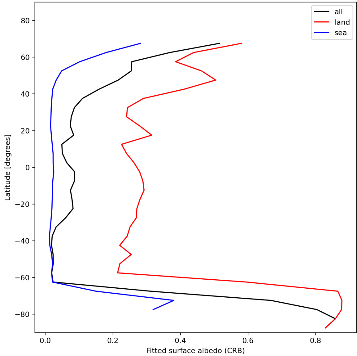
Figure 30: Zonal average of “Fitted surface albedo (CRB)” for 2024-01-21 to 2024-01-22.
