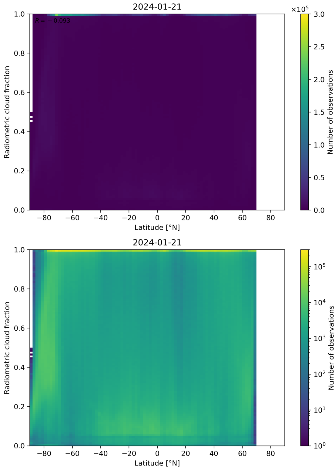
Figure 92: Scatter density plot of “Latitude” against “Radiometric cloud fraction” for 2024-01-21 to 2024-01-22.
