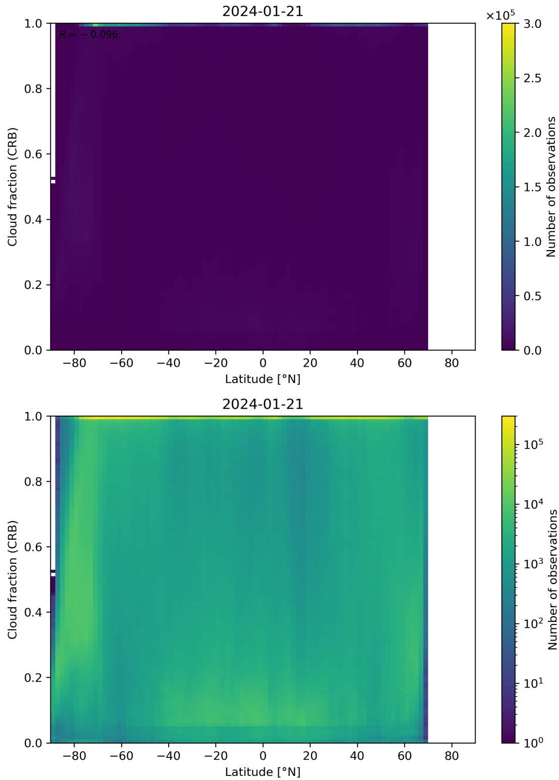
Figure 94: Scatter density plot of “Latitude” against “Cloud fraction (CRB)” for 2024-01-21 to 2024-01-22.
