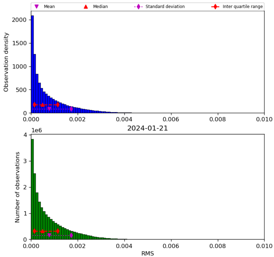
Figure 47: Histogram of “RMS” for 2024-01-21 to 2024-01-22
