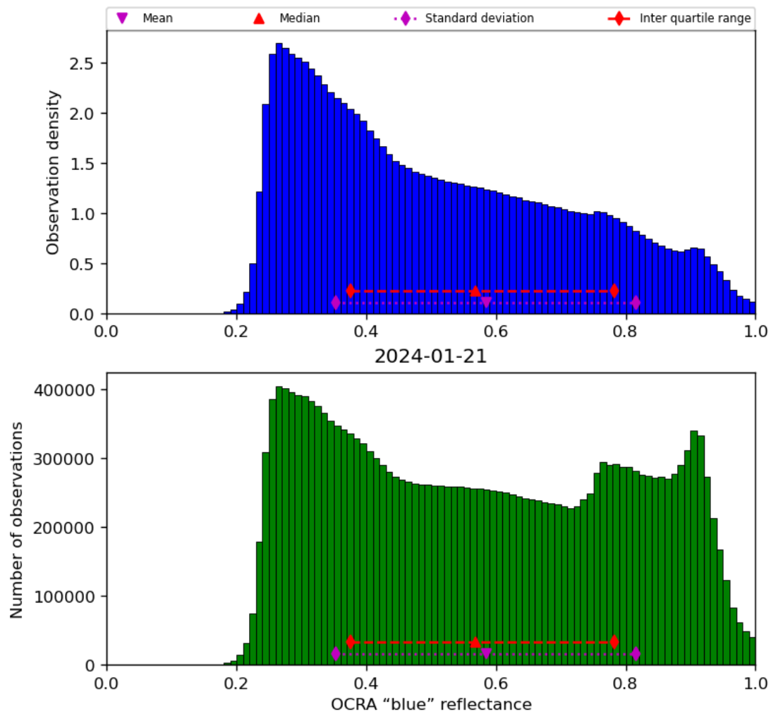
Figure 51: Histogram of “OCRA “blue” reflectance” for 2024-01-21 to 2024-01-22
