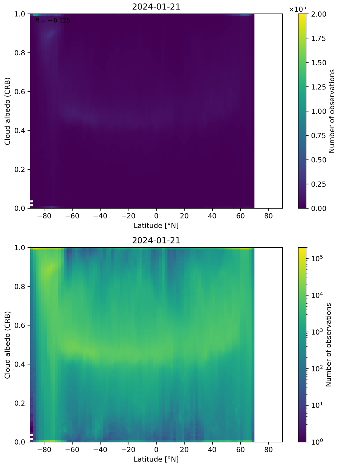
Figure 91: Scatter density plot of “Latitude” against “Cloud albedo (CRB)” for 2024-01-21 to 2024-01-22.
