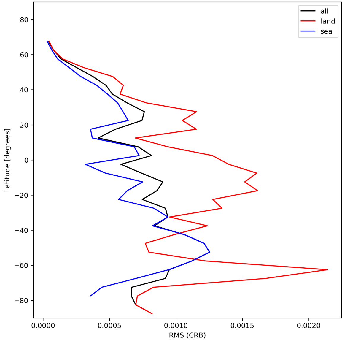
Figure 32: Zonal average of “RMS (CRB)” for 2024-01-21 to 2024-01-22.
