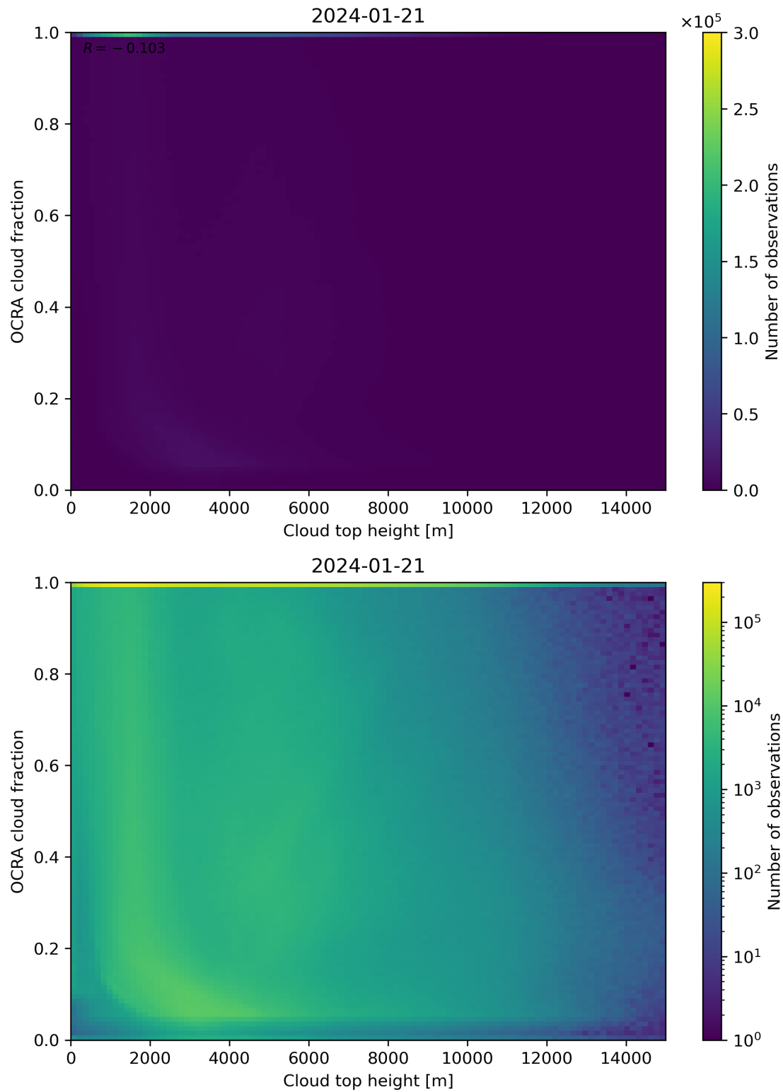
Figure 87: Scatter density plot of “Cloud top height” against “OCRA cloud fraction” for 2024-01-21 to 2024-01-22.
