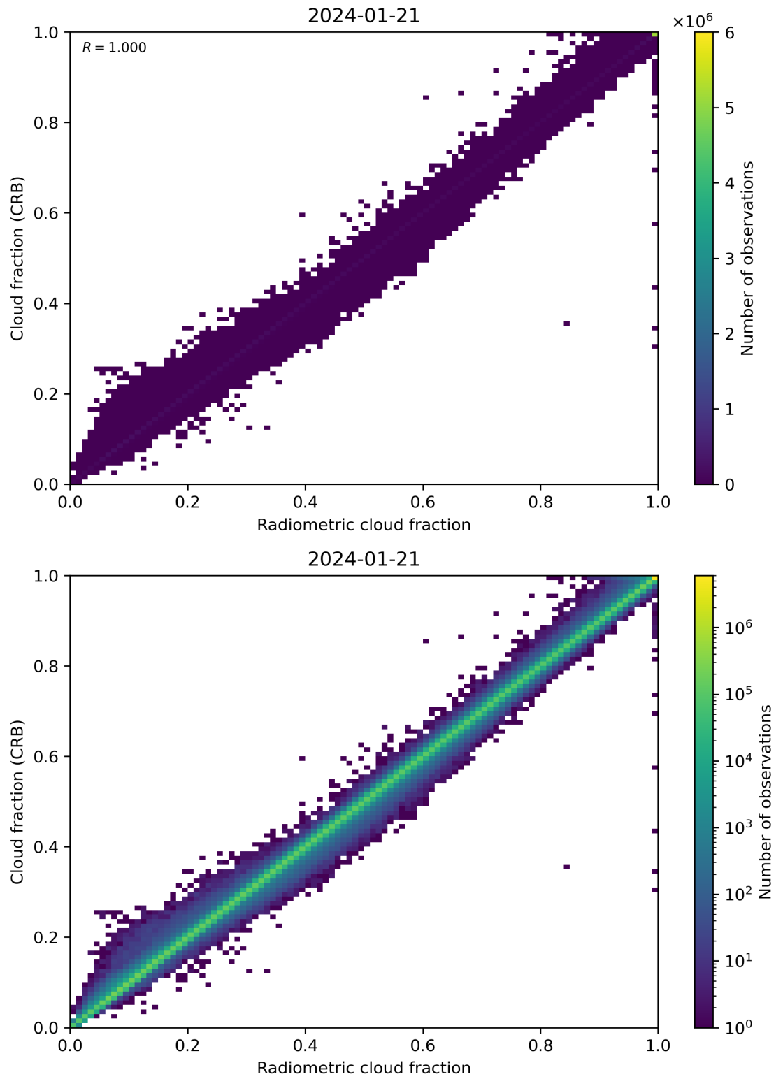
Figure 73: Scatter density plot of “Radiometric cloud fraction” against “Cloud fraction (CRB)” for 2024-01-21 to 2024-01-22.
