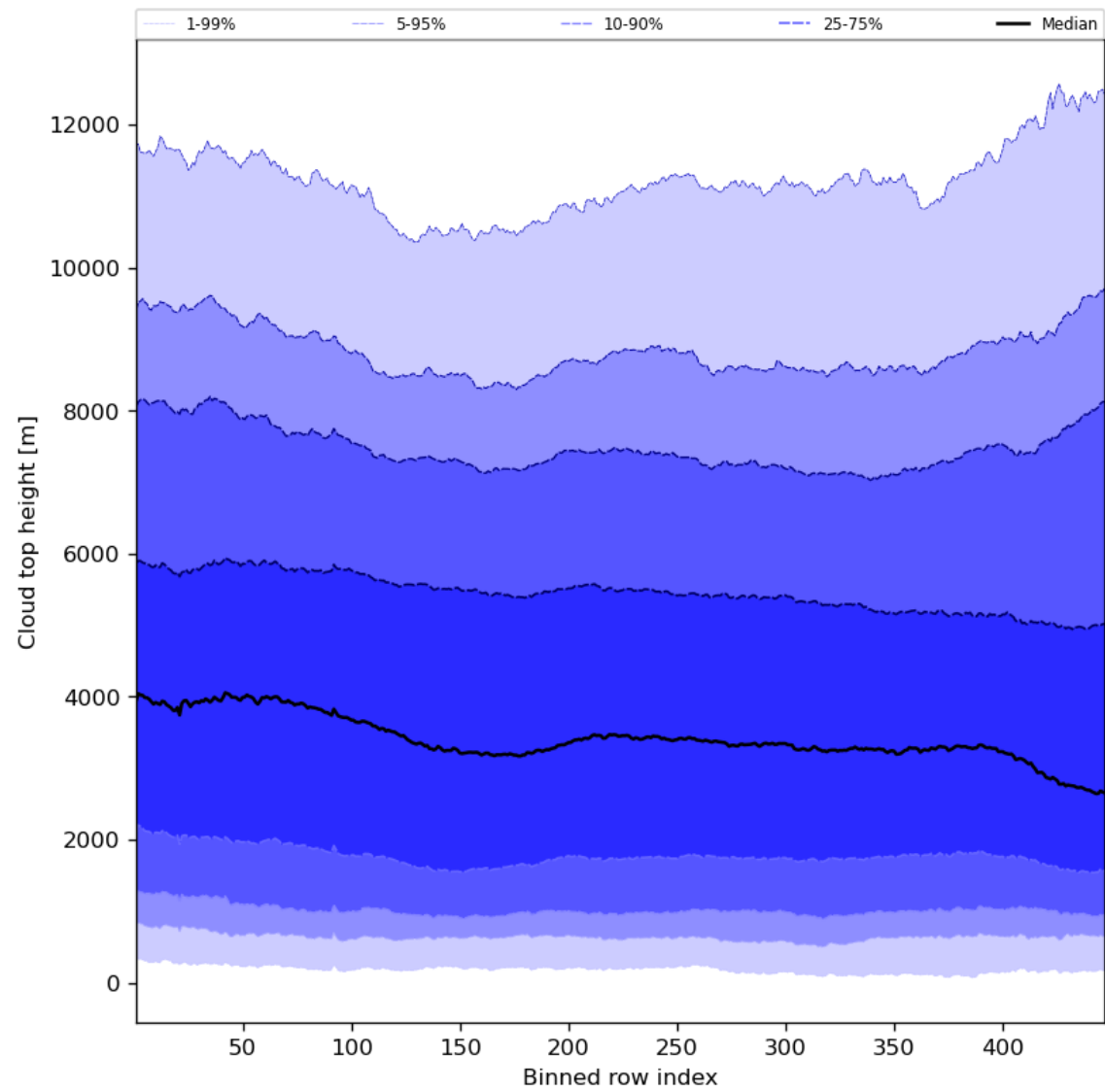
Figure 56: Along track statistics of “Cloud top height” for 2024-01-21 to 2024-01-22
