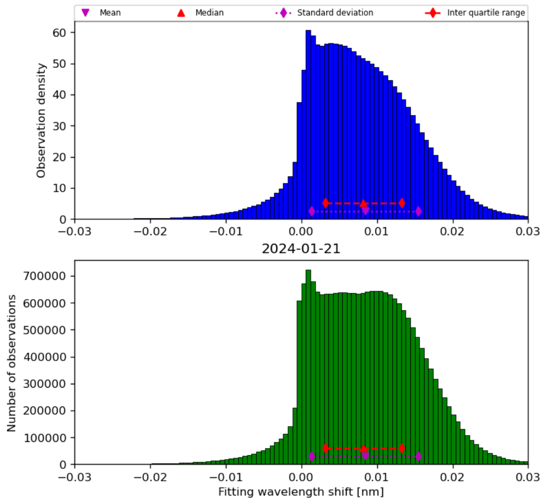
Figure 49: Histogram of “Fitting wavelength shift” for 2024-01-21 to 2024-01-22
