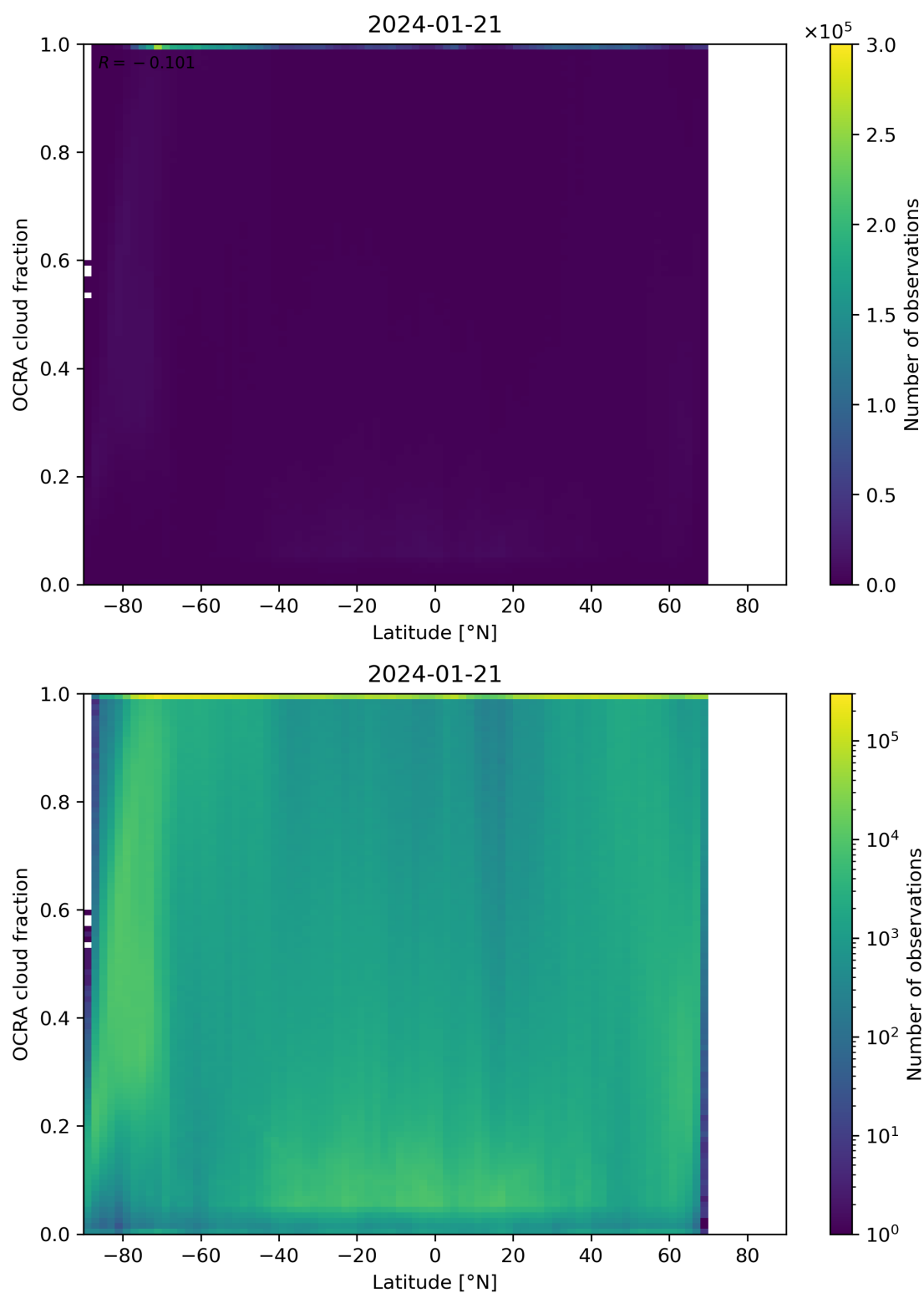
Figure 93: Scatter density plot of “Latitude” against “OCRA cloud fraction” for 2024-01-21 to 2024-01-22.
