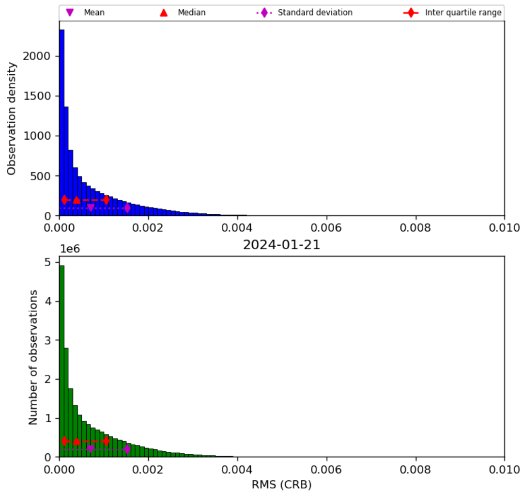
Figure 48: Histogram of “RMS (CRB)” for 2024-01-21 to 2024-01-22
