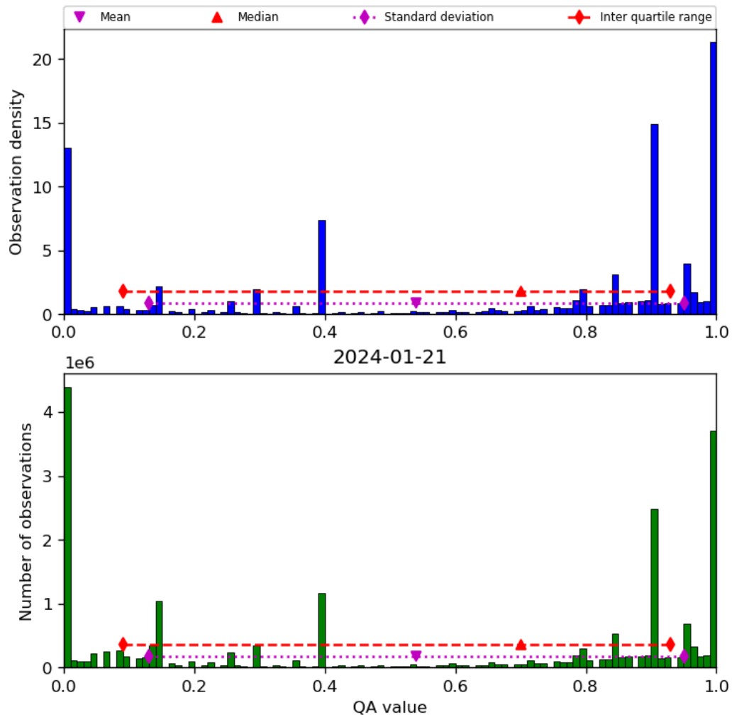
Figure 38: Histogram of “QA value” for 2024-01-21 to 2024-01-22
