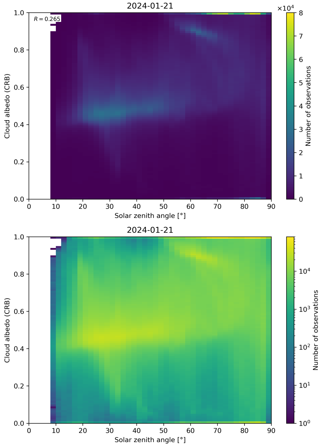
Figure 98: Scatter density plot of “Solar zenith angle” against “Cloud albedo (CRB)” for 2024-01-21 to 2024-01-22.
