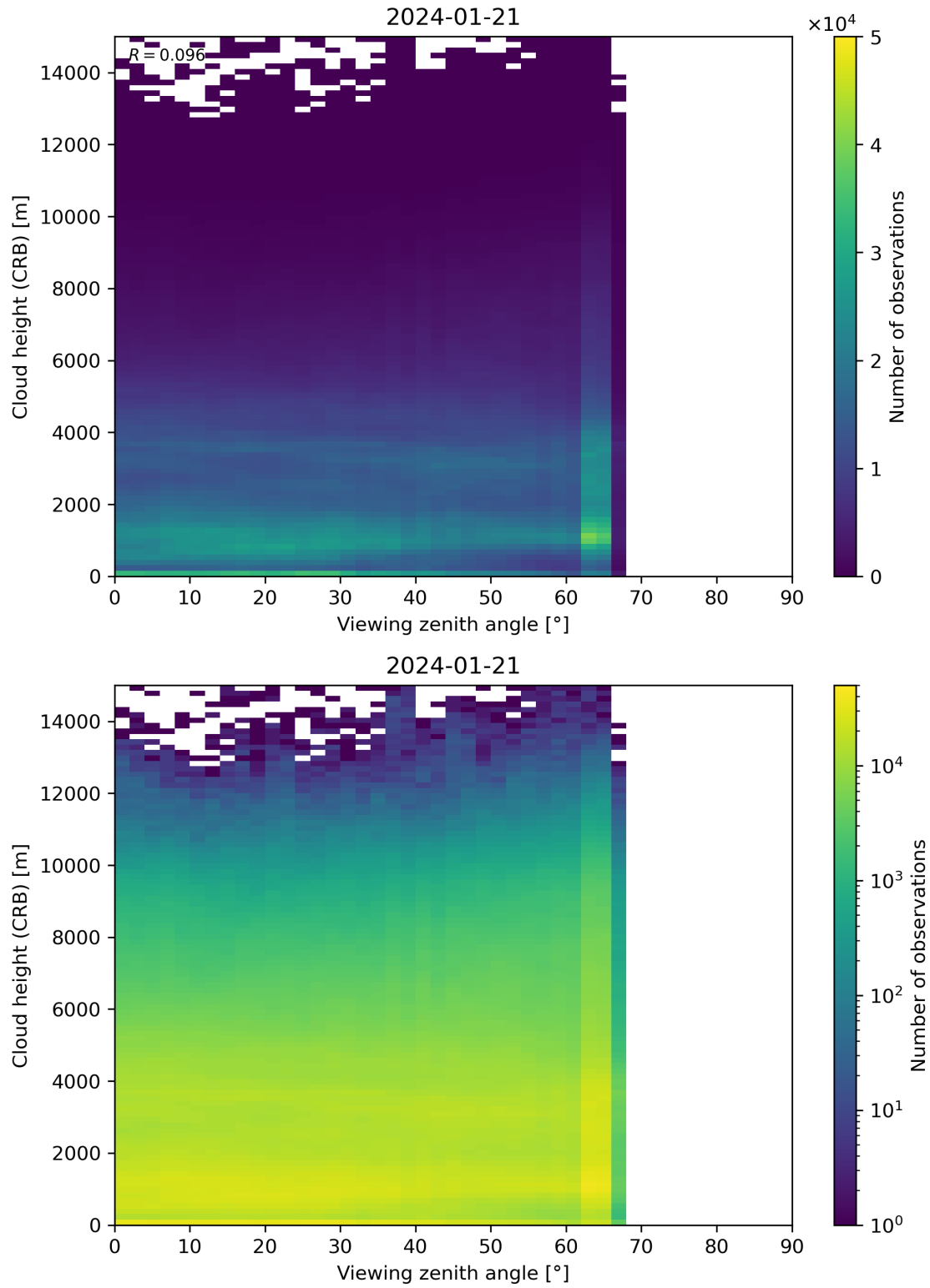
Figure 110: Scatter density plot of “Viewing zenith angle” against “Cloud height (CRB)” for 2024-01-21 to 2024-01-22.
