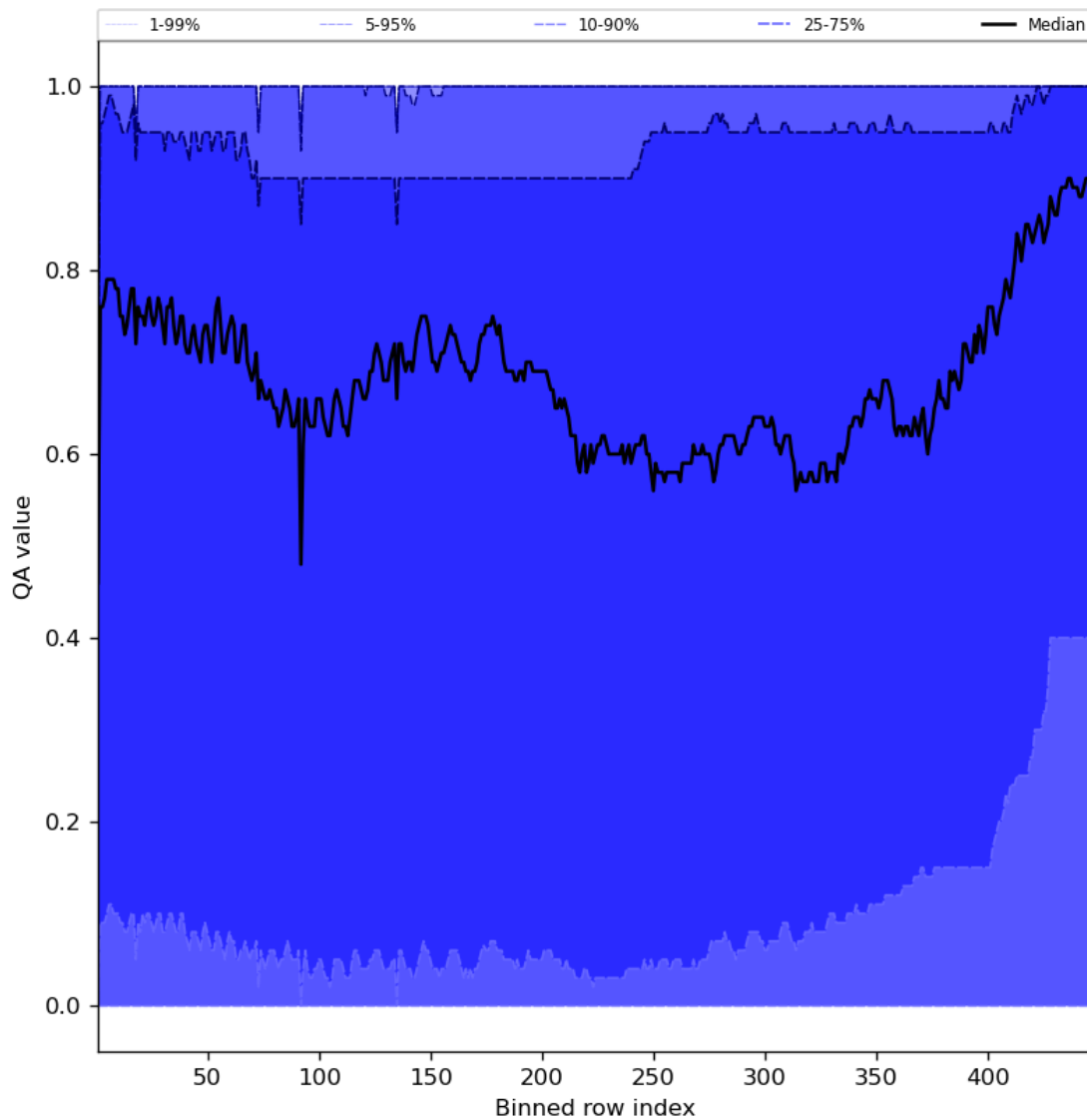
Figure 54: Along track statistics of “QA value” for 2024-01-21 to 2024-01-22
