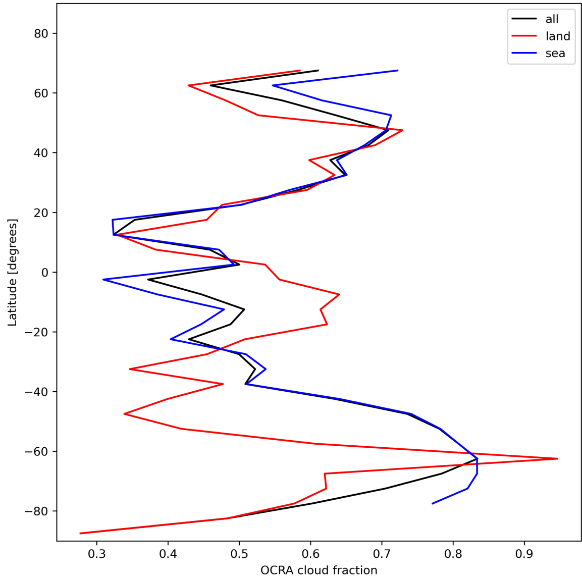
Figure 34: Zonal average of “OCRA cloud fraction” for 2024-01-21 to 2024-01-22.
