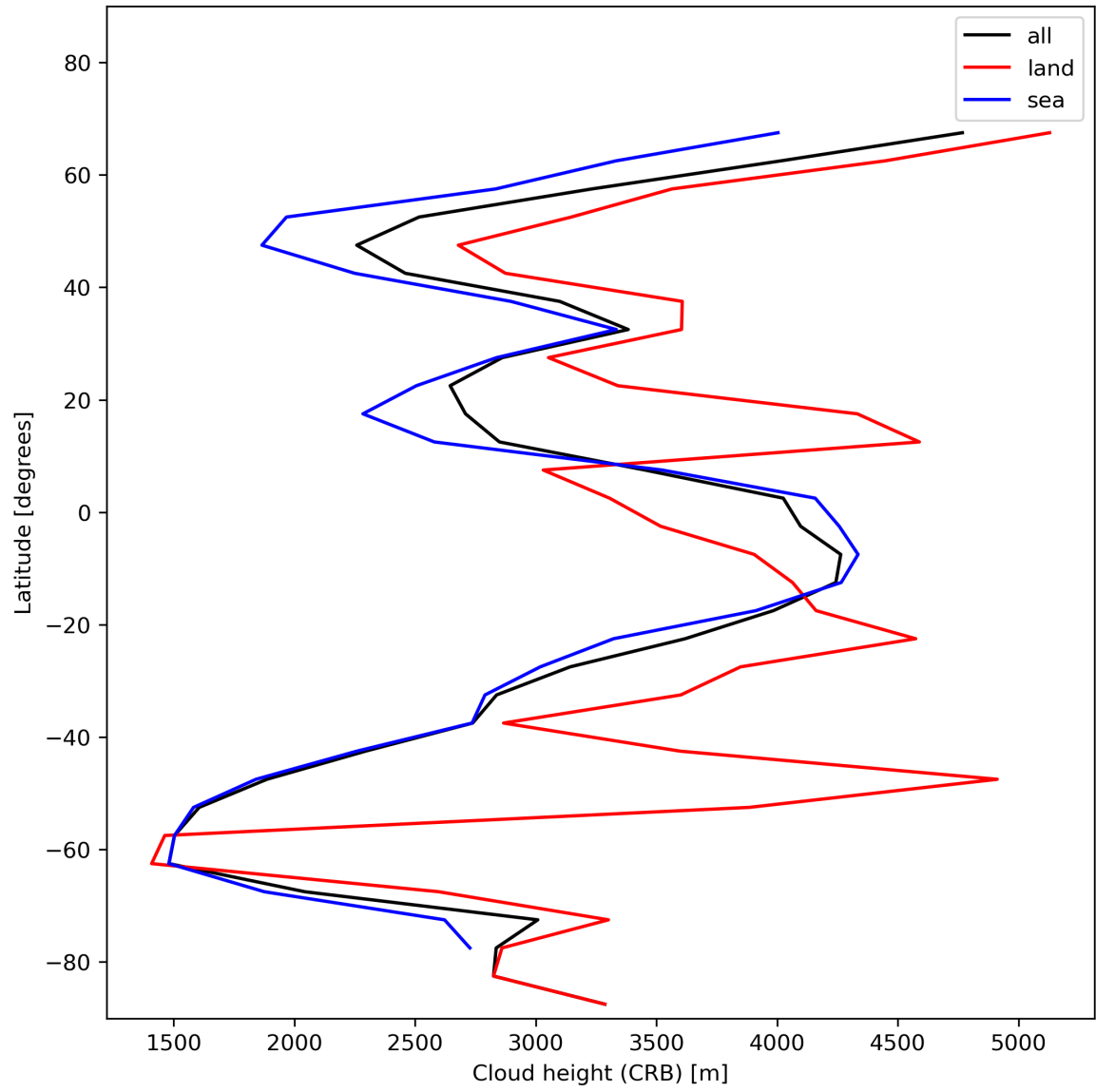
Figure 27: Zonal average of “Cloud height (CRB)” for 2024-01-21 to 2024-01-22.
