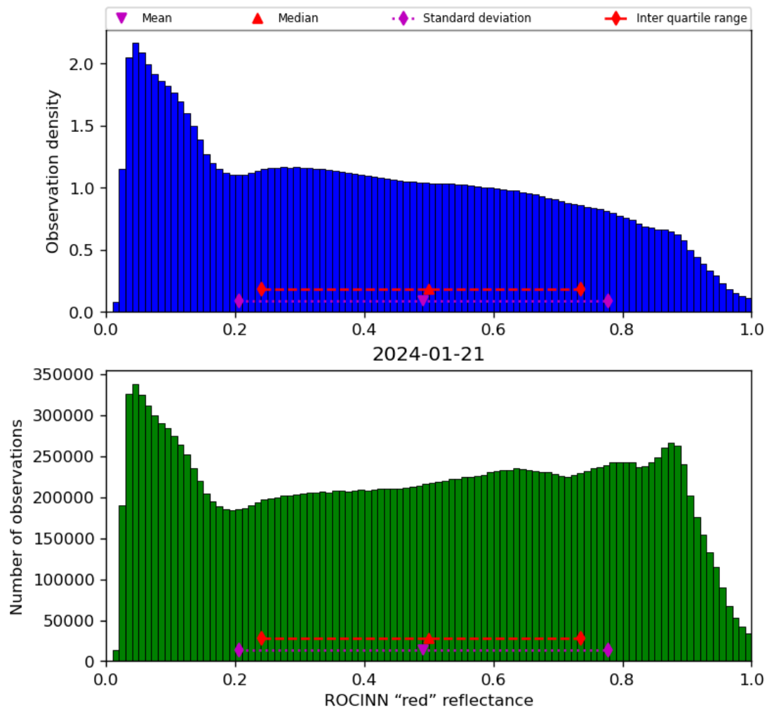
Figure 53: Histogram of “ROCINN “red” reflectance” for 2024-01-21 to 2024-01-22
