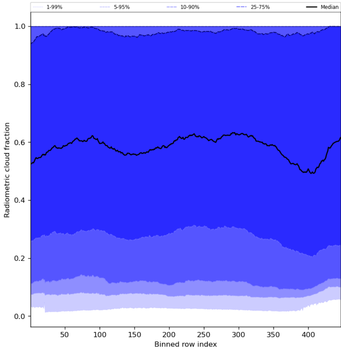
Figure 55: Along track statistics of “Radiometric cloud fraction” for 2024-01-21 to 2024-01-22
