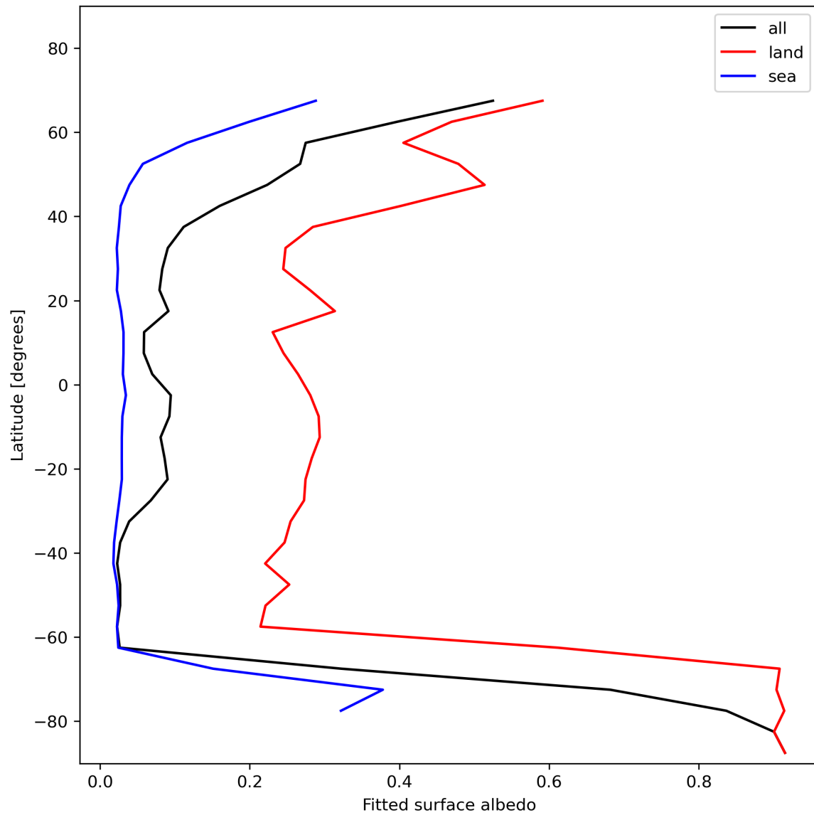
Figure 29: Zonal average of “Fitted surface albedo” for 2024-01-21 to 2024-01-22.
