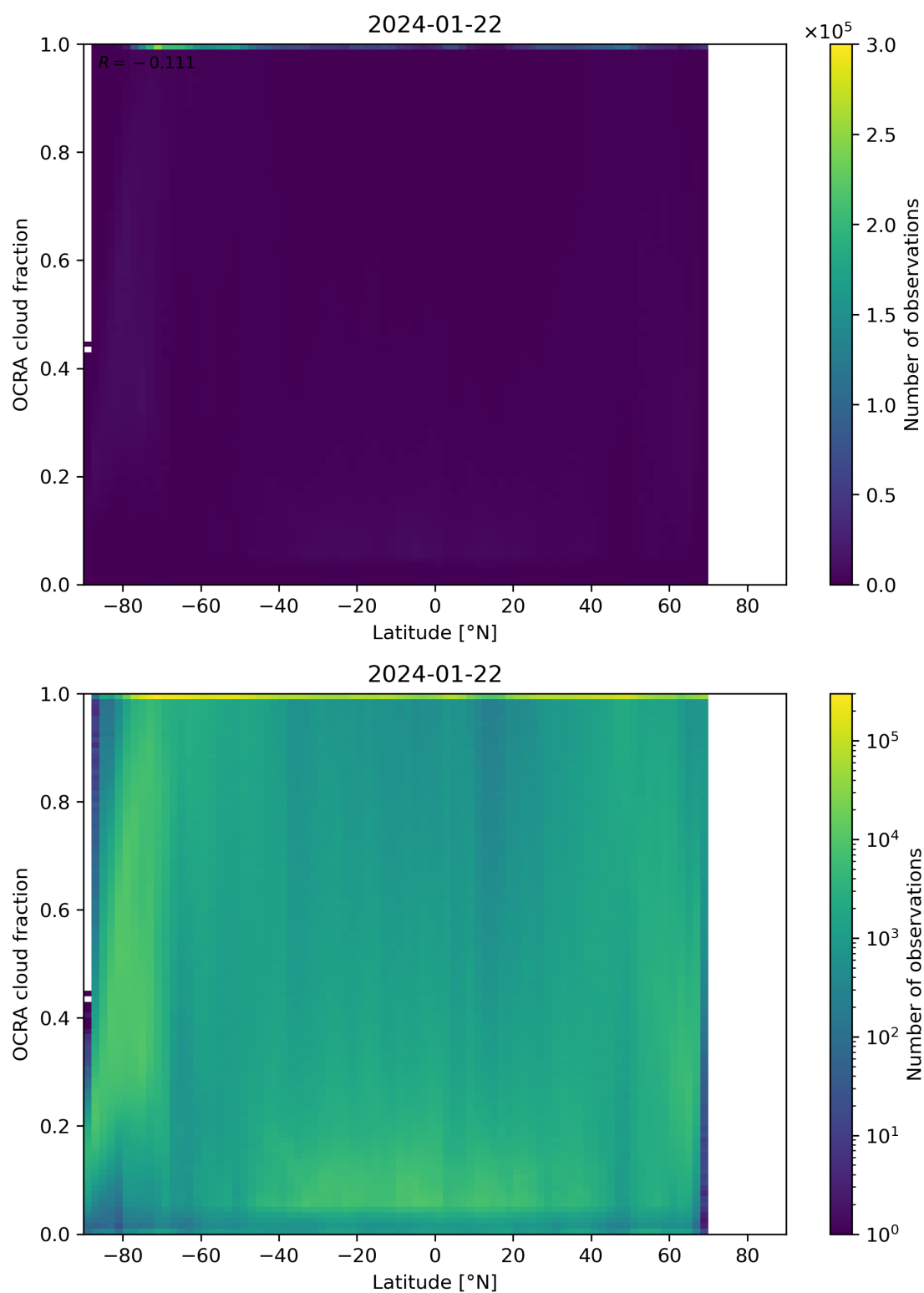
Figure 93: Scatter density plot of “Latitude” against “OCRA cloud fraction” for 2024-01-21 to 2024-01-23.
