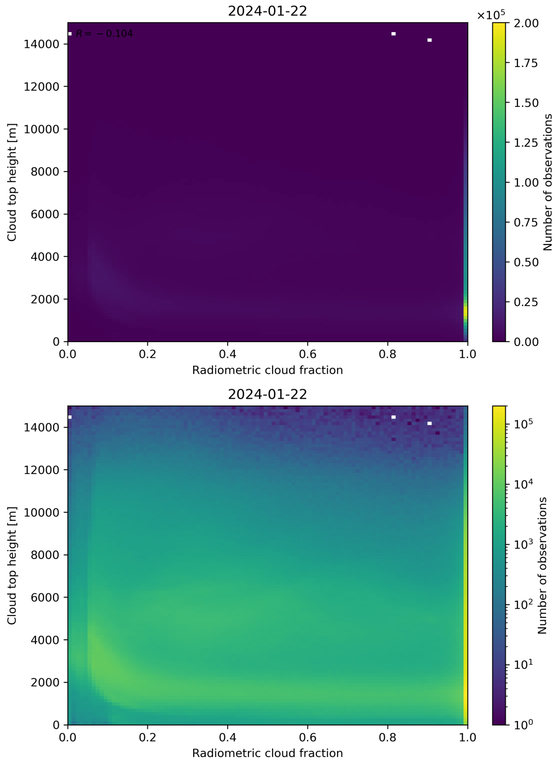
Figure 76: Scatter density plot of “Radiometric cloud fraction” against “Cloud top height” for 2024-01-21 to 2024-01-23.
