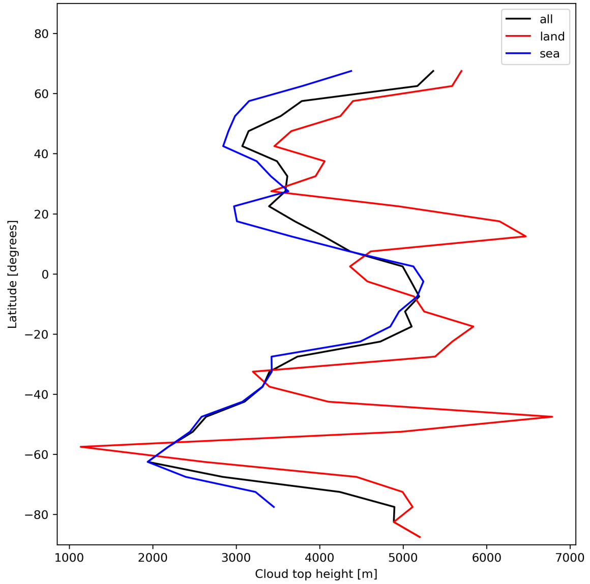
Figure 24: Zonal average of “Cloud top height” for 2024-01-21 to 2024-01-23.
