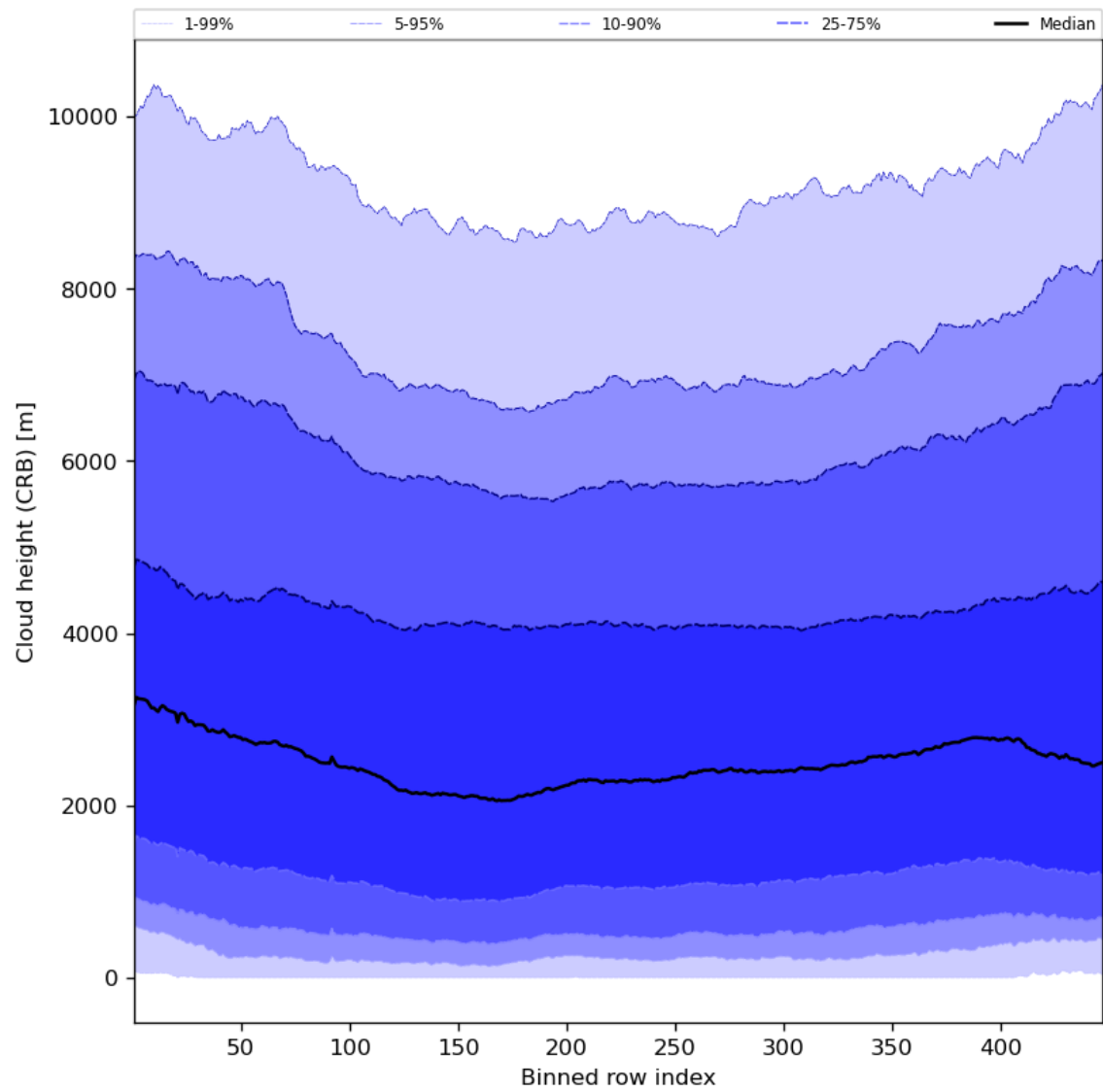
Figure 59: Along track statistics of “Cloud height (CRB)” for 2024-01-21 to 2024-01-23
