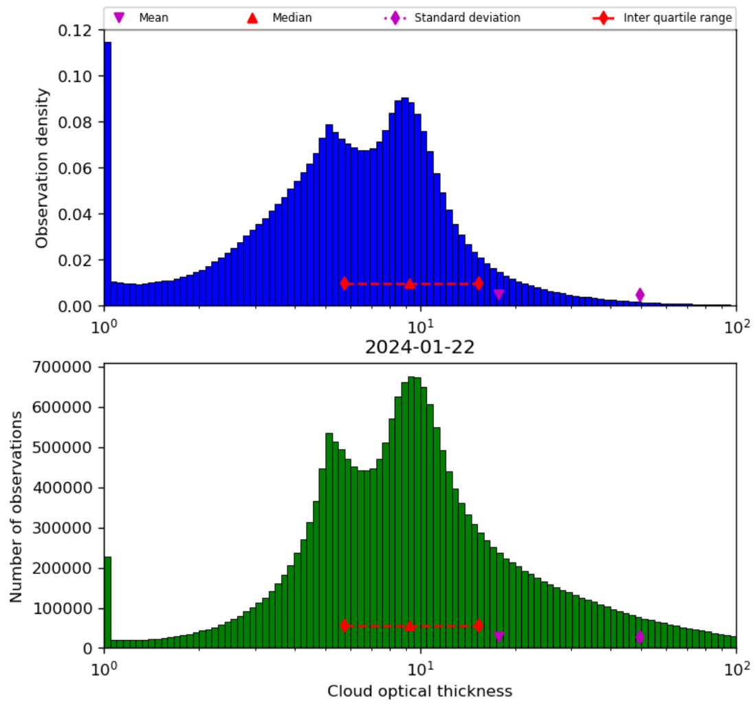
Figure 41: Histogram of “Cloud optical thickness” for 2024-01-21 to 2024-01-23
