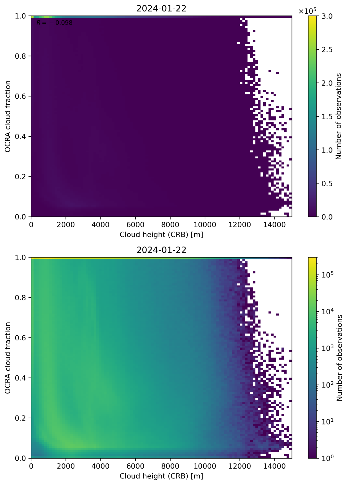
Figure 81: Scatter density plot of “Cloud height (CRB)” against “OCRA cloud fraction” for 2024-01-21 to 2024-01-23.
