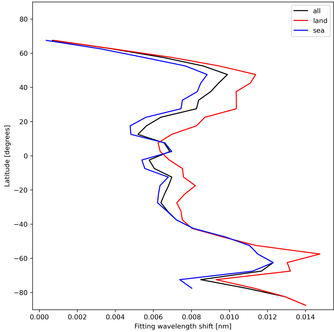
Figure 33: Zonal average of “Fitting wavelength shift” for 2024-01-21 to 2024-01-23.
