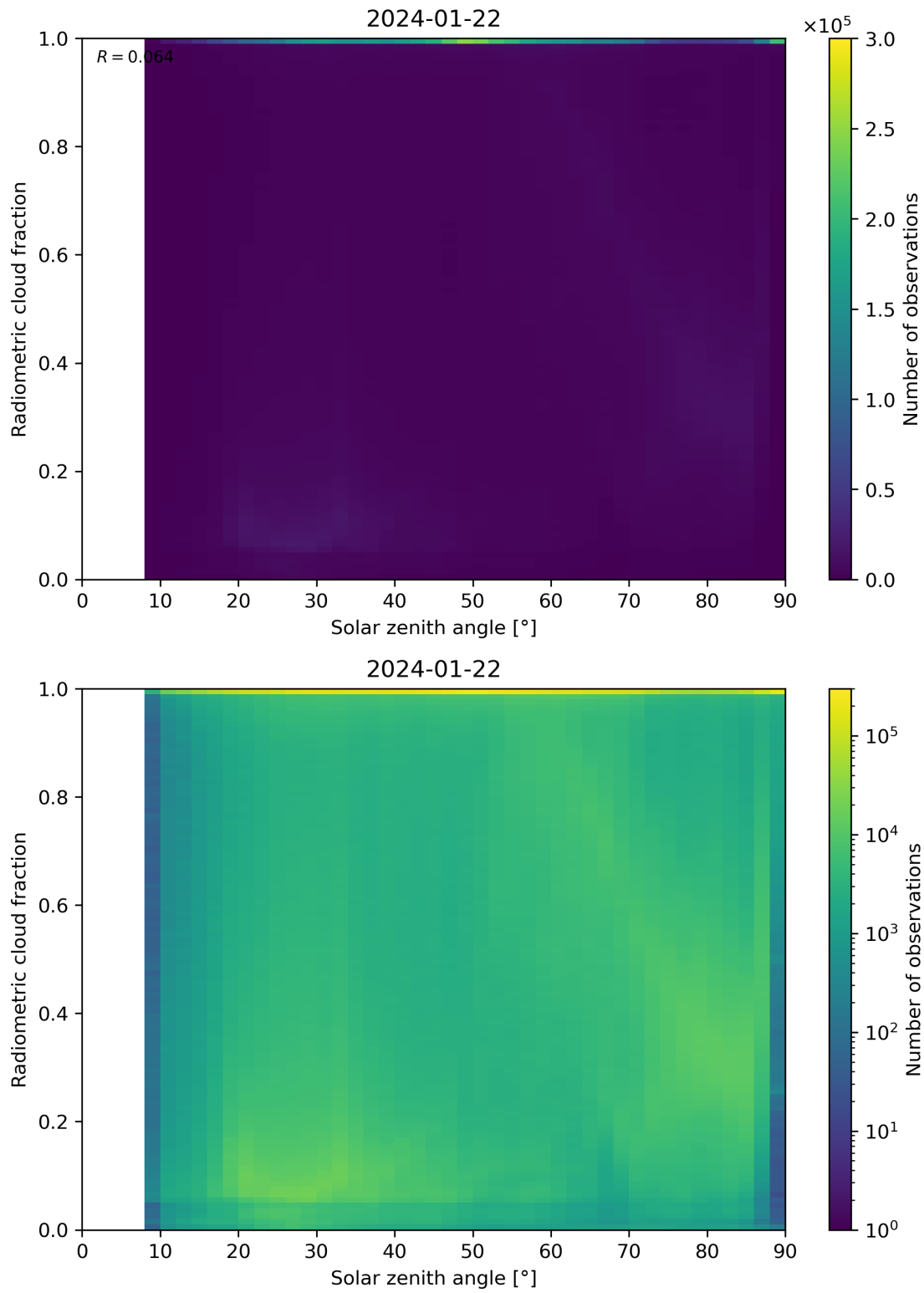
Figure 99: Scatter density plot of “Solar zenith angle” against “Radiometric cloud fraction” for 2024-01-21 to 2024-01-23.
