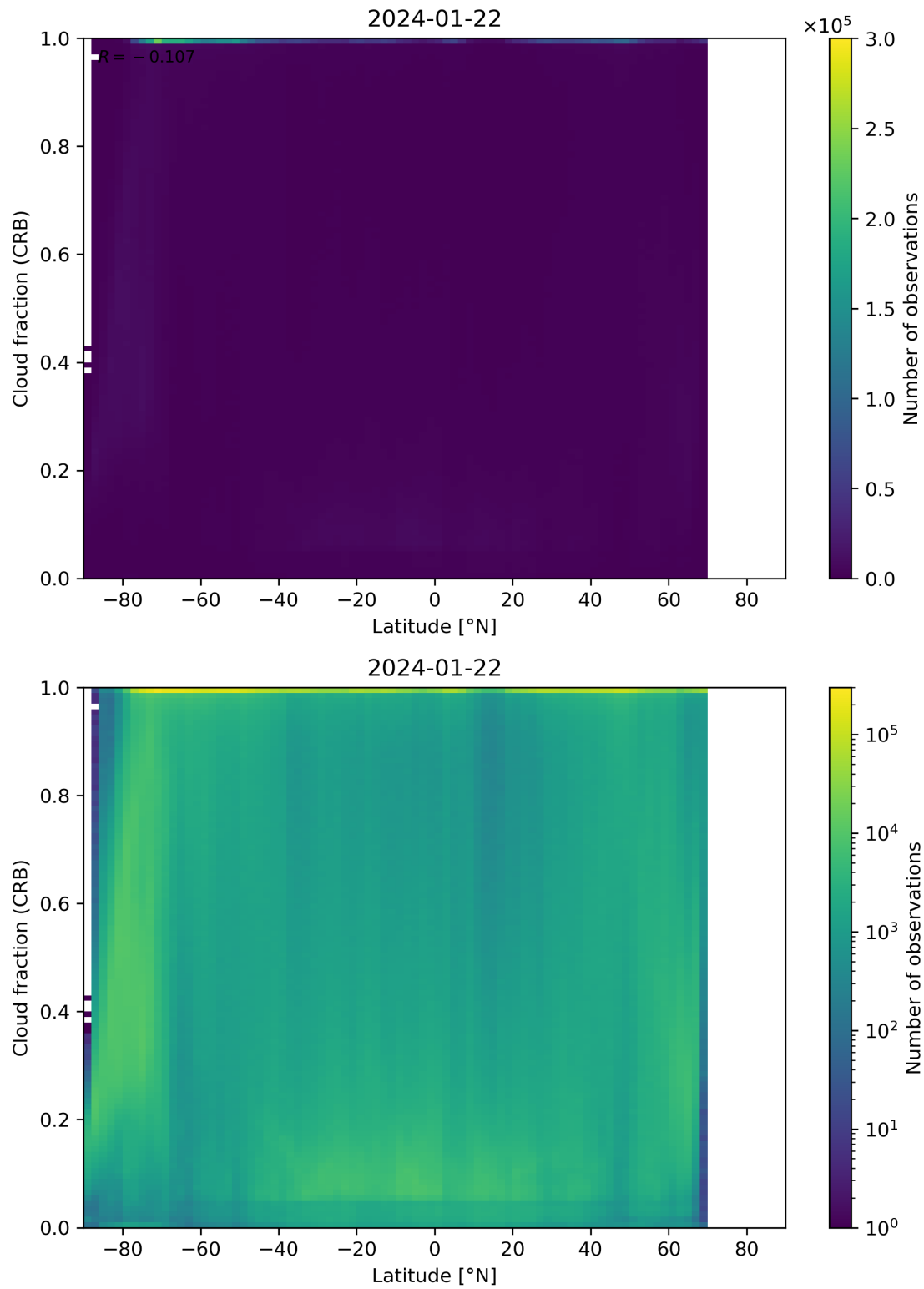
Figure 94: Scatter density plot of “Latitude” against “Cloud fraction (CRB)” for 2024-01-21 to 2024-01-23.
