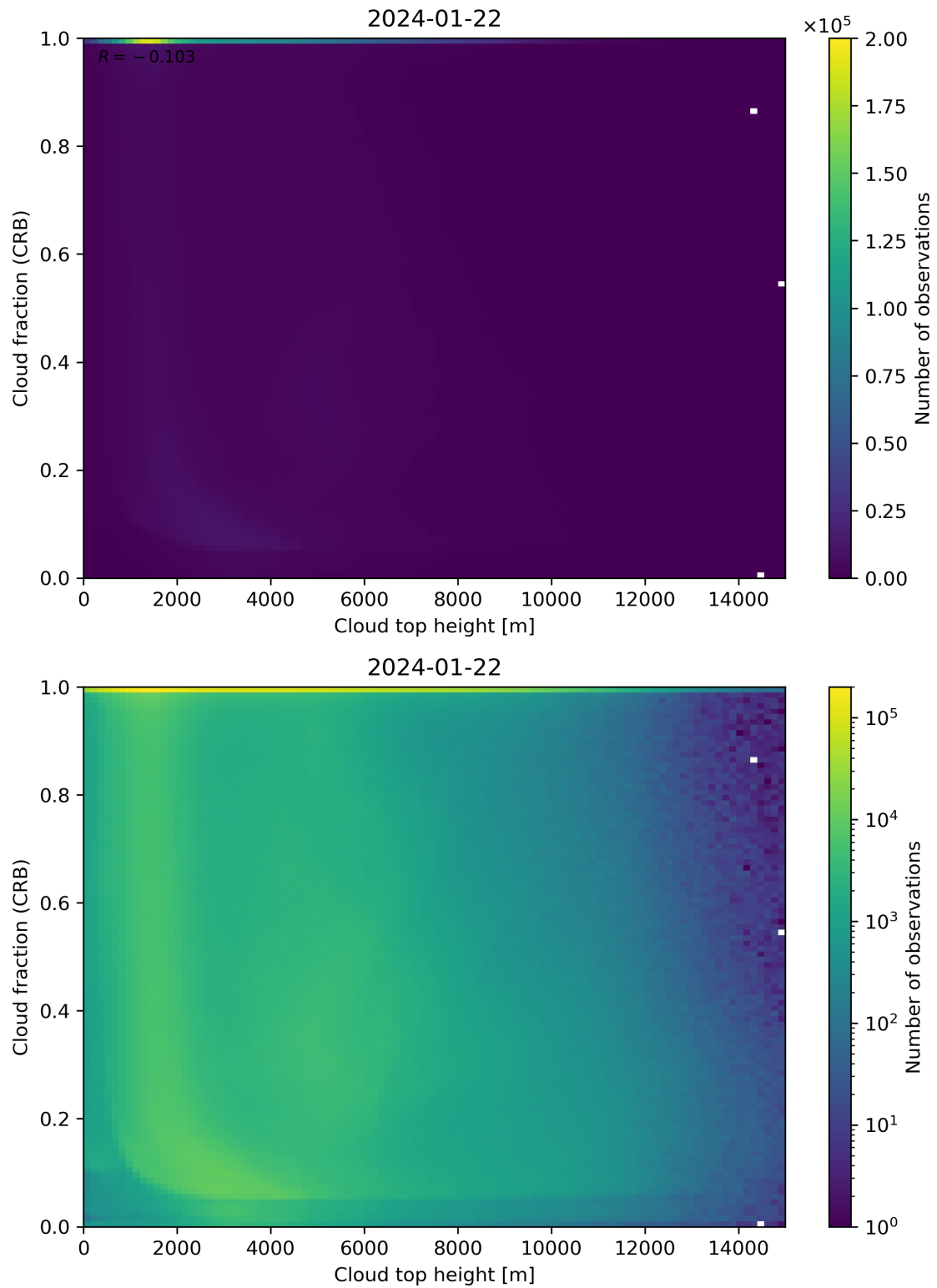
Figure 88: Scatter density plot of “Cloud top height” against “Cloud fraction (CRB)” for 2024-01-21 to 2024-01-23.
