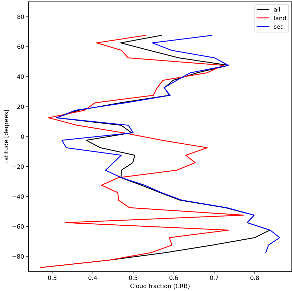
Figure 26: Zonal average of “Cloud fraction (CRB)” for 2024-01-21 to 2024-01-23.
