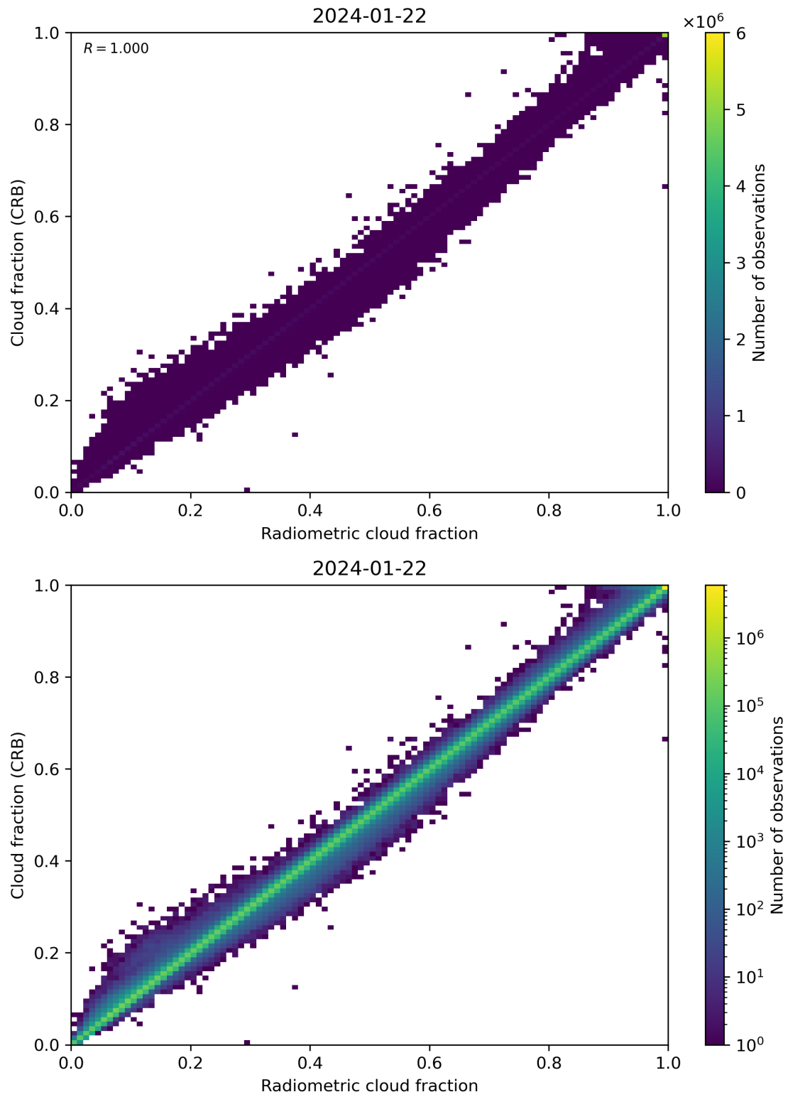
Figure 73: Scatter density plot of “Radiometric cloud fraction” against “Cloud fraction (CRB)” for 2024-01-21 to 2024-01-23.
