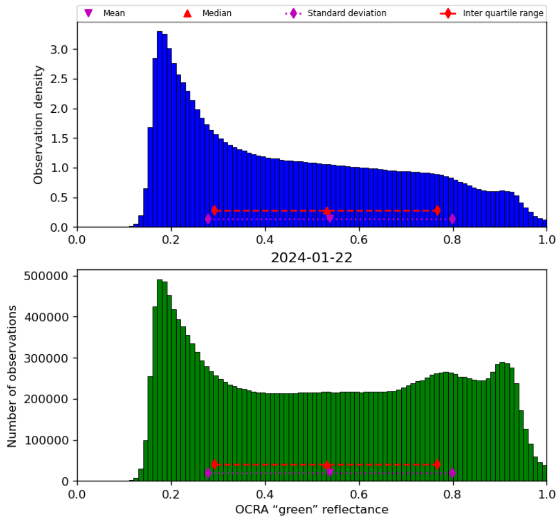
Figure 52: Histogram of “OCRA “green” reflectance” for 2024-01-21 to 2024-01-23
