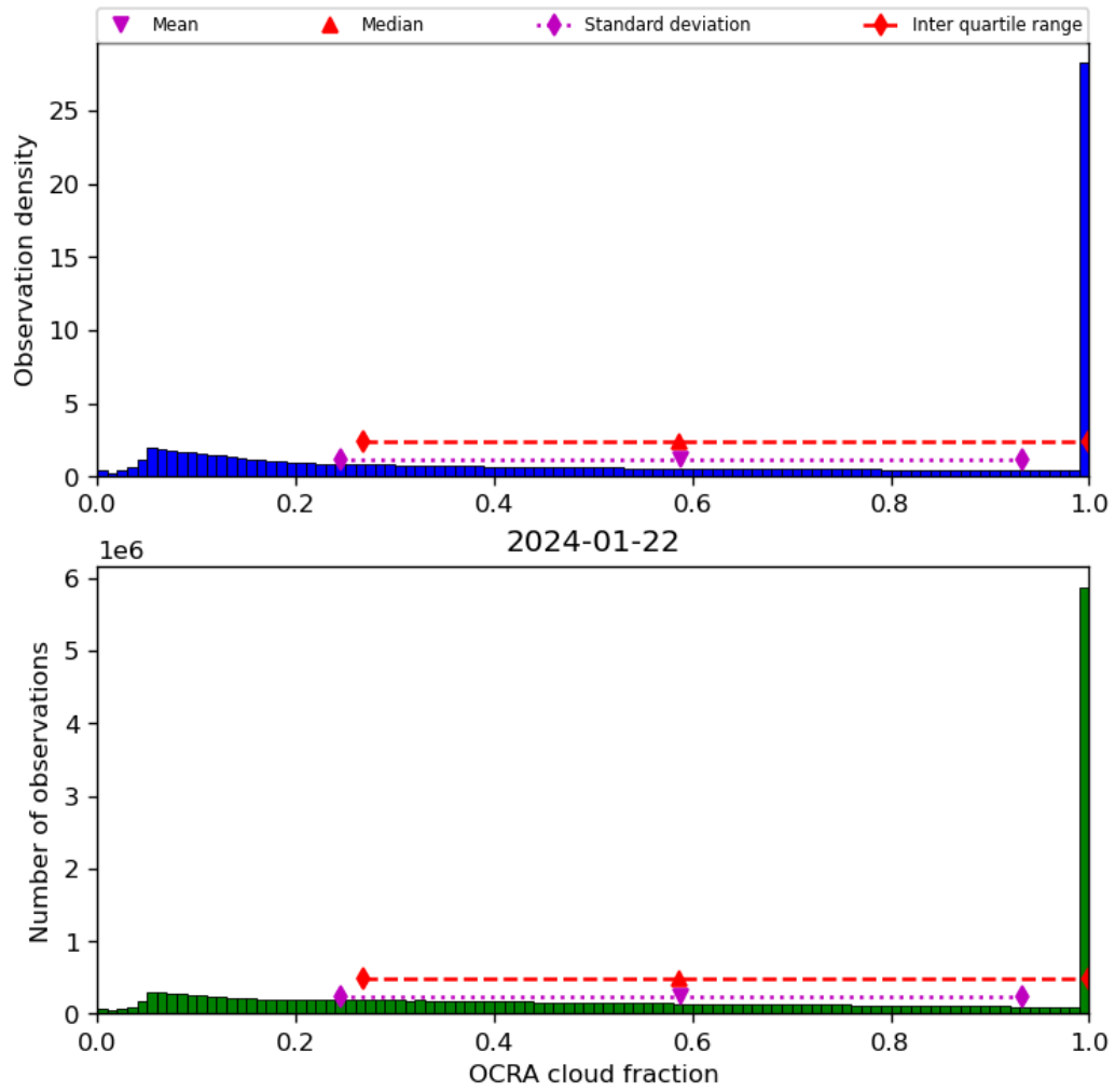
Figure 50: Histogram of “OCRA cloud fraction” for 2024-01-21 to 2024-01-23
