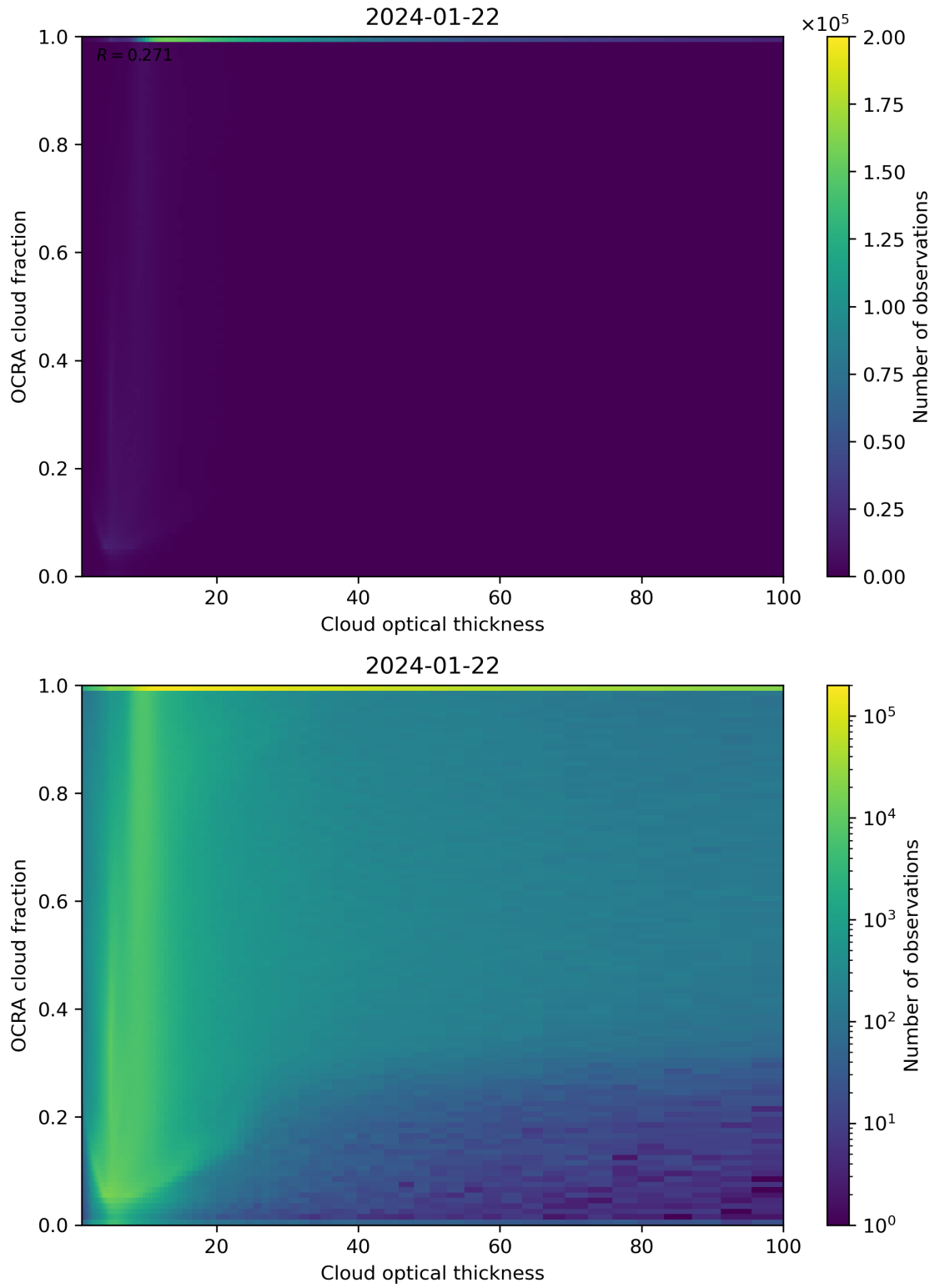
Figure 83: Scatter density plot of “Cloud optical thickness” against “OCRA cloud fraction” for 2024-01-21 to 2024-01-23.
