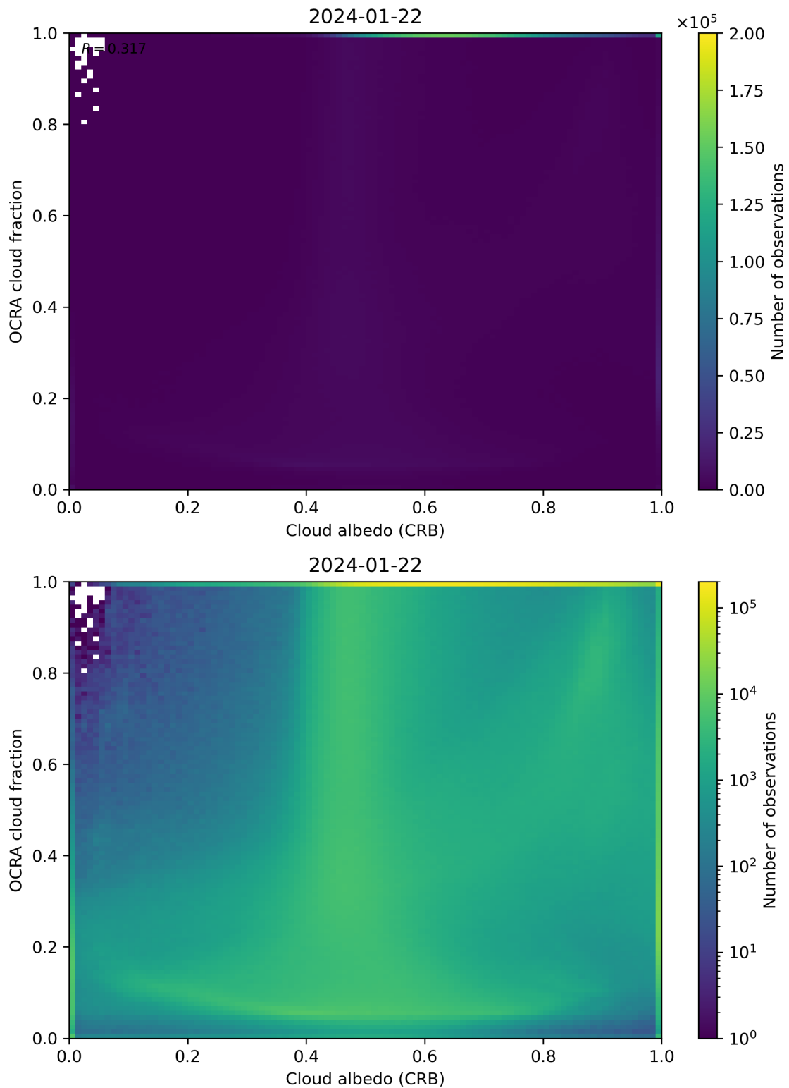
Figure 70: Scatter density plot of “Cloud albedo (CRB)” against “OCRA cloud fraction” for 2024-01-21 to 2024-01-23.
