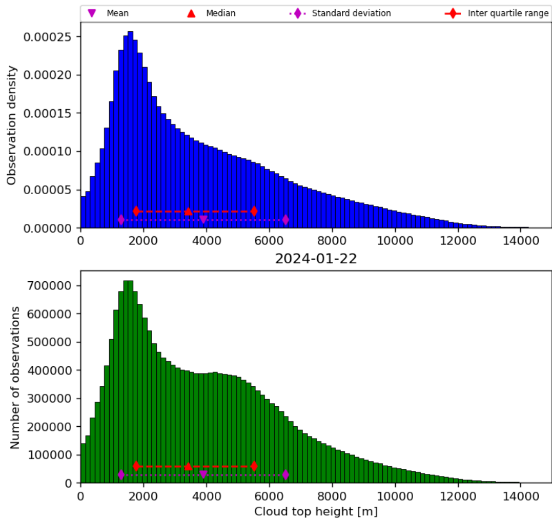
Figure 40: Histogram of “Cloud top height” for 2024-01-21 to 2024-01-23
