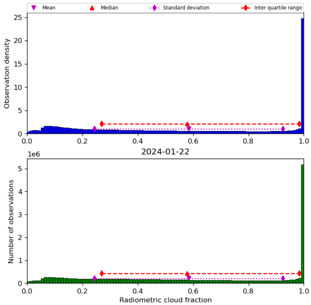
Figure 39: Histogram of “Radiometric cloud fraction” for 2024-01-21 to 2024-01-23
