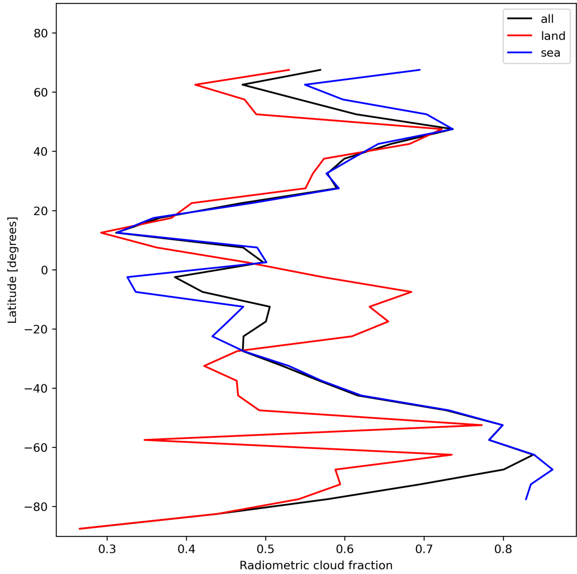
Figure 23: Zonal average of “Radiometric cloud fraction” for 2024-01-21 to 2024-01-23.
