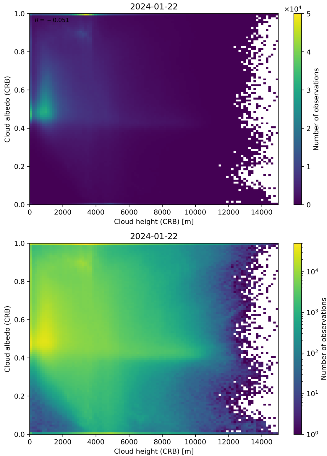
Figure 80: Scatter density plot of “Cloud height (CRB)” against “Cloud albedo (CRB)” for 2024-01-21 to 2024-01-23.
