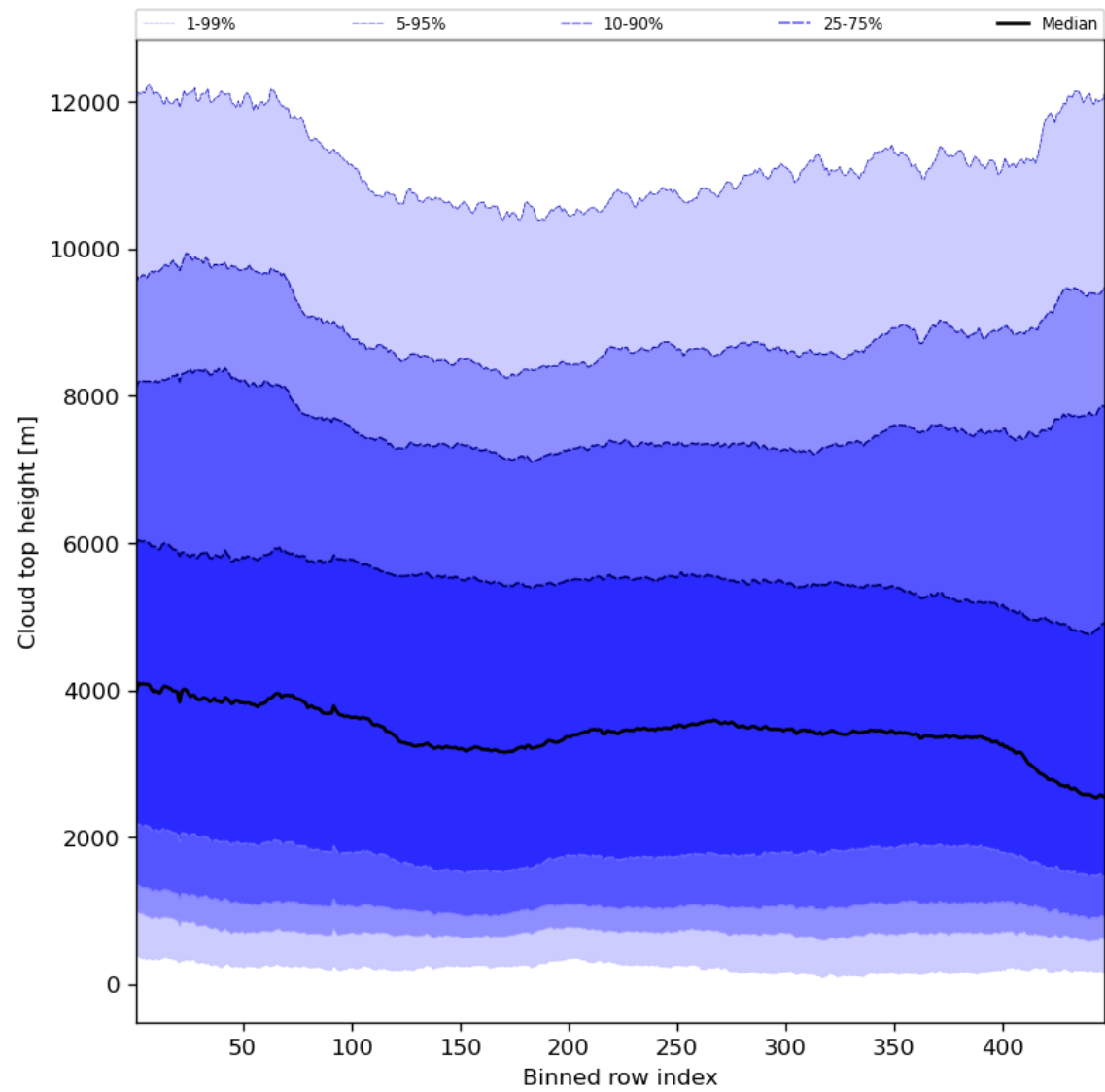
Figure 56: Along track statistics of “Cloud top height” for 2024-01-21 to 2024-01-23
