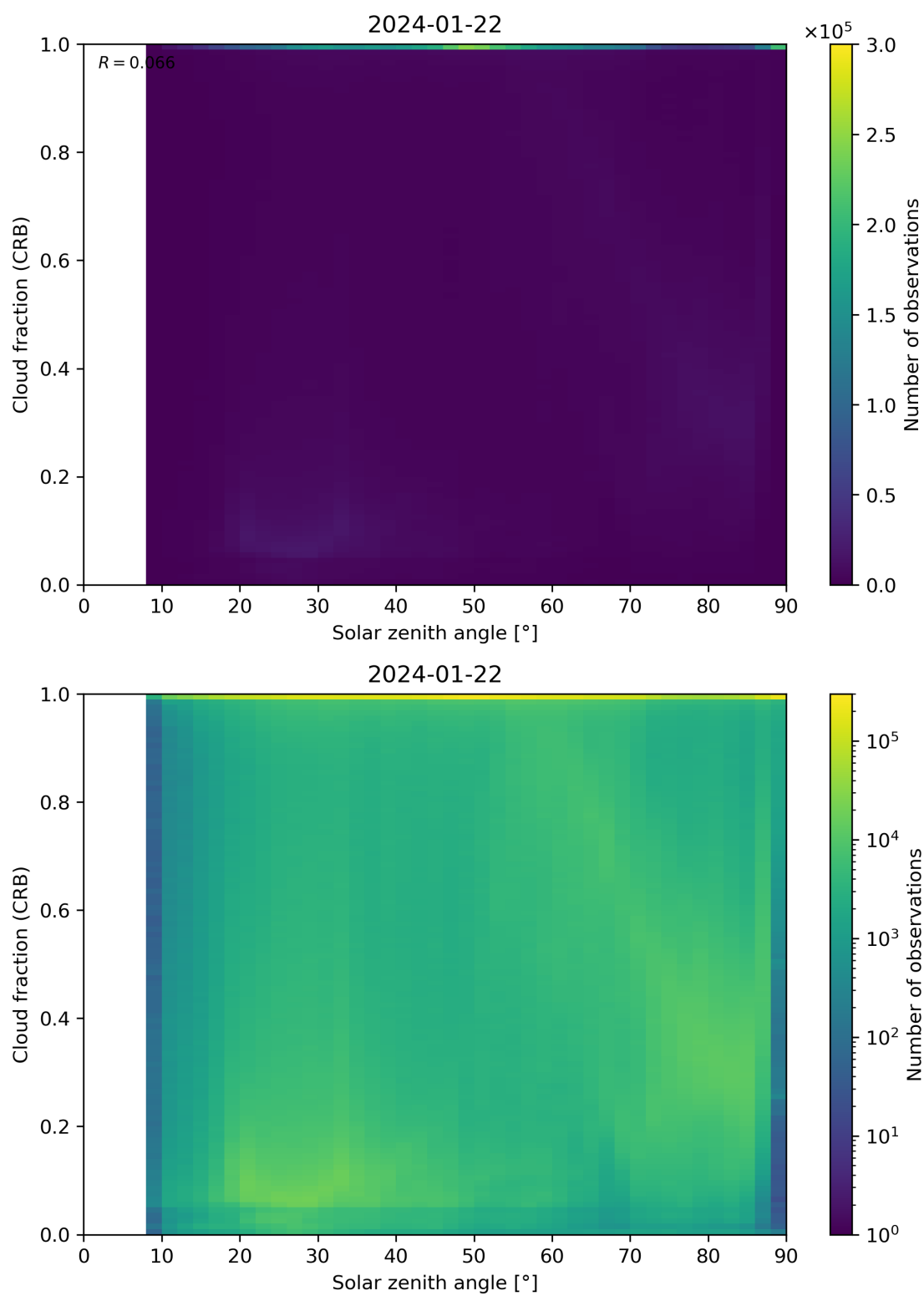
Figure 101: Scatter density plot of “Solar zenith angle” against “Cloud fraction (CRB)” for 2024-01-21 to 2024-01-23.
