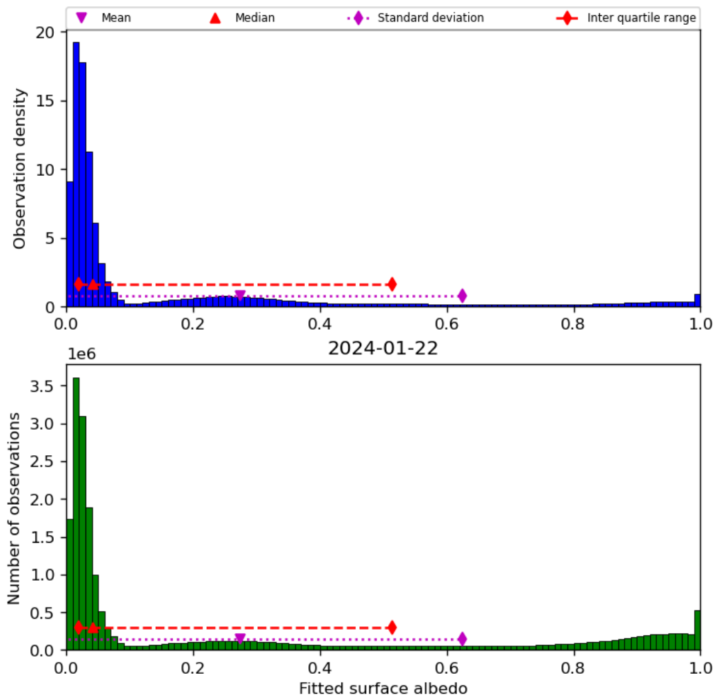
Figure 45: Histogram of “Fitted surface albedo” for 2024-01-21 to 2024-01-23
