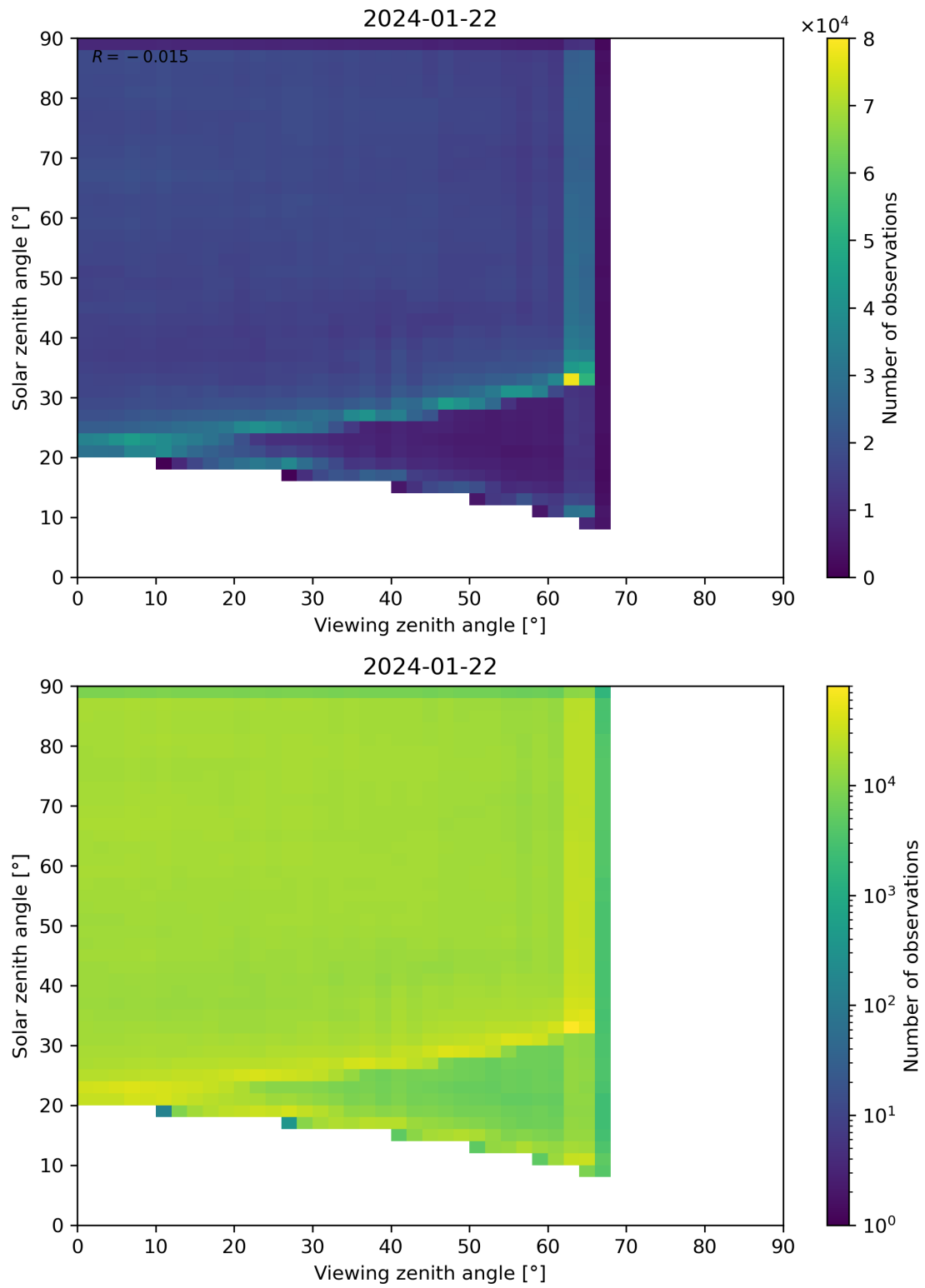
Figure 114: Scatter density plot of “Viewing zenith angle” against “Solar zenith angle” for 2024-01-21 to 2024-01-23.
