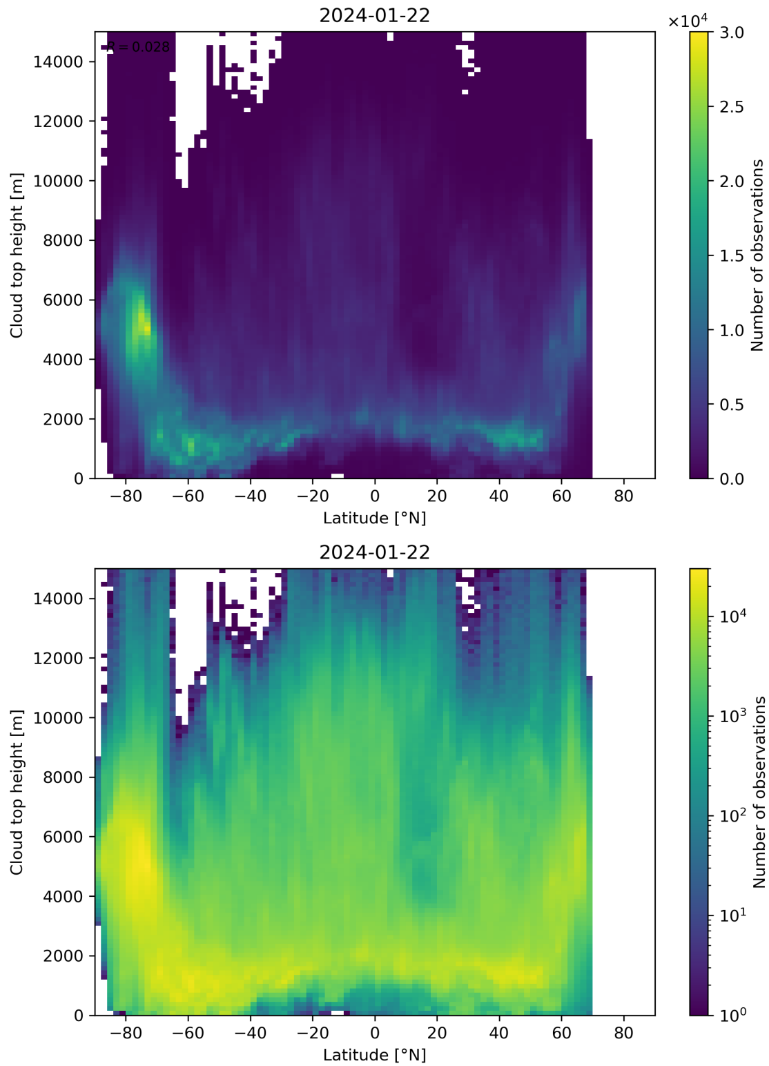
Figure 97: Scatter density plot of “Latitude” against “Cloud top height” for 2024-01-21 to 2024-01-23.
