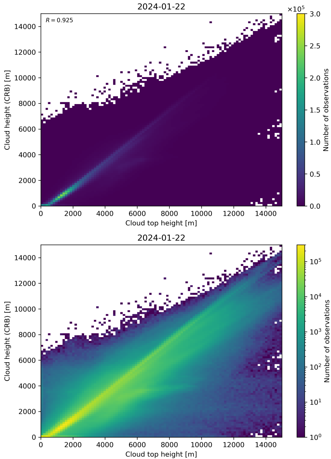
Figure 89: Scatter density plot of “Cloud top height” against “Cloud height (CRB)” for 2024-01-21 to 2024-01-23.
