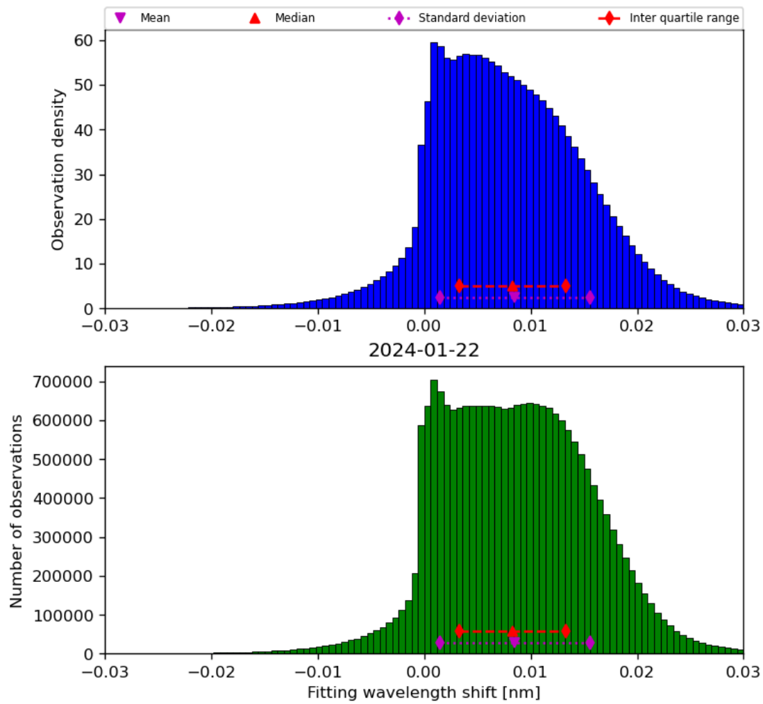
Figure 49: Histogram of “Fitting wavelength shift” for 2024-01-21 to 2024-01-23
