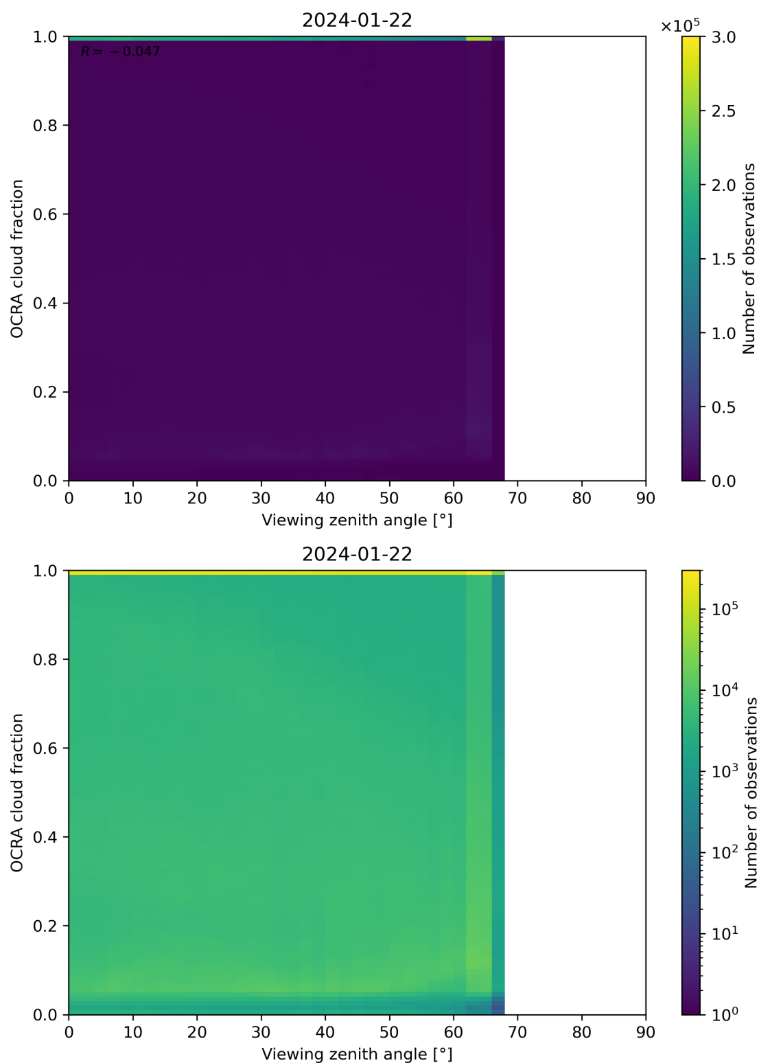
Figure 108: Scatter density plot of “Viewing zenith angle” against “OCRA cloud fraction” for 2024-01-21 to 2024-01-23.
