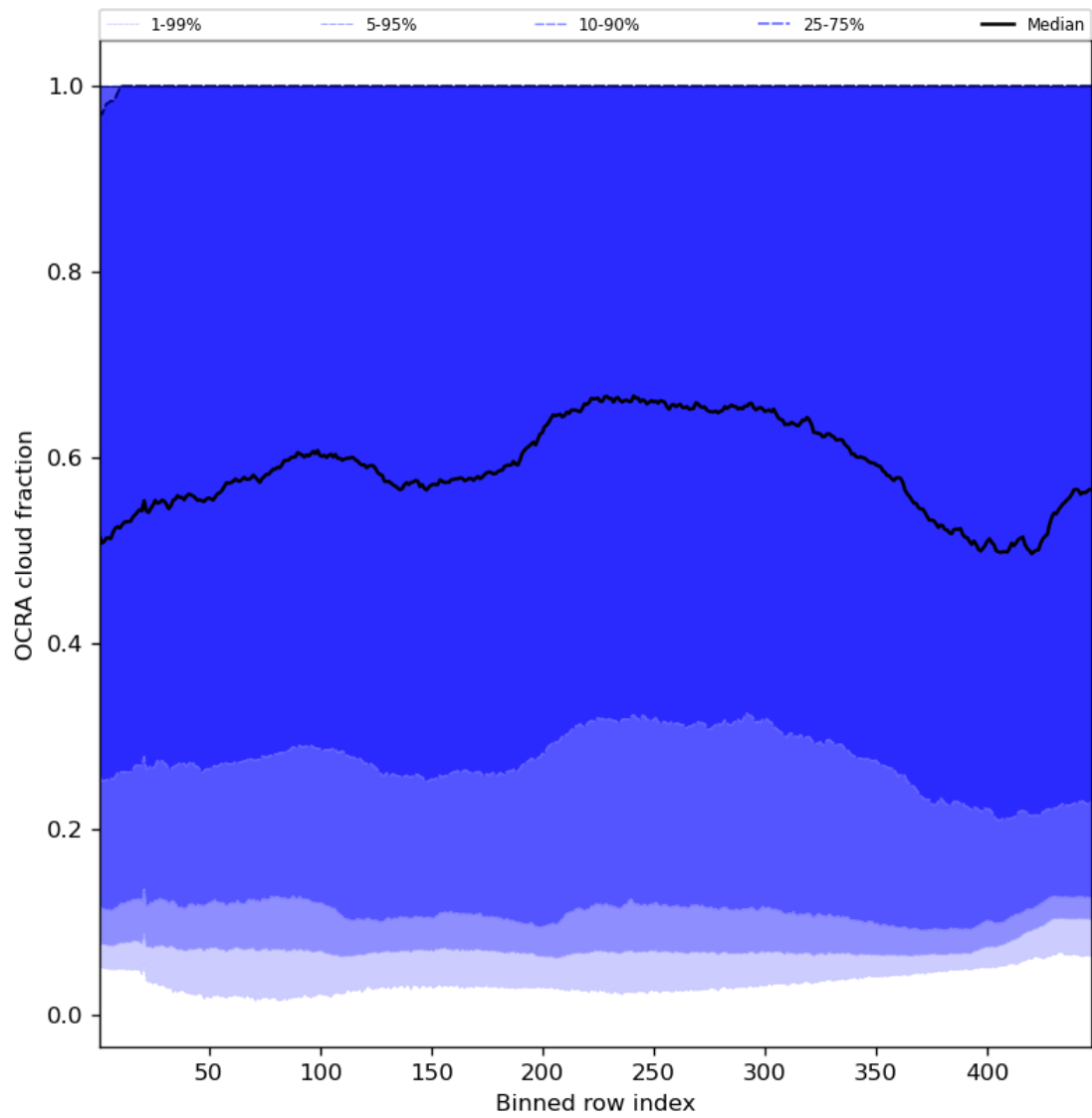
Figure 66: Along track statistics of “OCRA cloud fraction” for 2024-01-21 to 2024-01-23
