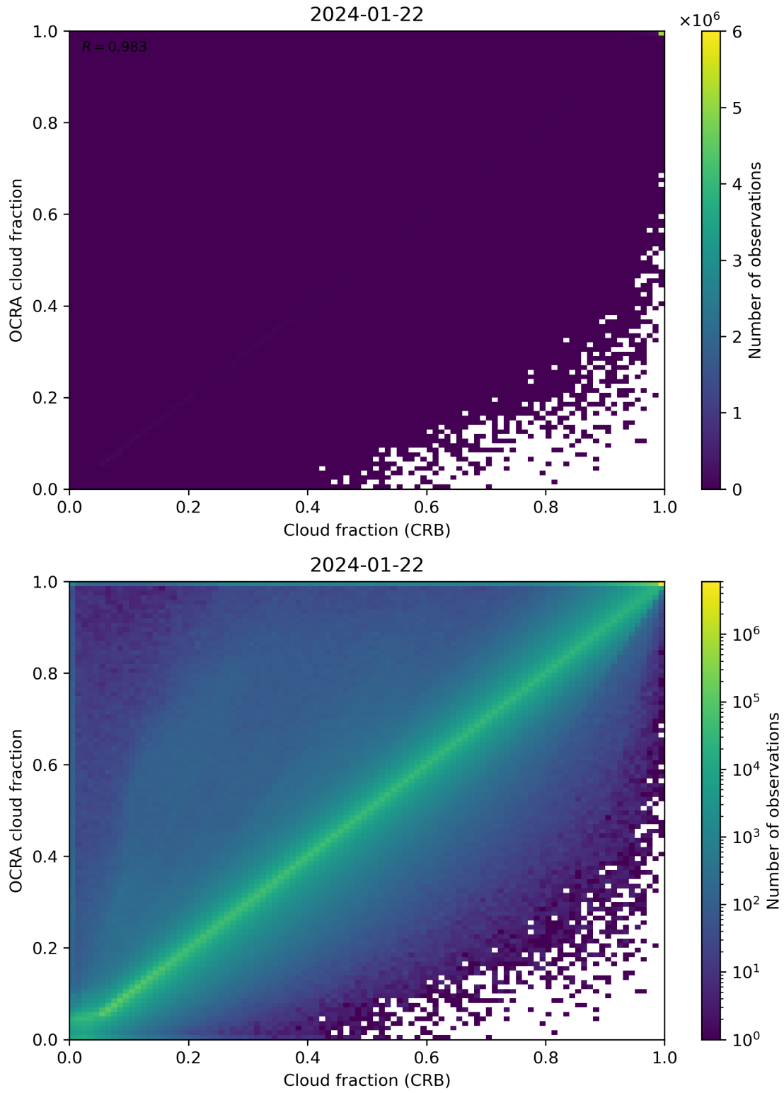
Figure 78: Scatter density plot of “Cloud fraction (CRB)” against “OCRA cloud fraction” for 2024-01-21 to 2024-01-23.
