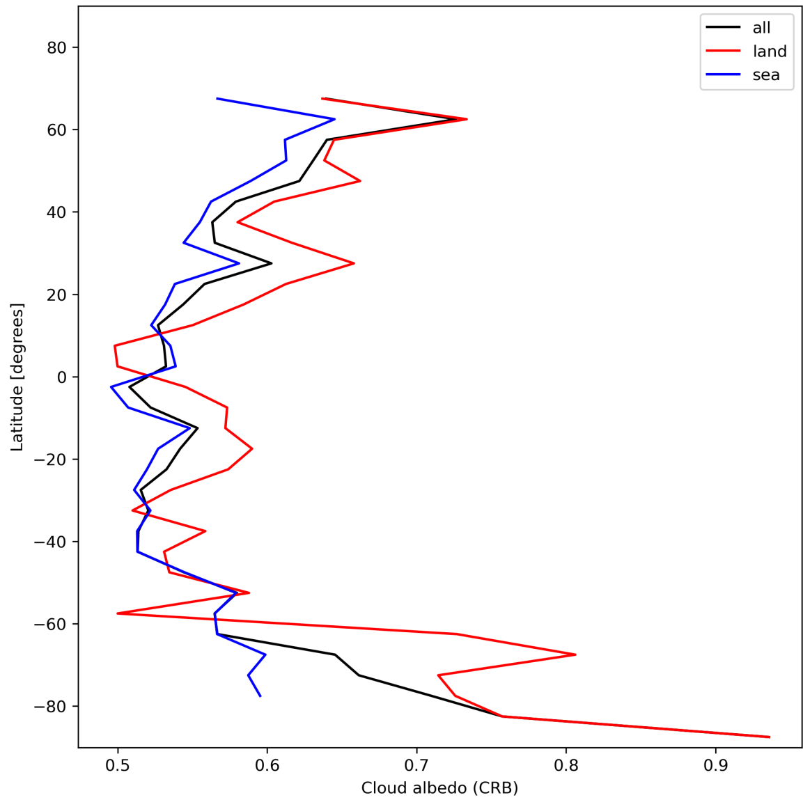
Figure 28: Zonal average of “Cloud albedo (CRB)” for 2024-01-21 to 2024-01-23.
