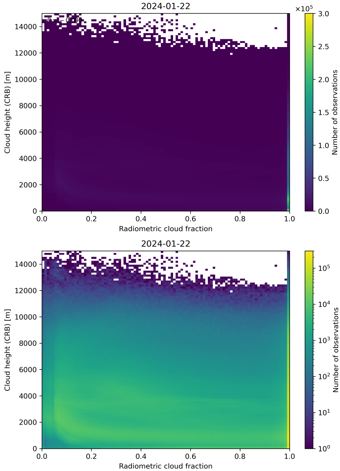
Figure 74: Scatter density plot of “Radiometric cloud fraction” against “Cloud height (CRB)” for 2024-01-21 to 2024-01-23.
