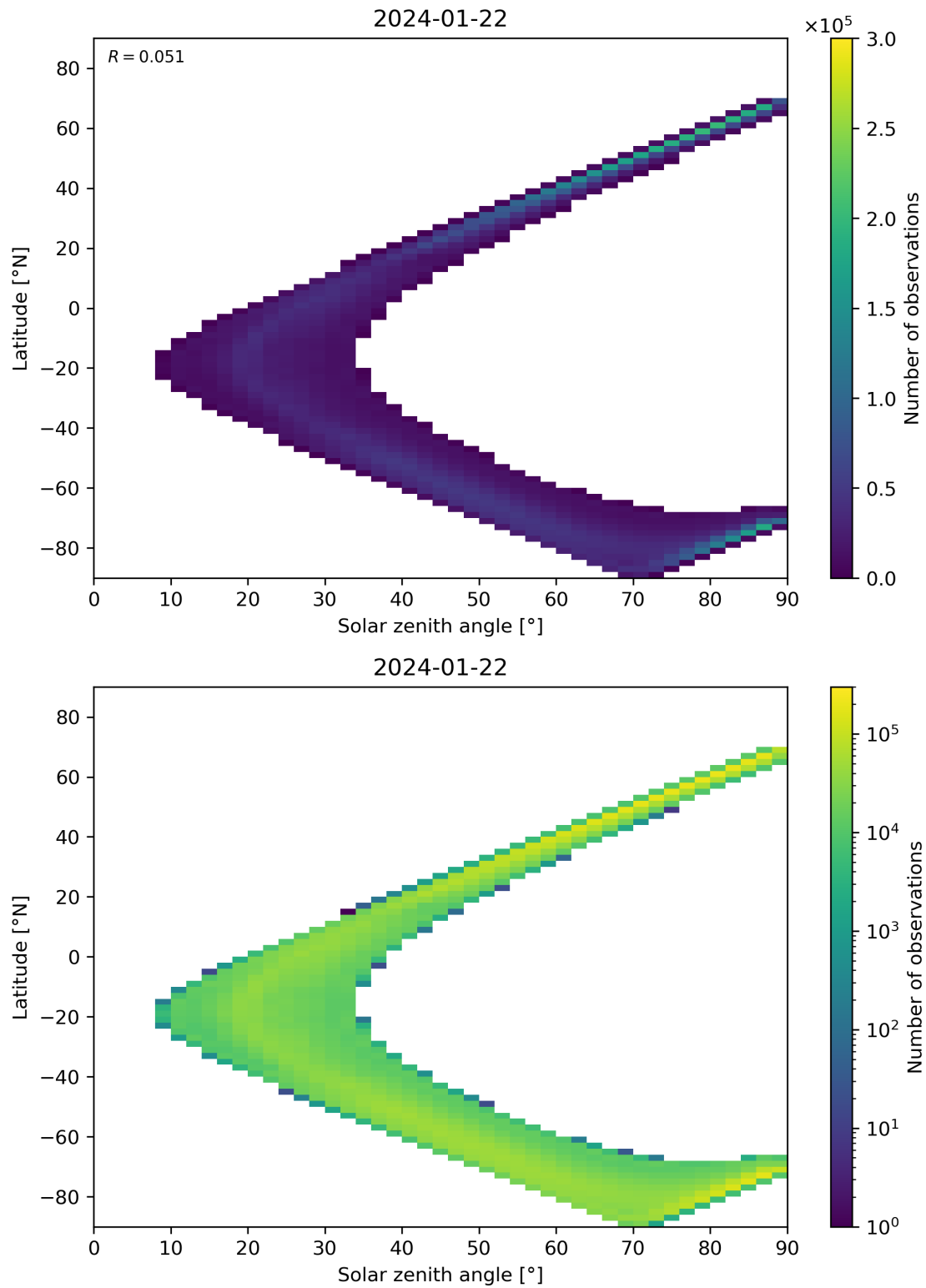
Figure 105: Scatter density plot of “Solar zenith angle” against “Latitude” for 2024-01-21 to 2024-01-23.
