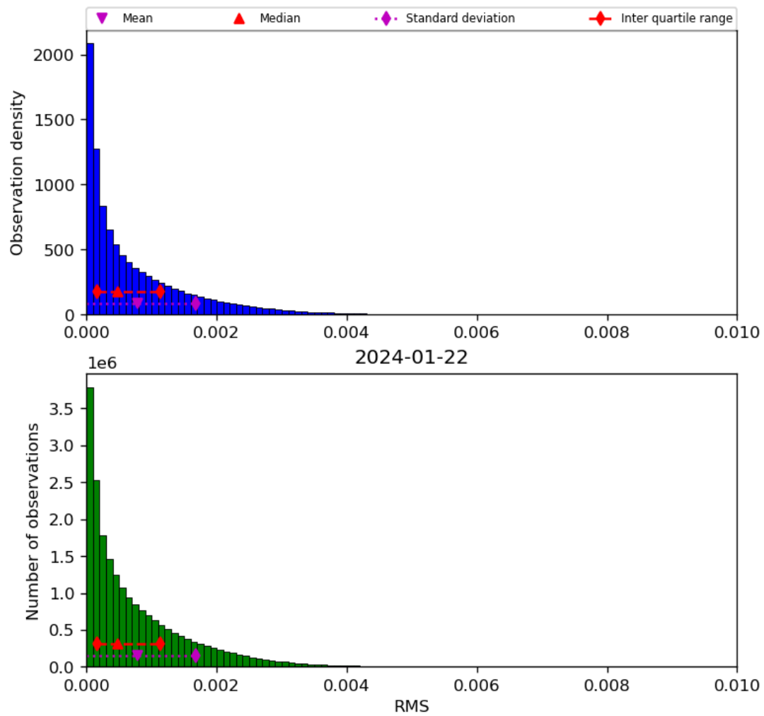
Figure 47: Histogram of “RMS” for 2024-01-21 to 2024-01-23
