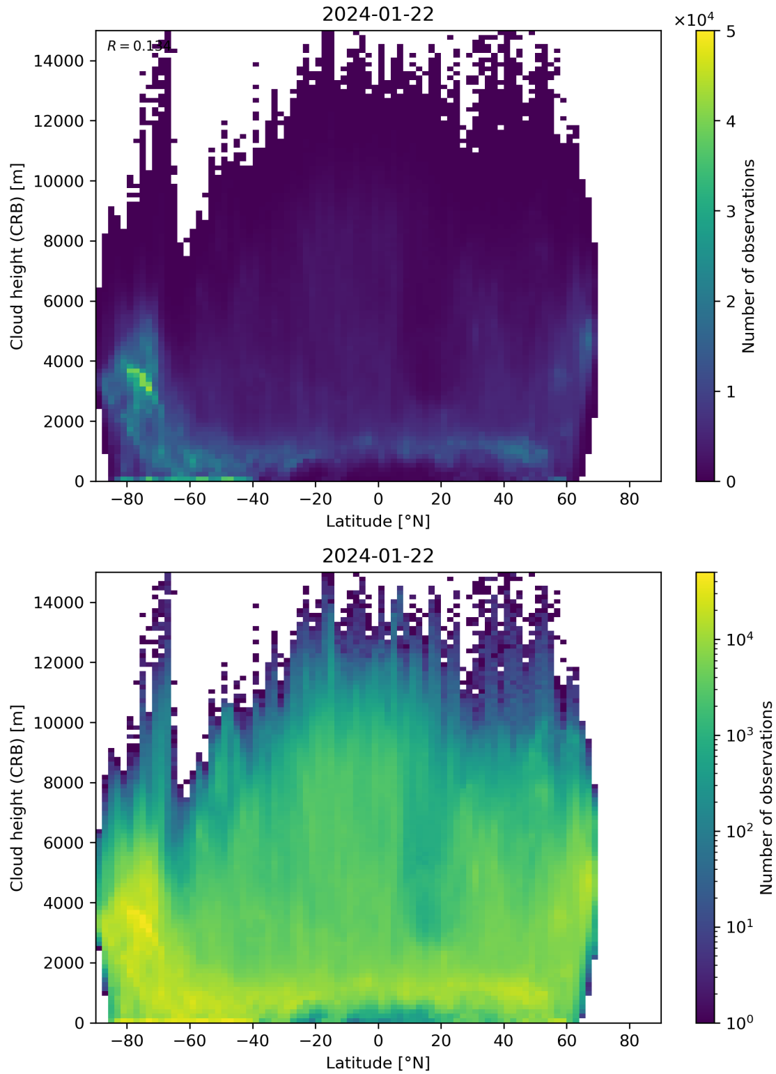
Figure 95: Scatter density plot of “Latitude” against “Cloud height (CRB)” for 2024-01-21 to 2024-01-23.
