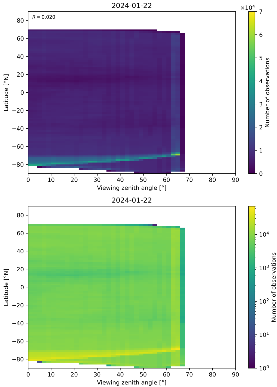
Figure 113: Scatter density plot of “Viewing zenith angle” against “Latitude” for 2024-01-21 to 2024-01-23.
