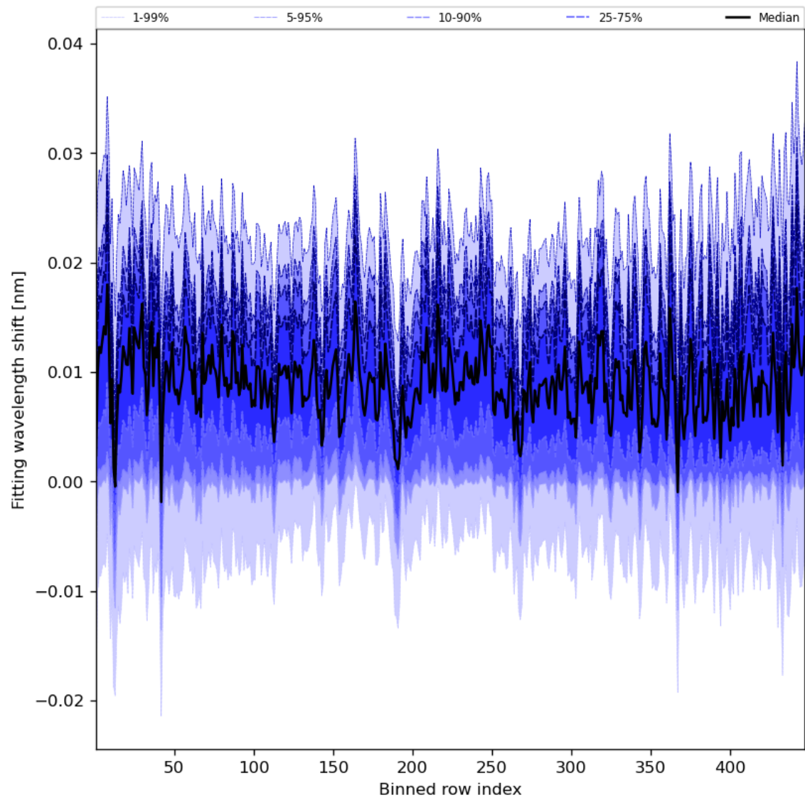
Figure 65: Along track statistics of “Fitting wavelength shift” for 2024-01-21 to 2024-01-23
