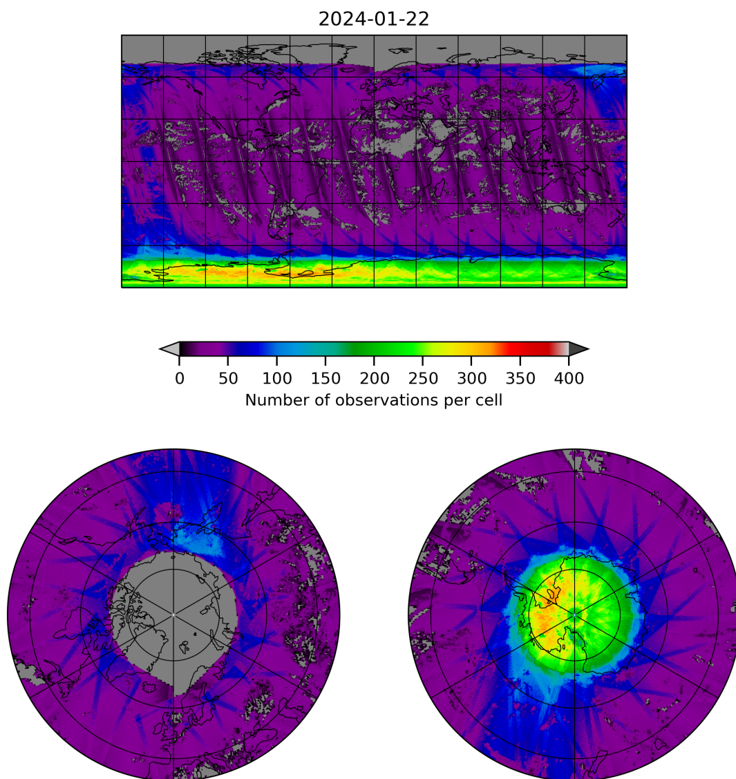
Figure 21: Map of the number of observations for 2024-01-21 to 2024-01-23
