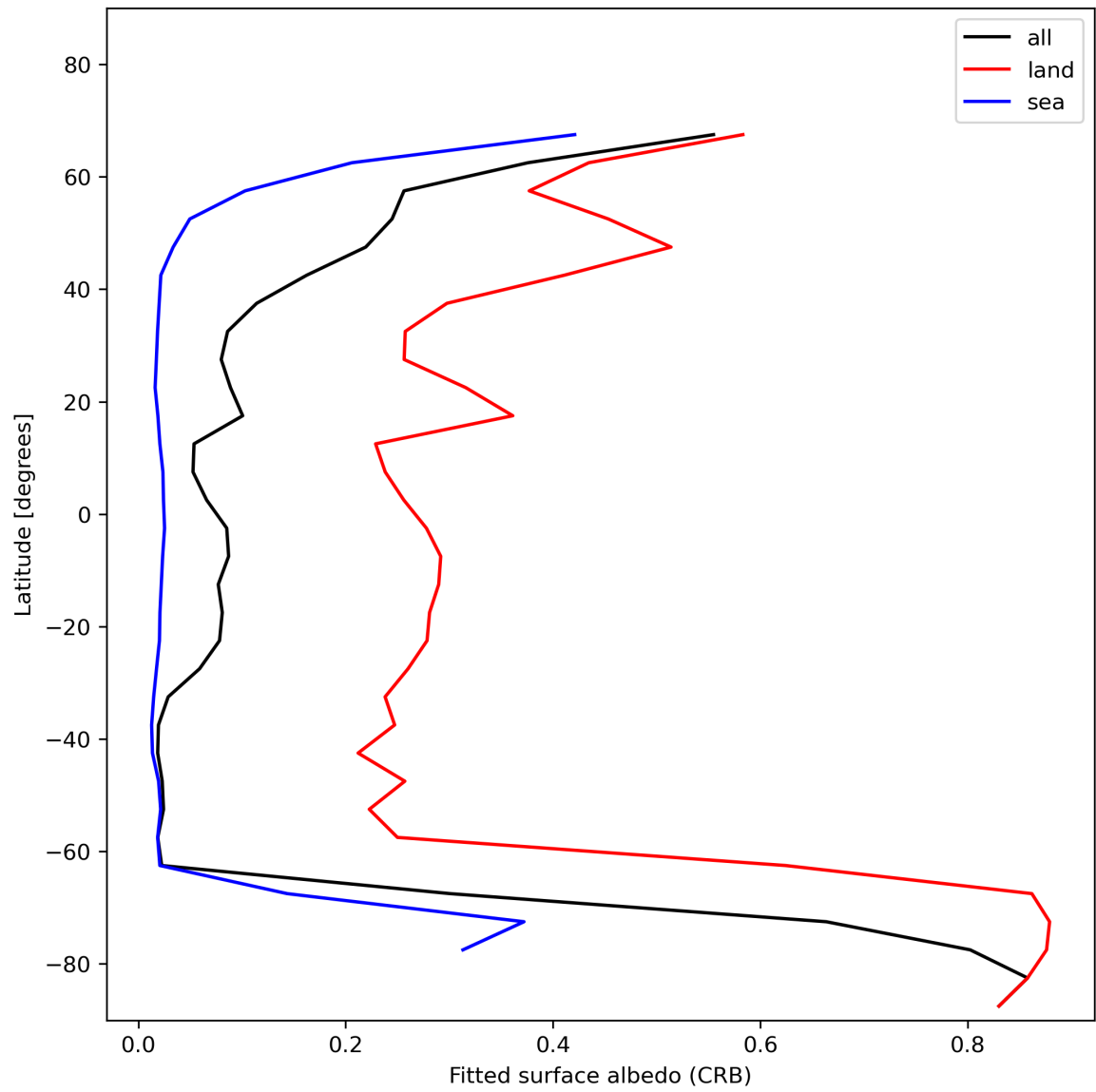
Figure 30: Zonal average of “Fitted surface albedo (CRB)” for 2024-01-21 to 2024-01-23.
