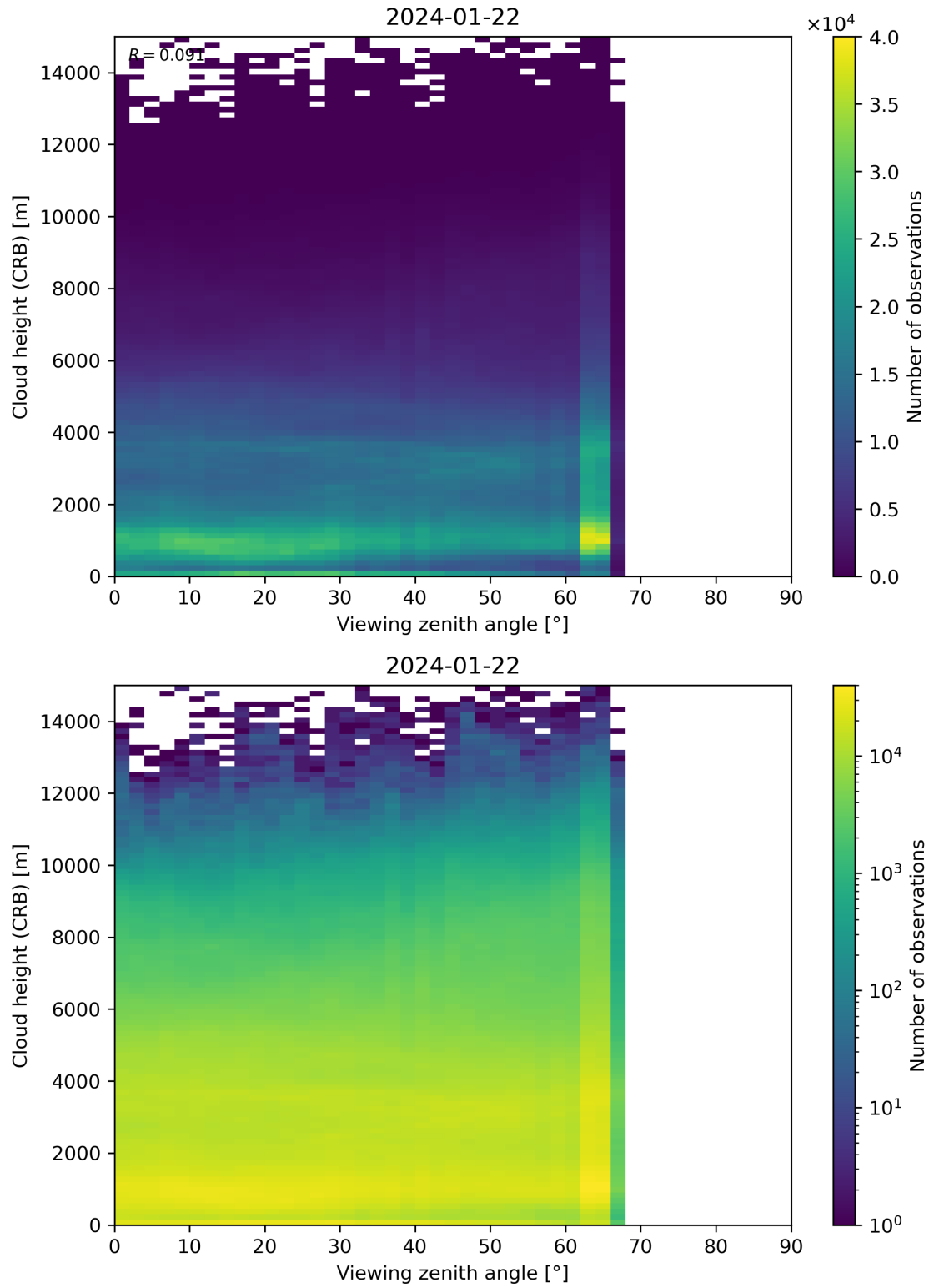
Figure 110: Scatter density plot of “Viewing zenith angle” against “Cloud height (CRB)” for 2024-01-21 to 2024-01-23.
