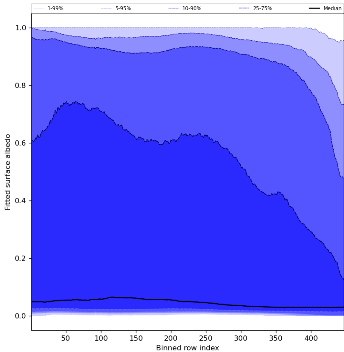
Figure 61: Along track statistics of “Fitted surface albedo” for 2024-01-21 to 2024-01-23
