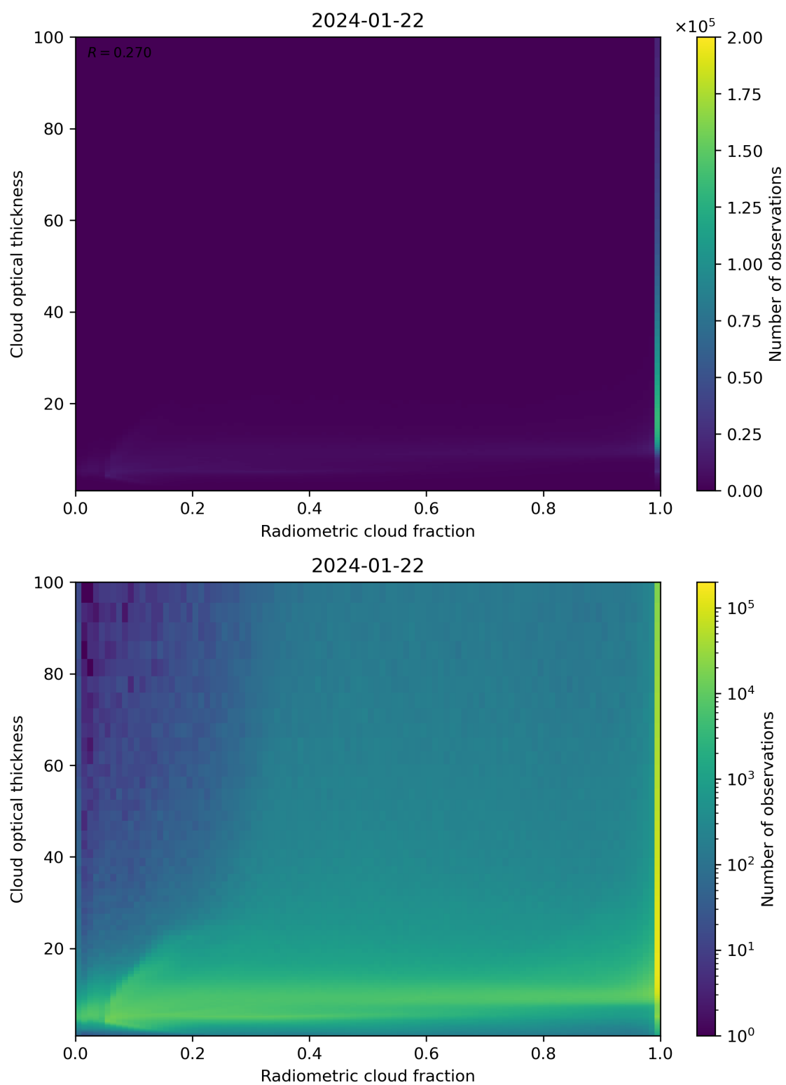
Figure 75: Scatter density plot of “Radiometric cloud fraction” against “Cloud optical thickness” for 2024-01-21 to 2024-01-23.
