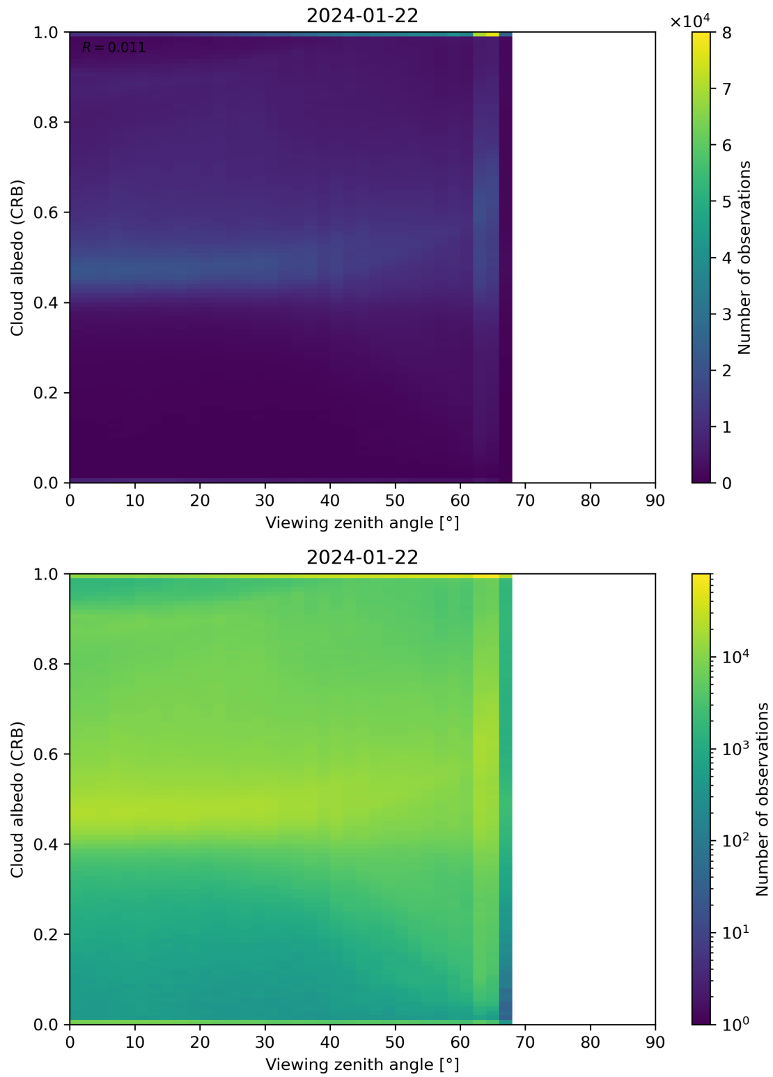
Figure 106: Scatter density plot of “Viewing zenith angle” against “Cloud albedo (CRB)” for 2024-01-21 to 2024-01-23.
