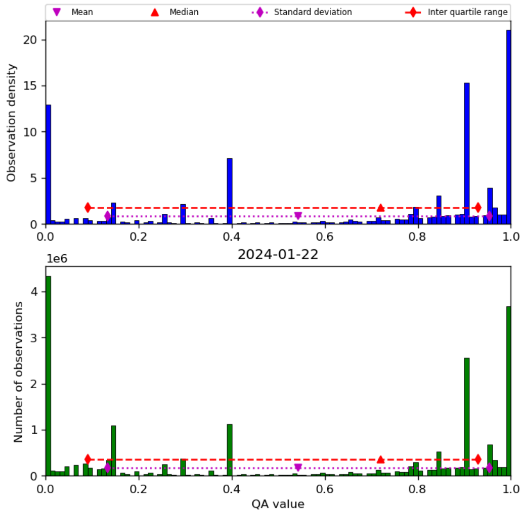
Figure 38: Histogram of “QA value” for 2024-01-21 to 2024-01-23
