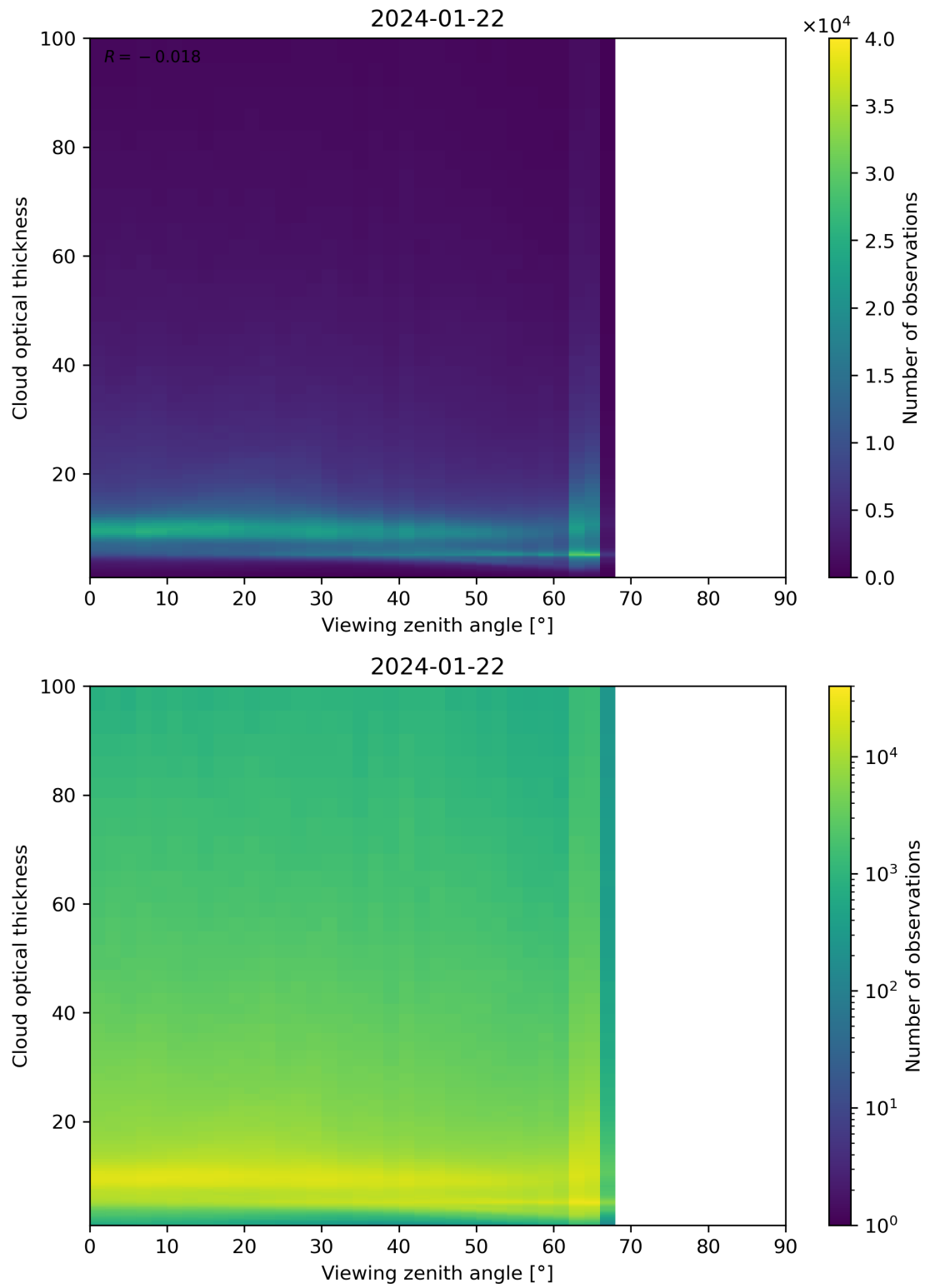
Figure 111: Scatter density plot of “Viewing zenith angle” against “Cloud optical thickness” for 2024-01-21 to 2024-01-23.
