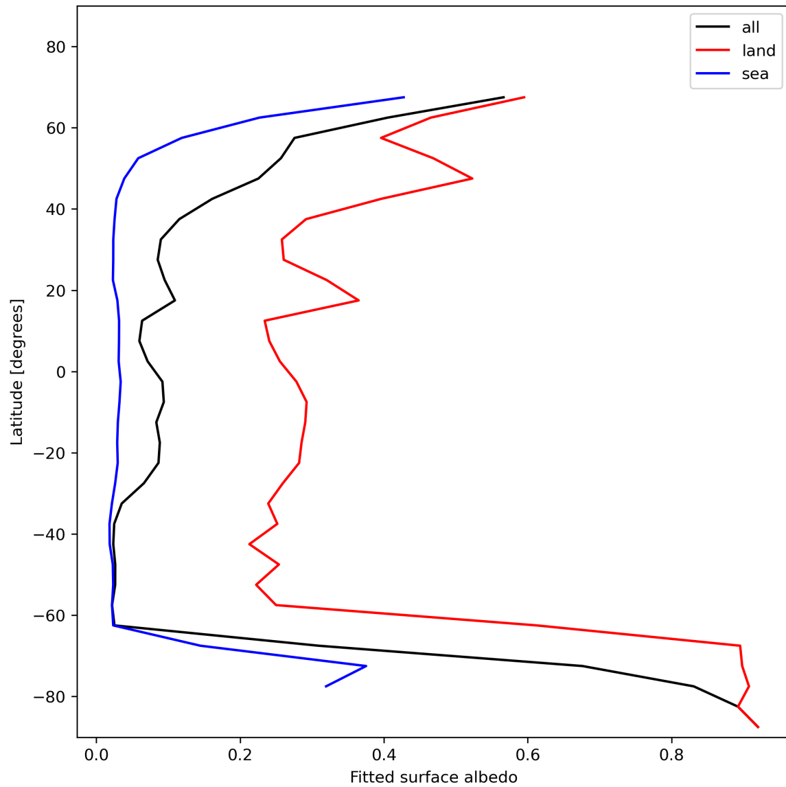
Figure 29: Zonal average of “Fitted surface albedo” for 2024-01-21 to 2024-01-23.
