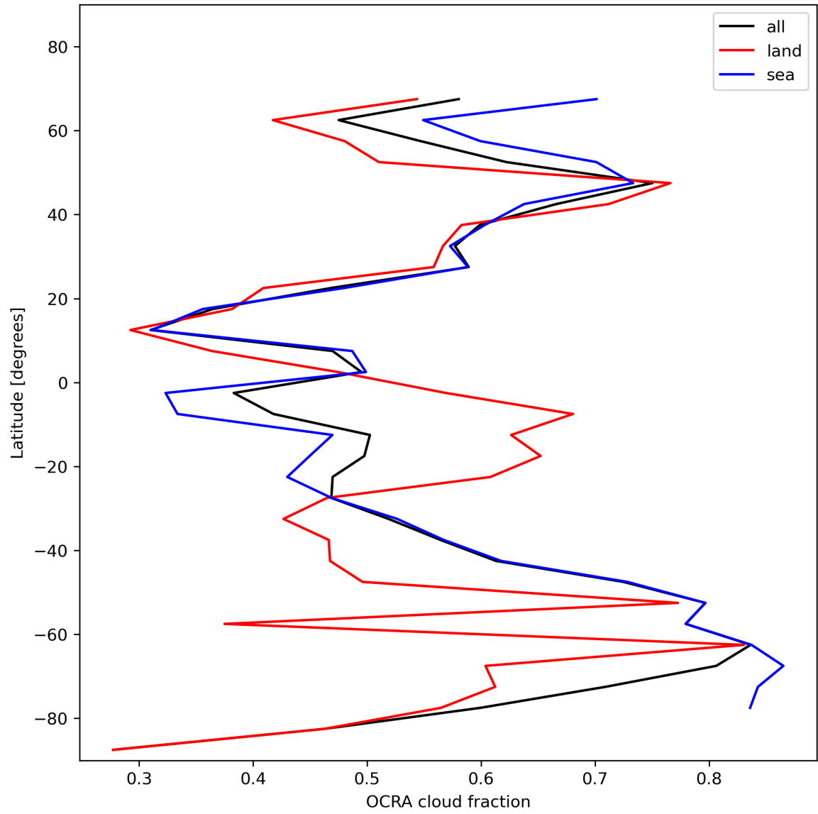
Figure 34: Zonal average of “OCRA cloud fraction” for 2024-01-21 to 2024-01-23.
