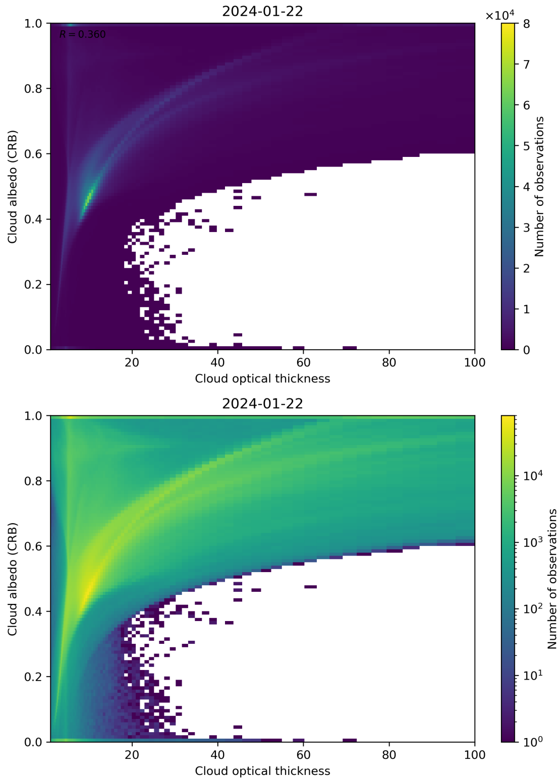
Figure 82: Scatter density plot of “Cloud optical thickness” against “Cloud albedo (CRB)” for 2024-01-21 to 2024-01-23.
