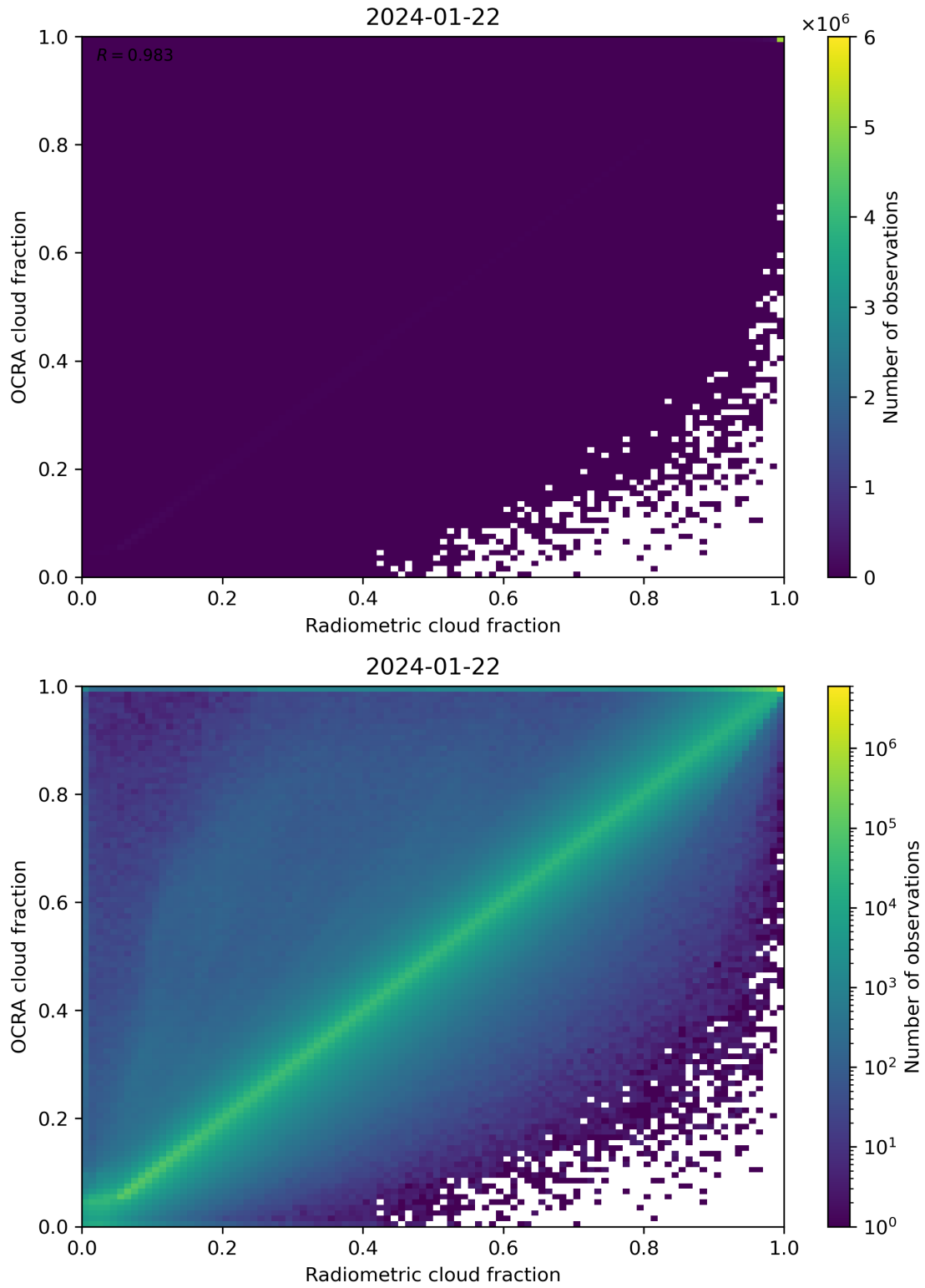
Figure 72: Scatter density plot of “Radiometric cloud fraction” against “OCRA cloud fraction” for 2024-01-21 to 2024-01-23.
