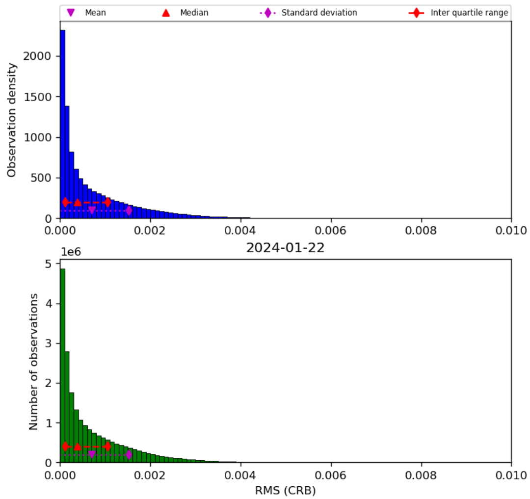
Figure 48: Histogram of “RMS (CRB)” for 2024-01-21 to 2024-01-23
