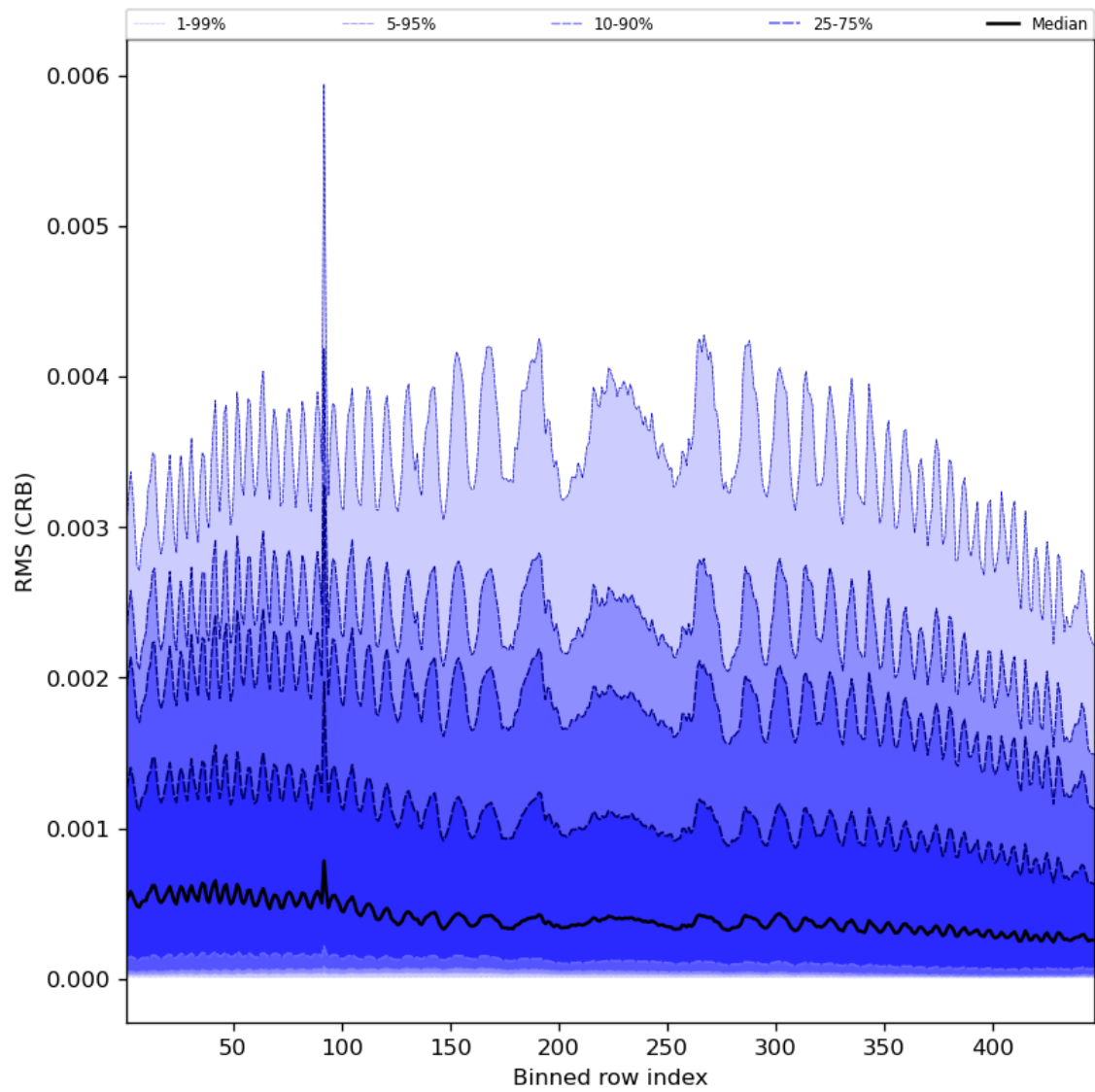
Figure 64: Along track statistics of “RMS (CRB)” for 2024-01-21 to 2024-01-23
