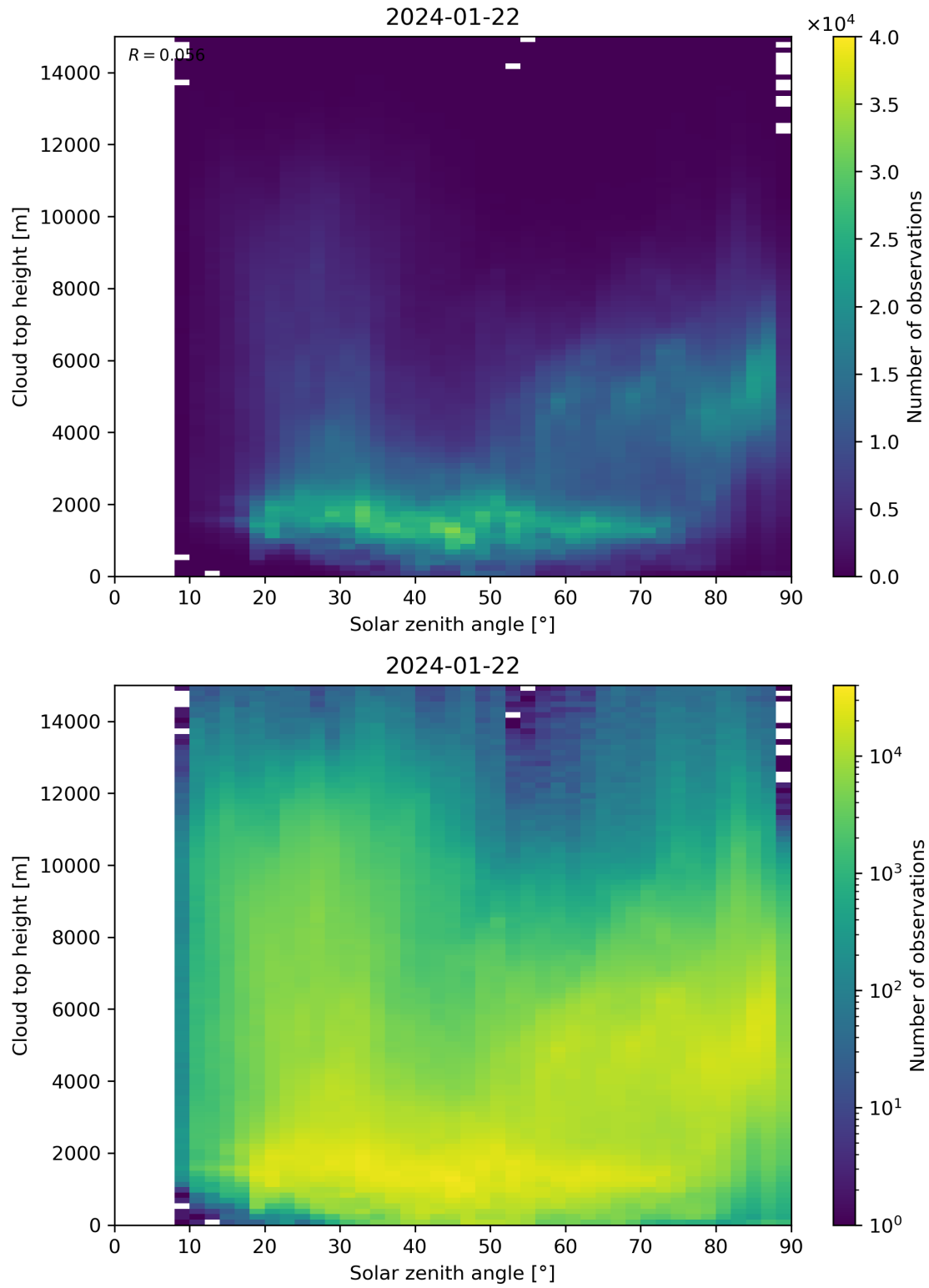
Figure 104: Scatter density plot of “Solar zenith angle” against “Cloud top height” for 2024-01-21 to 2024-01-23.
