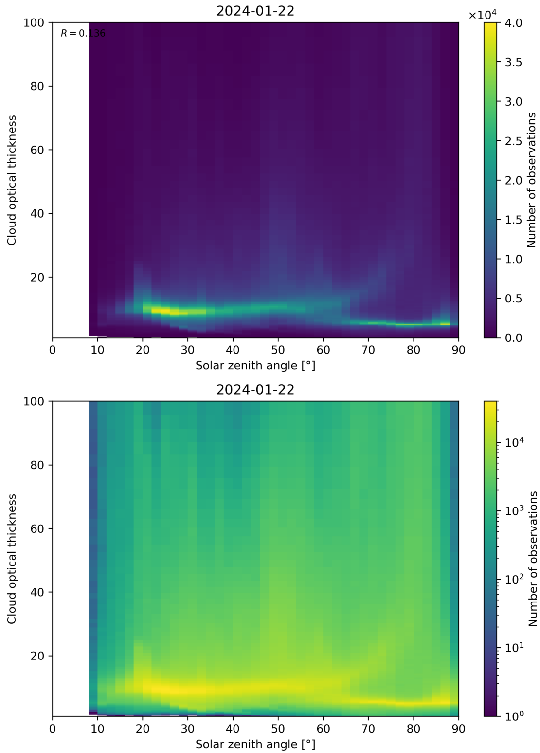
Figure 103: Scatter density plot of “Solar zenith angle” against “Cloud optical thickness” for 2024-01-21 to 2024-01-23.
