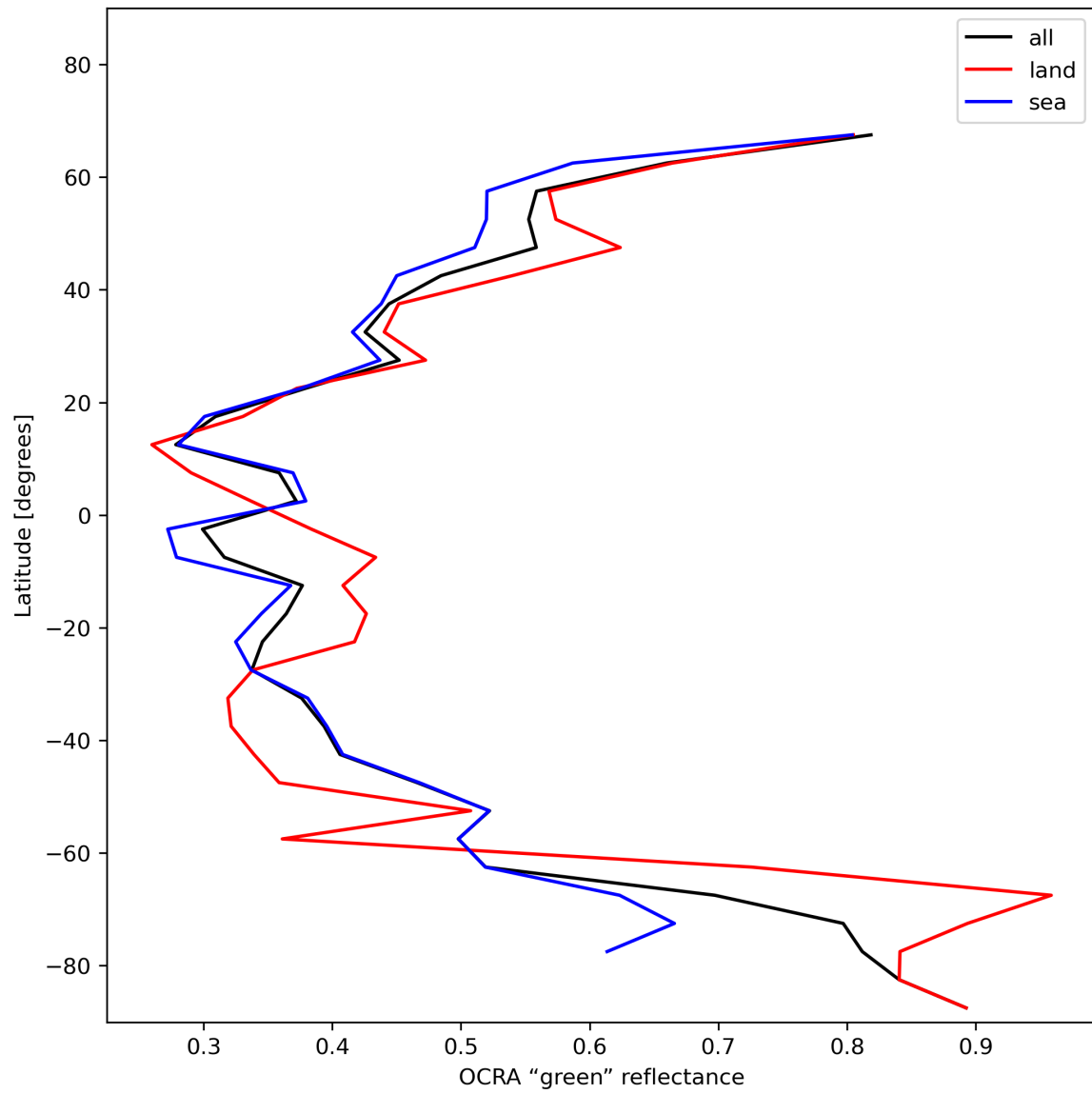
Figure 36: Zonal average of “OCRA “green” reflectance” for 2024-01-21 to 2024-01-23.
