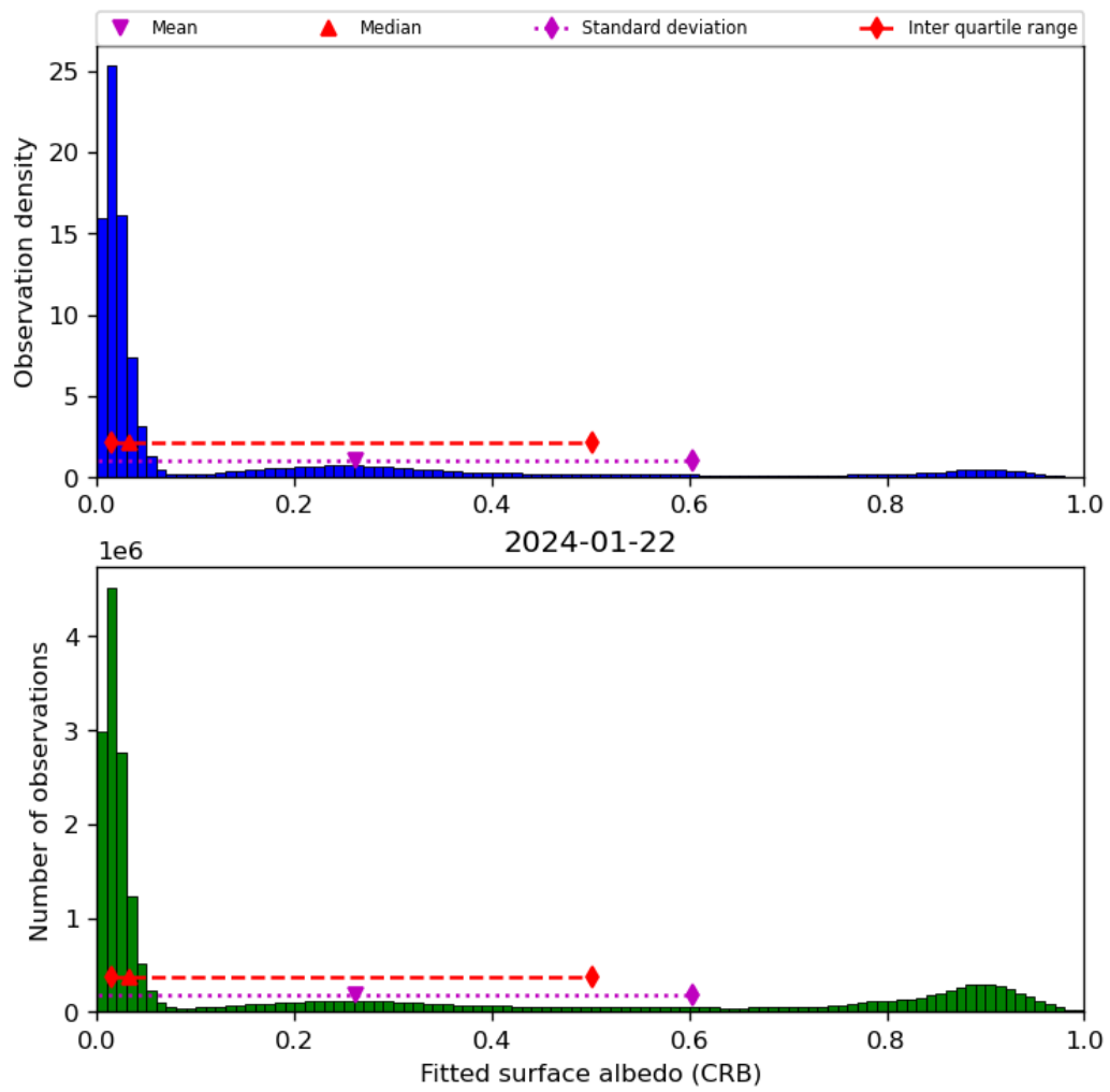
Figure 46: Histogram of “Fitted surface albedo (CRB)” for 2024-01-21 to 2024-01-23
