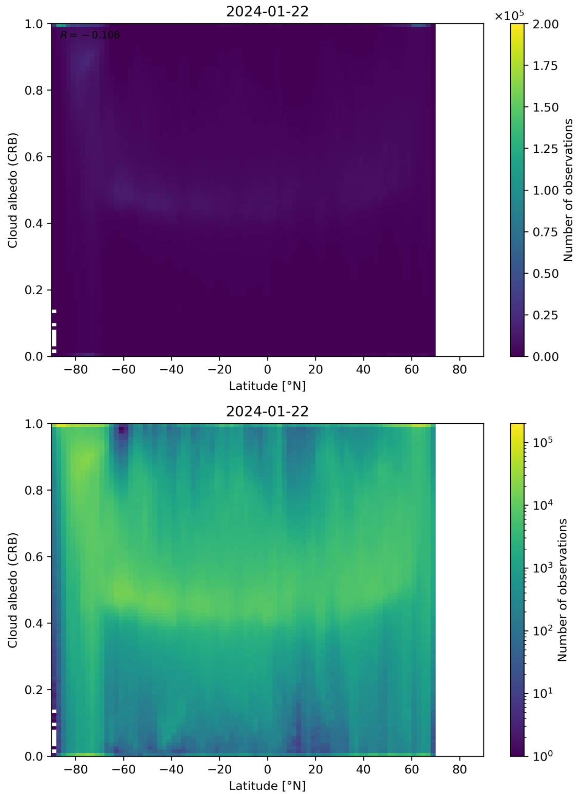
Figure 91: Scatter density plot of “Latitude” against “Cloud albedo (CRB)” for 2024-01-21 to 2024-01-23.
