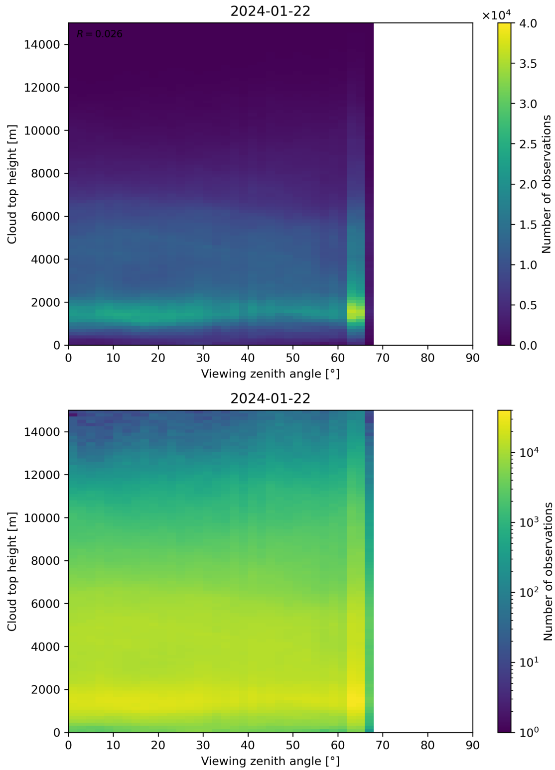
Figure 112: Scatter density plot of “Viewing zenith angle” against “Cloud top height” for 2024-01-21 to 2024-01-23.
