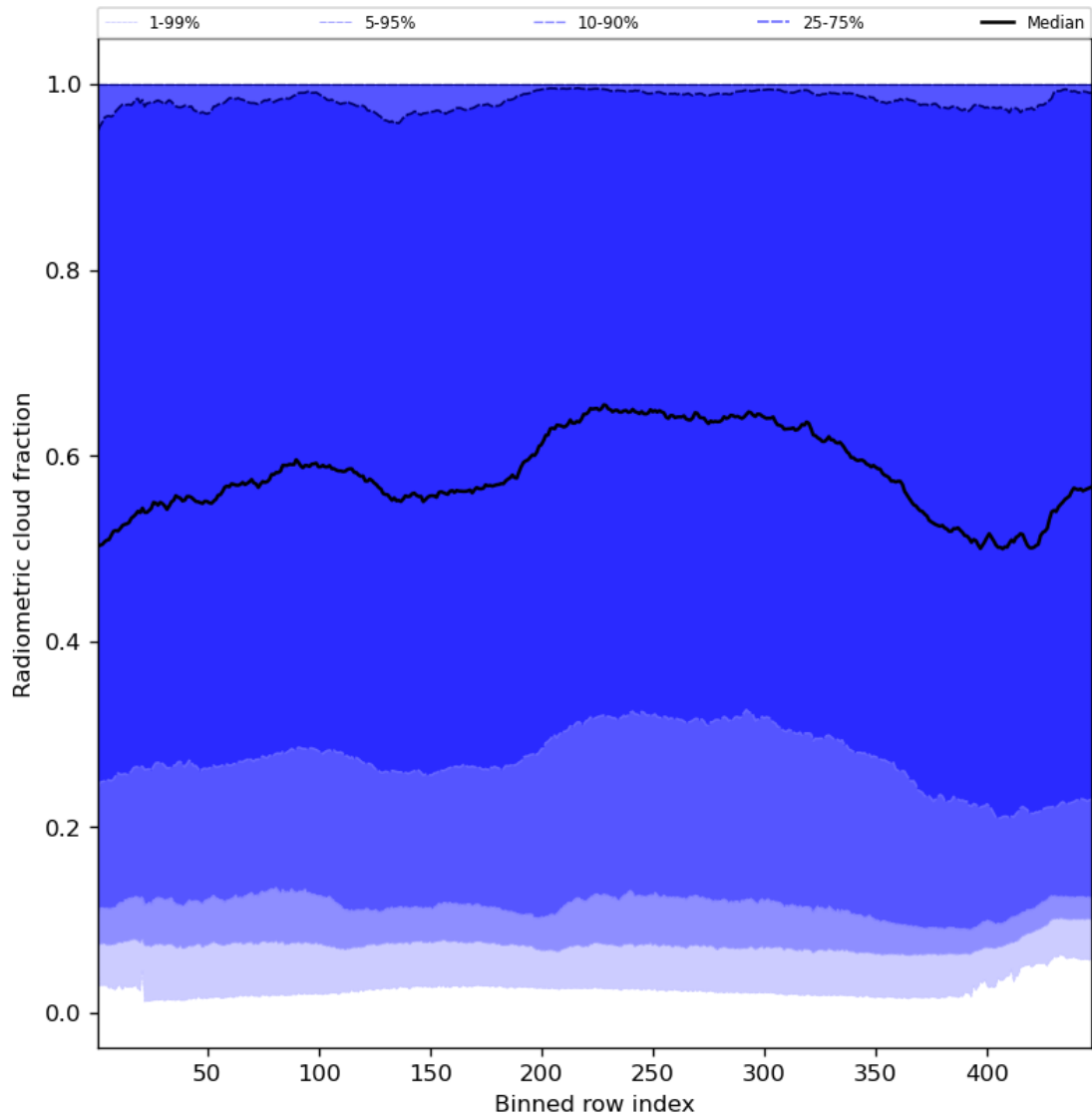
Figure 55: Along track statistics of “Radiometric cloud fraction” for 2024-01-21 to 2024-01-23
