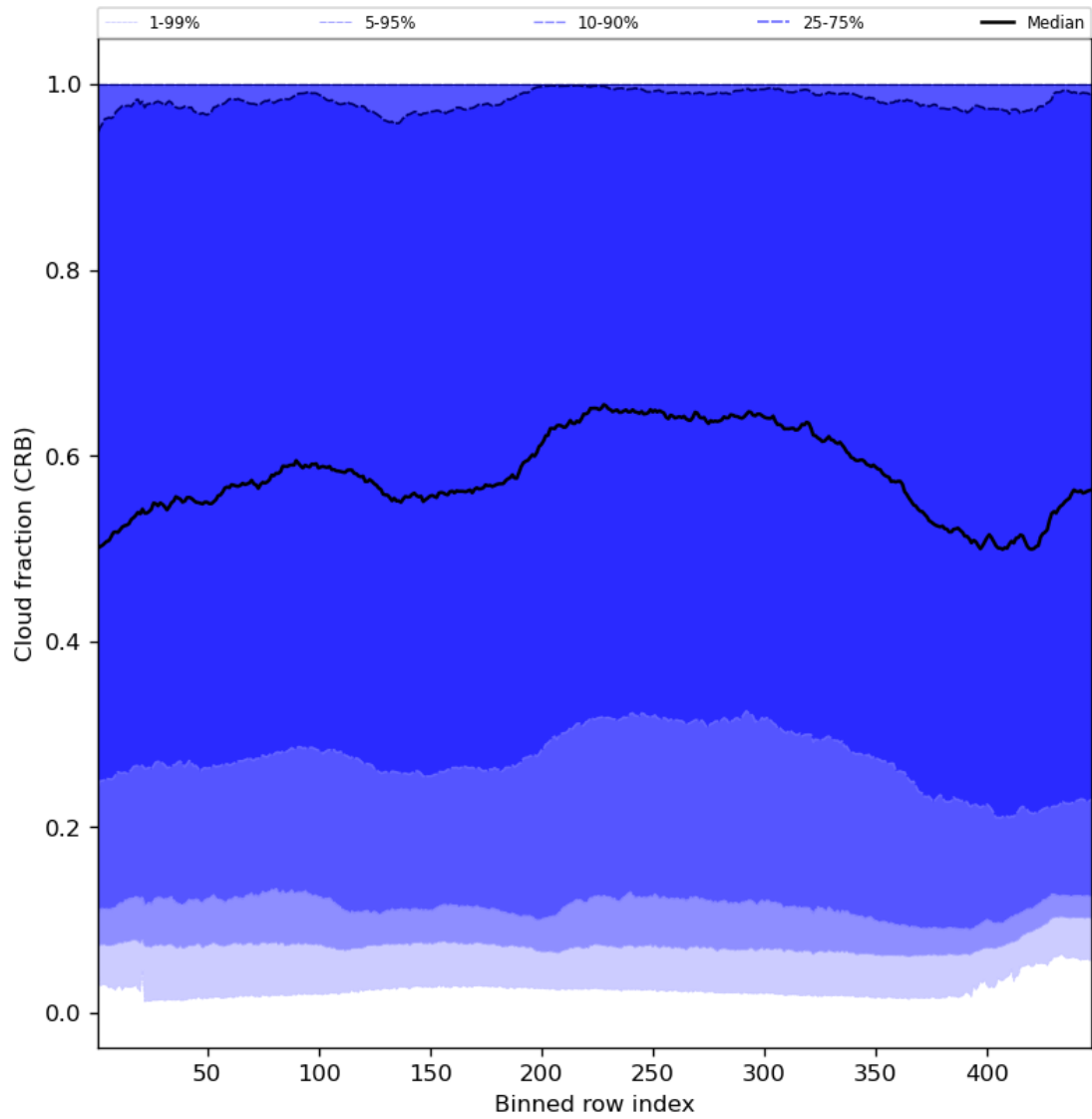
Figure 58: Along track statistics of “Cloud fraction (CRB)” for 2024-01-21 to 2024-01-23
