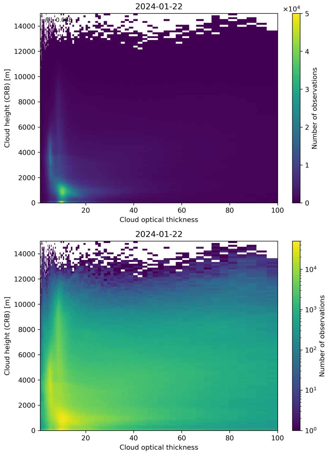
Figure 85: Scatter density plot of “Cloud optical thickness” against “Cloud height (CRB)” for 2024-01-21 to 2024-01-23.
