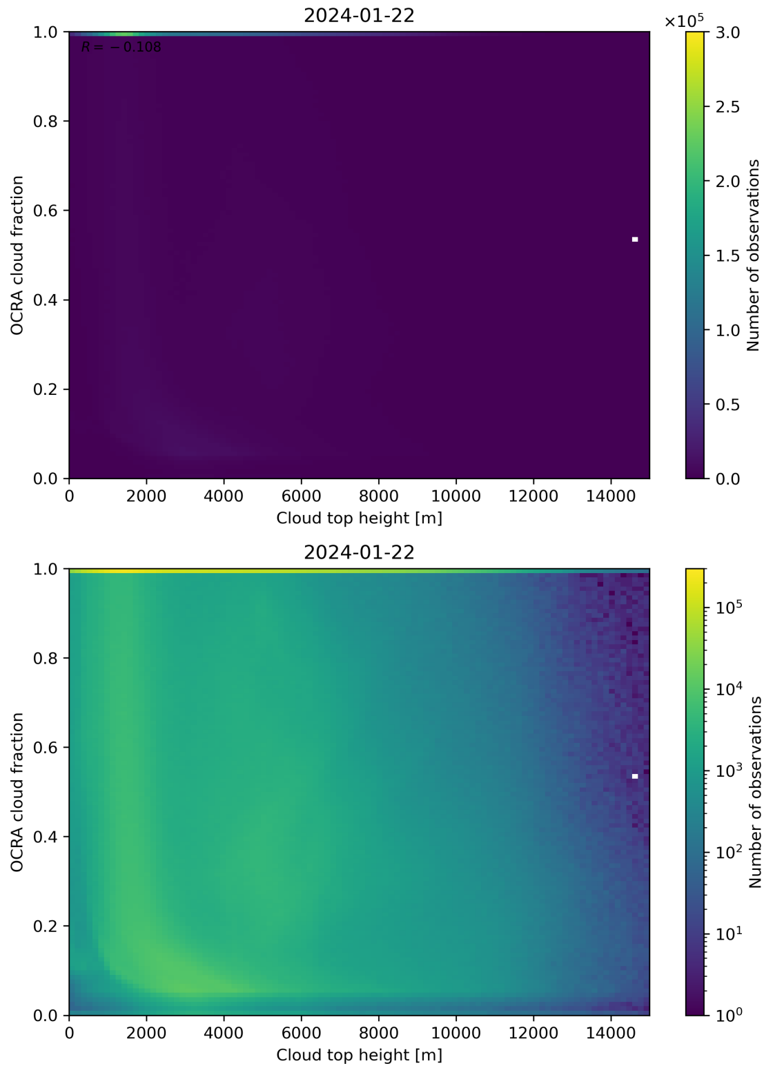
Figure 87: Scatter density plot of “Cloud top height” against “OCRA cloud fraction” for 2024-01-21 to 2024-01-23.
