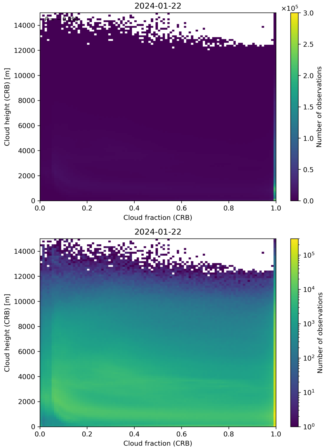
Figure 79: Scatter density plot of “Cloud fraction (CRB)” against “Cloud height (CRB)” for 2024-01-21 to 2024-01-23.
