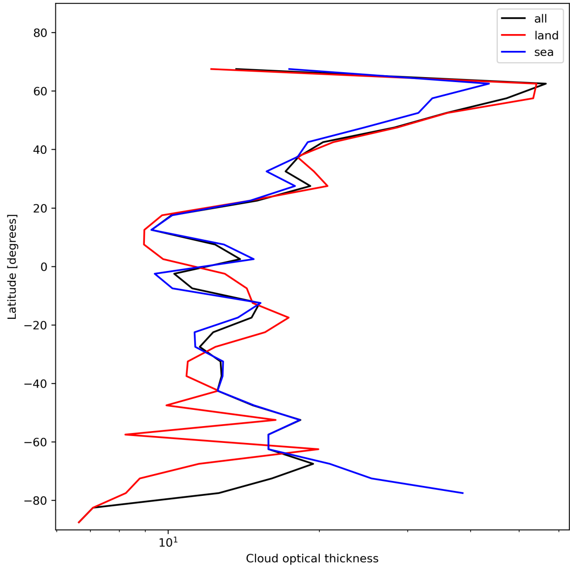
Figure 25: Zonal average of “Cloud optical thickness” for 2024-01-21 to 2024-01-23.
