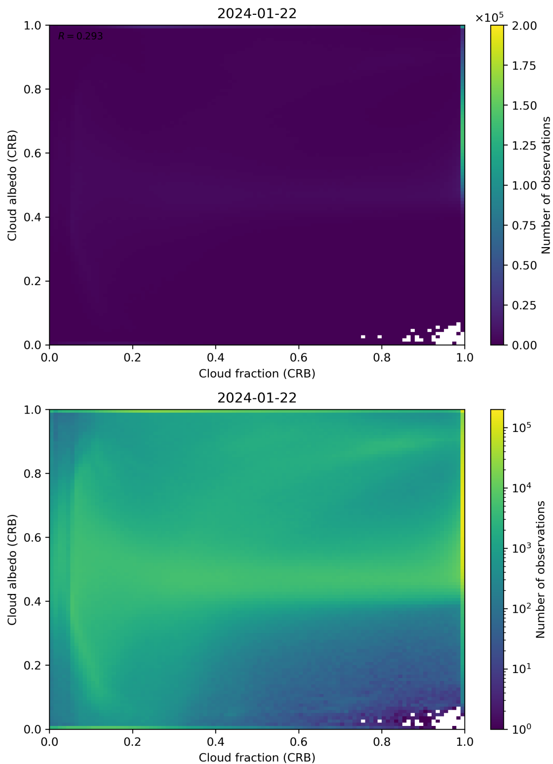
Figure 77: Scatter density plot of “Cloud fraction (CRB)” against “Cloud albedo (CRB)” for 2024-01-21 to 2024-01-23.
