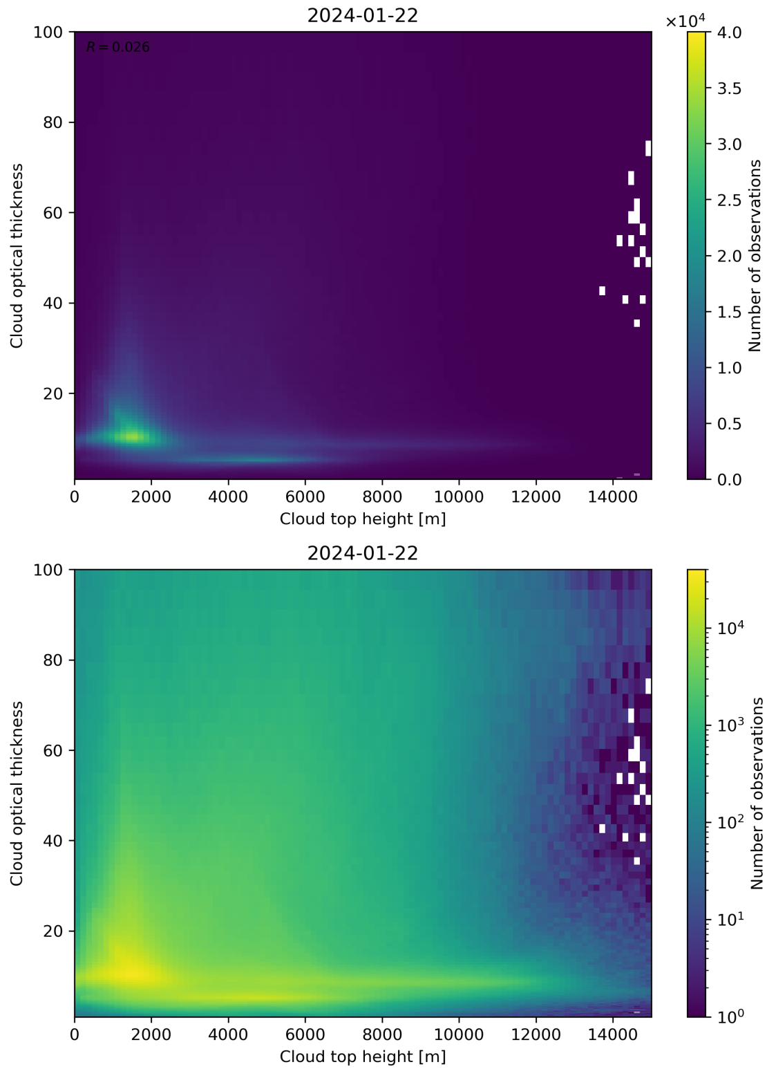
Figure 90: Scatter density plot of “Cloud top height” against “Cloud optical thickness” for 2024-01-21 to 2024-01-23.
