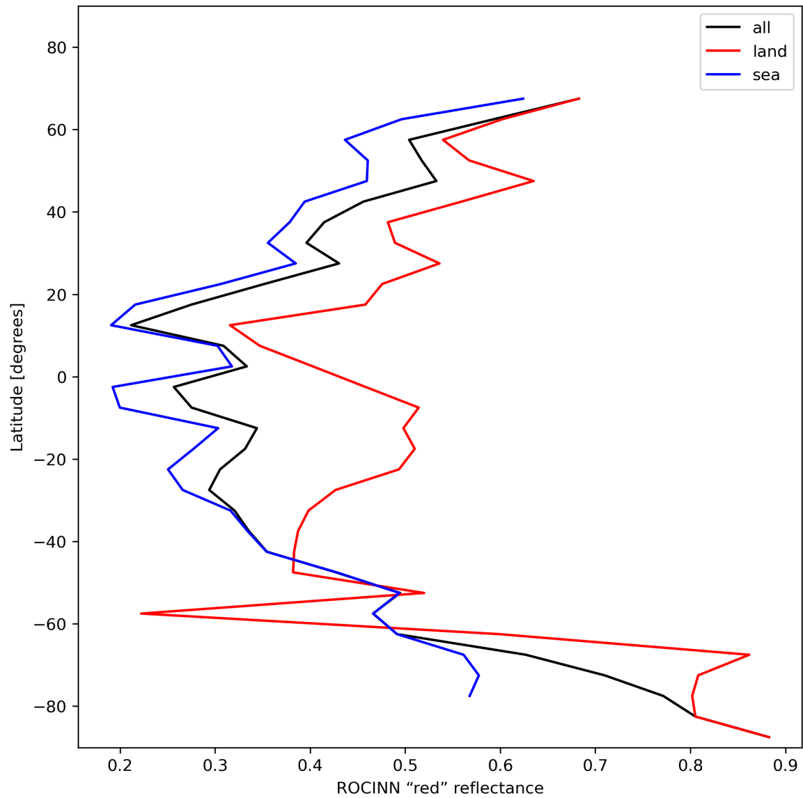
Figure 37: Zonal average of “ROCINN “red” reflectance” for 2024-01-21 to 2024-01-23.
