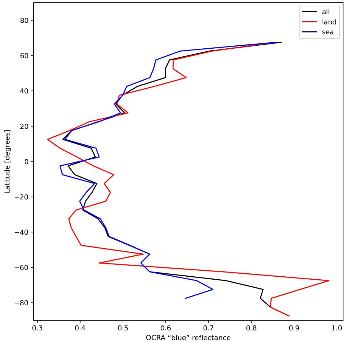
Figure 35: Zonal average of “OCRA “blue” reflectance” for 2024-01-21 to 2024-01-23.
