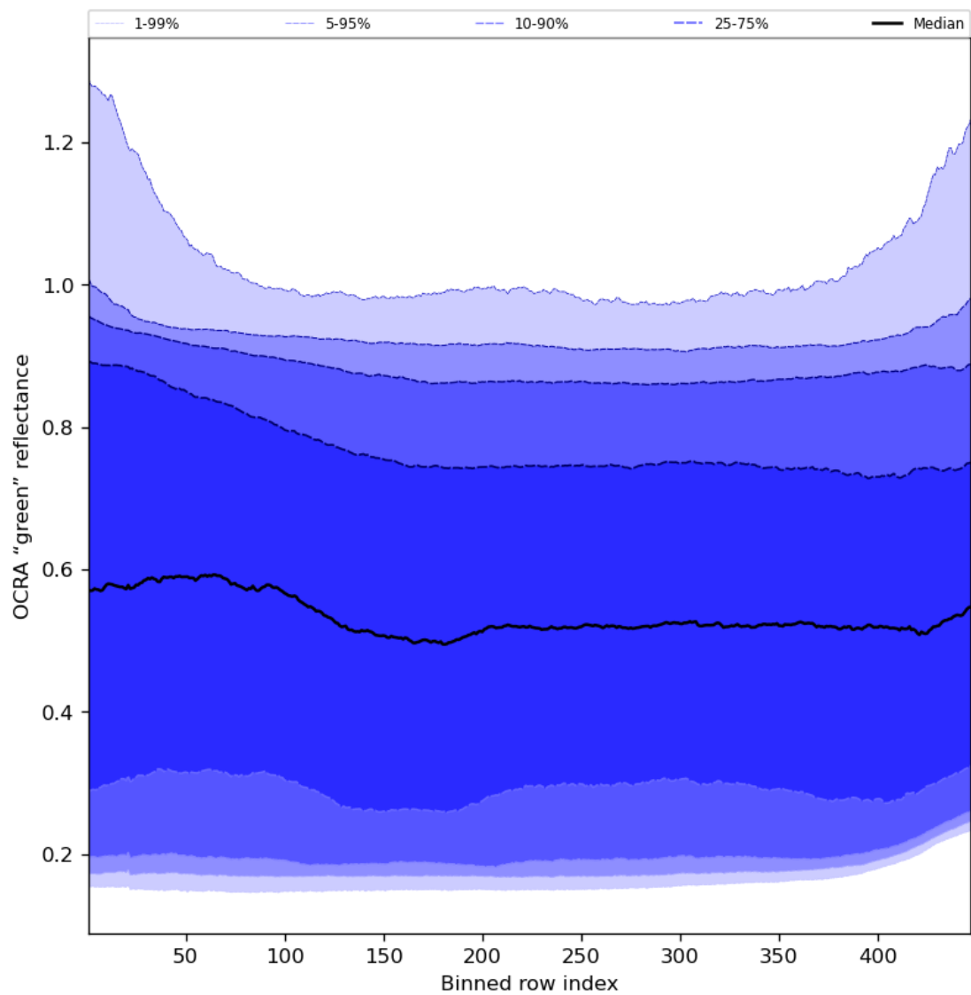
Figure 68: Along track statistics of “OCRA “green” reflectance” for 2024-01-21 to 2024-01-23
