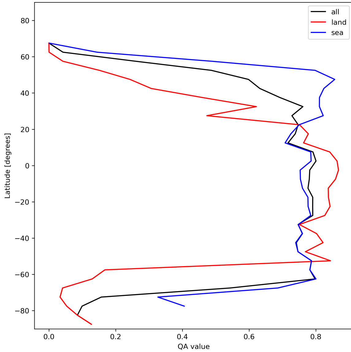
Figure 22: Zonal average of “QA value” for 2024-01-21 to 2024-01-23.
