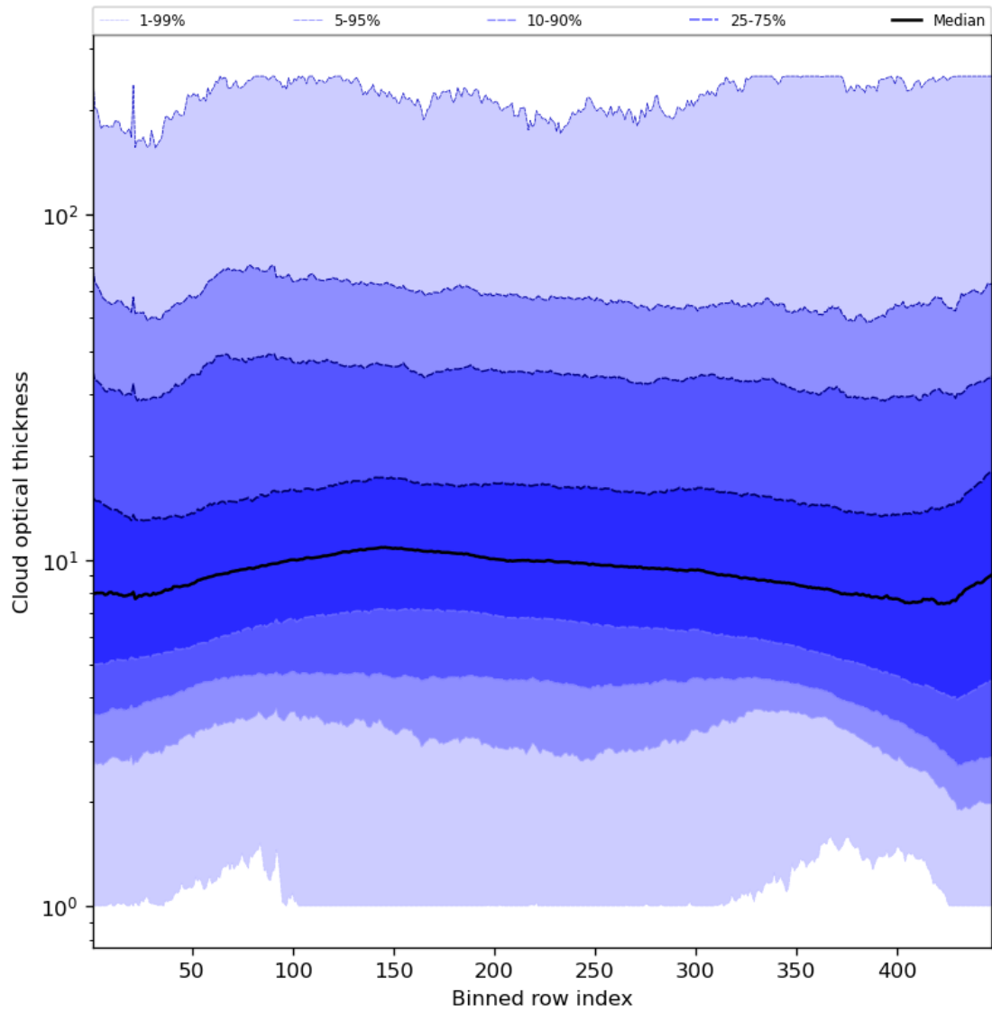
Figure 57: Along track statistics of “Cloud optical thickness” for 2024-01-21 to 2024-01-23
