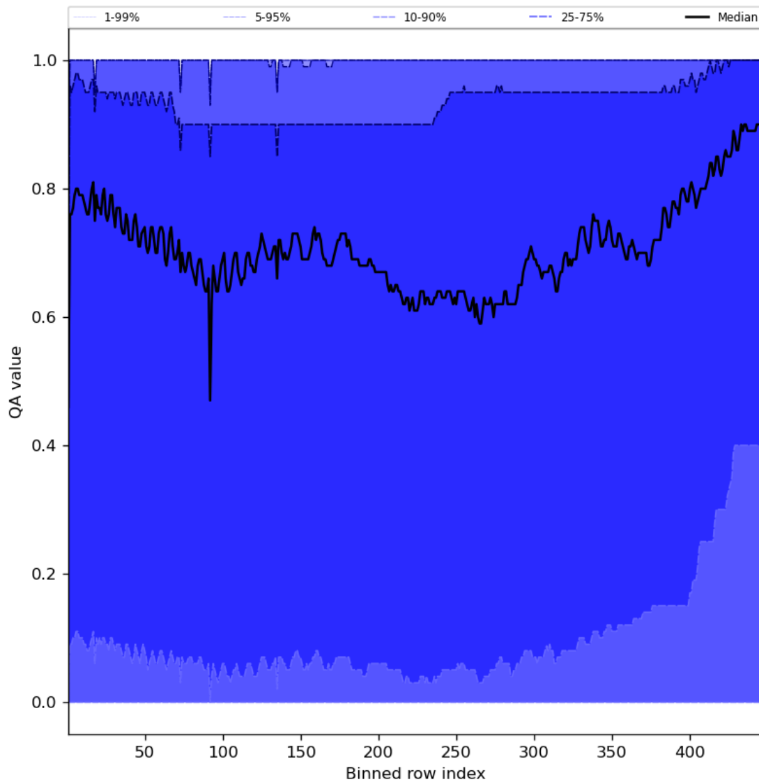
Figure 54: Along track statistics of “QA value” for 2024-01-21 to 2024-01-23
