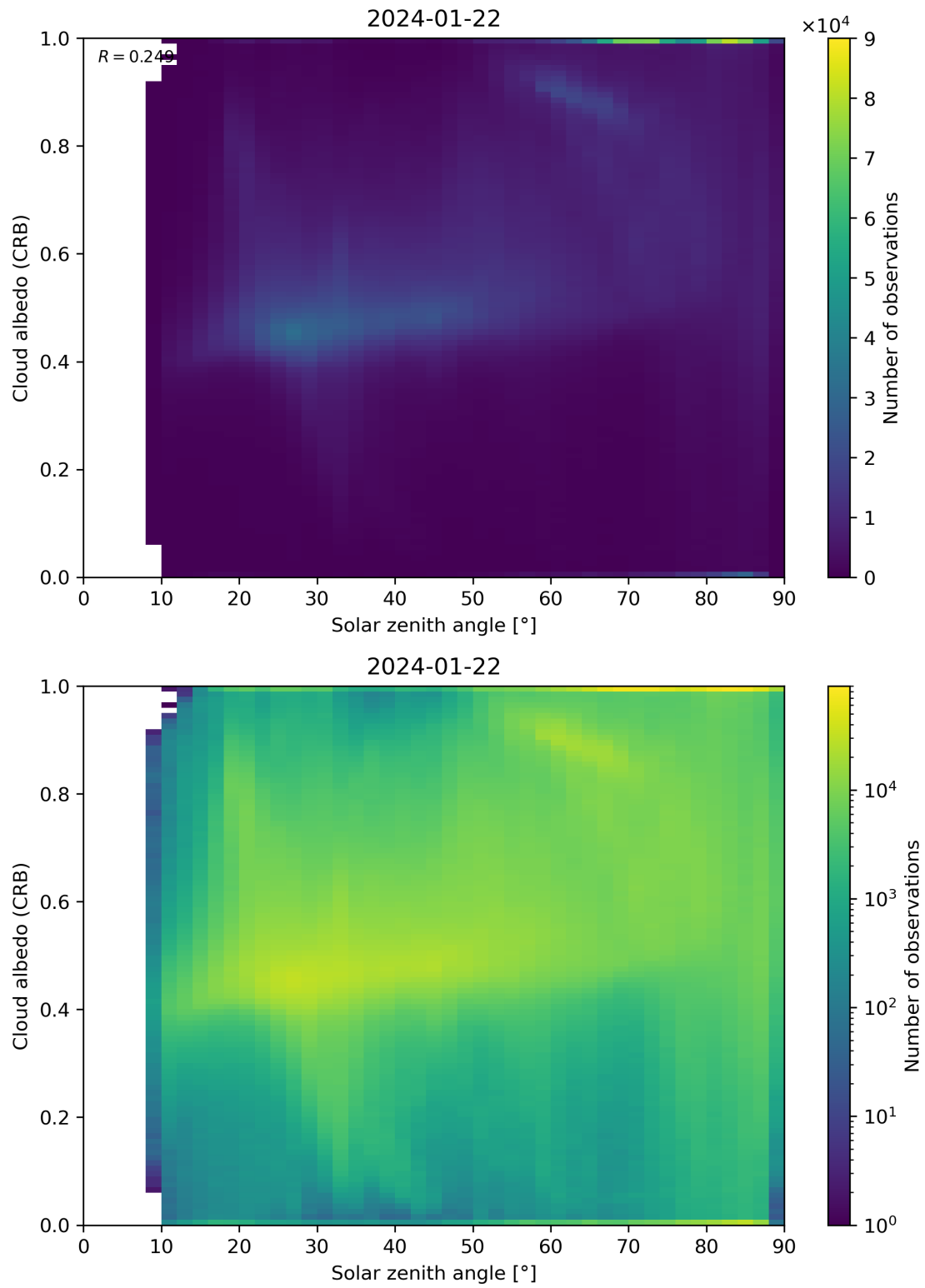
Figure 98: Scatter density plot of “Solar zenith angle” against “Cloud albedo (CRB)” for 2024-01-21 to 2024-01-23.
