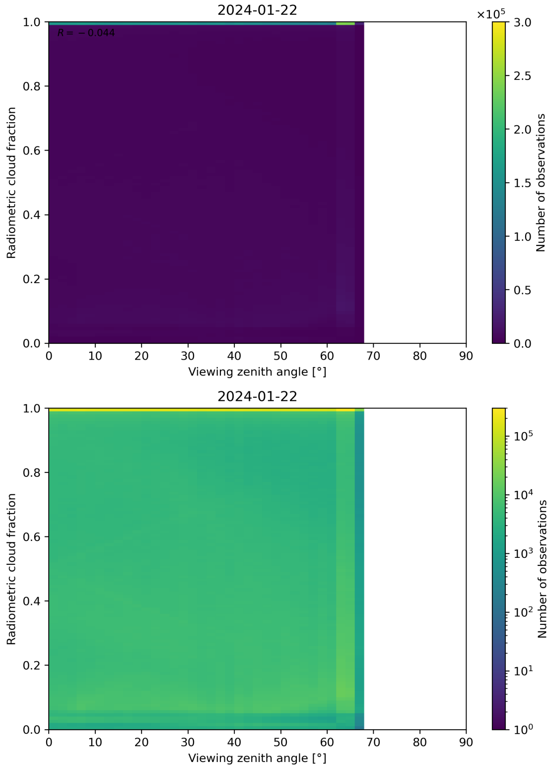
Figure 107: Scatter density plot of “Viewing zenith angle” against “Radiometric cloud fraction” for 2024-01-21 to 2024-01-23.
