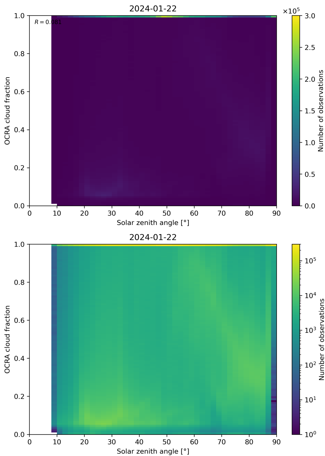
Figure 100: Scatter density plot of “Solar zenith angle” against “OCRA cloud fraction” for 2024-01-21 to 2024-01-23.
