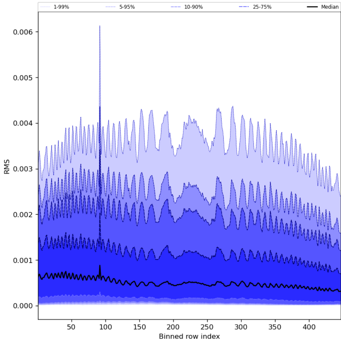
Figure 63: Along track statistics of “RMS” for 2024-01-21 to 2024-01-23
