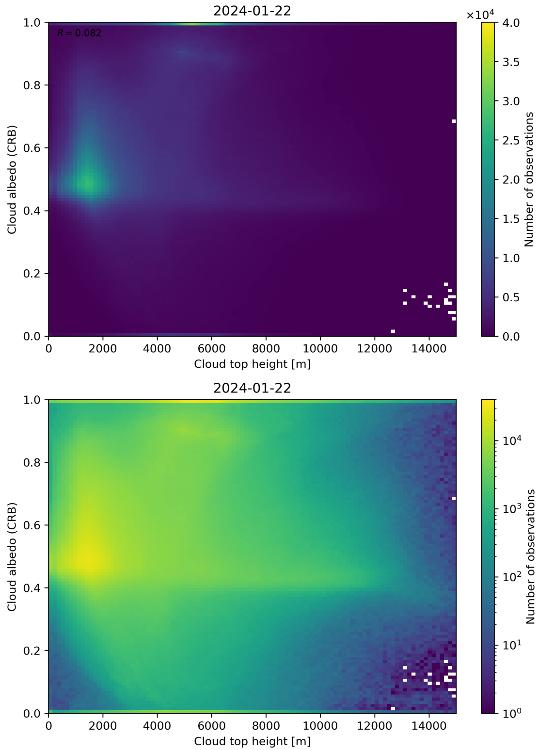
Figure 86: Scatter density plot of “Cloud top height” against “Cloud albedo (CRB)” for 2024-01-21 to 2024-01-23.
