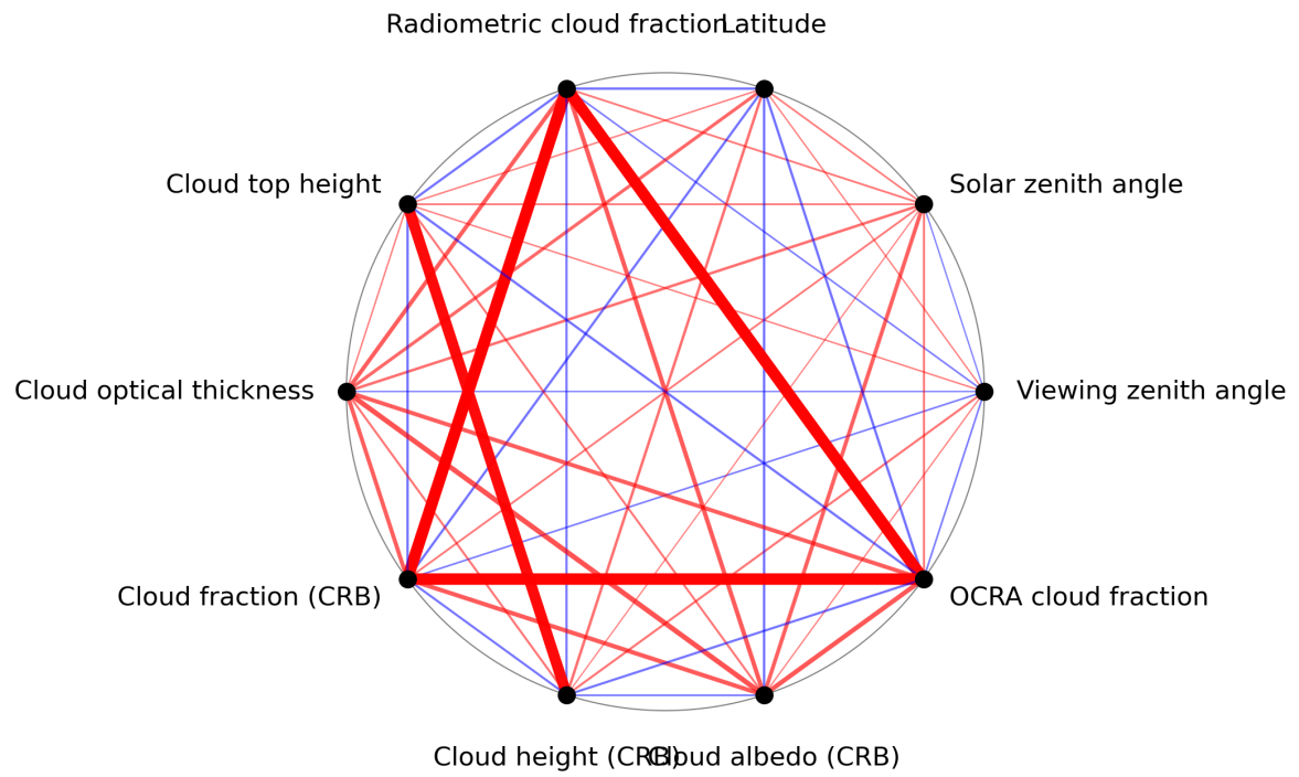
Figure 1: Map of correlation graph for 2024-01-21 to 2024-01-23.
