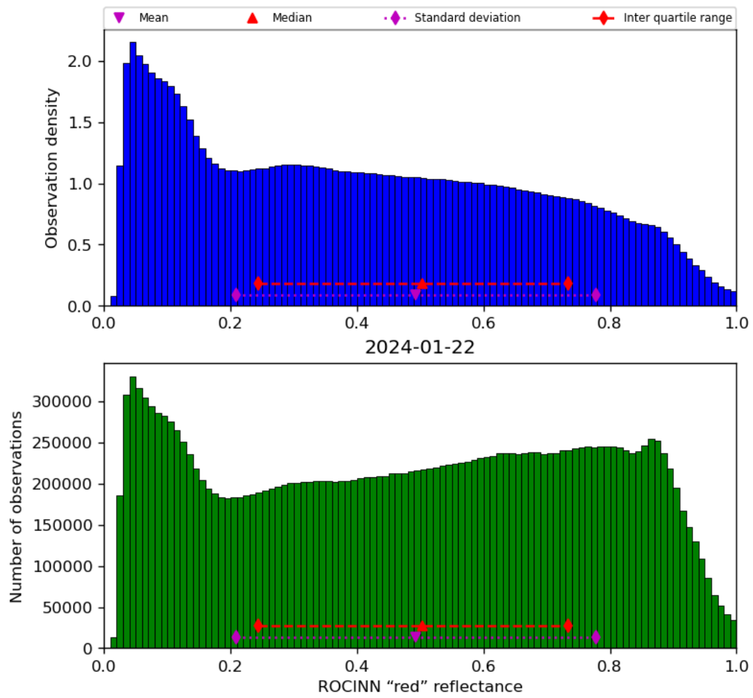
Figure 53: Histogram of “ROCINN “red” reflectance” for 2024-01-21 to 2024-01-23
