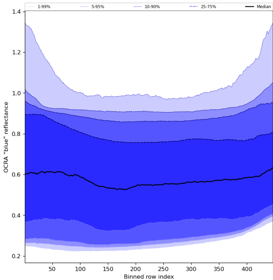
Figure 67: Along track statistics of “OCRA “blue” reflectance” for 2024-01-21 to 2024-01-23
