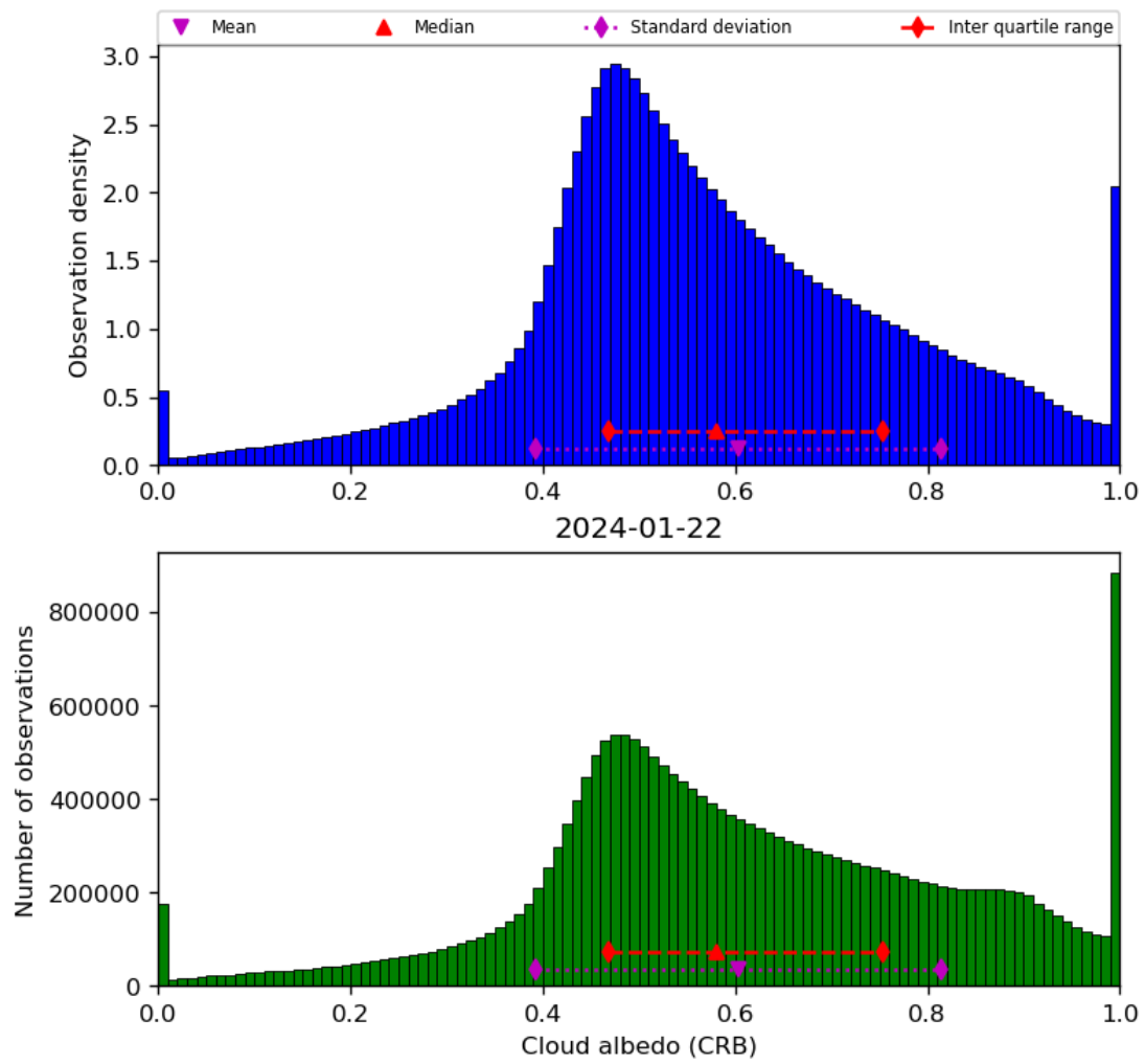
Figure 44: Histogram of “Cloud albedo (CRB)” for 2024-01-21 to 2024-01-23
