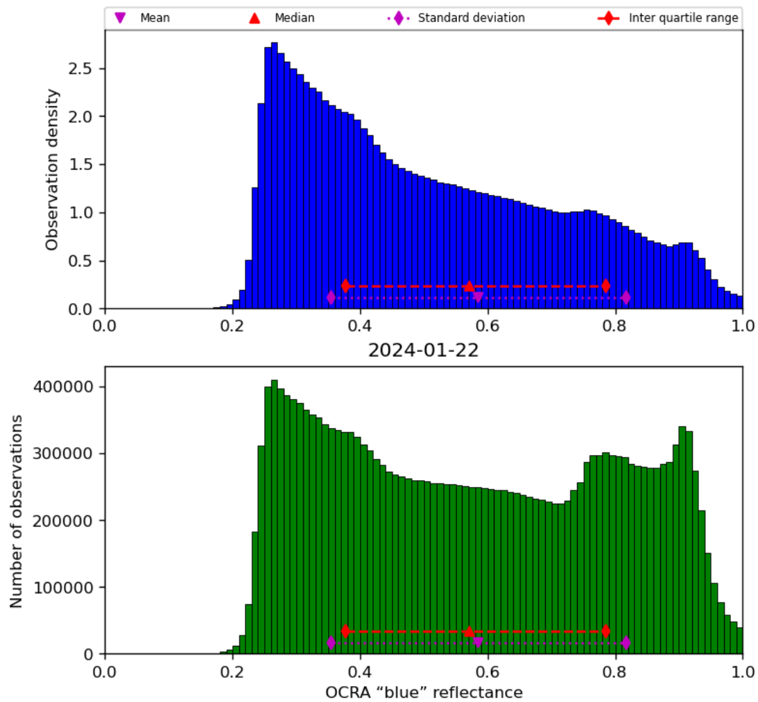
Figure 51: Histogram of “OCRA “blue” reflectance” for 2024-01-21 to 2024-01-23
