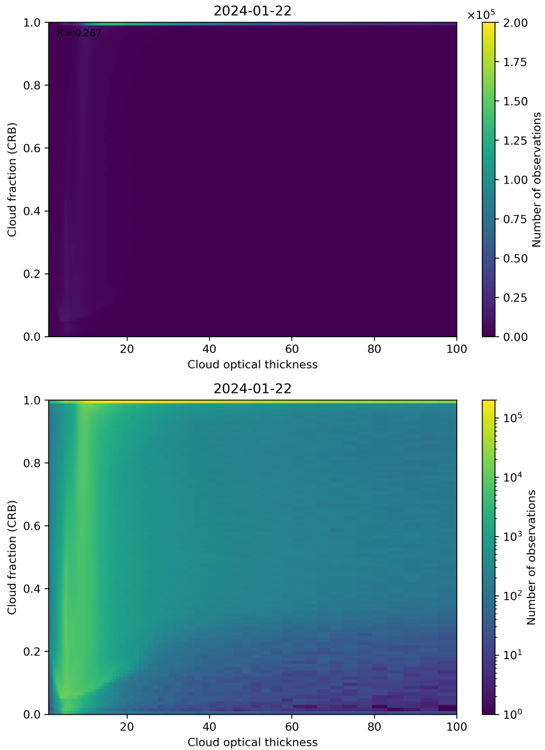
Figure 84: Scatter density plot of “Cloud optical thickness” against “Cloud fraction (CRB)” for 2024-01-21 to 2024-01-23.
