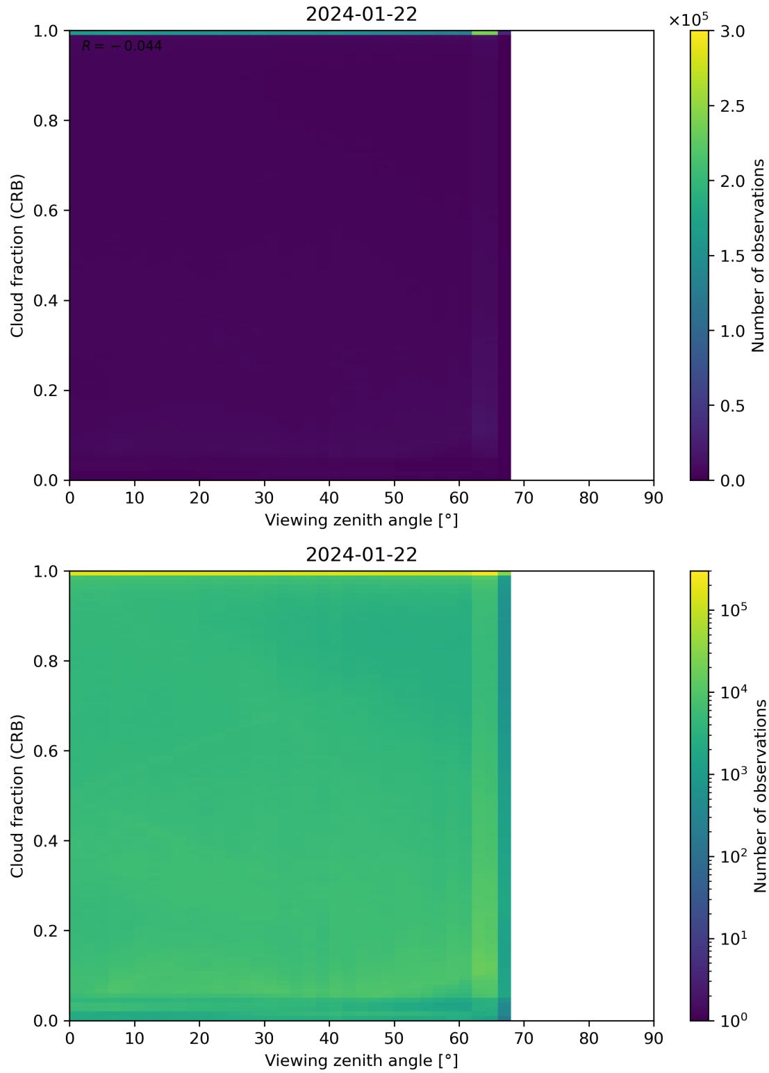
Figure 109: Scatter density plot of “Viewing zenith angle” against “Cloud fraction (CRB)” for 2024-01-21 to 2024-01-23.
