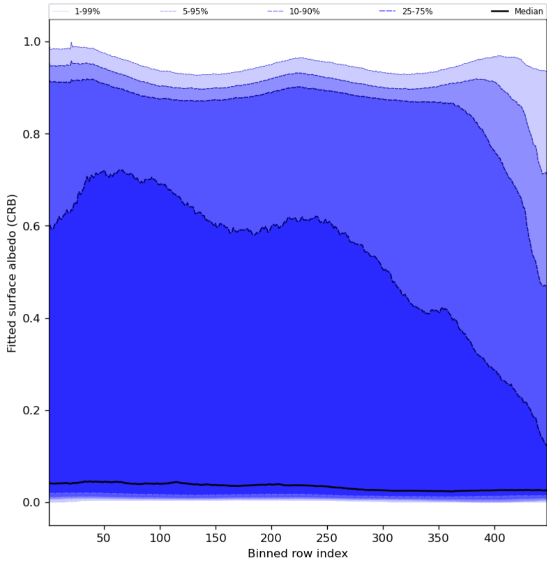
Figure 62: Along track statistics of “Fitted surface albedo (CRB)” for 2024-01-21 to 2024-01-23
