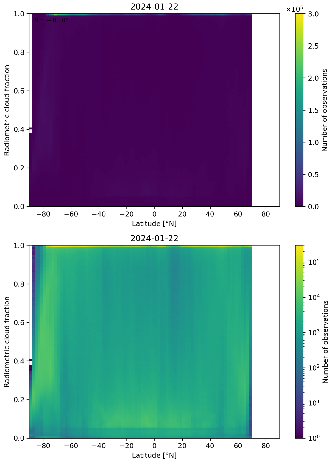
Figure 92: Scatter density plot of “Latitude” against “Radiometric cloud fraction” for 2024-01-21 to 2024-01-23.
