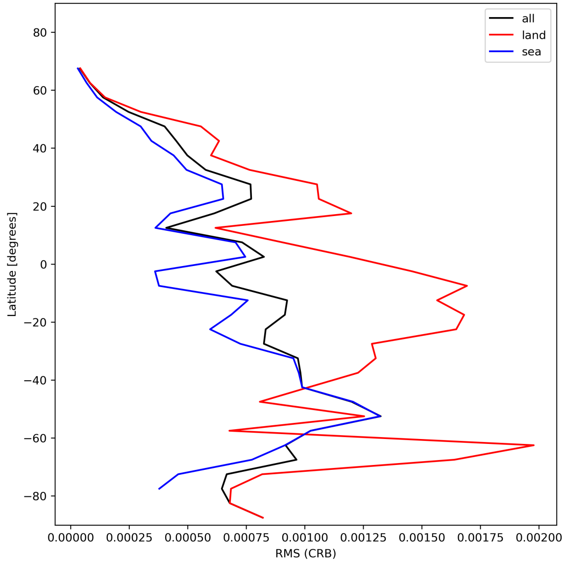
Figure 32: Zonal average of “RMS (CRB)” for 2024-01-21 to 2024-01-23.
