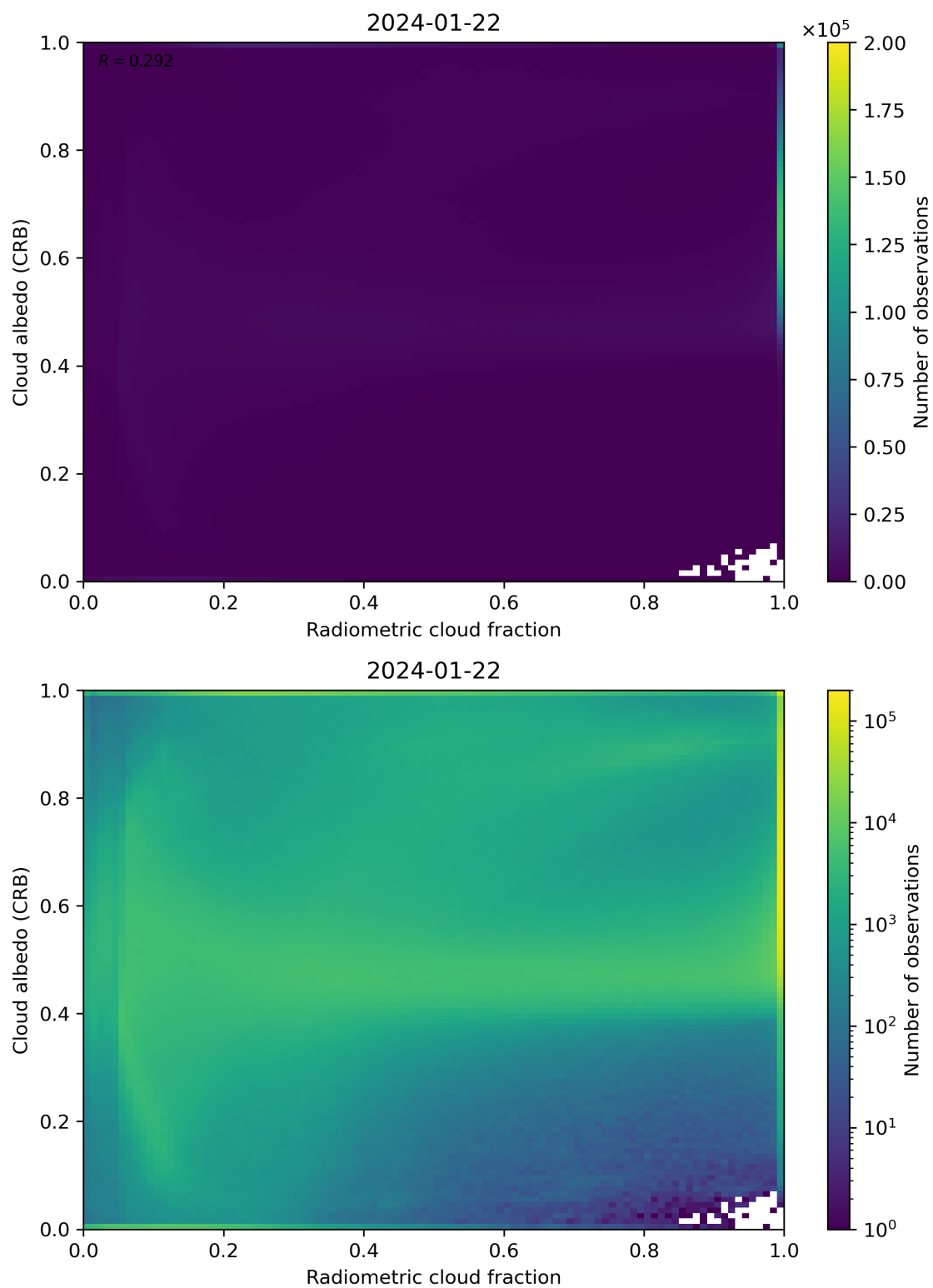
Figure 71: Scatter density plot of “Radiometric cloud fraction” against “Cloud albedo (CRB)” for 2024-01-21 to 2024-01-23.
