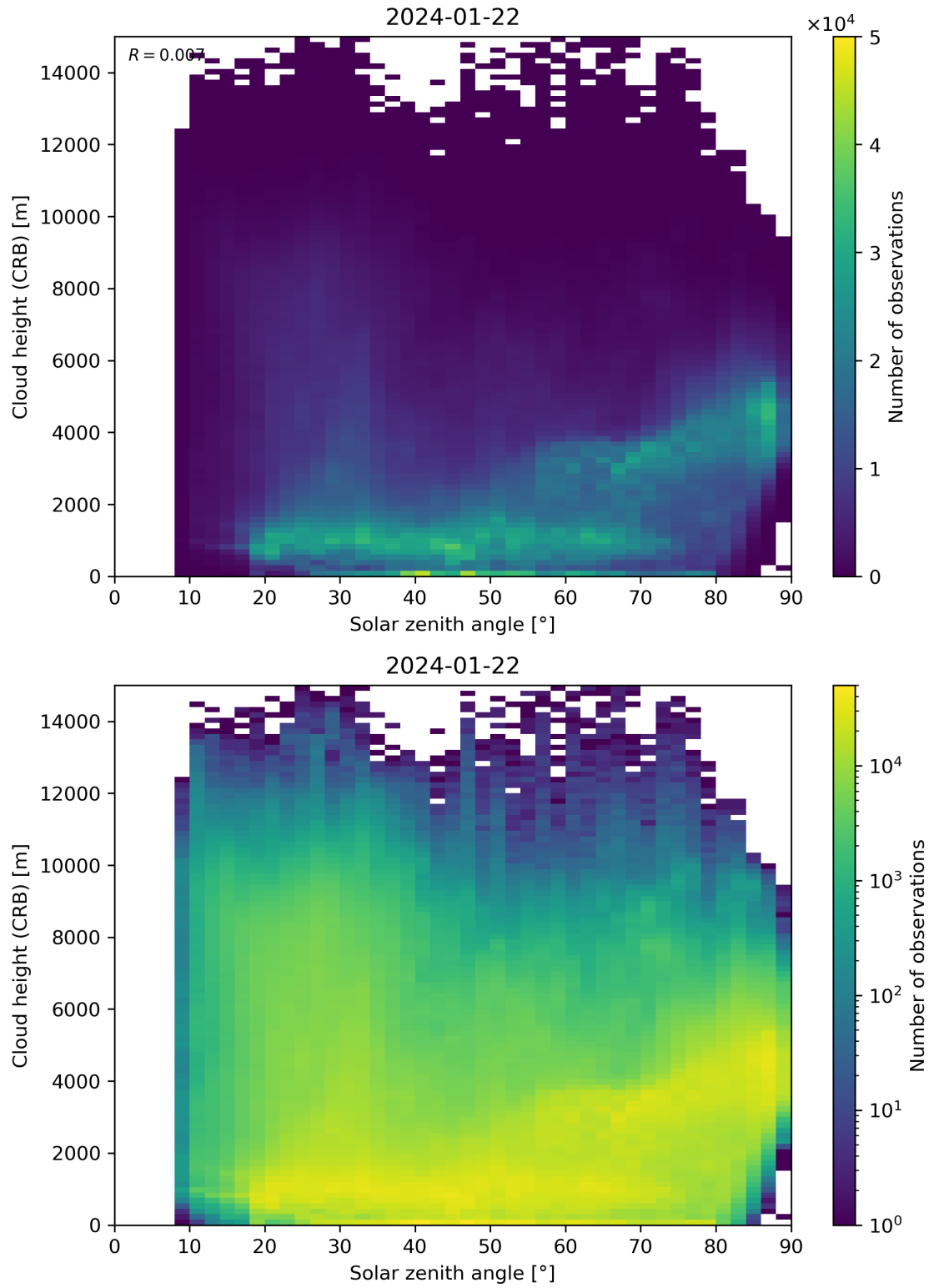
Figure 102: Scatter density plot of “Solar zenith angle” against “Cloud height (CRB)” for 2024-01-21 to 2024-01-23.
