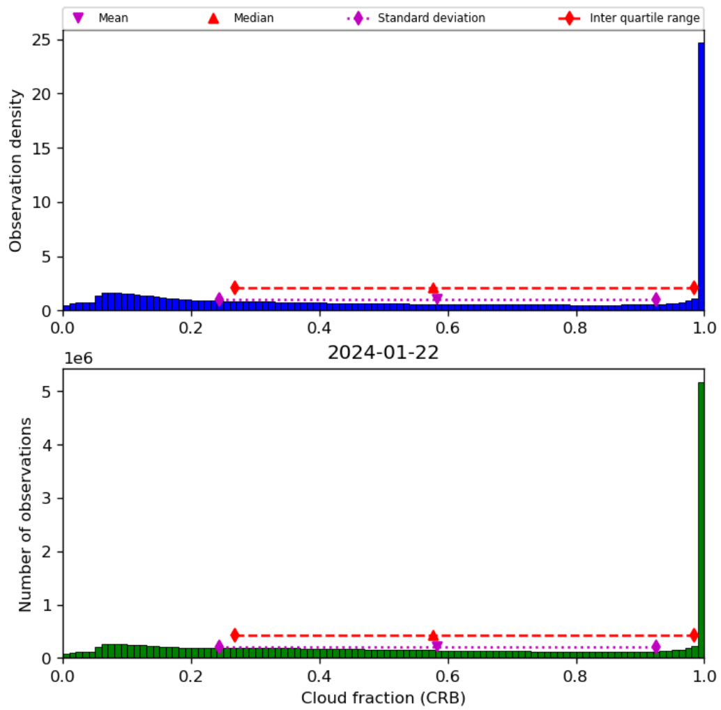
Figure 42: Histogram of “Cloud fraction (CRB)” for 2024-01-21 to 2024-01-23
