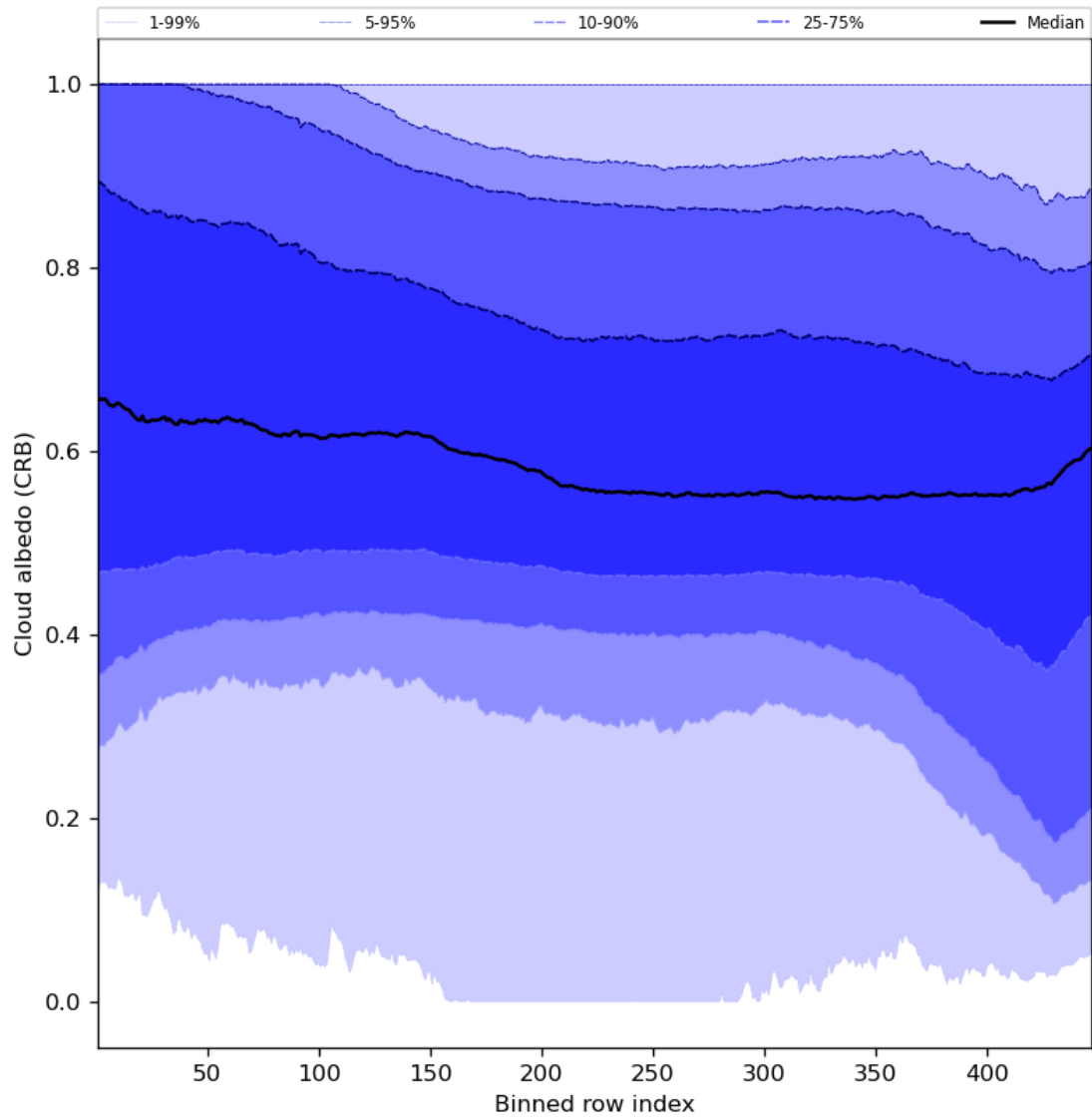
Figure 60: Along track statistics of “Cloud albedo (CRB)” for 2024-01-21 to 2024-01-23
