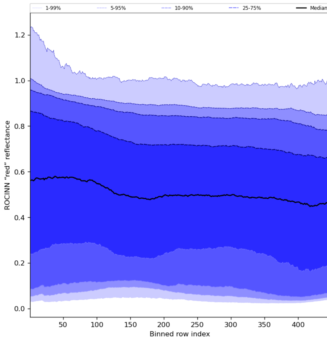
Figure 69: Along track statistics of “ROCINN “red” reflectance” for 2024-01-21 to 2024-01-23
