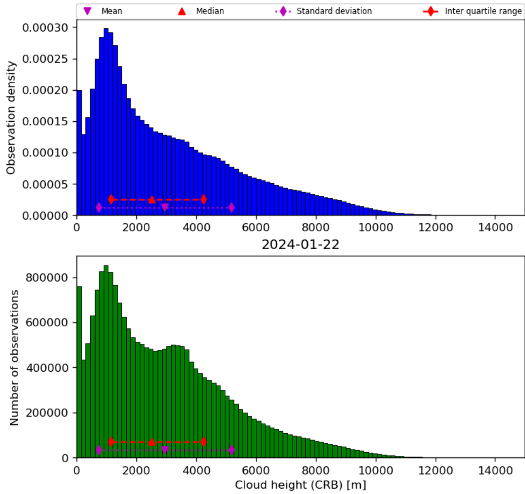
Figure 43: Histogram of “Cloud height (CRB)” for 2024-01-21 to 2024-01-23
