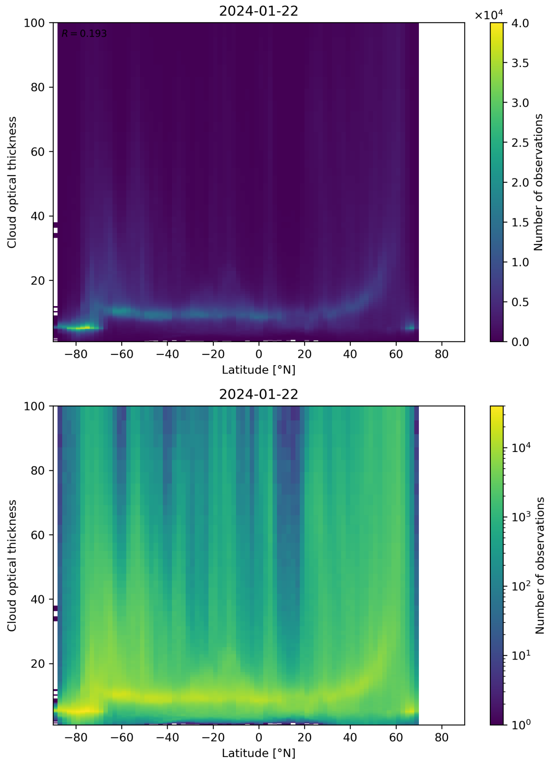
Figure 96: Scatter density plot of “Latitude” against “Cloud optical thickness” for 2024-01-21 to 2024-01-23.
