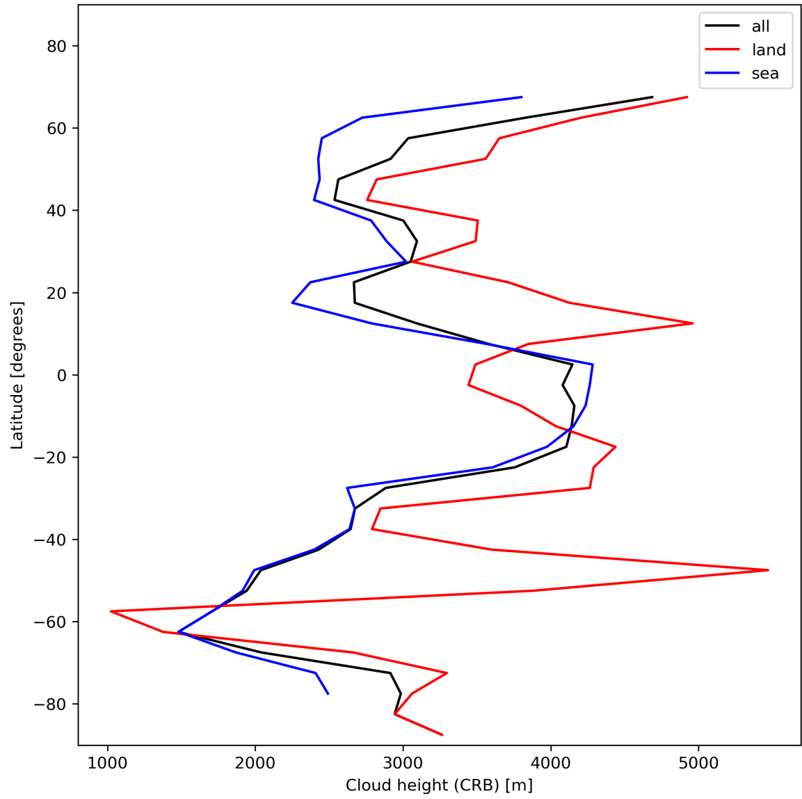
Figure 27: Zonal average of “Cloud height (CRB)” for 2024-01-21 to 2024-01-23.
