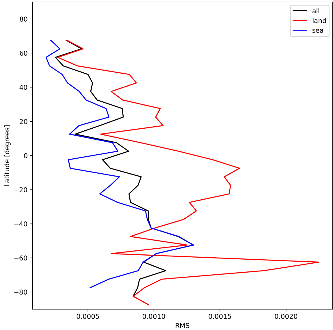
Figure 31: Zonal average of “RMS” for 2024-01-21 to 2024-01-23.
