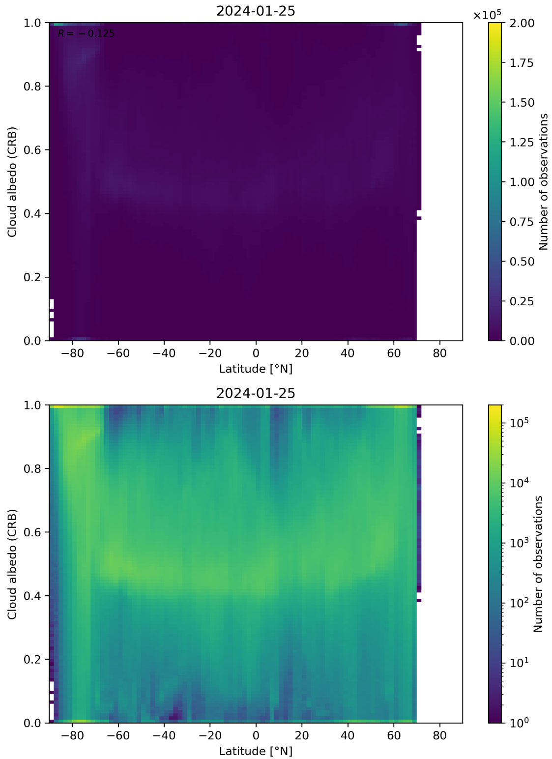
Figure 91: Scatter density plot of “Latitude” against “Cloud albedo (CRB)” for 2024-01-24 to 2024-01-26.
