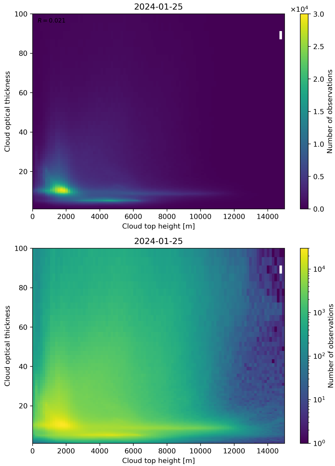
Figure 90: Scatter density plot of “Cloud top height” against “Cloud optical thickness” for 2024-01-24 to 2024-01-26.
