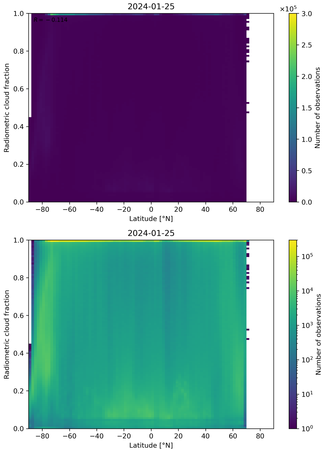
Figure 92: Scatter density plot of “Latitude” against “Radiometric cloud fraction” for 2024-01-24 to 2024-01-26.
