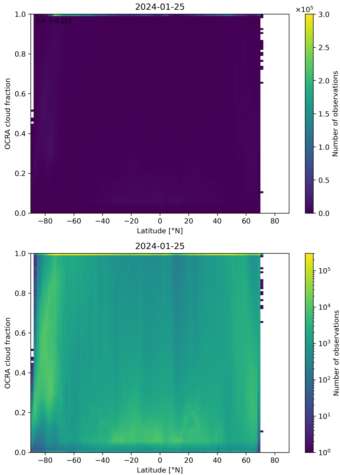
Figure 93: Scatter density plot of “Latitude” against “OCRA cloud fraction” for 2024-01-24 to 2024-01-26.
