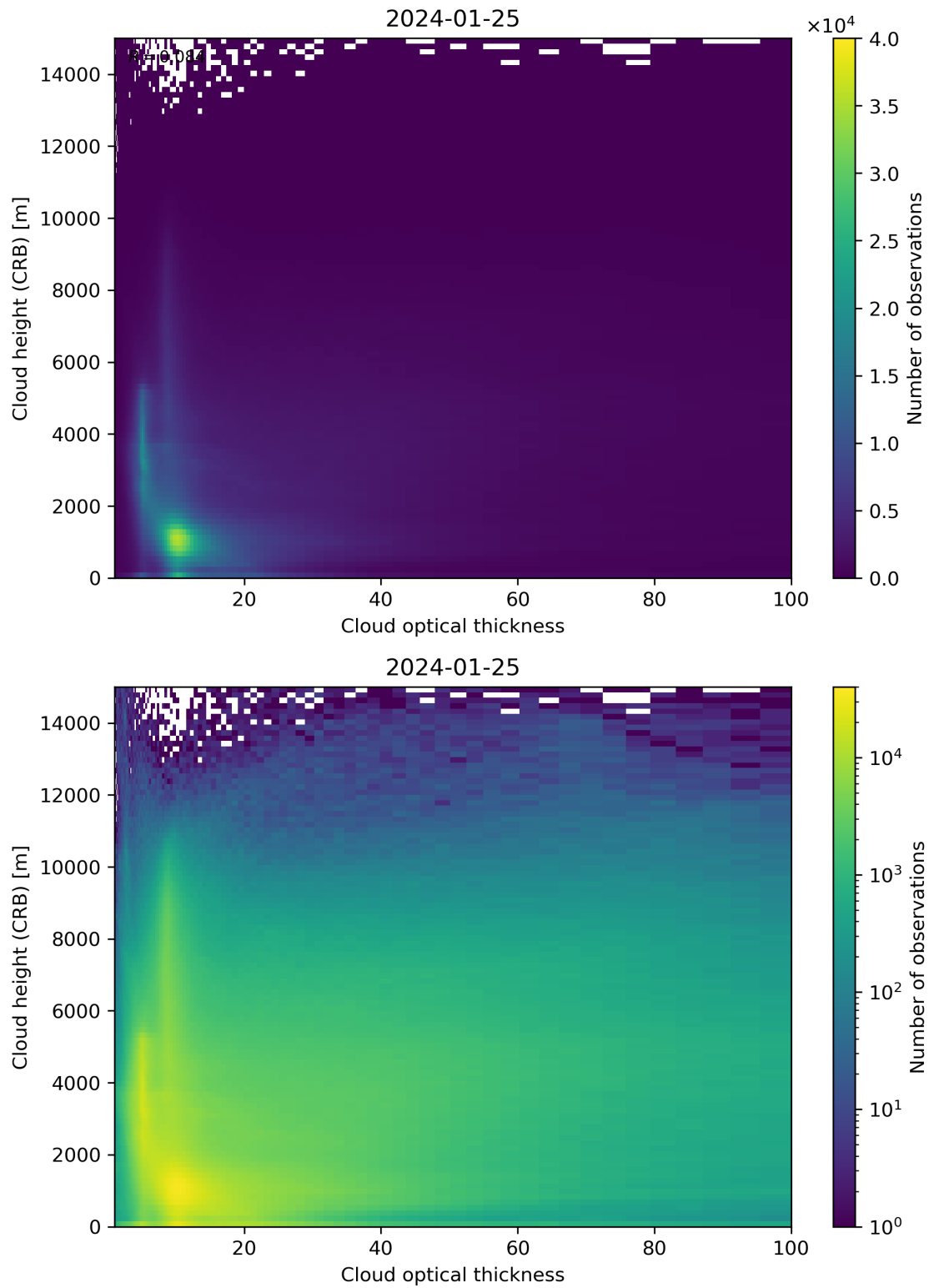
Figure 85: Scatter density plot of “Cloud optical thickness” against “Cloud height (CRB)” for 2024-01-24 to 2024-01-26.
