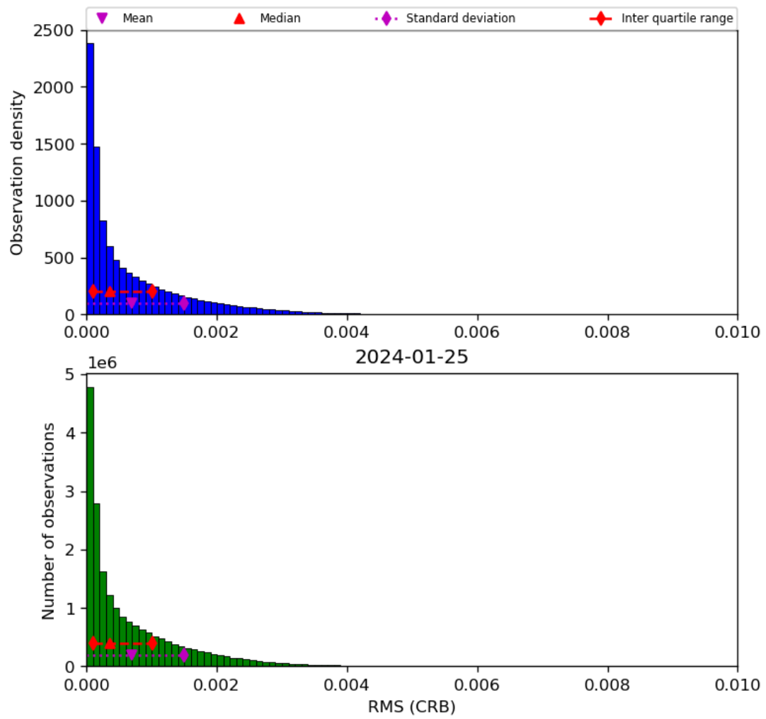
Figure 48: Histogram of “RMS (CRB)” for 2024-01-24 to 2024-01-26
