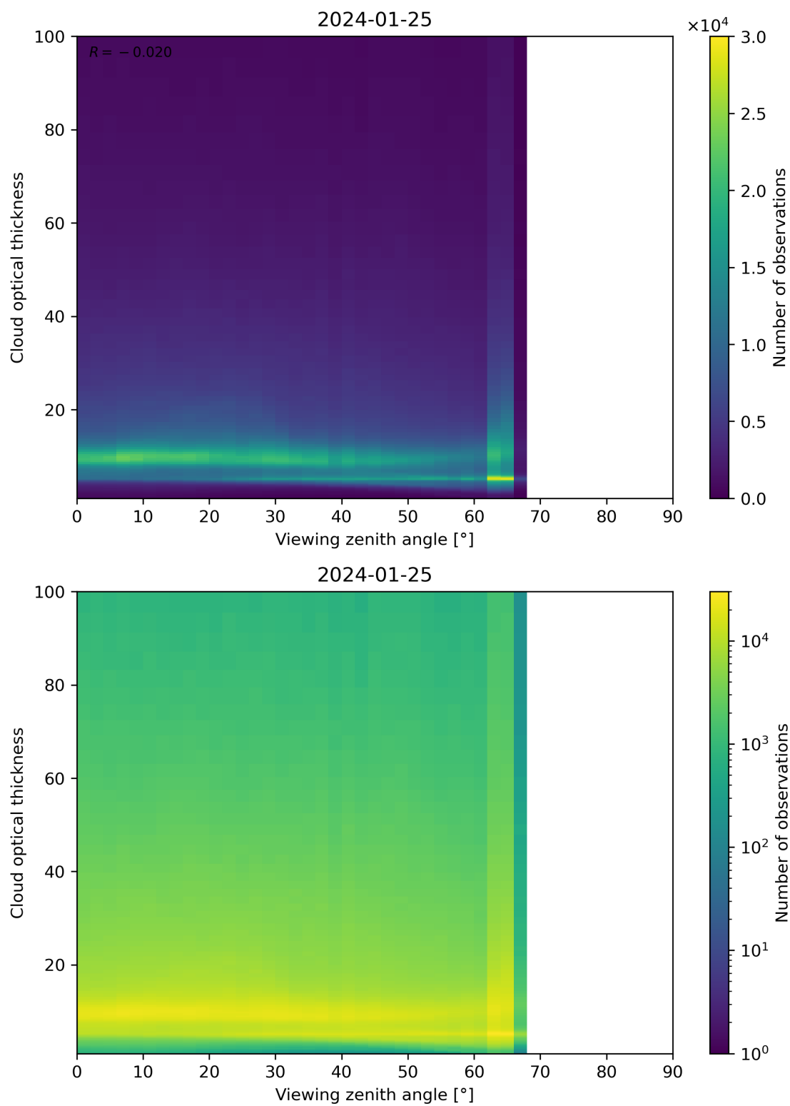
Figure 111: Scatter density plot of “Viewing zenith angle” against “Cloud optical thickness” for 2024-01-24 to 2024-01-26.
