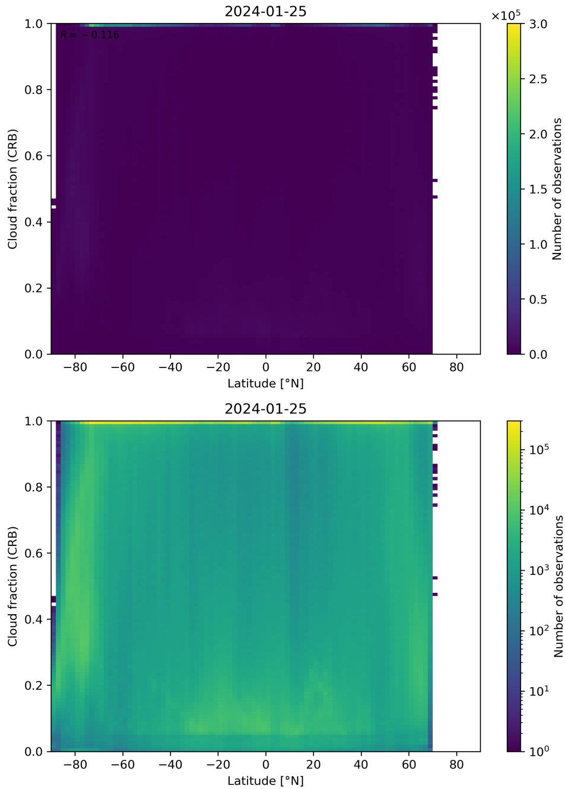
Figure 94: Scatter density plot of “Latitude” against “Cloud fraction (CRB)” for 2024-01-24 to 2024-01-26.
