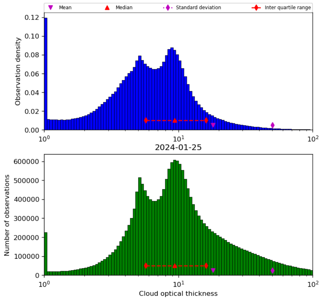
Figure 41: Histogram of “Cloud optical thickness” for 2024-01-24 to 2024-01-26
