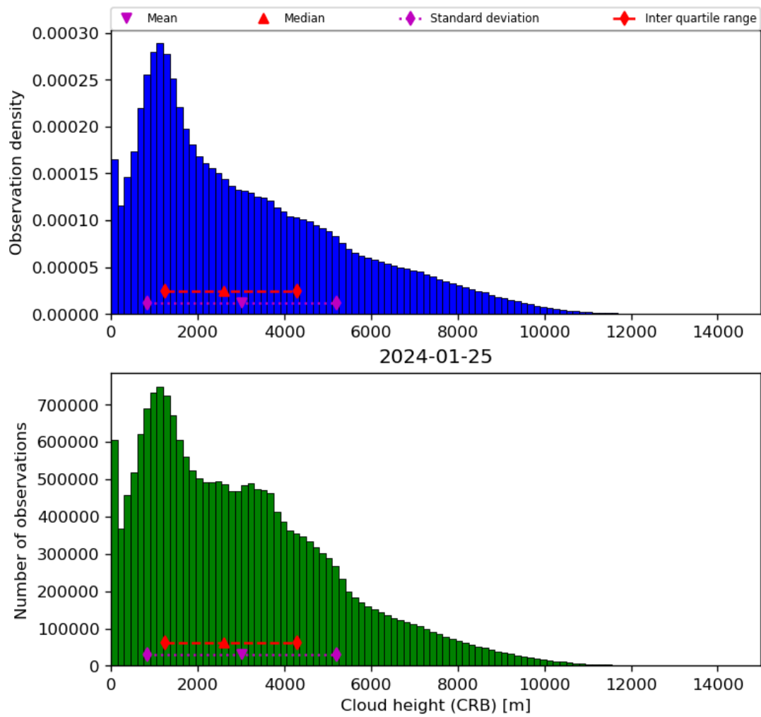
Figure 43: Histogram of “Cloud height (CRB)” for 2024-01-24 to 2024-01-26
