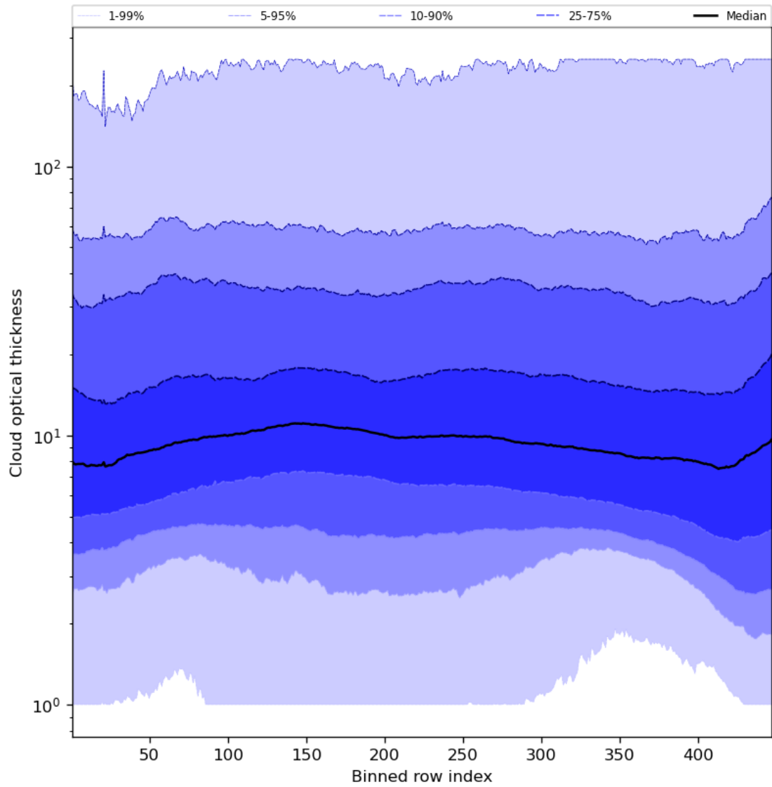
Figure 57: Along track statistics of “Cloud optical thickness” for 2024-01-24 to 2024-01-26
