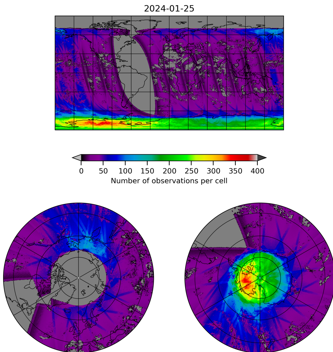
Figure 21: Map of the number of observations for 2024-01-24 to 2024-01-26
