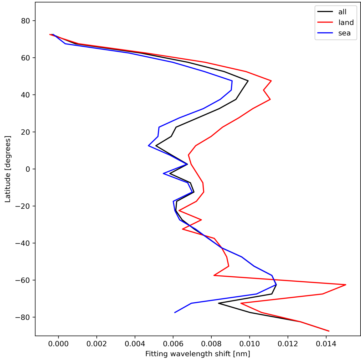
Figure 33: Zonal average of “Fitting wavelength shift” for 2024-01-24 to 2024-01-26.
