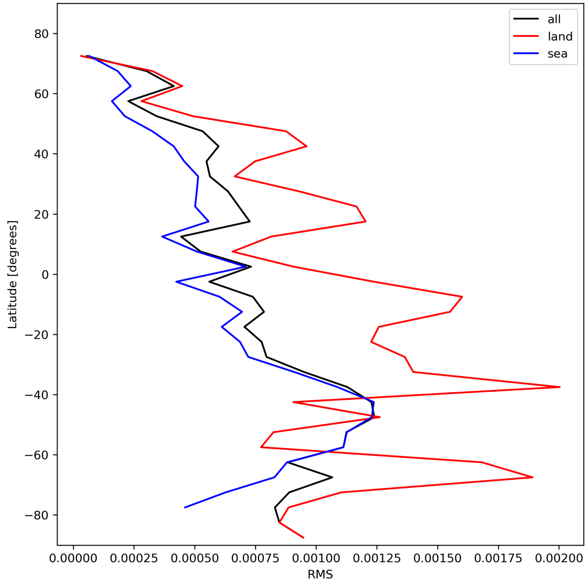
Figure 31: Zonal average of “RMS” for 2024-01-24 to 2024-01-26.
