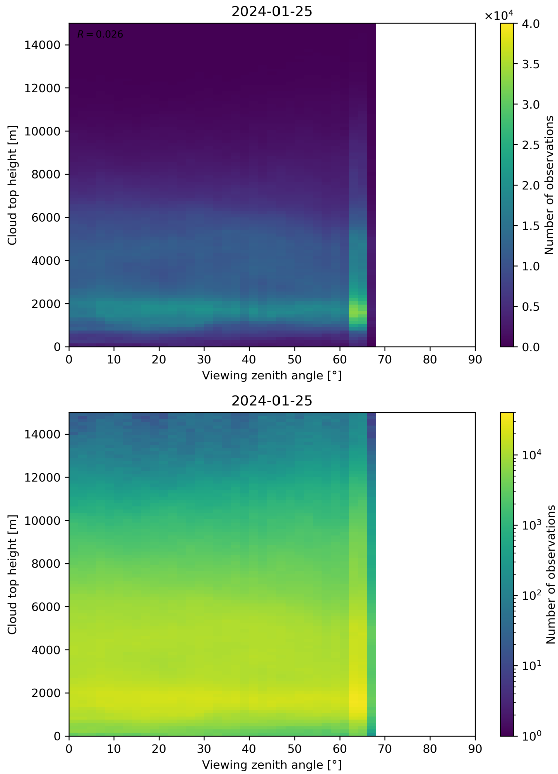
Figure 112: Scatter density plot of “Viewing zenith angle” against “Cloud top height” for 2024-01-24 to 2024-01-26.
