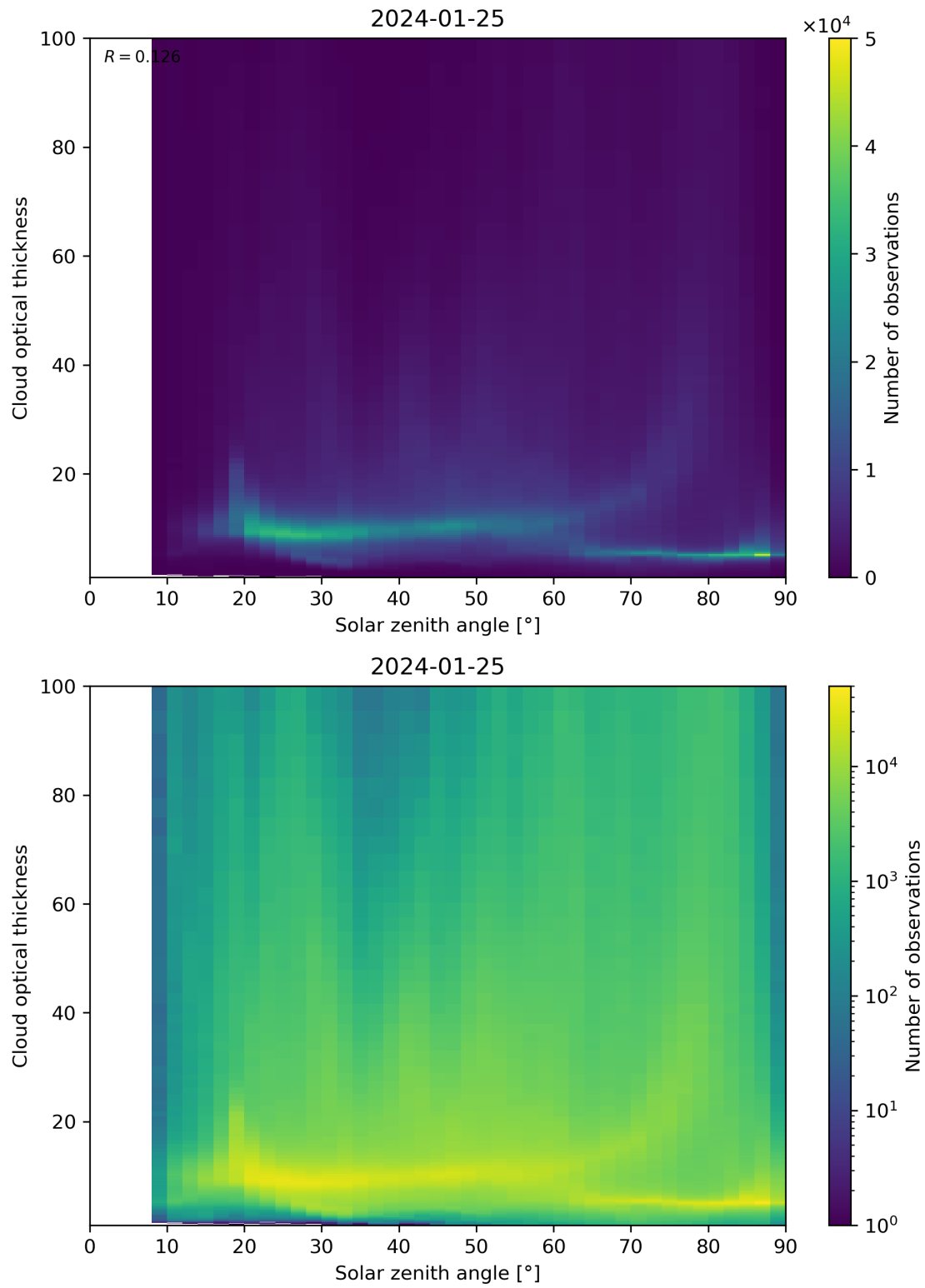
Figure 103: Scatter density plot of “Solar zenith angle” against “Cloud optical thickness” for 2024-01-24 to 2024-01-26.
