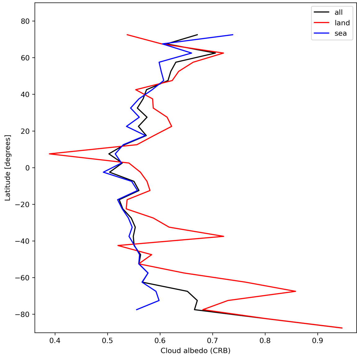
Figure 28: Zonal average of “Cloud albedo (CRB)” for 2024-01-24 to 2024-01-26.
