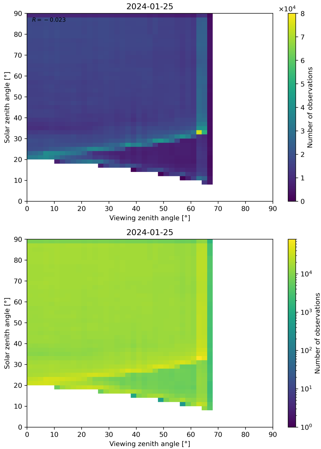
Figure 114: Scatter density plot of “Viewing zenith angle” against “Solar zenith angle” for 2024-01-24 to 2024-01-26.
