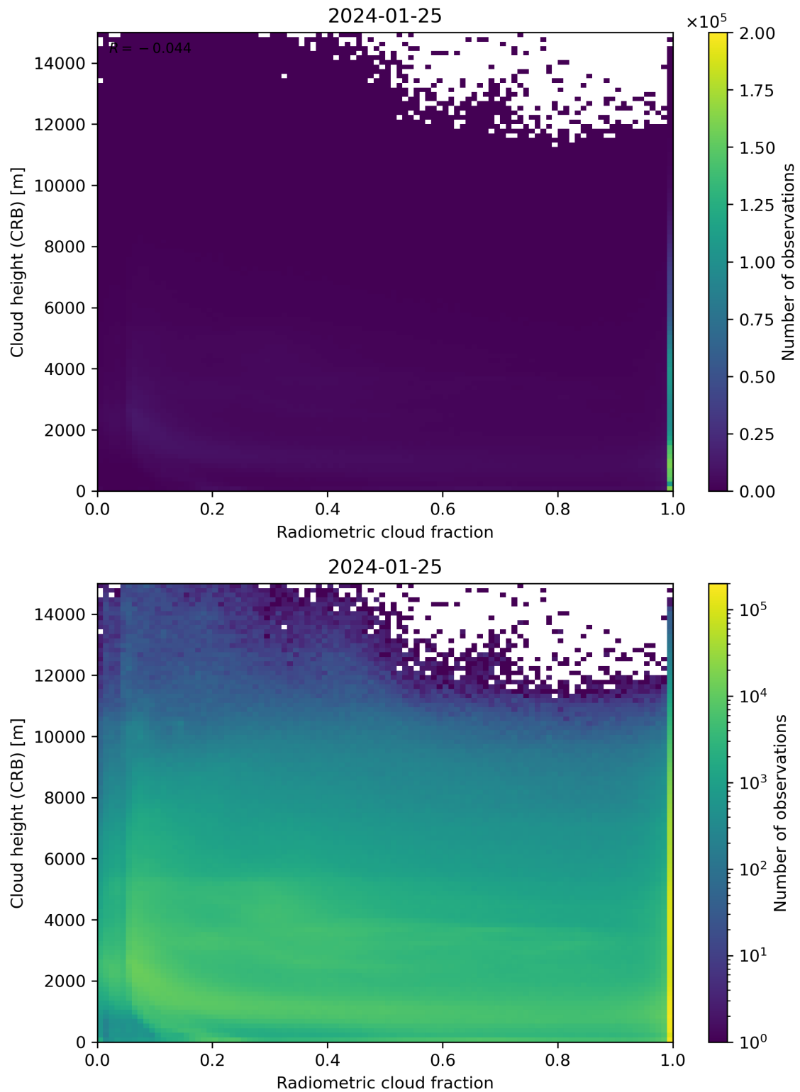
Figure 74: Scatter density plot of “Radiometric cloud fraction” against “Cloud height (CRB)” for 2024-01-24 to 2024-01-26.
