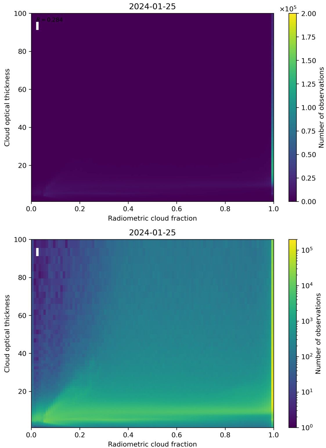
Figure 75: Scatter density plot of “Radiometric cloud fraction” against “Cloud optical thickness” for 2024-01-24 to 2024-01-26.
