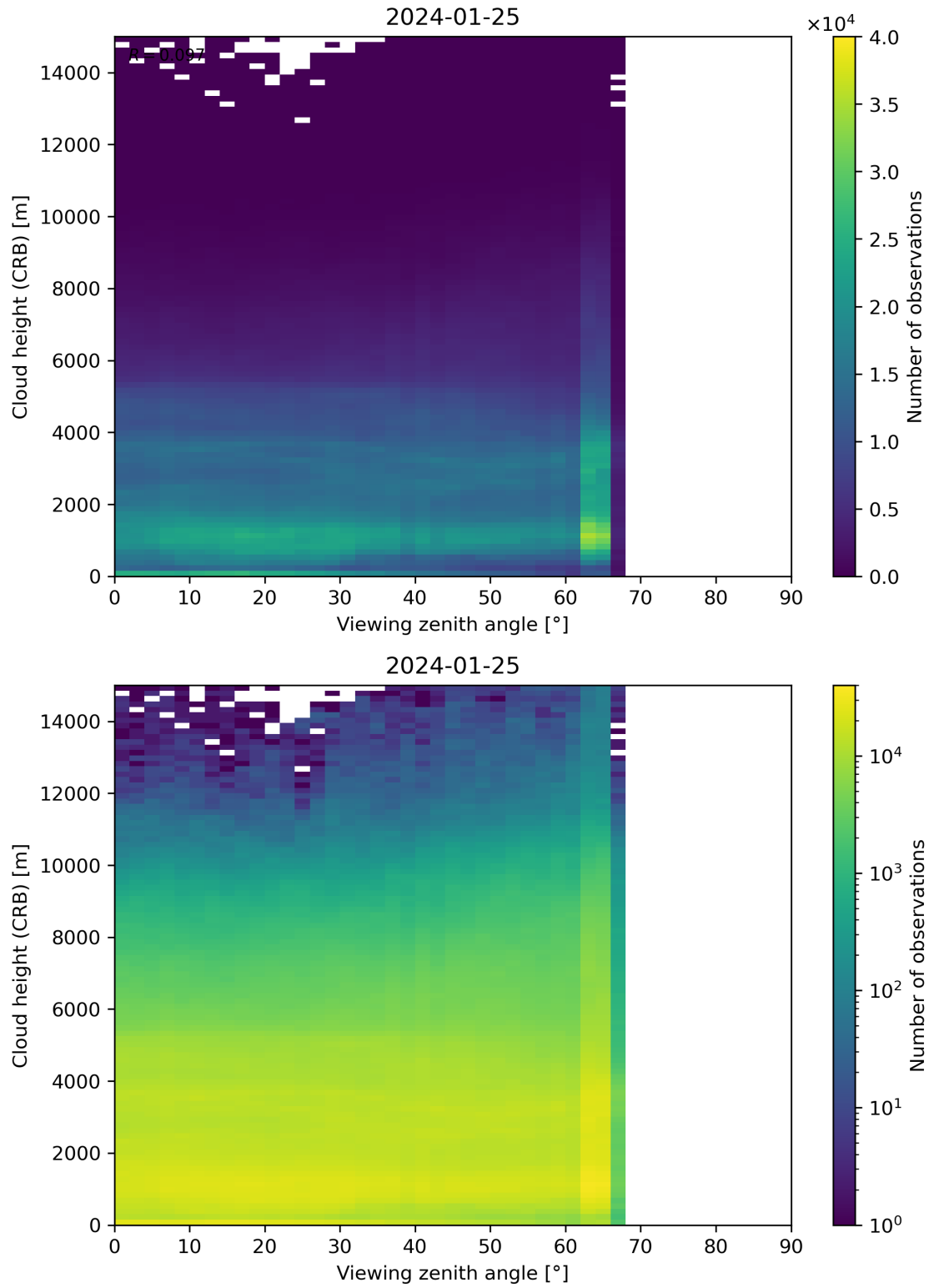
Figure 110: Scatter density plot of “Viewing zenith angle” against “Cloud height (CRB)” for 2024-01-24 to 2024-01-26.
