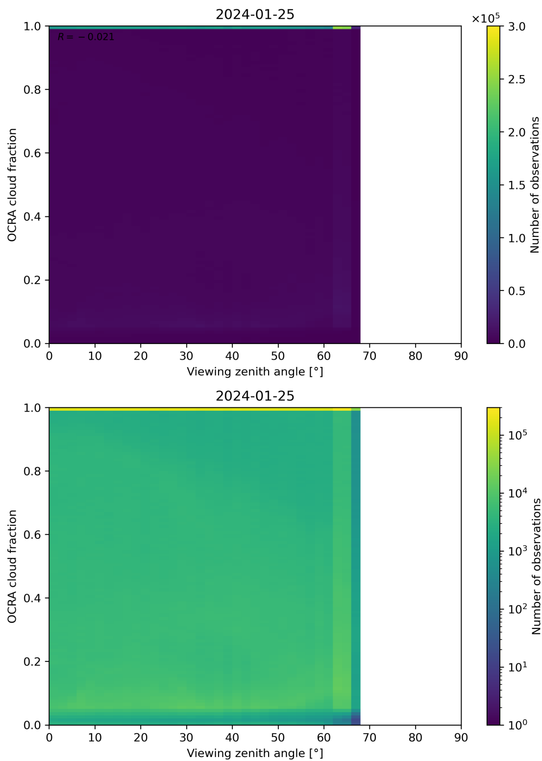
Figure 108: Scatter density plot of “Viewing zenith angle” against “OCRA cloud fraction” for 2024-01-24 to 2024-01-26.
