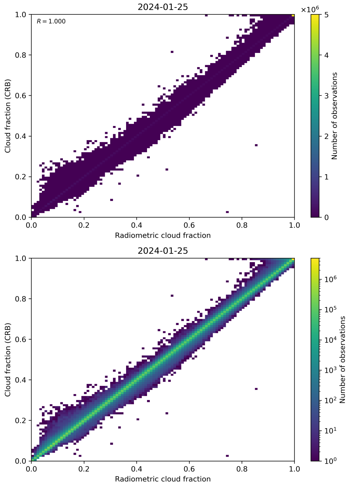
Figure 73: Scatter density plot of “Radiometric cloud fraction” against “Cloud fraction (CRB)” for 2024-01-24 to 2024-01-26.
