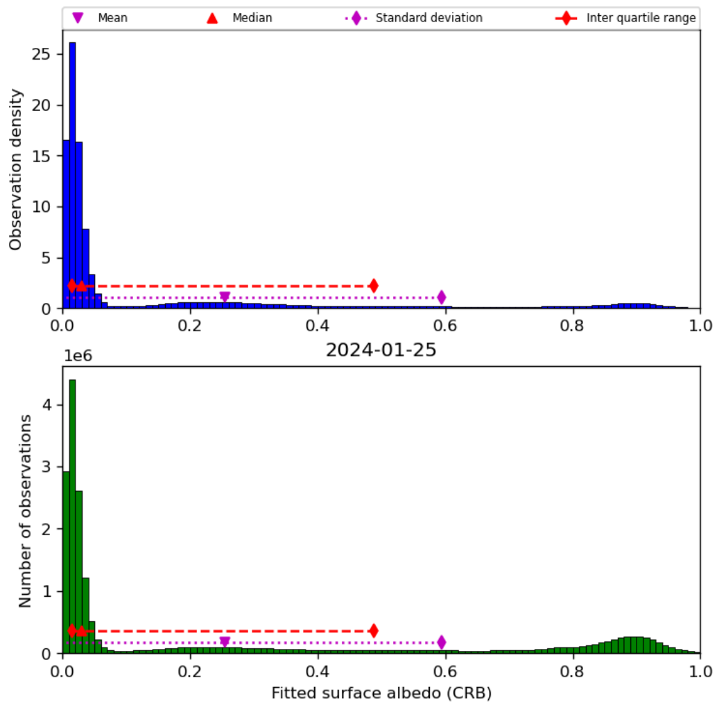
Figure 46: Histogram of “Fitted surface albedo (CRB)” for 2024-01-24 to 2024-01-26
