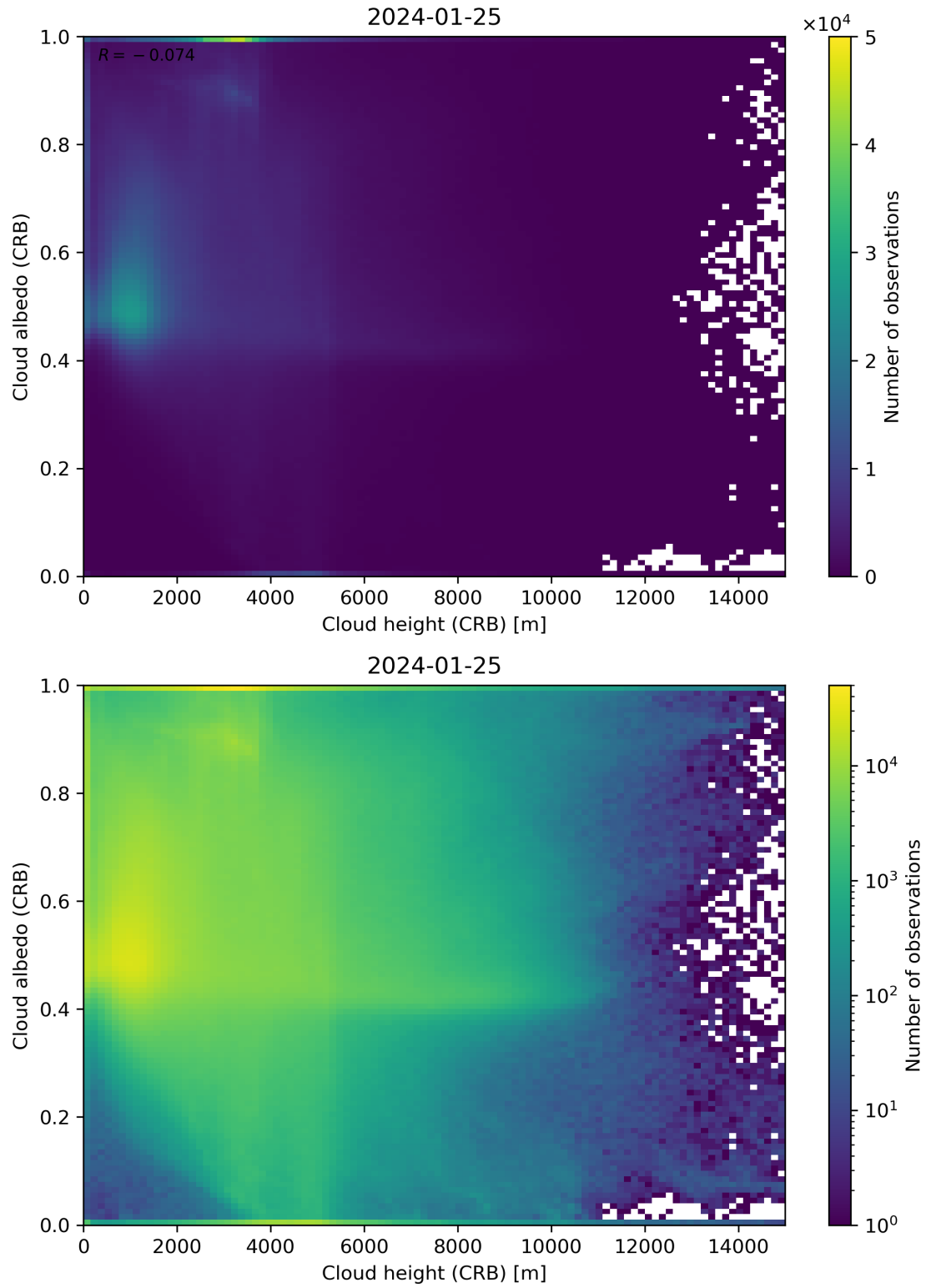
Figure 80: Scatter density plot of “Cloud height (CRB)” against “Cloud albedo (CRB)” for 2024-01-24 to 2024-01-26.
