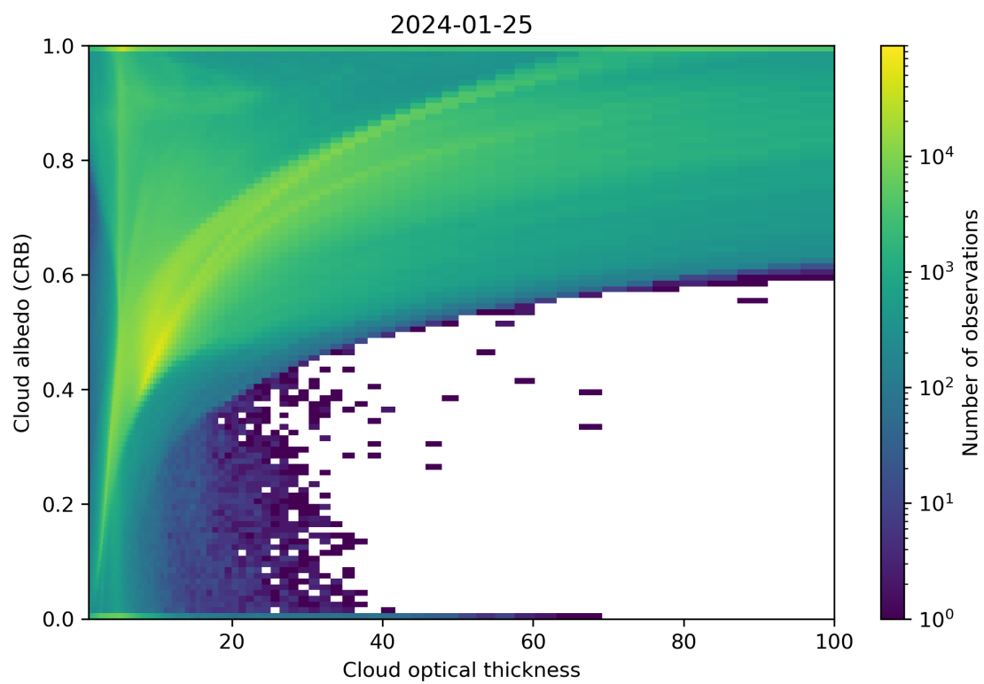
Figure 82: Scatter density plot of “Cloud optical thickness” against “Cloud albedo (CRB)” for 2024-01-24 to 2024-01-26.
