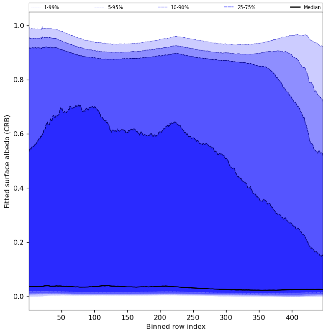
Figure 62: Along track statistics of “Fitted surface albedo (CRB)” for 2024-01-24 to 2024-01-26
