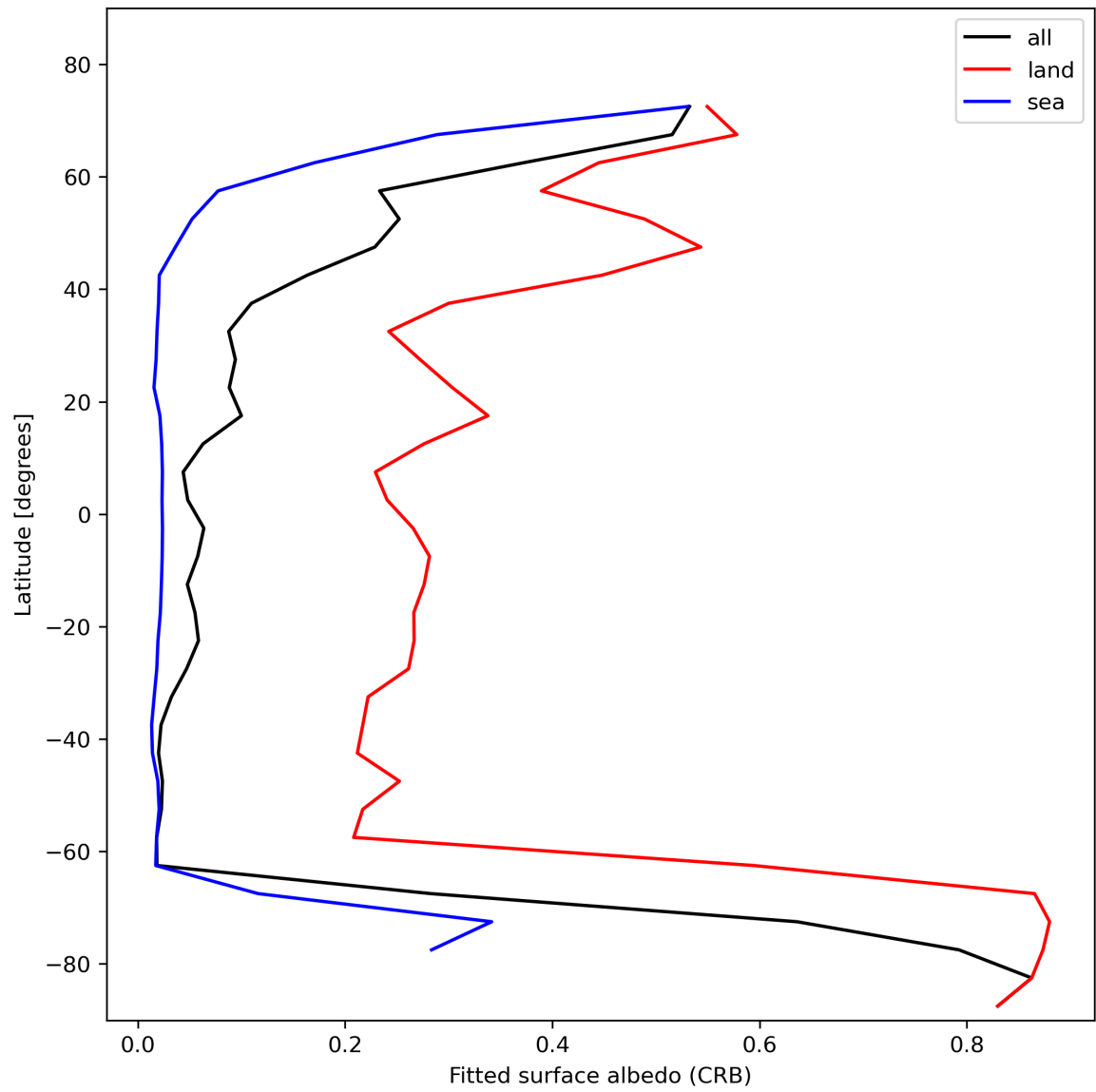
Figure 30: Zonal average of “Fitted surface albedo (CRB)” for 2024-01-24 to 2024-01-26.
