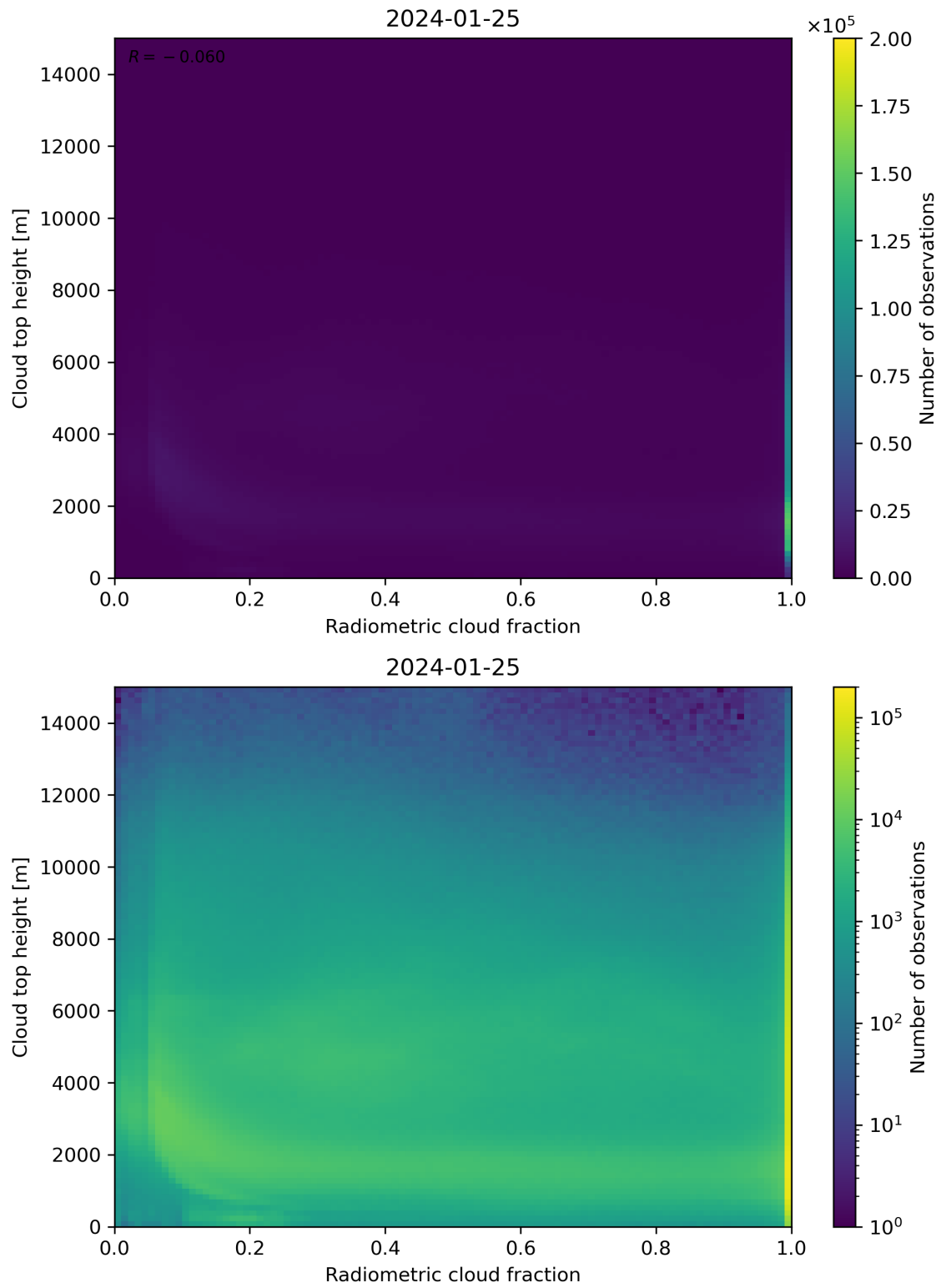
Figure 76: Scatter density plot of “Radiometric cloud fraction” against “Cloud top height” for 2024-01-24 to 2024-01-26.
