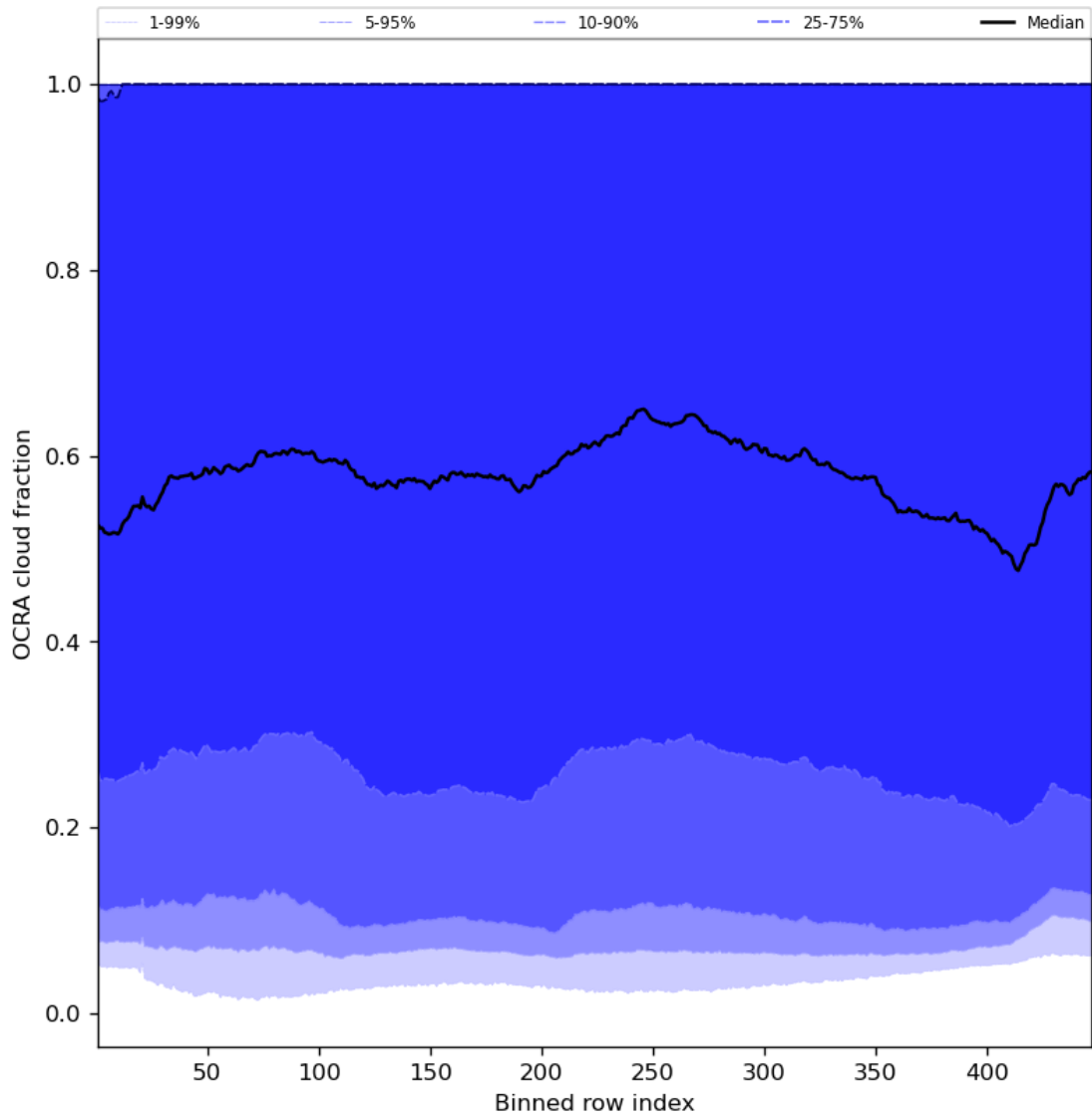
Figure 66: Along track statistics of “OCRA cloud fraction” for 2024-01-24 to 2024-01-26
