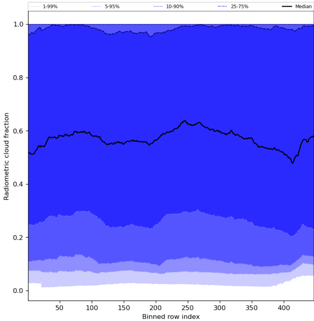
Figure 55: Along track statistics of “Radiometric cloud fraction” for 2024-01-24 to 2024-01-26
