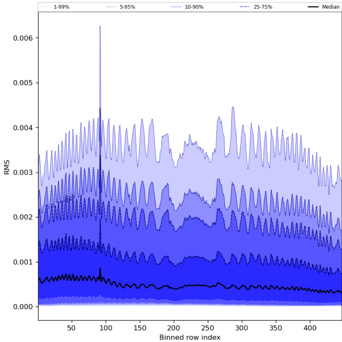
Figure 63: Along track statistics of “RMS” for 2024-01-24 to 2024-01-26
