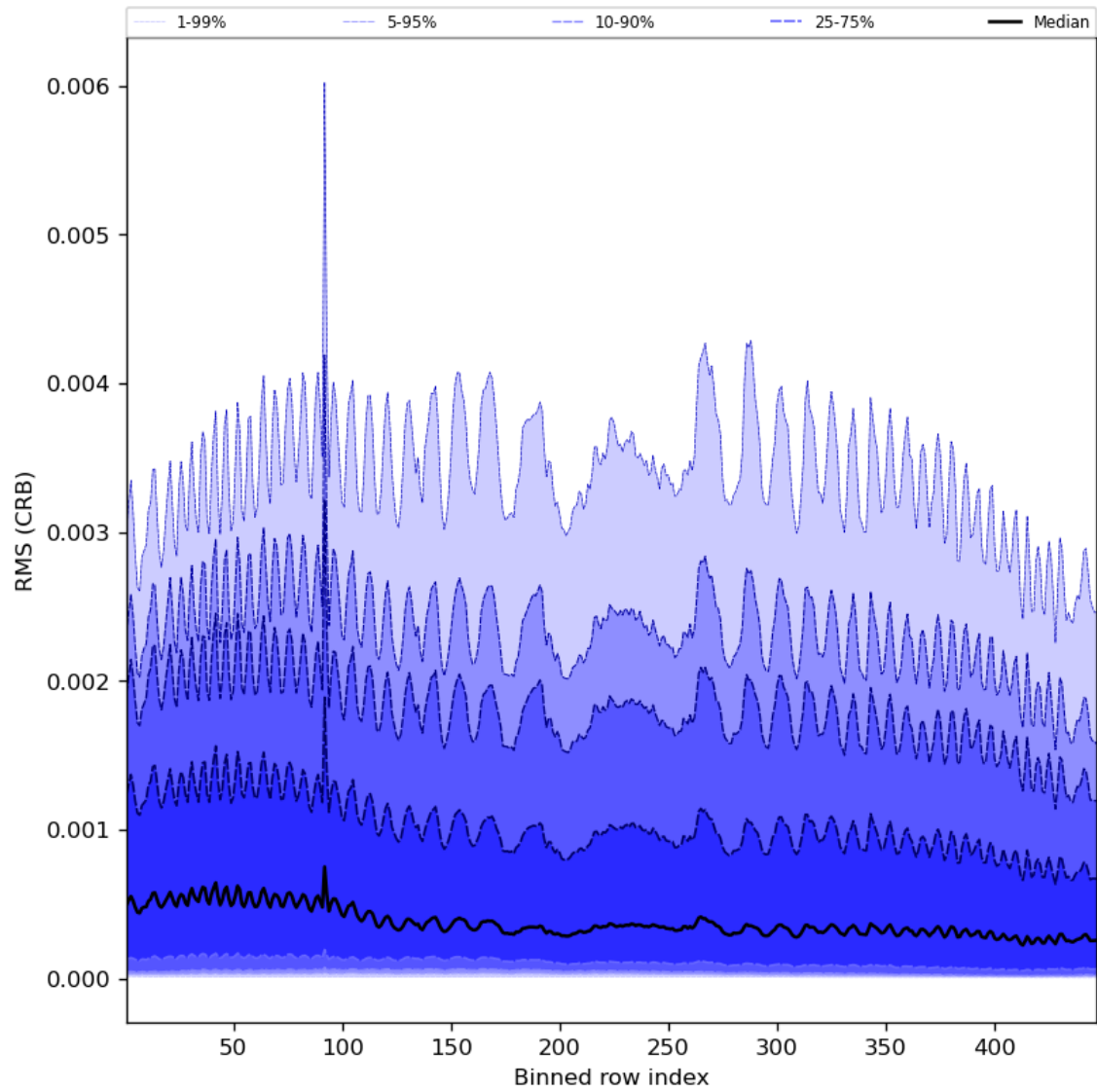
Figure 64: Along track statistics of “RMS (CRB)” for 2024-01-24 to 2024-01-26
