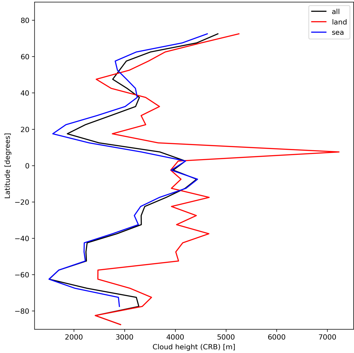
Figure 27: Zonal average of “Cloud height (CRB)” for 2024-01-24 to 2024-01-26.
