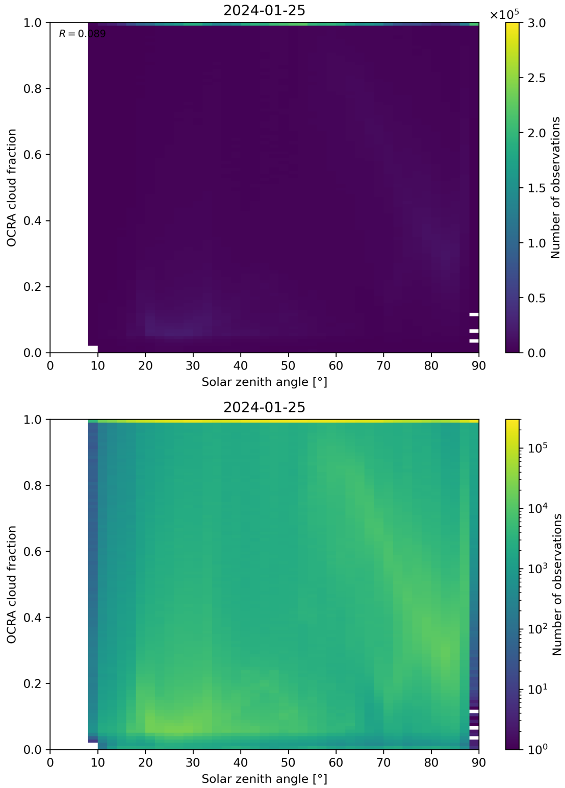
Figure 100: Scatter density plot of “Solar zenith angle” against “OCRA cloud fraction” for 2024-01-24 to 2024-01-26.
