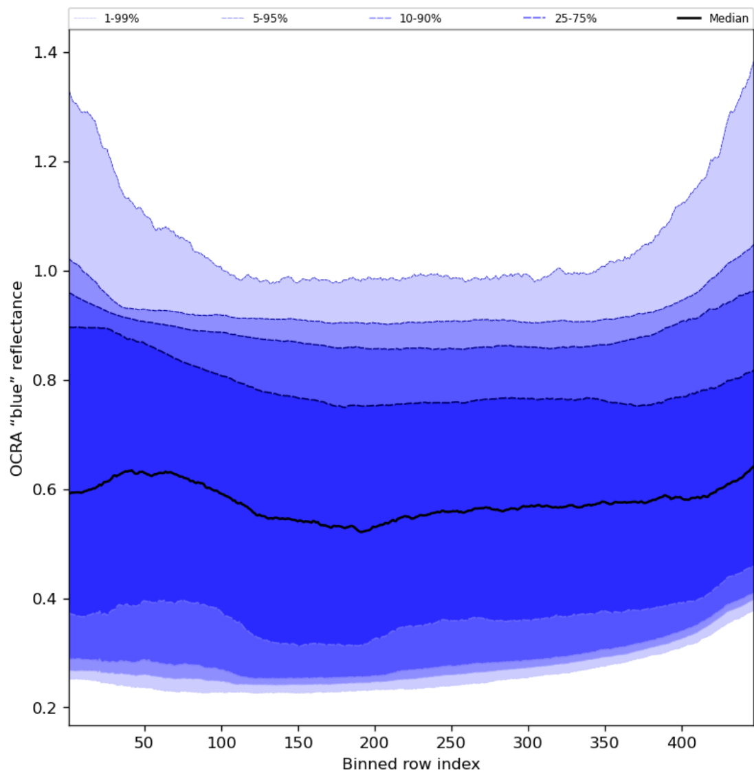
Figure 67: Along track statistics of “OCRA “blue” reflectance” for 2024-01-24 to 2024-01-26
