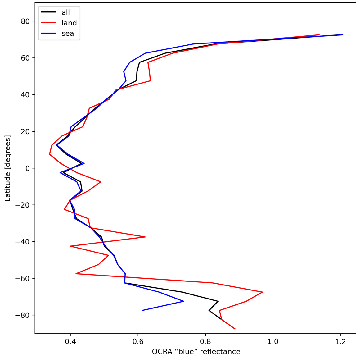
Figure 35: Zonal average of “OCRA “blue” reflectance” for 2024-01-24 to 2024-01-26.
