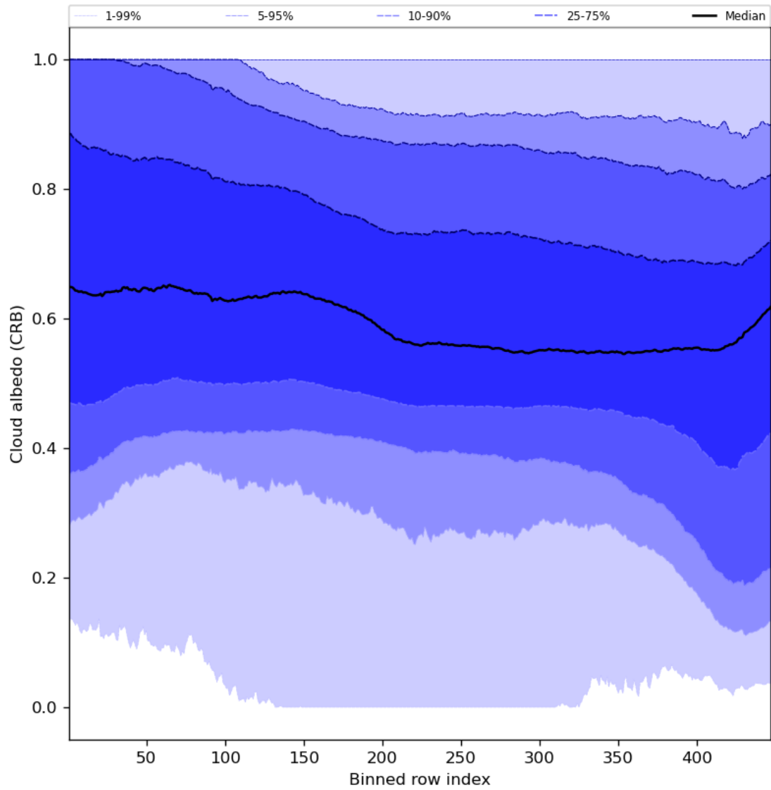
Figure 60: Along track statistics of “Cloud albedo (CRB)” for 2024-01-24 to 2024-01-26
