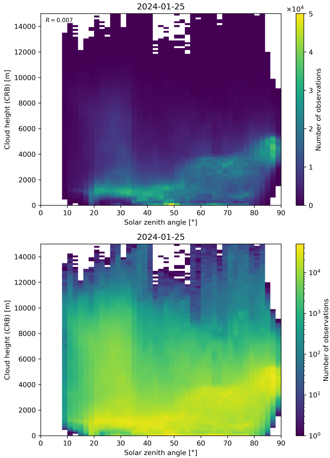
Figure 102: Scatter density plot of “Solar zenith angle” against “Cloud height (CRB)” for 2024-01-24 to 2024-01-26.
