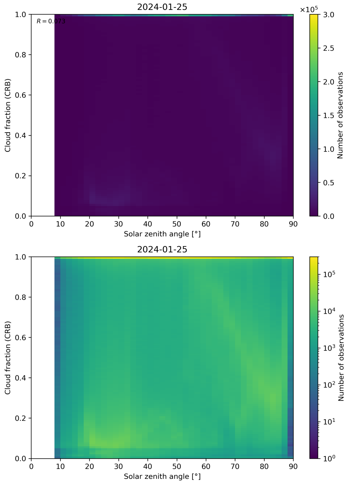
Figure 101: Scatter density plot of “Solar zenith angle” against “Cloud fraction (CRB)” for 2024-01-24 to 2024-01-26.
