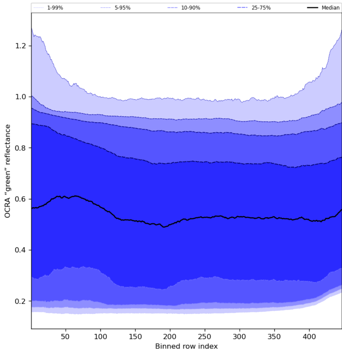
Figure 68: Along track statistics of “OCRA “green” reflectance” for 2024-01-24 to 2024-01-26
