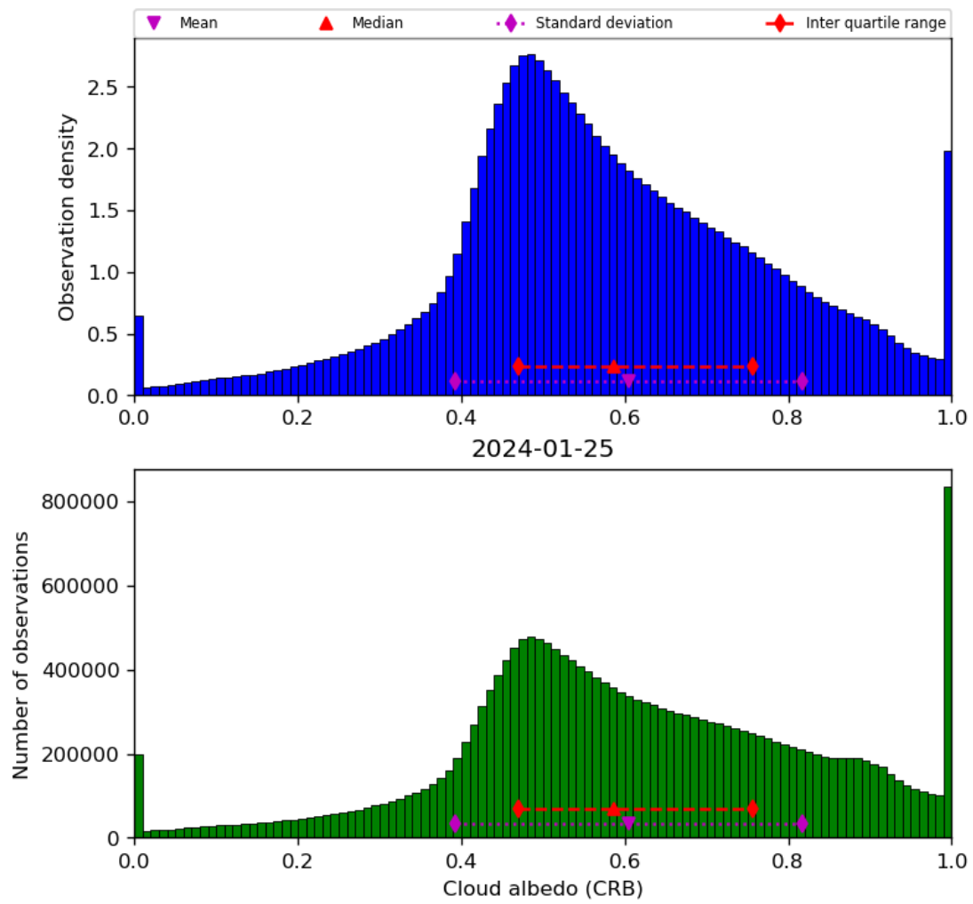
Figure 44: Histogram of “Cloud albedo (CRB)” for 2024-01-24 to 2024-01-26
