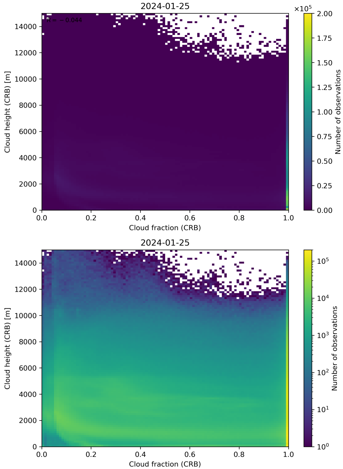
Figure 79: Scatter density plot of “Cloud fraction (CRB)” against “Cloud height (CRB)” for 2024-01-24 to 2024-01-26.
