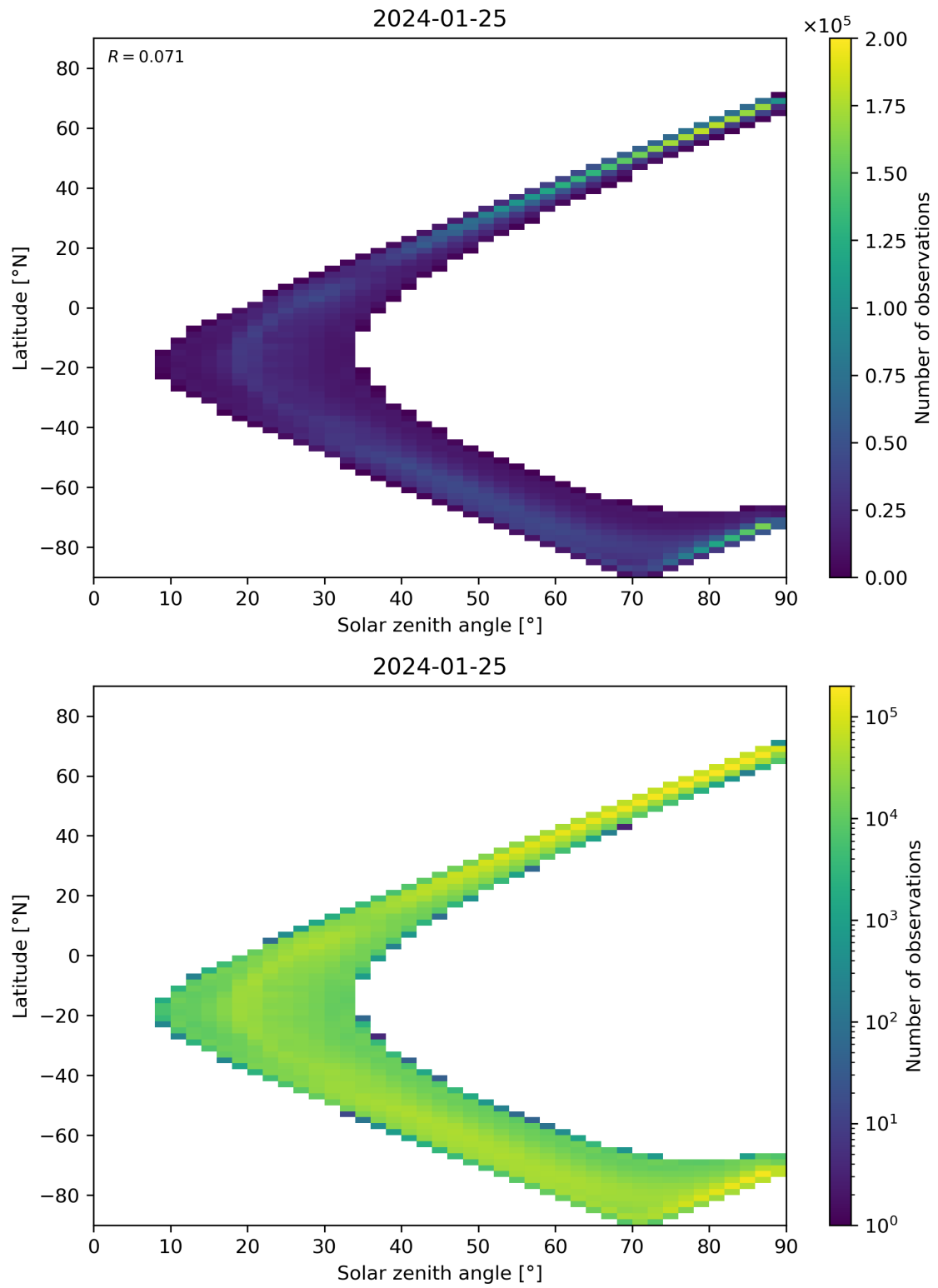
Figure 105: Scatter density plot of “Solar zenith angle” against “Latitude” for 2024-01-24 to 2024-01-26.
