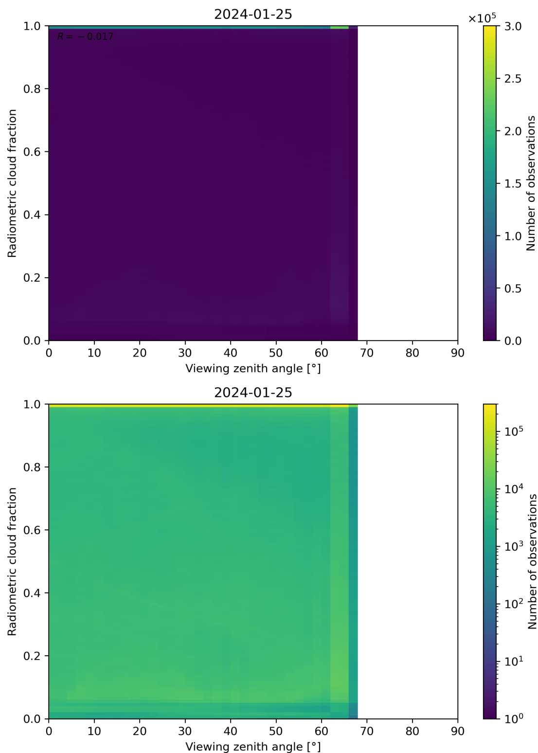
Figure 107: Scatter density plot of “Viewing zenith angle” against “Radiometric cloud fraction” for 2024-01-24 to 2024-01-26.
