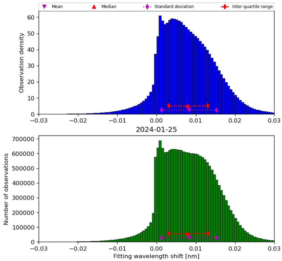
Figure 49: Histogram of “Fitting wavelength shift” for 2024-01-24 to 2024-01-26
