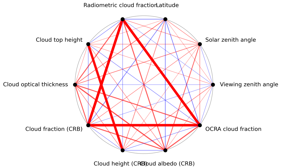
Figure 1: Map of correlation graph for 2024-01-24 to 2024-01-26.
