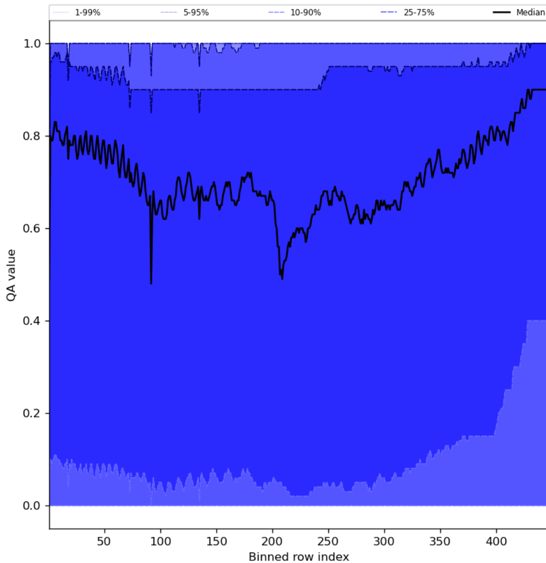
Figure 54: Along track statistics of “QA value” for 2024-01-24 to 2024-01-26
