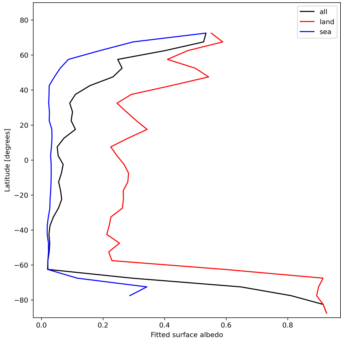
Figure 29: Zonal average of “Fitted surface albedo” for 2024-01-24 to 2024-01-26.
