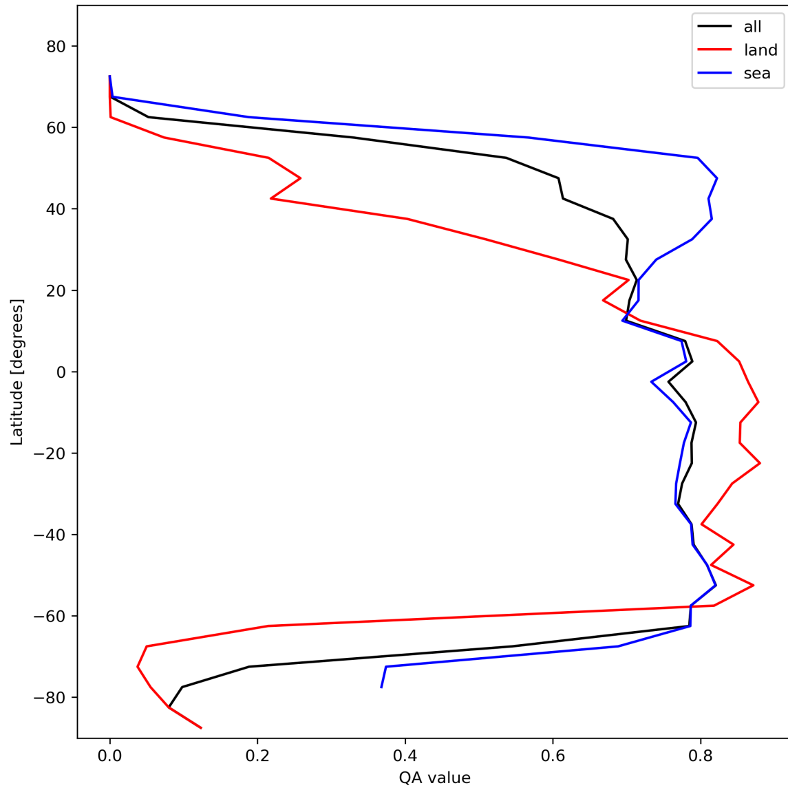
Figure 22: Zonal average of “QA value” for 2024-01-24 to 2024-01-26.
