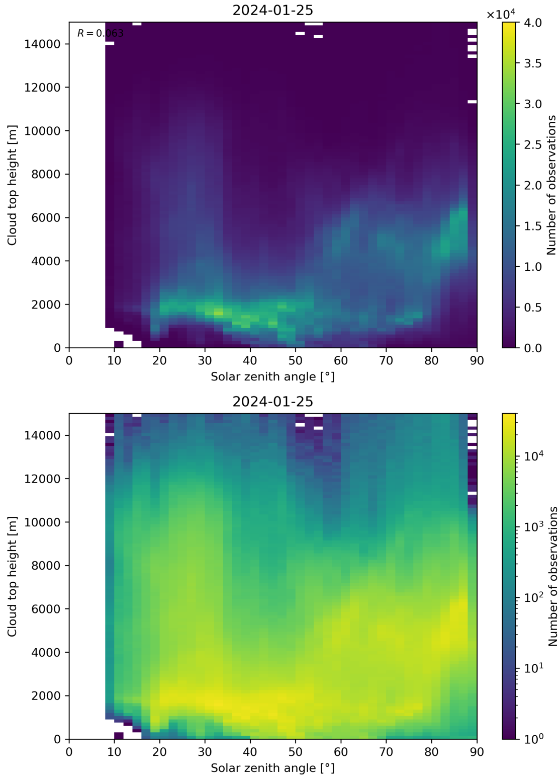
Figure 104: Scatter density plot of “Solar zenith angle” against “Cloud top height” for 2024-01-24 to 2024-01-26.
