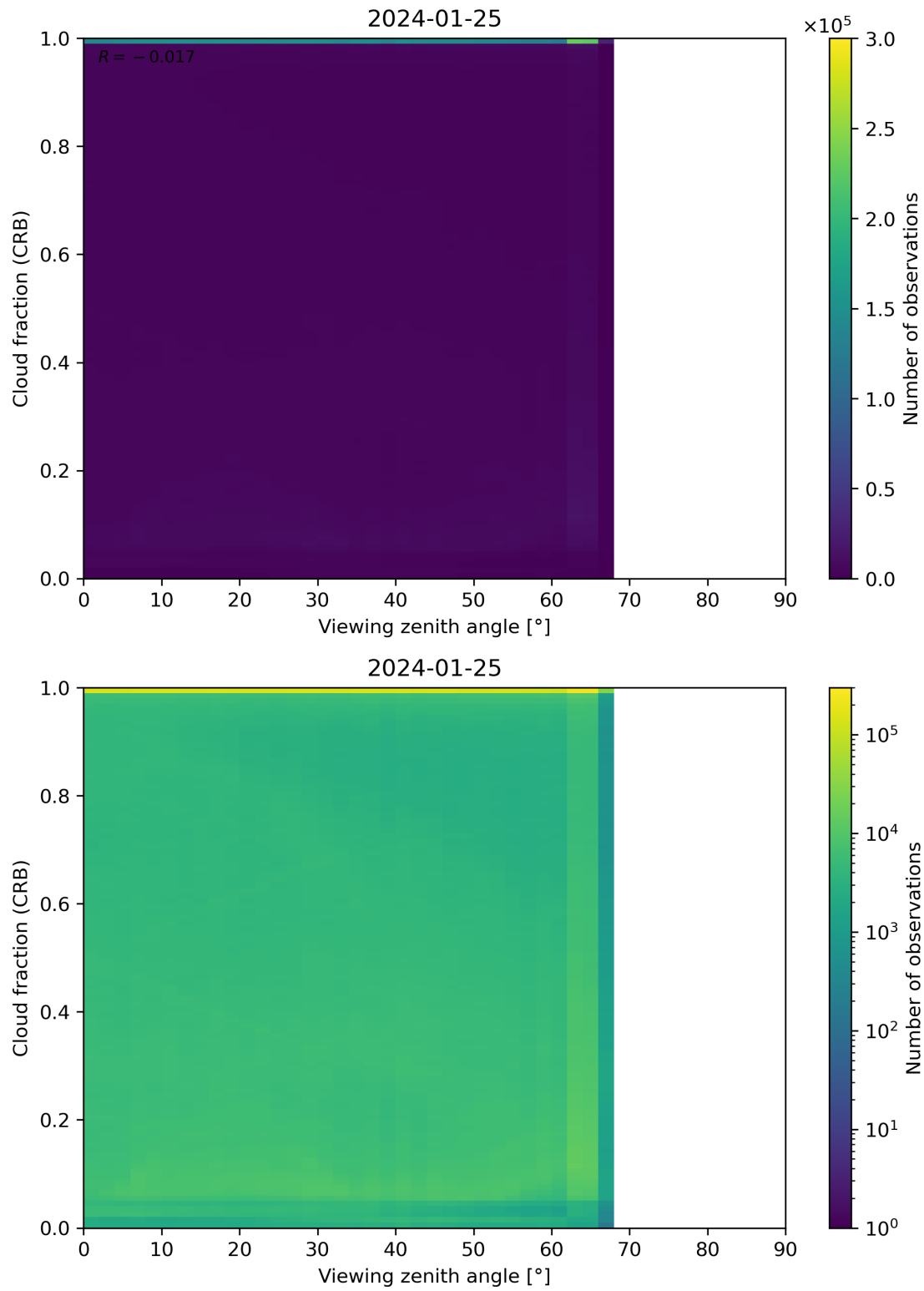
Figure 109: Scatter density plot of “Viewing zenith angle” against “Cloud fraction (CRB)” for 2024-01-24 to 2024-01-26.
