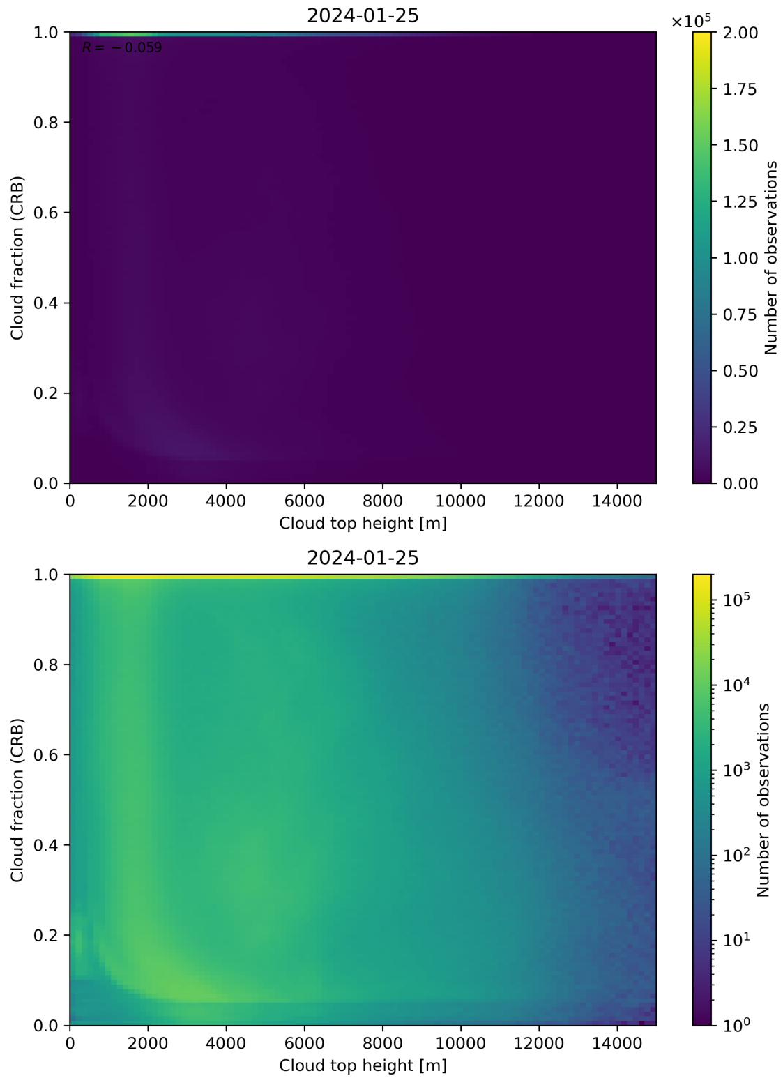
Figure 88: Scatter density plot of “Cloud top height” against “Cloud fraction (CRB)” for 2024-01-24 to 2024-01-26.
