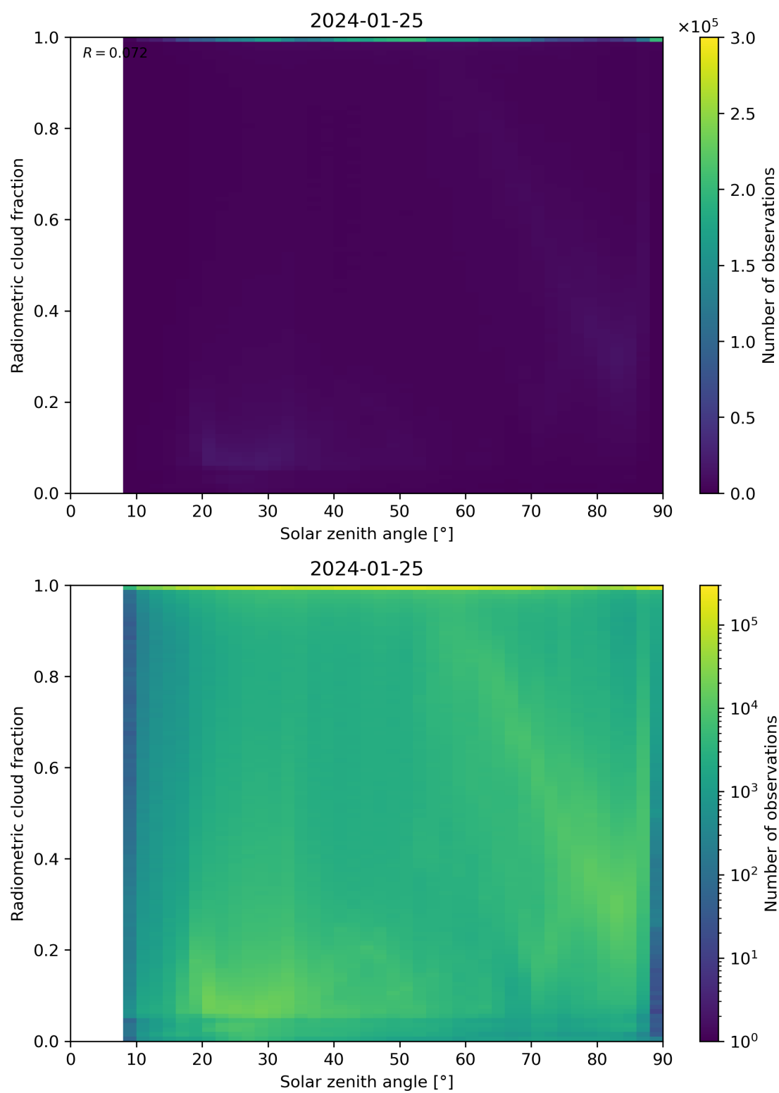
Figure 99: Scatter density plot of “Solar zenith angle” against “Radiometric cloud fraction” for 2024-01-24 to 2024-01-26.
