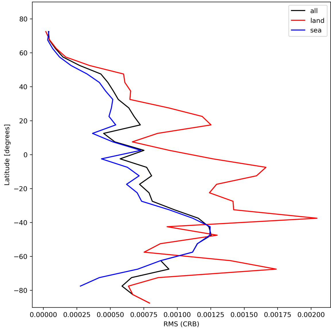
Figure 32: Zonal average of “RMS (CRB)” for 2024-01-24 to 2024-01-26.
