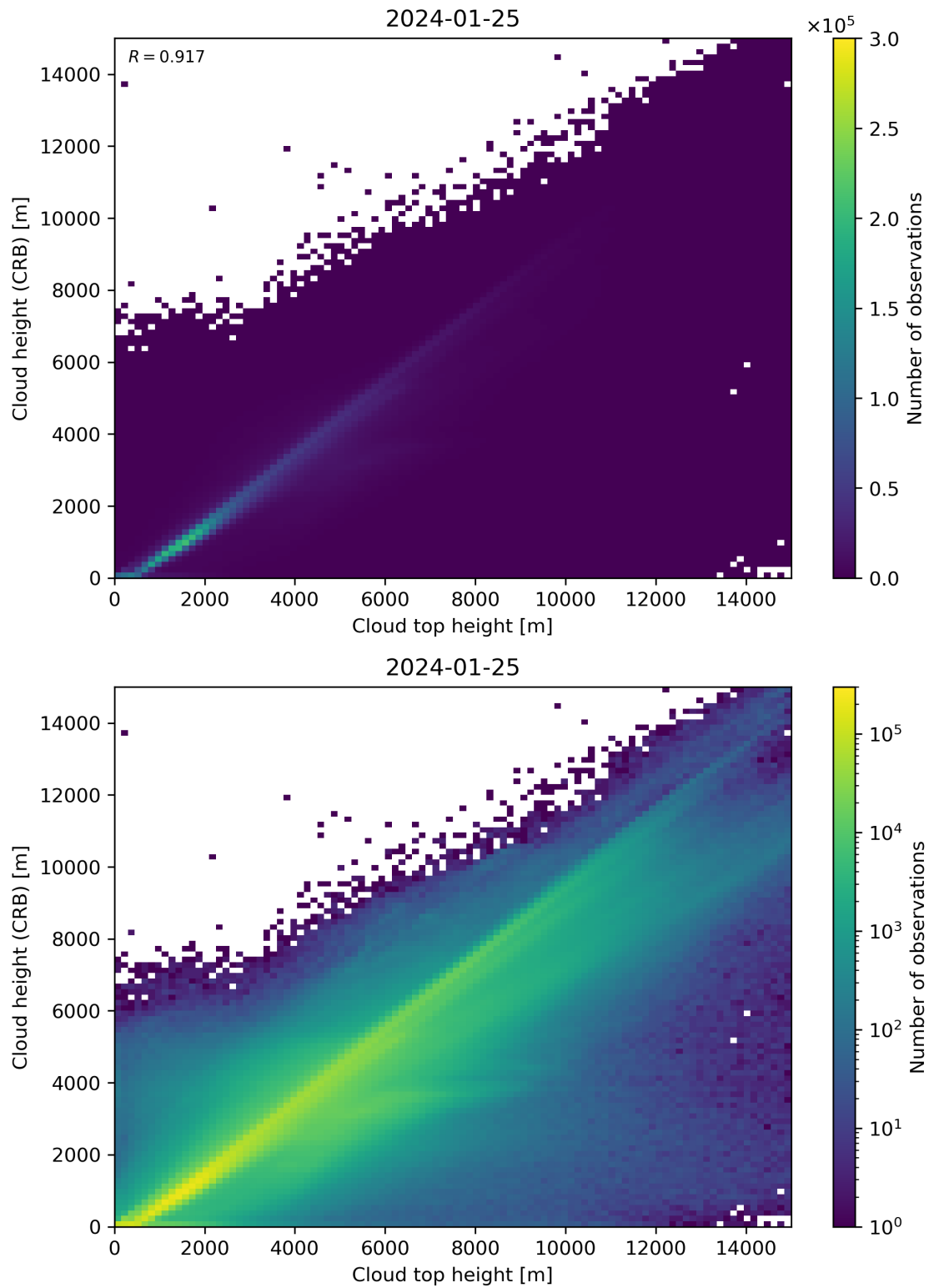
Figure 89: Scatter density plot of “Cloud top height” against “Cloud height (CRB)” for 2024-01-24 to 2024-01-26.
