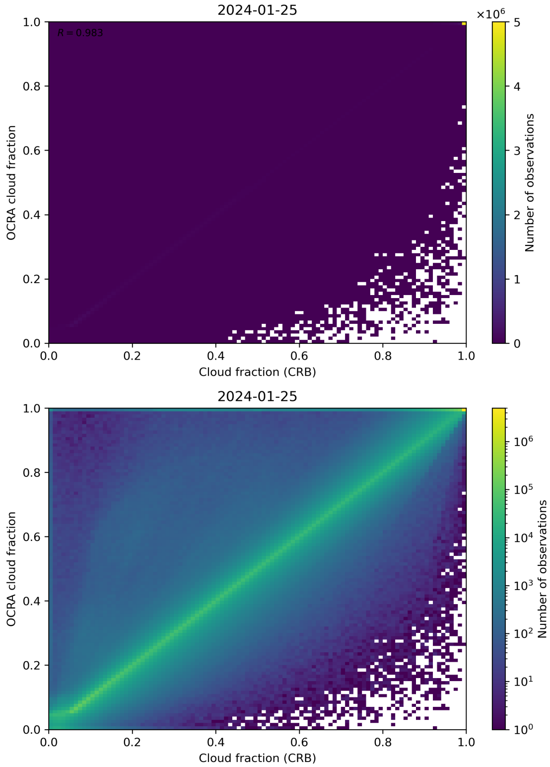
Figure 78: Scatter density plot of “Cloud fraction (CRB)” against “OCRA cloud fraction” for 2024-01-24 to 2024-01-26.
