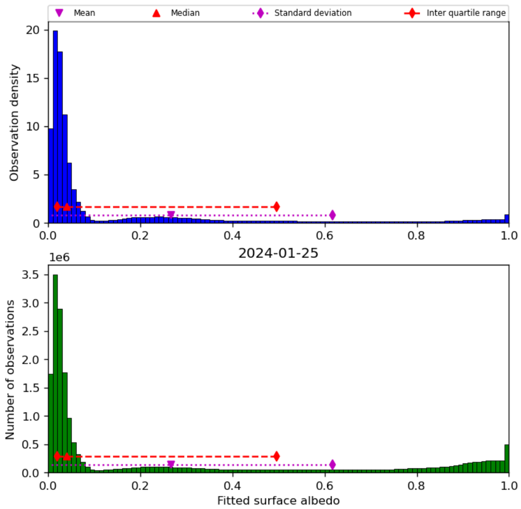
Figure 45: Histogram of “Fitted surface albedo” for 2024-01-24 to 2024-01-26
