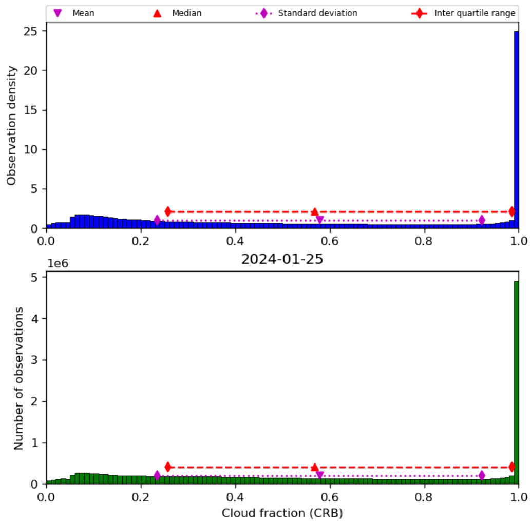
Figure 42: Histogram of “Cloud fraction (CRB)” for 2024-01-24 to 2024-01-26
