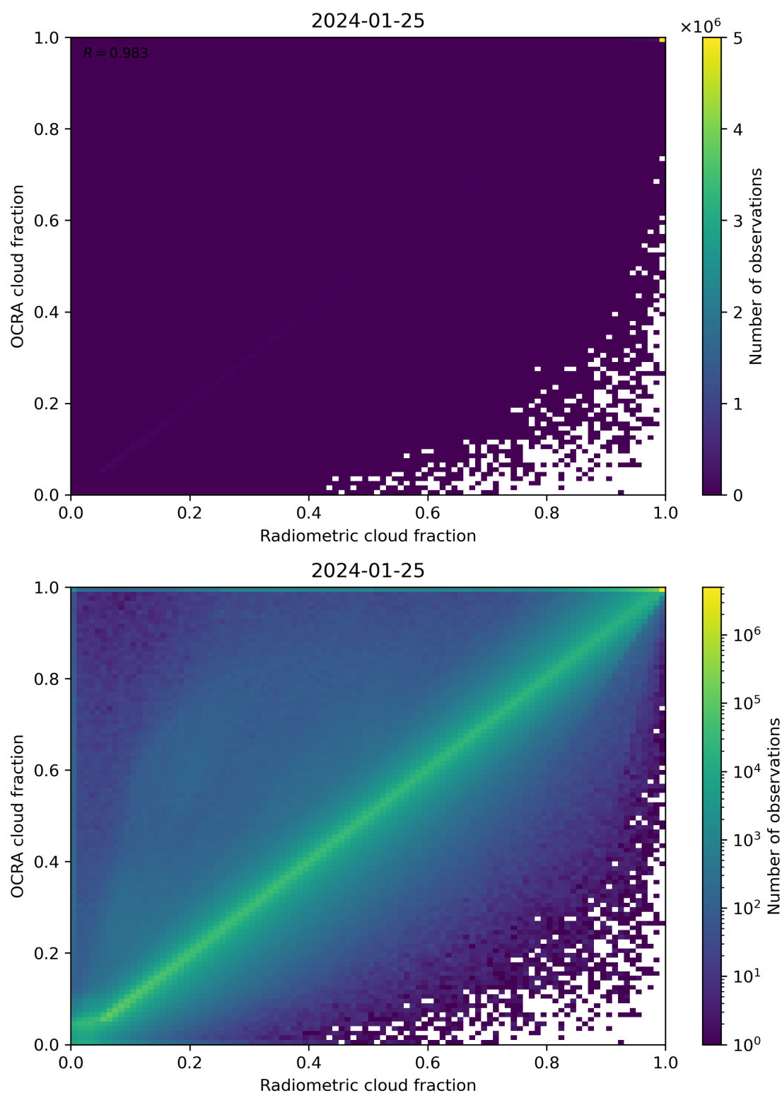
Figure 72: Scatter density plot of “Radiometric cloud fraction” against “OCRA cloud fraction” for 2024-01-24 to 2024-01-26.
