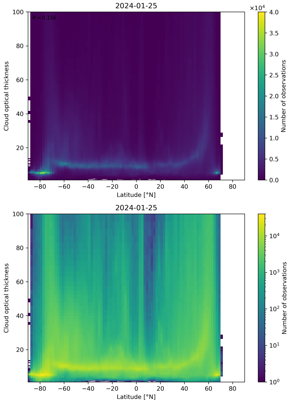
Figure 96: Scatter density plot of “Latitude” against “Cloud optical thickness” for 2024-01-24 to 2024-01-26.
