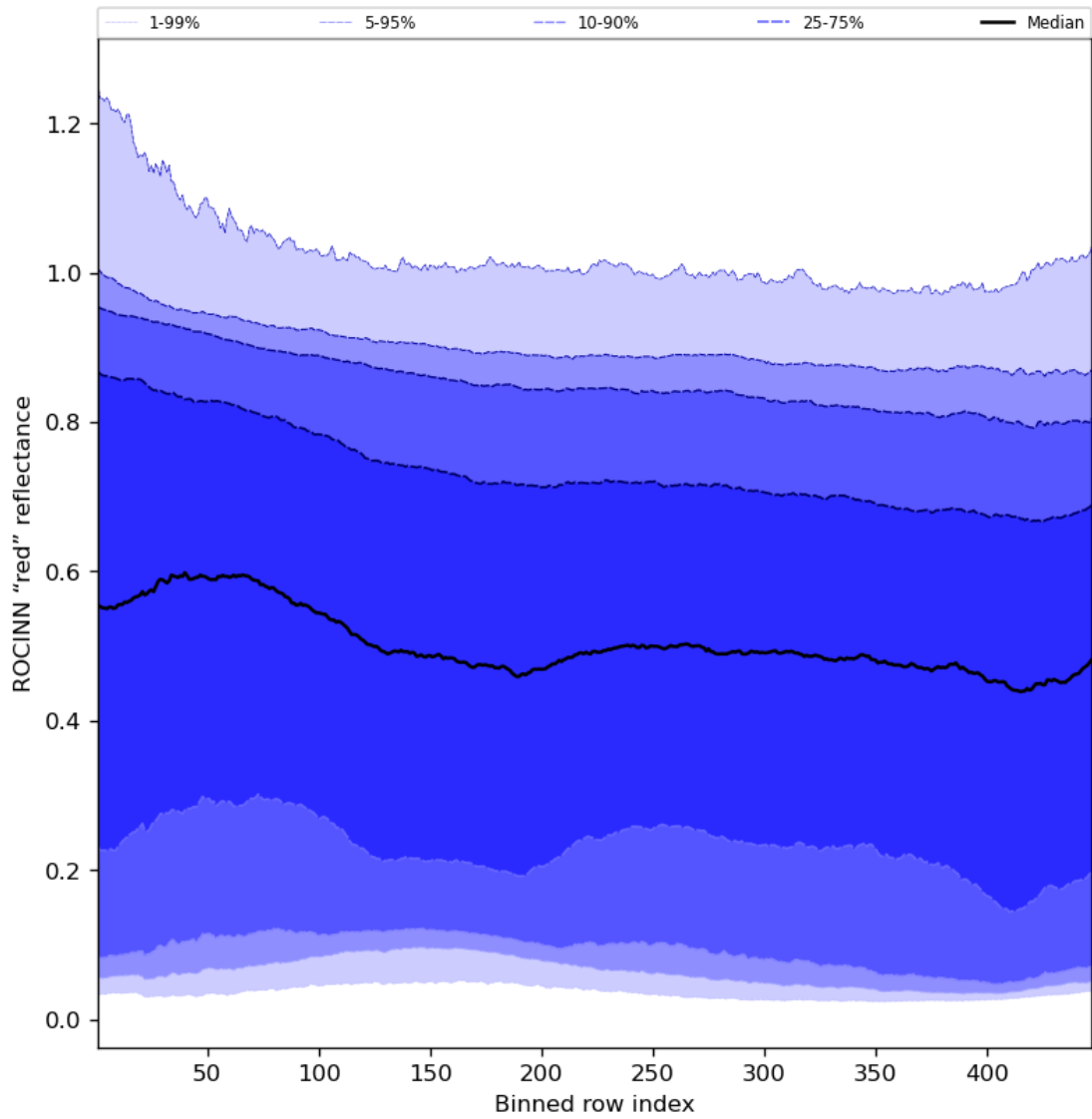
Figure 69: Along track statistics of “ROCINN “red” reflectance” for 2024-01-24 to 2024-01-26
