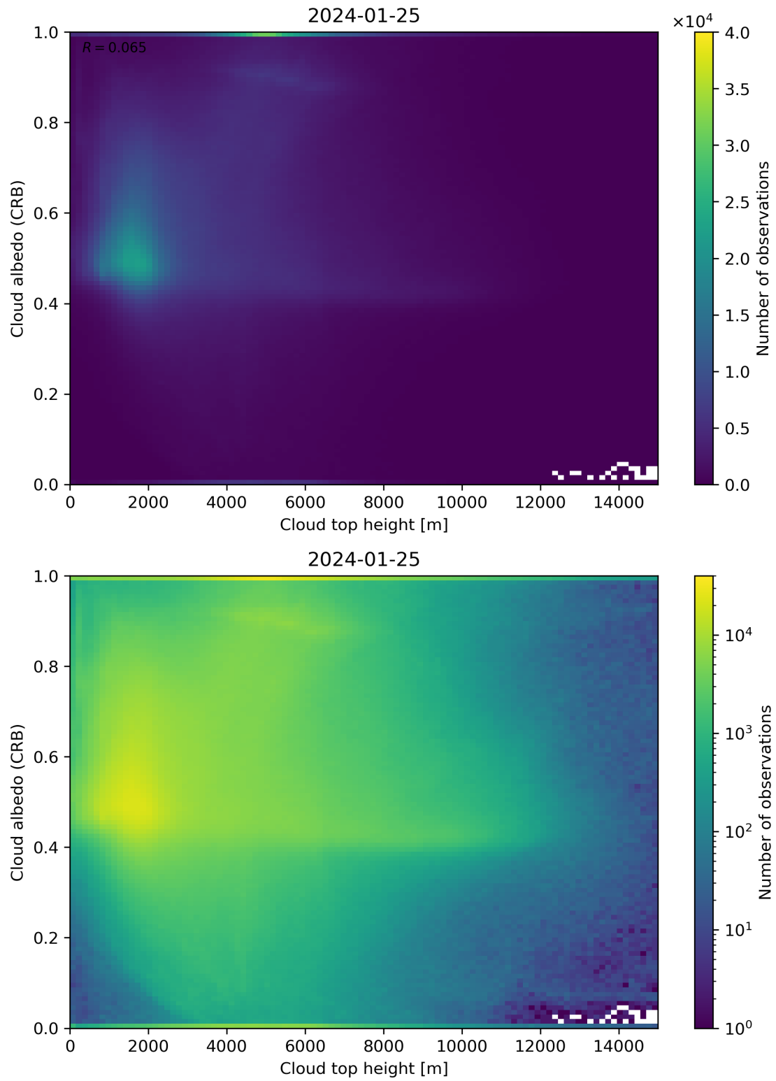
Figure 86: Scatter density plot of “Cloud top height” against “Cloud albedo (CRB)” for 2024-01-24 to 2024-01-26.
