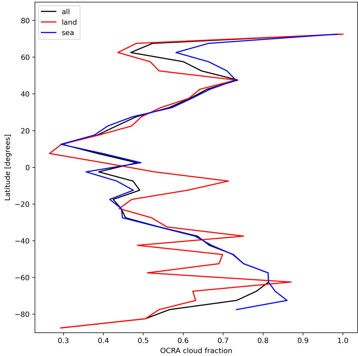
Figure 34: Zonal average of “OCRA cloud fraction” for 2024-01-24 to 2024-01-26.
