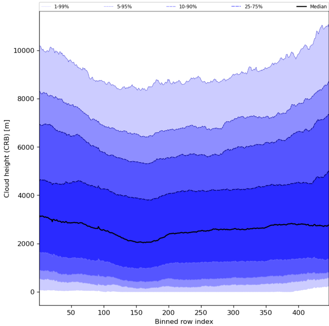
Figure 59: Along track statistics of “Cloud height (CRB)” for 2024-01-24 to 2024-01-26
