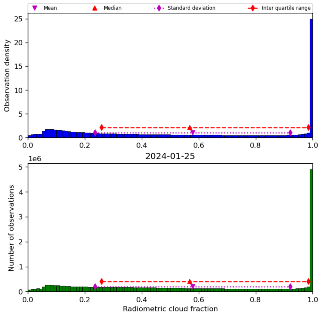
Figure 39: Histogram of “Radiometric cloud fraction” for 2024-01-24 to 2024-01-26
