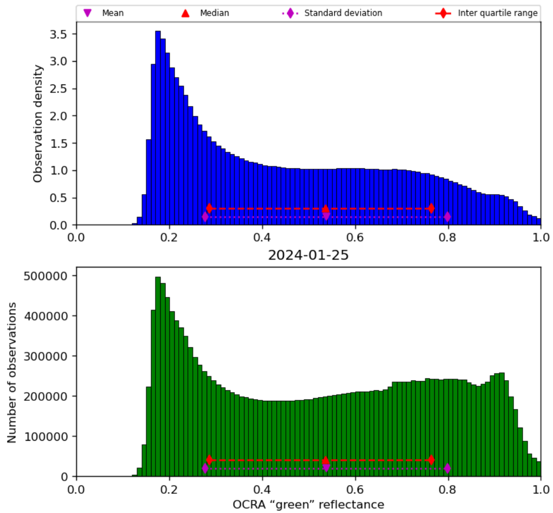
Figure 52: Histogram of “OCRA “green” reflectance” for 2024-01-24 to 2024-01-26
