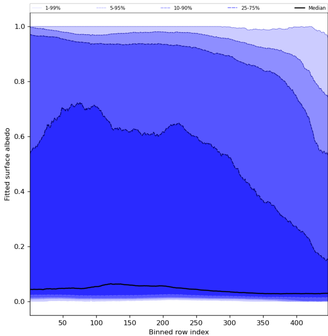
Figure 61: Along track statistics of “Fitted surface albedo” for 2024-01-24 to 2024-01-26
