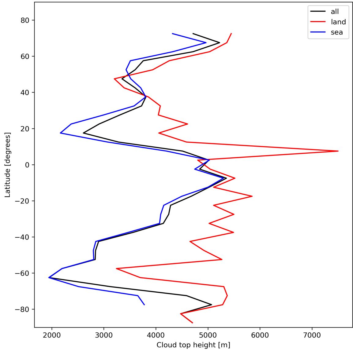
Figure 24: Zonal average of “Cloud top height” for 2024-01-24 to 2024-01-26.
