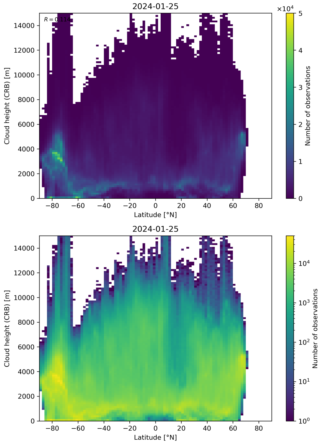
Figure 95: Scatter density plot of “Latitude” against “Cloud height (CRB)” for 2024-01-24 to 2024-01-26.
