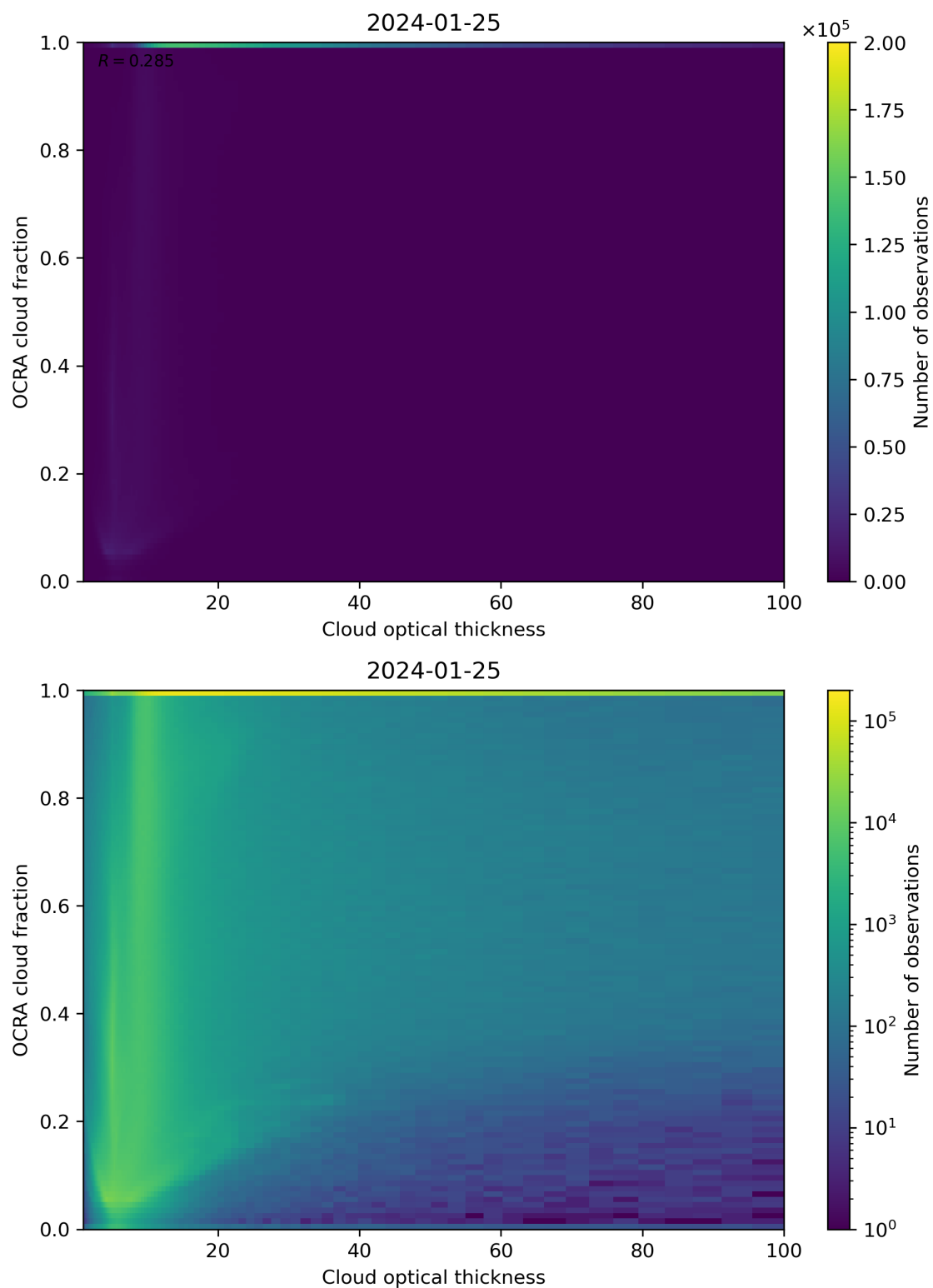
Figure 83: Scatter density plot of “Cloud optical thickness” against “OCRA cloud fraction” for 2024-01-24 to 2024-01-26.
