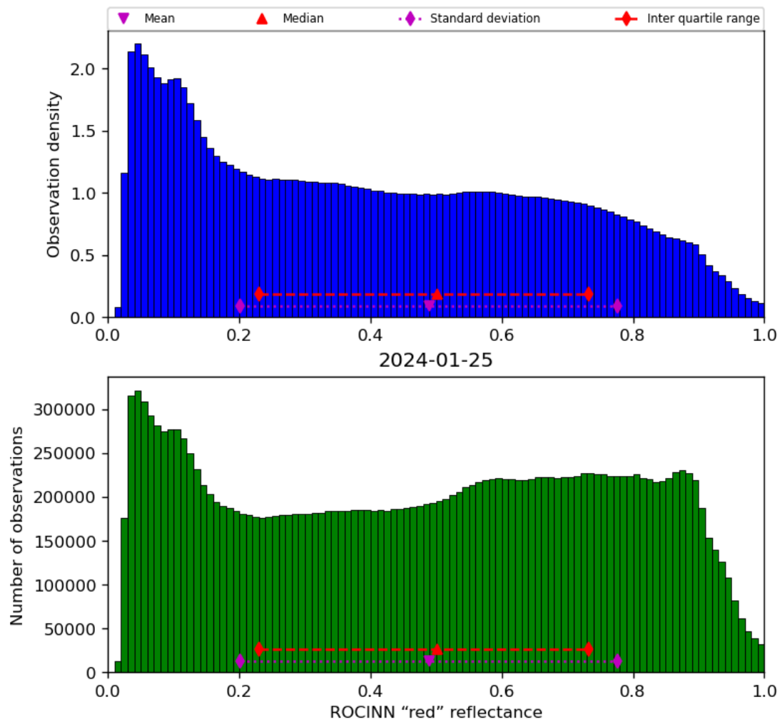
Figure 53: Histogram of “ROCINN “red” reflectance” for 2024-01-24 to 2024-01-26
