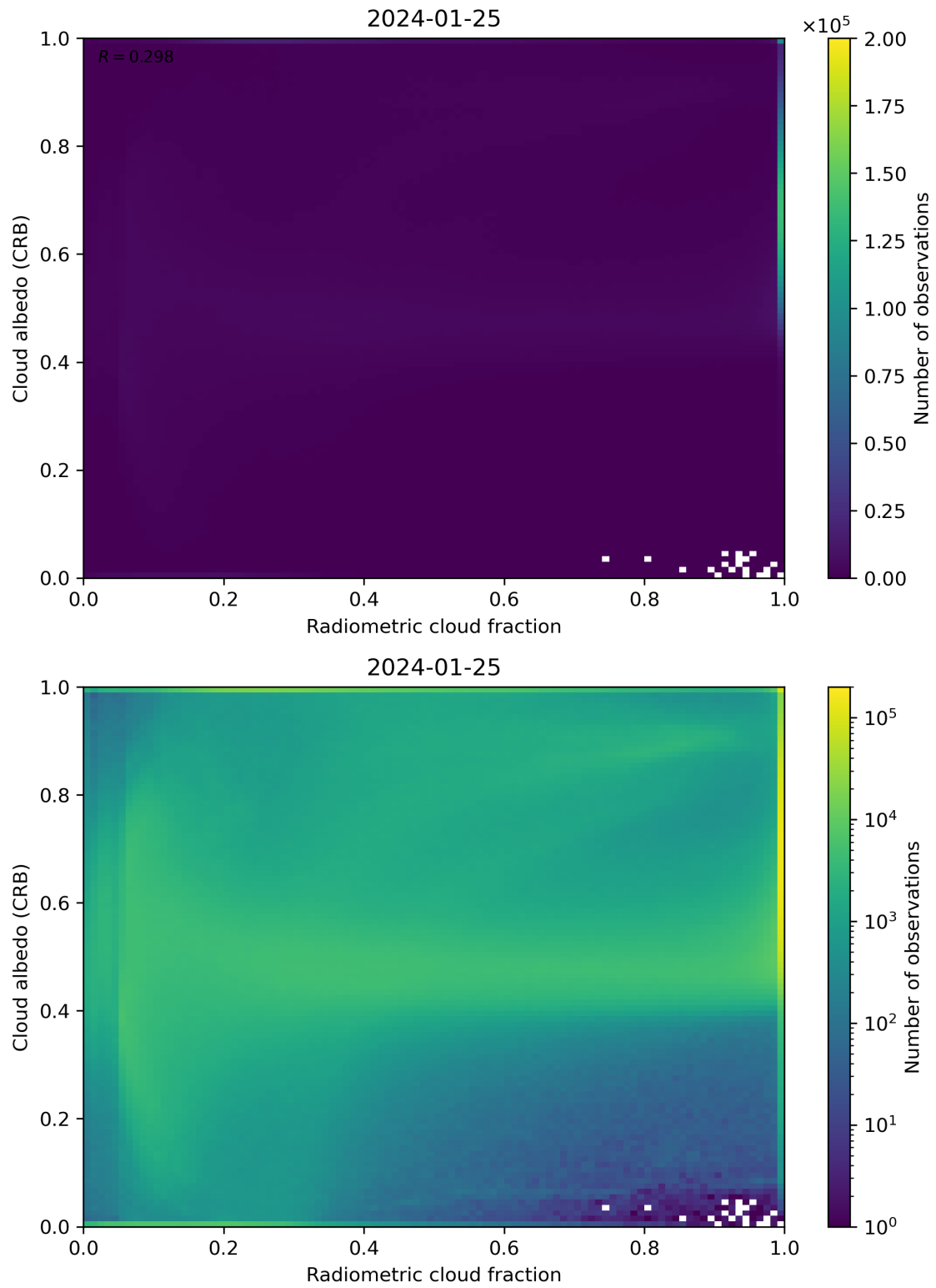
Figure 71: Scatter density plot of “Radiometric cloud fraction” against “Cloud albedo (CRB)” for 2024-01-24 to 2024-01-26.
