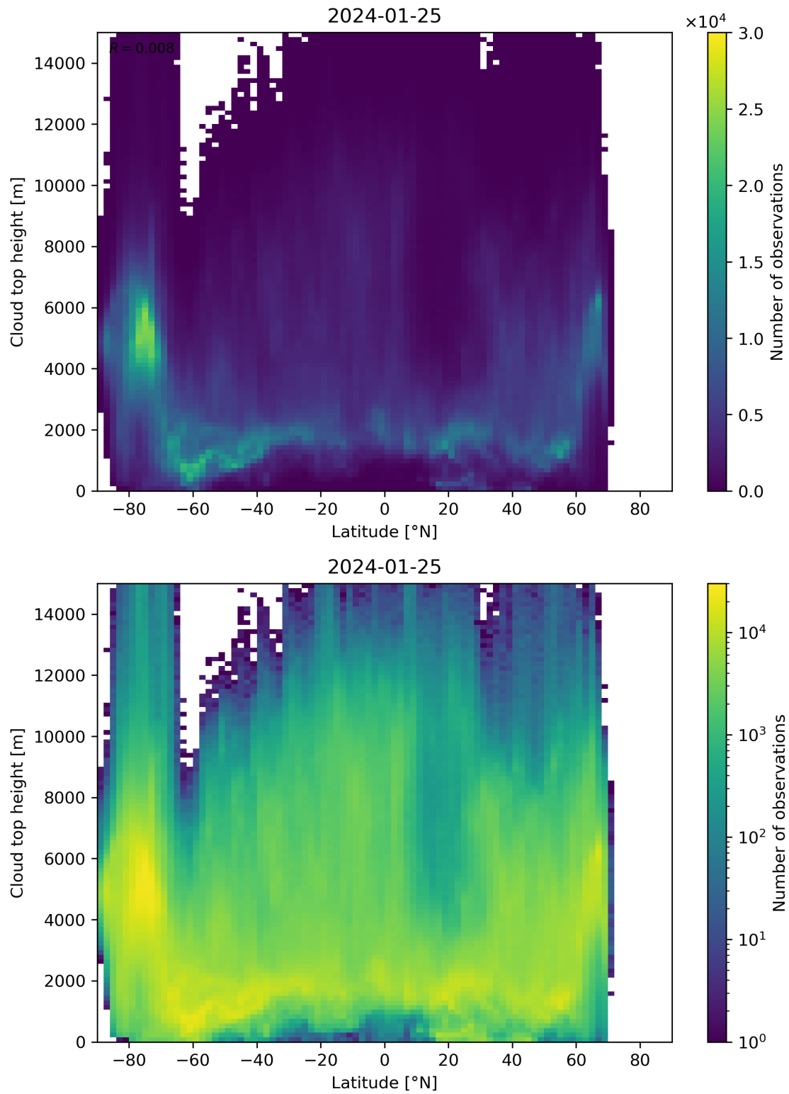
Figure 97: Scatter density plot of “Latitude” against “Cloud top height” for 2024-01-24 to 2024-01-26.
