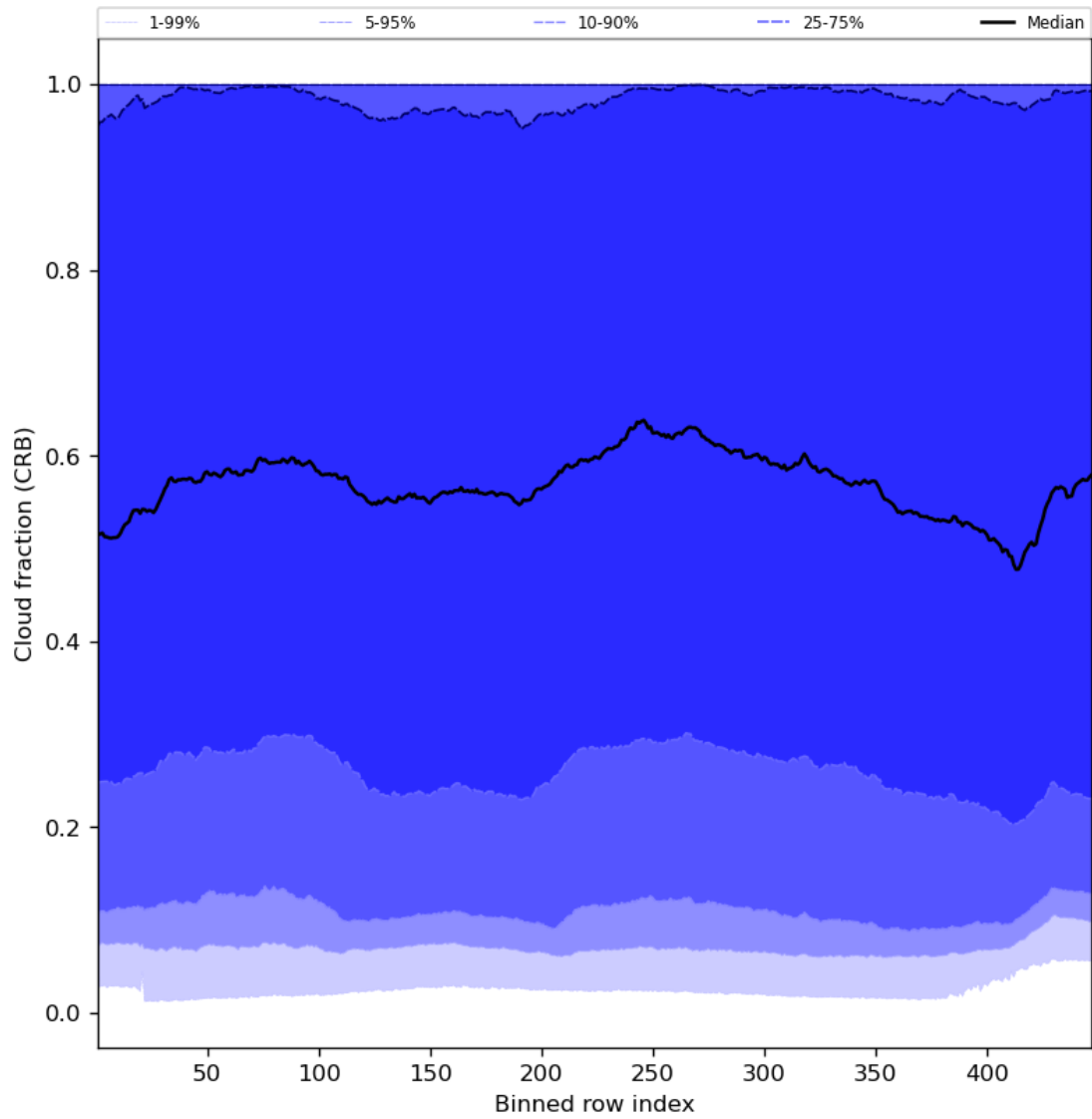
Figure 58: Along track statistics of “Cloud fraction (CRB)” for 2024-01-24 to 2024-01-26
