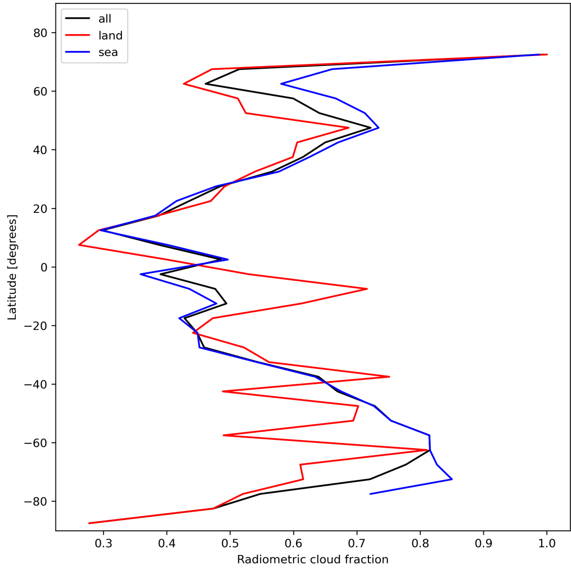
Figure 23: Zonal average of “Radiometric cloud fraction” for 2024-01-24 to 2024-01-26.
