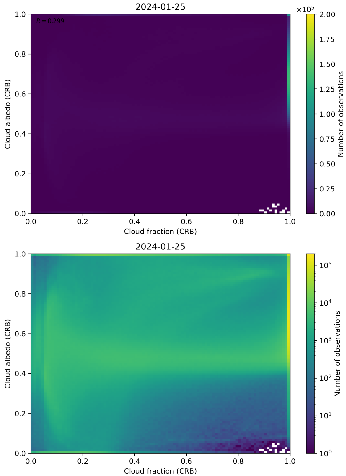
Figure 77: Scatter density plot of “Cloud fraction (CRB)” against “Cloud albedo (CRB)” for 2024-01-24 to 2024-01-26.
