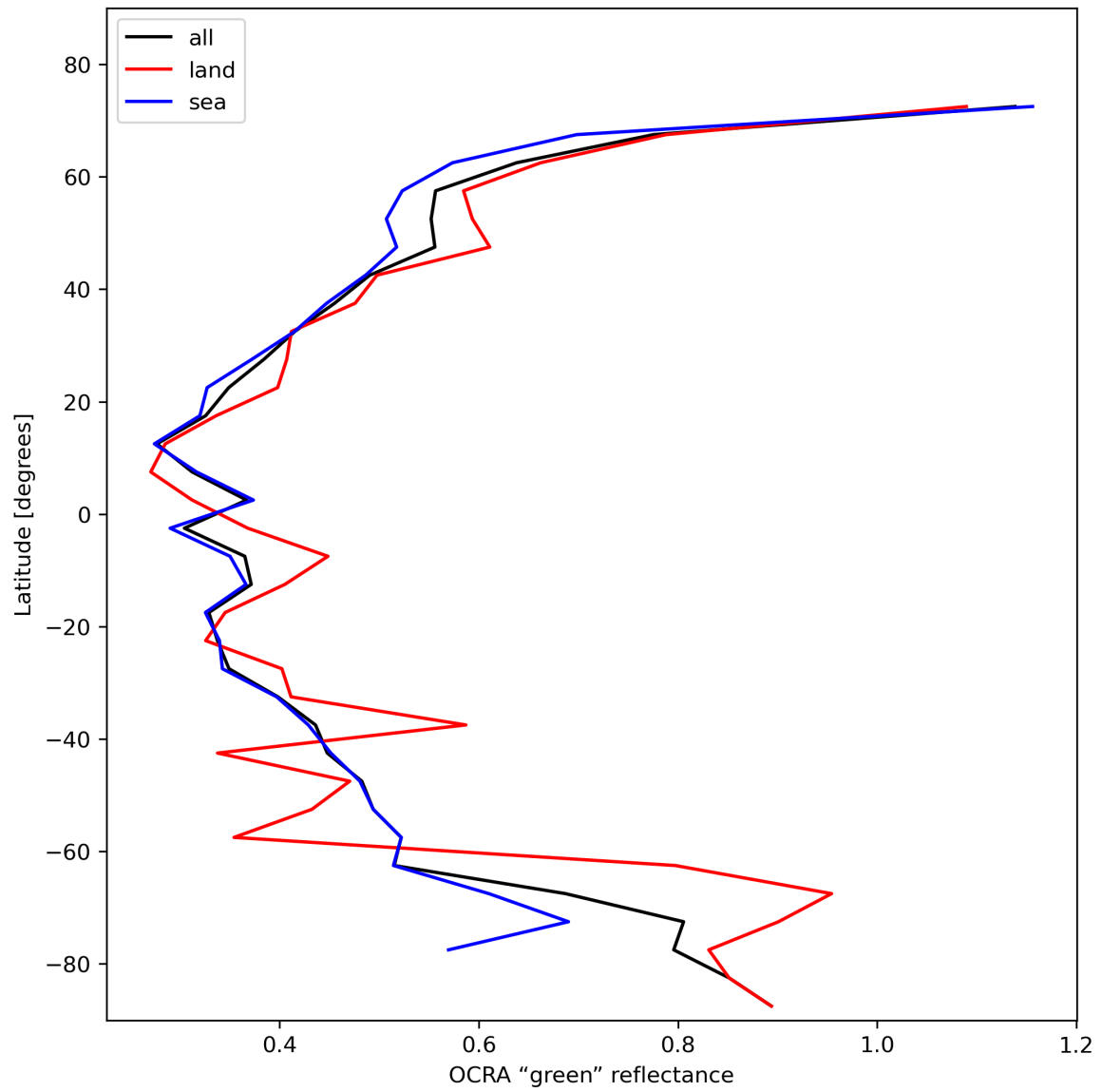
Figure 36: Zonal average of “OCRA “green” reflectance” for 2024-01-24 to 2024-01-26.
