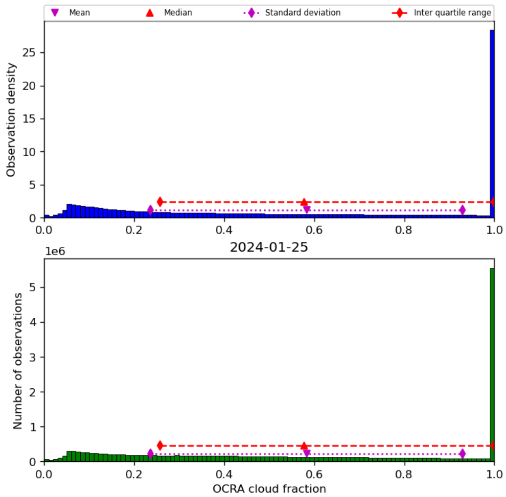
Figure 50: Histogram of “OCRA cloud fraction” for 2024-01-24 to 2024-01-26
