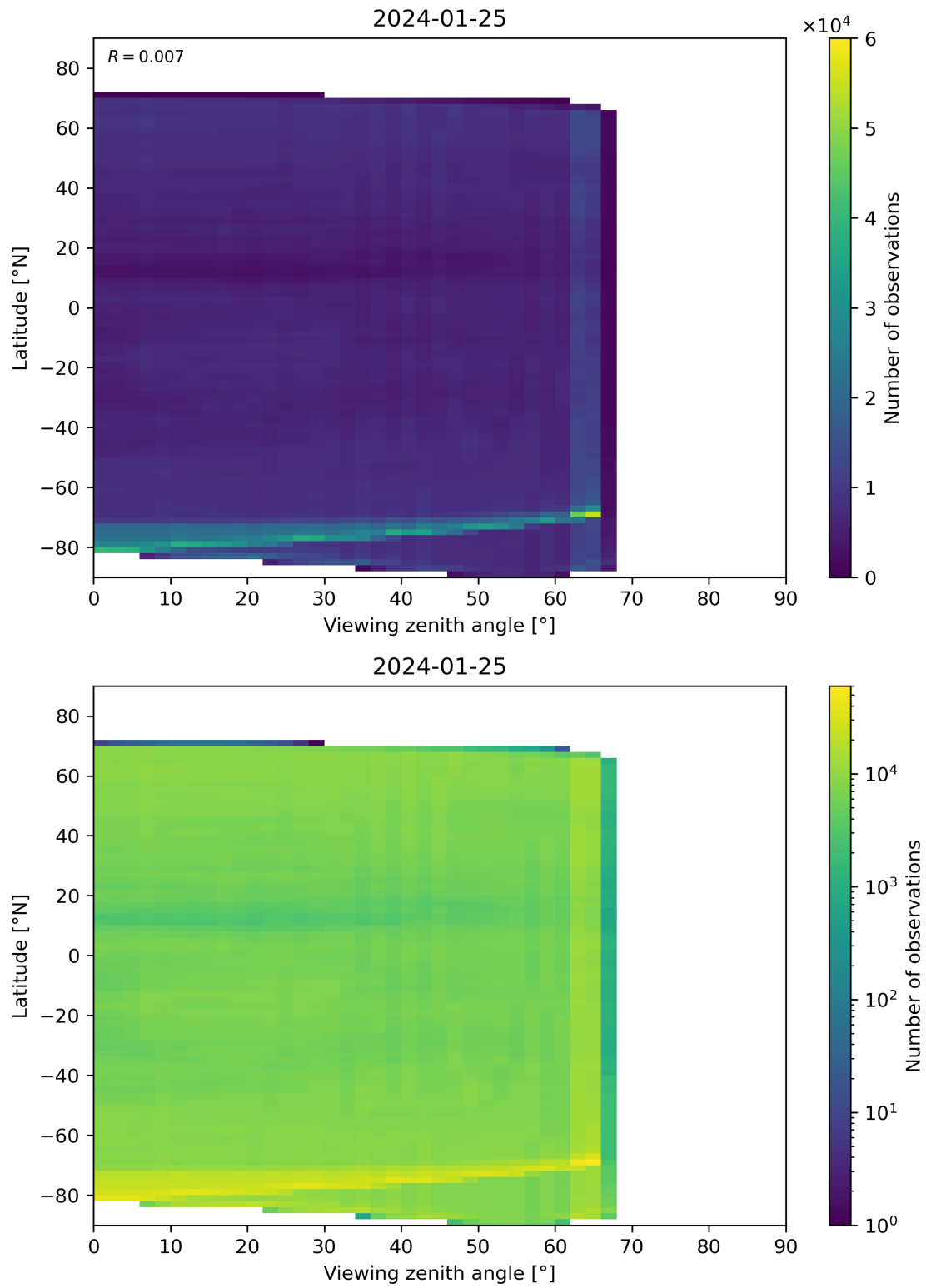
Figure 113: Scatter density plot of “Viewing zenith angle” against “Latitude” for 2024-01-24 to 2024-01-26.
