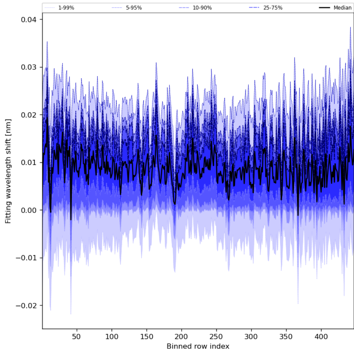
Figure 65: Along track statistics of “Fitting wavelength shift” for 2024-01-24 to 2024-01-26
