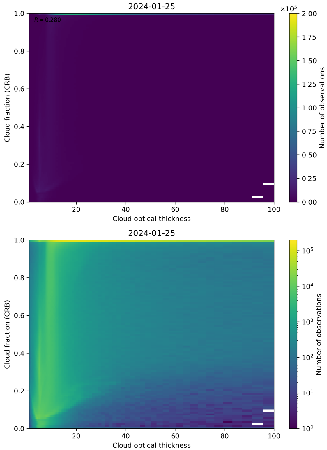
Figure 84: Scatter density plot of “Cloud optical thickness” against “Cloud fraction (CRB)” for 2024-01-24 to 2024-01-26.
