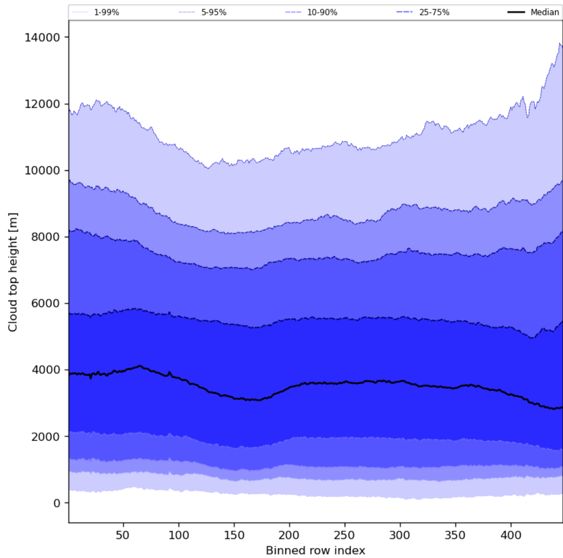
Figure 56: Along track statistics of “Cloud top height” for 2024-01-24 to 2024-01-26
