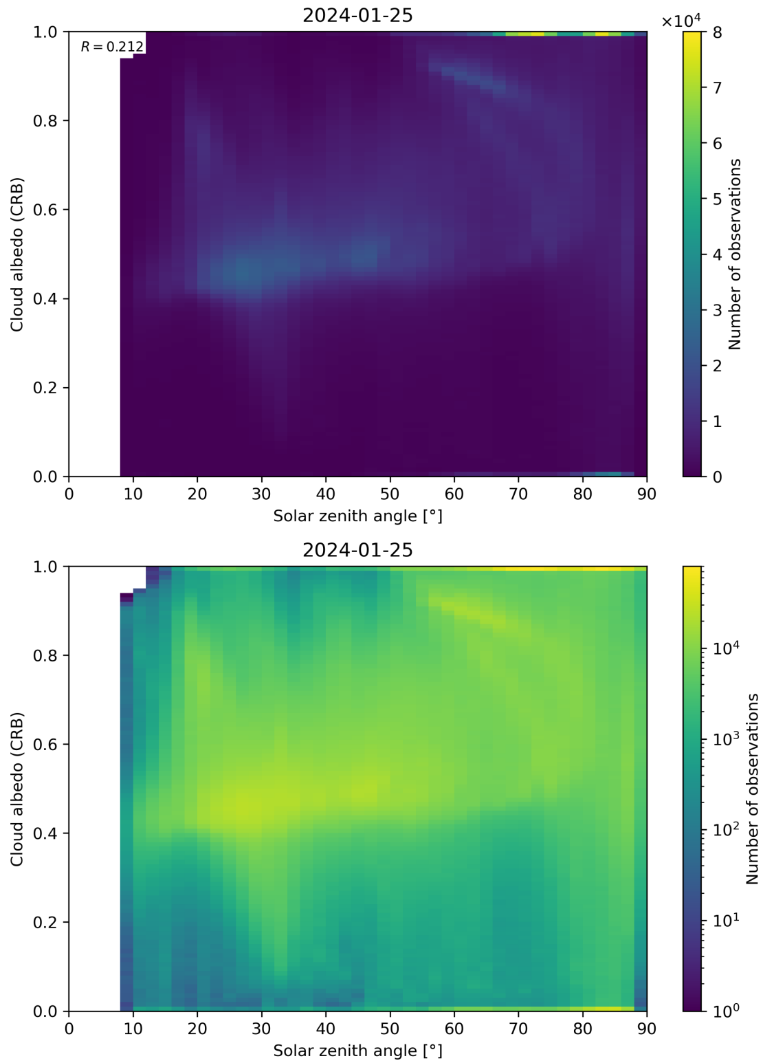
Figure 98: Scatter density plot of “Solar zenith angle” against “Cloud albedo (CRB)” for 2024-01-24 to 2024-01-26.
