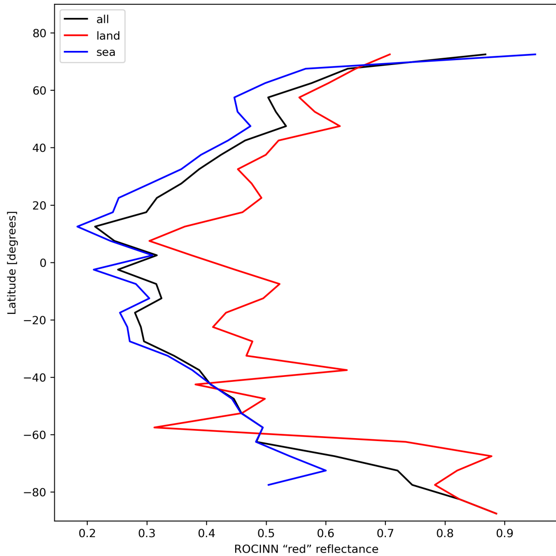
Figure 37: Zonal average of “ROCINN “red” reflectance” for 2024-01-24 to 2024-01-26.
