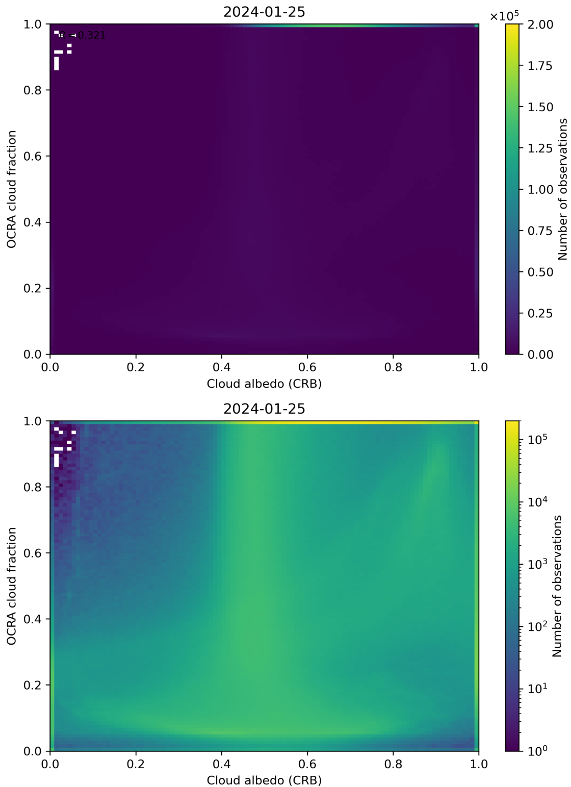
Figure 70: Scatter density plot of “Cloud albedo (CRB)” against “OCRA cloud fraction” for 2024-01-24 to 2024-01-26.
