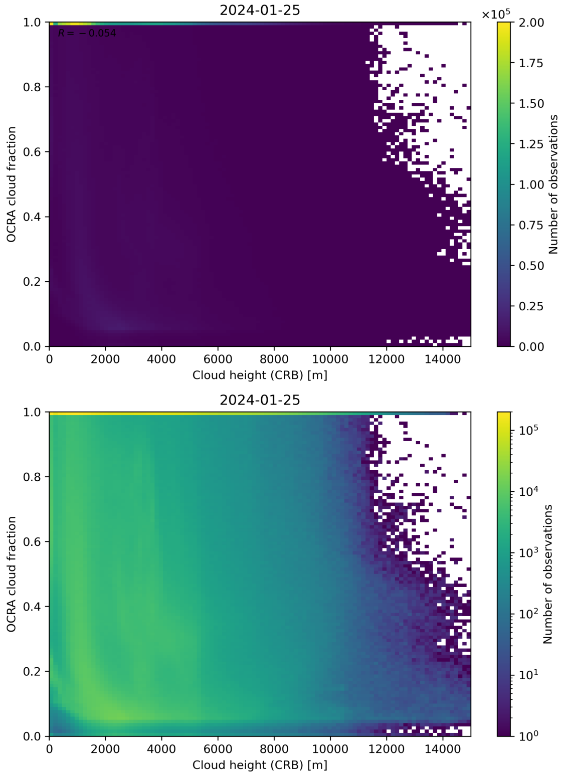
Figure 81: Scatter density plot of “Cloud height (CRB)” against “OCRA cloud fraction” for 2024-01-24 to 2024-01-26.
