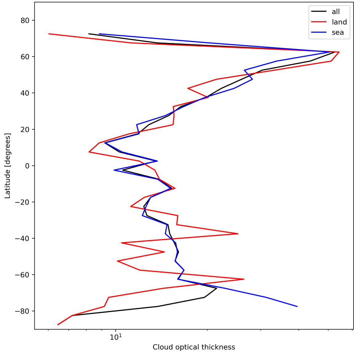
Figure 25: Zonal average of “Cloud optical thickness” for 2024-01-24 to 2024-01-26.
