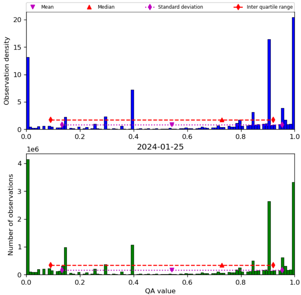
Figure 38: Histogram of “QA value” for 2024-01-24 to 2024-01-26
