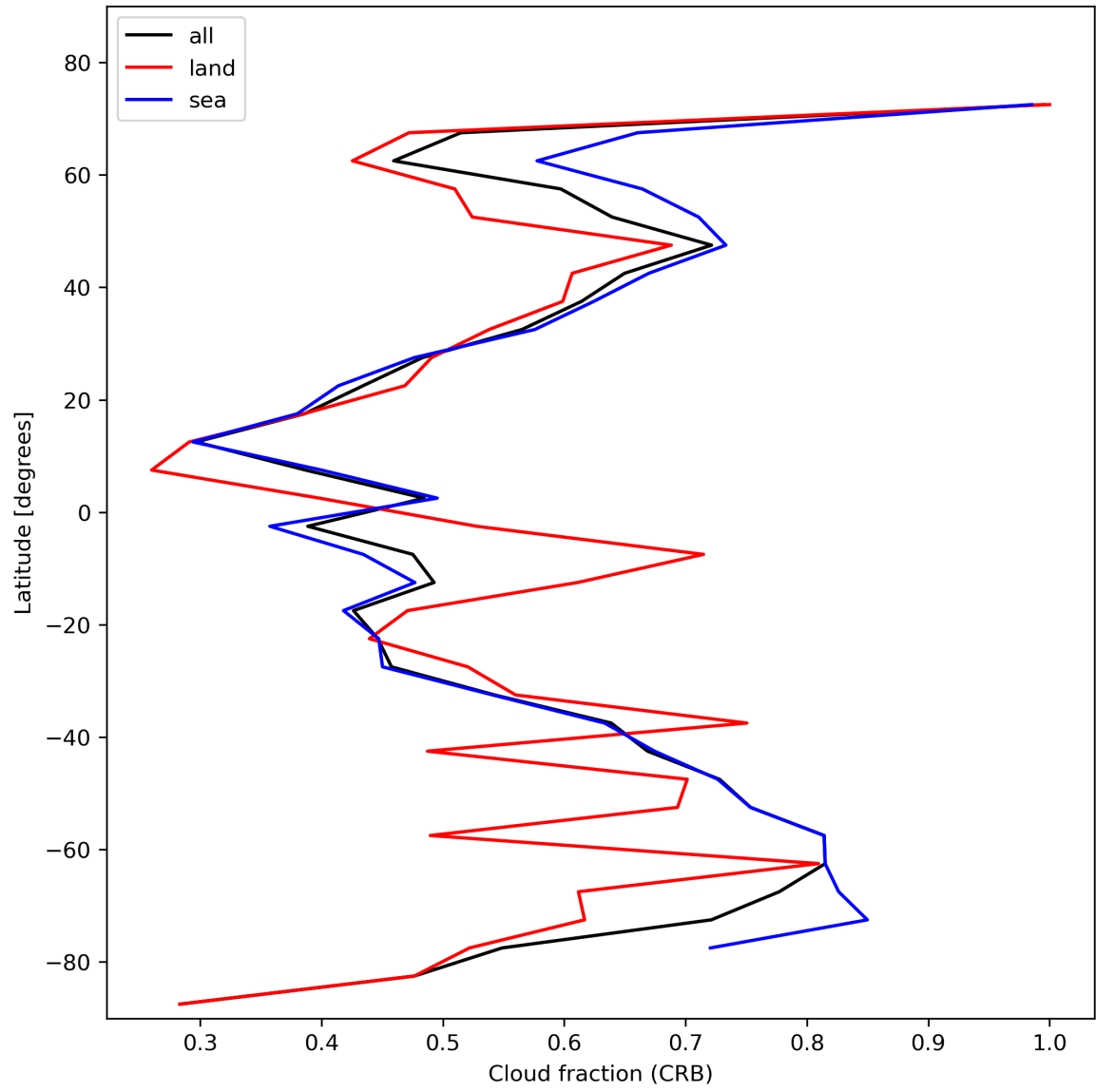
Figure 26: Zonal average of “Cloud fraction (CRB)” for 2024-01-24 to 2024-01-26.
