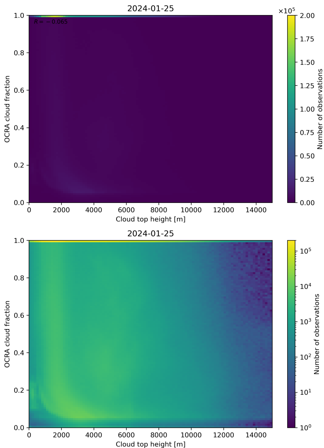
Figure 87: Scatter density plot of “Cloud top height” against “OCRA cloud fraction” for 2024-01-24 to 2024-01-26.
