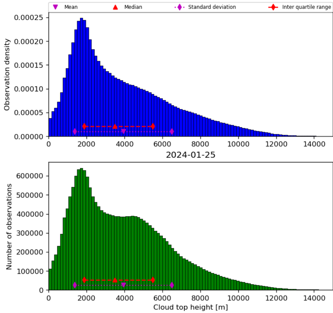
Figure 40: Histogram of “Cloud top height” for 2024-01-24 to 2024-01-26
