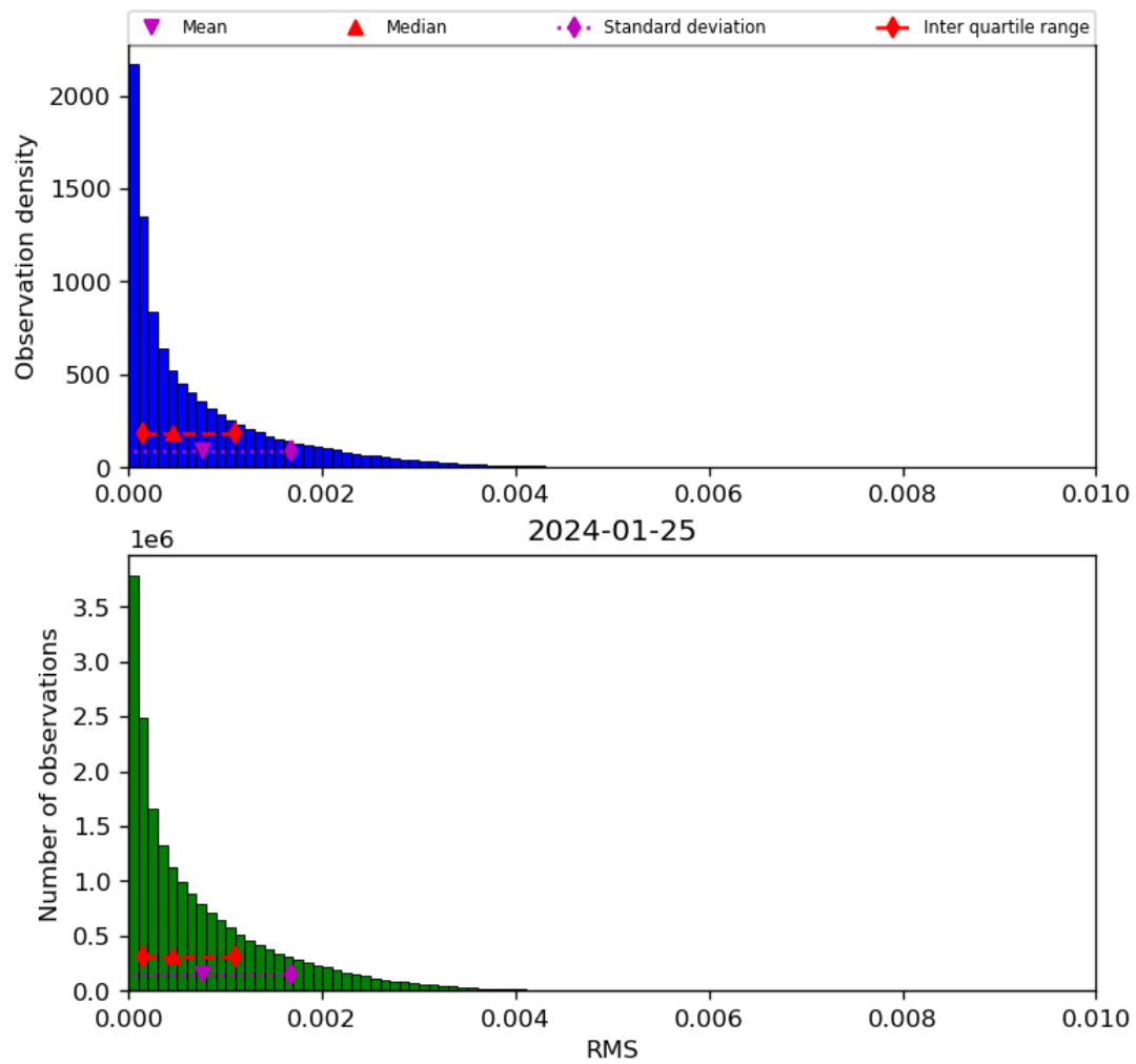
Figure 47: Histogram of “RMS” for 2024-01-24 to 2024-01-26
