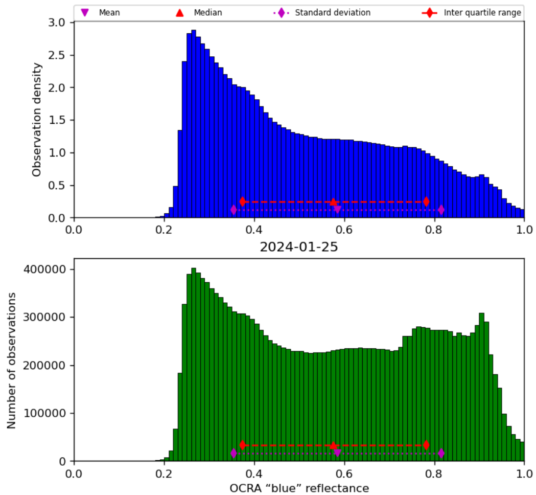
Figure 51: Histogram of “OCRA “blue” reflectance” for 2024-01-24 to 2024-01-26
