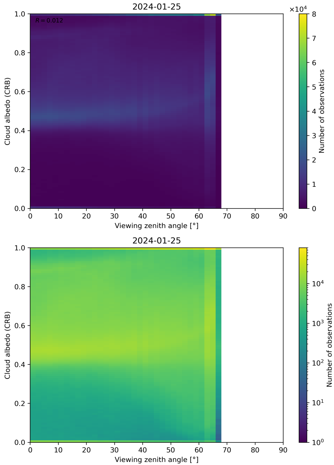
Figure 106: Scatter density plot of “Viewing zenith angle” against “Cloud albedo (CRB)” for 2024-01-24 to 2024-01-26.
