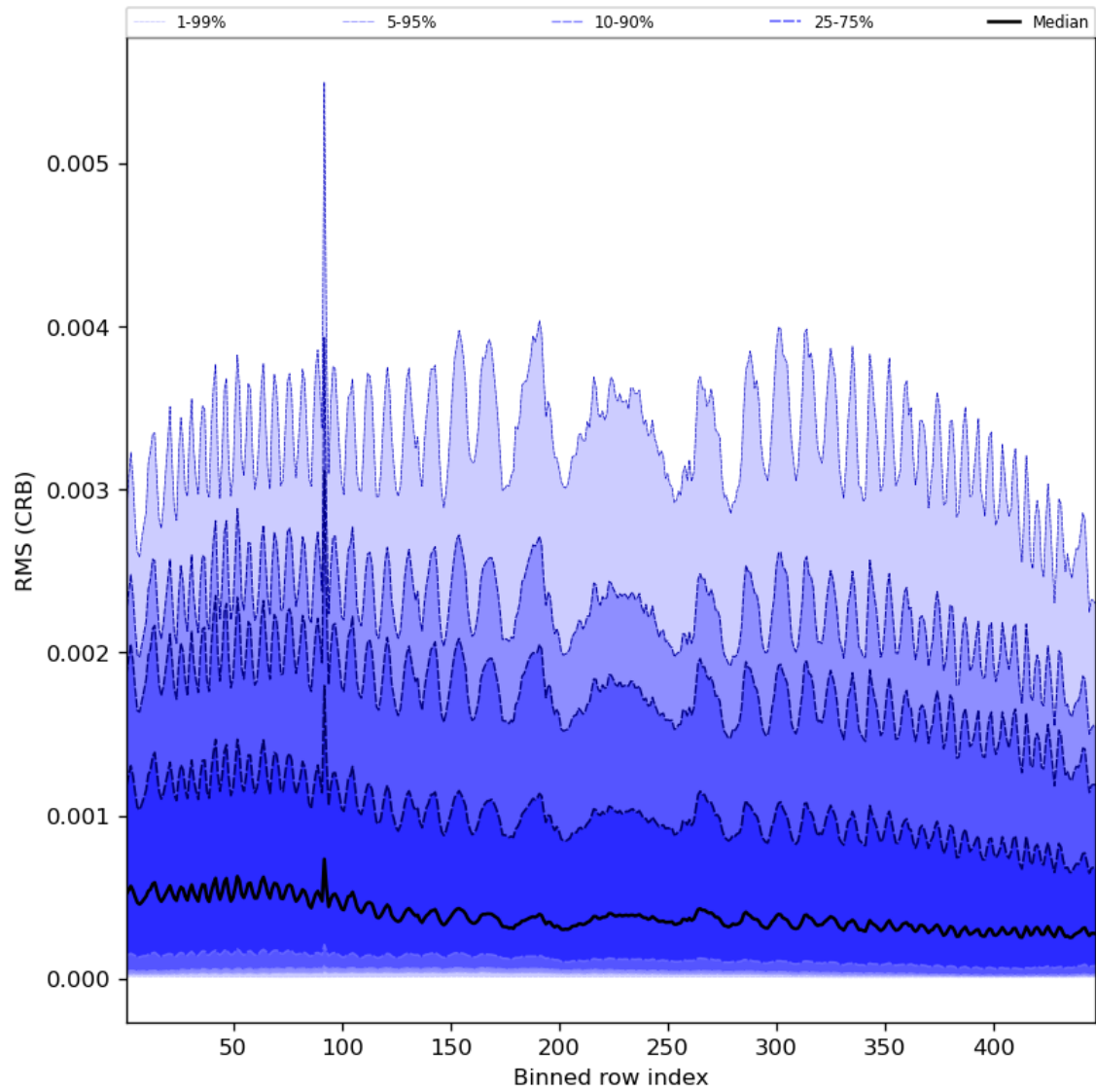
Figure 64: Along track statistics of “RMS (CRB)” for 2024-01-26 to 2024-01-28
