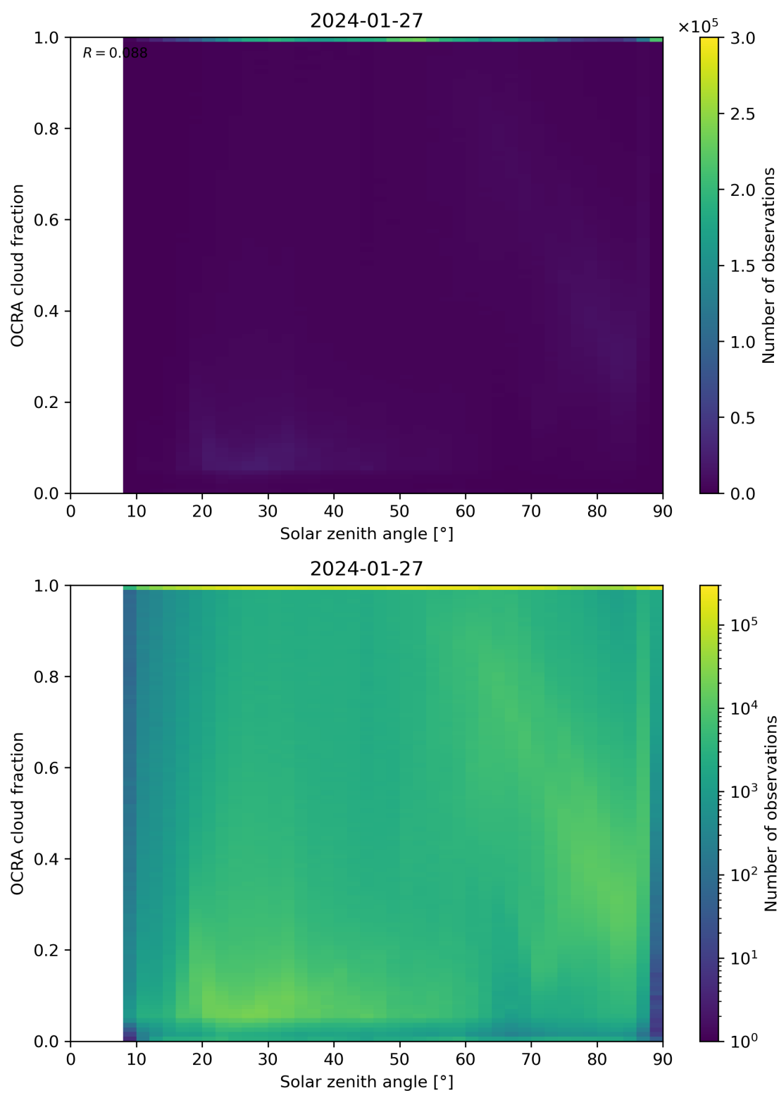
Figure 100: Scatter density plot of “Solar zenith angle” against “OCRA cloud fraction” for 2024-01-26 to 2024-01-28.
