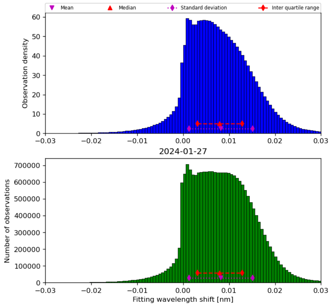
Figure 49: Histogram of “Fitting wavelength shift” for 2024-01-26 to 2024-01-28
