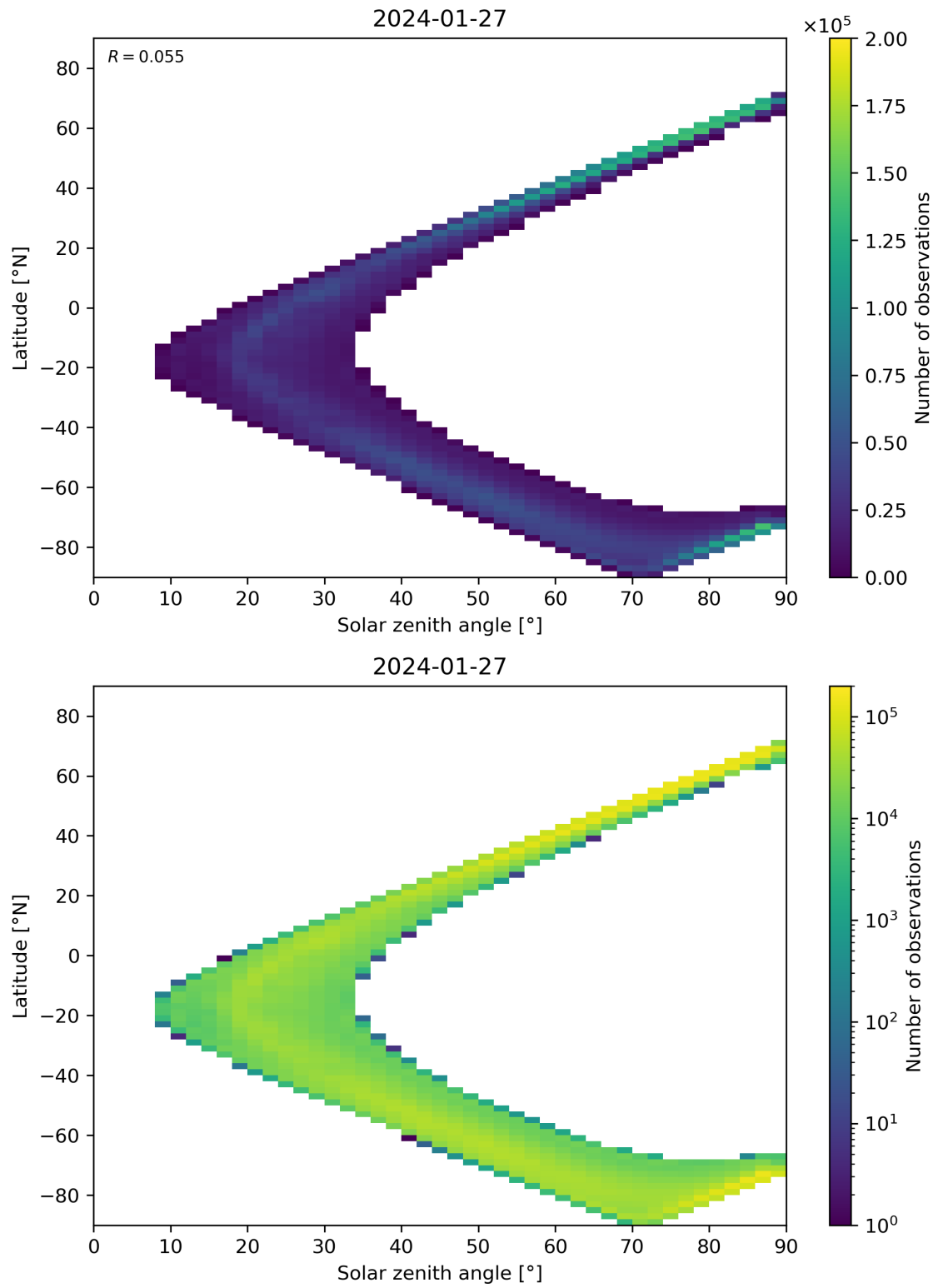
Figure 105: Scatter density plot of “Solar zenith angle” against “Latitude” for 2024-01-26 to 2024-01-28.
