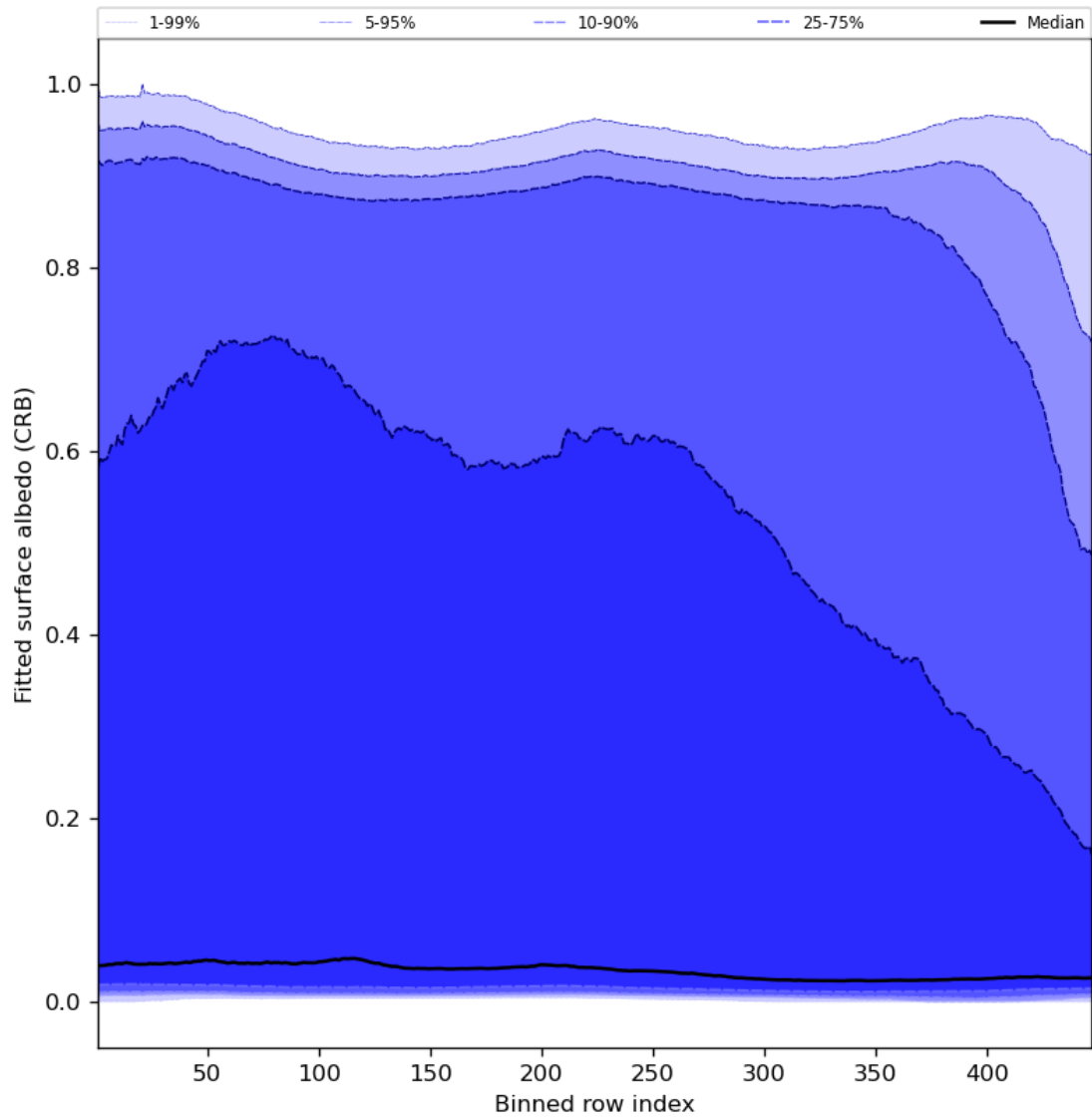
Figure 62: Along track statistics of “Fitted surface albedo (CRB)” for 2024-01-26 to 2024-01-28
