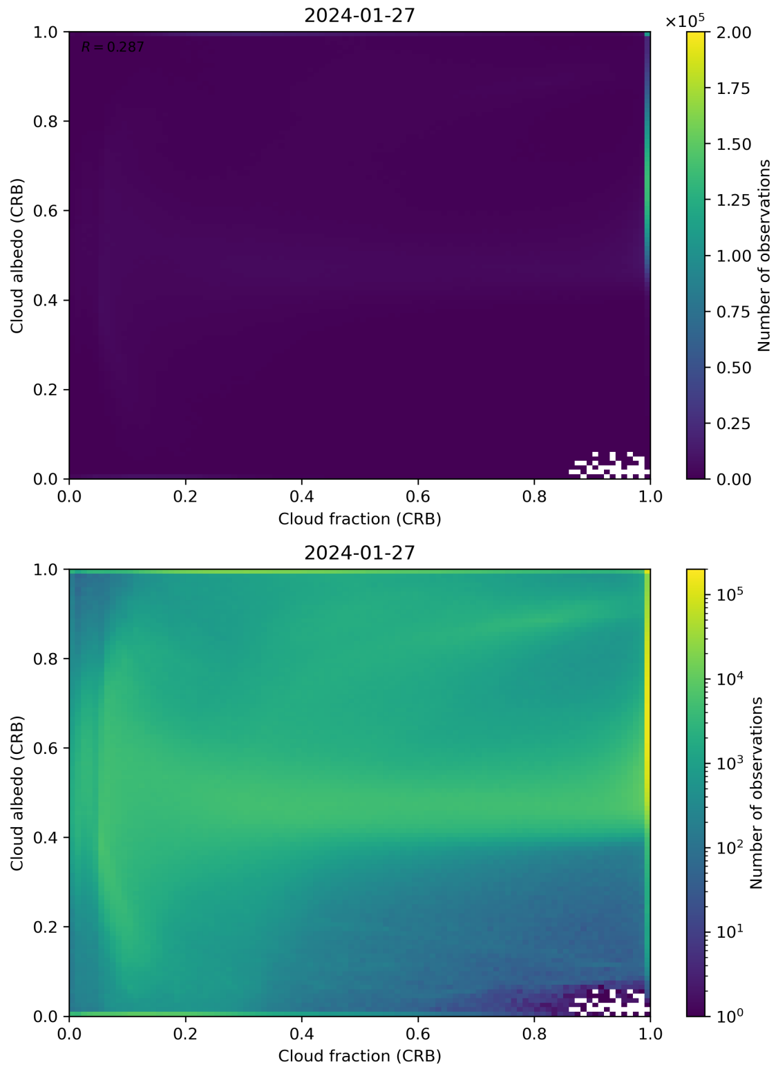
Figure 77: Scatter density plot of “Cloud fraction (CRB)” against “Cloud albedo (CRB)” for 2024-01-26 to 2024-01-28.
