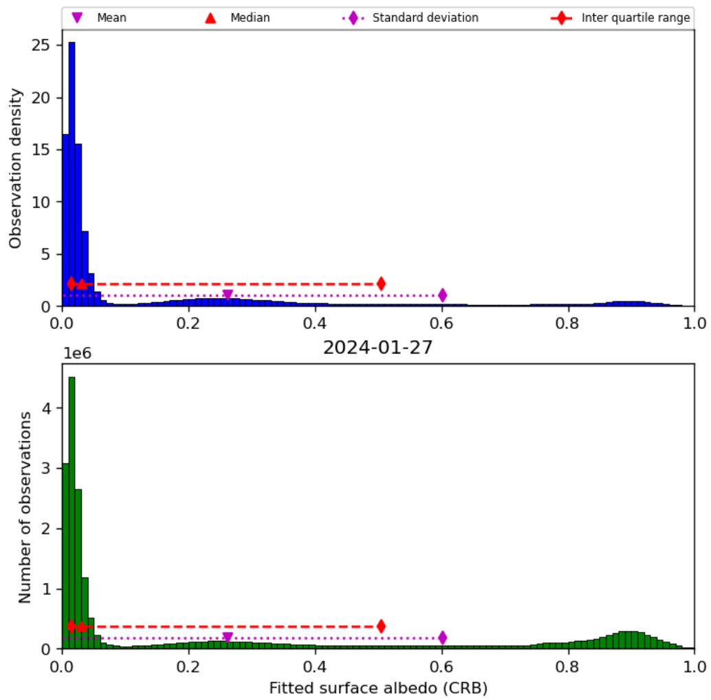
Figure 46: Histogram of “Fitted surface albedo (CRB)” for 2024-01-26 to 2024-01-28
