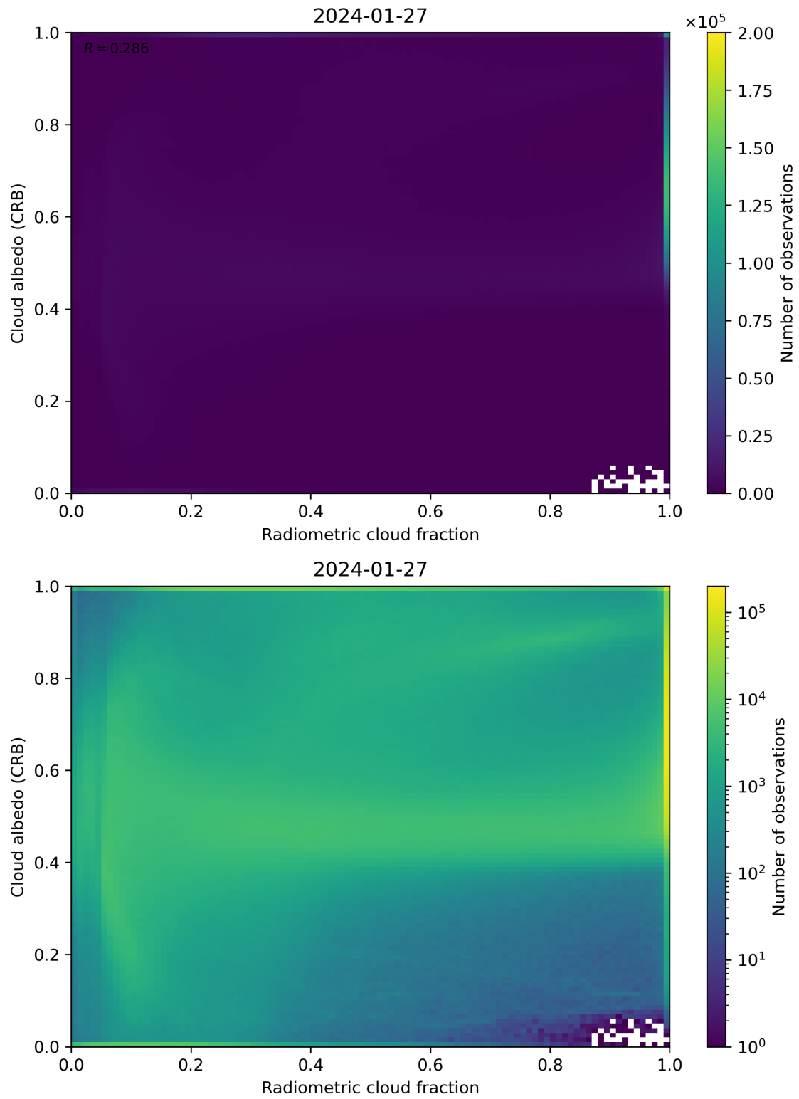
Figure 71: Scatter density plot of “Radiometric cloud fraction” against “Cloud albedo (CRB)” for 2024-01-26 to 2024-01-28.
