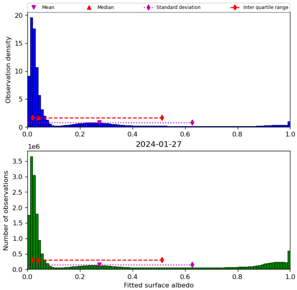
Figure 45: Histogram of “Fitted surface albedo” for 2024-01-26 to 2024-01-28
