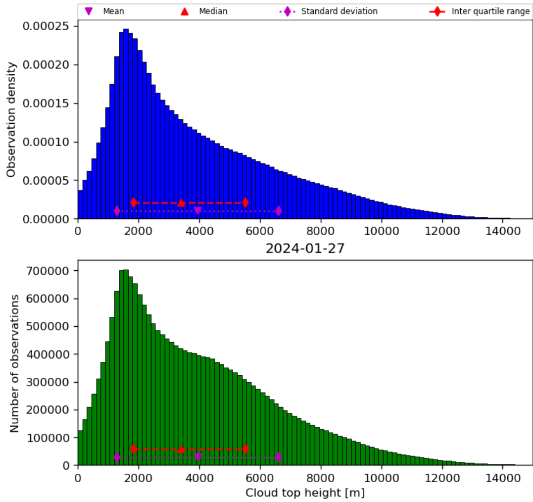
Figure 40: Histogram of “Cloud top height” for 2024-01-26 to 2024-01-28
