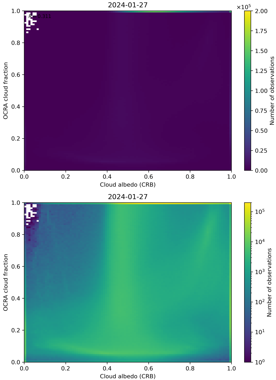
Figure 70: Scatter density plot of “Cloud albedo (CRB)” against “OCRA cloud fraction” for 2024-01-26 to 2024-01-28.
