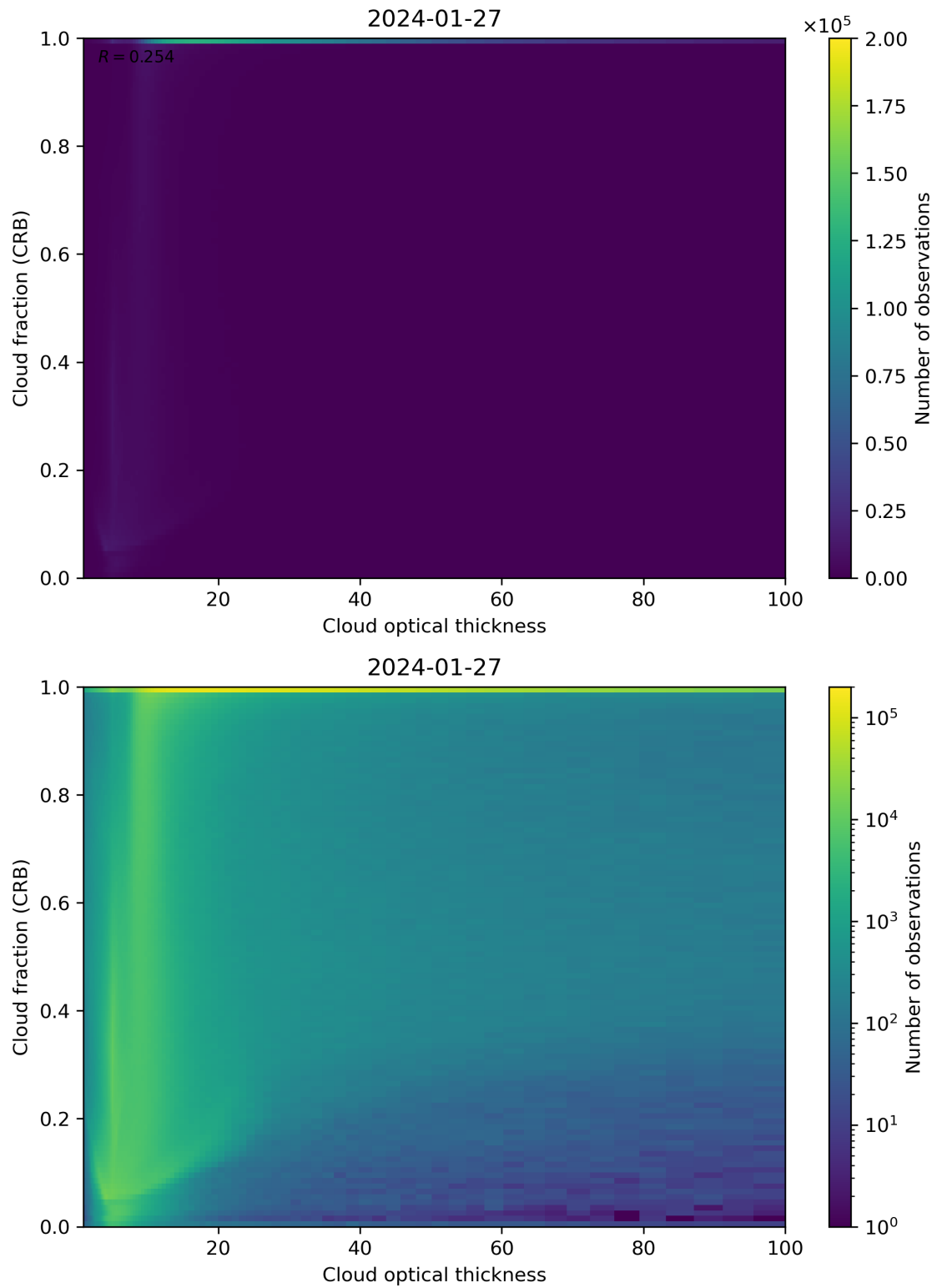
Figure 84: Scatter density plot of “Cloud optical thickness” against “Cloud fraction (CRB)” for 2024-01-26 to 2024-01-28.
