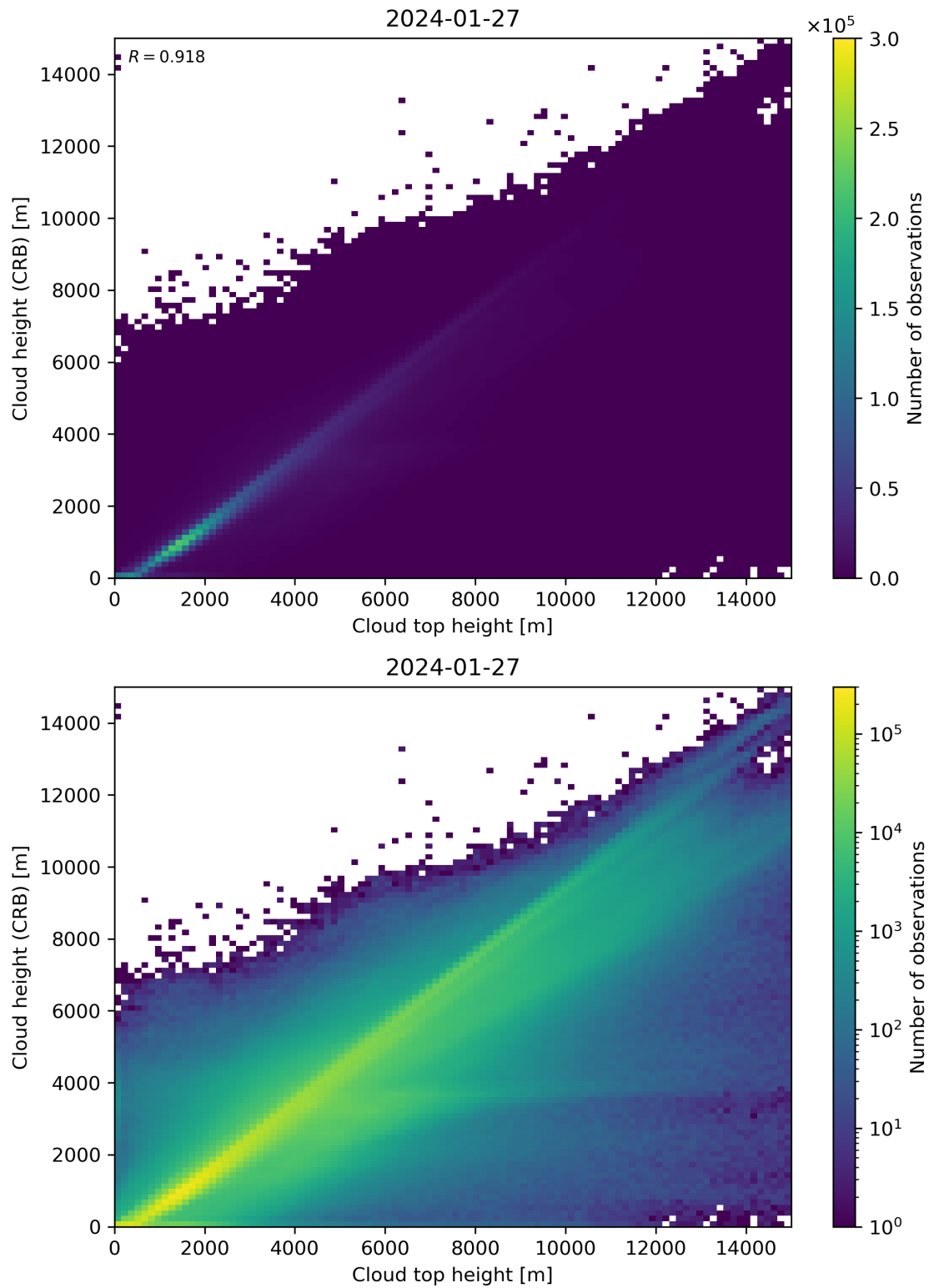
Figure 89: Scatter density plot of “Cloud top height” against “Cloud height (CRB)” for 2024-01-26 to 2024-01-28.
