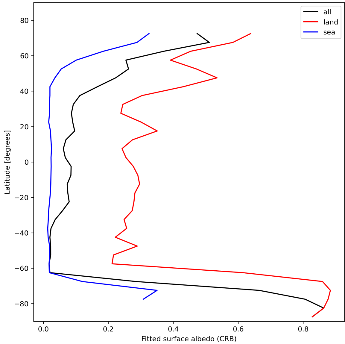
Figure 30: Zonal average of “Fitted surface albedo (CRB)” for 2024-01-26 to 2024-01-28.
