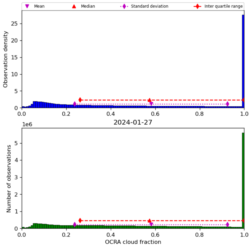
Figure 50: Histogram of “OCRA cloud fraction” for 2024-01-26 to 2024-01-28
