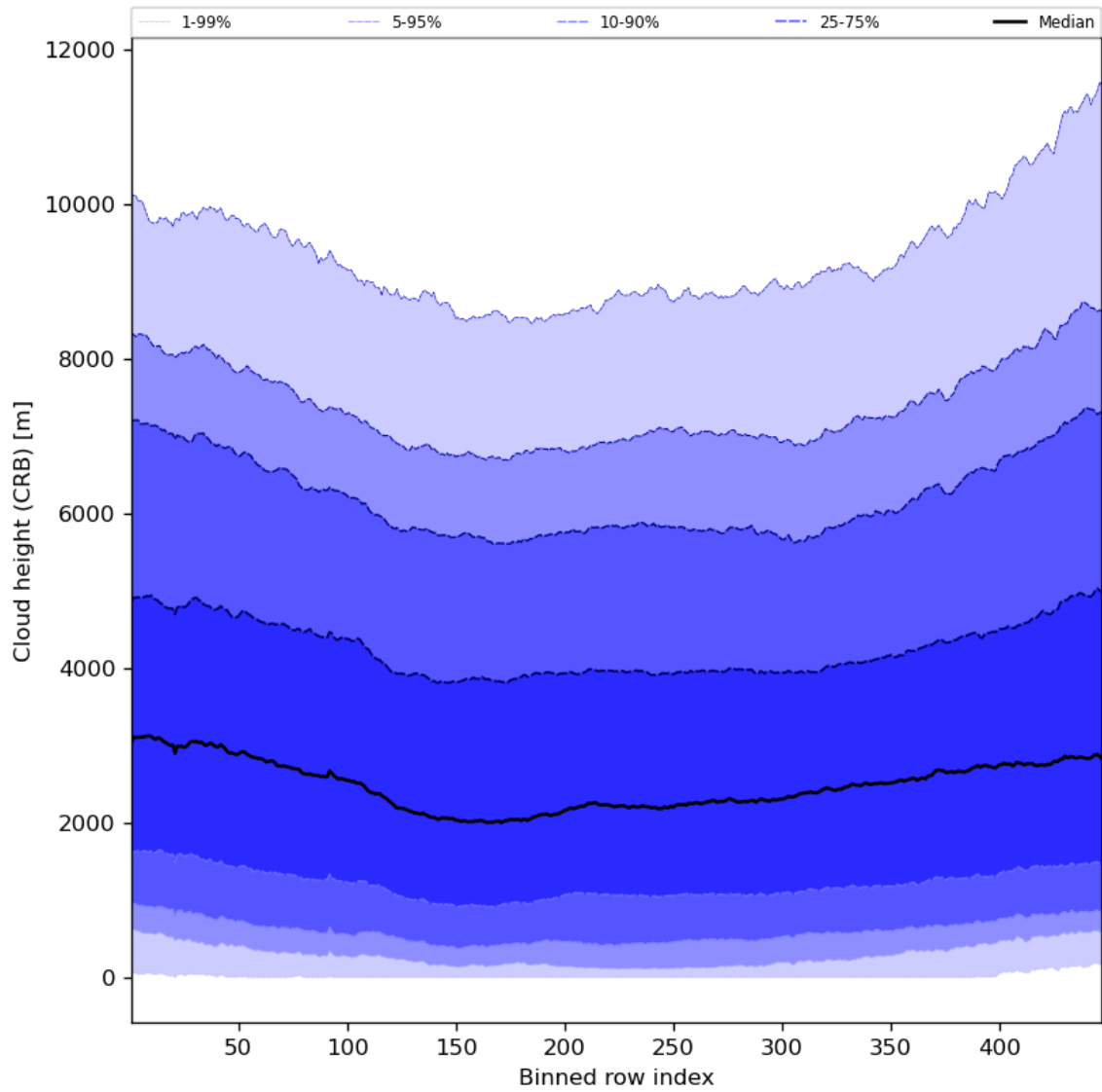
Figure 59: Along track statistics of “Cloud height (CRB)” for 2024-01-26 to 2024-01-28
