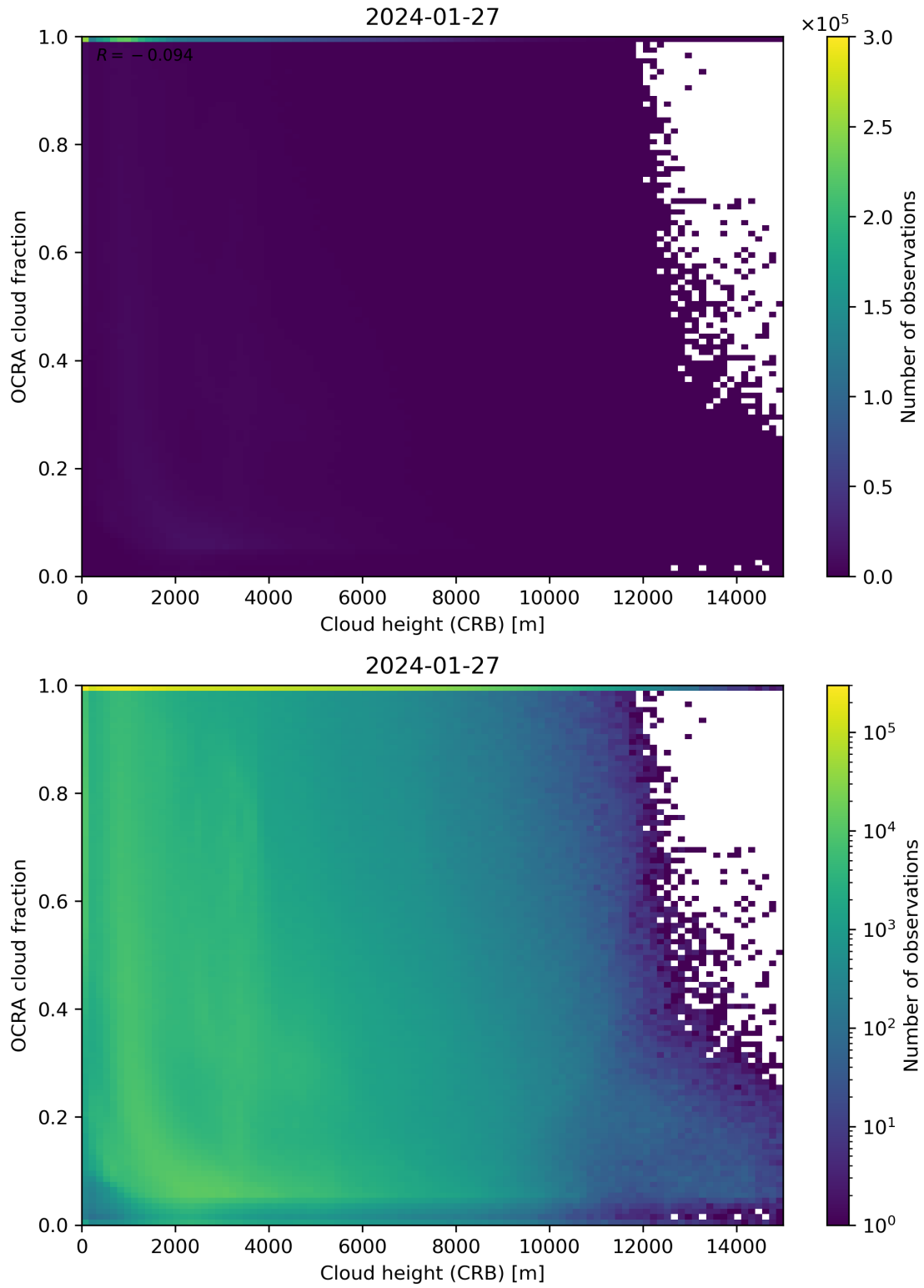
Figure 81: Scatter density plot of “Cloud height (CRB)” against “OCRA cloud fraction” for 2024-01-26 to 2024-01-28.
