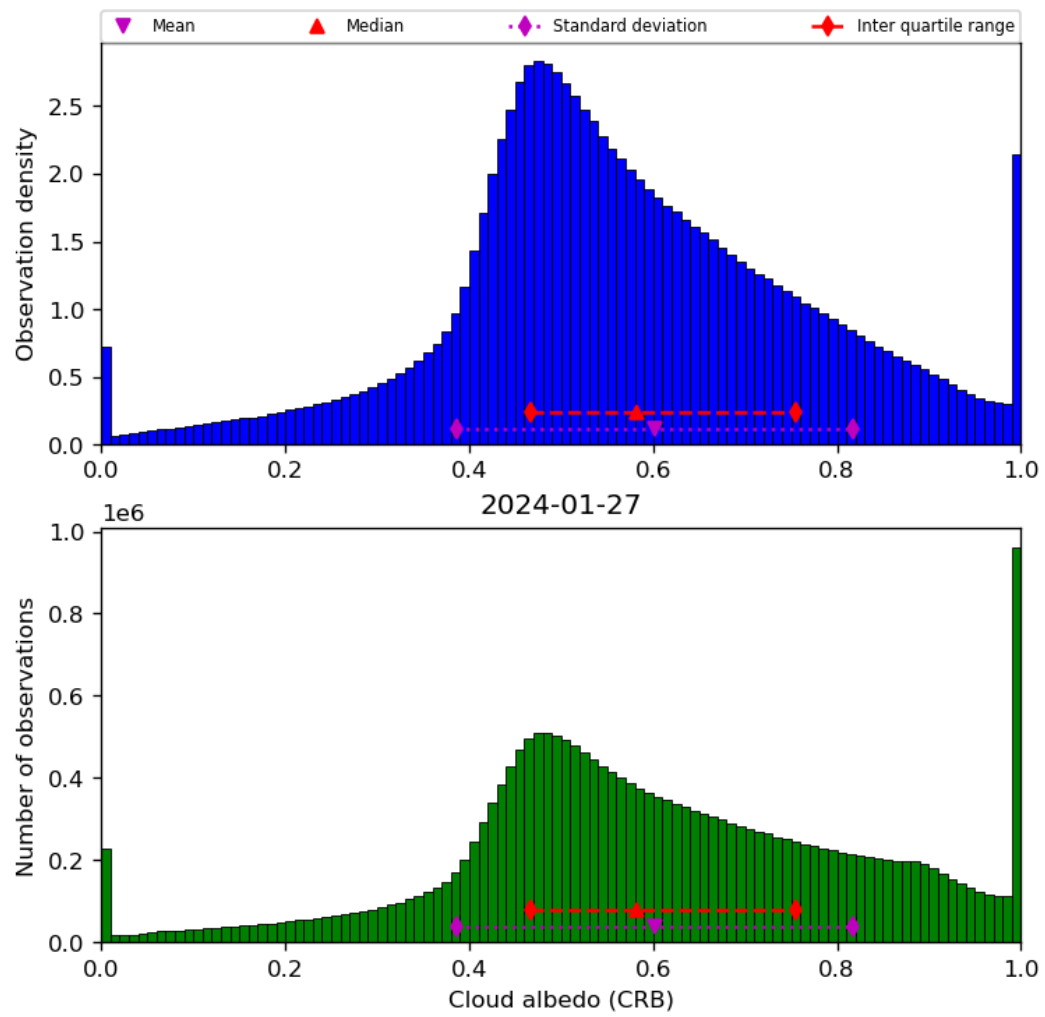
Figure 44: Histogram of “Cloud albedo (CRB)” for 2024-01-26 to 2024-01-28
