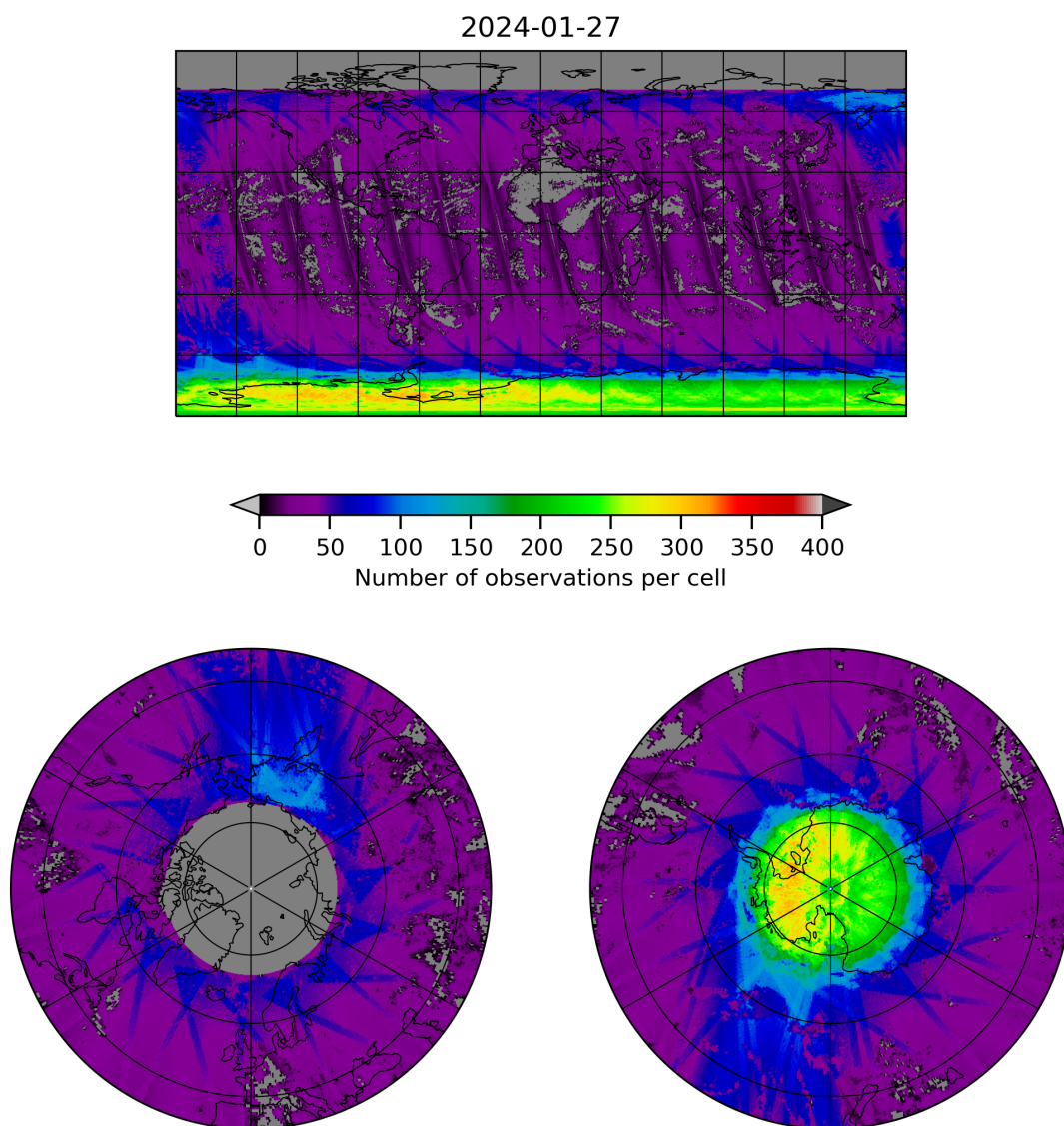
Figure 21: Map of the number of observations for 2024-01-26 to 2024-01-28
