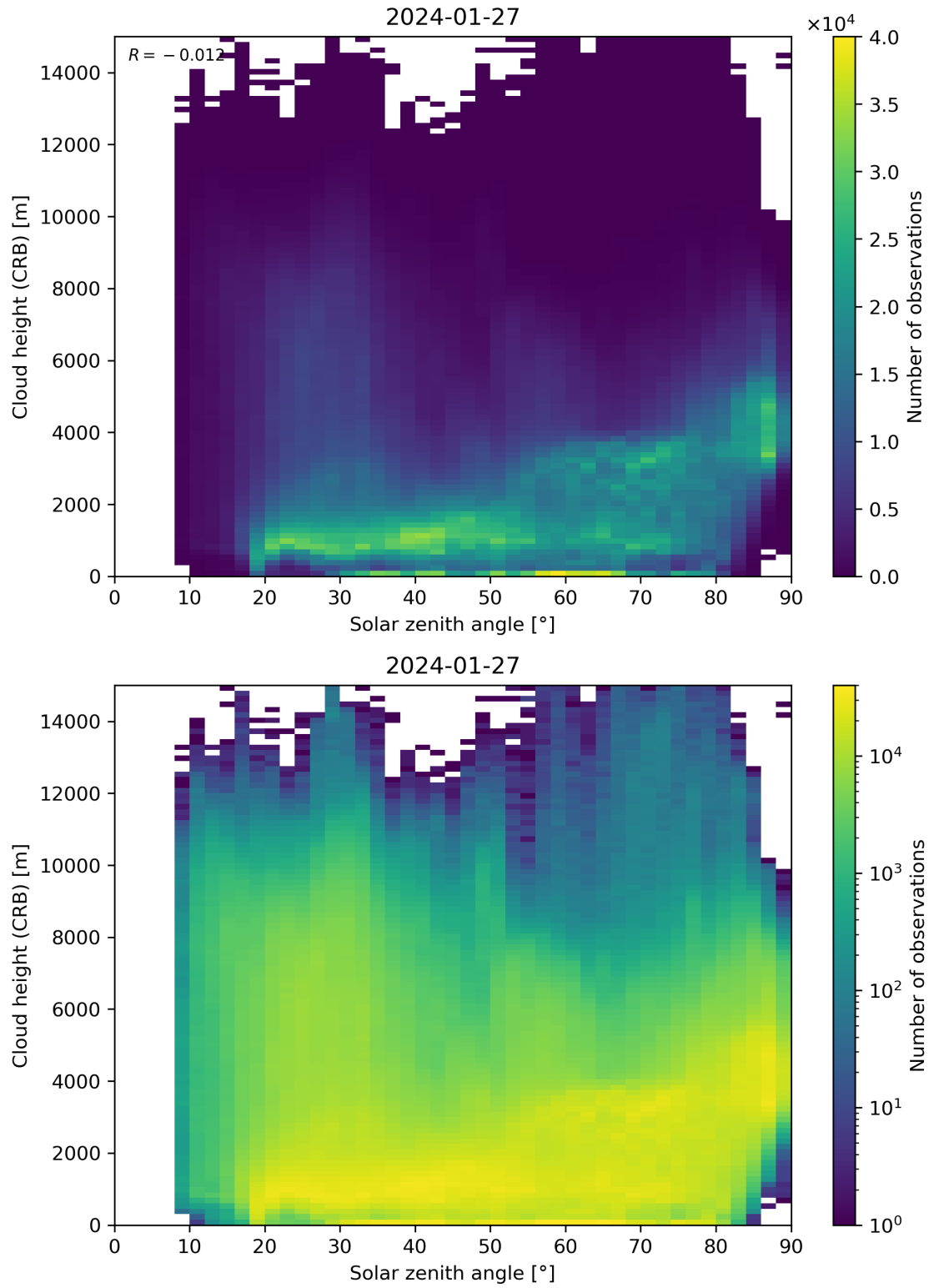
Figure 102: Scatter density plot of “Solar zenith angle” against “Cloud height (CRB)” for 2024-01-26 to 2024-01-28.
