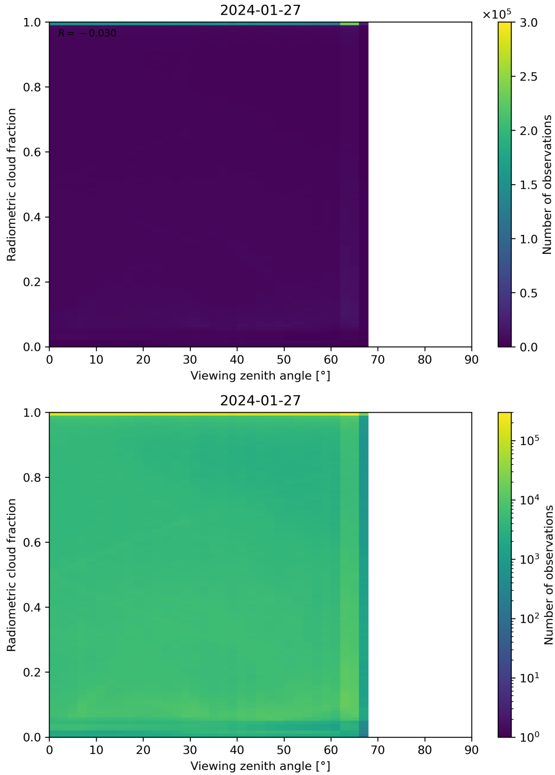
Figure 107: Scatter density plot of “Viewing zenith angle” against “Radiometric cloud fraction” for 2024-01-26 to 2024-01-28.
