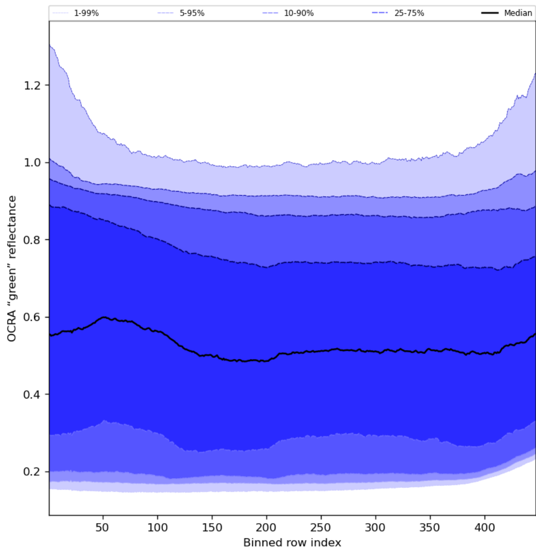
Figure 68: Along track statistics of “OCRA “green” reflectance” for 2024-01-26 to 2024-01-28
