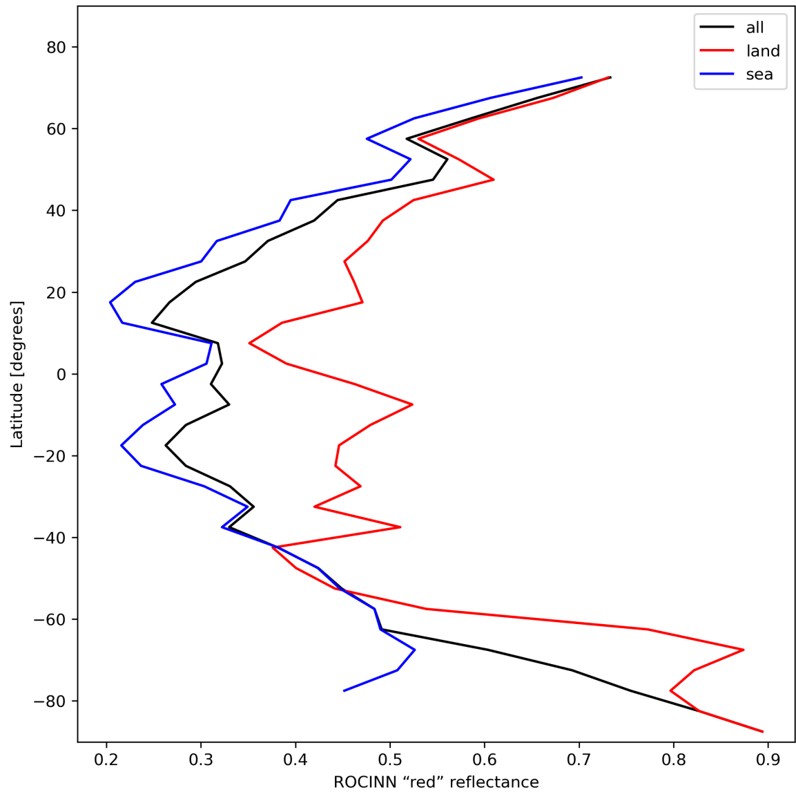
Figure 37: Zonal average of “ROCINN “red” reflectance” for 2024-01-26 to 2024-01-28.
