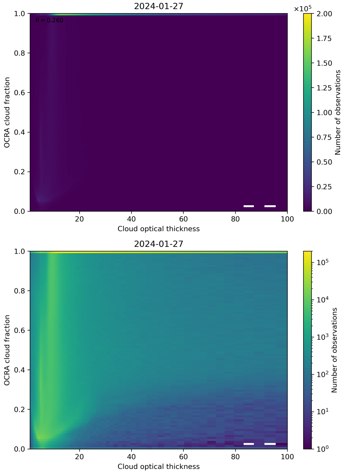
Figure 83: Scatter density plot of “Cloud optical thickness” against “OCRA cloud fraction” for 2024-01-26 to 2024-01-28.
