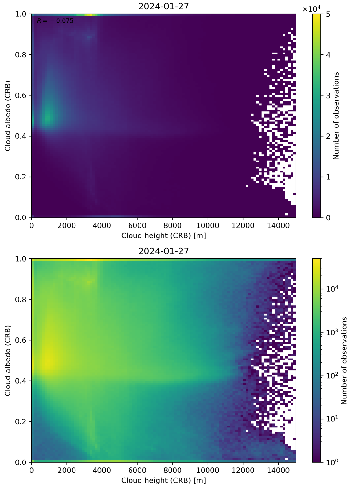
Figure 80: Scatter density plot of “Cloud height (CRB)” against “Cloud albedo (CRB)” for 2024-01-26 to 2024-01-28.
