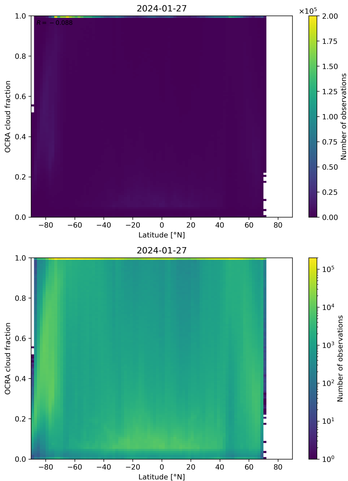
Figure 93: Scatter density plot of “Latitude” against “OCRA cloud fraction” for 2024-01-26 to 2024-01-28.
