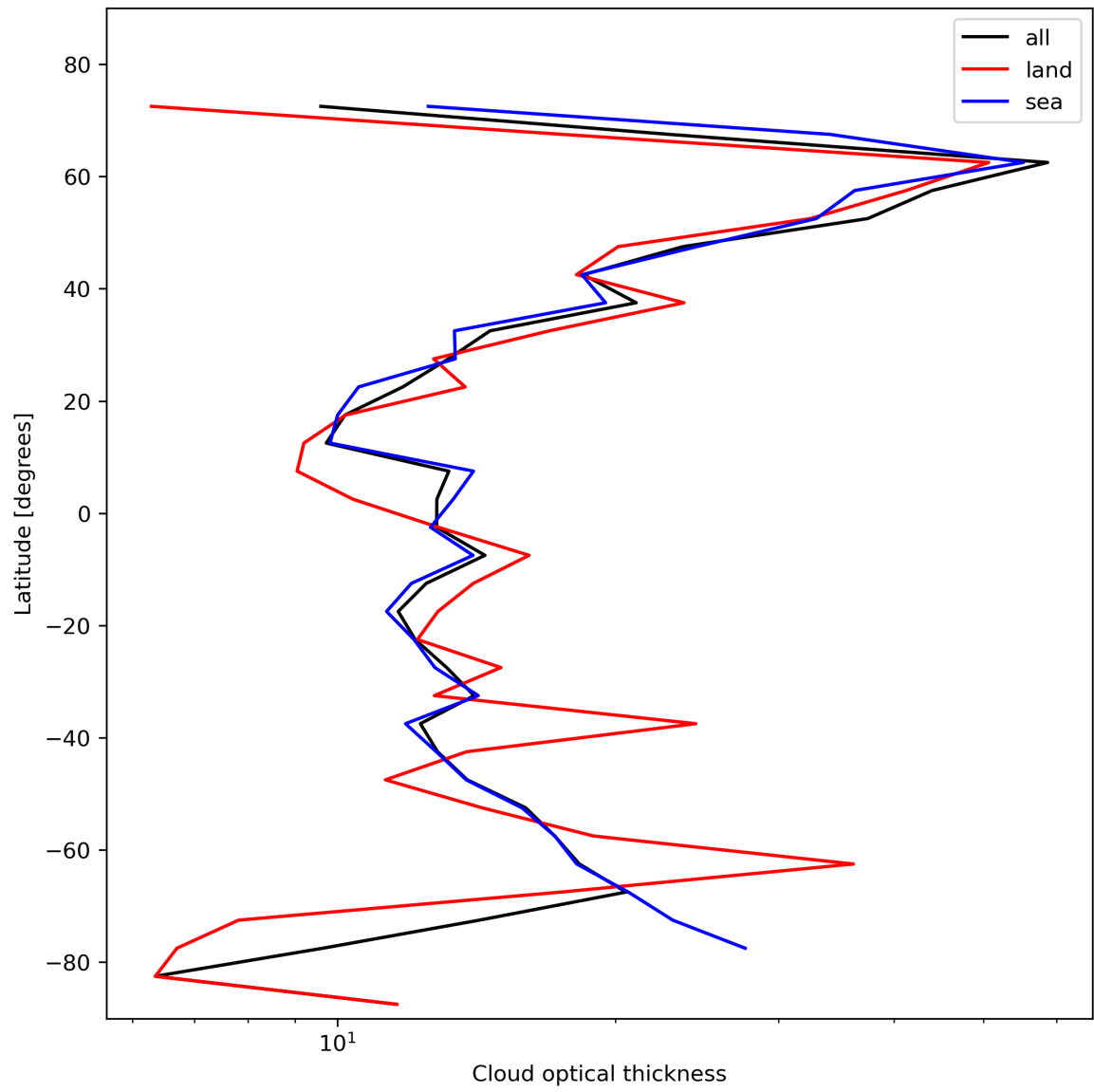
Figure 25: Zonal average of “Cloud optical thickness” for 2024-01-26 to 2024-01-28.
