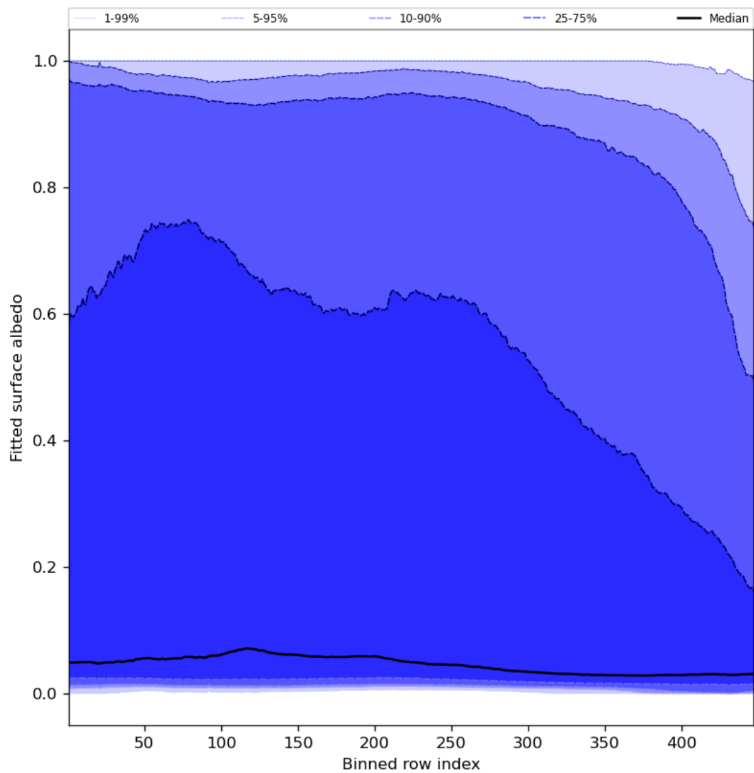
Figure 61: Along track statistics of “Fitted surface albedo” for 2024-01-26 to 2024-01-28
