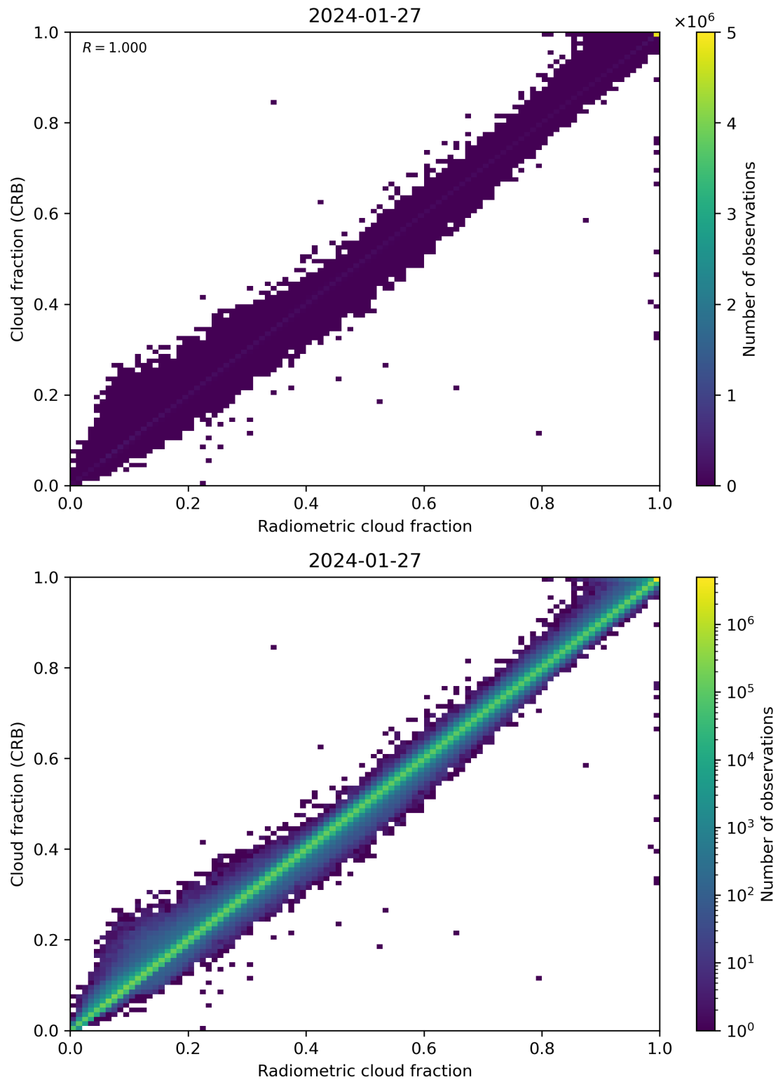
Figure 73: Scatter density plot of “Radiometric cloud fraction” against “Cloud fraction (CRB)” for 2024-01-26 to 2024-01-28.
