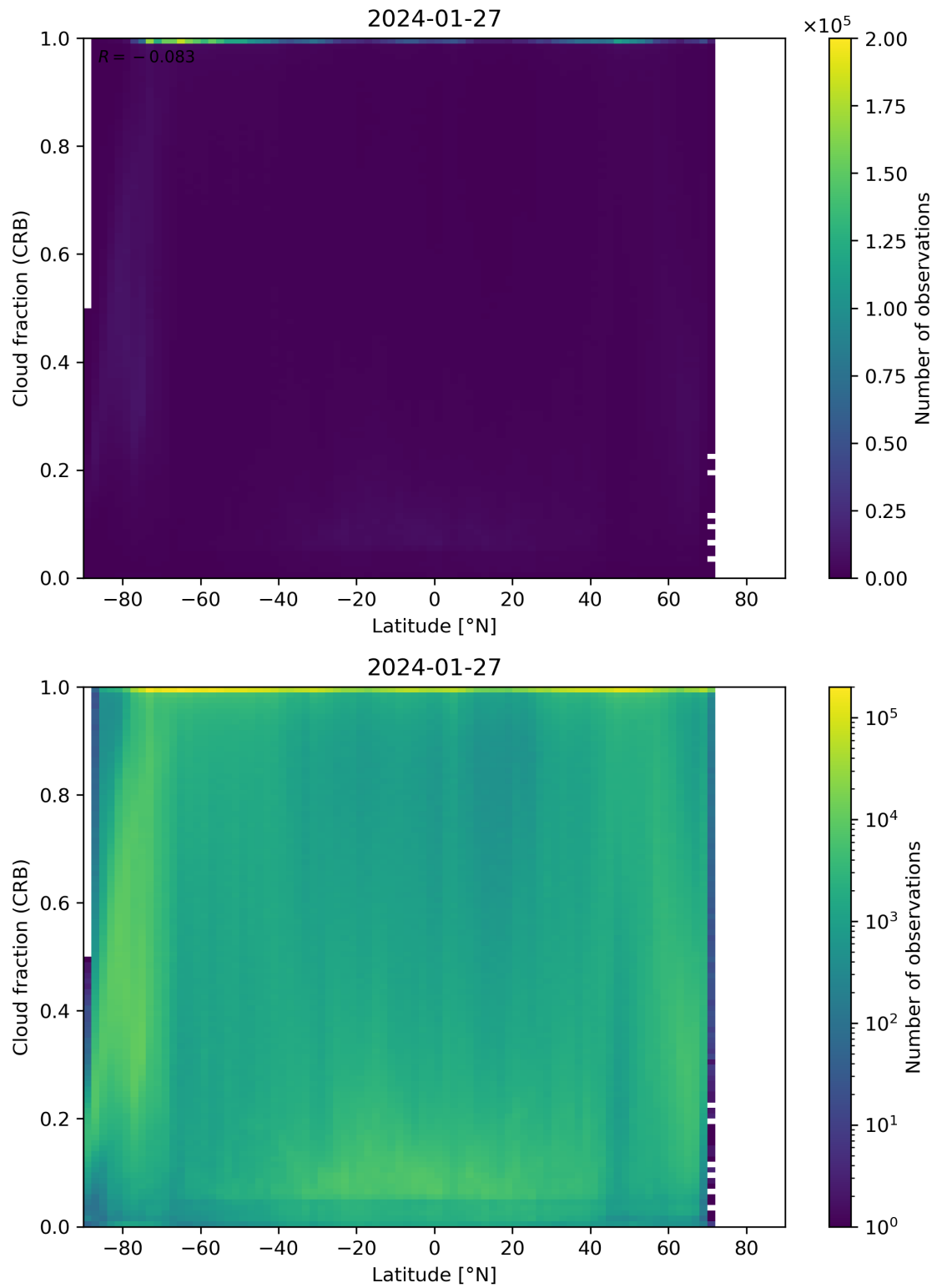
Figure 94: Scatter density plot of “Latitude” against “Cloud fraction (CRB)” for 2024-01-26 to 2024-01-28.
