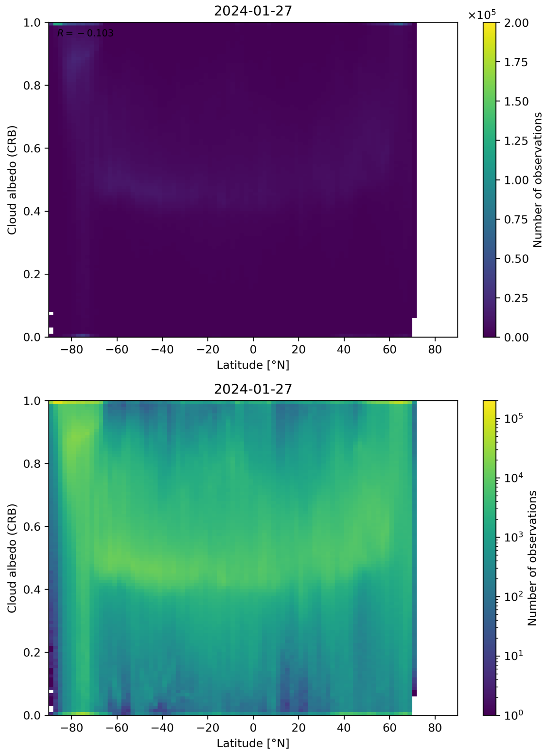
Figure 91: Scatter density plot of “Latitude” against “Cloud albedo (CRB)” for 2024-01-26 to 2024-01-28.
