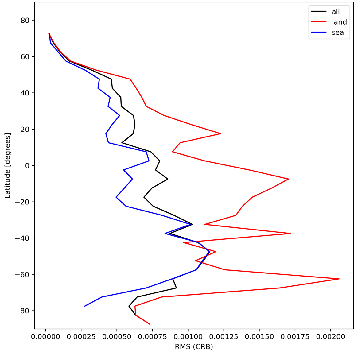
Figure 32: Zonal average of “RMS (CRB)” for 2024-01-26 to 2024-01-28.
