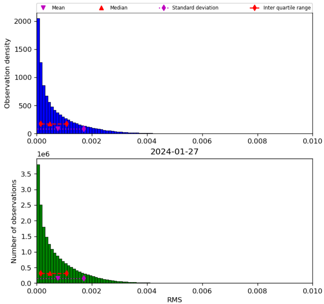
Figure 47: Histogram of “RMS” for 2024-01-26 to 2024-01-28
