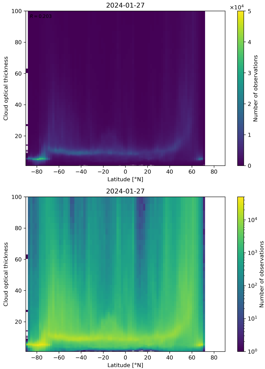
Figure 96: Scatter density plot of “Latitude” against “Cloud optical thickness” for 2024-01-26 to 2024-01-28.
