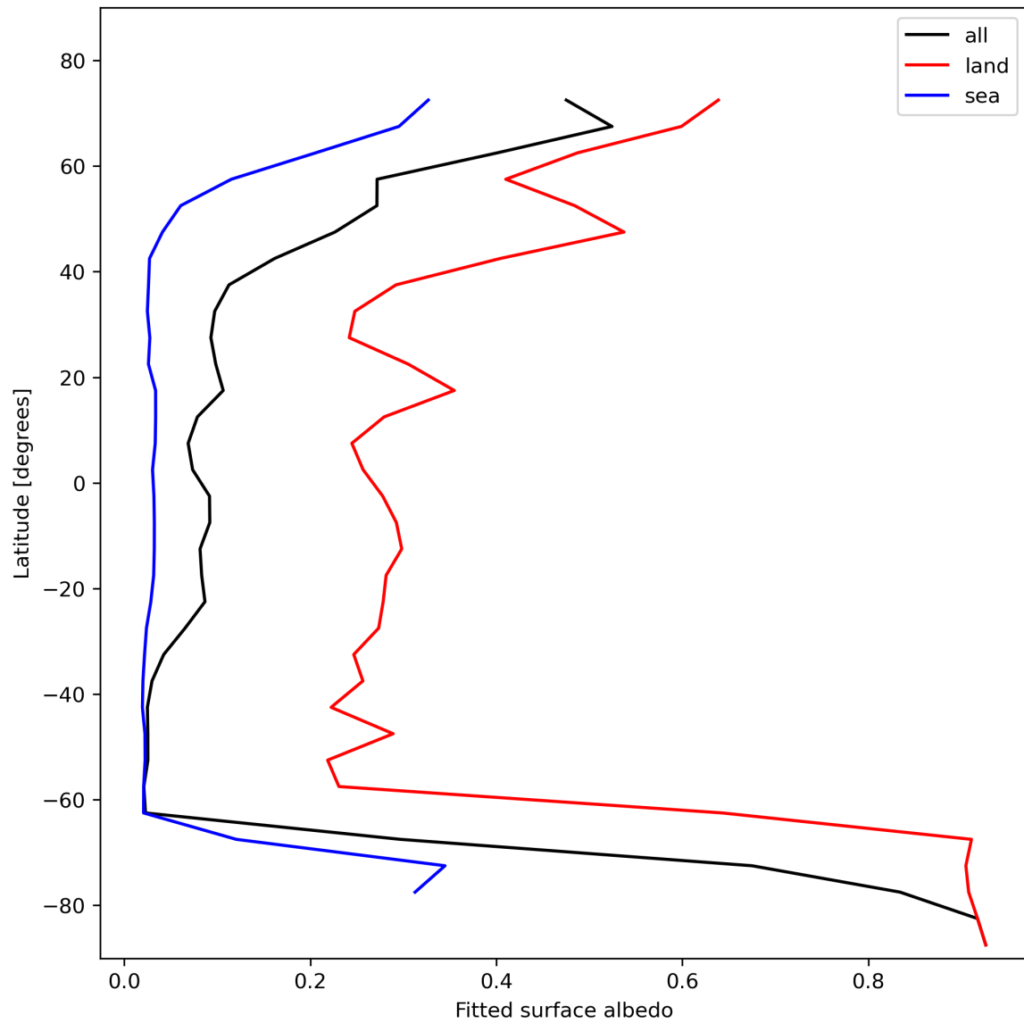
Figure 29: Zonal average of “Fitted surface albedo” for 2024-01-26 to 2024-01-28.
