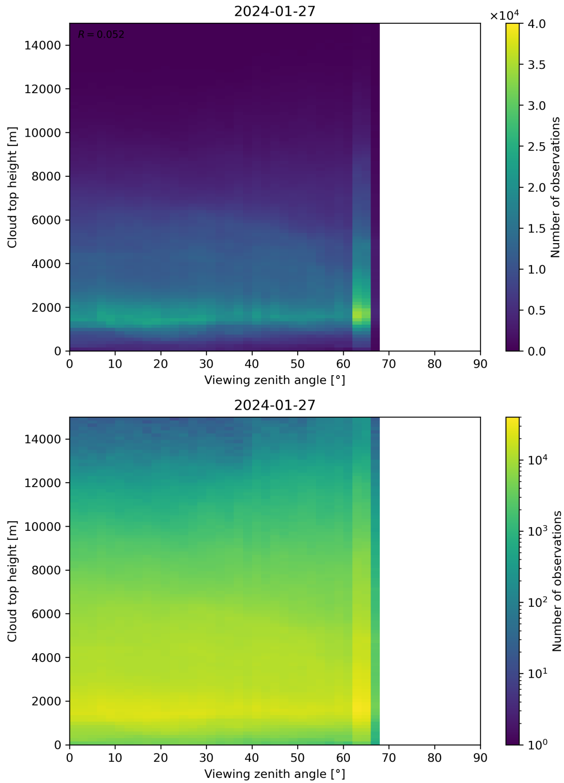
Figure 112: Scatter density plot of “Viewing zenith angle” against “Cloud top height” for 2024-01-26 to 2024-01-28.
