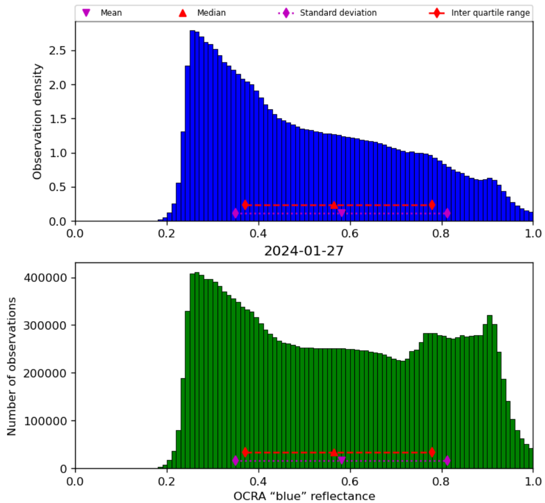
Figure 51: Histogram of “OCRA “blue” reflectance” for 2024-01-26 to 2024-01-28
