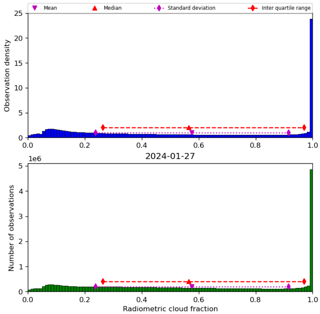
Figure 39: Histogram of “Radiometric cloud fraction” for 2024-01-26 to 2024-01-28
