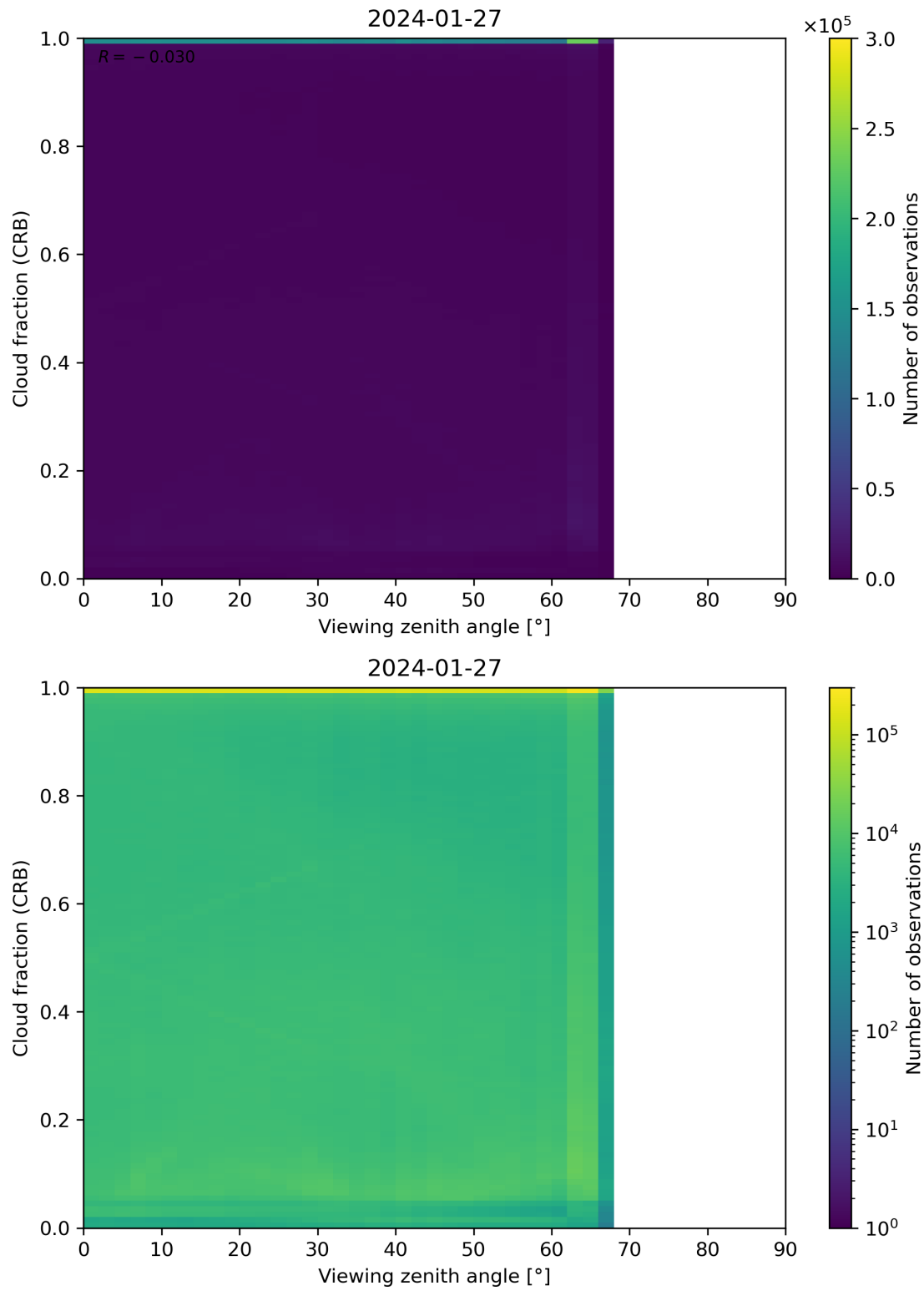
Figure 109: Scatter density plot of “Viewing zenith angle” against “Cloud fraction (CRB)” for 2024-01-26 to 2024-01-28.
