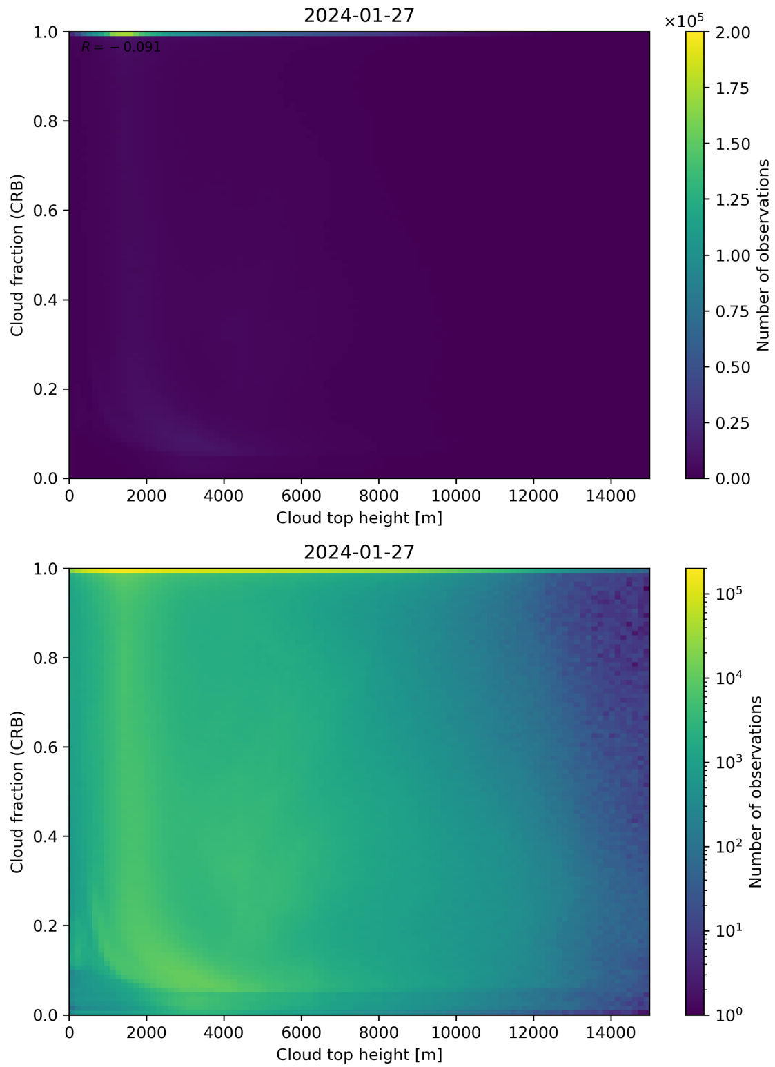
Figure 88: Scatter density plot of “Cloud top height” against “Cloud fraction (CRB)” for 2024-01-26 to 2024-01-28.
