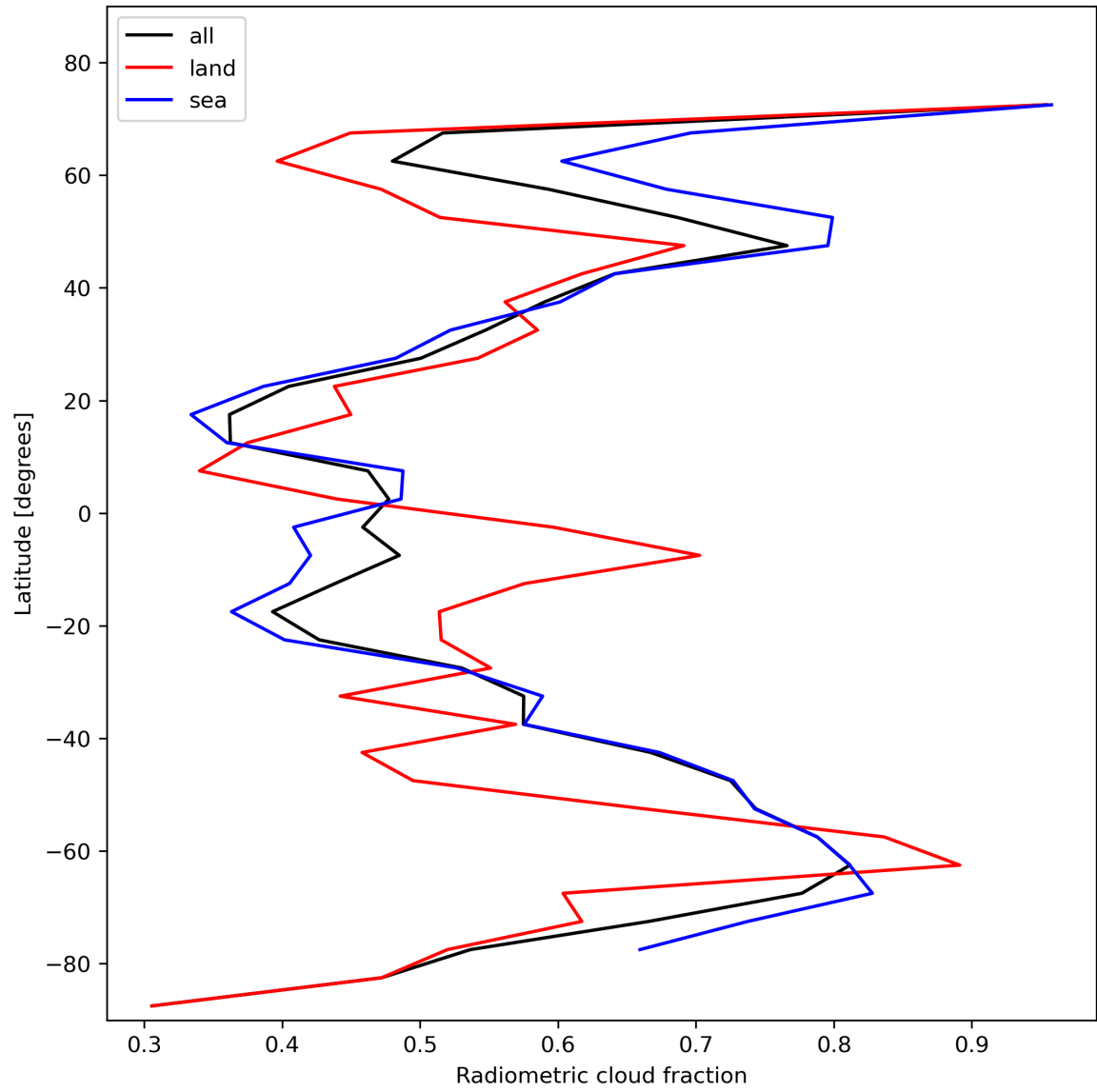
Figure 23: Zonal average of “Radiometric cloud fraction” for 2024-01-26 to 2024-01-28.
