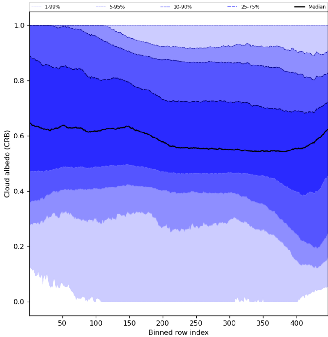
Figure 60: Along track statistics of “Cloud albedo (CRB)” for 2024-01-26 to 2024-01-28
