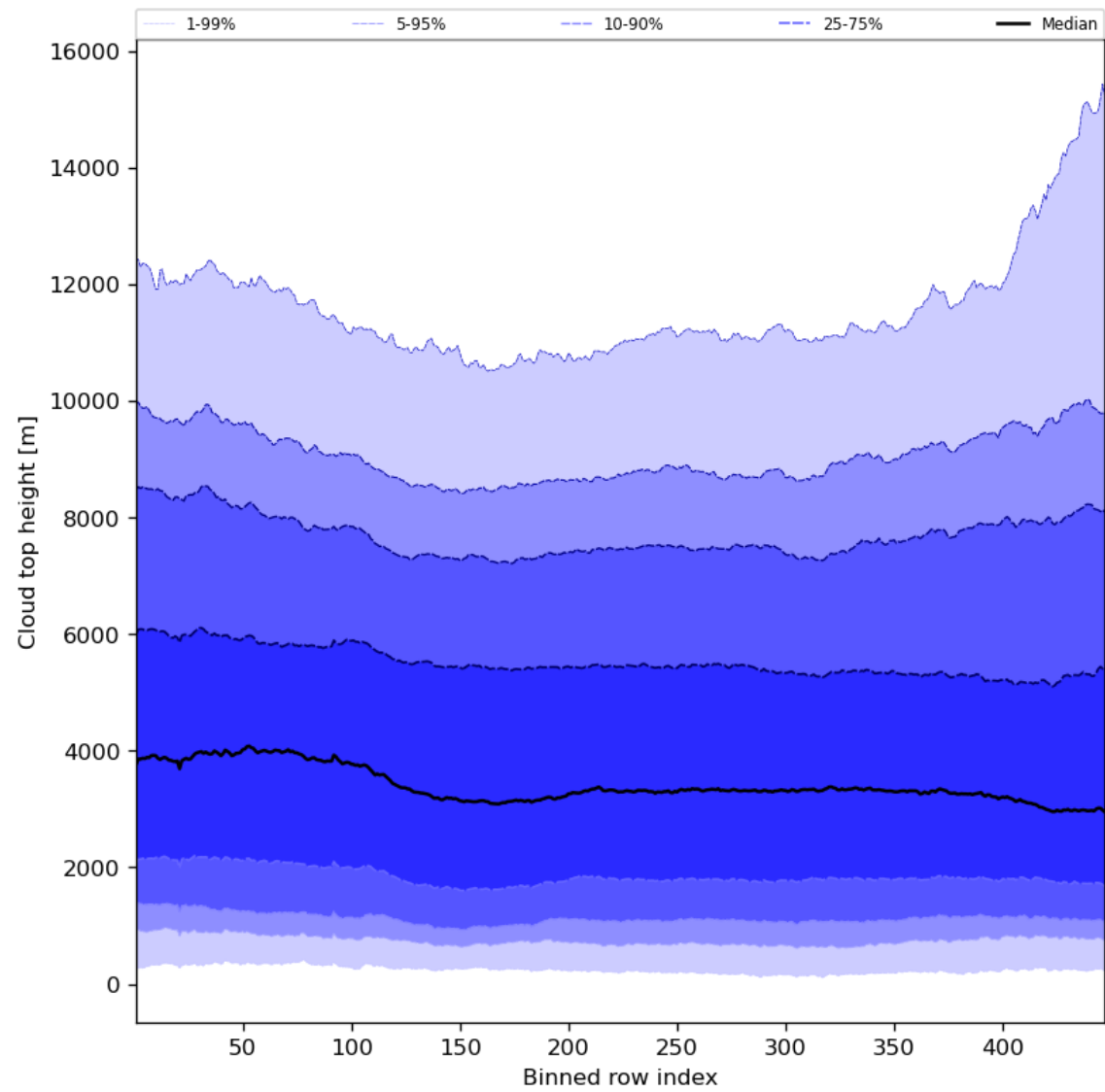
Figure 56: Along track statistics of “Cloud top height” for 2024-01-26 to 2024-01-28
