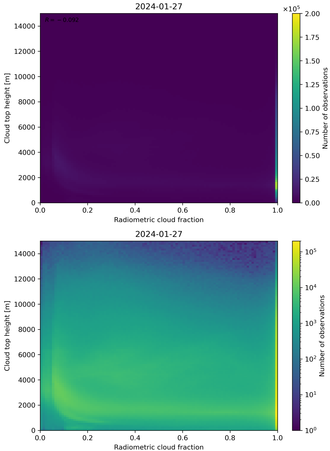
Figure 76: Scatter density plot of “Radiometric cloud fraction” against “Cloud top height” for 2024-01-26 to 2024-01-28.
