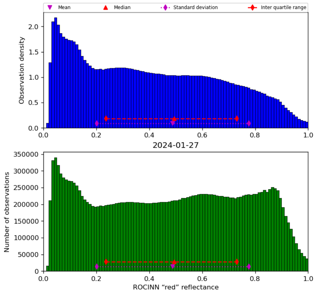
Figure 53: Histogram of “ROCINN “red” reflectance” for 2024-01-26 to 2024-01-28
