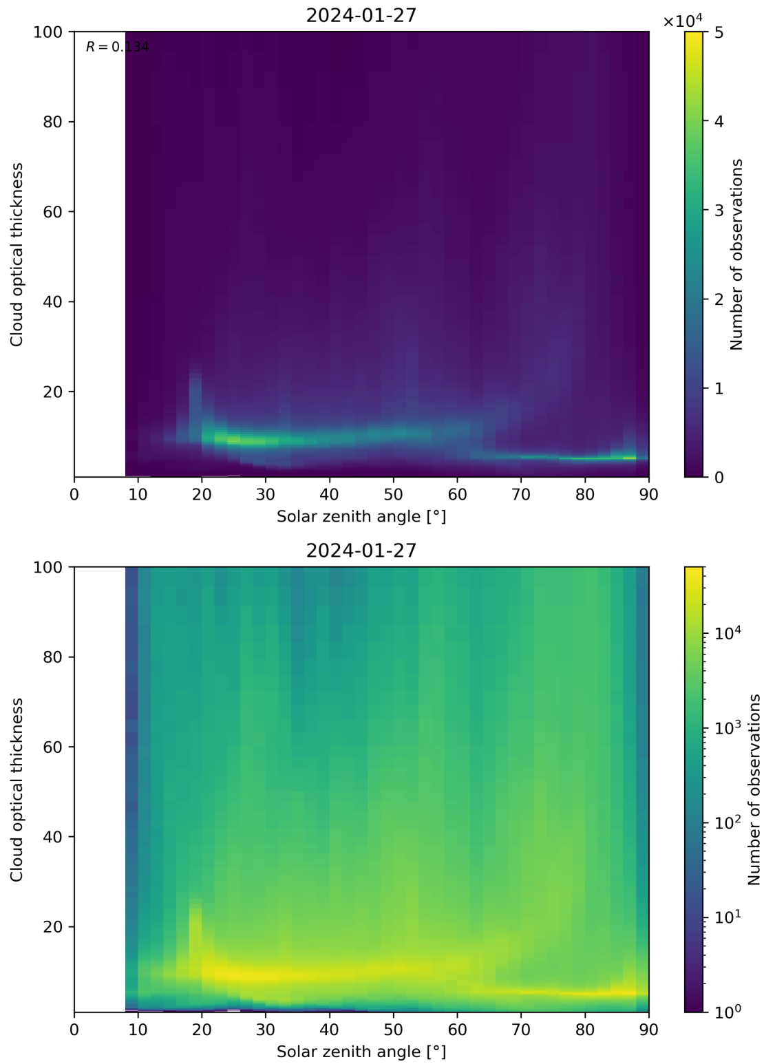
Figure 103: Scatter density plot of “Solar zenith angle” against “Cloud optical thickness” for 2024-01-26 to 2024-01-28.
