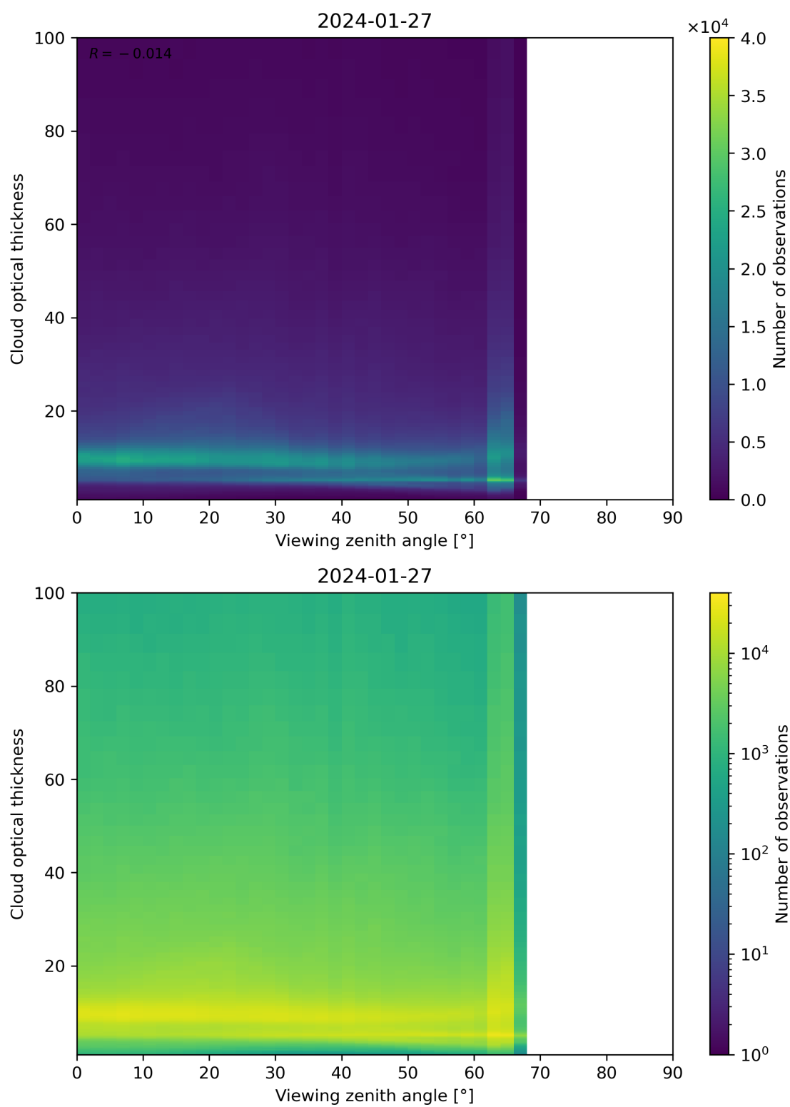
Figure 111: Scatter density plot of “Viewing zenith angle” against “Cloud optical thickness” for 2024-01-26 to 2024-01-28.
