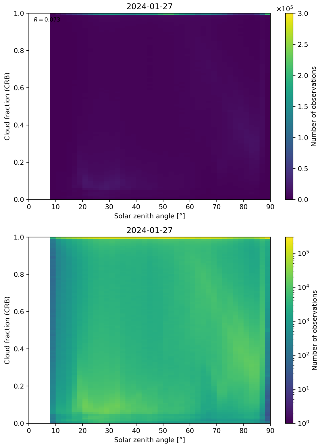
Figure 101: Scatter density plot of “Solar zenith angle” against “Cloud fraction (CRB)” for 2024-01-26 to 2024-01-28.
