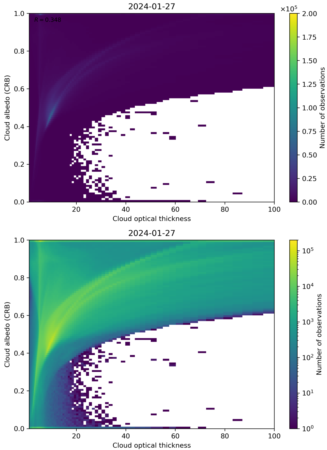
Figure 82: Scatter density plot of “Cloud optical thickness” against “Cloud albedo (CRB)” for 2024-01-26 to 2024-01-28.
