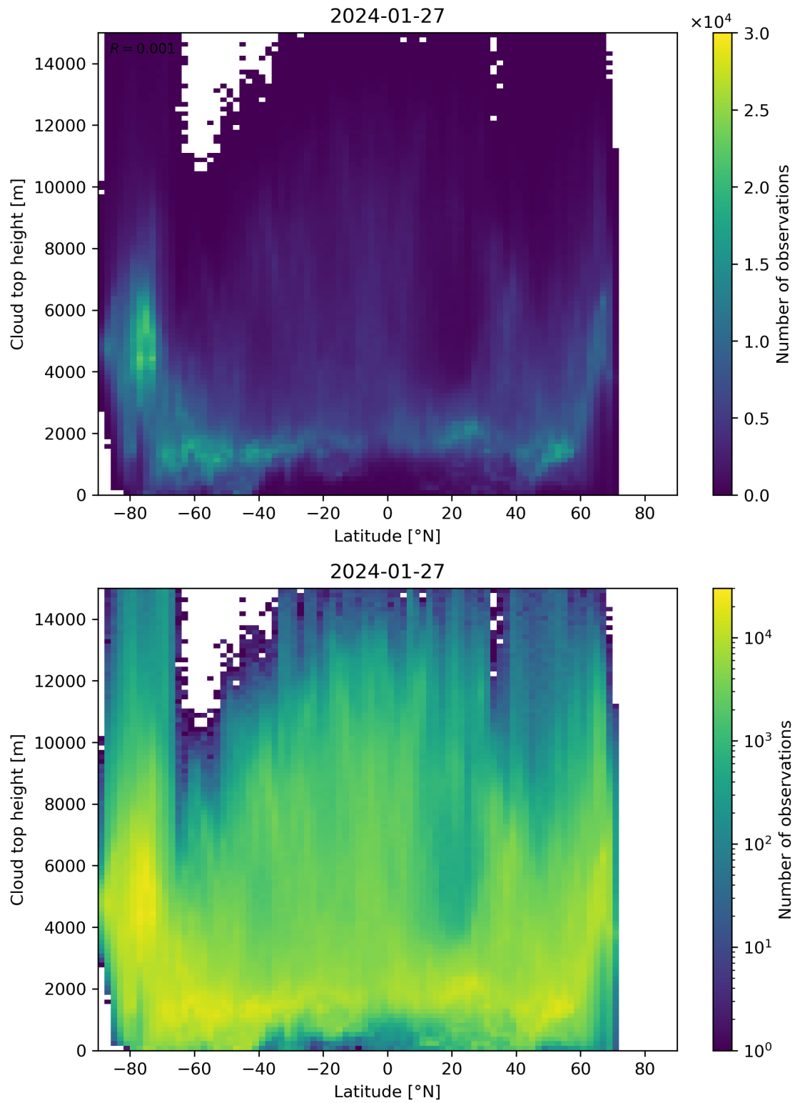
Figure 97: Scatter density plot of “Latitude” against “Cloud top height” for 2024-01-26 to 2024-01-28.
