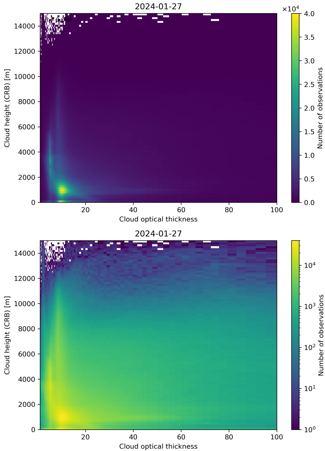
Figure 85: Scatter density plot of “Cloud optical thickness” against “Cloud height (CRB)” for 2024-01-26 to 2024-01-28.
