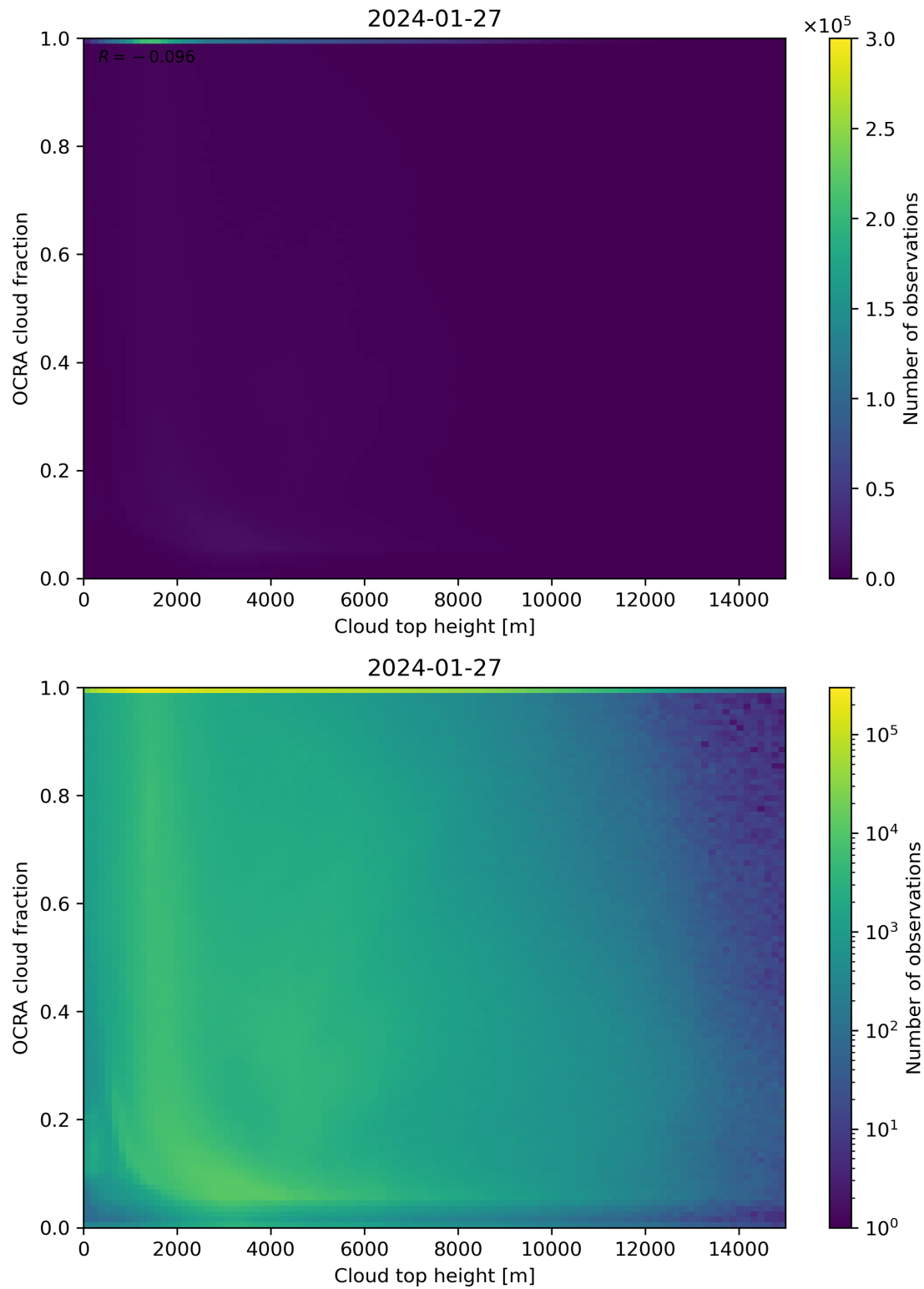
Figure 87: Scatter density plot of “Cloud top height” against “OCRA cloud fraction” for 2024-01-26 to 2024-01-28.
