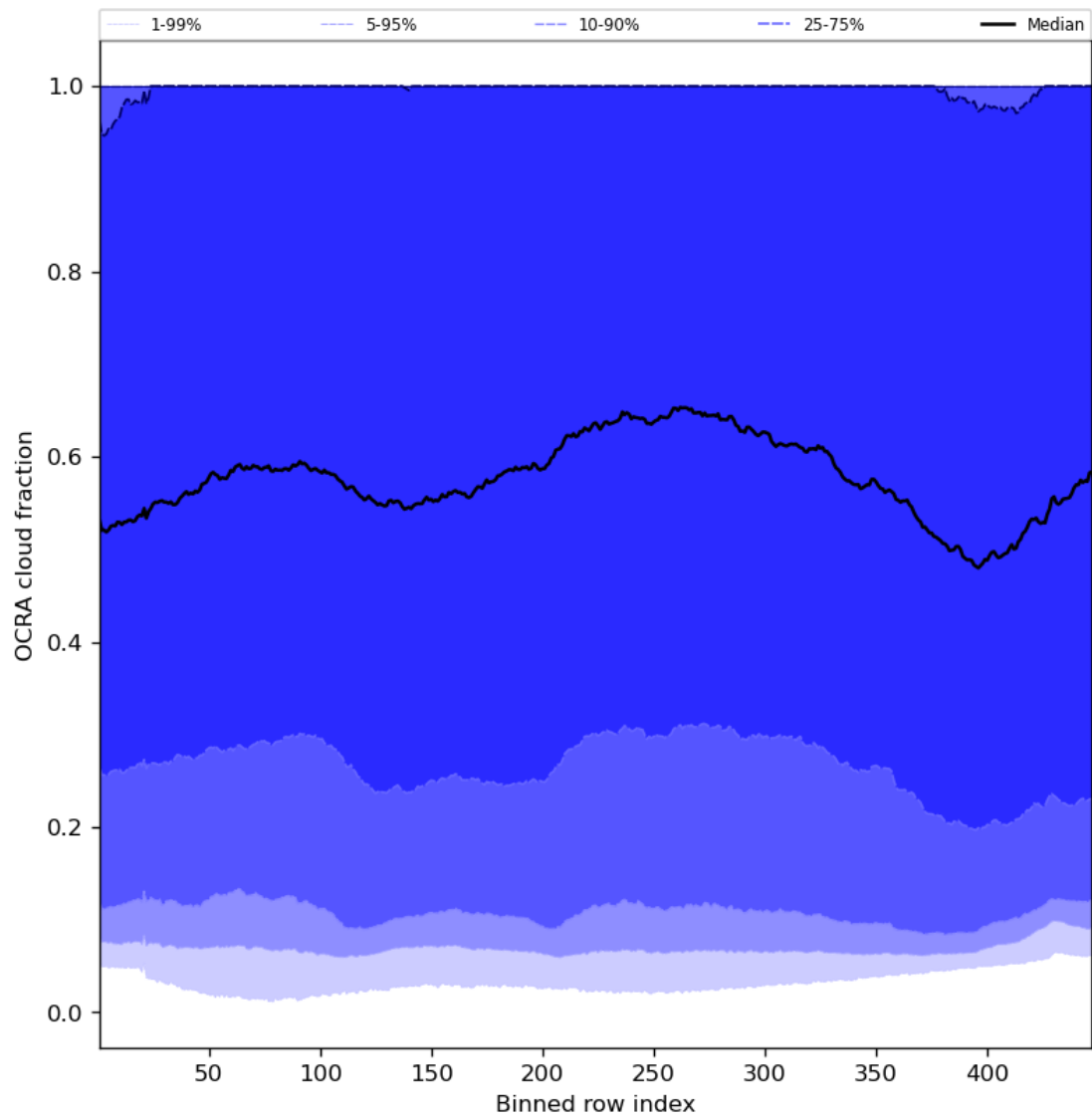
Figure 66: Along track statistics of “OCRA cloud fraction” for 2024-01-26 to 2024-01-28
