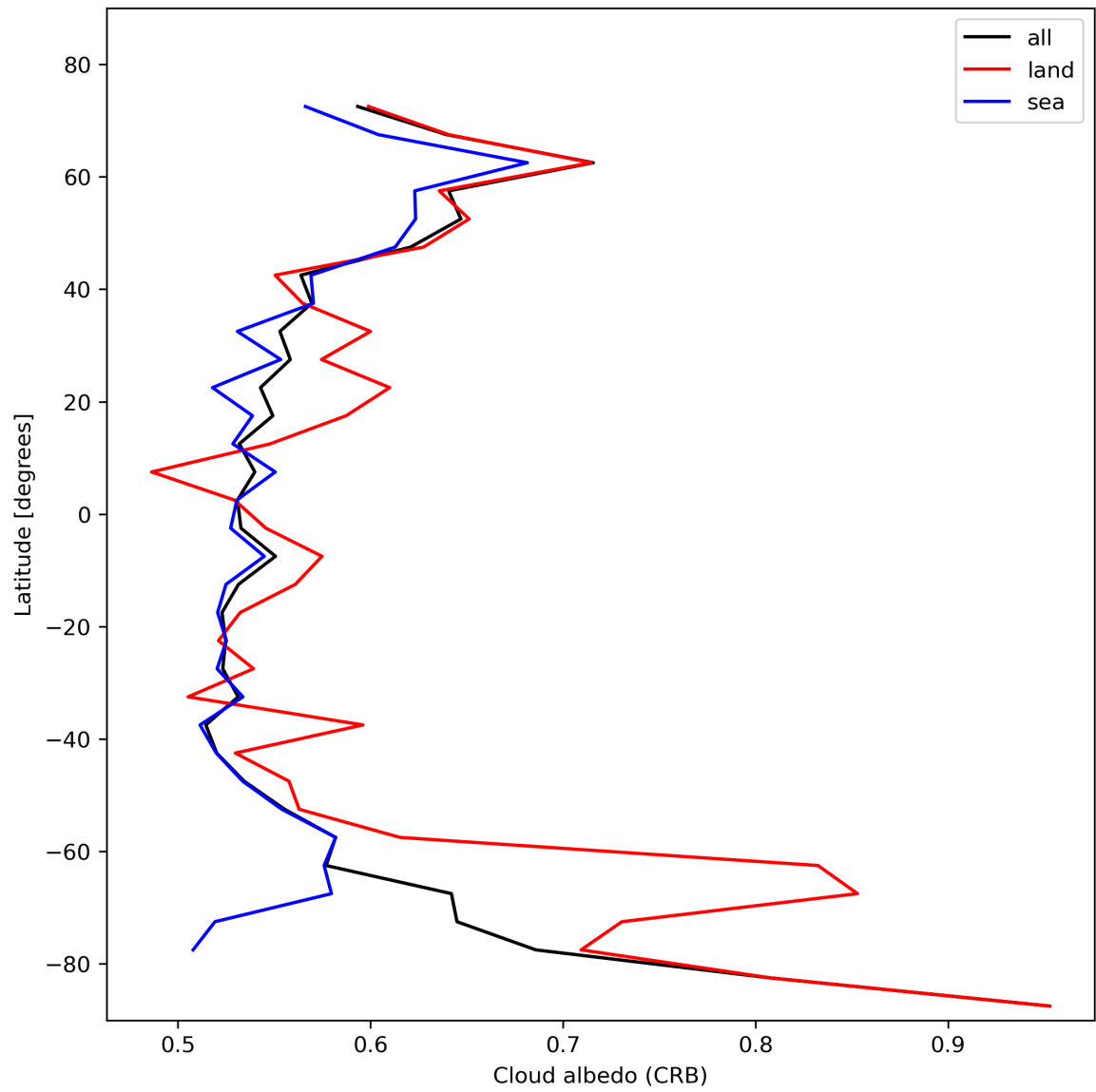
Figure 28: Zonal average of “Cloud albedo (CRB)” for 2024-01-26 to 2024-01-28.
