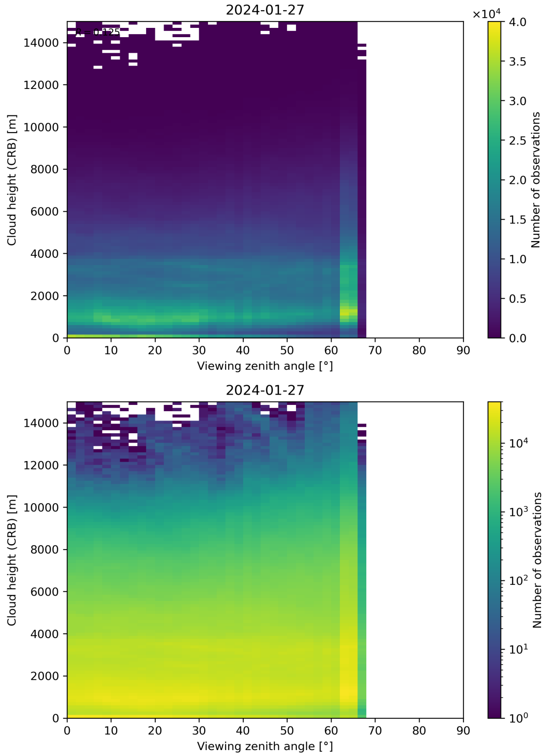
Figure 110: Scatter density plot of “Viewing zenith angle” against “Cloud height (CRB)” for 2024-01-26 to 2024-01-28.
