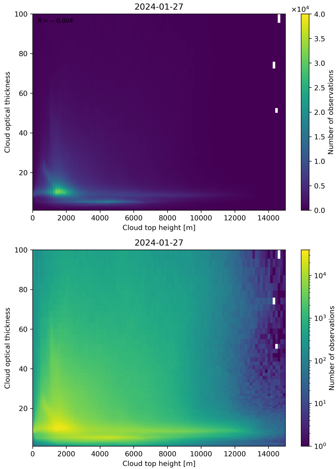
Figure 90: Scatter density plot of “Cloud top height” against “Cloud optical thickness” for 2024-01-26 to 2024-01-28.
