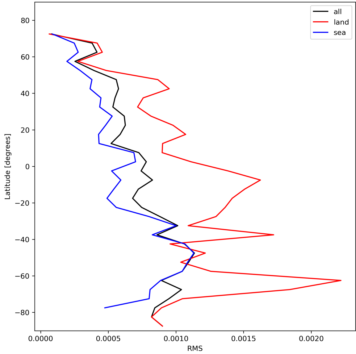
Figure 31: Zonal average of “RMS” for 2024-01-26 to 2024-01-28.
