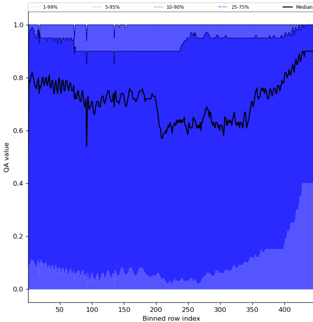
Figure 54: Along track statistics of “QA value” for 2024-01-26 to 2024-01-28
