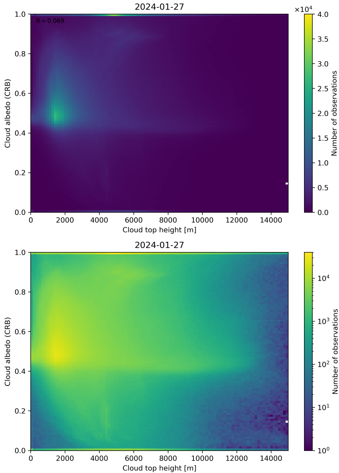
Figure 86: Scatter density plot of “Cloud top height” against “Cloud albedo (CRB)” for 2024-01-26 to 2024-01-28.
