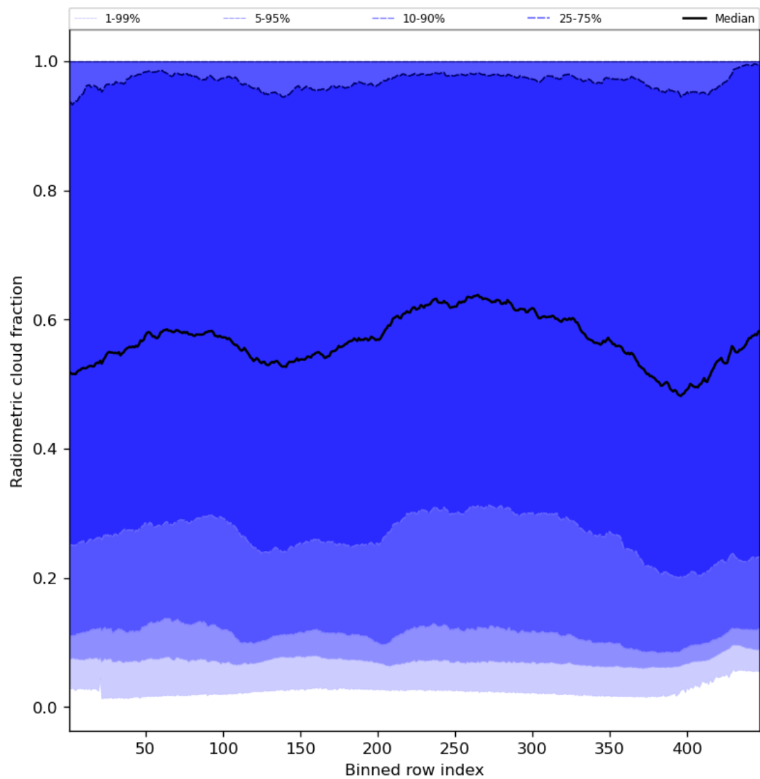
Figure 55: Along track statistics of “Radiometric cloud fraction” for 2024-01-26 to 2024-01-28
