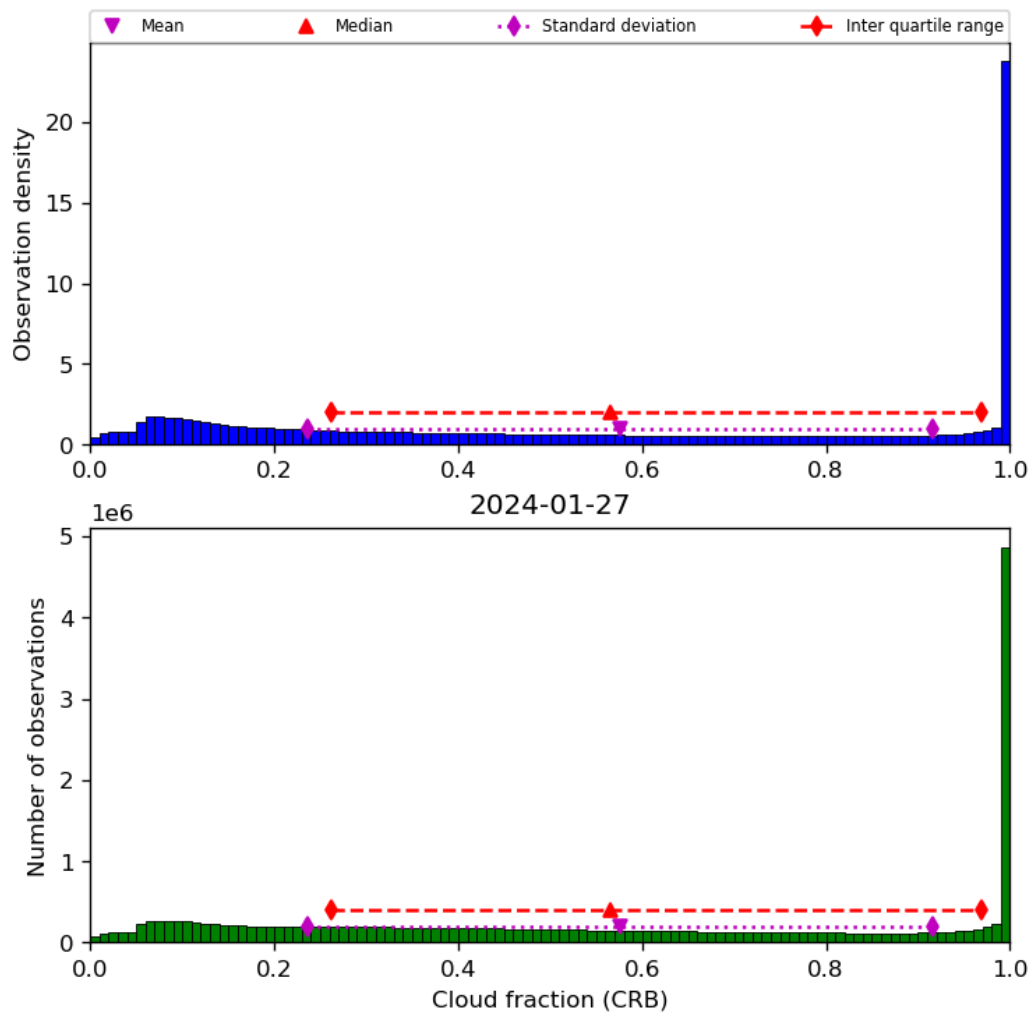
Figure 42: Histogram of “Cloud fraction (CRB)” for 2024-01-26 to 2024-01-28
