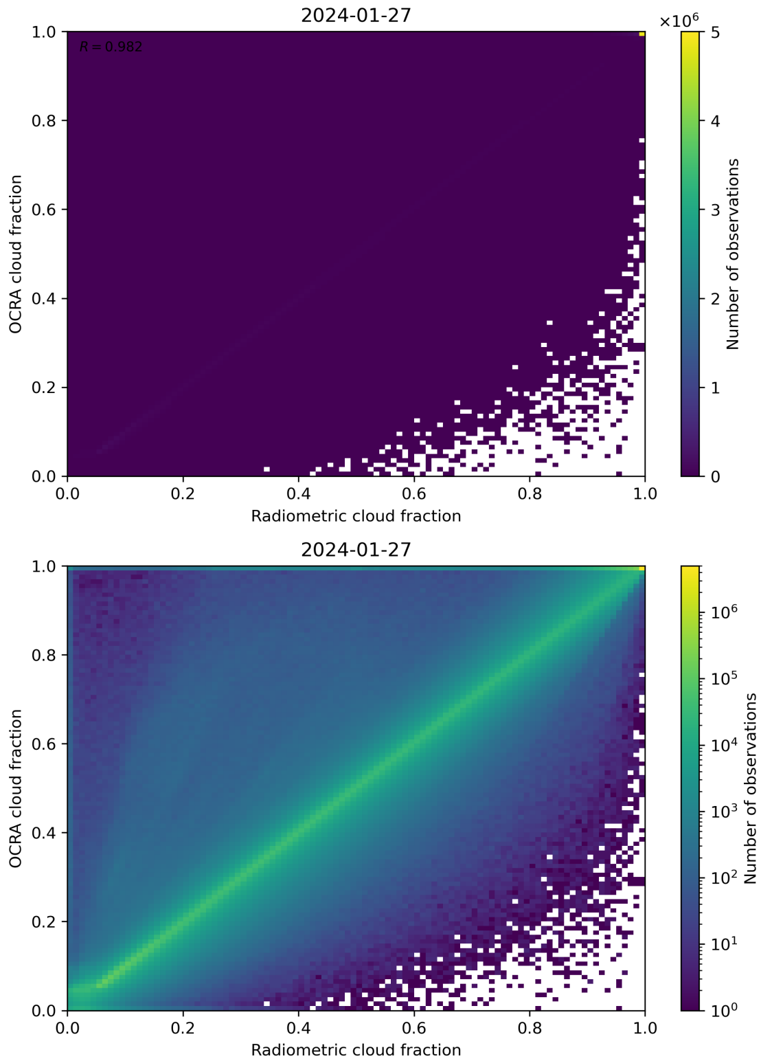
Figure 72: Scatter density plot of “Radiometric cloud fraction” against “OCRA cloud fraction” for 2024-01-26 to 2024-01-28.
