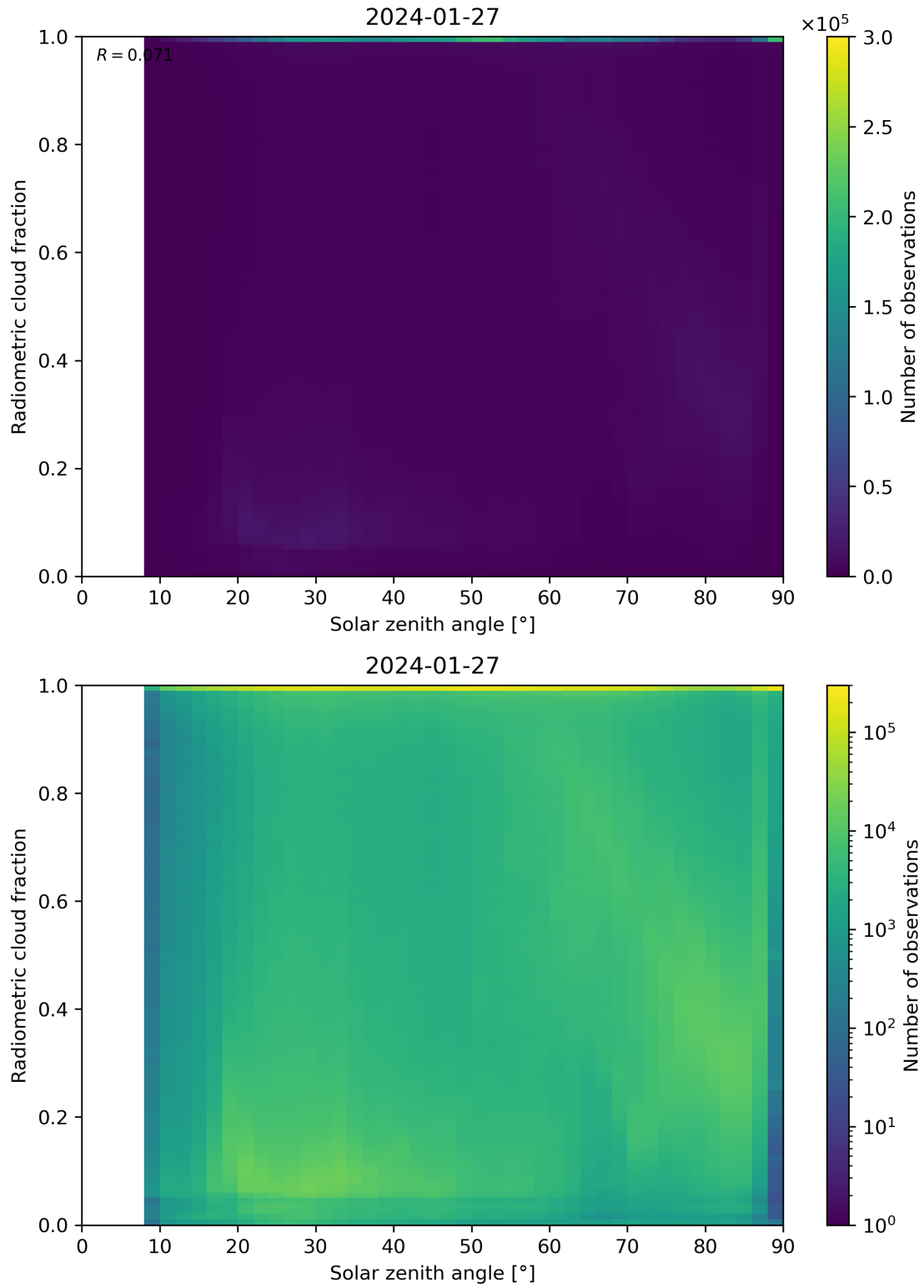
Figure 99: Scatter density plot of “Solar zenith angle” against “Radiometric cloud fraction” for 2024-01-26 to 2024-01-28.
