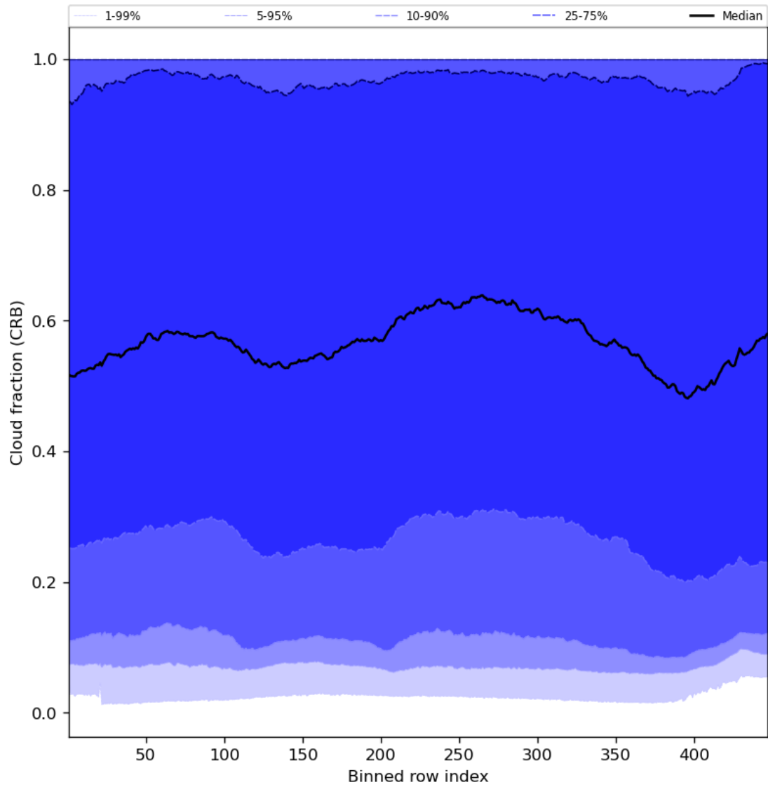
Figure 58: Along track statistics of “Cloud fraction (CRB)” for 2024-01-26 to 2024-01-28
