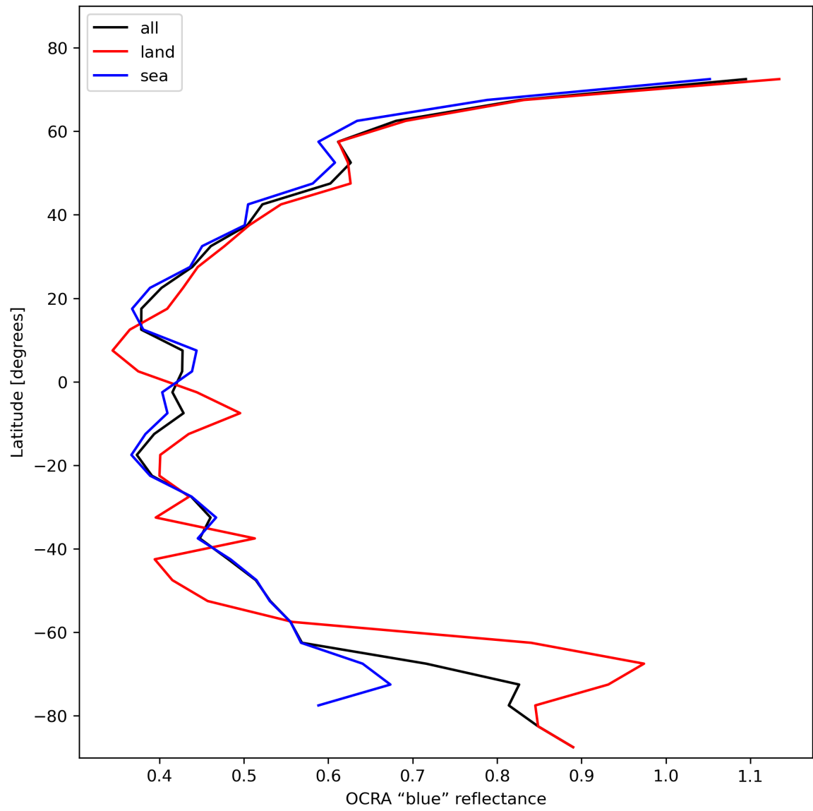
Figure 35: Zonal average of “OCRA “blue” reflectance” for 2024-01-26 to 2024-01-28.
