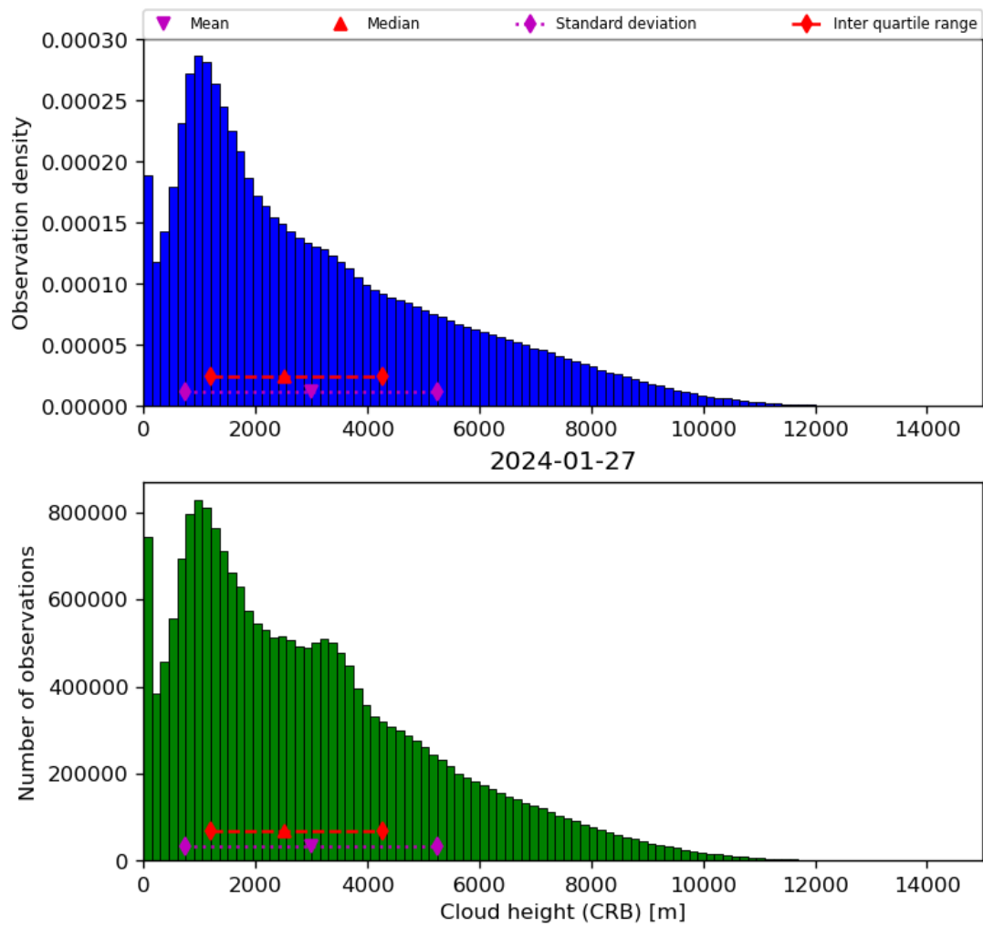
Figure 43: Histogram of “Cloud height (CRB)” for 2024-01-26 to 2024-01-28
