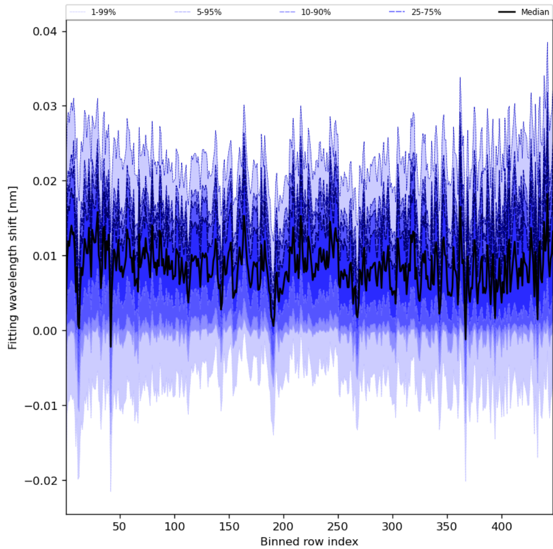
Figure 65: Along track statistics of “Fitting wavelength shift” for 2024-01-26 to 2024-01-28
