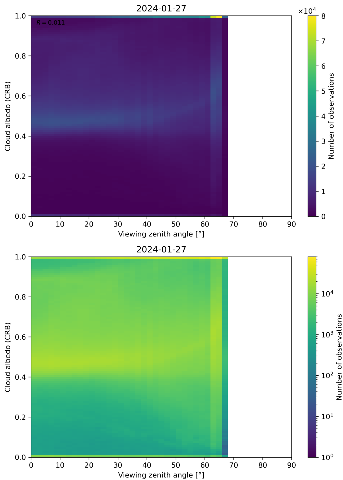
Figure 106: Scatter density plot of “Viewing zenith angle” against “Cloud albedo (CRB)” for 2024-01-26 to 2024-01-28.
