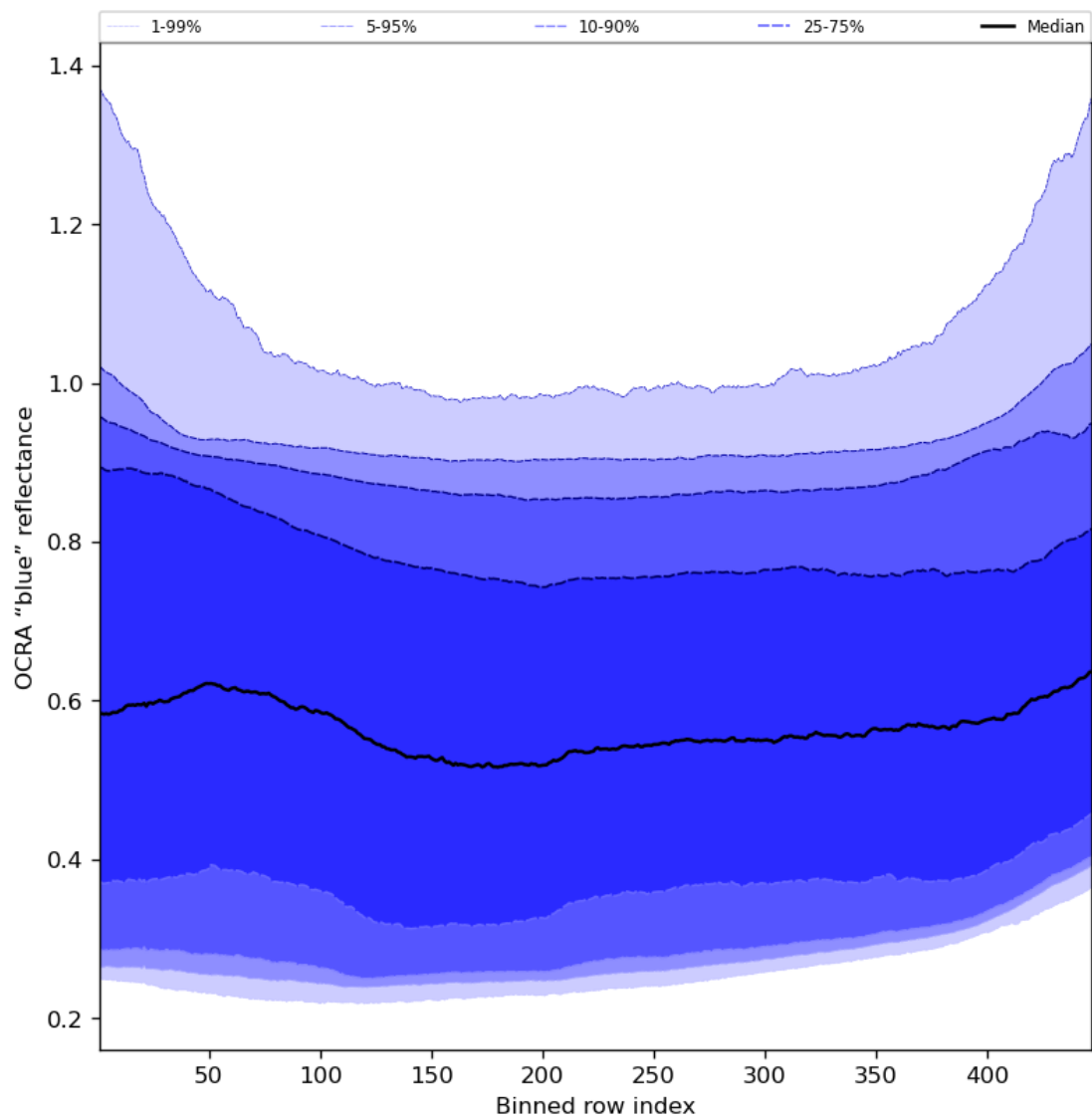
Figure 67: Along track statistics of “OCRA “blue” reflectance” for 2024-01-26 to 2024-01-28
