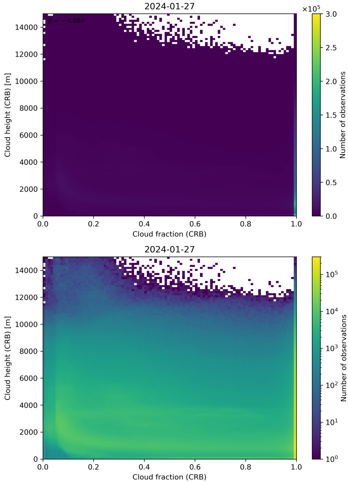
Figure 79: Scatter density plot of “Cloud fraction (CRB)” against “Cloud height (CRB)” for 2024-01-26 to 2024-01-28.
