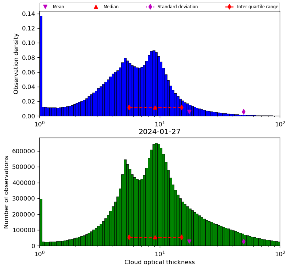
Figure 41: Histogram of “Cloud optical thickness” for 2024-01-26 to 2024-01-28
