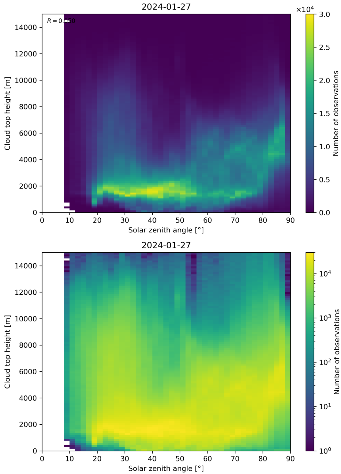
Figure 104: Scatter density plot of “Solar zenith angle” against “Cloud top height” for 2024-01-26 to 2024-01-28.
