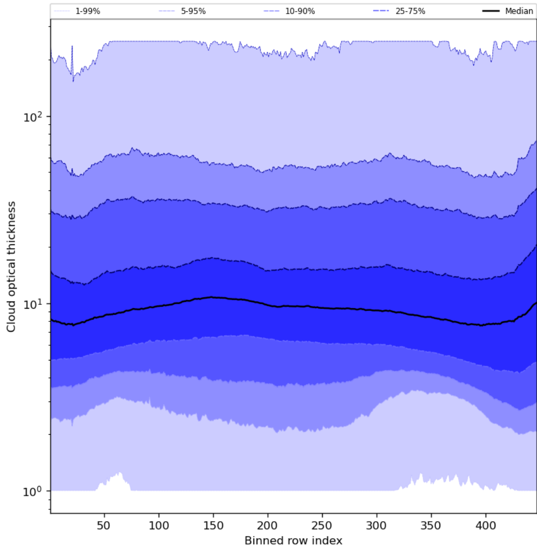
Figure 57: Along track statistics of “Cloud optical thickness” for 2024-01-26 to 2024-01-28
