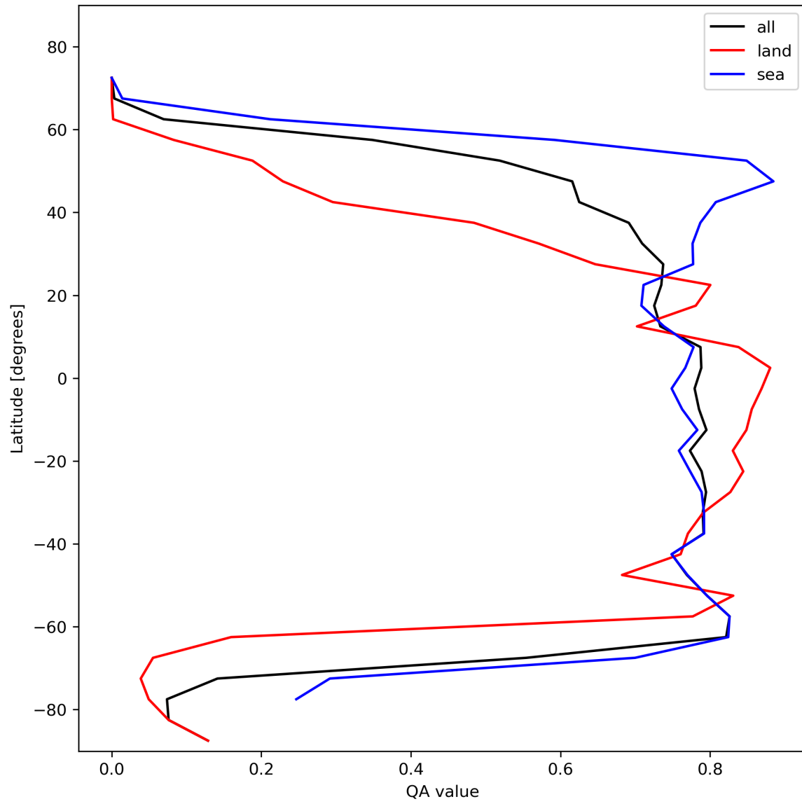
Figure 22: Zonal average of “QA value” for 2024-01-26 to 2024-01-28.
