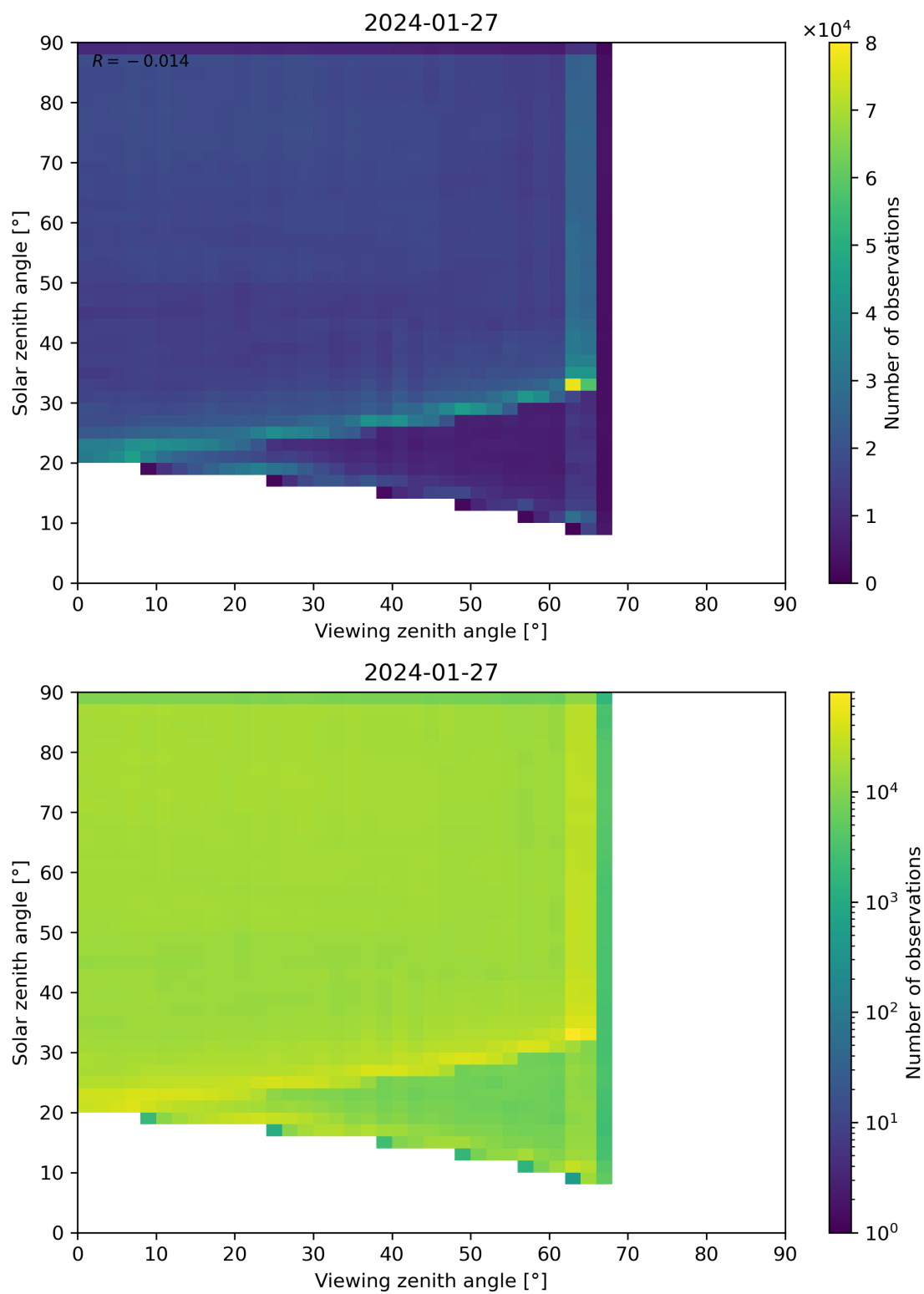
Figure 114: Scatter density plot of “Viewing zenith angle” against “Solar zenith angle” for 2024-01-26 to 2024-01-28.
