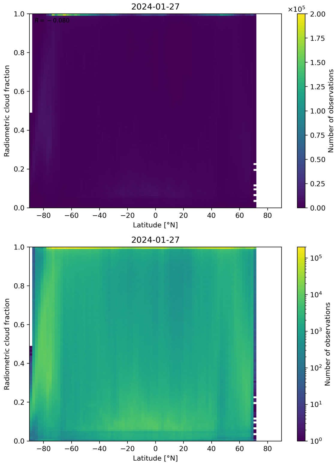
Figure 92: Scatter density plot of “Latitude” against “Radiometric cloud fraction” for 2024-01-26 to 2024-01-28.
