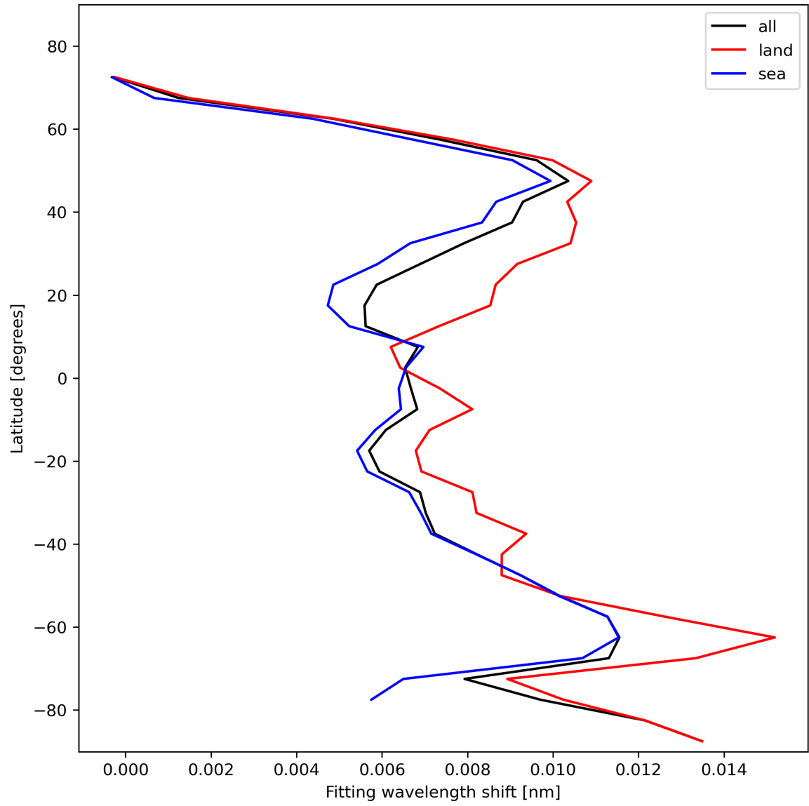
Figure 33: Zonal average of “Fitting wavelength shift” for 2024-01-26 to 2024-01-28.
