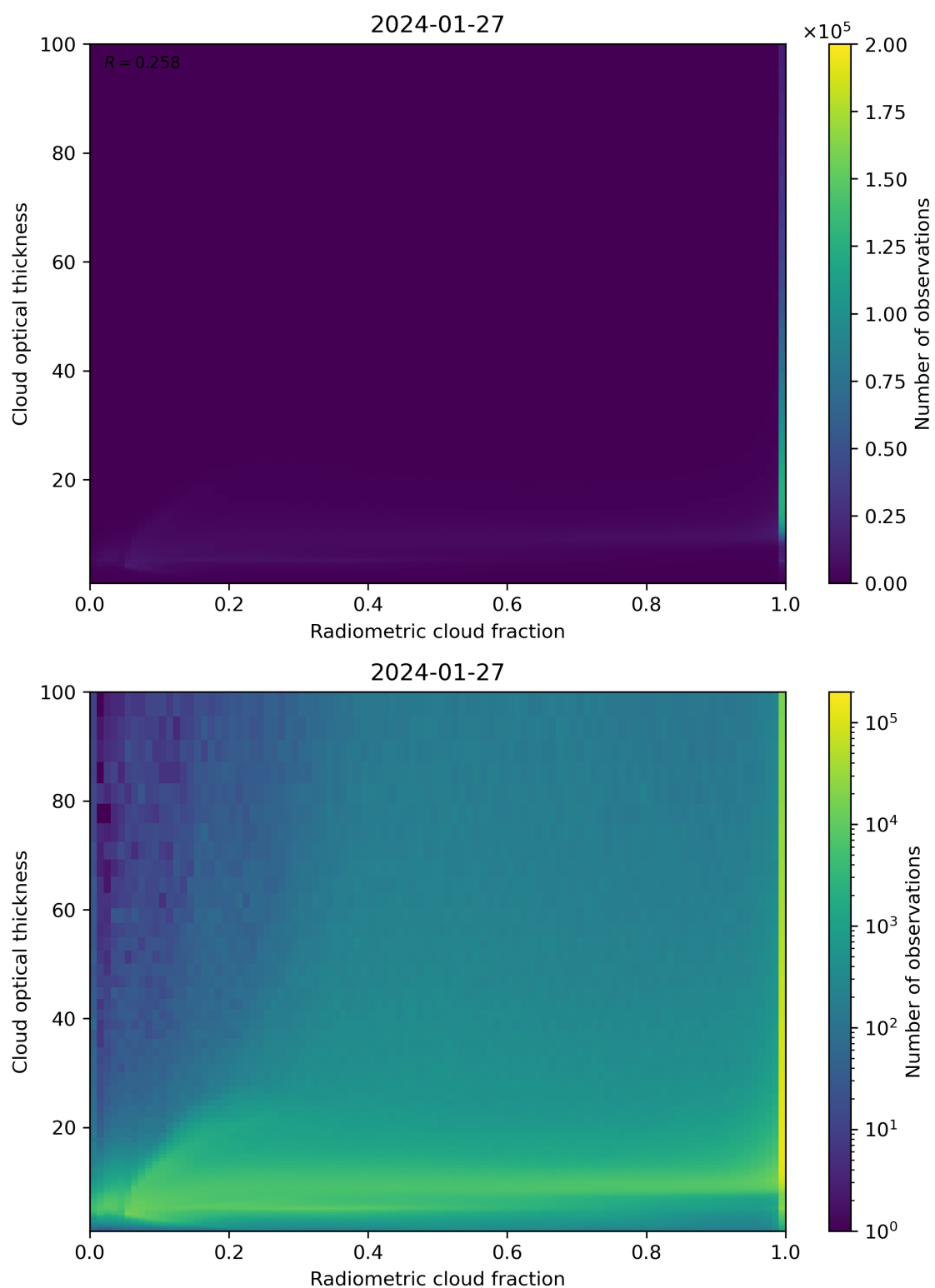
Figure 75: Scatter density plot of “Radiometric cloud fraction” against “Cloud optical thickness” for 2024-01-26 to 2024-01-28.
