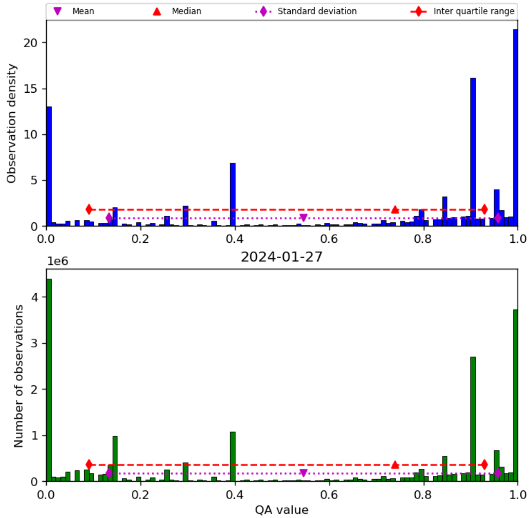
Figure 38: Histogram of “QA value” for 2024-01-26 to 2024-01-28
