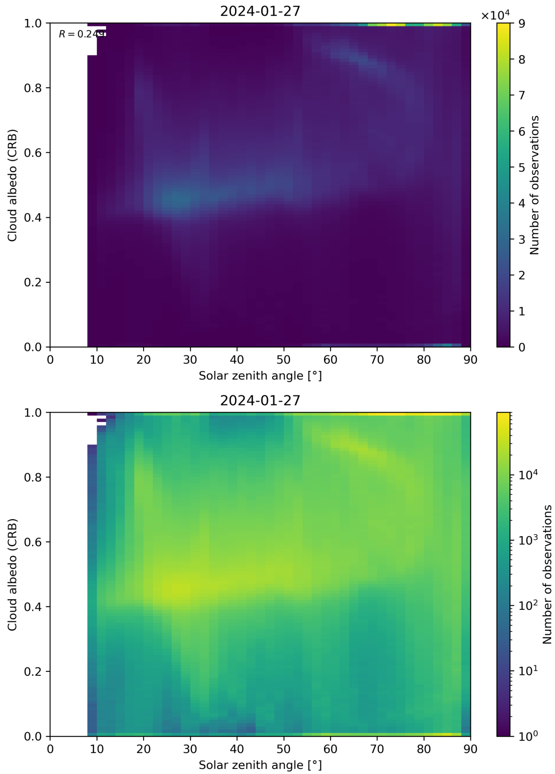
Figure 98: Scatter density plot of “Solar zenith angle” against “Cloud albedo (CRB)” for 2024-01-26 to 2024-01-28.
