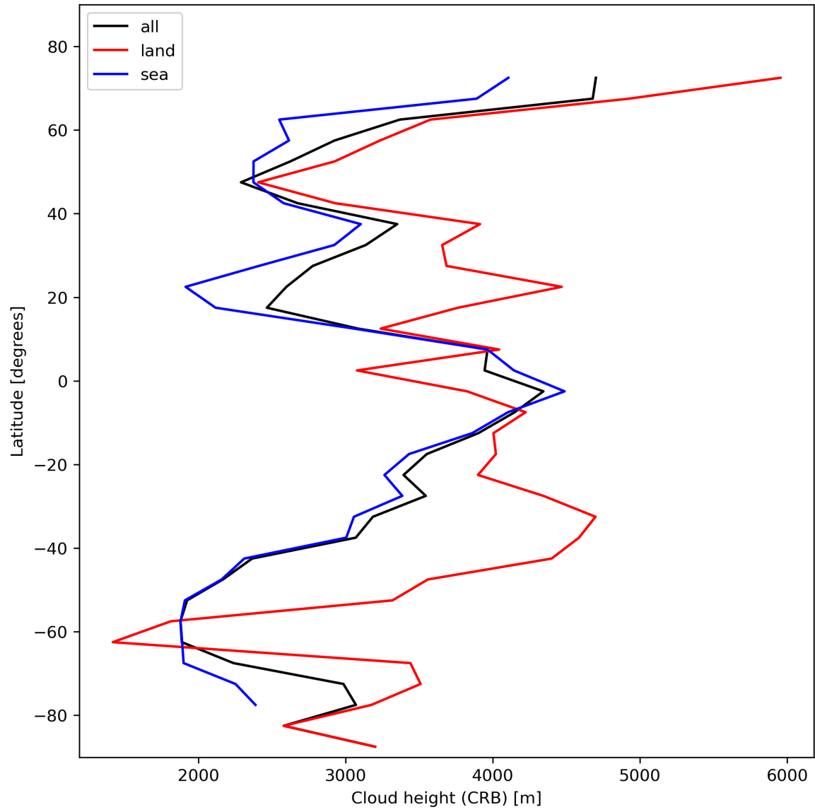
Figure 27: Zonal average of “Cloud height (CRB)” for 2024-01-26 to 2024-01-28.
