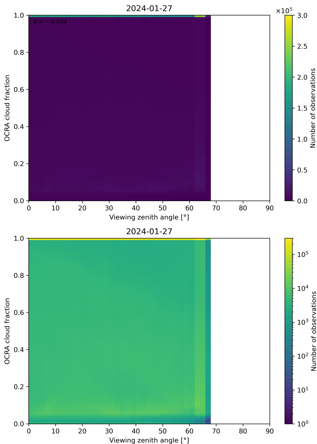
Figure 108: Scatter density plot of “Viewing zenith angle” against “OCRA cloud fraction” for 2024-01-26 to 2024-01-28.
