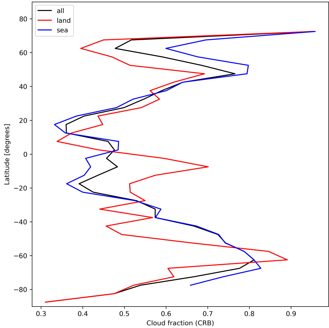
Figure 26: Zonal average of “Cloud fraction (CRB)” for 2024-01-26 to 2024-01-28.
