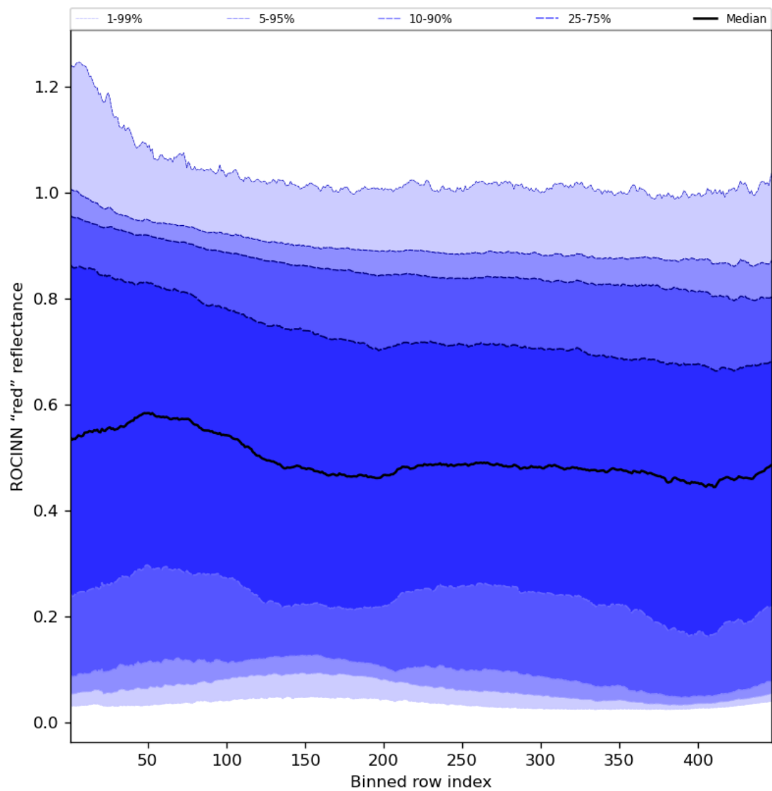
Figure 69: Along track statistics of “ROCINN “red” reflectance” for 2024-01-26 to 2024-01-28
