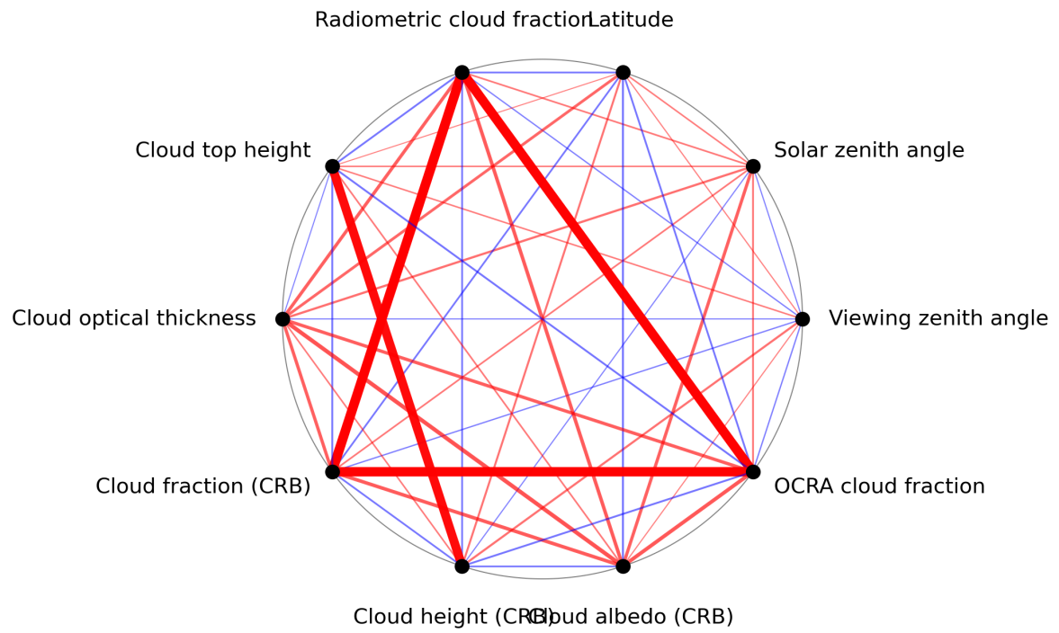
Figure 1: Map of correlation graph for 2024-01-26 to 2024-01-28.
