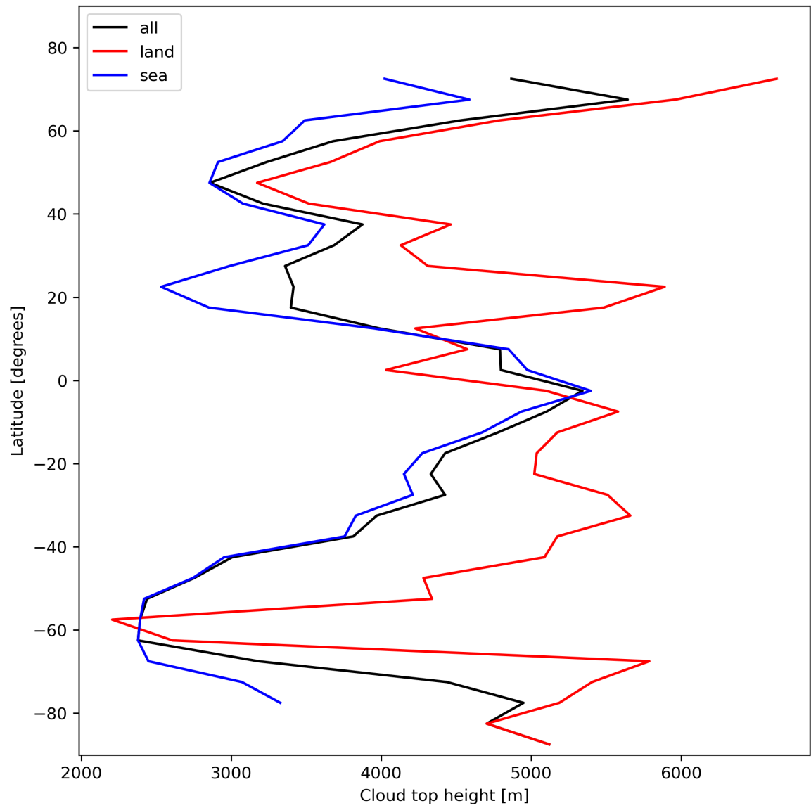
Figure 24: Zonal average of “Cloud top height” for 2024-01-26 to 2024-01-28.
