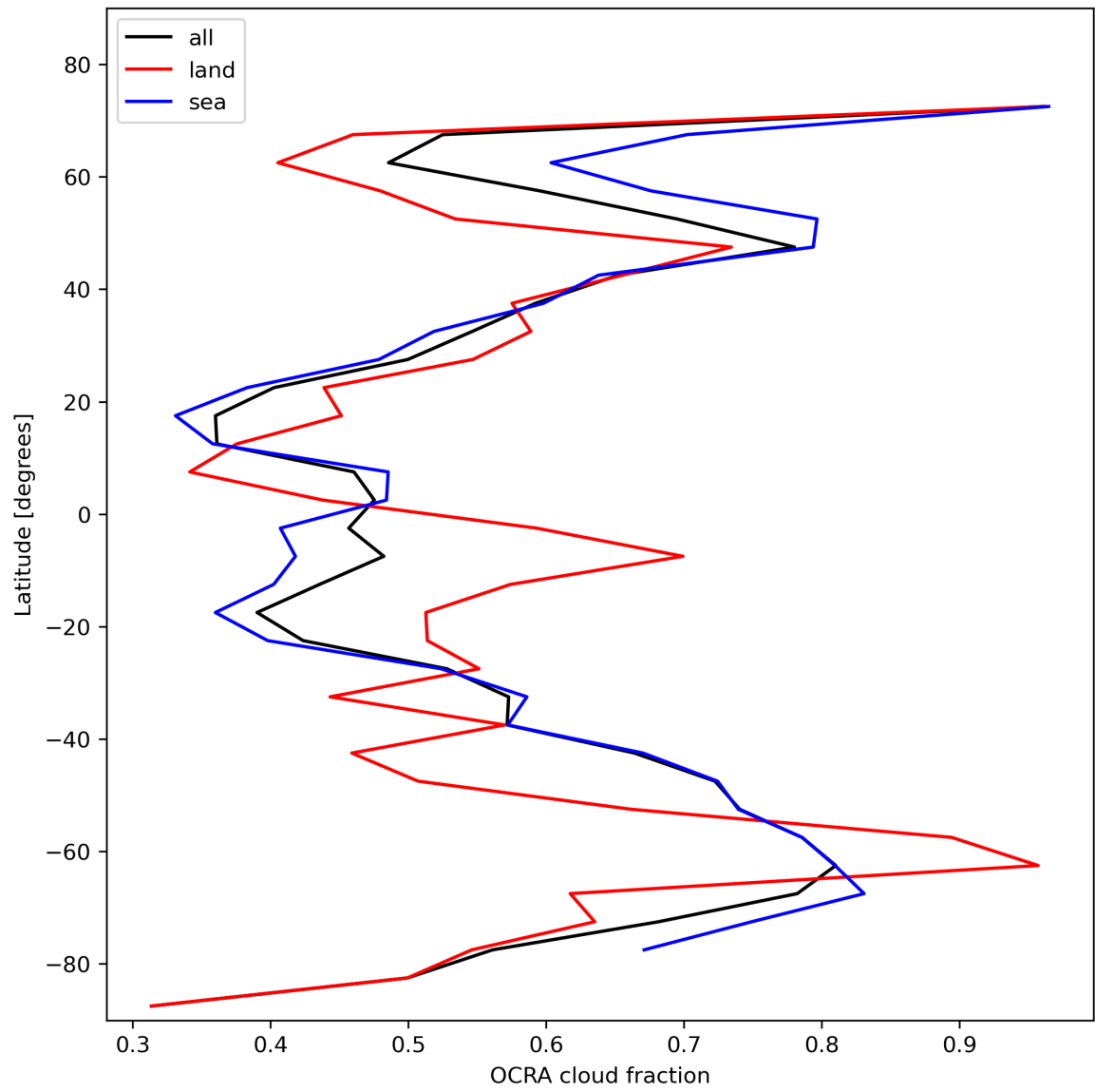
Figure 34: Zonal average of “OCRA cloud fraction” for 2024-01-26 to 2024-01-28.
