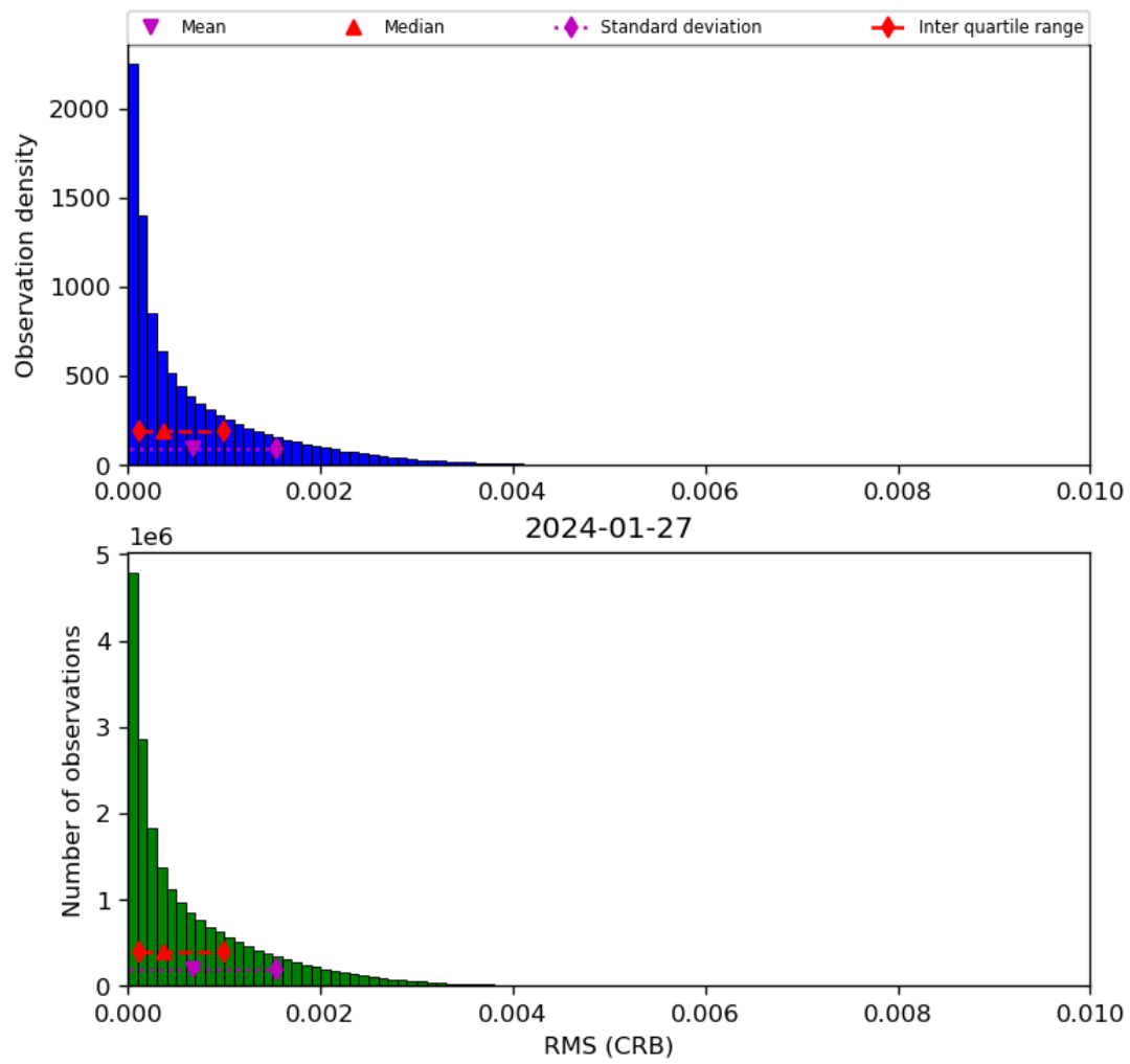
Figure 48: Histogram of “RMS (CRB)” for 2024-01-26 to 2024-01-28
