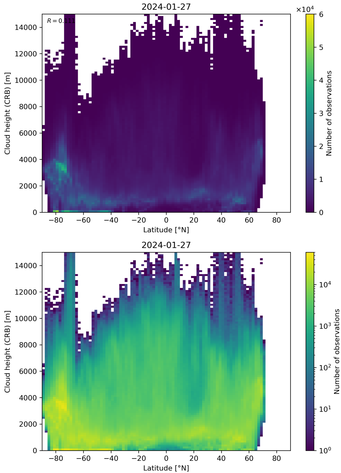
Figure 95: Scatter density plot of “Latitude” against “Cloud height (CRB)” for 2024-01-26 to 2024-01-28.
