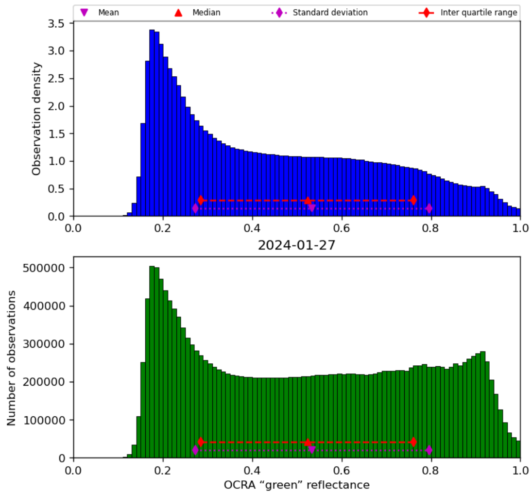
Figure 52: Histogram of “OCRA “green” reflectance” for 2024-01-26 to 2024-01-28
