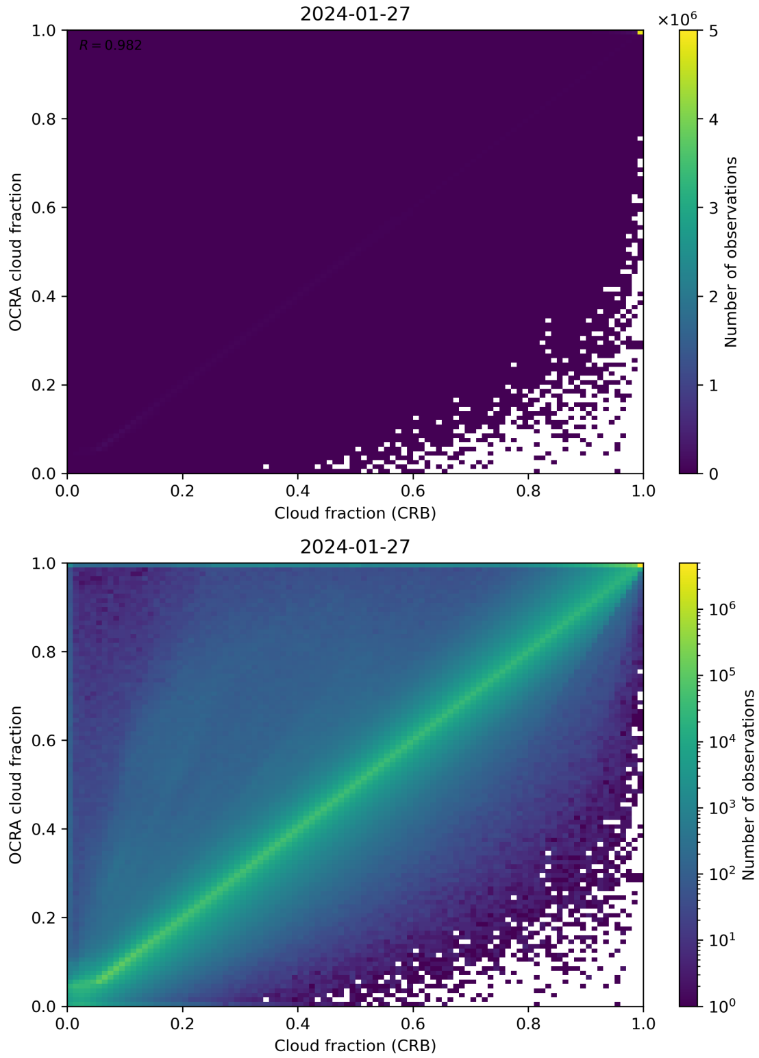
Figure 78: Scatter density plot of “Cloud fraction (CRB)” against “OCRA cloud fraction” for 2024-01-26 to 2024-01-28.
