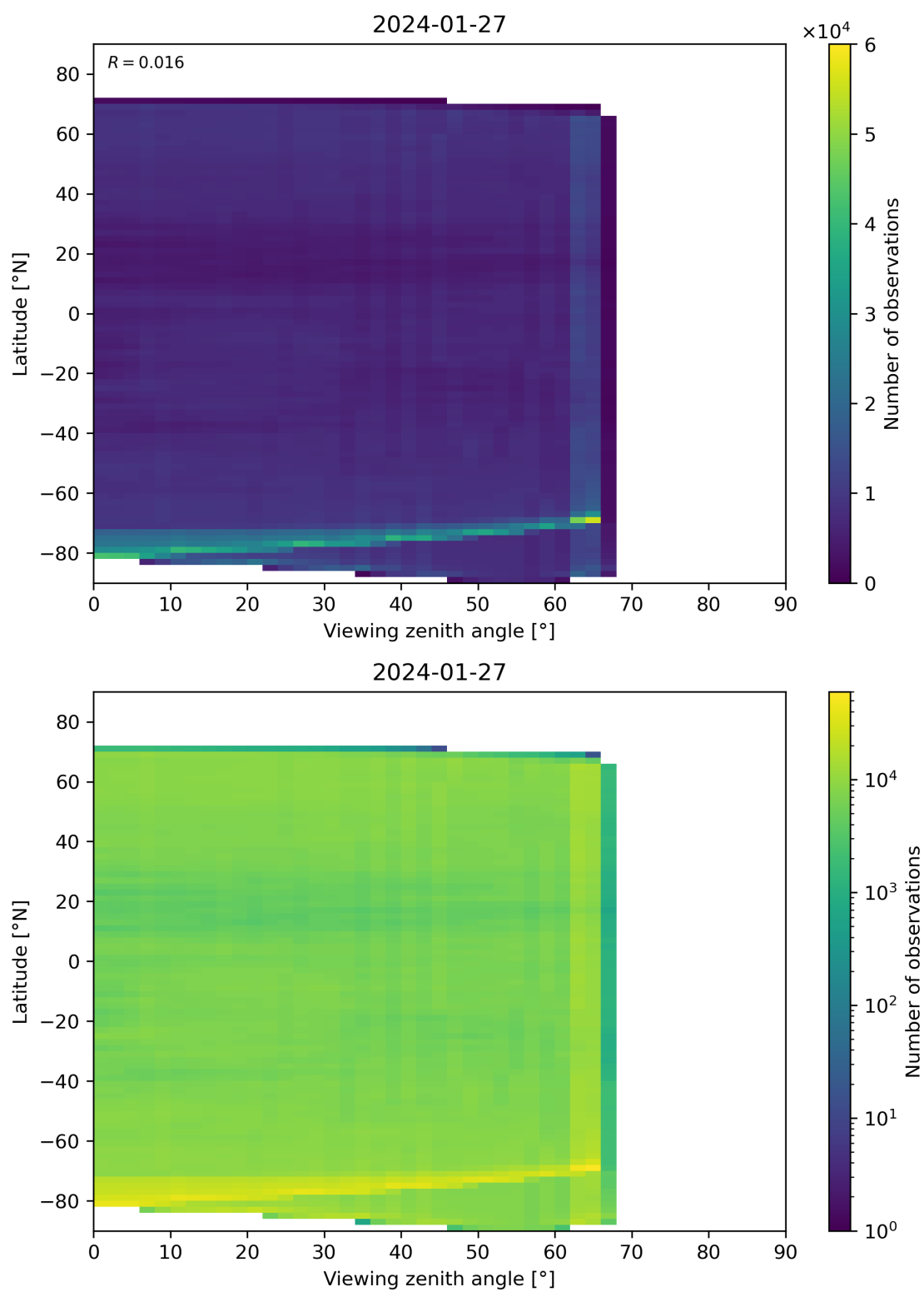
Figure 113: Scatter density plot of “Viewing zenith angle” against “Latitude” for 2024-01-26 to 2024-01-28.
