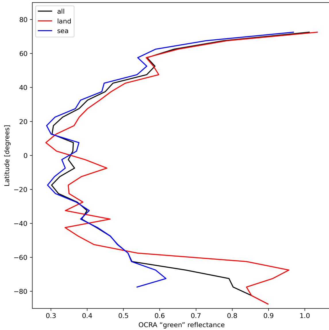
Figure 36: Zonal average of “OCRA “green” reflectance” for 2024-01-26 to 2024-01-28.
