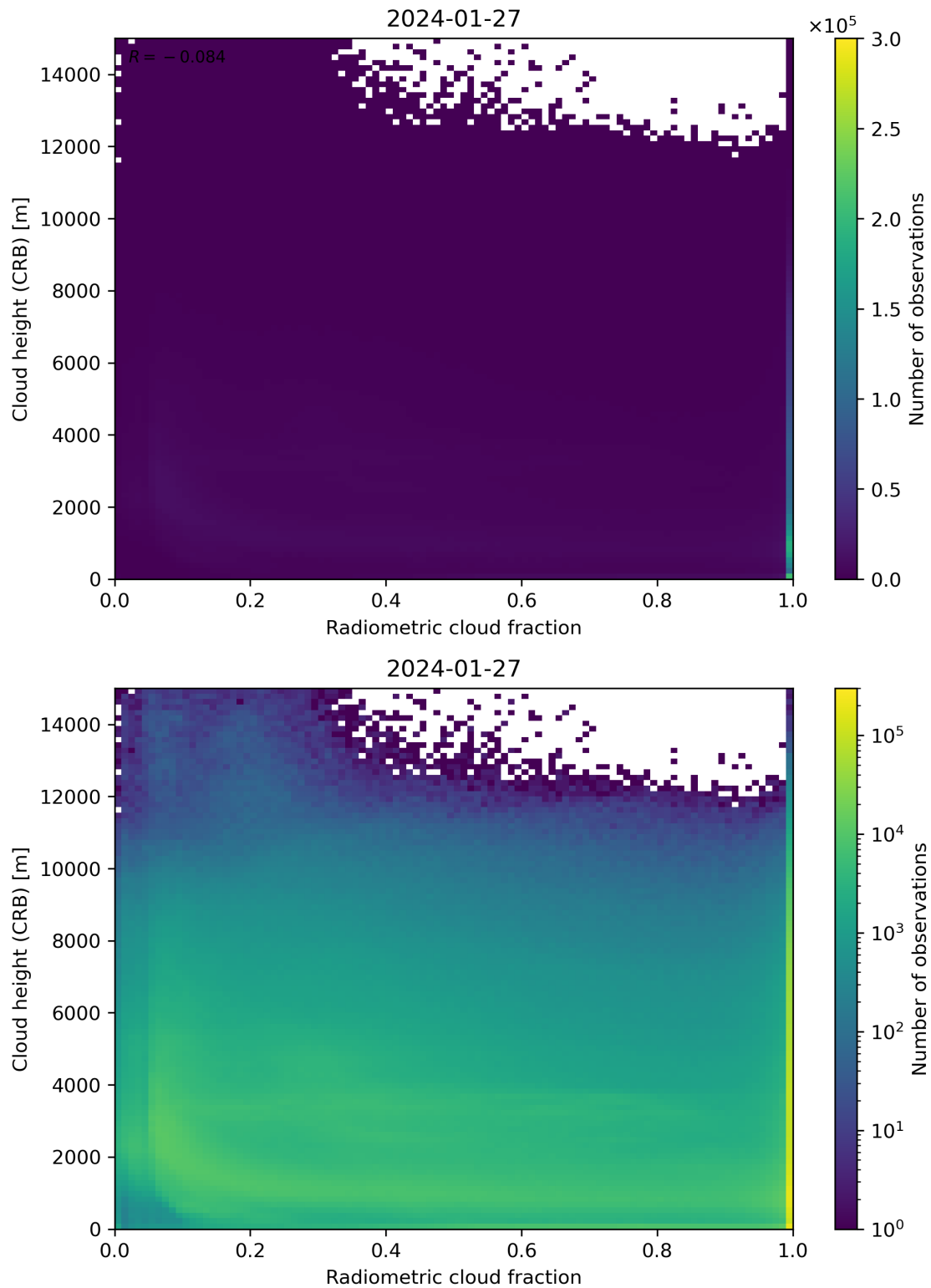
Figure 74: Scatter density plot of “Radiometric cloud fraction” against “Cloud height (CRB)” for 2024-01-26 to 2024-01-28.
