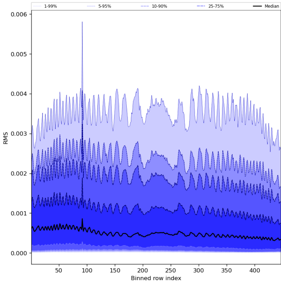
Figure 63: Along track statistics of “RMS” for 2024-01-26 to 2024-01-28
