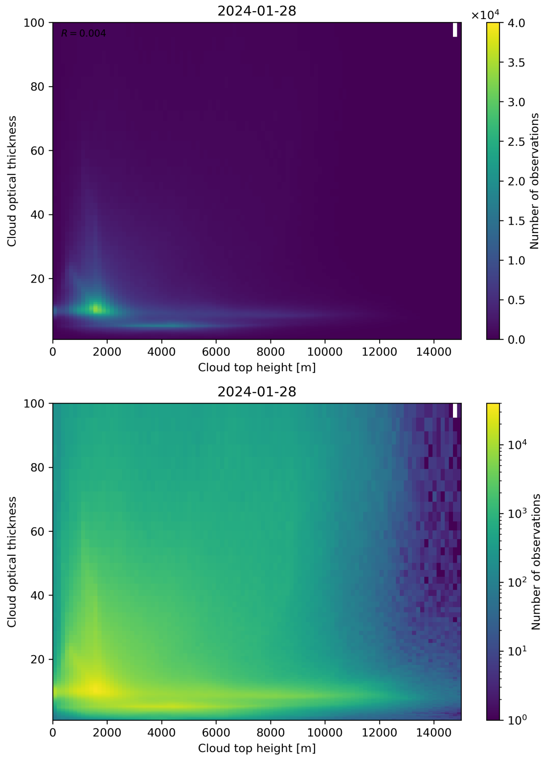
Figure 90: Scatter density plot of “Cloud top height” against “Cloud optical thickness” for 2024-01-27 to 2024-01-29.
