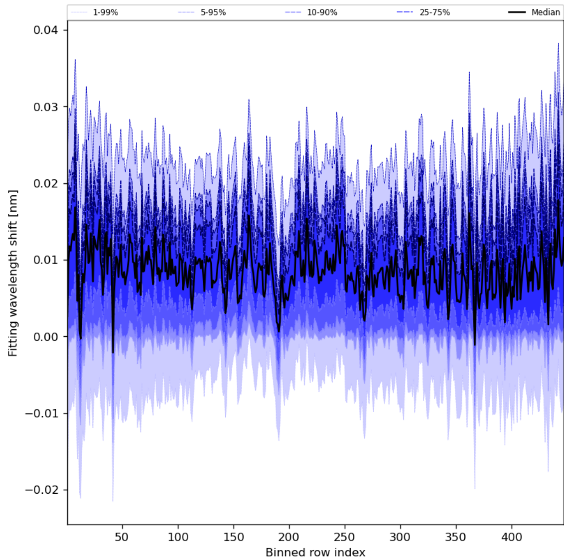
Figure 65: Along track statistics of “Fitting wavelength shift” for 2024-01-27 to 2024-01-29
