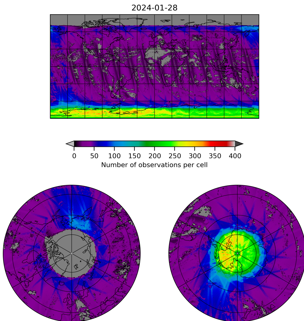
Figure 21: Map of the number of observations for 2024-01-27 to 2024-01-29
