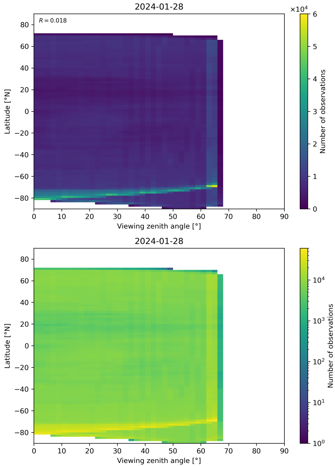
Figure 113: Scatter density plot of “Viewing zenith angle” against “Latitude” for 2024-01-27 to 2024-01-29.
