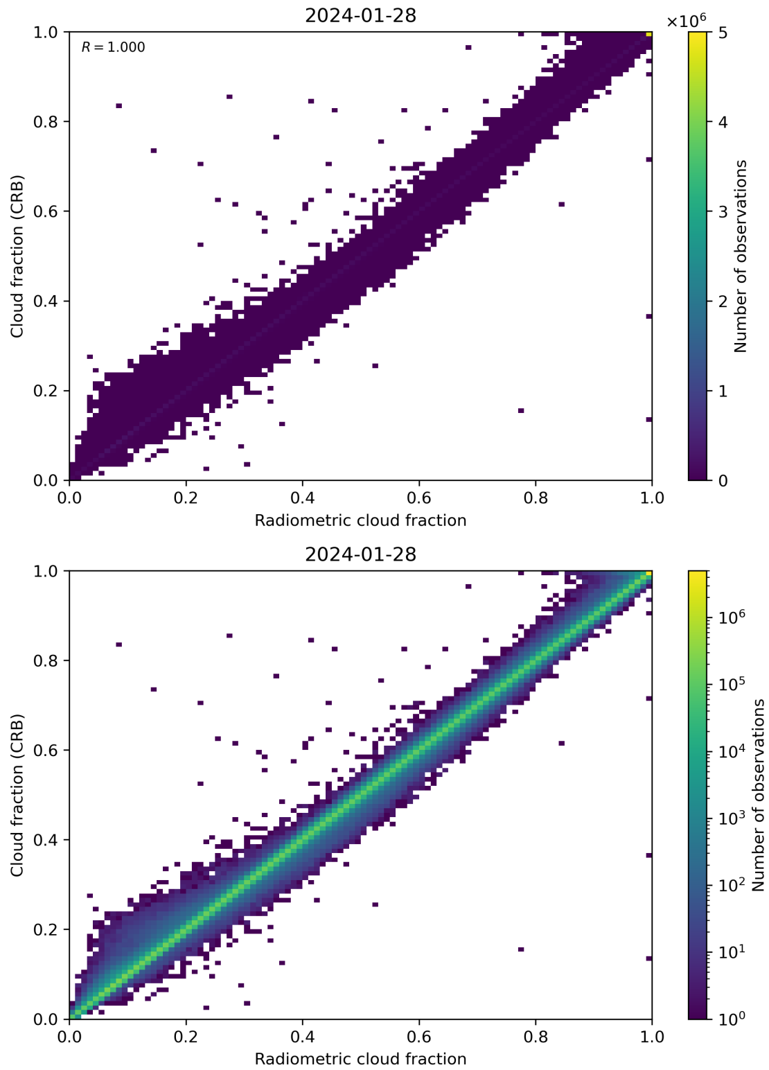
Figure 73: Scatter density plot of “Radiometric cloud fraction” against “Cloud fraction (CRB)” for 2024-01-27 to 2024-01-29.
