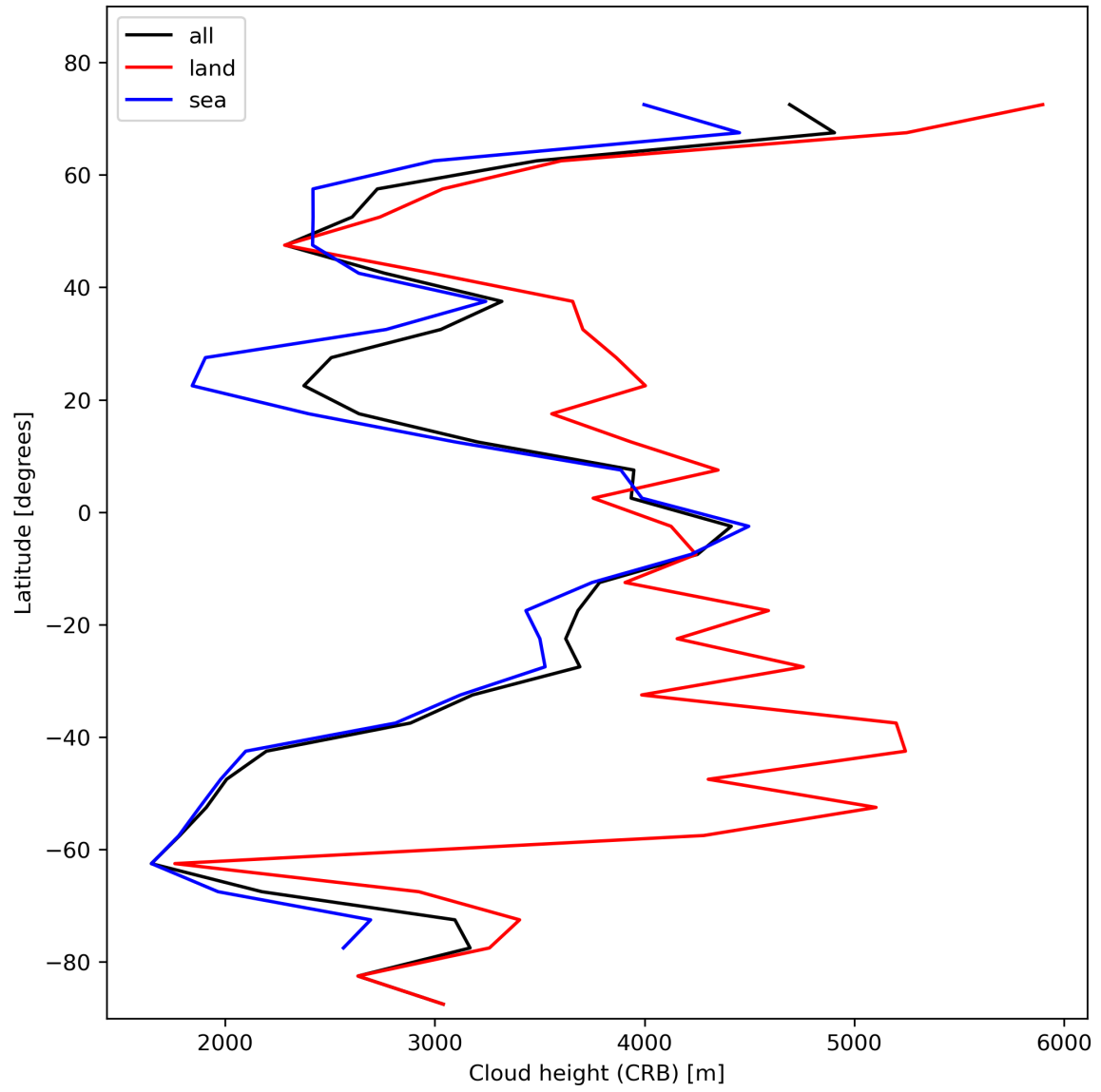
Figure 27: Zonal average of “Cloud height (CRB)” for 2024-01-27 to 2024-01-29.
