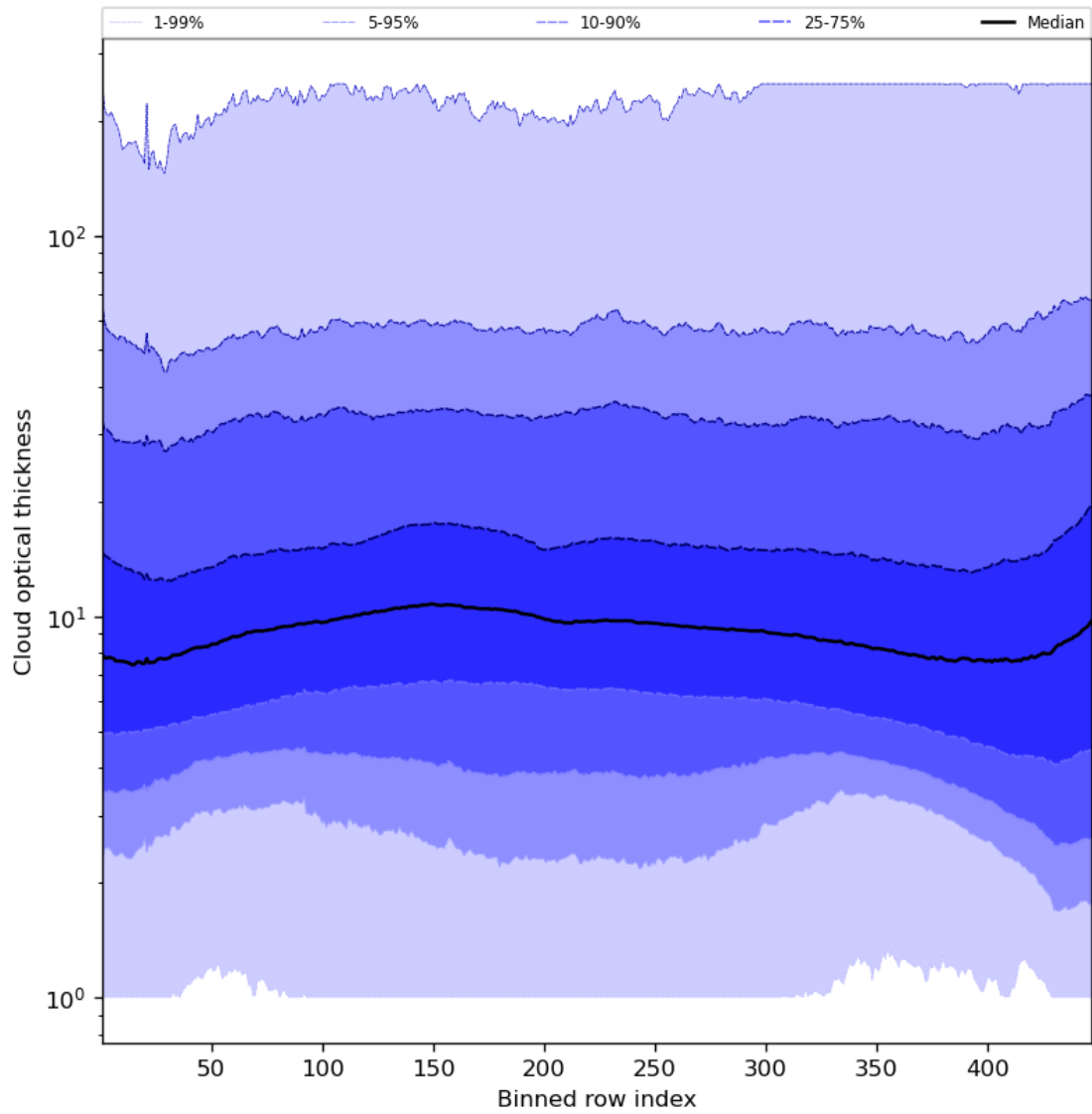
Figure 57: Along track statistics of “Cloud optical thickness” for 2024-01-27 to 2024-01-29
