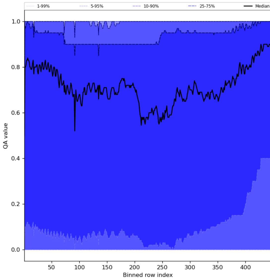
Figure 54: Along track statistics of “QA value” for 2024-01-27 to 2024-01-29
