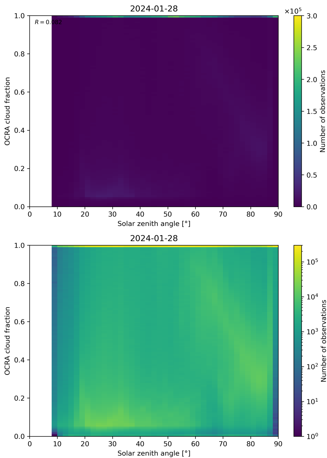
Figure 100: Scatter density plot of “Solar zenith angle” against “OCRA cloud fraction” for 2024-01-27 to 2024-01-29.
