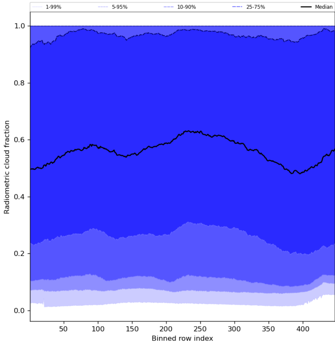
Figure 55: Along track statistics of “Radiometric cloud fraction” for 2024-01-27 to 2024-01-29
