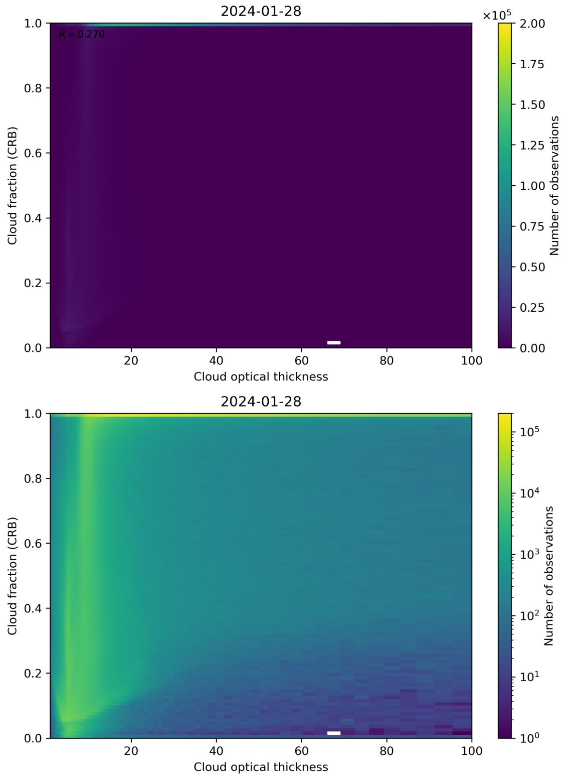
Figure 84: Scatter density plot of “Cloud optical thickness” against “Cloud fraction (CRB)” for 2024-01-27 to 2024-01-29.
