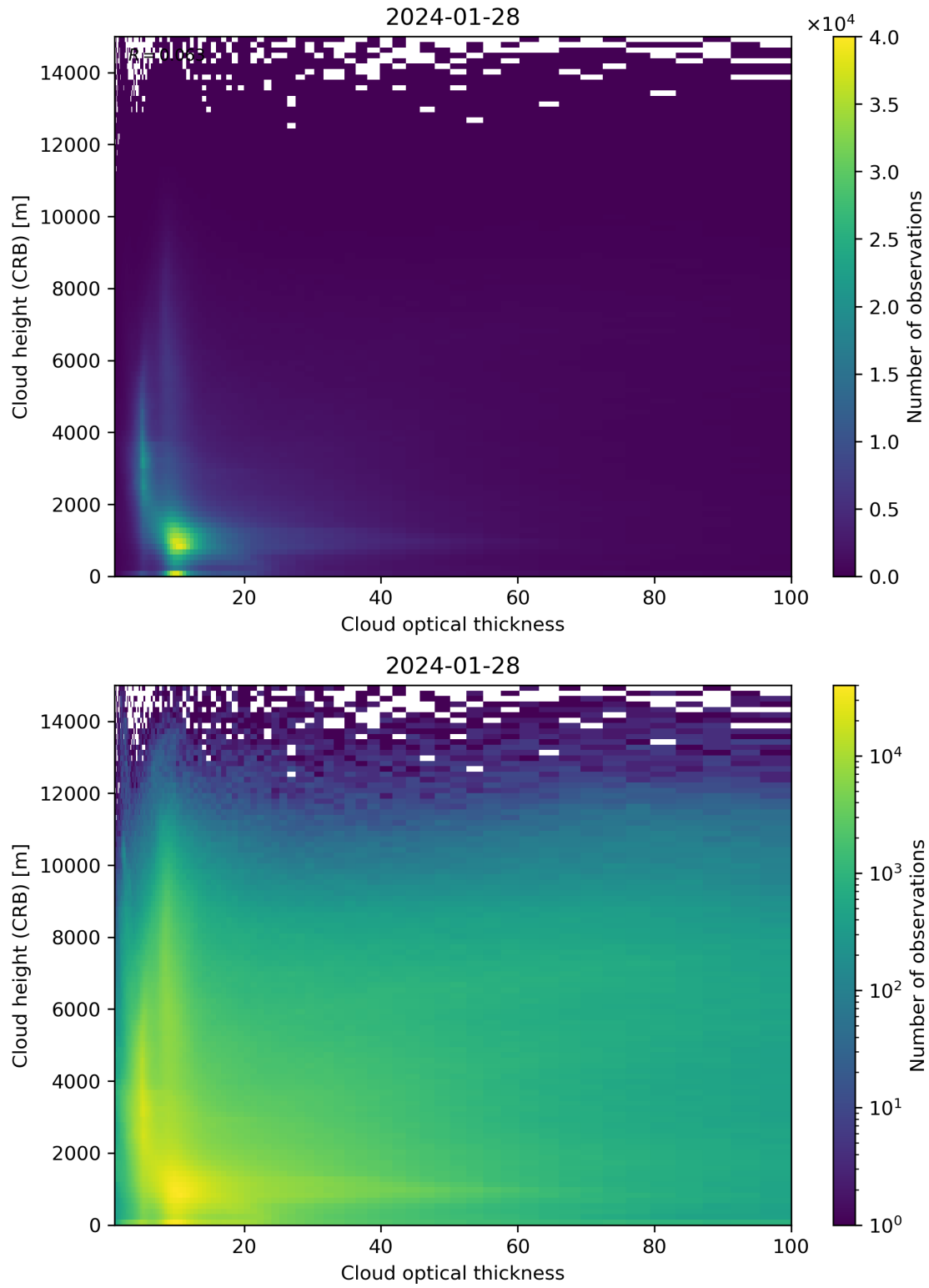
Figure 85: Scatter density plot of “Cloud optical thickness” against “Cloud height (CRB)” for 2024-01-27 to 2024-01-29.
