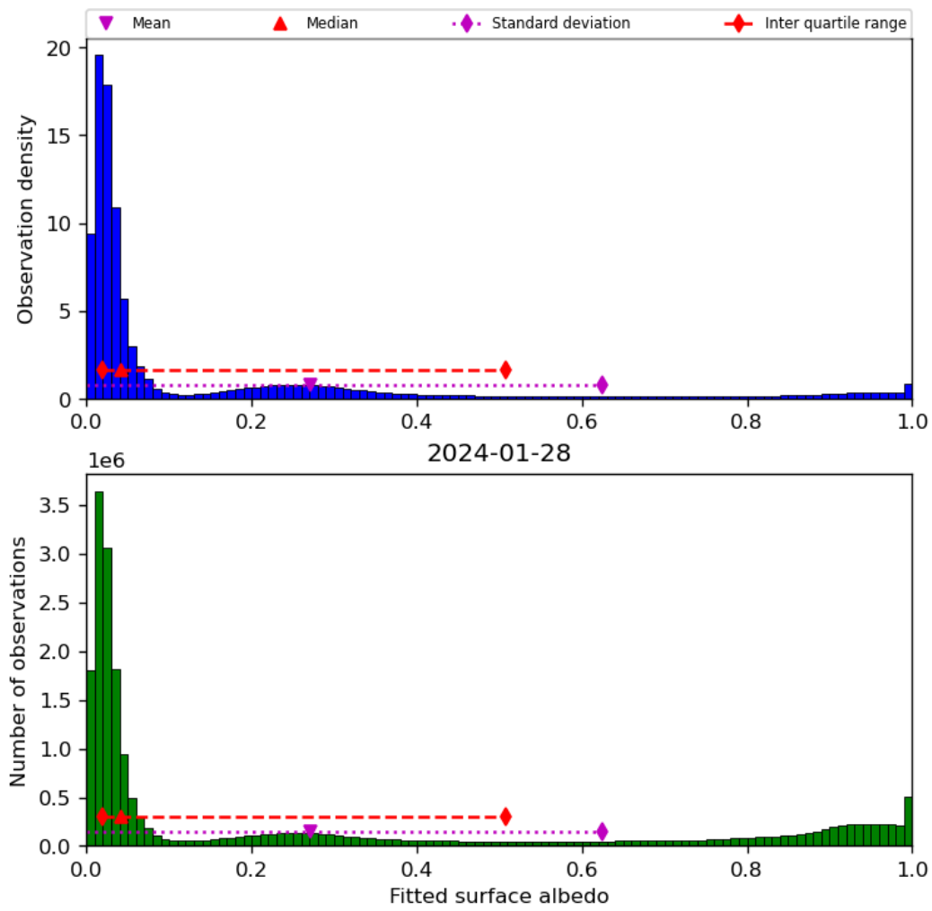
Figure 45: Histogram of “Fitted surface albedo” for 2024-01-27 to 2024-01-29
