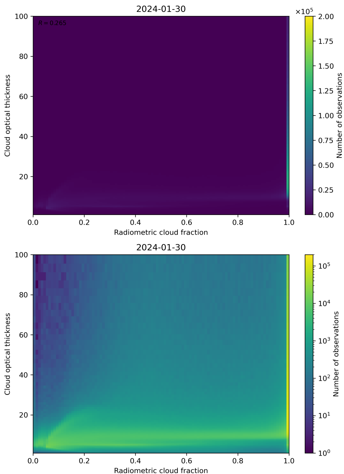
Figure 75: Scatter density plot of “Radiometric cloud fraction” against “Cloud optical thickness” for 2024-01-29 to 2024-01-31.
