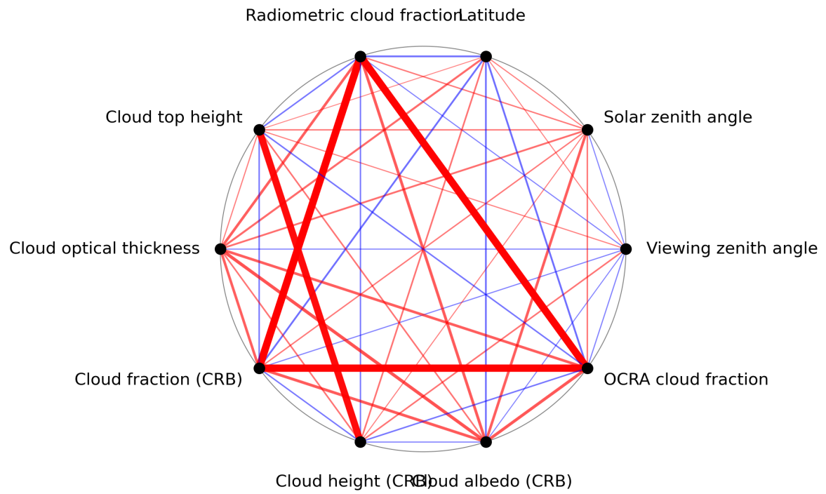
Figure 1: Map of correlation graph for 2024-01-29 to 2024-01-31.
