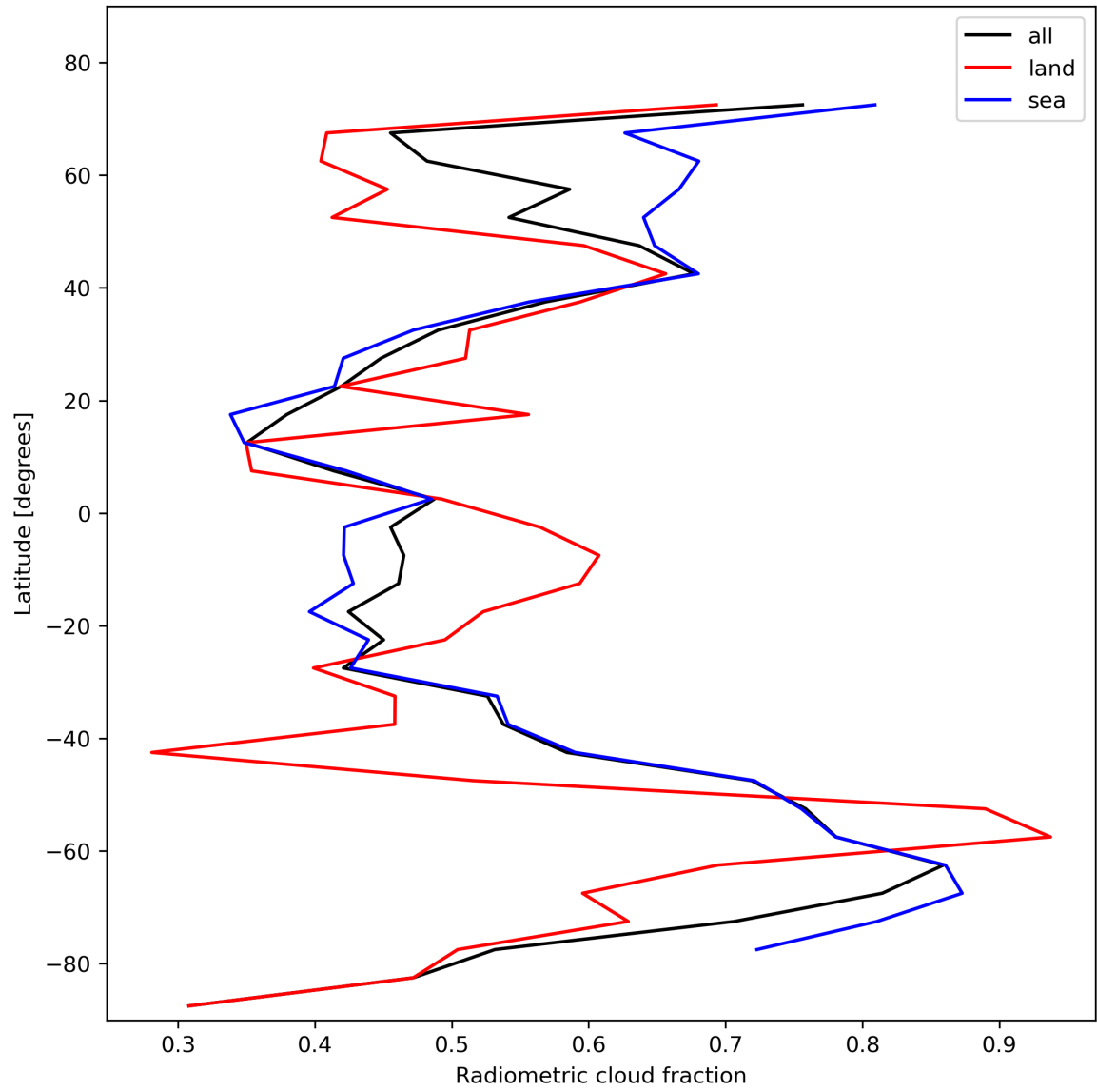
Figure 23: Zonal average of “Radiometric cloud fraction” for 2024-01-29 to 2024-01-31.
