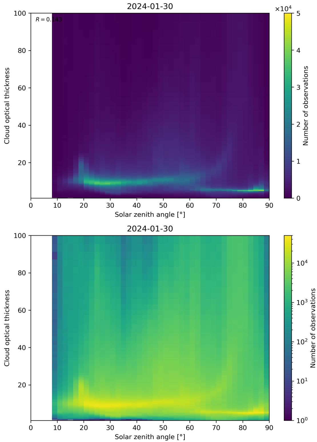
Figure 103: Scatter density plot of “Solar zenith angle” against “Cloud optical thickness” for 2024-01-29 to 2024-01-31.
