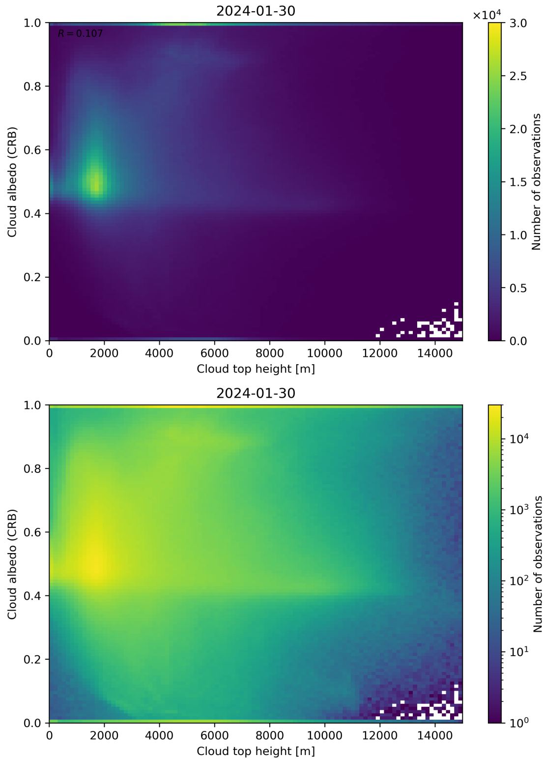
Figure 86: Scatter density plot of “Cloud top height” against “Cloud albedo (CRB)” for 2024-01-29 to 2024-01-31.
