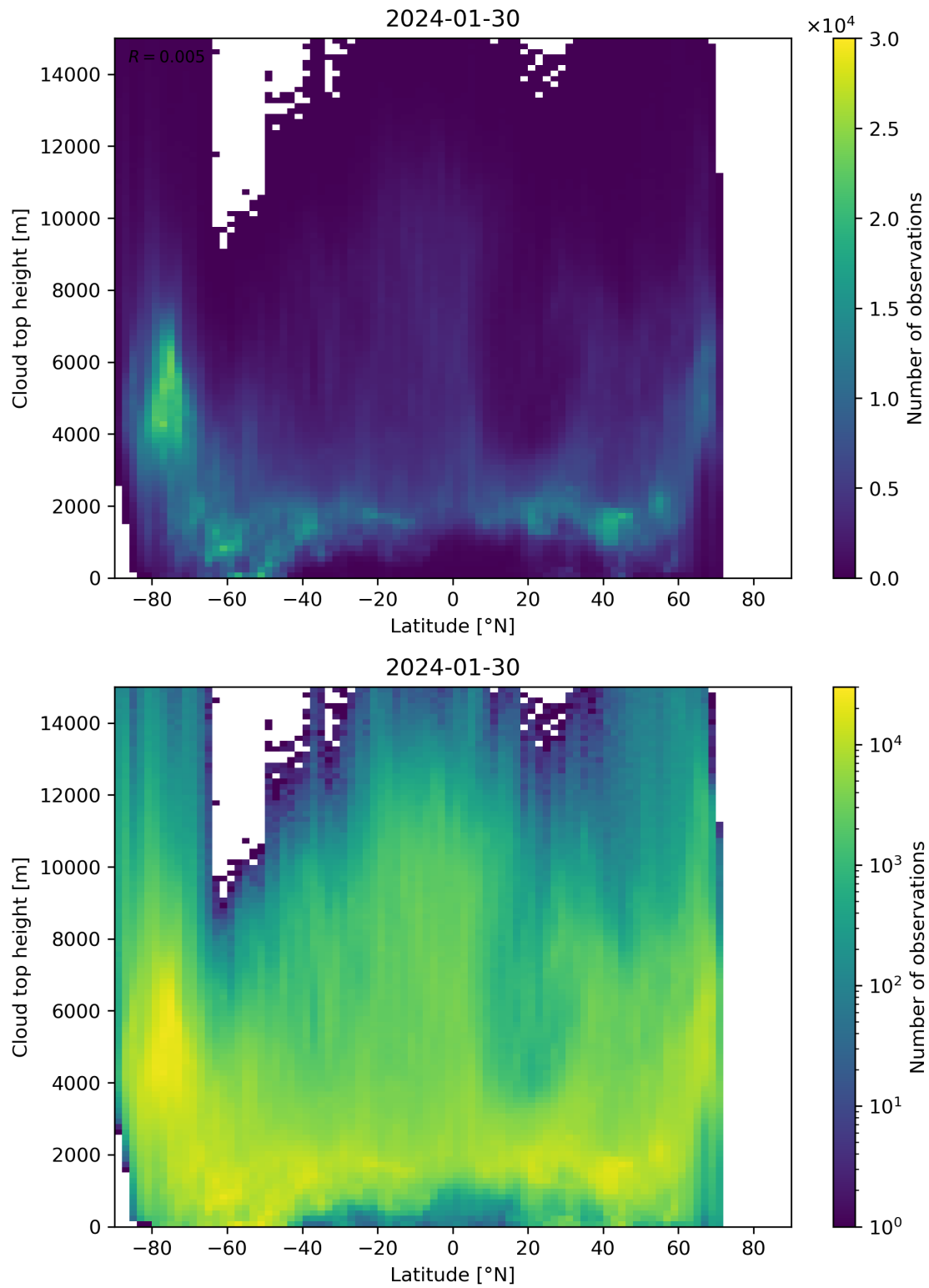
Figure 97: Scatter density plot of “Latitude” against “Cloud top height” for 2024-01-29 to 2024-01-31.
