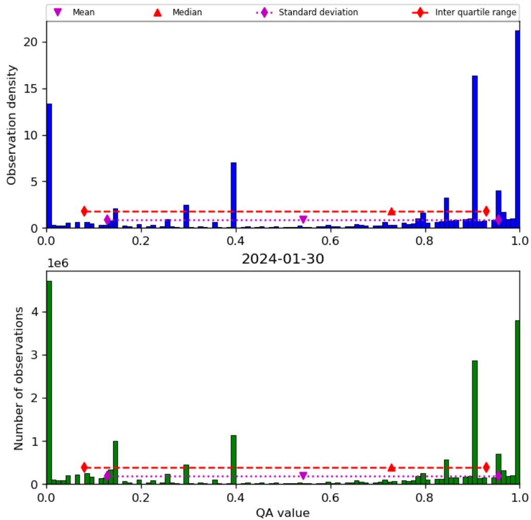
Figure 38: Histogram of “QA value” for 2024-01-29 to 2024-01-31
