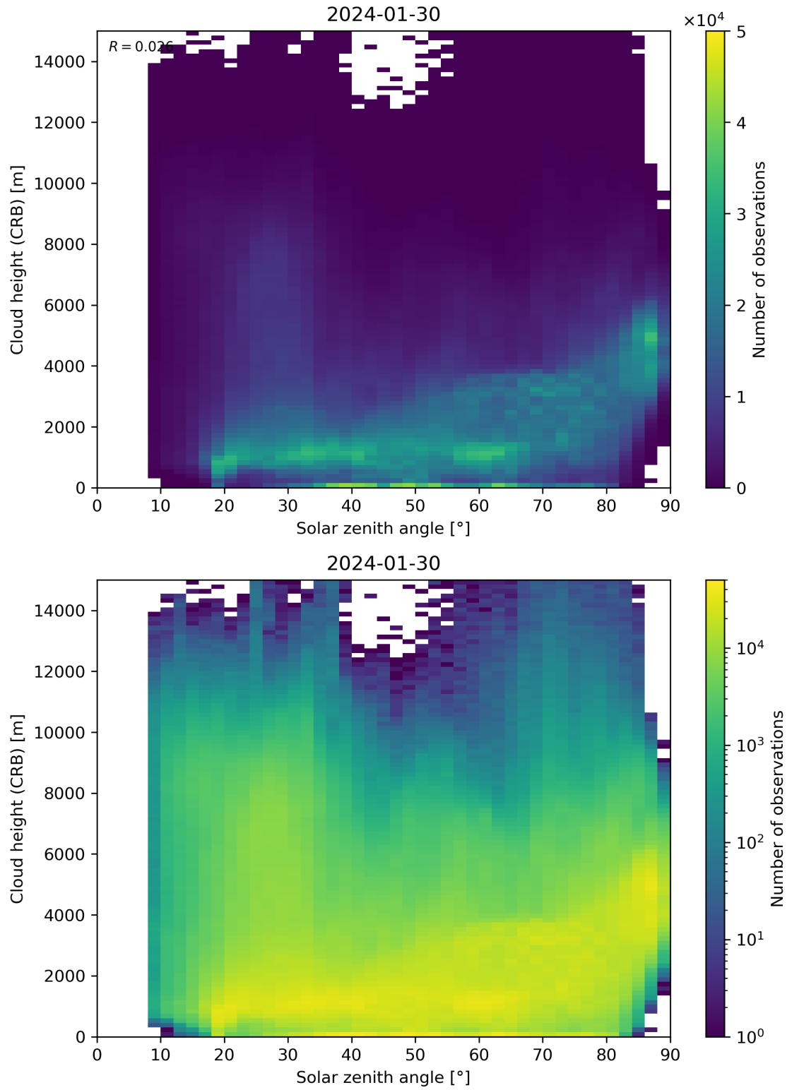
Figure 102: Scatter density plot of “Solar zenith angle” against “Cloud height (CRB)” for 2024-01-29 to 2024-01-31.
