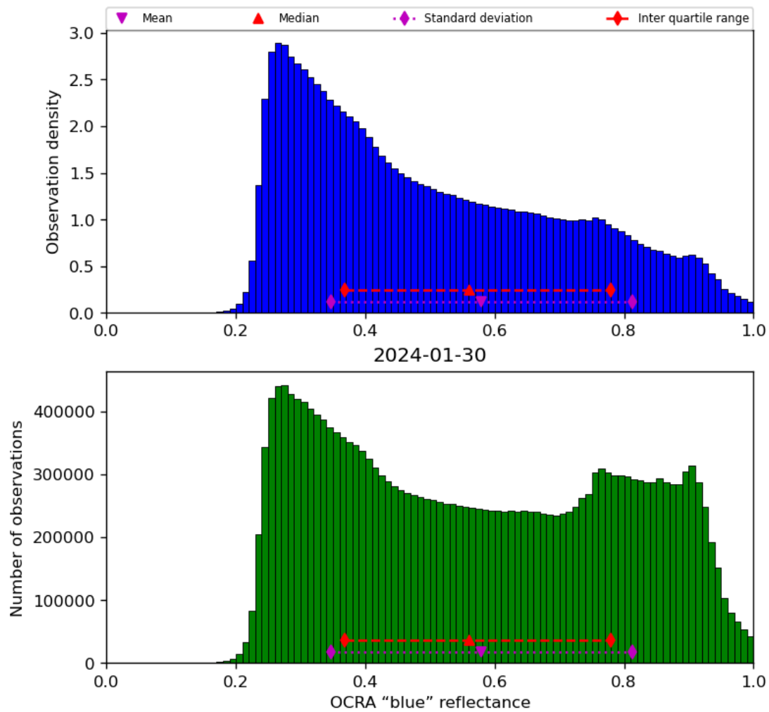
Figure 51: Histogram of “OCRA “blue” reflectance” for 2024-01-29 to 2024-01-31
