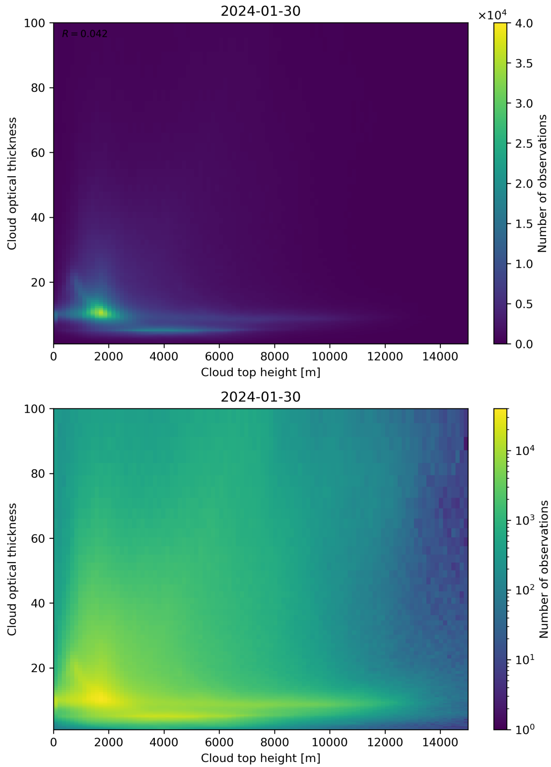
Figure 90: Scatter density plot of “Cloud top height” against “Cloud optical thickness” for 2024-01-29 to 2024-01-31.
