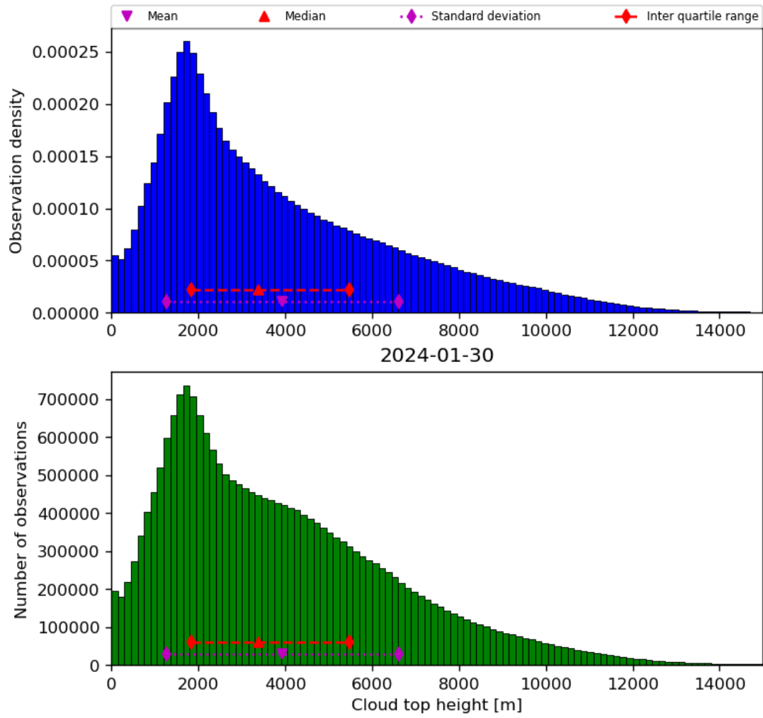
Figure 40: Histogram of “Cloud top height” for 2024-01-29 to 2024-01-31
