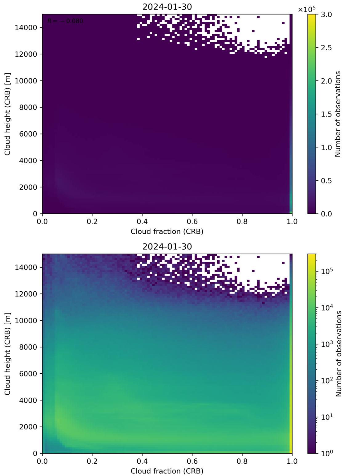
Figure 79: Scatter density plot of “Cloud fraction (CRB)” against “Cloud height (CRB)” for 2024-01-29 to 2024-01-31.
