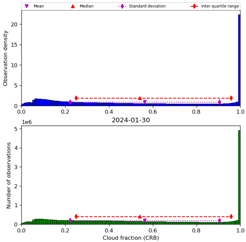
Figure 42: Histogram of “Cloud fraction (CRB)” for 2024-01-29 to 2024-01-31
