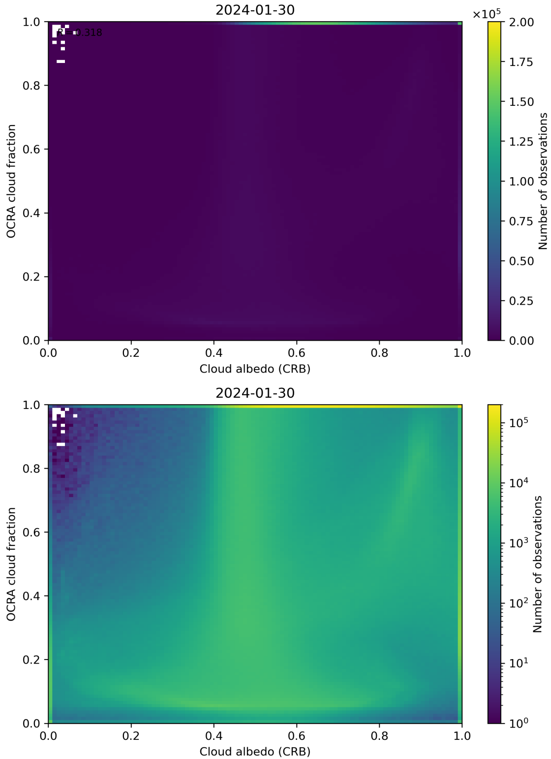
Figure 70: Scatter density plot of “Cloud albedo (CRB)” against “OCRA cloud fraction” for 2024-01-29 to 2024-01-31.
