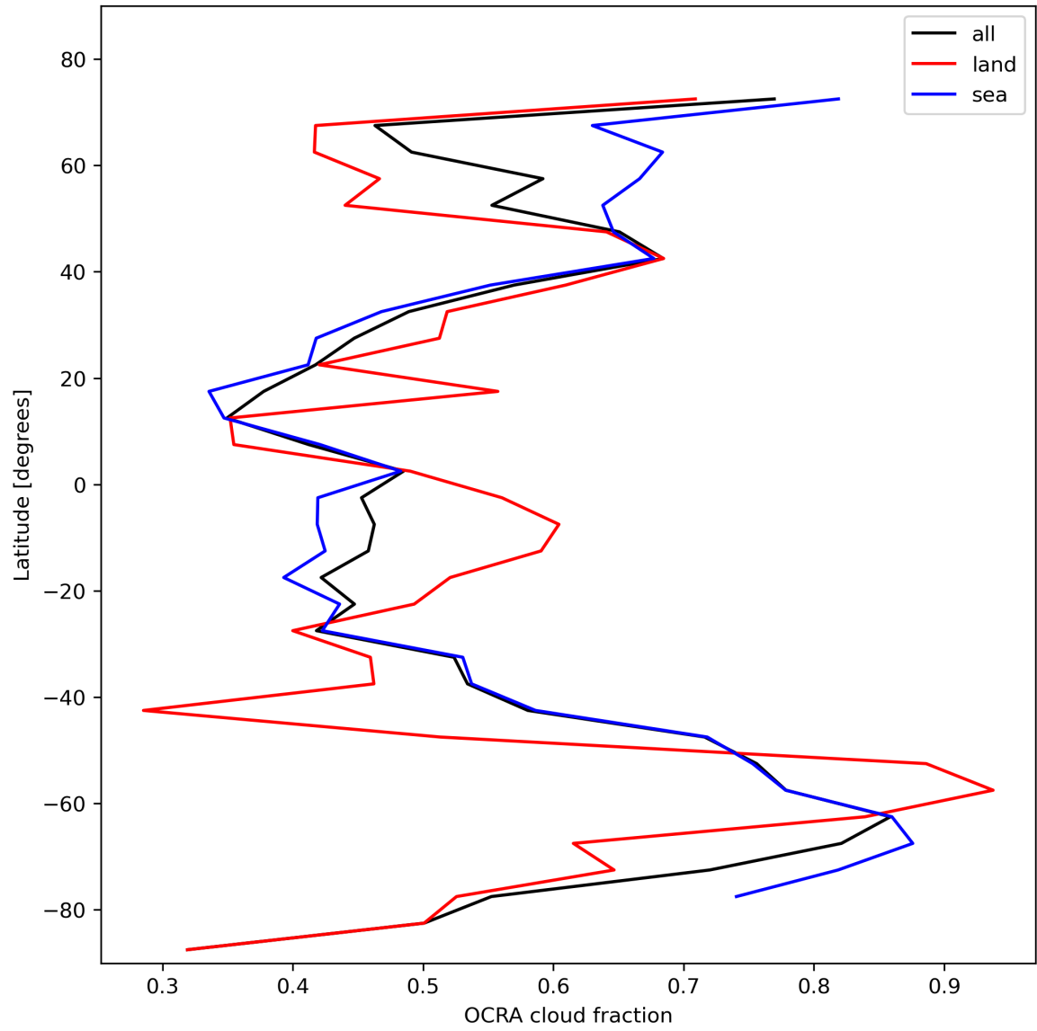
Figure 34: Zonal average of “OCRA cloud fraction” for 2024-01-29 to 2024-01-31.
