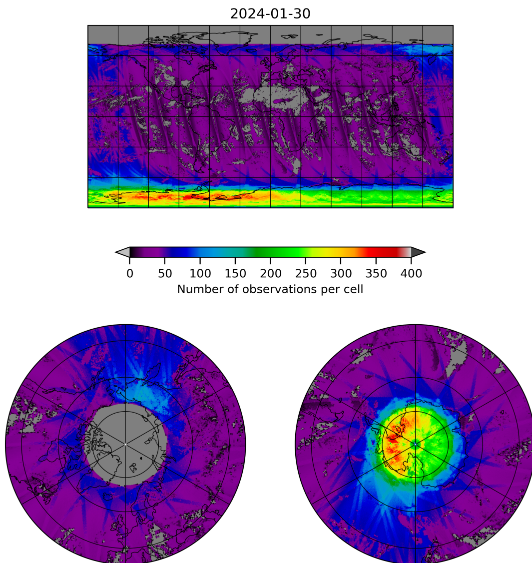
Figure 21: Map of the number of observations for 2024-01-29 to 2024-01-31
