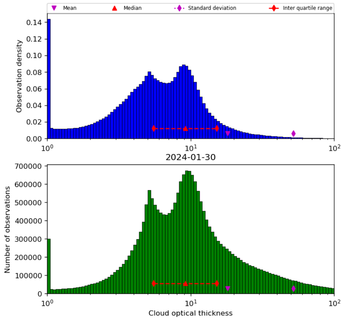
Figure 41: Histogram of “Cloud optical thickness” for 2024-01-29 to 2024-01-31
