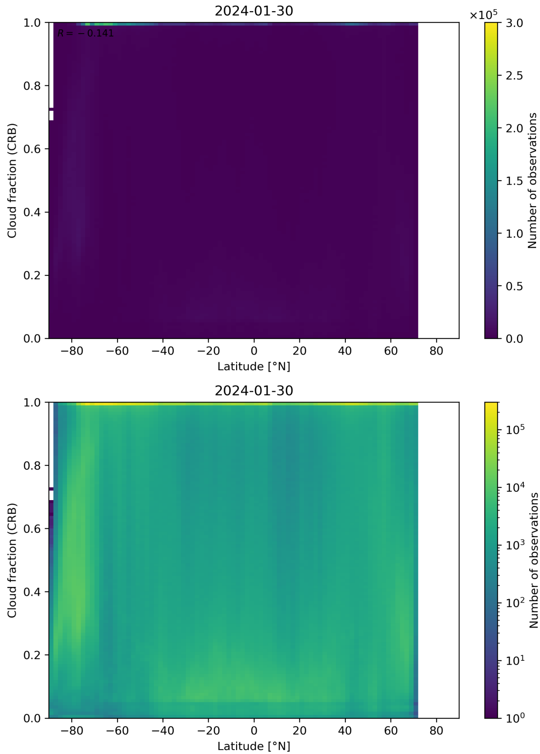
Figure 94: Scatter density plot of “Latitude” against “Cloud fraction (CRB)” for 2024-01-29 to 2024-01-31.
