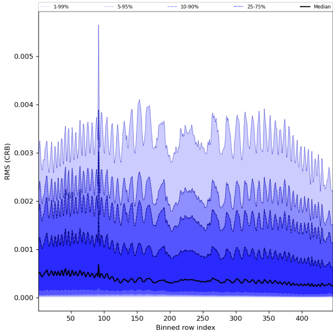
Figure 64: Along track statistics of “RMS (CRB)” for 2024-01-29 to 2024-01-31
