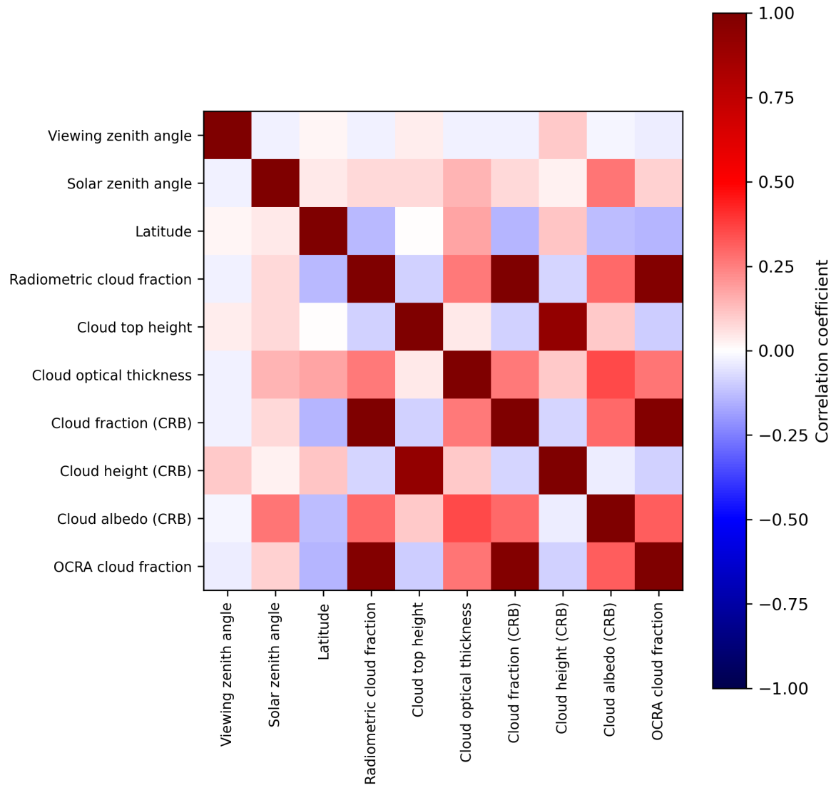
Figure 2: Map of correlation matrix for 2024-01-29 to 2024-01-31.
