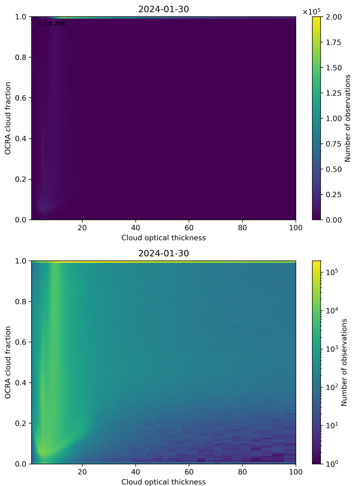
Figure 83: Scatter density plot of “Cloud optical thickness” against “OCRA cloud fraction” for 2024-01-29 to 2024-01-31.
