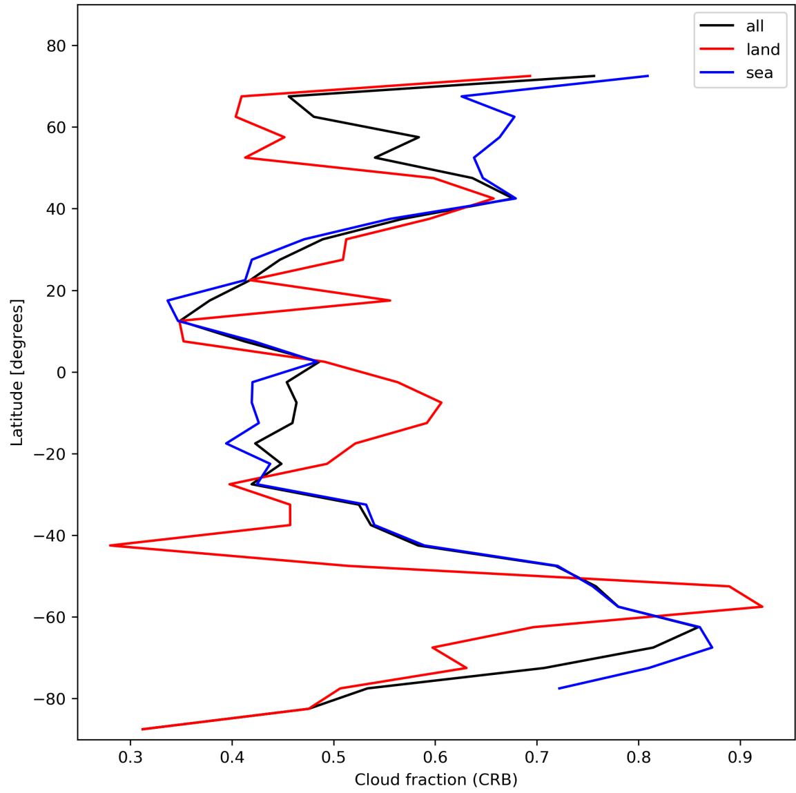
Figure 26: Zonal average of “Cloud fraction (CRB)” for 2024-01-29 to 2024-01-31.
