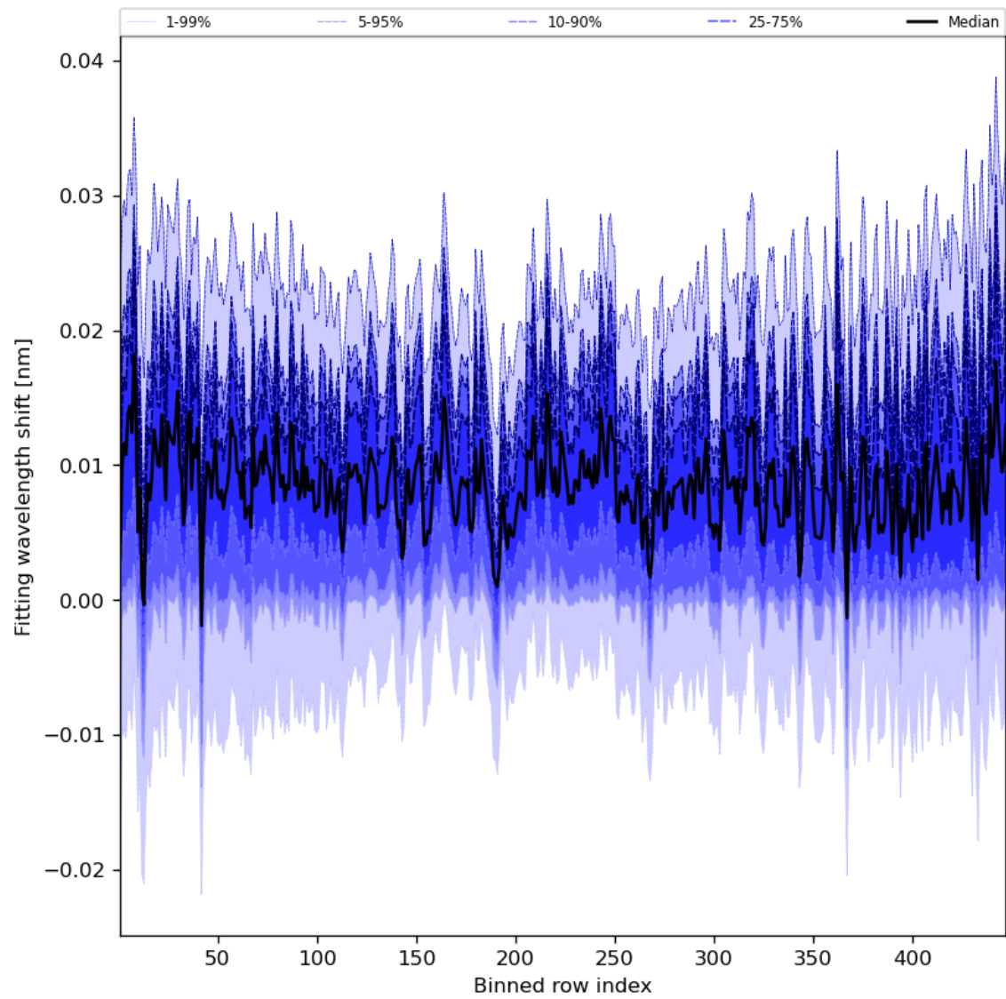
Figure 65: Along track statistics of “Fitting wavelength shift” for 2024-01-29 to 2024-01-31
