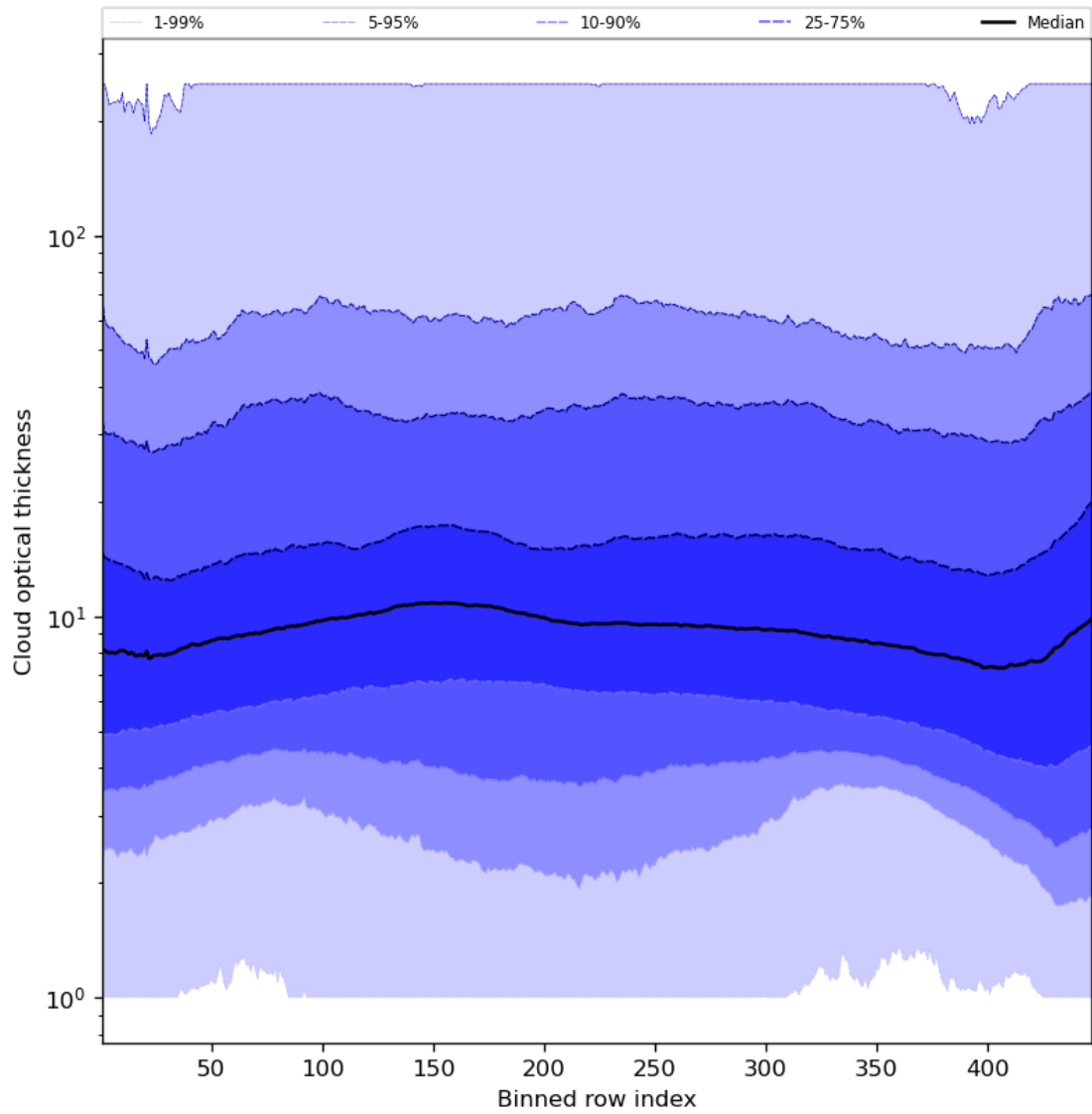
Figure 57: Along track statistics of “Cloud optical thickness” for 2024-01-29 to 2024-01-31
