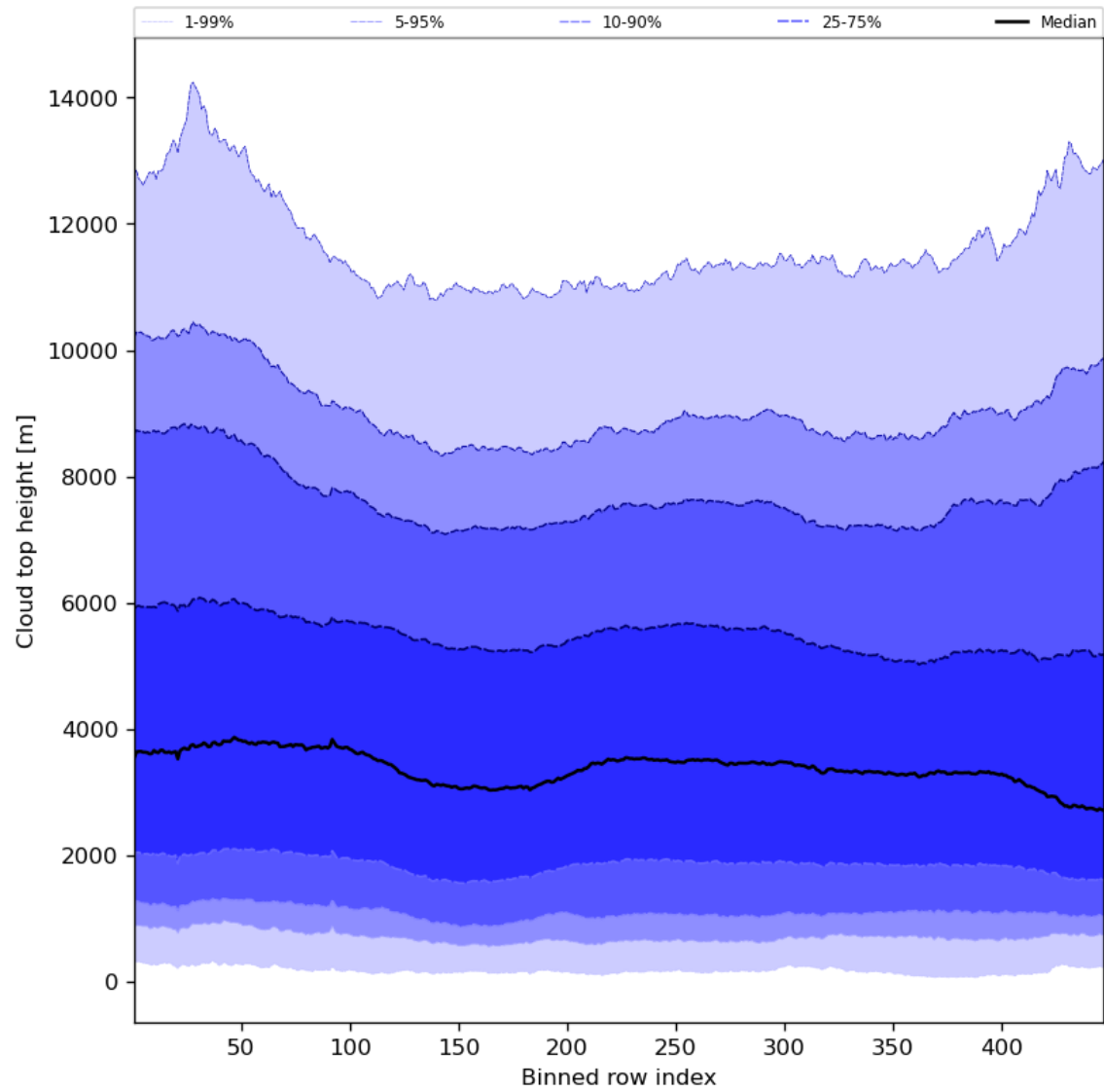
Figure 56: Along track statistics of “Cloud top height” for 2024-01-29 to 2024-01-31
