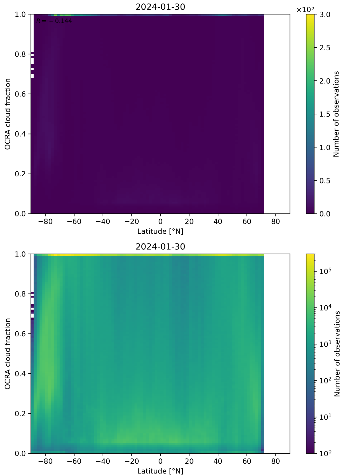
Figure 93: Scatter density plot of “Latitude” against “OCRA cloud fraction” for 2024-01-29 to 2024-01-31.
