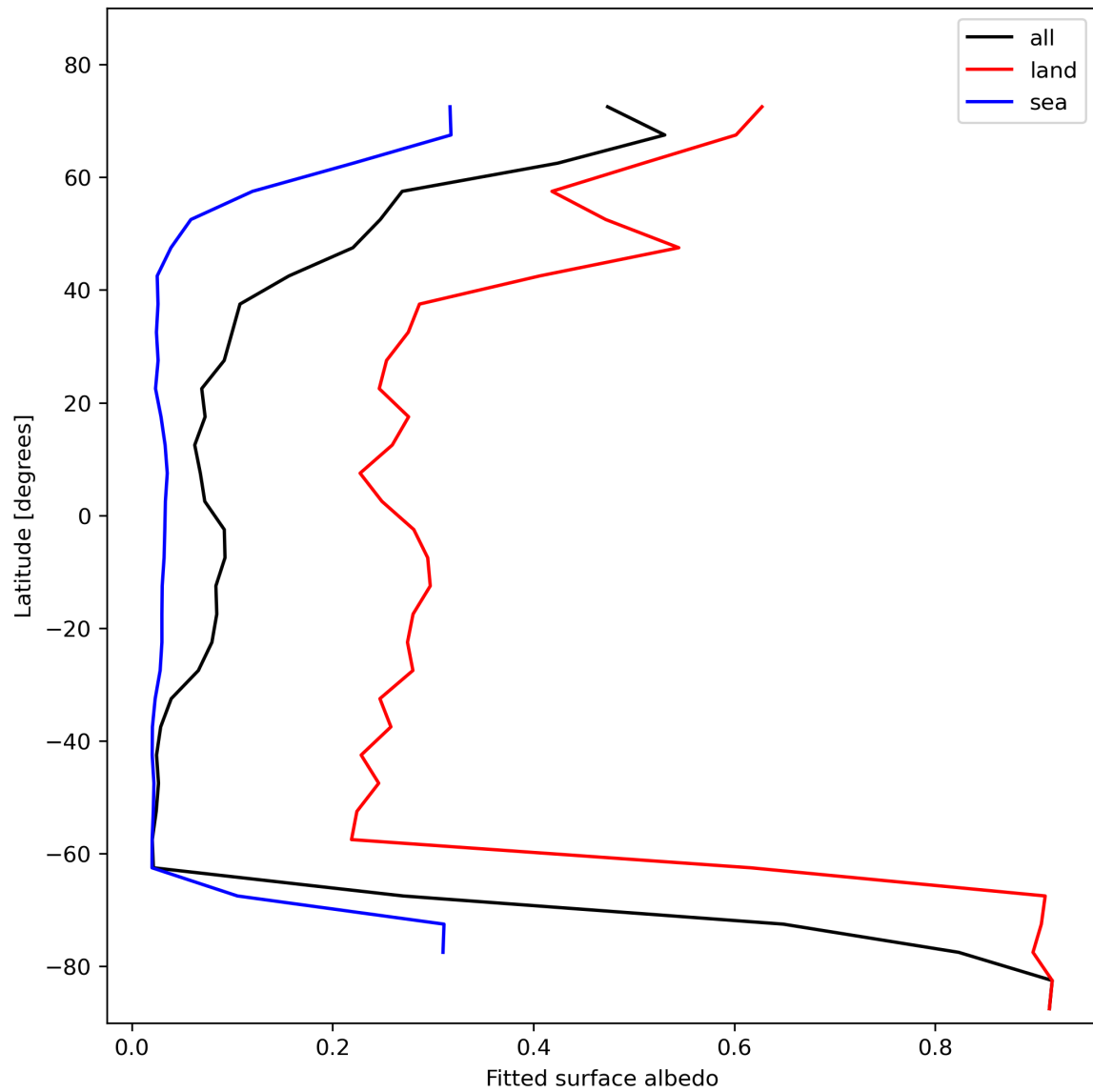
Figure 29: Zonal average of “Fitted surface albedo” for 2024-01-29 to 2024-01-31.
