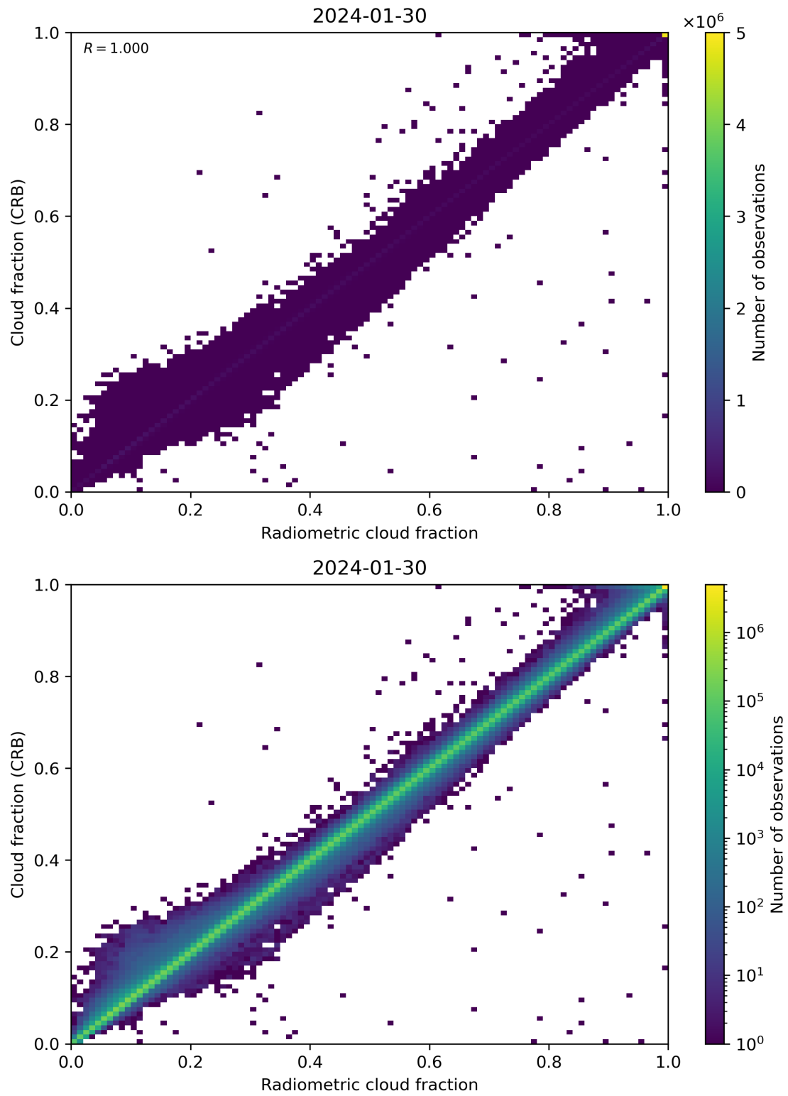
Figure 73: Scatter density plot of “Radiometric cloud fraction” against “Cloud fraction (CRB)” for 2024-01-29 to 2024-01-31.
