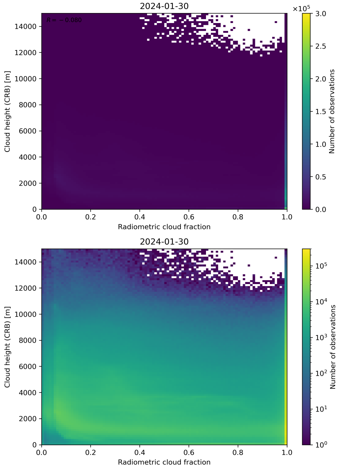
Figure 74: Scatter density plot of “Radiometric cloud fraction” against “Cloud height (CRB)” for 2024-01-29 to 2024-01-31.
