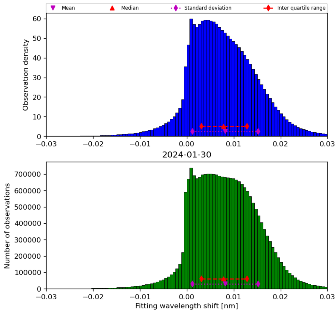
Figure 49: Histogram of “Fitting wavelength shift” for 2024-01-29 to 2024-01-31
