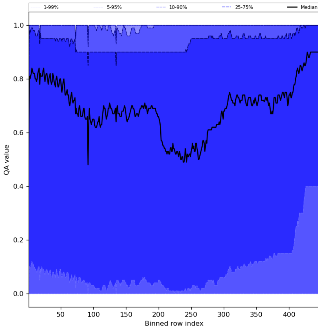
Figure 54: Along track statistics of “QA value” for 2024-01-29 to 2024-01-31
