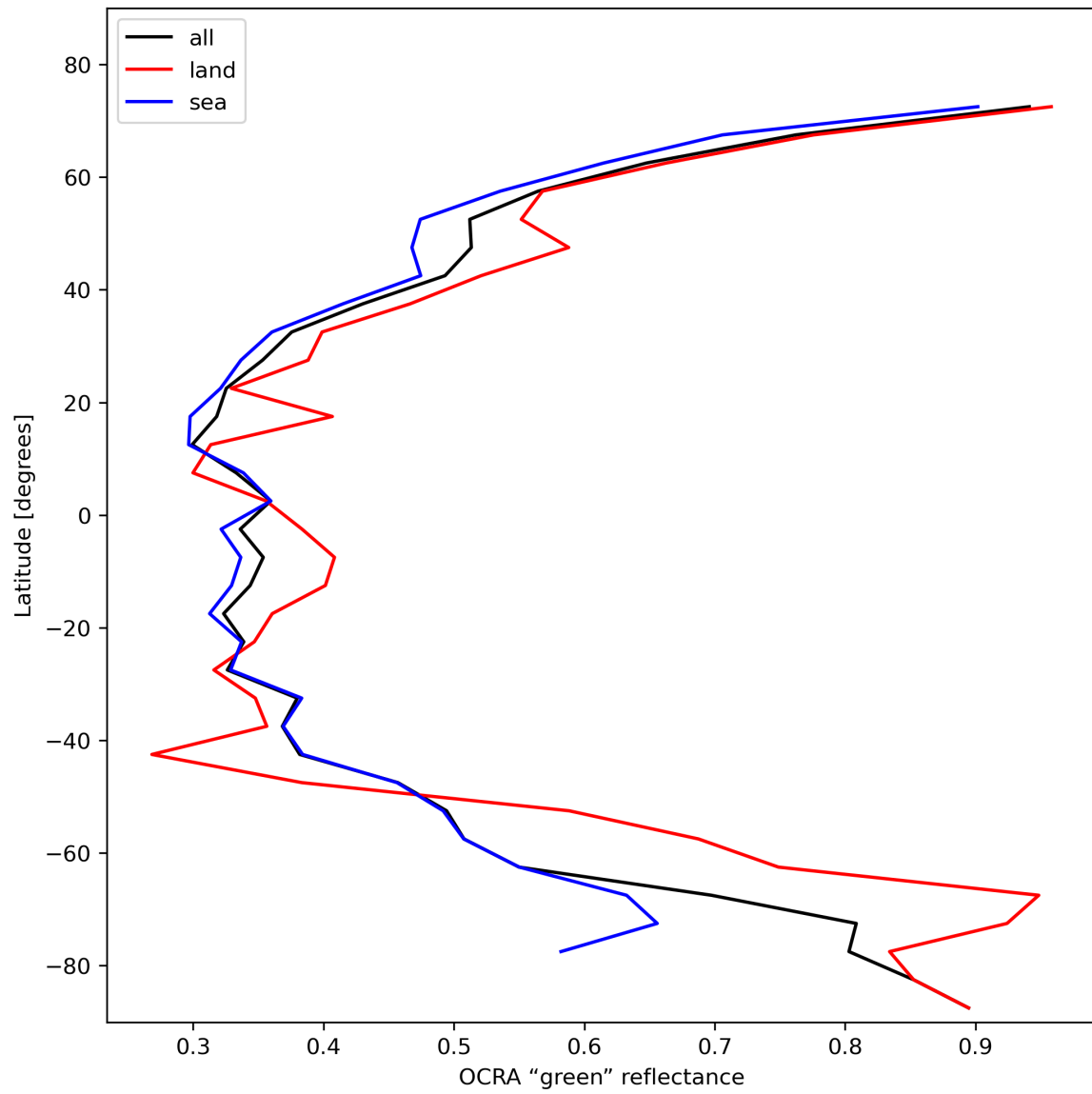
Figure 36: Zonal average of “OCRA “green” reflectance” for 2024-01-29 to 2024-01-31.
