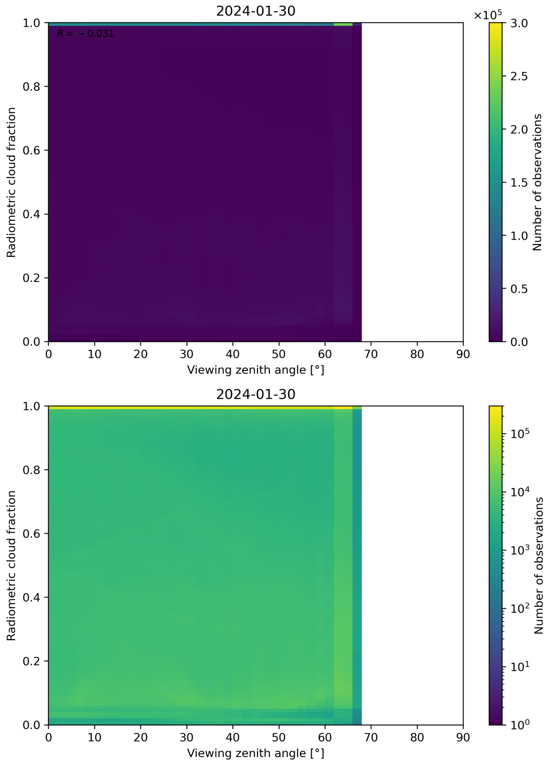
Figure 107: Scatter density plot of “Viewing zenith angle” against “Radiometric cloud fraction” for 2024-01-29 to 2024-01-31.
