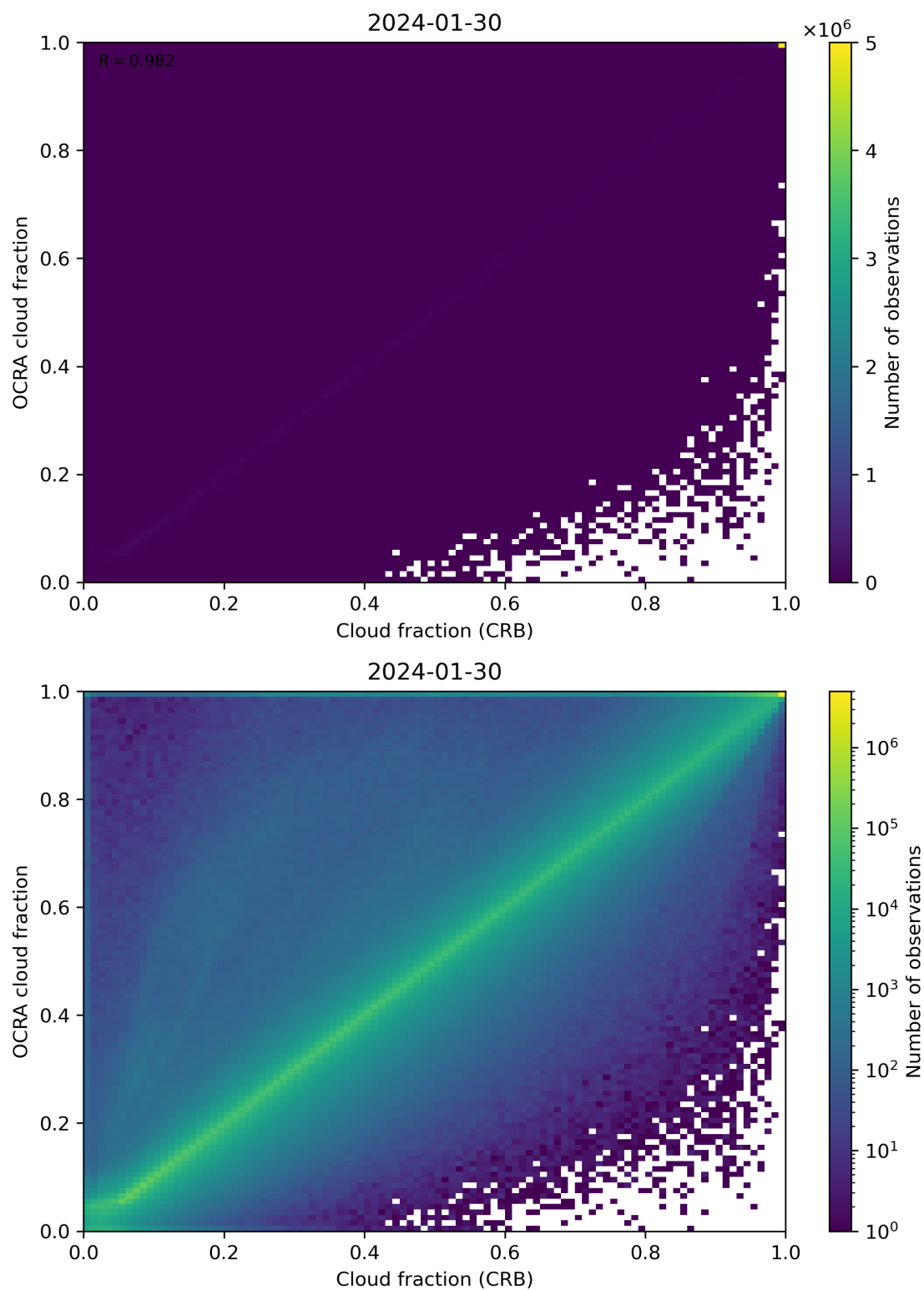
Figure 78: Scatter density plot of “Cloud fraction (CRB)” against “OCRA cloud fraction” for 2024-01-29 to 2024-01-31.
