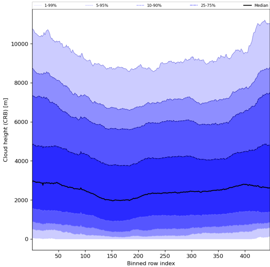
Figure 59: Along track statistics of “Cloud height (CRB)” for 2024-01-29 to 2024-01-31
