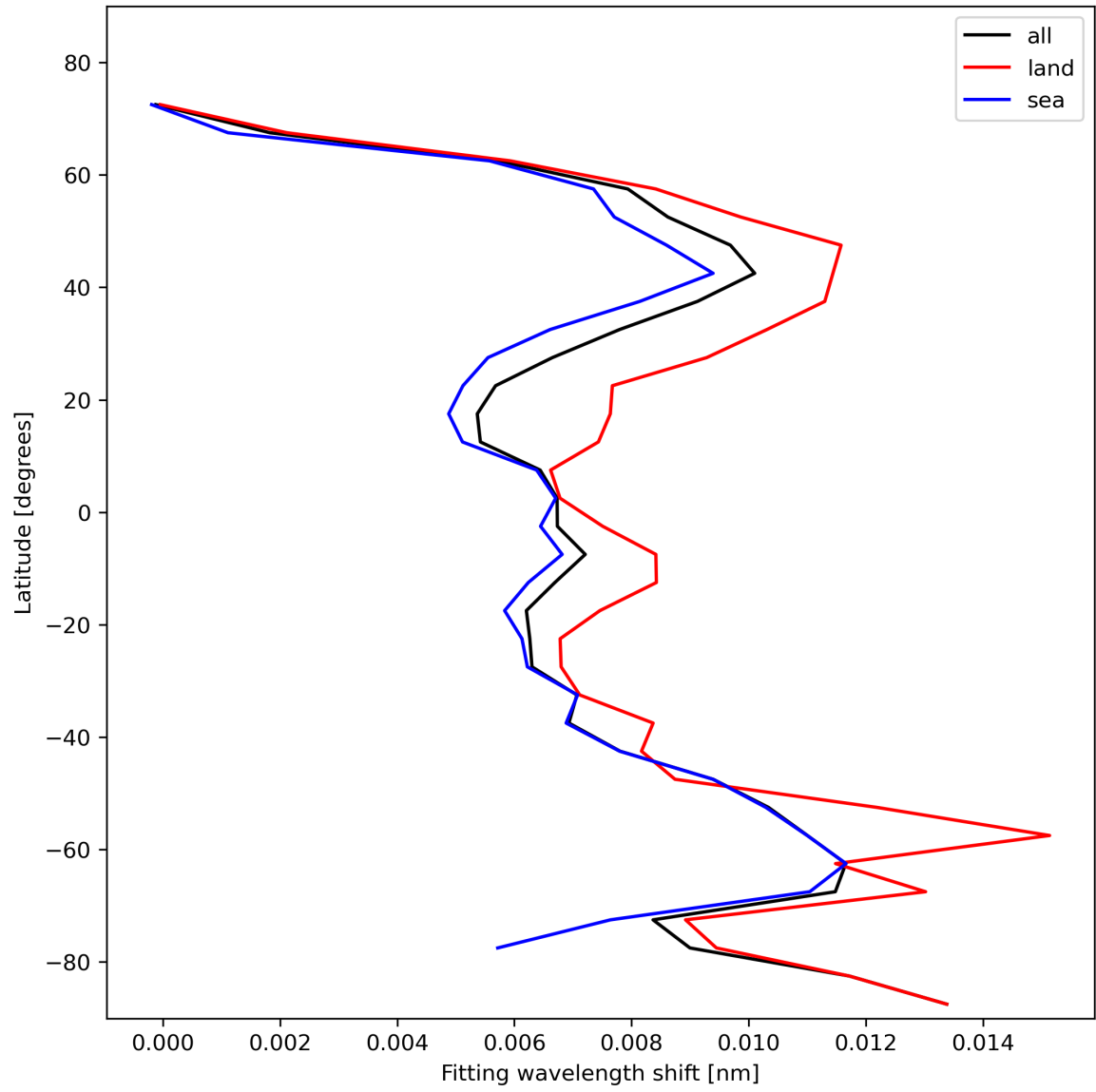
Figure 33: Zonal average of “Fitting wavelength shift” for 2024-01-29 to 2024-01-31.
