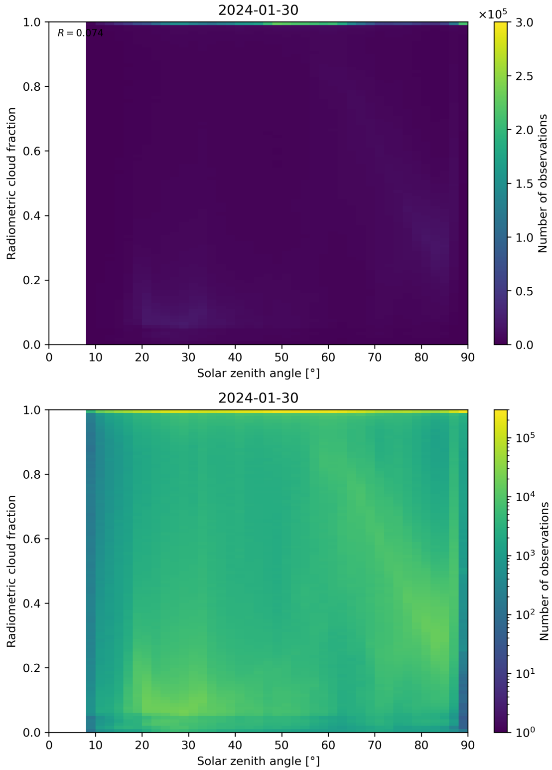
Figure 99: Scatter density plot of “Solar zenith angle” against “Radiometric cloud fraction” for 2024-01-29 to 2024-01-31.
