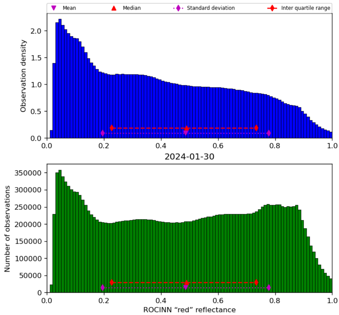
Figure 53: Histogram of “ROCINN “red” reflectance” for 2024-01-29 to 2024-01-31
