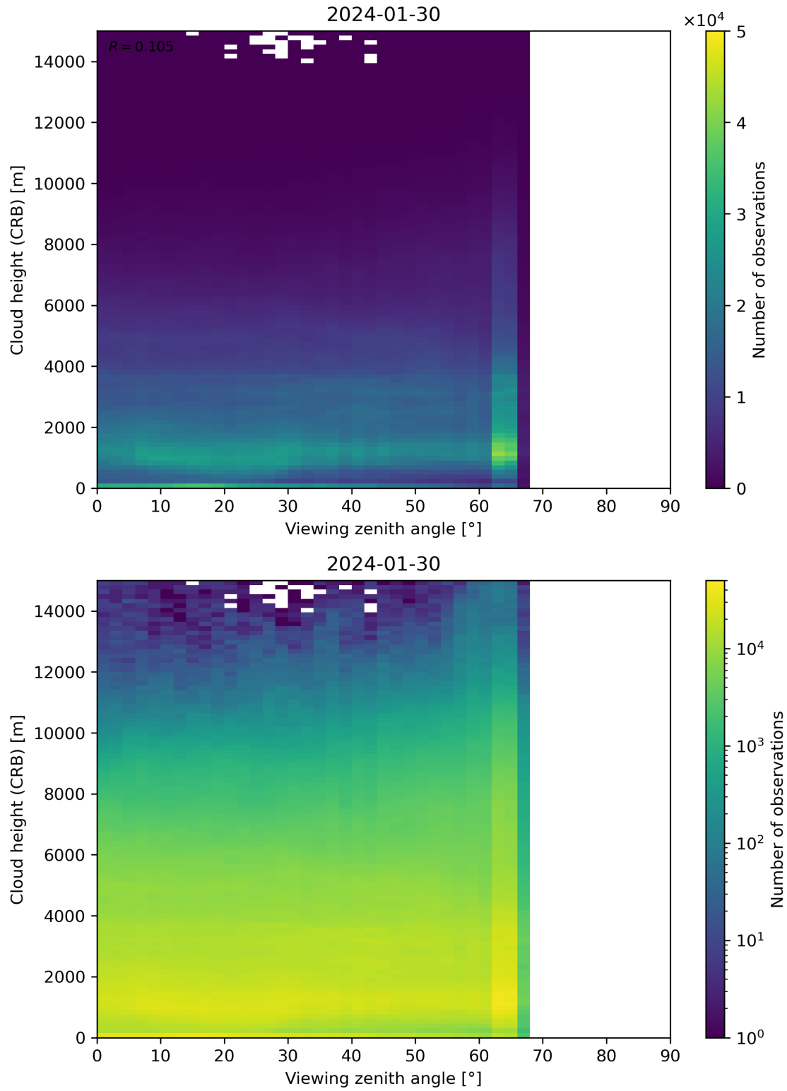
Figure 110: Scatter density plot of “Viewing zenith angle” against “Cloud height (CRB)” for 2024-01-29 to 2024-01-31.
