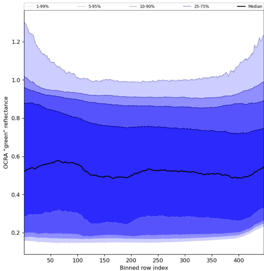
Figure 68: Along track statistics of "OCRA "green" reflectance" for 2024-01-29 to 2024-01-31
