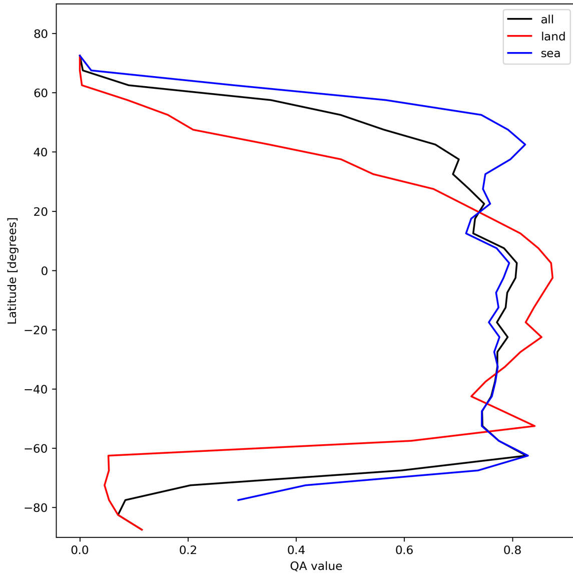
Figure 22: Zonal average of “QA value” for 2024-01-29 to 2024-01-31.
