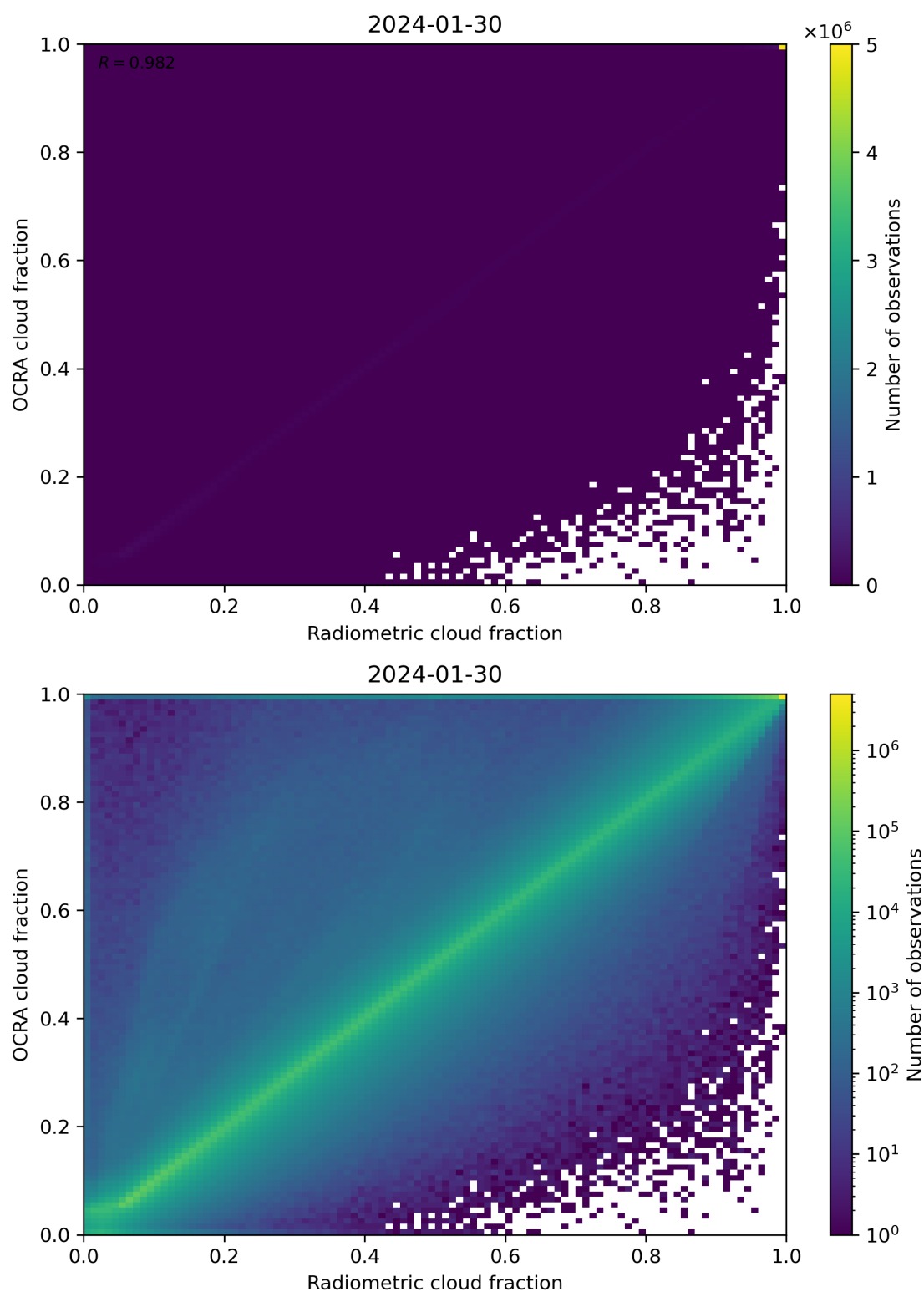
Figure 72: Scatter density plot of “Radiometric cloud fraction” against “OCRA cloud fraction” for 2024-01-29 to 2024-01-31.
