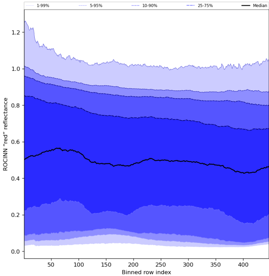
Figure 69: Along track statistics of "ROCINN "red" reflectance" for 2024-01-29 to 2024-01-31
