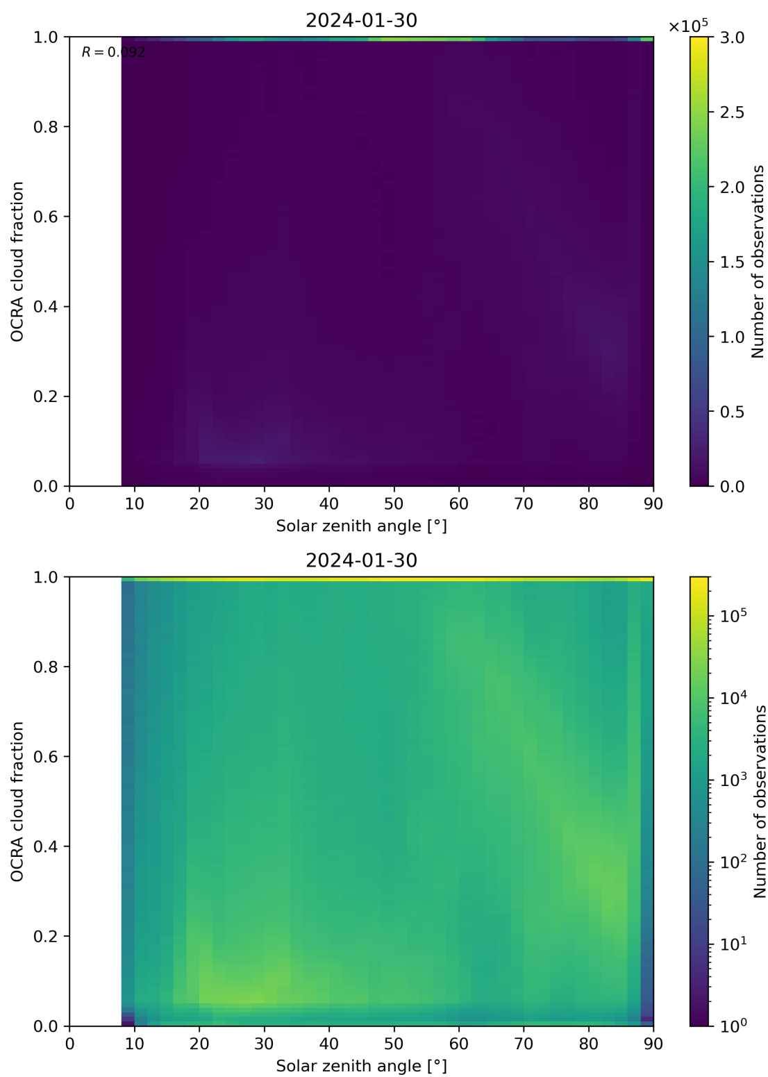
Figure 100: Scatter density plot of “Solar zenith angle” against “OCRA cloud fraction” for 2024-01-29 to 2024-01-31.
