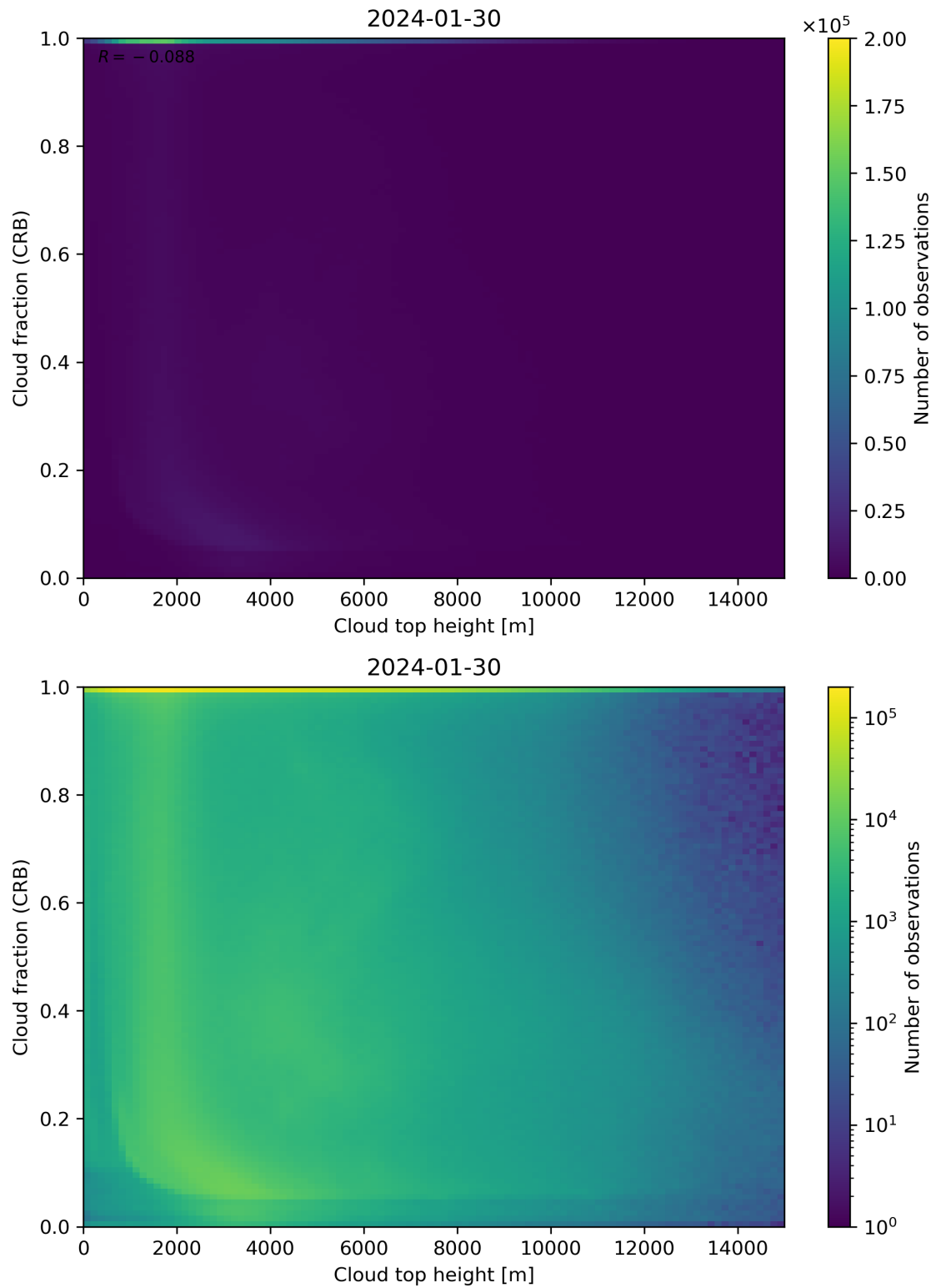
Figure 88: Scatter density plot of “Cloud top height” against “Cloud fraction (CRB)” for 2024-01-29 to 2024-01-31.
