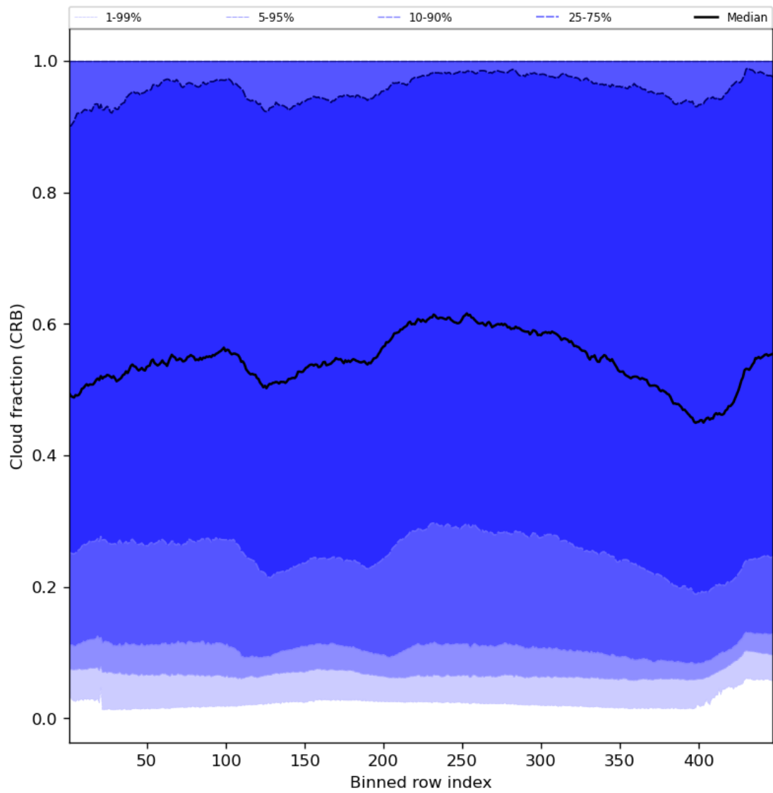
Figure 58: Along track statistics of “Cloud fraction (CRB)” for 2024-01-29 to 2024-01-31
