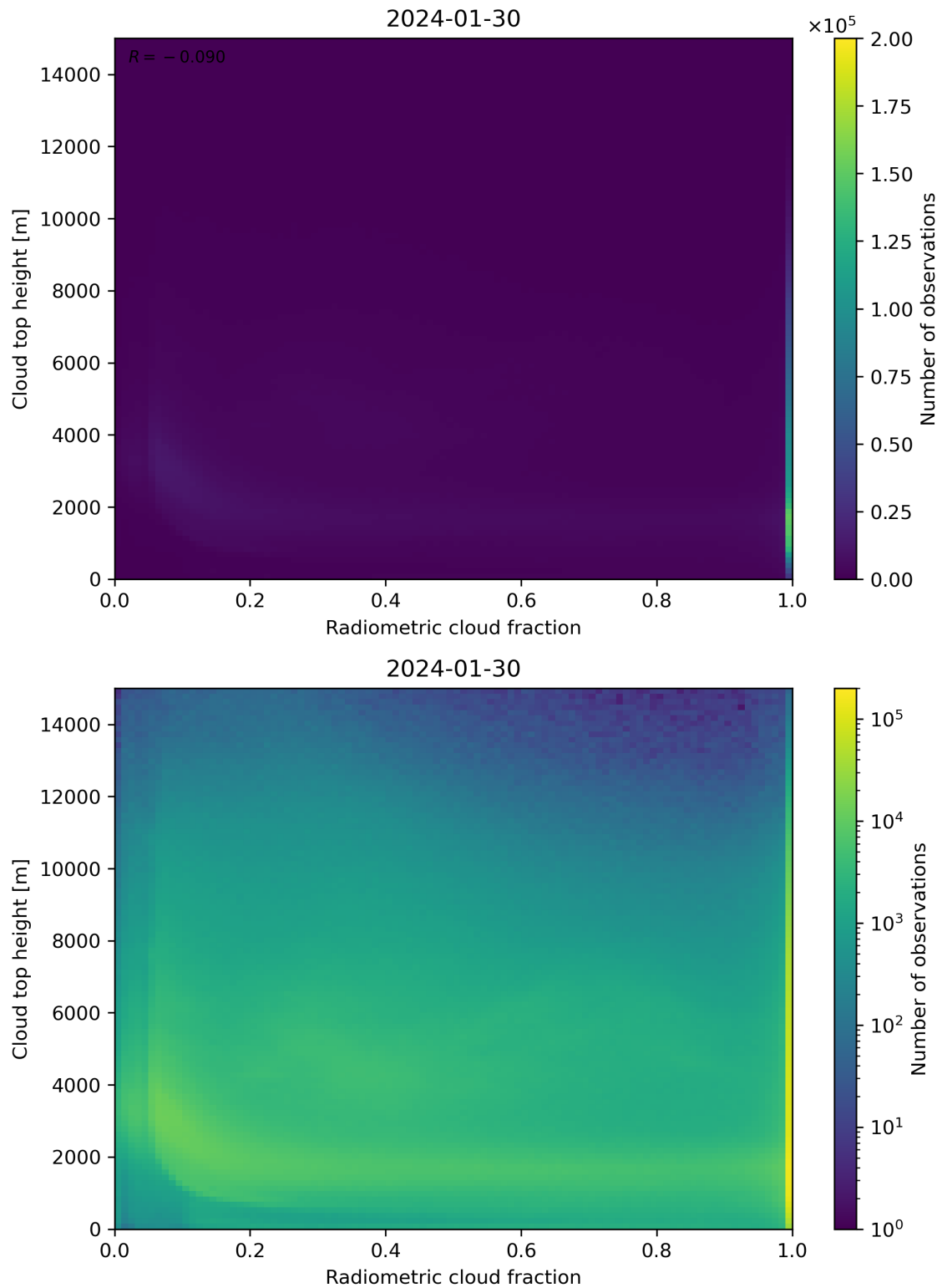
Figure 76: Scatter density plot of “Radiometric cloud fraction” against “Cloud top height” for 2024-01-29 to 2024-01-31.
