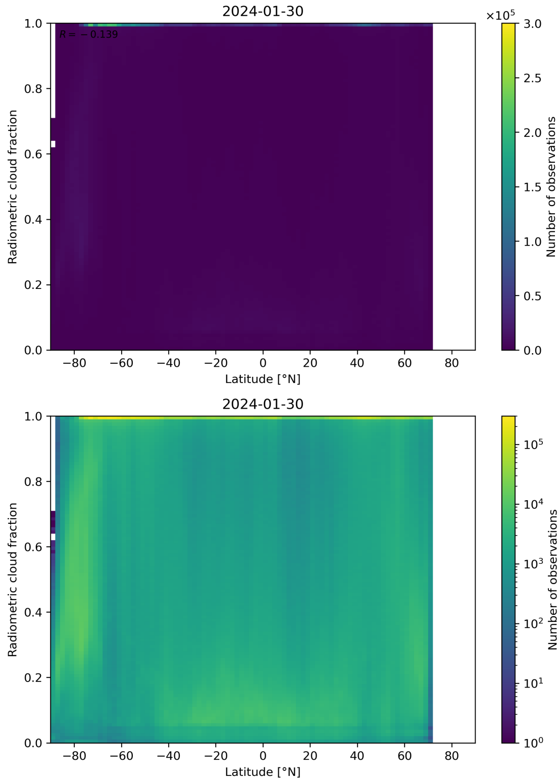
Figure 92: Scatter density plot of “Latitude” against “Radiometric cloud fraction” for 2024-01-29 to 2024-01-31.
