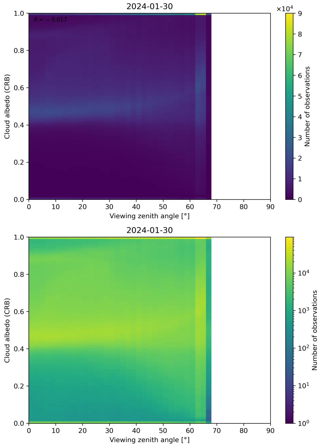
Figure 106: Scatter density plot of “Viewing zenith angle” against “Cloud albedo (CRB)” for 2024-01-29 to 2024-01-31.
