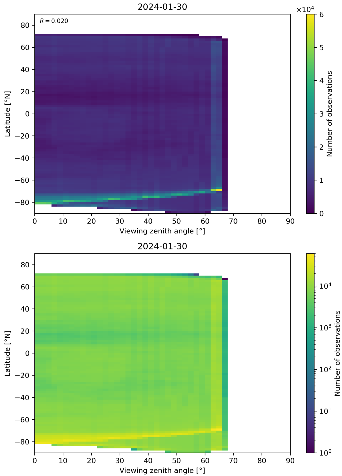
Figure 113: Scatter density plot of “Viewing zenith angle” against “Latitude” for 2024-01-29 to 2024-01-31.
