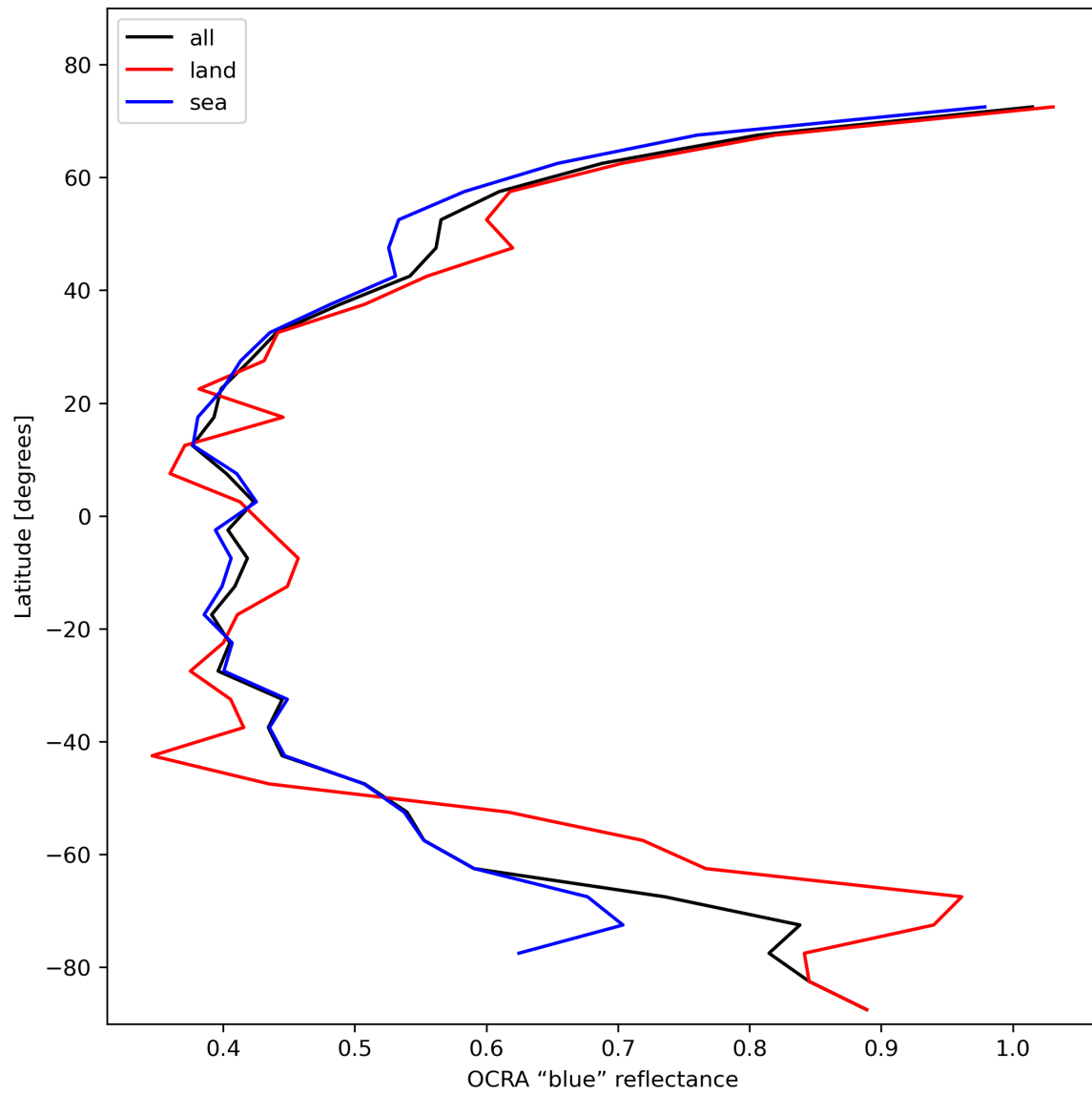
Figure 35: Zonal average of “OCRA “blue” reflectance” for 2024-01-29 to 2024-01-31.
