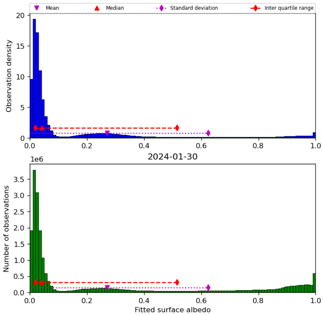
Figure 45: Histogram of “Fitted surface albedo” for 2024-01-29 to 2024-01-31
