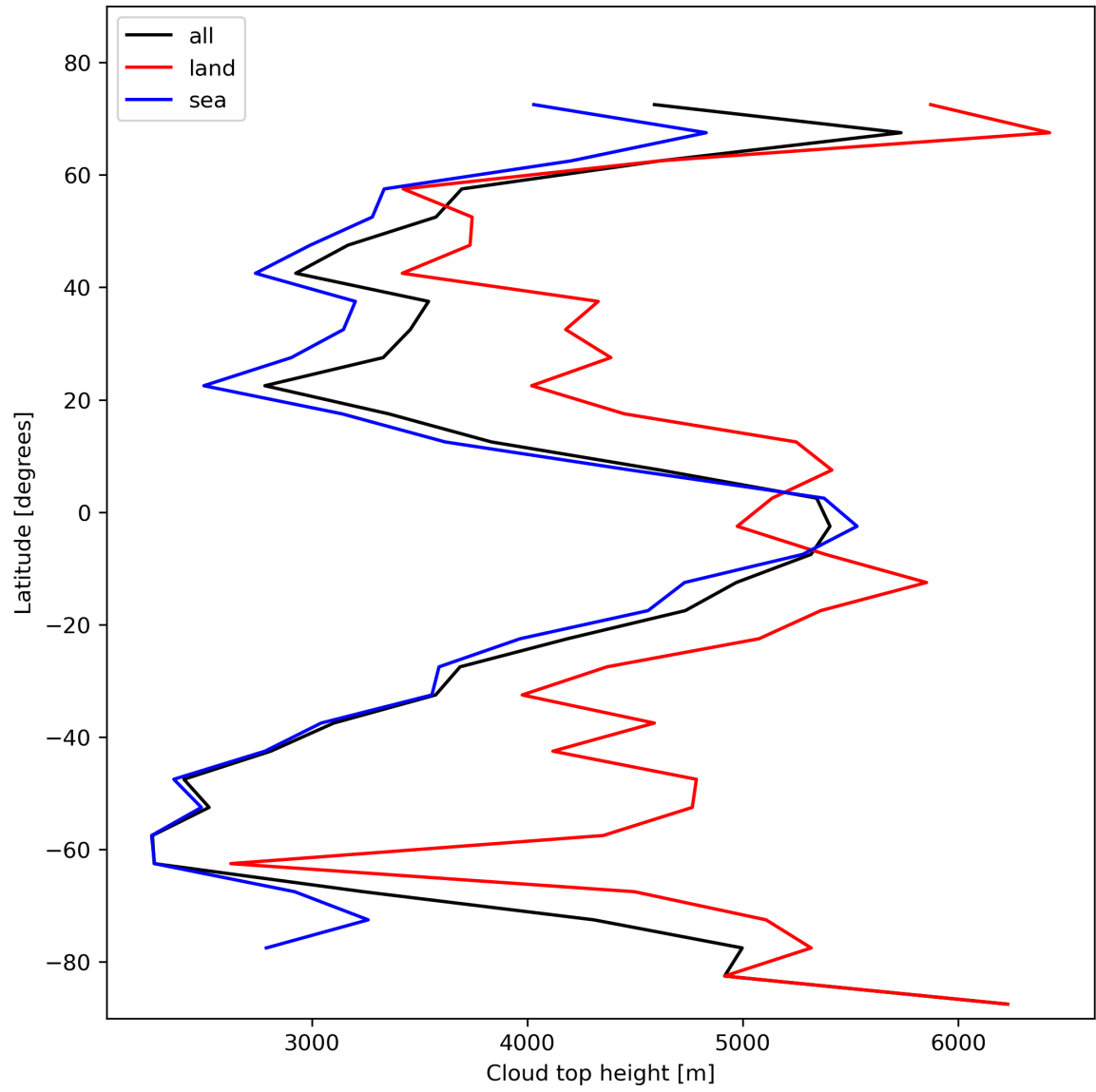
Figure 24: Zonal average of “Cloud top height” for 2024-01-29 to 2024-01-31.
