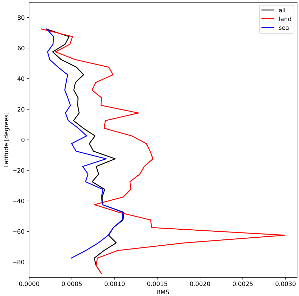
Figure 31: Zonal average of “RMS” for 2024-01-29 to 2024-01-31.
