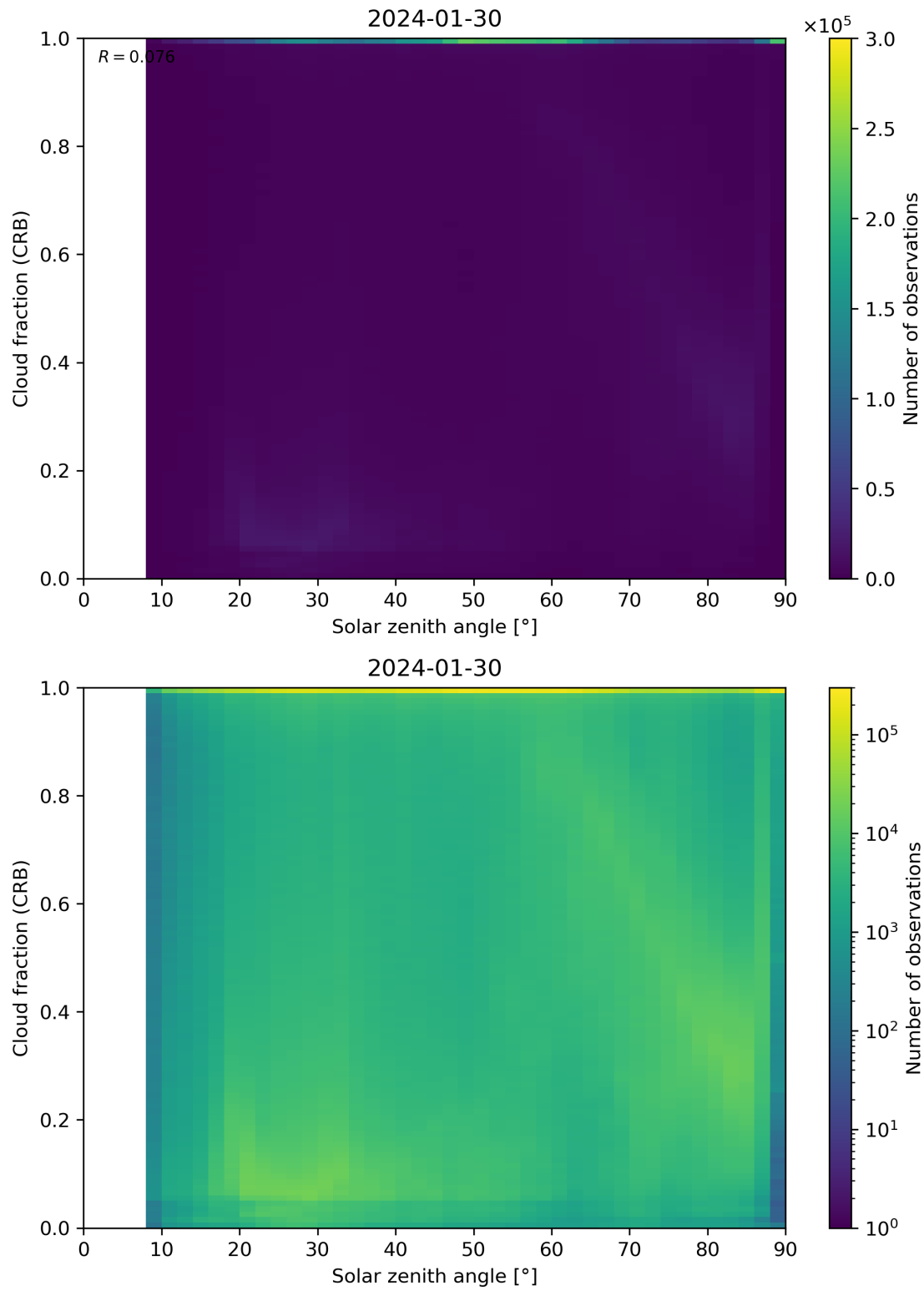
Figure 101: Scatter density plot of “Solar zenith angle” against “Cloud fraction (CRB)” for 2024-01-29 to 2024-01-31.
