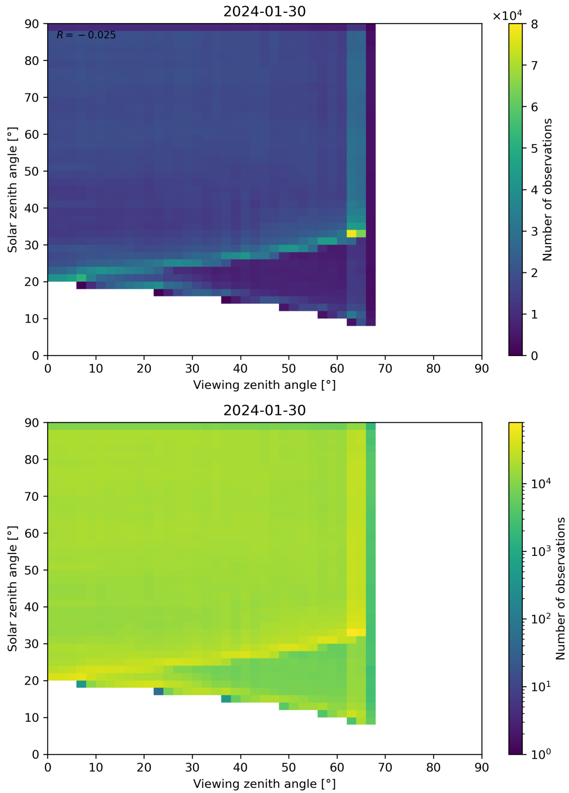
Figure 114: Scatter density plot of “Viewing zenith angle” against “Solar zenith angle” for 2024-01-29 to 2024-01-31.
