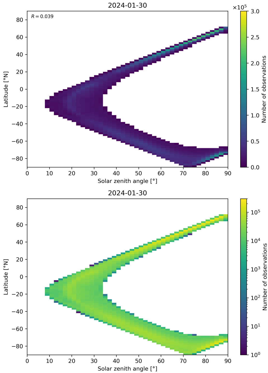
Figure 105: Scatter density plot of “Solar zenith angle” against “Latitude” for 2024-01-29 to 2024-01-31.
