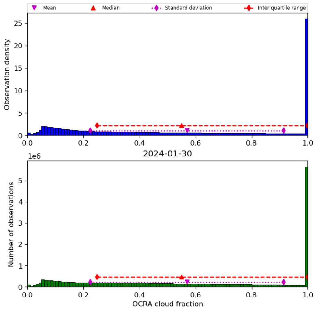
Figure 50: Histogram of “OCRA cloud fraction” for 2024-01-29 to 2024-01-31
