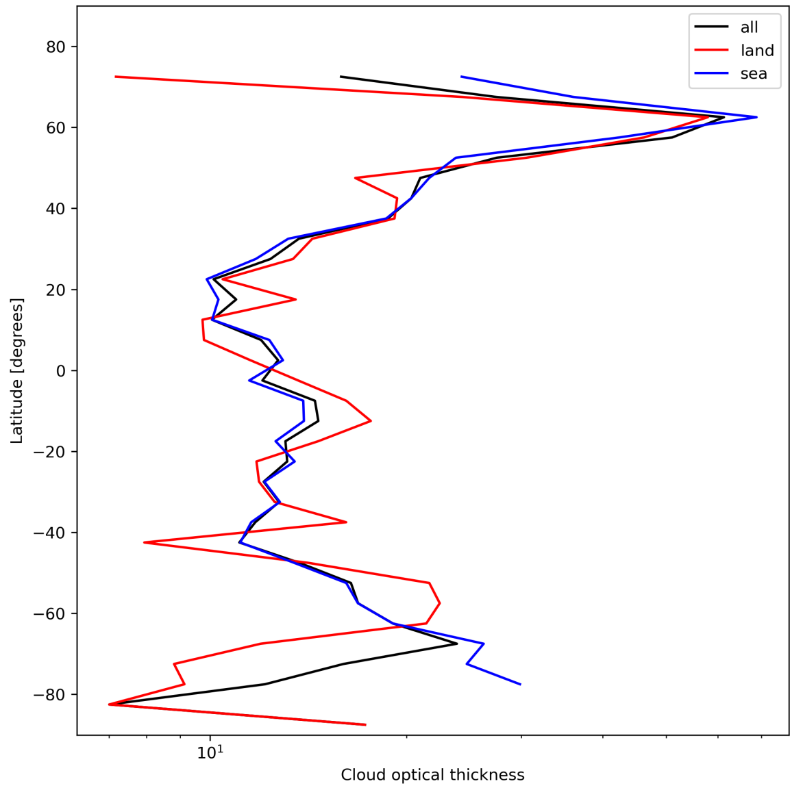
Figure 25: Zonal average of “Cloud optical thickness” for 2024-01-29 to 2024-01-31.
