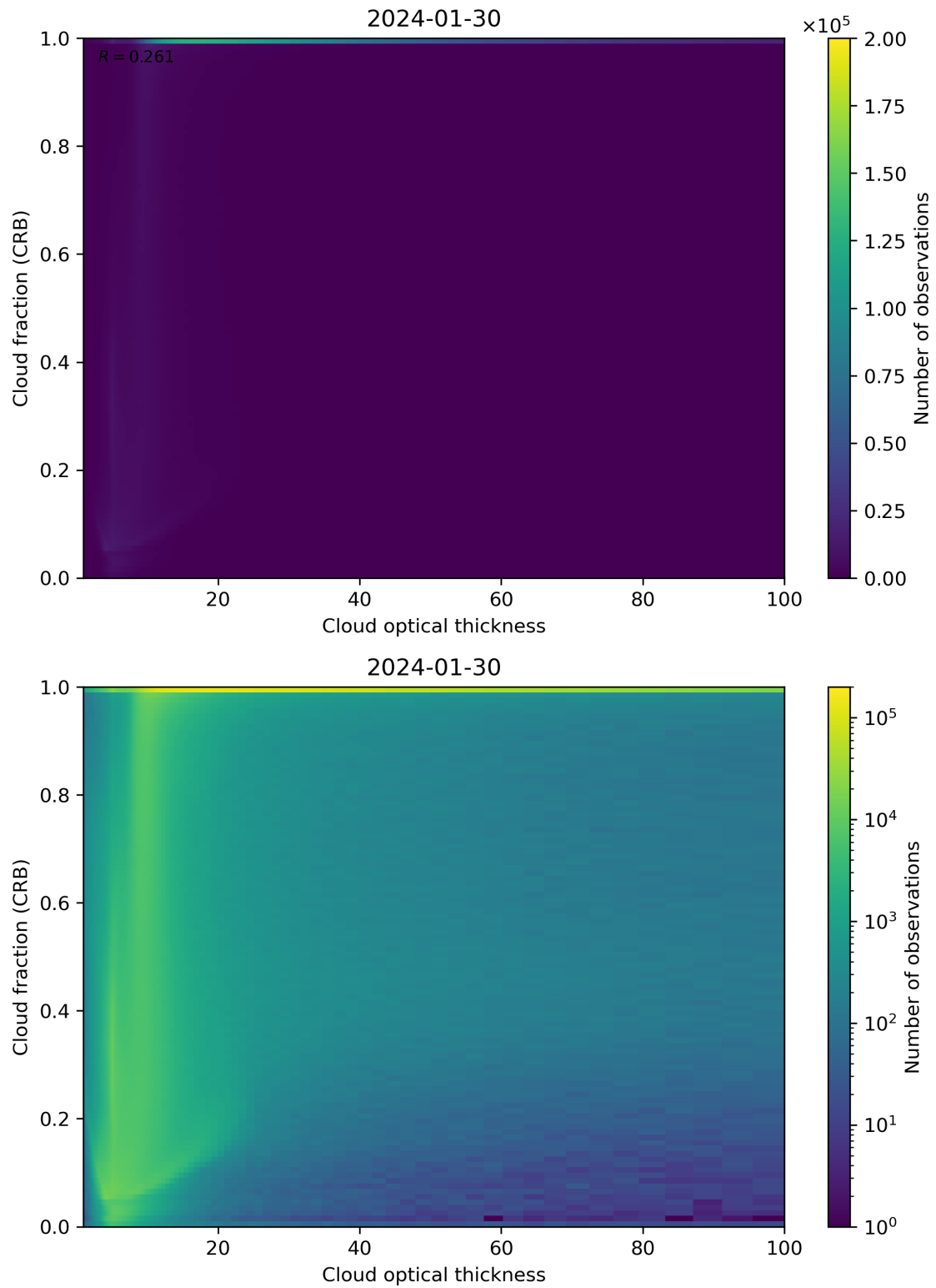
Figure 84: Scatter density plot of “Cloud optical thickness” against “Cloud fraction (CRB)” for 2024-01-29 to 2024-01-31.
