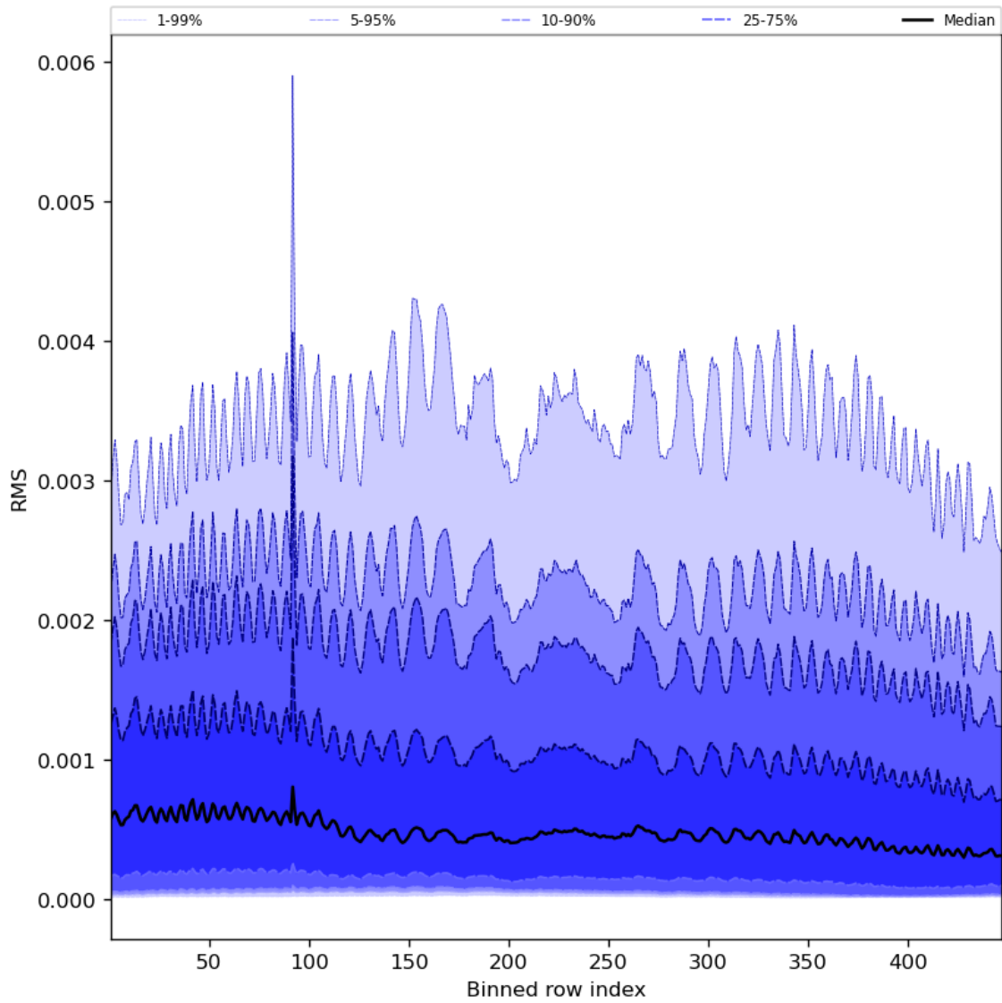
Figure 63: Along track statistics of “RMS” for 2024-01-29 to 2024-01-31
