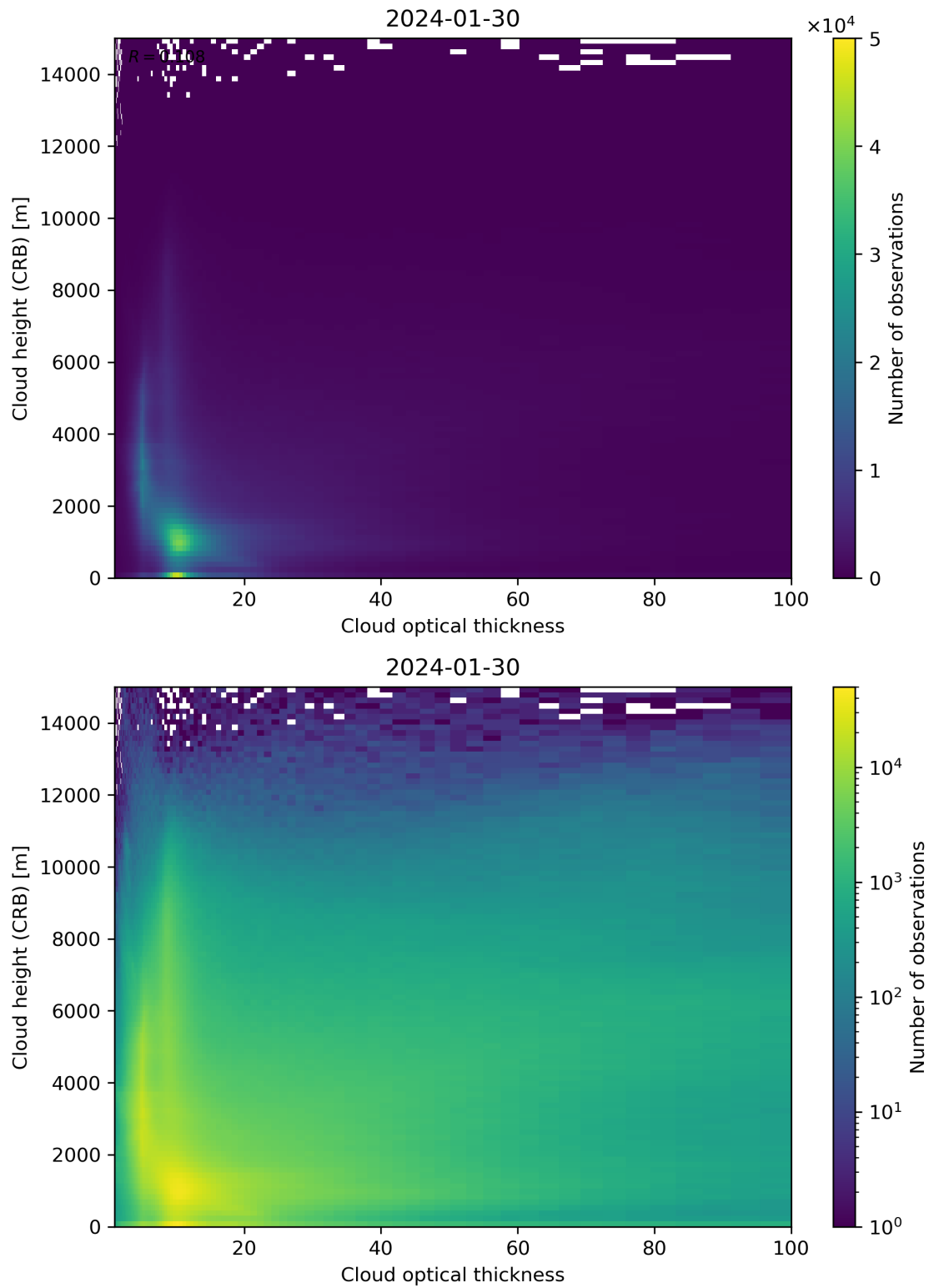
Figure 85: Scatter density plot of “Cloud optical thickness” against “Cloud height (CRB)” for 2024-01-29 to 2024-01-31.
