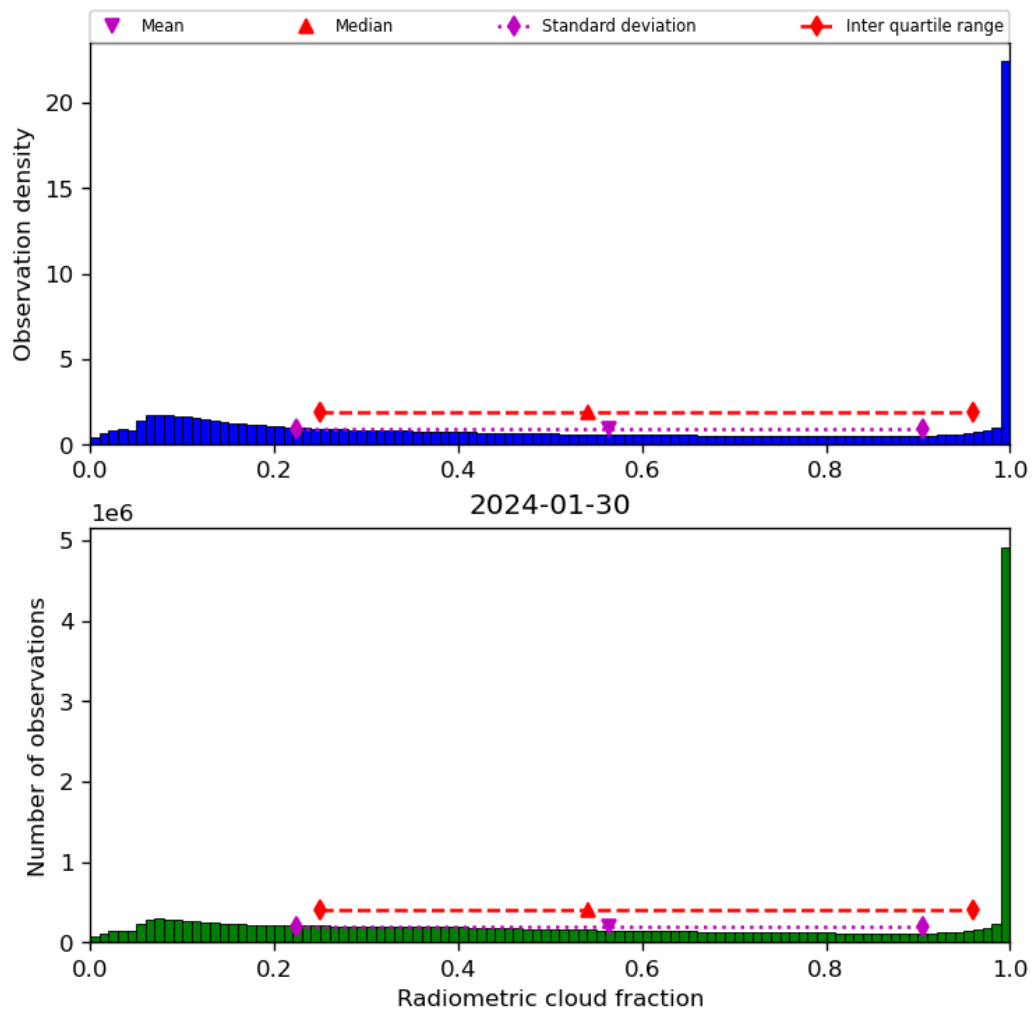
Figure 39: Histogram of “Radiometric cloud fraction” for 2024-01-29 to 2024-01-31
