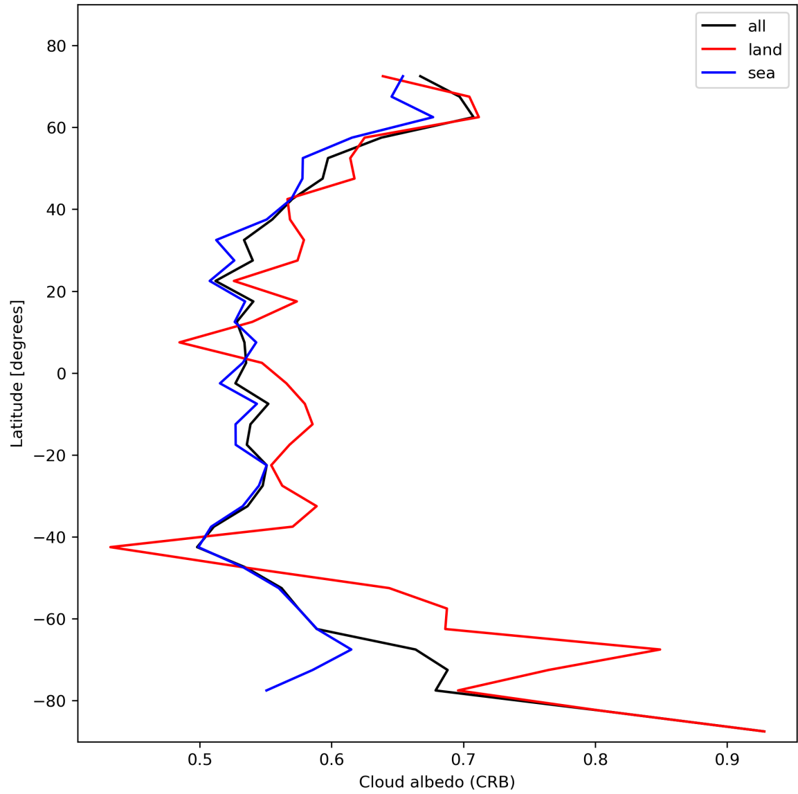
Figure 28: Zonal average of “Cloud albedo (CRB)” for 2024-01-29 to 2024-01-31.
