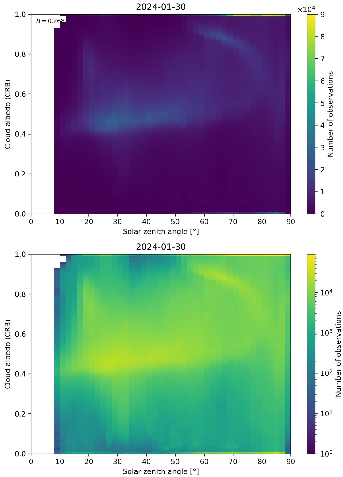
Figure 98: Scatter density plot of “Solar zenith angle” against “Cloud albedo (CRB)” for 2024-01-29 to 2024-01-31.
