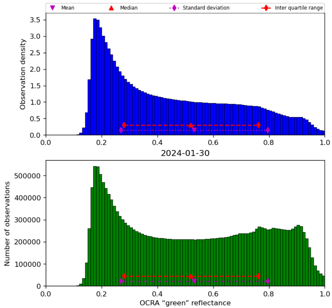
Figure 52: Histogram of “OCRA “green” reflectance” for 2024-01-29 to 2024-01-31
