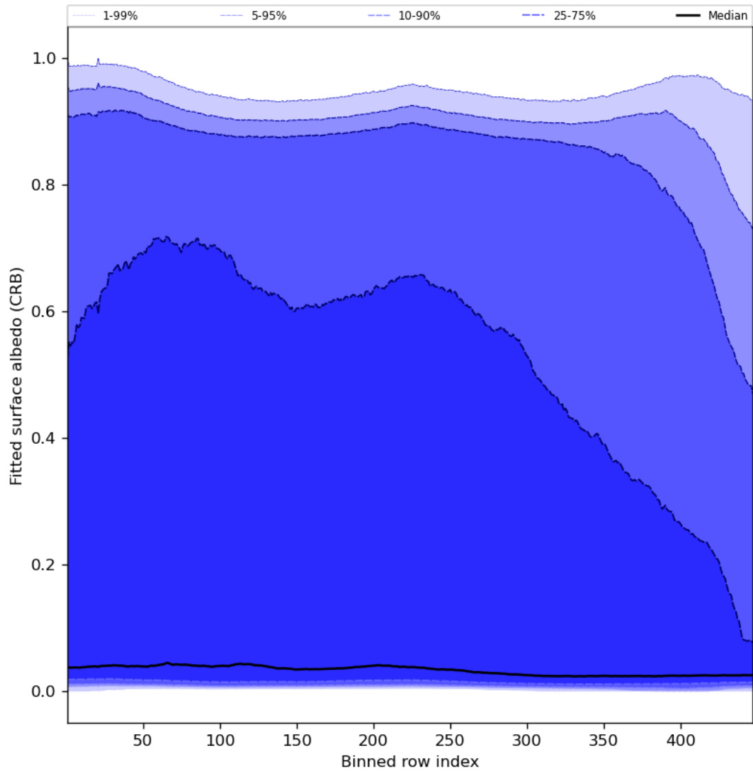
Figure 62: Along track statistics of “Fitted surface albedo (CRB)” for 2024-01-29 to 2024-01-31
