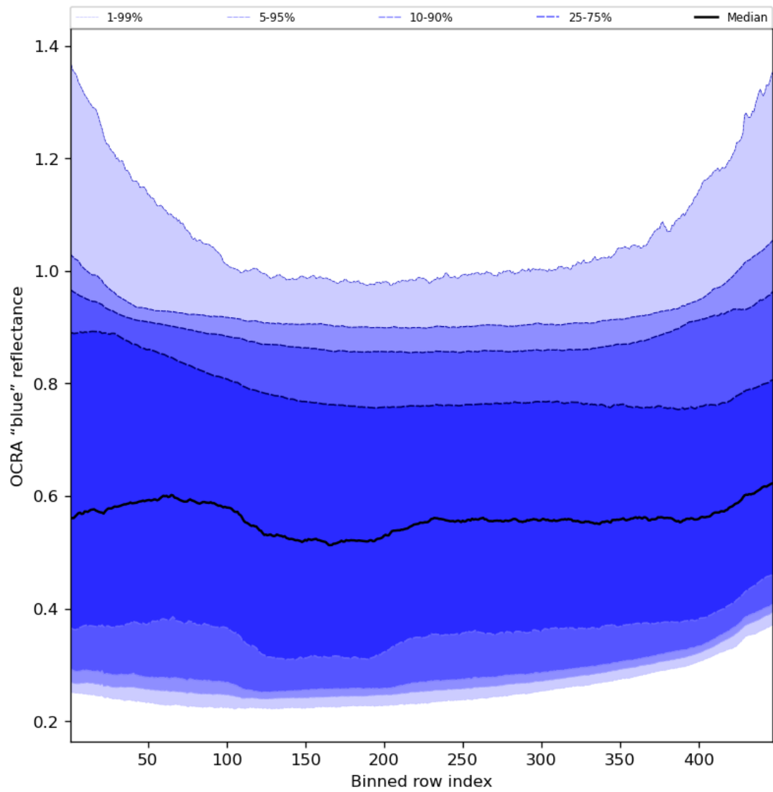
Figure 67: Along track statistics of “OCRA “blue” reflectance” for 2024-01-29 to 2024-01-31
