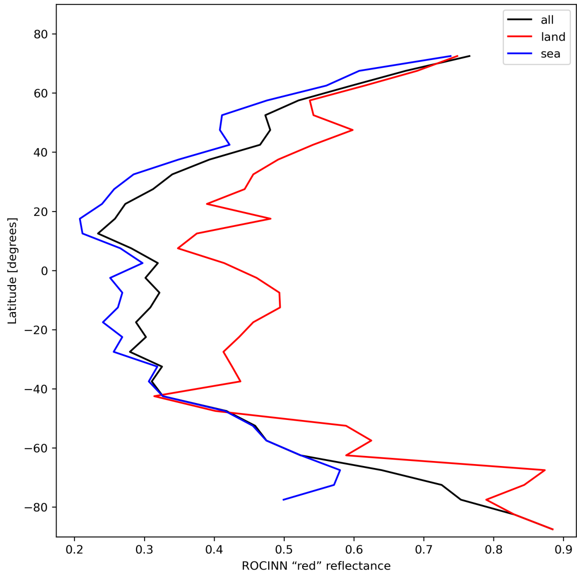
Figure 37: Zonal average of “ROCINN “red” reflectance” for 2024-01-29 to 2024-01-31.
