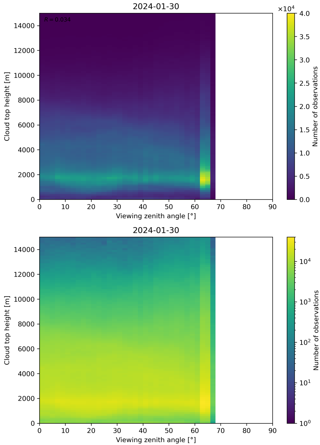
Figure 112: Scatter density plot of “Viewing zenith angle” against “Cloud top height” for 2024-01-29 to 2024-01-31.
