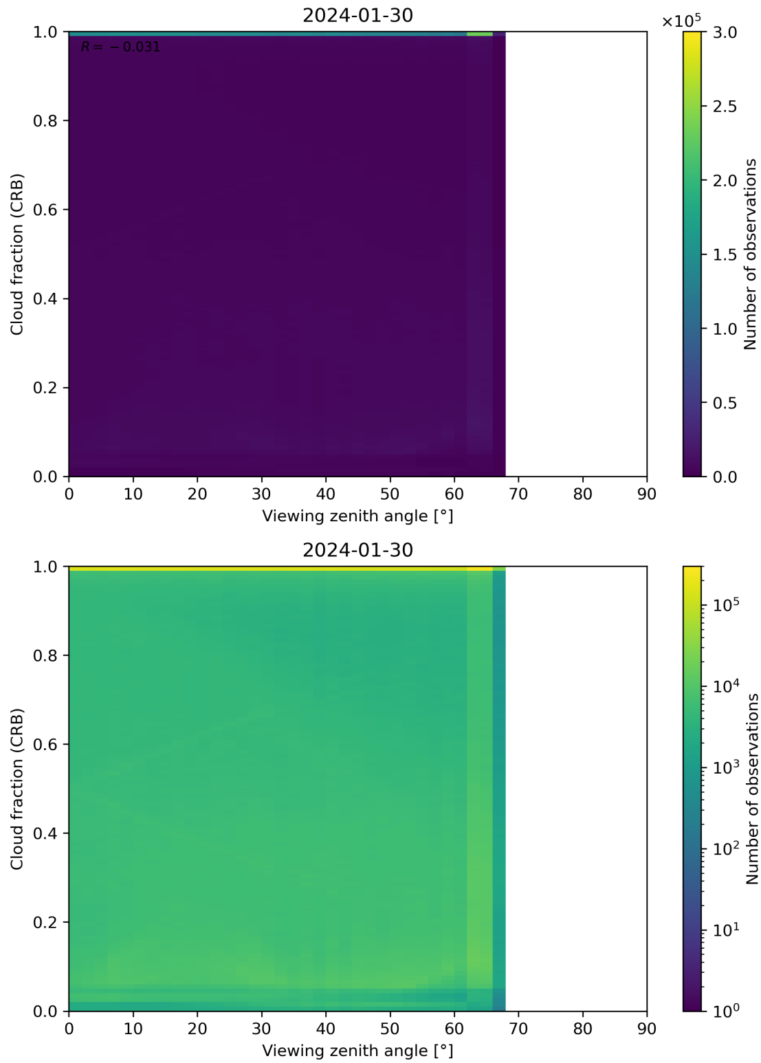
Figure 109: Scatter density plot of “Viewing zenith angle” against “Cloud fraction (CRB)” for 2024-01-29 to 2024-01-31.
