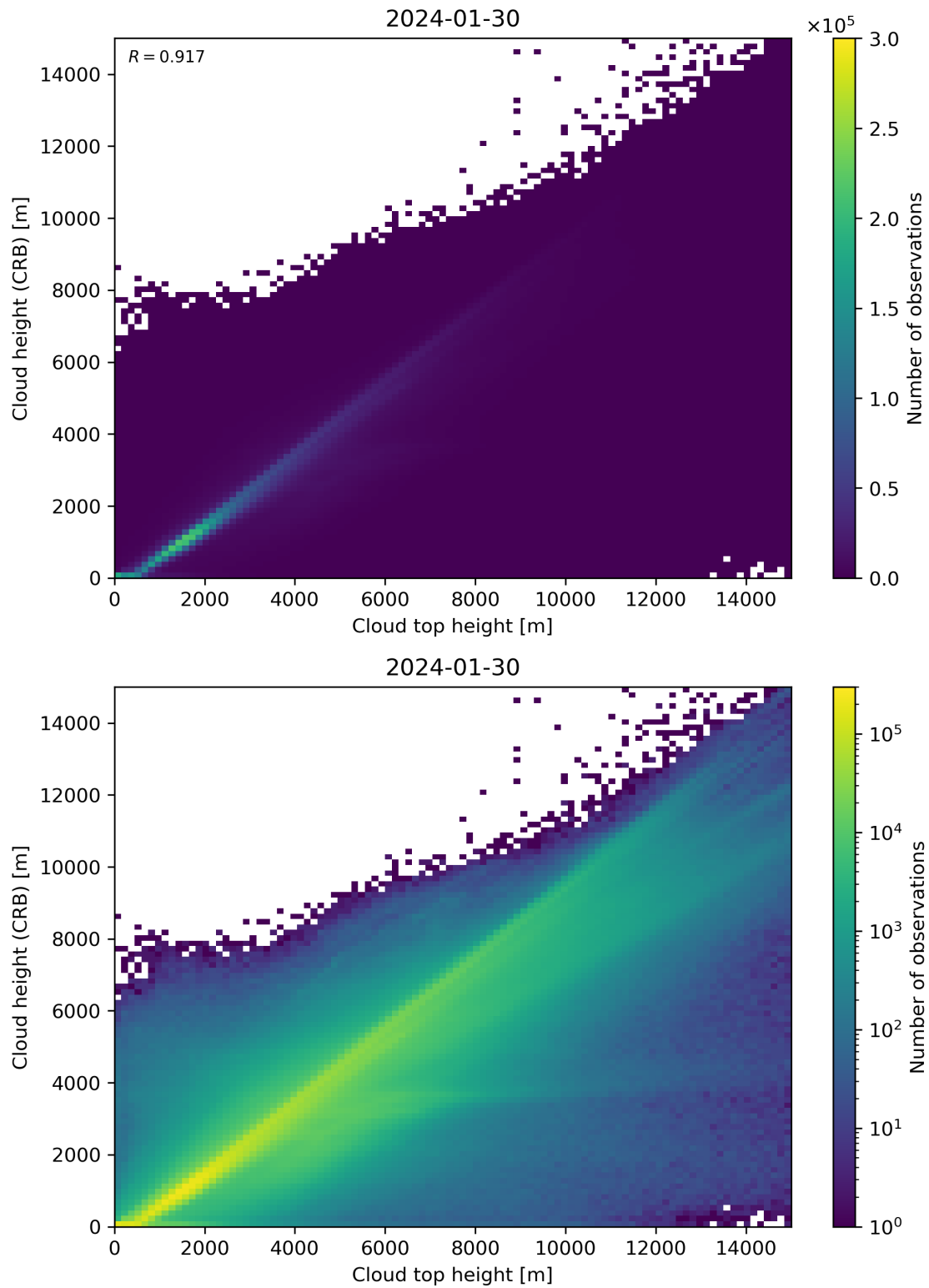
Figure 89: Scatter density plot of “Cloud top height” against “Cloud height (CRB)” for 2024-01-29 to 2024-01-31.
