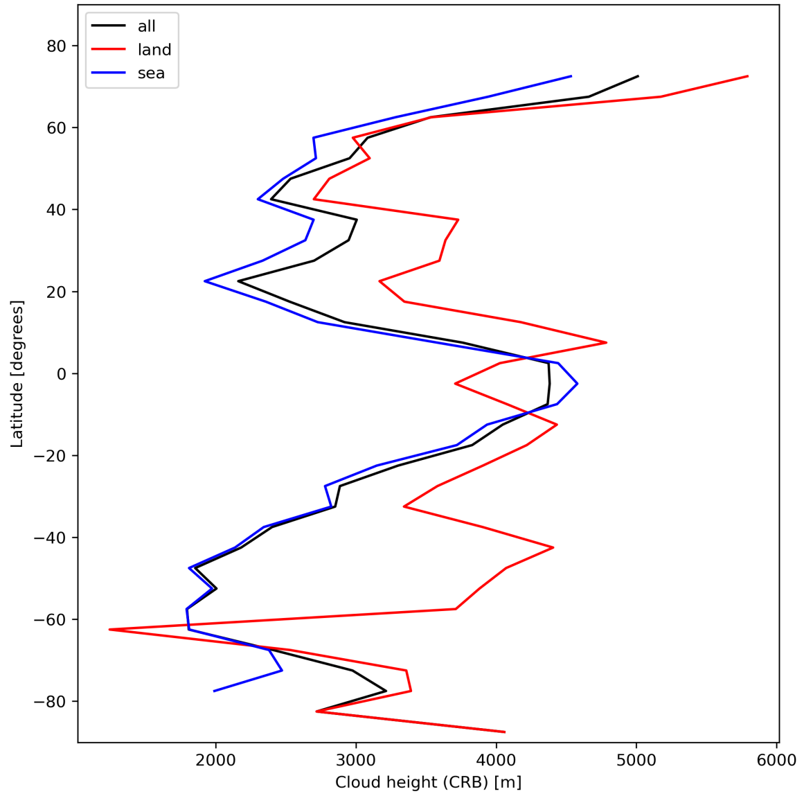
Figure 27: Zonal average of “Cloud height (CRB)” for 2024-01-29 to 2024-01-31.
