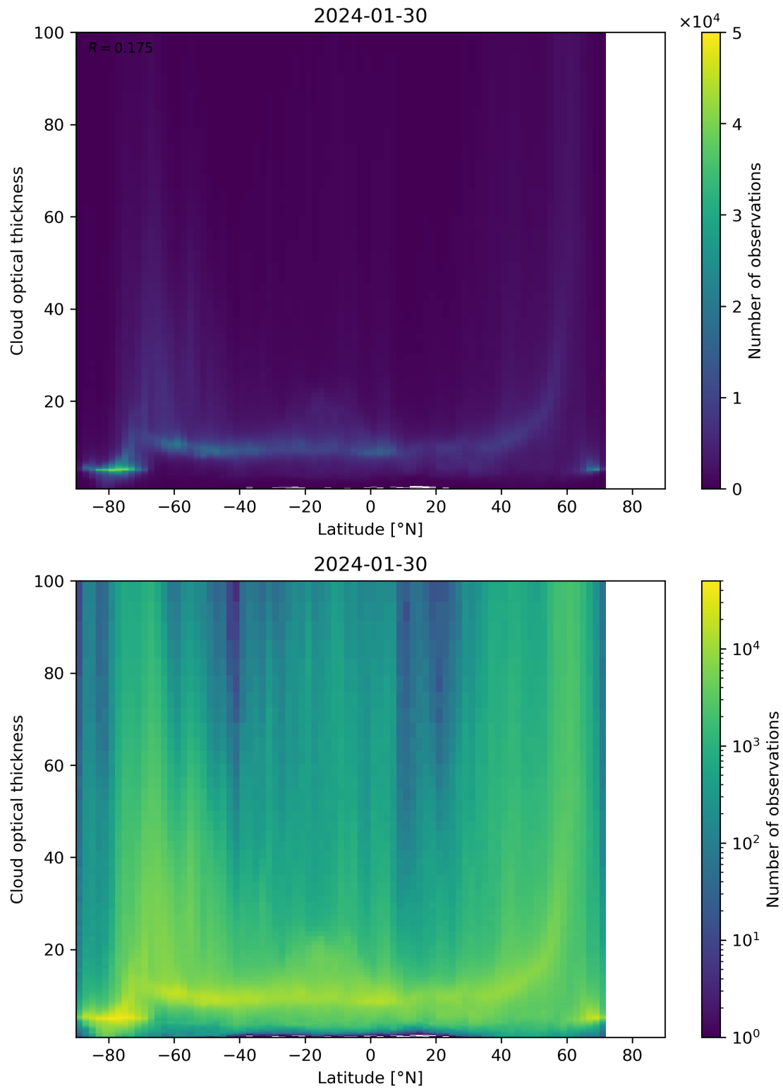
Figure 96: Scatter density plot of “Latitude” against “Cloud optical thickness” for 2024-01-29 to 2024-01-31.
