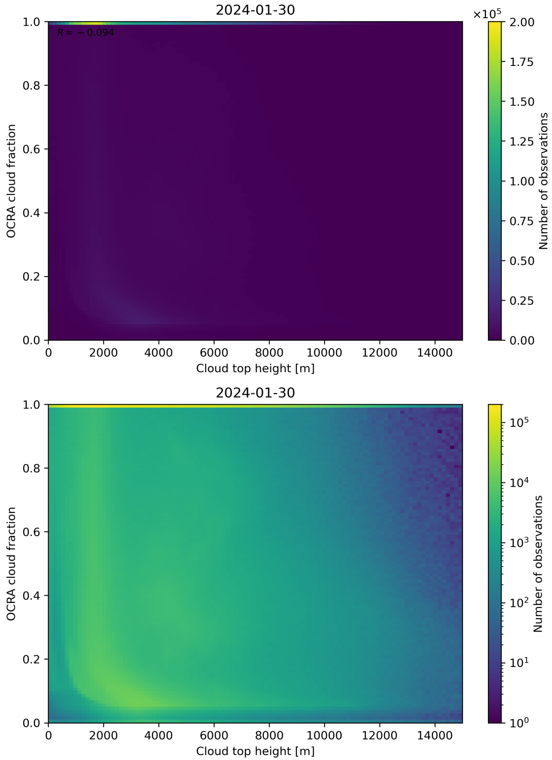
Figure 87: Scatter density plot of “Cloud top height” against “OCRA cloud fraction” for 2024-01-29 to 2024-01-31.
