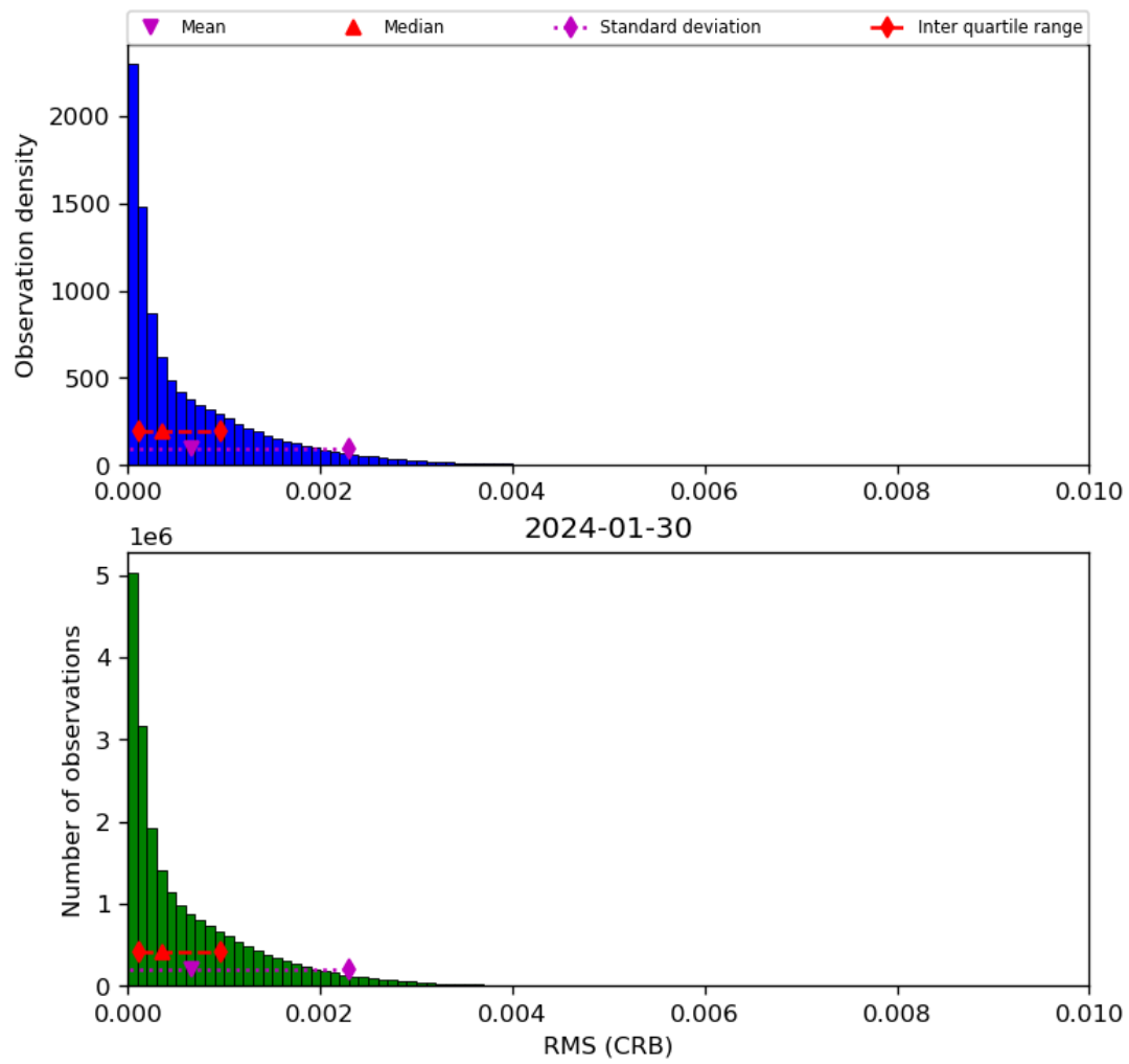
Figure 48: Histogram of “RMS (CRB)” for 2024-01-29 to 2024-01-31
