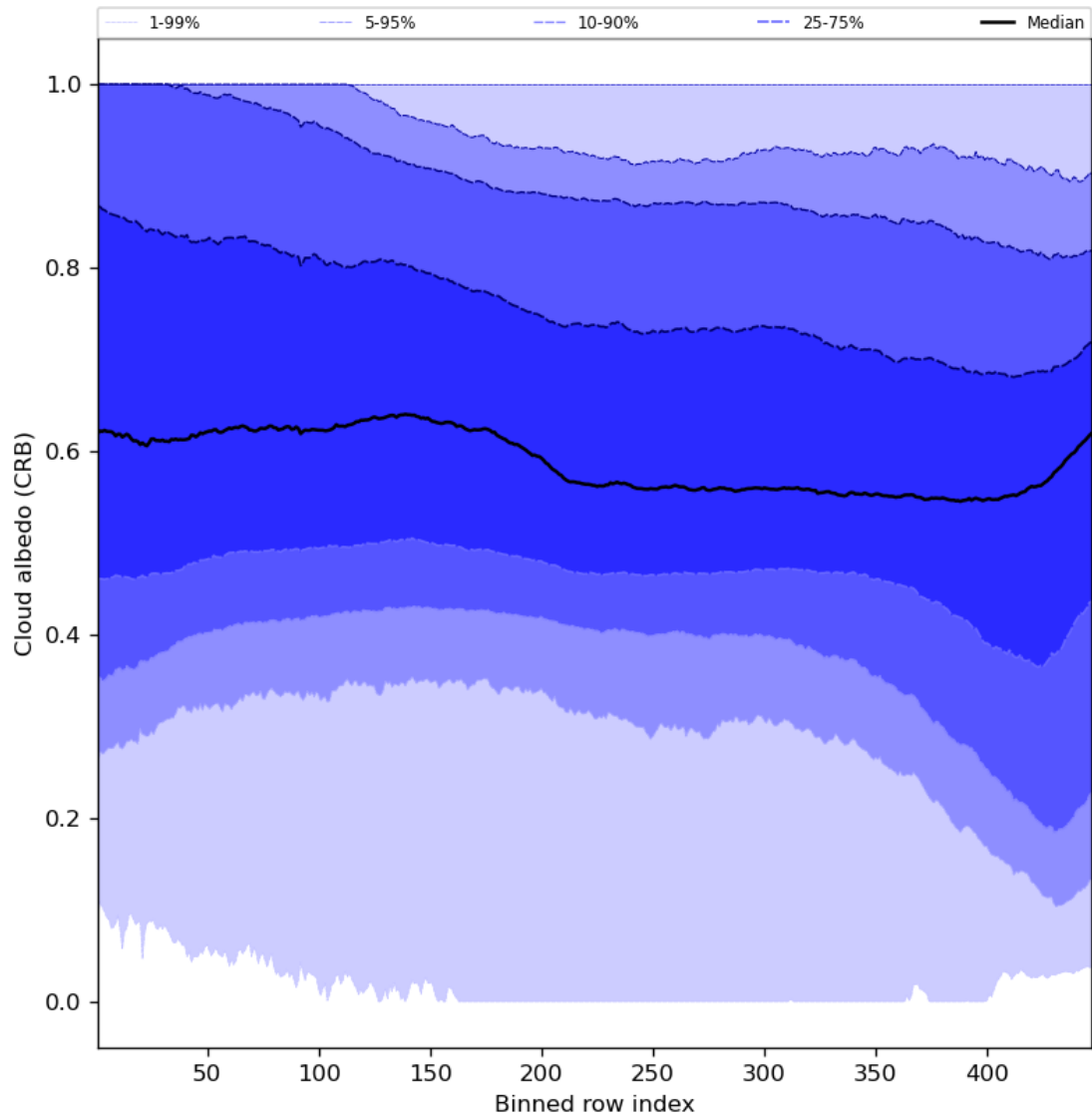
Figure 60: Along track statistics of “Cloud albedo (CRB)” for 2024-01-29 to 2024-01-31
