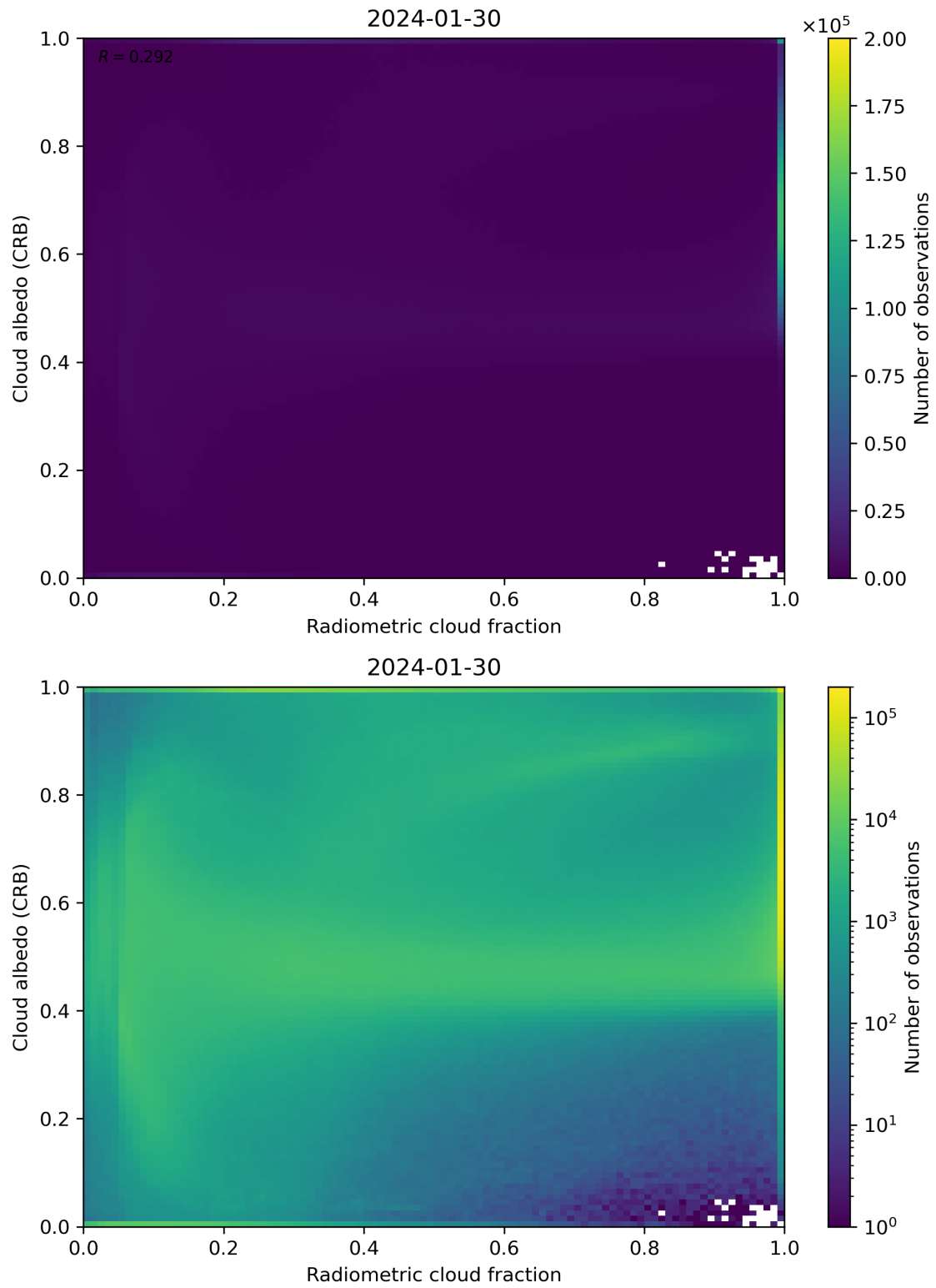
Figure 71: Scatter density plot of “Radiometric cloud fraction” against “Cloud albedo (CRB)” for 2024-01-29 to 2024-01-31.
