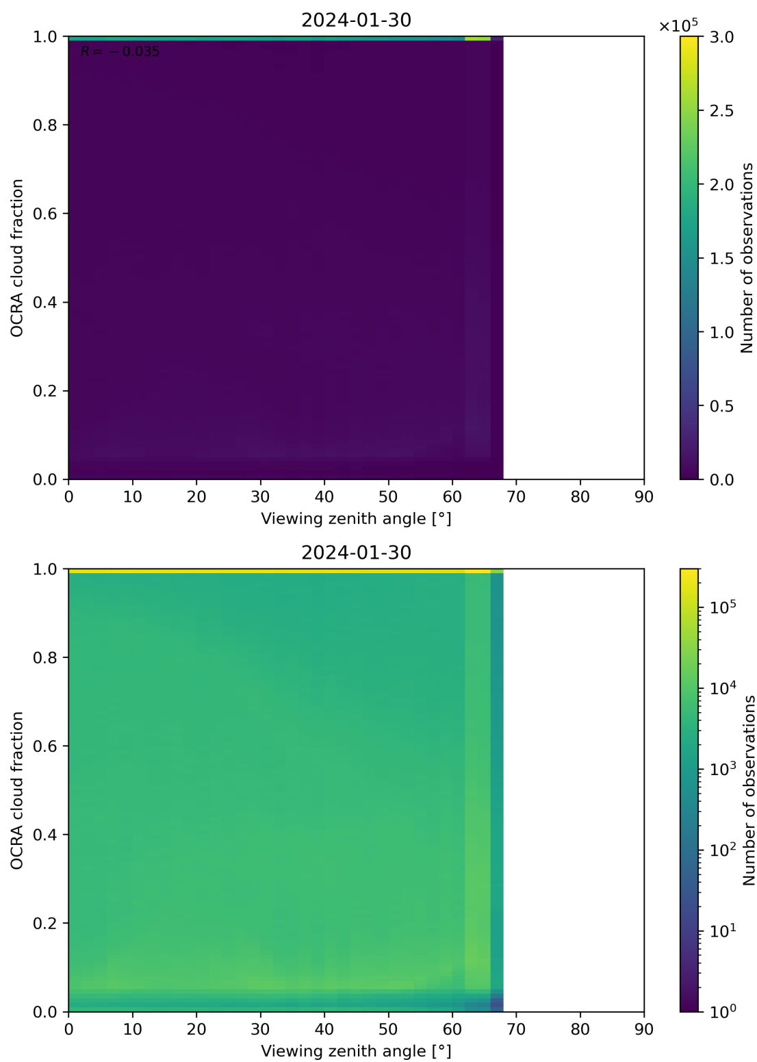
Figure 108: Scatter density plot of “Viewing zenith angle” against “OCRA cloud fraction” for 2024-01-29 to 2024-01-31.
