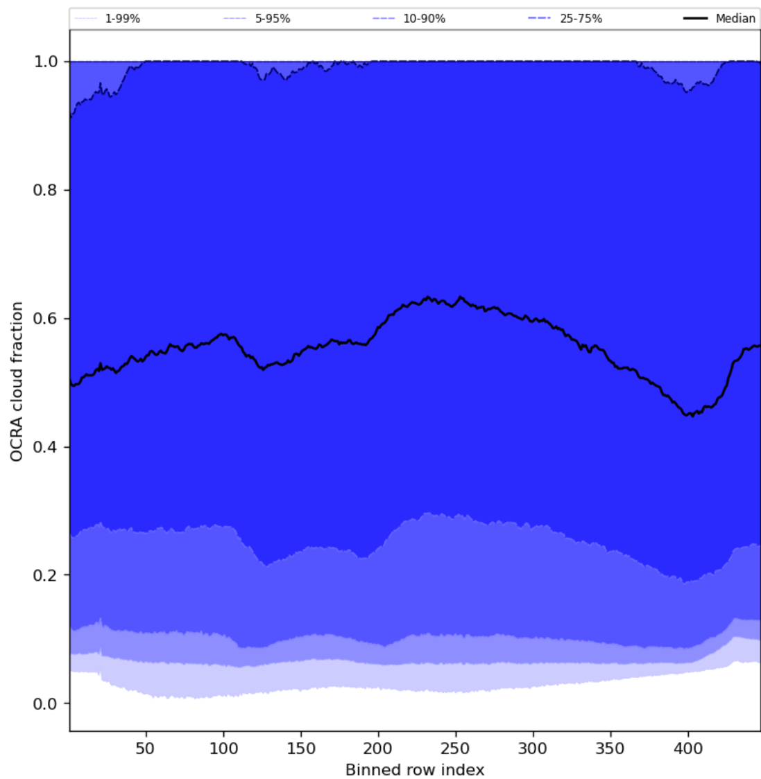
Figure 66: Along track statistics of “OCRA cloud fraction” for 2024-01-29 to 2024-01-31
