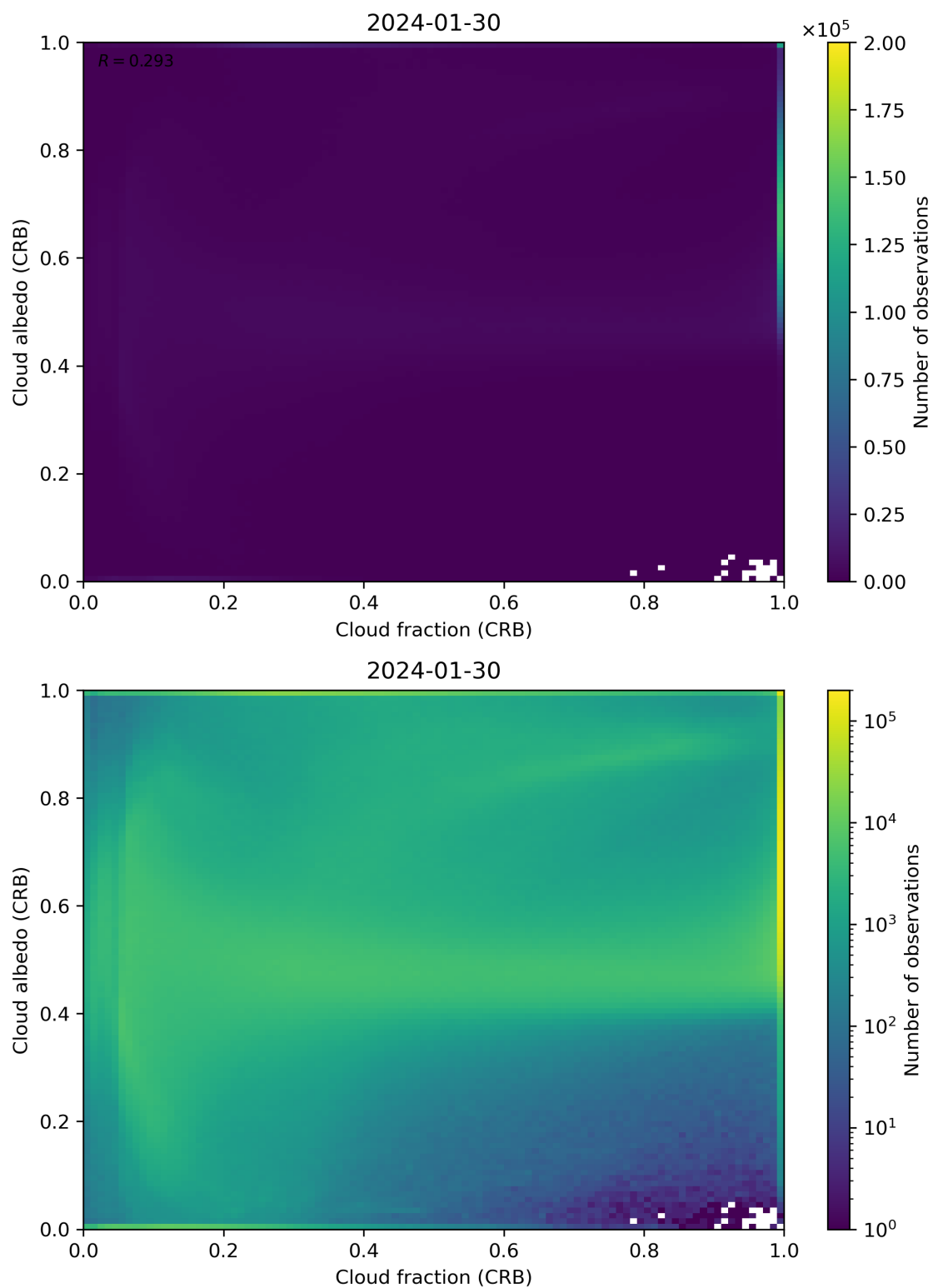
Figure 77: Scatter density plot of “Cloud fraction (CRB)” against “Cloud albedo (CRB)” for 2024-01-29 to 2024-01-31.
