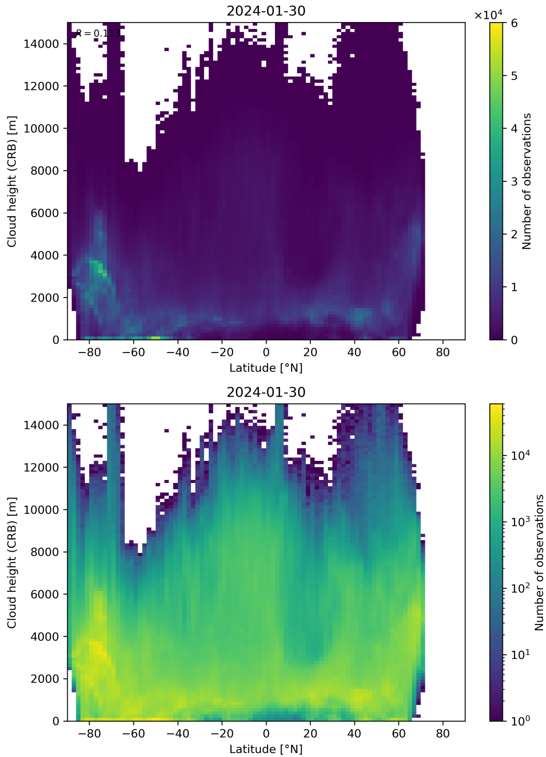
Figure 95: Scatter density plot of “Latitude” against “Cloud height (CRB)” for 2024-01-29 to 2024-01-31.
