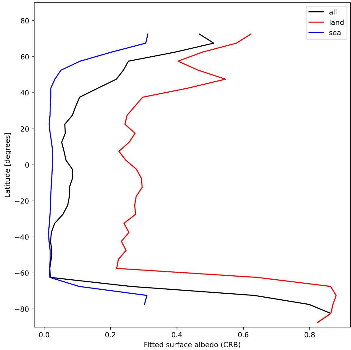
Figure 30: Zonal average of “Fitted surface albedo (CRB)” for 2024-01-29 to 2024-01-31.
