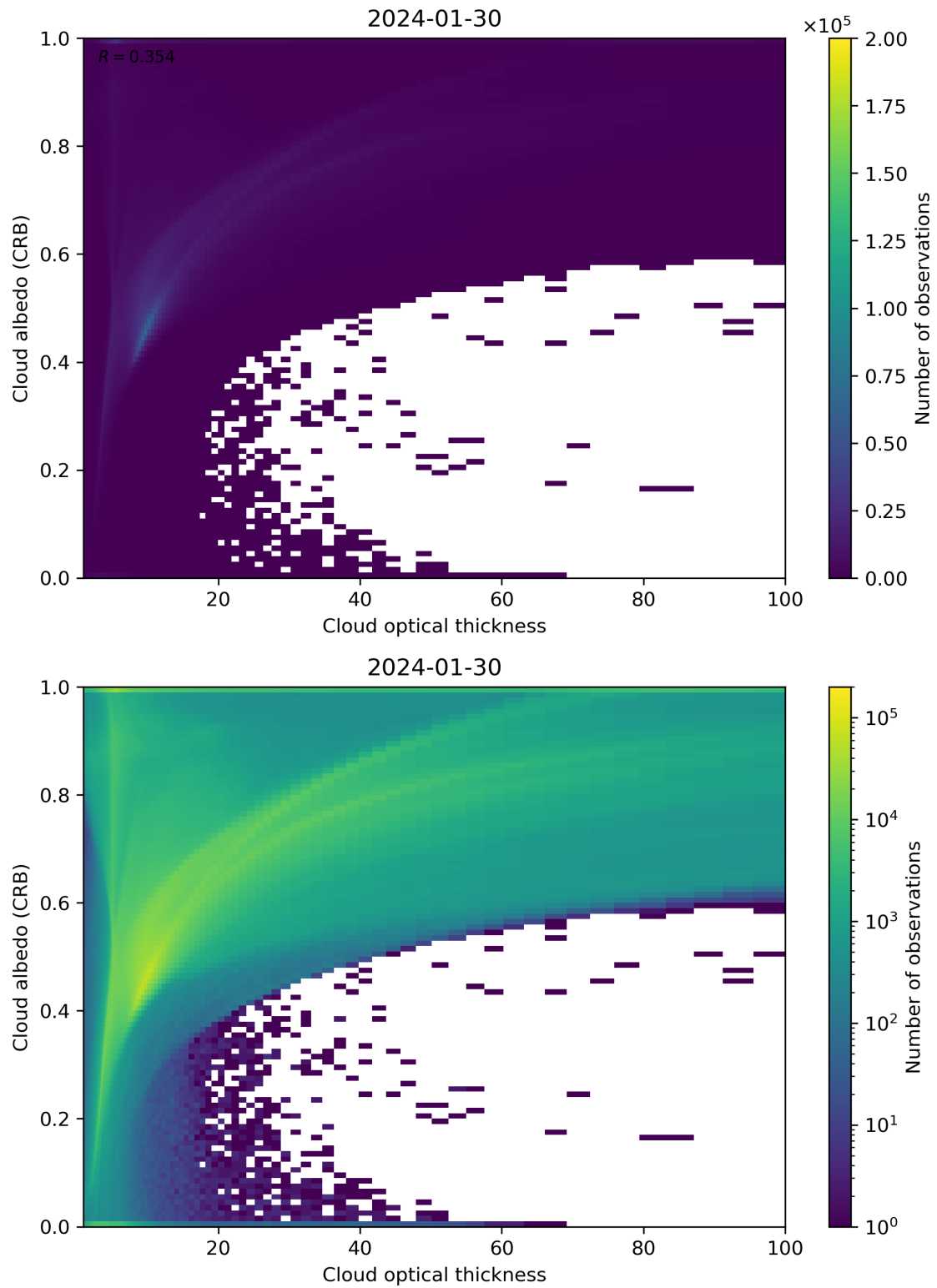
Figure 82: Scatter density plot of “Cloud optical thickness” against “Cloud albedo (CRB)” for 2024-01-29 to 2024-01-31.
