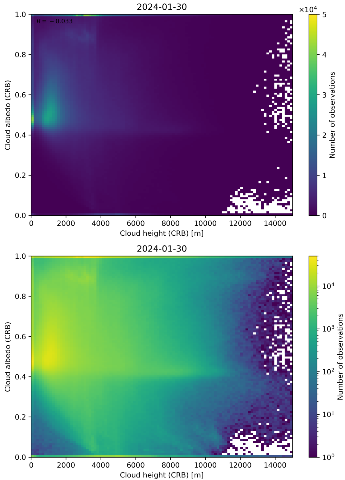
Figure 80: Scatter density plot of “Cloud height (CRB)” against “Cloud albedo (CRB)” for 2024-01-29 to 2024-01-31.
