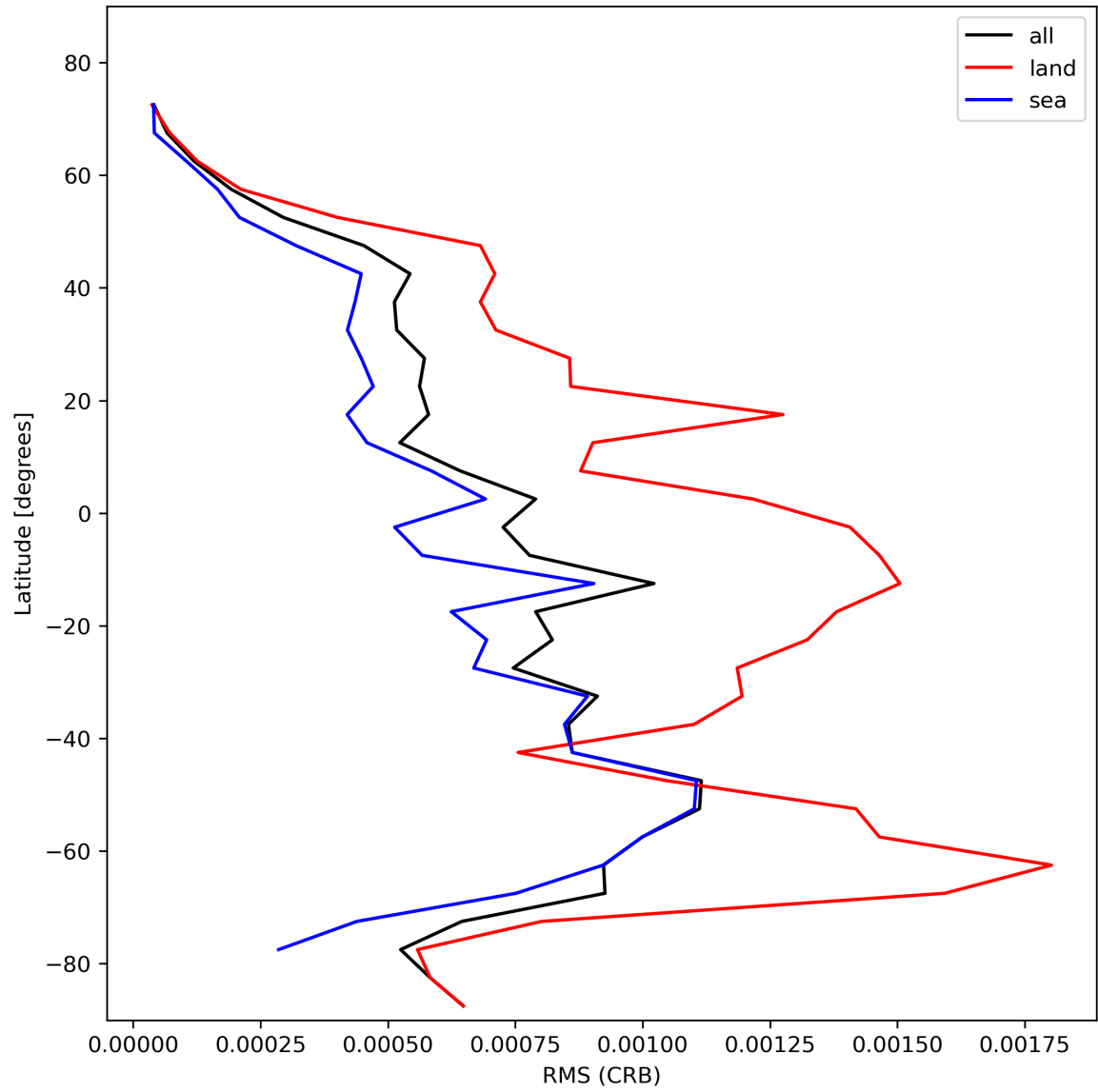
Figure 32: Zonal average of “RMS (CRB)” for 2024-01-29 to 2024-01-31.
