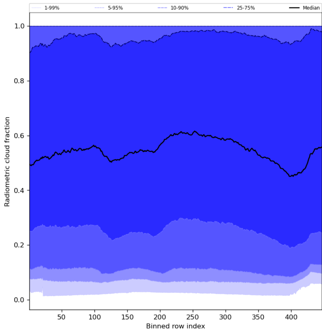
Figure 55: Along track statistics of “Radiometric cloud fraction” for 2024-01-29 to 2024-01-31
