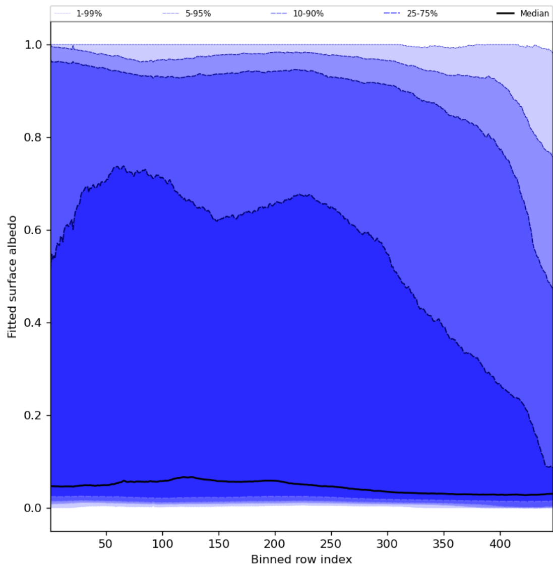
Figure 61: Along track statistics of “Fitted surface albedo” for 2024-01-29 to 2024-01-31
