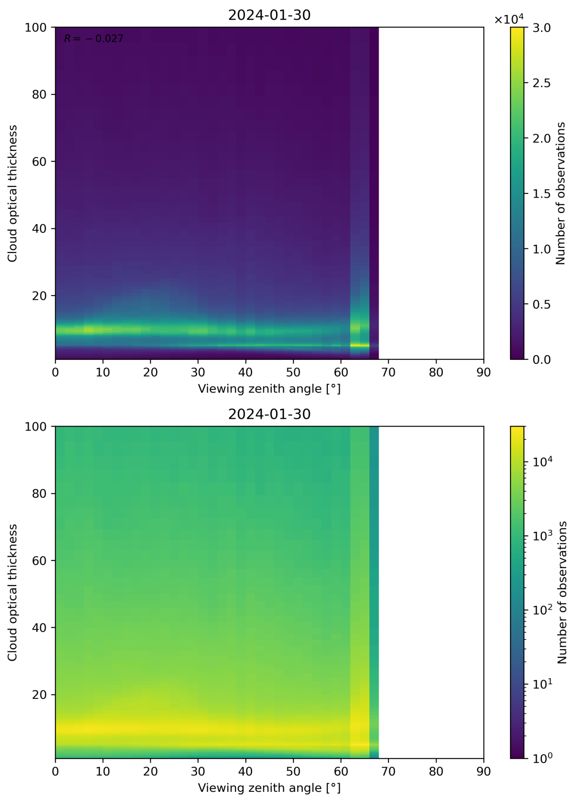
Figure 111: Scatter density plot of “Viewing zenith angle” against “Cloud optical thickness” for 2024-01-29 to 2024-01-31.
