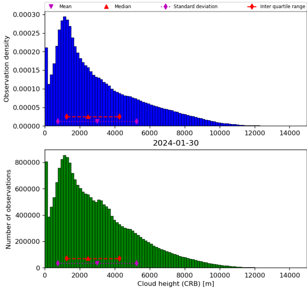
Figure 43: Histogram of “Cloud height (CRB)” for 2024-01-29 to 2024-01-31
