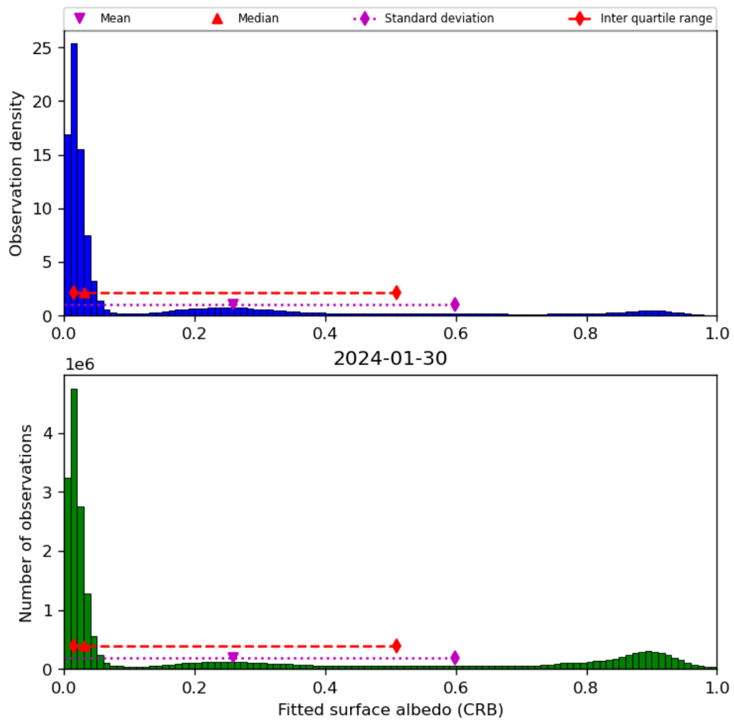
Figure 46: Histogram of “Fitted surface albedo (CRB)” for 2024-01-29 to 2024-01-31
