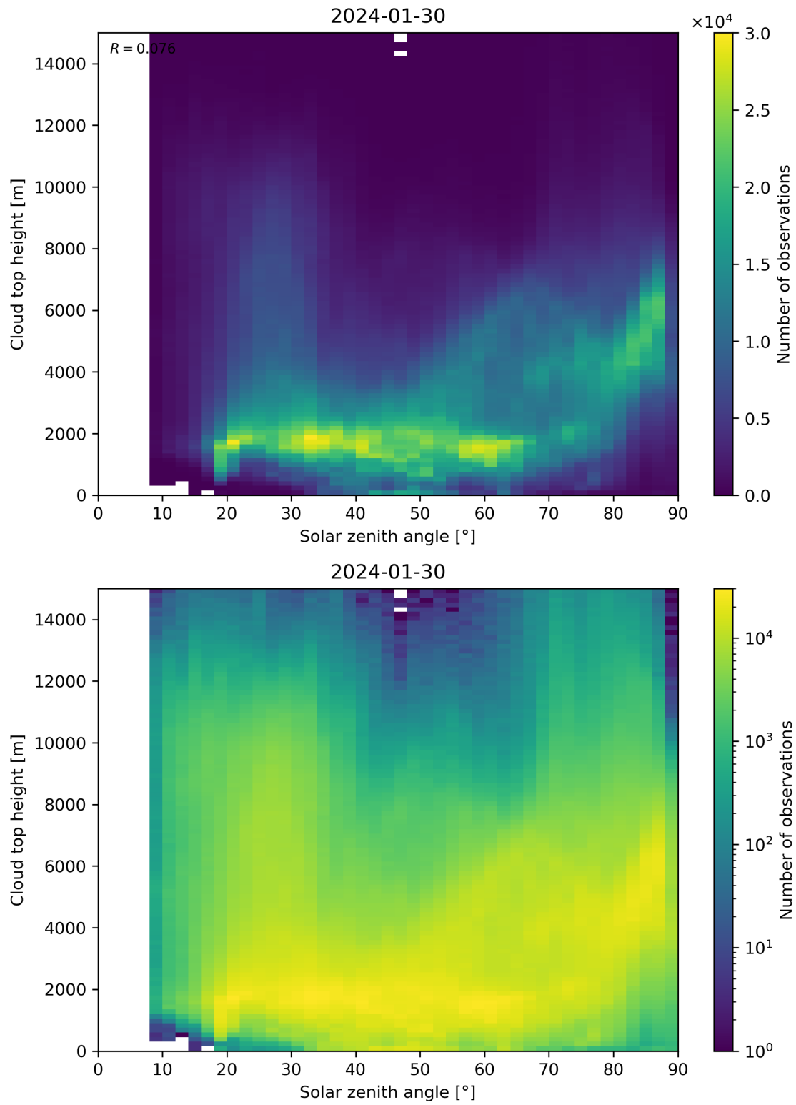
Figure 104: Scatter density plot of “Solar zenith angle” against “Cloud top height” for 2024-01-29 to 2024-01-31.
