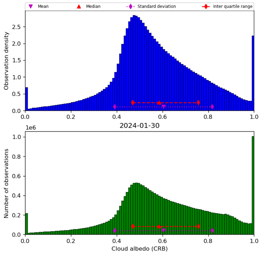
Figure 44: Histogram of “Cloud albedo (CRB)” for 2024-01-29 to 2024-01-31
