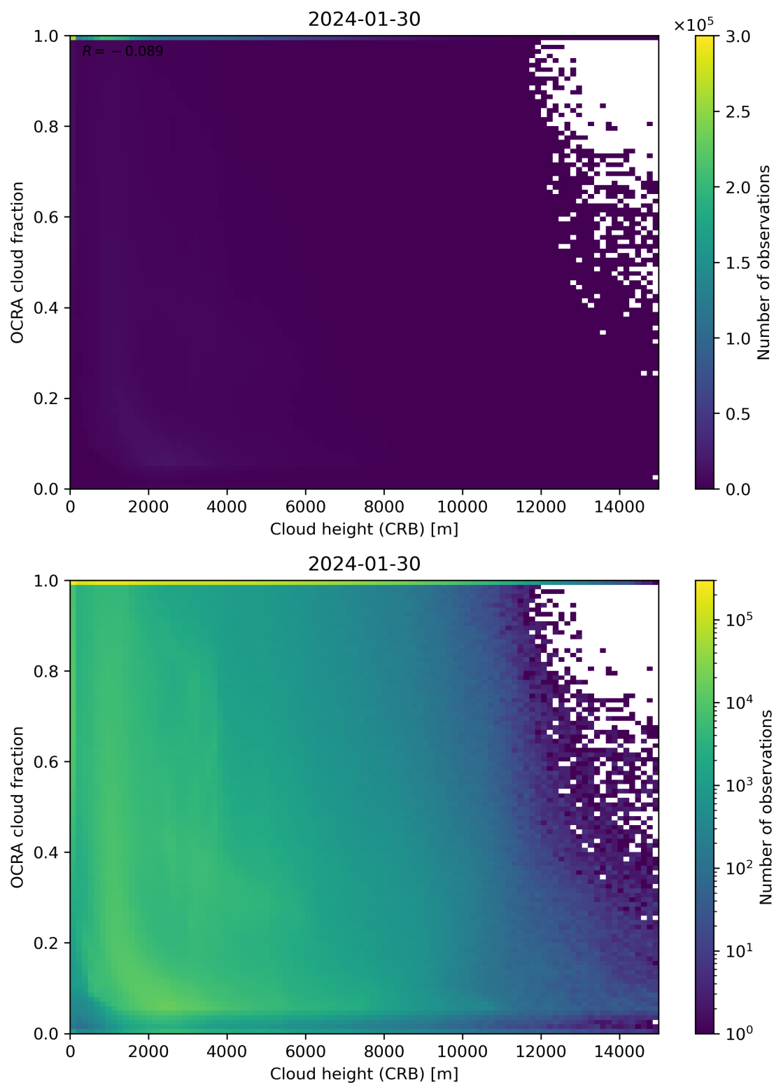
Figure 81: Scatter density plot of “Cloud height (CRB)” against “OCRA cloud fraction” for 2024-01-29 to 2024-01-31.
