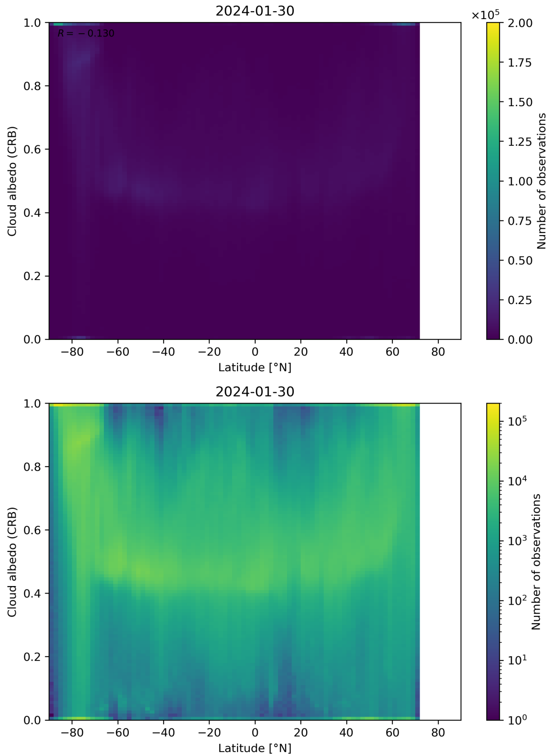
Figure 91: Scatter density plot of “Latitude” against “Cloud albedo (CRB)” for 2024-01-29 to 2024-01-31.
