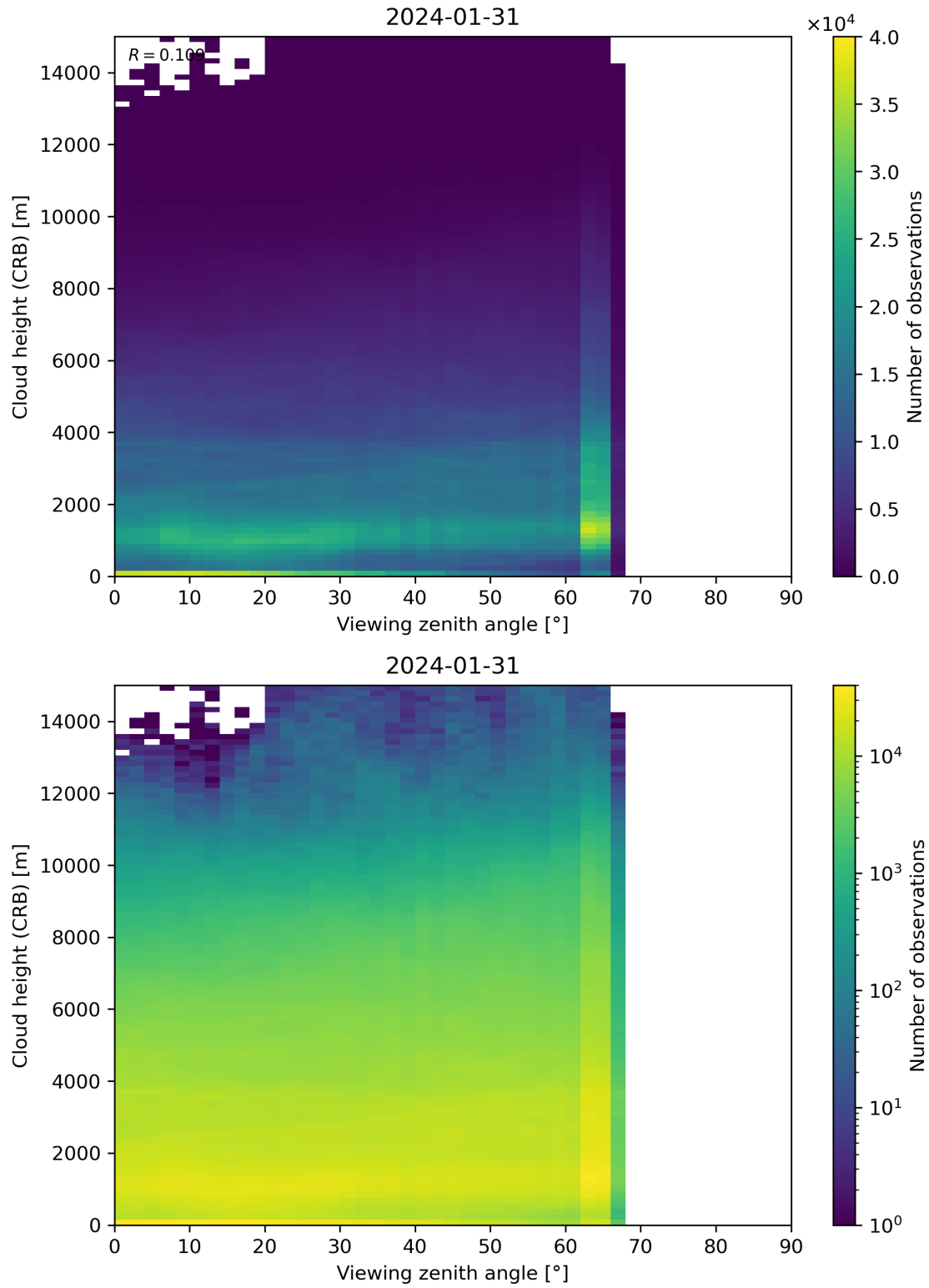
Figure 110: Scatter density plot of “Viewing zenith angle” against “Cloud height (CRB)” for 2024-01-31 to 2024-02-01.
