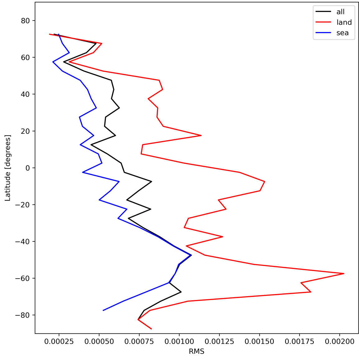
Figure 31: Zonal average of “RMS” for 2024-01-31 to 2024-02-01.
