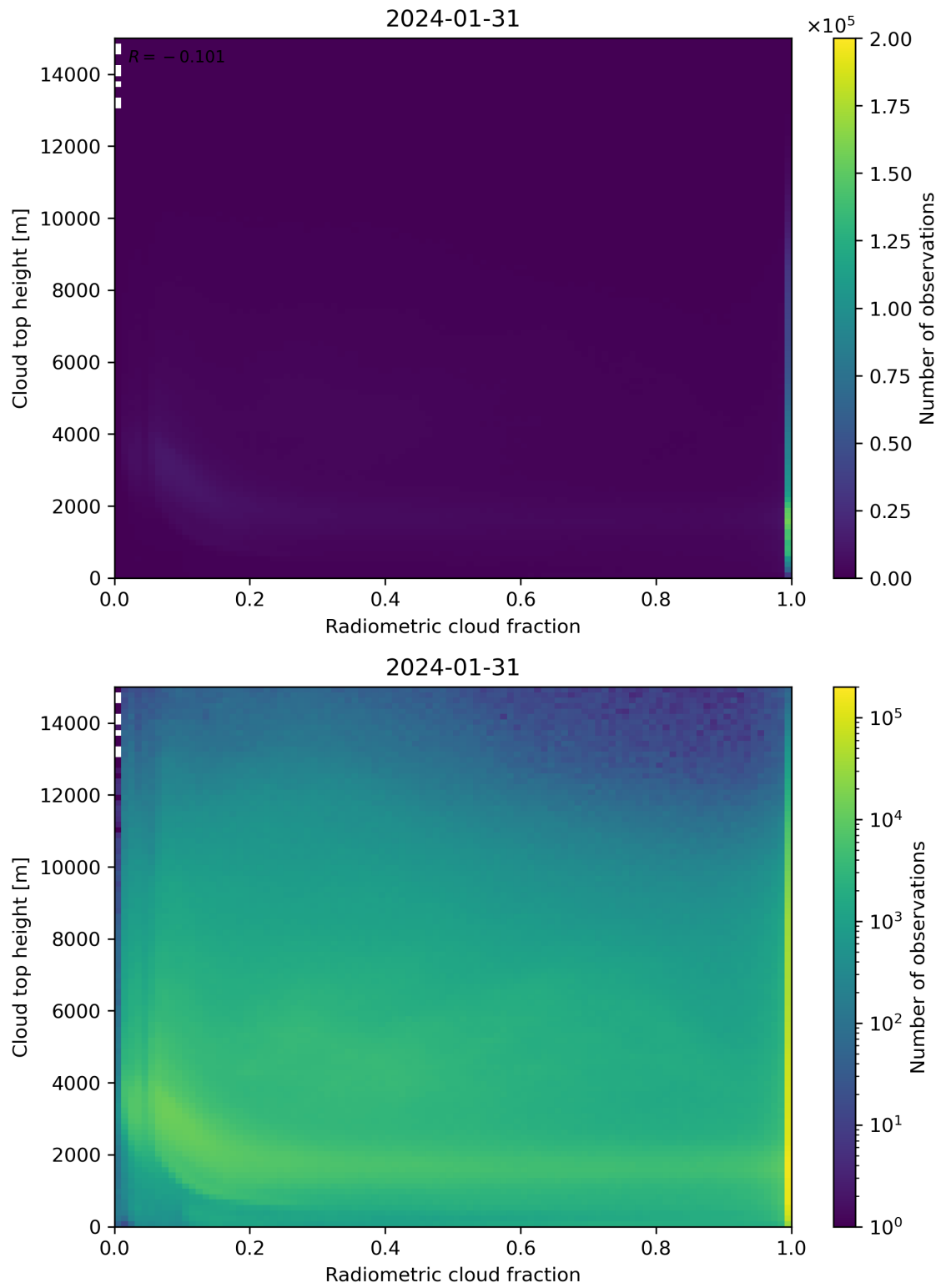
Figure 76: Scatter density plot of “Radiometric cloud fraction” against “Cloud top height” for 2024-01-31 to 2024-02-01.
