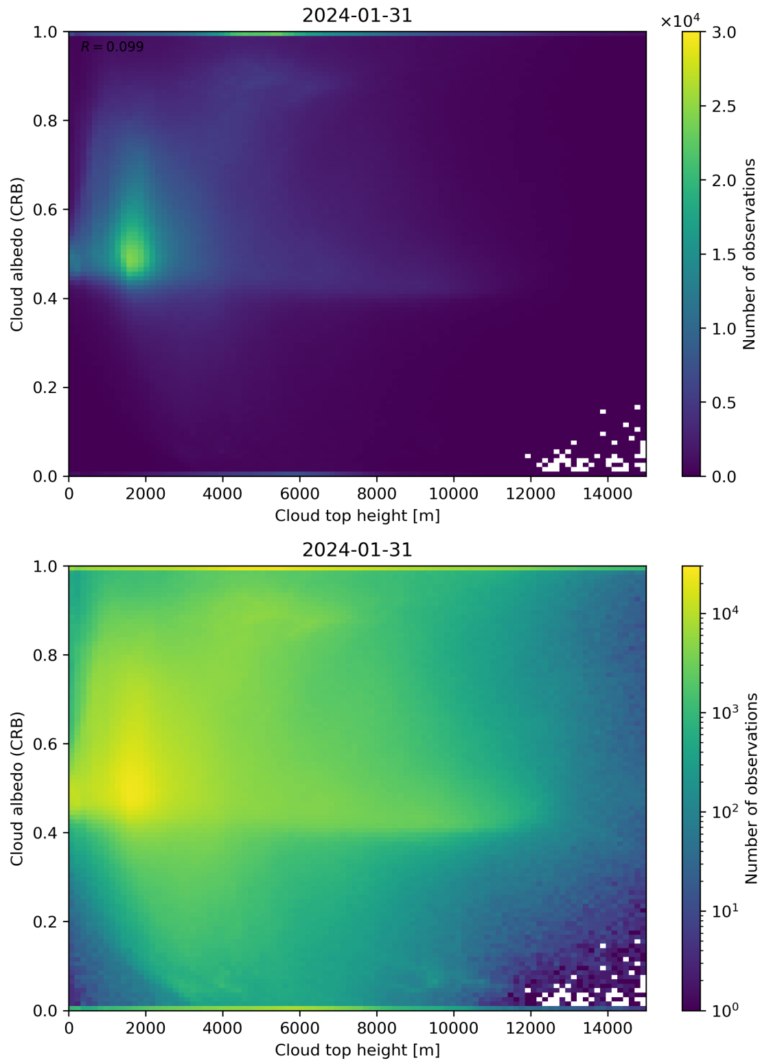
Figure 86: Scatter density plot of “Cloud top height” against “Cloud albedo (CRB)” for 2024-01-31 to 2024-02-01.
