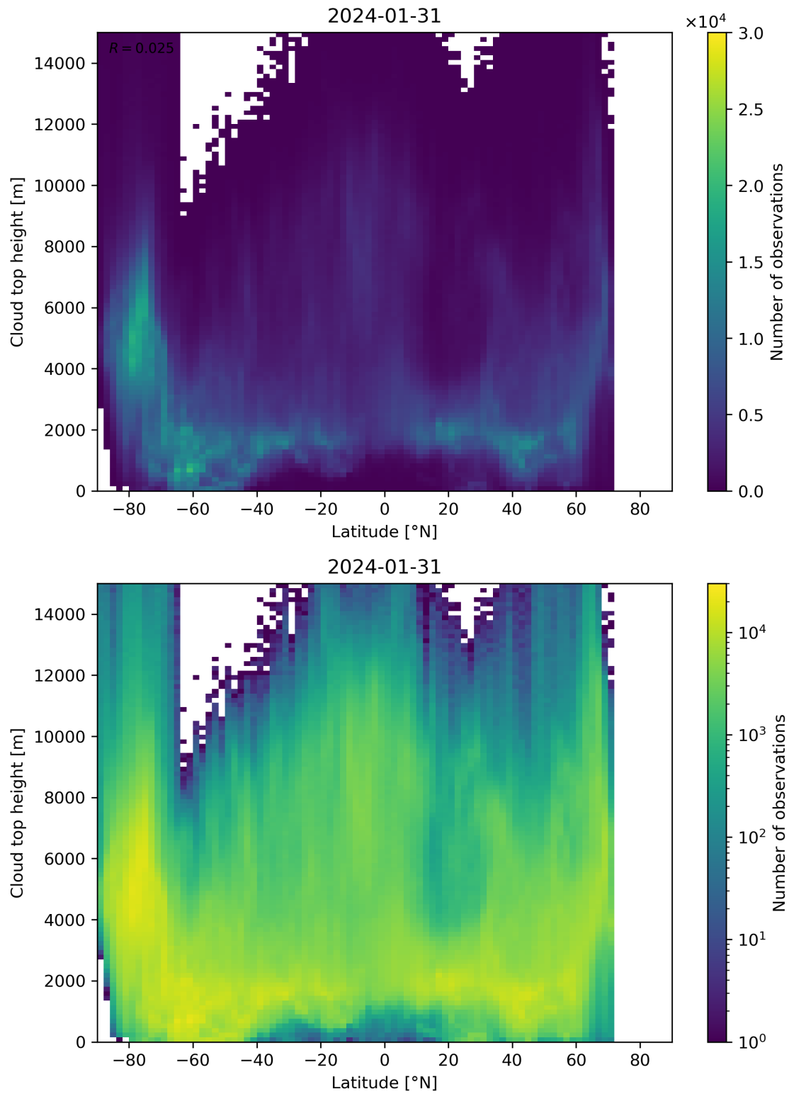
Figure 97: Scatter density plot of “Latitude” against “Cloud top height” for 2024-01-31 to 2024-02-01.
