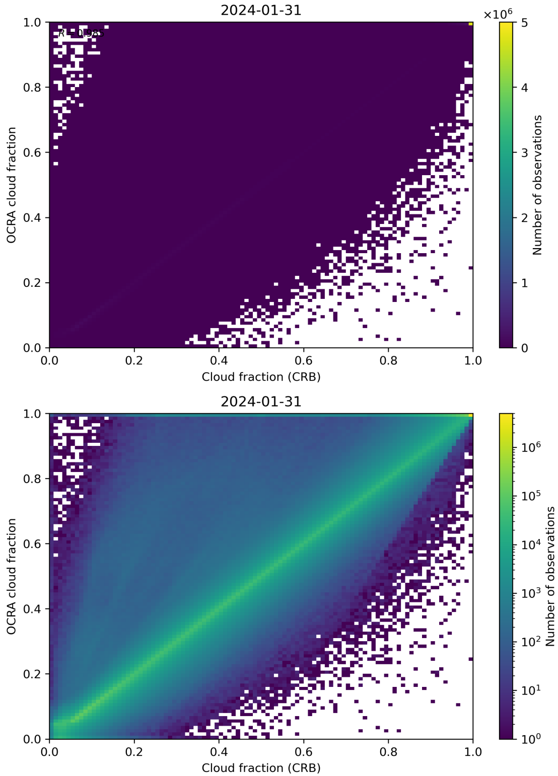
Figure 78: Scatter density plot of “Cloud fraction (CRB)” against “OCRA cloud fraction” for 2024-01-31 to 2024-02-01.
