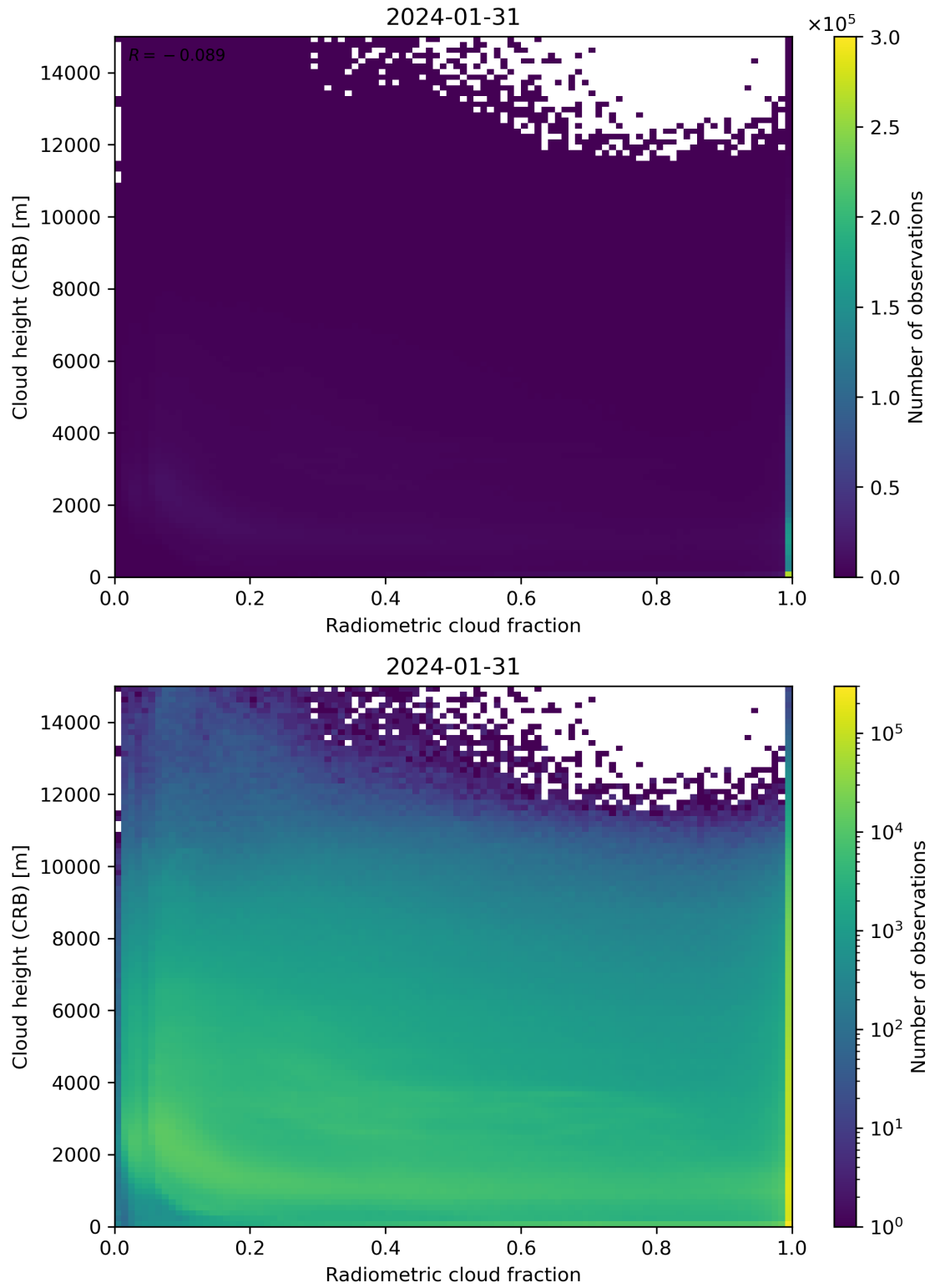
Figure 74: Scatter density plot of “Radiometric cloud fraction” against “Cloud height (CRB)” for 2024-01-31 to 2024-02-01.
