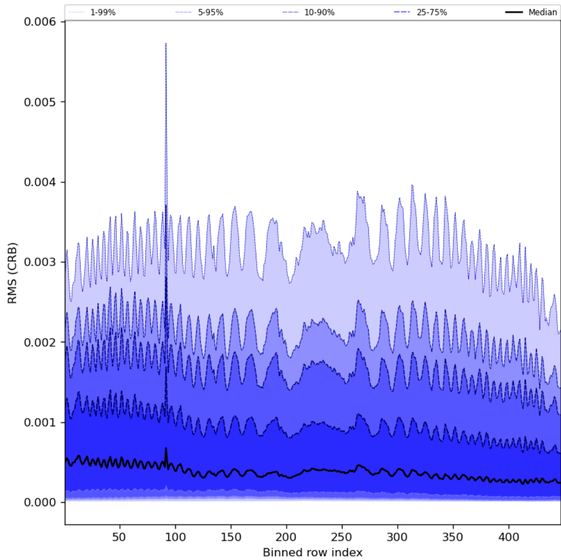
Figure 64: Along track statistics of “RMS (CRB)” for 2024-01-31 to 2024-02-01
