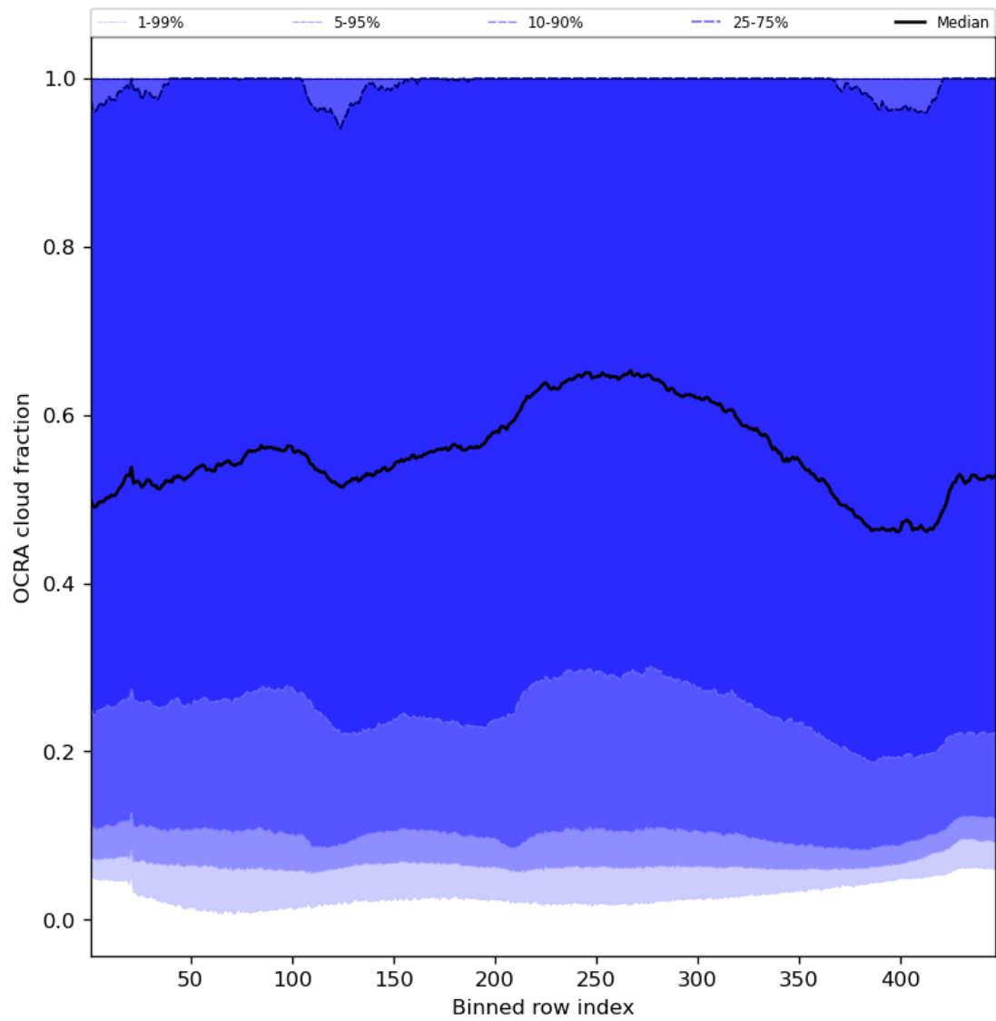
Figure 66: Along track statistics of “OCRA cloud fraction” for 2024-01-31 to 2024-02-01
