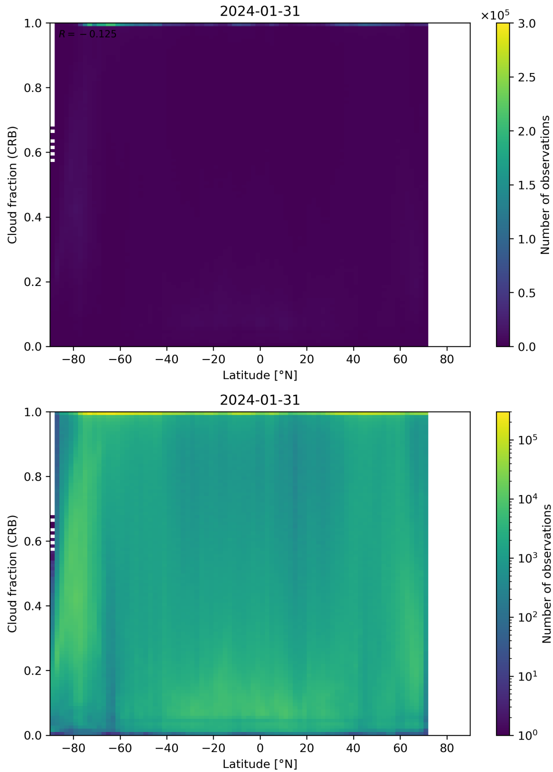
Figure 94: Scatter density plot of “Latitude” against “Cloud fraction (CRB)” for 2024-01-31 to 2024-02-01.
