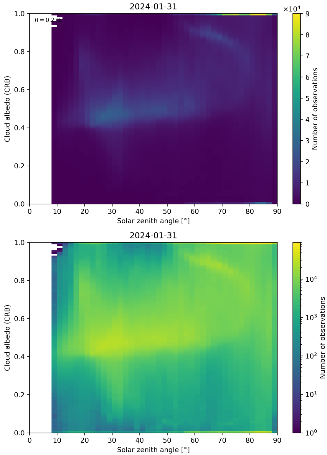
Figure 98: Scatter density plot of “Solar zenith angle” against “Cloud albedo (CRB)” for 2024-01-31 to 2024-02-01.
