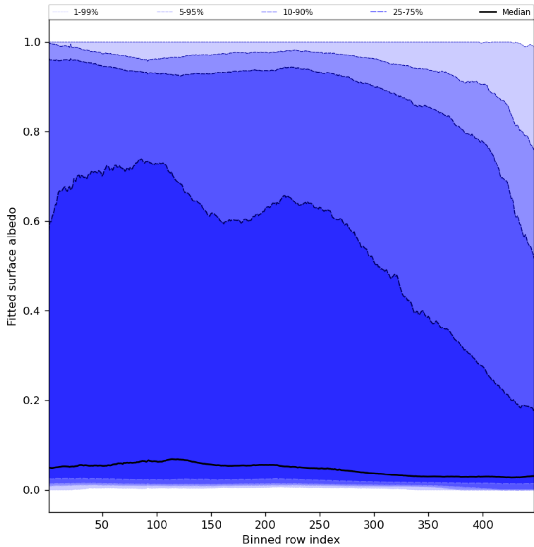
Figure 61: Along track statistics of “Fitted surface albedo” for 2024-01-31 to 2024-02-01
