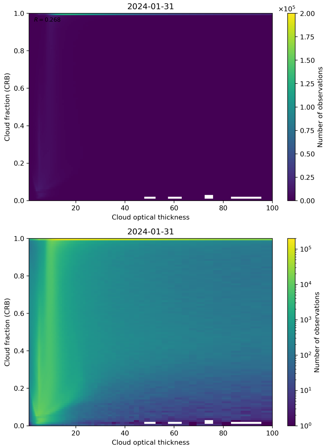
Figure 84: Scatter density plot of “Cloud optical thickness” against “Cloud fraction (CRB)” for 2024-01-31 to 2024-02-01.
