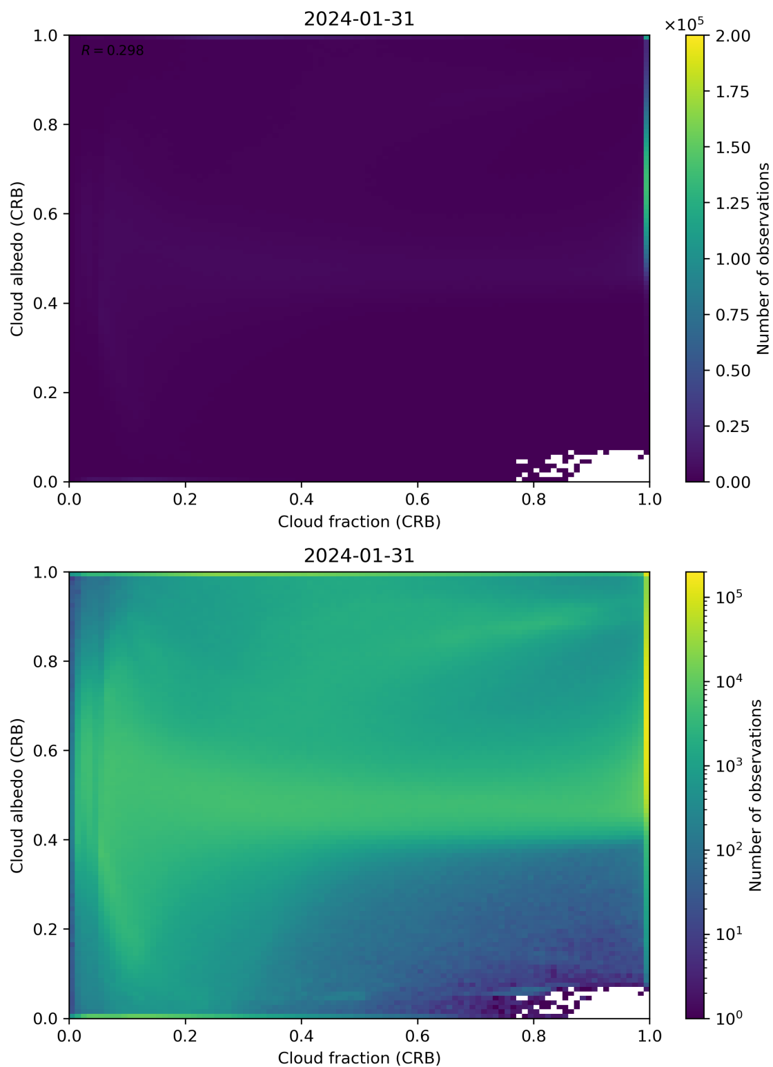
Figure 77: Scatter density plot of “Cloud fraction (CRB)” against “Cloud albedo (CRB)” for 2024-01-31 to 2024-02-01.
