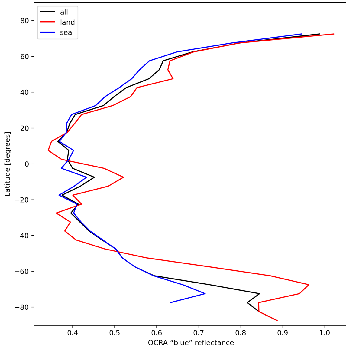
Figure 35: Zonal average of "OCRA "blue" reflectance" for 2024-01-31 to 2024-02-01.
