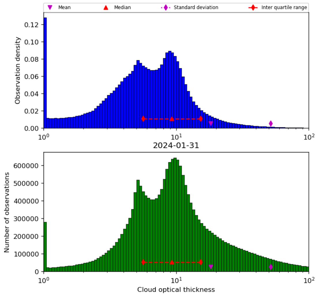
Figure 41: Histogram of “Cloud optical thickness” for 2024-01-31 to 2024-02-01
