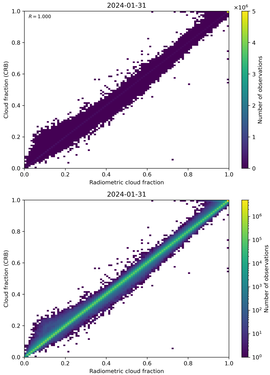
Figure 73: Scatter density plot of “Radiometric cloud fraction” against “Cloud fraction (CRB)” for 2024-01-31 to 2024-02-01.
