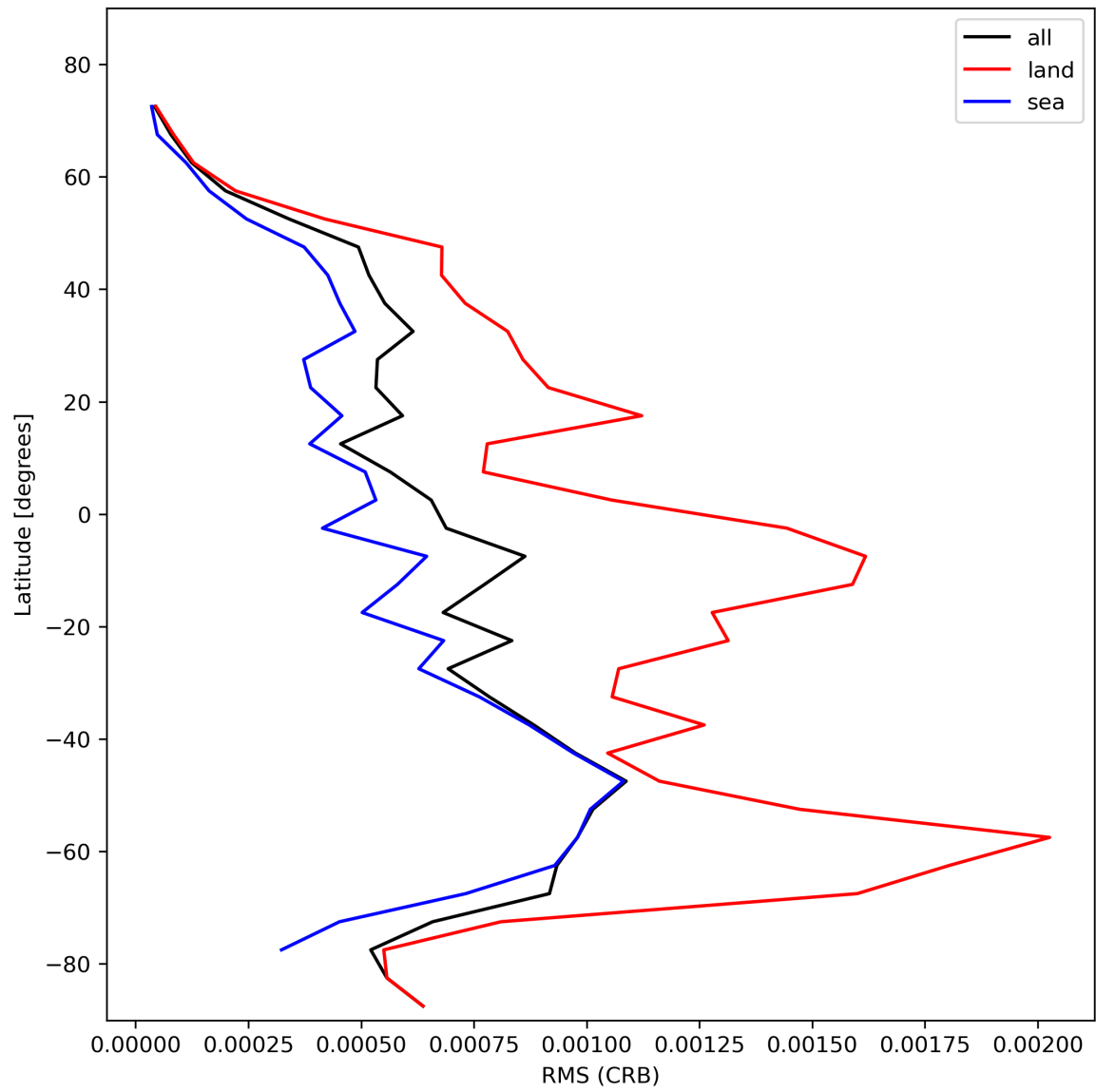
Figure 32: Zonal average of “RMS (CRB)” for 2024-01-31 to 2024-02-01.
