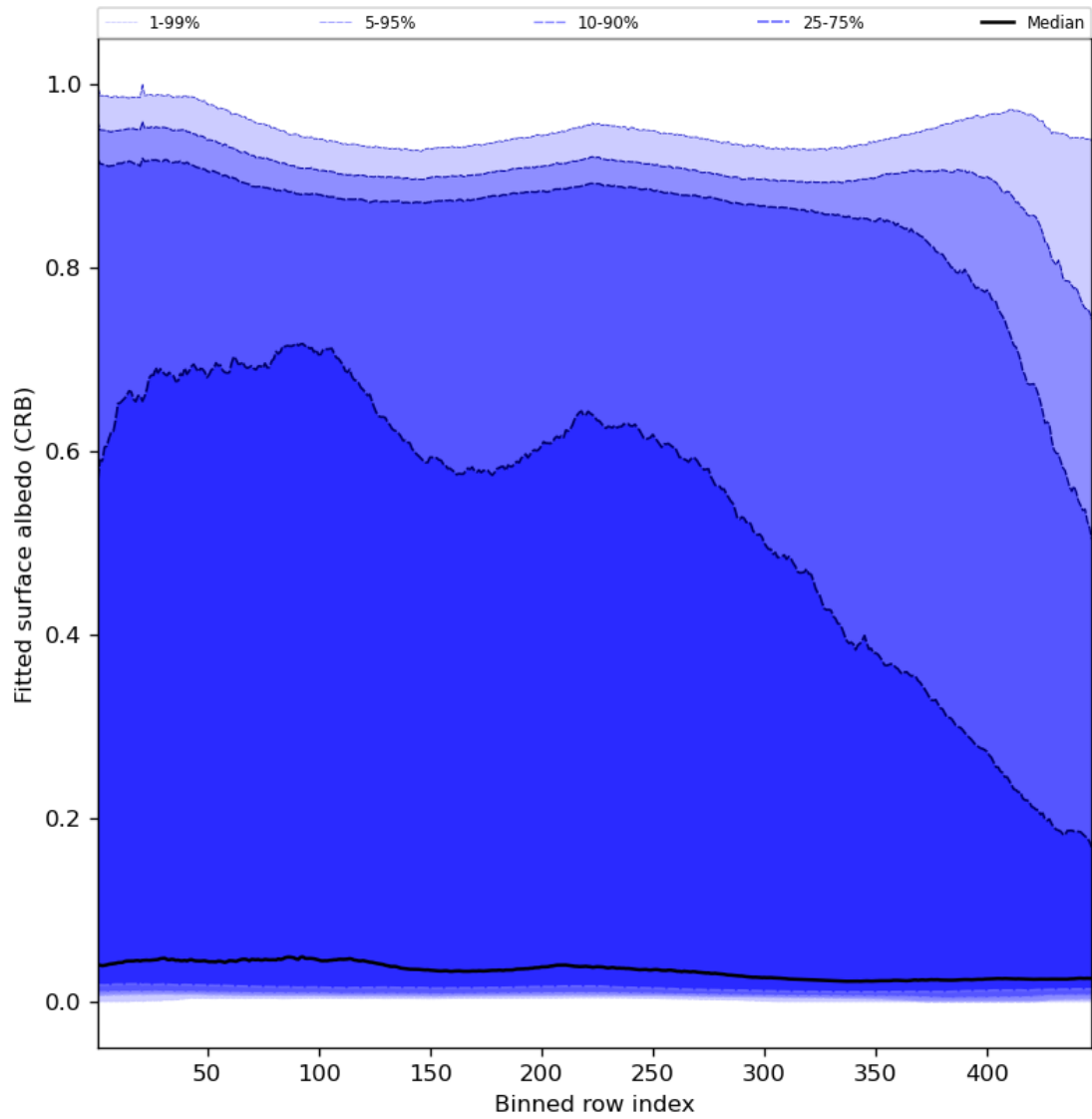
Figure 62: Along track statistics of “Fitted surface albedo (CRB)” for 2024-01-31 to 2024-02-01
