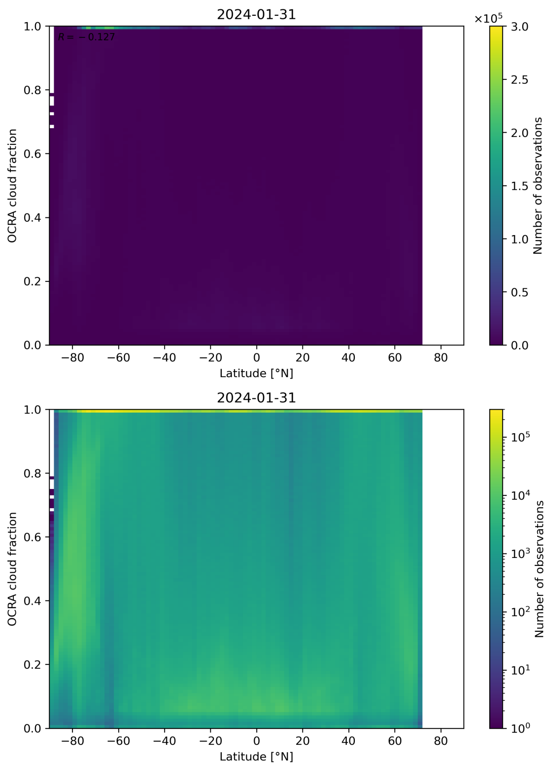
Figure 93: Scatter density plot of “Latitude” against “OCRA cloud fraction” for 2024-01-31 to 2024-02-01.
