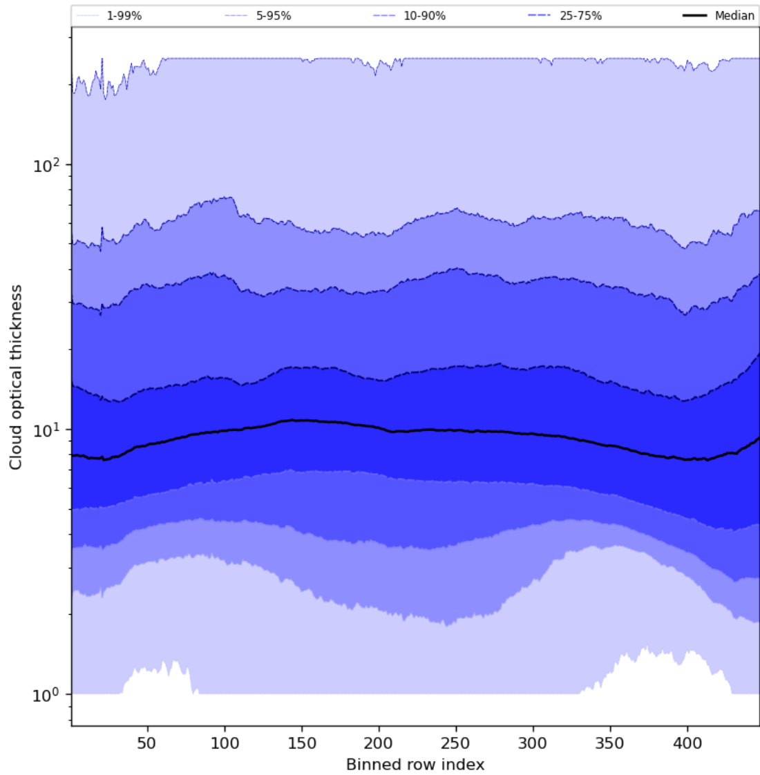
Figure 57: Along track statistics of “Cloud optical thickness” for 2024-01-31 to 2024-02-01
