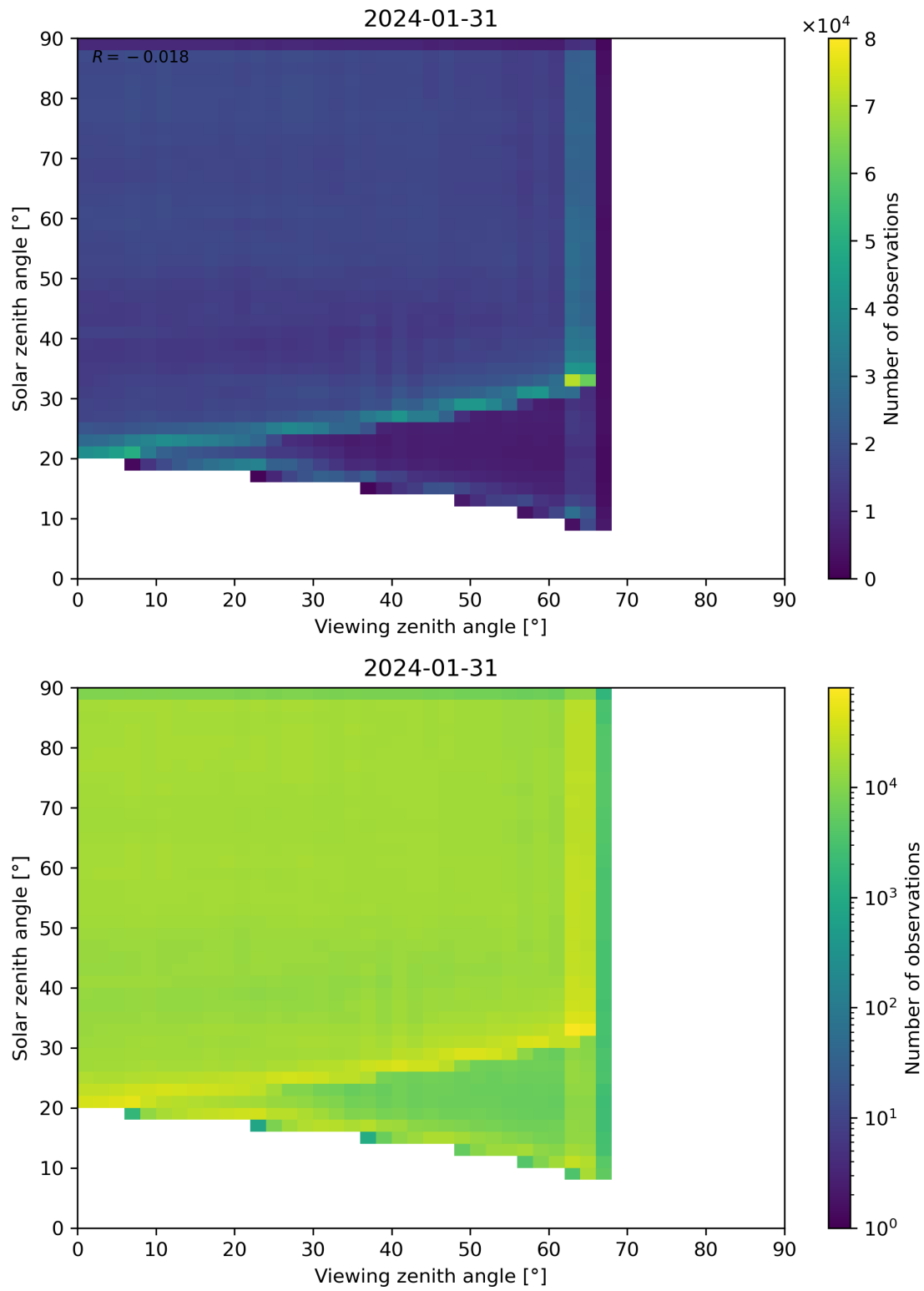
Figure 114: Scatter density plot of “Viewing zenith angle” against “Solar zenith angle” for 2024-01-31 to 2024-02-01.
