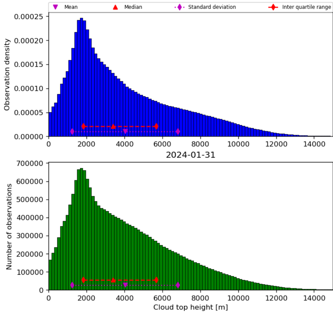
Figure 40: Histogram of “Cloud top height” for 2024-01-31 to 2024-02-01
