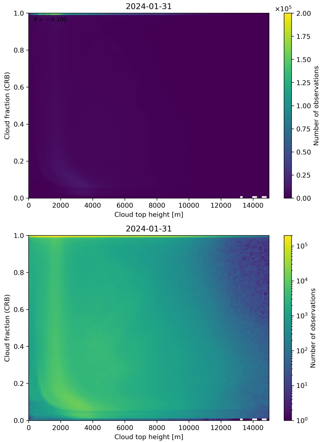
Figure 88: Scatter density plot of “Cloud top height” against “Cloud fraction (CRB)” for 2024-01-31 to 2024-02-01.
