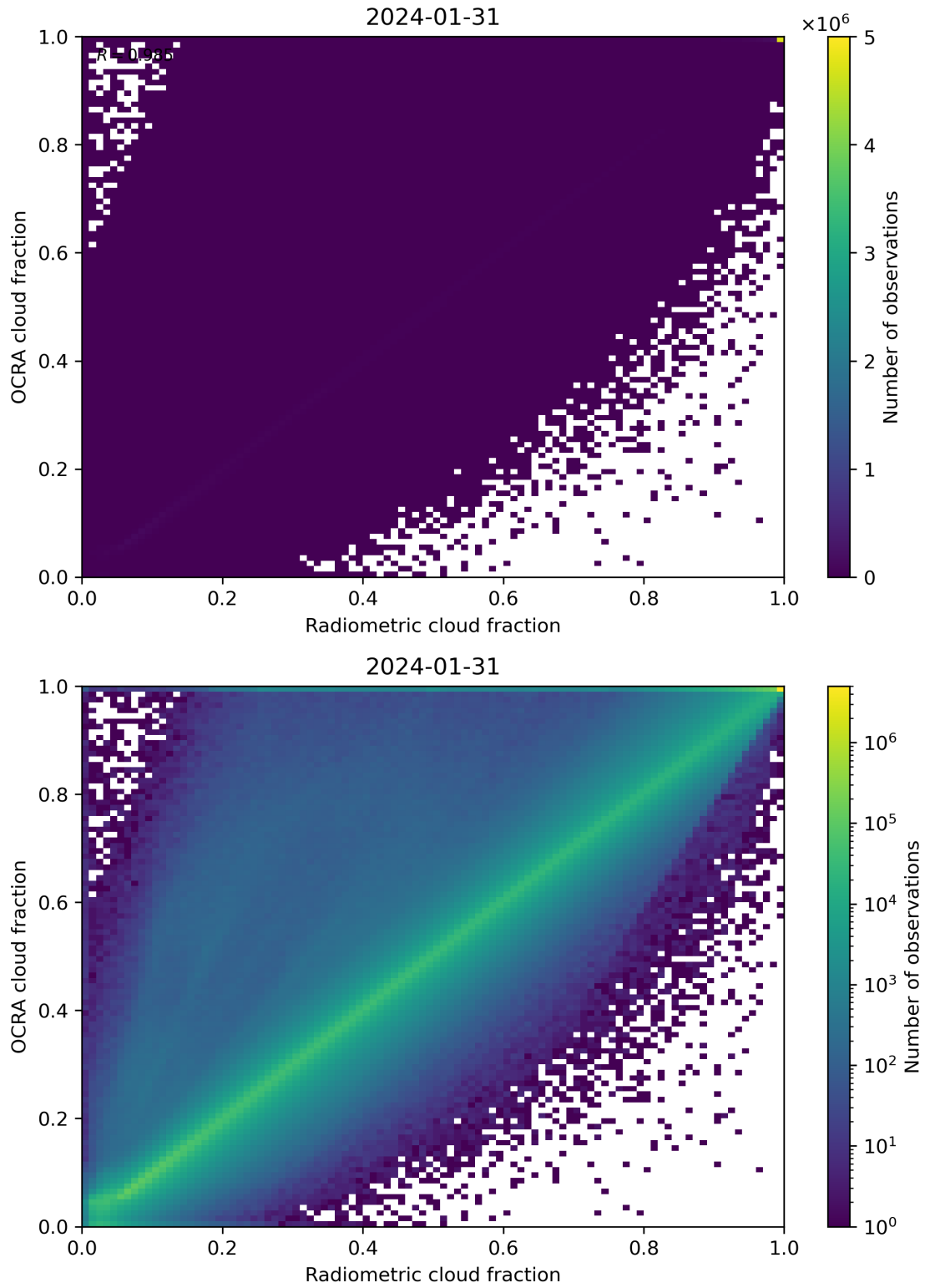
Figure 72: Scatter density plot of “Radiometric cloud fraction” against “OCRA cloud fraction” for 2024-01-31 to 2024-02-01.
