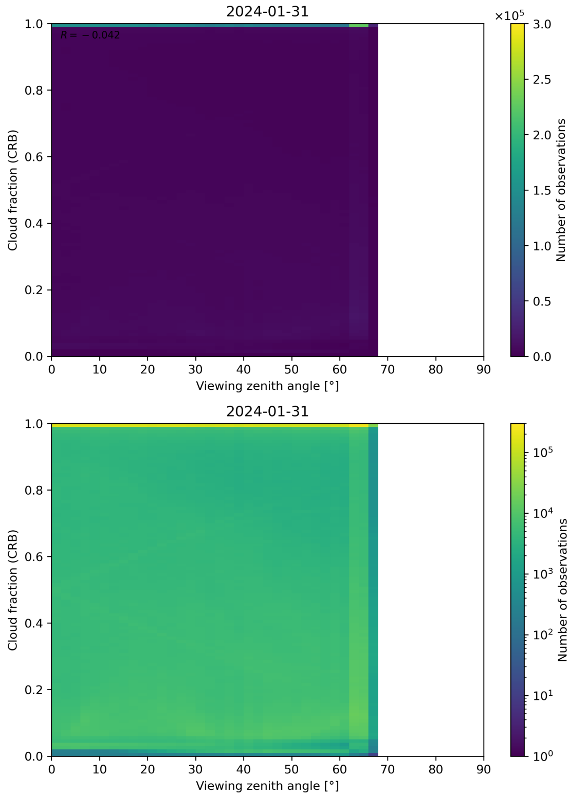
Figure 109: Scatter density plot of “Viewing zenith angle” against “Cloud fraction (CRB)” for 2024-01-31 to 2024-02-01.
