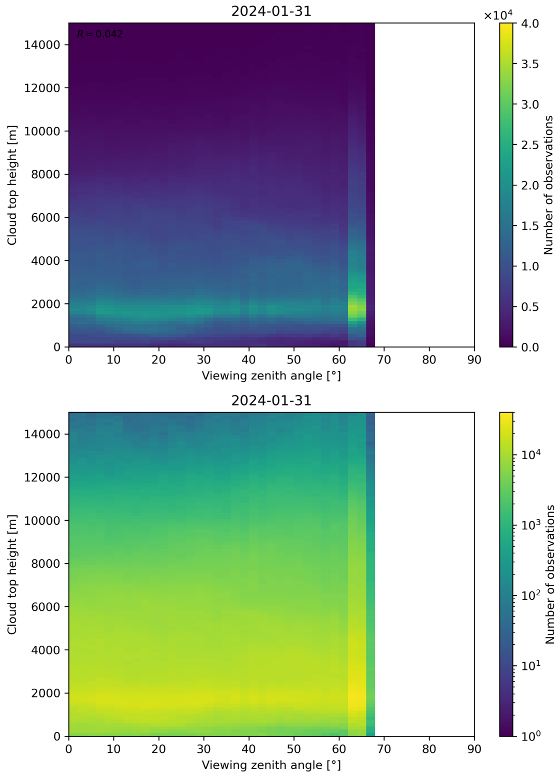
Figure 112: Scatter density plot of “Viewing zenith angle” against “Cloud top height” for 2024-01-31 to 2024-02-01.
