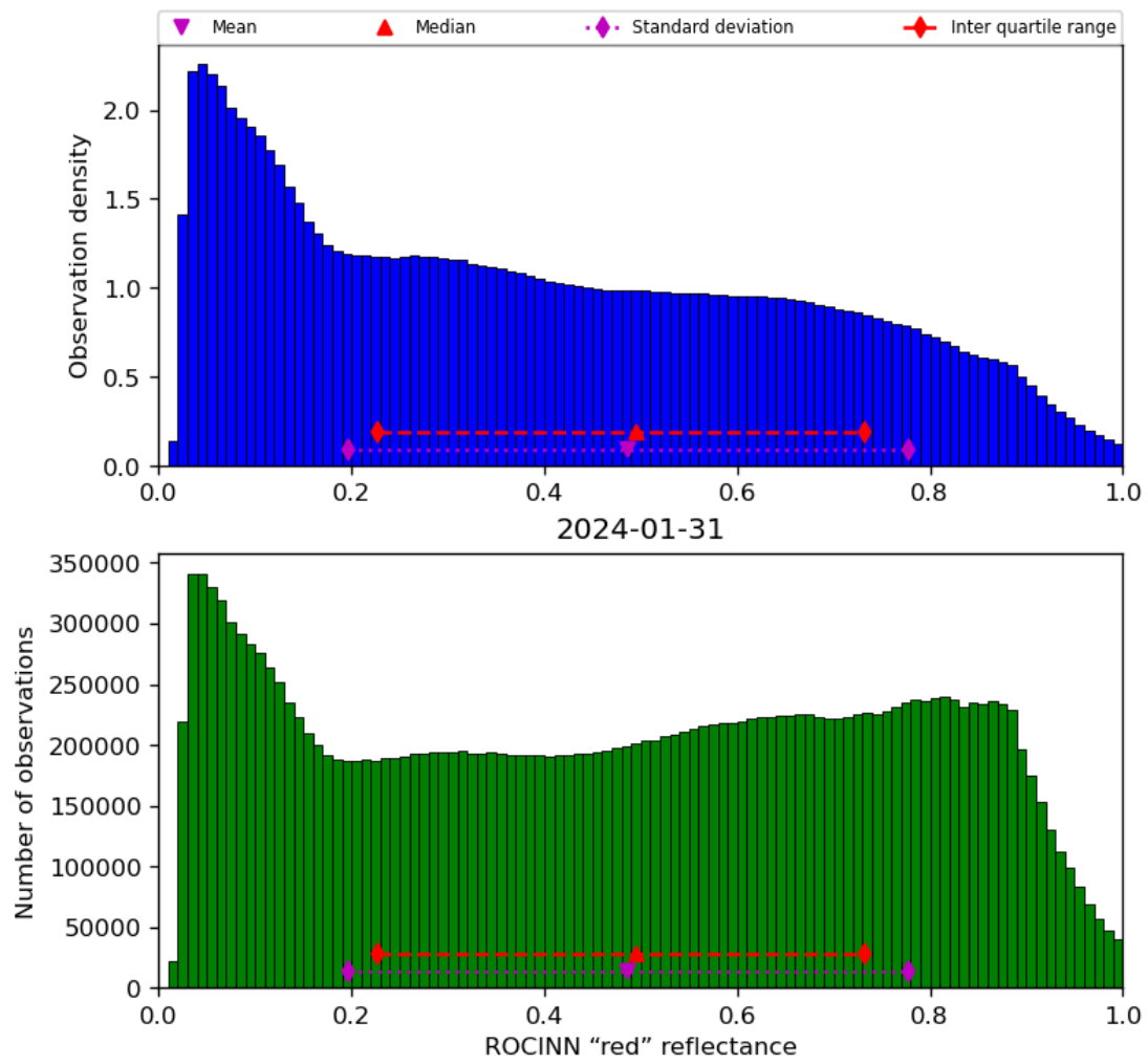
Figure 53: Histogram of “ROCINN “red” reflectance” for 2024-01-31 to 2024-02-01
