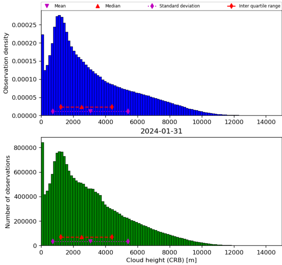
Figure 43: Histogram of “Cloud height (CRB)” for 2024-01-31 to 2024-02-01
