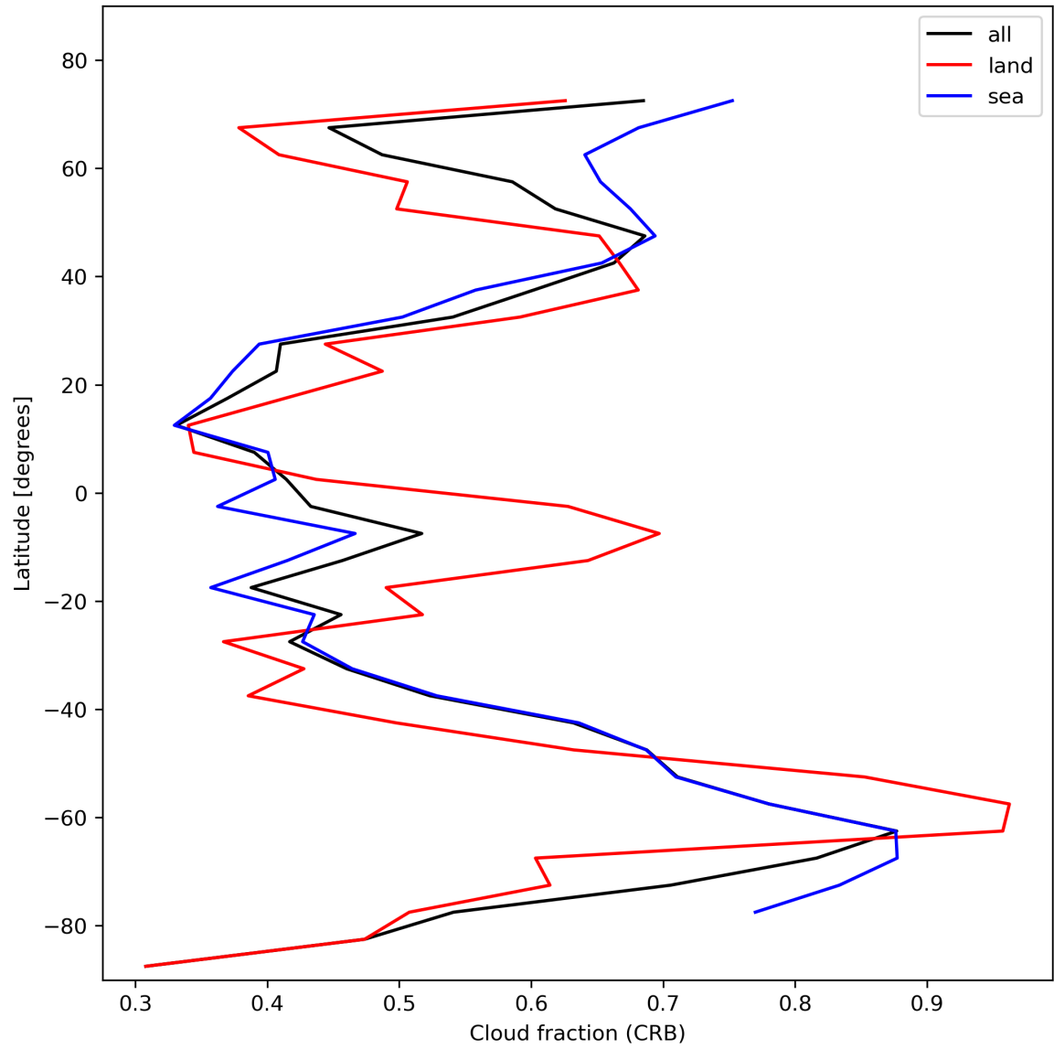
Figure 26: Zonal average of “Cloud fraction (CRB)” for 2024-01-31 to 2024-02-01.
