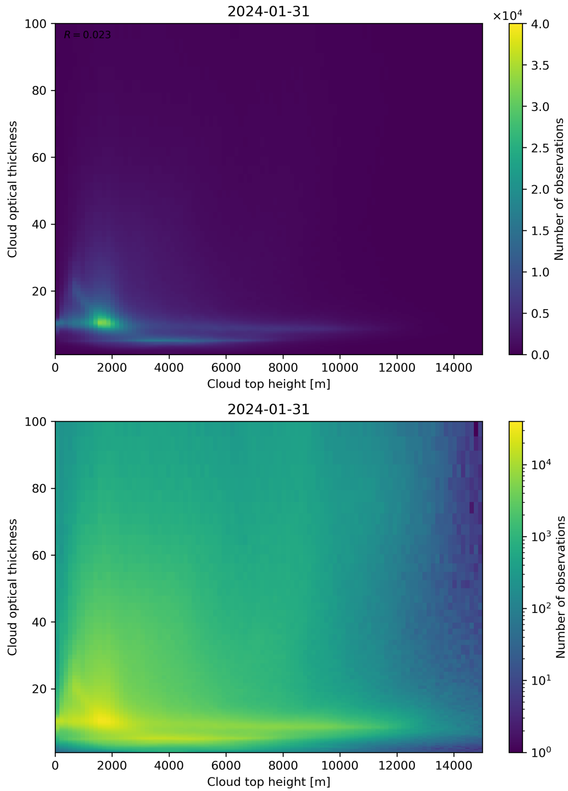
Figure 90: Scatter density plot of “Cloud top height” against “Cloud optical thickness” for 2024-01-31 to 2024-02-01.
