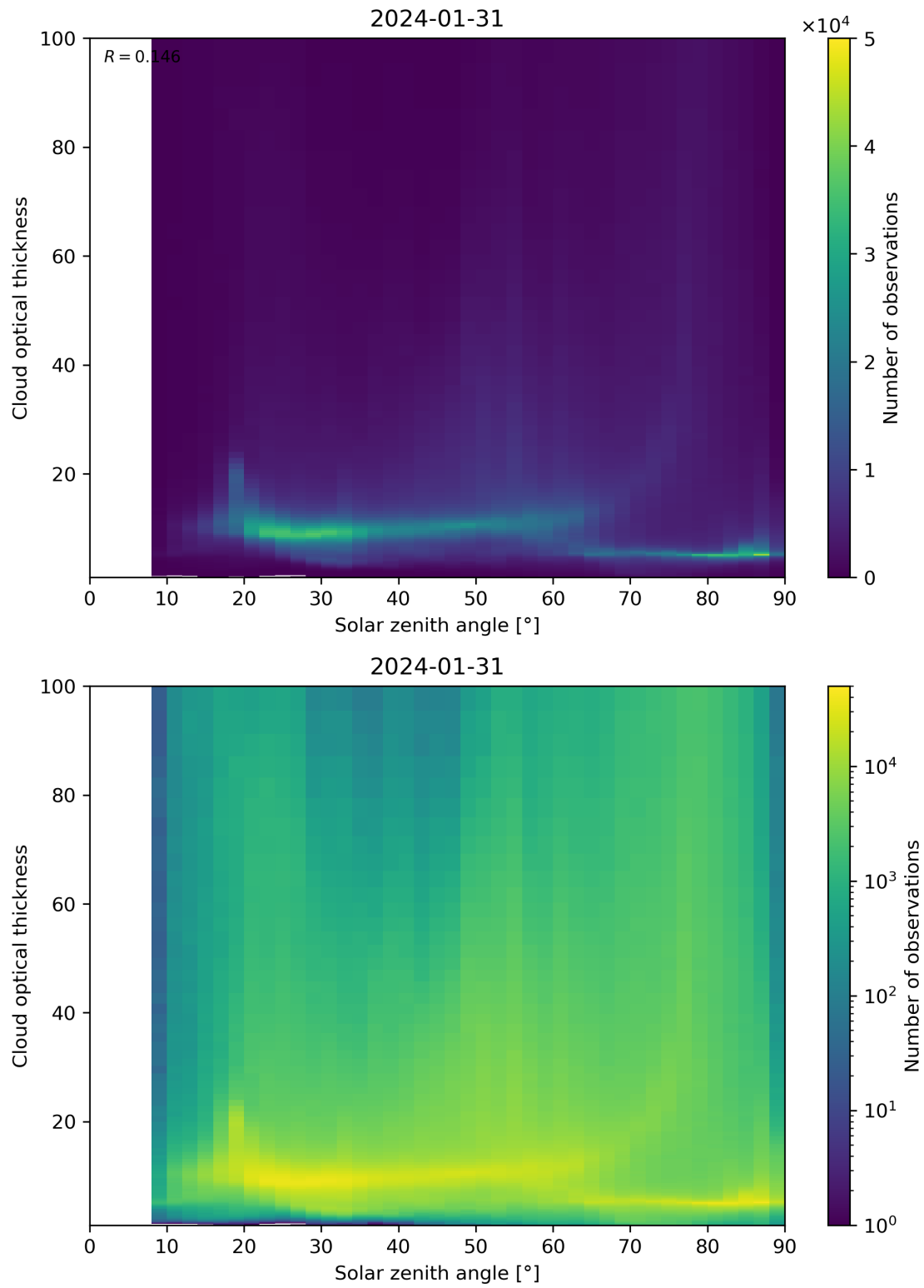
Figure 103: Scatter density plot of “Solar zenith angle” against “Cloud optical thickness” for 2024-01-31 to 2024-02-01.
