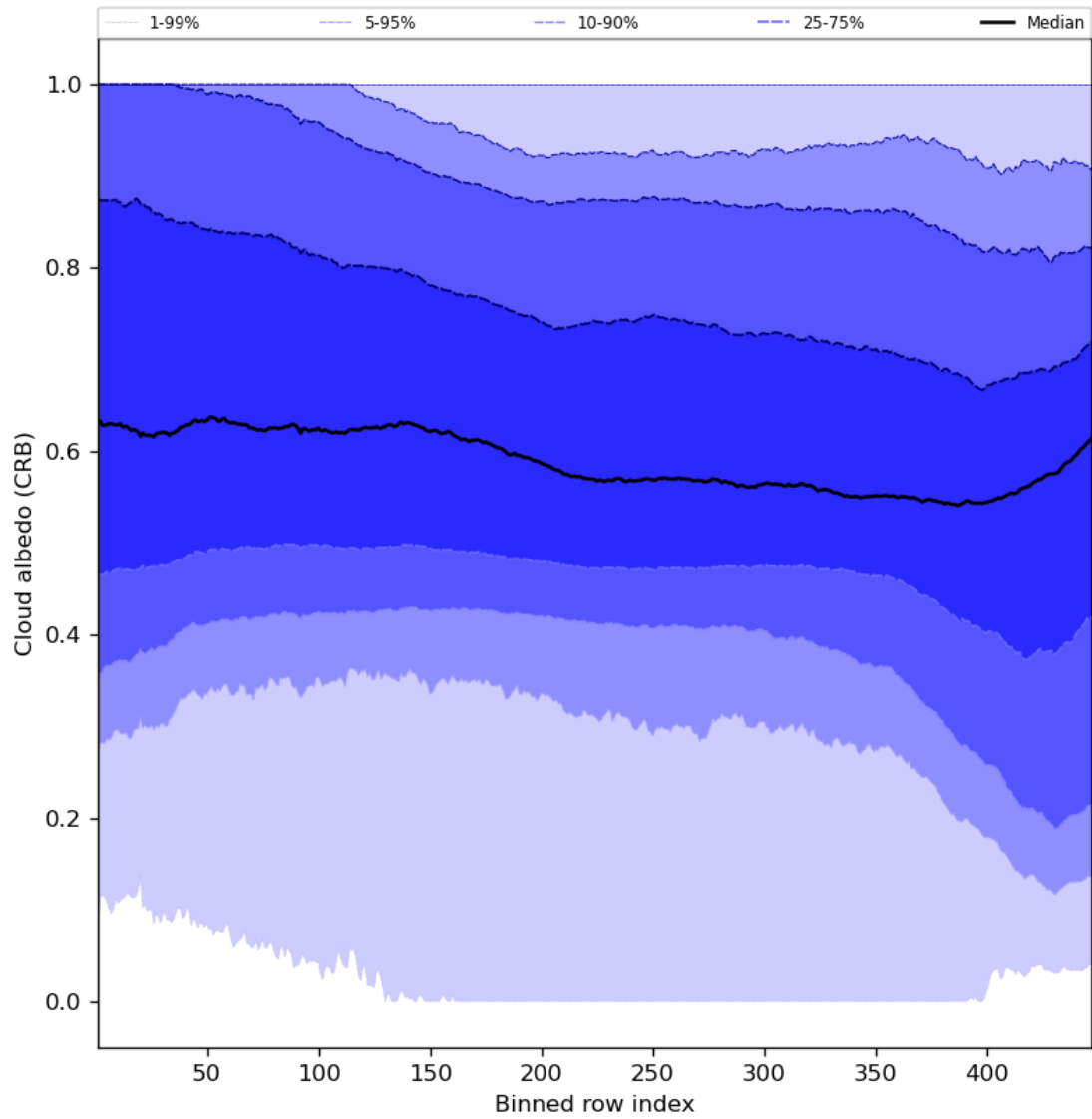
Figure 60: Along track statistics of “Cloud albedo (CRB)” for 2024-01-31 to 2024-02-01
