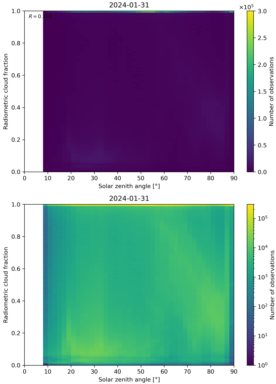
Figure 99: Scatter density plot of “Solar zenith angle” against “Radiometric cloud fraction” for 2024-01-31 to 2024-02-01.
