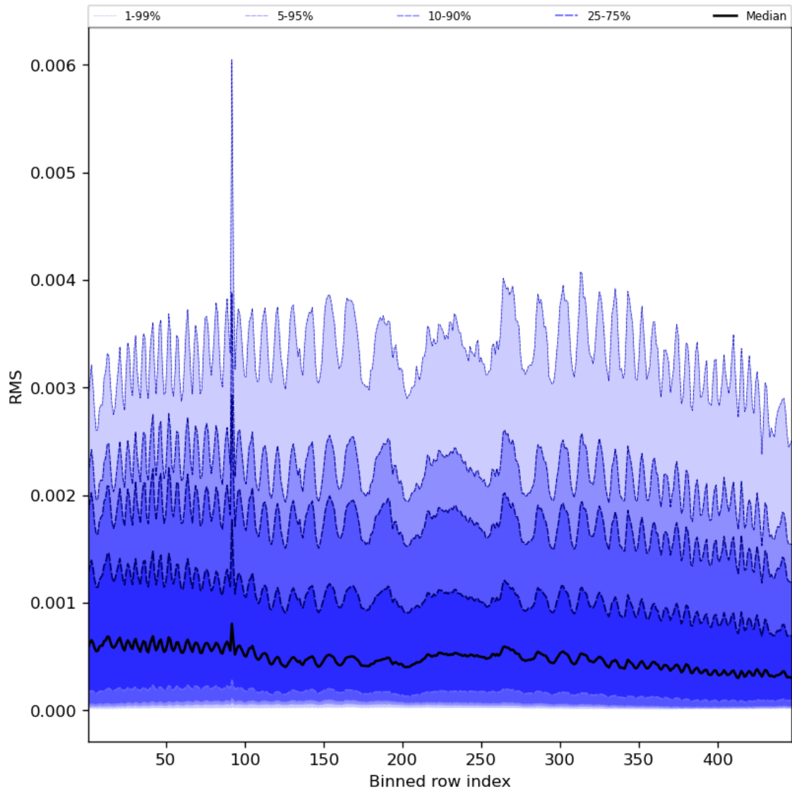
Figure 63: Along track statistics of “RMS” for 2024-01-31 to 2024-02-01
