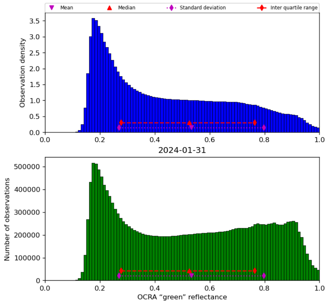
Figure 52: Histogram of “OCRA “green” reflectance” for 2024-01-31 to 2024-02-01
