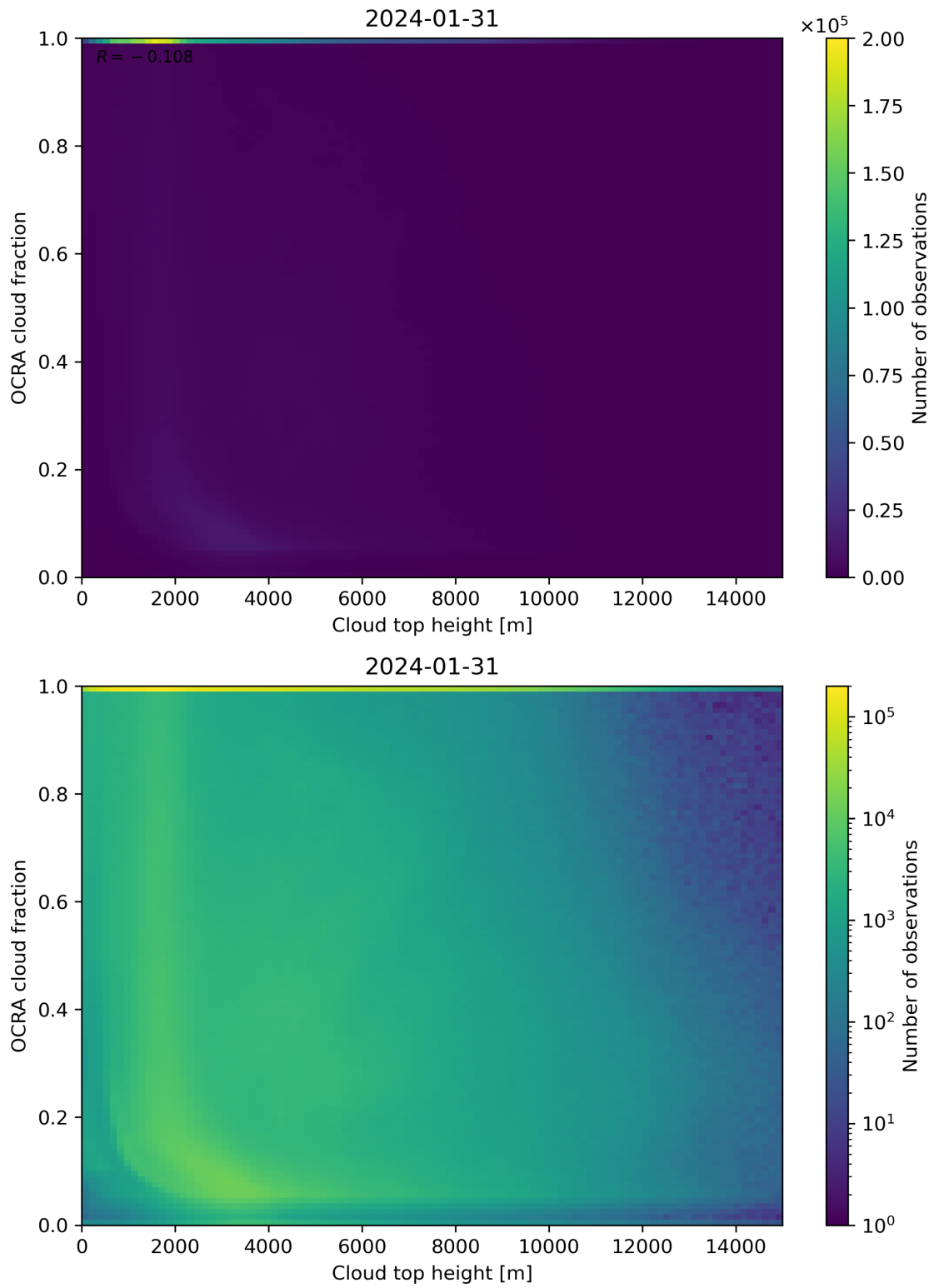
Figure 87: Scatter density plot of “Cloud top height” against “OCRA cloud fraction” for 2024-01-31 to 2024-02-01.
