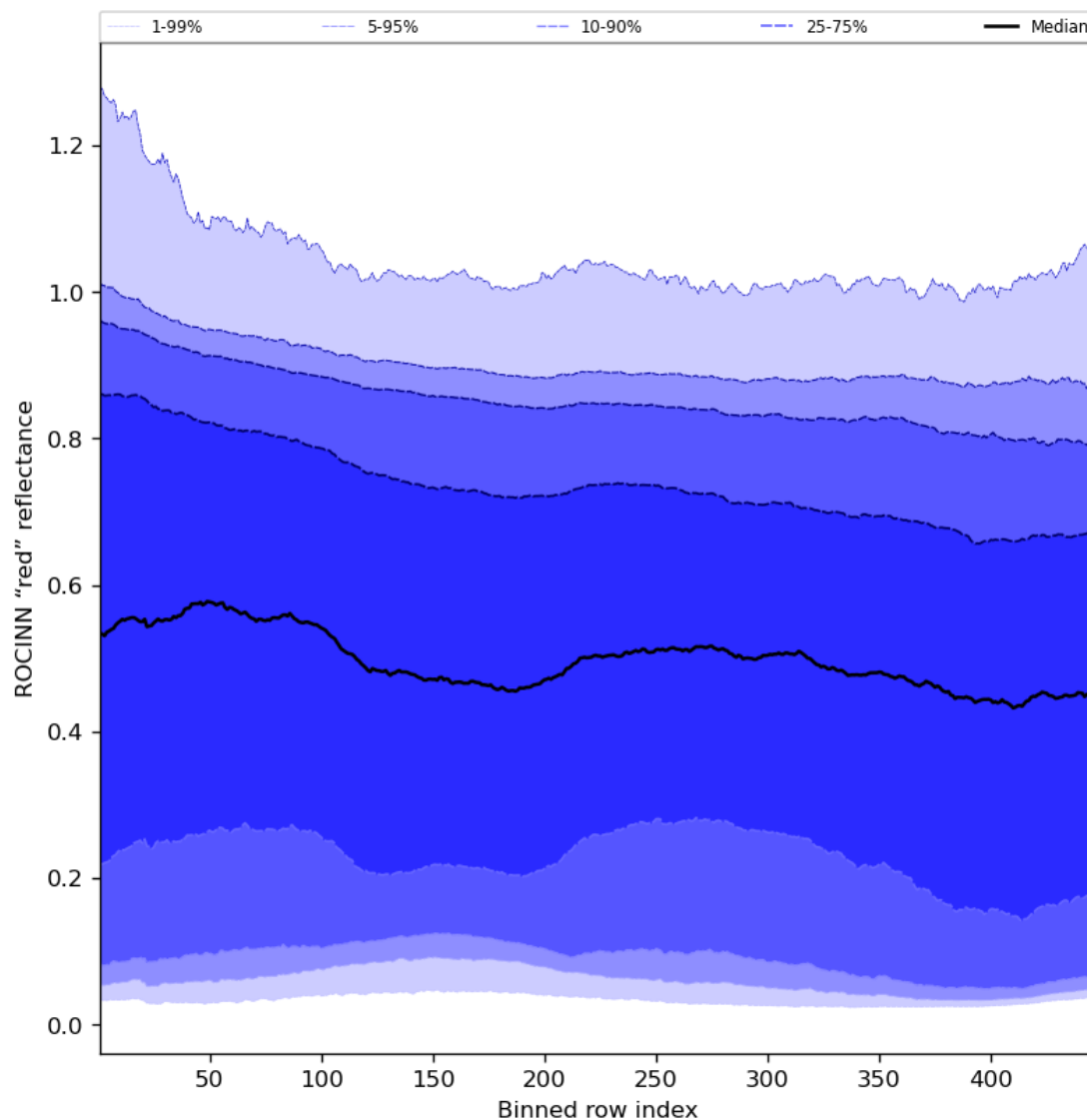
Figure 69: Along track statistics of “ROCINN “red” reflectance” for 2024-01-31 to 2024-02-01
