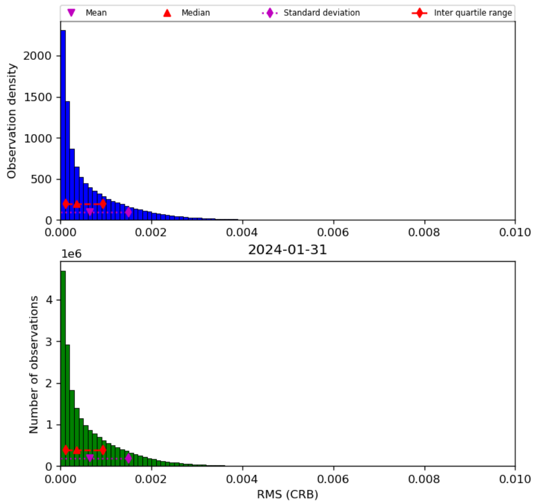
Figure 48: Histogram of “RMS (CRB)” for 2024-01-31 to 2024-02-01
