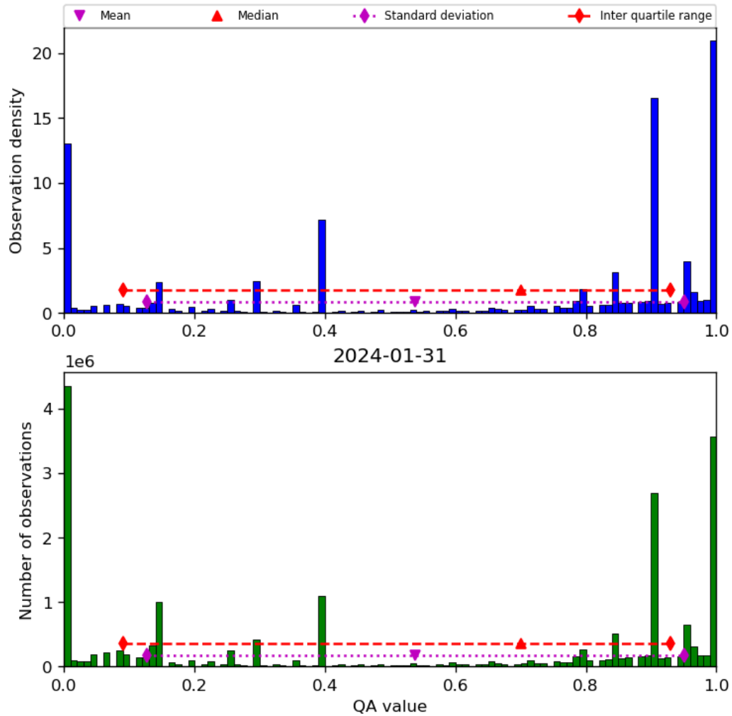
Figure 38: Histogram of “QA value” for 2024-01-31 to 2024-02-01
