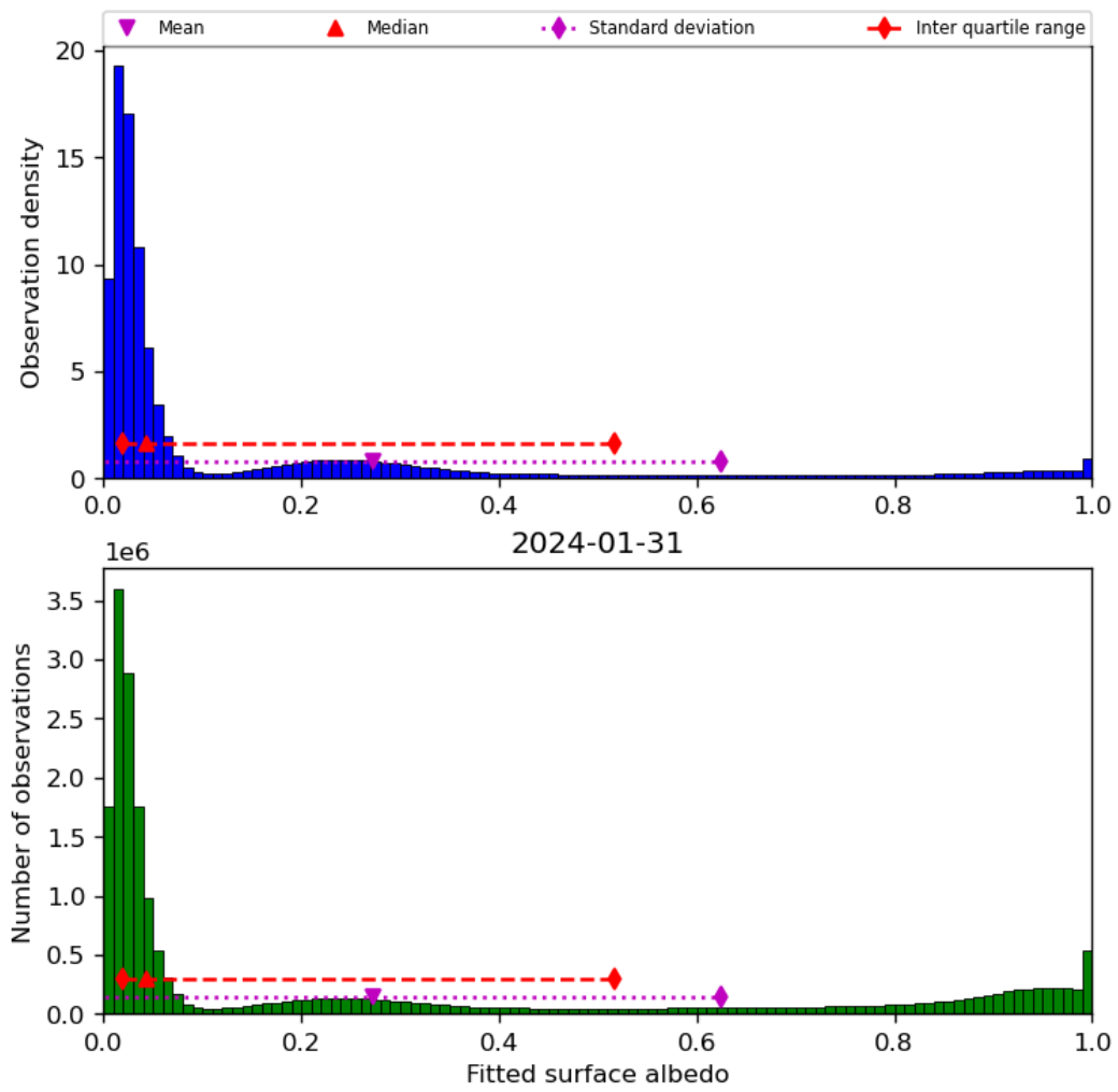
Figure 45: Histogram of “Fitted surface albedo” for 2024-01-31 to 2024-02-01
