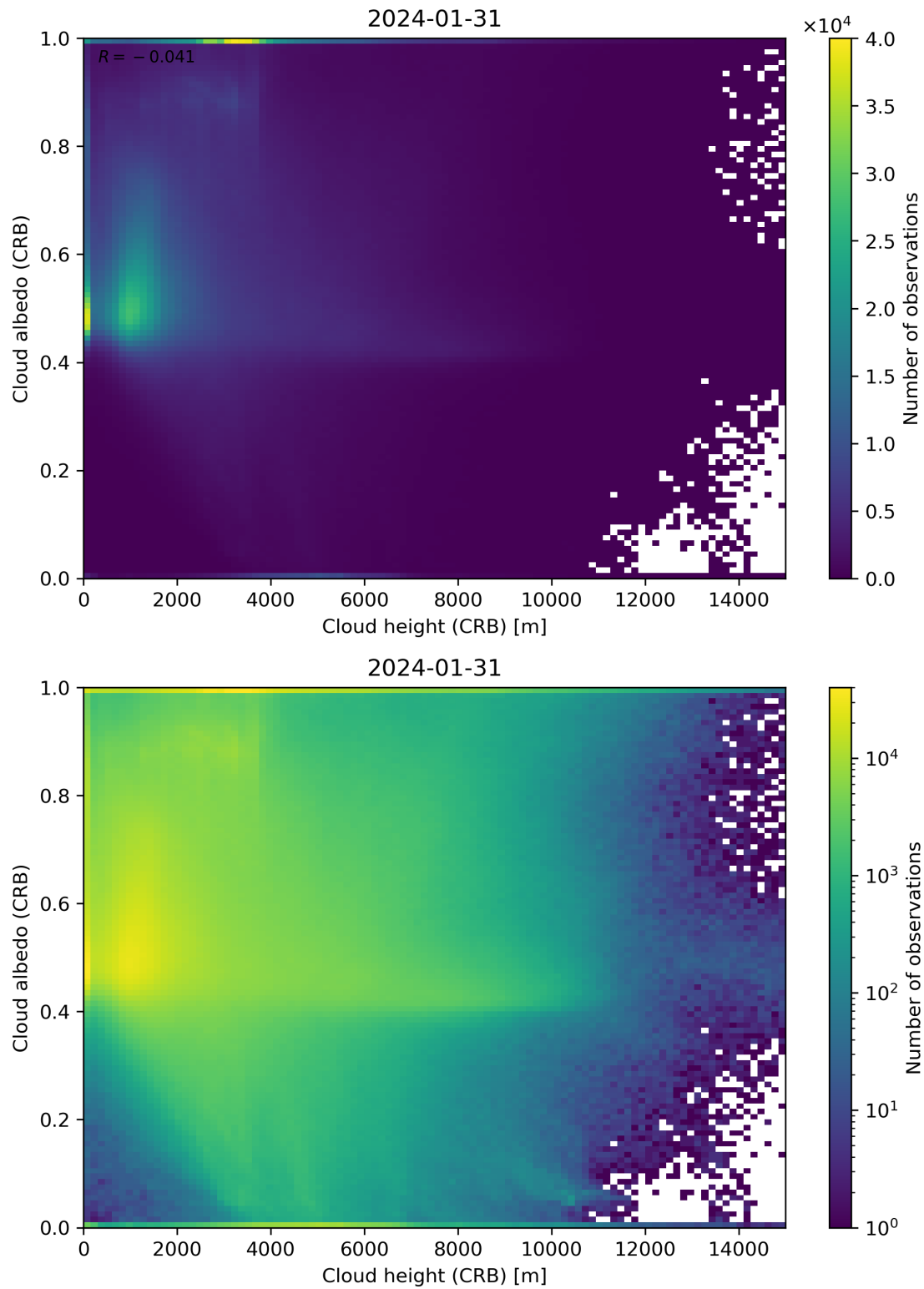
Figure 80: Scatter density plot of “Cloud height (CRB)” against “Cloud albedo (CRB)” for 2024-01-31 to 2024-02-01.
