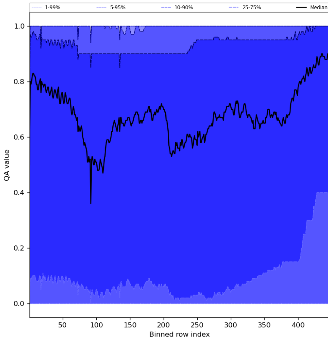
Figure 54: Along track statistics of “QA value” for 2024-01-31 to 2024-02-01
