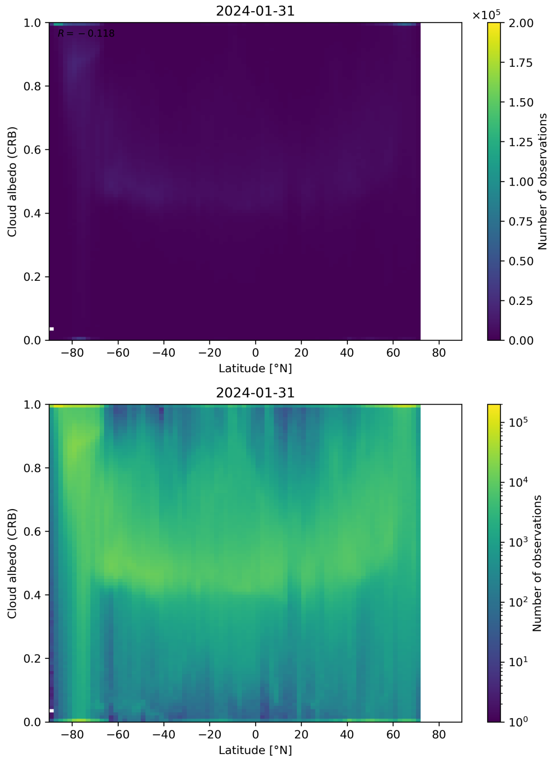
Figure 91: Scatter density plot of “Latitude” against “Cloud albedo (CRB)” for 2024-01-31 to 2024-02-01.
