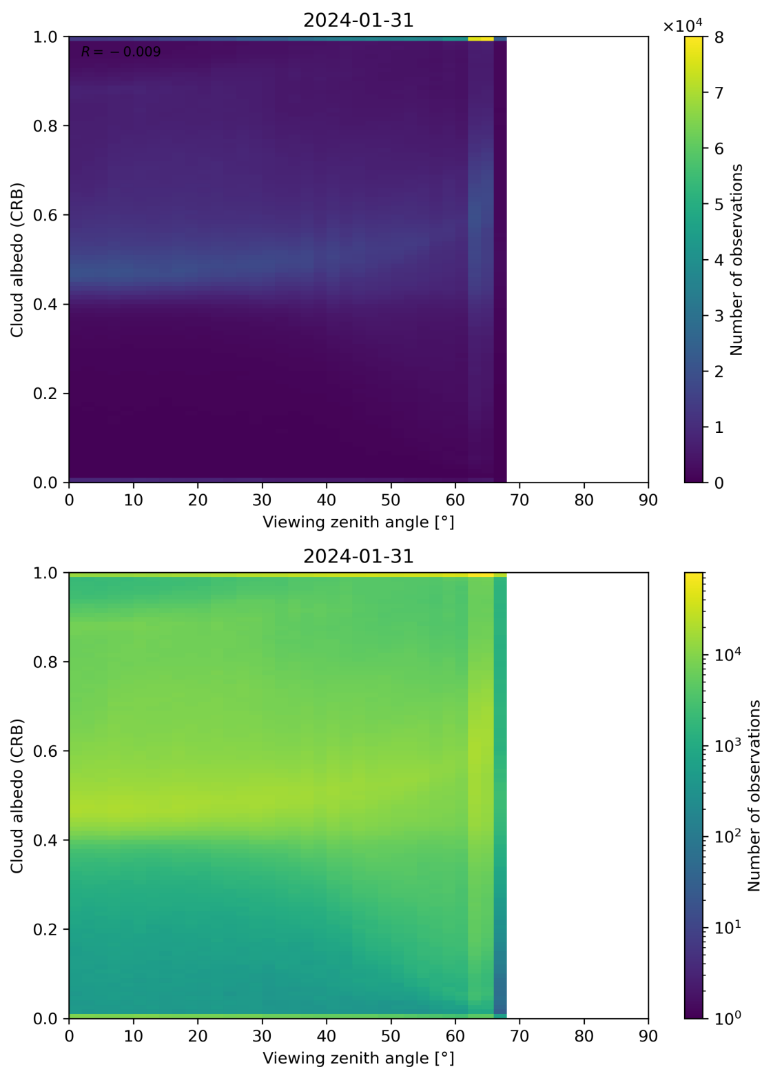
Figure 106: Scatter density plot of “Viewing zenith angle” against “Cloud albedo (CRB)” for 2024-01-31 to 2024-02-01.
