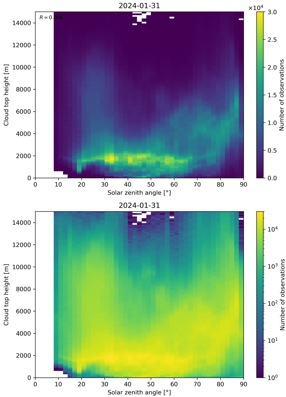
Figure 104: Scatter density plot of “Solar zenith angle” against “Cloud top height” for 2024-01-31 to 2024-02-01.
