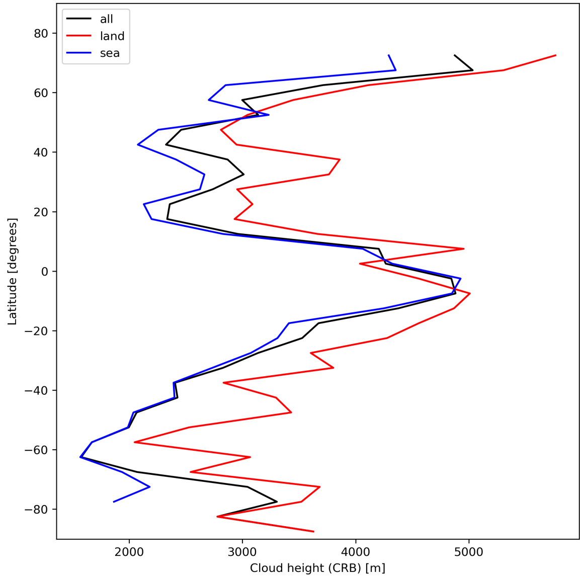
Figure 27: Zonal average of “Cloud height (CRB)” for 2024-01-31 to 2024-02-01.
