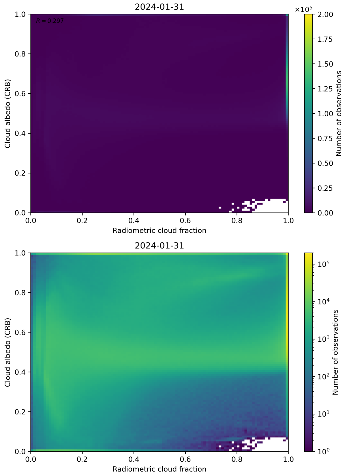
Figure 71: Scatter density plot of “Radiometric cloud fraction” against “Cloud albedo (CRB)” for 2024-01-31 to 2024-02-01.
