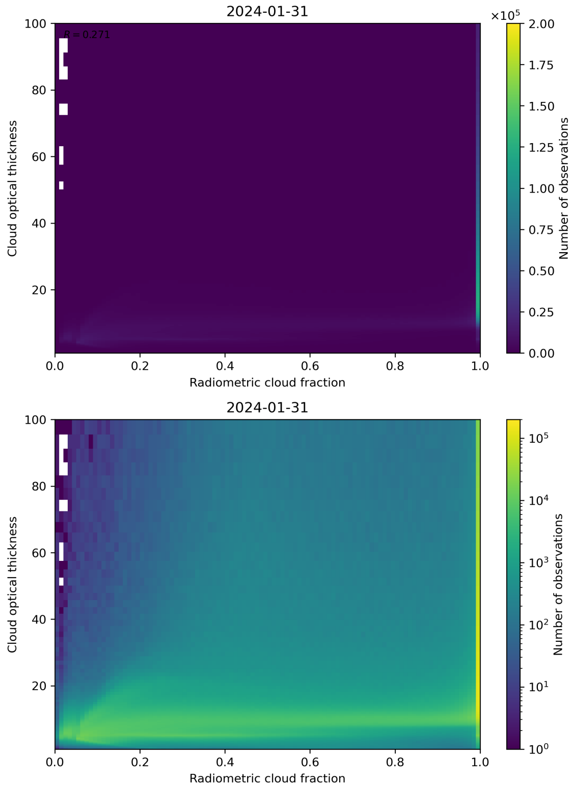
Figure 75: Scatter density plot of “Radiometric cloud fraction” against “Cloud optical thickness” for 2024-01-31 to 2024-02-01.
