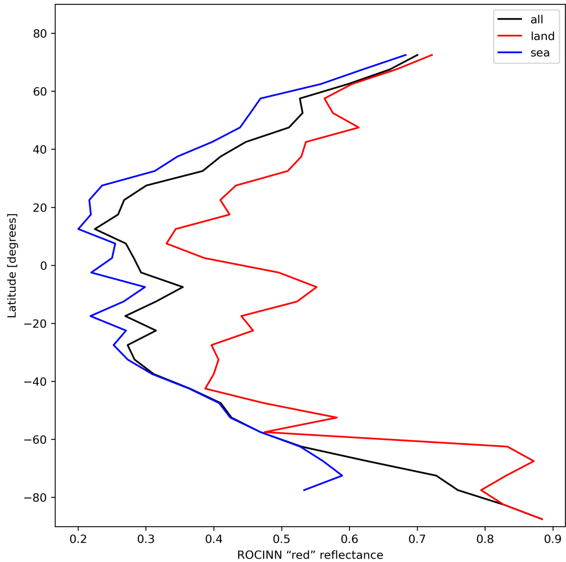
Figure 37: Zonal average of "ROCINN "red" reflectance" for 2024-01-31 to 2024-02-01.
