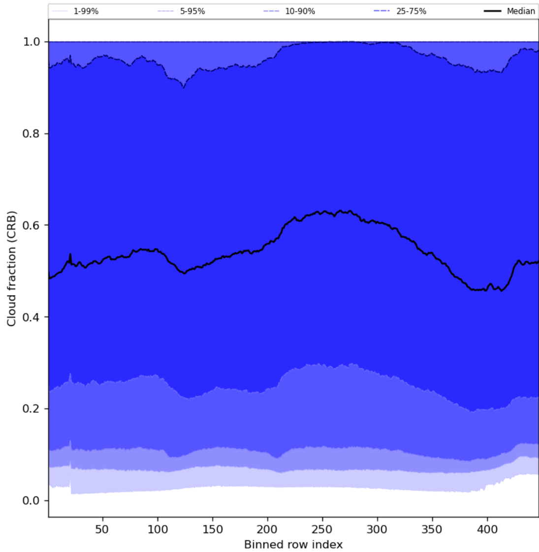
Figure 58: Along track statistics of “Cloud fraction (CRB)” for 2024-01-31 to 2024-02-01
