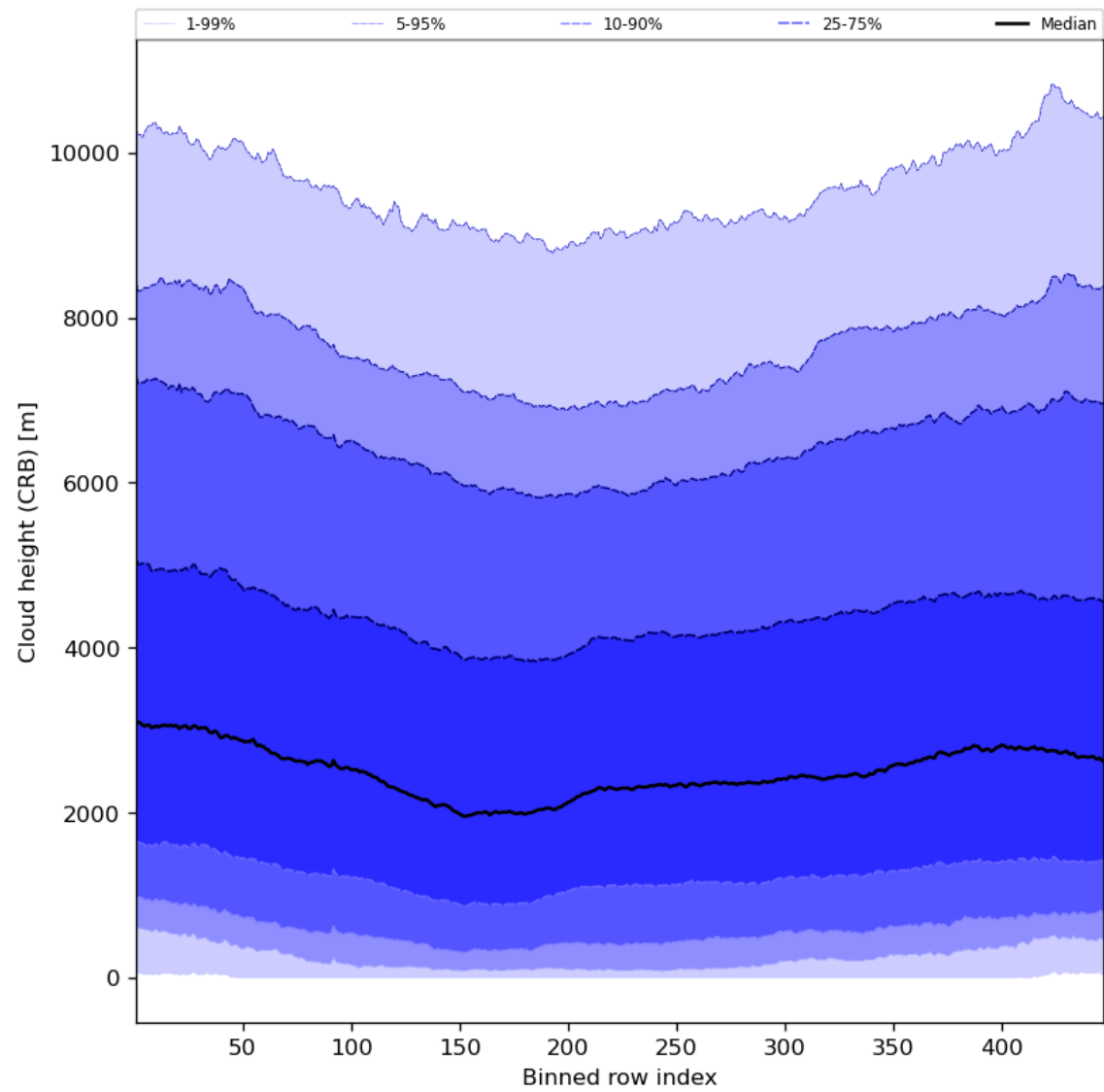
Figure 59: Along track statistics of “Cloud height (CRB)” for 2024-01-31 to 2024-02-01
