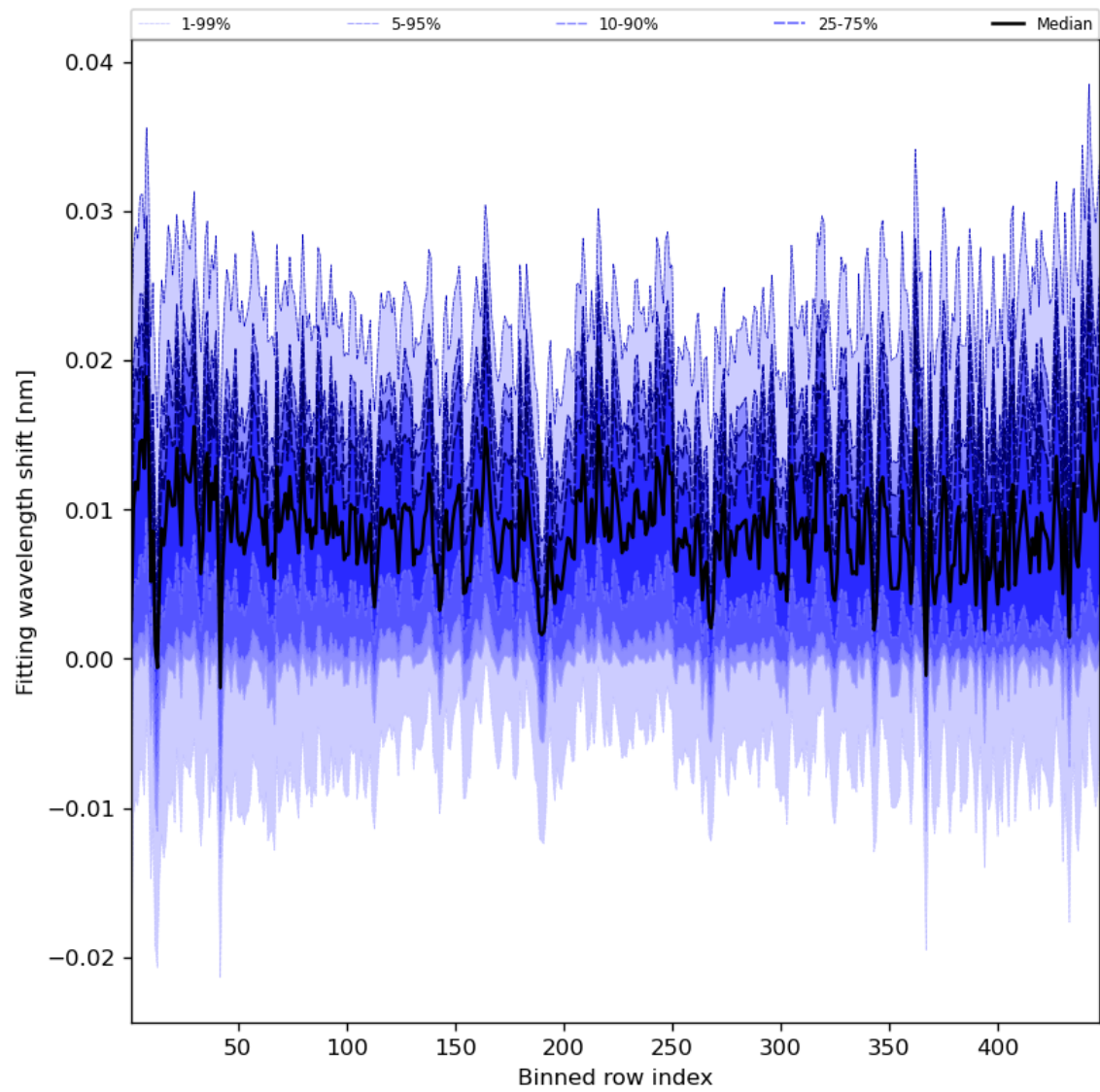
Figure 65: Along track statistics of “Fitting wavelength shift” for 2024-01-31 to 2024-02-01
