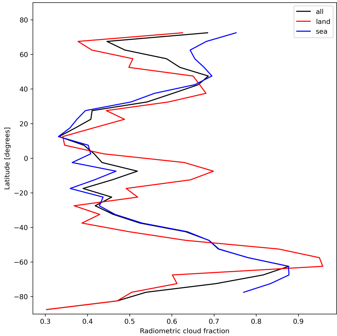
Figure 23: Zonal average of “Radiometric cloud fraction” for 2024-01-31 to 2024-02-01.
