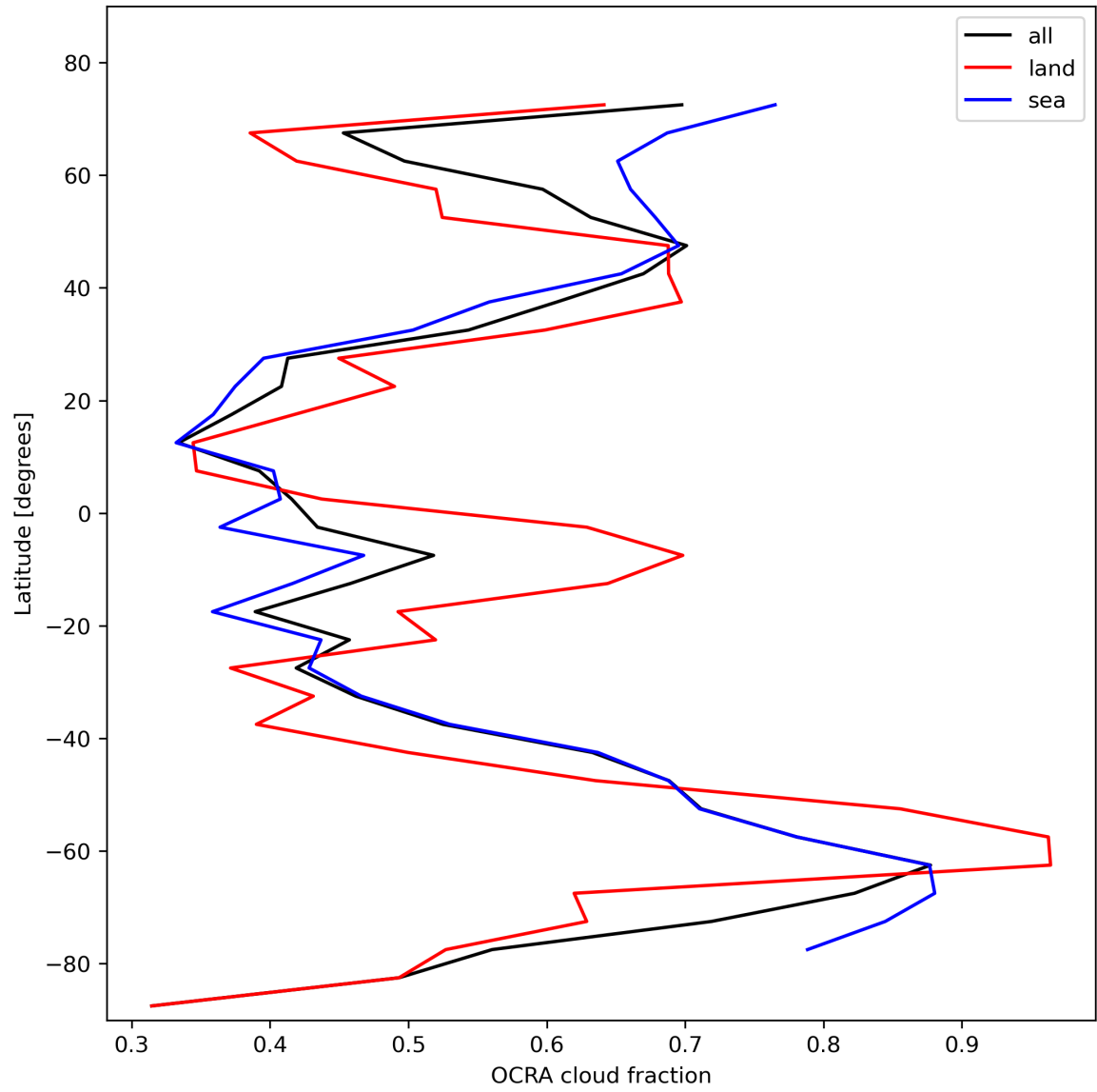
Figure 34: Zonal average of “OCRA cloud fraction” for 2024-01-31 to 2024-02-01.
