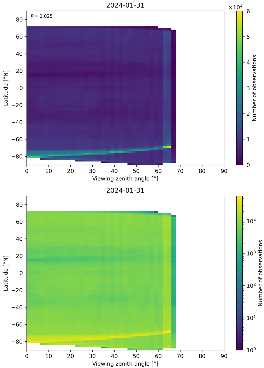
Figure 113: Scatter density plot of “Viewing zenith angle” against “Latitude” for 2024-01-31 to 2024-02-01.
