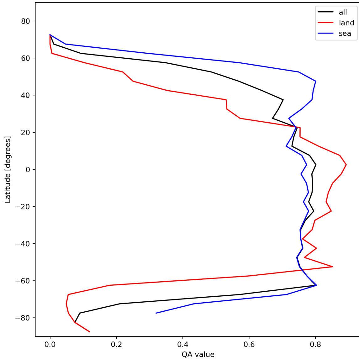
Figure 22: Zonal average of “QA value” for 2024-01-31 to 2024-02-01.
