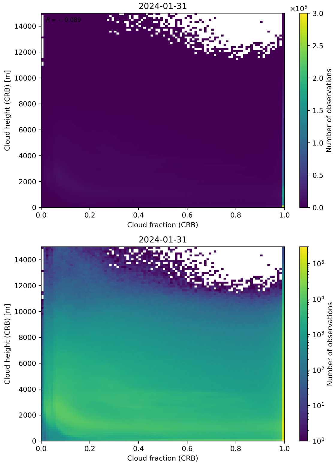
Figure 79: Scatter density plot of “Cloud fraction (CRB)” against “Cloud height (CRB)” for 2024-01-31 to 2024-02-01.
