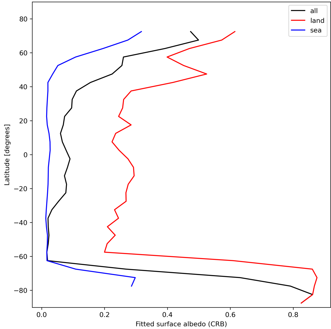
Figure 30: Zonal average of “Fitted surface albedo (CRB)” for 2024-01-31 to 2024-02-01.
