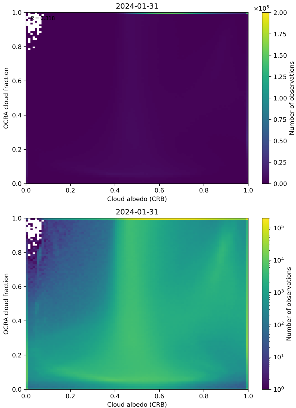
Figure 70: Scatter density plot of “Cloud albedo (CRB)” against “OCRA cloud fraction” for 2024-01-31 to 2024-02-01.
