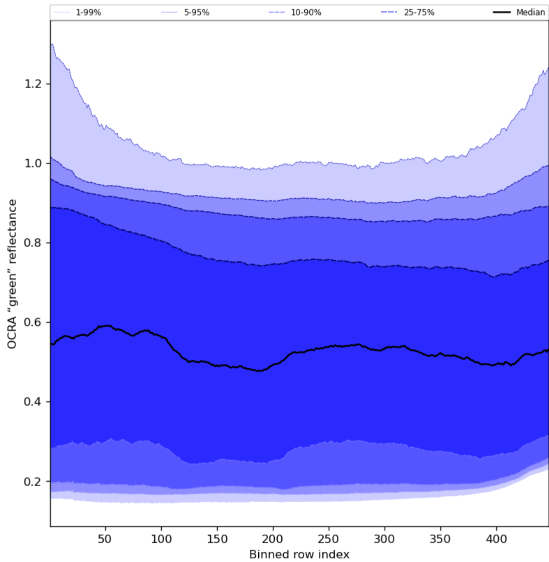
Figure 68: Along track statistics of “OCRA “green” reflectance” for 2024-01-31 to 2024-02-01
