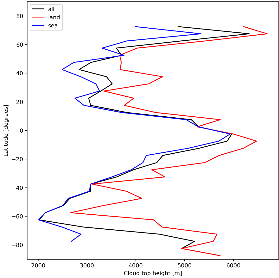
Figure 24: Zonal average of “Cloud top height” for 2024-01-31 to 2024-02-01.
