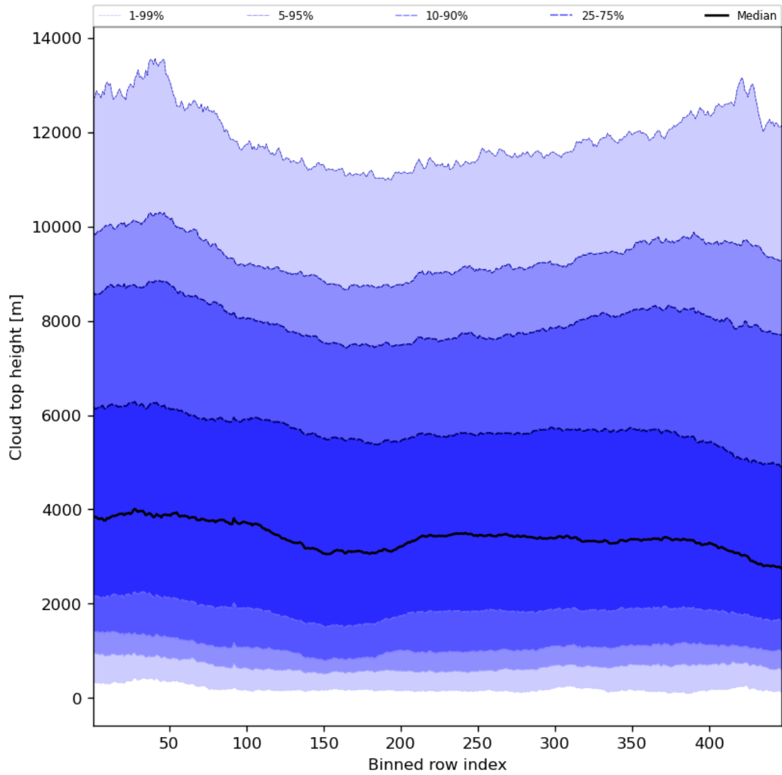
Figure 56: Along track statistics of “Cloud top height” for 2024-01-31 to 2024-02-01
