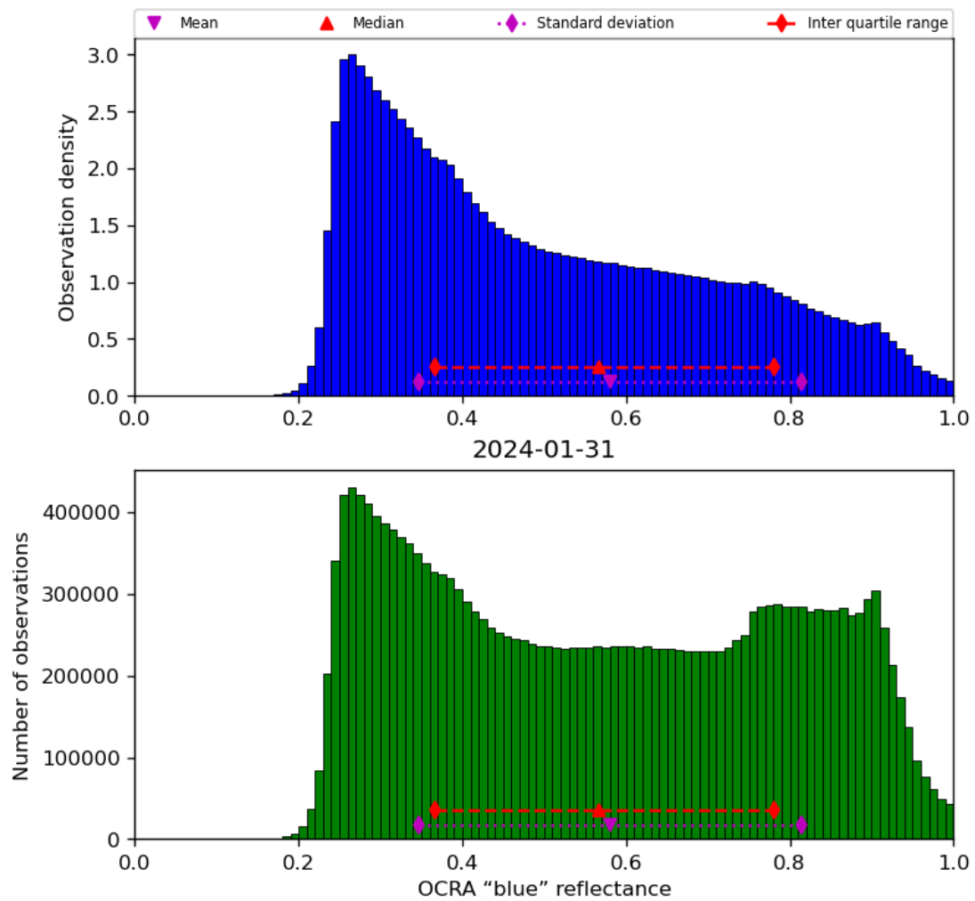
Figure 51: Histogram of “OCRA “blue” reflectance” for 2024-01-31 to 2024-02-01
