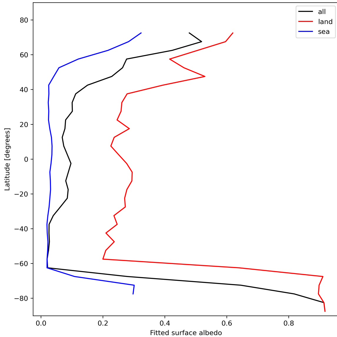
Figure 29: Zonal average of “Fitted surface albedo” for 2024-01-31 to 2024-02-01.
