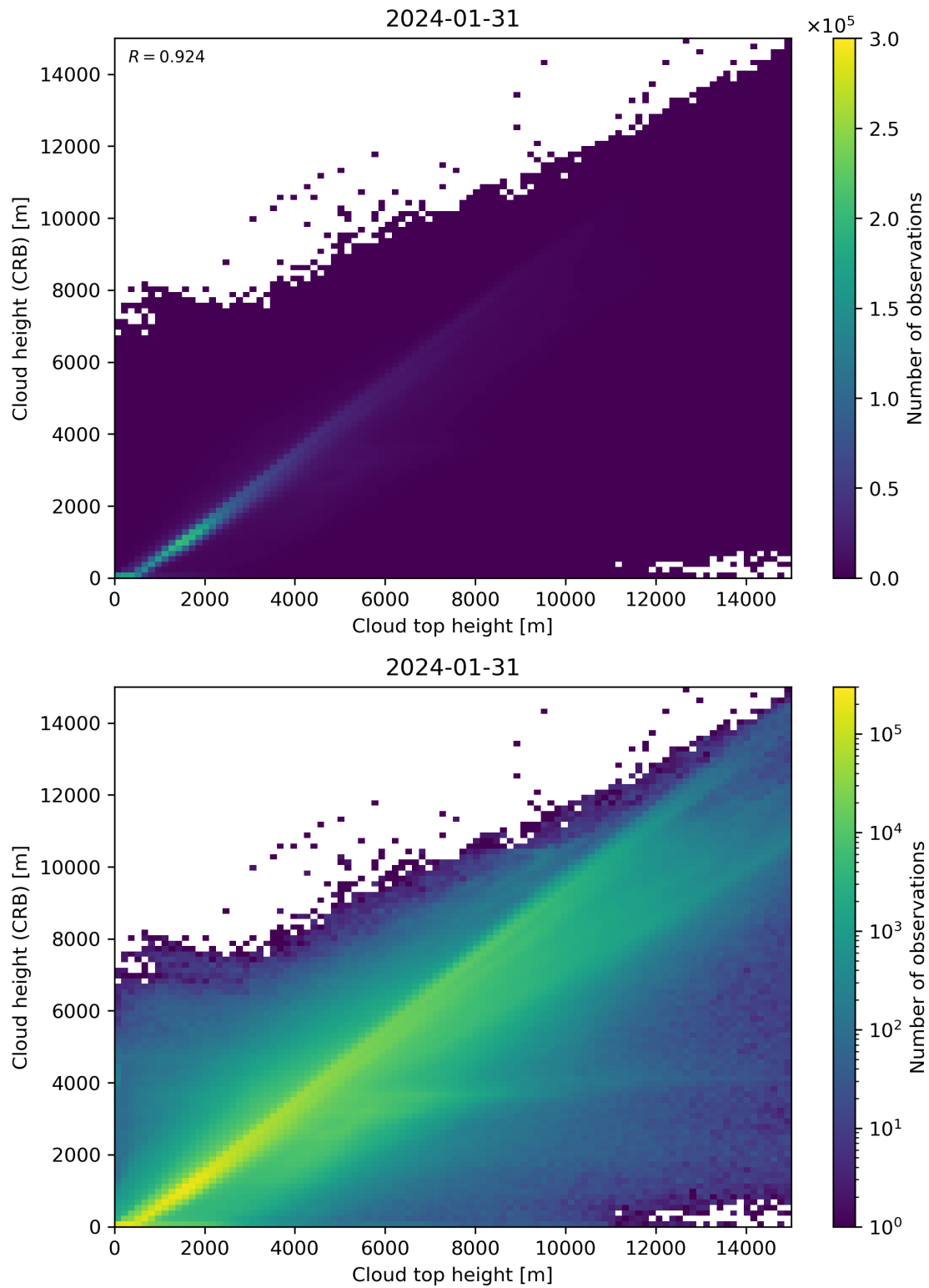
Figure 89: Scatter density plot of “Cloud top height” against “Cloud height (CRB)” for 2024-01-31 to 2024-02-01.
