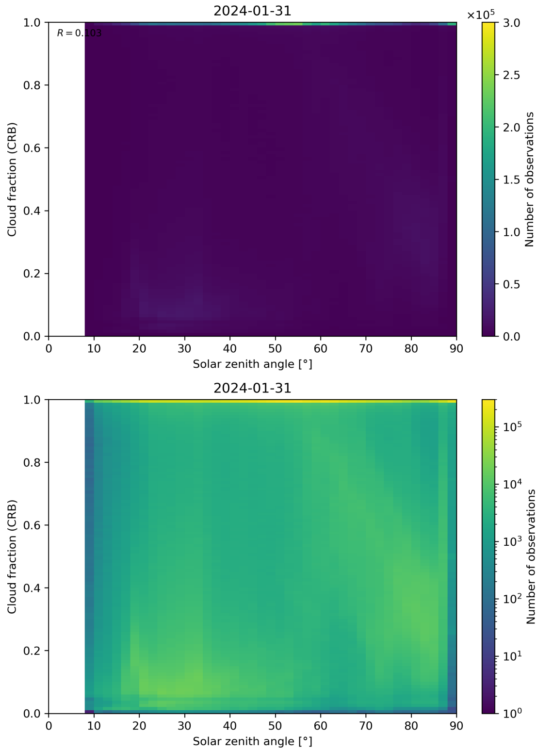
Figure 101: Scatter density plot of “Solar zenith angle” against “Cloud fraction (CRB)” for 2024-01-31 to 2024-02-01.
