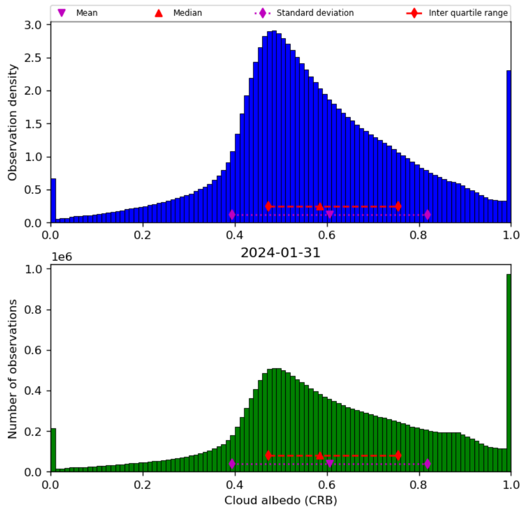
Figure 44: Histogram of “Cloud albedo (CRB)” for 2024-01-31 to 2024-02-01
