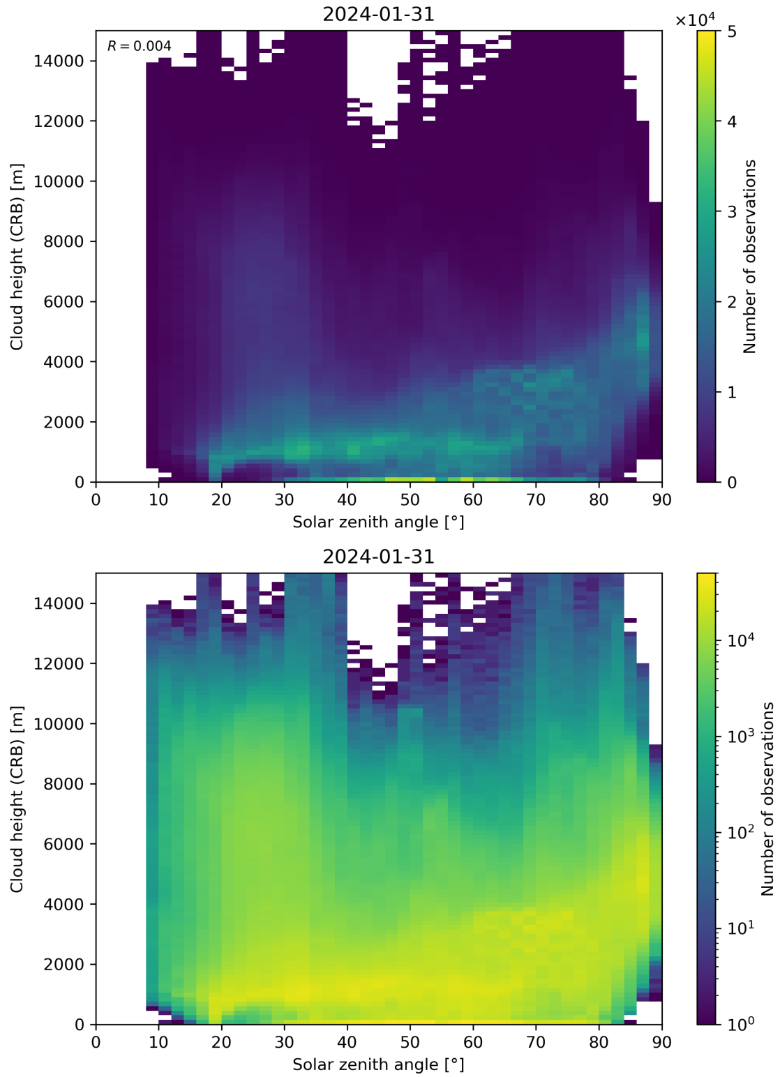
Figure 102: Scatter density plot of “Solar zenith angle” against “Cloud height (CRB)” for 2024-01-31 to 2024-02-01.
