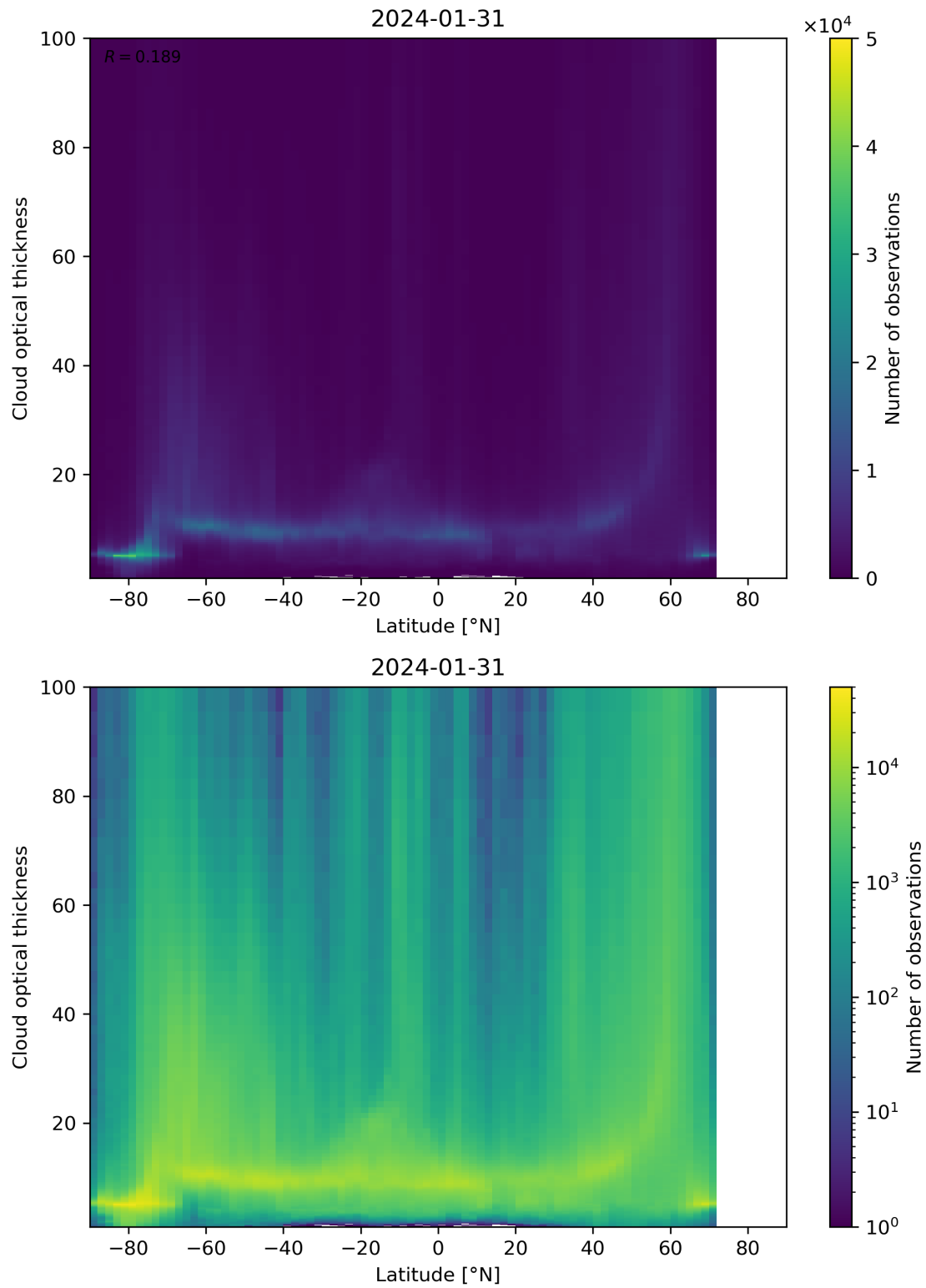
Figure 96: Scatter density plot of “Latitude” against “Cloud optical thickness” for 2024-01-31 to 2024-02-01.
