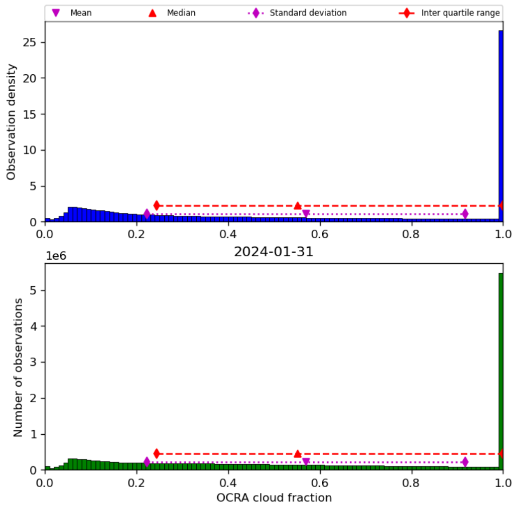
Figure 50: Histogram of “OCRA cloud fraction” for 2024-01-31 to 2024-02-01
