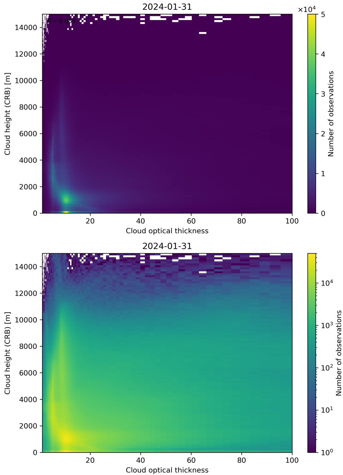
Figure 85: Scatter density plot of “Cloud optical thickness” against “Cloud height (CRB)” for 2024-01-31 to 2024-02-01.
