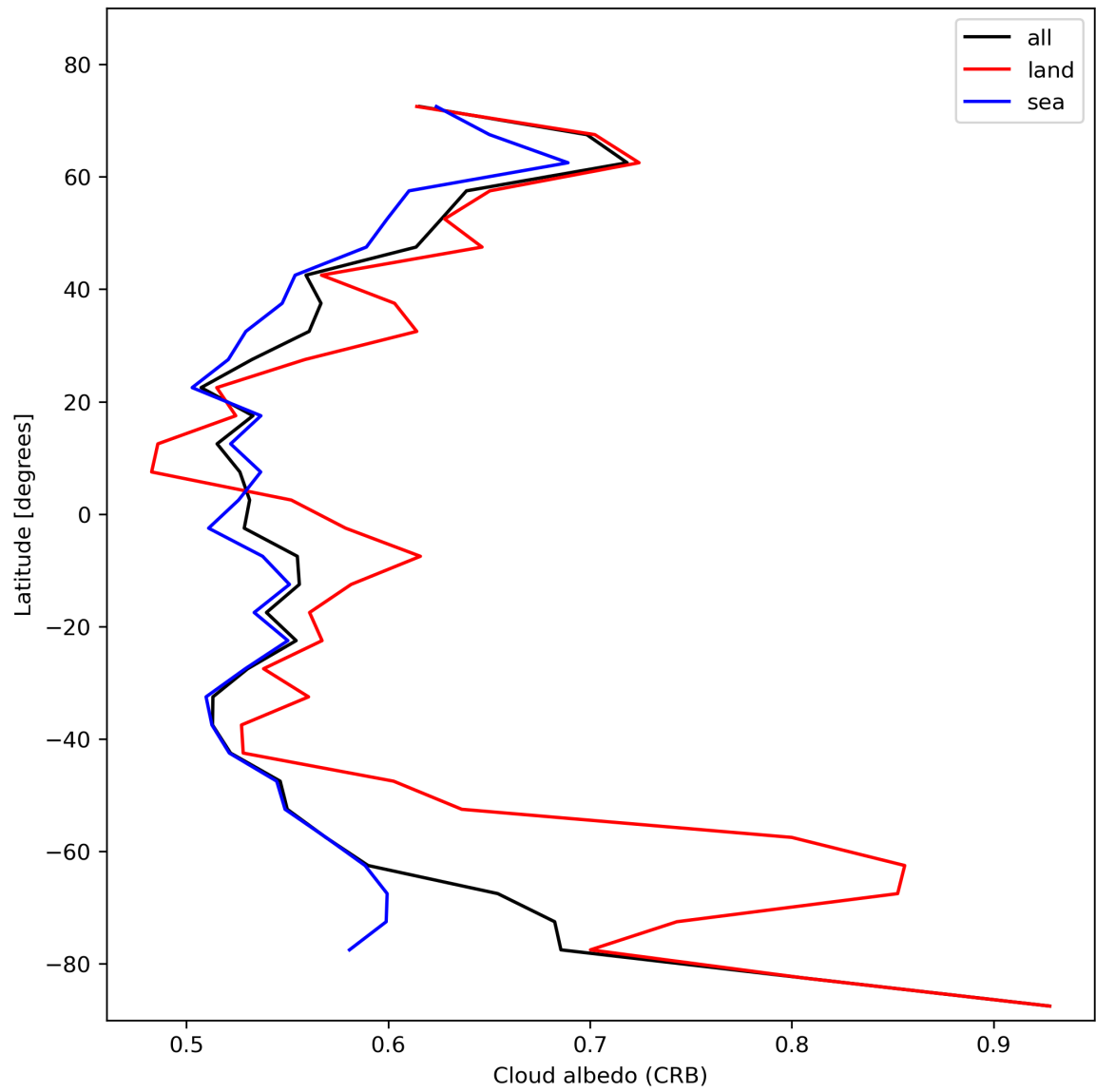
Figure 28: Zonal average of “Cloud albedo (CRB)” for 2024-01-31 to 2024-02-01.
