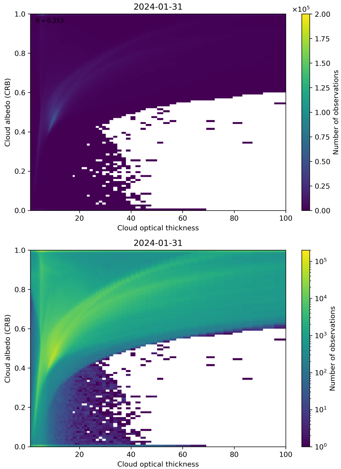
Figure 82: Scatter density plot of “Cloud optical thickness” against “Cloud albedo (CRB)” for 2024-01-31 to 2024-02-01.
