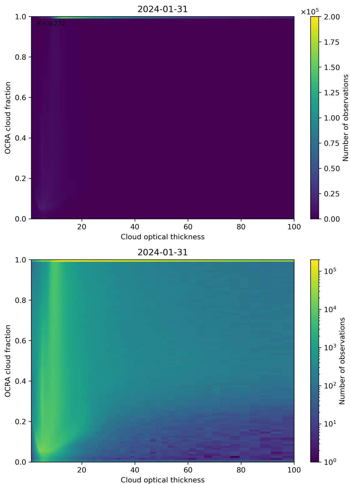
Figure 83: Scatter density plot of “Cloud optical thickness” against “OCRA cloud fraction” for 2024-01-31 to 2024-02-01.
