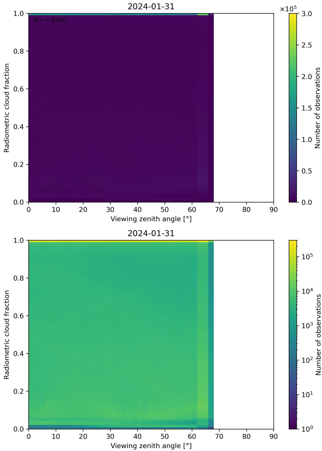
Figure 107: Scatter density plot of “Viewing zenith angle” against “Radiometric cloud fraction” for 2024-01-31 to 2024-02-01.
