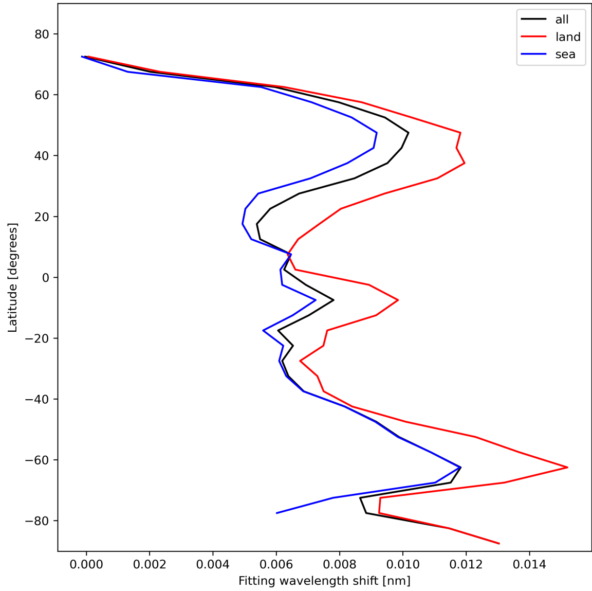
Figure 33: Zonal average of “Fitting wavelength shift” for 2024-01-31 to 2024-02-01.
