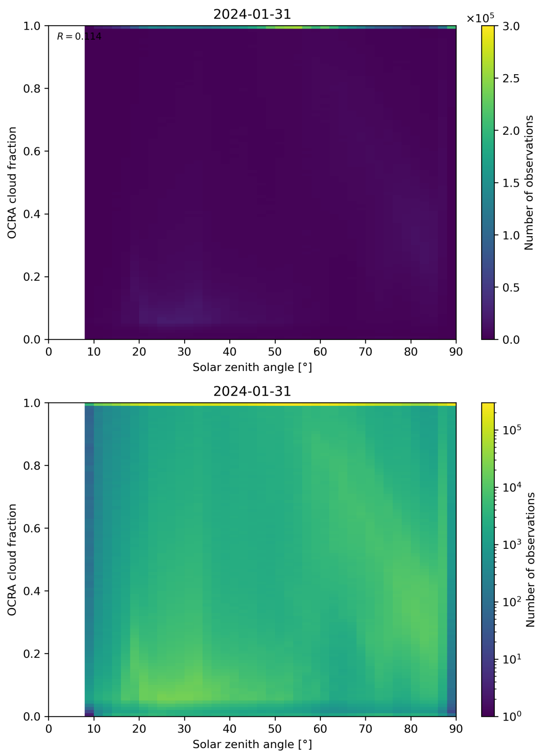
Figure 100: Scatter density plot of “Solar zenith angle” against “OCRA cloud fraction” for 2024-01-31 to 2024-02-01.
