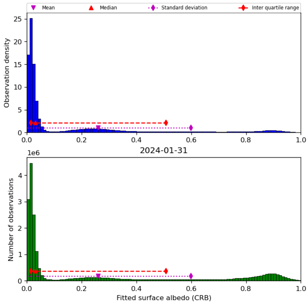
Figure 46: Histogram of “Fitted surface albedo (CRB)” for 2024-01-31 to 2024-02-01
