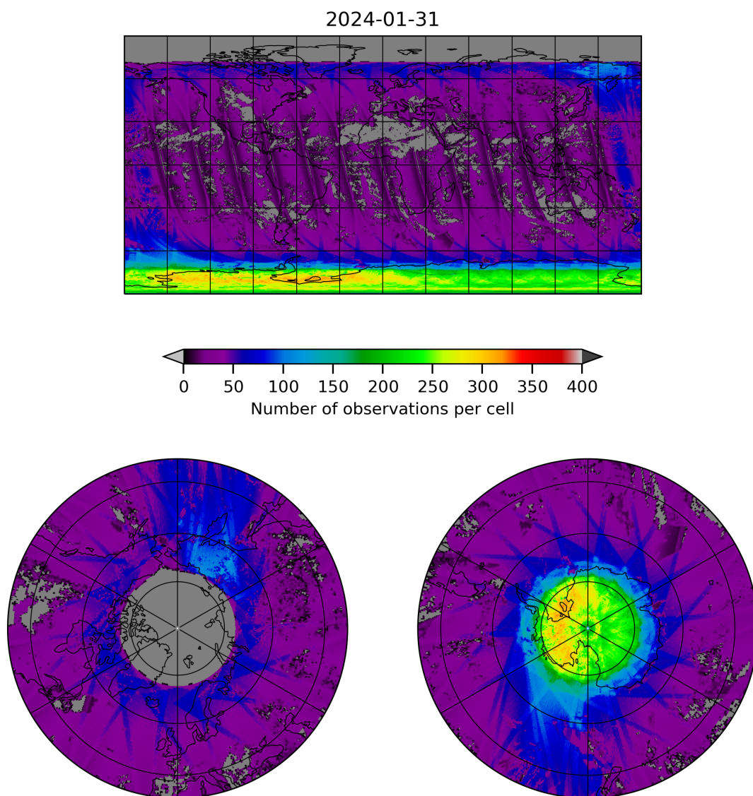
Figure 21: Map of the number of observations for 2024-01-31 to 2024-02-01
