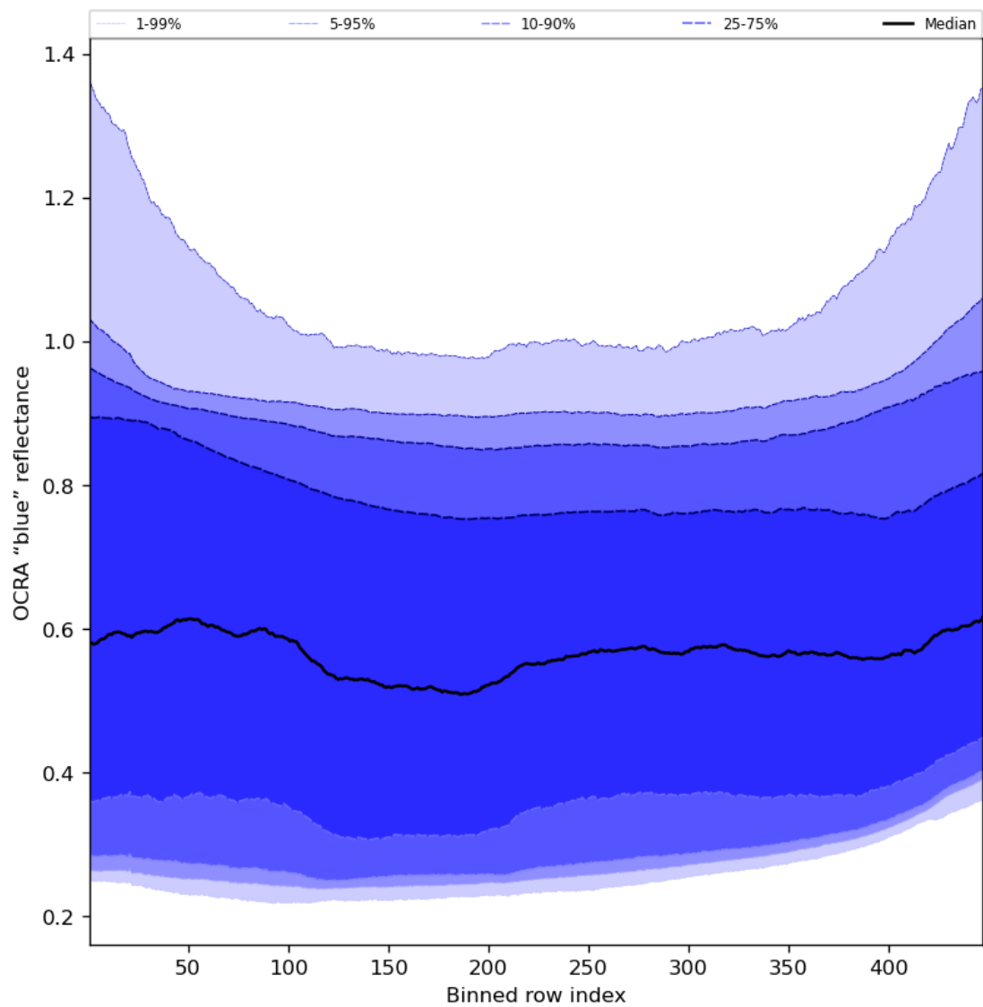
Figure 67: Along track statistics of “OCRA “blue” reflectance” for 2024-01-31 to 2024-02-01
