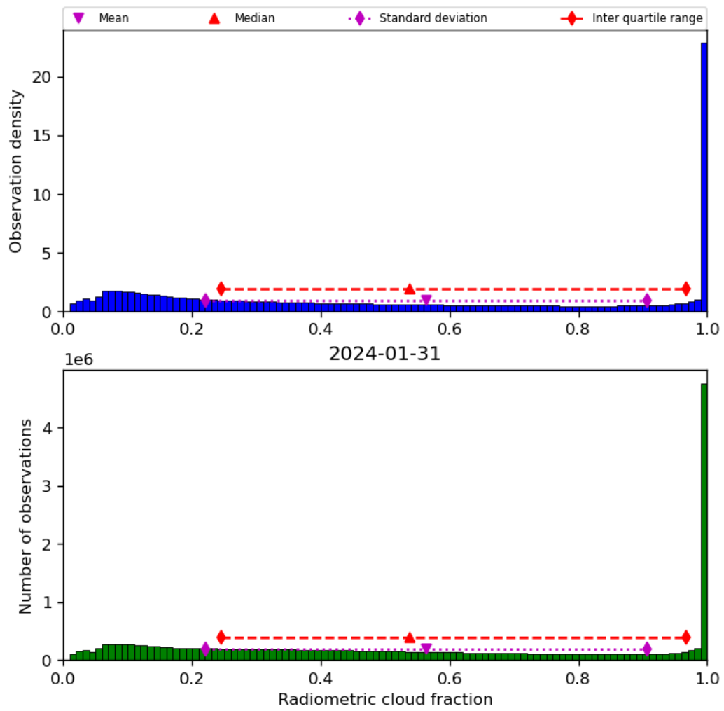
Figure 39: Histogram of “Radiometric cloud fraction” for 2024-01-31 to 2024-02-01
