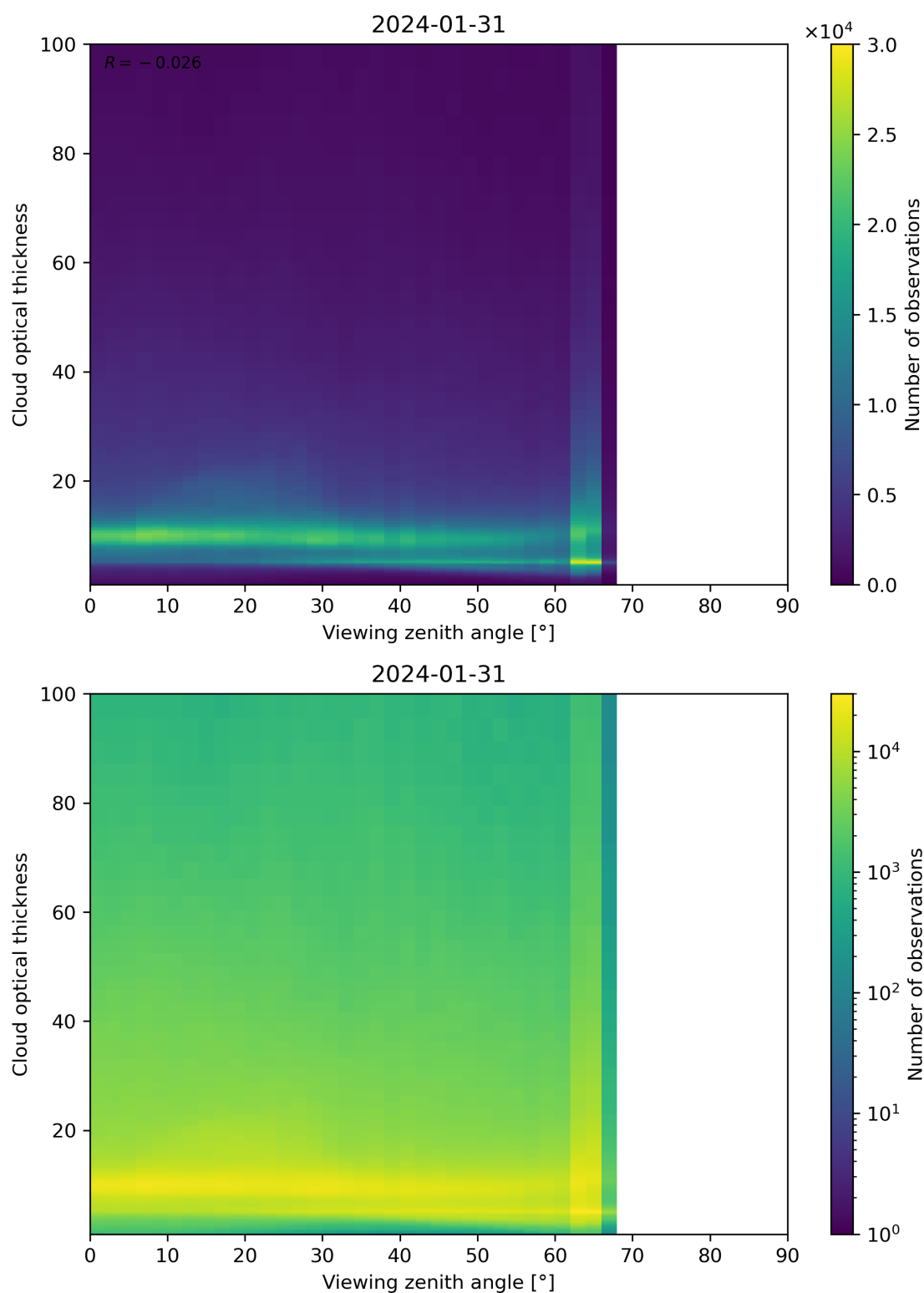
Figure 111: Scatter density plot of “Viewing zenith angle” against “Cloud optical thickness” for 2024-01-31 to 2024-02-01.
