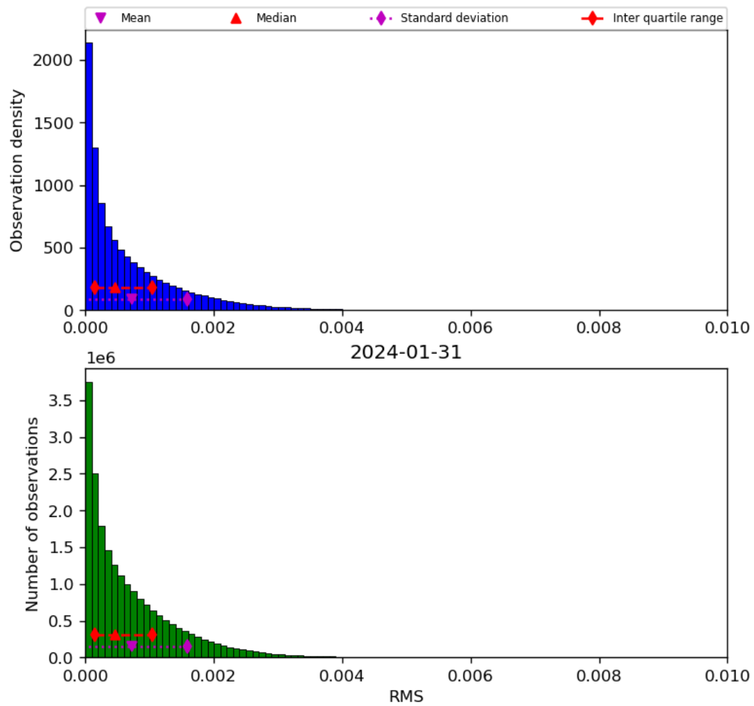
Figure 47: Histogram of “RMS” for 2024-01-31 to 2024-02-01
