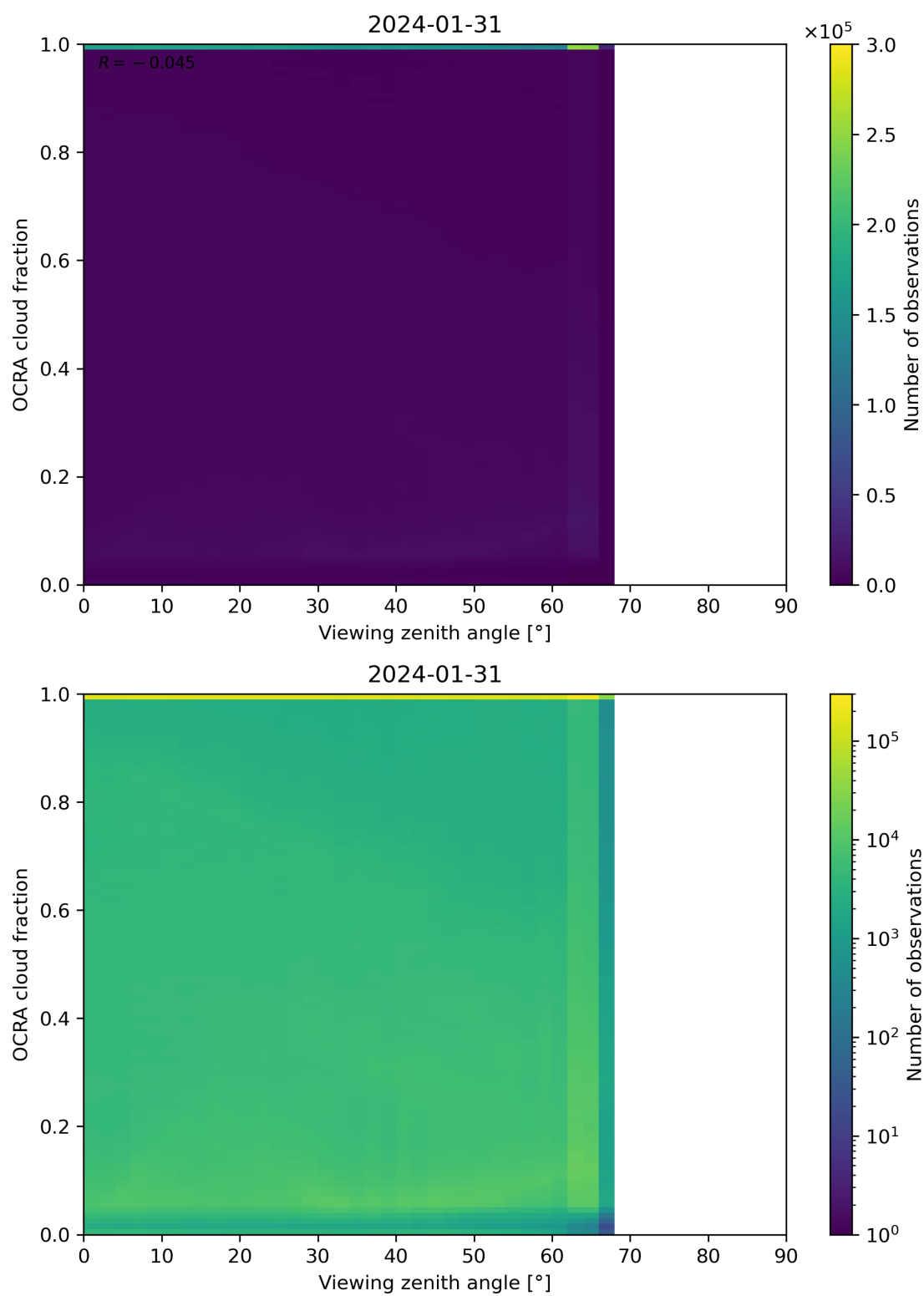
Figure 108: Scatter density plot of “Viewing zenith angle” against “OCRA cloud fraction” for 2024-01-31 to 2024-02-01.
