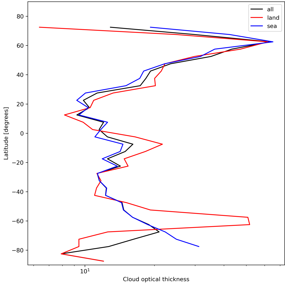
Figure 25: Zonal average of “Cloud optical thickness” for 2024-01-31 to 2024-02-01.
