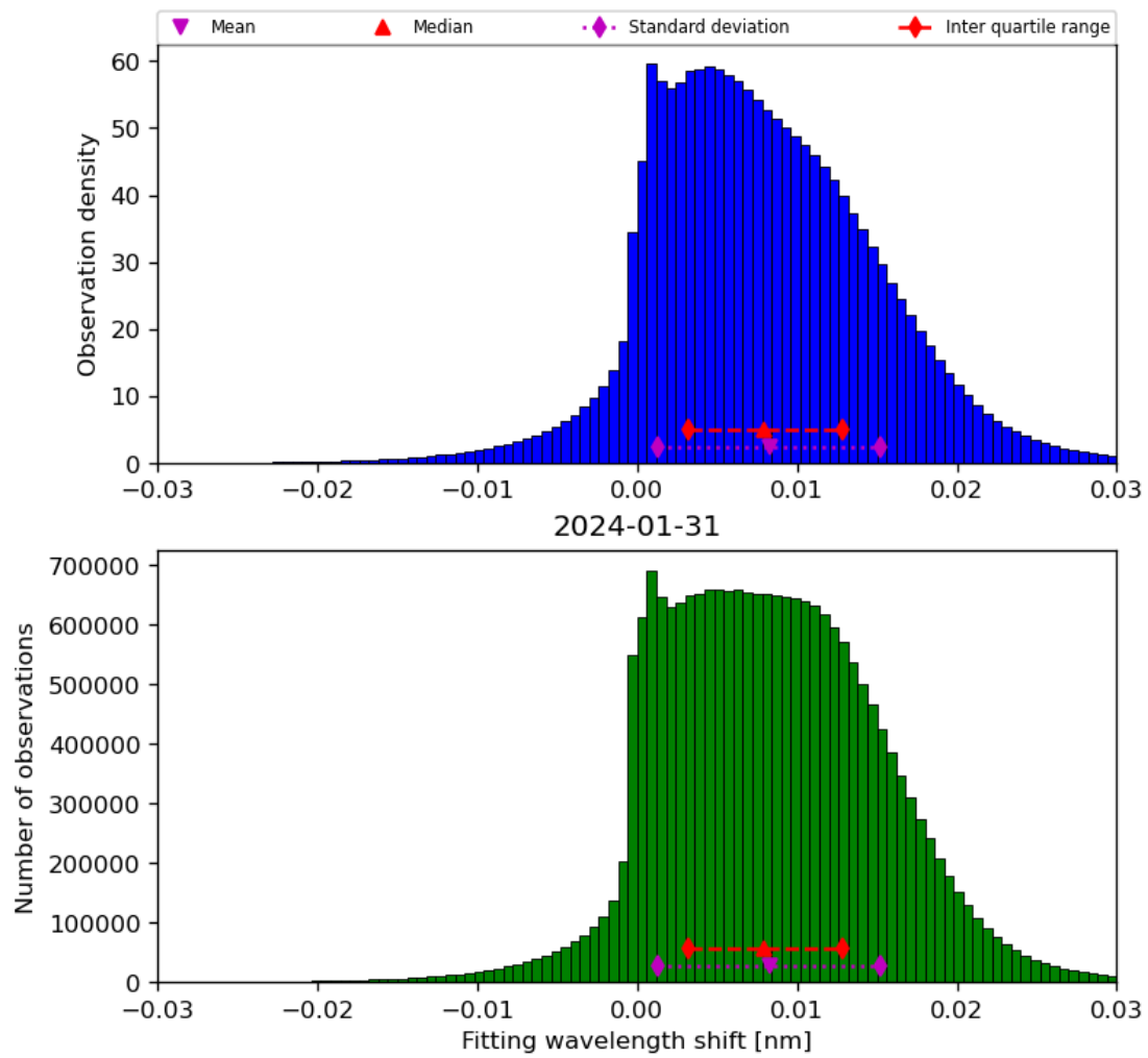
Figure 49: Histogram of “Fitting wavelength shift” for 2024-01-31 to 2024-02-01
