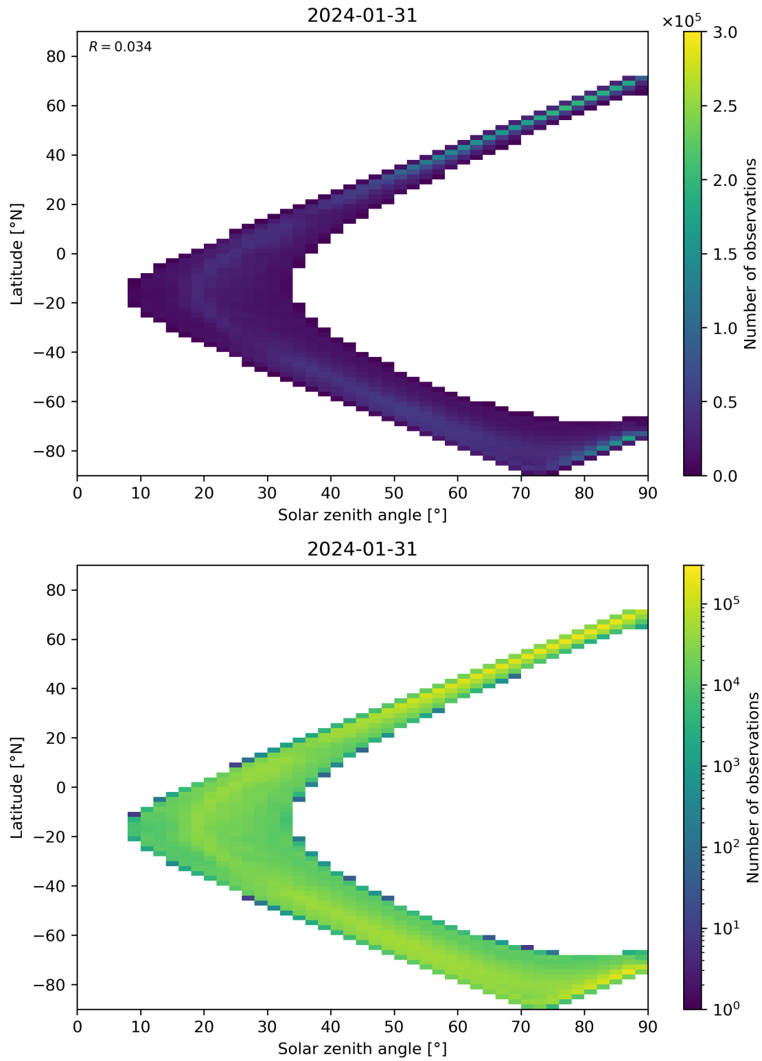
Figure 105: Scatter density plot of “Solar zenith angle” against “Latitude” for 2024-01-31 to 2024-02-01.
