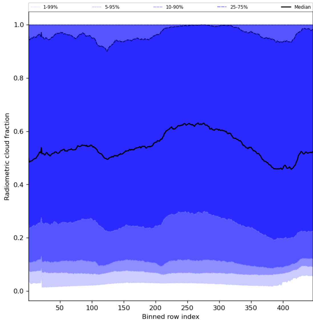
Figure 55: Along track statistics of “Radiometric cloud fraction” for 2024-01-31 to 2024-02-01
