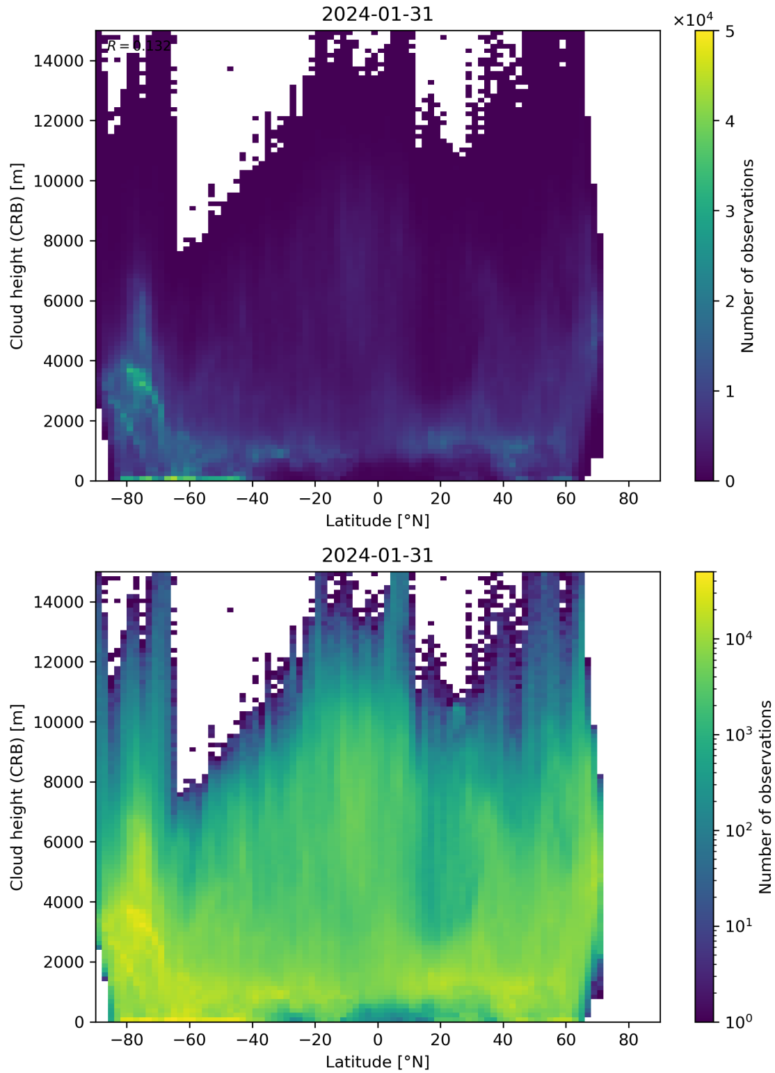
Figure 95: Scatter density plot of “Latitude” against “Cloud height (CRB)” for 2024-01-31 to 2024-02-01.
