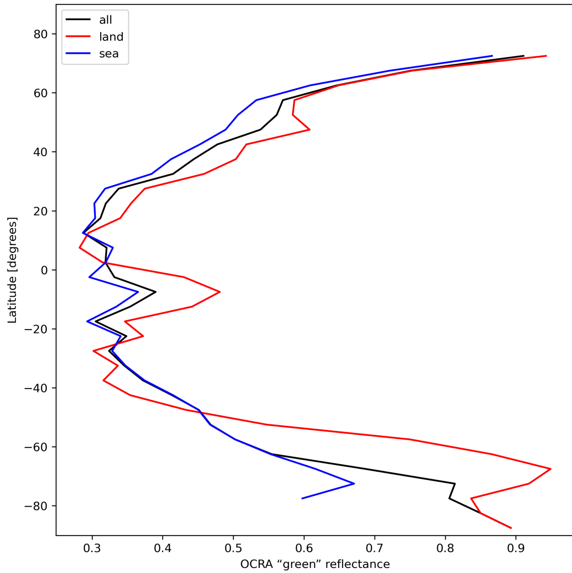
Figure 36: Zonal average of “OCRA “green” reflectance” for 2024-01-31 to 2024-02-01.
