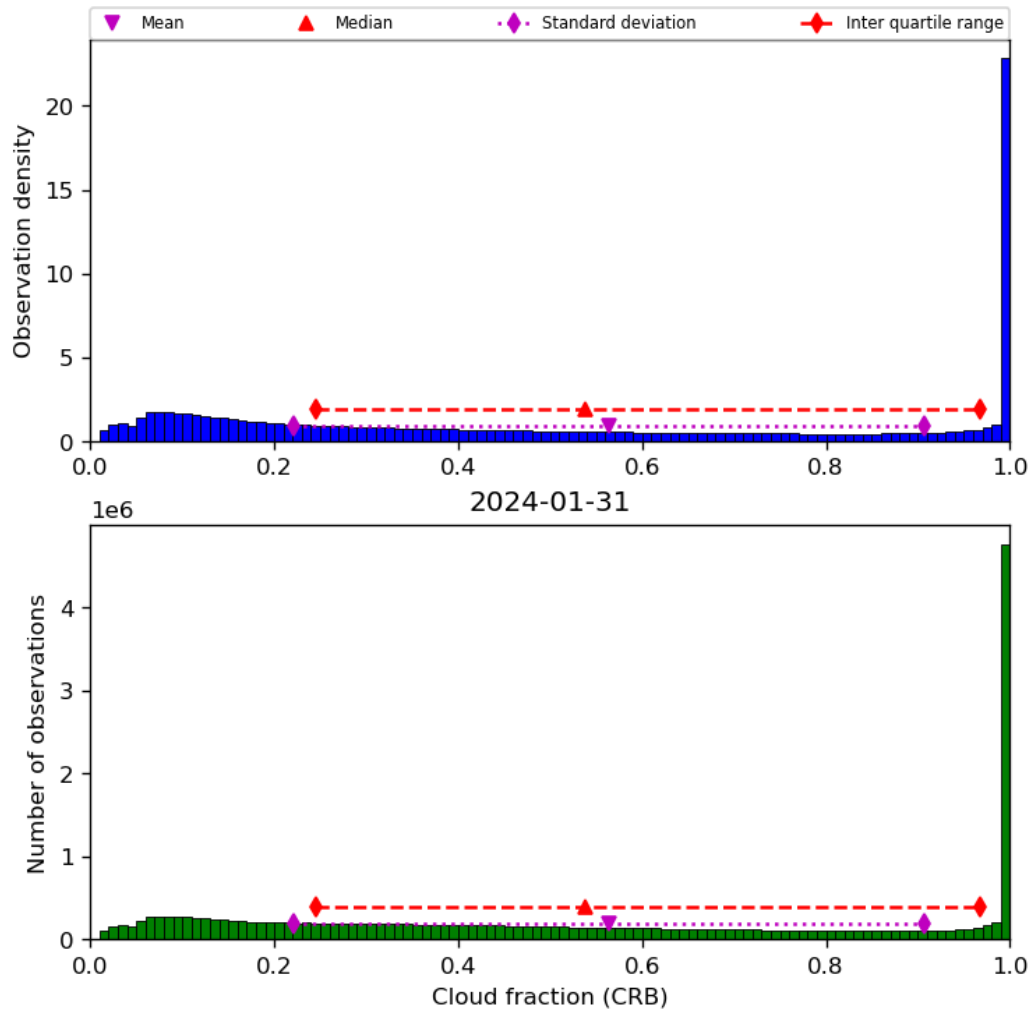
Figure 42: Histogram of “Cloud fraction (CRB)” for 2024-01-31 to 2024-02-01
