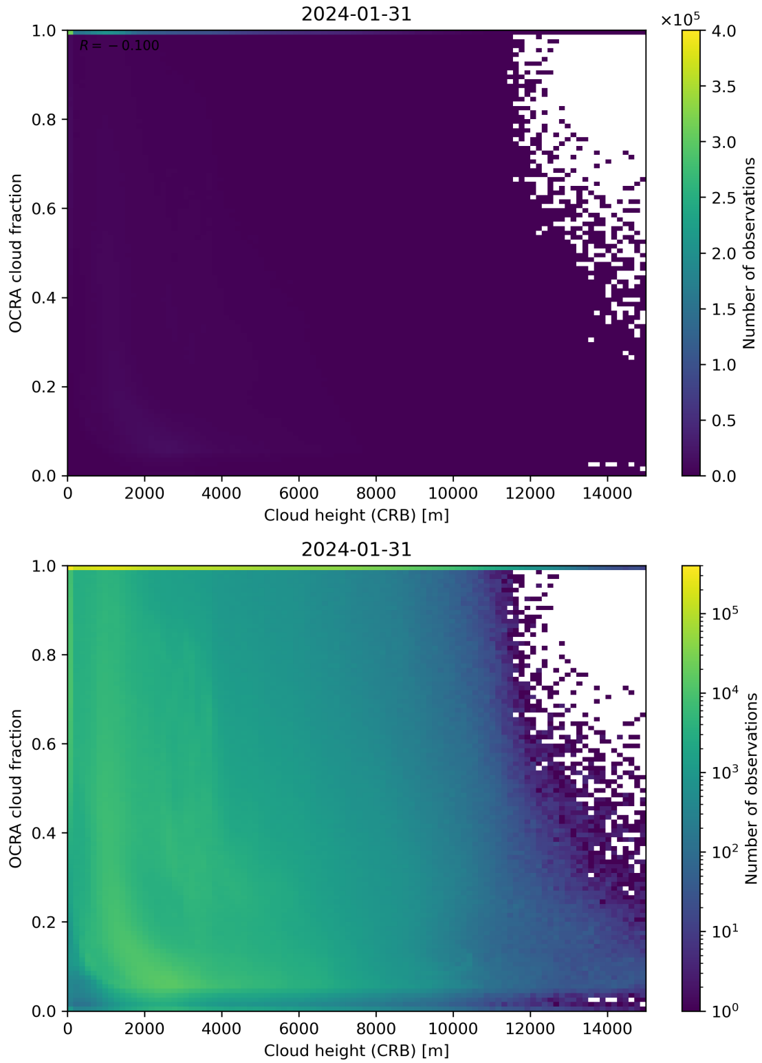
Figure 81: Scatter density plot of “Cloud height (CRB)” against “OCRA cloud fraction” for 2024-01-31 to 2024-02-01.
