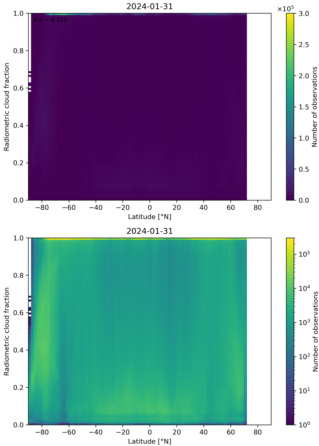
Figure 92: Scatter density plot of “Latitude” against “Radiometric cloud fraction” for 2024-01-31 to 2024-02-01.
