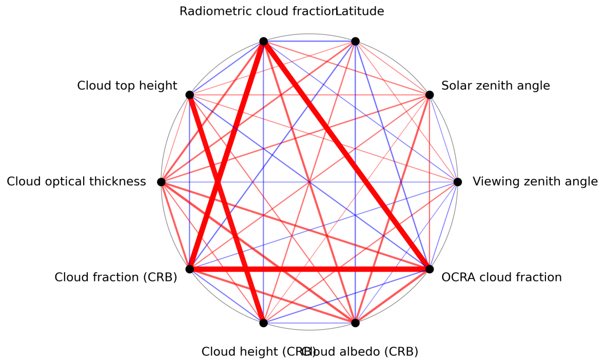
Figure 1: Map of correlation graph for 2024-01-31 to 2024-02-01.
