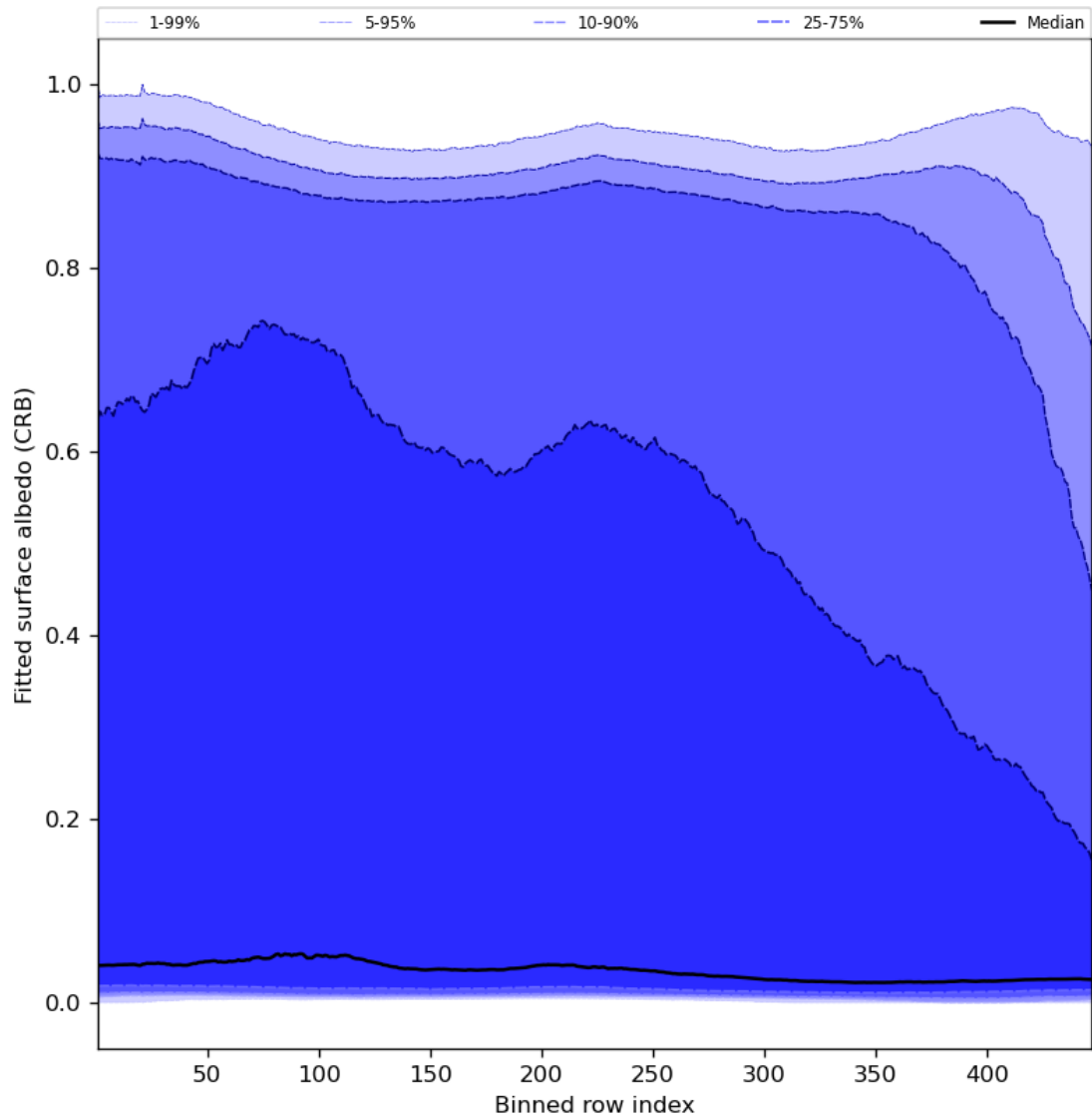
Figure 62: Along track statistics of “Fitted surface albedo (CRB)” for 2024-01-31 to 2024-02-02
