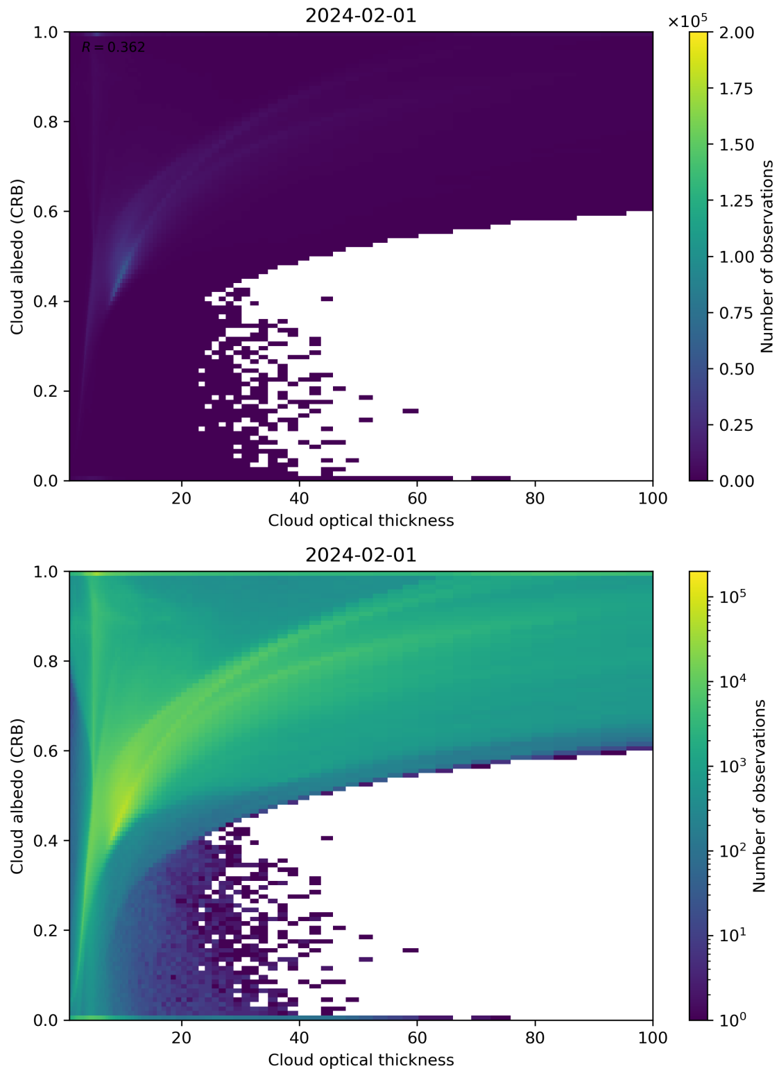
Figure 82: Scatter density plot of “Cloud optical thickness” against “Cloud albedo (CRB)” for 2024-01-31 to 2024-02-02.
