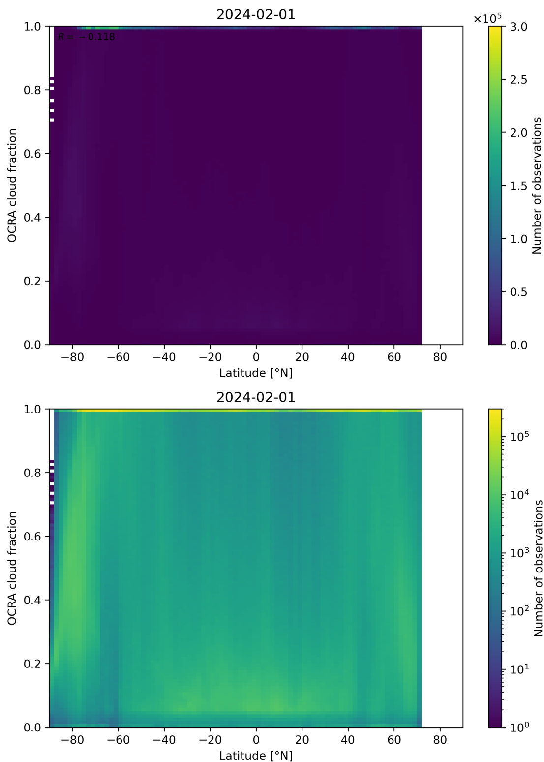
Figure 93: Scatter density plot of “Latitude” against “OCRA cloud fraction” for 2024-01-31 to 2024-02-02.
