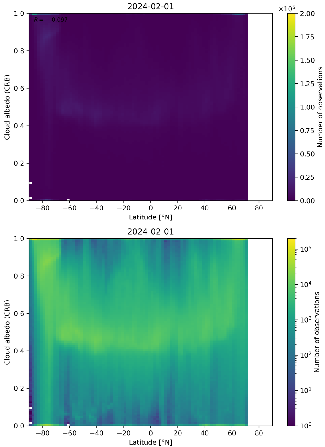
Figure 91: Scatter density plot of “Latitude” against “Cloud albedo (CRB)” for 2024-01-31 to 2024-02-02.
