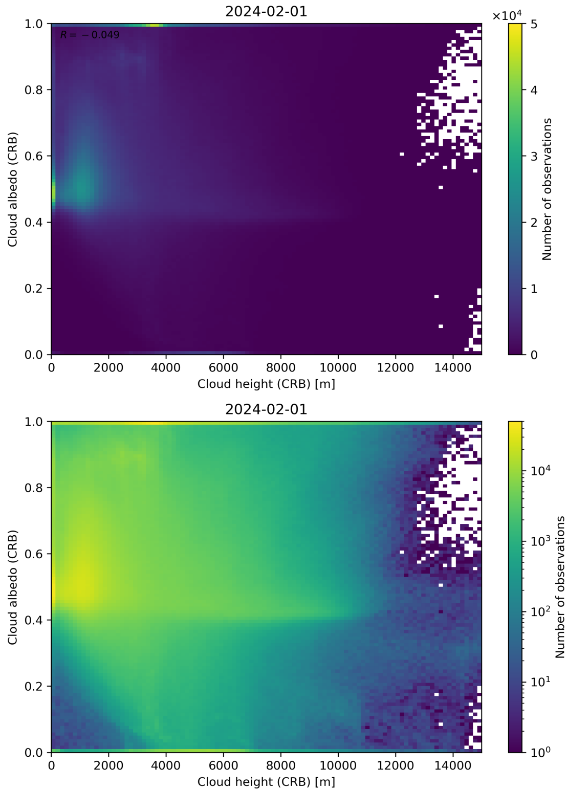
Figure 80: Scatter density plot of “Cloud height (CRB)” against “Cloud albedo (CRB)” for 2024-01-31 to 2024-02-02.
