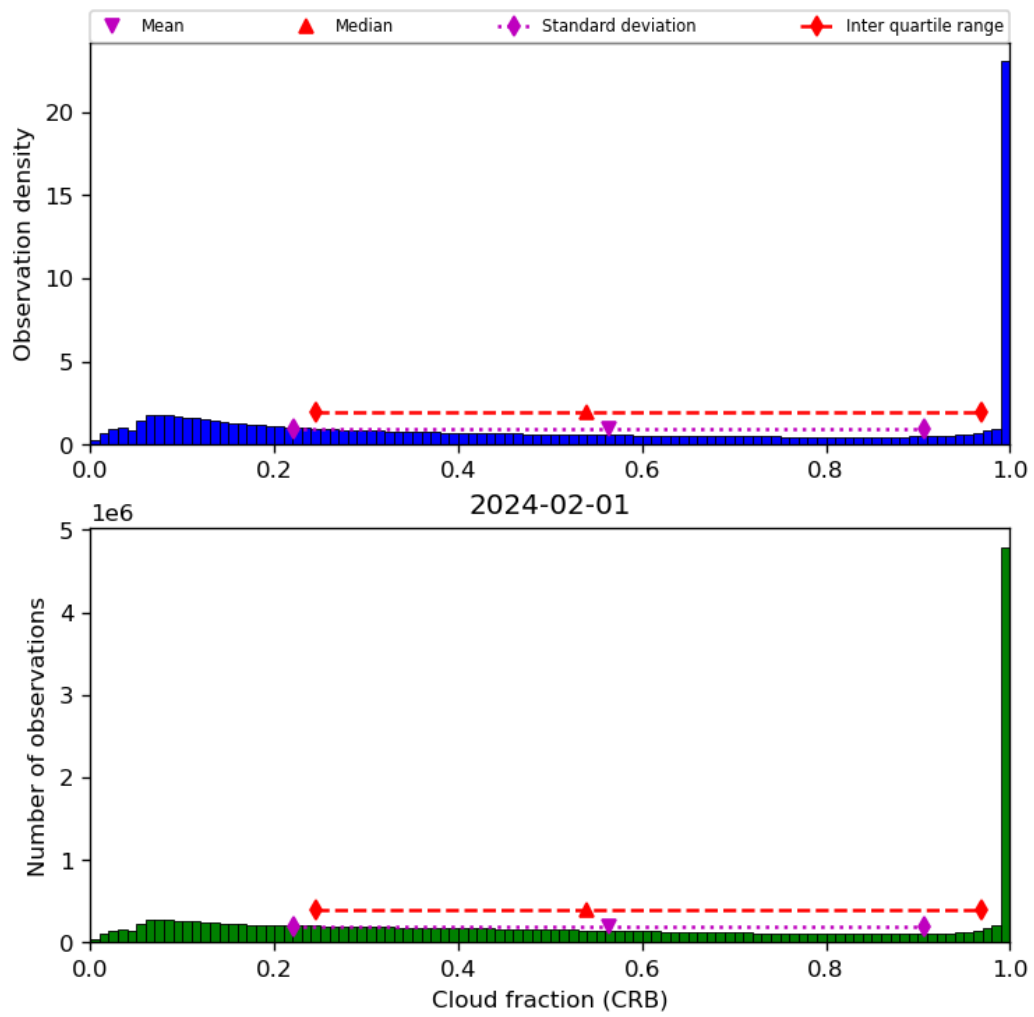
Figure 42: Histogram of “Cloud fraction (CRB)” for 2024-01-31 to 2024-02-02
