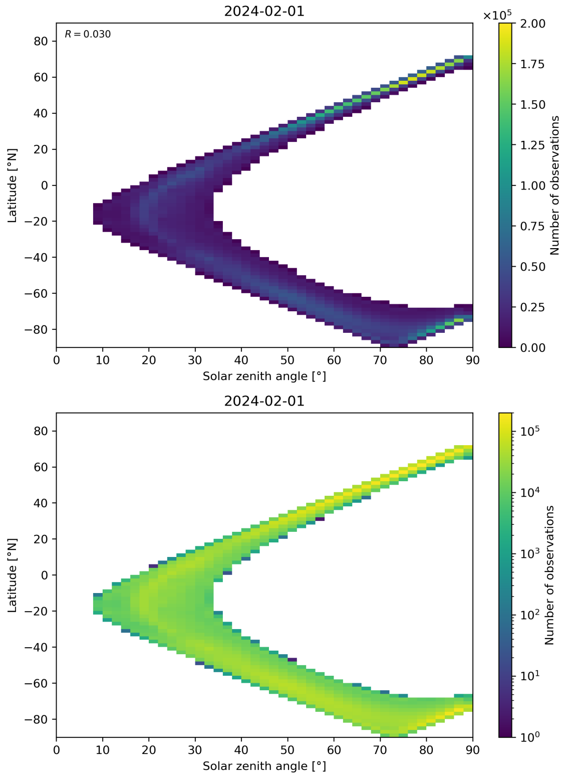
Figure 105: Scatter density plot of “Solar zenith angle” against “Latitude” for 2024-01-31 to 2024-02-02.
