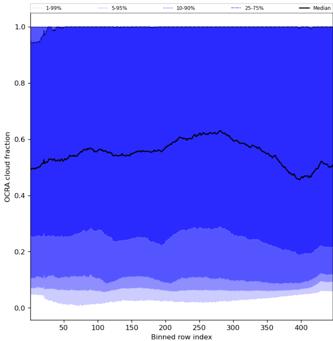
Figure 66: Along track statistics of “OCRA cloud fraction” for 2024-01-31 to 2024-02-02
