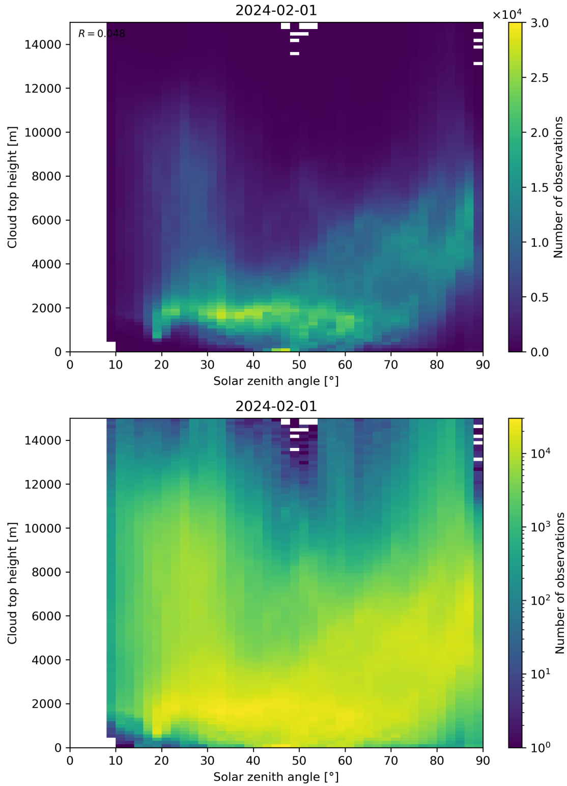
Figure 104: Scatter density plot of “Solar zenith angle” against “Cloud top height” for 2024-01-31 to 2024-02-02.
