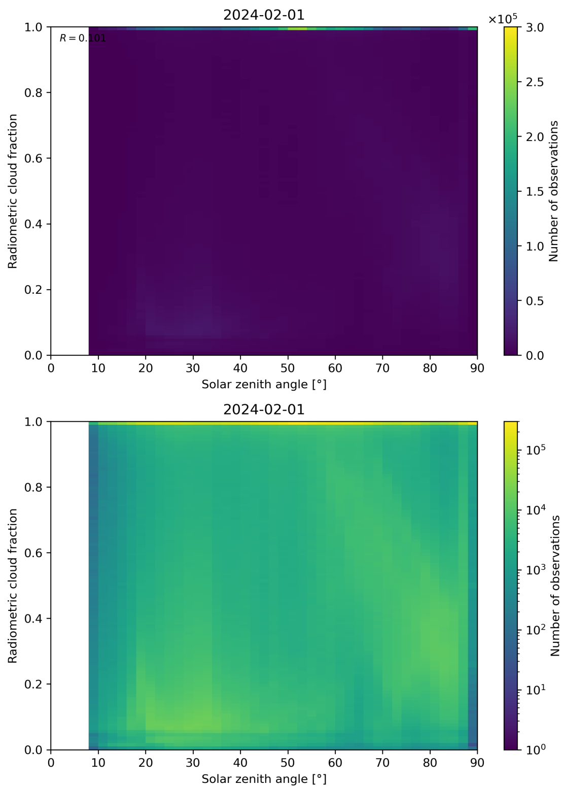
Figure 99: Scatter density plot of “Solar zenith angle” against “Radiometric cloud fraction” for 2024-01-31 to 2024-02-02.
