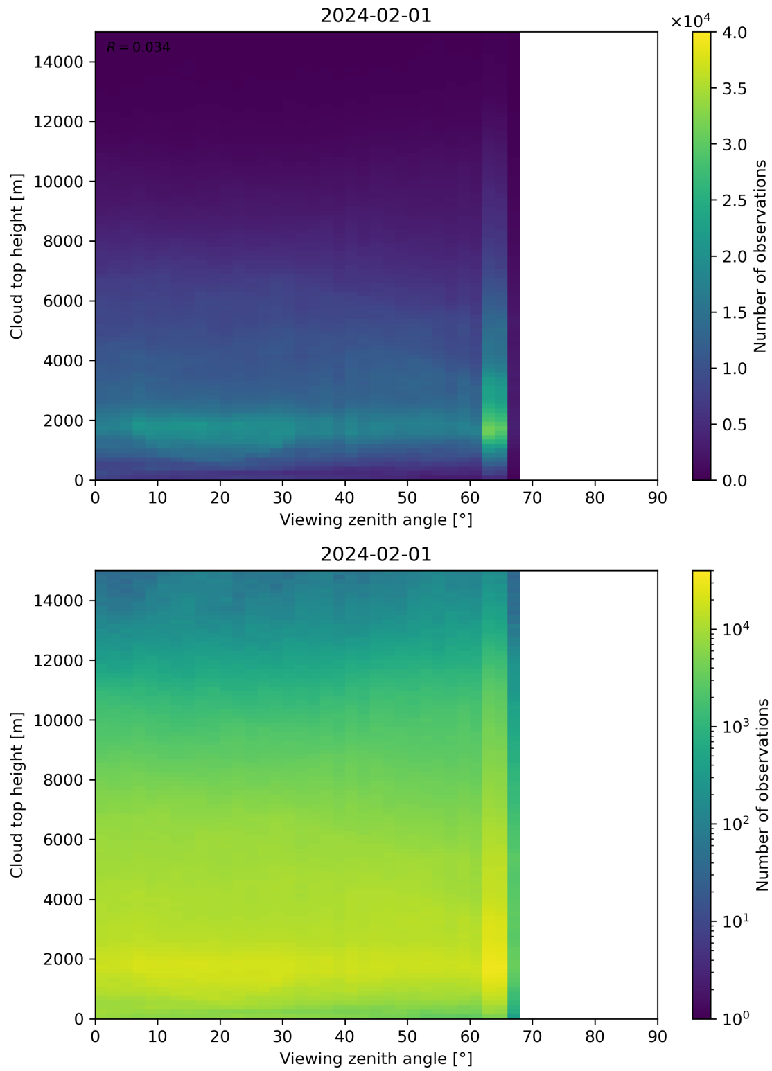
Figure 112: Scatter density plot of “Viewing zenith angle” against “Cloud top height” for 2024-01-31 to 2024-02-02.
