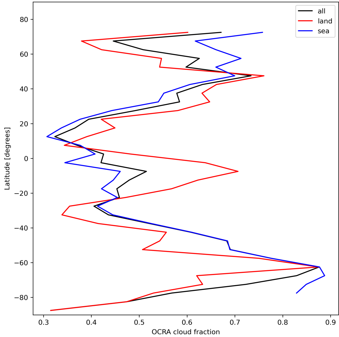
Figure 34: Zonal average of “OCRA cloud fraction” for 2024-01-31 to 2024-02-02.
