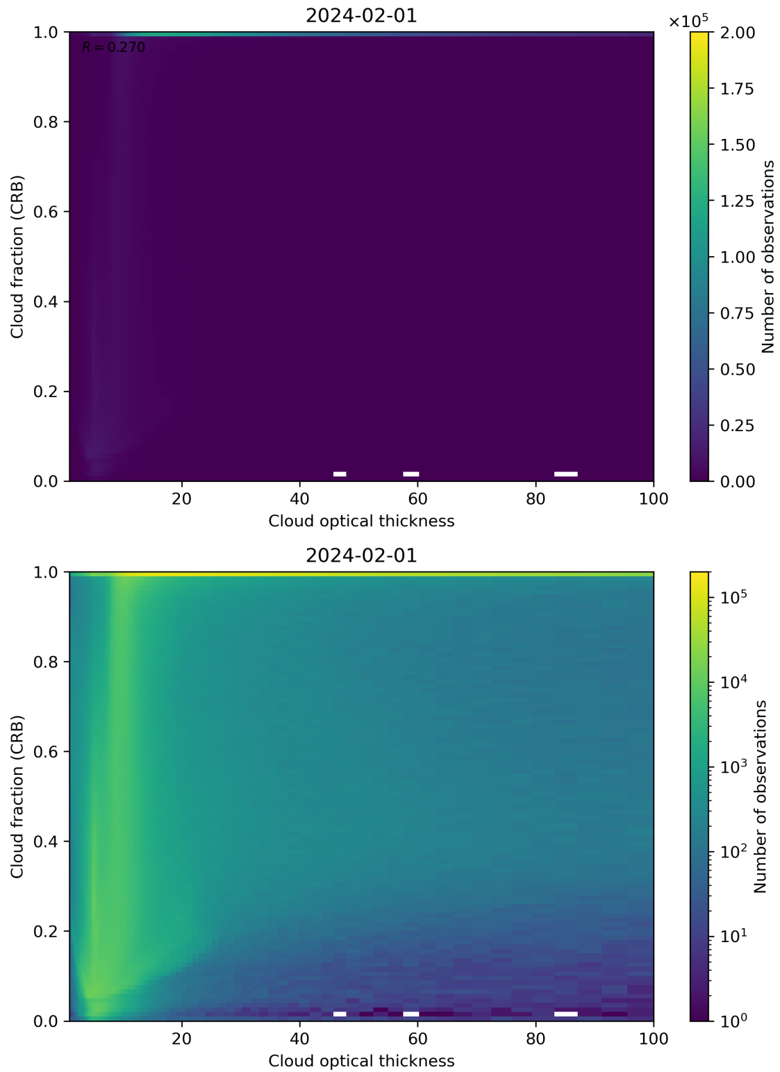
Figure 84: Scatter density plot of “Cloud optical thickness” against “Cloud fraction (CRB)” for 2024-01-31 to 2024-02-02.
