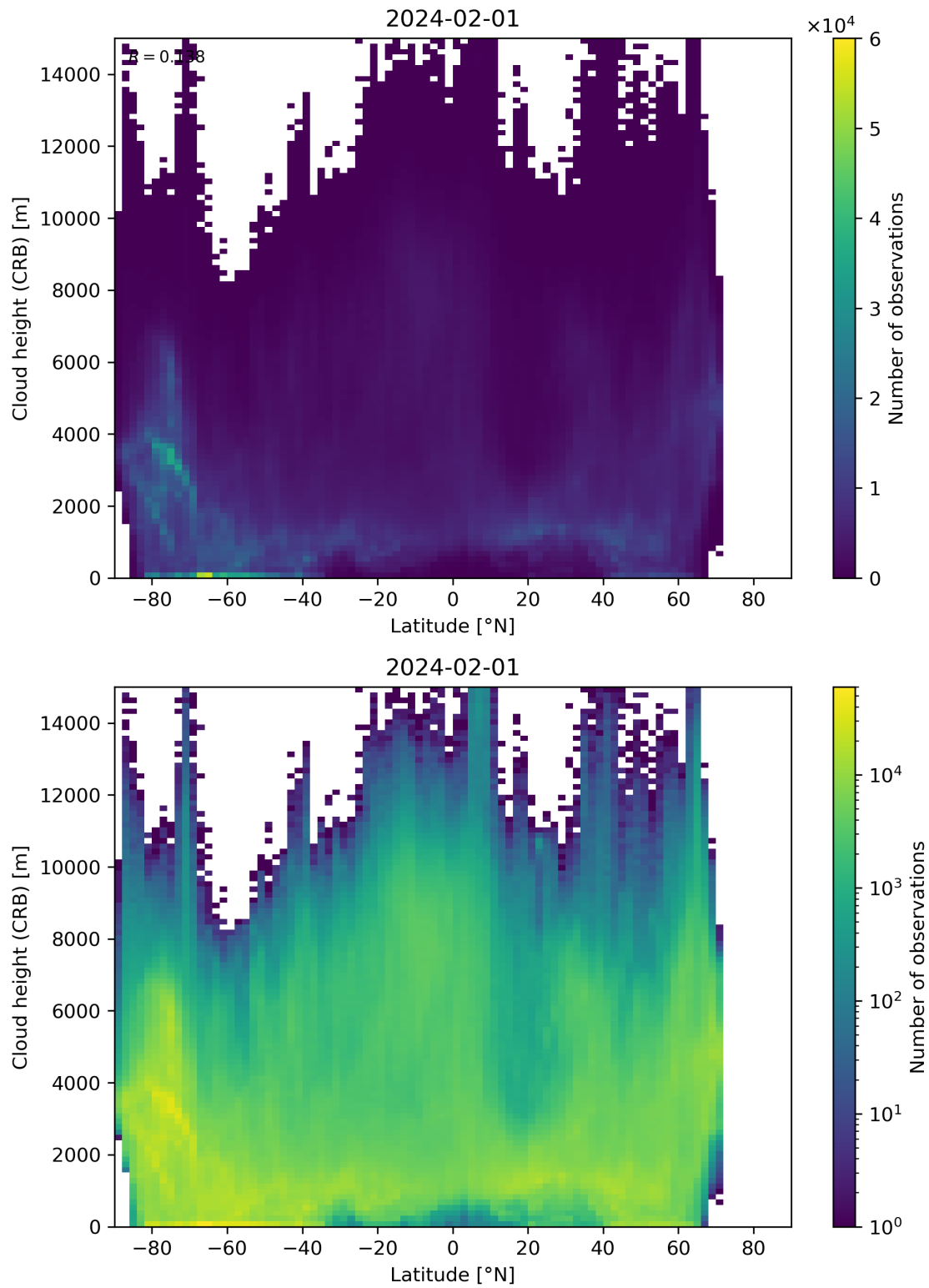
Figure 95: Scatter density plot of “Latitude” against “Cloud height (CRB)” for 2024-01-31 to 2024-02-02.
