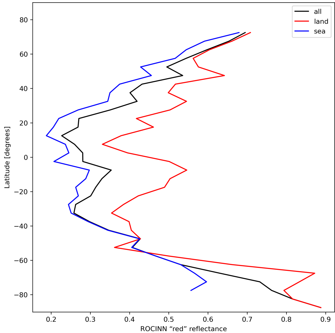
Figure 37: Zonal average of “ROCINN “red” reflectance” for 2024-01-31 to 2024-02-02.
