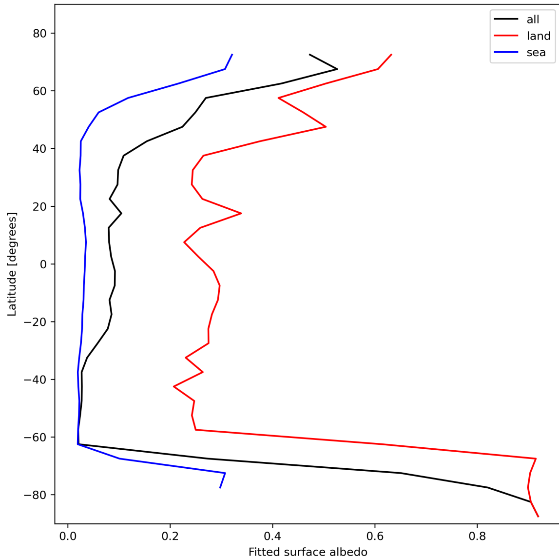
Figure 29: Zonal average of “Fitted surface albedo” for 2024-01-31 to 2024-02-02.
