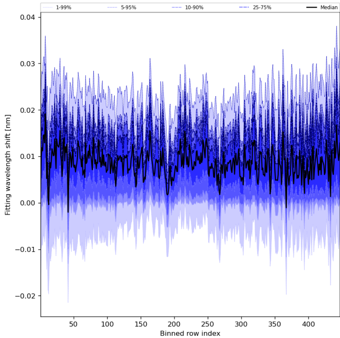
Figure 65: Along track statistics of “Fitting wavelength shift” for 2024-01-31 to 2024-02-02
