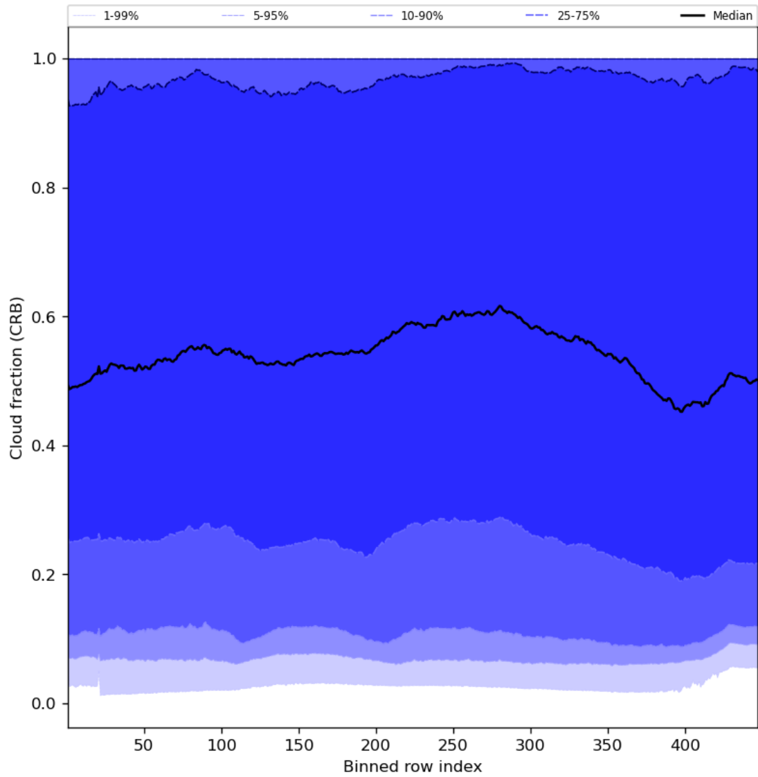
Figure 58: Along track statistics of “Cloud fraction (CRB)” for 2024-01-31 to 2024-02-02
