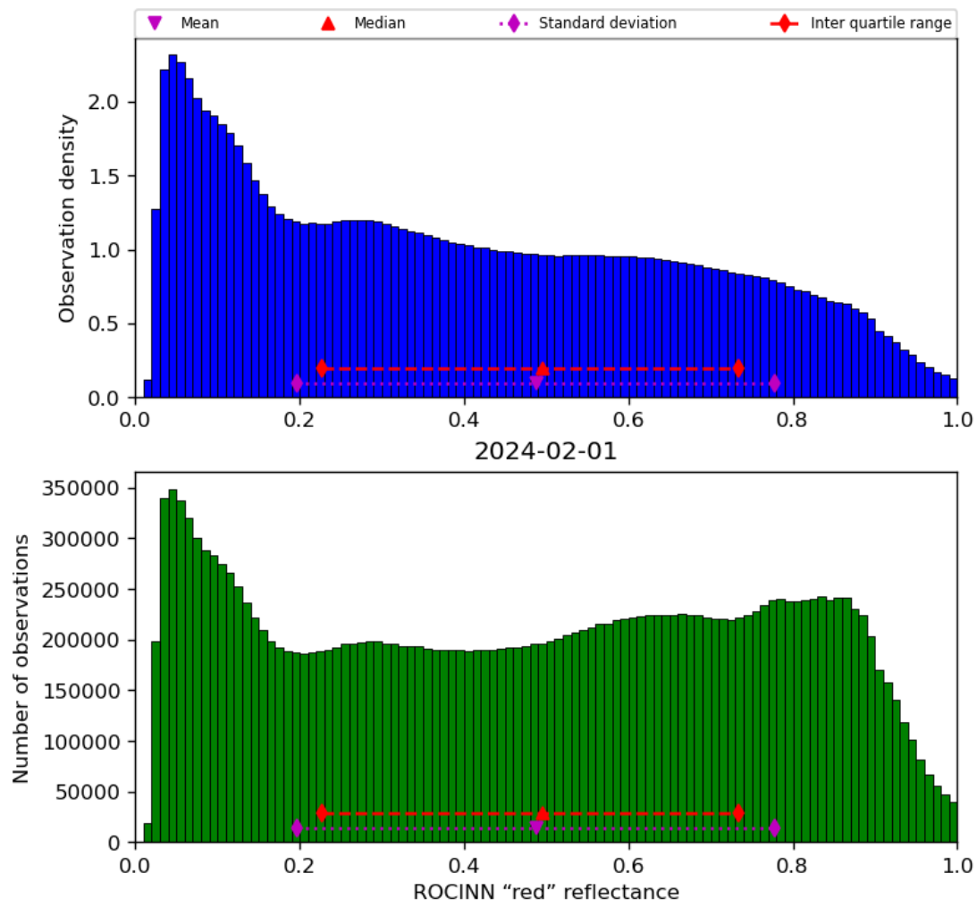
Figure 53: Histogram of “ROCINN “red” reflectance” for 2024-01-31 to 2024-02-02
