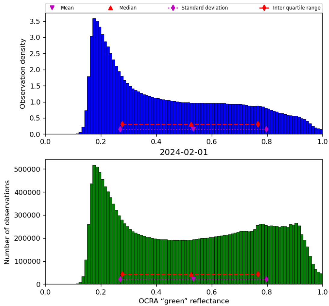
Figure 52: Histogram of “OCRA “green” reflectance” for 2024-01-31 to 2024-02-02
