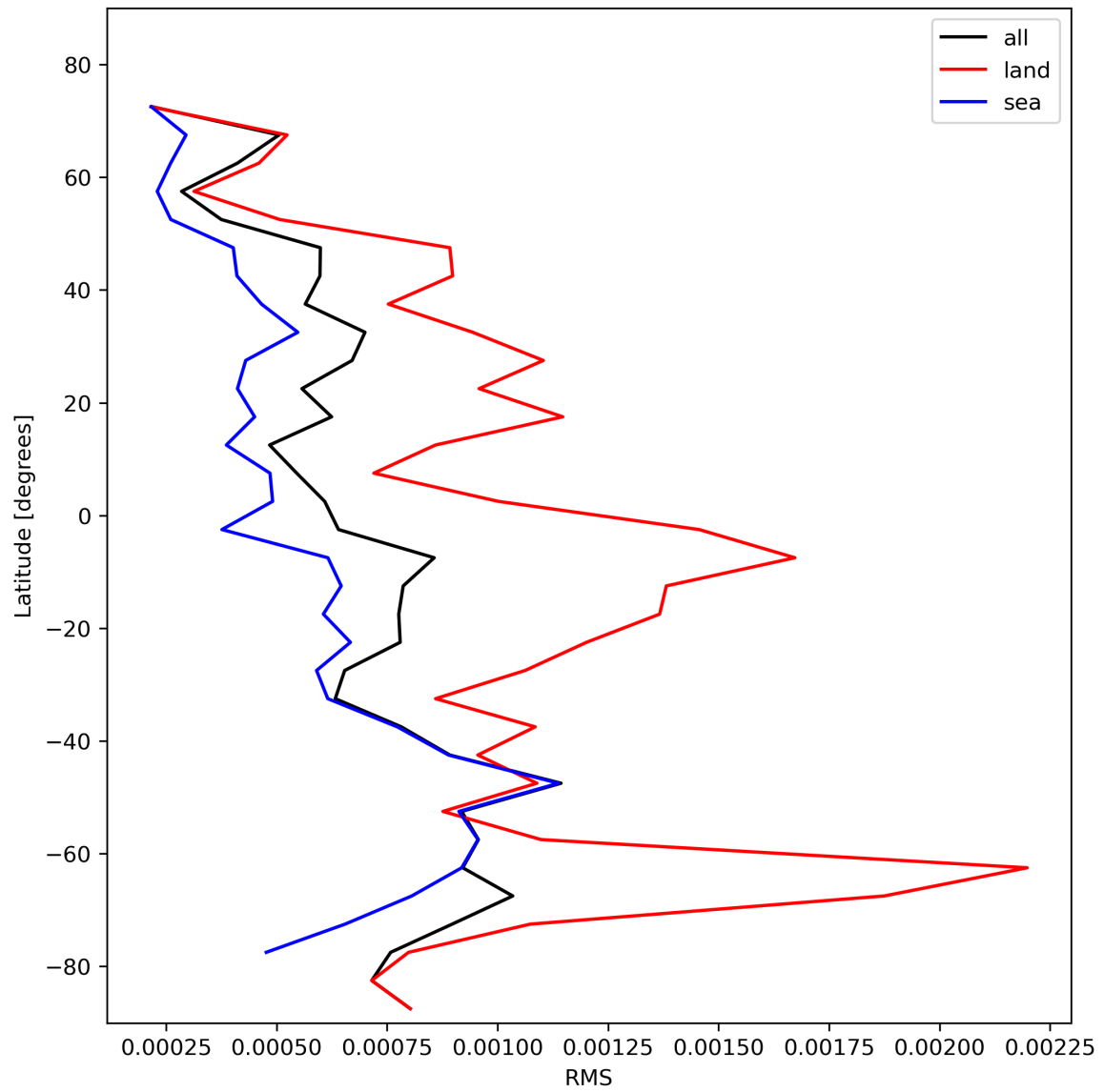
Figure 31: Zonal average of “RMS” for 2024-01-31 to 2024-02-02.
