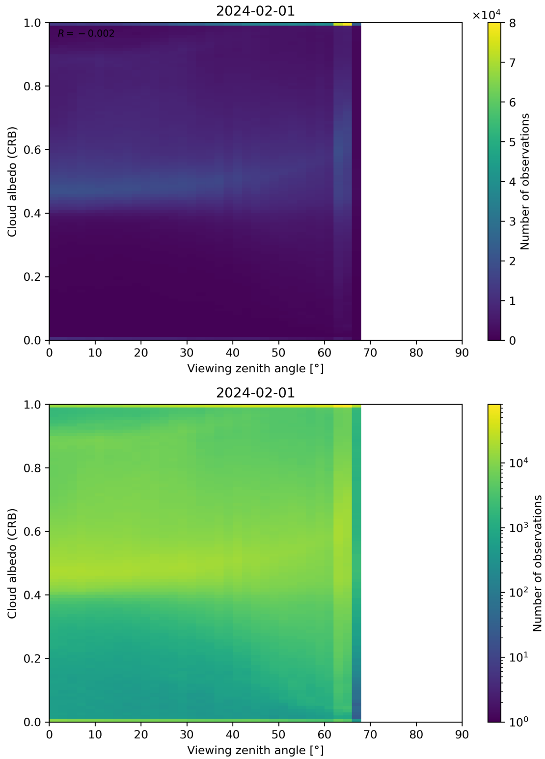
Figure 106: Scatter density plot of “Viewing zenith angle” against “Cloud albedo (CRB)” for 2024-01-31 to 2024-02-02.
