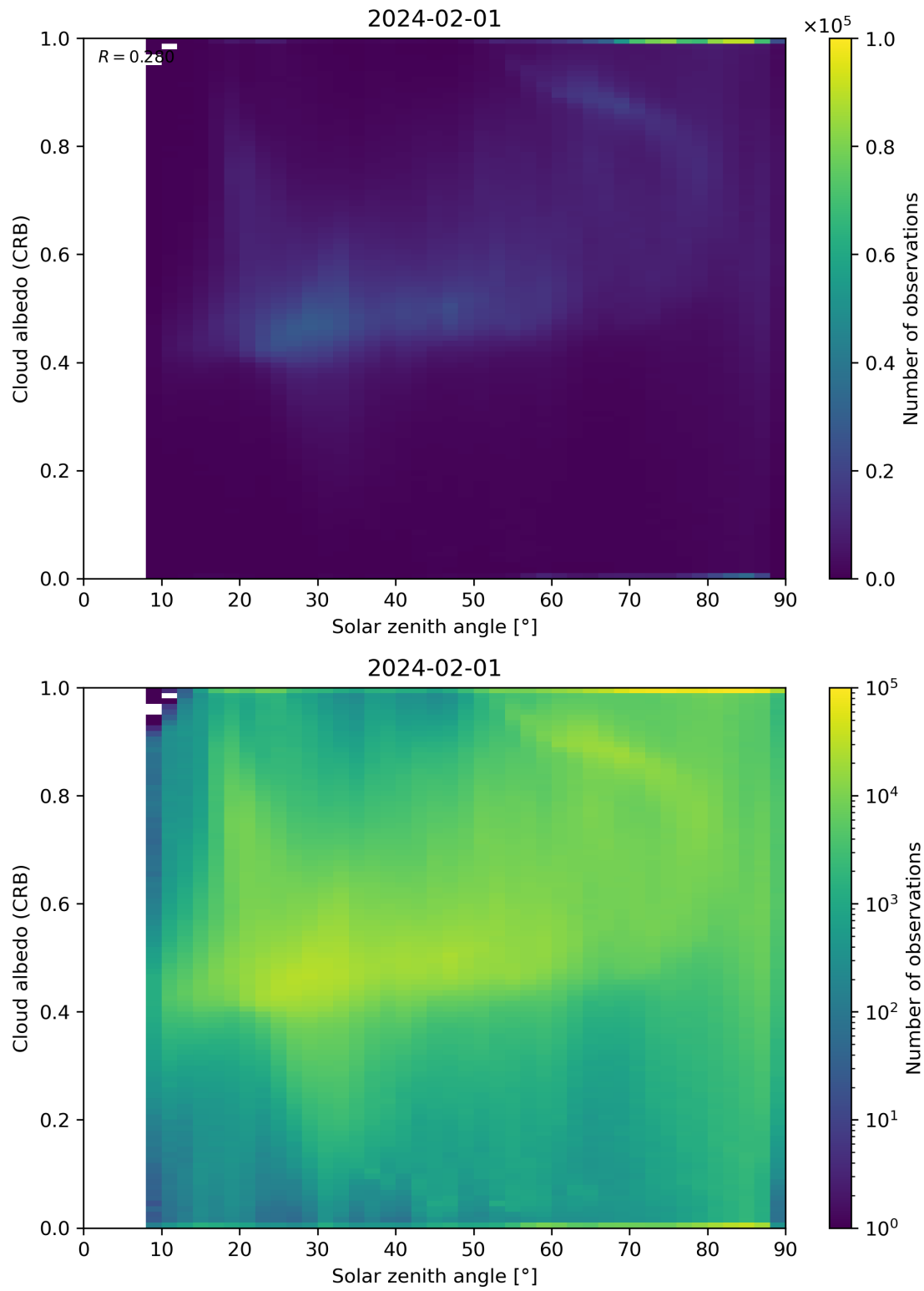
Figure 98: Scatter density plot of “Solar zenith angle” against “Cloud albedo (CRB)” for 2024-01-31 to 2024-02-02.
