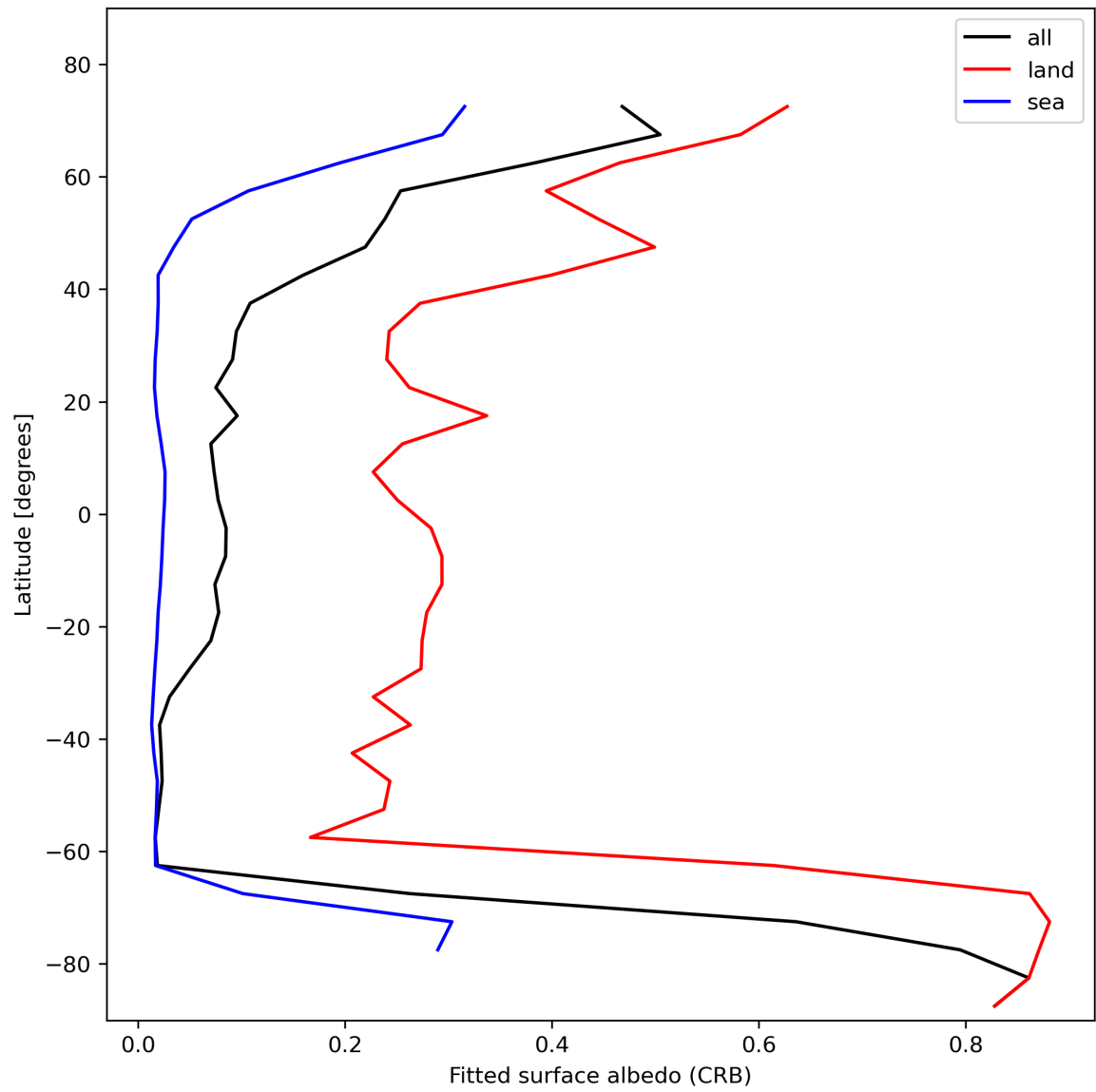
Figure 30: Zonal average of “Fitted surface albedo (CRB)” for 2024-01-31 to 2024-02-02.
