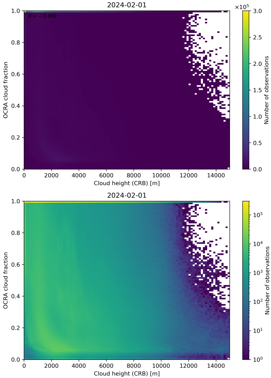
Figure 81: Scatter density plot of “Cloud height (CRB)” against “OCRA cloud fraction” for 2024-01-31 to 2024-02-02.
