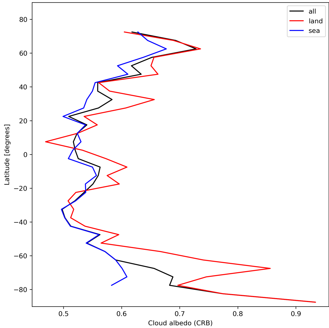
Figure 28: Zonal average of “Cloud albedo (CRB)” for 2024-01-31 to 2024-02-02.
