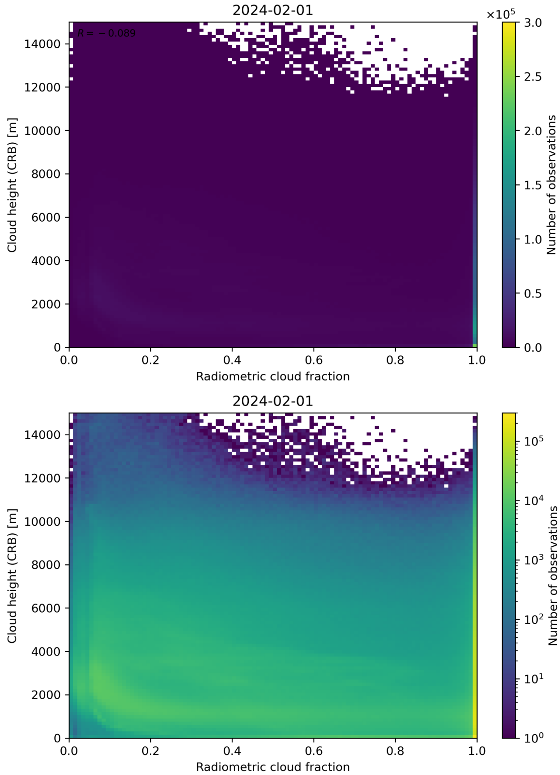
Figure 74: Scatter density plot of “Radiometric cloud fraction” against “Cloud height (CRB)” for 2024-01-31 to 2024-02-02.
