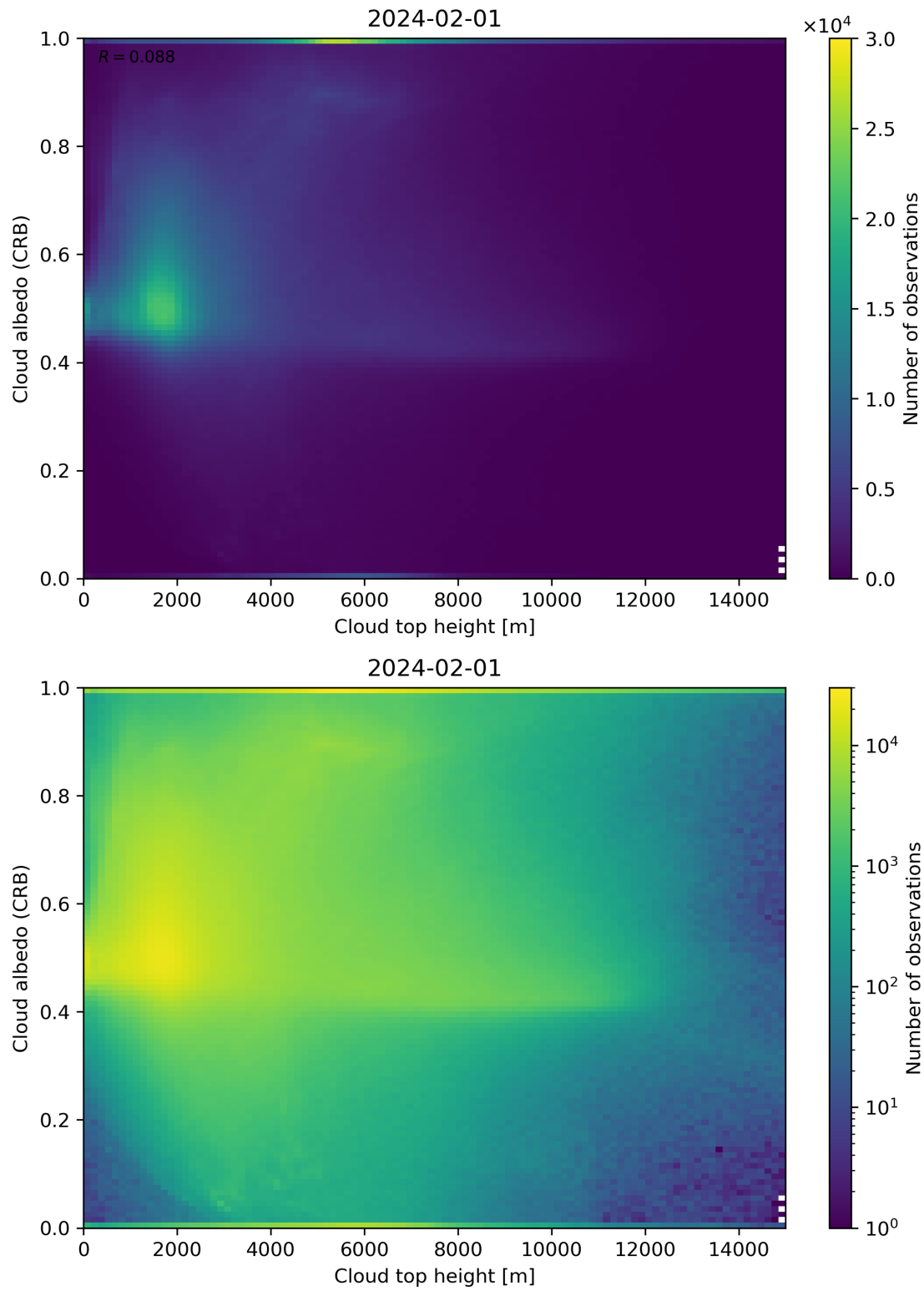
Figure 86: Scatter density plot of “Cloud top height” against “Cloud albedo (CRB)” for 2024-01-31 to 2024-02-02.
