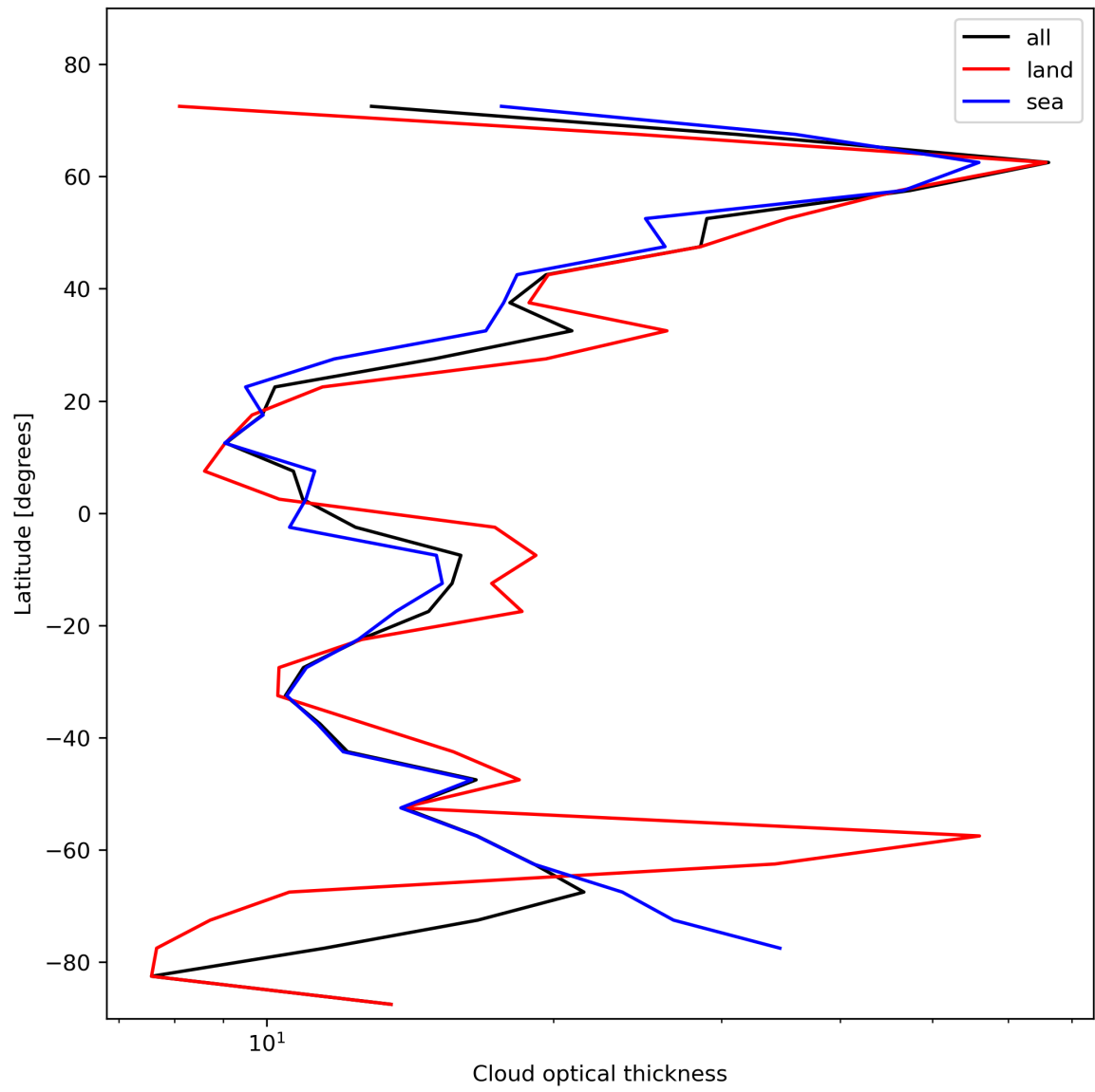
Figure 25: Zonal average of “Cloud optical thickness” for 2024-01-31 to 2024-02-02.
