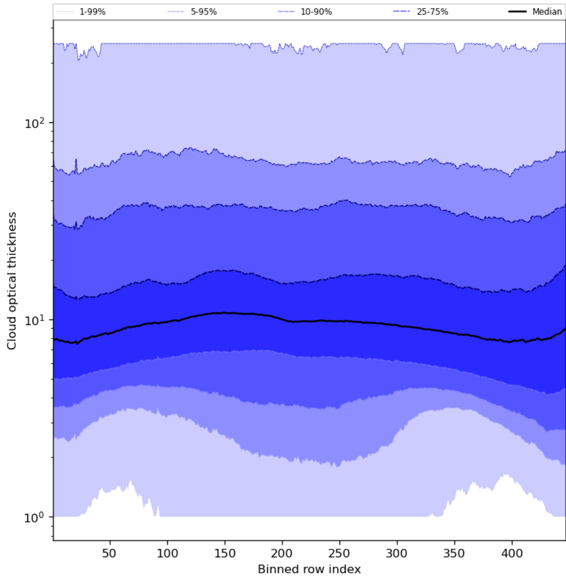
Figure 57: Along track statistics of “Cloud optical thickness” for 2024-01-31 to 2024-02-02
