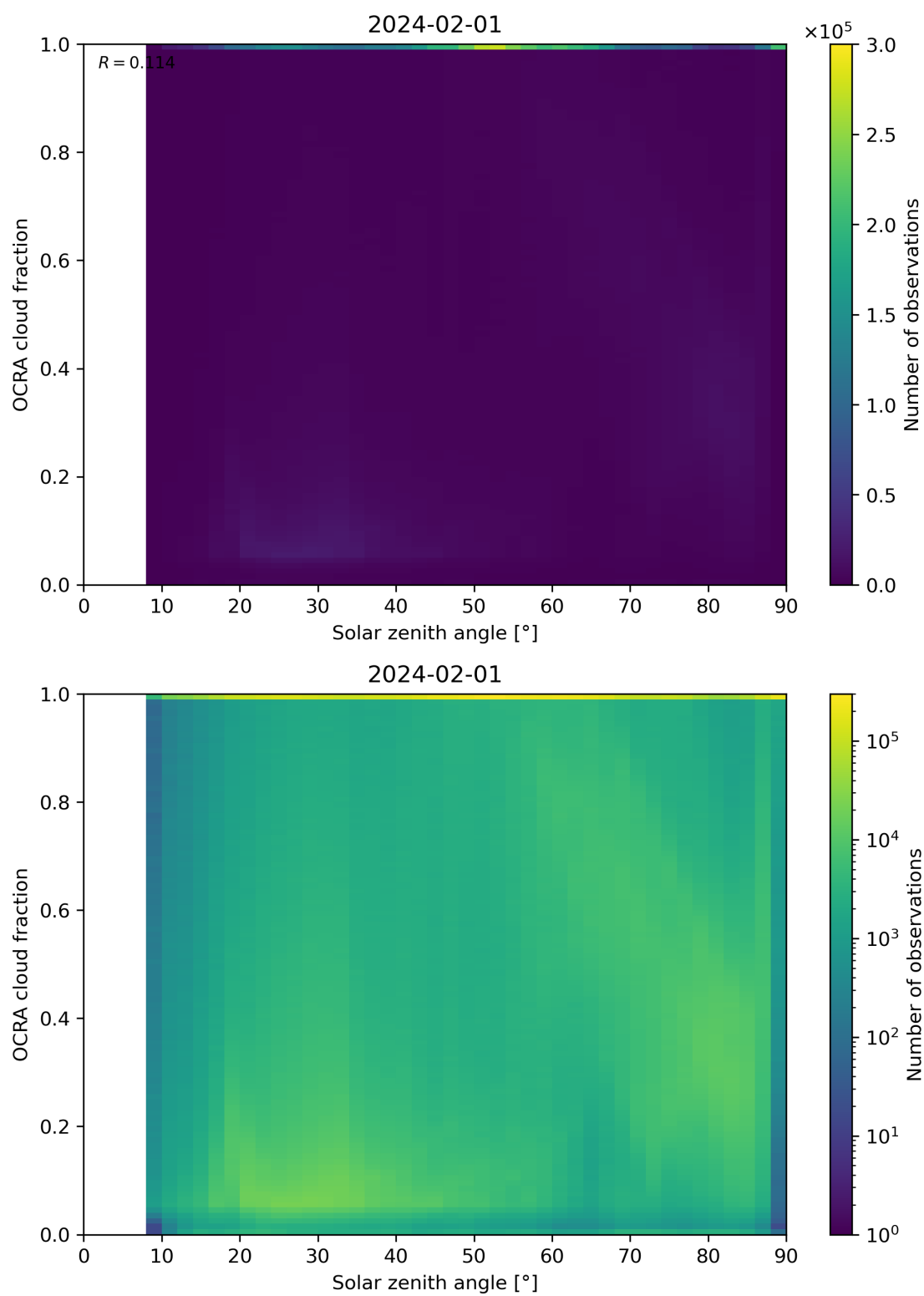
Figure 100: Scatter density plot of “Solar zenith angle” against “OCRA cloud fraction” for 2024-01-31 to 2024-02-02.
