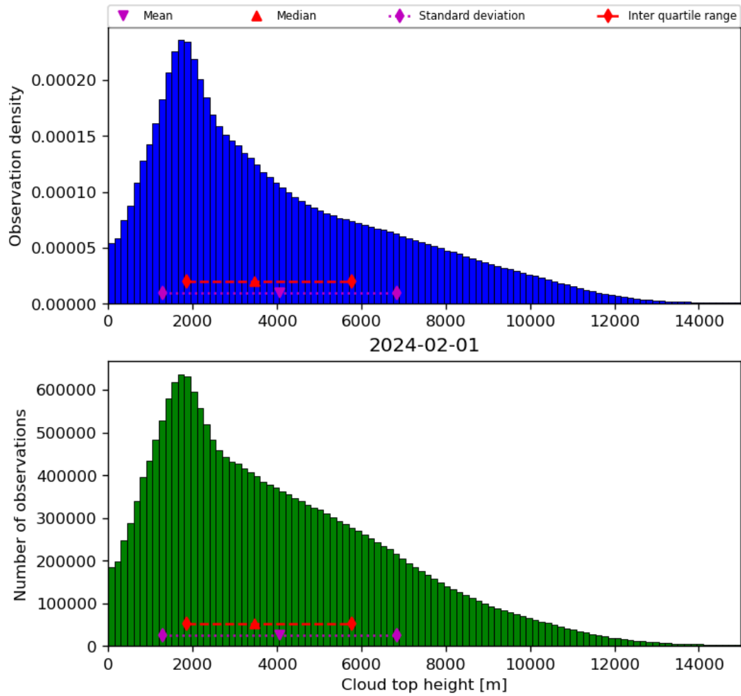
Figure 40: Histogram of “Cloud top height” for 2024-01-31 to 2024-02-02
