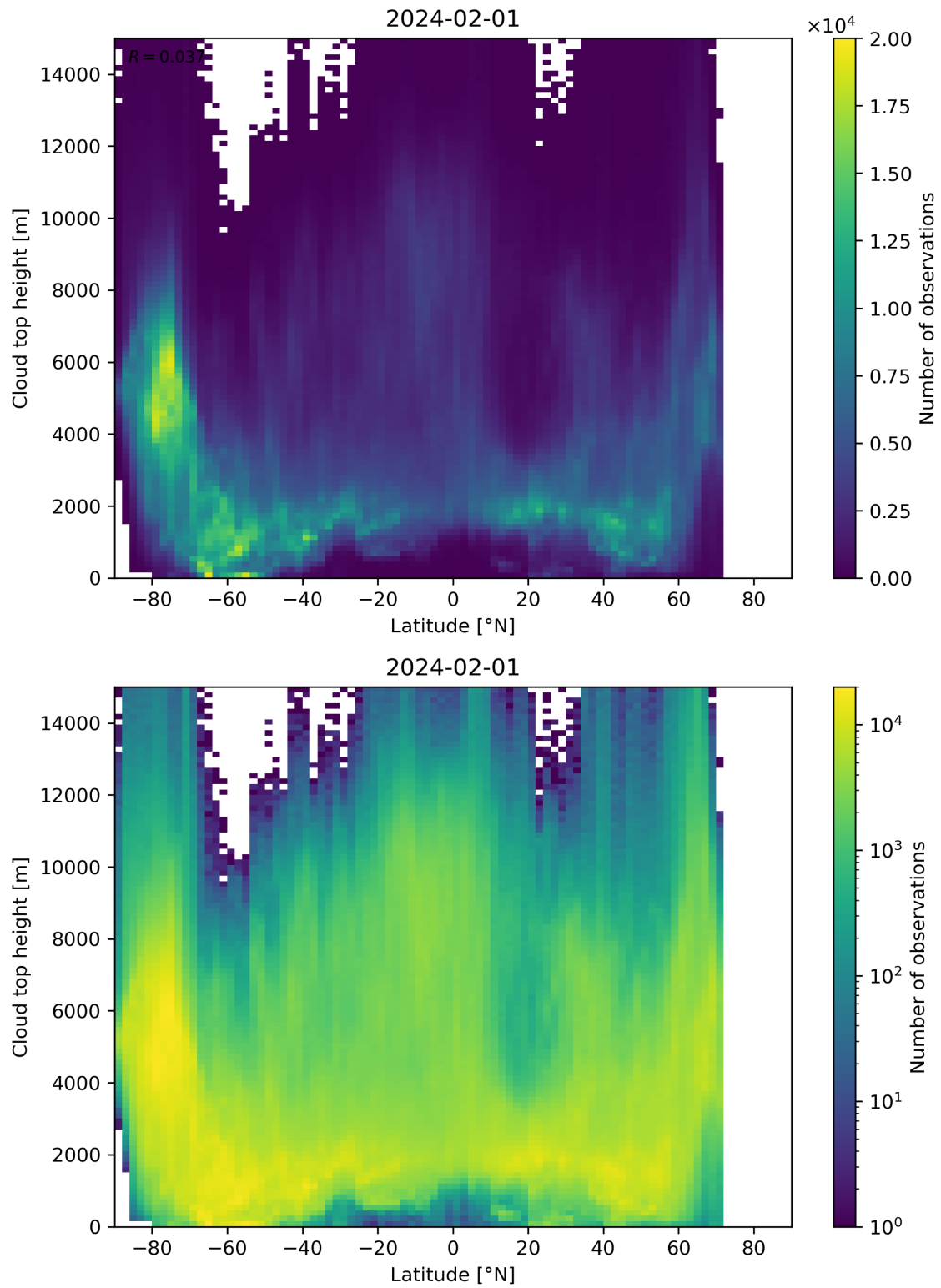
Figure 97: Scatter density plot of “Latitude” against “Cloud top height” for 2024-01-31 to 2024-02-02.
