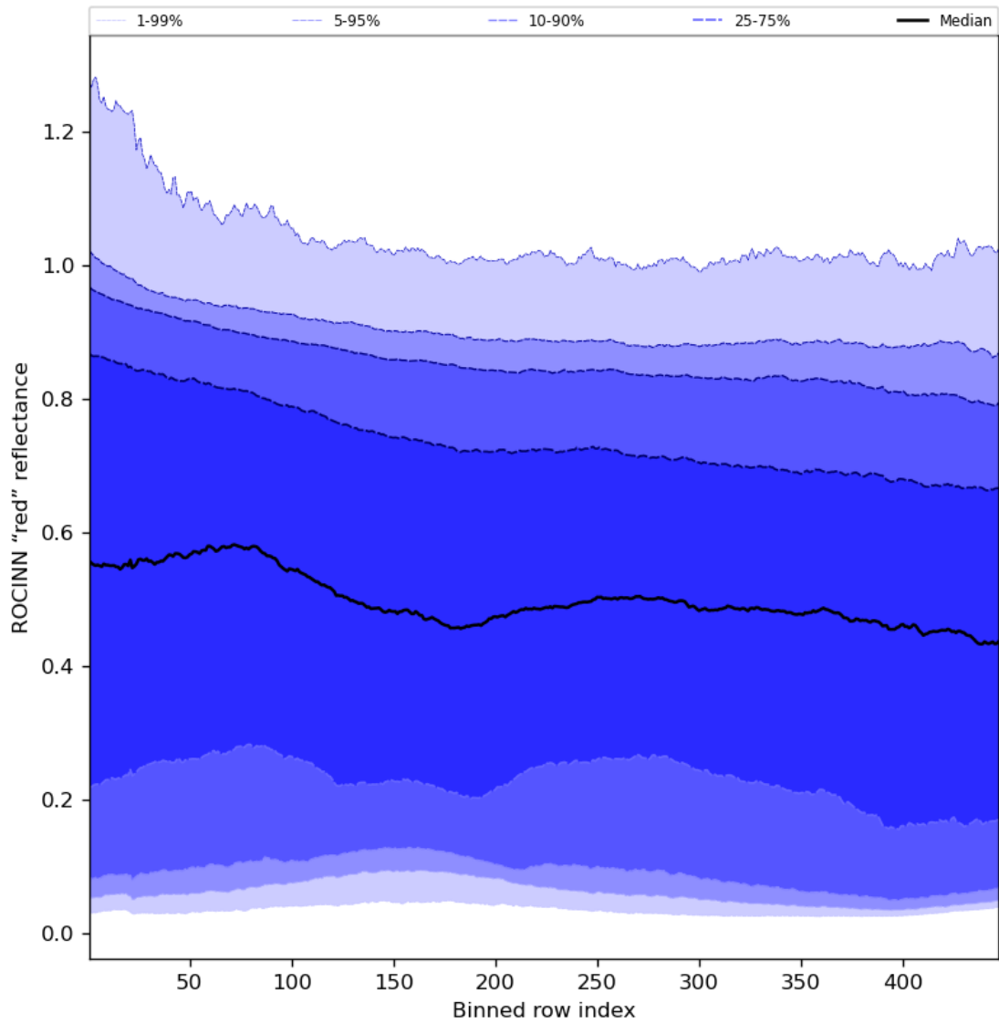
Figure 69: Along track statistics of “ROCINN “red” reflectance” for 2024-01-31 to 2024-02-02
