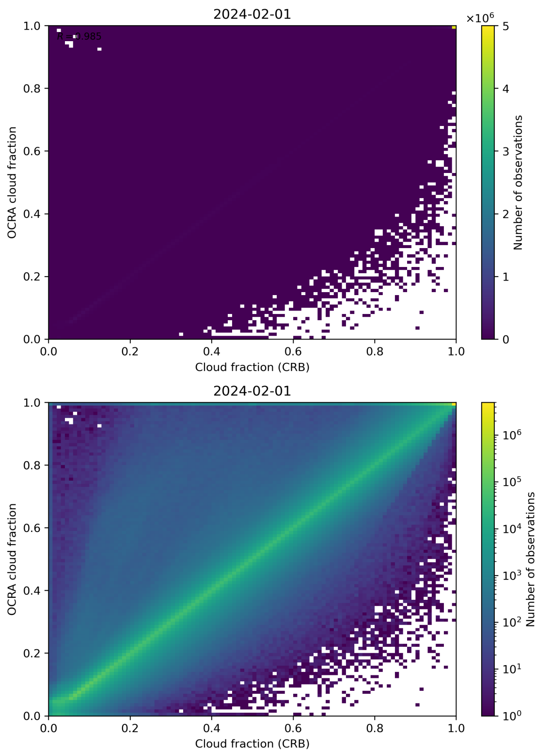
Figure 78: Scatter density plot of “Cloud fraction (CRB)” against “OCRA cloud fraction” for 2024-01-31 to 2024-02-02.
