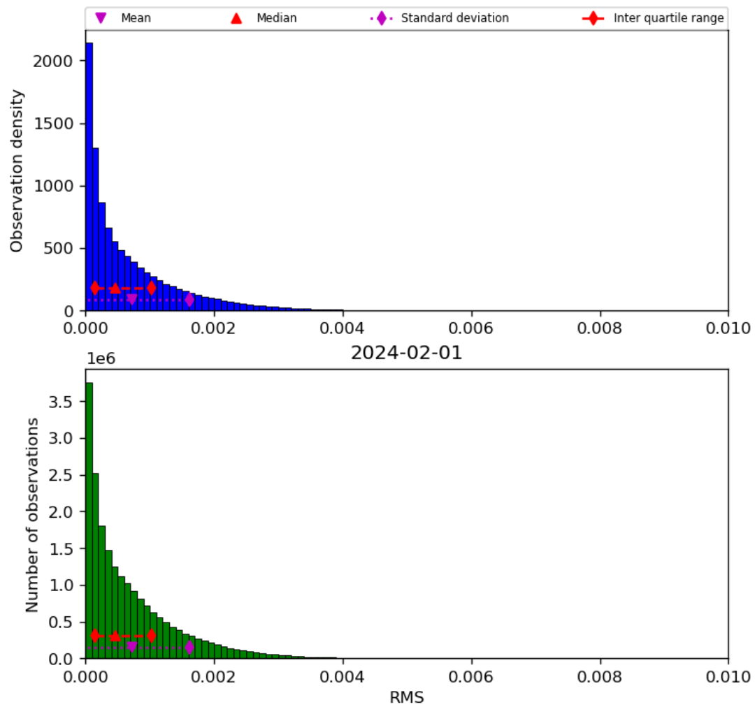
Figure 47: Histogram of “RMS” for 2024-01-31 to 2024-02-02
