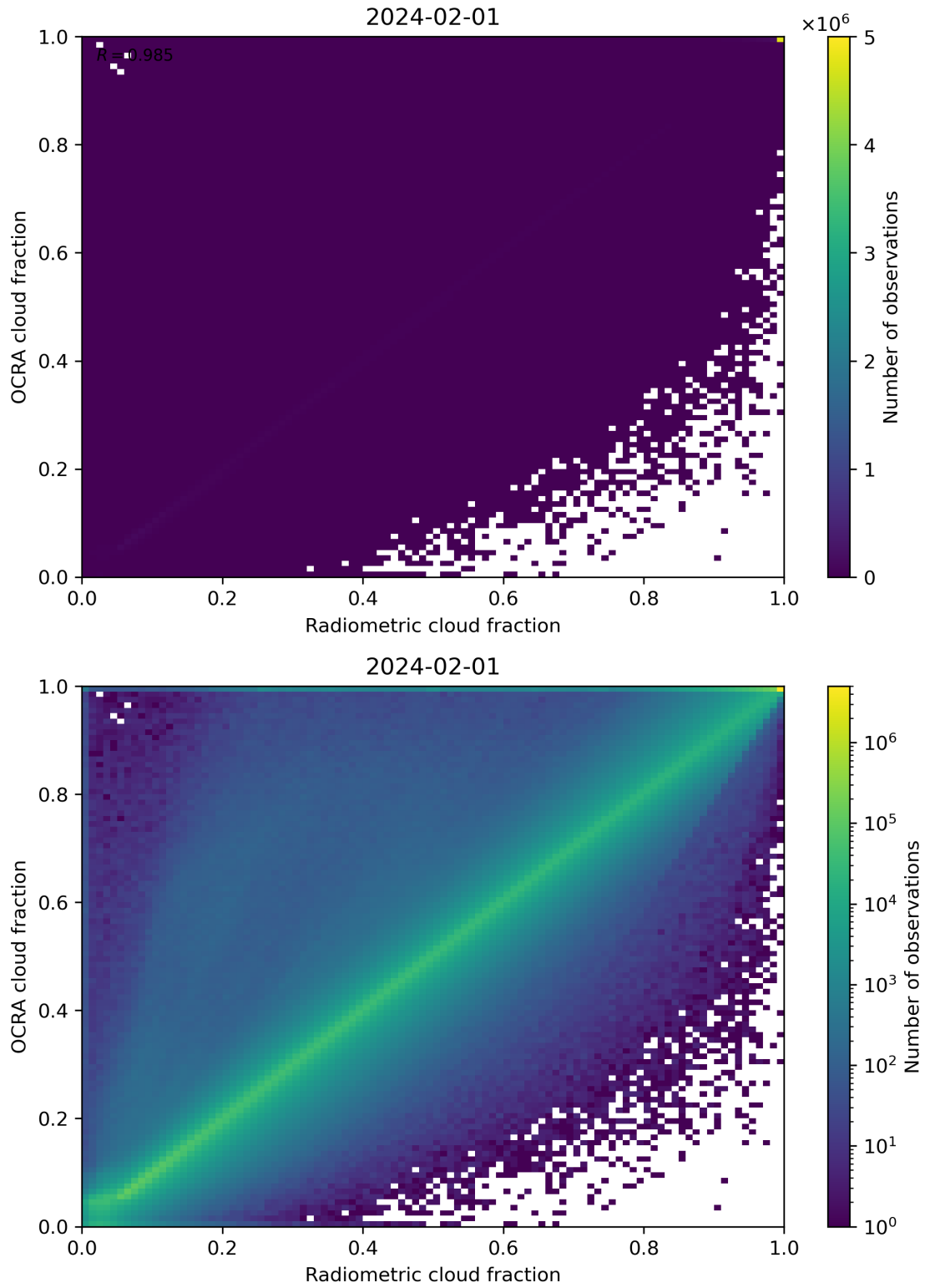
Figure 72: Scatter density plot of “Radiometric cloud fraction” against “OCRA cloud fraction” for 2024-01-31 to 2024-02-02.
