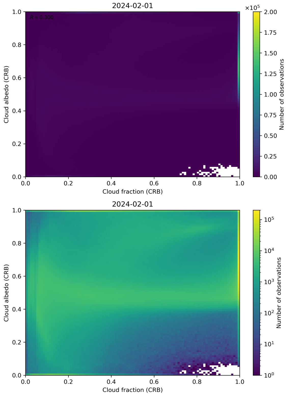
Figure 77: Scatter density plot of “Cloud fraction (CRB)” against “Cloud albedo (CRB)” for 2024-01-31 to 2024-02-02.
