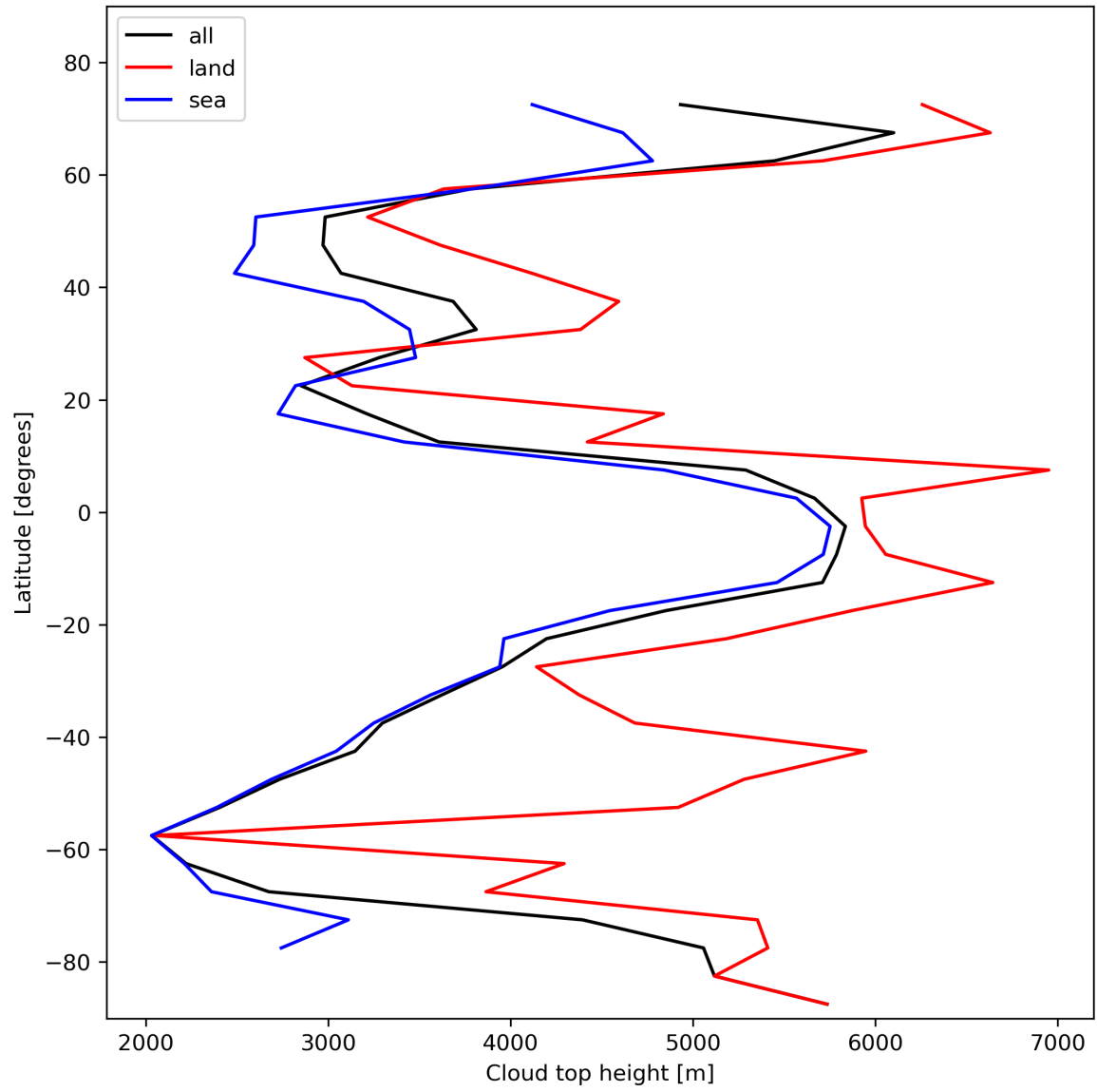
Figure 24: Zonal average of “Cloud top height” for 2024-01-31 to 2024-02-02.
