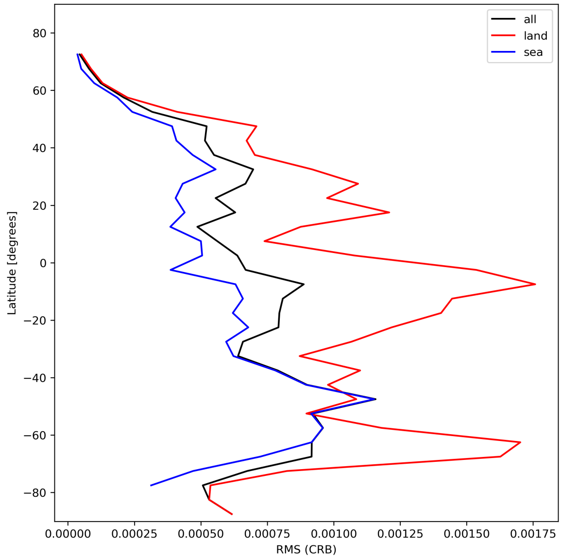
Figure 32: Zonal average of “RMS (CRB)” for 2024-01-31 to 2024-02-02.
