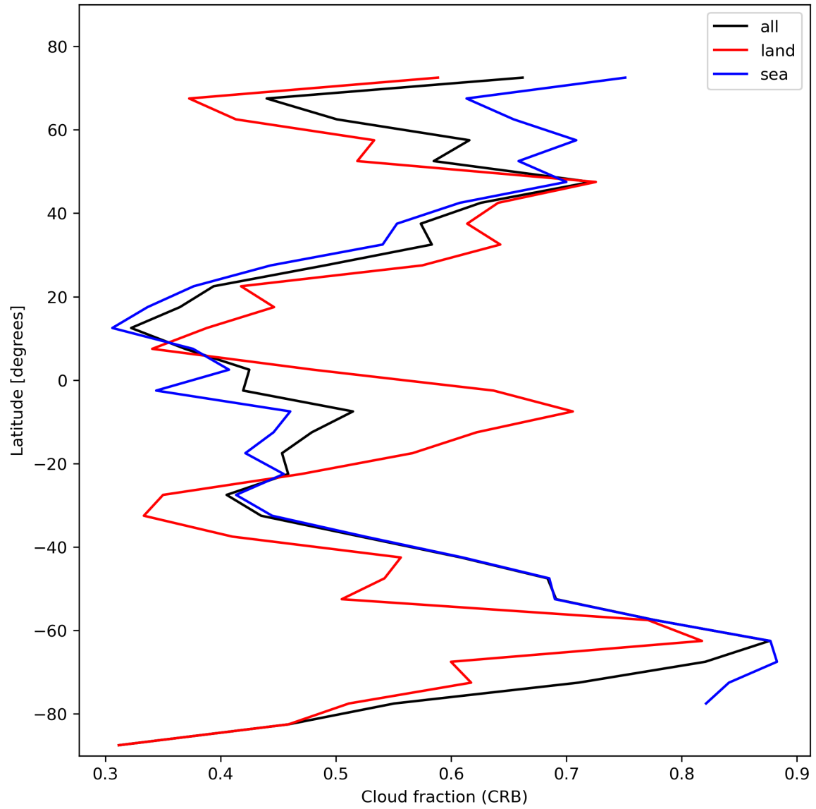
Figure 26: Zonal average of “Cloud fraction (CRB)” for 2024-01-31 to 2024-02-02.
