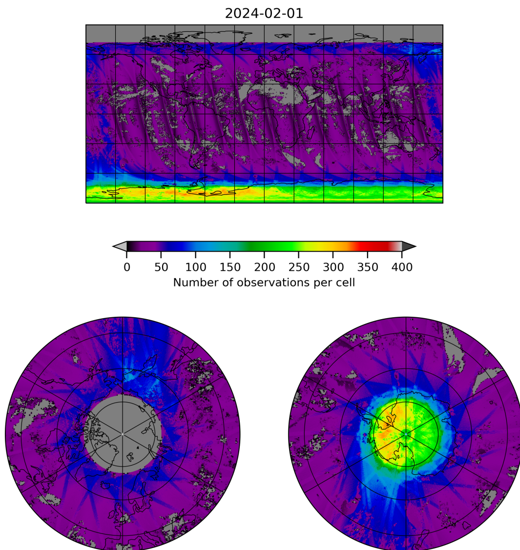
Figure 21: Map of the number of observations for 2024-01-31 to 2024-02-02
