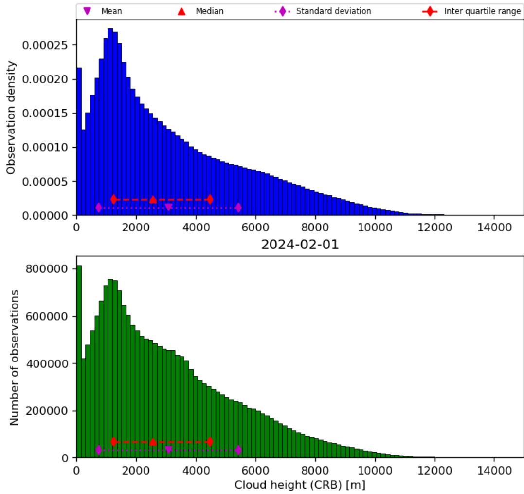
Figure 43: Histogram of “Cloud height (CRB)” for 2024-01-31 to 2024-02-02
