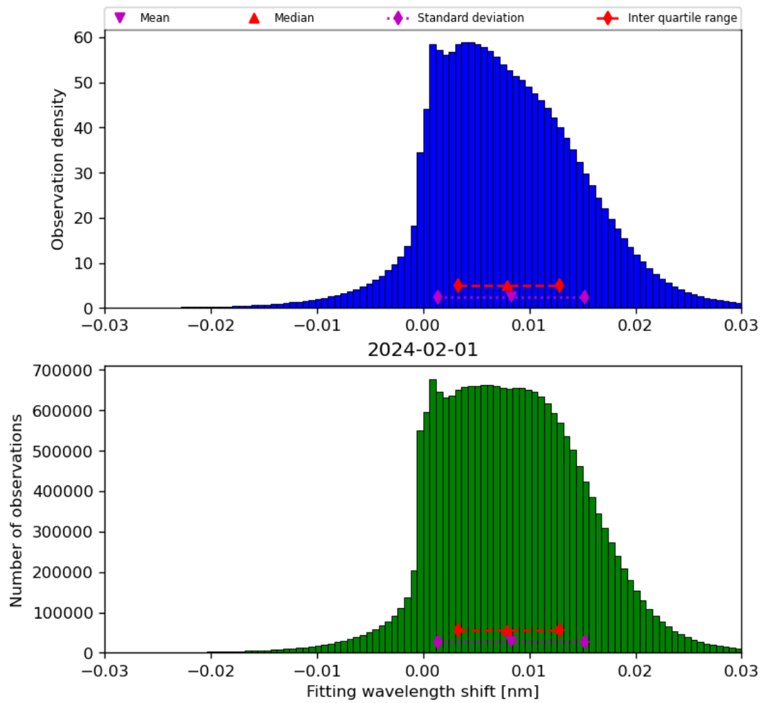
Figure 49: Histogram of “Fitting wavelength shift” for 2024-01-31 to 2024-02-02
