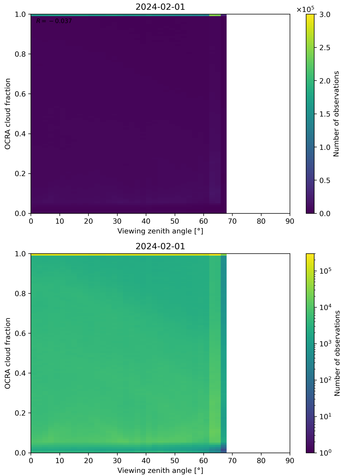
Figure 108: Scatter density plot of “Viewing zenith angle” against “OCRA cloud fraction” for 2024-01-31 to 2024-02-02.
