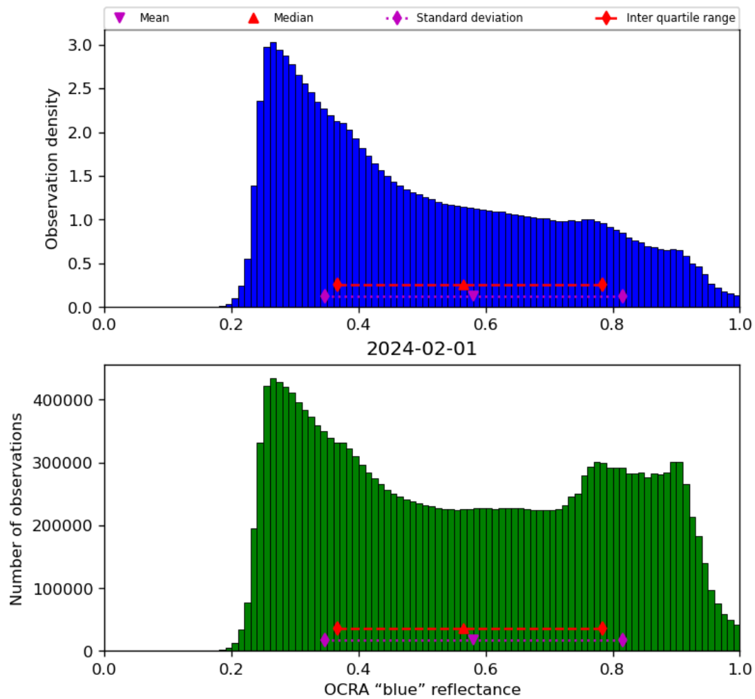
Figure 51: Histogram of “OCRA “blue” reflectance” for 2024-01-31 to 2024-02-02
