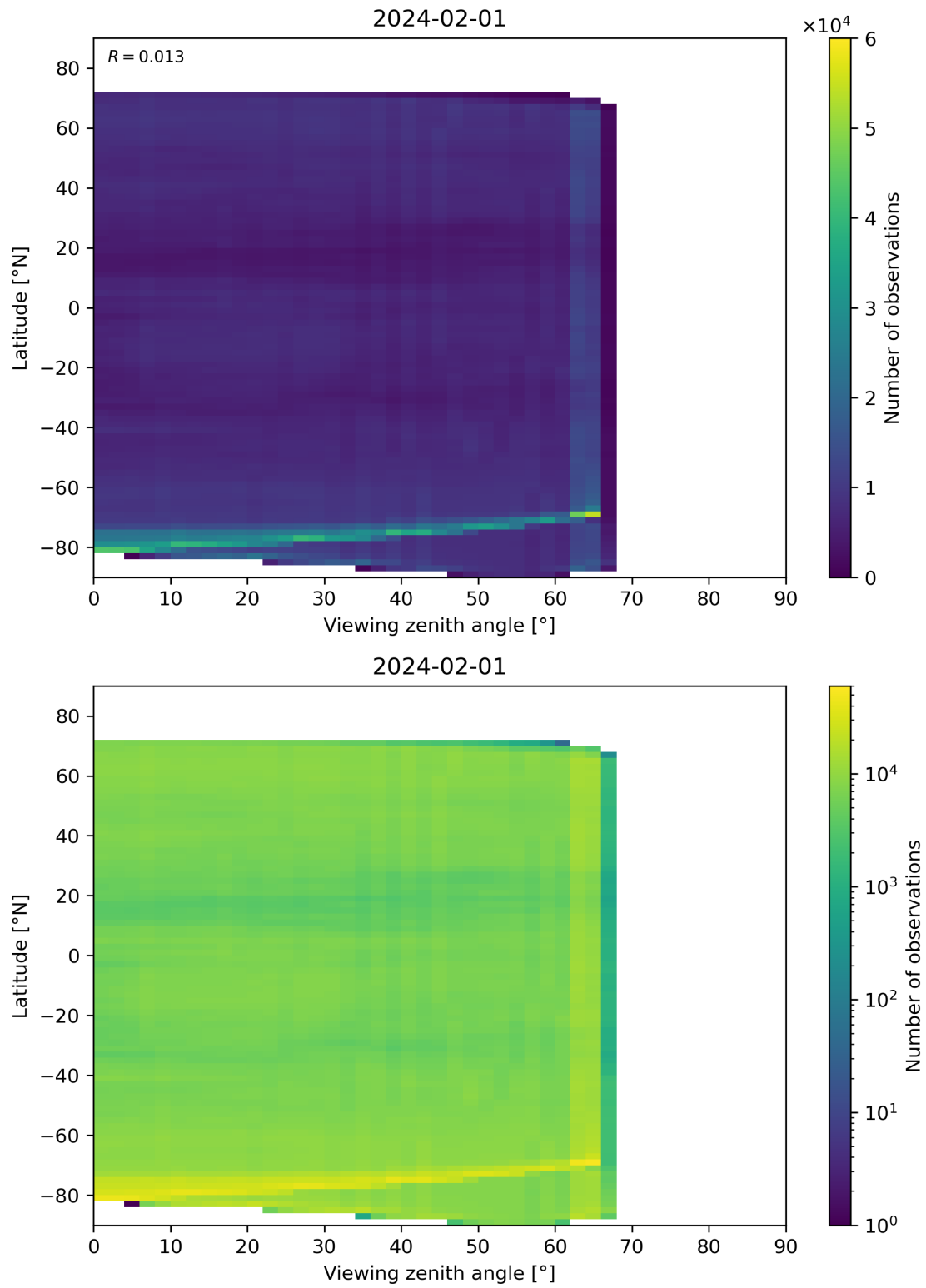
Figure 113: Scatter density plot of “Viewing zenith angle” against “Latitude” for 2024-01-31 to 2024-02-02.
