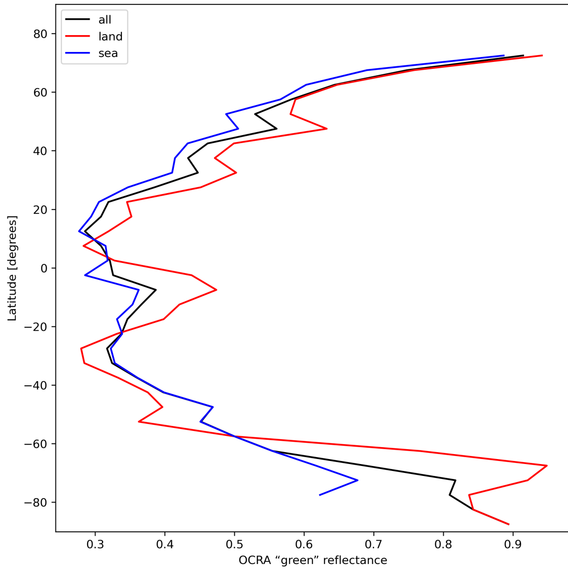
Figure 36: Zonal average of “OCRA “green” reflectance” for 2024-01-31 to 2024-02-02.
