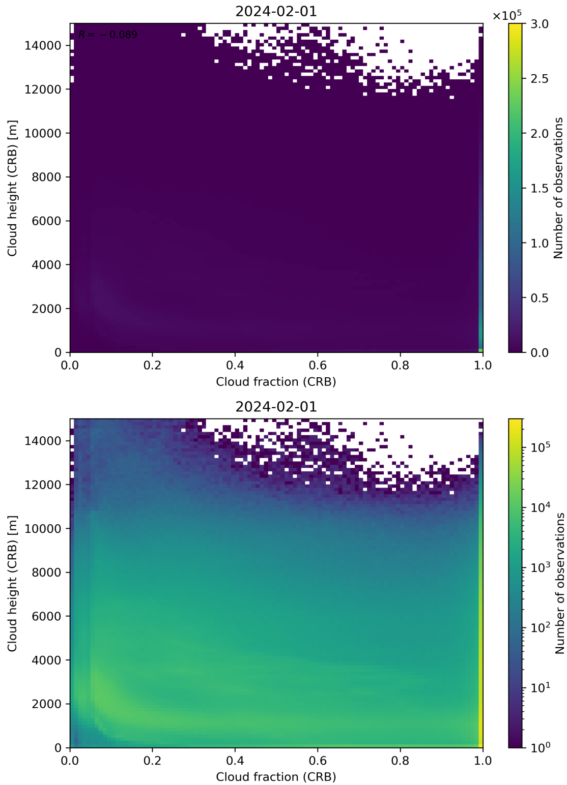
Figure 79: Scatter density plot of “Cloud fraction (CRB)” against “Cloud height (CRB)” for 2024-01-31 to 2024-02-02.
