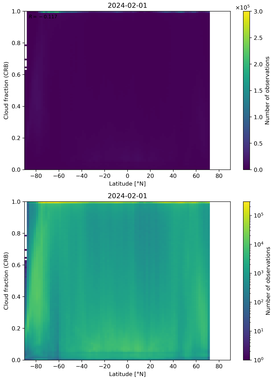
Figure 94: Scatter density plot of “Latitude” against “Cloud fraction (CRB)” for 2024-01-31 to 2024-02-02.
