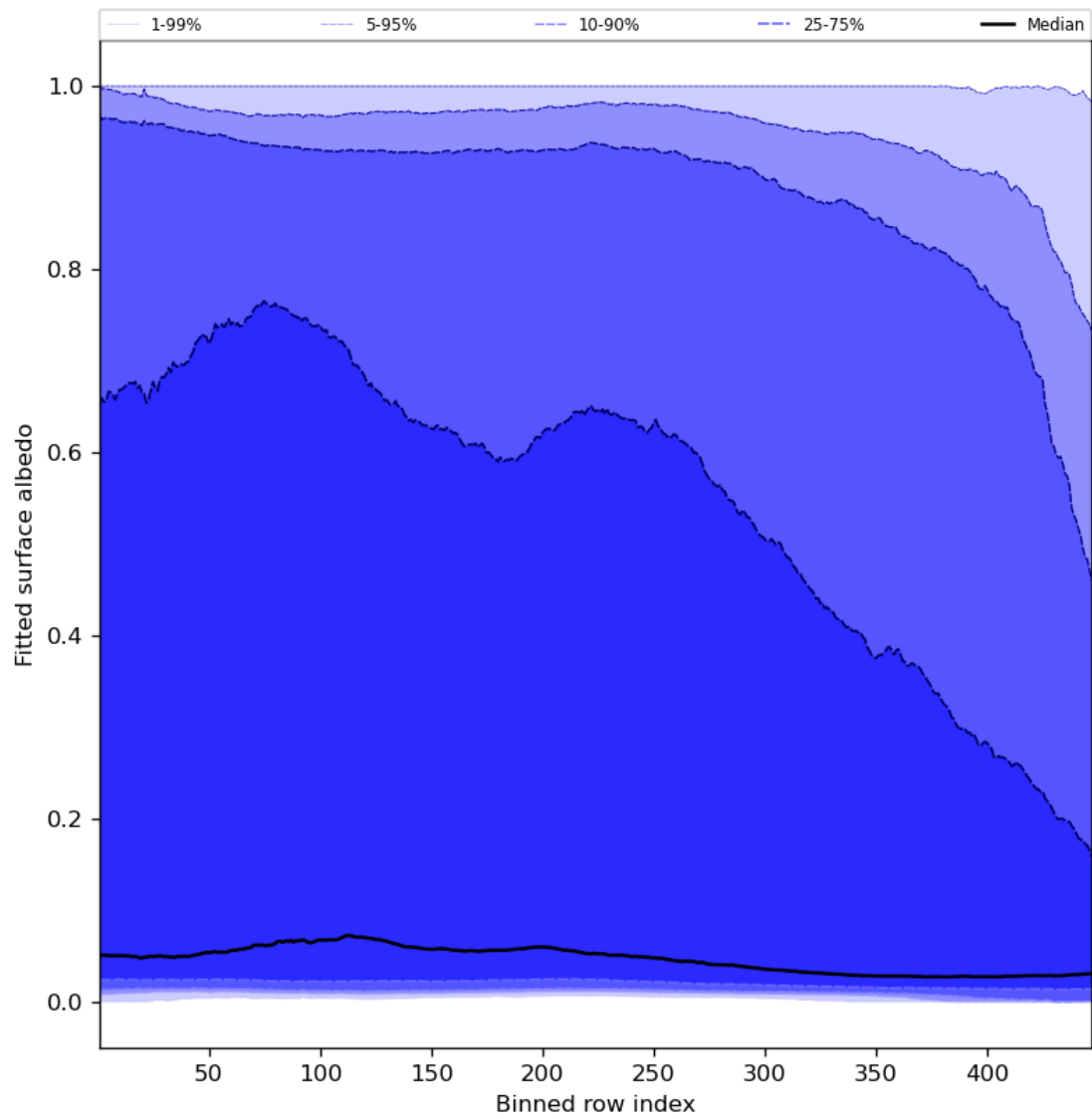
Figure 61: Along track statistics of “Fitted surface albedo” for 2024-01-31 to 2024-02-02
