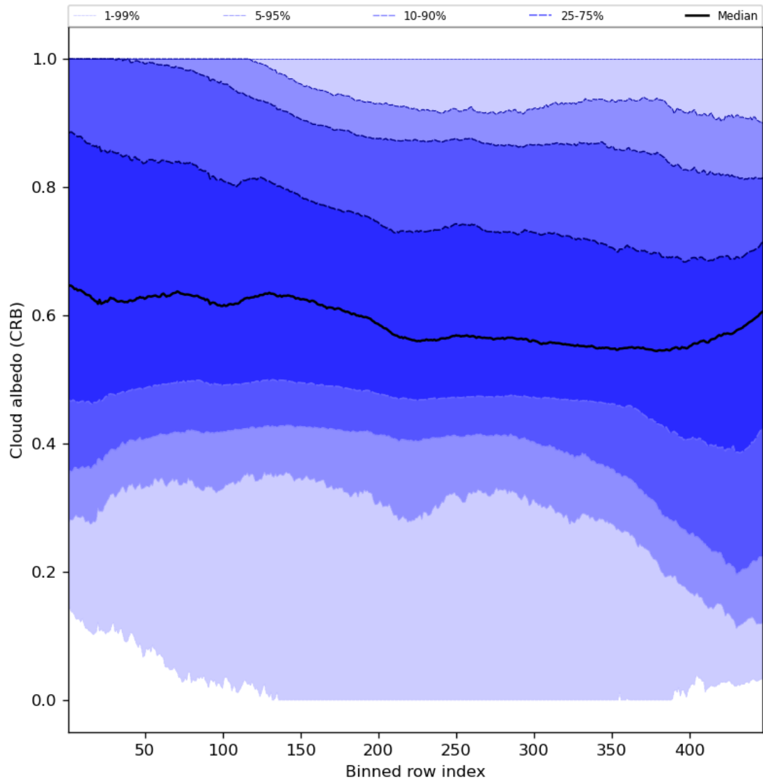
Figure 60: Along track statistics of “Cloud albedo (CRB)” for 2024-01-31 to 2024-02-02
