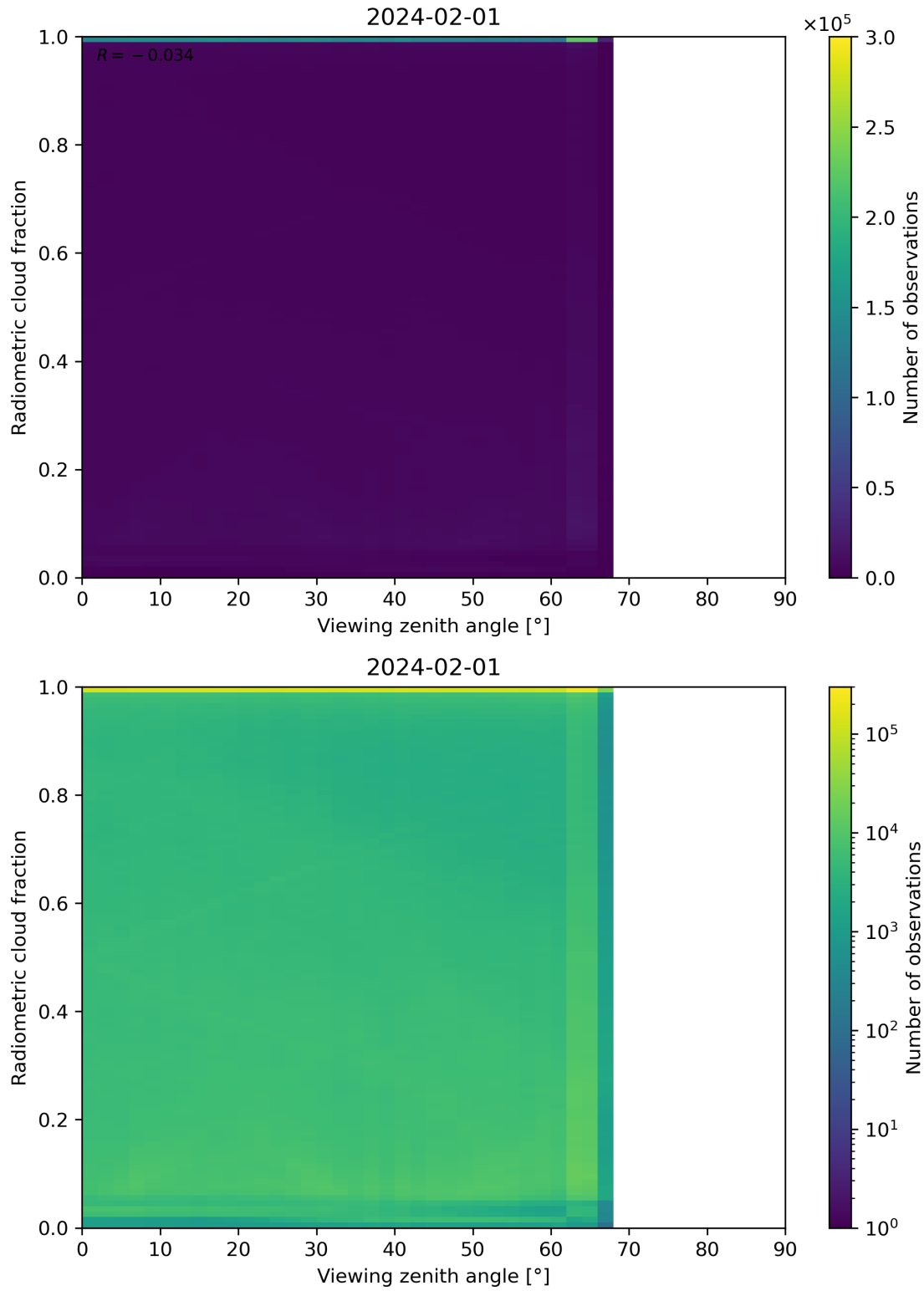
Figure 107: Scatter density plot of “Viewing zenith angle” against “Radiometric cloud fraction” for 2024-01-31 to 2024-02-02.
