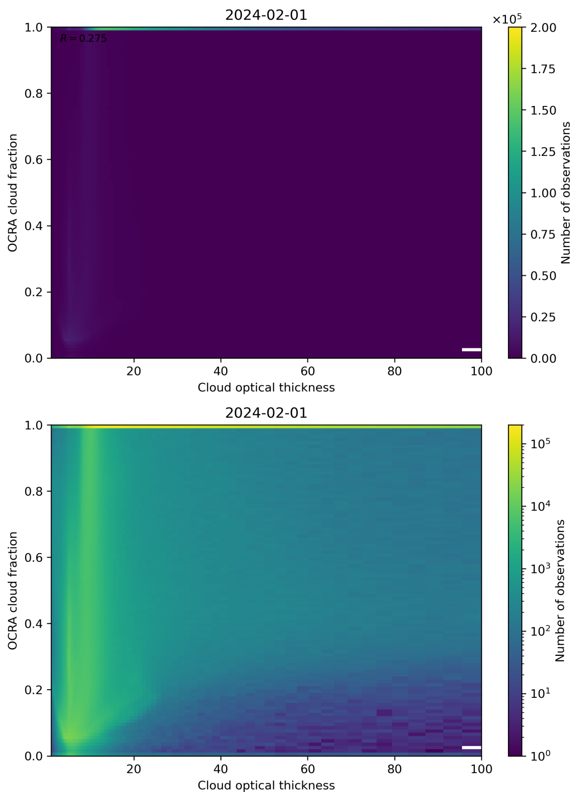
Figure 83: Scatter density plot of “Cloud optical thickness” against “OCRA cloud fraction” for 2024-01-31 to 2024-02-02.
