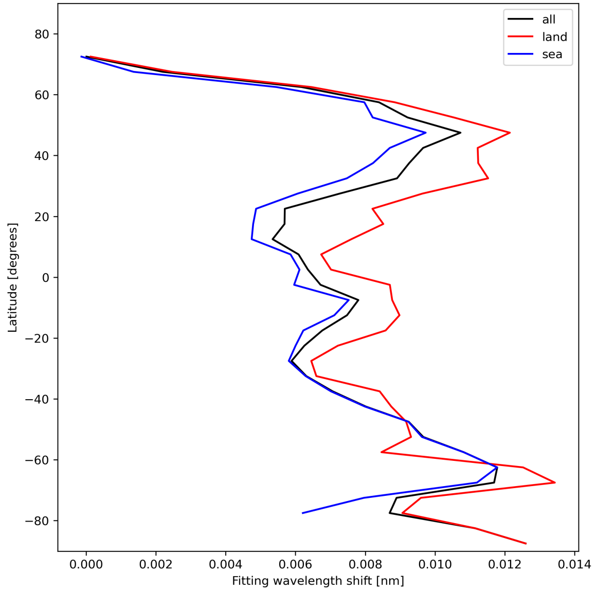
Figure 33: Zonal average of “Fitting wavelength shift” for 2024-01-31 to 2024-02-02.
