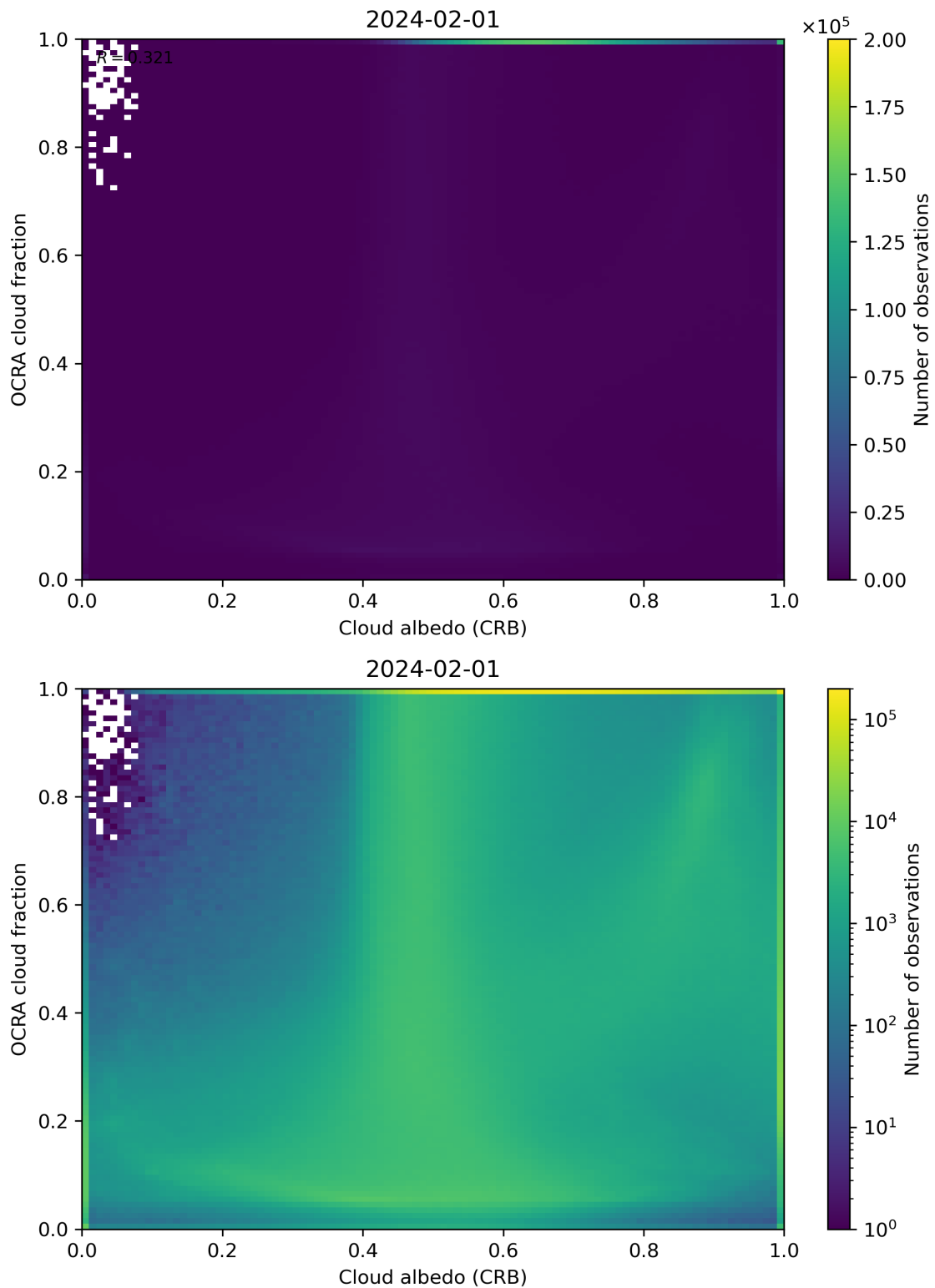
Figure 70: Scatter density plot of “Cloud albedo (CRB)” against “OCRA cloud fraction” for 2024-01-31 to 2024-02-02.
