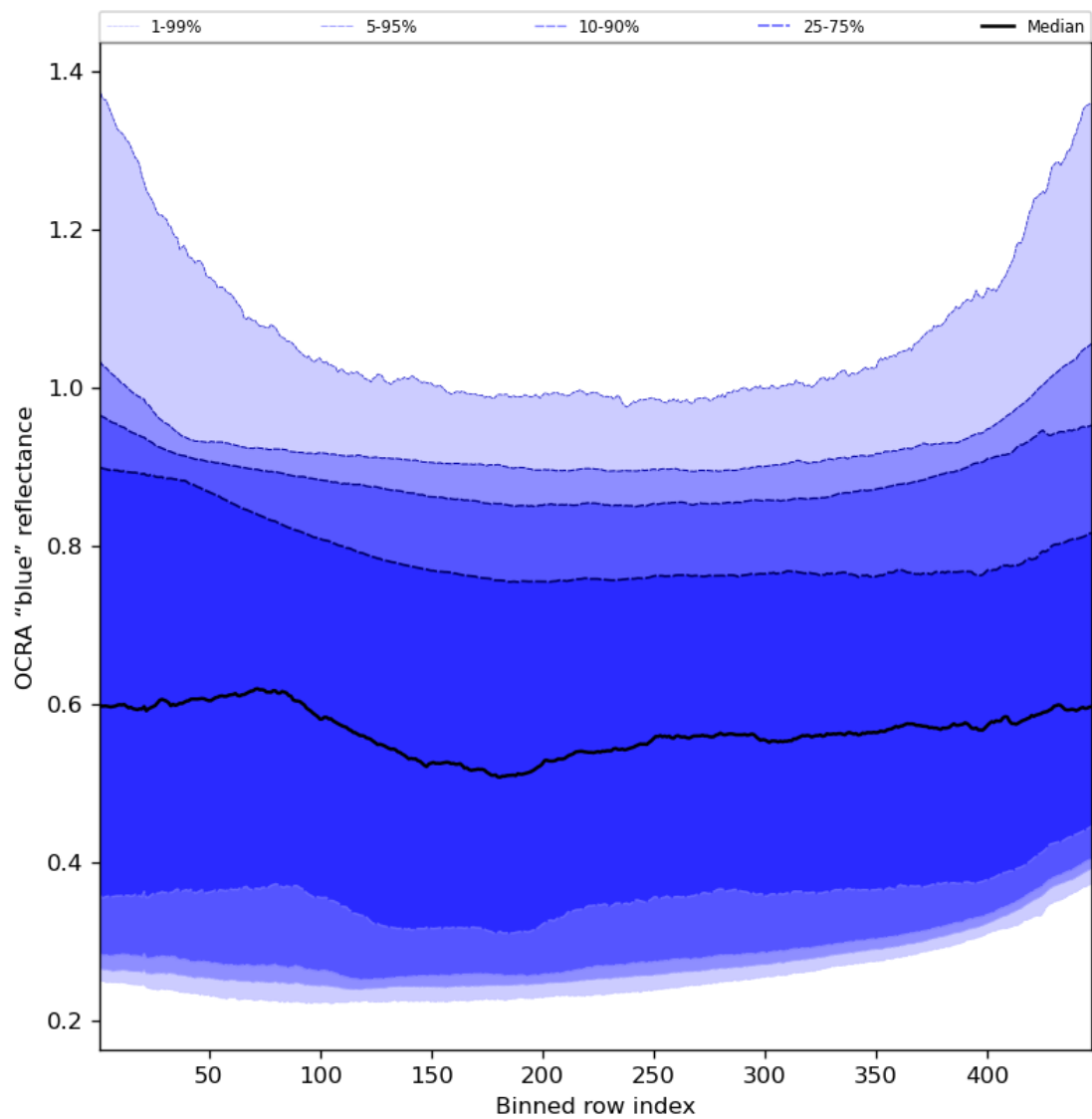
Figure 67: Along track statistics of “OCRA “blue” reflectance” for 2024-01-31 to 2024-02-02
