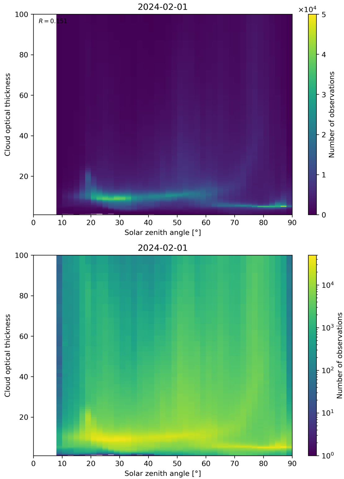
Figure 103: Scatter density plot of “Solar zenith angle” against “Cloud optical thickness” for 2024-01-31 to 2024-02-02.
