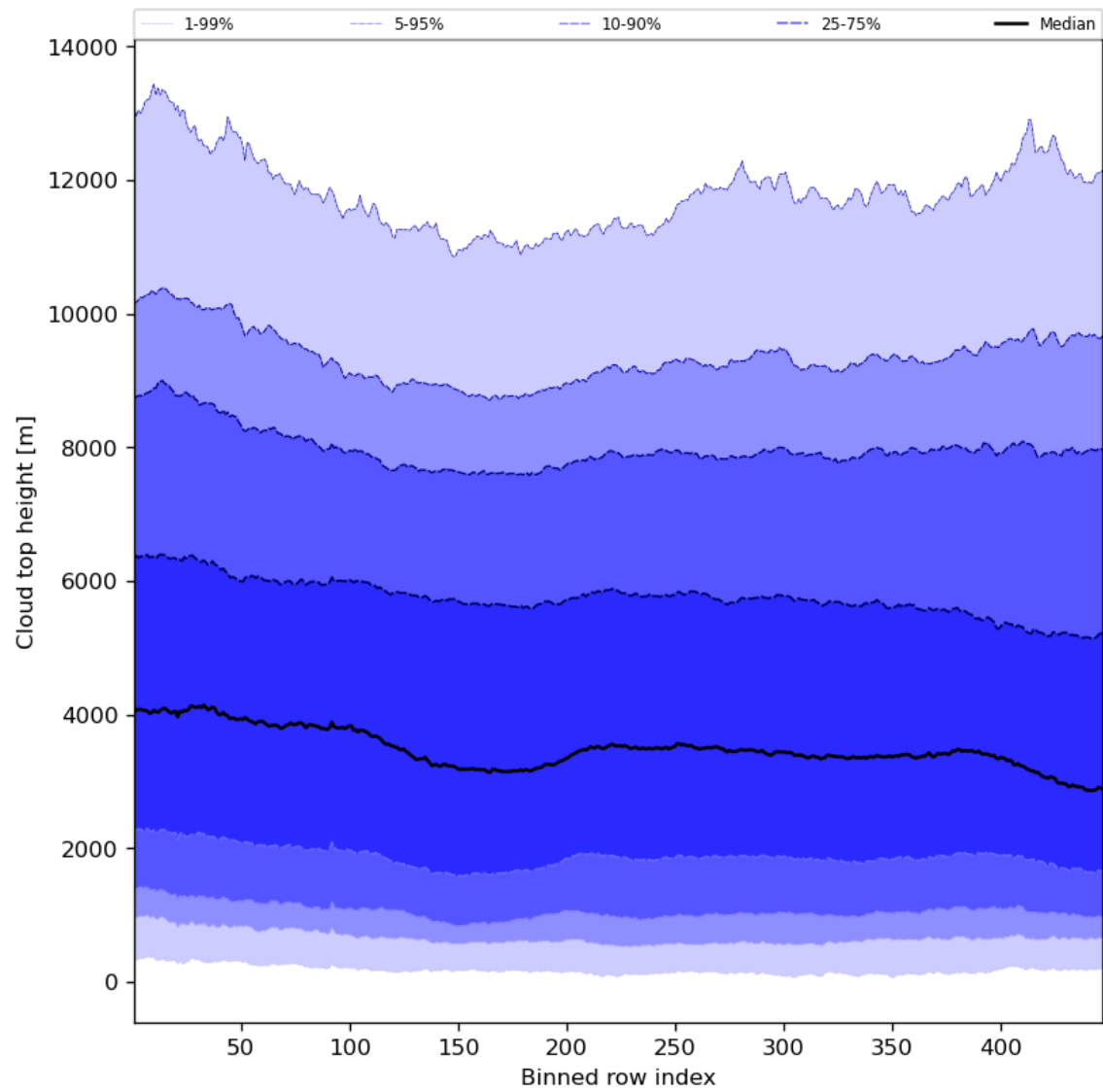
Figure 56: Along track statistics of “Cloud top height” for 2024-01-31 to 2024-02-02
