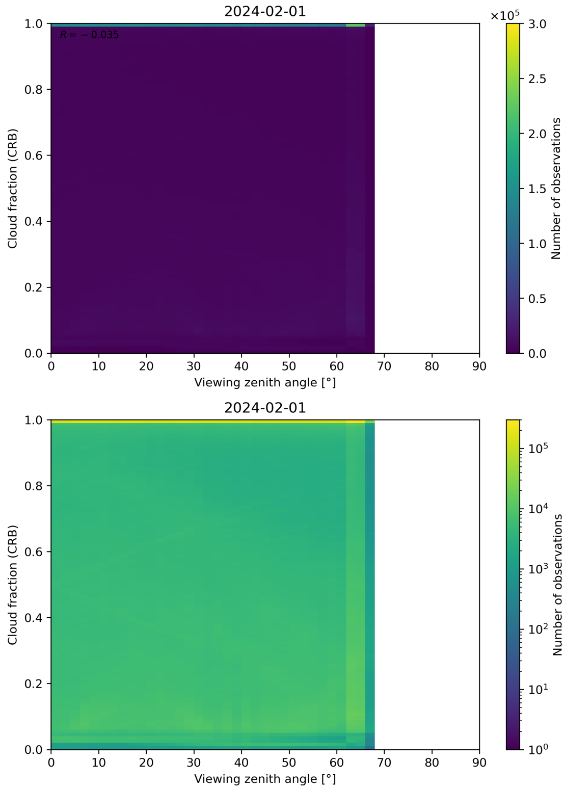
Figure 109: Scatter density plot of “Viewing zenith angle” against “Cloud fraction (CRB)” for 2024-01-31 to 2024-02-02.
