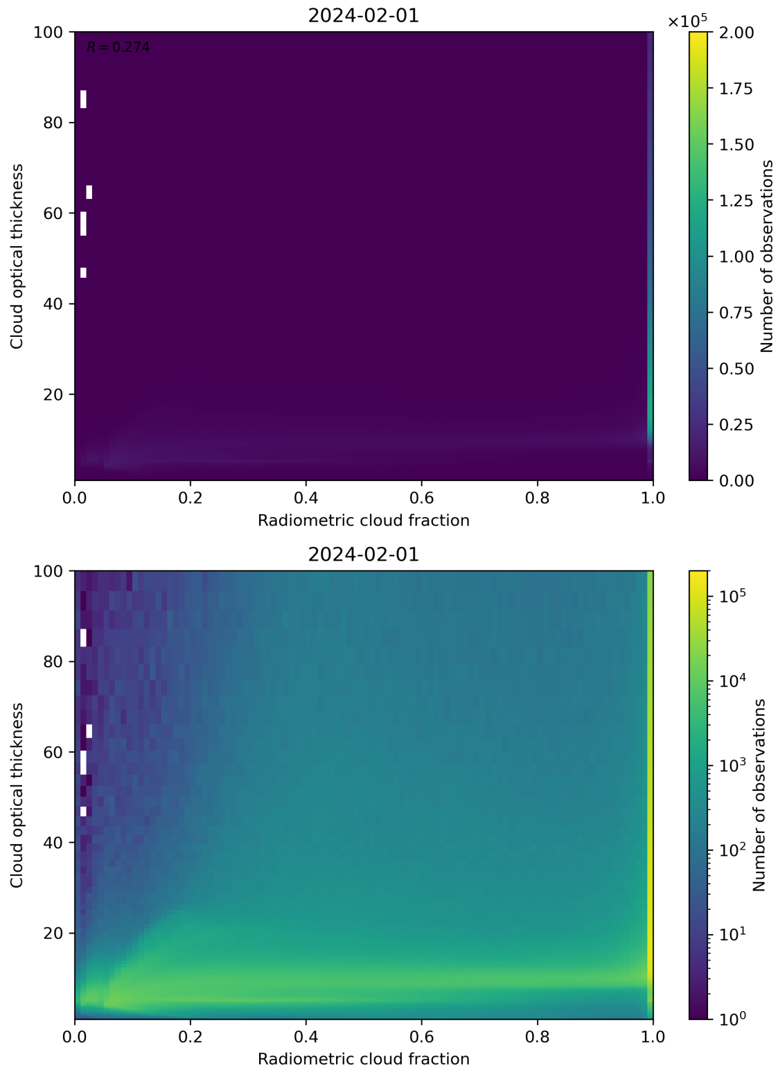
Figure 75: Scatter density plot of “Radiometric cloud fraction” against “Cloud optical thickness” for 2024-01-31 to 2024-02-02.
