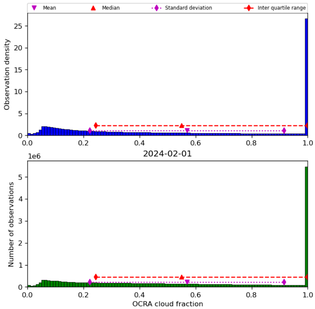
Figure 50: Histogram of “OCRA cloud fraction” for 2024-01-31 to 2024-02-02
