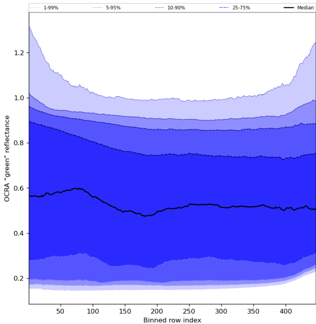
Figure 68: Along track statistics of “OCRA “green” reflectance” for 2024-01-31 to 2024-02-02
