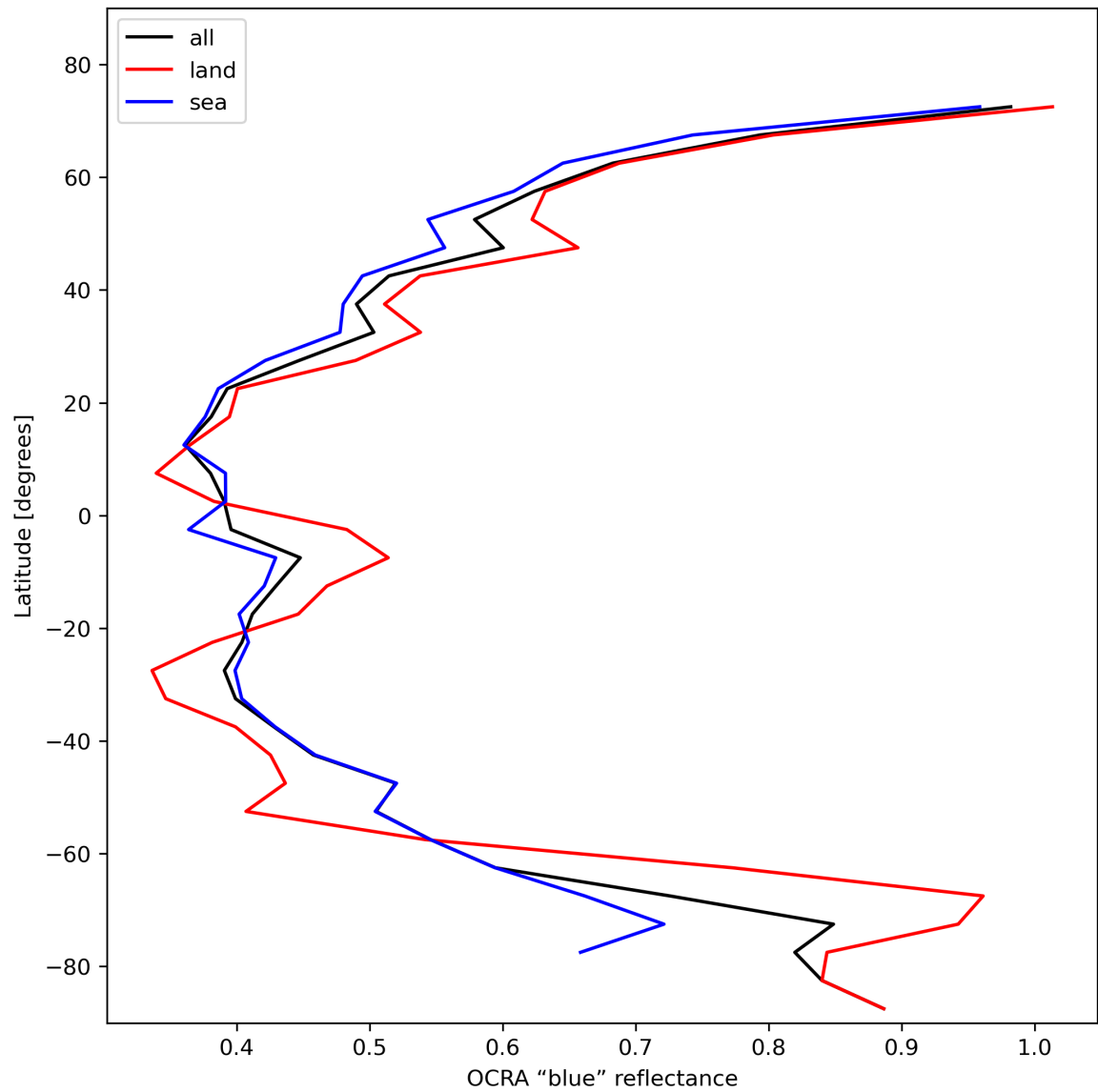
Figure 35: Zonal average of “OCRA “blue” reflectance” for 2024-01-31 to 2024-02-02.
