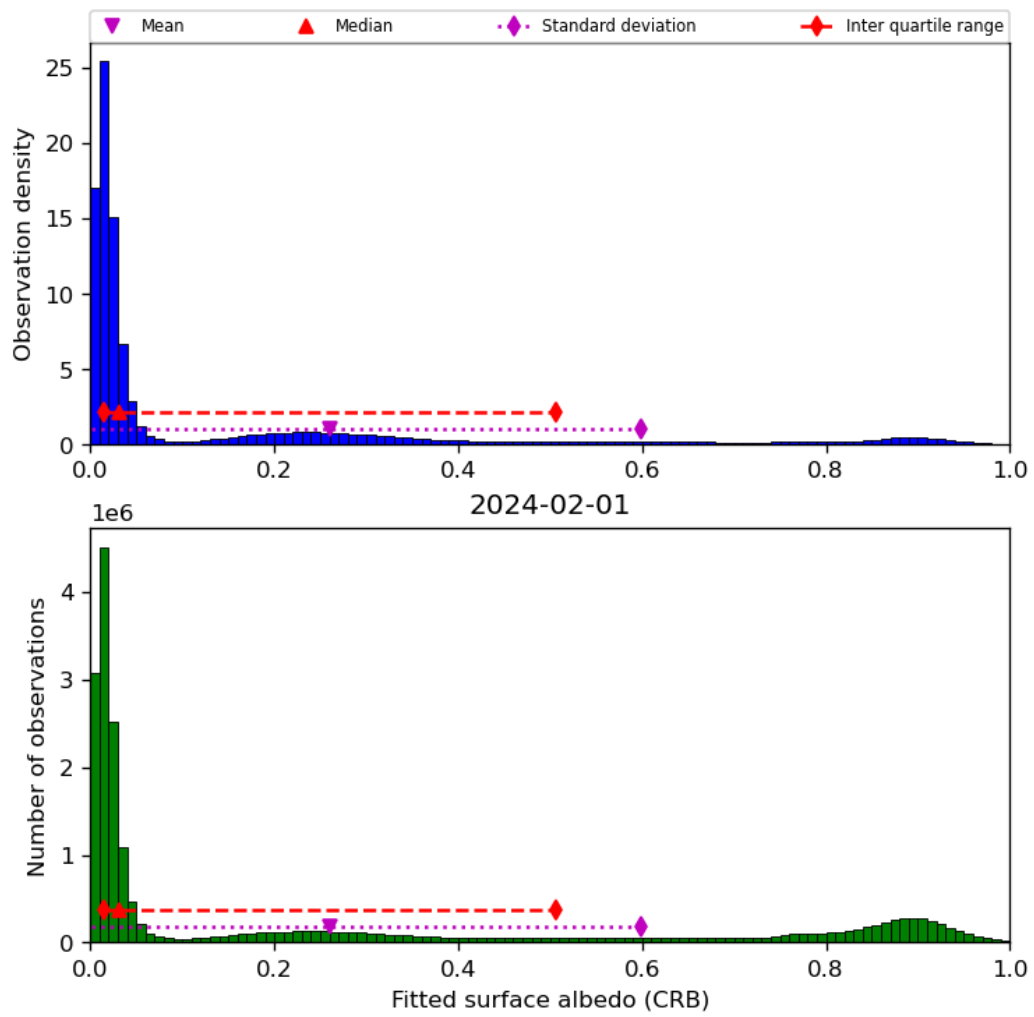
Figure 46: Histogram of “Fitted surface albedo (CRB)” for 2024-01-31 to 2024-02-02
