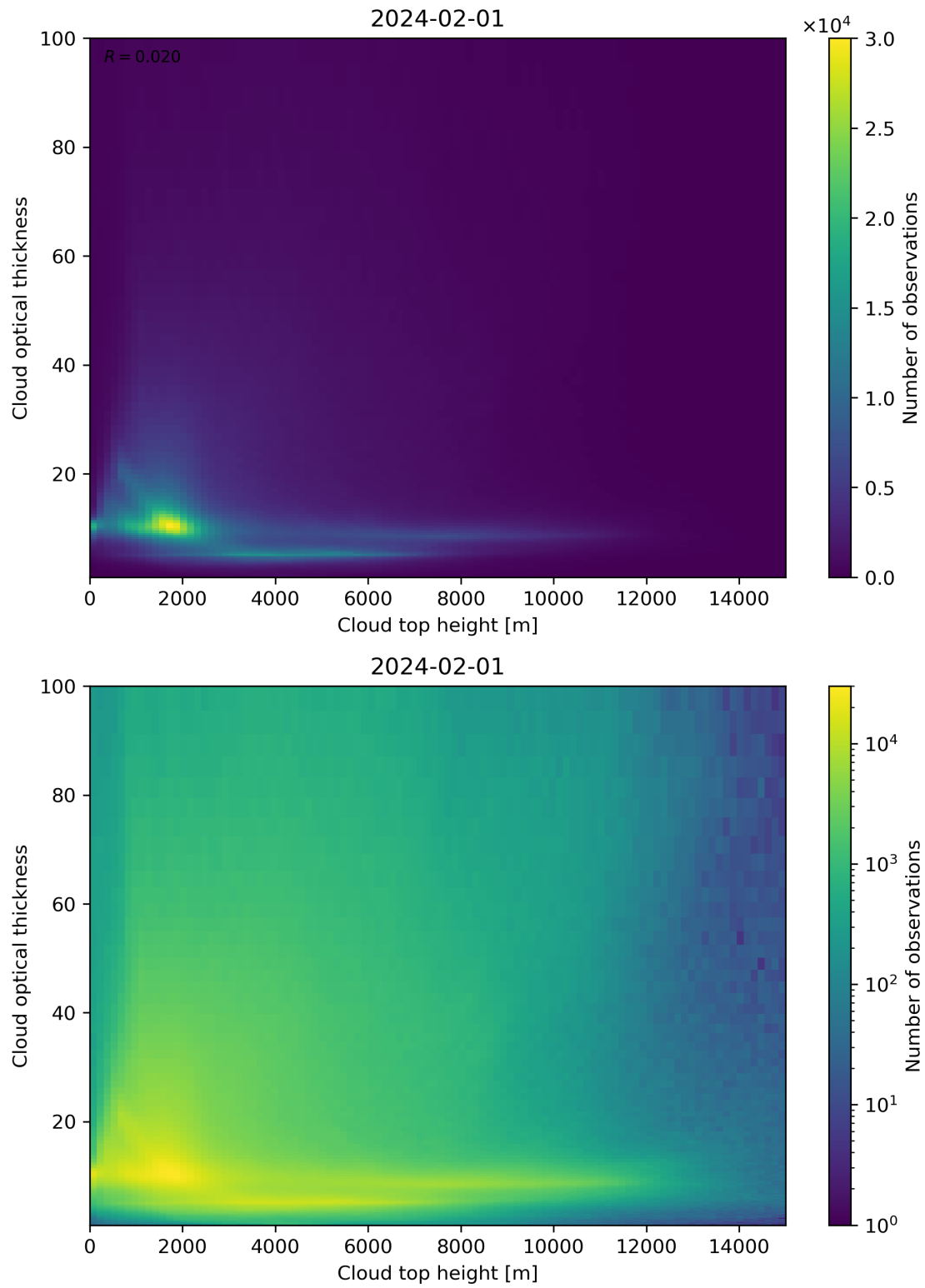
Figure 90: Scatter density plot of “Cloud top height” against “Cloud optical thickness” for 2024-01-31 to 2024-02-02.
