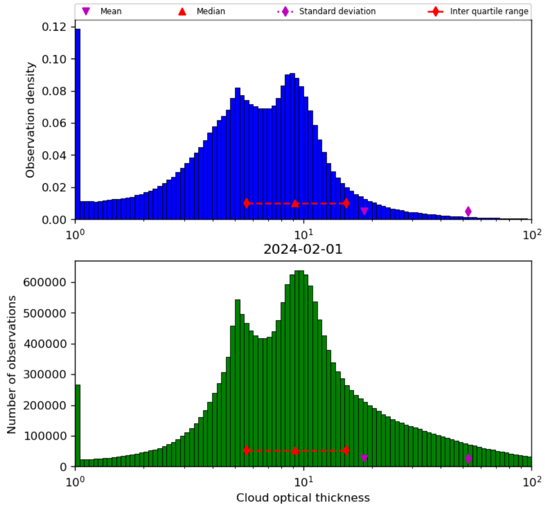
Figure 41: Histogram of “Cloud optical thickness” for 2024-01-31 to 2024-02-02
