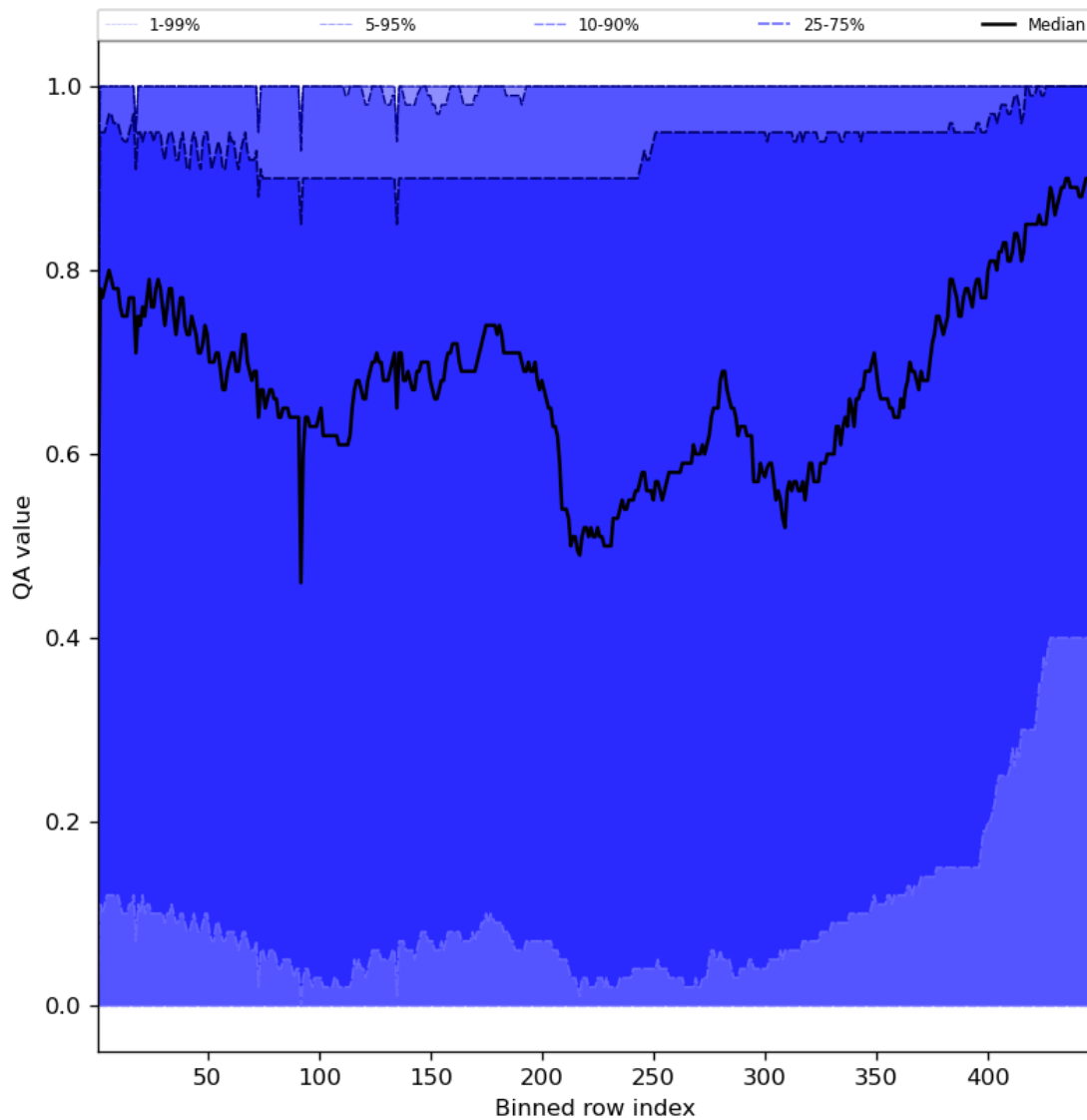
Figure 54: Along track statistics of “QA value” for 2024-01-31 to 2024-02-02
