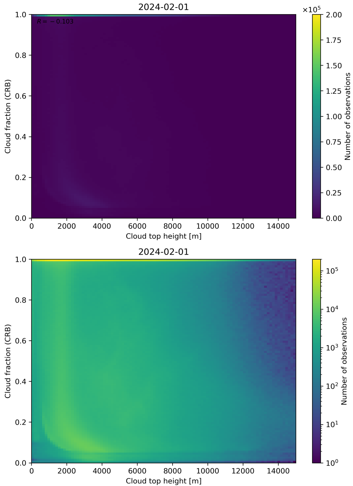
Figure 88: Scatter density plot of “Cloud top height” against “Cloud fraction (CRB)” for 2024-01-31 to 2024-02-02.
