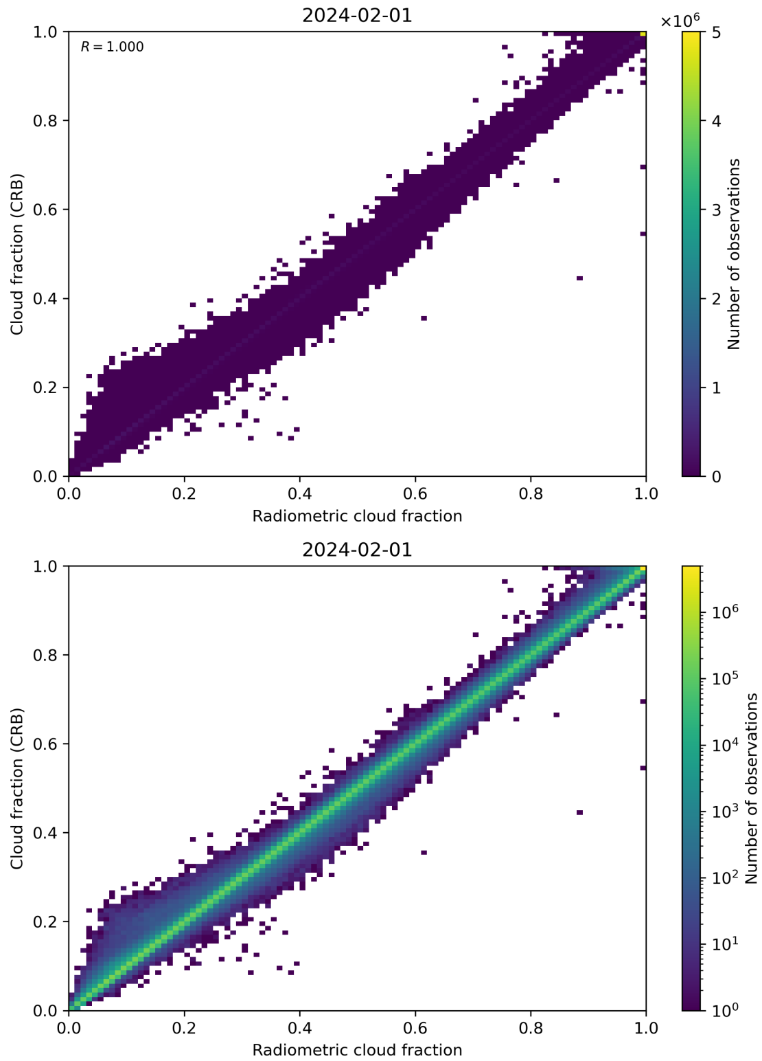
Figure 73: Scatter density plot of “Radiometric cloud fraction” against “Cloud fraction (CRB)” for 2024-01-31 to 2024-02-02.
