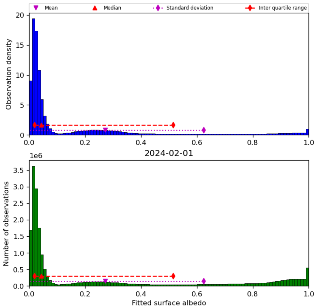
Figure 45: Histogram of “Fitted surface albedo” for 2024-01-31 to 2024-02-02
