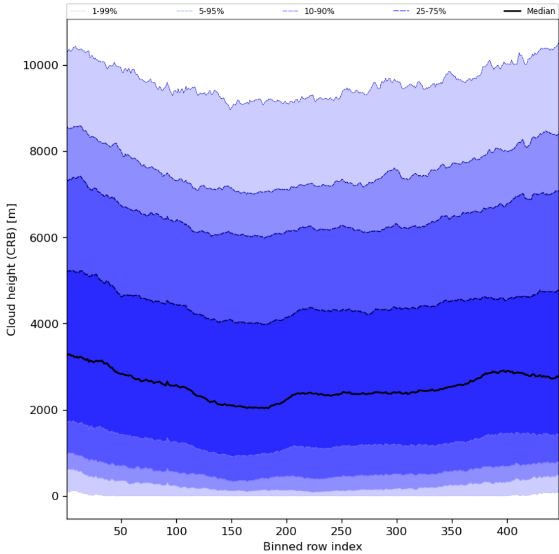
Figure 59: Along track statistics of “Cloud height (CRB)” for 2024-01-31 to 2024-02-02
