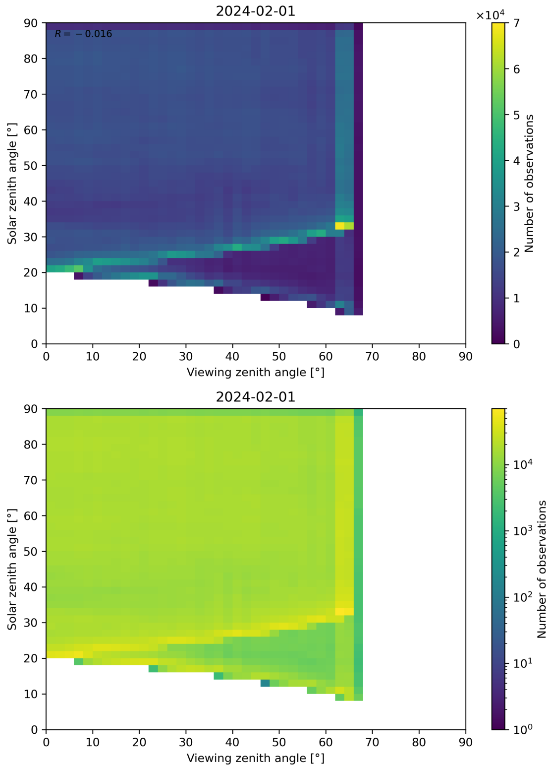
Figure 114: Scatter density plot of “Viewing zenith angle” against “Solar zenith angle” for 2024-01-31 to 2024-02-02.
