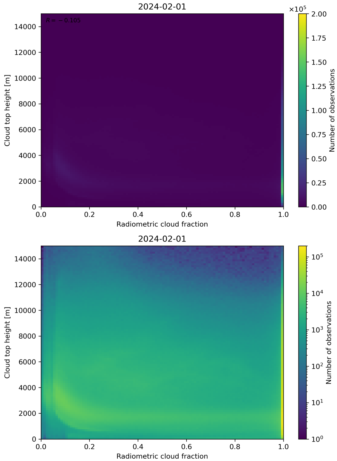
Figure 76: Scatter density plot of “Radiometric cloud fraction” against “Cloud top height” for 2024-01-31 to 2024-02-02.
