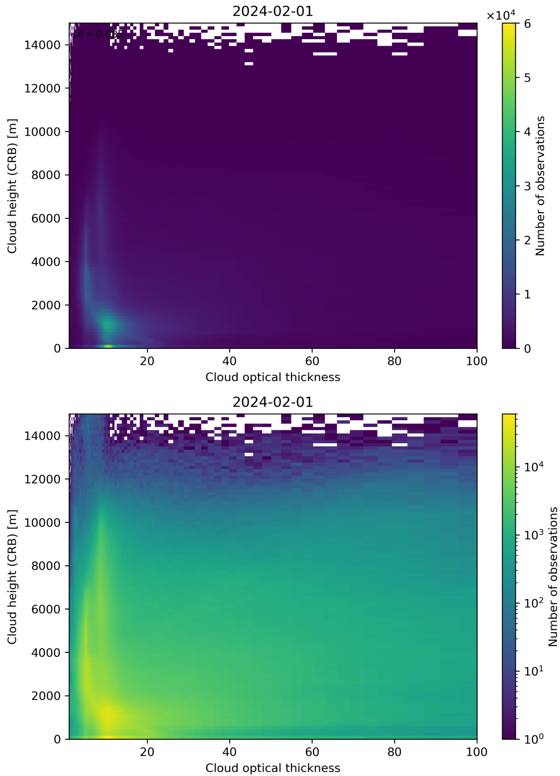
Figure 85: Scatter density plot of “Cloud optical thickness” against “Cloud height (CRB)” for 2024-01-31 to 2024-02-02.
