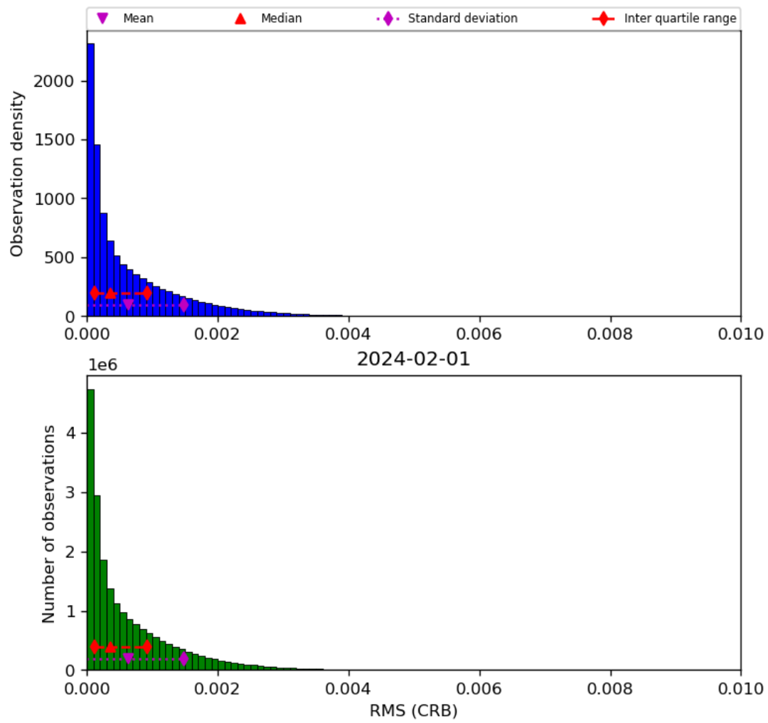
Figure 48: Histogram of “RMS (CRB)” for 2024-01-31 to 2024-02-02
