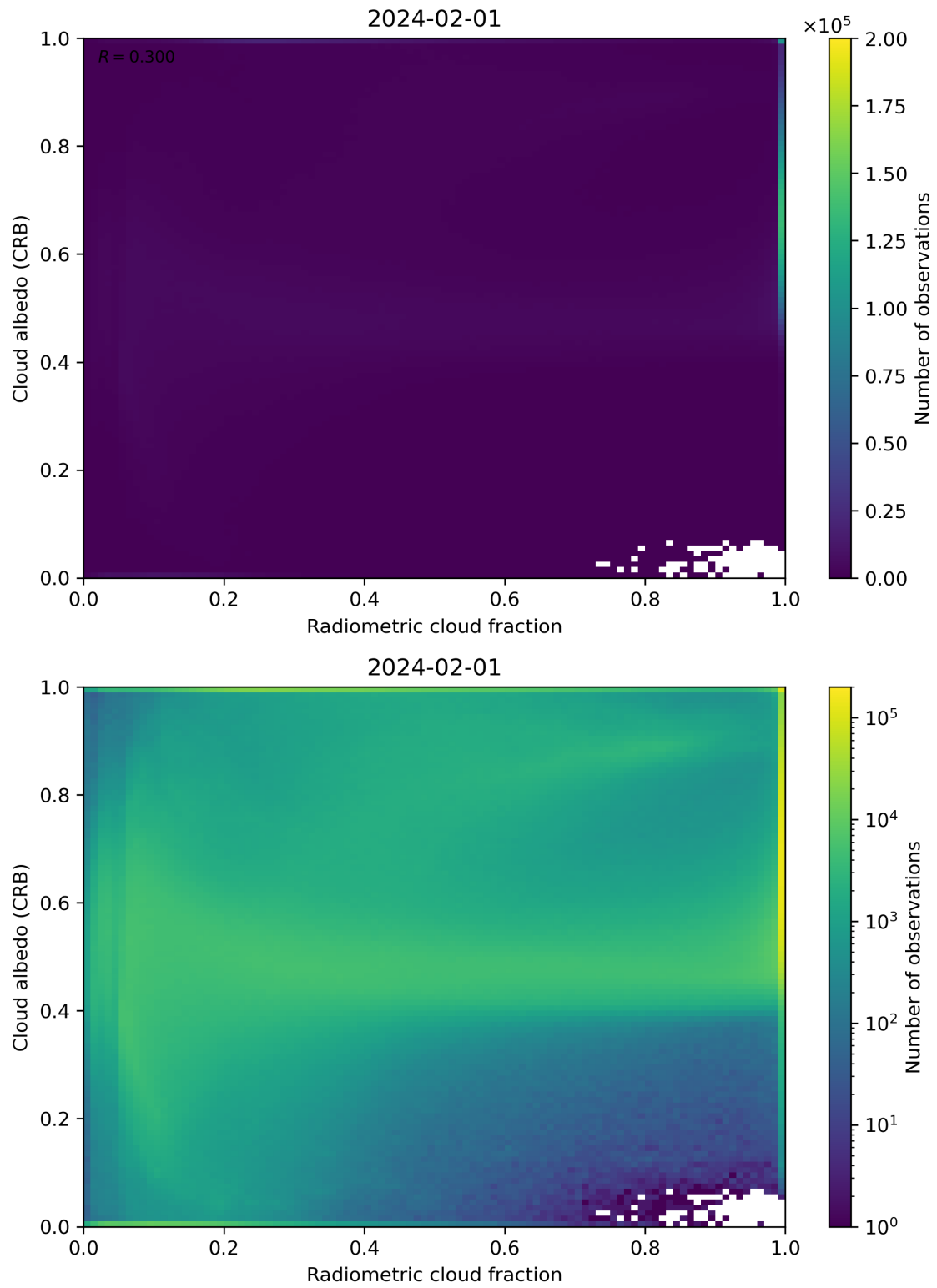
Figure 71: Scatter density plot of “Radiometric cloud fraction” against “Cloud albedo (CRB)” for 2024-01-31 to 2024-02-02.
