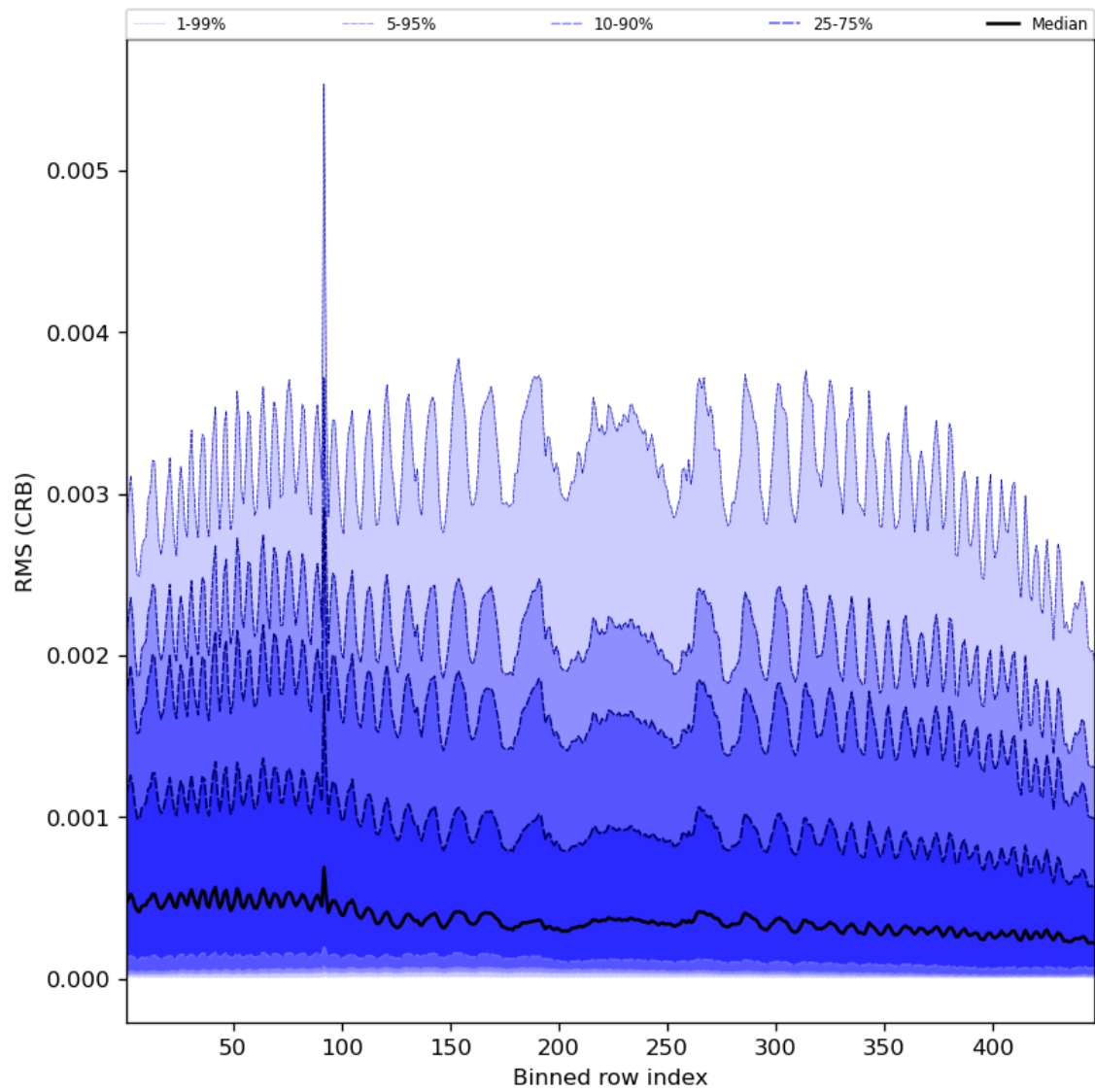
Figure 64: Along track statistics of “RMS (CRB)” for 2024-01-31 to 2024-02-02
