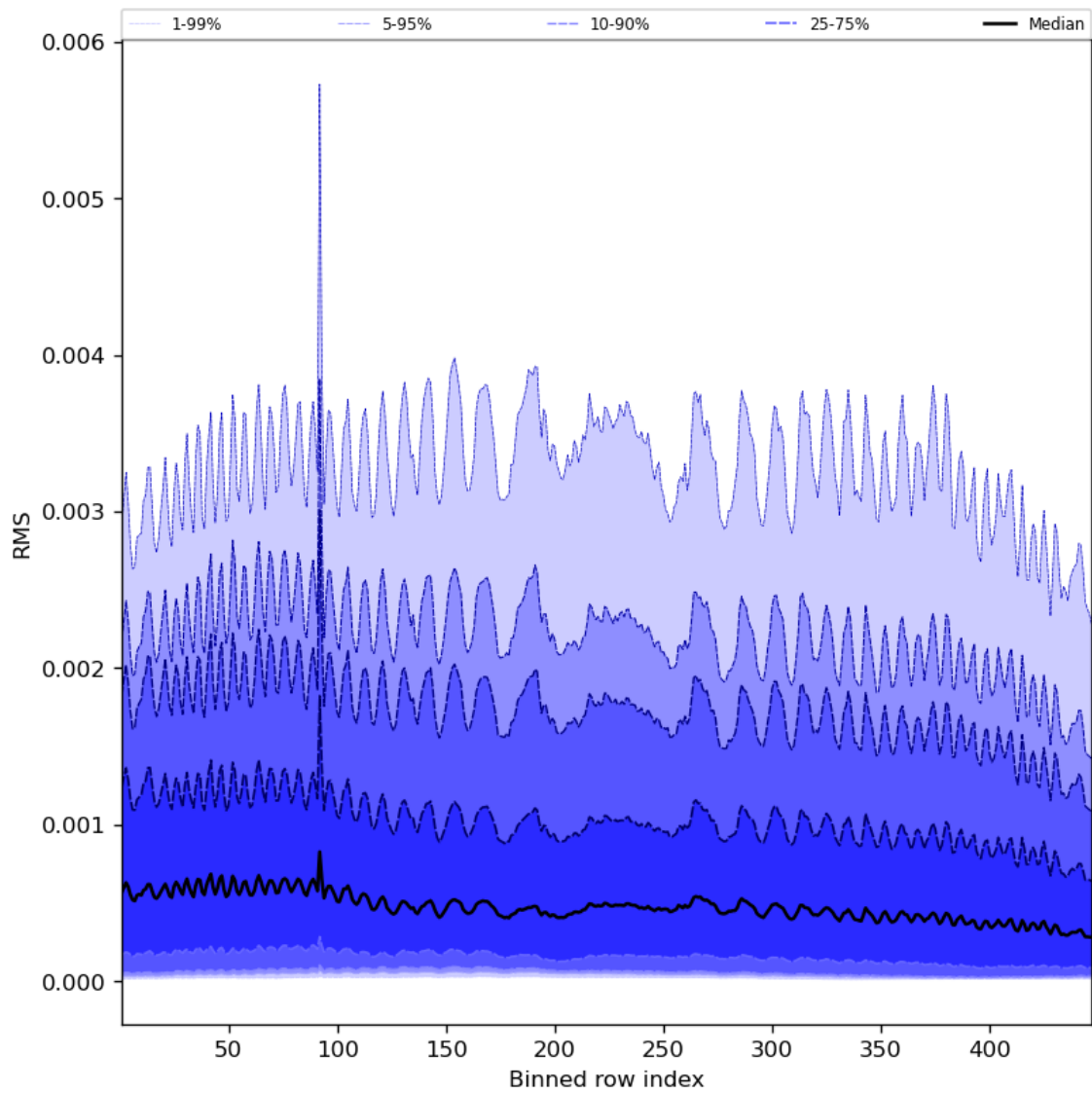
Figure 63: Along track statistics of “RMS” for 2024-01-31 to 2024-02-02
