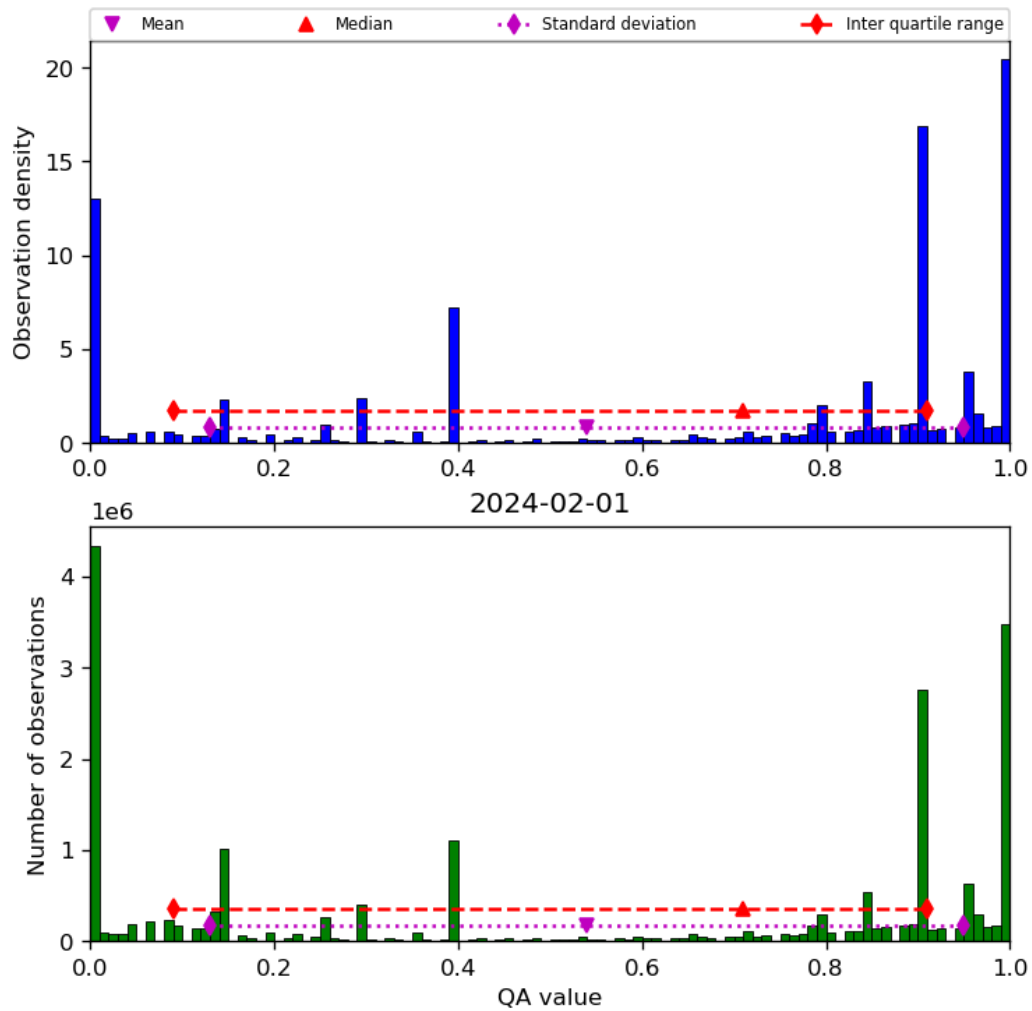
Figure 38: Histogram of “QA value” for 2024-01-31 to 2024-02-02
