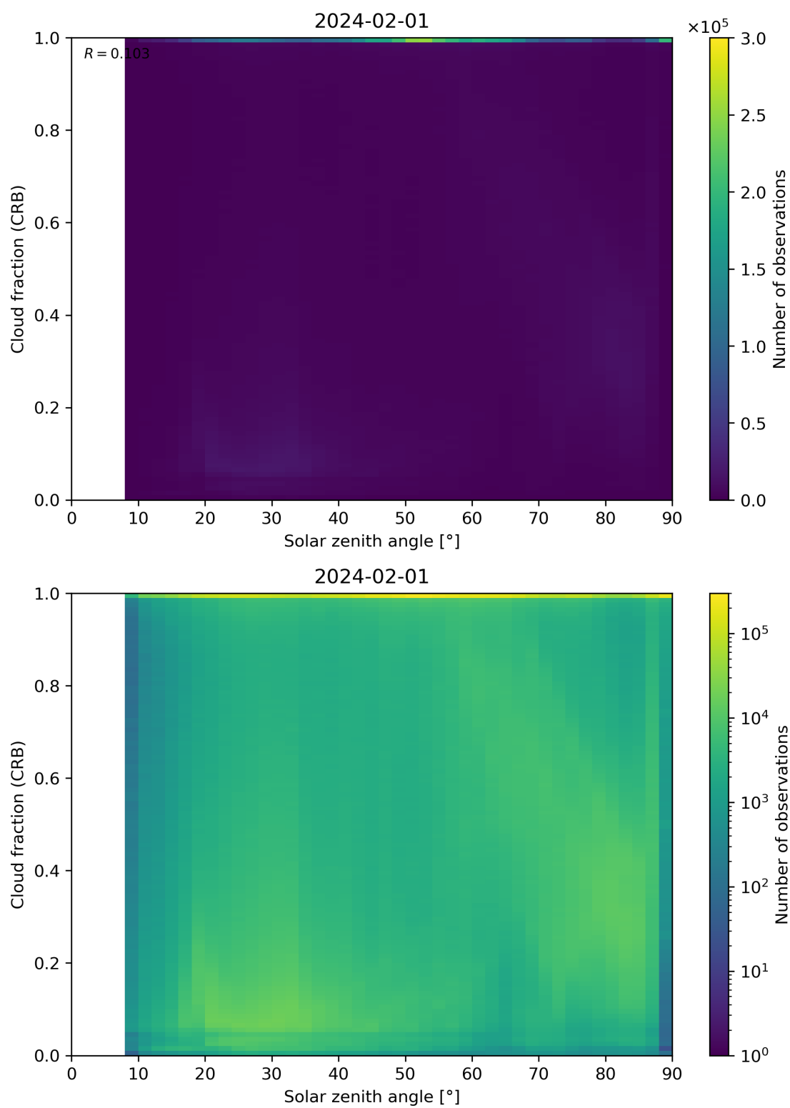
Figure 101: Scatter density plot of “Solar zenith angle” against “Cloud fraction (CRB)” for 2024-01-31 to 2024-02-02.
