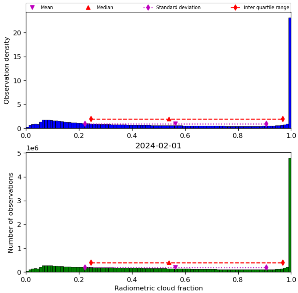
Figure 39: Histogram of “Radiometric cloud fraction” for 2024-01-31 to 2024-02-02
