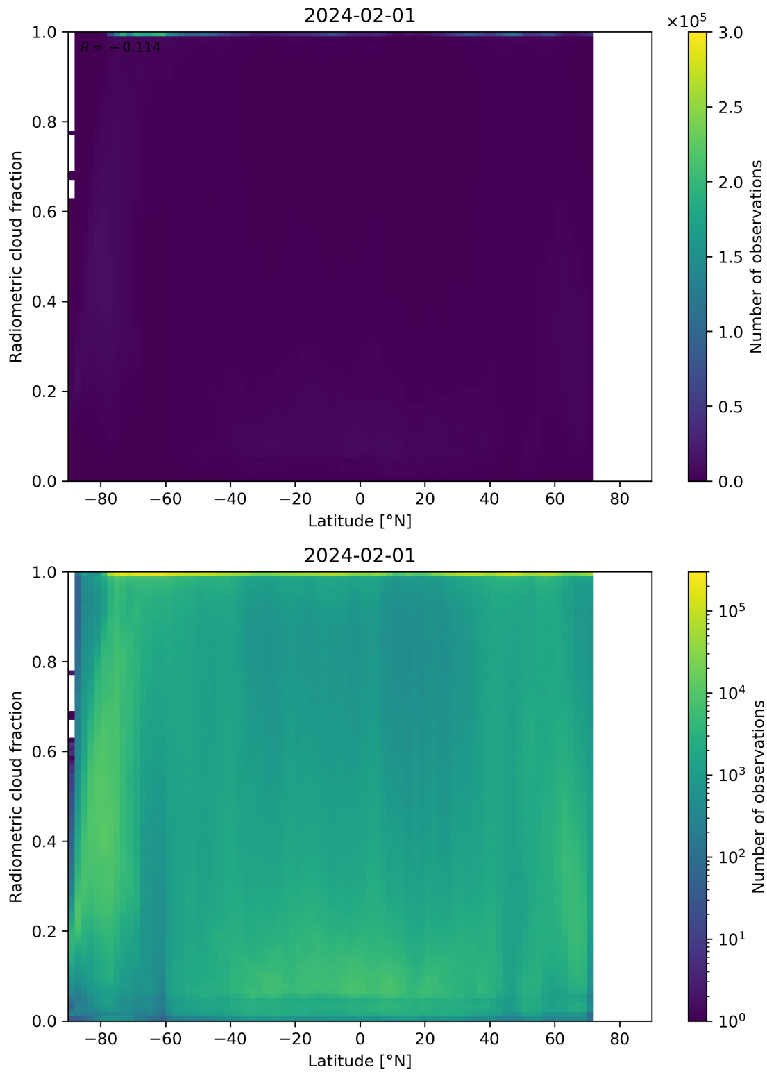
Figure 92: Scatter density plot of “Latitude” against “Radiometric cloud fraction” for 2024-01-31 to 2024-02-02.
