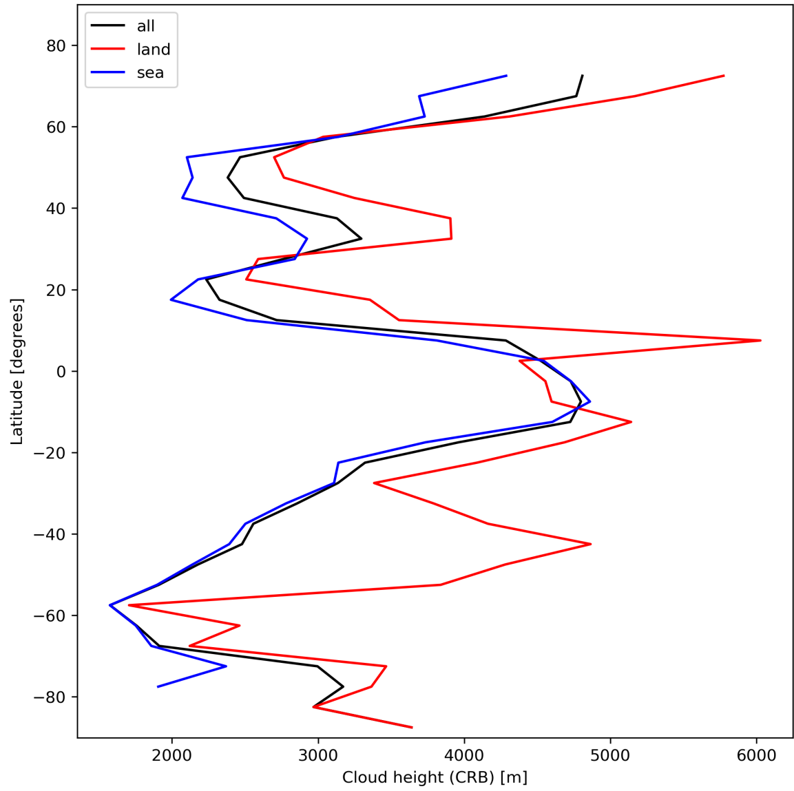
Figure 27: Zonal average of “Cloud height (CRB)” for 2024-01-31 to 2024-02-02.
