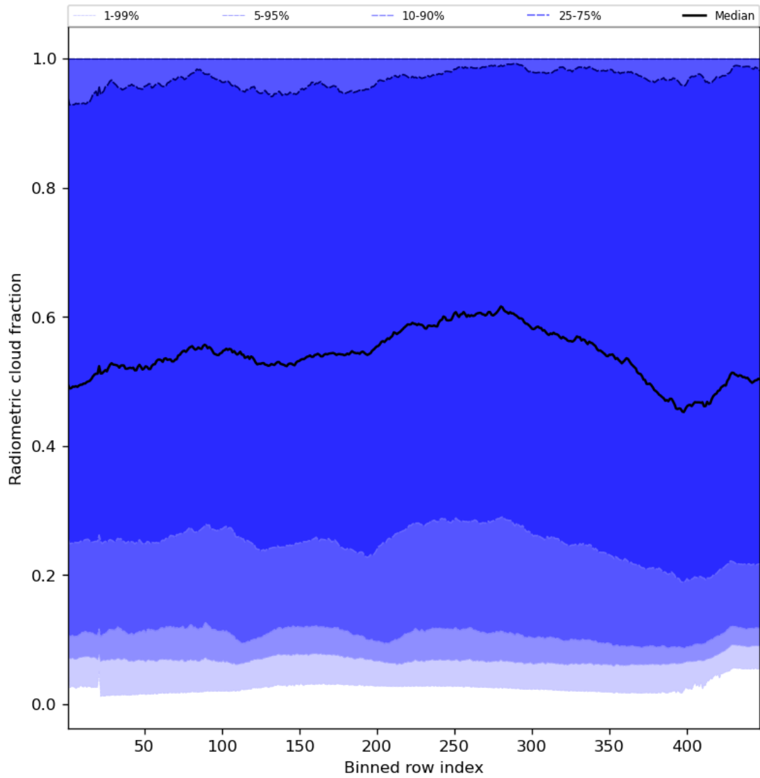
Figure 55: Along track statistics of “Radiometric cloud fraction” for 2024-01-31 to 2024-02-02
