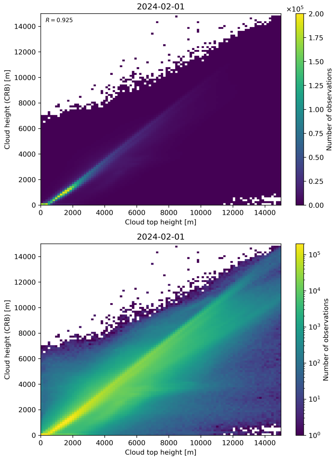
Figure 89: Scatter density plot of “Cloud top height” against “Cloud height (CRB)” for 2024-01-31 to 2024-02-02.
