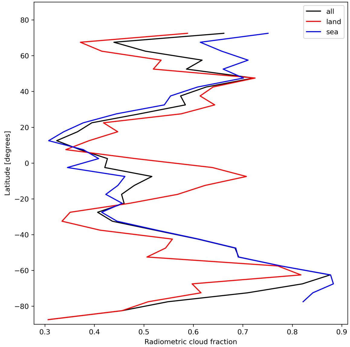
Figure 23: Zonal average of “Radiometric cloud fraction” for 2024-01-31 to 2024-02-02.
