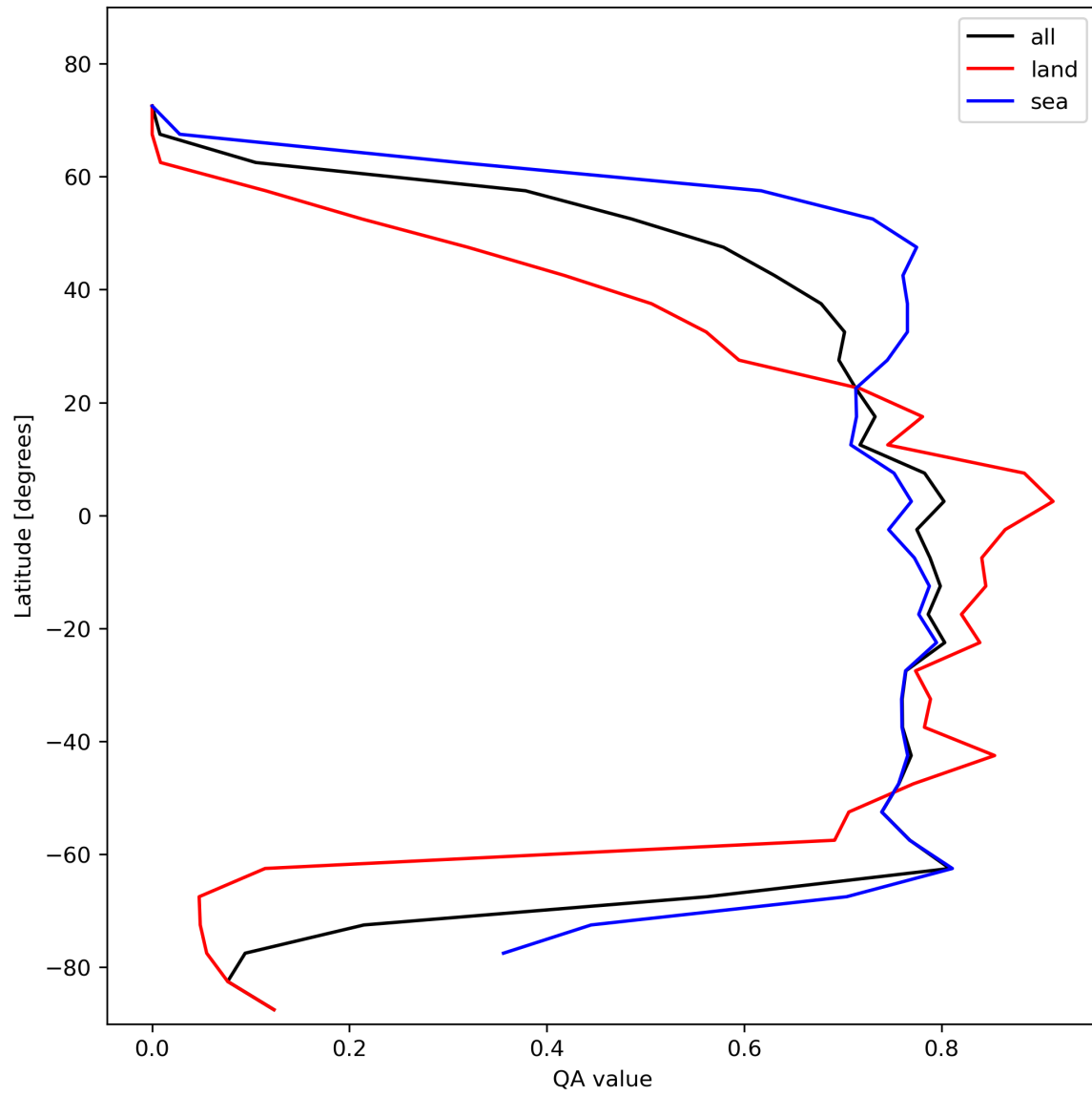
Figure 22: Zonal average of “QA value” for 2024-01-31 to 2024-02-02.
