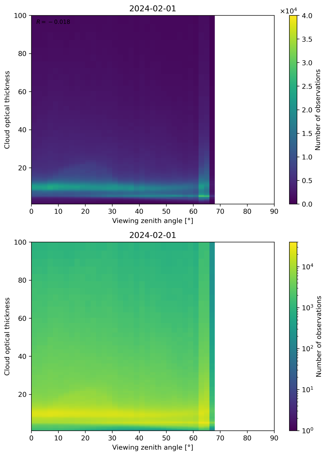
Figure 111: Scatter density plot of “Viewing zenith angle” against “Cloud optical thickness” for 2024-01-31 to 2024-02-02.
