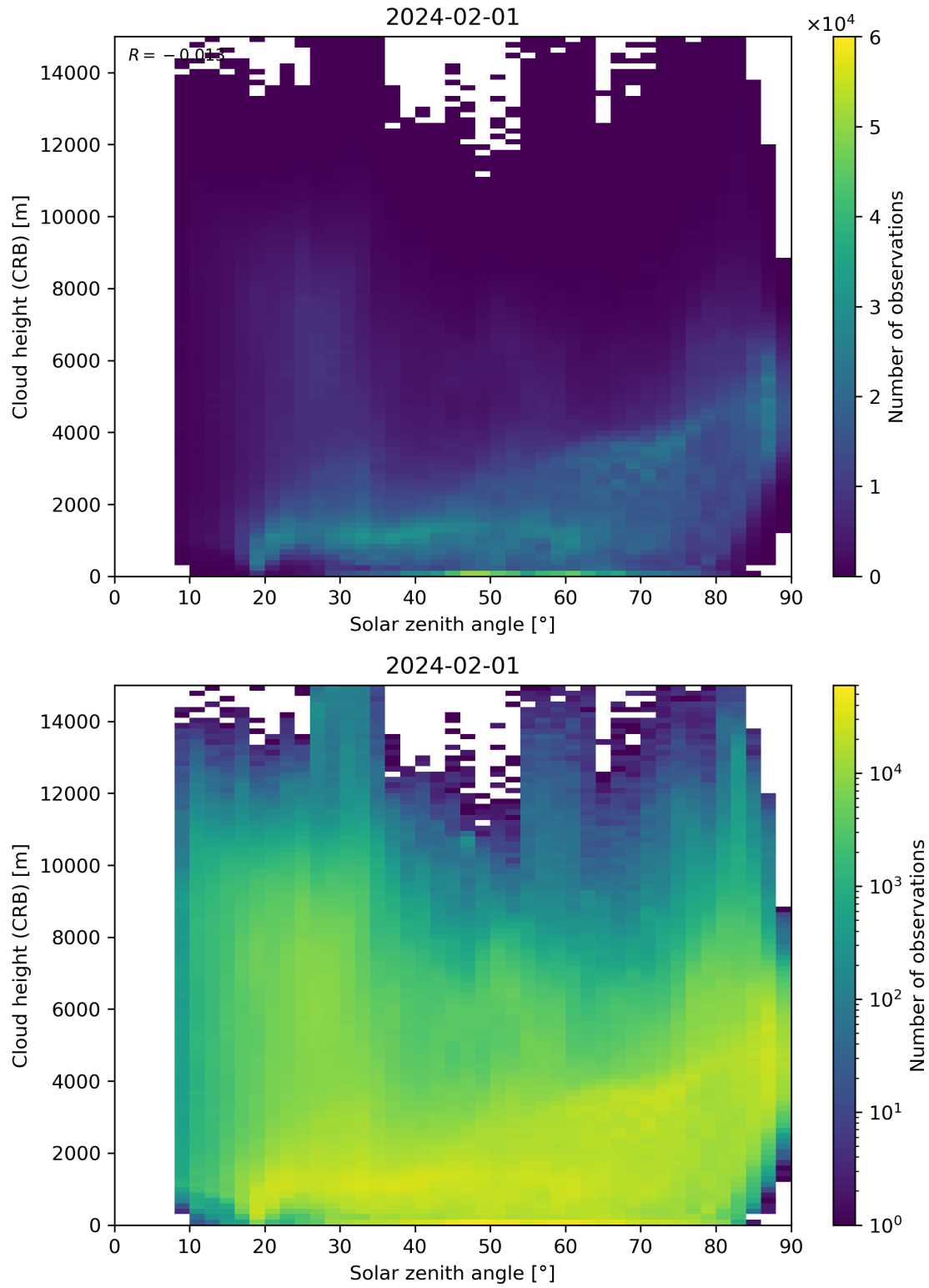
Figure 102: Scatter density plot of “Solar zenith angle” against “Cloud height (CRB)” for 2024-01-31 to 2024-02-02.
