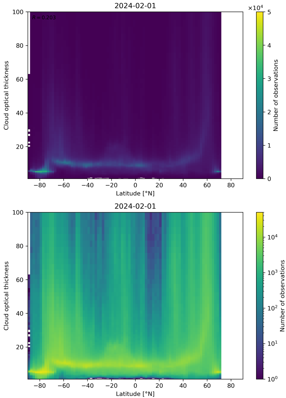
Figure 96: Scatter density plot of “Latitude” against “Cloud optical thickness” for 2024-01-31 to 2024-02-02.
