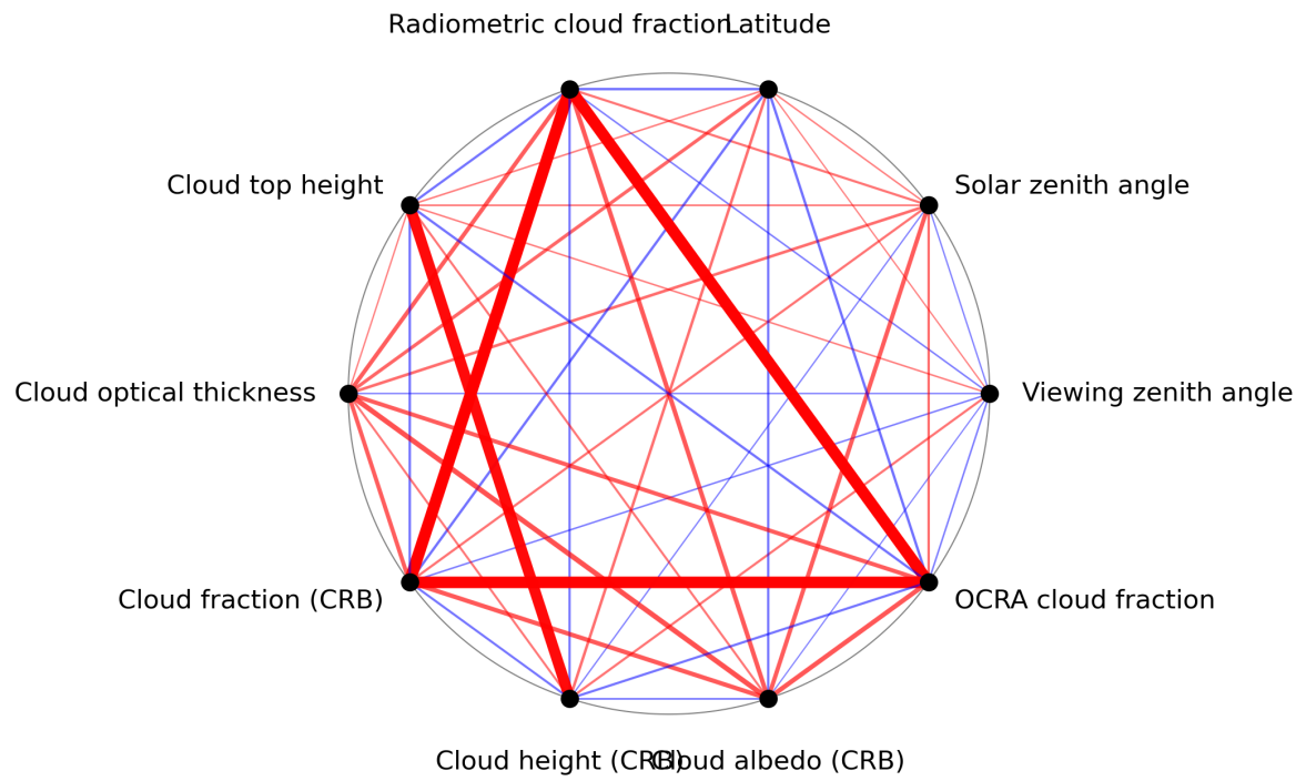
Figure 1: Map of correlation graph for 2024-01-31 to 2024-02-02.
