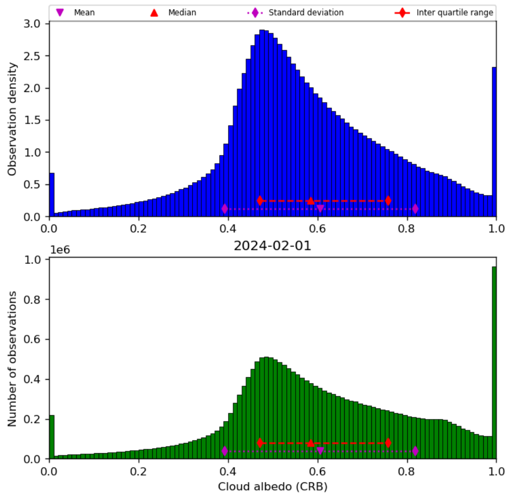
Figure 44: Histogram of “Cloud albedo (CRB)” for 2024-01-31 to 2024-02-02
