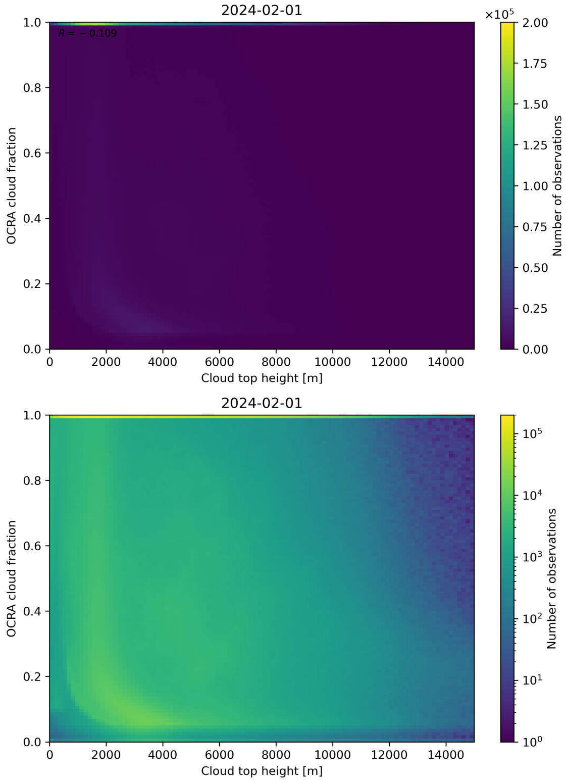
Figure 87: Scatter density plot of “Cloud top height” against “OCRA cloud fraction” for 2024-01-31 to 2024-02-02.
