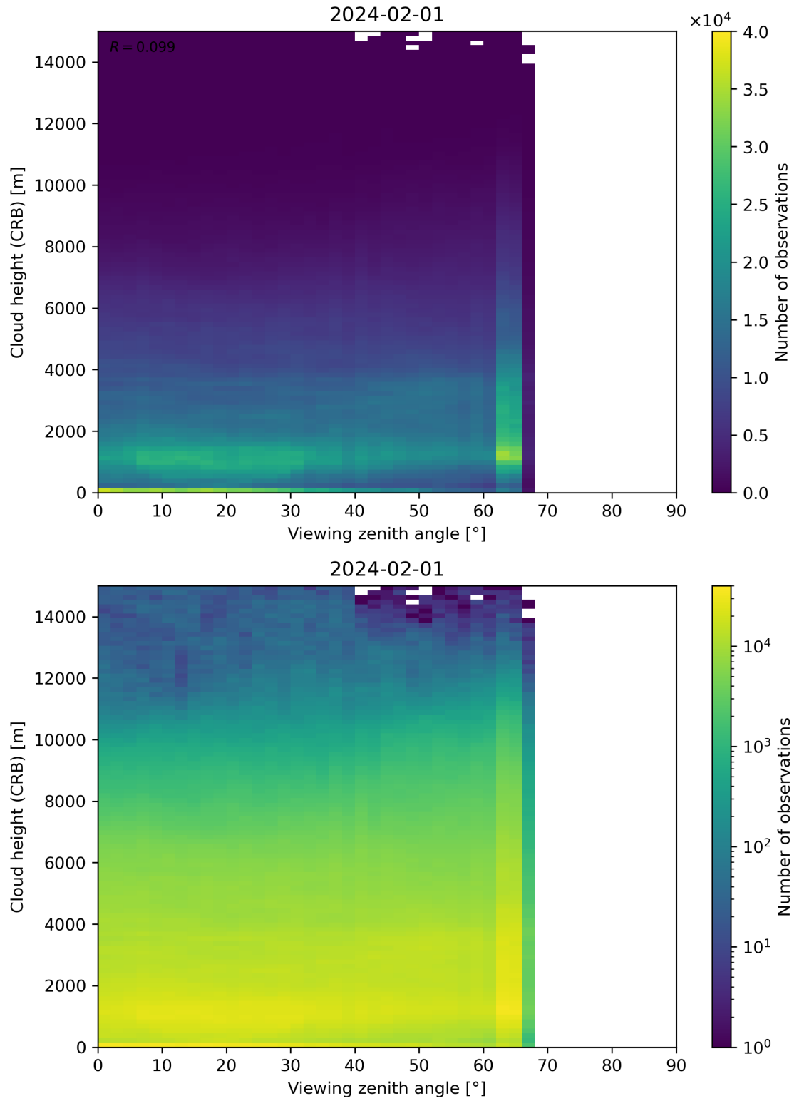
Figure 110: Scatter density plot of “Viewing zenith angle” against “Cloud height (CRB)” for 2024-01-31 to 2024-02-02.
