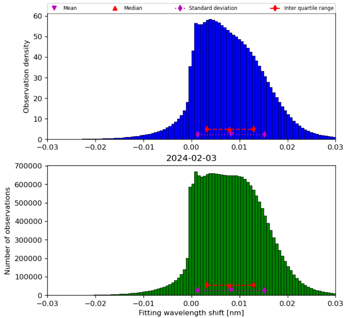
Figure 49: Histogram of “Fitting wavelength shift” for 2024-02-02 to 2024-02-04
