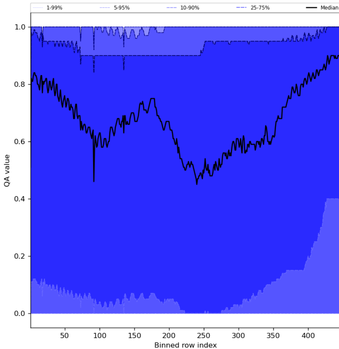
Figure 54: Along track statistics of “QA value” for 2024-02-02 to 2024-02-04
