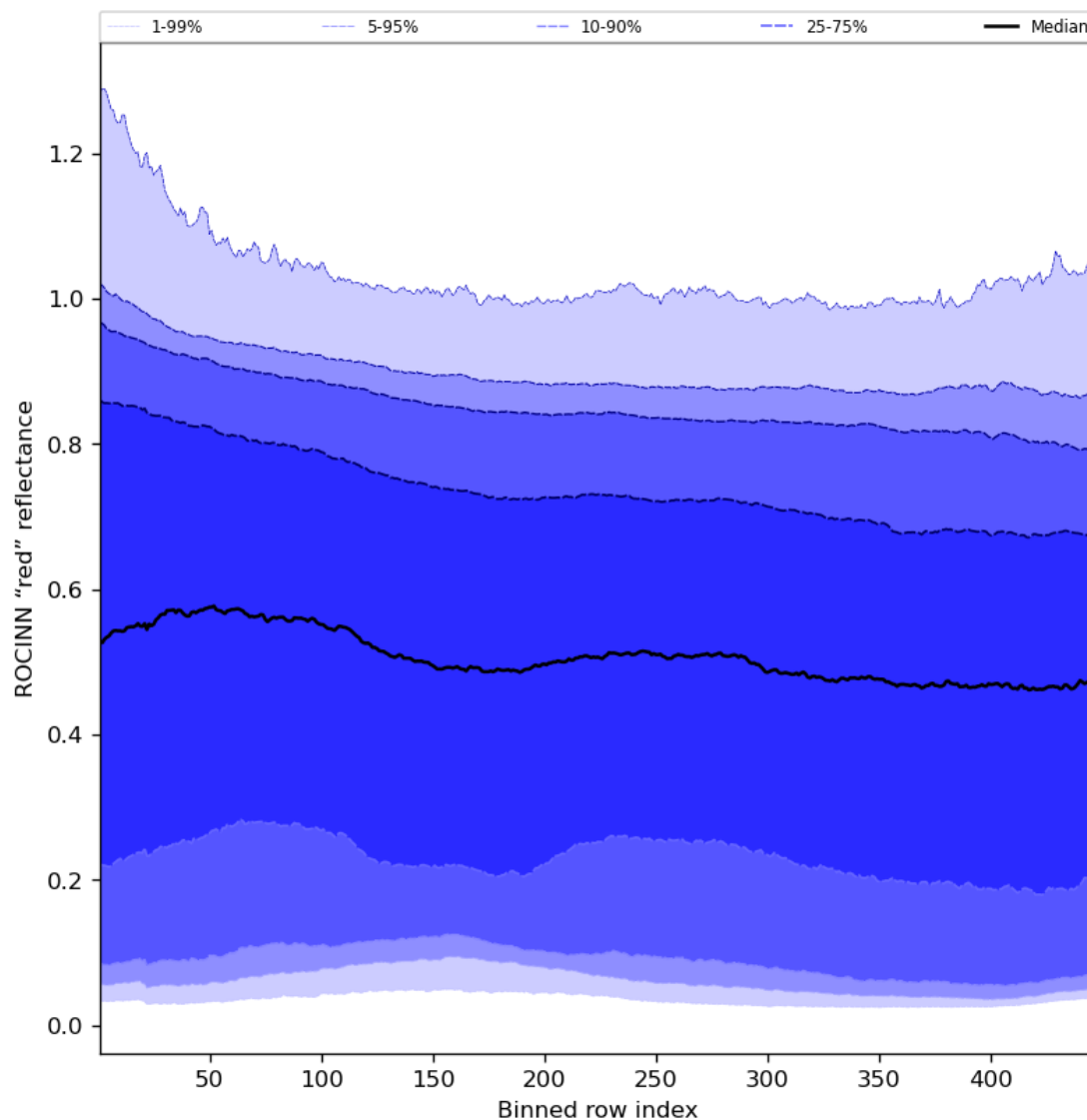
Figure 69: Along track statistics of “ROCINN “red” reflectance” for 2024-02-02 to 2024-02-04
