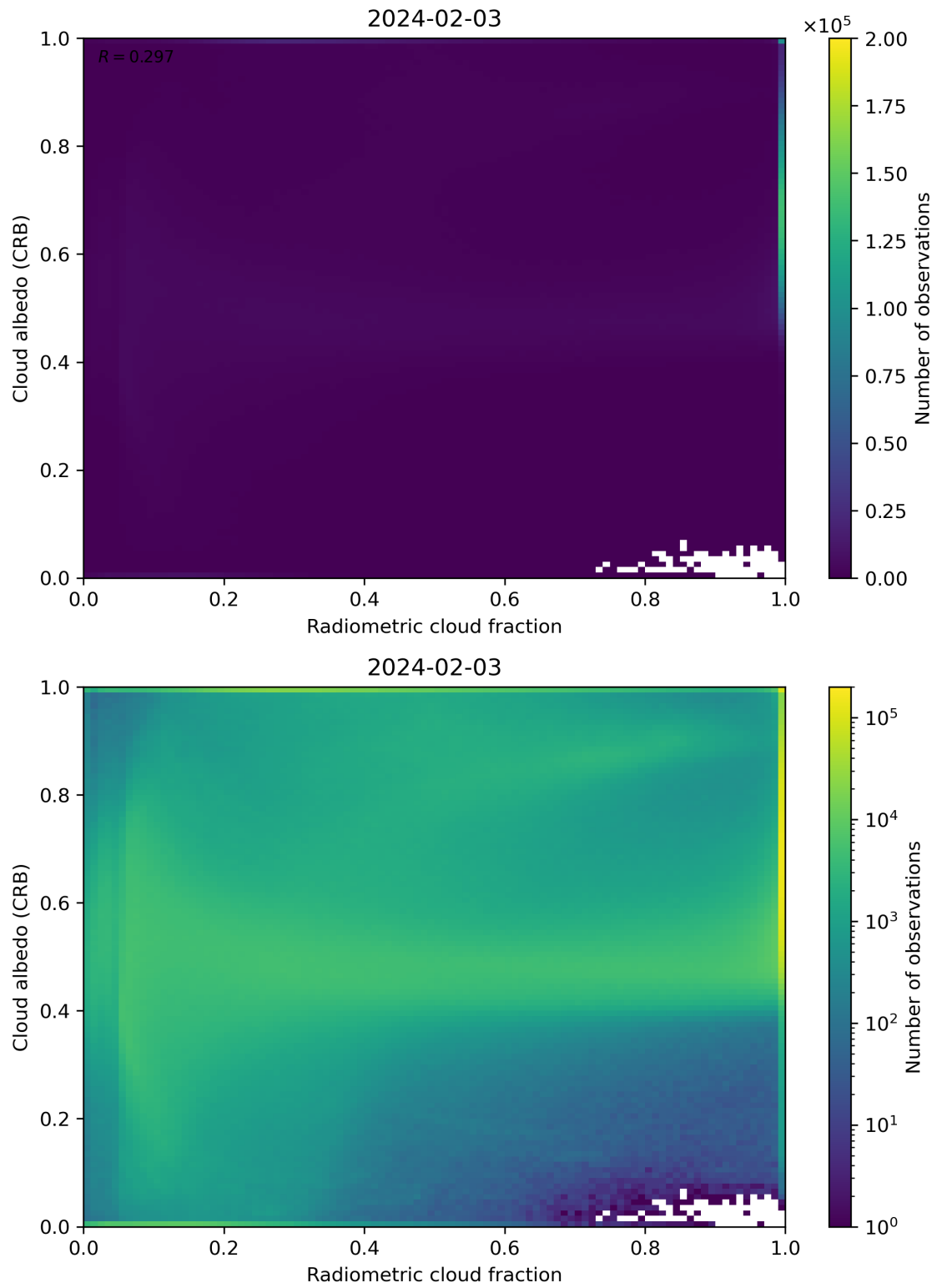
Figure 71: Scatter density plot of “Radiometric cloud fraction” against “Cloud albedo (CRB)” for 2024-02-02 to 2024-02-04.
