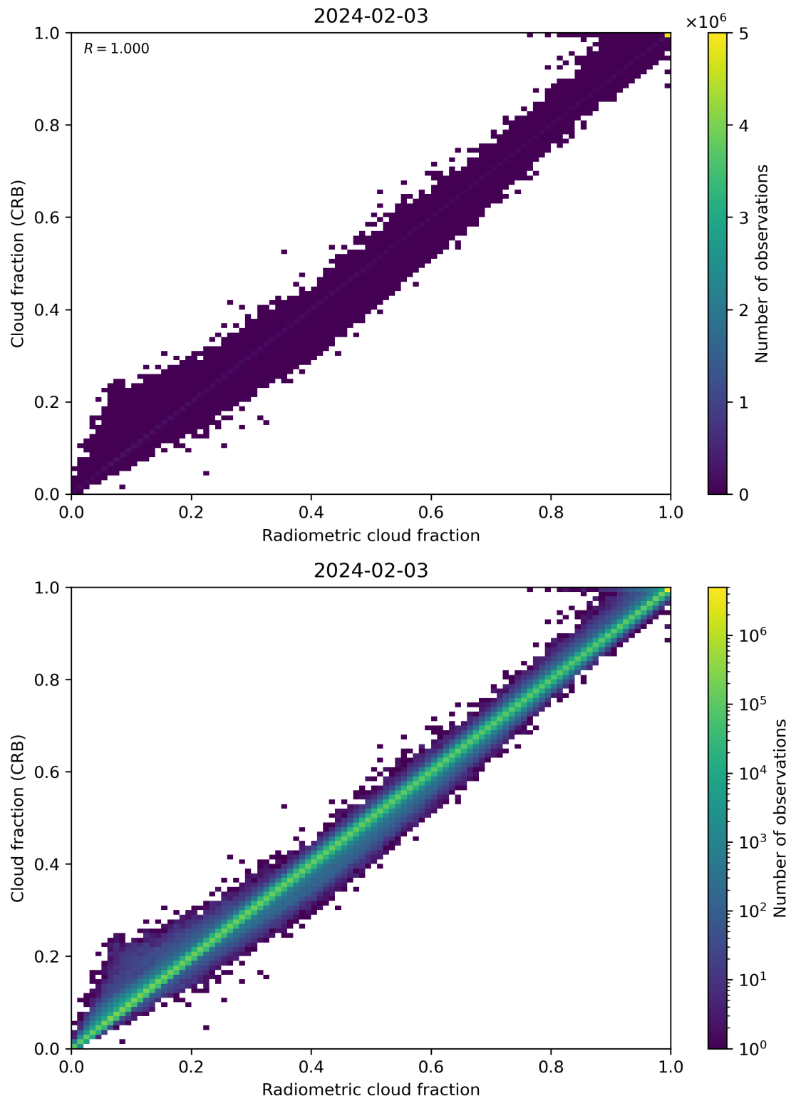
Figure 73: Scatter density plot of “Radiometric cloud fraction” against “Cloud fraction (CRB)” for 2024-02-02 to 2024-02-04.
