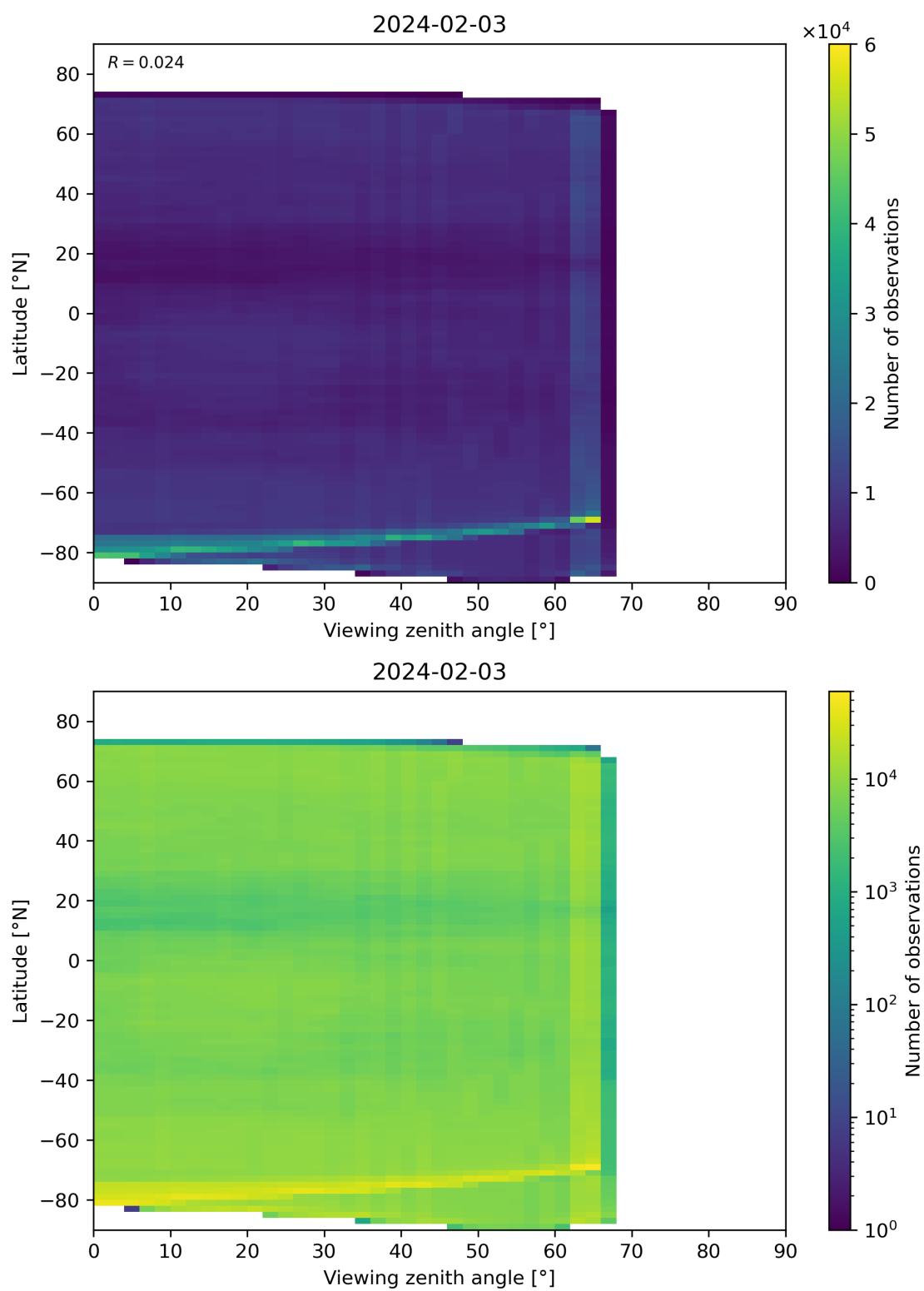
Figure 113: Scatter density plot of “Viewing zenith angle” against “Latitude” for 2024-02-02 to 2024-02-04.
