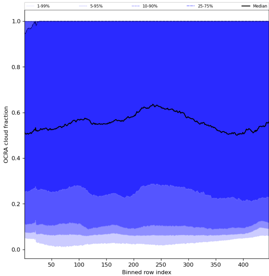
Figure 66: Along track statistics of “OCRA cloud fraction” for 2024-02-02 to 2024-02-04
