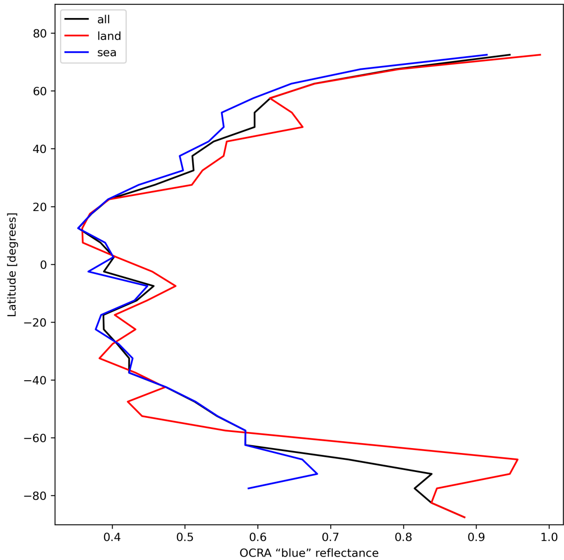
Figure 35: Zonal average of “OCRA “blue” reflectance” for 2024-02-02 to 2024-02-04.
