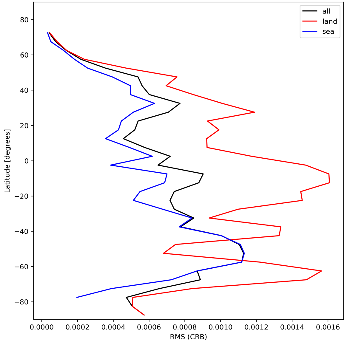
Figure 32: Zonal average of “RMS (CRB)” for 2024-02-02 to 2024-02-04.
