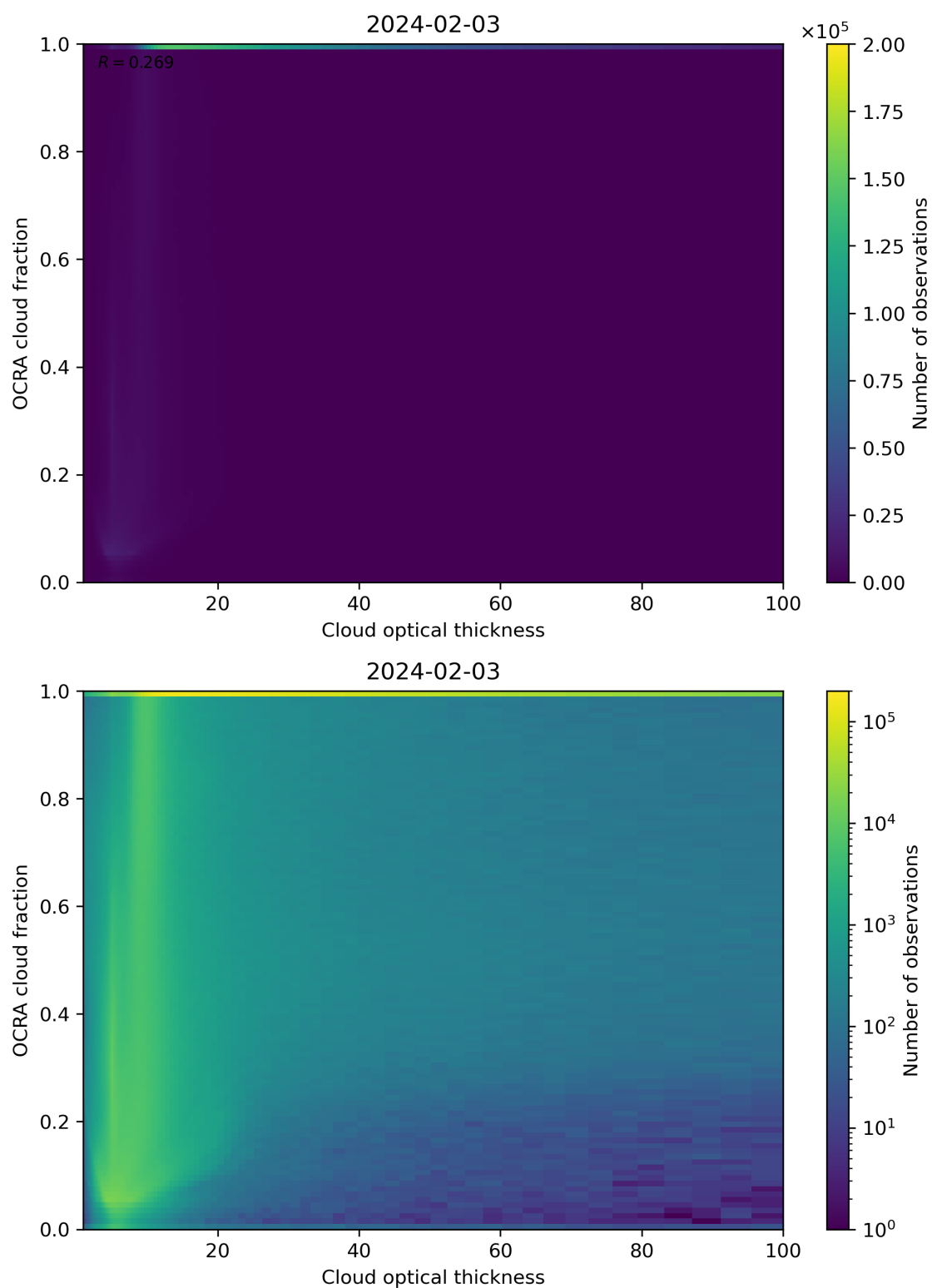
Figure 83: Scatter density plot of “Cloud optical thickness” against “OCRA cloud fraction” for 2024-02-02 to 2024-02-04.
