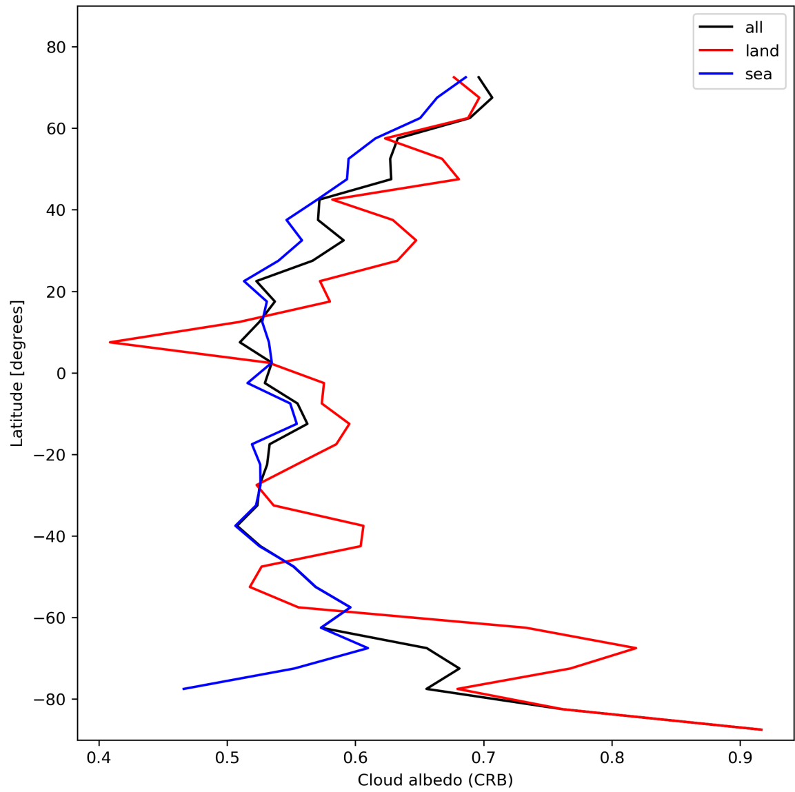
Figure 28: Zonal average of “Cloud albedo (CRB)” for 2024-02-02 to 2024-02-04.
