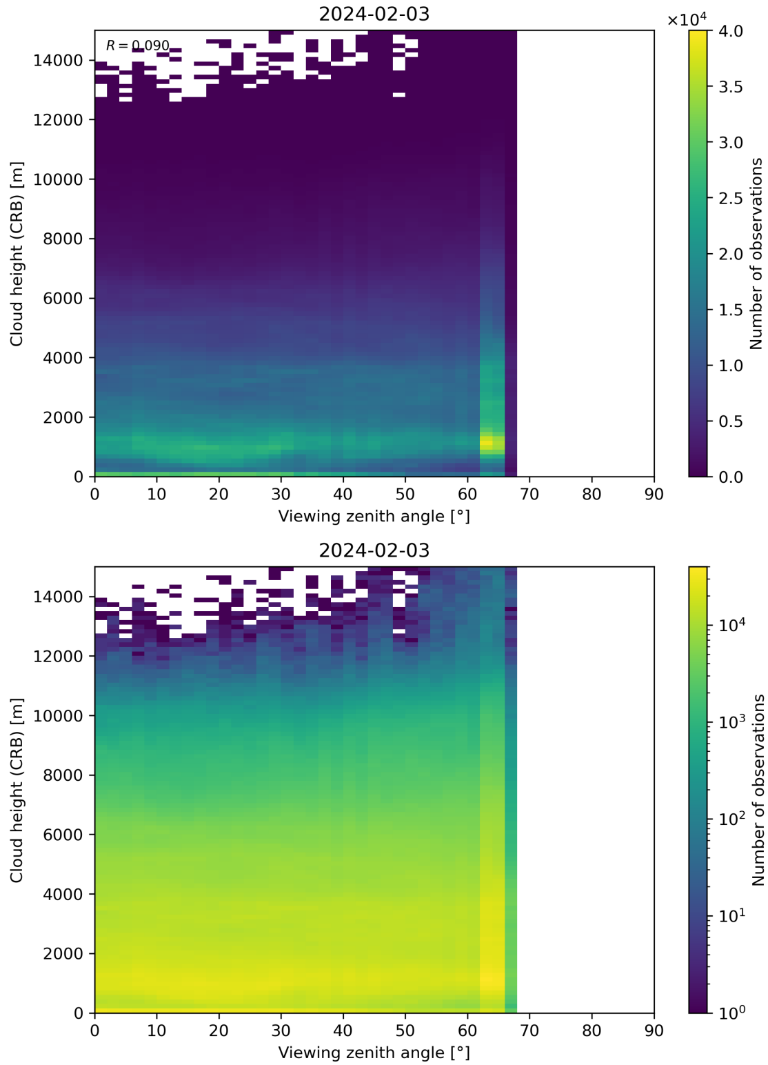
Figure 110: Scatter density plot of “Viewing zenith angle” against “Cloud height (CRB)” for 2024-02-02 to 2024-02-04.
