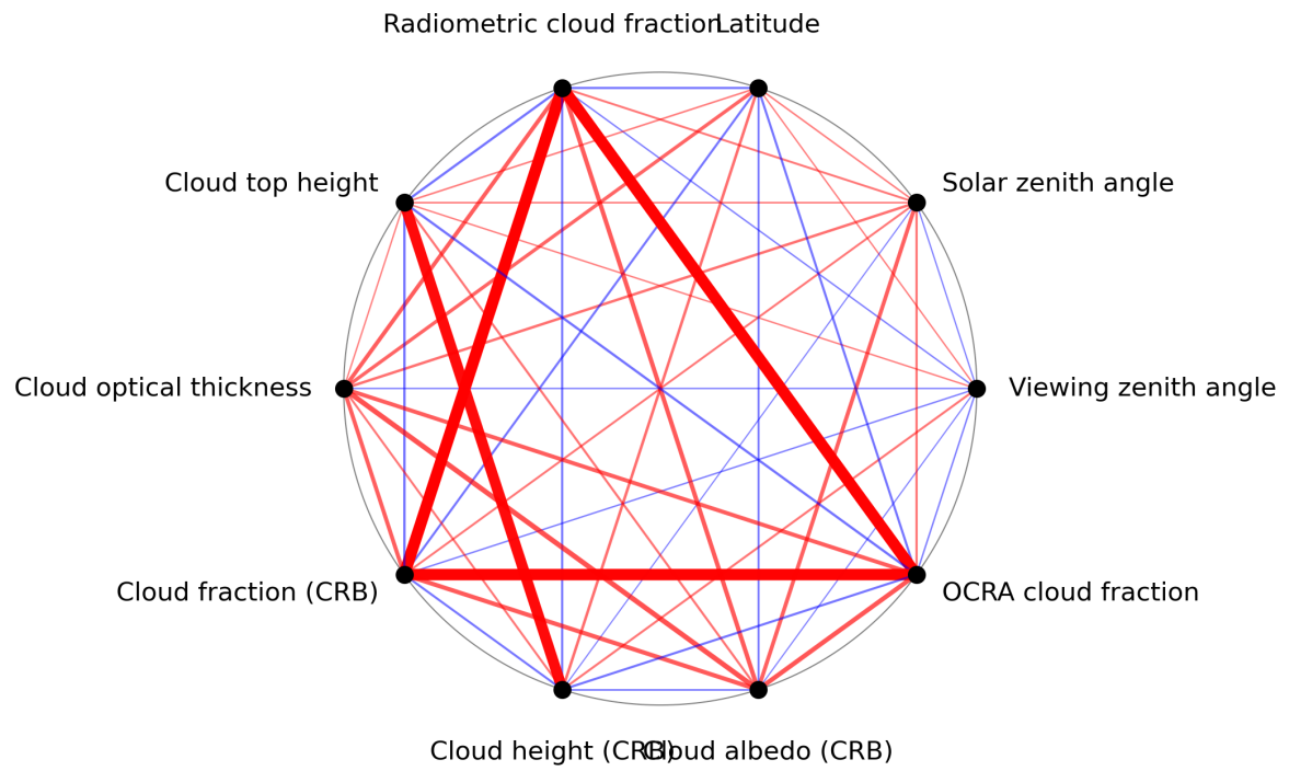
Figure 1: Map of correlation graph for 2024-02-02 to 2024-02-04.
