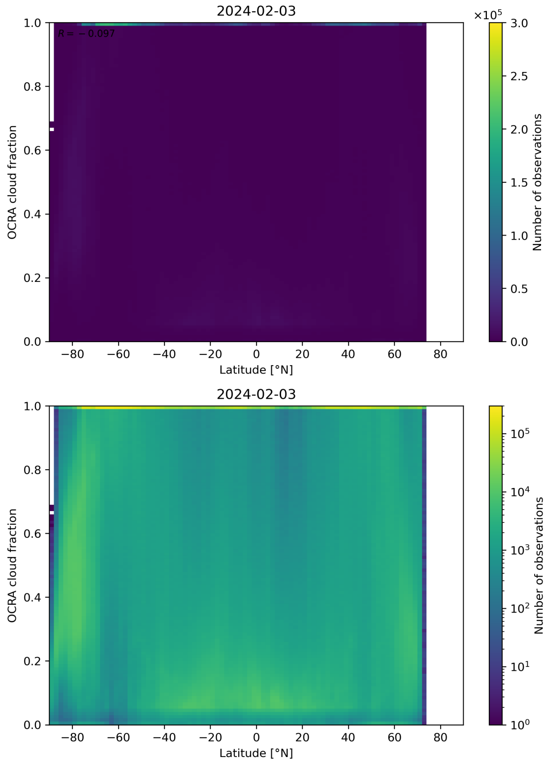
Figure 93: Scatter density plot of “Latitude” against “OCRA cloud fraction” for 2024-02-02 to 2024-02-04.
