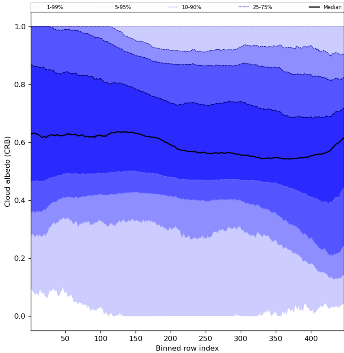
Figure 60: Along track statistics of “Cloud albedo (CRB)” for 2024-02-02 to 2024-02-04
