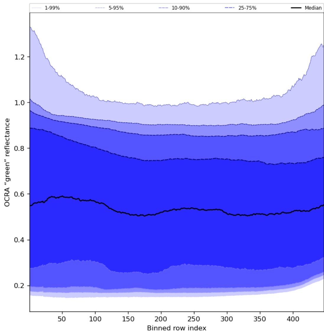
Figure 68: Along track statistics of “OCRA “green” reflectance” for 2024-02-02 to 2024-02-04
