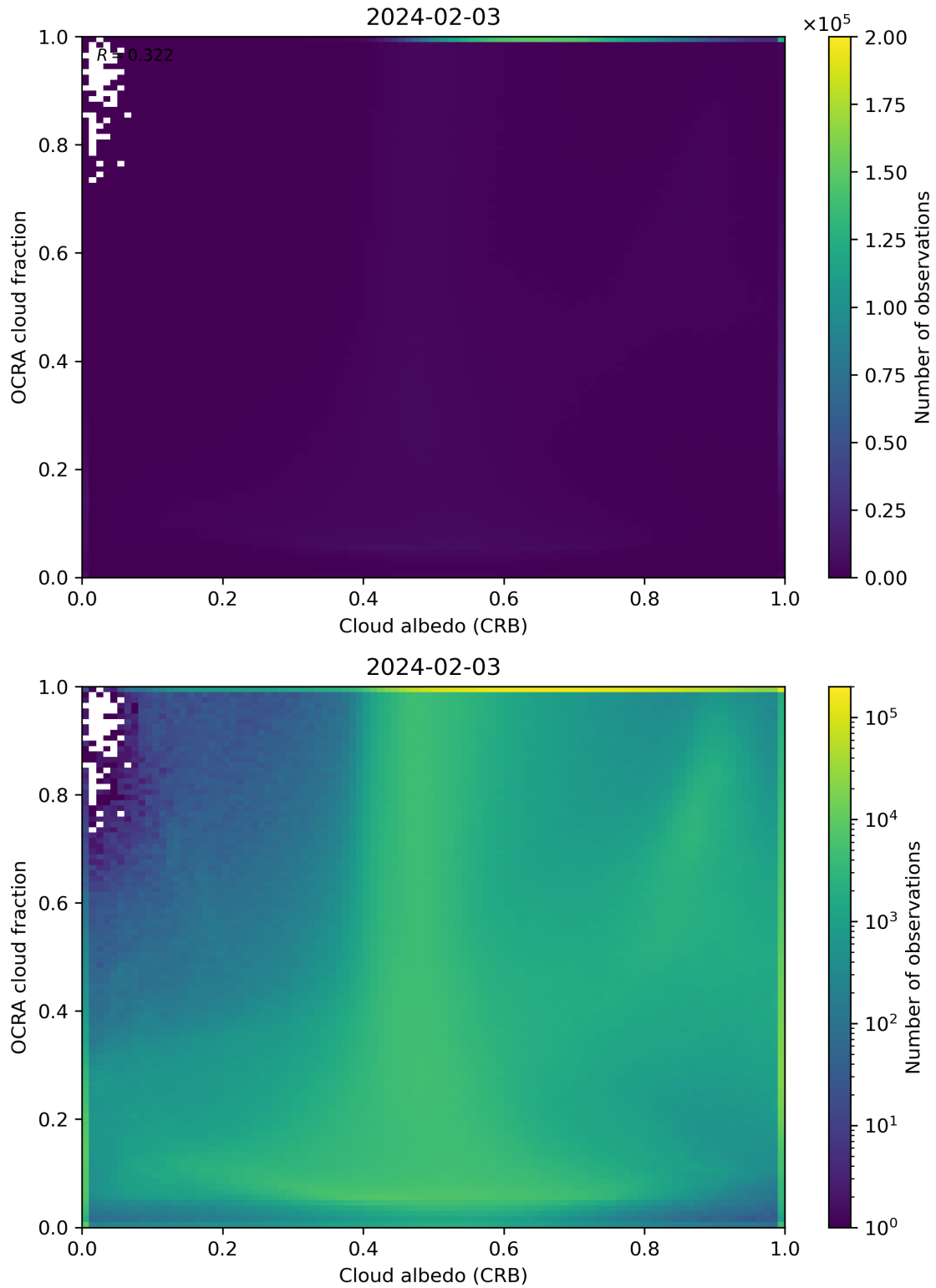
Figure 70: Scatter density plot of “Cloud albedo (CRB)” against “OCRA cloud fraction” for 2024-02-02 to 2024-02-04.
