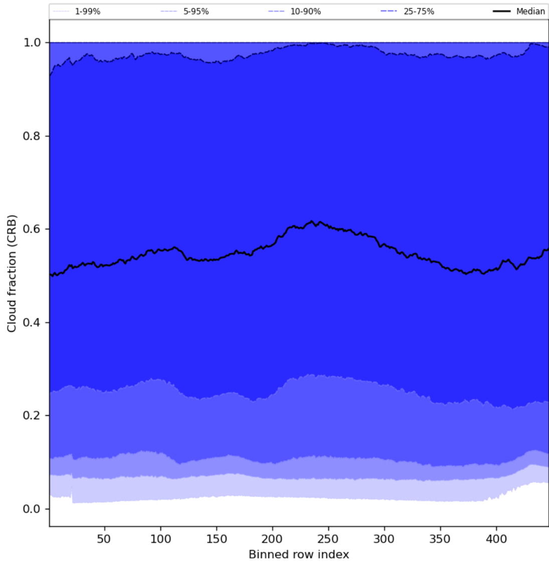
Figure 58: Along track statistics of “Cloud fraction (CRB)” for 2024-02-02 to 2024-02-04
