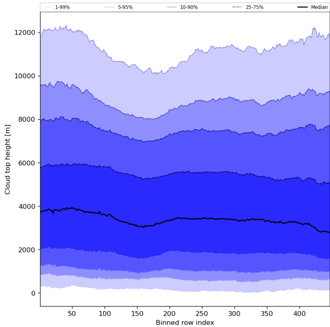
Figure 56: Along track statistics of “Cloud top height” for 2024-02-02 to 2024-02-04
