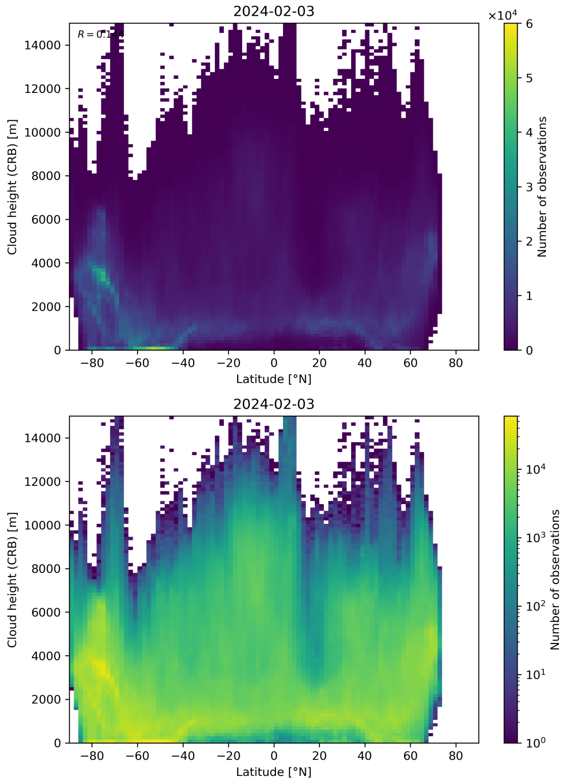
Figure 95: Scatter density plot of “Latitude” against “Cloud height (CRB)” for 2024-02-02 to 2024-02-04.
