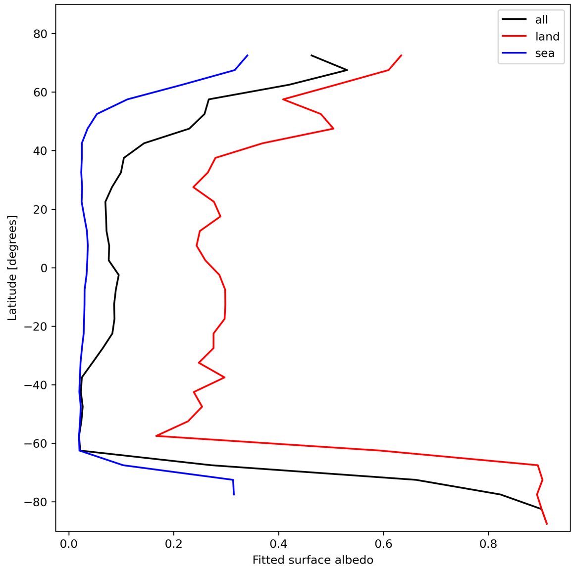
Figure 29: Zonal average of “Fitted surface albedo” for 2024-02-02 to 2024-02-04.
