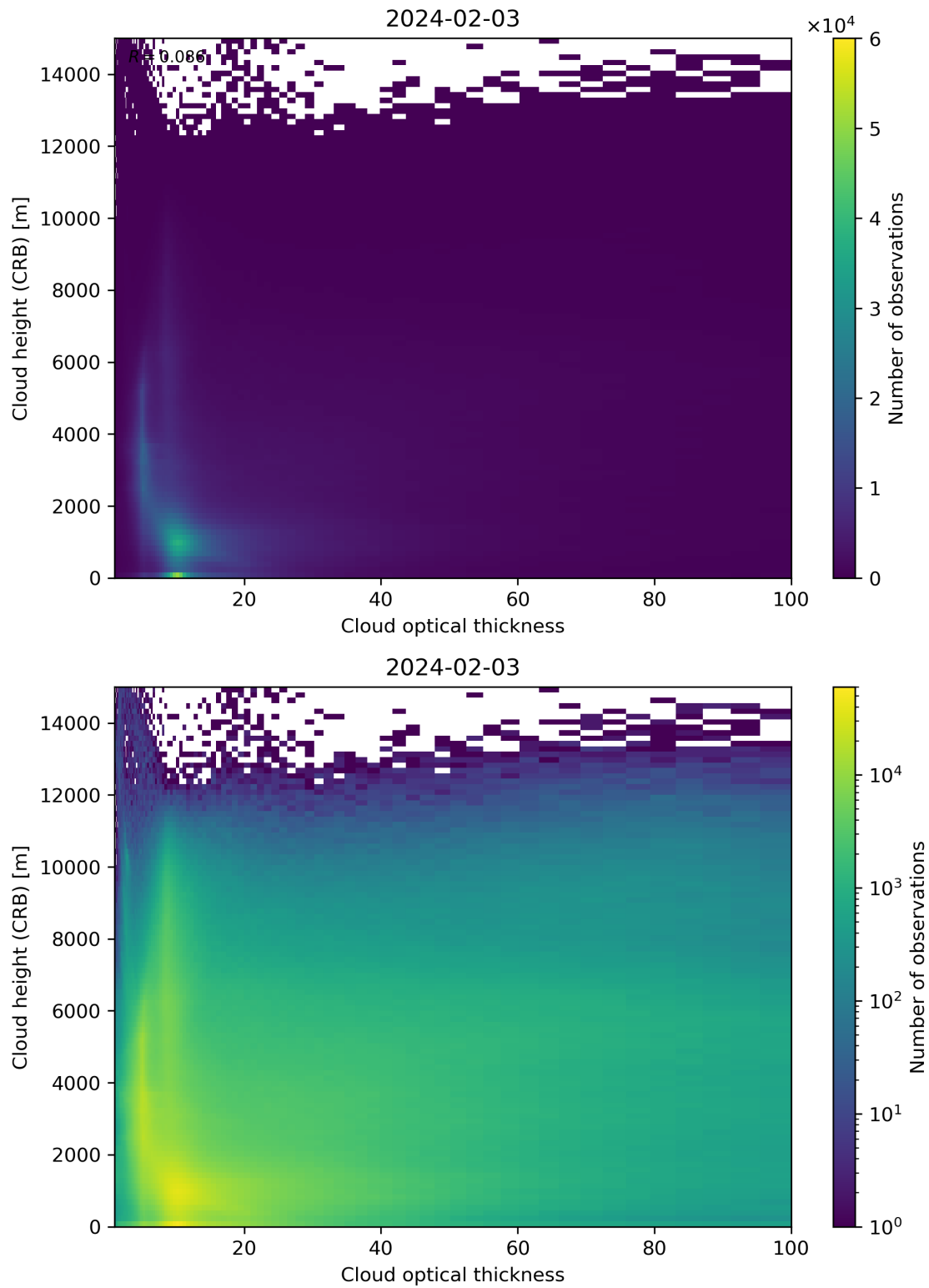
Figure 85: Scatter density plot of “Cloud optical thickness” against “Cloud height (CRB)” for 2024-02-02 to 2024-02-04.
