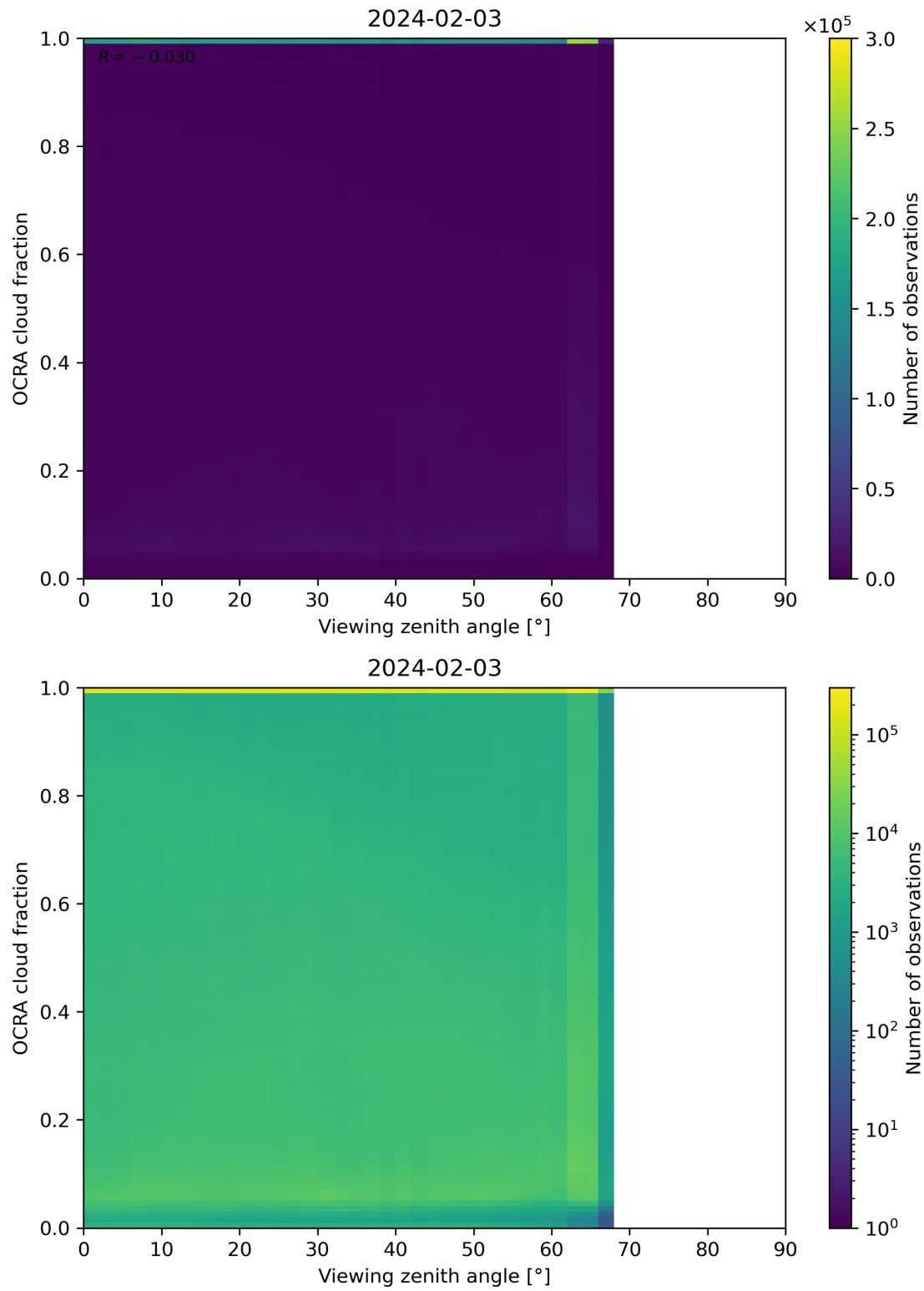
Figure 108: Scatter density plot of “Viewing zenith angle” against “OCRA cloud fraction” for 2024-02-02 to 2024-02-04.
