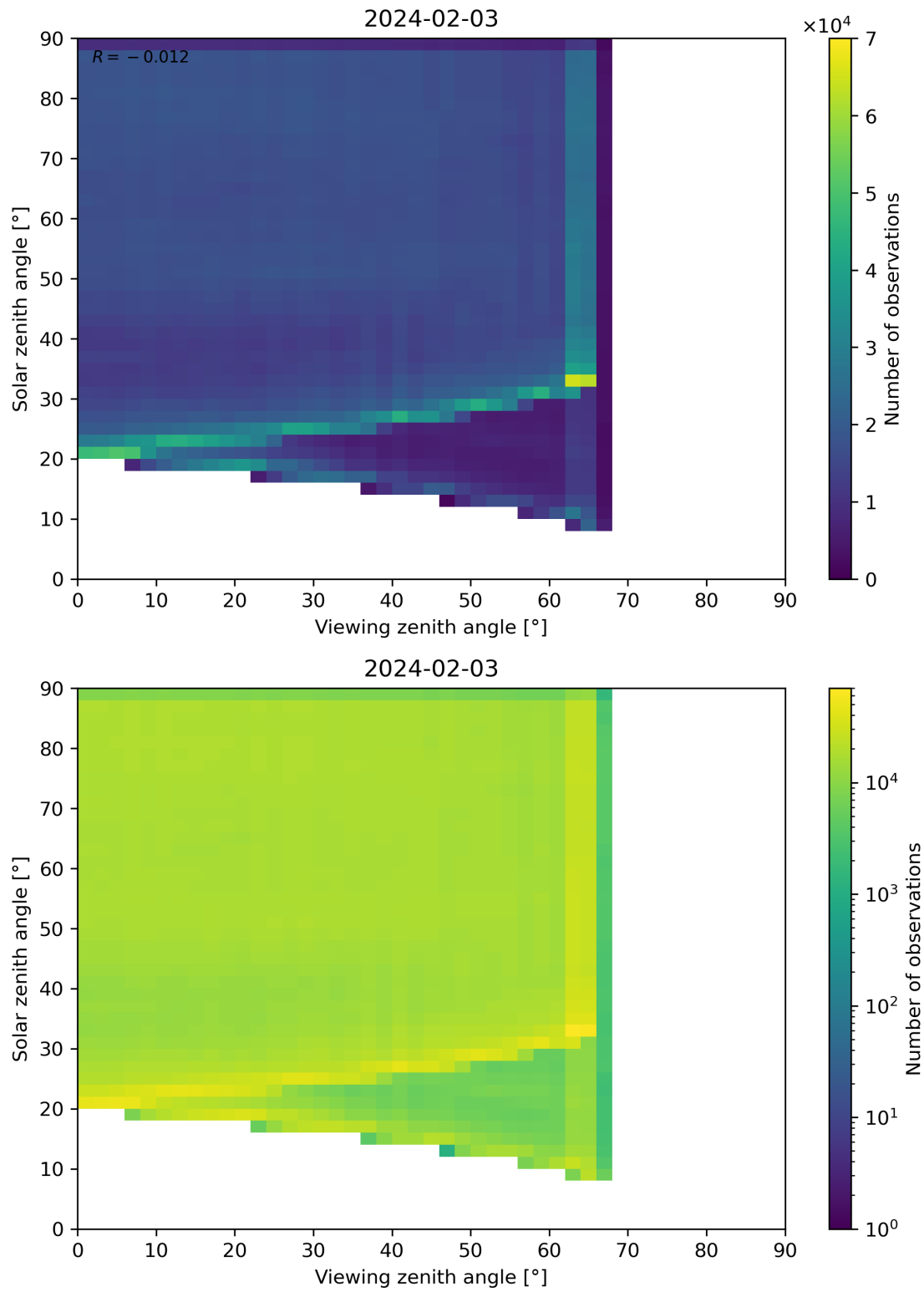
Figure 114: Scatter density plot of “Viewing zenith angle” against “Solar zenith angle” for 2024-02-02 to 2024-02-04.
