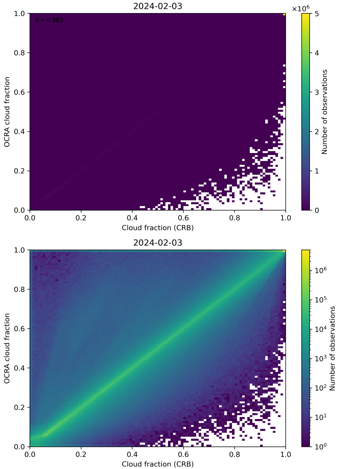
Figure 78: Scatter density plot of “Cloud fraction (CRB)” against “OCRA cloud fraction” for 2024-02-02 to 2024-02-04.
