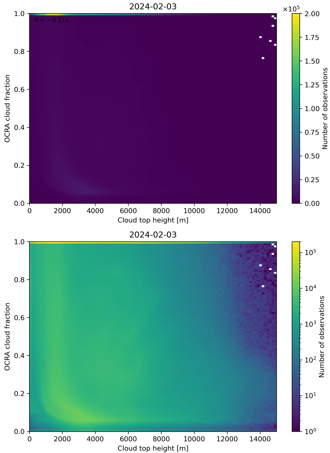
Figure 87: Scatter density plot of “Cloud top height” against “OCRA cloud fraction” for 2024-02-02 to 2024-02-04.
