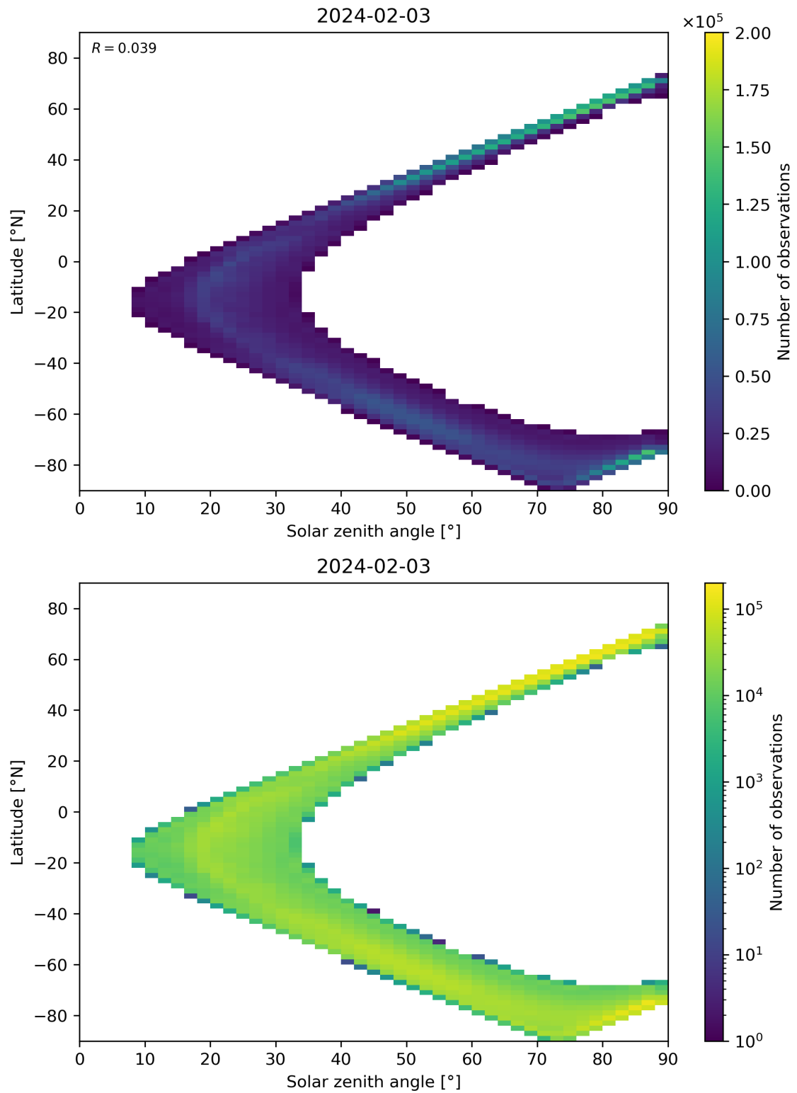
Figure 105: Scatter density plot of “Solar zenith angle” against “Latitude” for 2024-02-02 to 2024-02-04.
