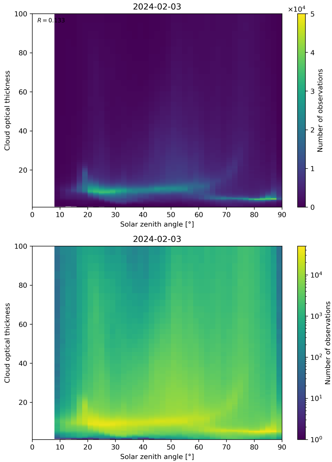
Figure 103: Scatter density plot of “Solar zenith angle” against “Cloud optical thickness” for 2024-02-02 to 2024-02-04.
