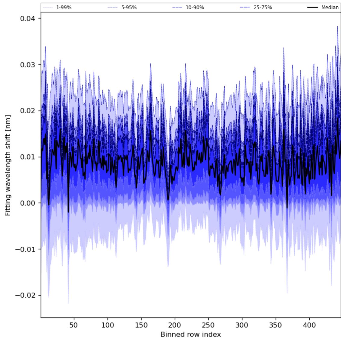
Figure 65: Along track statistics of “Fitting wavelength shift” for 2024-02-02 to 2024-02-04
