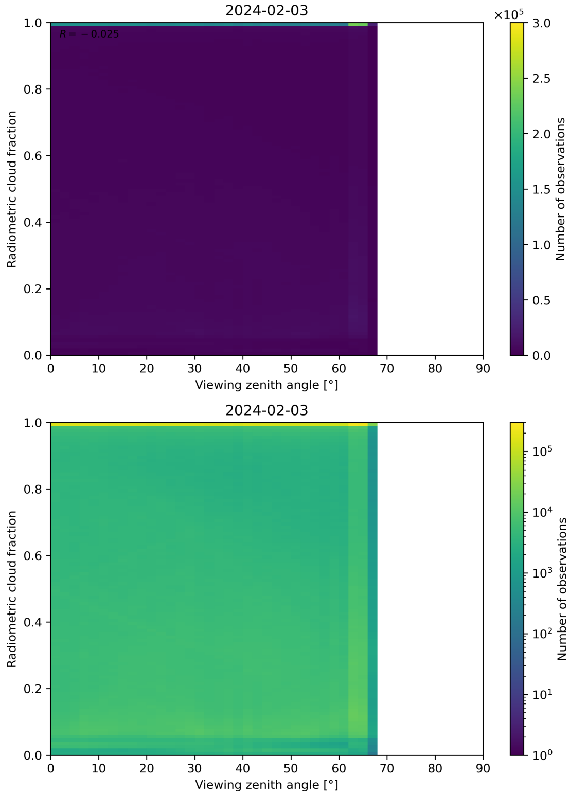
Figure 107: Scatter density plot of “Viewing zenith angle” against “Radiometric cloud fraction” for 2024-02-02 to 2024-02-04.
