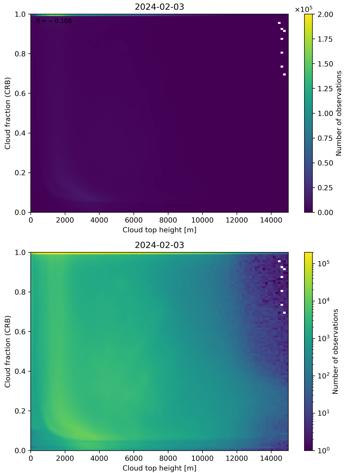
Figure 88: Scatter density plot of “Cloud top height” against “Cloud fraction (CRB)” for 2024-02-02 to 2024-02-04.
