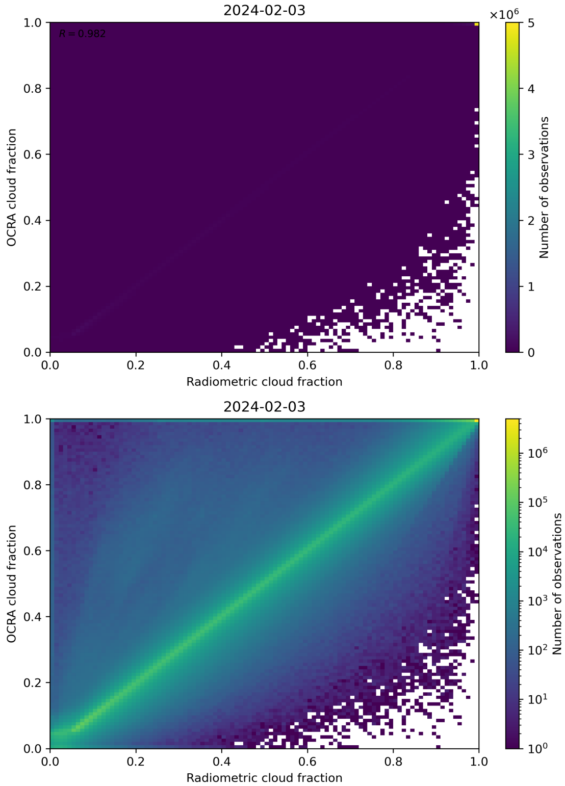
Figure 72: Scatter density plot of “Radiometric cloud fraction” against “OCRA cloud fraction” for 2024-02-02 to 2024-02-04.
