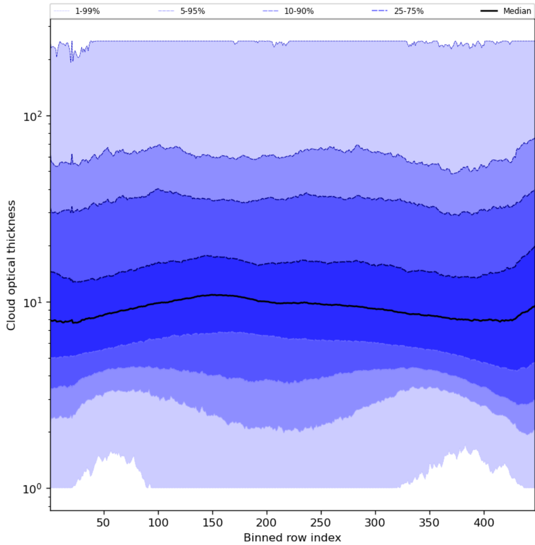
Figure 57: Along track statistics of “Cloud optical thickness” for 2024-02-02 to 2024-02-04
