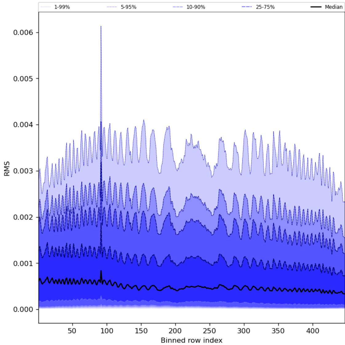
Figure 63: Along track statistics of “RMS” for 2024-02-02 to 2024-02-04
