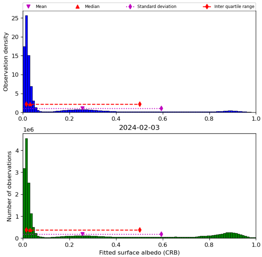
Figure 46: Histogram of “Fitted surface albedo (CRB)” for 2024-02-02 to 2024-02-04
