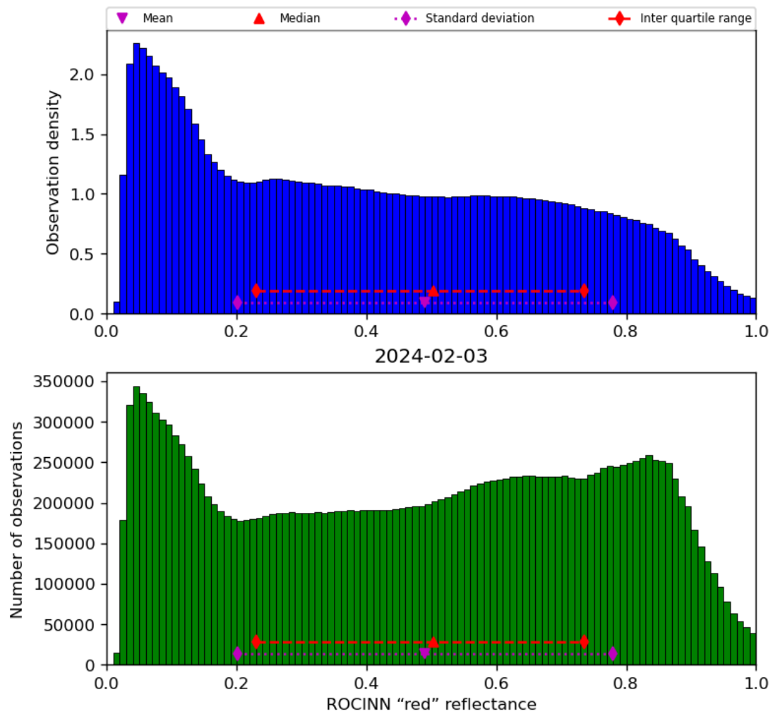
Figure 53: Histogram of “ROCINN “red” reflectance” for 2024-02-02 to 2024-02-04
