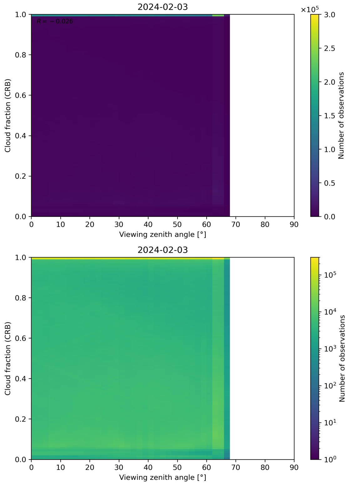
Figure 109: Scatter density plot of “Viewing zenith angle” against “Cloud fraction (CRB)” for 2024-02-02 to 2024-02-04.
