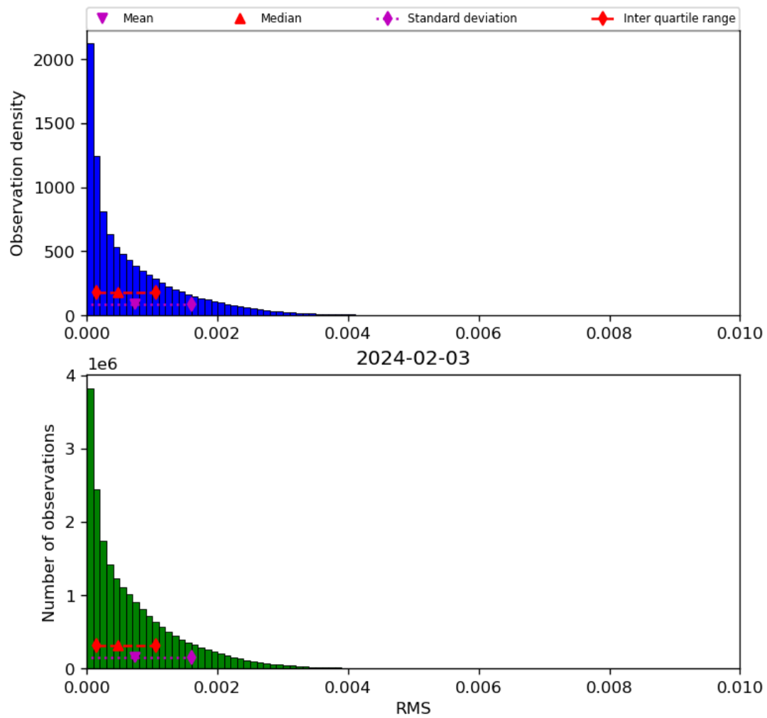
Figure 47: Histogram of “RMS” for 2024-02-02 to 2024-02-04
