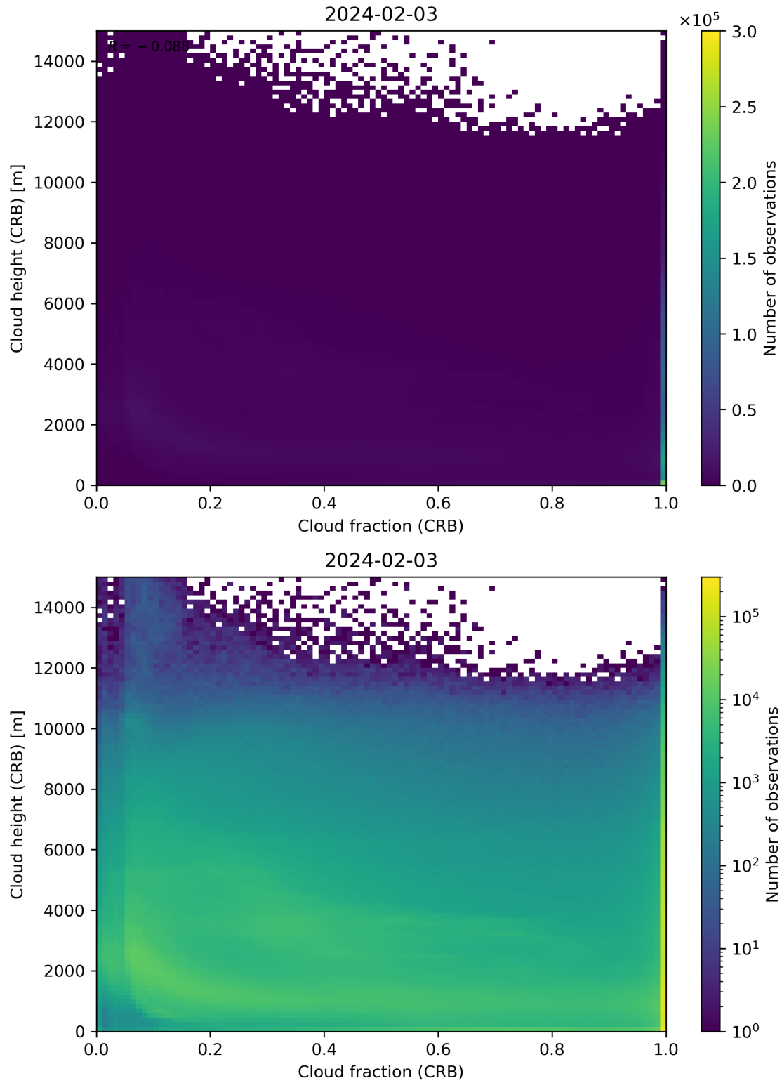
Figure 79: Scatter density plot of “Cloud fraction (CRB)” against “Cloud height (CRB)” for 2024-02-02 to 2024-02-04.
