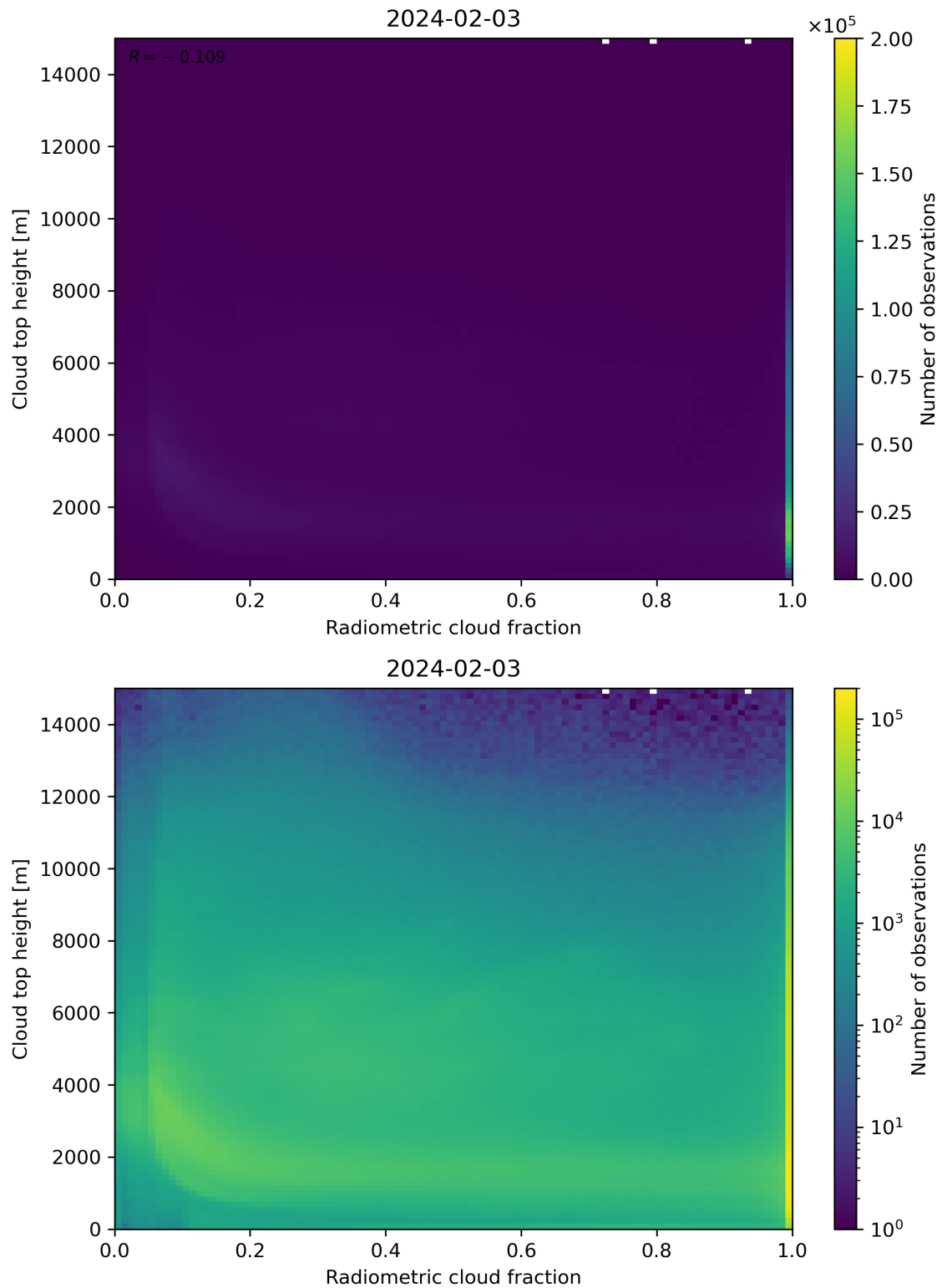
Figure 76: Scatter density plot of “Radiometric cloud fraction” against “Cloud top height” for 2024-02-02 to 2024-02-04.
