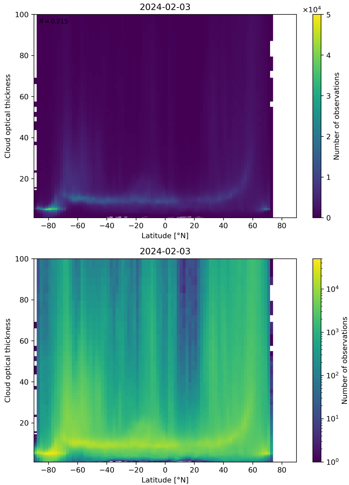
Figure 96: Scatter density plot of “Latitude” against “Cloud optical thickness” for 2024-02-02 to 2024-02-04.
