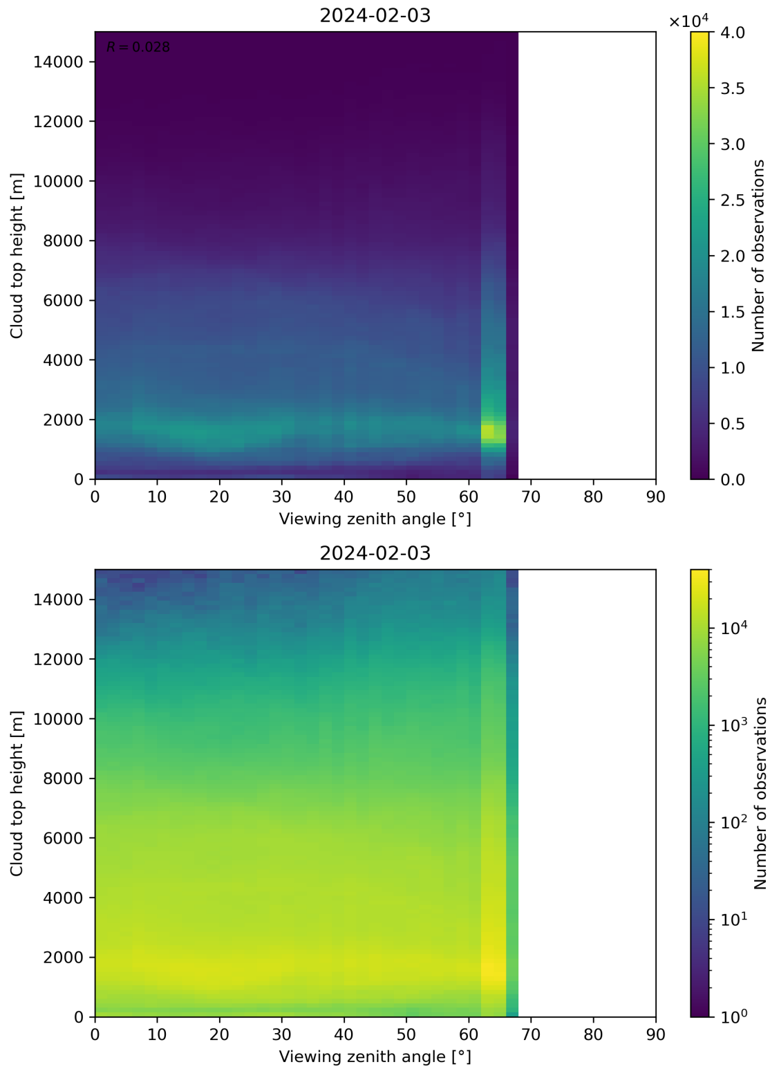
Figure 112: Scatter density plot of “Viewing zenith angle” against “Cloud top height” for 2024-02-02 to 2024-02-04.
