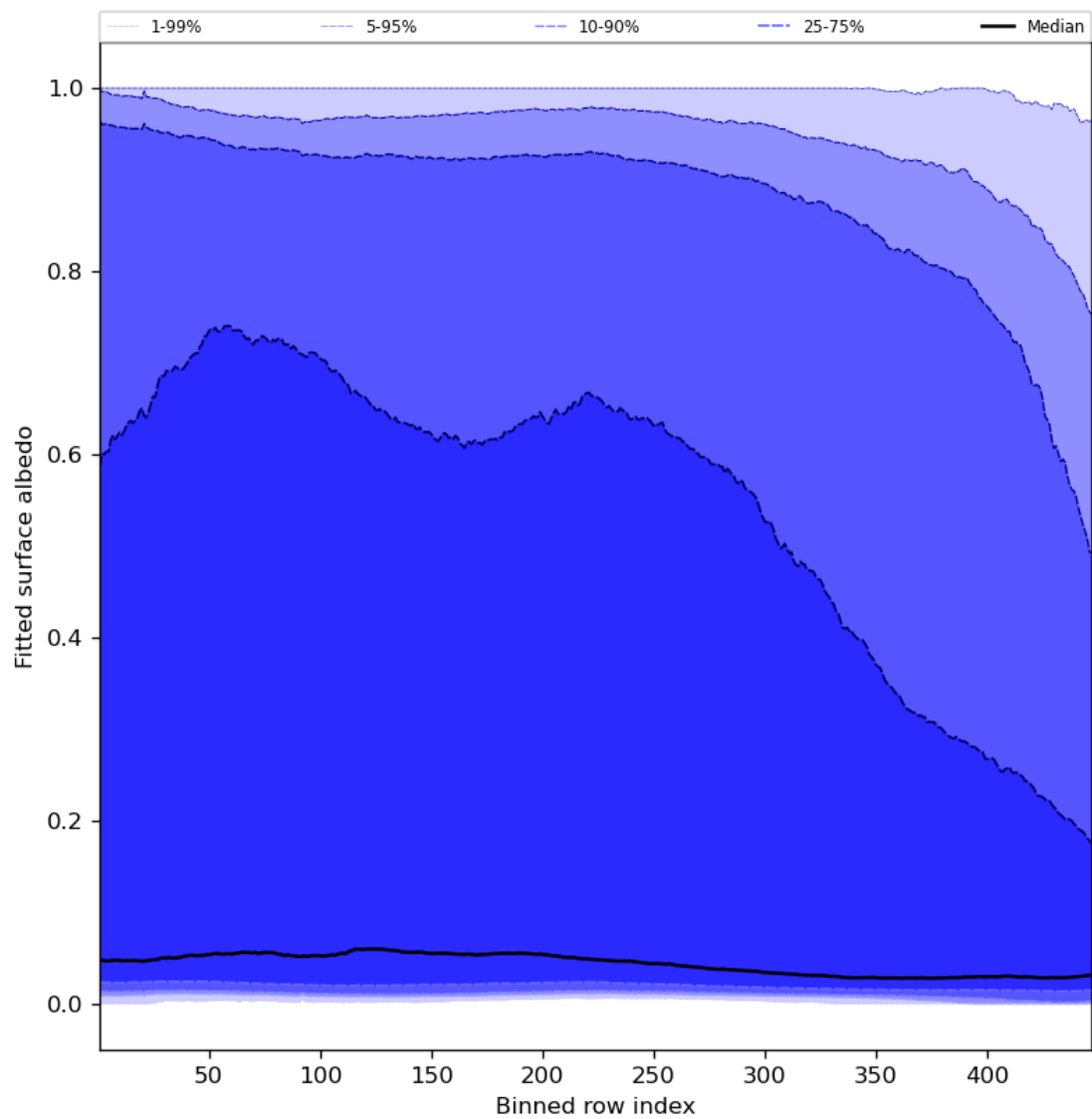
Figure 61: Along track statistics of “Fitted surface albedo” for 2024-02-02 to 2024-02-04
