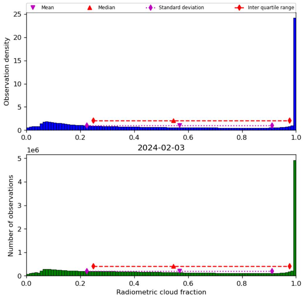
Figure 39: Histogram of “Radiometric cloud fraction” for 2024-02-02 to 2024-02-04
