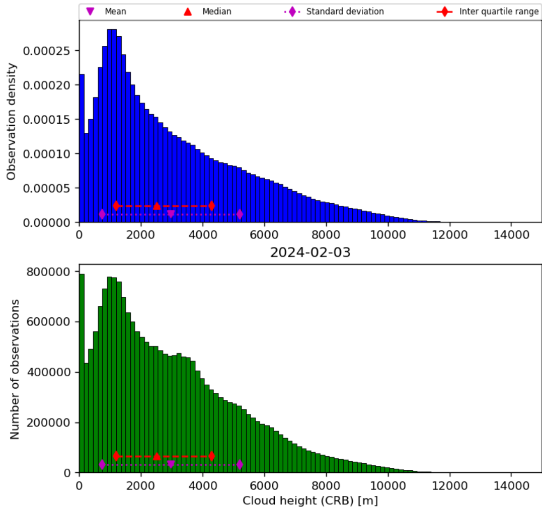
Figure 43: Histogram of “Cloud height (CRB)” for 2024-02-02 to 2024-02-04
