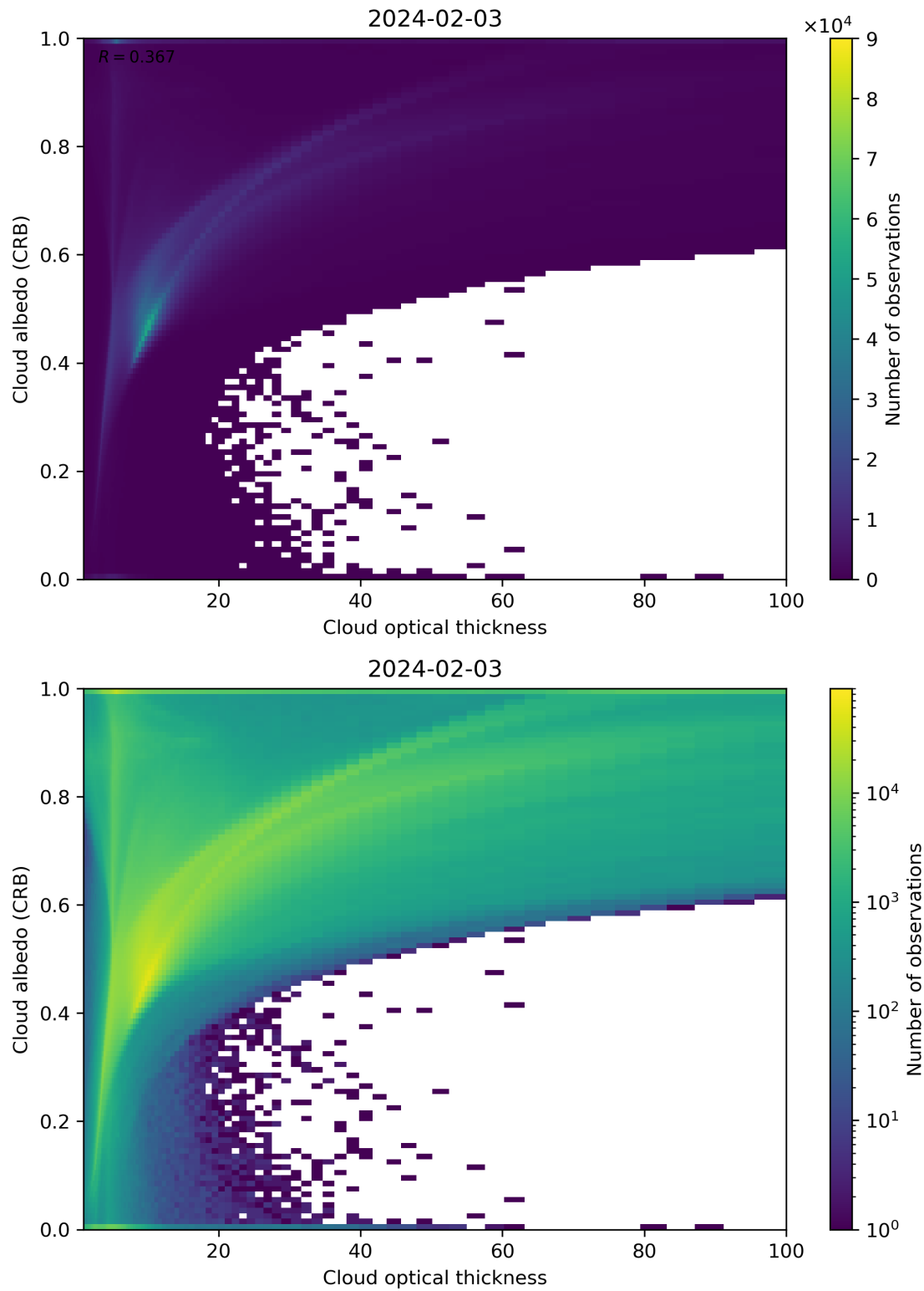
Figure 82: Scatter density plot of “Cloud optical thickness” against “Cloud albedo (CRB)” for 2024-02-02 to 2024-02-04.
