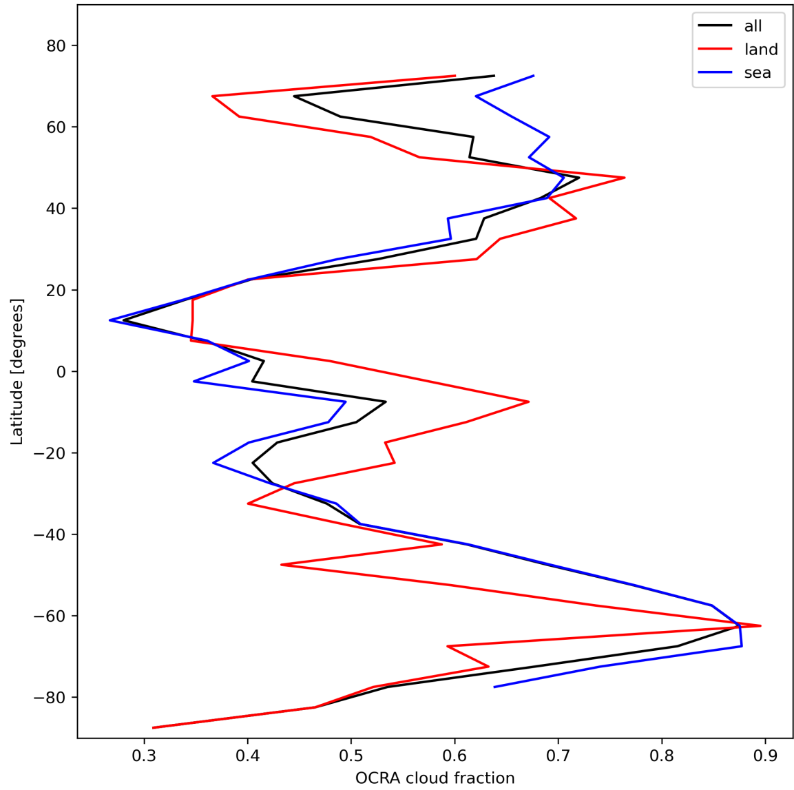
Figure 34: Zonal average of “OCRA cloud fraction” for 2024-02-02 to 2024-02-04.
