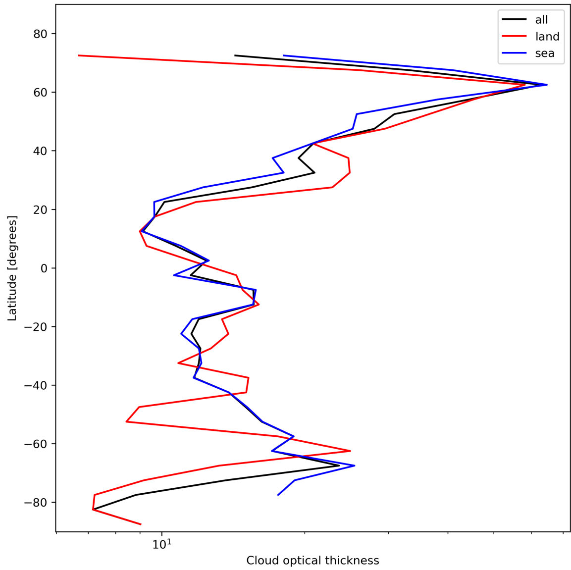
Figure 25: Zonal average of “Cloud optical thickness” for 2024-02-02 to 2024-02-04.
