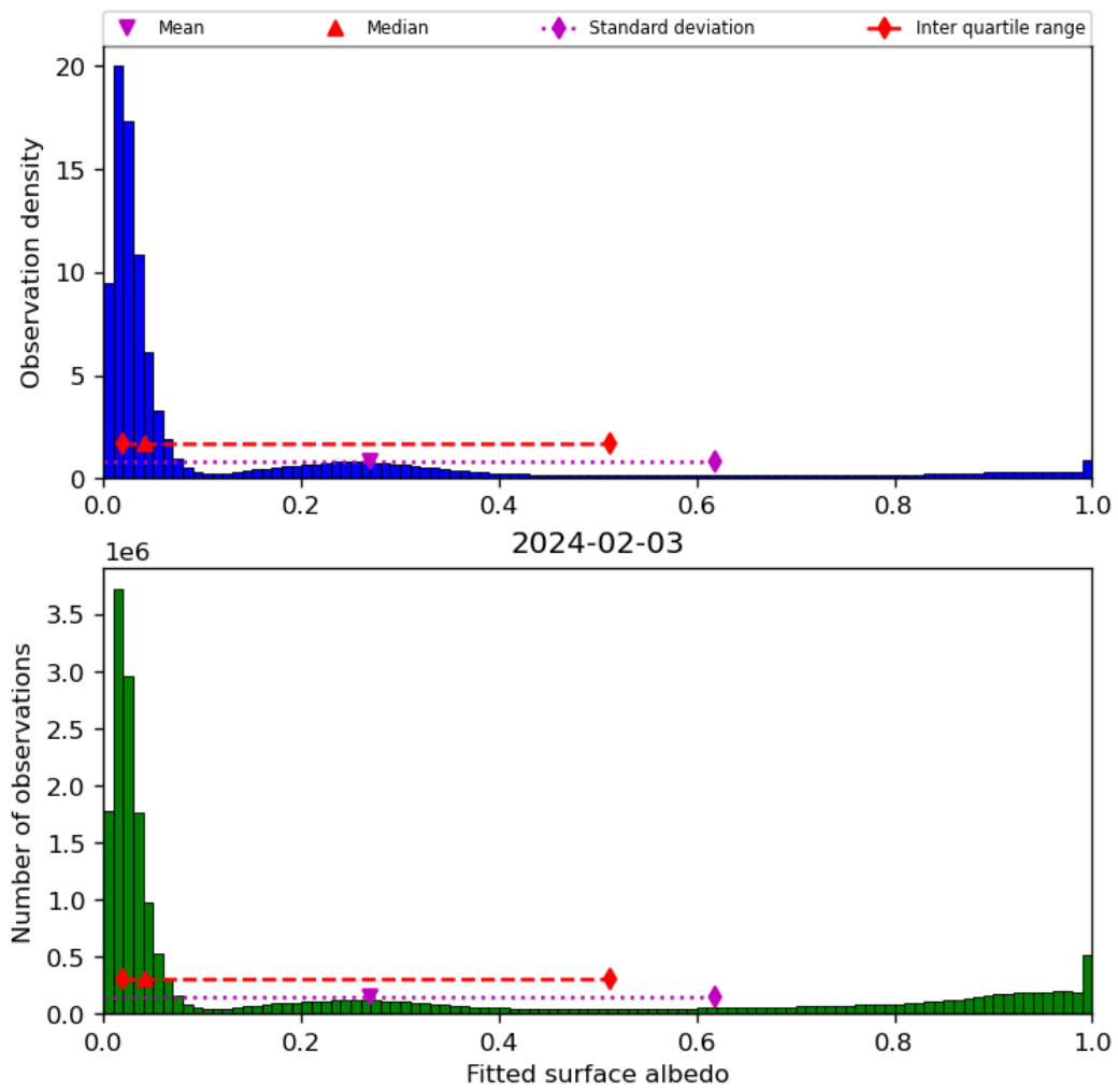
Figure 45: Histogram of “Fitted surface albedo” for 2024-02-02 to 2024-02-04
