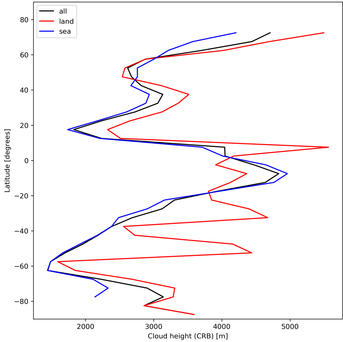
Figure 27: Zonal average of “Cloud height (CRB)” for 2024-02-02 to 2024-02-04.
