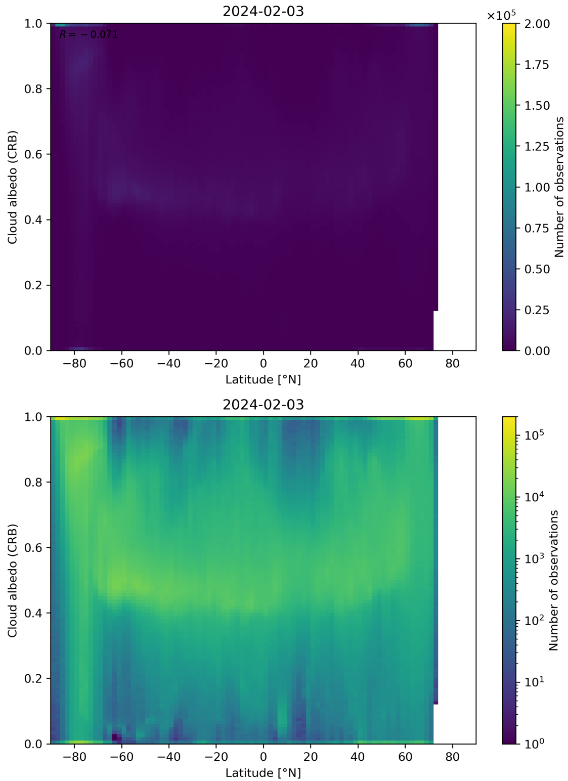
Figure 91: Scatter density plot of “Latitude” against “Cloud albedo (CRB)” for 2024-02-02 to 2024-02-04.
