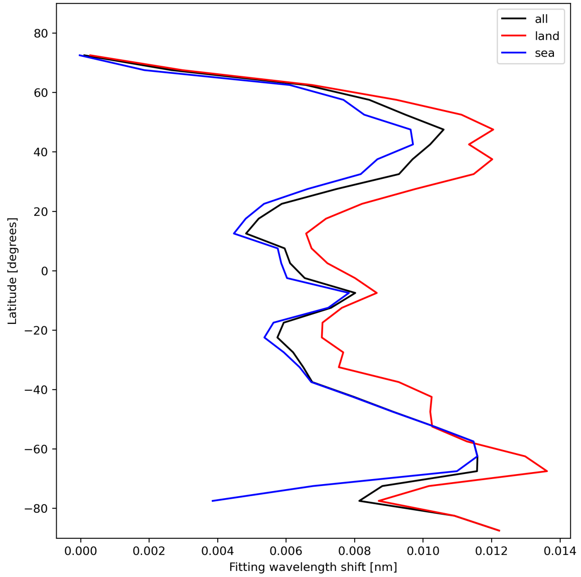
Figure 33: Zonal average of “Fitting wavelength shift” for 2024-02-02 to 2024-02-04.
