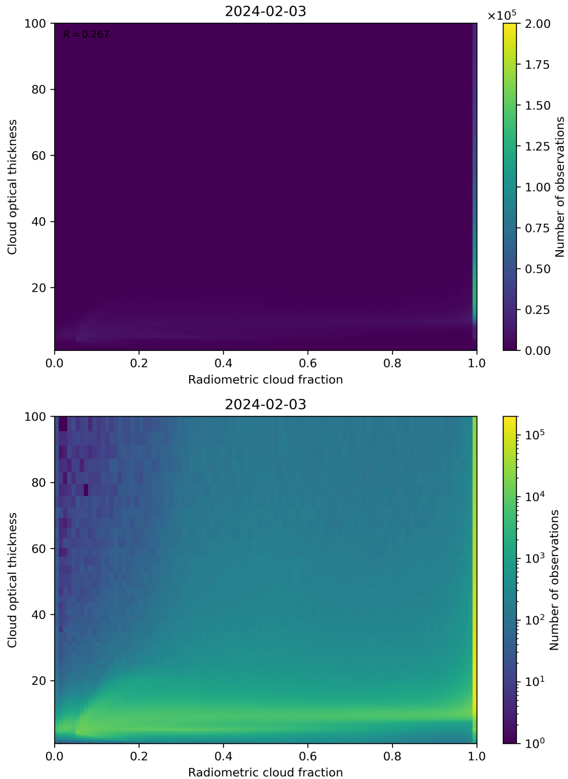
Figure 75: Scatter density plot of “Radiometric cloud fraction” against “Cloud optical thickness” for 2024-02-02 to 2024-02-04.
