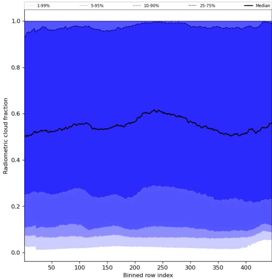
Figure 55: Along track statistics of “Radiometric cloud fraction” for 2024-02-02 to 2024-02-04
