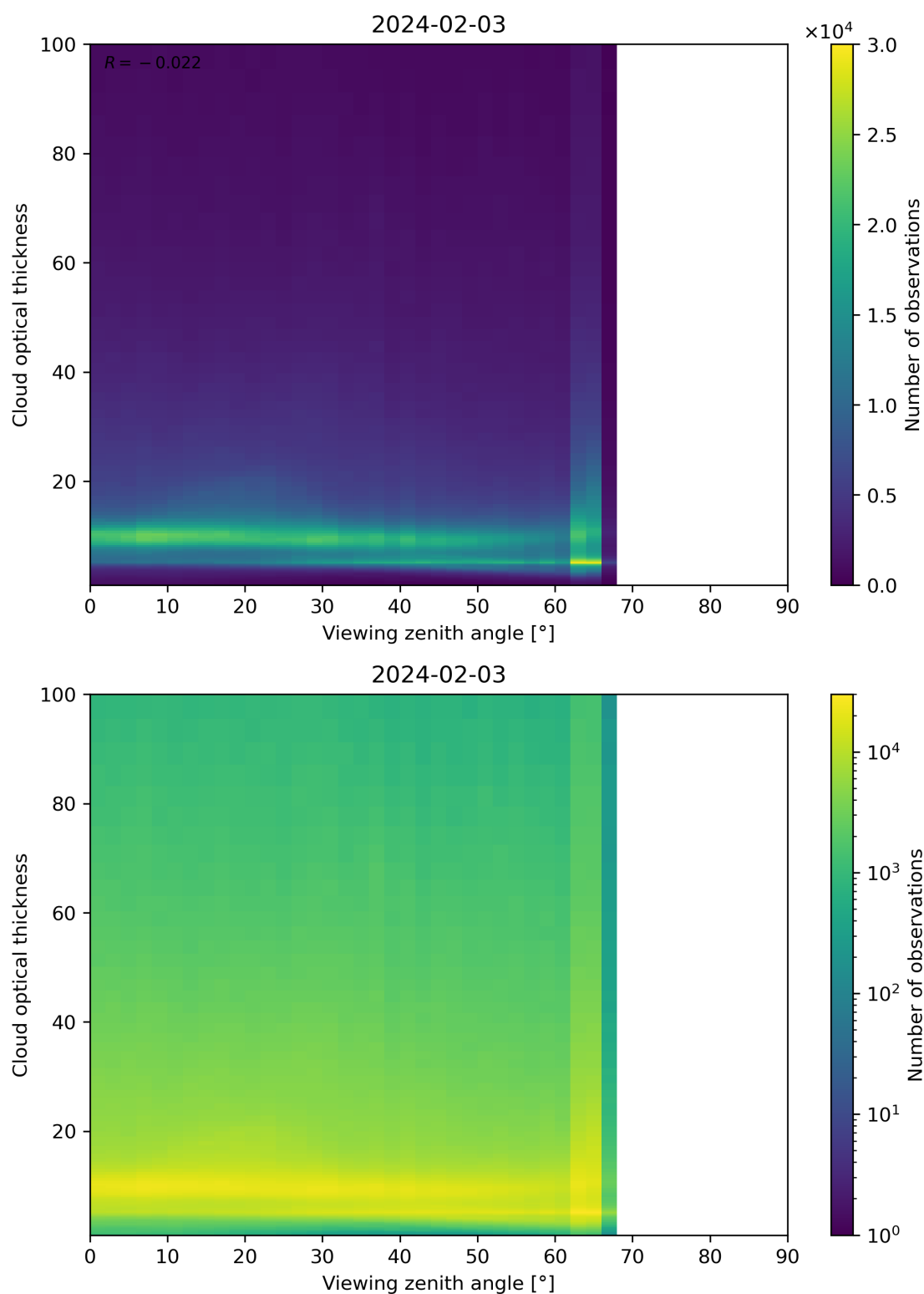
Figure 111: Scatter density plot of “Viewing zenith angle” against “Cloud optical thickness” for 2024-02-02 to 2024-02-04.
