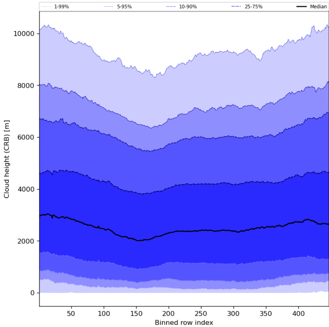
Figure 59: Along track statistics of “Cloud height (CRB)” for 2024-02-02 to 2024-02-04
