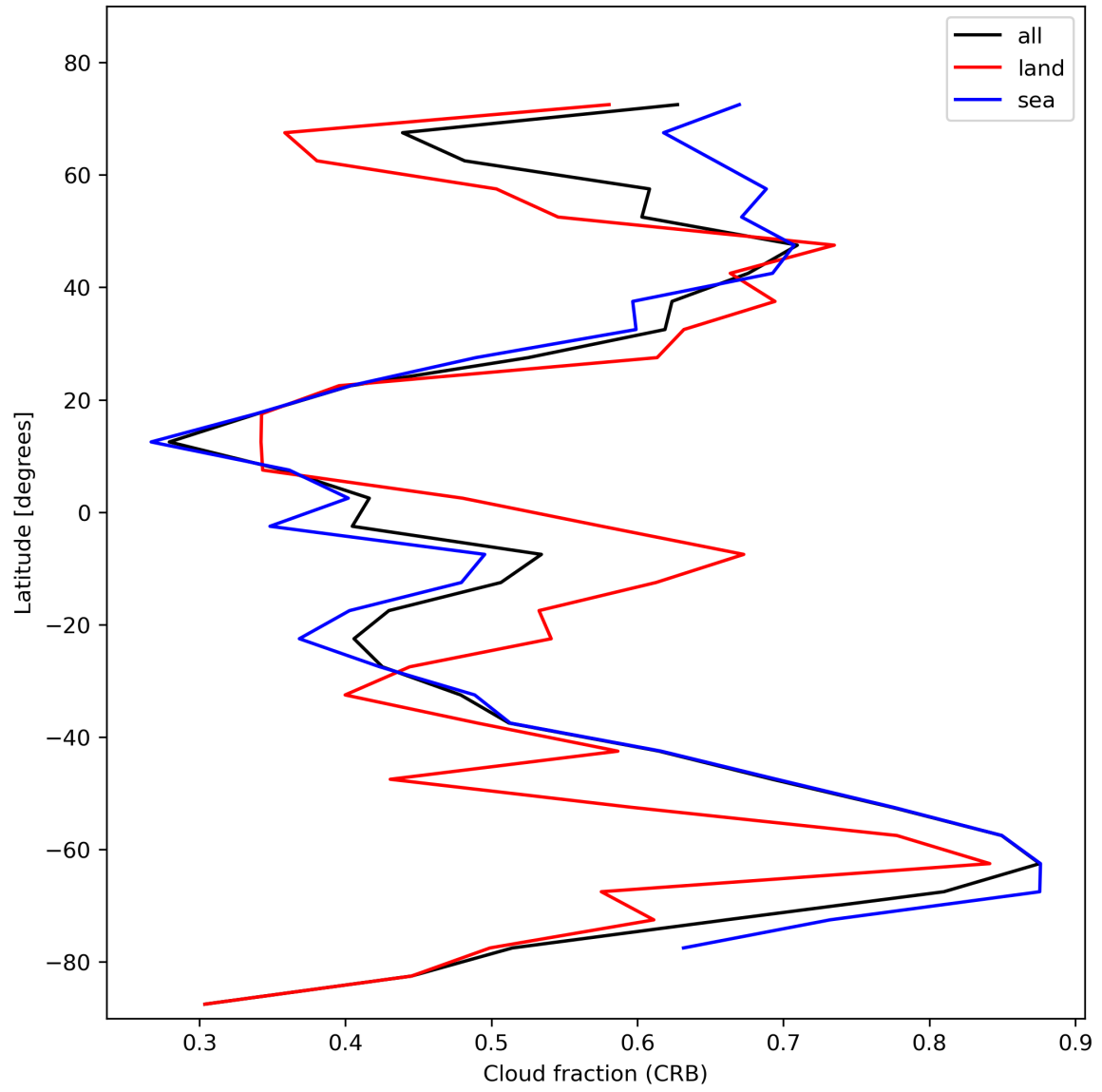
Figure 26: Zonal average of “Cloud fraction (CRB)” for 2024-02-02 to 2024-02-04.
