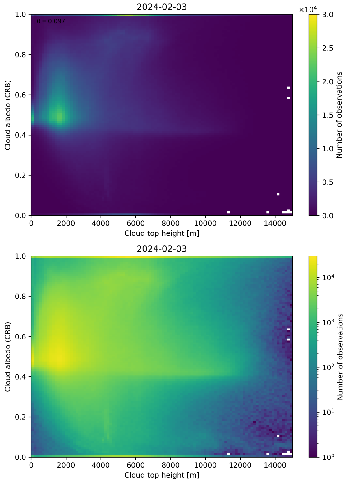
Figure 86: Scatter density plot of “Cloud top height” against “Cloud albedo (CRB)” for 2024-02-02 to 2024-02-04.
