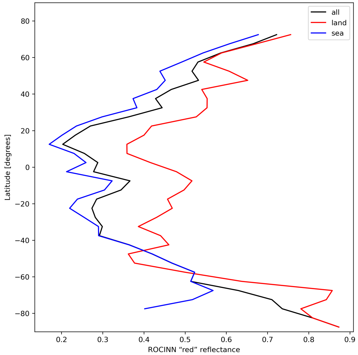
Figure 37: Zonal average of “ROCINN “red” reflectance” for 2024-02-02 to 2024-02-04.
