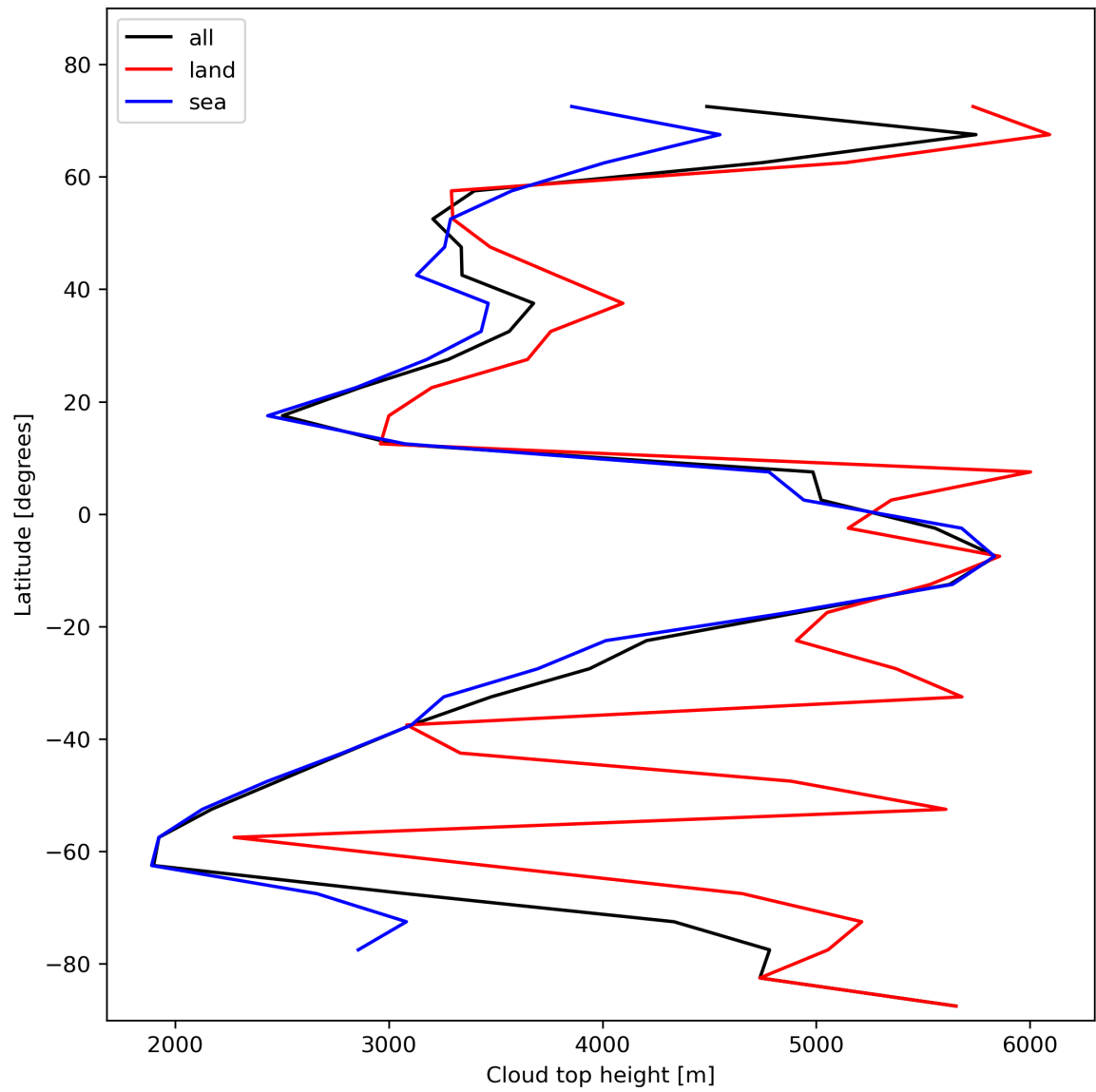
Figure 24: Zonal average of “Cloud top height” for 2024-02-02 to 2024-02-04.
