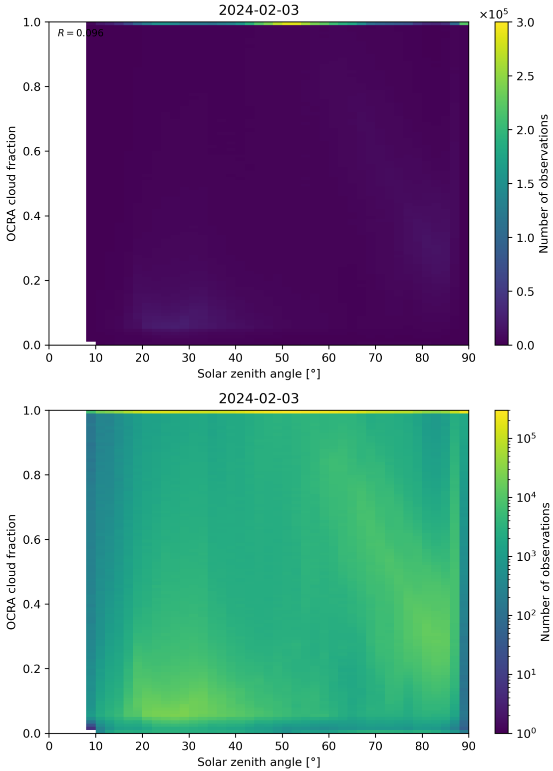
Figure 100: Scatter density plot of “Solar zenith angle” against “OCRA cloud fraction” for 2024-02-02 to 2024-02-04.
