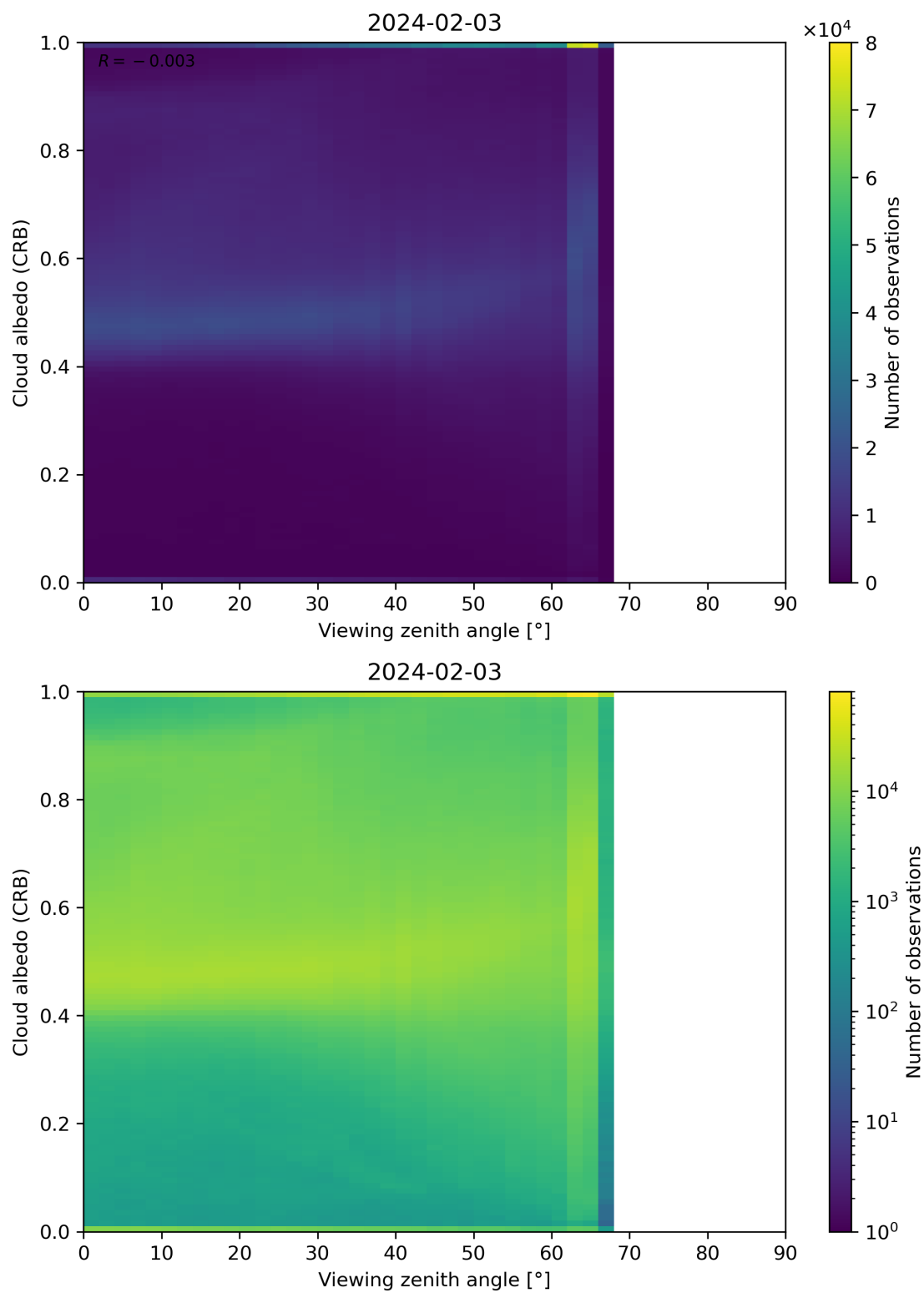
Figure 106: Scatter density plot of “Viewing zenith angle” against “Cloud albedo (CRB)” for 2024-02-02 to 2024-02-04.
