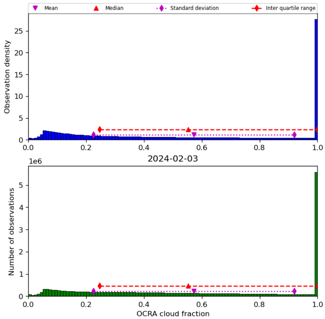
Figure 50: Histogram of “OCRA cloud fraction” for 2024-02-02 to 2024-02-04
