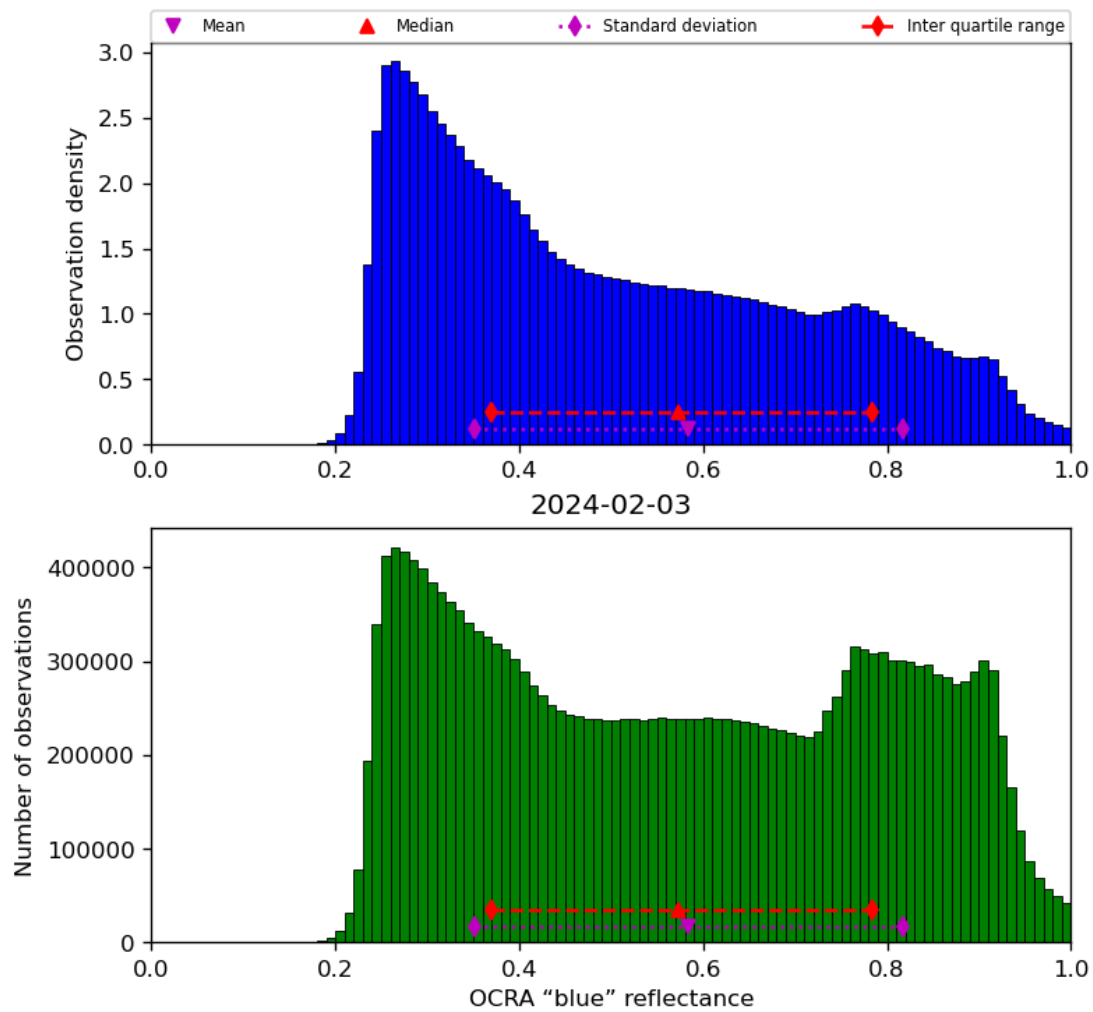
Figure 51: Histogram of “OCRA “blue” reflectance” for 2024-02-02 to 2024-02-04
