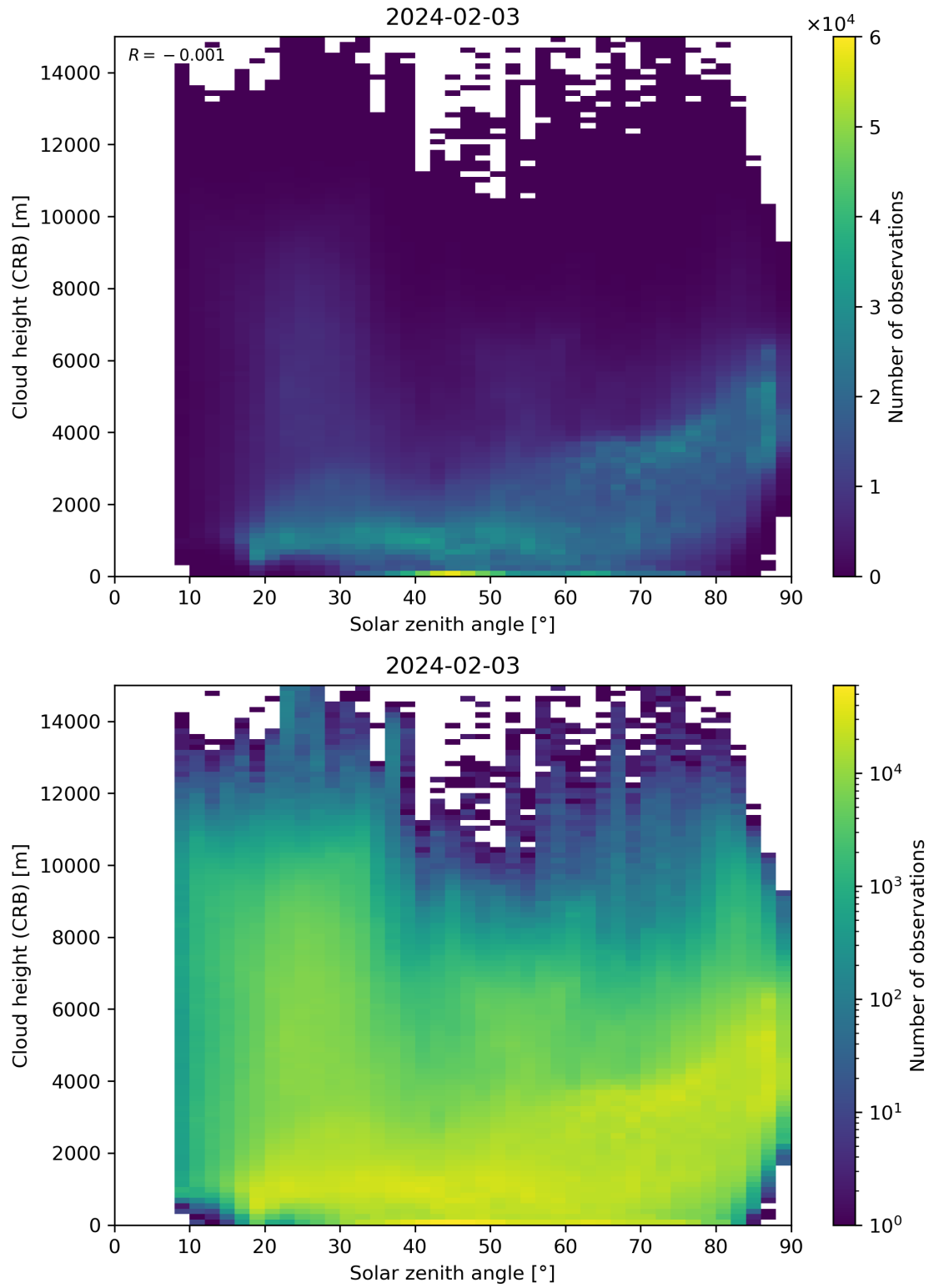
Figure 102: Scatter density plot of “Solar zenith angle” against “Cloud height (CRB)” for 2024-02-02 to 2024-02-04.
