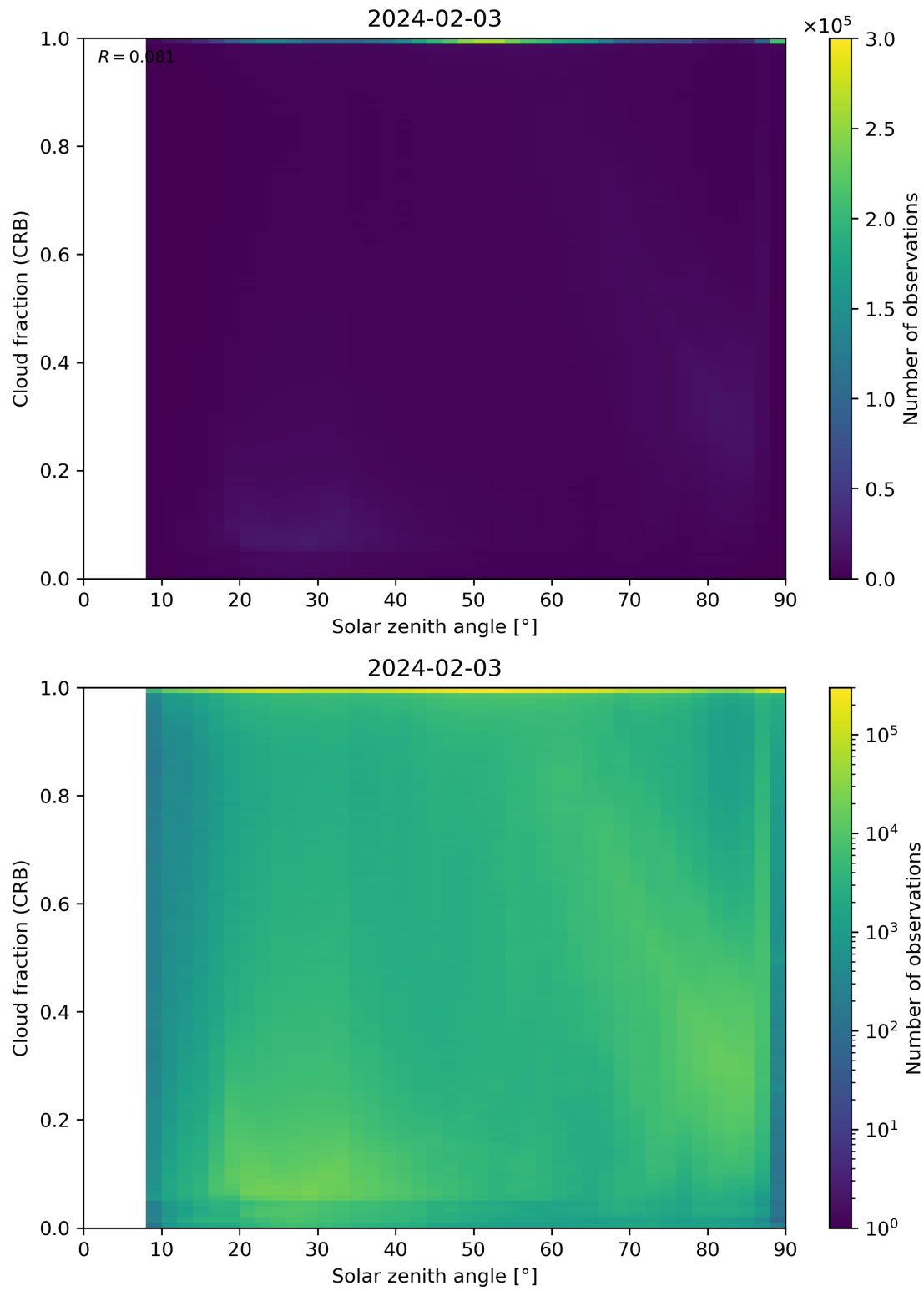
Figure 101: Scatter density plot of “Solar zenith angle” against “Cloud fraction (CRB)” for 2024-02-02 to 2024-02-04.
