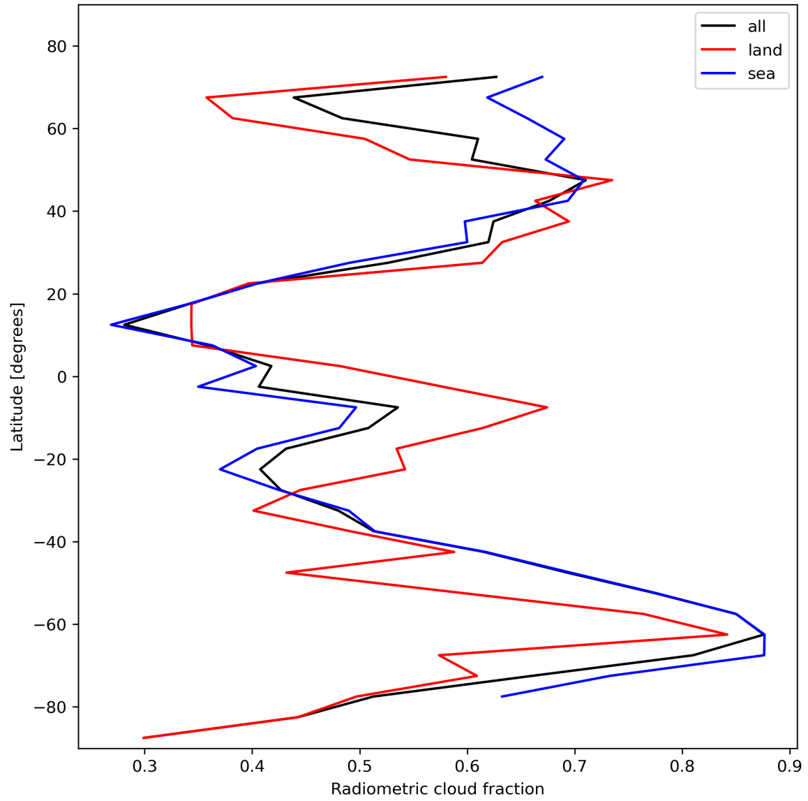
Figure 23: Zonal average of “Radiometric cloud fraction” for 2024-02-02 to 2024-02-04.
