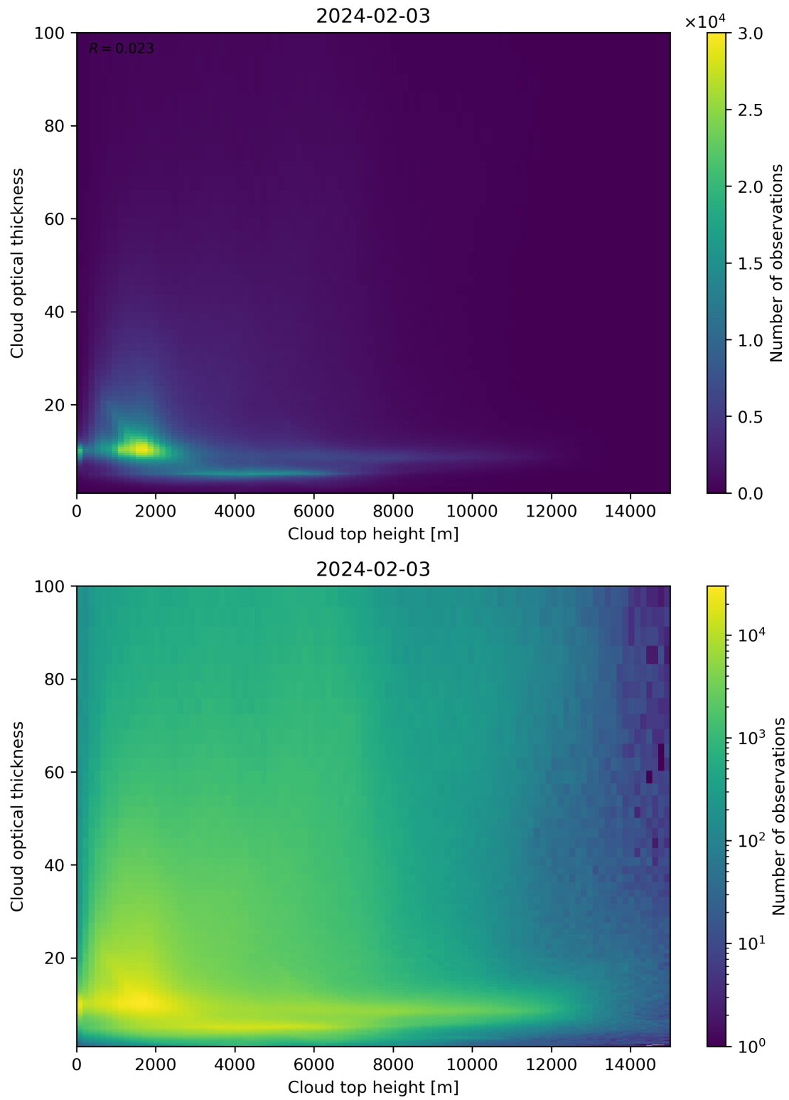
Figure 90: Scatter density plot of “Cloud top height” against “Cloud optical thickness” for 2024-02-02 to 2024-02-04.
