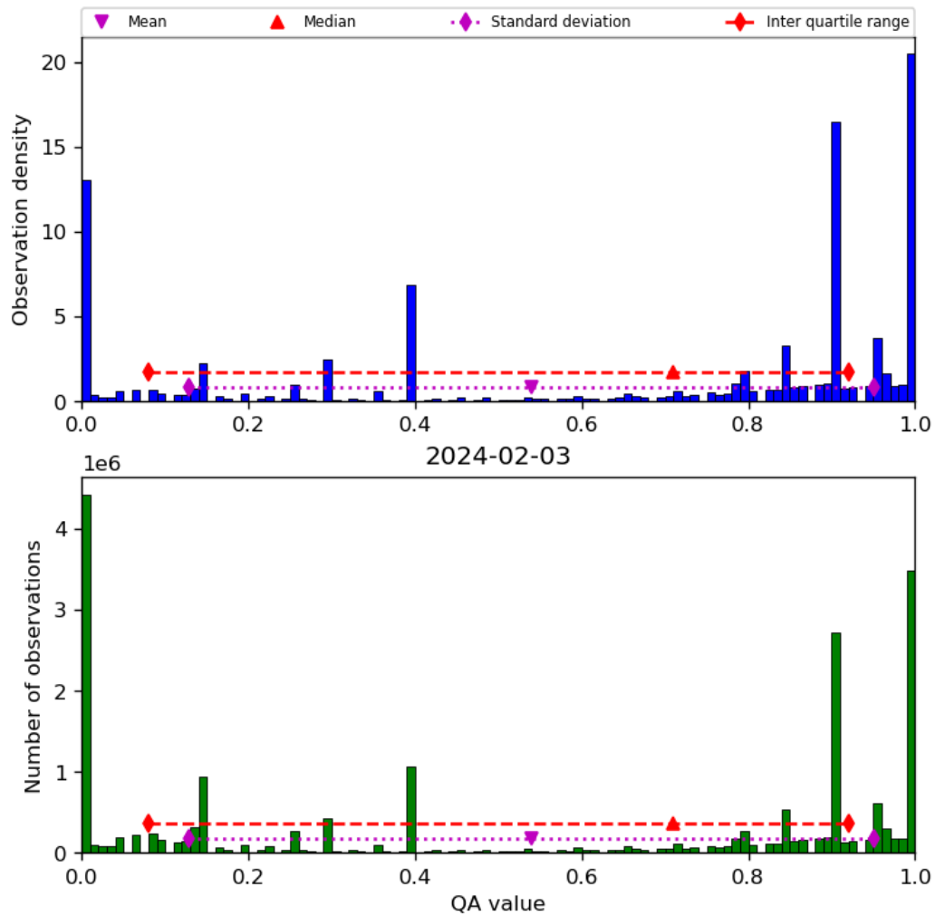
Figure 38: Histogram of “QA value” for 2024-02-02 to 2024-02-04
