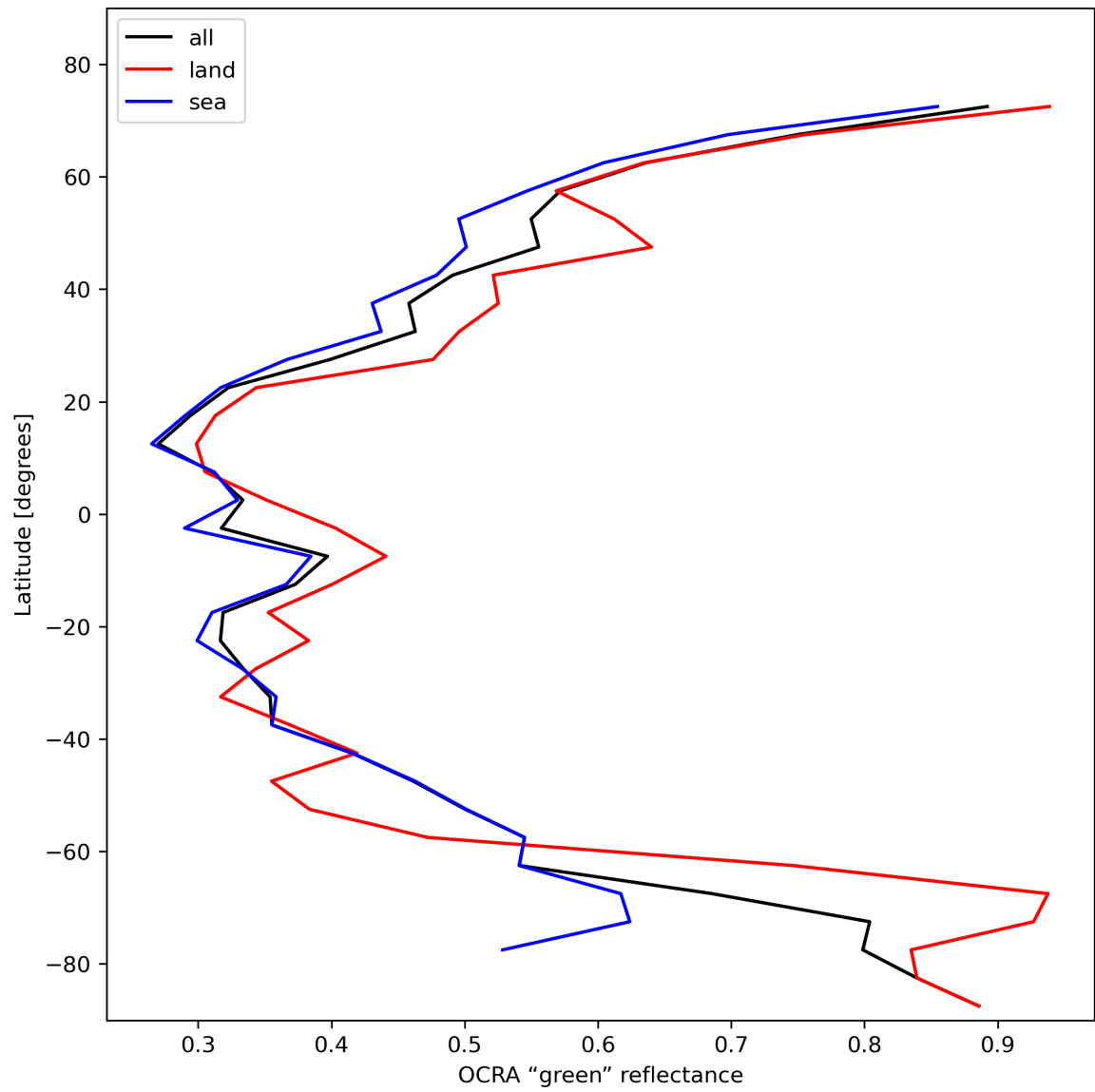
Figure 36: Zonal average of “OCRA “green” reflectance” for 2024-02-02 to 2024-02-04.
