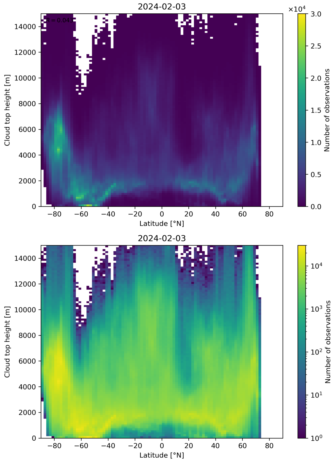
Figure 97: Scatter density plot of “Latitude” against “Cloud top height” for 2024-02-02 to 2024-02-04.
