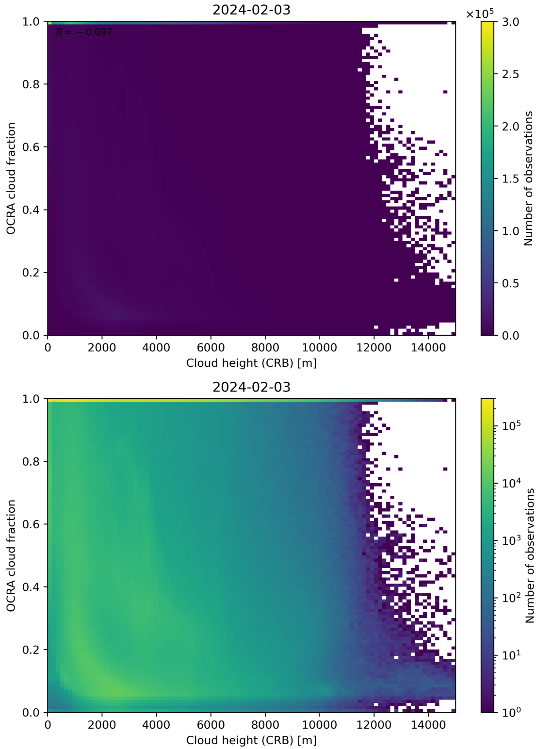
Figure 81: Scatter density plot of “Cloud height (CRB)” against “OCRA cloud fraction” for 2024-02-02 to 2024-02-04.
