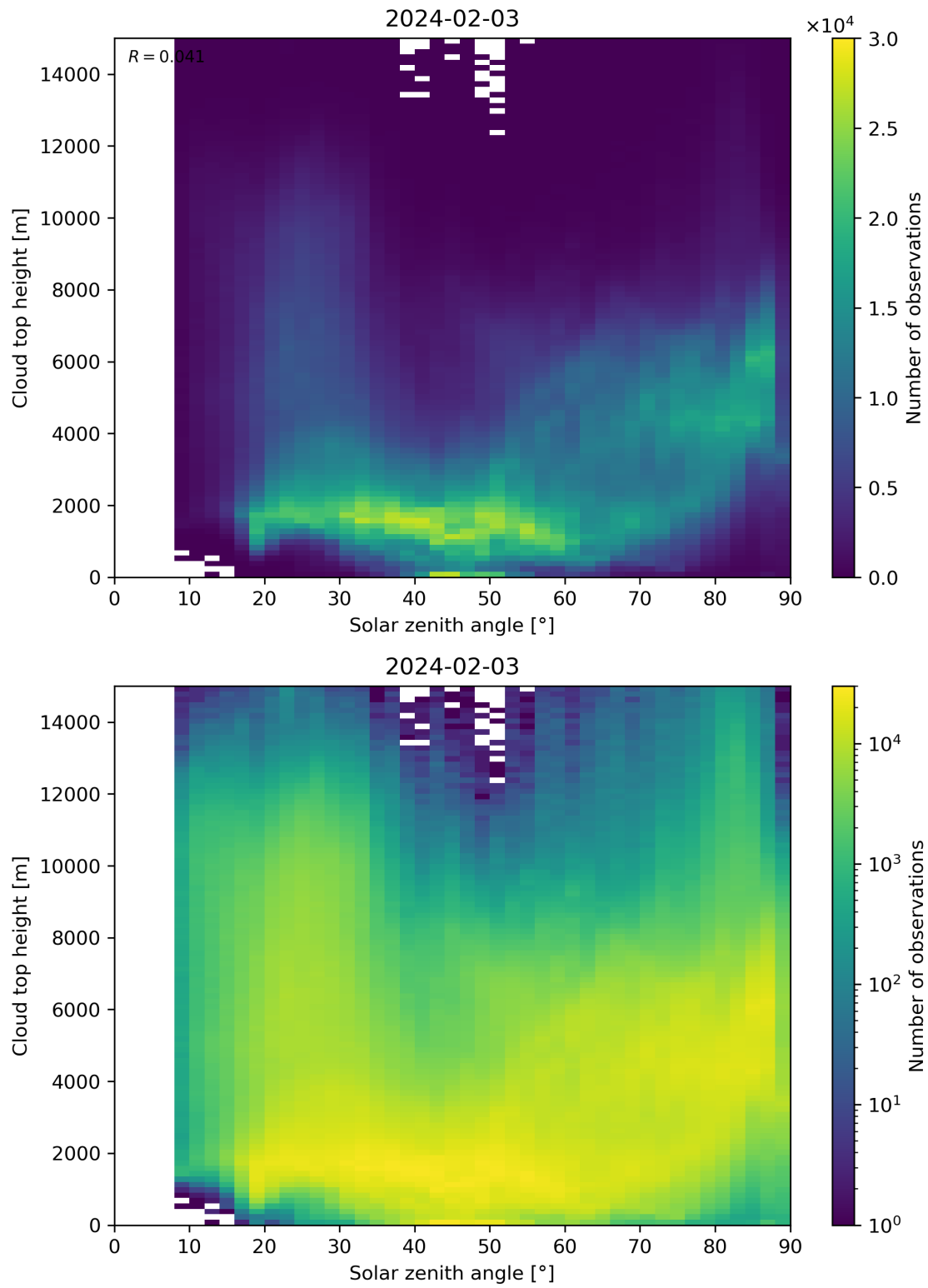
Figure 104: Scatter density plot of “Solar zenith angle” against “Cloud top height” for 2024-02-02 to 2024-02-04.
