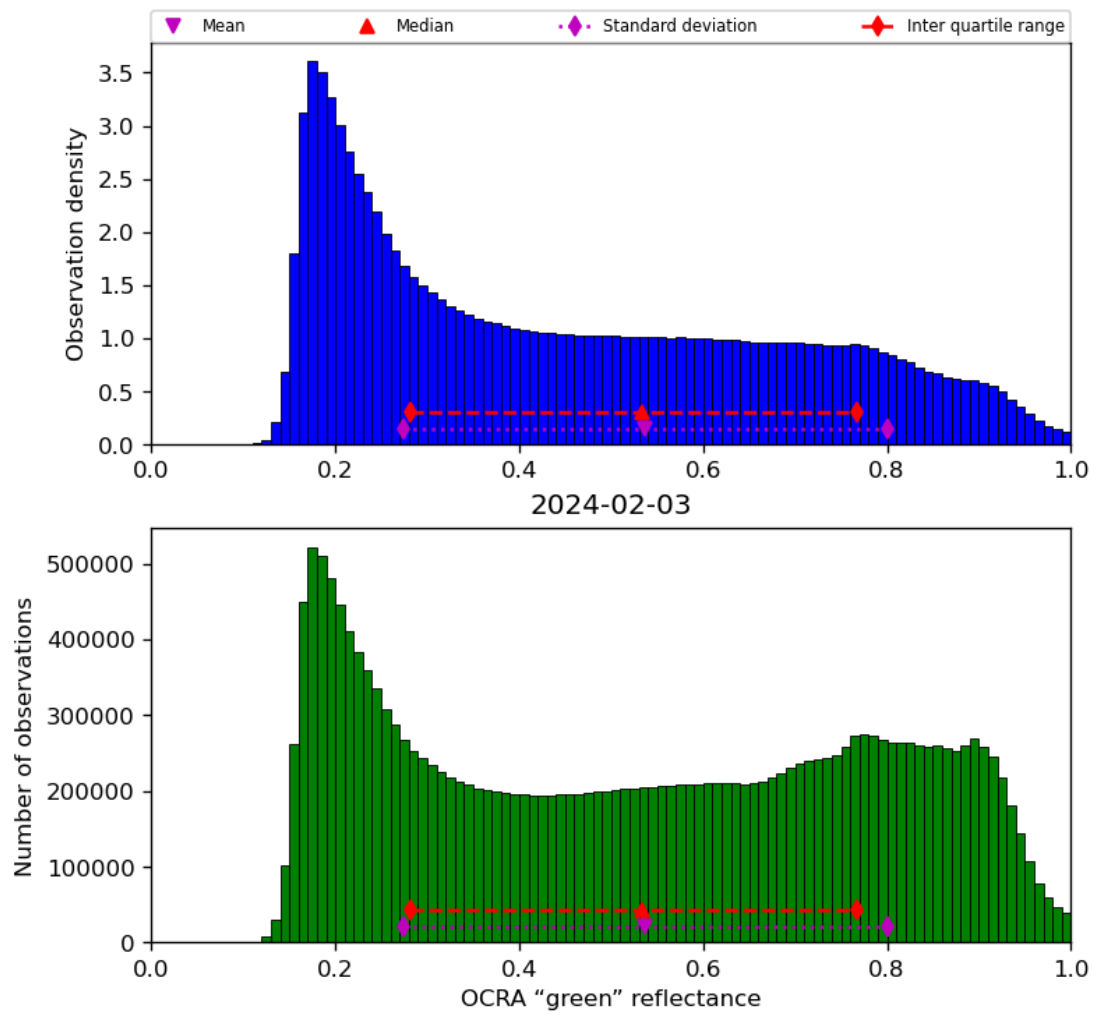
Figure 52: Histogram of “OCRA “green” reflectance” for 2024-02-02 to 2024-02-04
