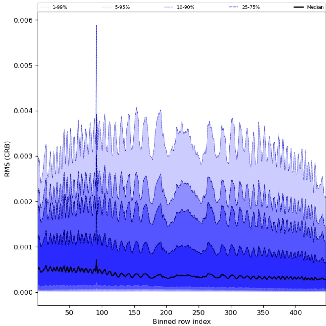
Figure 64: Along track statistics of “RMS (CRB)” for 2024-02-02 to 2024-02-04
