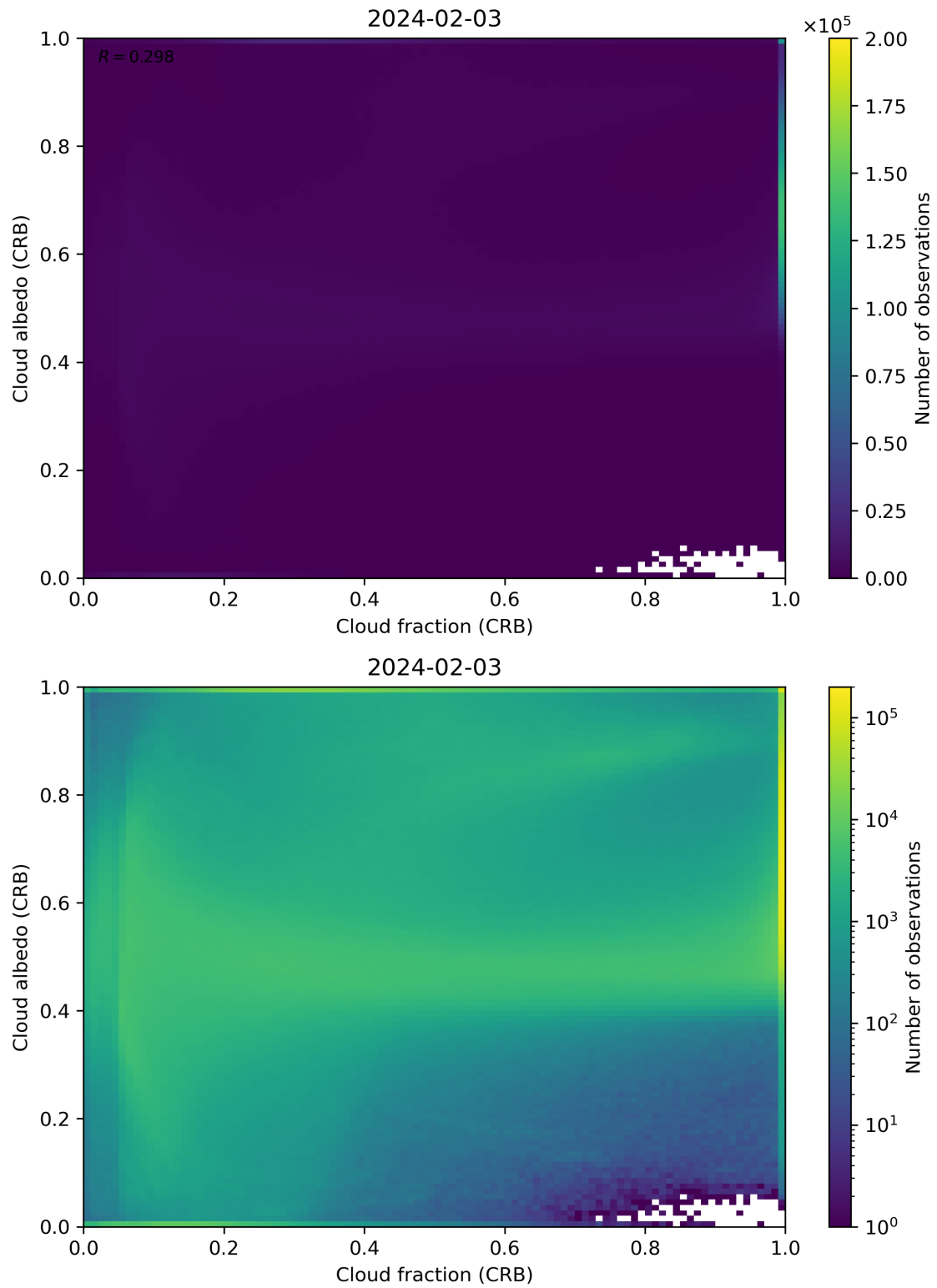
Figure 77: Scatter density plot of “Cloud fraction (CRB)” against “Cloud albedo (CRB)” for 2024-02-02 to 2024-02-04.
