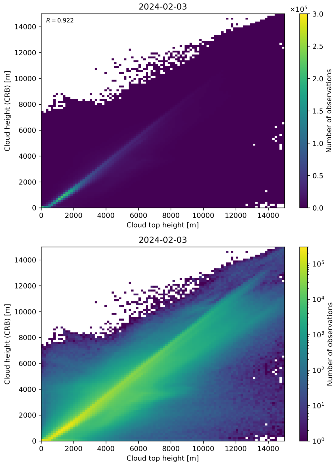
Figure 89: Scatter density plot of “Cloud top height” against “Cloud height (CRB)” for 2024-02-02 to 2024-02-04.
