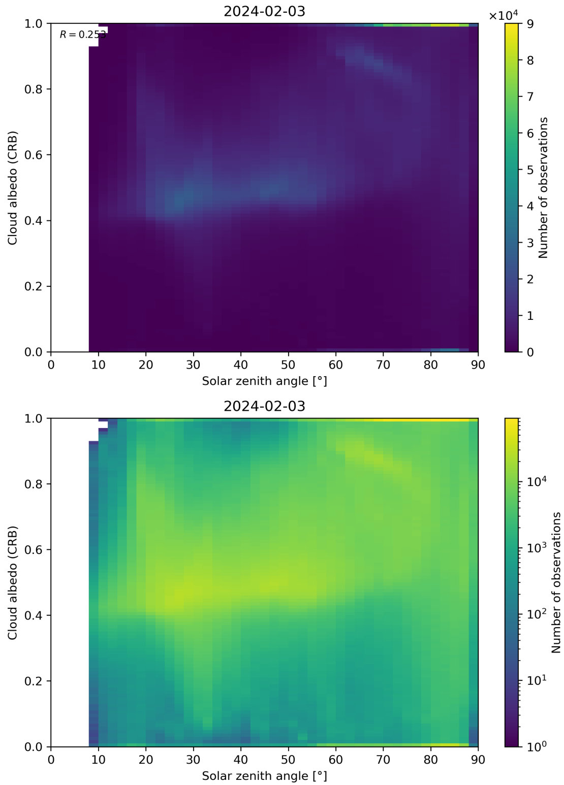
Figure 98: Scatter density plot of “Solar zenith angle” against “Cloud albedo (CRB)” for 2024-02-02 to 2024-02-04.
