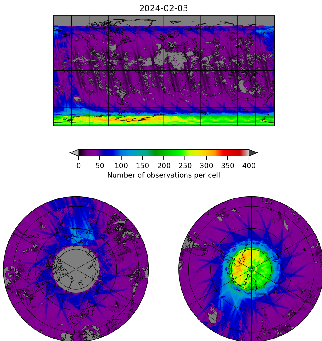
Figure 21: Map of the number of observations for 2024-02-02 to 2024-02-04
