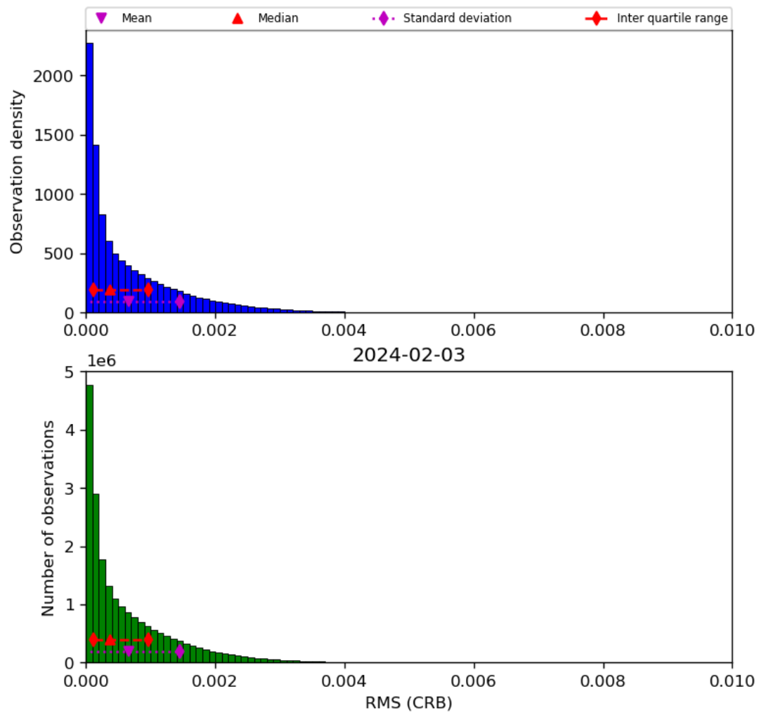
Figure 48: Histogram of “RMS (CRB)” for 2024-02-02 to 2024-02-04
