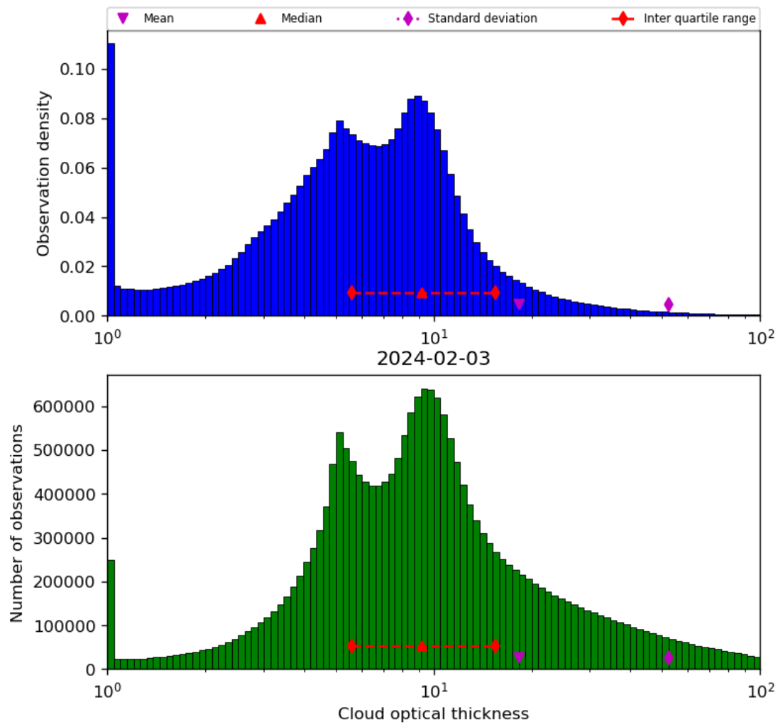
Figure 41: Histogram of “Cloud optical thickness” for 2024-02-02 to 2024-02-04
