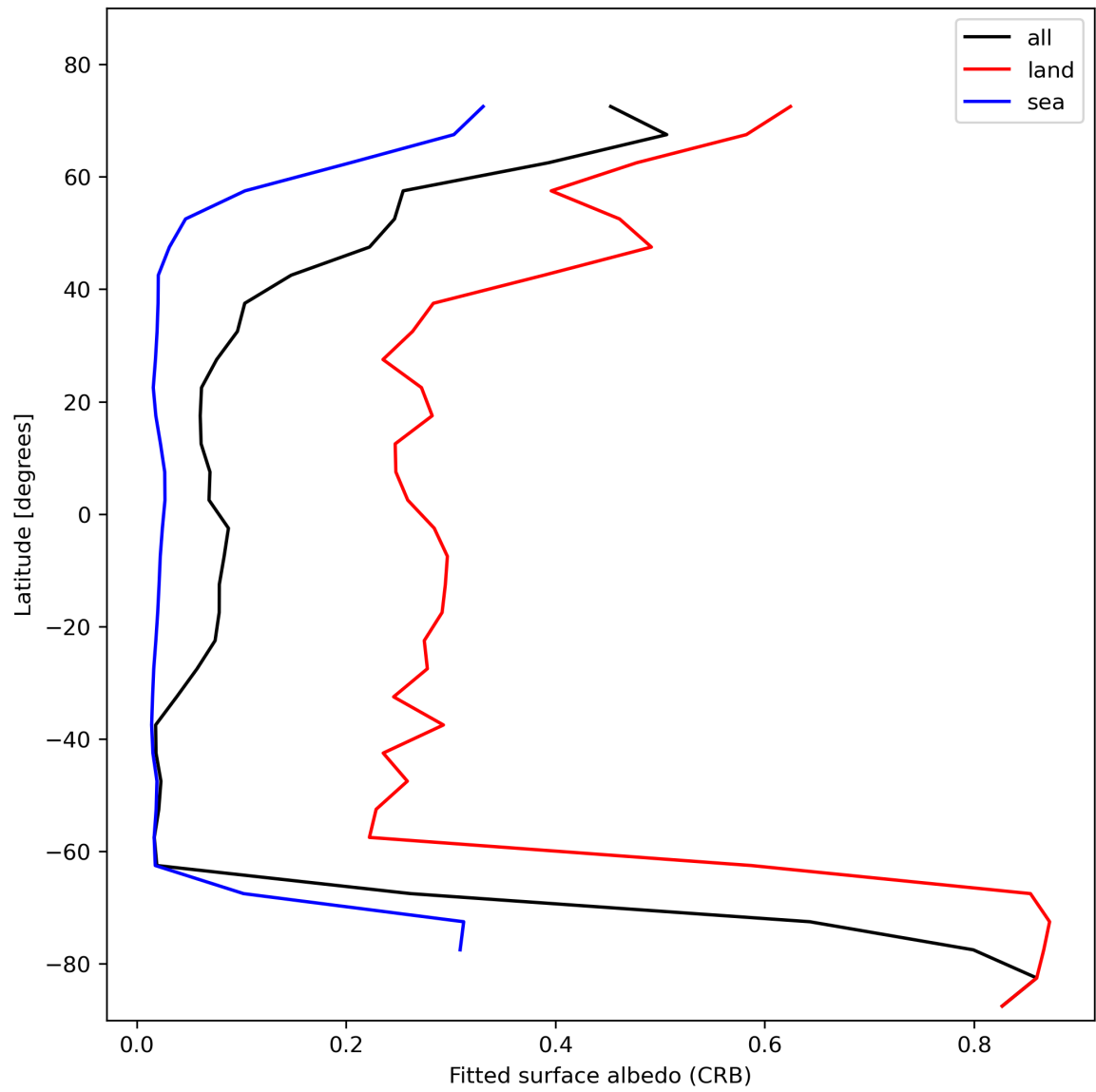
Figure 30: Zonal average of “Fitted surface albedo (CRB)” for 2024-02-02 to 2024-02-04.
