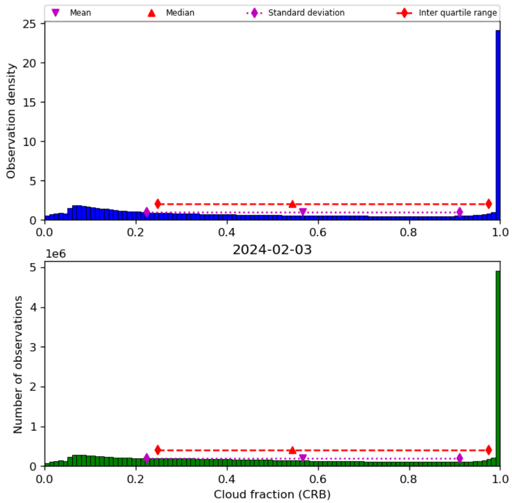
Figure 42: Histogram of “Cloud fraction (CRB)” for 2024-02-02 to 2024-02-04
