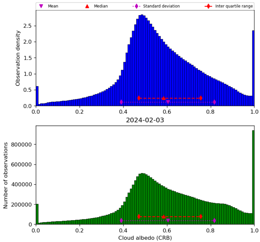
Figure 44: Histogram of “Cloud albedo (CRB)” for 2024-02-02 to 2024-02-04
