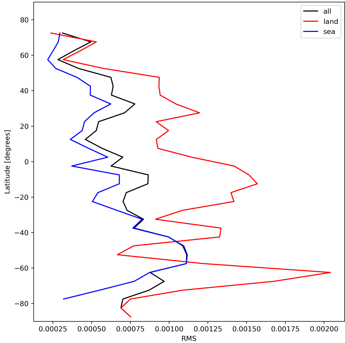
Figure 31: Zonal average of “RMS” for 2024-02-02 to 2024-02-04.
