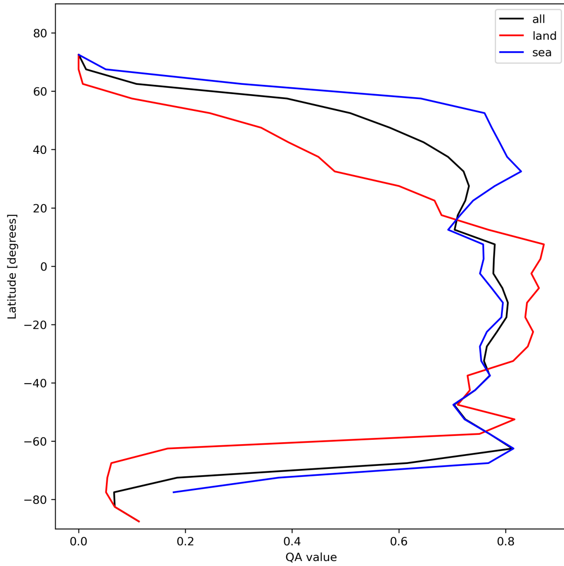
Figure 22: Zonal average of “QA value” for 2024-02-02 to 2024-02-04.
