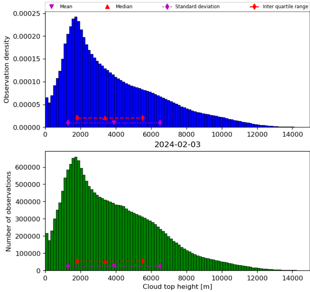
Figure 40: Histogram of “Cloud top height” for 2024-02-02 to 2024-02-04
