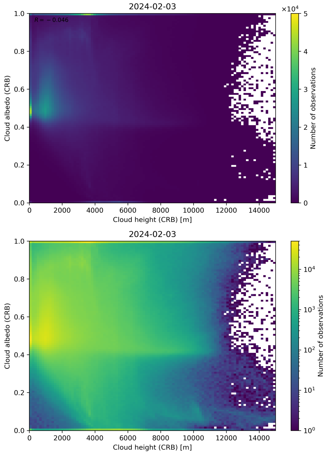
Figure 80: Scatter density plot of “Cloud height (CRB)” against “Cloud albedo (CRB)” for 2024-02-02 to 2024-02-04.
