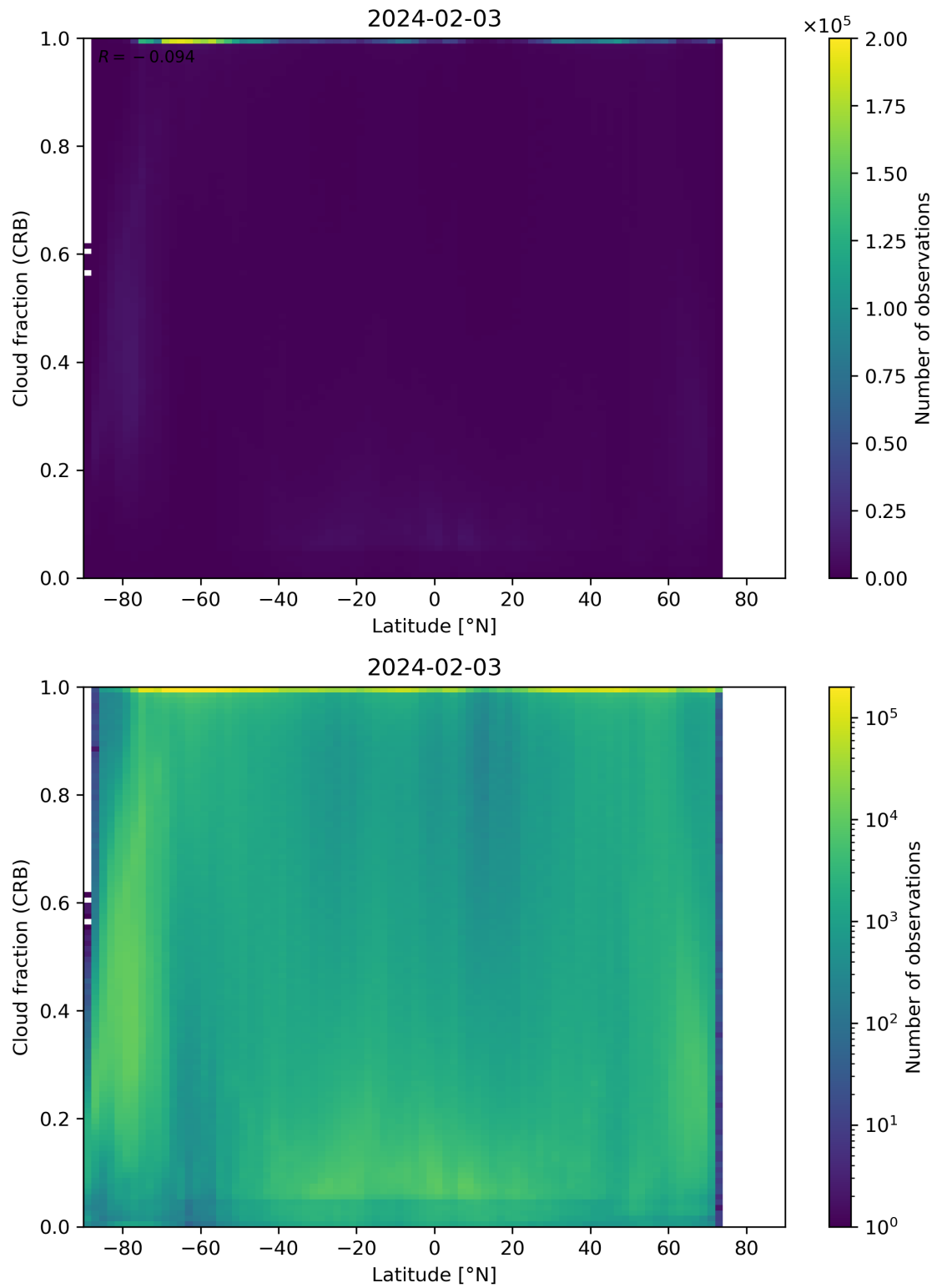
Figure 94: Scatter density plot of “Latitude” against “Cloud fraction (CRB)” for 2024-02-02 to 2024-02-04.
