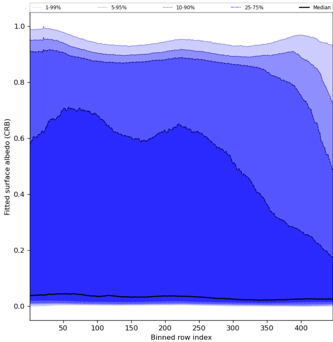
Figure 62: Along track statistics of “Fitted surface albedo (CRB)” for 2024-02-02 to 2024-02-04
