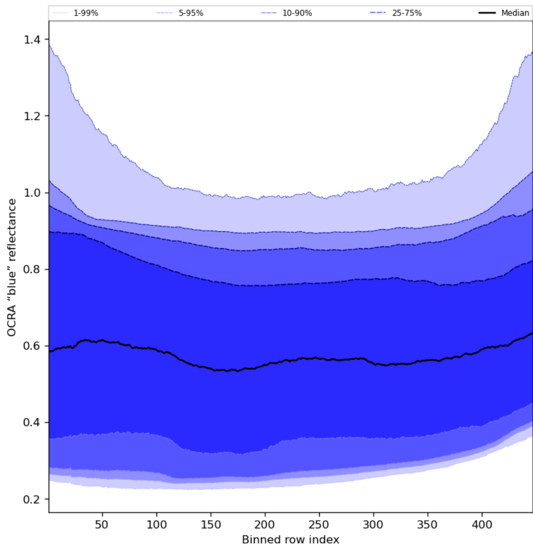
Figure 67: Along track statistics of “OCRA “blue” reflectance” for 2024-02-02 to 2024-02-04
