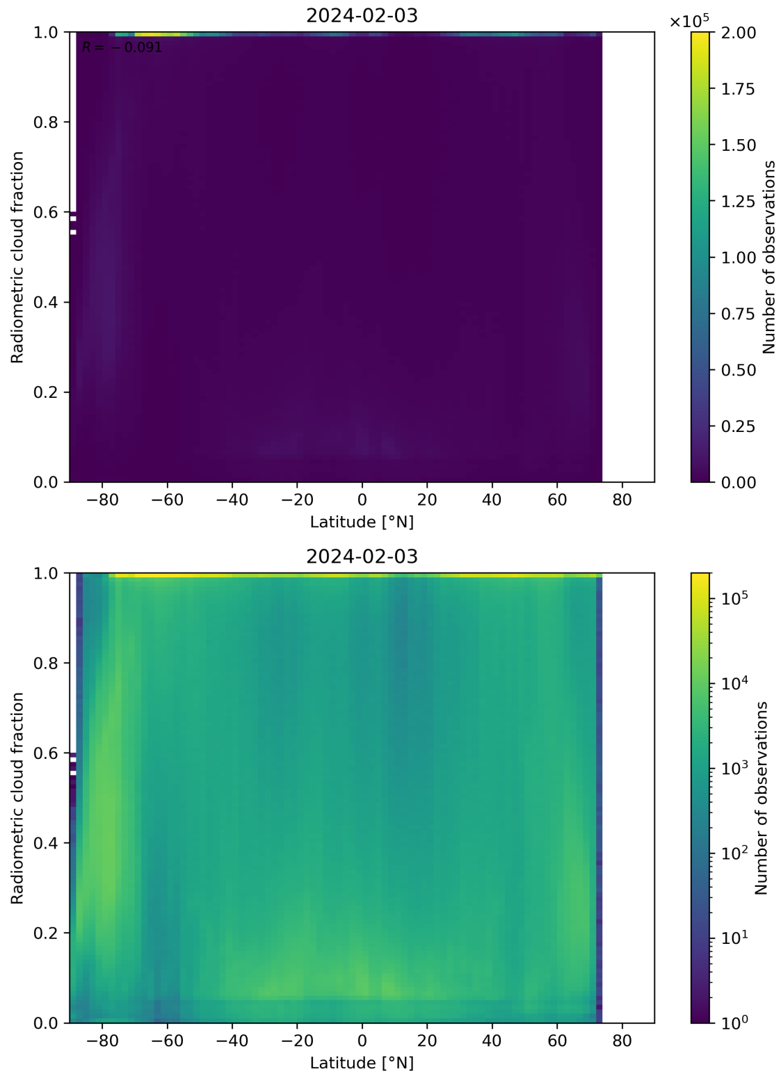
Figure 92: Scatter density plot of “Latitude” against “Radiometric cloud fraction” for 2024-02-02 to 2024-02-04.
