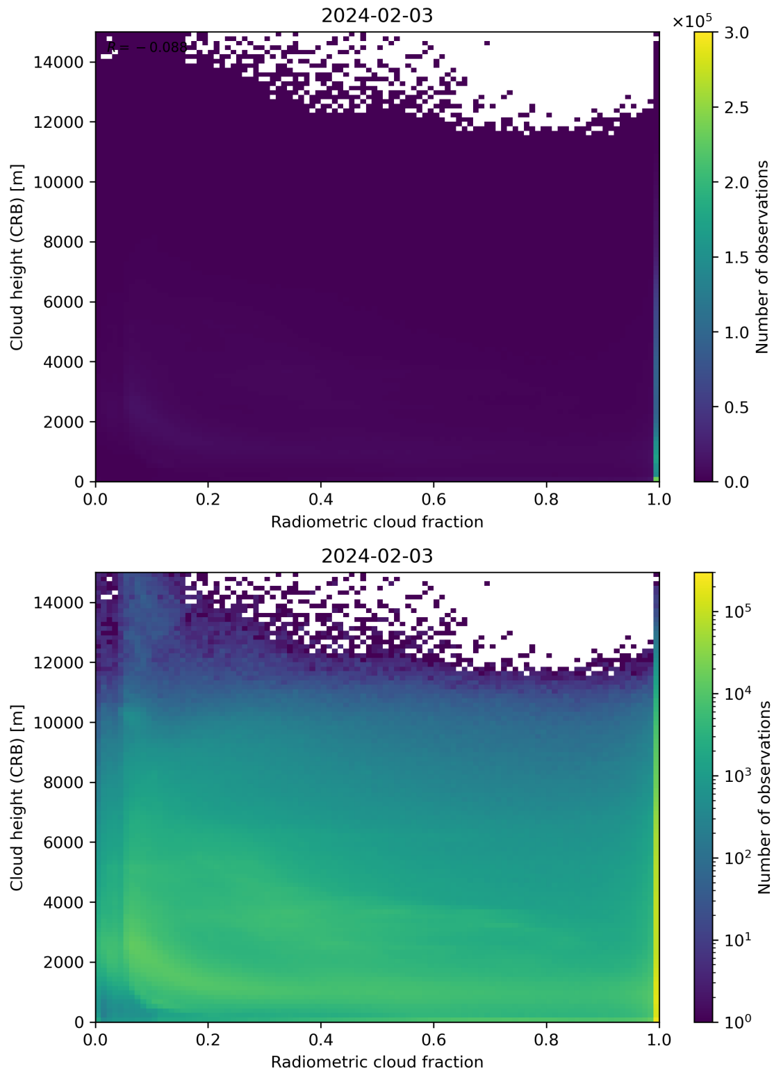
Figure 74: Scatter density plot of “Radiometric cloud fraction” against “Cloud height (CRB)” for 2024-02-02 to 2024-02-04.
