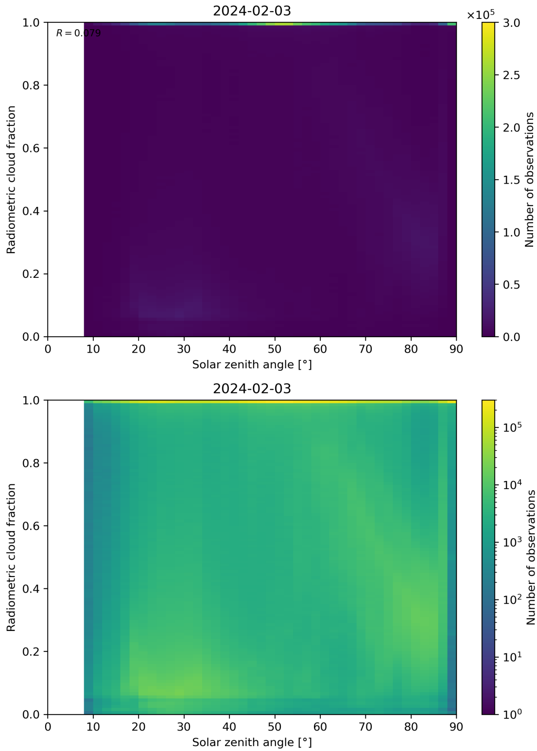
Figure 99: Scatter density plot of “Solar zenith angle” against “Radiometric cloud fraction” for 2024-02-02 to 2024-02-04.
