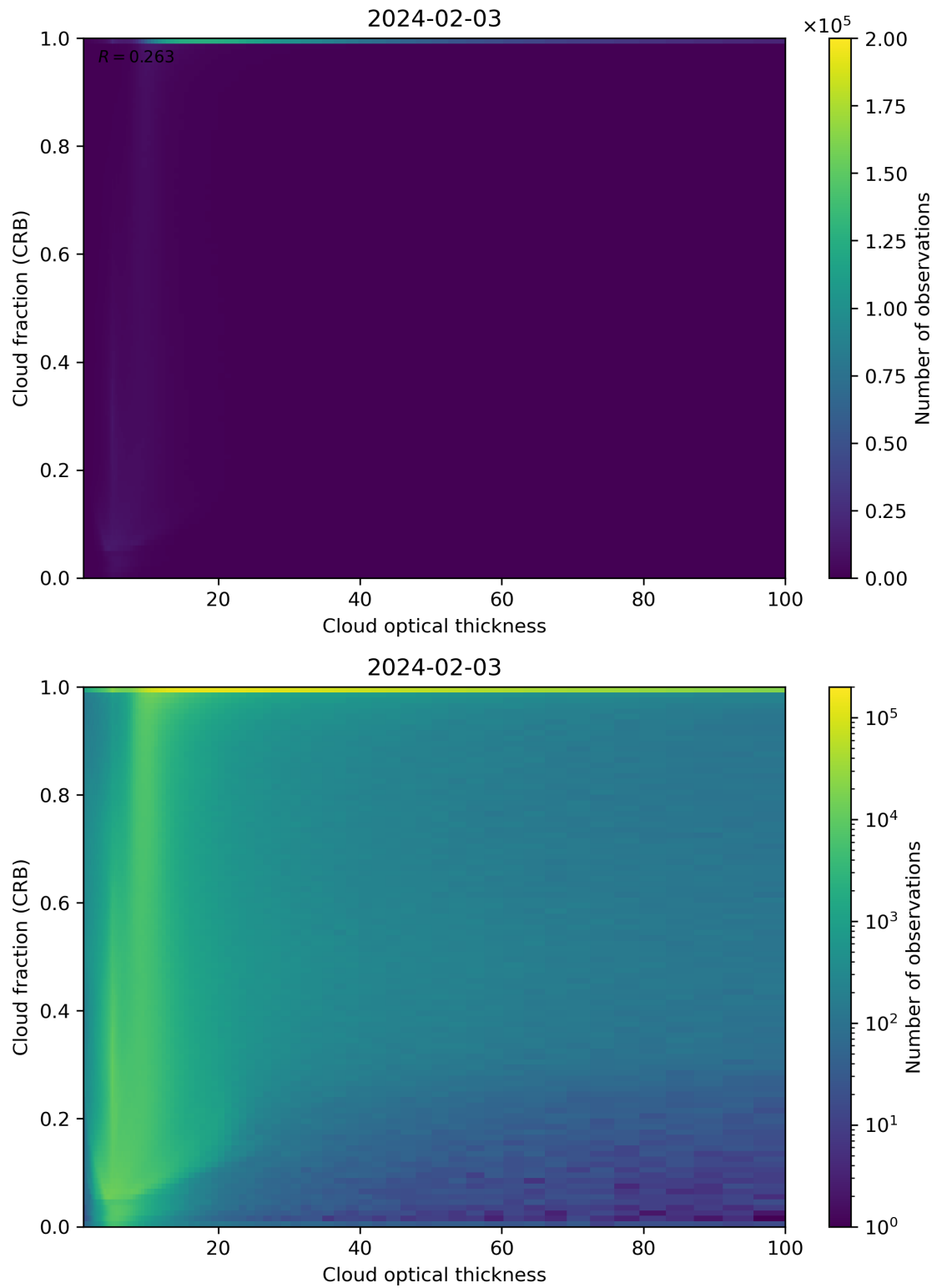
Figure 84: Scatter density plot of “Cloud optical thickness” against “Cloud fraction (CRB)” for 2024-02-02 to 2024-02-04.
