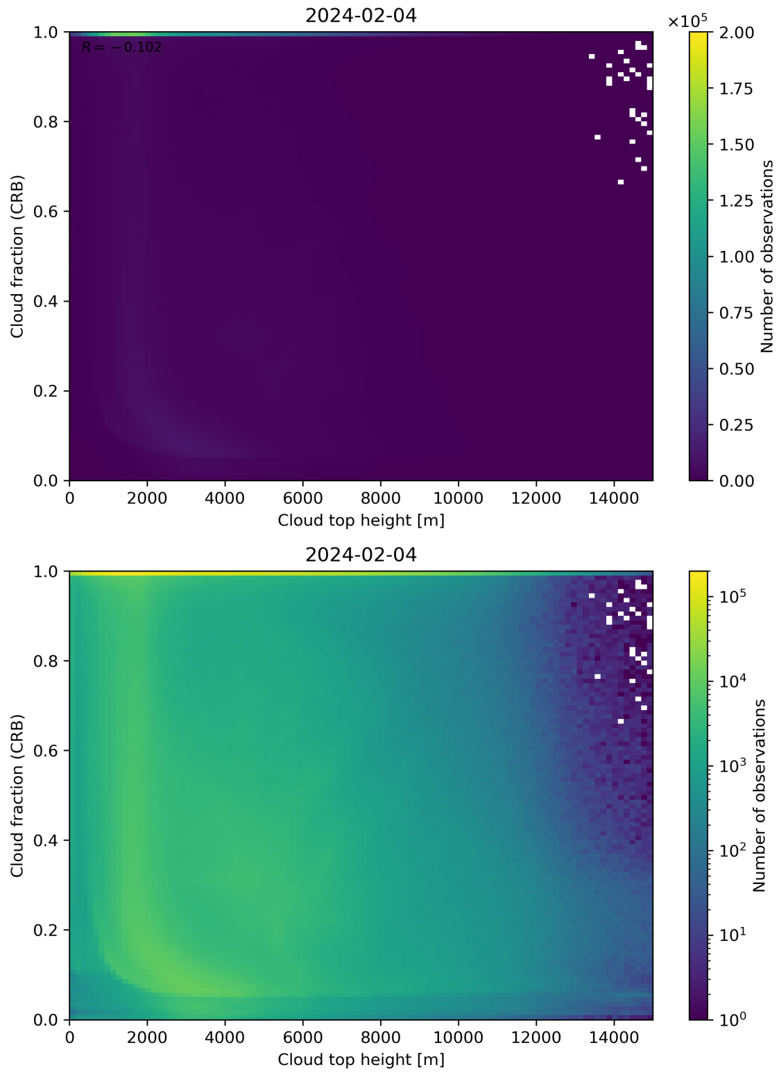
Figure 88: Scatter density plot of “Cloud top height” against “Cloud fraction (CRB)” for 2024-02-03 to 2024-02-05.
