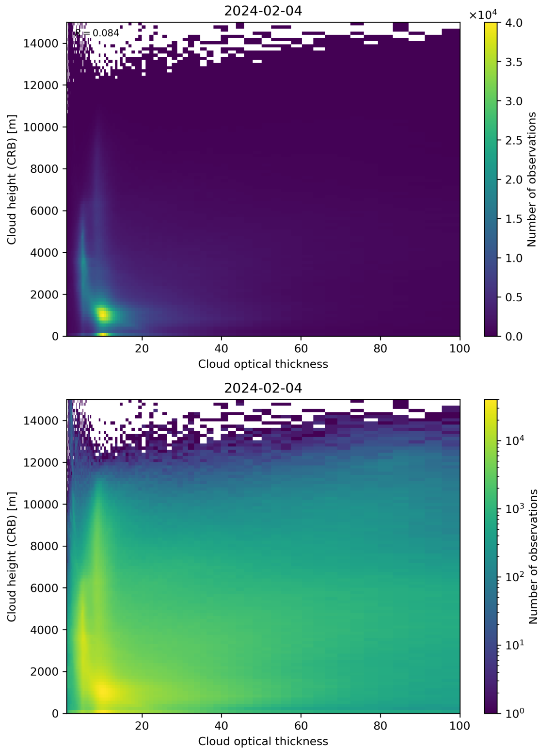
Figure 85: Scatter density plot of “Cloud optical thickness” against “Cloud height (CRB)” for 2024-02-03 to 2024-02-05.
