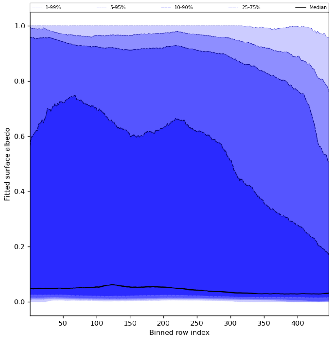
Figure 61: Along track statistics of “Fitted surface albedo” for 2024-02-03 to 2024-02-05
