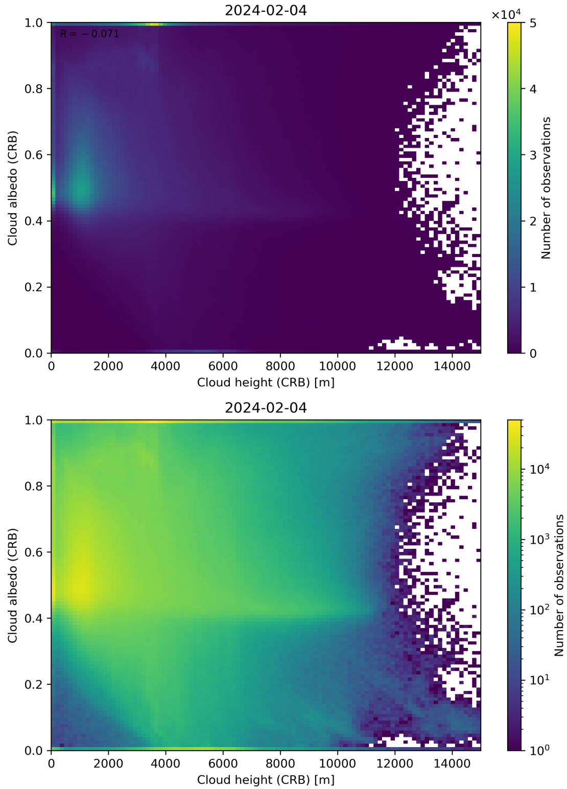
Figure 80: Scatter density plot of “Cloud height (CRB)” against “Cloud albedo (CRB)” for 2024-02-03 to 2024-02-05.
