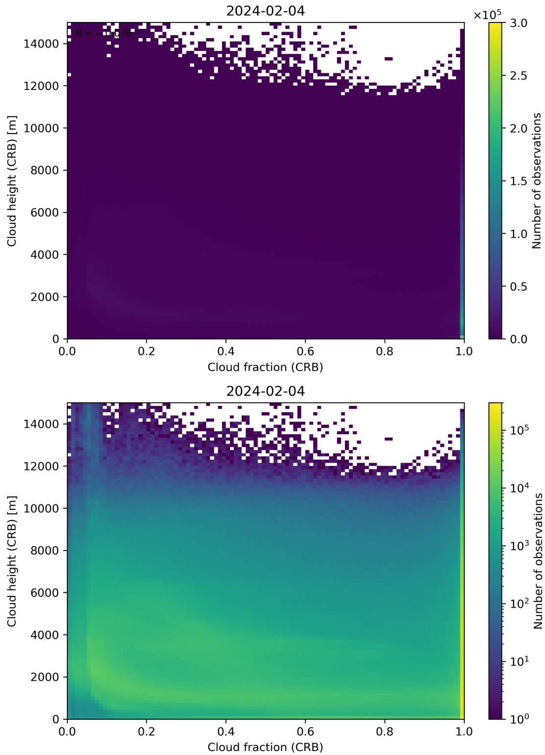
Figure 79: Scatter density plot of “Cloud fraction (CRB)” against “Cloud height (CRB)” for 2024-02-03 to 2024-02-05.
