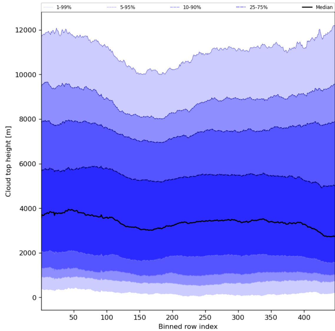
Figure 56: Along track statistics of “Cloud top height” for 2024-02-03 to 2024-02-05
