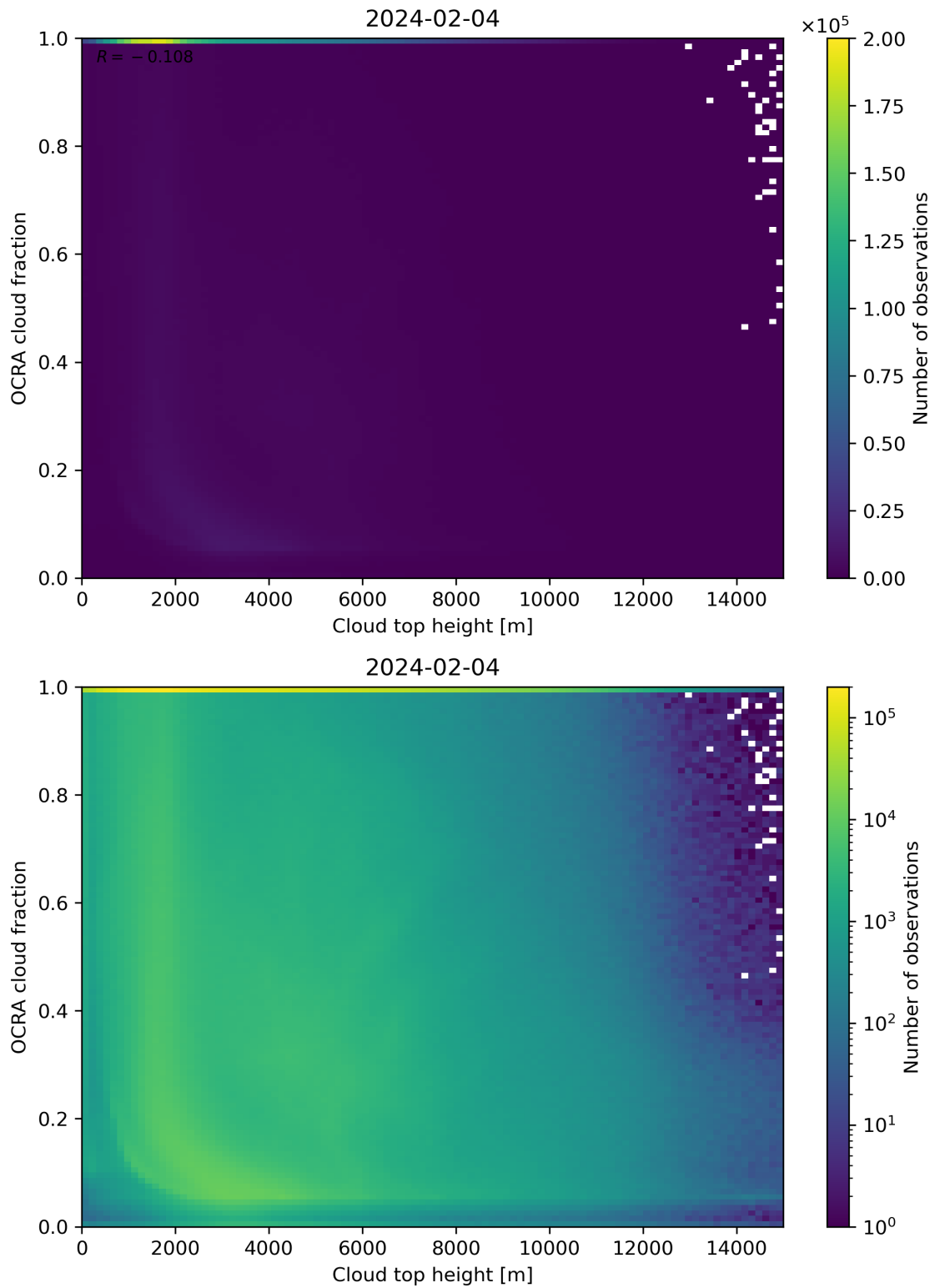
Figure 87: Scatter density plot of “Cloud top height” against “OCRA cloud fraction” for 2024-02-03 to 2024-02-05.
