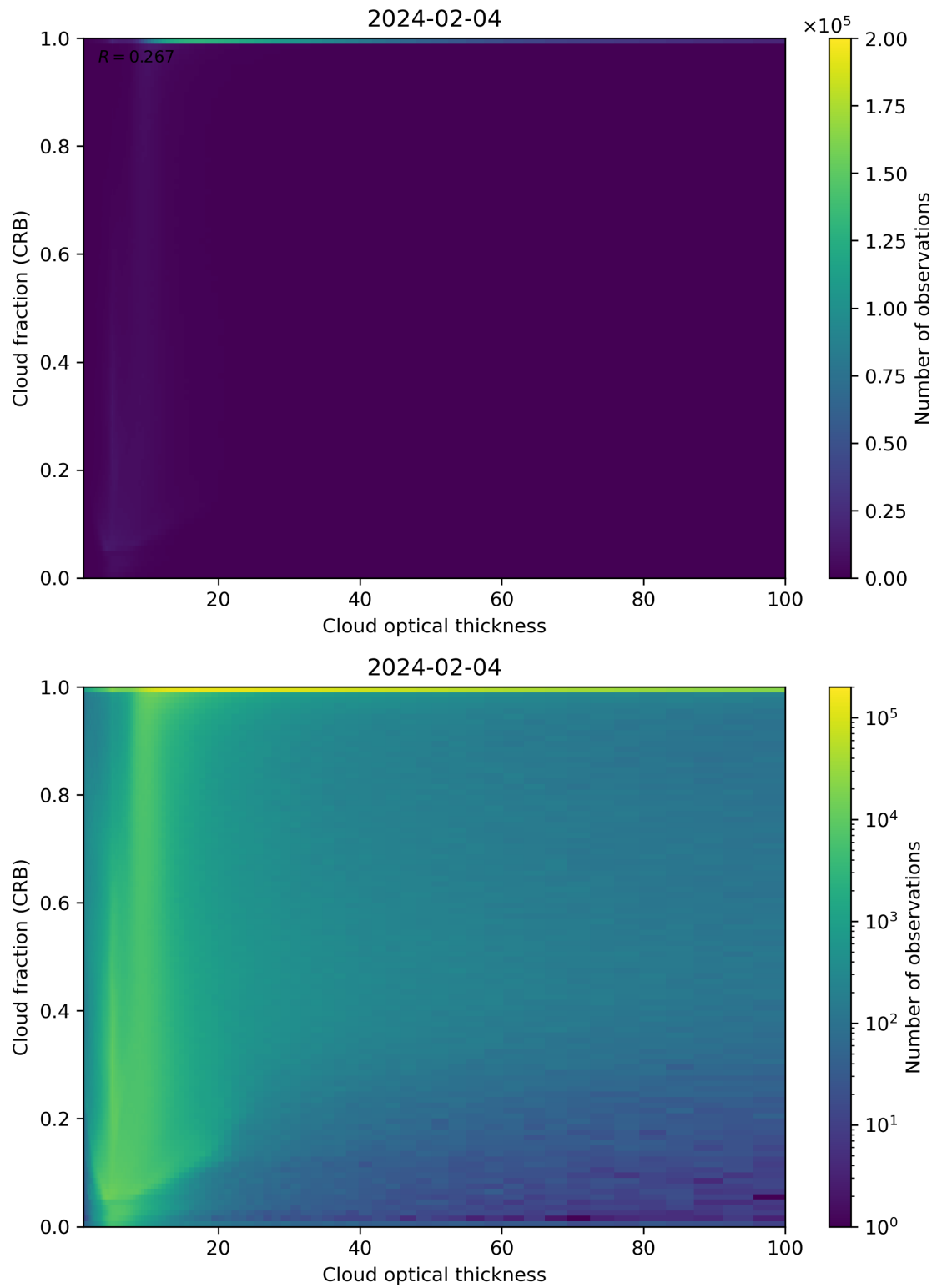
Figure 84: Scatter density plot of “Cloud optical thickness” against “Cloud fraction (CRB)” for 2024-02-03 to 2024-02-05.
