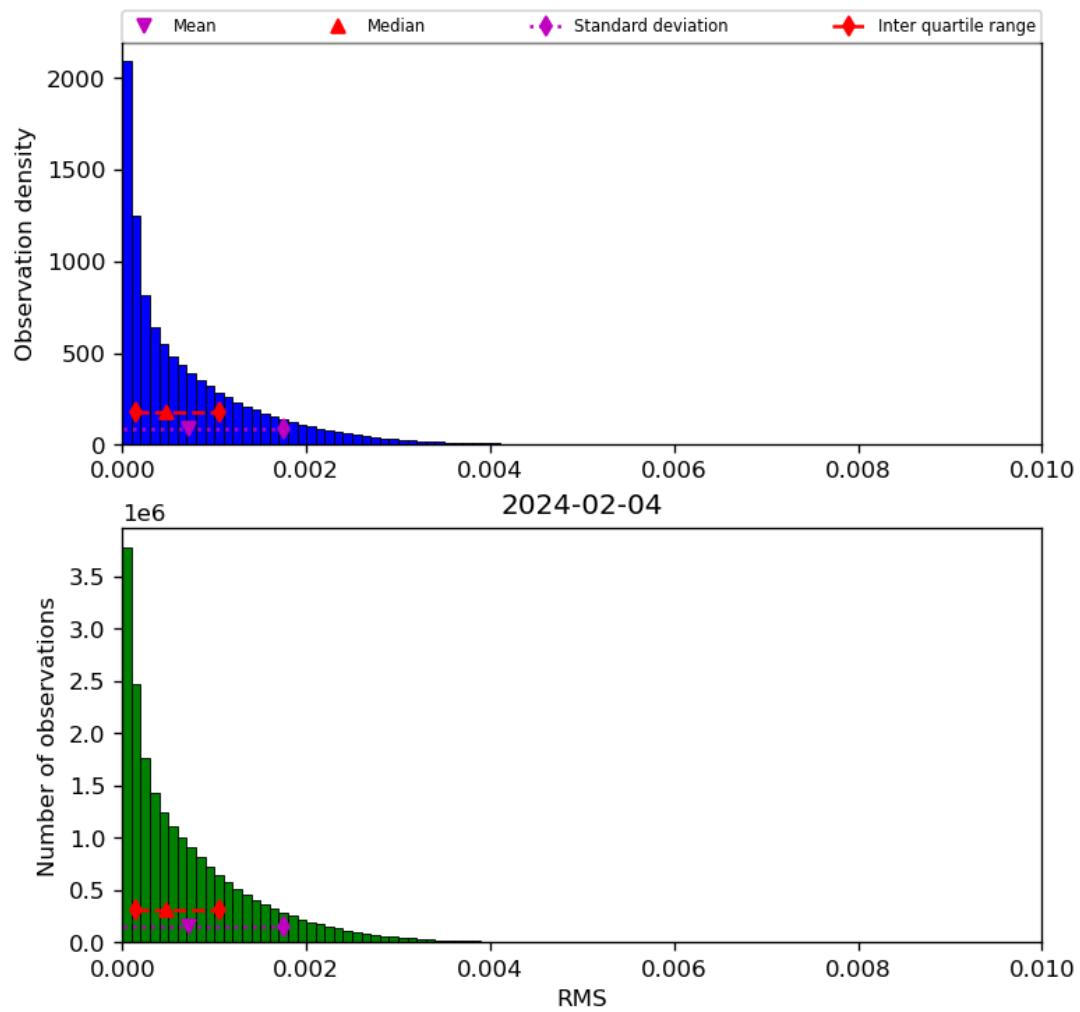
Figure 47: Histogram of “RMS” for 2024-02-03 to 2024-02-05
