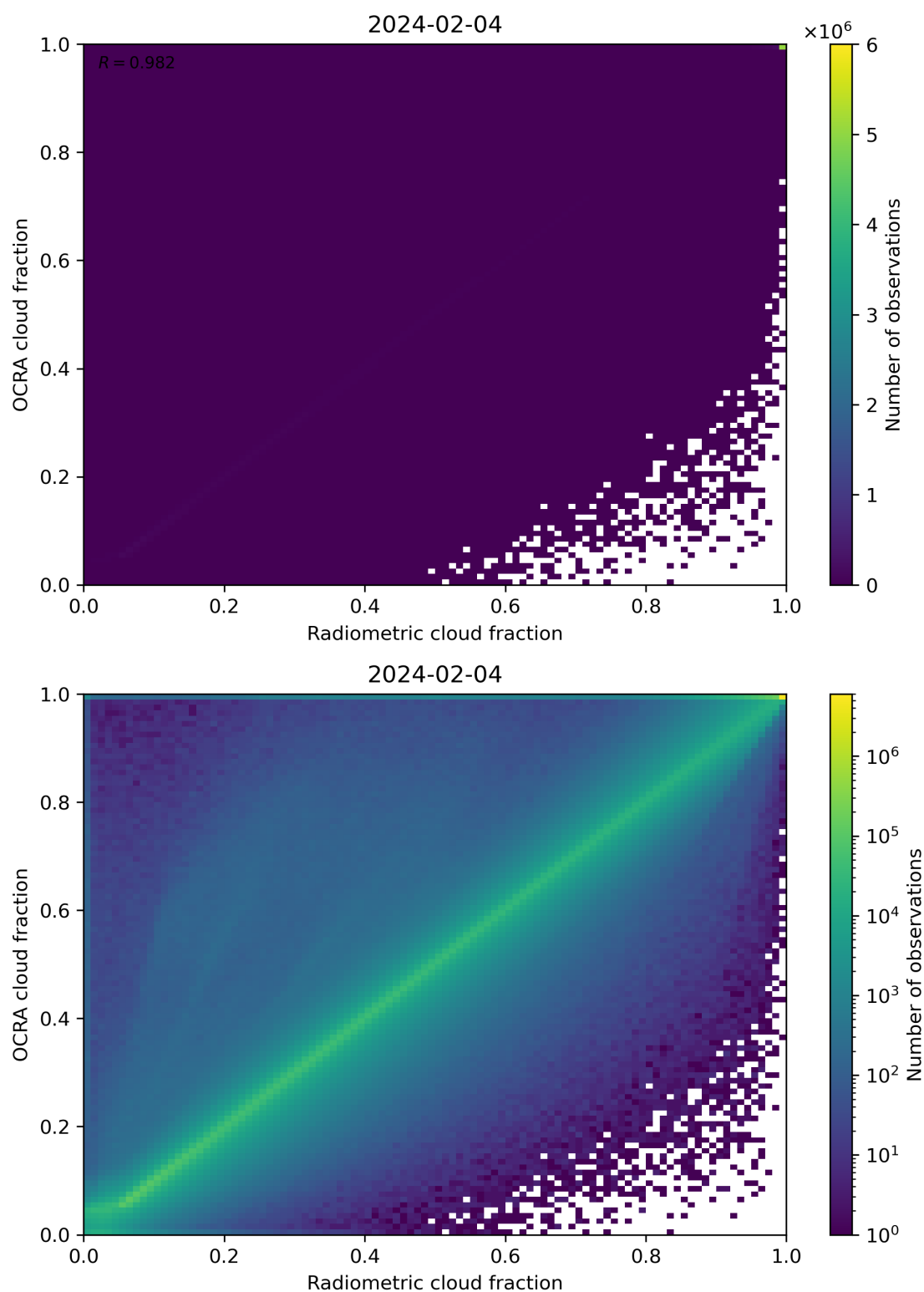
Figure 72: Scatter density plot of “Radiometric cloud fraction” against “OCRA cloud fraction” for 2024-02-03 to 2024-02-05.
