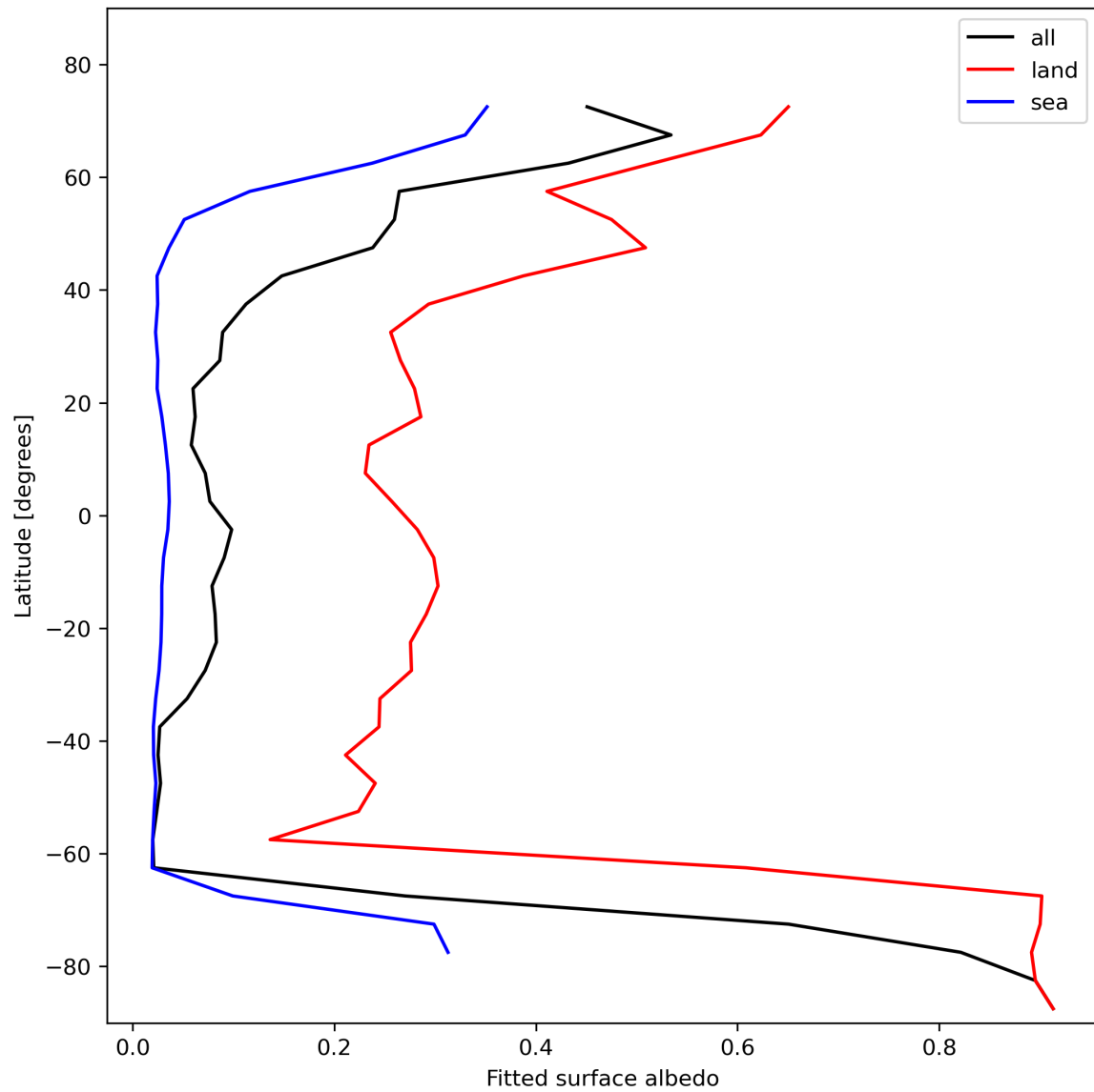
Figure 29: Zonal average of “Fitted surface albedo” for 2024-02-03 to 2024-02-05.
