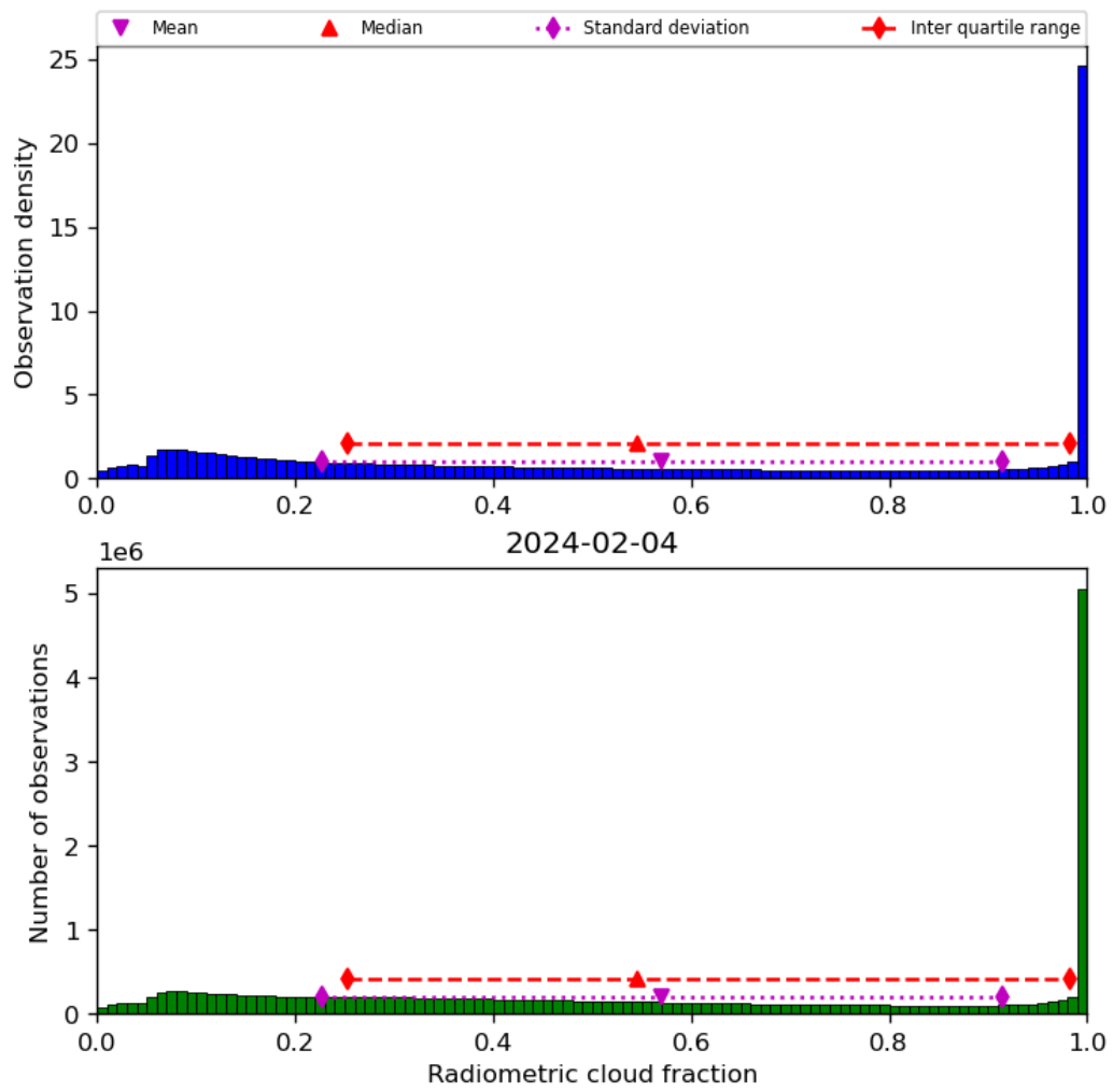
Figure 39: Histogram of “Radiometric cloud fraction” for 2024-02-03 to 2024-02-05
