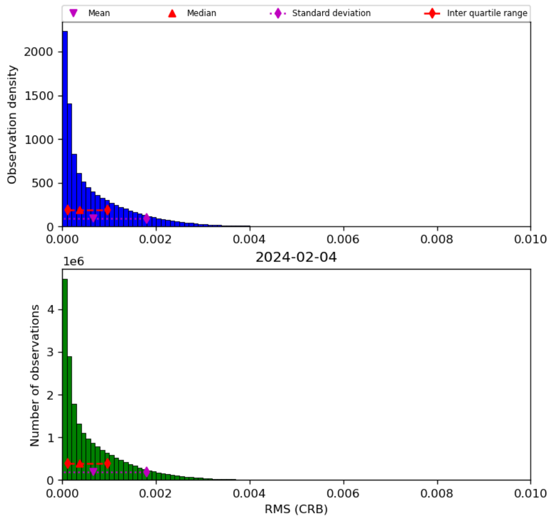
Figure 48: Histogram of “RMS (CRB)” for 2024-02-03 to 2024-02-05
