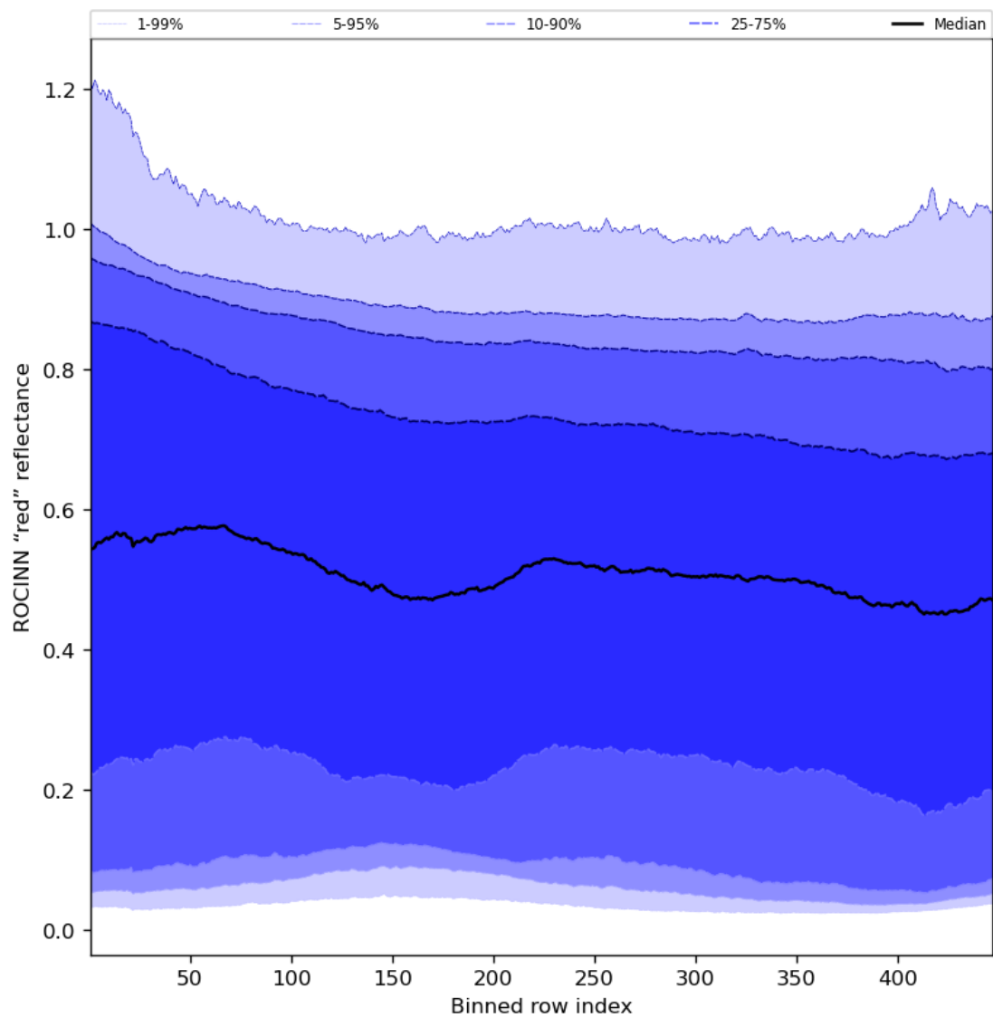
Figure 69: Along track statistics of “ROCINN “red” reflectance” for 2024-02-03 to 2024-02-05
