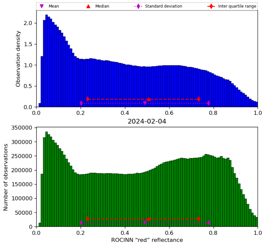
Figure 53: Histogram of “ROCINN “red” reflectance” for 2024-02-03 to 2024-02-05
