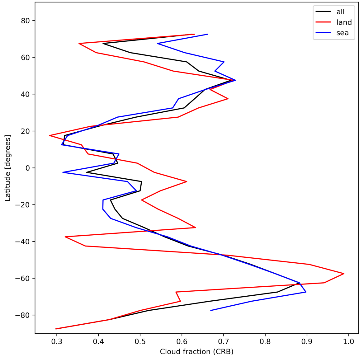
Figure 26: Zonal average of “Cloud fraction (CRB)” for 2024-02-03 to 2024-02-05.
