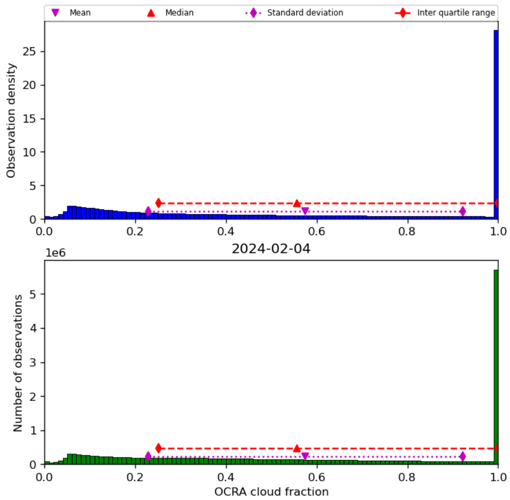
Figure 50: Histogram of “OCRA cloud fraction” for 2024-02-03 to 2024-02-05
