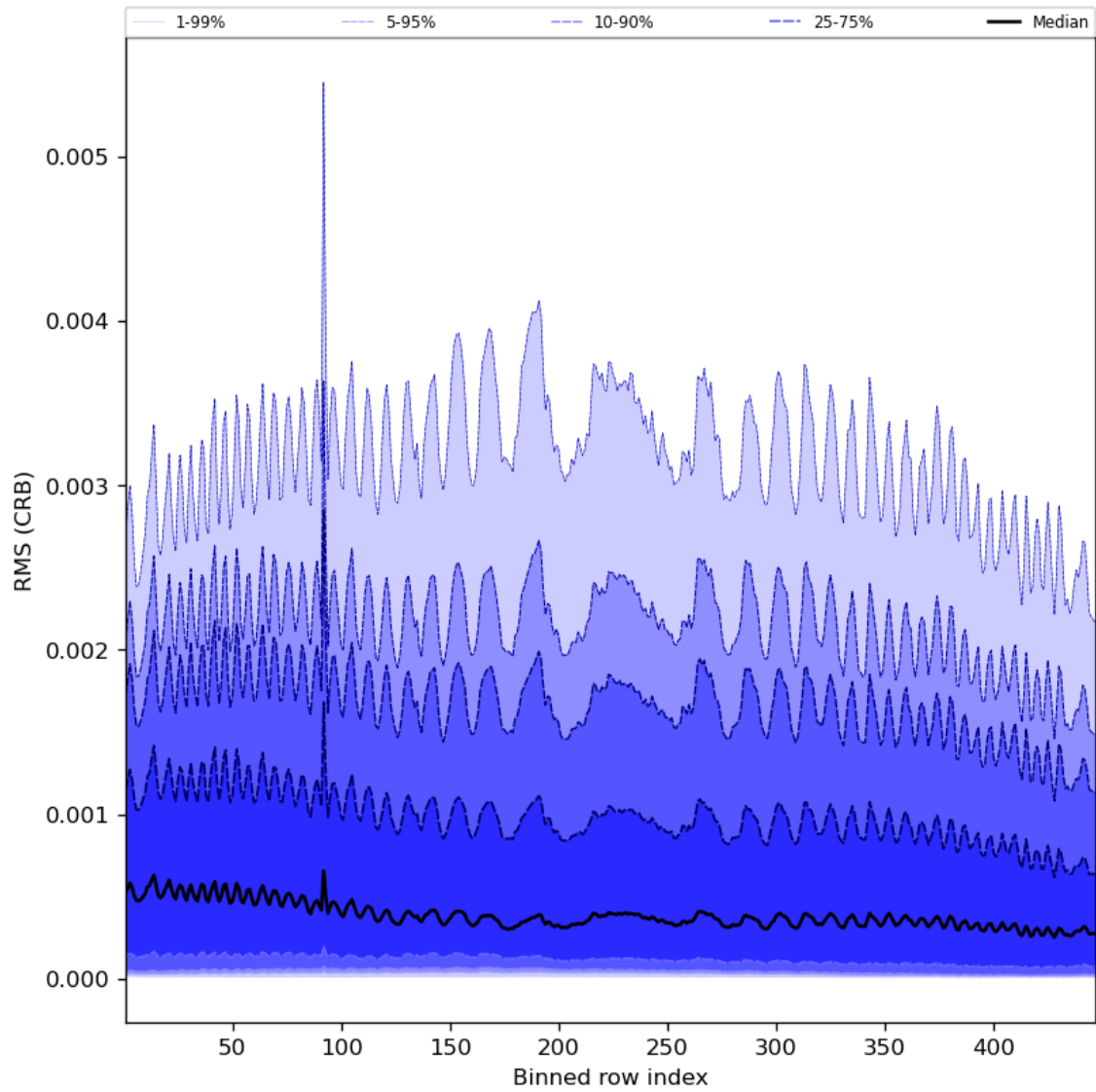
Figure 64: Along track statistics of “RMS (CRB)” for 2024-02-03 to 2024-02-05
