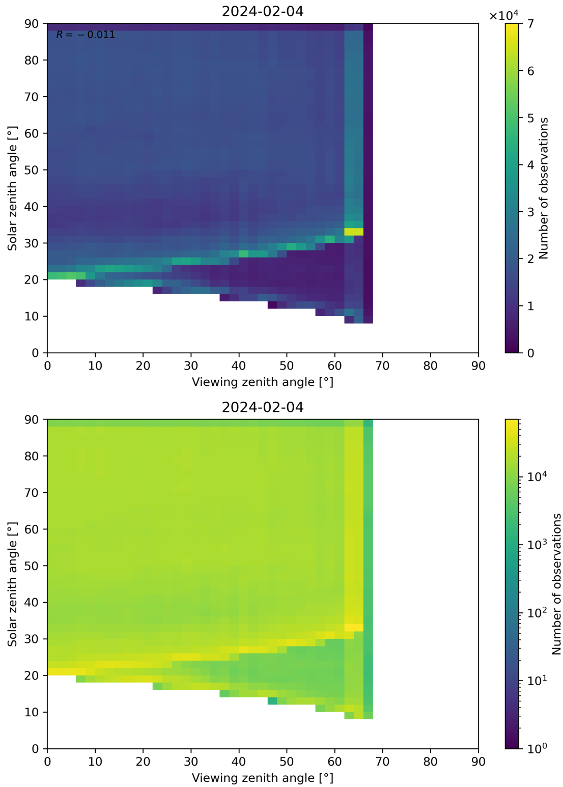
Figure 114: Scatter density plot of “Viewing zenith angle” against “Solar zenith angle” for 2024-02-03 to 2024-02-05.
