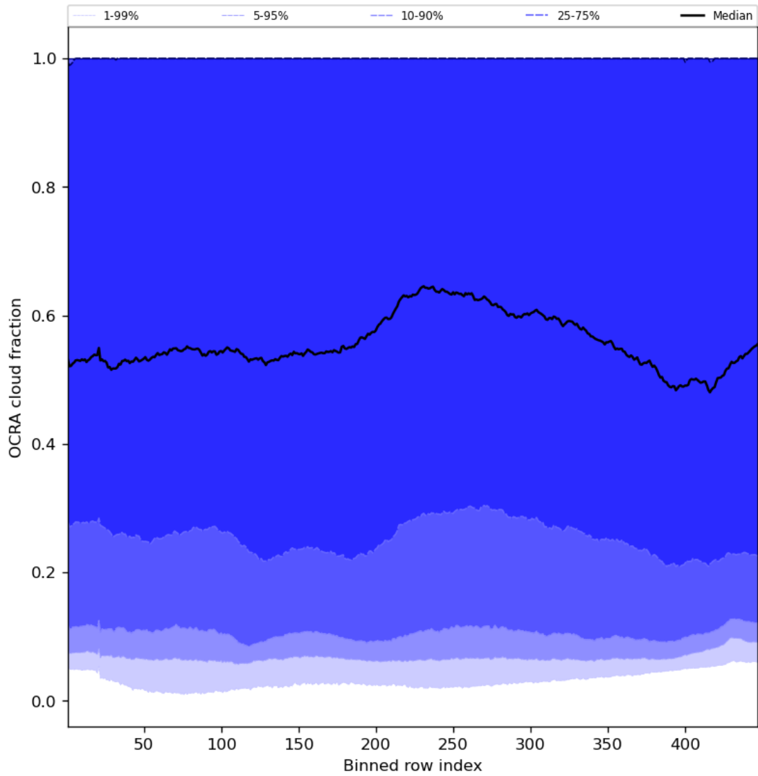
Figure 66: Along track statistics of “OCRA cloud fraction” for 2024-02-03 to 2024-02-05
