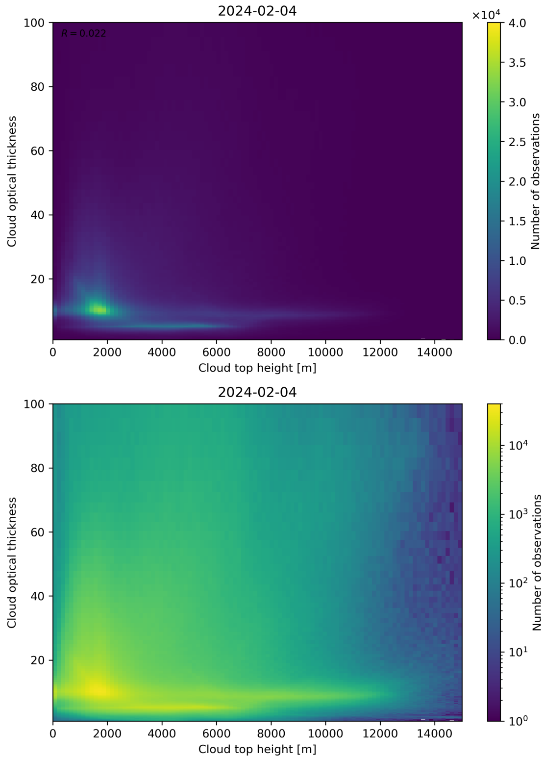
Figure 90: Scatter density plot of “Cloud top height” against “Cloud optical thickness” for 2024-02-03 to 2024-02-05.
