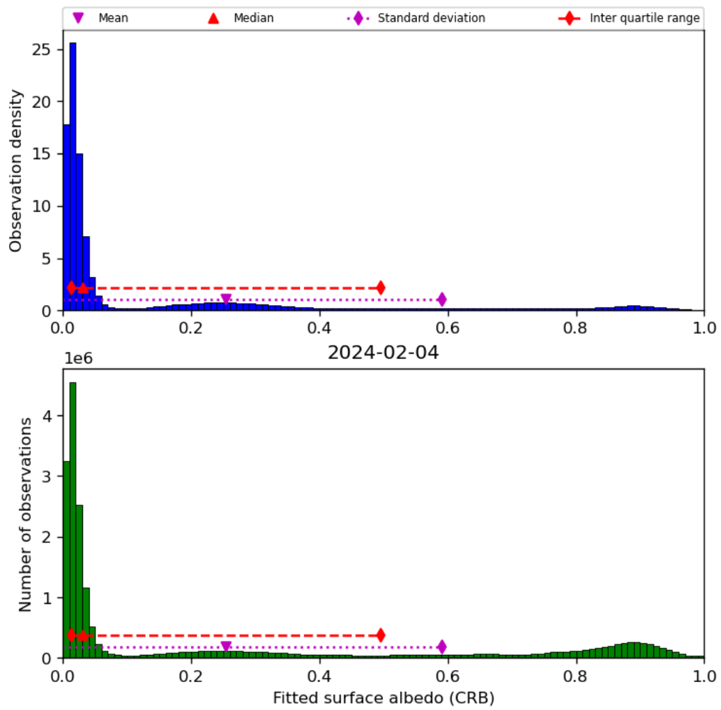
Figure 46: Histogram of “Fitted surface albedo (CRB)” for 2024-02-03 to 2024-02-05
