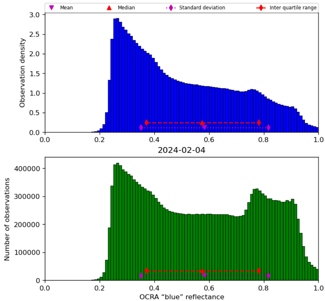
Figure 51: Histogram of “OCRA “blue” reflectance” for 2024-02-03 to 2024-02-05
