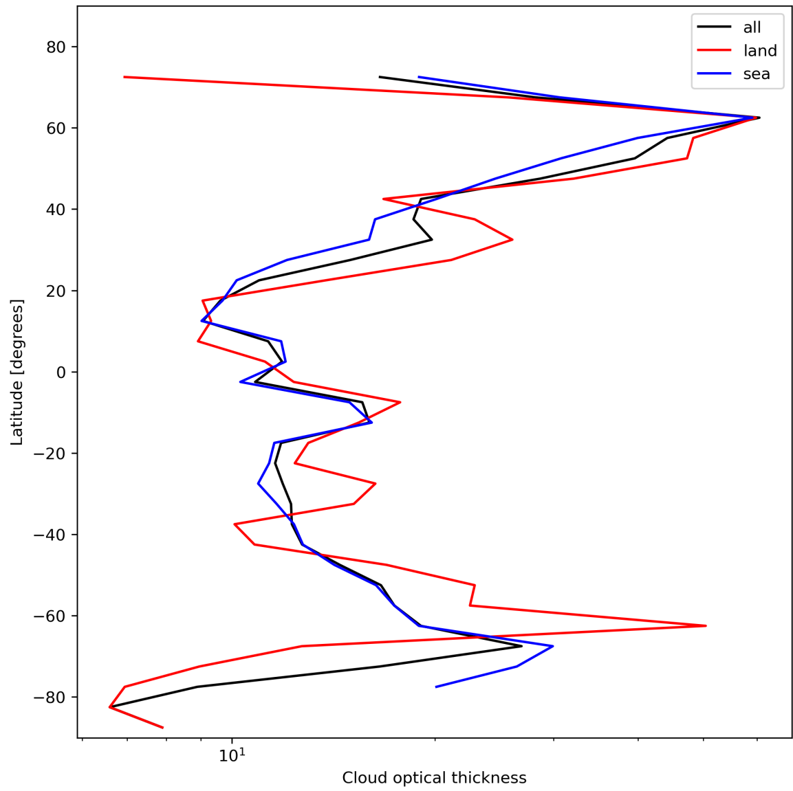
Figure 25: Zonal average of “Cloud optical thickness” for 2024-02-03 to 2024-02-05.
