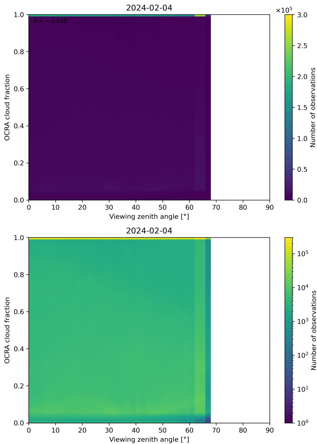
Figure 108: Scatter density plot of “Viewing zenith angle” against “OCRA cloud fraction” for 2024-02-03 to 2024-02-05.
