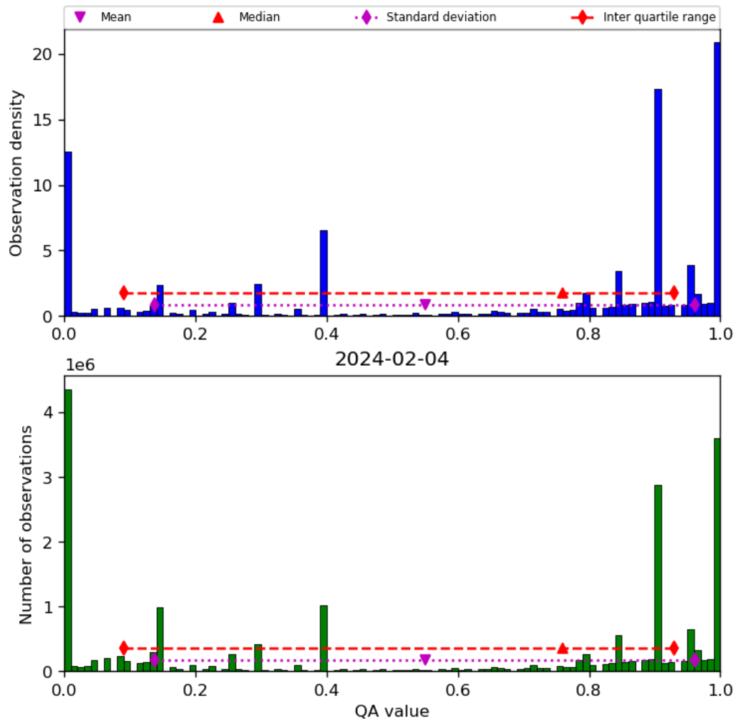
Figure 38: Histogram of “QA value” for 2024-02-03 to 2024-02-05
