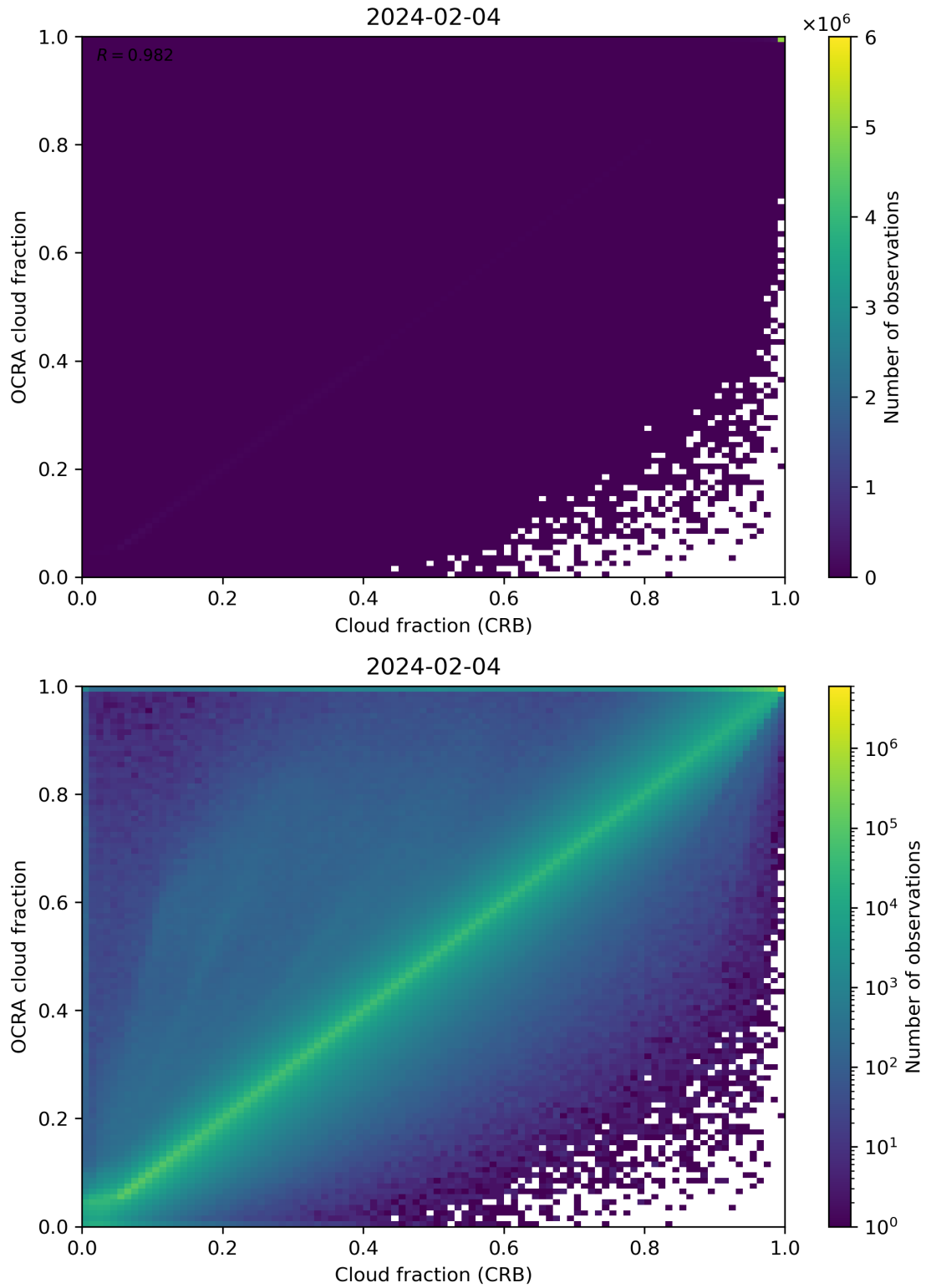
Figure 78: Scatter density plot of “Cloud fraction (CRB)” against “OCRA cloud fraction” for 2024-02-03 to 2024-02-05.
