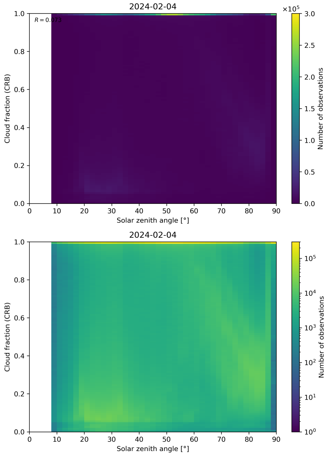
Figure 101: Scatter density plot of “Solar zenith angle” against “Cloud fraction (CRB)” for 2024-02-03 to 2024-02-05.
