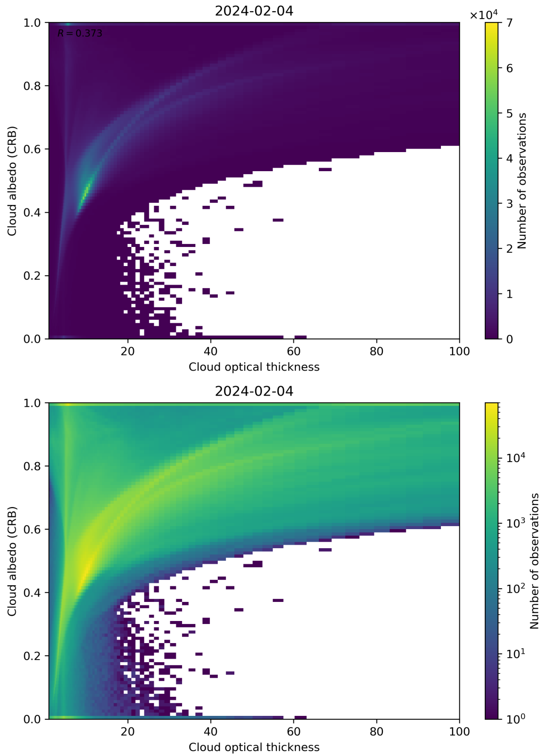
Figure 82: Scatter density plot of “Cloud optical thickness” against “Cloud albedo (CRB)” for 2024-02-03 to 2024-02-05.
