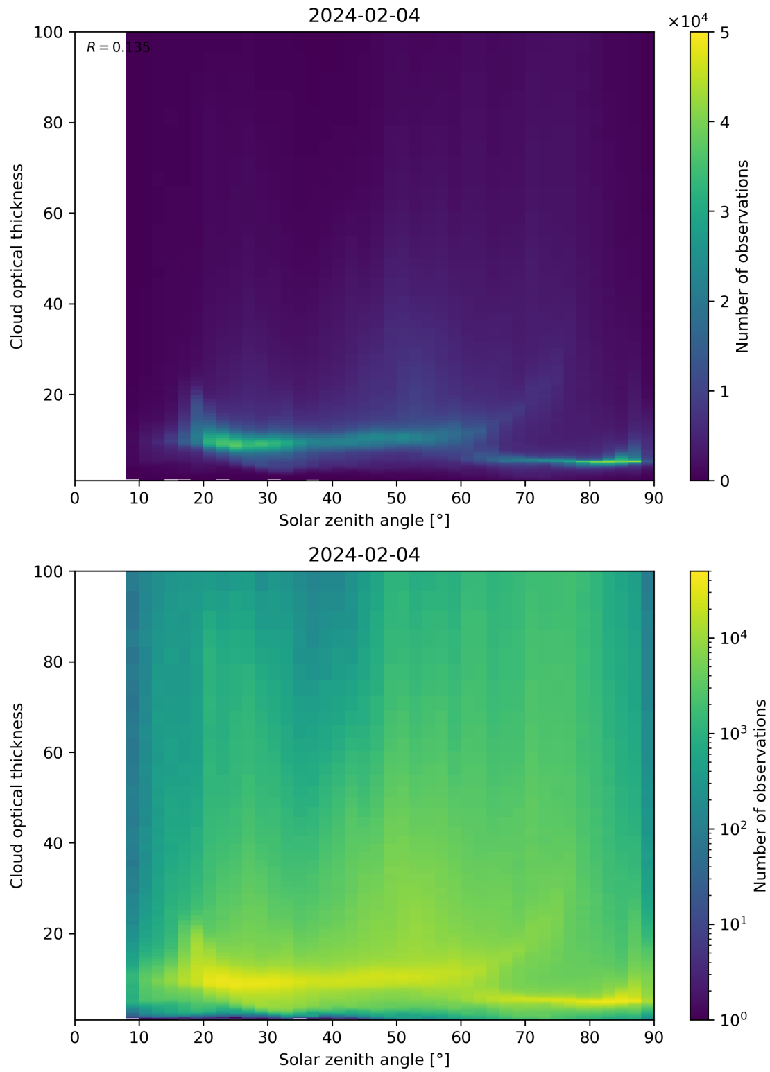
Figure 103: Scatter density plot of “Solar zenith angle” against “Cloud optical thickness” for 2024-02-03 to 2024-02-05.
