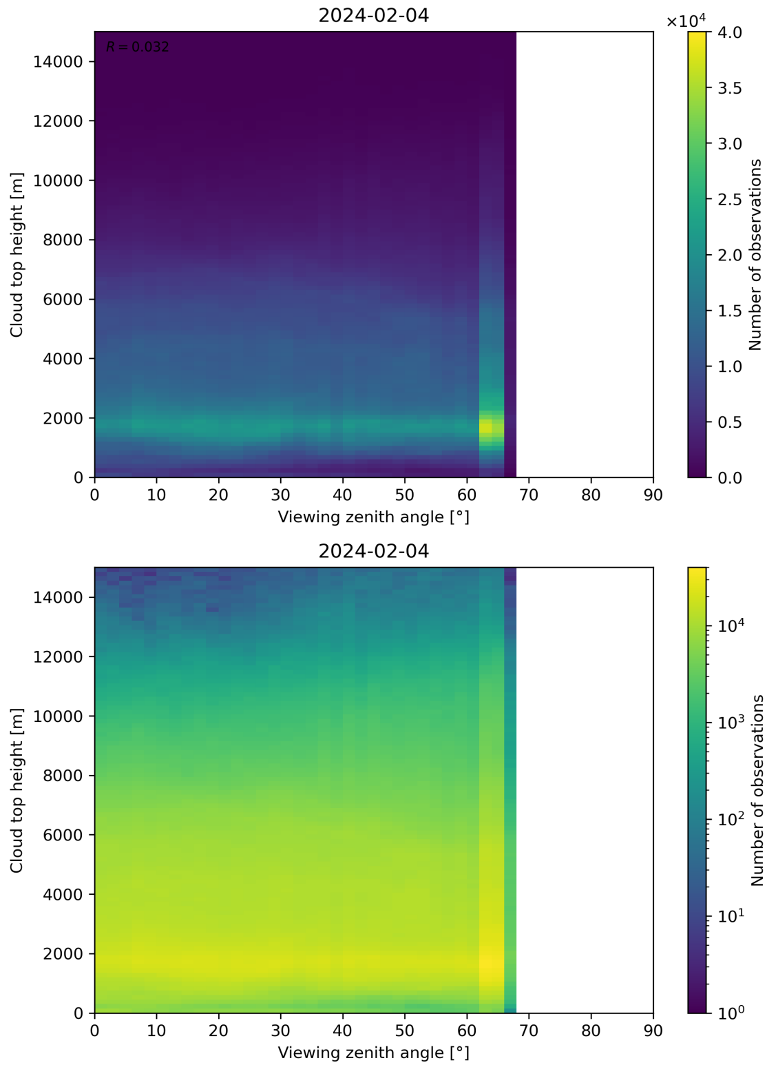
Figure 112: Scatter density plot of “Viewing zenith angle” against “Cloud top height” for 2024-02-03 to 2024-02-05.
