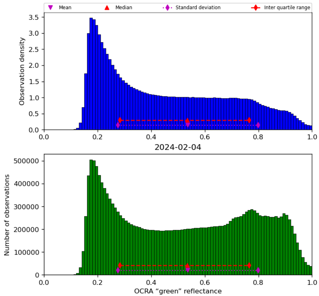
Figure 52: Histogram of “OCRA “green” reflectance” for 2024-02-03 to 2024-02-05
