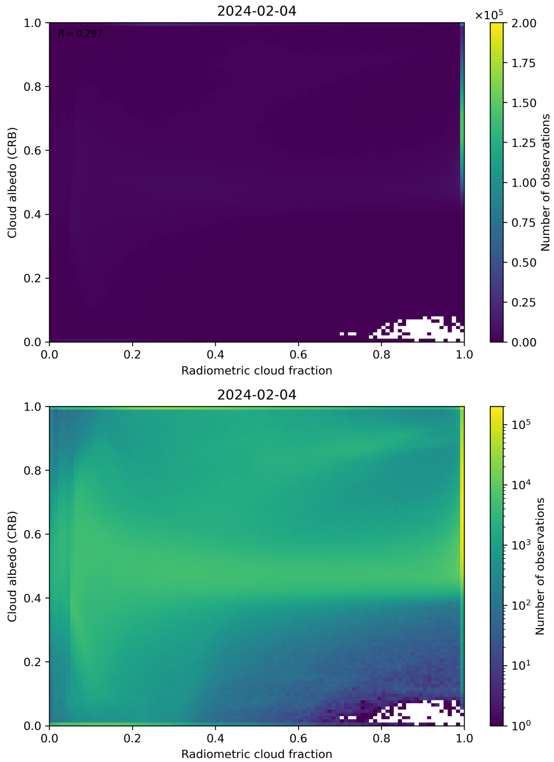
Figure 71: Scatter density plot of “Radiometric cloud fraction” against “Cloud albedo (CRB)” for 2024-02-03 to 2024-02-05.
