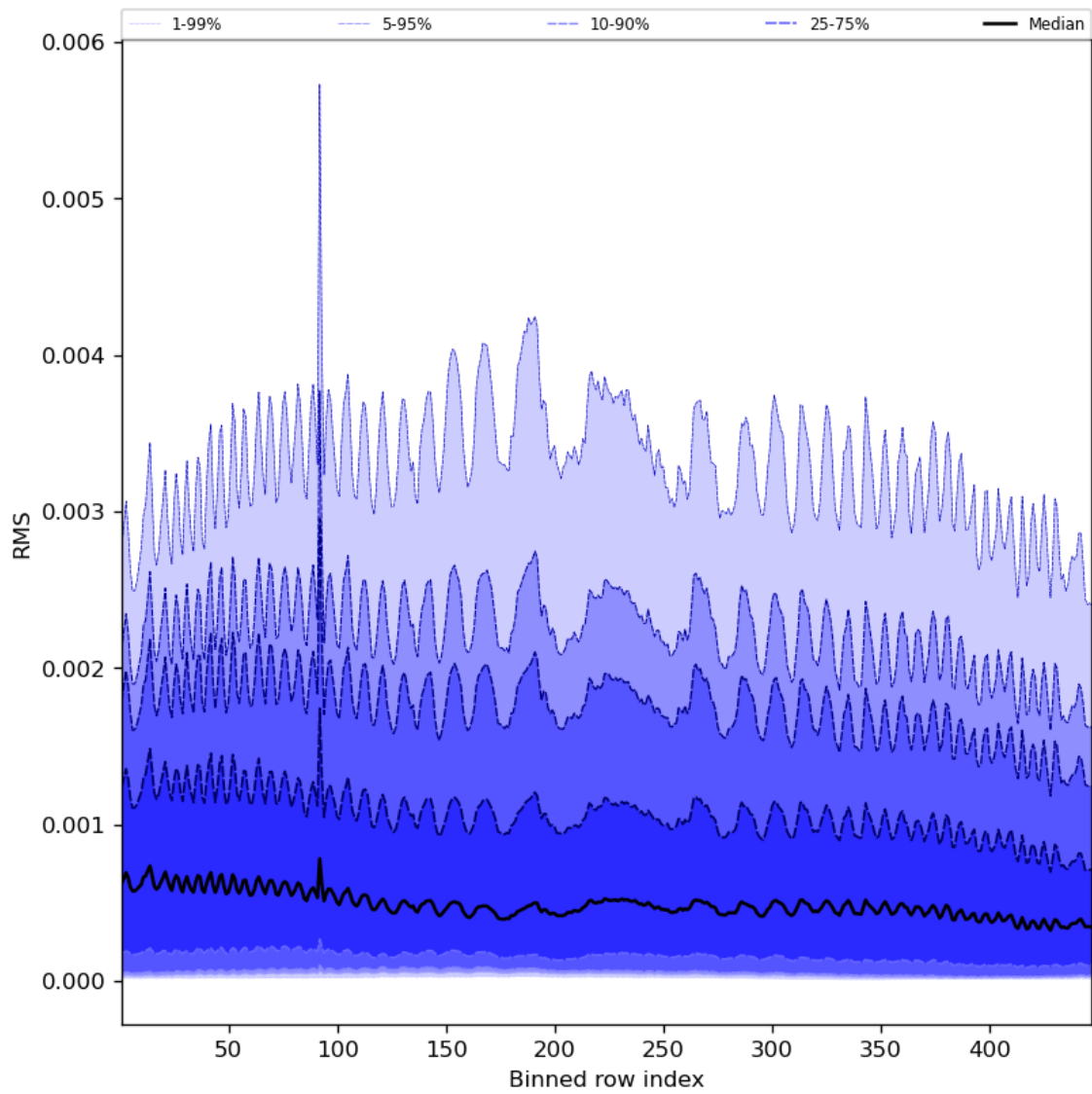
Figure 63: Along track statistics of “RMS” for 2024-02-03 to 2024-02-05
