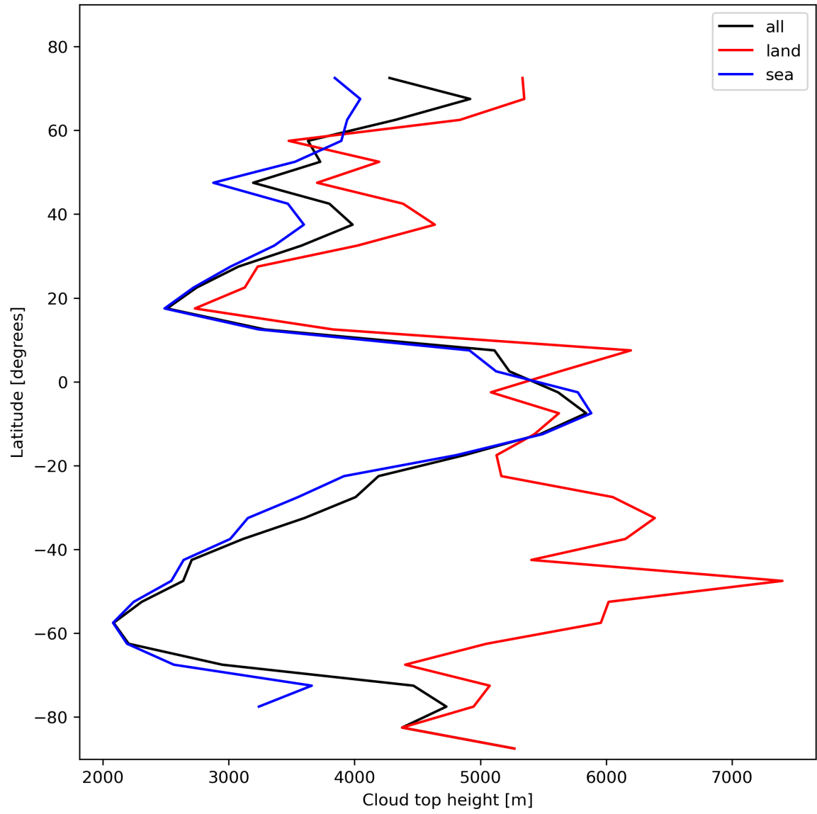
Figure 24: Zonal average of “Cloud top height” for 2024-02-03 to 2024-02-05.
