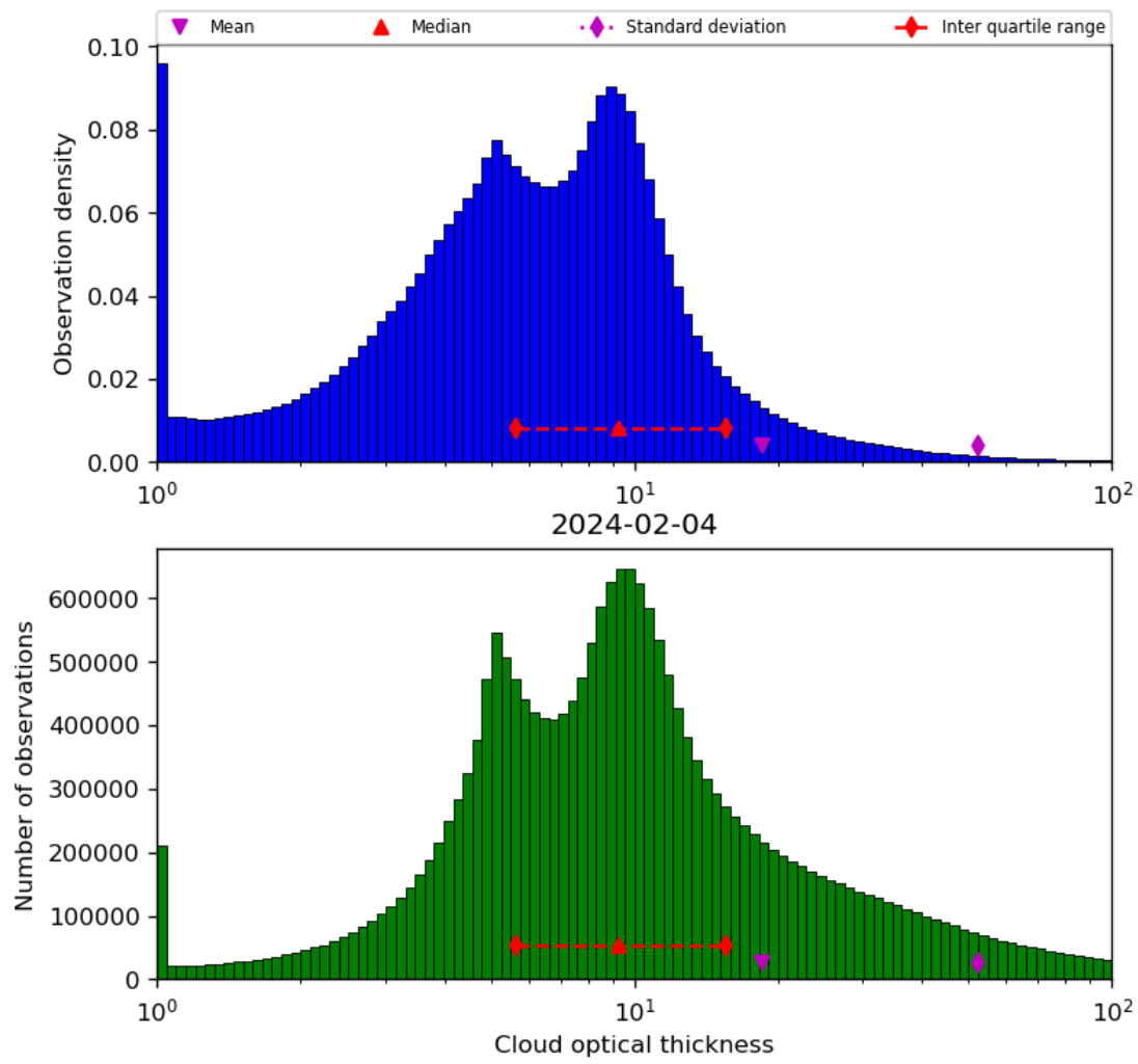
Figure 41: Histogram of “Cloud optical thickness” for 2024-02-03 to 2024-02-05
