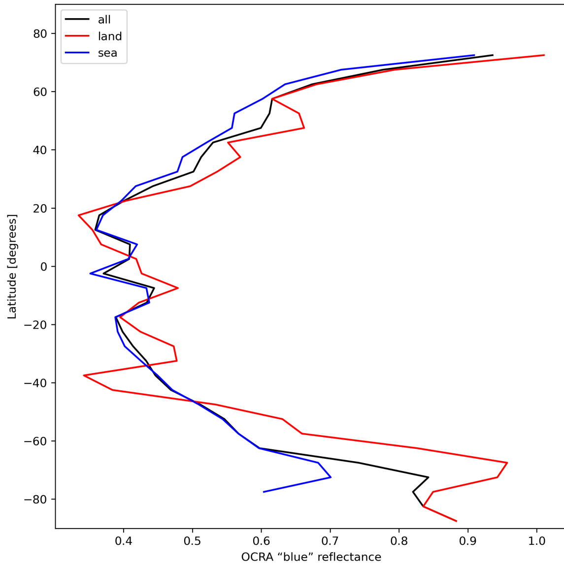
Figure 35: Zonal average of “OCRA “blue” reflectance” for 2024-02-03 to 2024-02-05.
