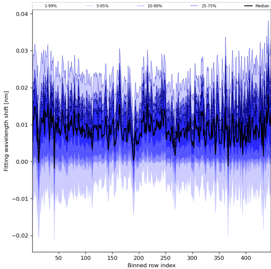
Figure 65: Along track statistics of “Fitting wavelength shift” for 2024-02-03 to 2024-02-05
