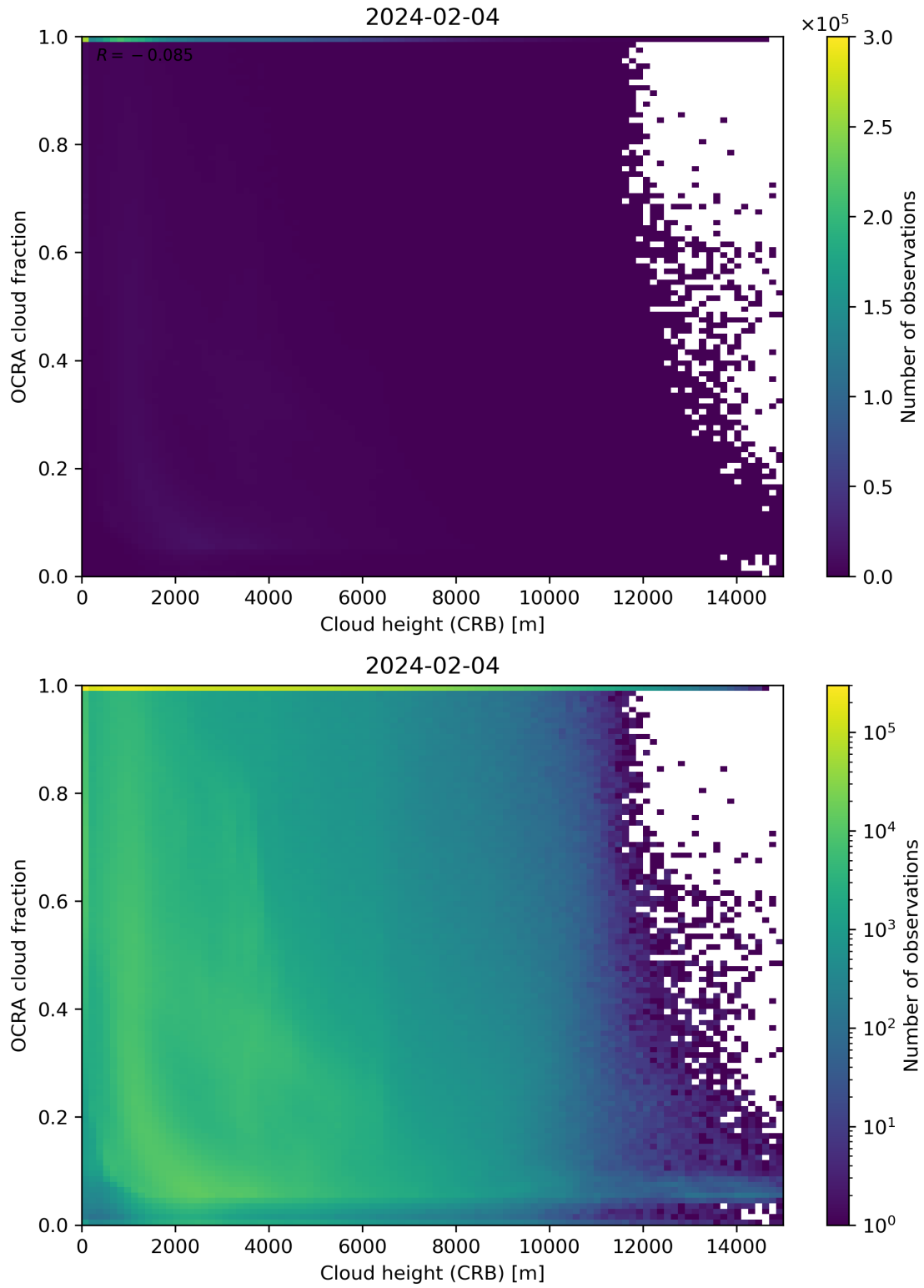
Figure 81: Scatter density plot of “Cloud height (CRB)” against “OCRA cloud fraction” for 2024-02-03 to 2024-02-05.
