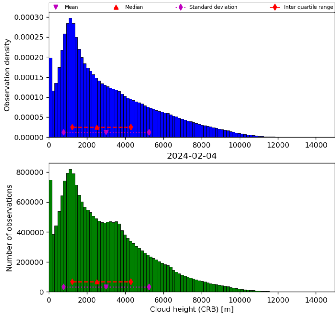
Figure 43: Histogram of “Cloud height (CRB)” for 2024-02-03 to 2024-02-05
