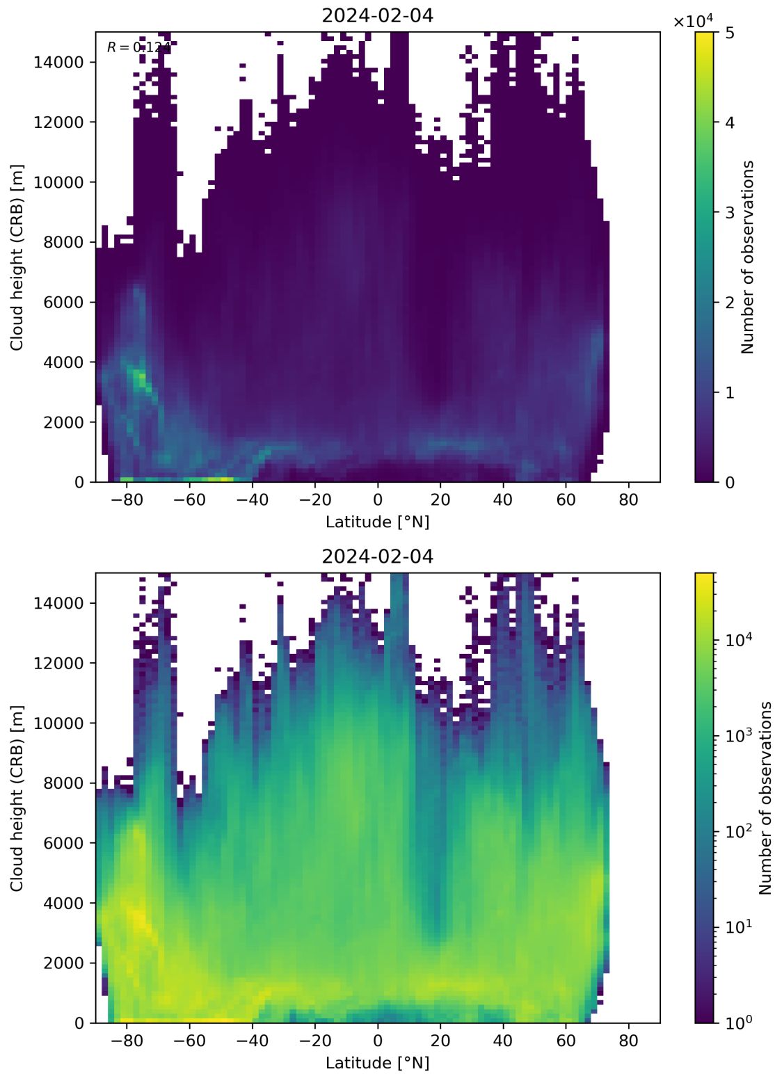
Figure 95: Scatter density plot of “Latitude” against “Cloud height (CRB)” for 2024-02-03 to 2024-02-05.
