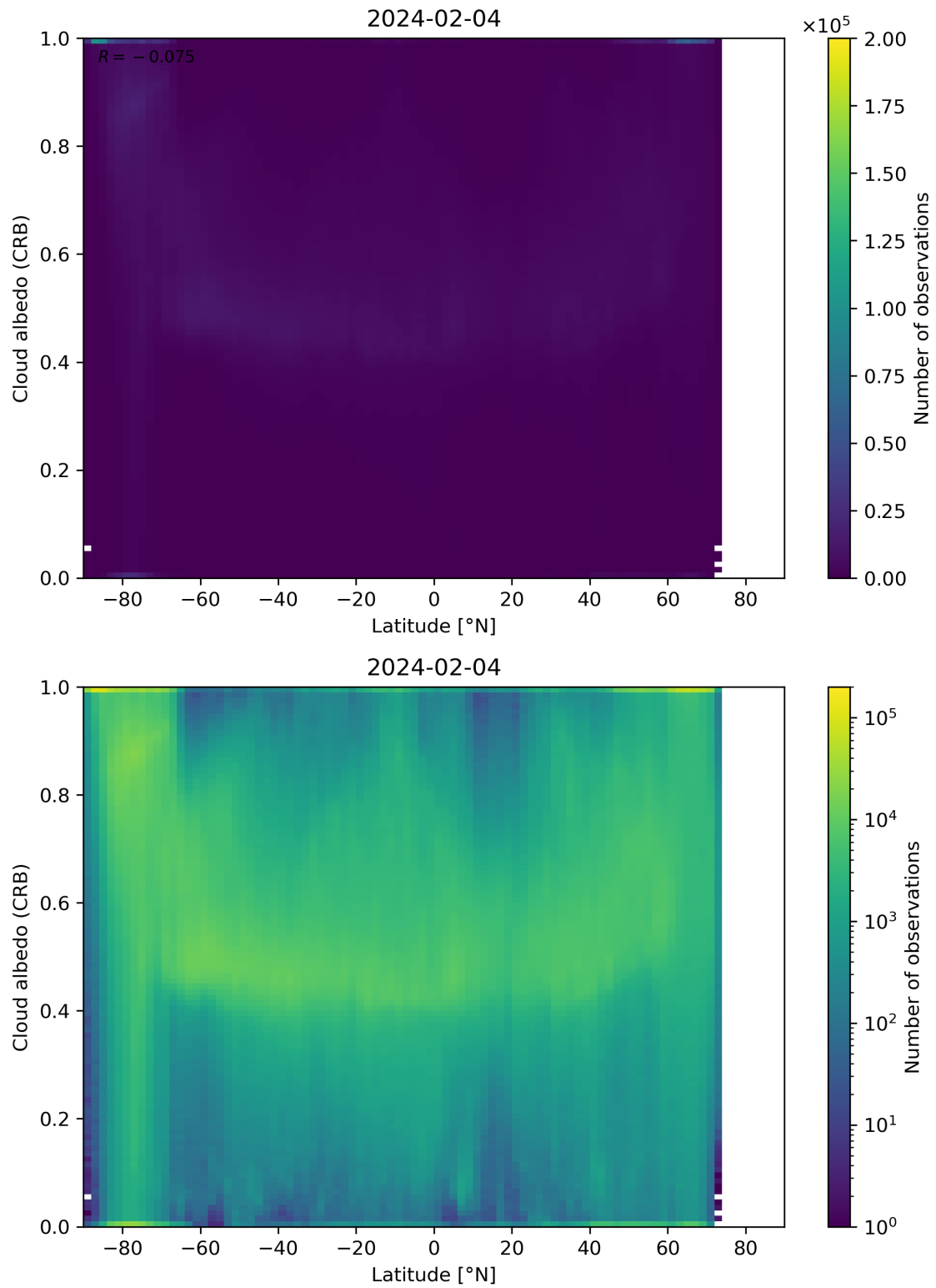
Figure 91: Scatter density plot of “Latitude” against “Cloud albedo (CRB)” for 2024-02-03 to 2024-02-05.
