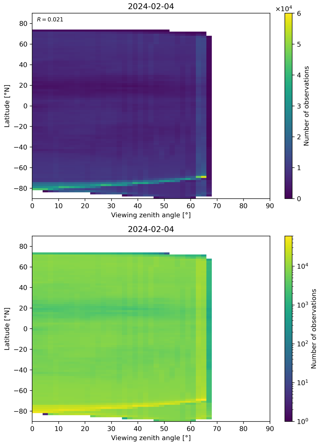
Figure 113: Scatter density plot of “Viewing zenith angle” against “Latitude” for 2024-02-03 to 2024-02-05.
