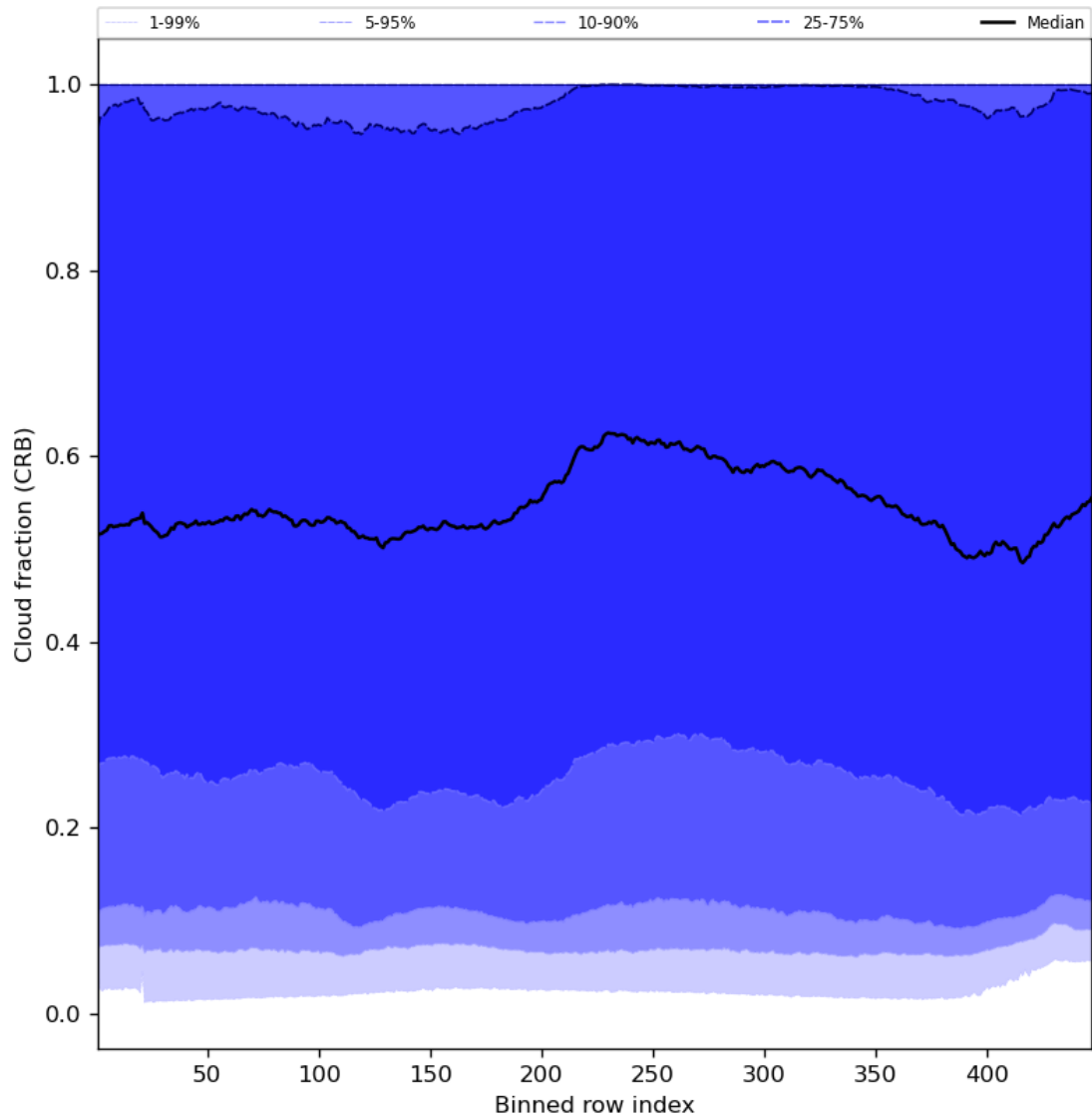
Figure 58: Along track statistics of “Cloud fraction (CRB)” for 2024-02-03 to 2024-02-05
