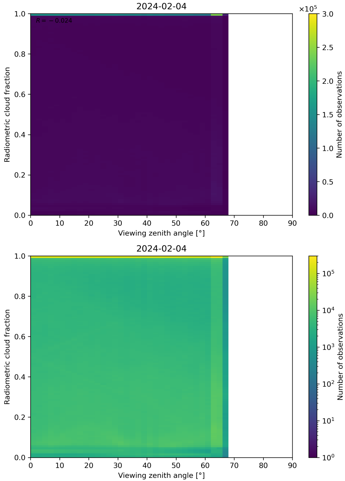
Figure 107: Scatter density plot of “Viewing zenith angle” against “Radiometric cloud fraction” for 2024-02-03 to 2024-02-05.
