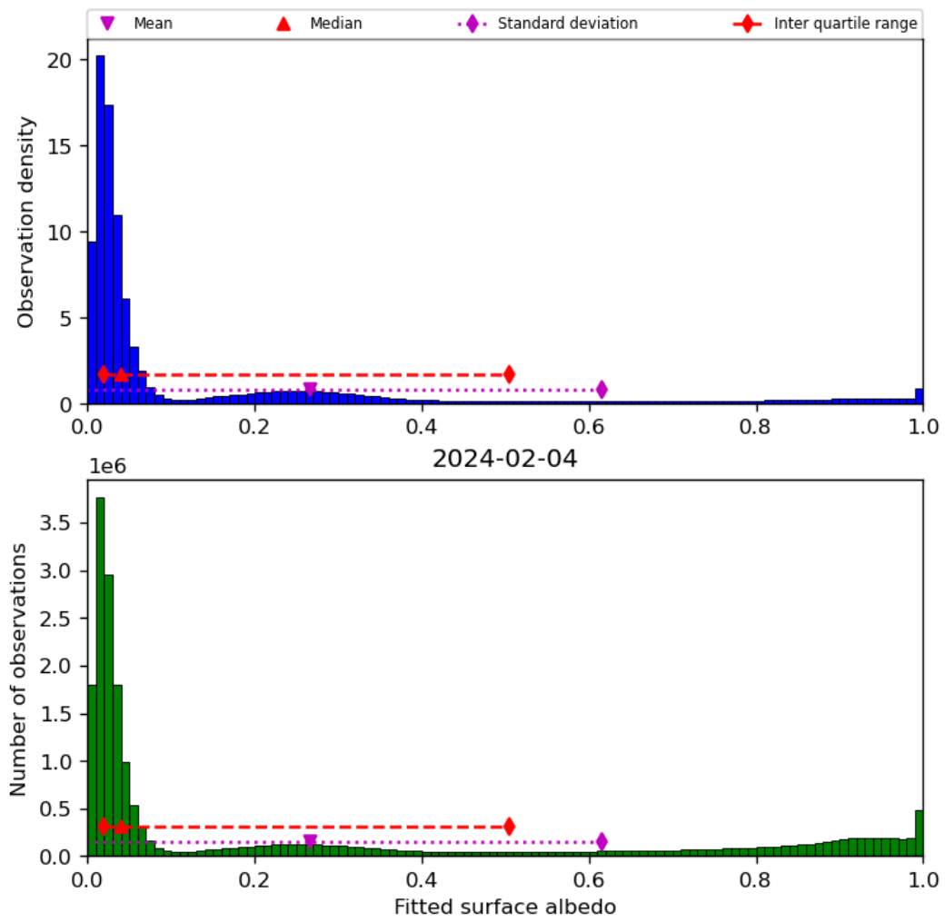
Figure 45: Histogram of “Fitted surface albedo” for 2024-02-03 to 2024-02-05
