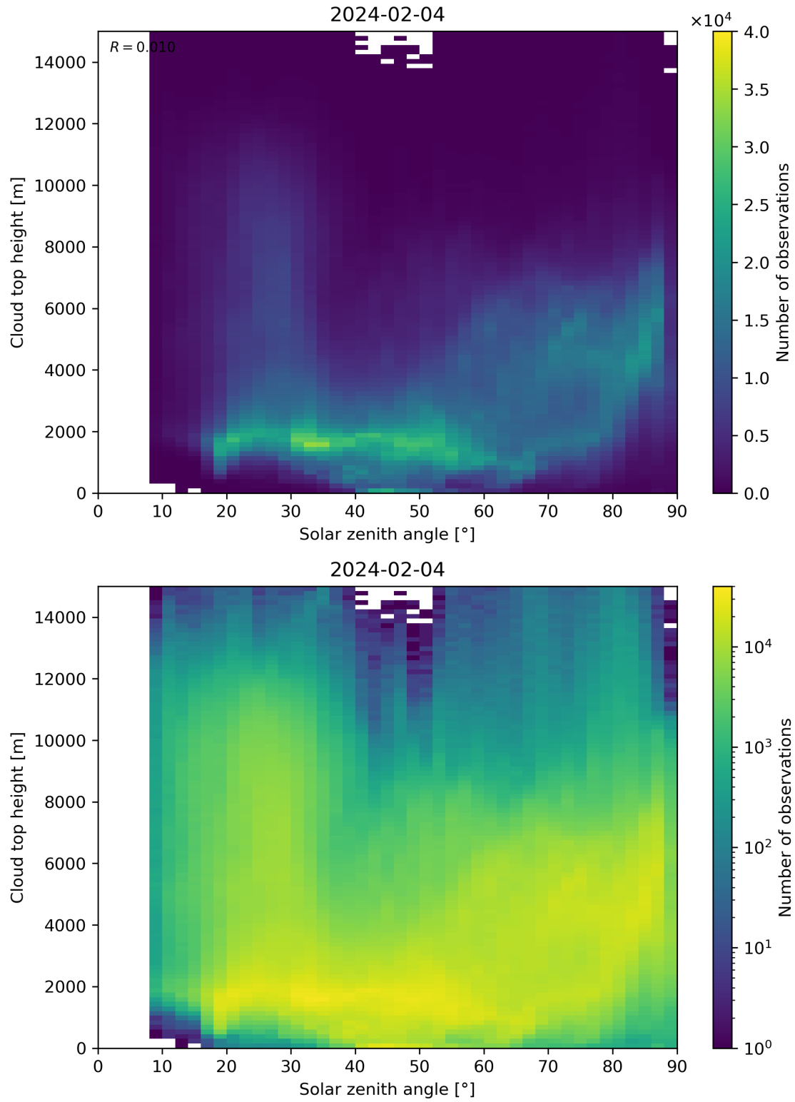
Figure 104: Scatter density plot of “Solar zenith angle” against “Cloud top height” for 2024-02-03 to 2024-02-05.
