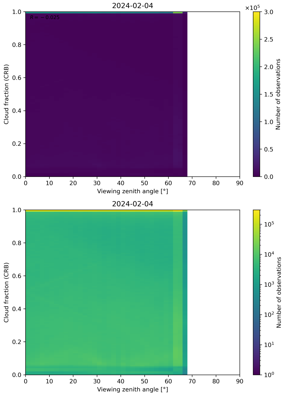
Figure 109: Scatter density plot of “Viewing zenith angle” against “Cloud fraction (CRB)” for 2024-02-03 to 2024-02-05.
