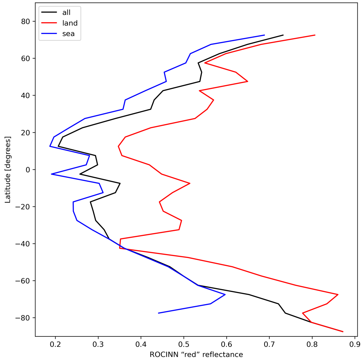
Figure 37: Zonal average of “ROCINN “red” reflectance” for 2024-02-03 to 2024-02-05.
