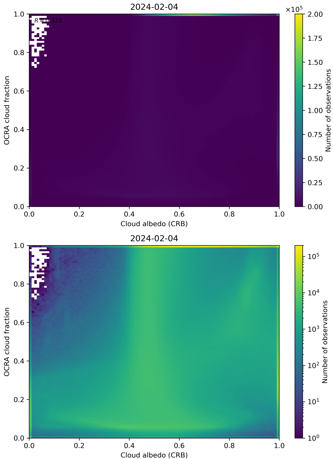
Figure 70: Scatter density plot of “Cloud albedo (CRB)” against “OCRA cloud fraction” for 2024-02-03 to 2024-02-05.
