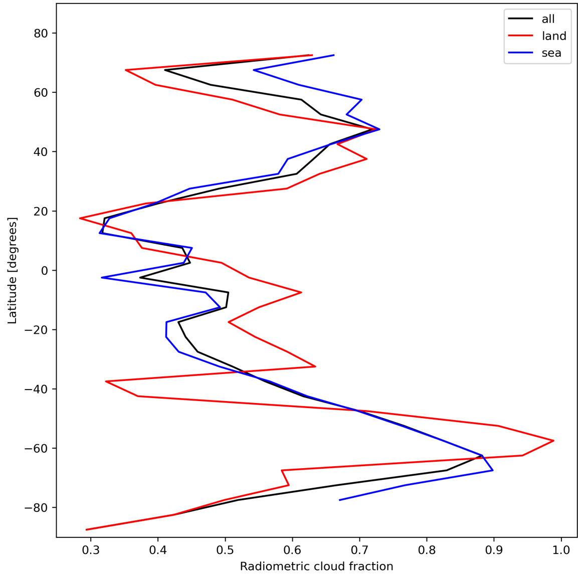
Figure 23: Zonal average of “Radiometric cloud fraction” for 2024-02-03 to 2024-02-05.
