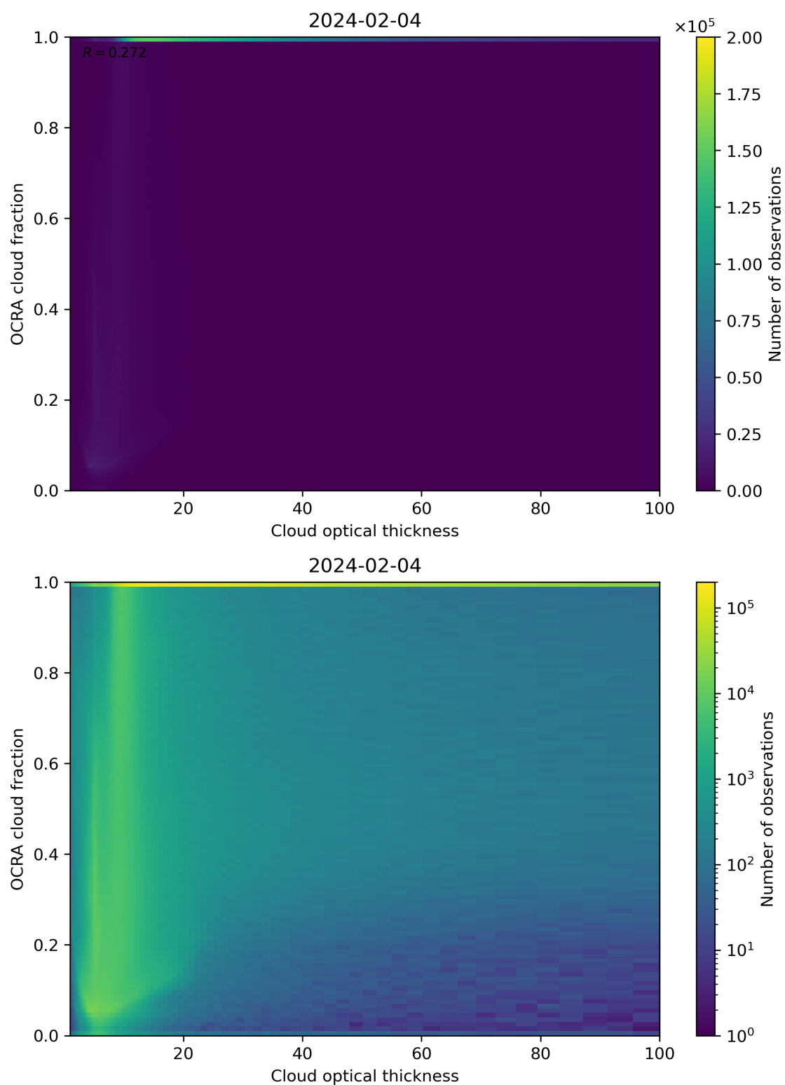
Figure 83: Scatter density plot of “Cloud optical thickness” against “OCRA cloud fraction” for 2024-02-03 to 2024-02-05.
