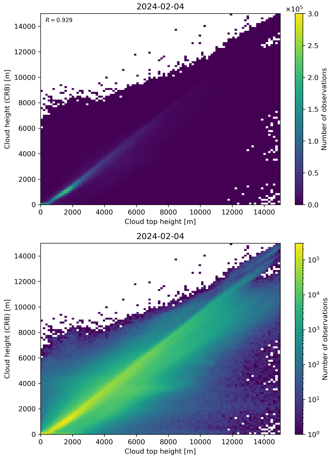
Figure 89: Scatter density plot of “Cloud top height” against “Cloud height (CRB)” for 2024-02-03 to 2024-02-05.
