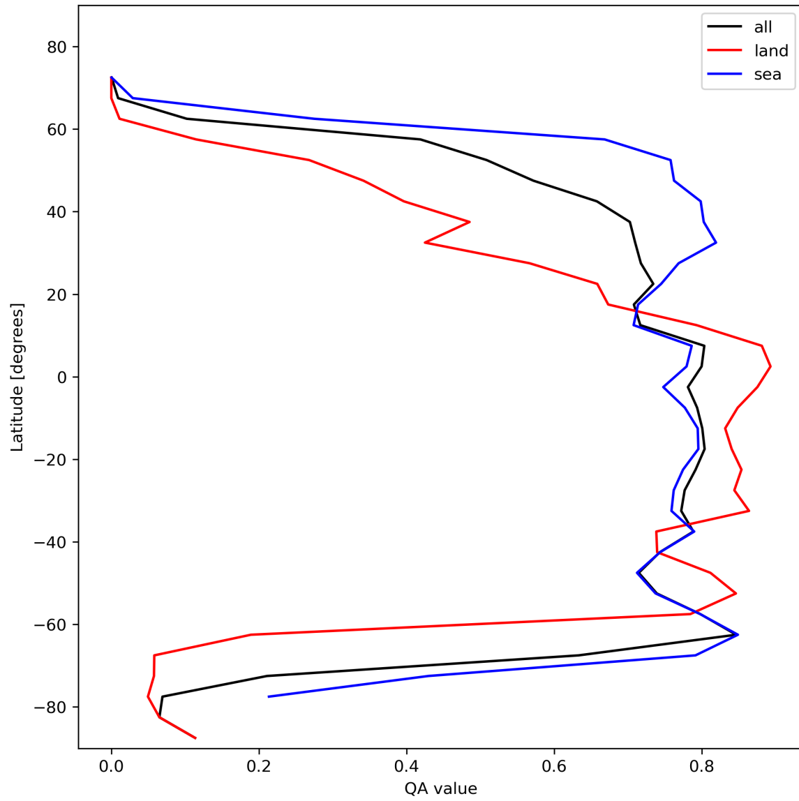
Figure 22: Zonal average of “QA value” for 2024-02-03 to 2024-02-05.
