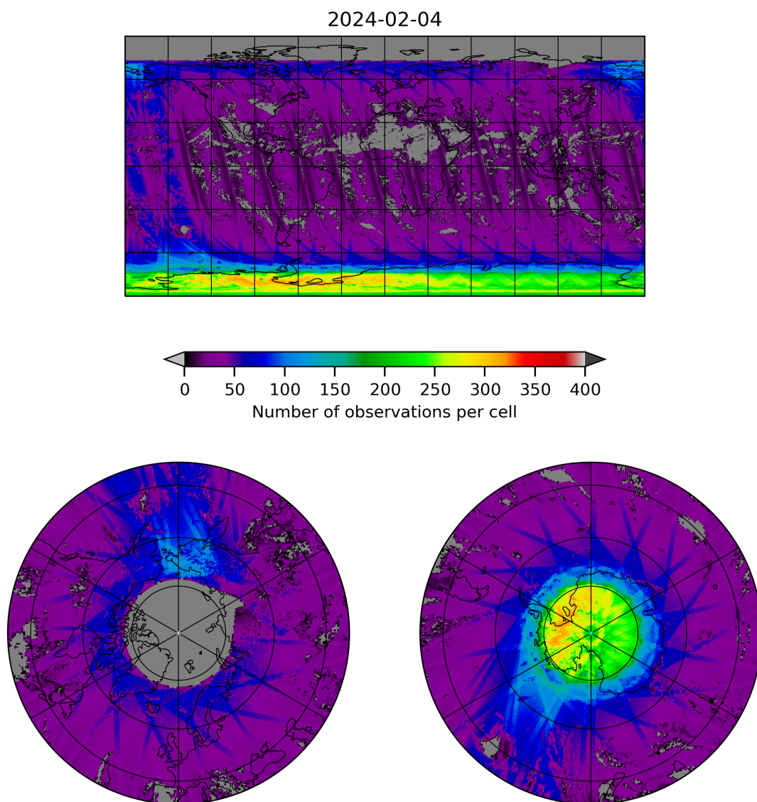
Figure 21: Map of the number of observations for 2024-02-03 to 2024-02-05
