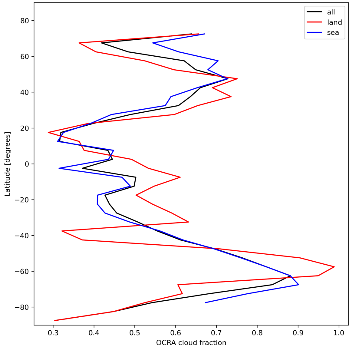
Figure 34: Zonal average of “OCRA cloud fraction” for 2024-02-03 to 2024-02-05.
