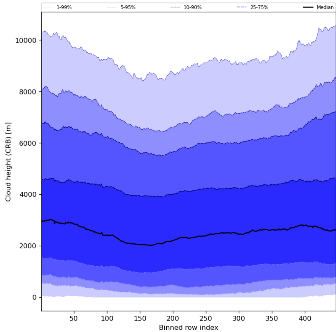
Figure 59: Along track statistics of “Cloud height (CRB)” for 2024-02-03 to 2024-02-05
