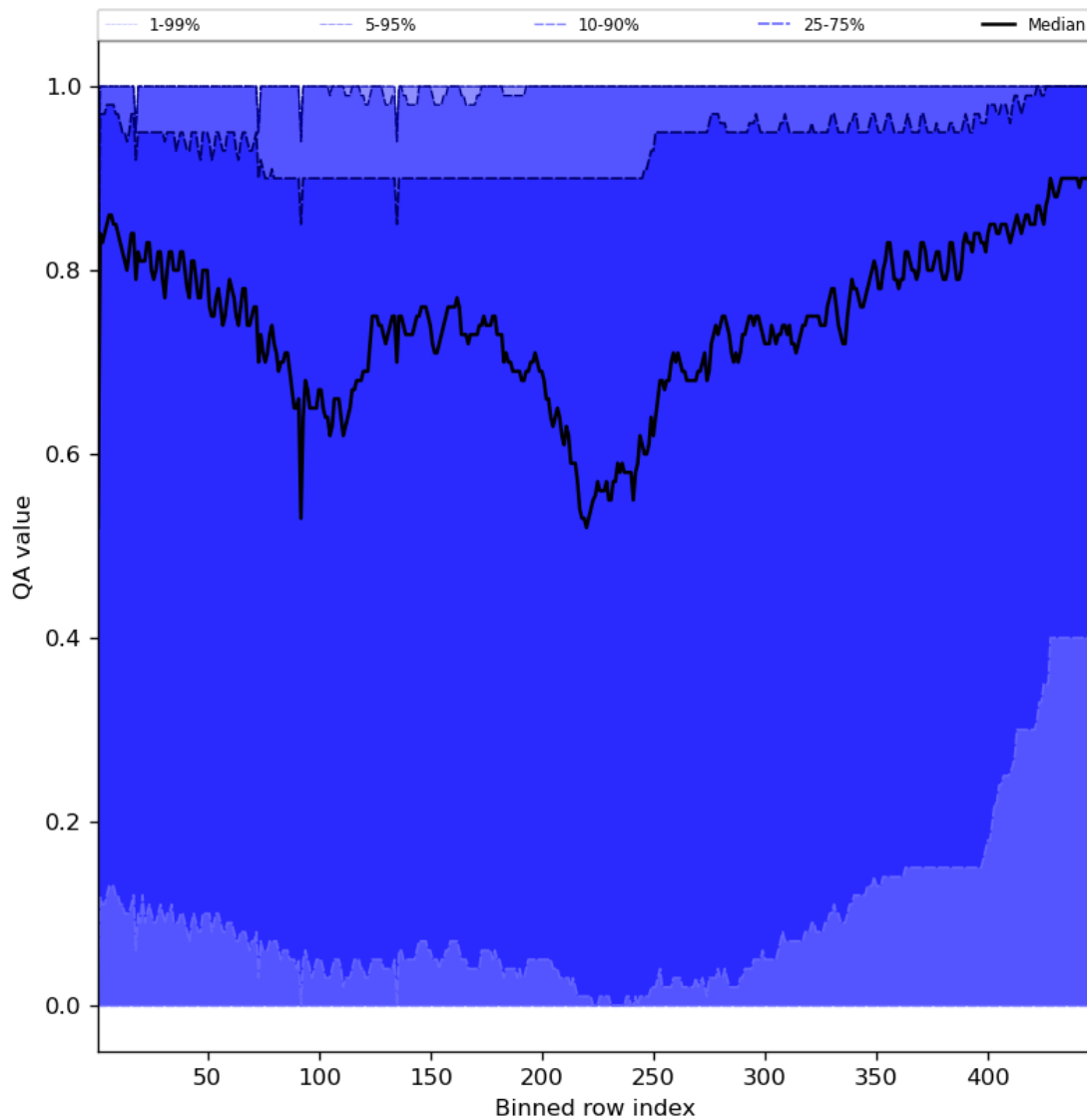
Figure 54: Along track statistics of “QA value” for 2024-02-03 to 2024-02-05
