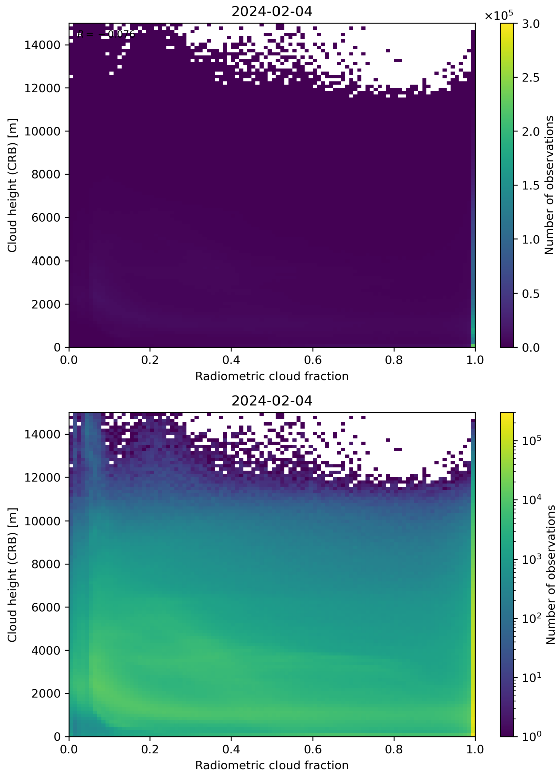
Figure 74: Scatter density plot of “Radiometric cloud fraction” against “Cloud height (CRB)” for 2024-02-03 to 2024-02-05.
