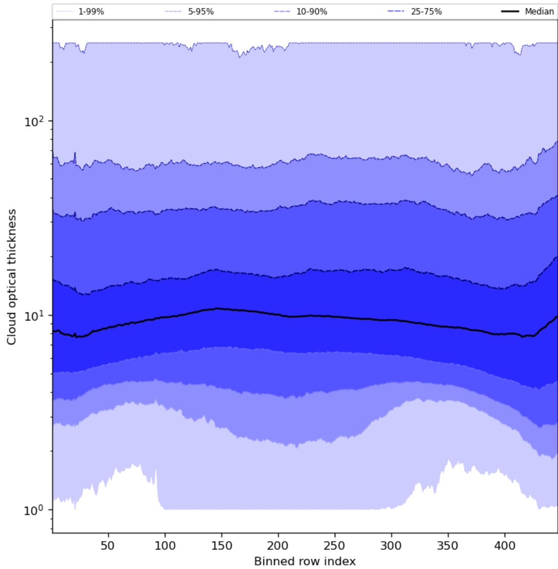
Figure 57: Along track statistics of “Cloud optical thickness” for 2024-02-03 to 2024-02-05
