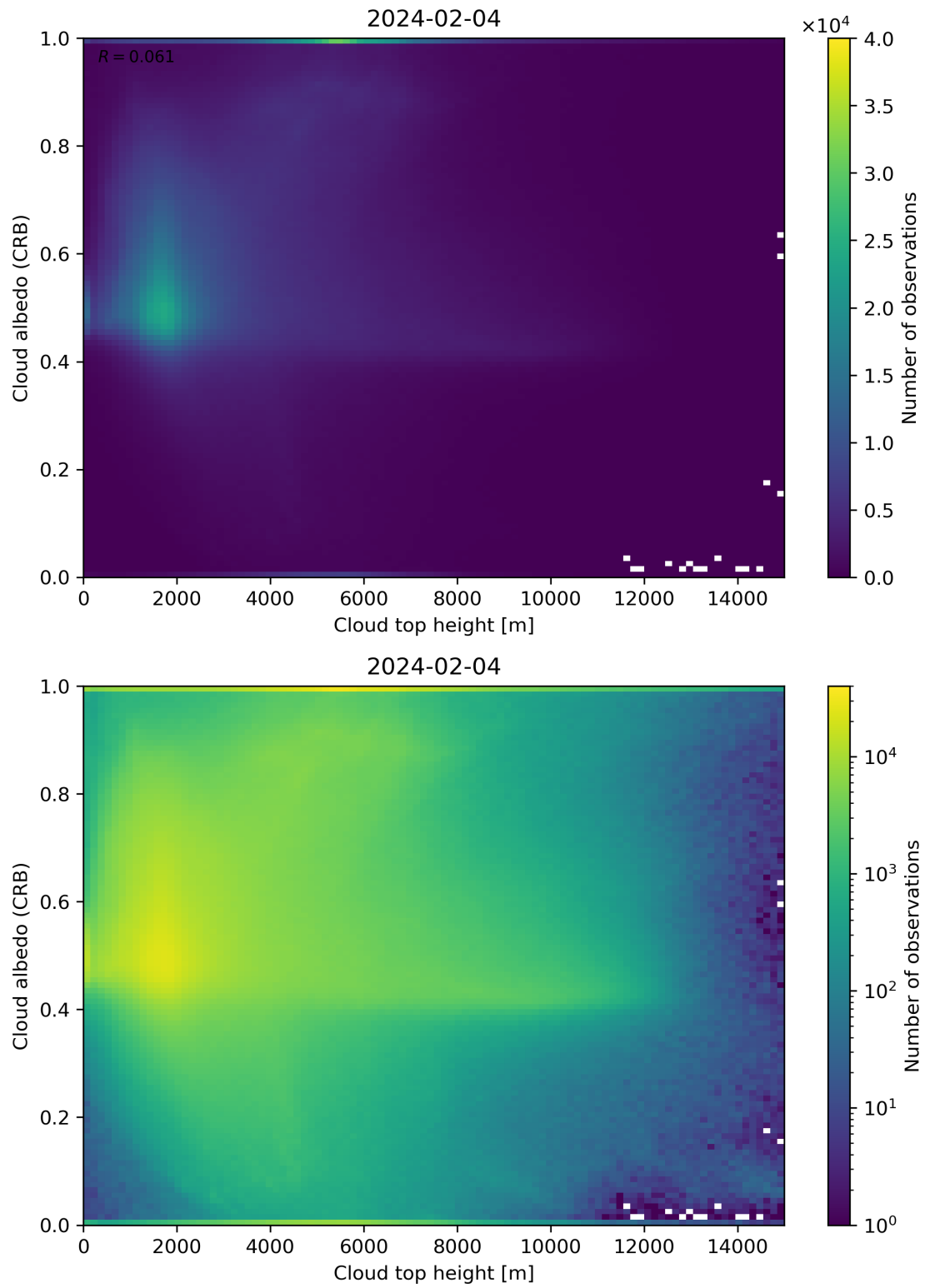
Figure 86: Scatter density plot of “Cloud top height” against “Cloud albedo (CRB)” for 2024-02-03 to 2024-02-05.
