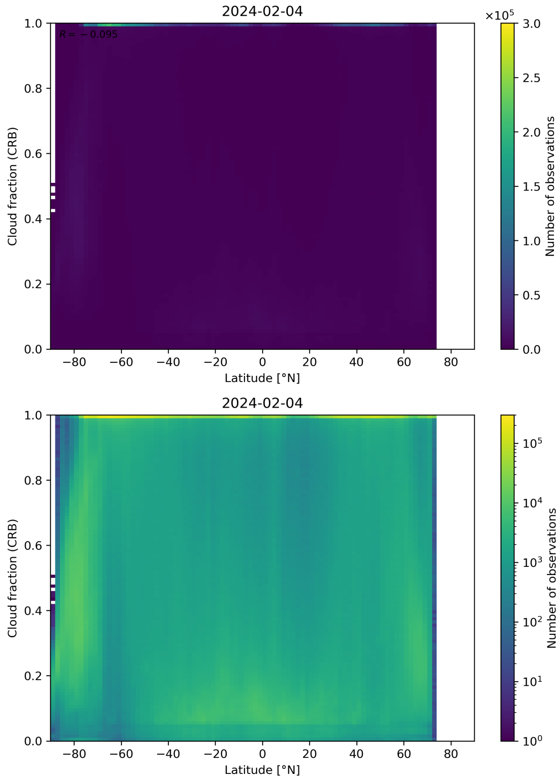
Figure 94: Scatter density plot of “Latitude” against “Cloud fraction (CRB)” for 2024-02-03 to 2024-02-05.
