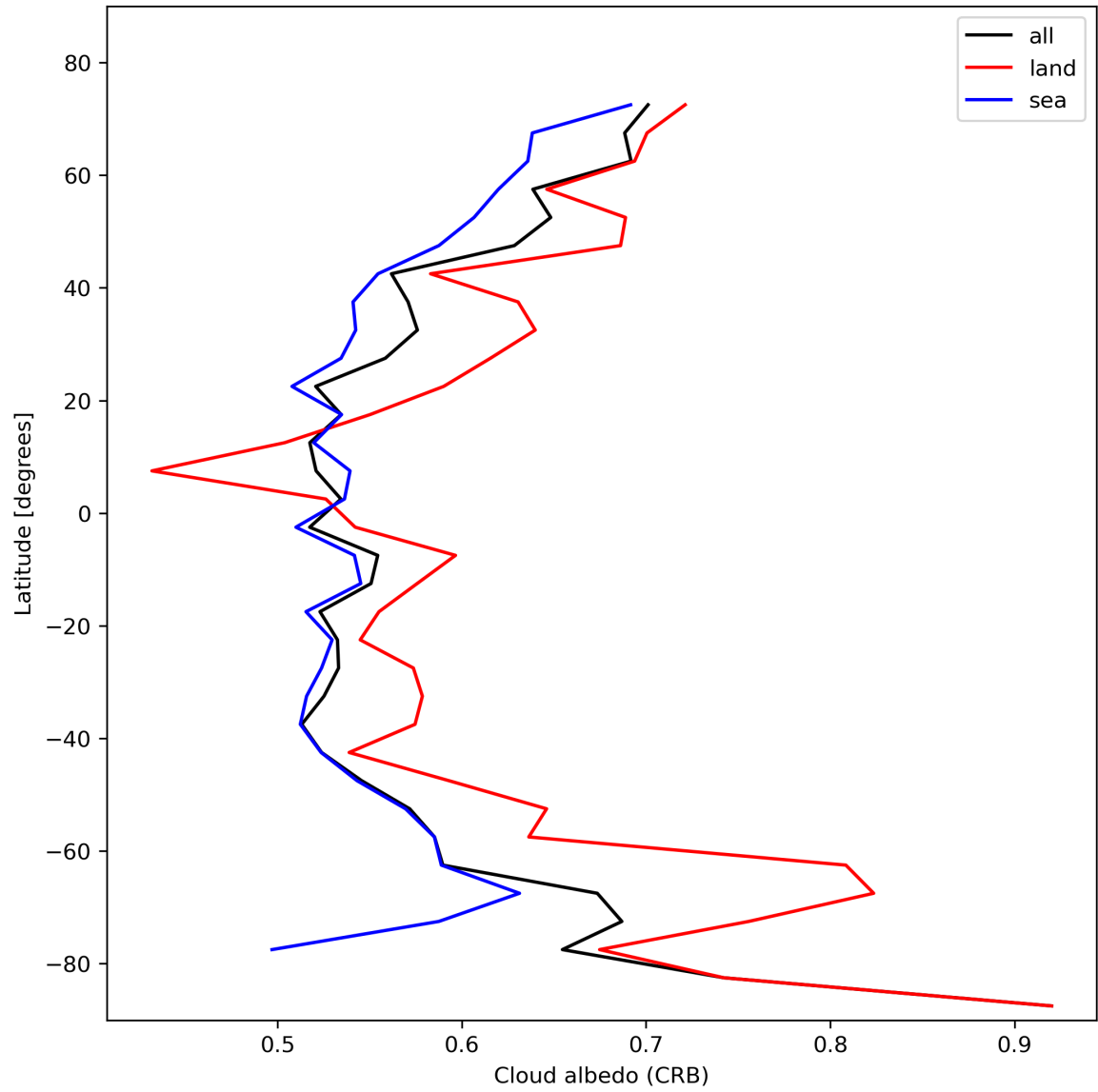
Figure 28: Zonal average of “Cloud albedo (CRB)” for 2024-02-03 to 2024-02-05.
