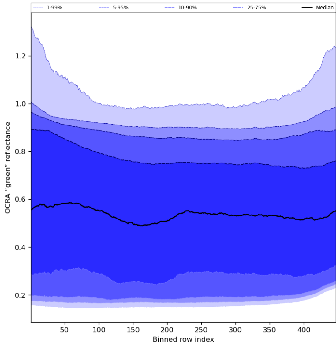
Figure 68: Along track statistics of "OCRA "green" reflectance" for 2024-02-03 to 2024-02-05
