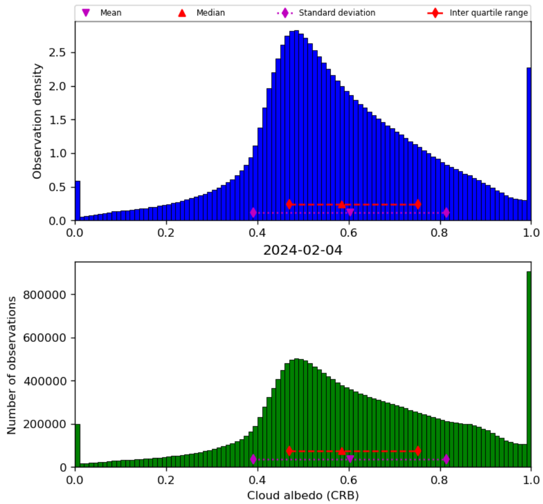
Figure 44: Histogram of “Cloud albedo (CRB)” for 2024-02-03 to 2024-02-05
