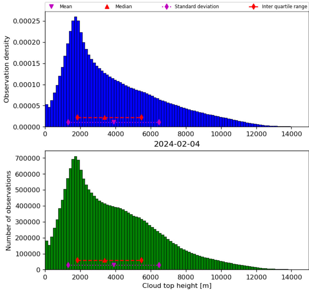
Figure 40: Histogram of “Cloud top height” for 2024-02-03 to 2024-02-05
