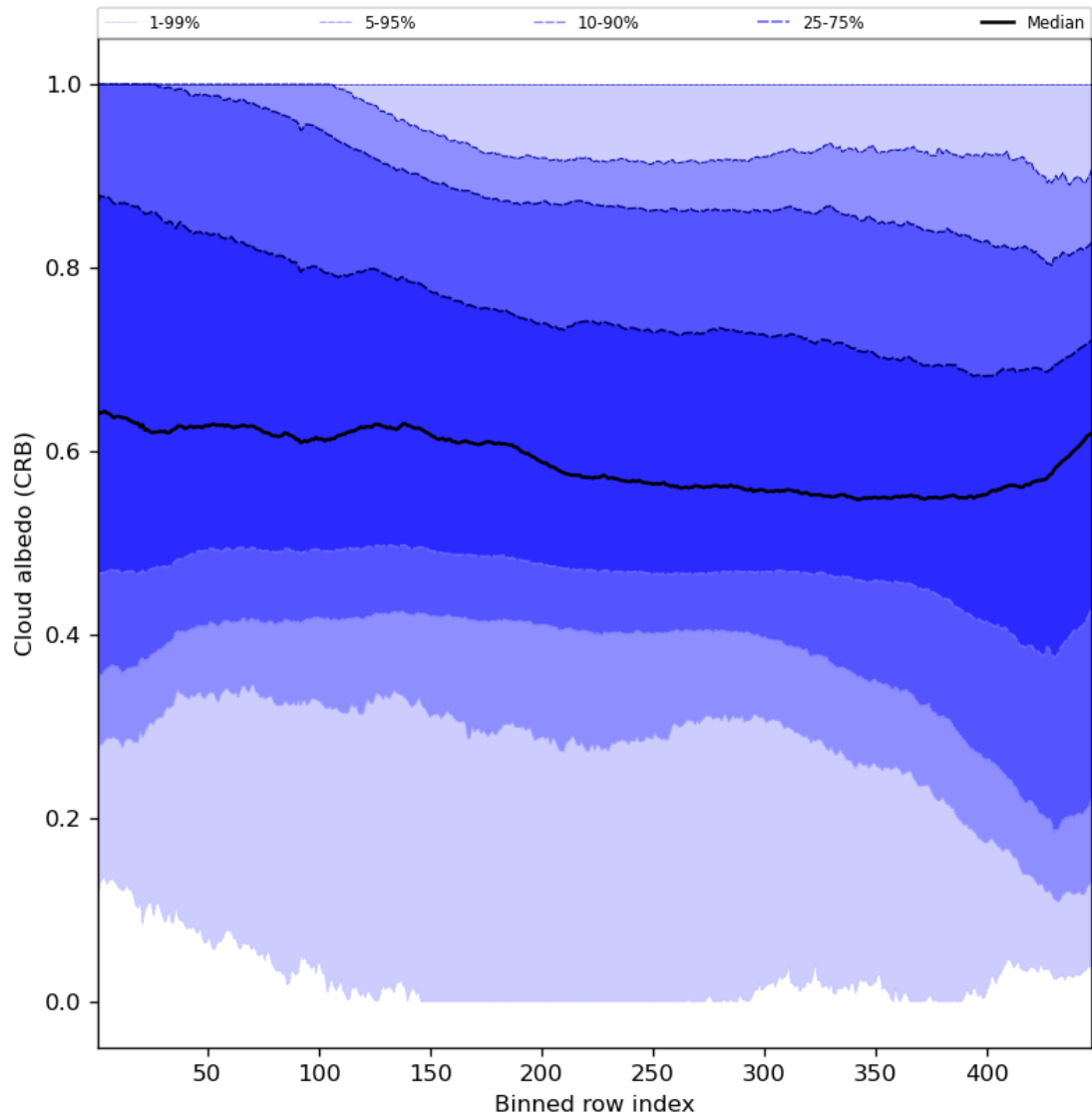
Figure 60: Along track statistics of “Cloud albedo (CRB)” for 2024-02-03 to 2024-02-05
