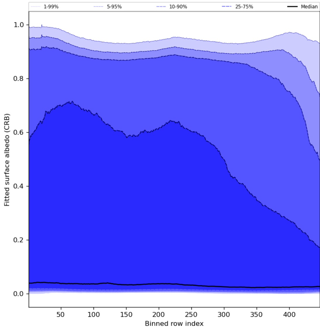
Figure 62: Along track statistics of “Fitted surface albedo (CRB)” for 2024-02-03 to 2024-02-05
