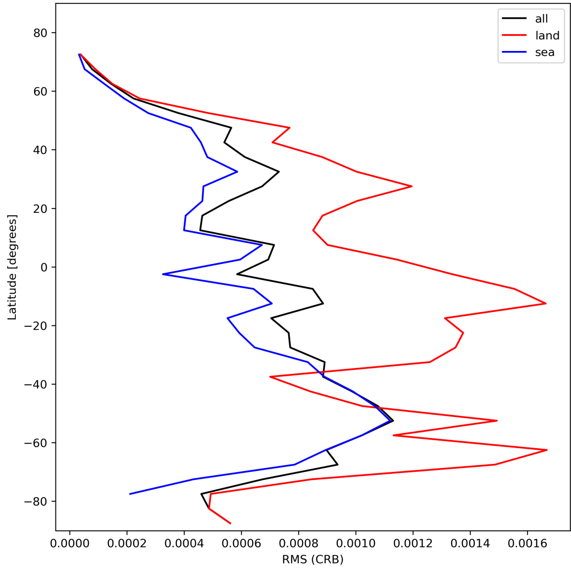
Figure 32: Zonal average of “RMS (CRB)” for 2024-02-03 to 2024-02-05.
