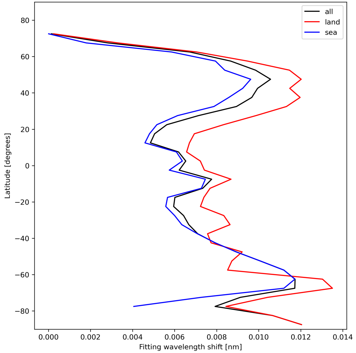
Figure 33: Zonal average of “Fitting wavelength shift” for 2024-02-03 to 2024-02-05.
