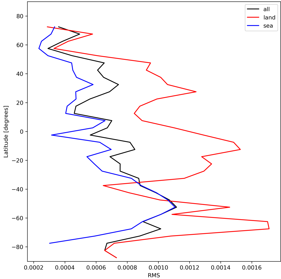
Figure 31: Zonal average of “RMS” for 2024-02-03 to 2024-02-05.
