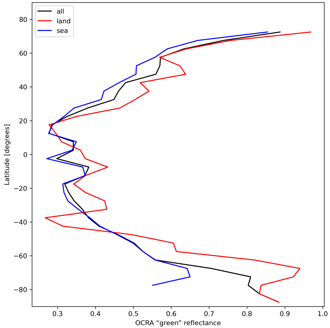
Figure 36: Zonal average of “OCRA “green” reflectance” for 2024-02-03 to 2024-02-05.
