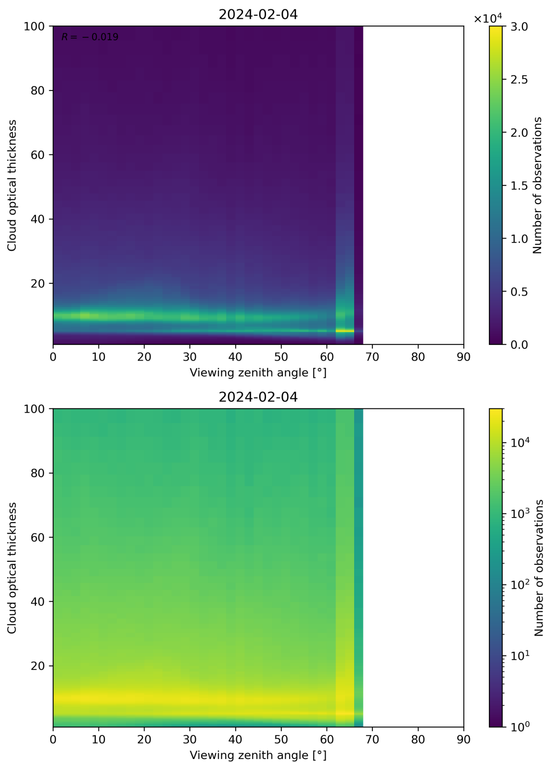
Figure 111: Scatter density plot of “Viewing zenith angle” against “Cloud optical thickness” for 2024-02-03 to 2024-02-05.
