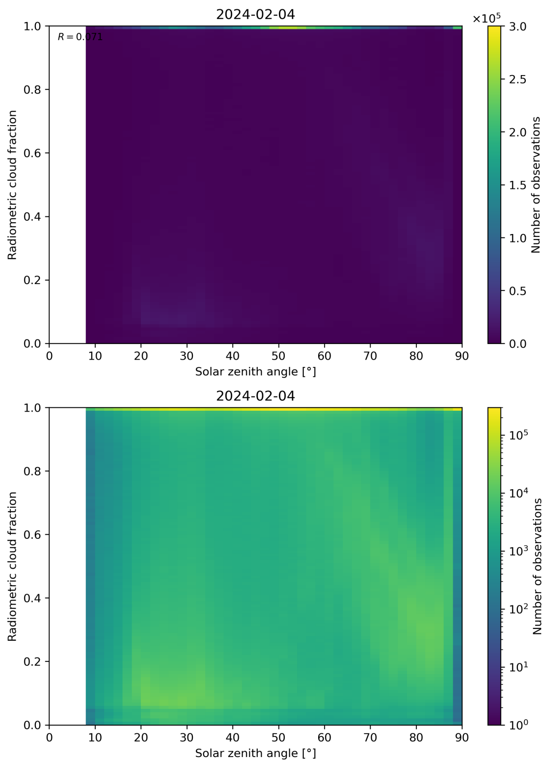
Figure 99: Scatter density plot of “Solar zenith angle” against “Radiometric cloud fraction” for 2024-02-03 to 2024-02-05.
