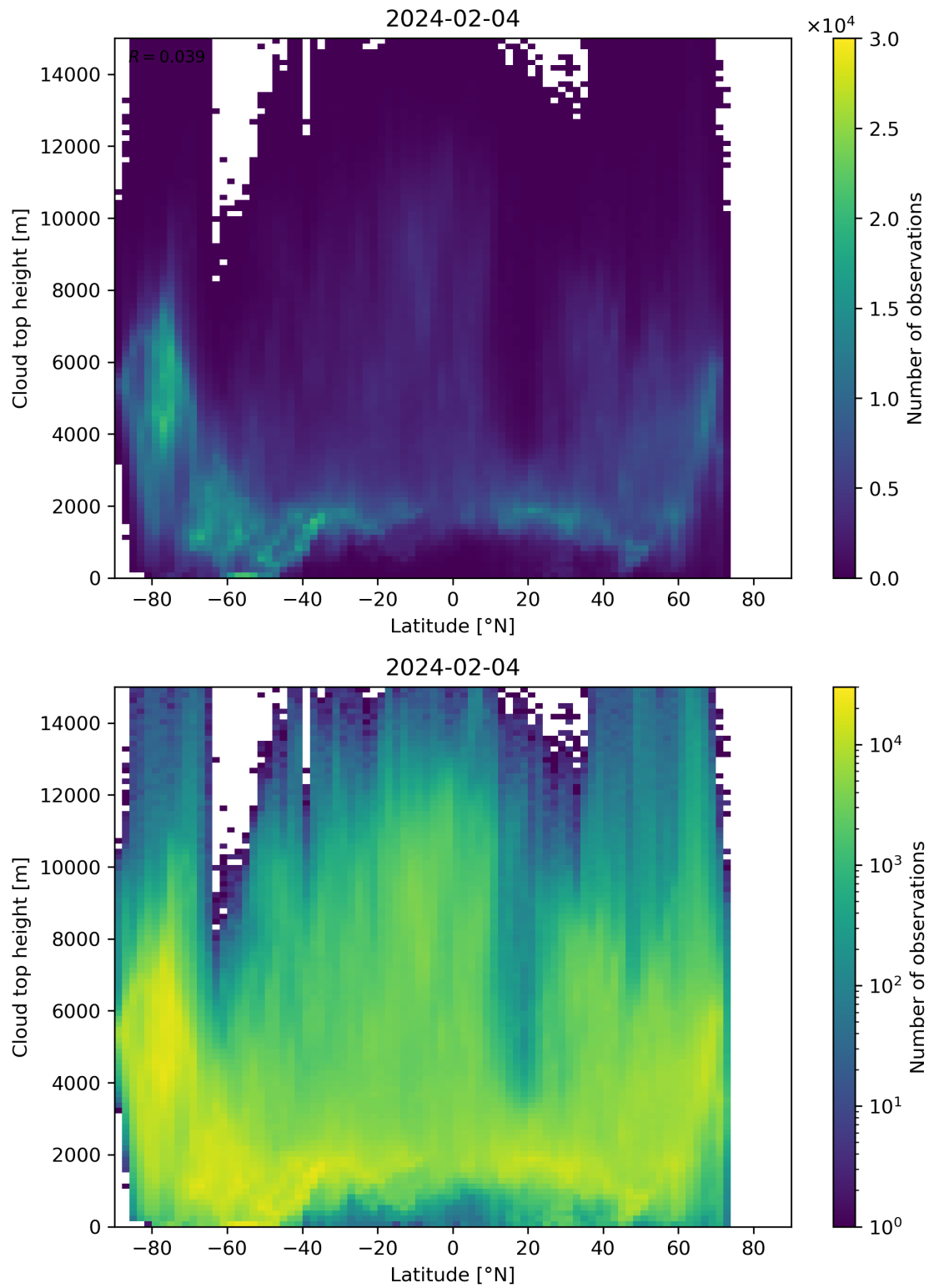
Figure 97: Scatter density plot of “Latitude” against “Cloud top height” for 2024-02-03 to 2024-02-05.
