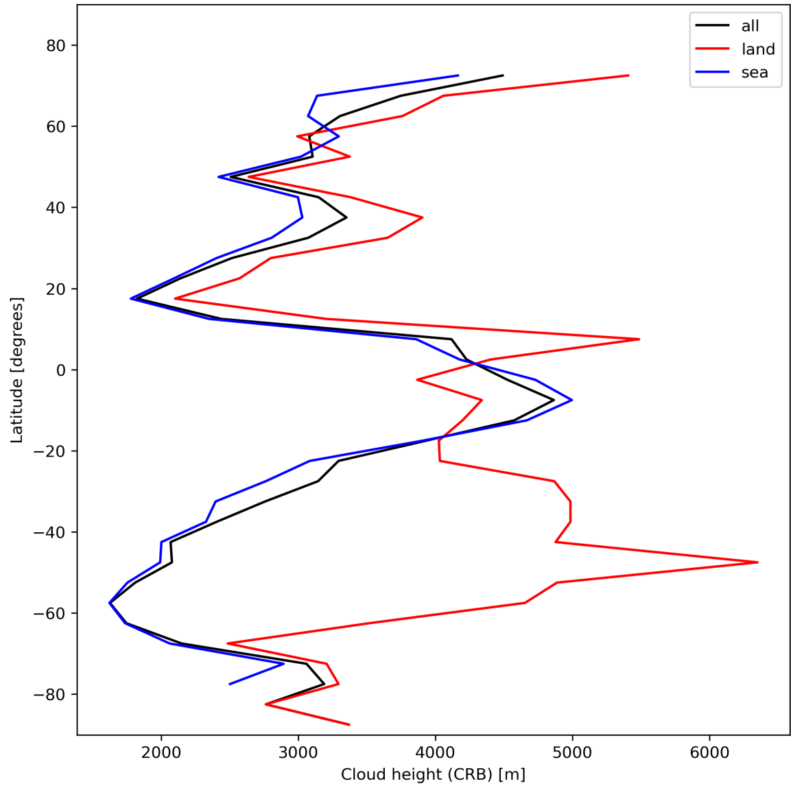
Figure 27: Zonal average of “Cloud height (CRB)” for 2024-02-03 to 2024-02-05.
