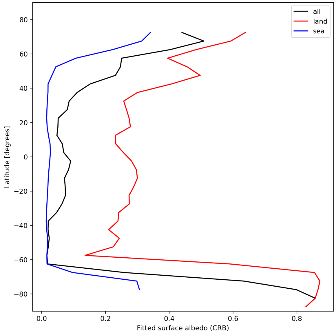
Figure 30: Zonal average of “Fitted surface albedo (CRB)” for 2024-02-03 to 2024-02-05.
