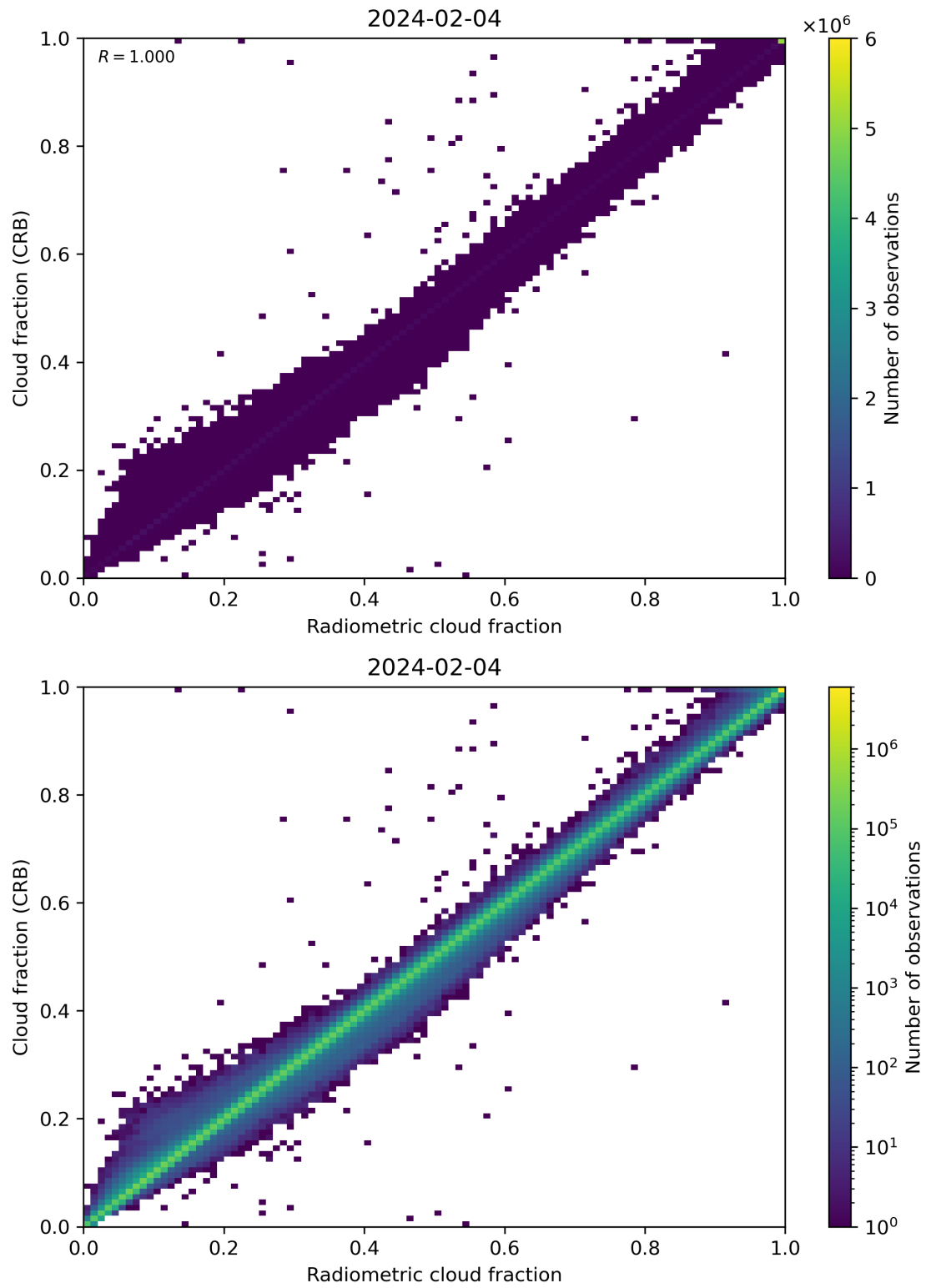
Figure 73: Scatter density plot of “Radiometric cloud fraction” against “Cloud fraction (CRB)” for 2024-02-03 to 2024-02-05.
