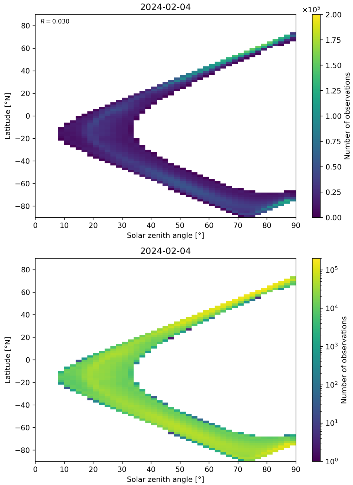
Figure 105: Scatter density plot of “Solar zenith angle” against “Latitude” for 2024-02-03 to 2024-02-05.
