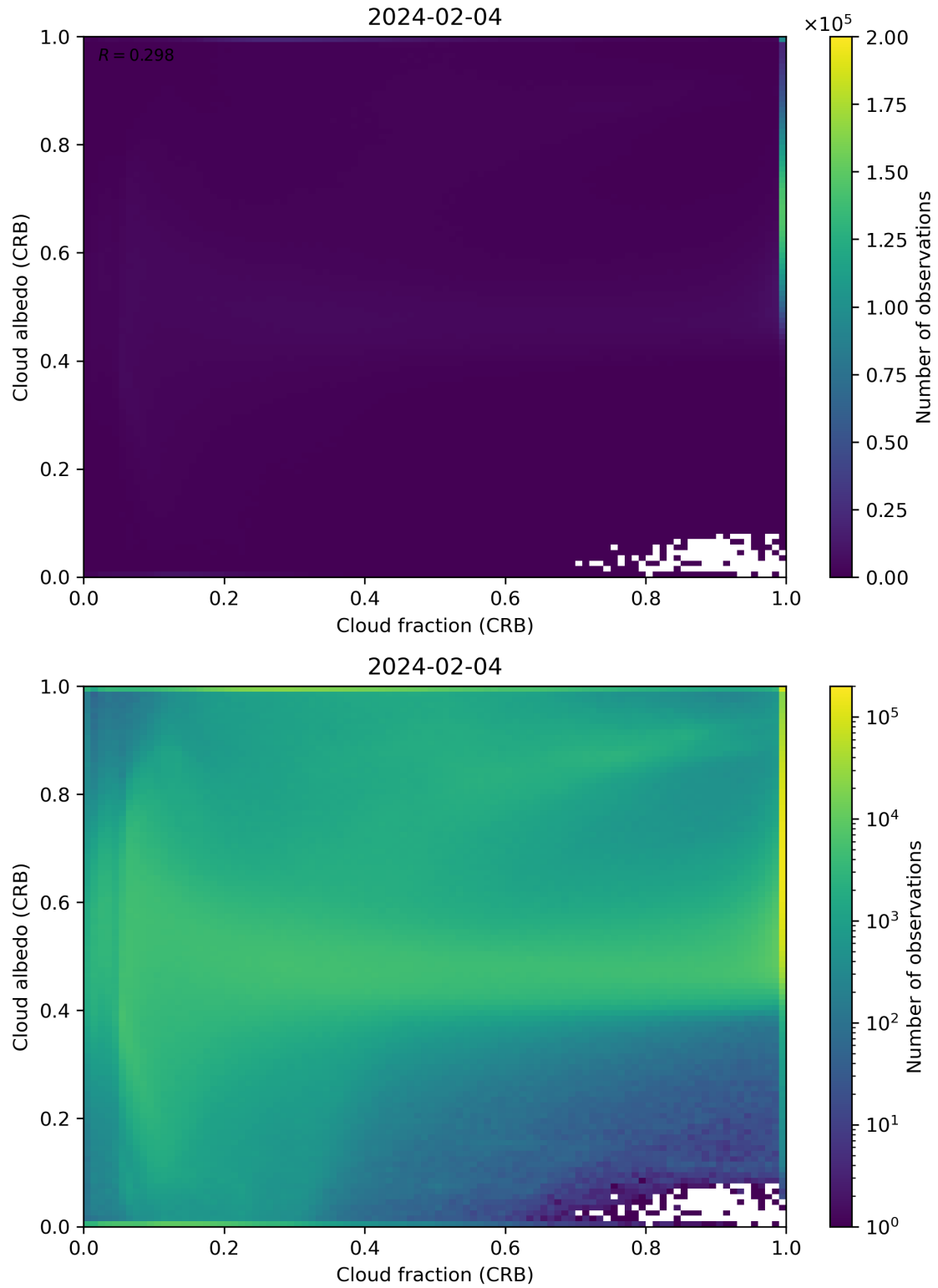
Figure 77: Scatter density plot of “Cloud fraction (CRB)” against “Cloud albedo (CRB)” for 2024-02-03 to 2024-02-05.
