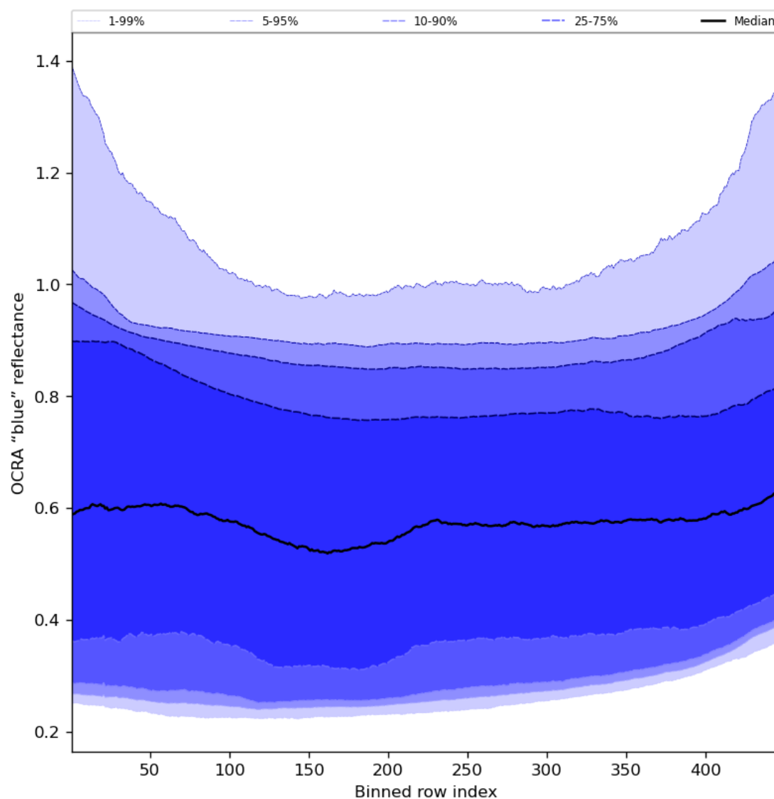
Figure 67: Along track statistics of “OCRA “blue” reflectance” for 2024-02-03 to 2024-02-05
