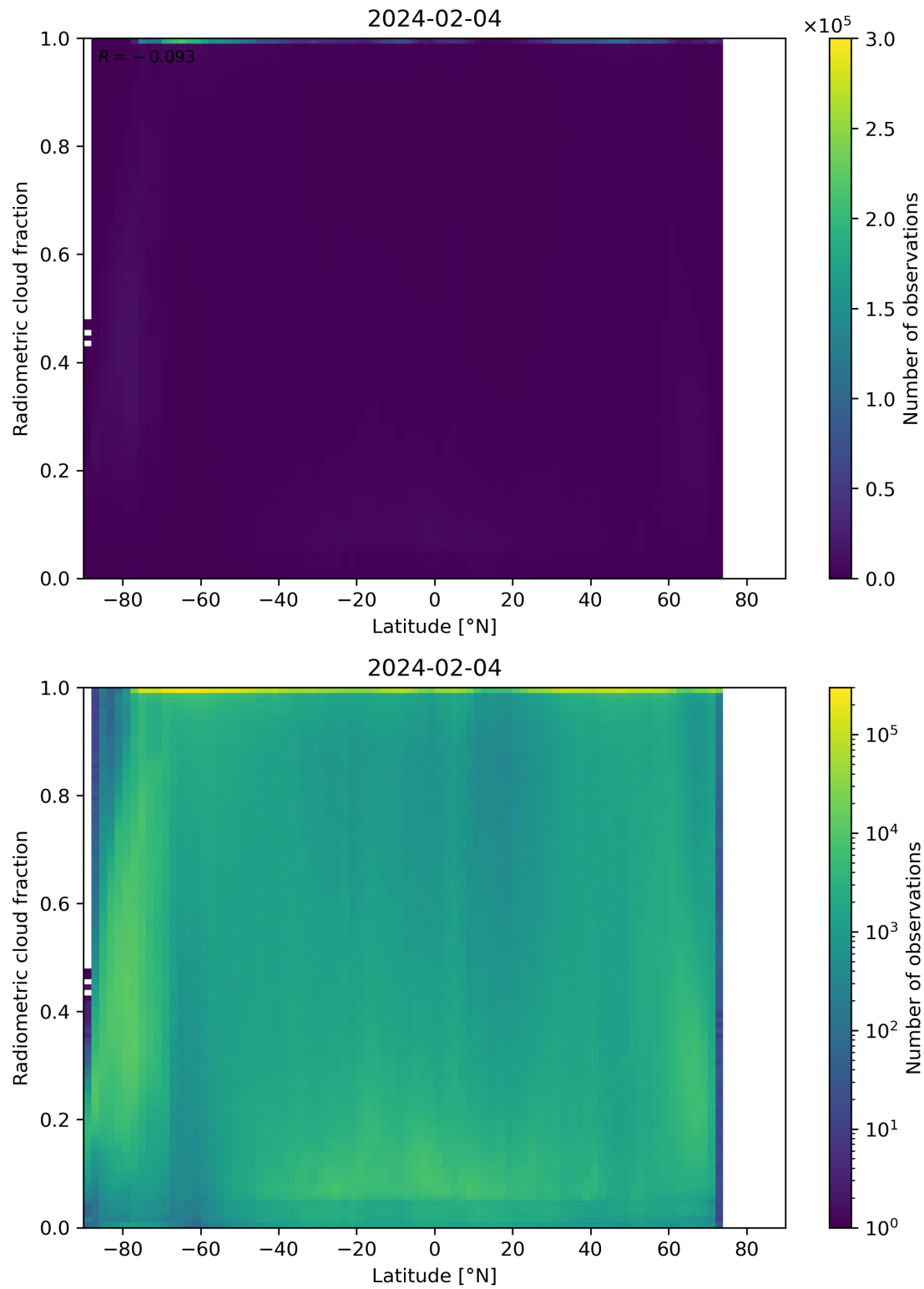
Figure 92: Scatter density plot of “Latitude” against “Radiometric cloud fraction” for 2024-02-03 to 2024-02-05.
