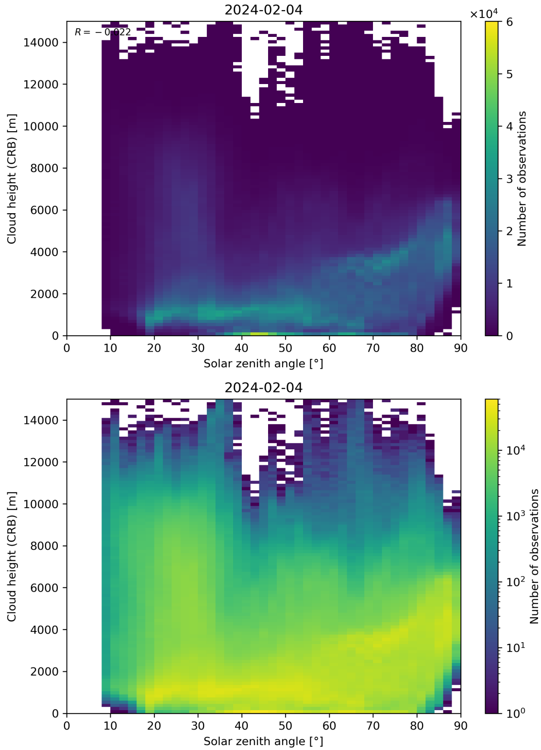
Figure 102: Scatter density plot of “Solar zenith angle” against “Cloud height (CRB)” for 2024-02-03 to 2024-02-05.
