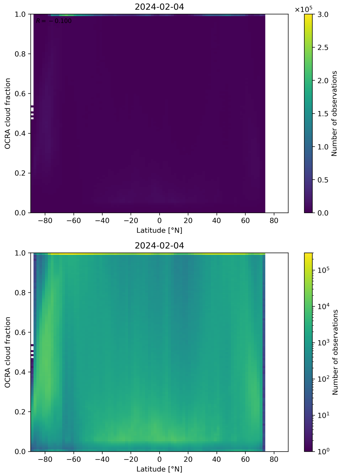
Figure 93: Scatter density plot of “Latitude” against “OCRA cloud fraction” for 2024-02-03 to 2024-02-05.
