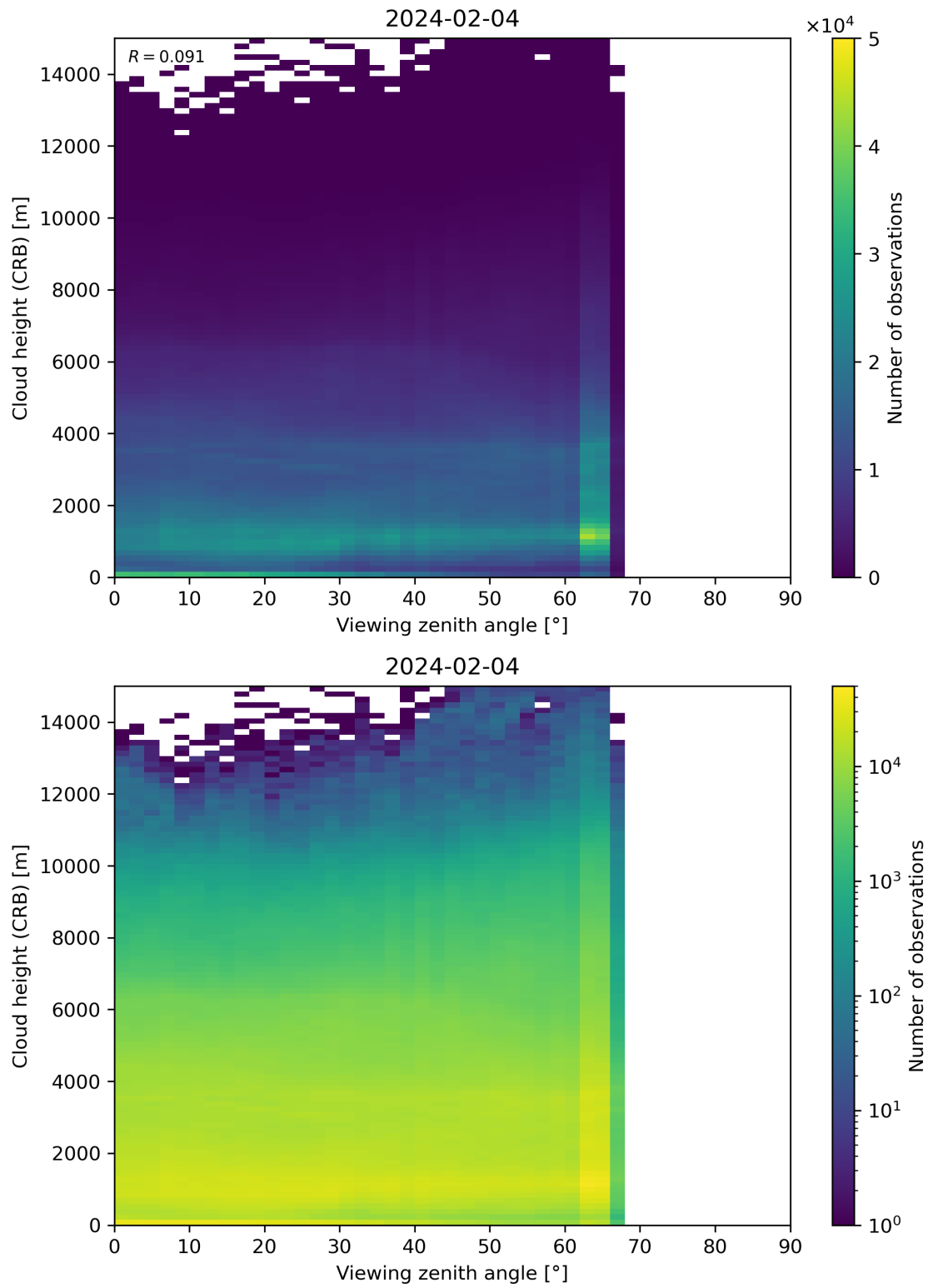
Figure 110: Scatter density plot of “Viewing zenith angle” against “Cloud height (CRB)” for 2024-02-03 to 2024-02-05.
