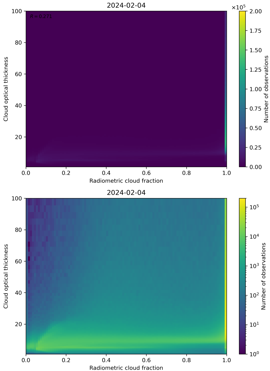
Figure 75: Scatter density plot of “Radiometric cloud fraction” against “Cloud optical thickness” for 2024-02-03 to 2024-02-05.
