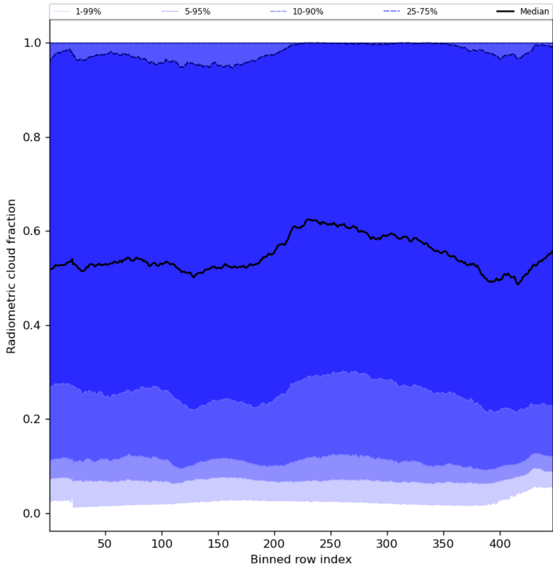
Figure 55: Along track statistics of “Radiometric cloud fraction” for 2024-02-03 to 2024-02-05
