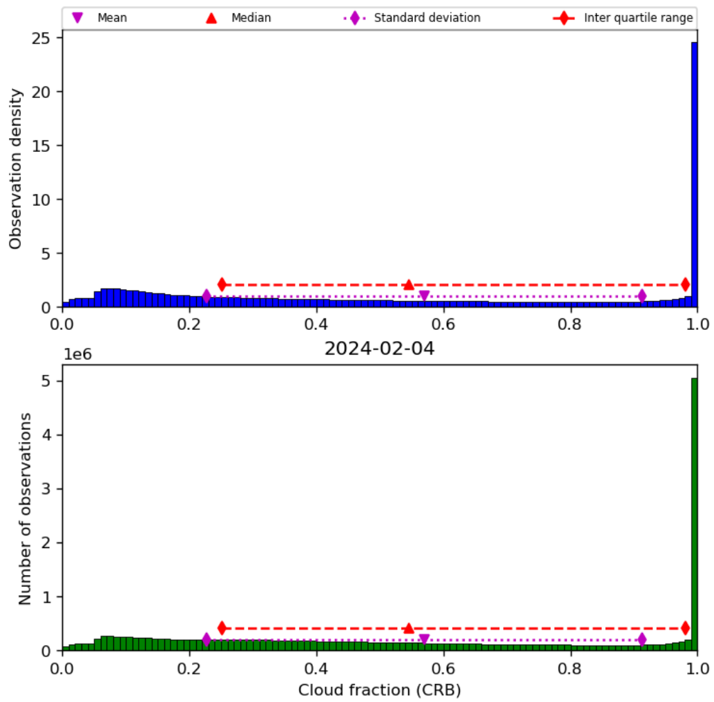
Figure 42: Histogram of “Cloud fraction (CRB)” for 2024-02-03 to 2024-02-05
