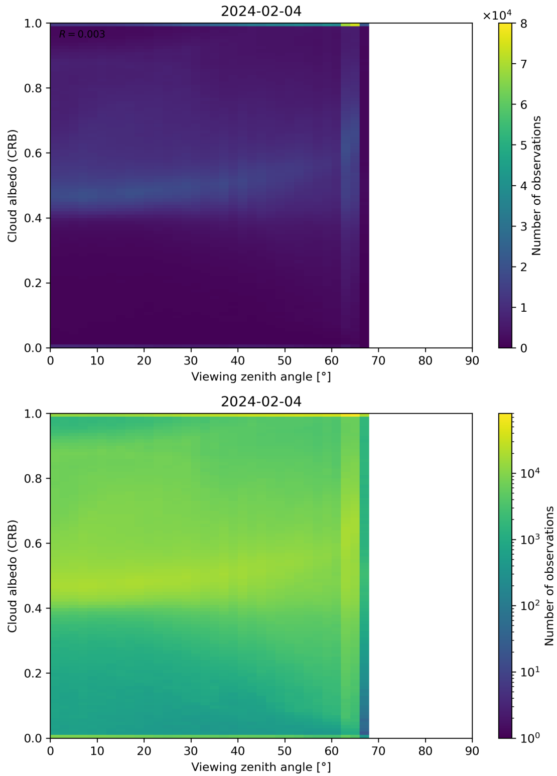
Figure 106: Scatter density plot of “Viewing zenith angle” against “Cloud albedo (CRB)” for 2024-02-03 to 2024-02-05.
