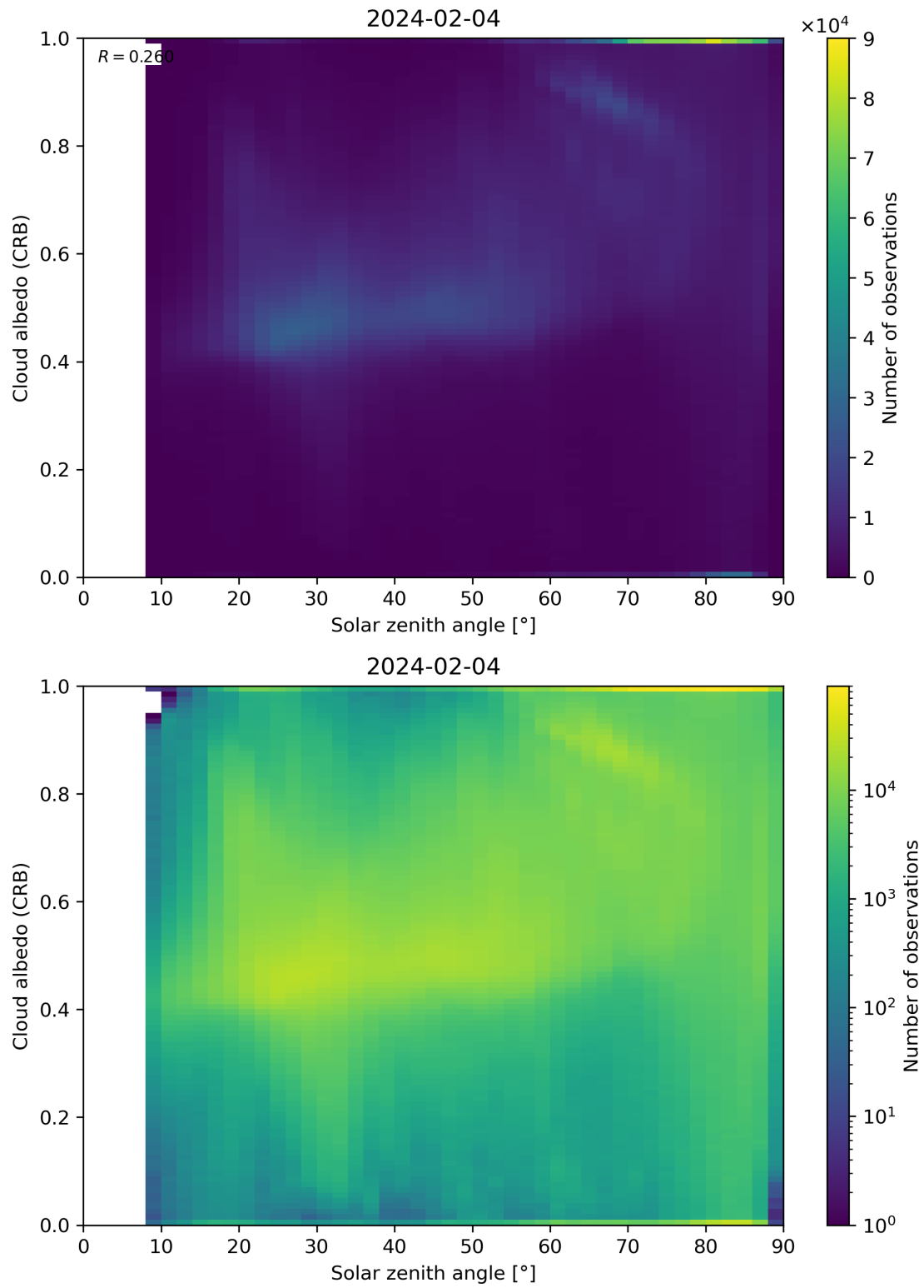
Figure 98: Scatter density plot of “Solar zenith angle” against “Cloud albedo (CRB)” for 2024-02-03 to 2024-02-05.
