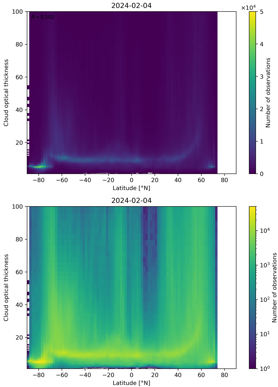
Figure 96: Scatter density plot of “Latitude” against “Cloud optical thickness” for 2024-02-03 to 2024-02-05.
