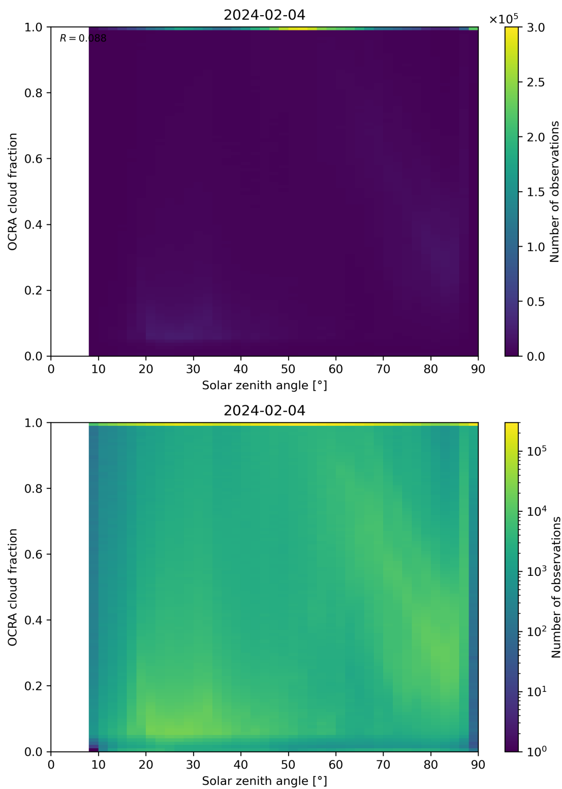
Figure 100: Scatter density plot of “Solar zenith angle” against “OCRA cloud fraction” for 2024-02-03 to 2024-02-05.
