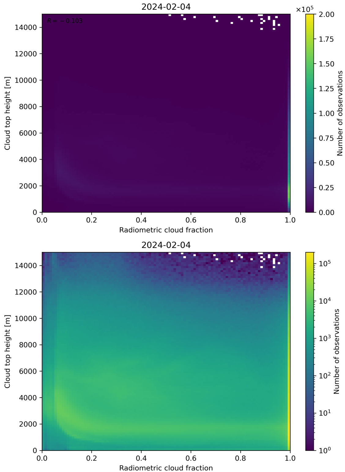
Figure 76: Scatter density plot of “Radiometric cloud fraction” against “Cloud top height” for 2024-02-03 to 2024-02-05.
