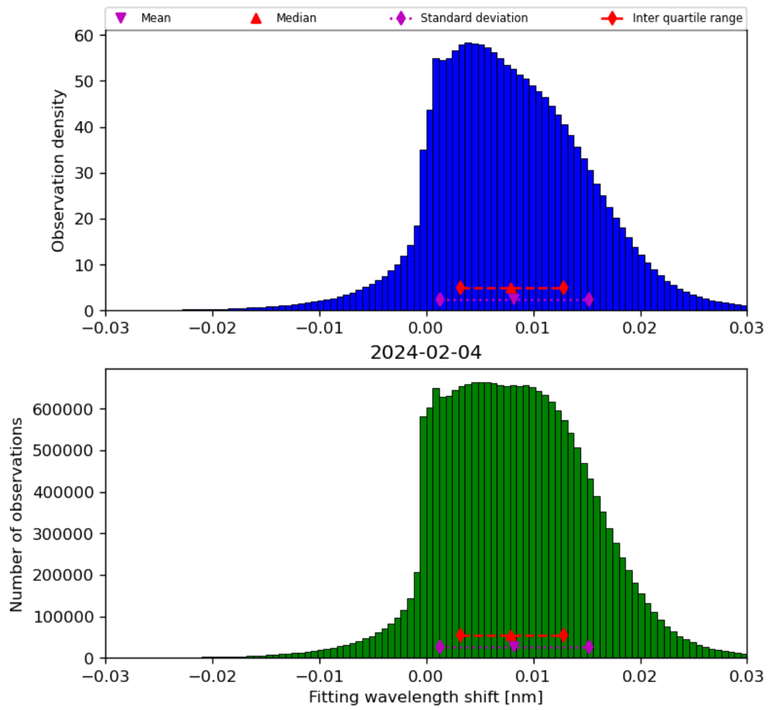
Figure 49: Histogram of “Fitting wavelength shift” for 2024-02-03 to 2024-02-05
