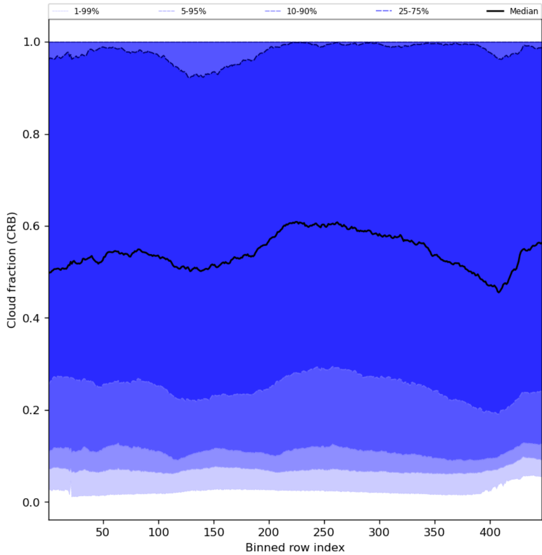
Figure 58: Along track statistics of “Cloud fraction (CRB)” for 2024-02-04 to 2024-02-06
