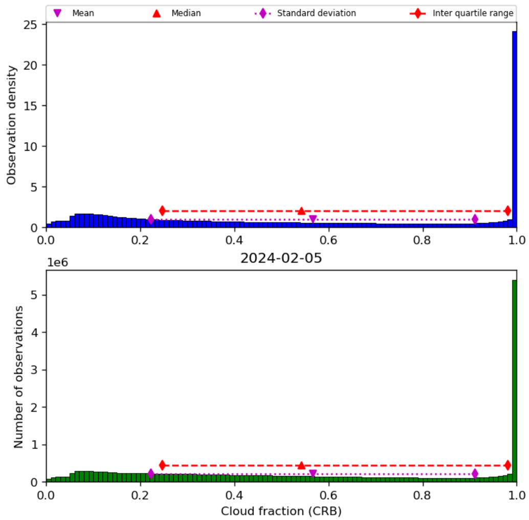
Figure 42: Histogram of “Cloud fraction (CRB)” for 2024-02-04 to 2024-02-06
