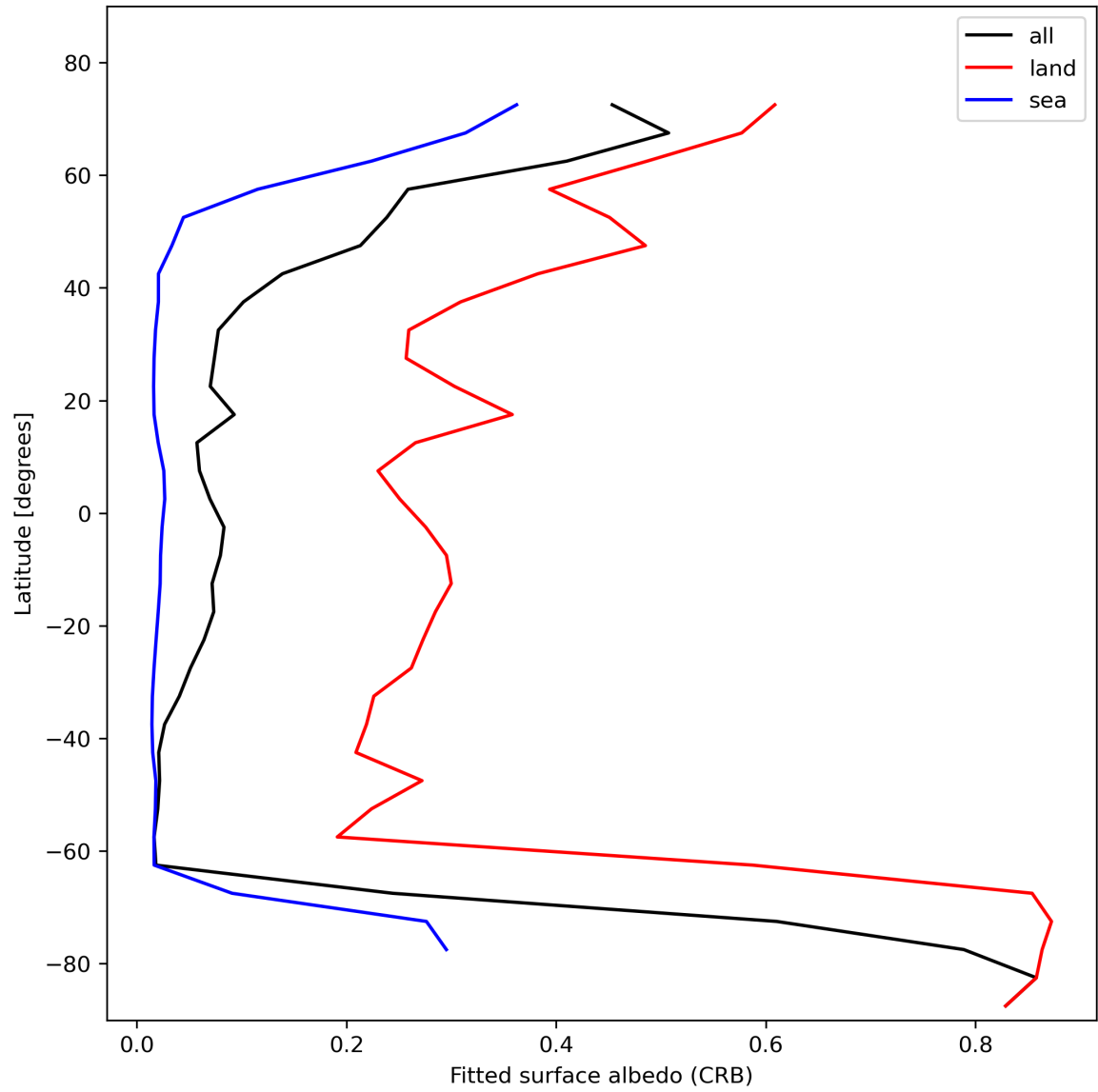
Figure 30: Zonal average of “Fitted surface albedo (CRB)” for 2024-02-04 to 2024-02-06.
