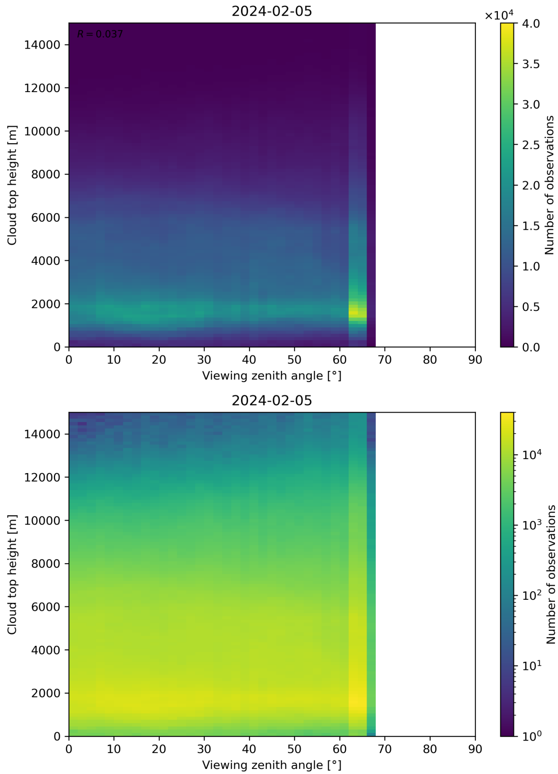
Figure 112: Scatter density plot of “Viewing zenith angle” against “Cloud top height” for 2024-02-04 to 2024-02-06.
