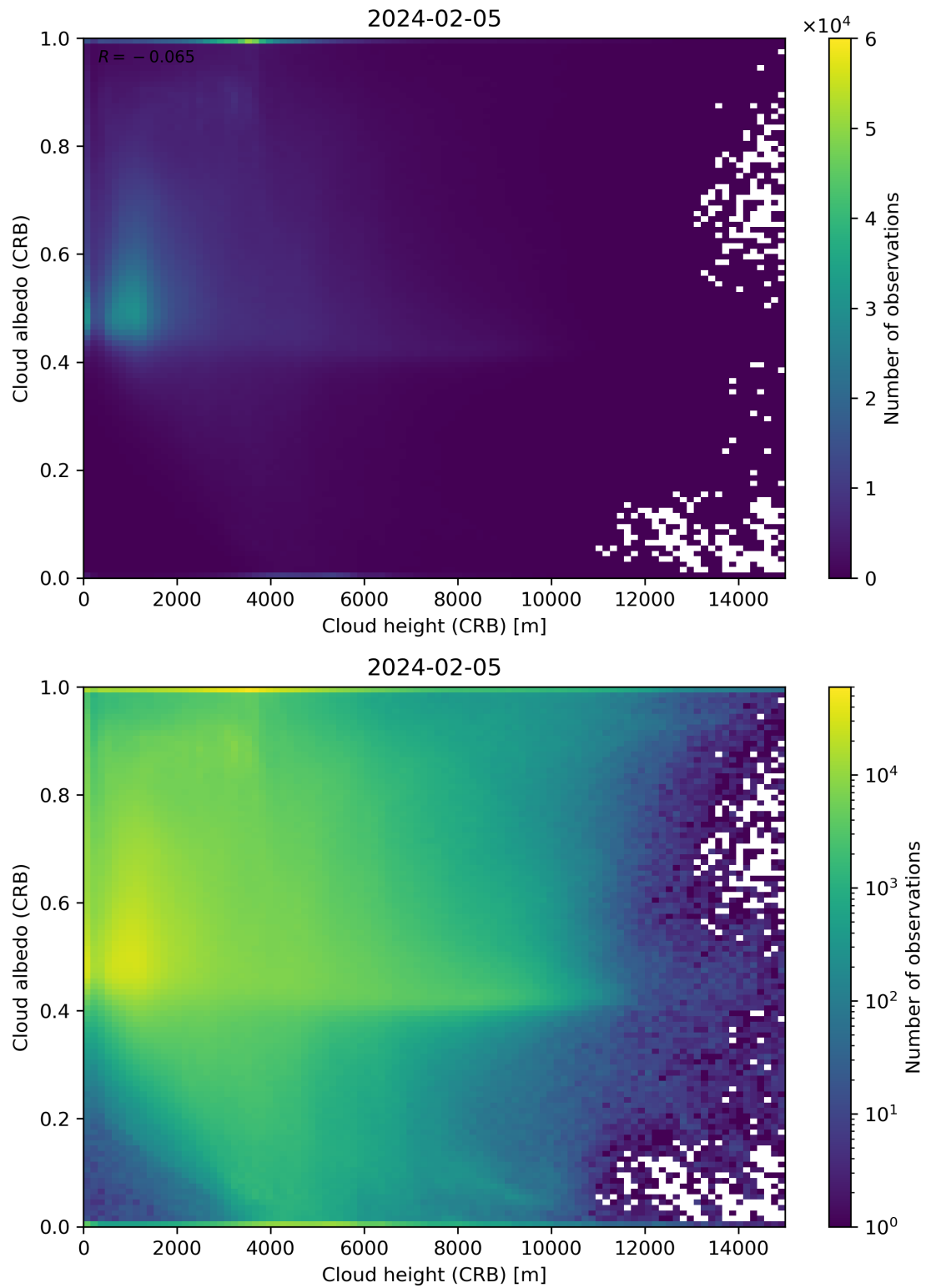
Figure 80: Scatter density plot of “Cloud height (CRB)” against “Cloud albedo (CRB)” for 2024-02-04 to 2024-02-06.
