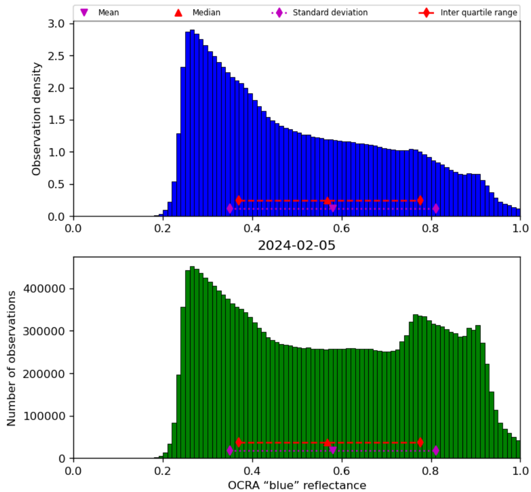
Figure 51: Histogram of “OCRA “blue” reflectance” for 2024-02-04 to 2024-02-06
