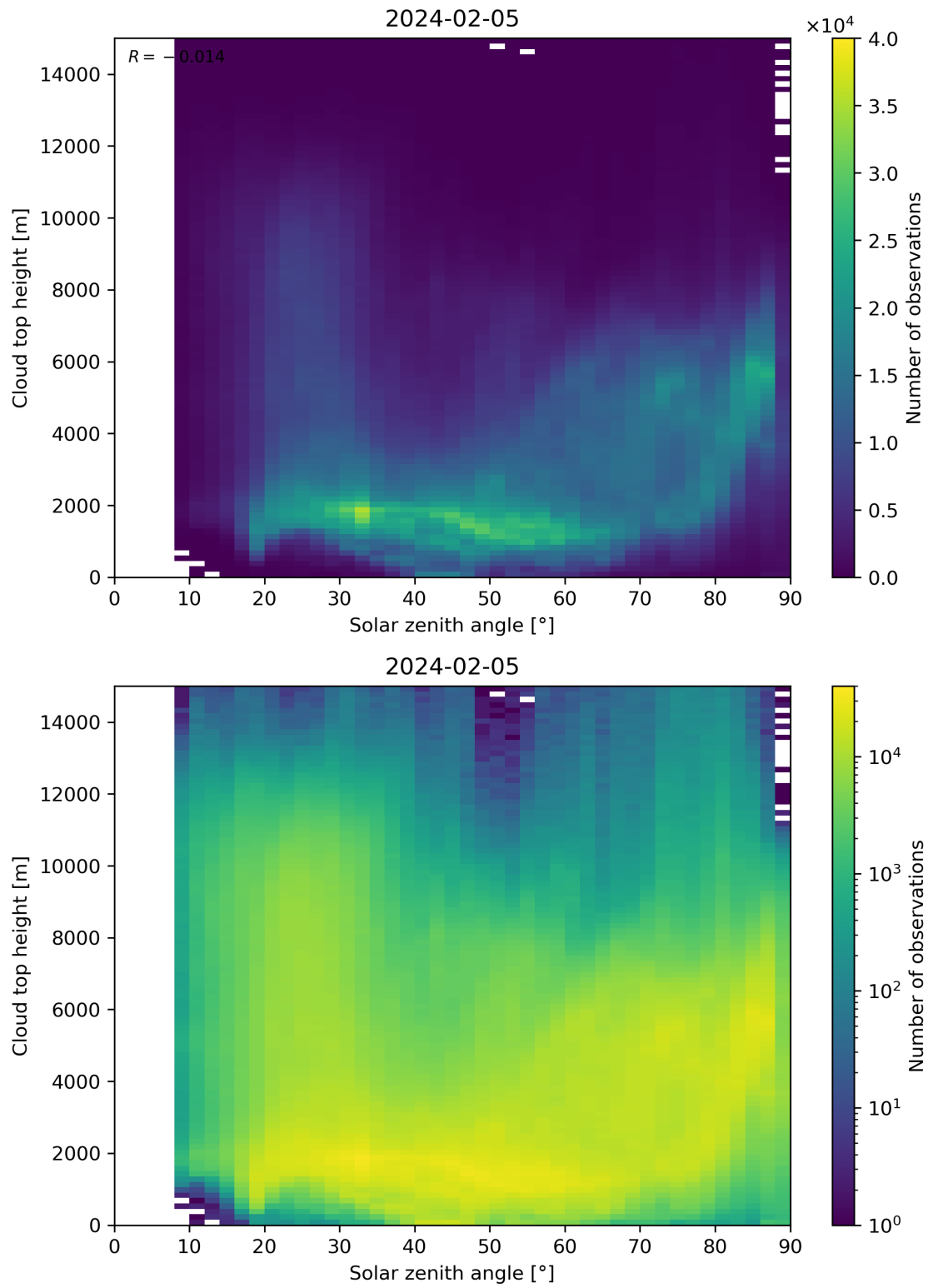
Figure 104: Scatter density plot of “Solar zenith angle” against “Cloud top height” for 2024-02-04 to 2024-02-06.
