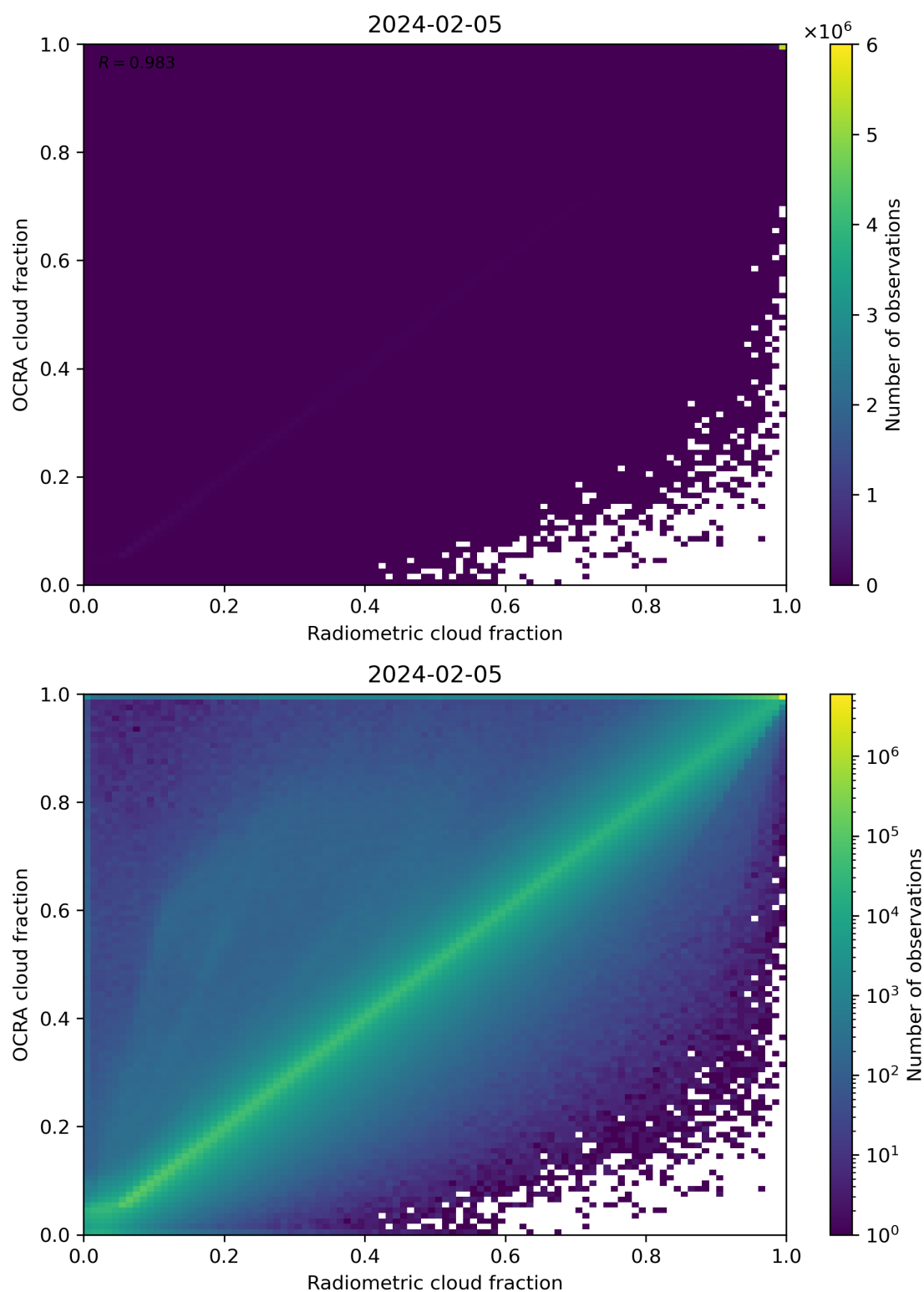
Figure 72: Scatter density plot of “Radiometric cloud fraction” against “OCRA cloud fraction” for 2024-02-04 to 2024-02-06.
