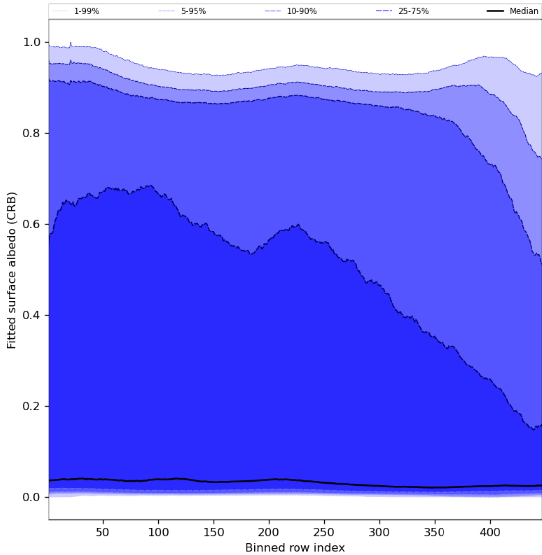
Figure 62: Along track statistics of “Fitted surface albedo (CRB)” for 2024-02-04 to 2024-02-06
