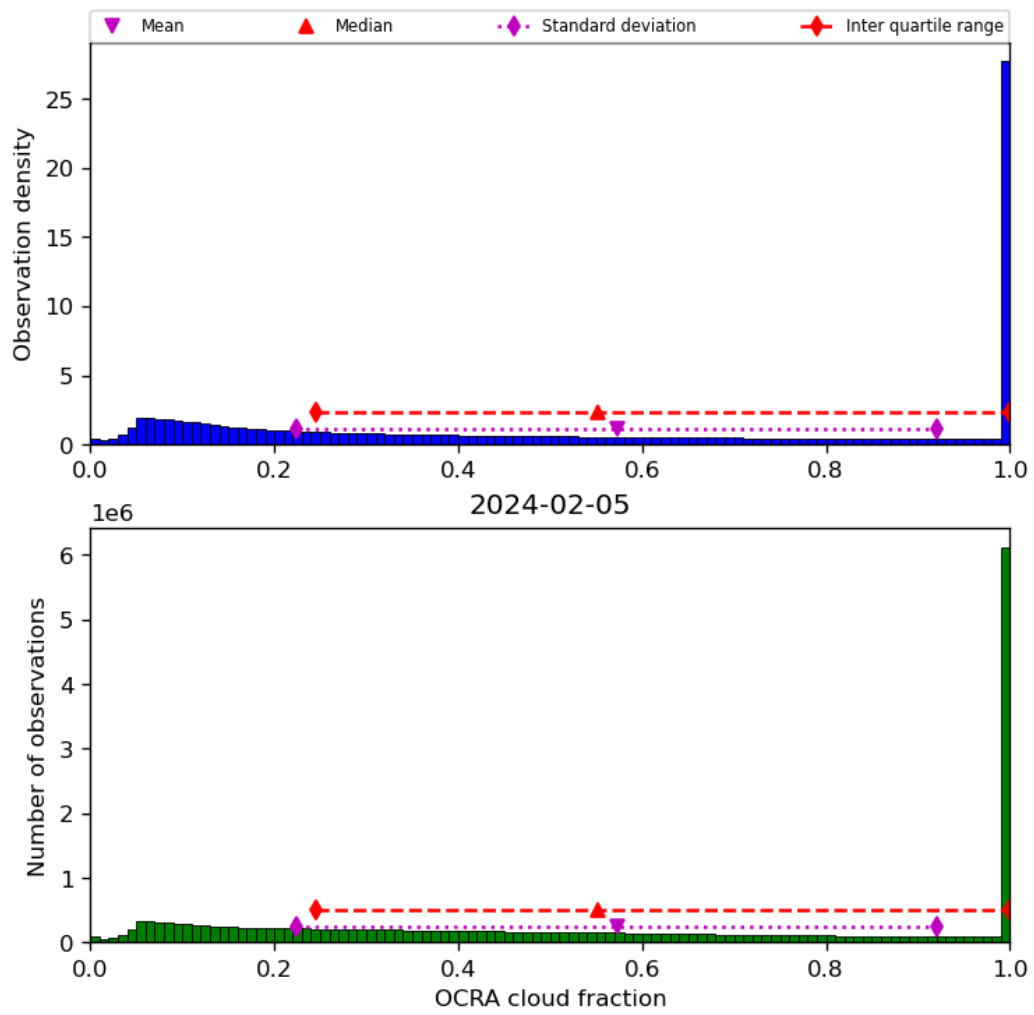
Figure 50: Histogram of “OCRA cloud fraction” for 2024-02-04 to 2024-02-06
