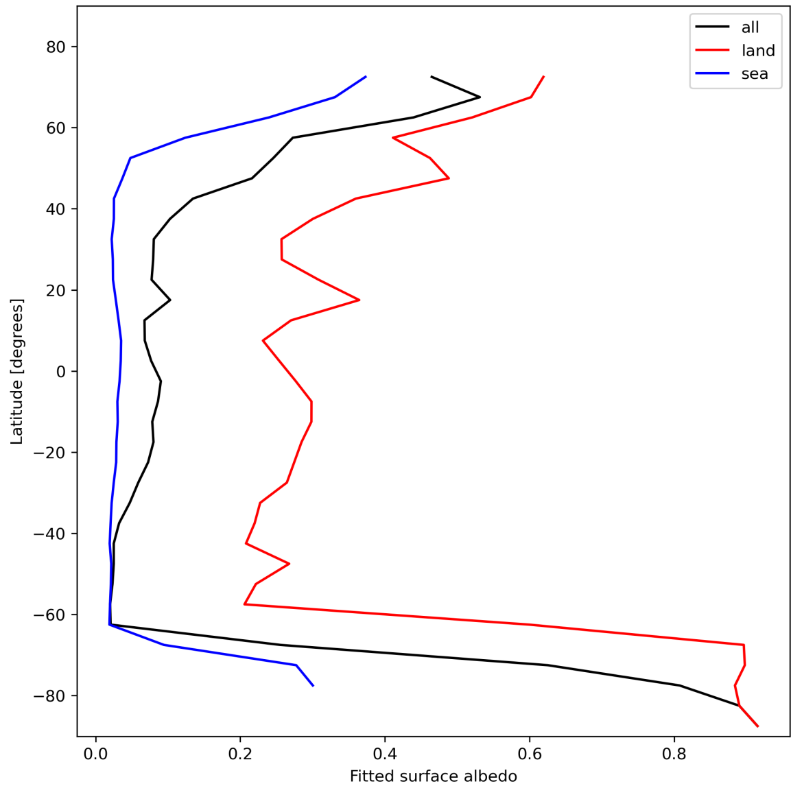
Figure 29: Zonal average of “Fitted surface albedo” for 2024-02-04 to 2024-02-06.
