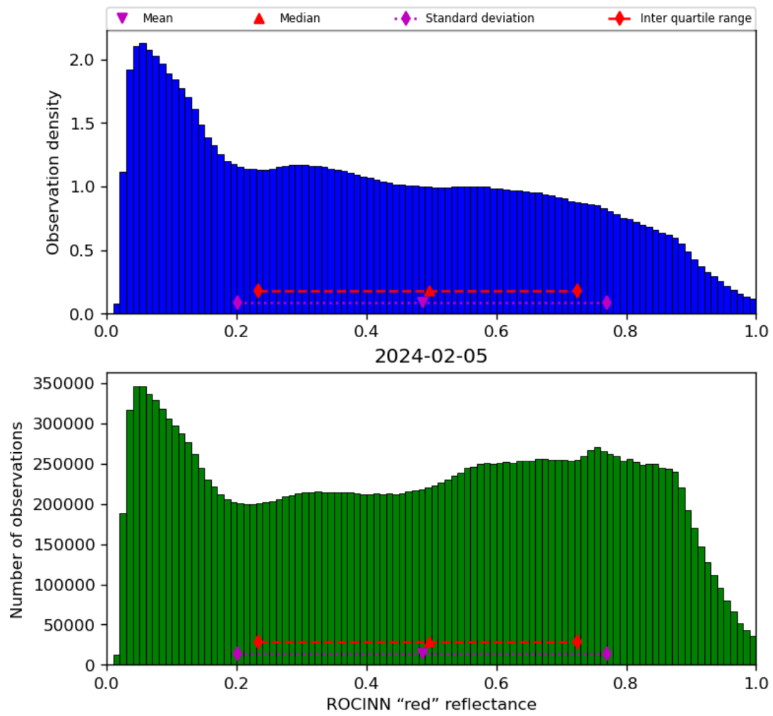
Figure 53: Histogram of “ROCINN “red” reflectance” for 2024-02-04 to 2024-02-06
