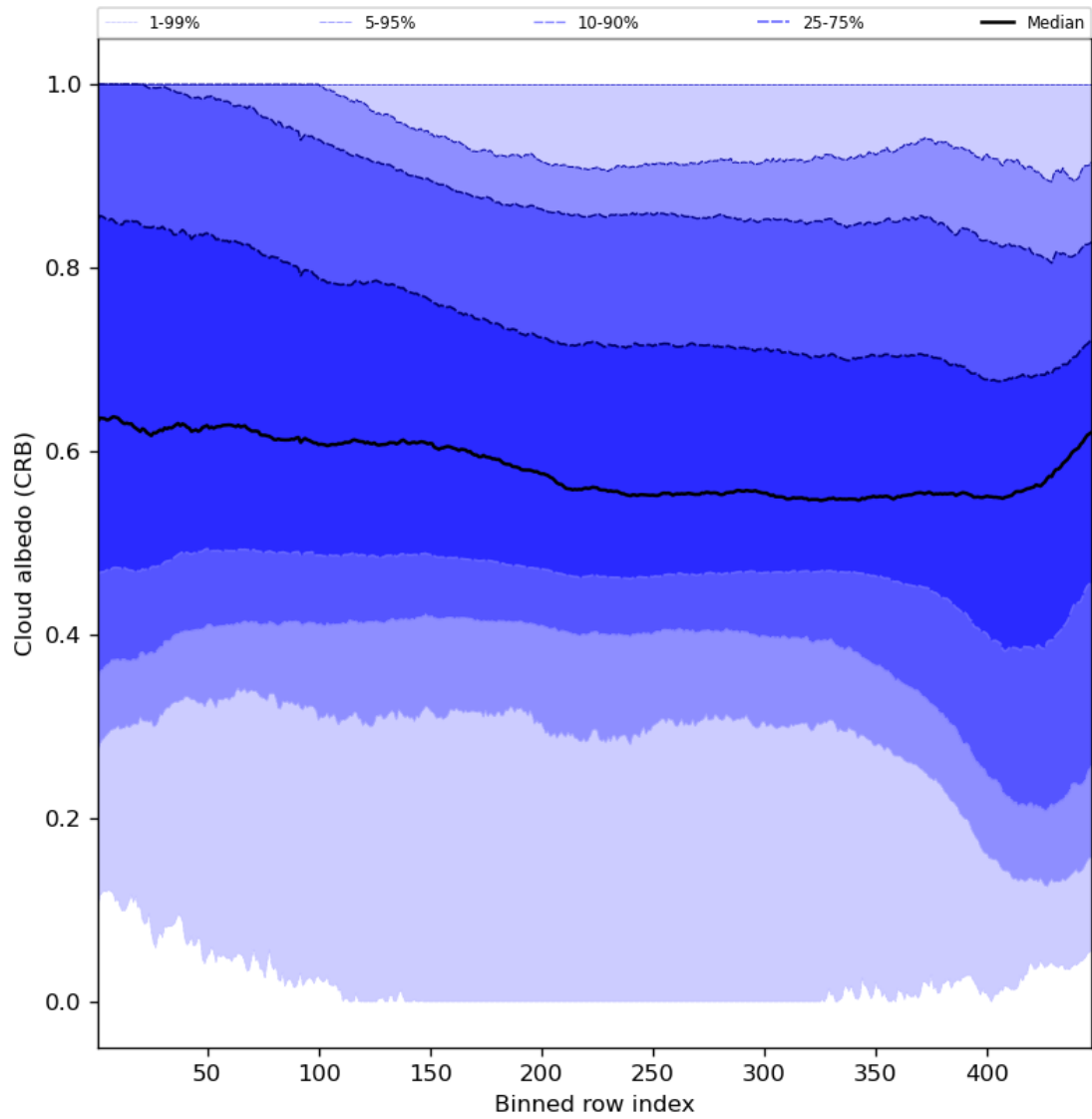
Figure 60: Along track statistics of “Cloud albedo (CRB)” for 2024-02-04 to 2024-02-06
