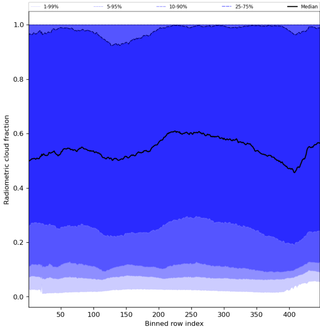
Figure 55: Along track statistics of “Radiometric cloud fraction” for 2024-02-04 to 2024-02-06
