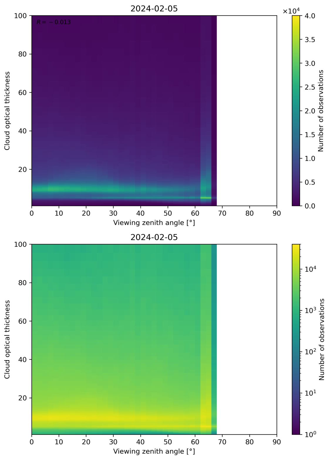
Figure 111: Scatter density plot of “Viewing zenith angle” against “Cloud optical thickness” for 2024-02-04 to 2024-02-06.
