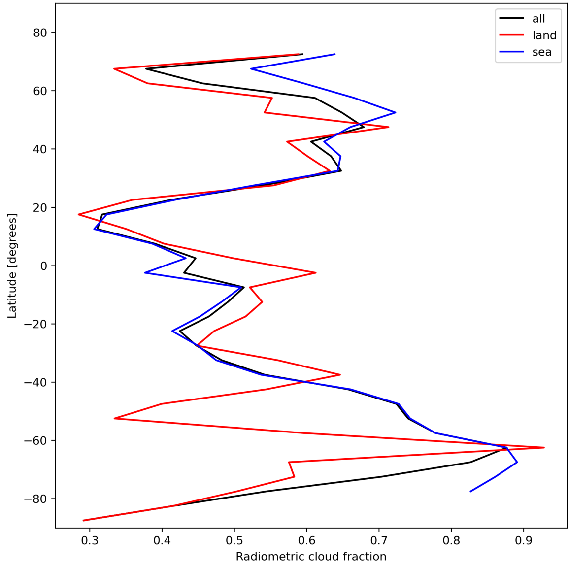
Figure 23: Zonal average of “Radiometric cloud fraction” for 2024-02-04 to 2024-02-06.
