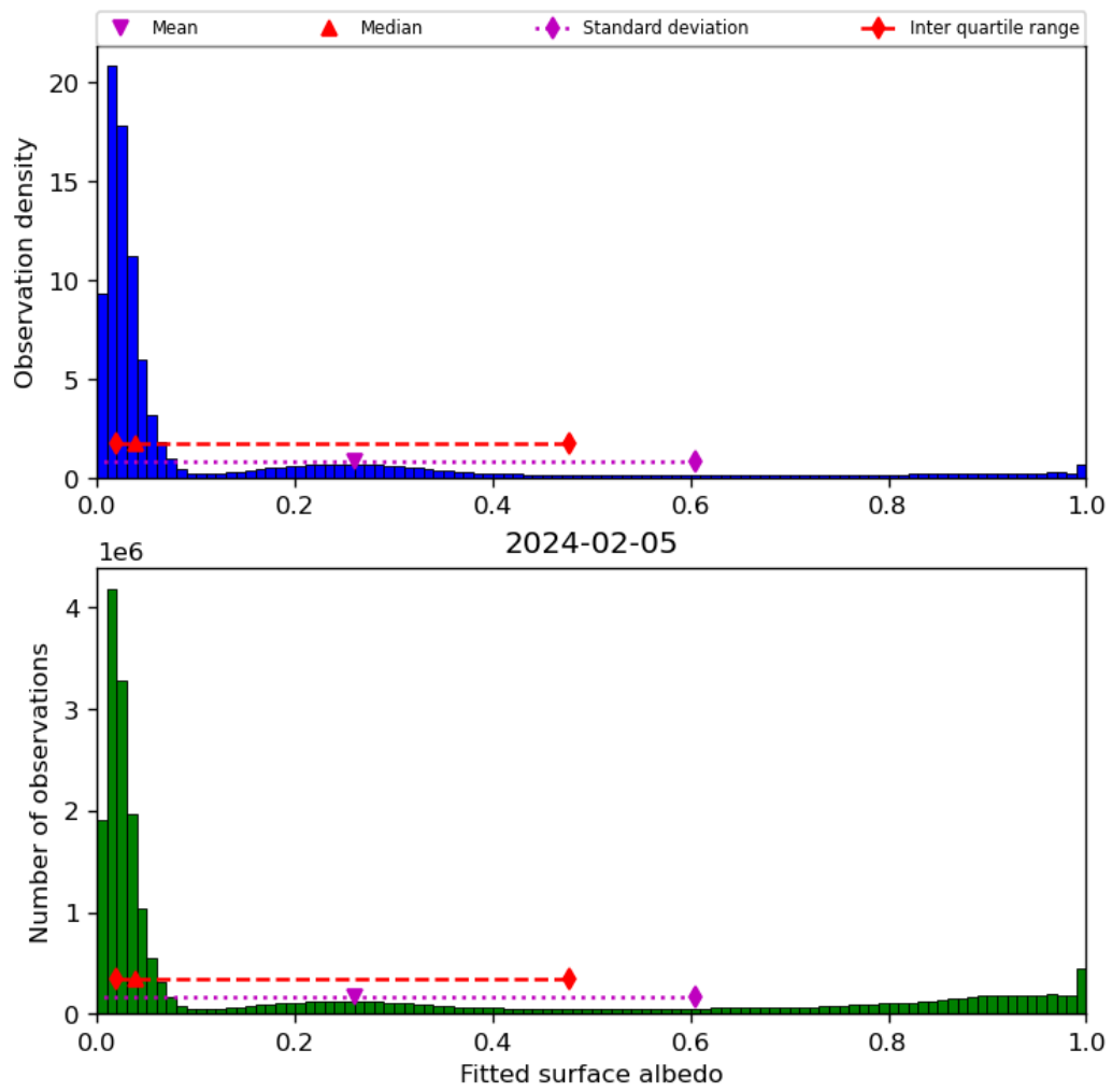
Figure 45: Histogram of “Fitted surface albedo” for 2024-02-04 to 2024-02-06
