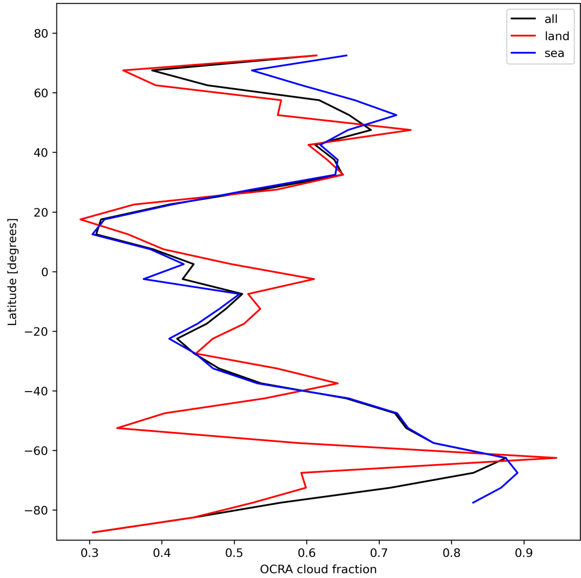
Figure 34: Zonal average of “OCRA cloud fraction” for 2024-02-04 to 2024-02-06.
