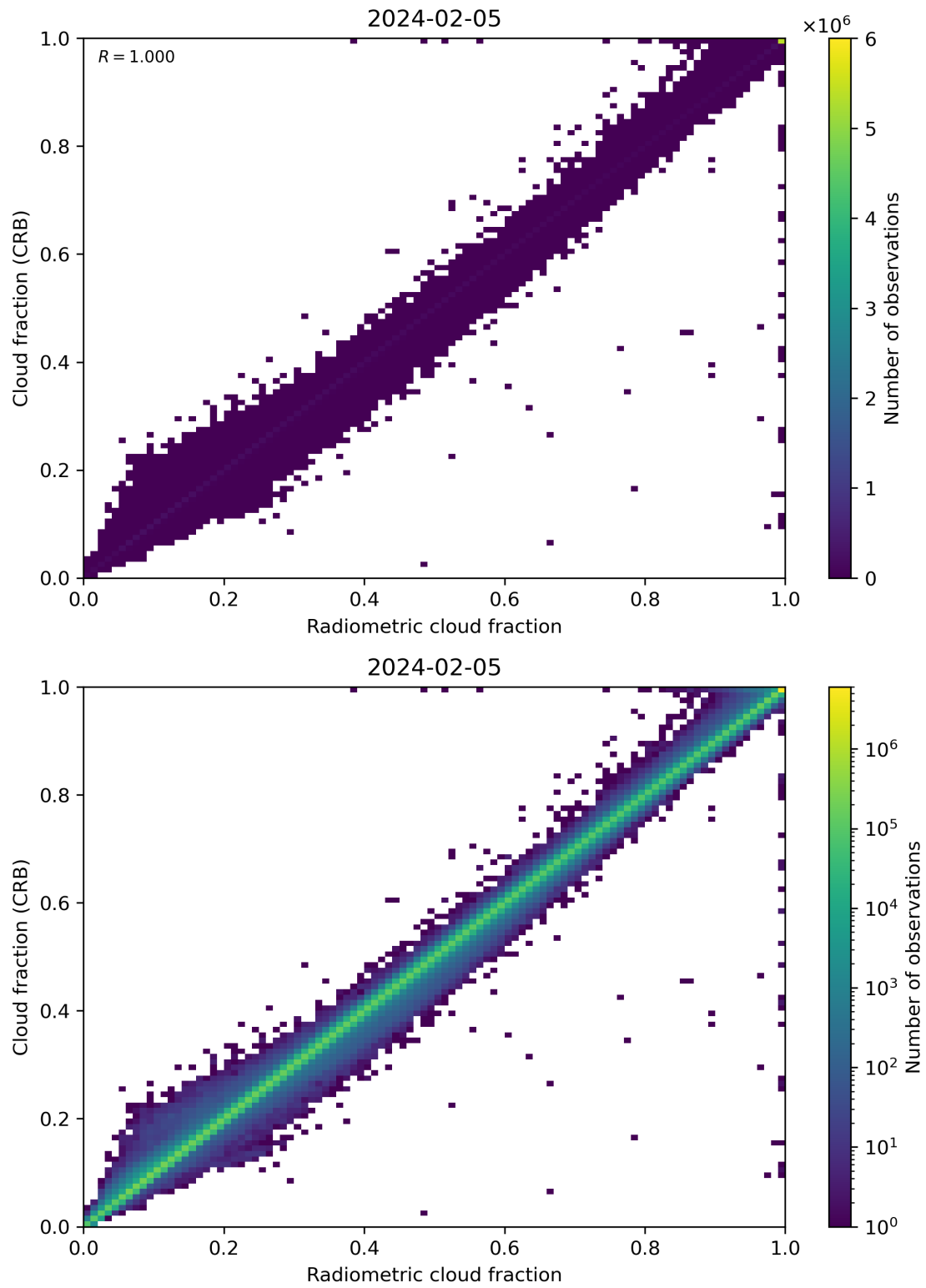
Figure 73: Scatter density plot of “Radiometric cloud fraction” against “Cloud fraction (CRB)” for 2024-02-04 to 2024-02-06.
