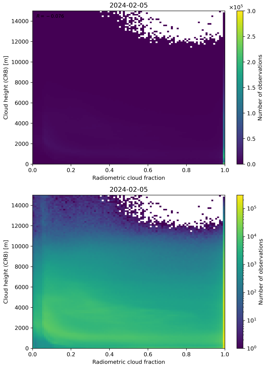
Figure 74: Scatter density plot of “Radiometric cloud fraction” against “Cloud height (CRB)” for 2024-02-04 to 2024-02-06.
