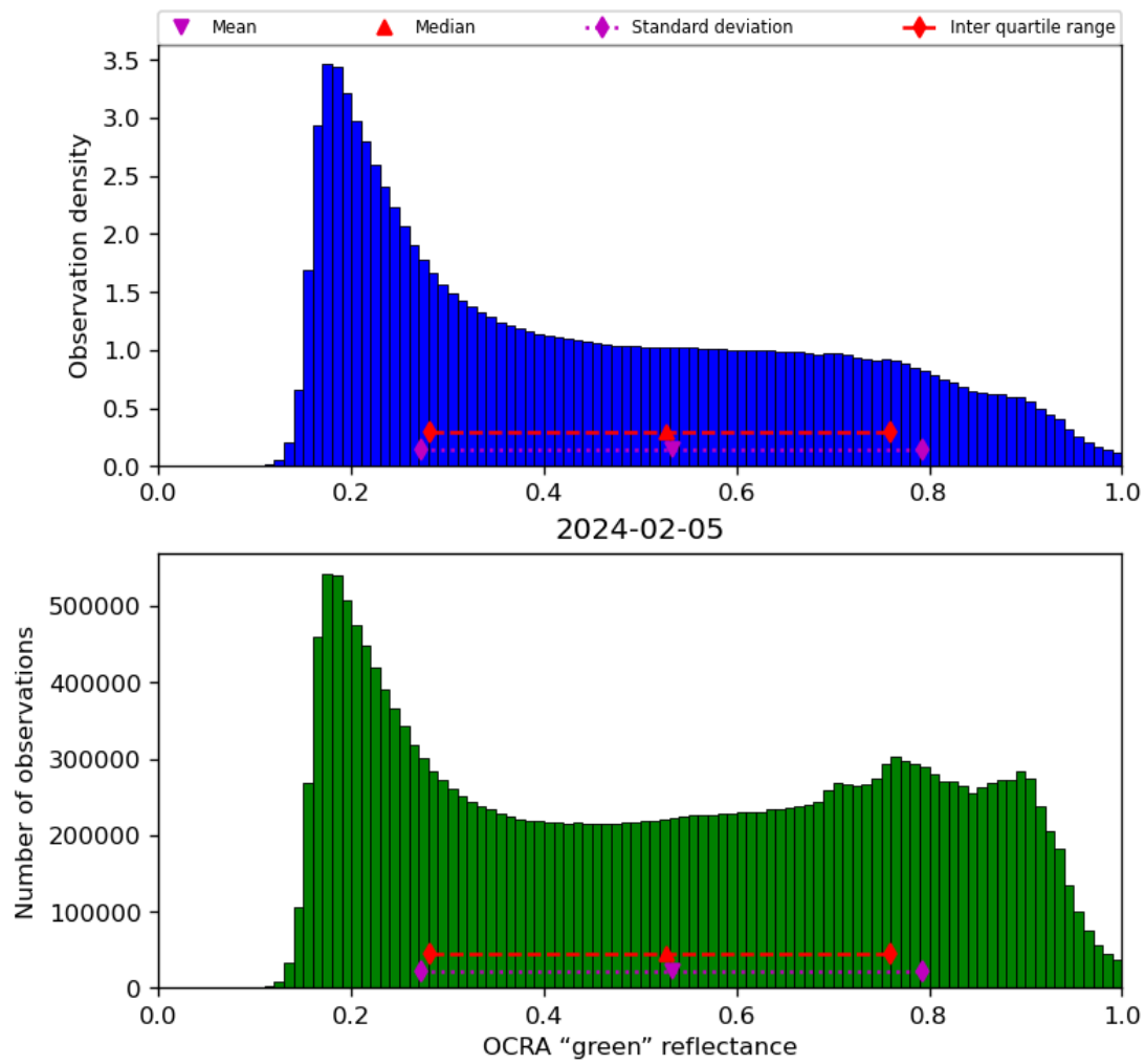
Figure 52: Histogram of “OCRA “green” reflectance” for 2024-02-04 to 2024-02-06
