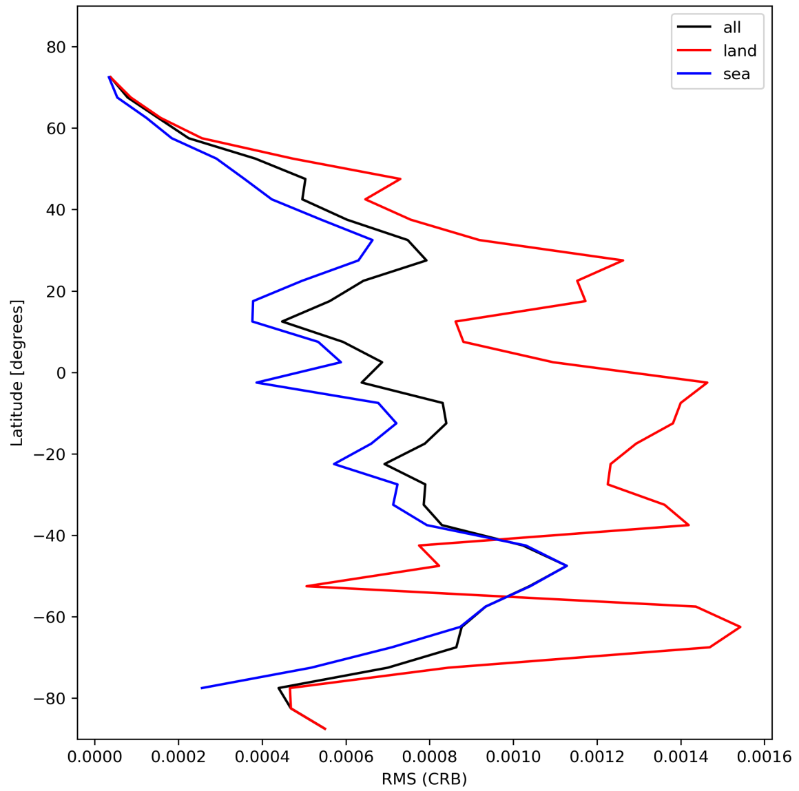
Figure 32: Zonal average of “RMS (CRB)” for 2024-02-04 to 2024-02-06.
