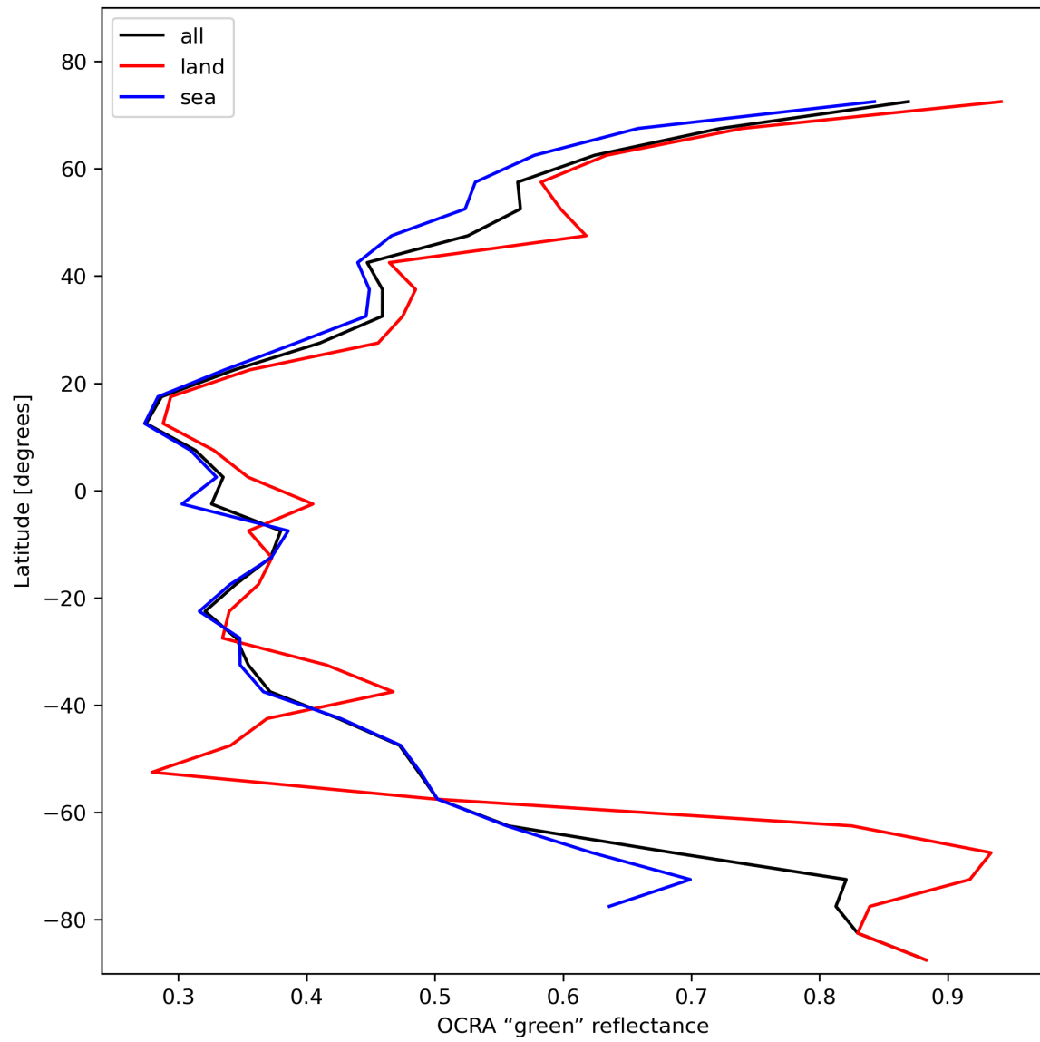
Figure 36: Zonal average of “OCRA “green” reflectance” for 2024-02-04 to 2024-02-06.
