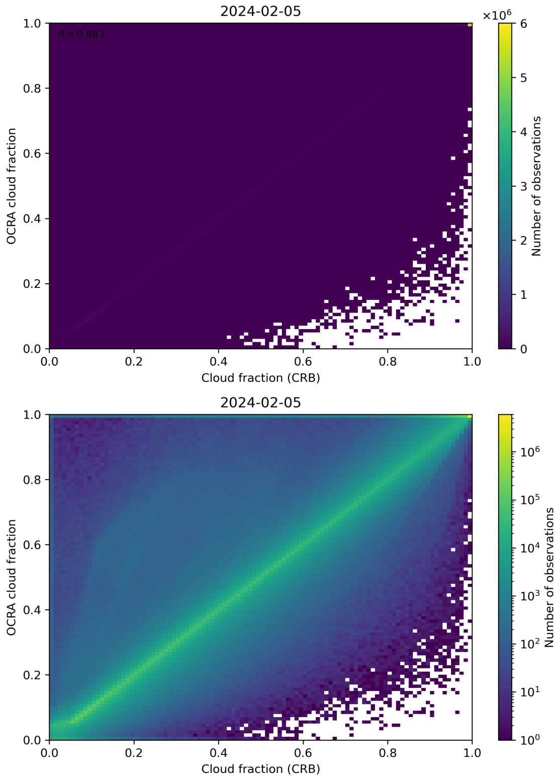
Figure 78: Scatter density plot of “Cloud fraction (CRB)” against “OCRA cloud fraction” for 2024-02-04 to 2024-02-06.
