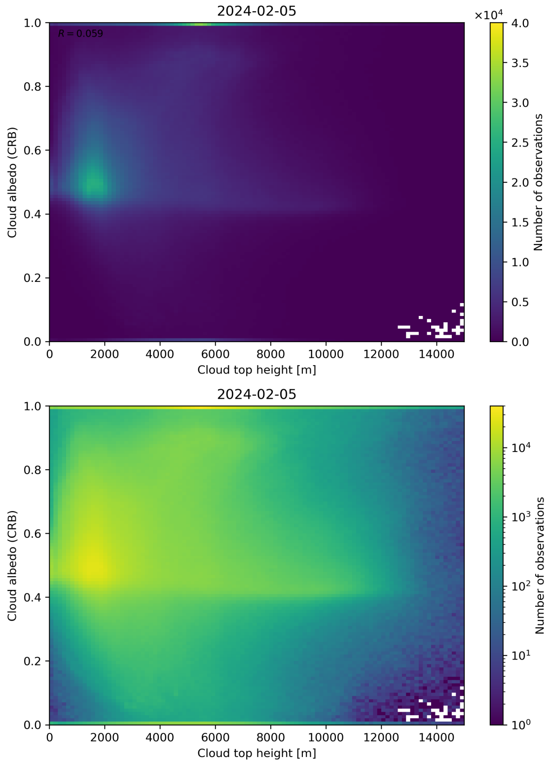
Figure 86: Scatter density plot of “Cloud top height” against “Cloud albedo (CRB)” for 2024-02-04 to 2024-02-06.
