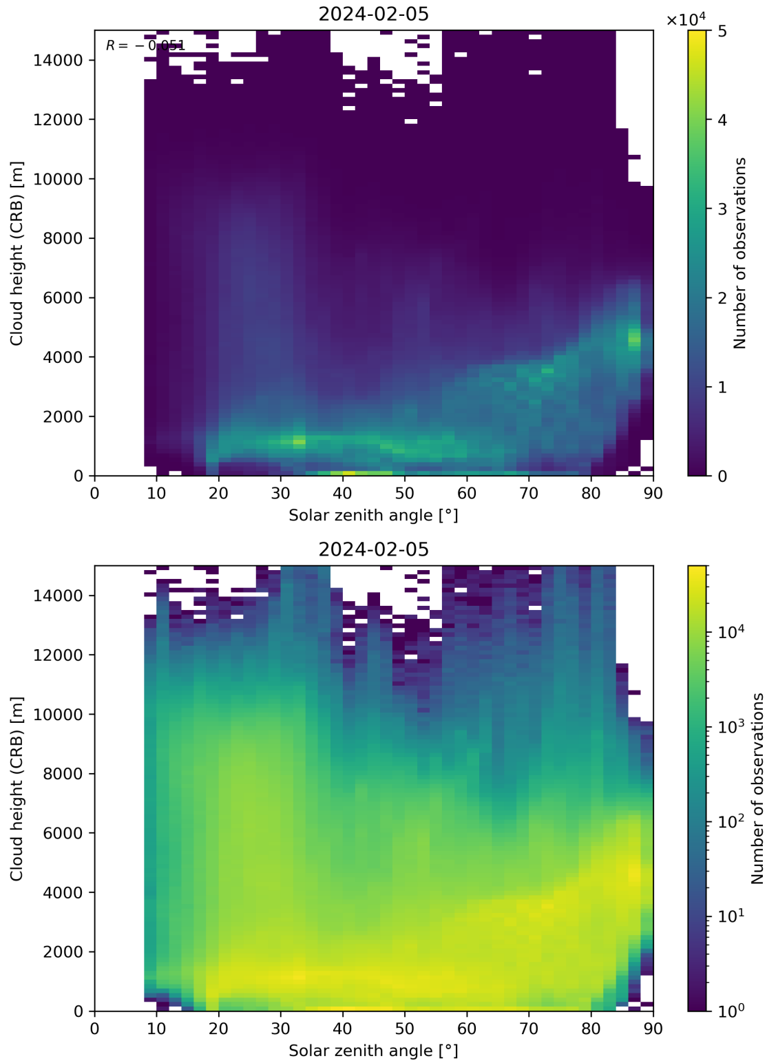
Figure 102: Scatter density plot of “Solar zenith angle” against “Cloud height (CRB)” for 2024-02-04 to 2024-02-06.
