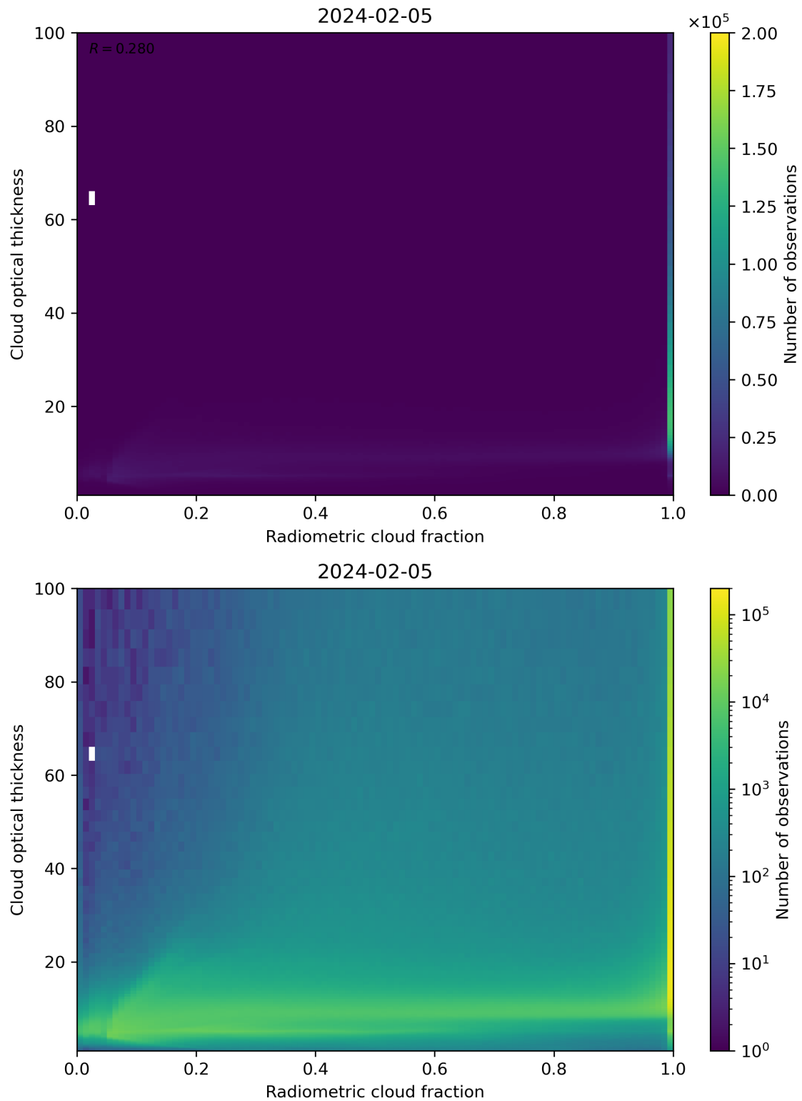
Figure 75: Scatter density plot of “Radiometric cloud fraction” against “Cloud optical thickness” for 2024-02-04 to 2024-02-06.
