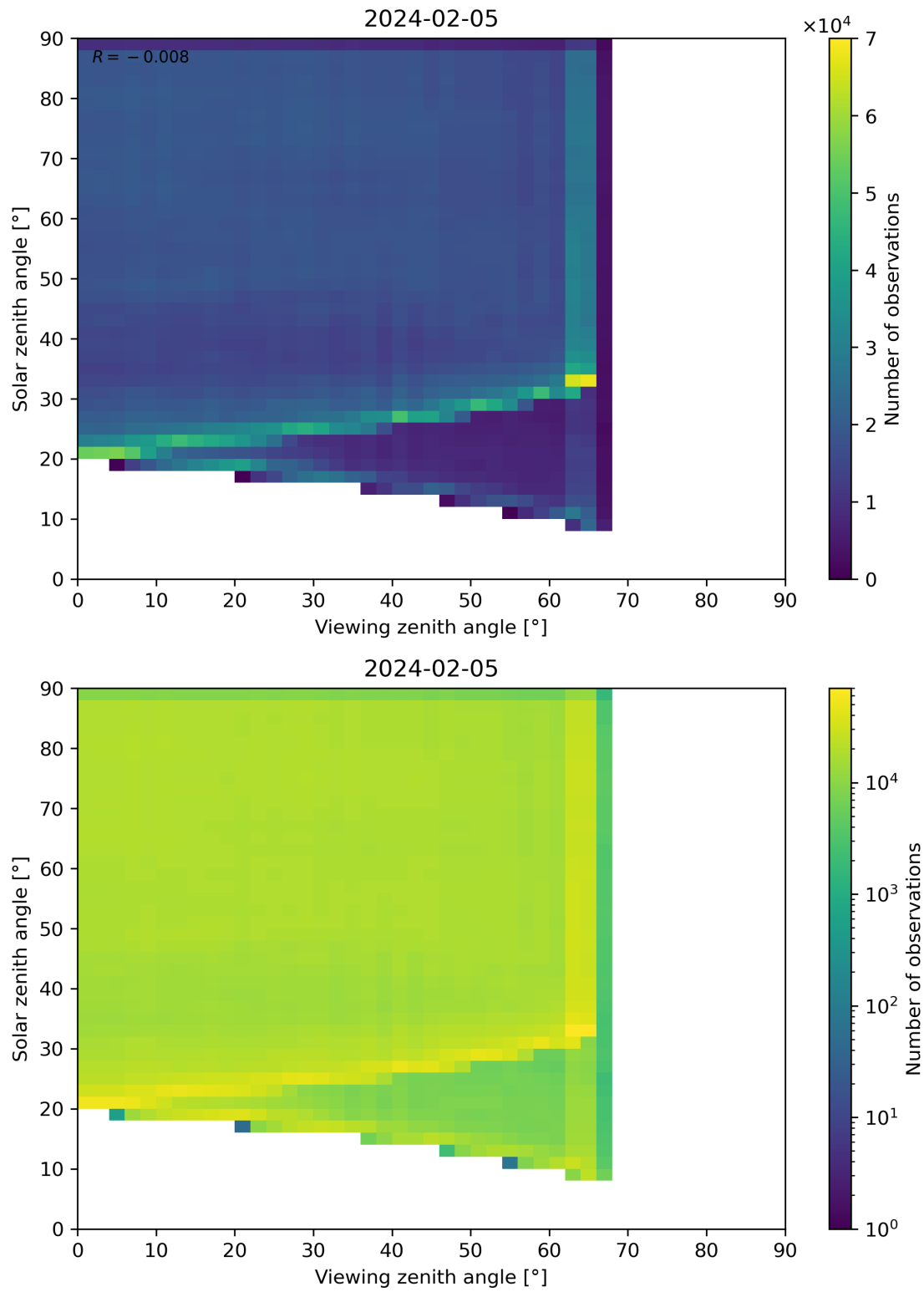
Figure 114: Scatter density plot of “Viewing zenith angle” against “Solar zenith angle” for 2024-02-04 to 2024-02-06.
