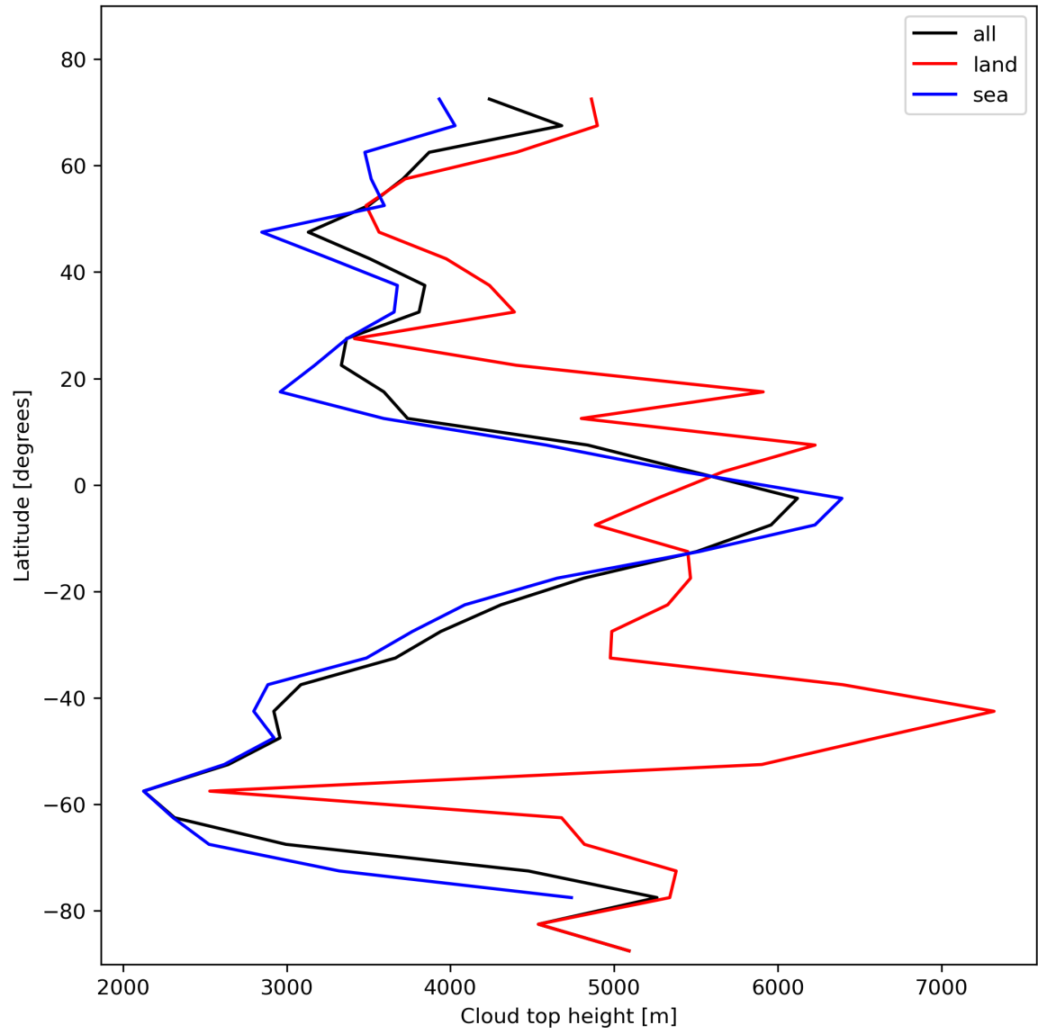
Figure 24: Zonal average of “Cloud top height” for 2024-02-04 to 2024-02-06.
