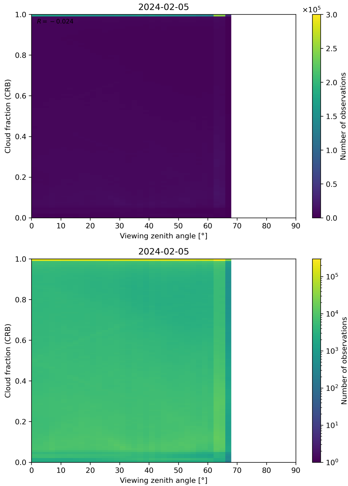
Figure 109: Scatter density plot of “Viewing zenith angle” against “Cloud fraction (CRB)” for 2024-02-04 to 2024-02-06.
