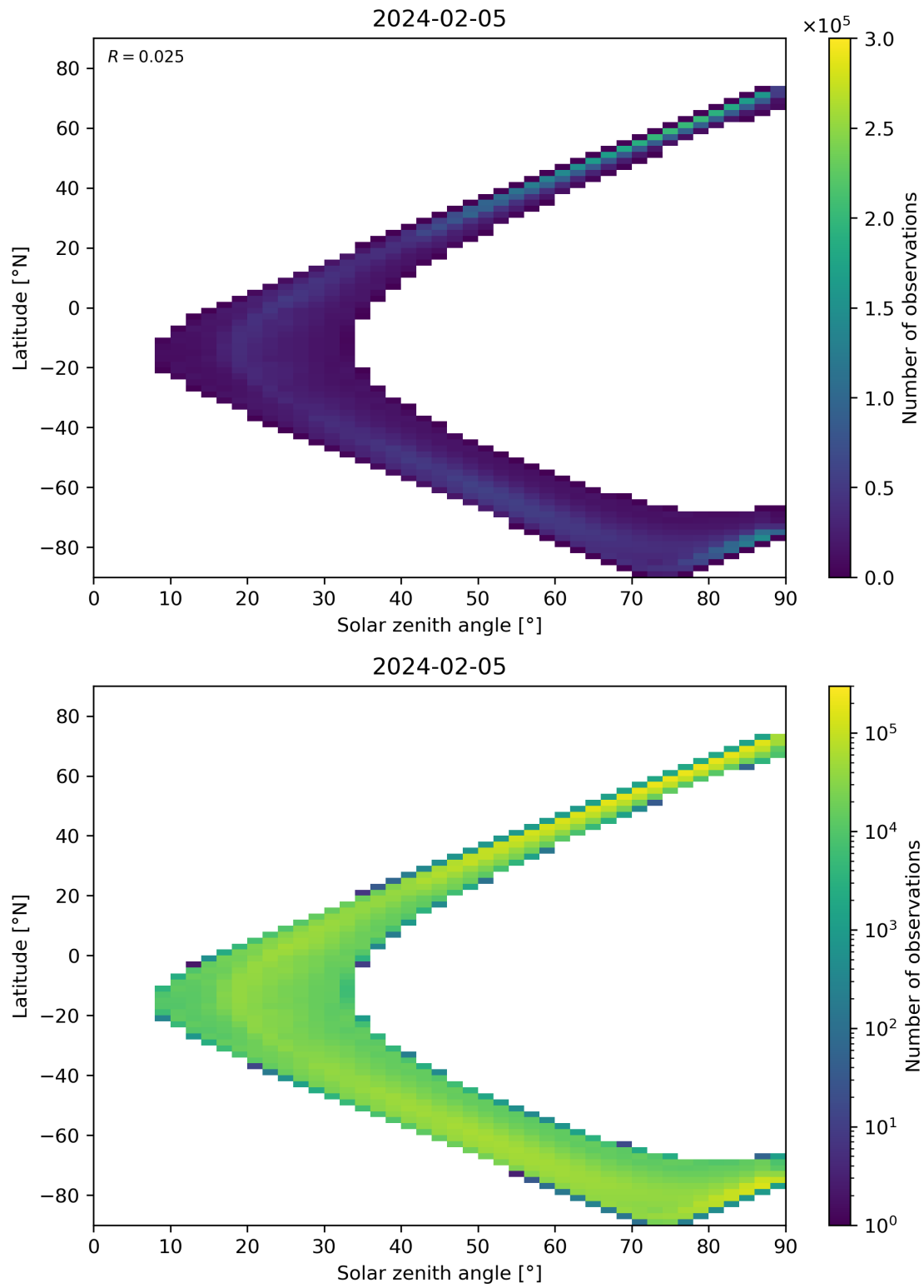
Figure 105: Scatter density plot of “Solar zenith angle” against “Latitude” for 2024-02-04 to 2024-02-06.
