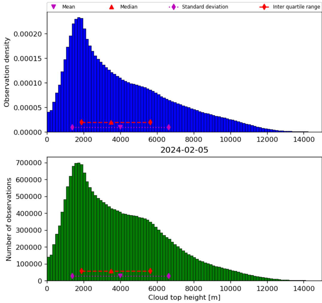
Figure 40: Histogram of “Cloud top height” for 2024-02-04 to 2024-02-06
