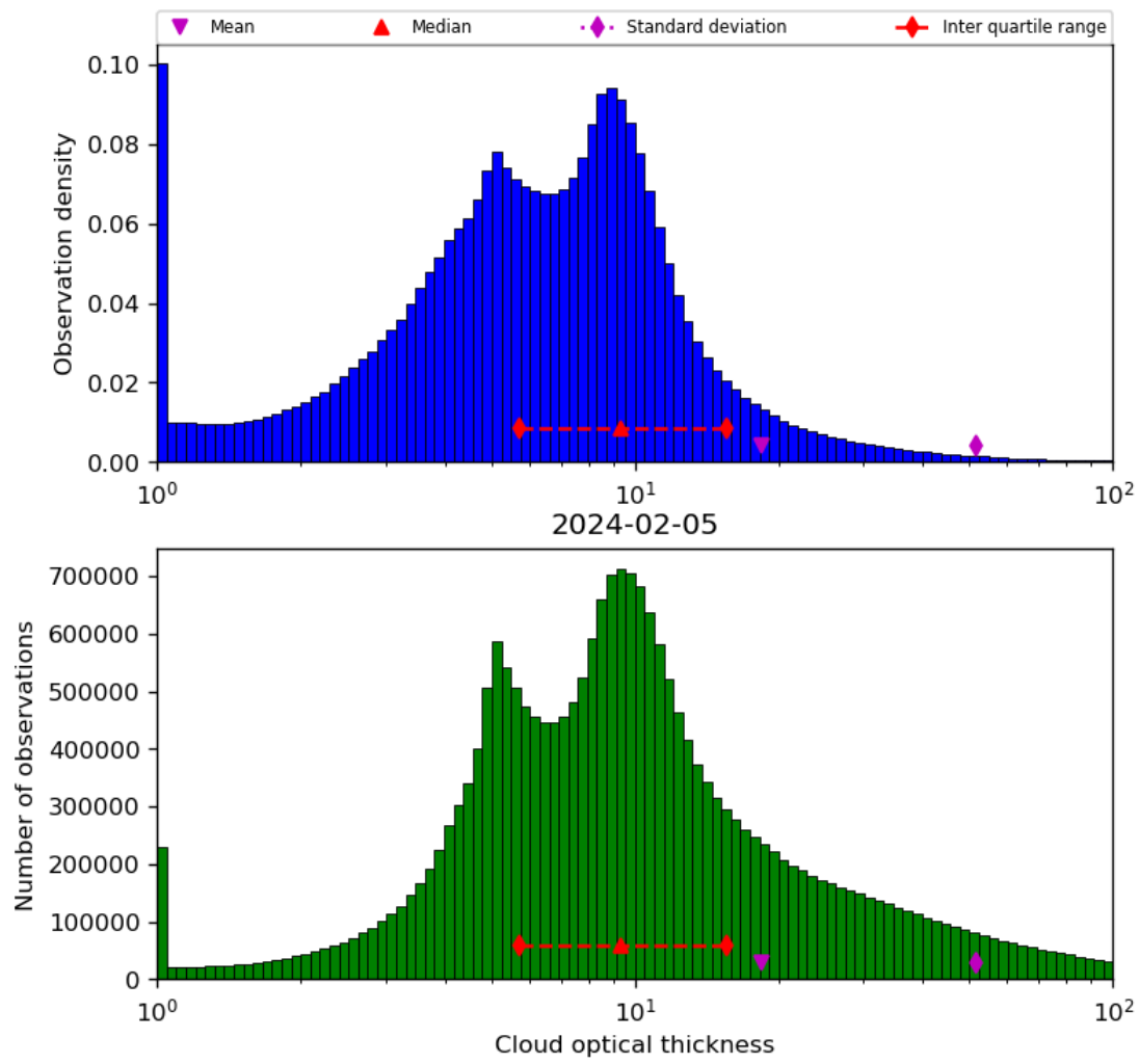
Figure 41: Histogram of “Cloud optical thickness” for 2024-02-04 to 2024-02-06
