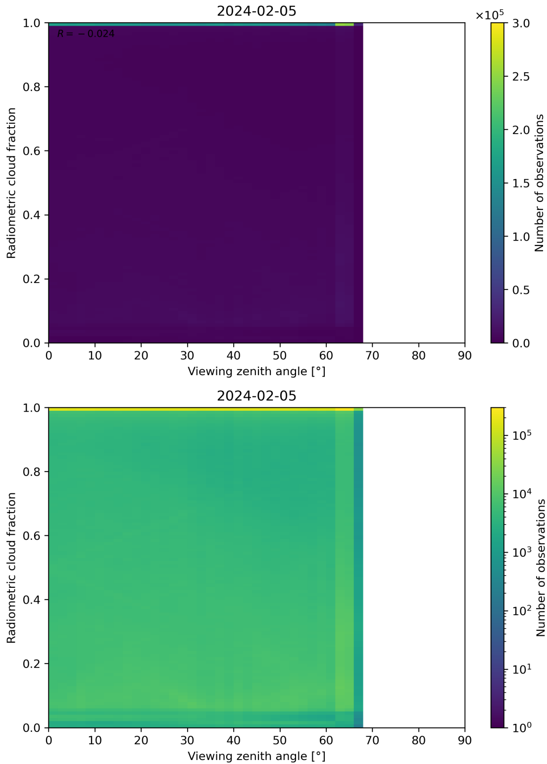
Figure 107: Scatter density plot of “Viewing zenith angle” against “Radiometric cloud fraction” for 2024-02-04 to 2024-02-06.
