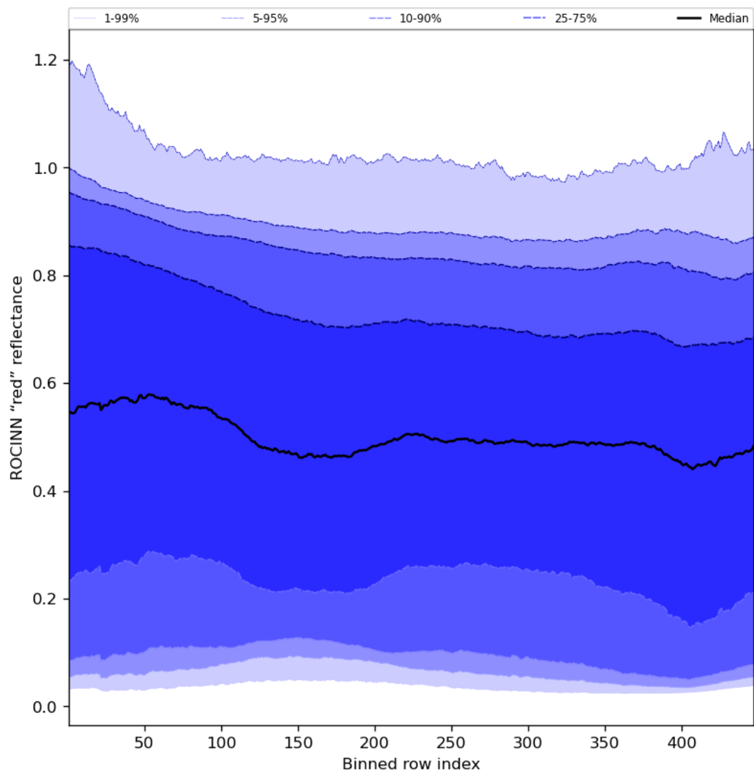
Figure 69: Along track statistics of "ROCINN "red" reflectance" for 2024-02-04 to 2024-02-06
