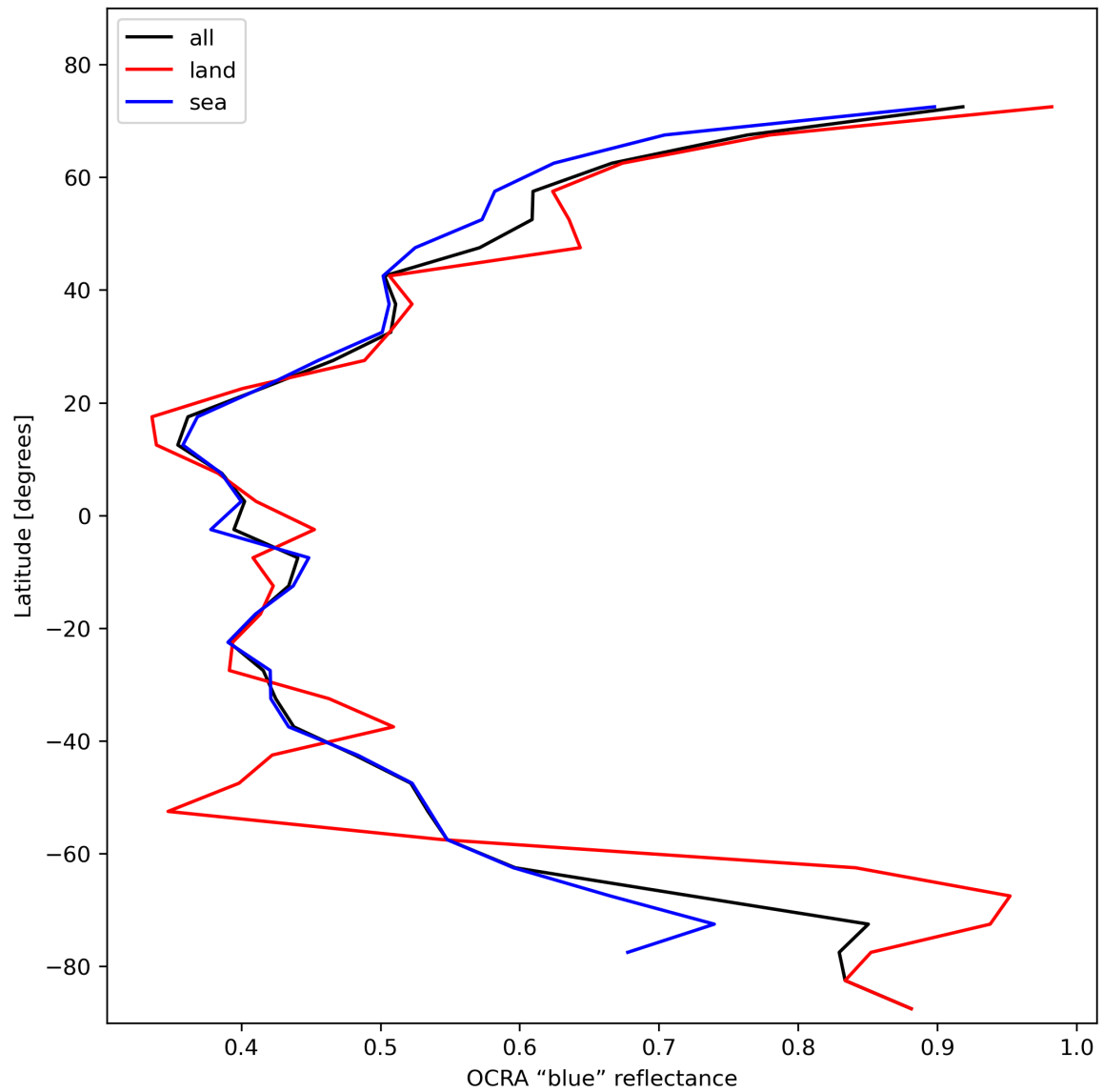
Figure 35: Zonal average of “OCRA “blue” reflectance” for 2024-02-04 to 2024-02-06.
