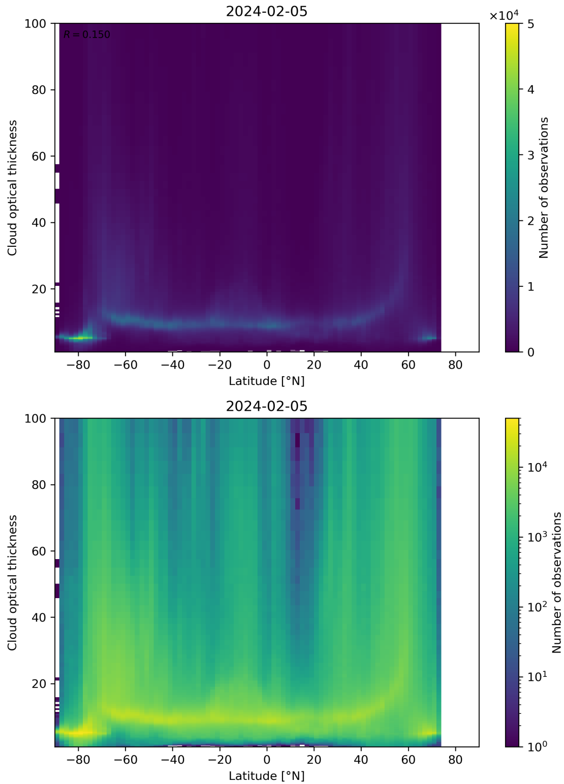
Figure 96: Scatter density plot of “Latitude” against “Cloud optical thickness” for 2024-02-04 to 2024-02-06.
