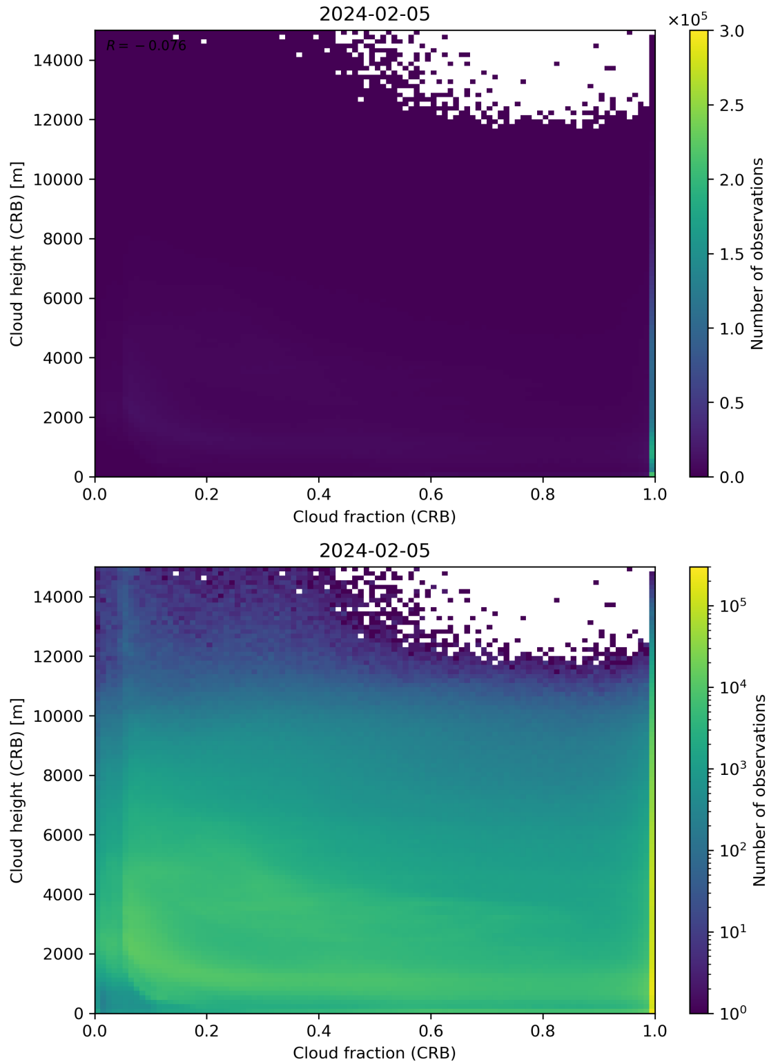
Figure 79: Scatter density plot of “Cloud fraction (CRB)” against “Cloud height (CRB)” for 2024-02-04 to 2024-02-06.
