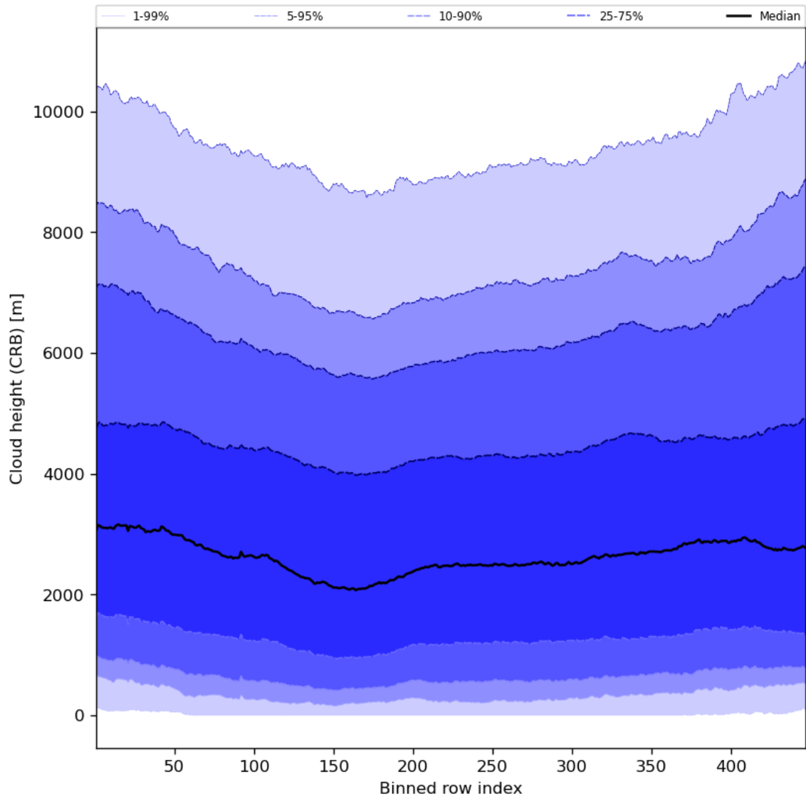
Figure 59: Along track statistics of “Cloud height (CRB)” for 2024-02-04 to 2024-02-06
