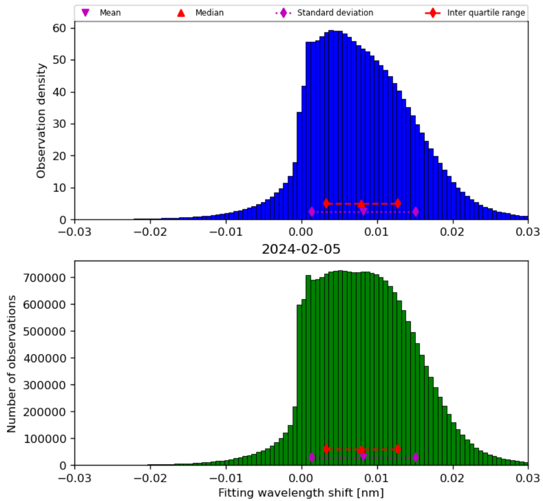
Figure 49: Histogram of “Fitting wavelength shift” for 2024-02-04 to 2024-02-06
