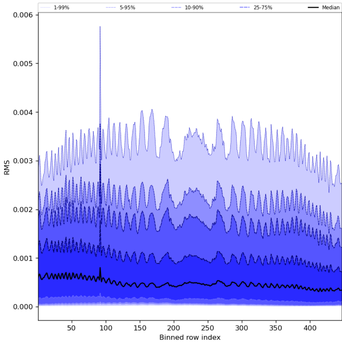
Figure 63: Along track statistics of “RMS” for 2024-02-04 to 2024-02-06
