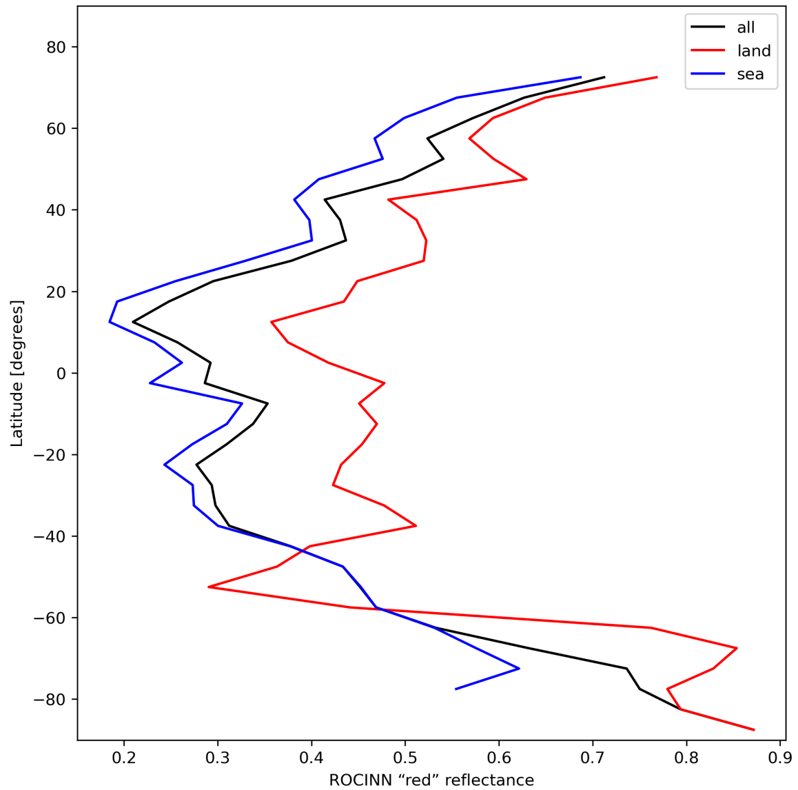
Figure 37: Zonal average of “ROCINN “red” reflectance” for 2024-02-04 to 2024-02-06.
