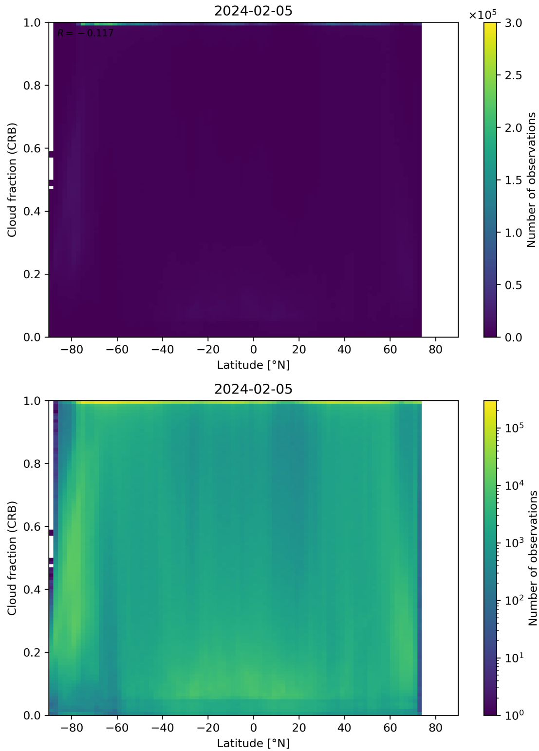
Figure 94: Scatter density plot of “Latitude” against “Cloud fraction (CRB)” for 2024-02-04 to 2024-02-06.
