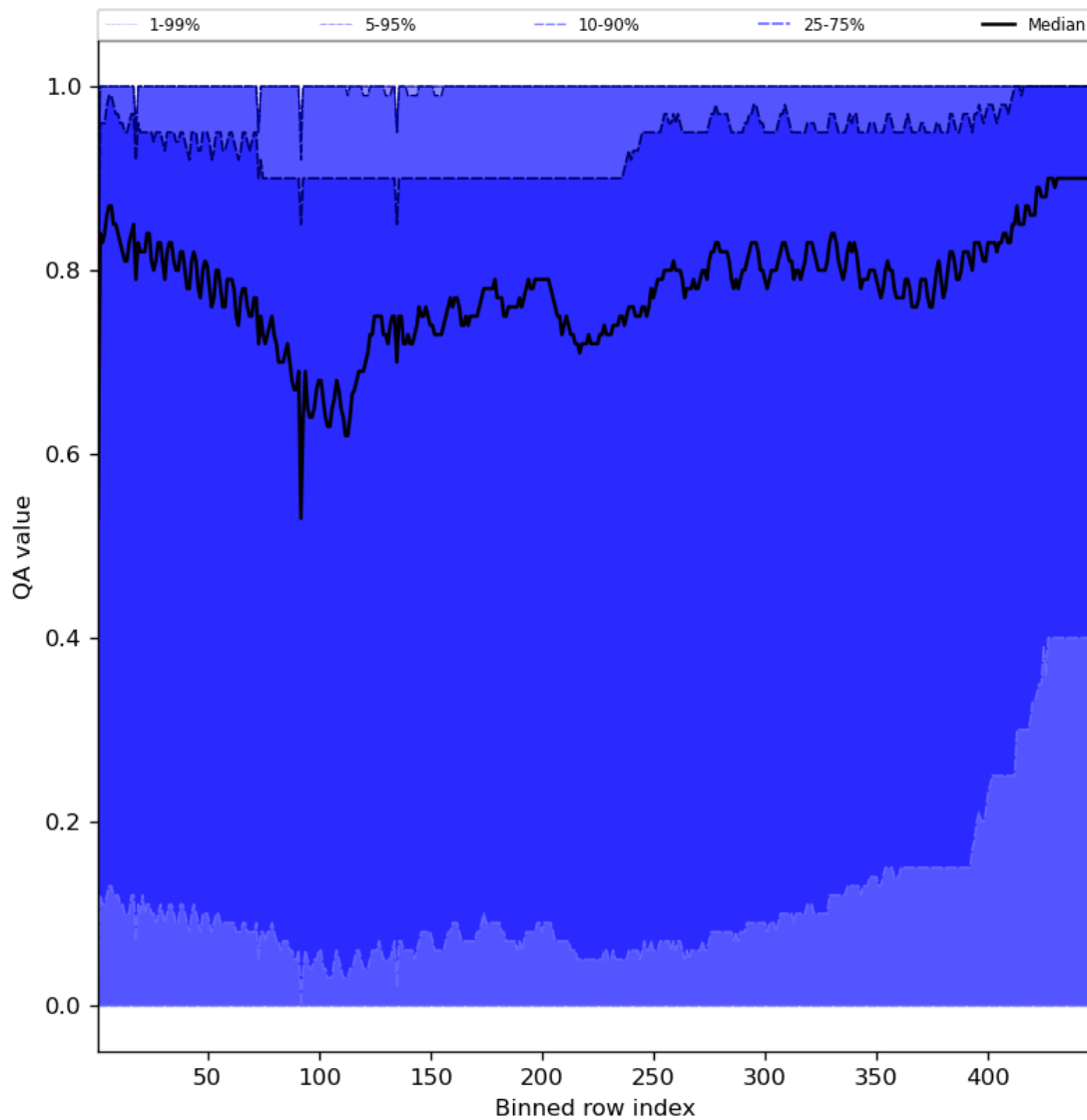
Figure 54: Along track statistics of “QA value” for 2024-02-04 to 2024-02-06
