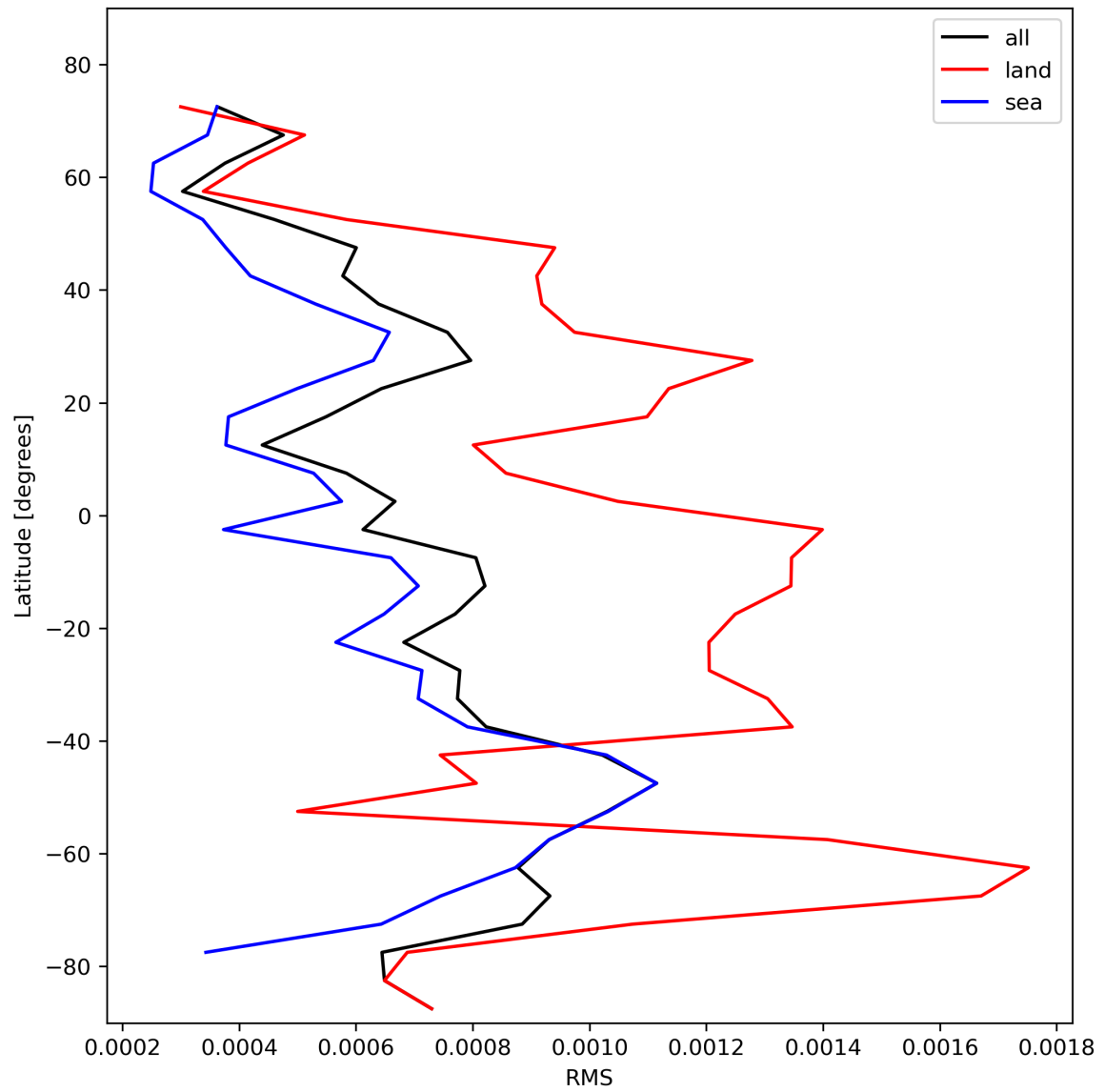
Figure 31: Zonal average of “RMS” for 2024-02-04 to 2024-02-06.
