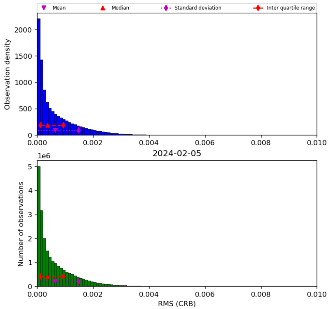
Figure 48: Histogram of “RMS (CRB)” for 2024-02-04 to 2024-02-06
