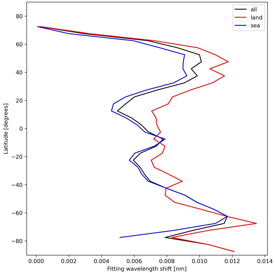
Figure 33: Zonal average of “Fitting wavelength shift” for 2024-02-04 to 2024-02-06.
