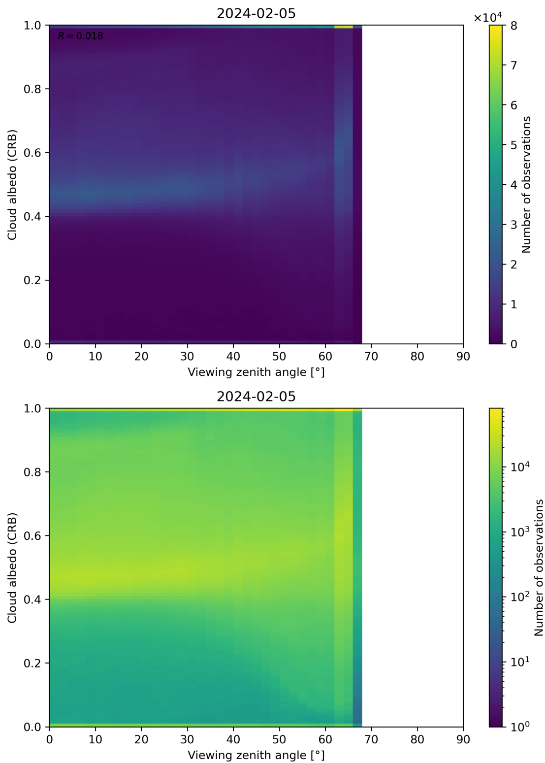
Figure 106: Scatter density plot of “Viewing zenith angle” against “Cloud albedo (CRB)” for 2024-02-04 to 2024-02-06.
