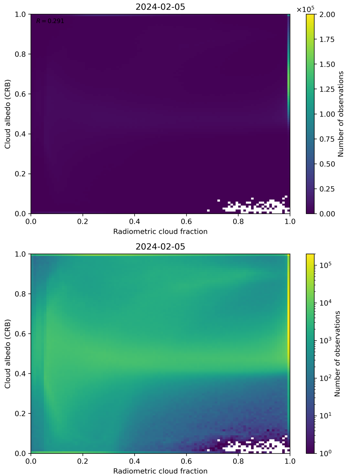
Figure 71: Scatter density plot of “Radiometric cloud fraction” against “Cloud albedo (CRB)” for 2024-02-04 to 2024-02-06.
