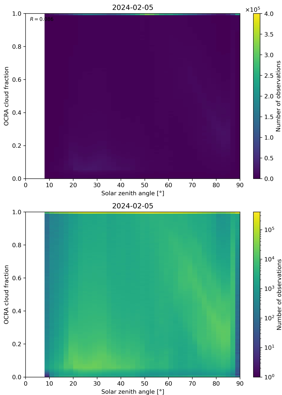
Figure 100: Scatter density plot of “Solar zenith angle” against “OCRA cloud fraction” for 2024-02-04 to 2024-02-06.
