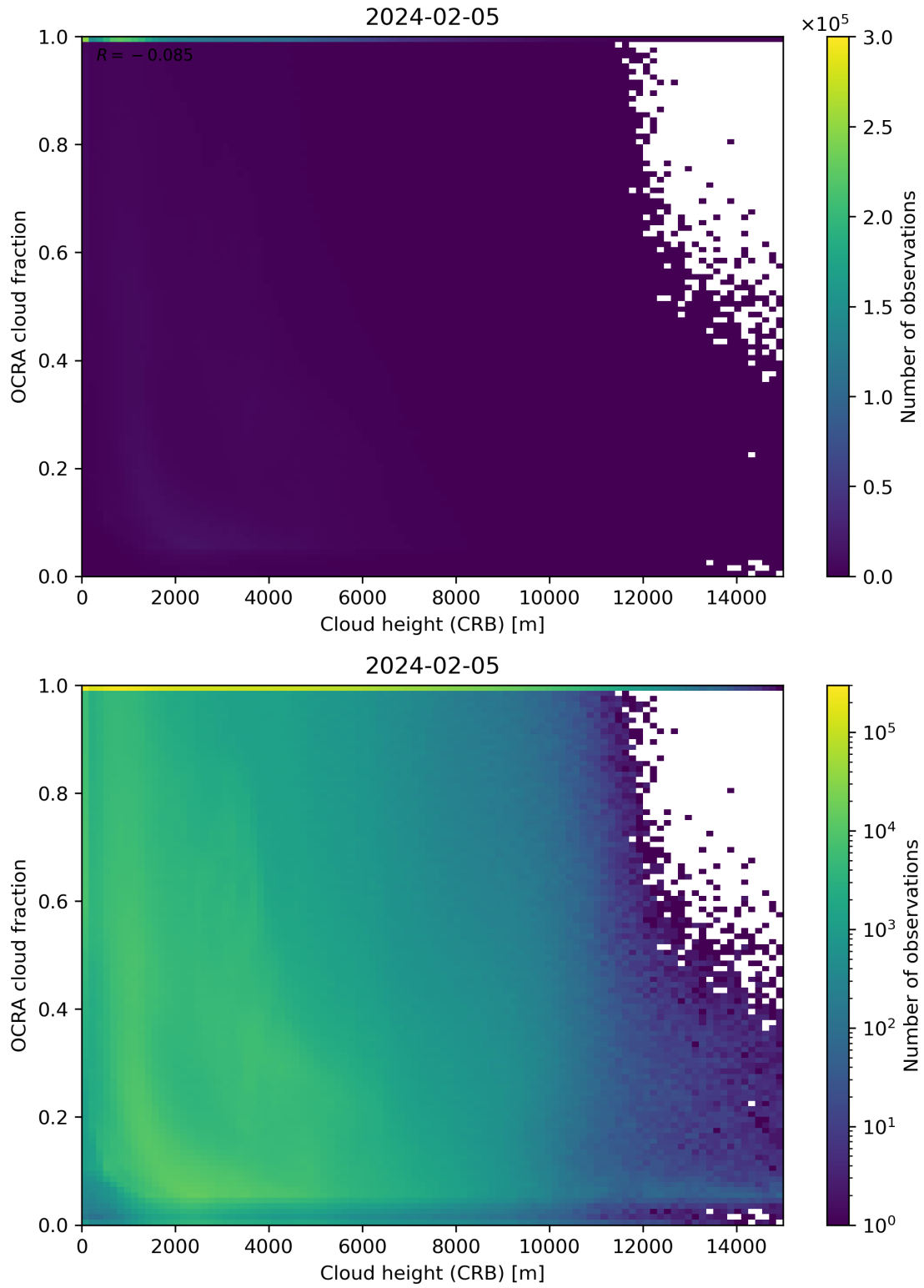
Figure 81: Scatter density plot of “Cloud height (CRB)” against “OCRA cloud fraction” for 2024-02-04 to 2024-02-06.
