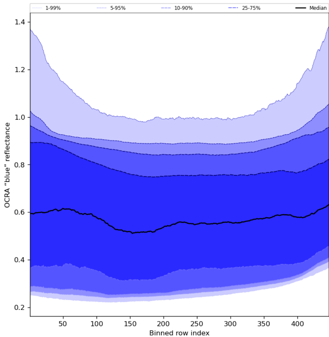
Figure 67: Along track statistics of "OCRA "blue" reflectance" for 2024-02-04 to 2024-02-06
