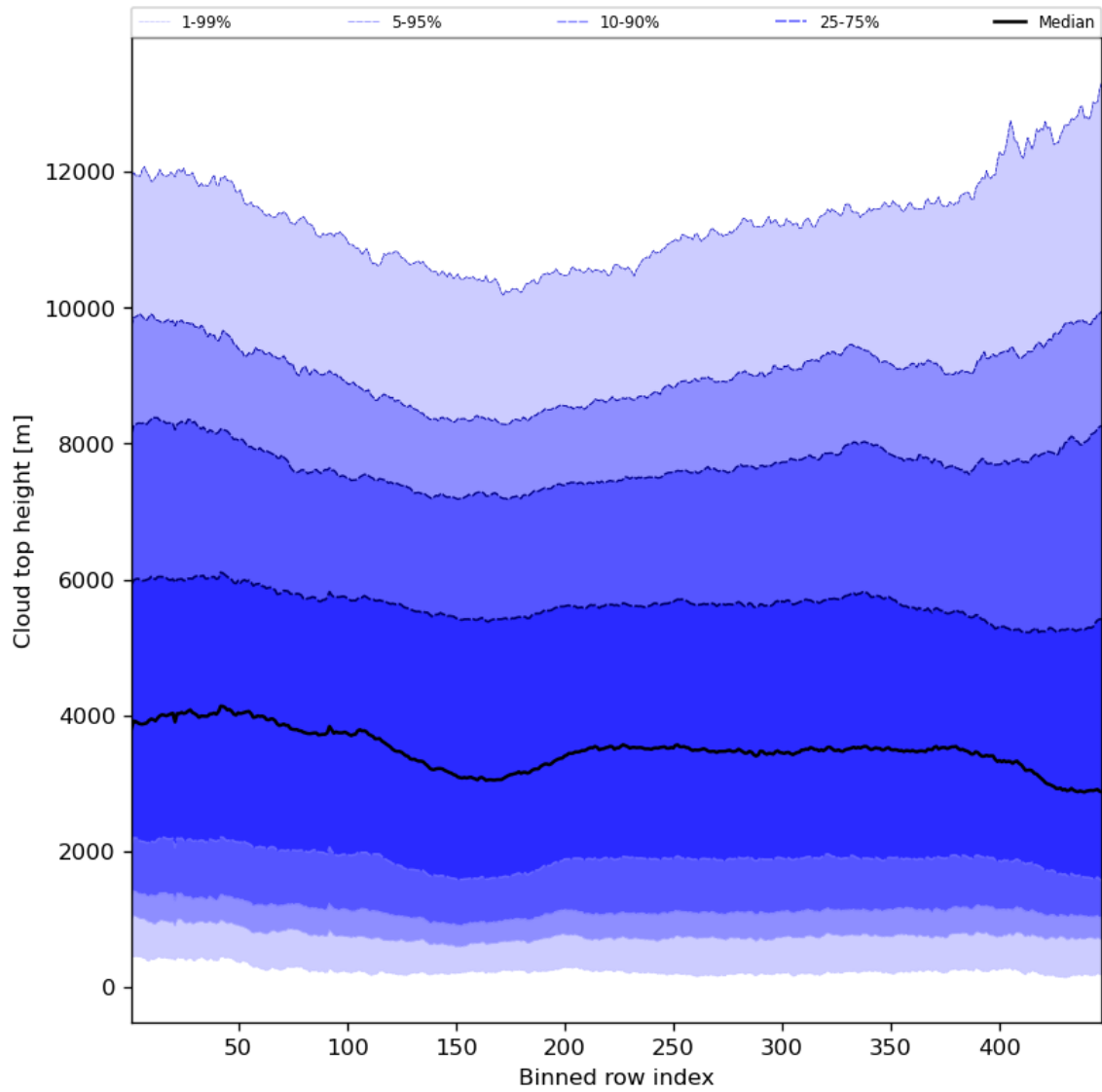
Figure 56: Along track statistics of “Cloud top height” for 2024-02-04 to 2024-02-06
