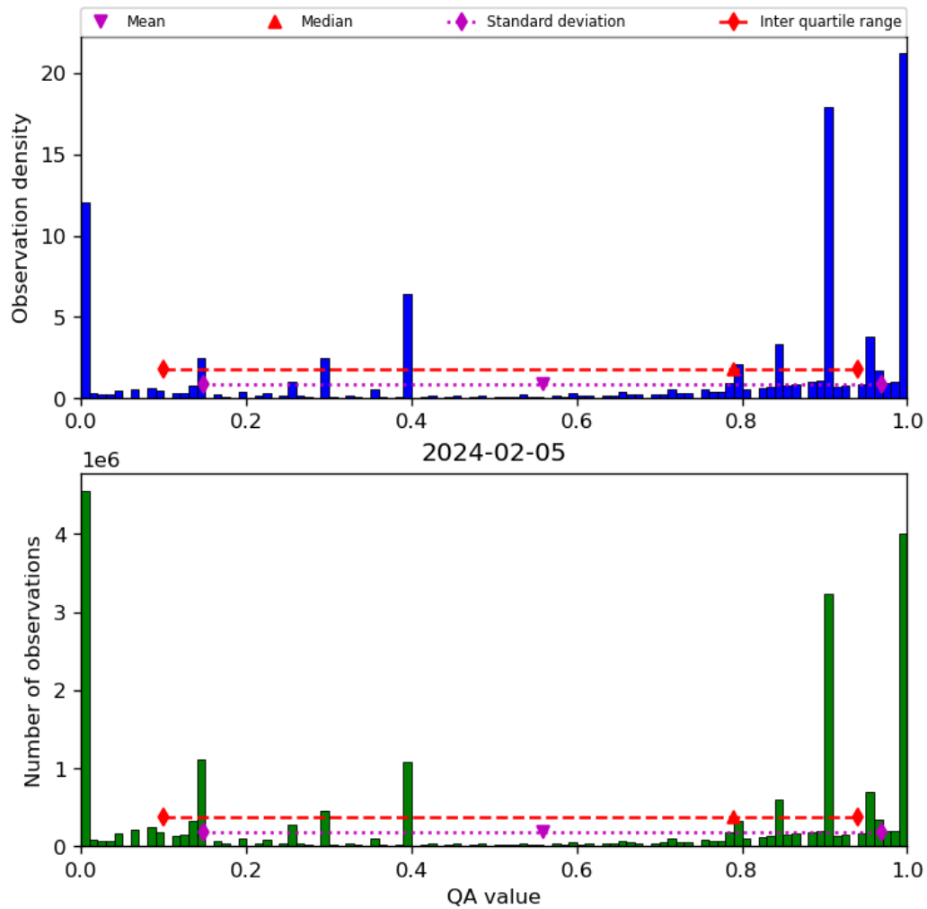
Figure 38: Histogram of “QA value” for 2024-02-04 to 2024-02-06
