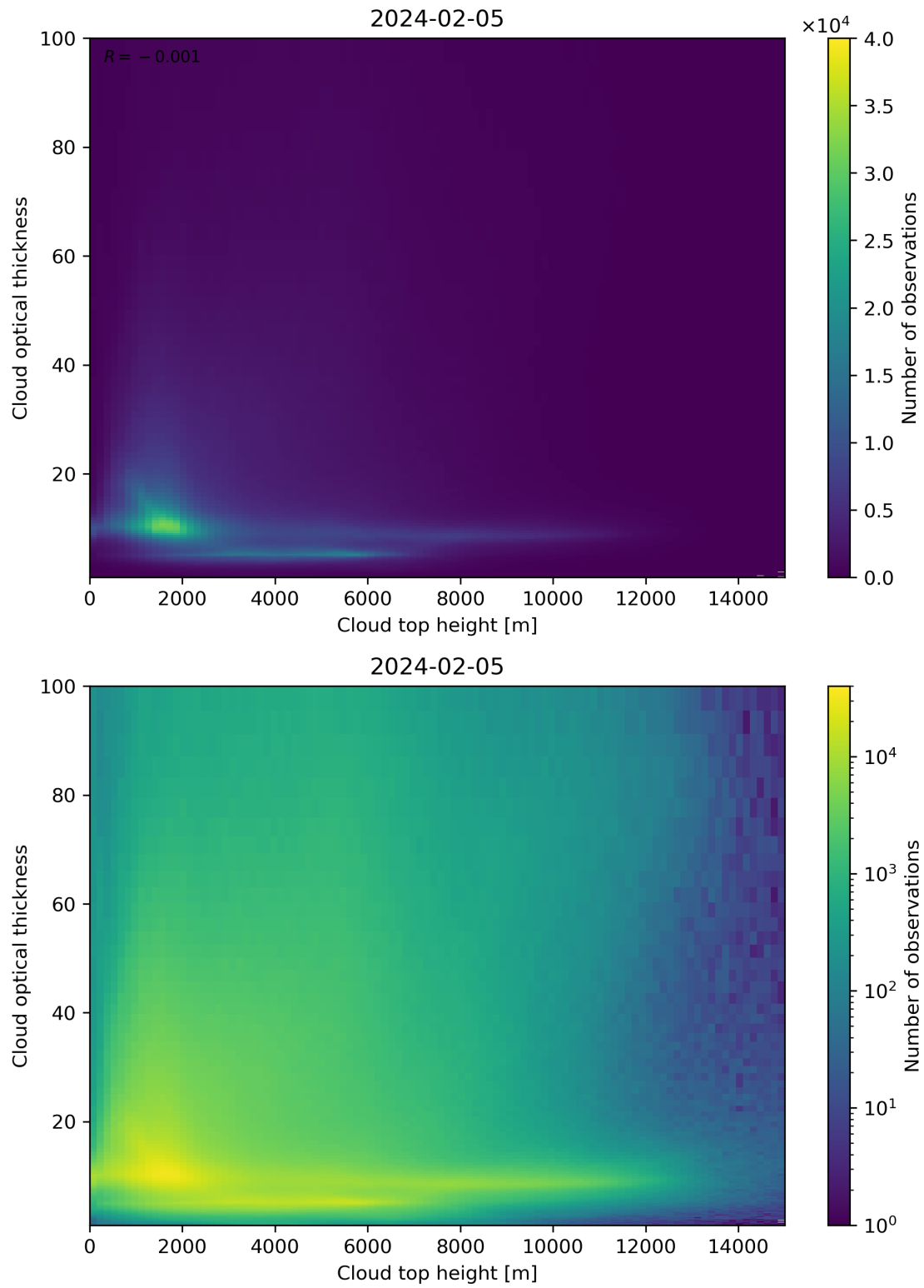
Figure 90: Scatter density plot of “Cloud top height” against “Cloud optical thickness” for 2024-02-04 to 2024-02-06.
