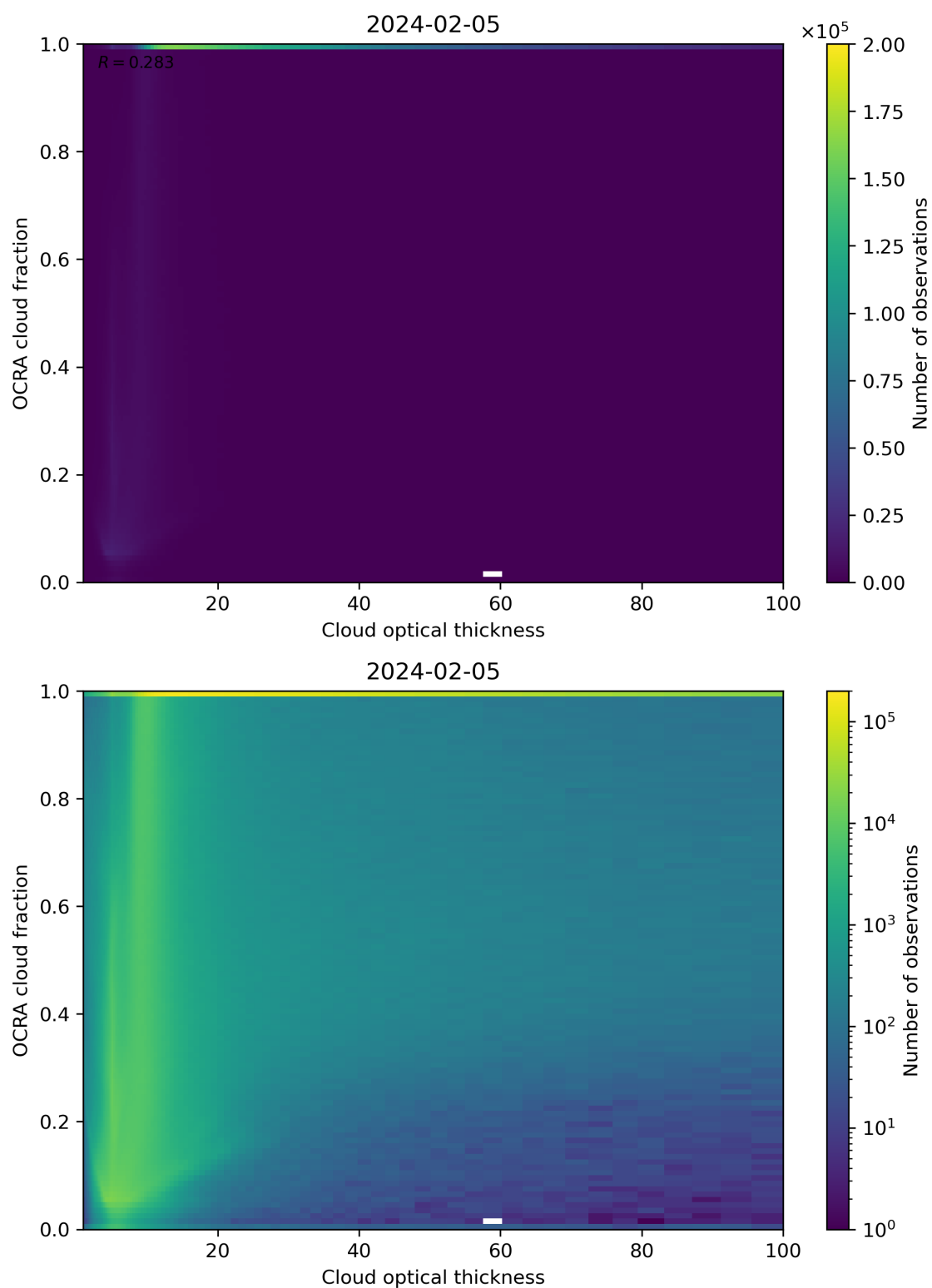
Figure 83: Scatter density plot of “Cloud optical thickness” against “OCRA cloud fraction” for 2024-02-04 to 2024-02-06.
