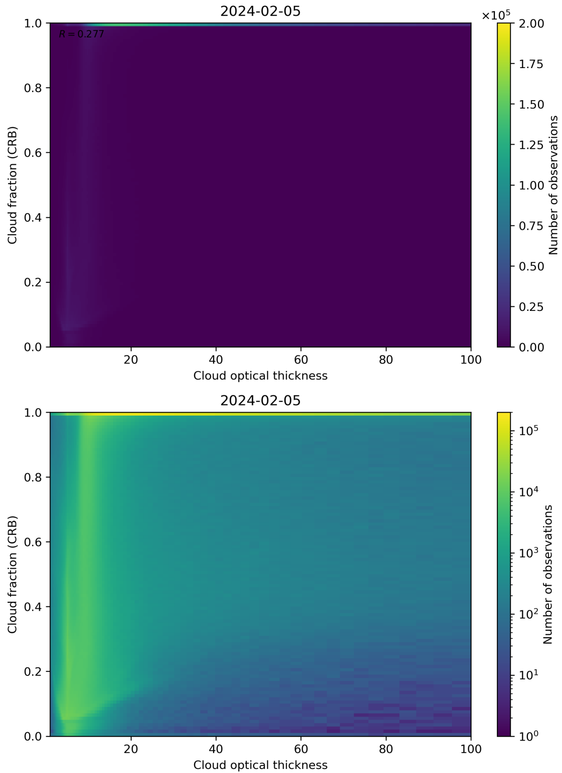
Figure 84: Scatter density plot of “Cloud optical thickness” against “Cloud fraction (CRB)” for 2024-02-04 to 2024-02-06.
