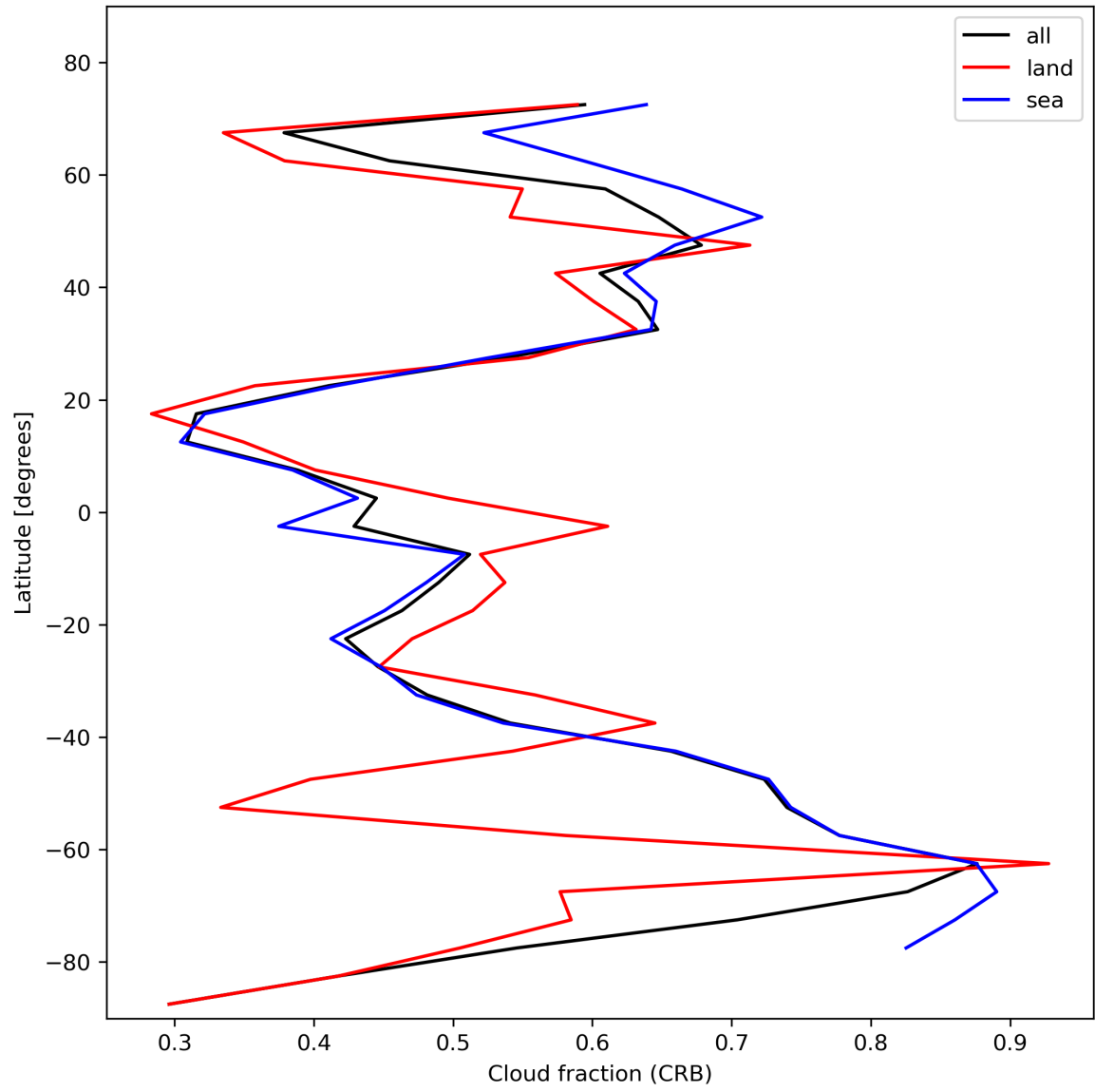
Figure 26: Zonal average of “Cloud fraction (CRB)” for 2024-02-04 to 2024-02-06.
