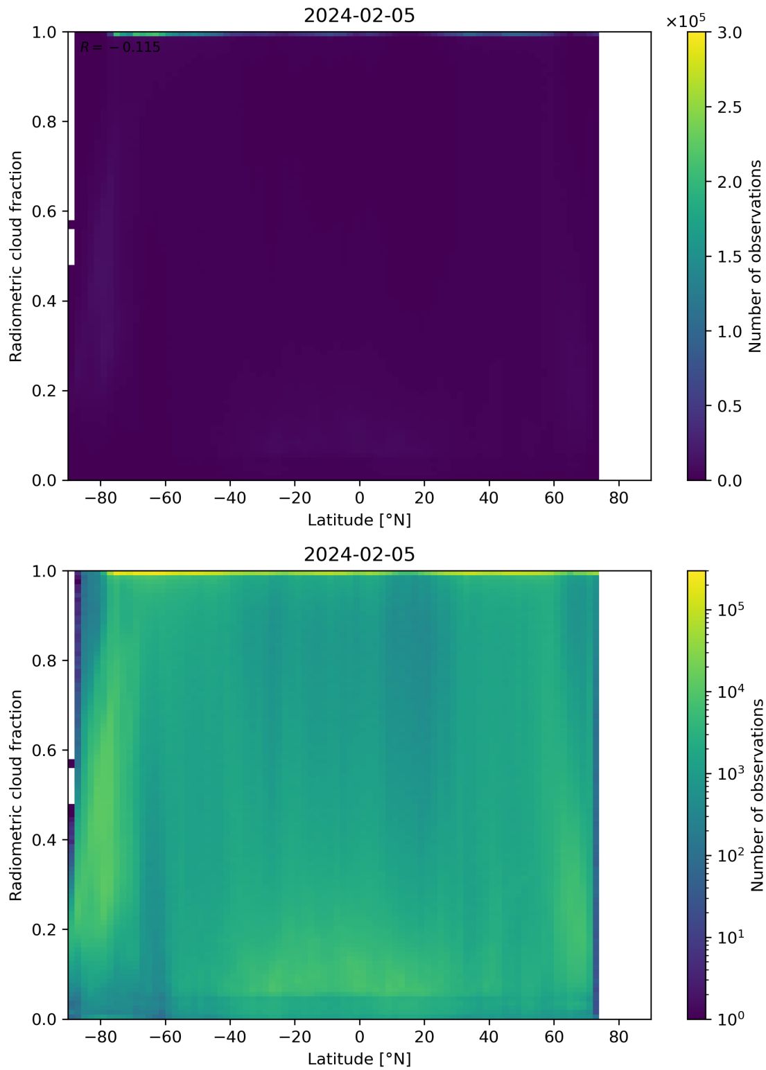
Figure 92: Scatter density plot of “Latitude” against “Radiometric cloud fraction” for 2024-02-04 to 2024-02-06.
