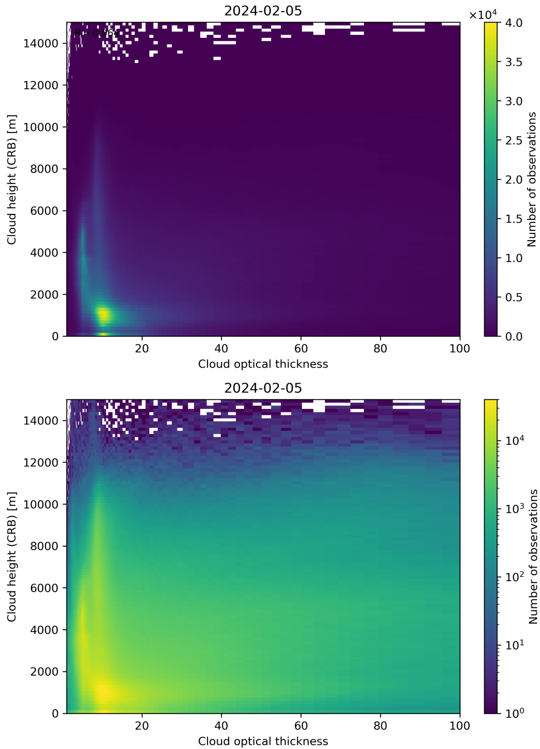
Figure 85: Scatter density plot of “Cloud optical thickness” against “Cloud height (CRB)” for 2024-02-04 to 2024-02-06.
