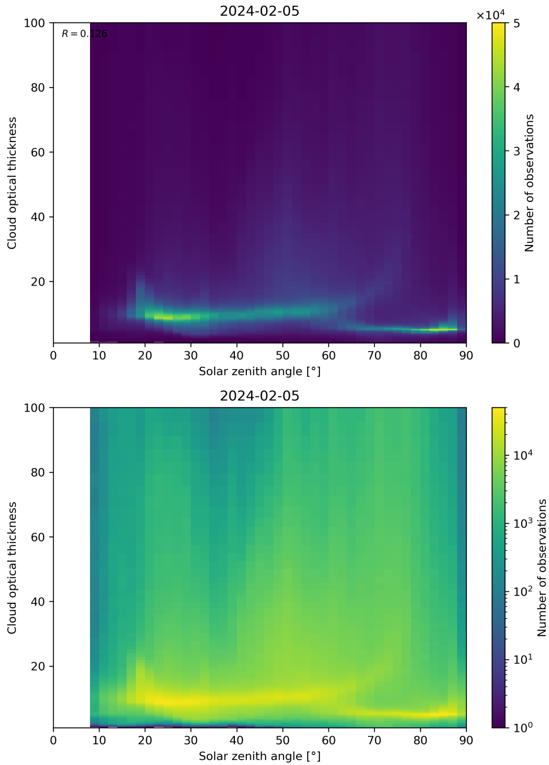
Figure 103: Scatter density plot of “Solar zenith angle” against “Cloud optical thickness” for 2024-02-04 to 2024-02-06.
