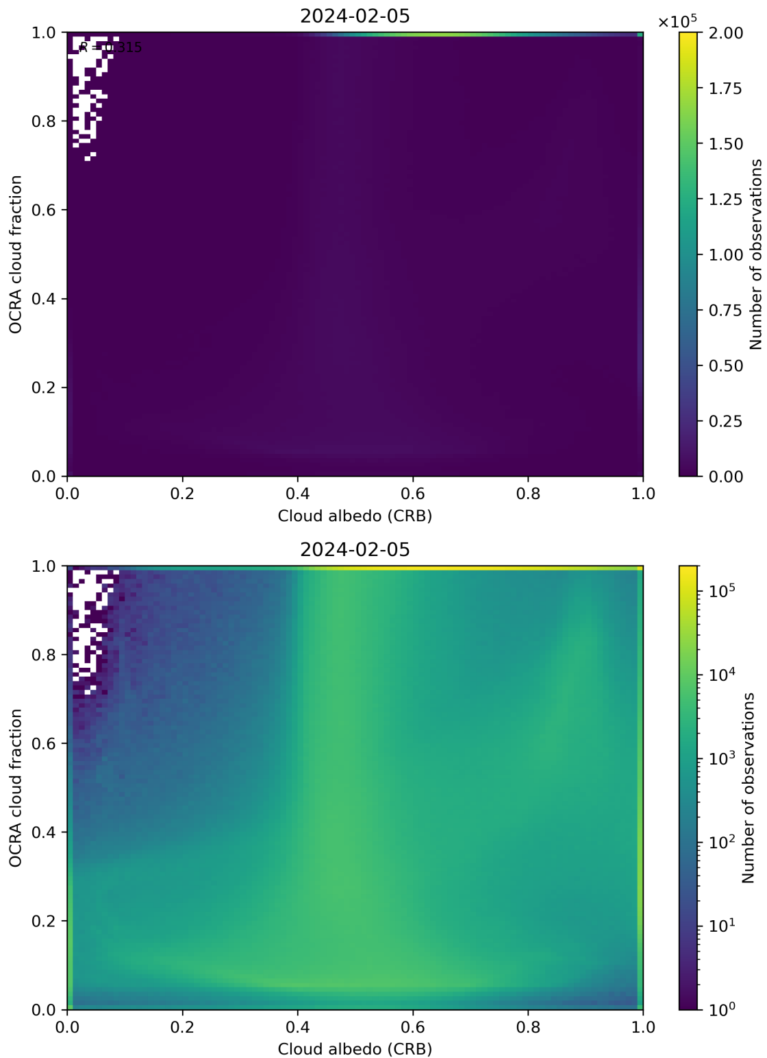
Figure 70: Scatter density plot of “Cloud albedo (CRB)” against “OCRA cloud fraction” for 2024-02-04 to 2024-02-06.
