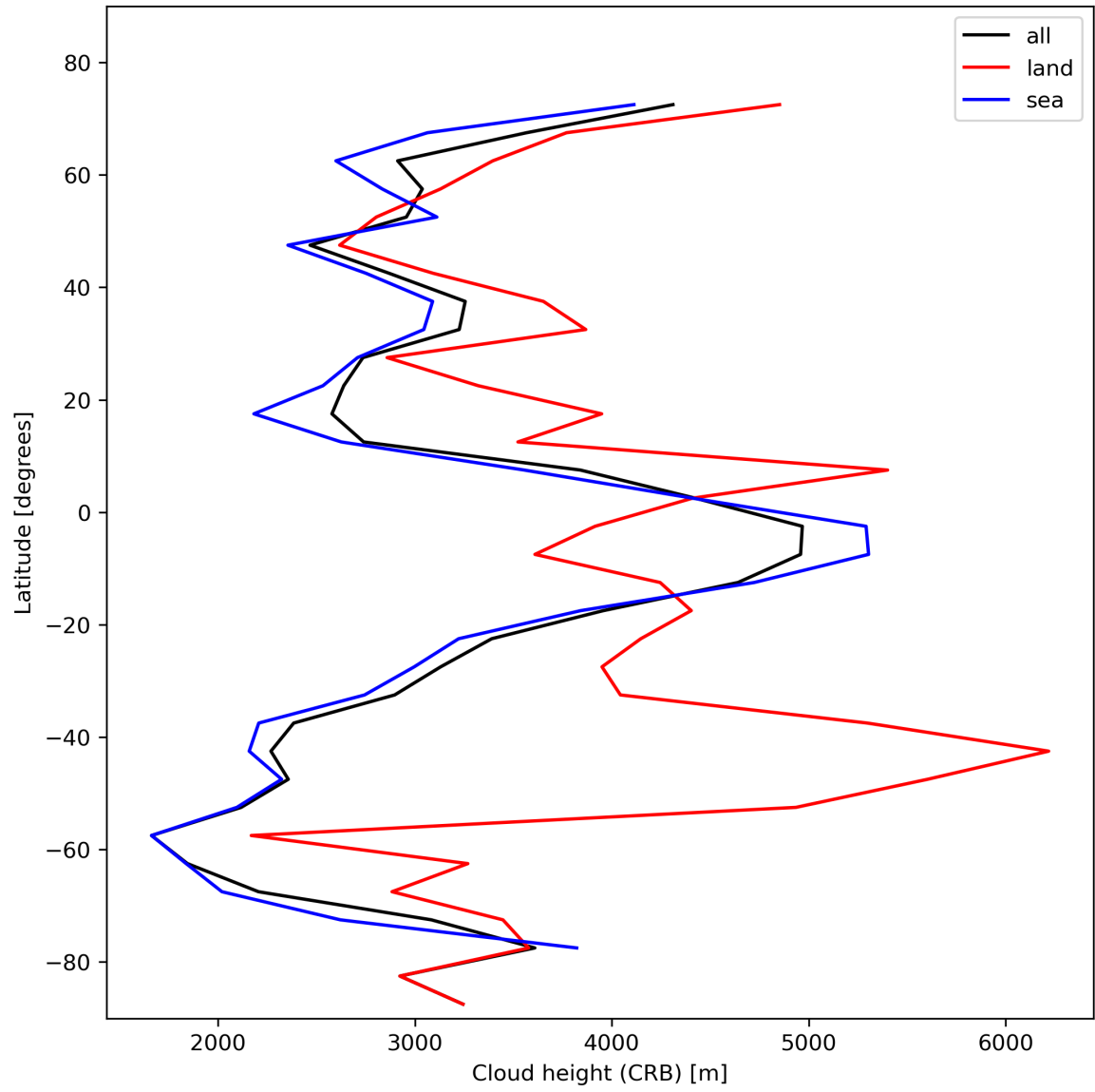
Figure 27: Zonal average of “Cloud height (CRB)” for 2024-02-04 to 2024-02-06.
