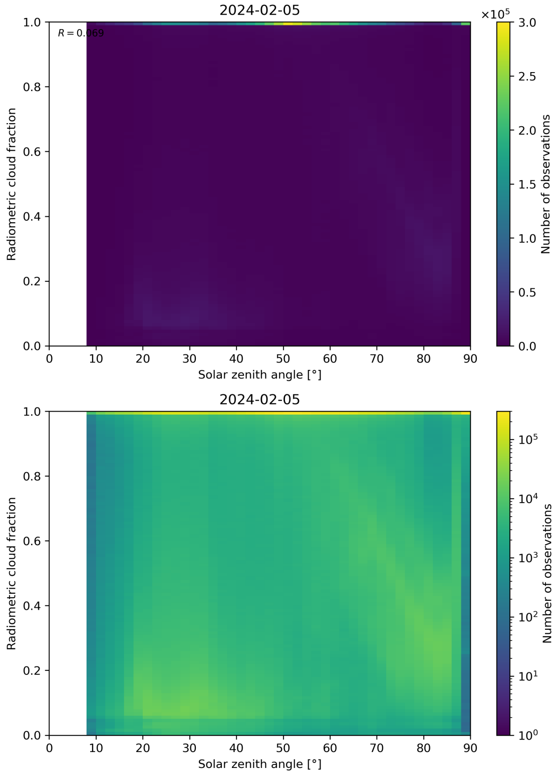
Figure 99: Scatter density plot of “Solar zenith angle” against “Radiometric cloud fraction” for 2024-02-04 to 2024-02-06.
