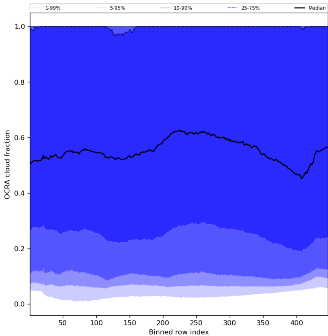
Figure 66: Along track statistics of “OCRA cloud fraction” for 2024-02-04 to 2024-02-06
