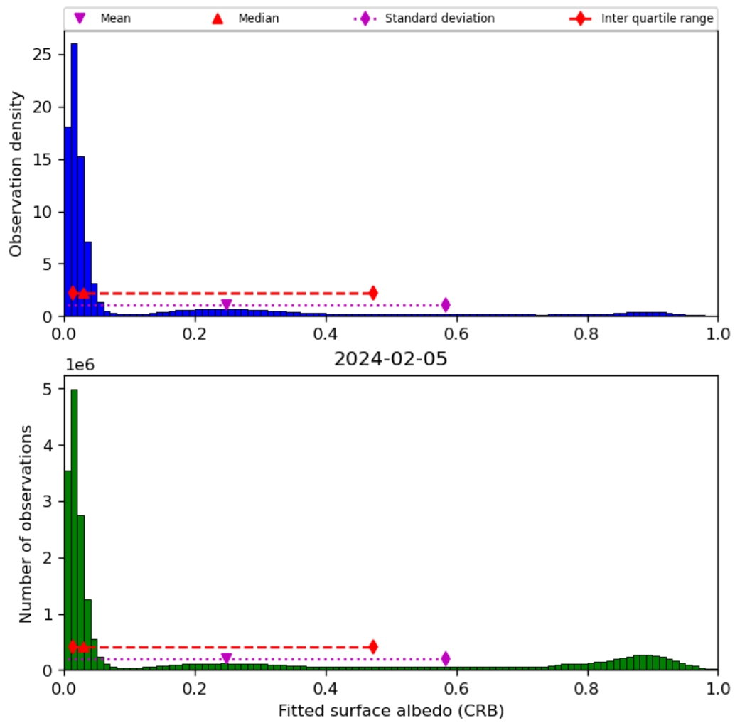
Figure 46: Histogram of “Fitted surface albedo (CRB)” for 2024-02-04 to 2024-02-06
