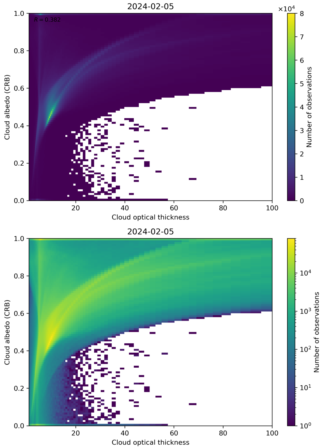
Figure 82: Scatter density plot of “Cloud optical thickness” against “Cloud albedo (CRB)” for 2024-02-04 to 2024-02-06.
