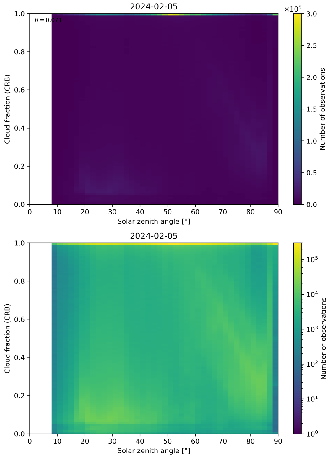
Figure 101: Scatter density plot of “Solar zenith angle” against “Cloud fraction (CRB)” for 2024-02-04 to 2024-02-06.
