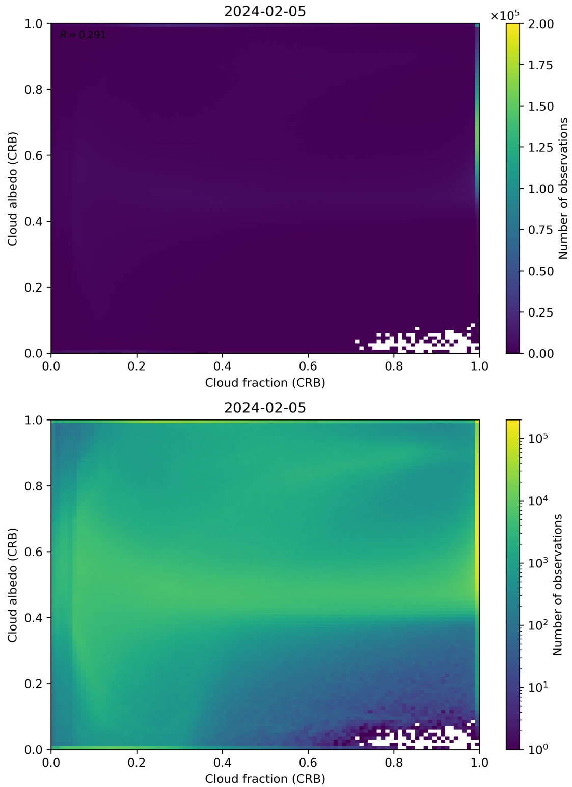
Figure 77: Scatter density plot of “Cloud fraction (CRB)” against “Cloud albedo (CRB)” for 2024-02-04 to 2024-02-06.
