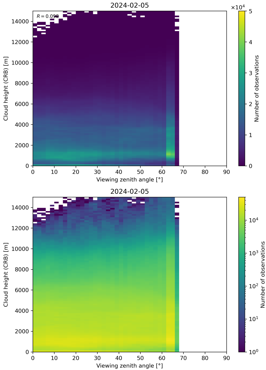
Figure 110: Scatter density plot of “Viewing zenith angle” against “Cloud height (CRB)” for 2024-02-04 to 2024-02-06.
