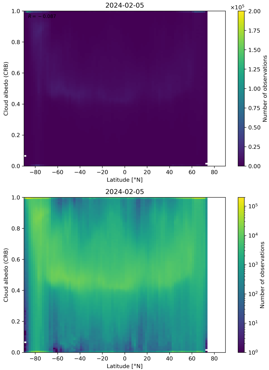
Figure 91: Scatter density plot of “Latitude” against “Cloud albedo (CRB)” for 2024-02-04 to 2024-02-06.
