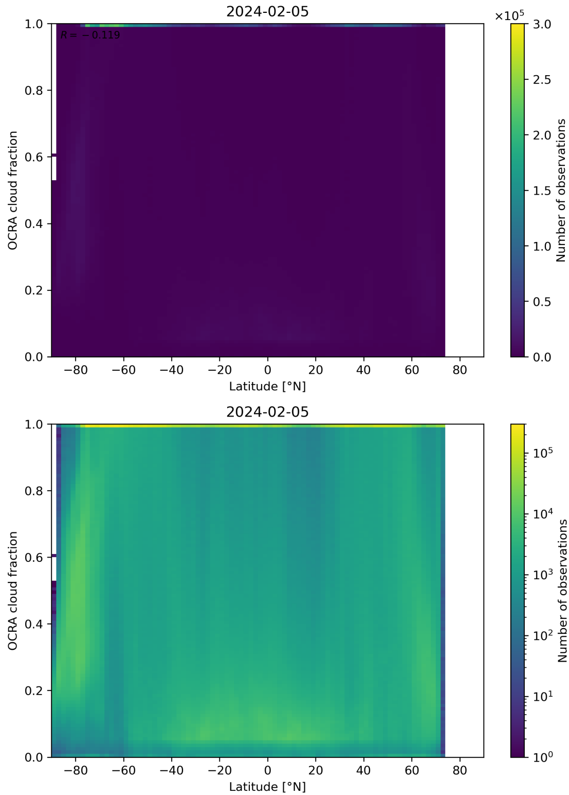
Figure 93: Scatter density plot of “Latitude” against “OCRA cloud fraction” for 2024-02-04 to 2024-02-06.
