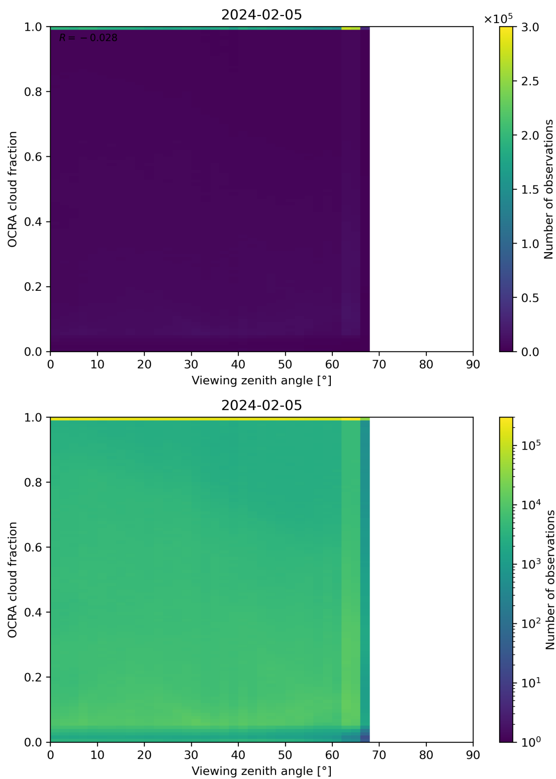
Figure 108: Scatter density plot of “Viewing zenith angle” against “OCRA cloud fraction” for 2024-02-04 to 2024-02-06.
