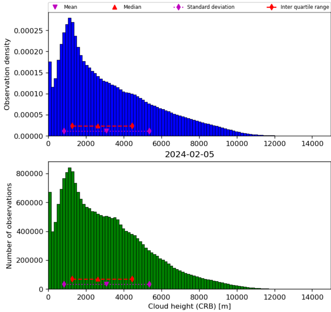
Figure 43: Histogram of “Cloud height (CRB)” for 2024-02-04 to 2024-02-06
