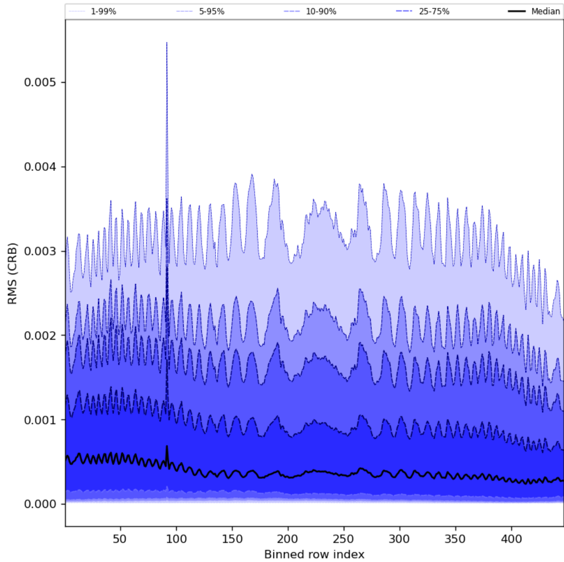
Figure 64: Along track statistics of "RMS (CRB)" for 2024-02-04 to 2024-02-06
