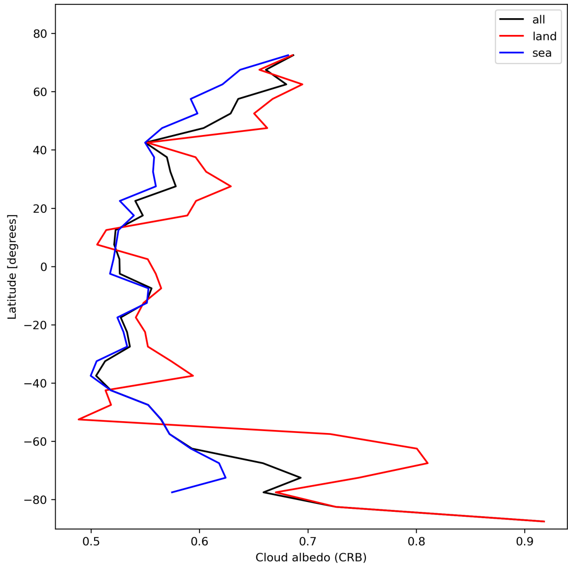
Figure 28: Zonal average of “Cloud albedo (CRB)” for 2024-02-04 to 2024-02-06.
