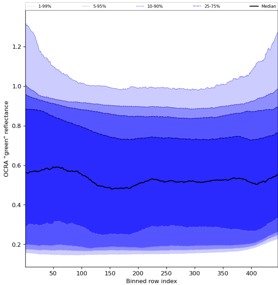
Figure 68: Along track statistics of “OCRA “green” reflectance” for 2024-02-04 to 2024-02-06
