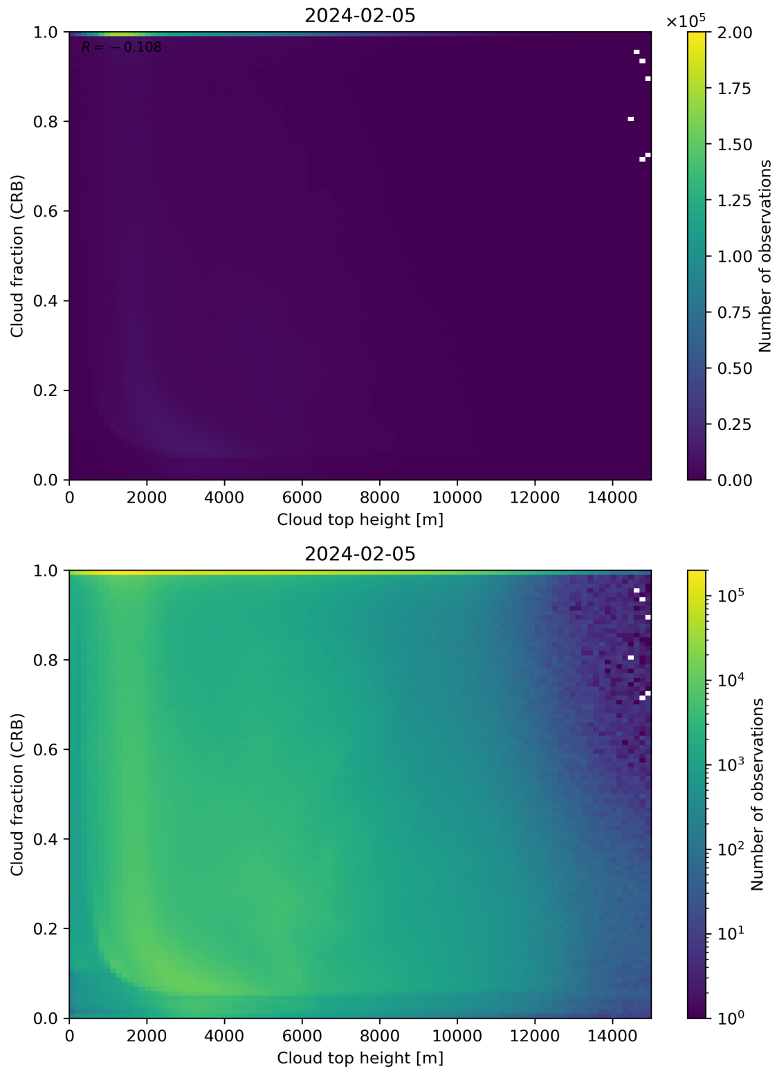
Figure 88: Scatter density plot of “Cloud top height” against “Cloud fraction (CRB)” for 2024-02-04 to 2024-02-06.
