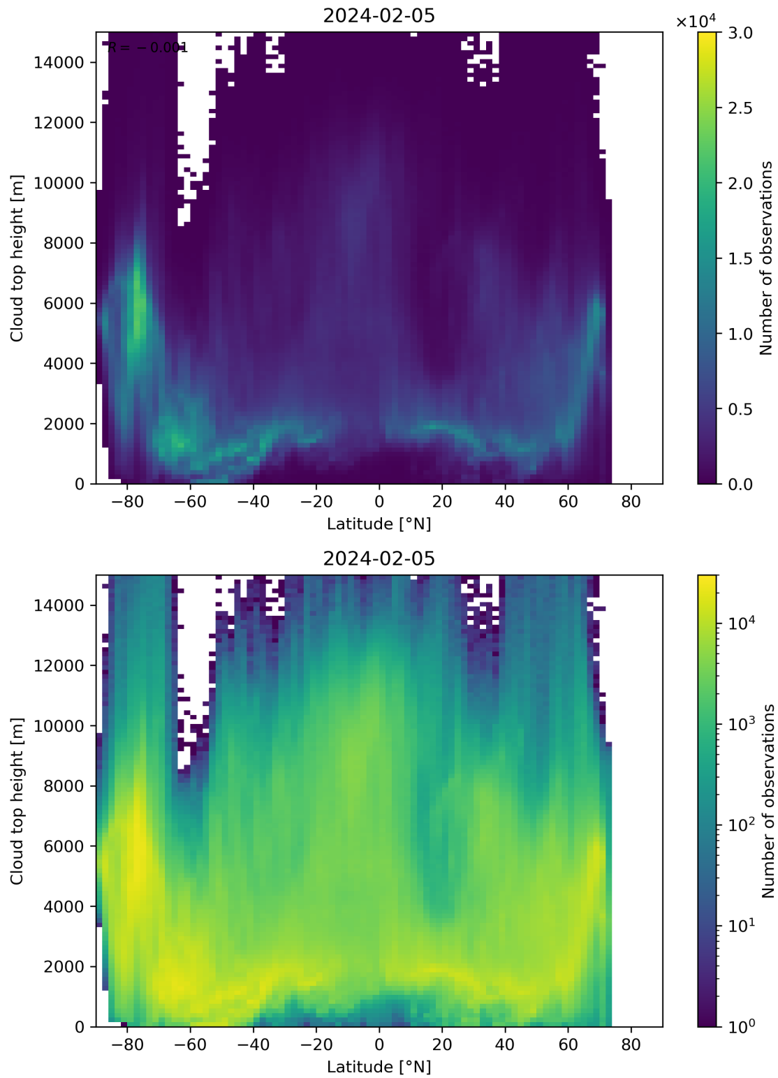
Figure 97: Scatter density plot of “Latitude” against “Cloud top height” for 2024-02-04 to 2024-02-06.
