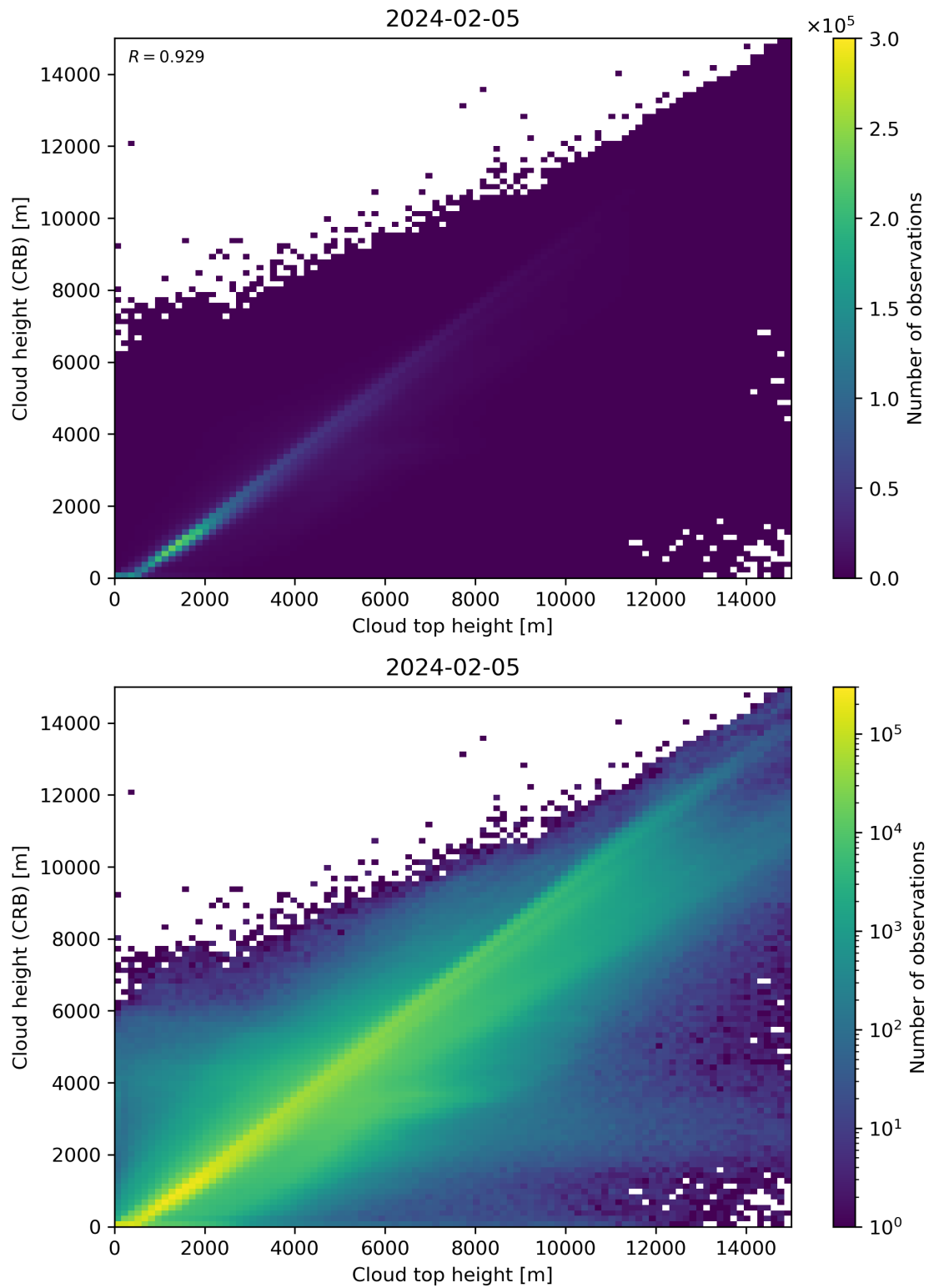
Figure 89: Scatter density plot of “Cloud top height” against “Cloud height (CRB)” for 2024-02-04 to 2024-02-06.
