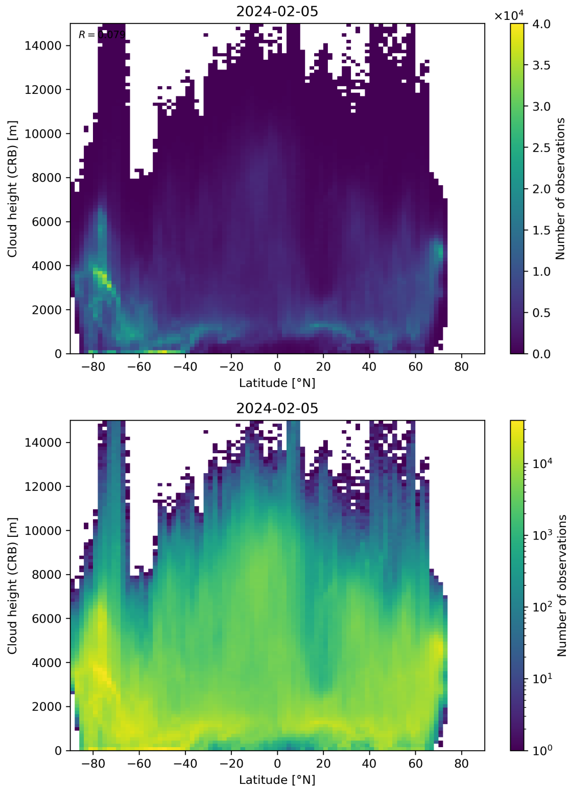
Figure 95: Scatter density plot of “Latitude” against “Cloud height (CRB)” for 2024-02-04 to 2024-02-06.
