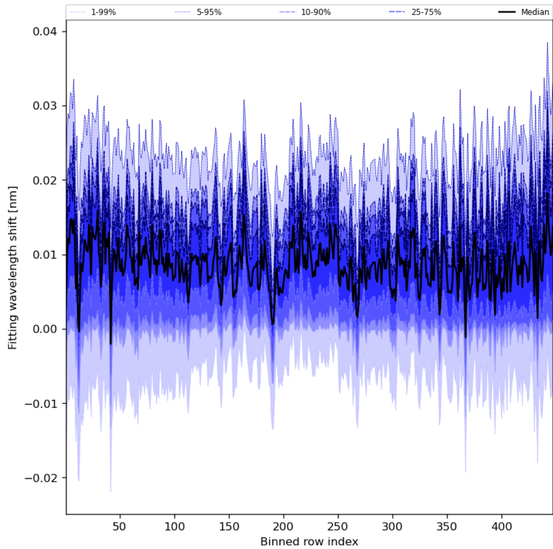
Figure 65: Along track statistics of “Fitting wavelength shift” for 2024-02-04 to 2024-02-06
