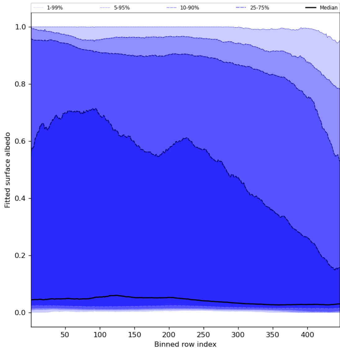
Figure 61: Along track statistics of “Fitted surface albedo” for 2024-02-04 to 2024-02-06
