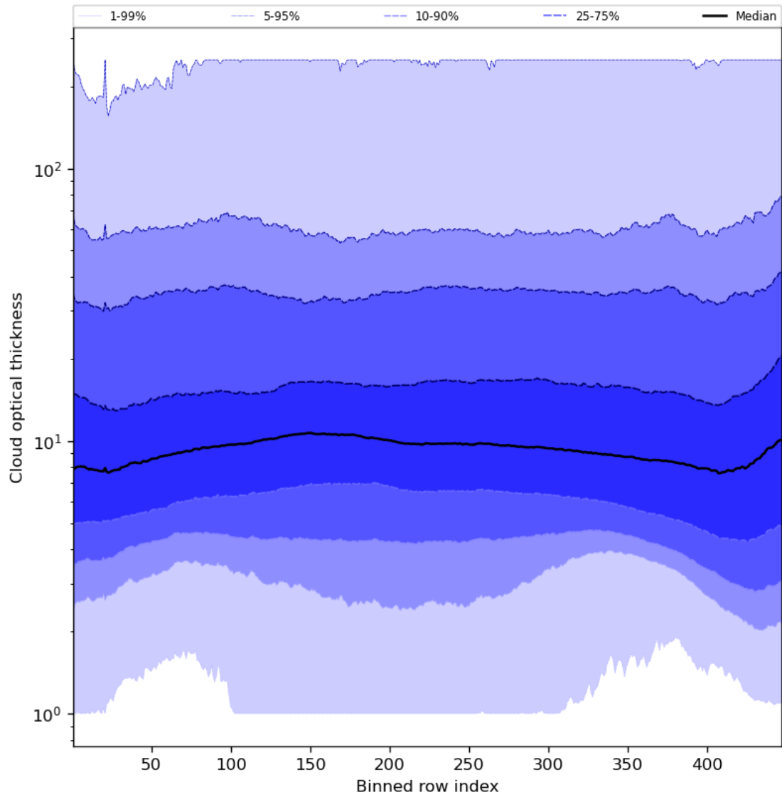
Figure 57: Along track statistics of “Cloud optical thickness” for 2024-02-04 to 2024-02-06
