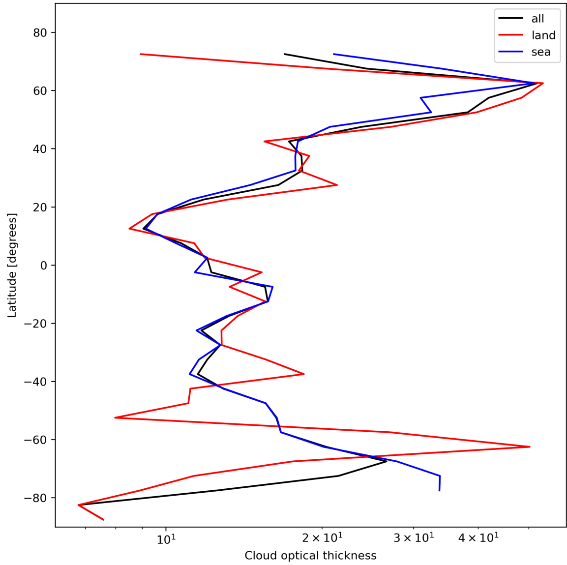
Figure 25: Zonal average of “Cloud optical thickness” for 2024-02-04 to 2024-02-06.
