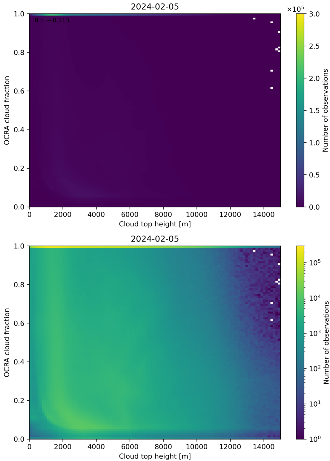
Figure 87: Scatter density plot of “Cloud top height” against “OCRA cloud fraction” for 2024-02-04 to 2024-02-06.
