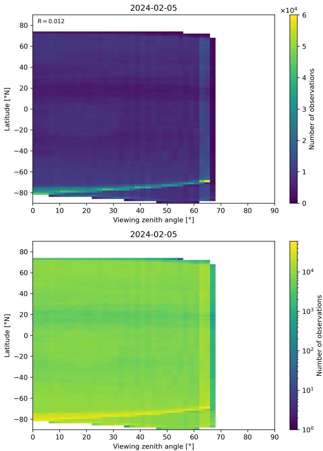
Figure 113: Scatter density plot of “Viewing zenith angle” against “Latitude” for 2024-02-04 to 2024-02-06.
