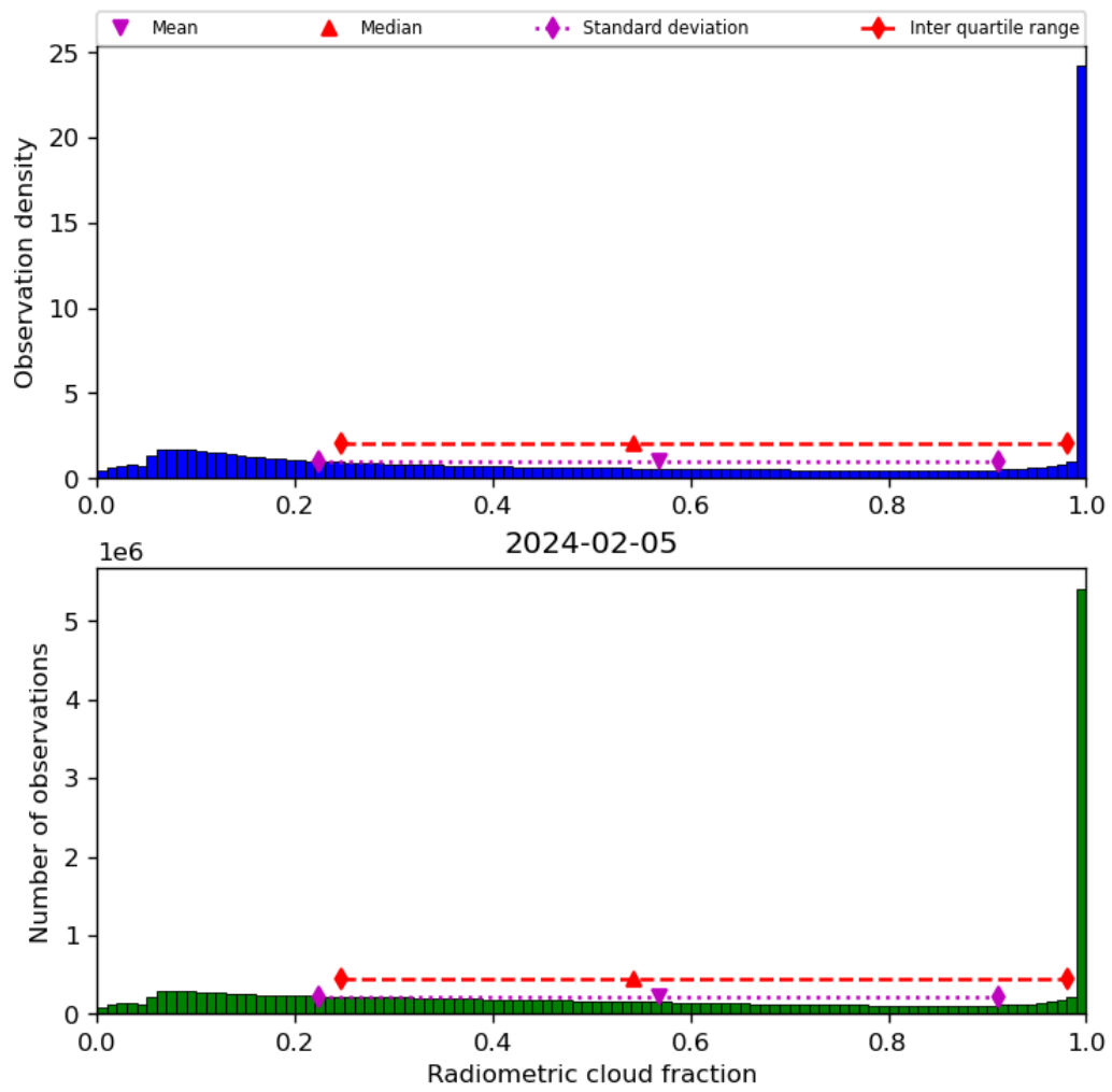
Figure 39: Histogram of “Radiometric cloud fraction” for 2024-02-04 to 2024-02-06
