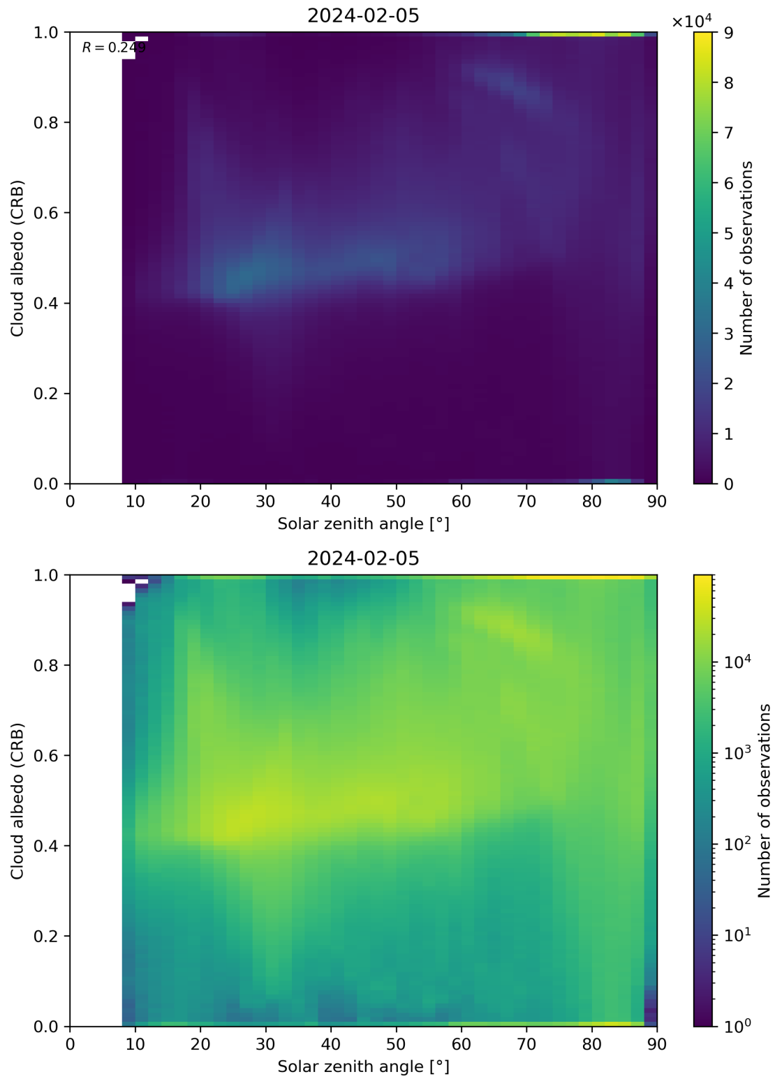
Figure 98: Scatter density plot of “Solar zenith angle” against “Cloud albedo (CRB)” for 2024-02-04 to 2024-02-06.
