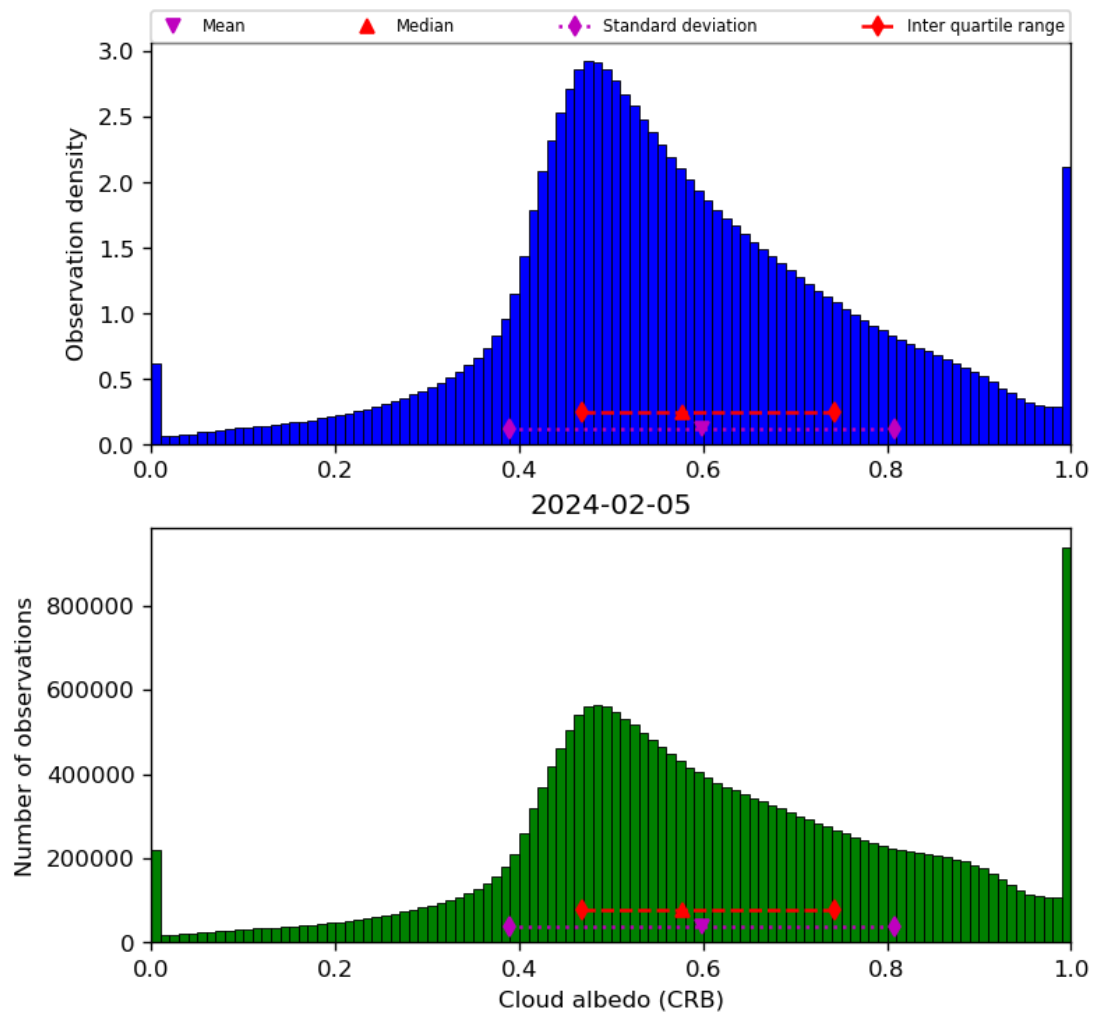
Figure 44: Histogram of “Cloud albedo (CRB)” for 2024-02-04 to 2024-02-06
