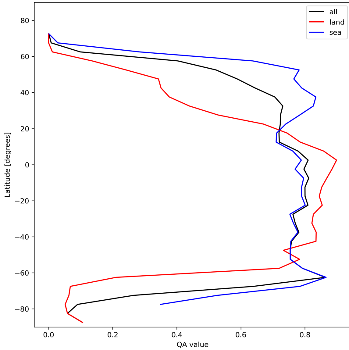
Figure 22: Zonal average of “QA value” for 2024-02-04 to 2024-02-06.
