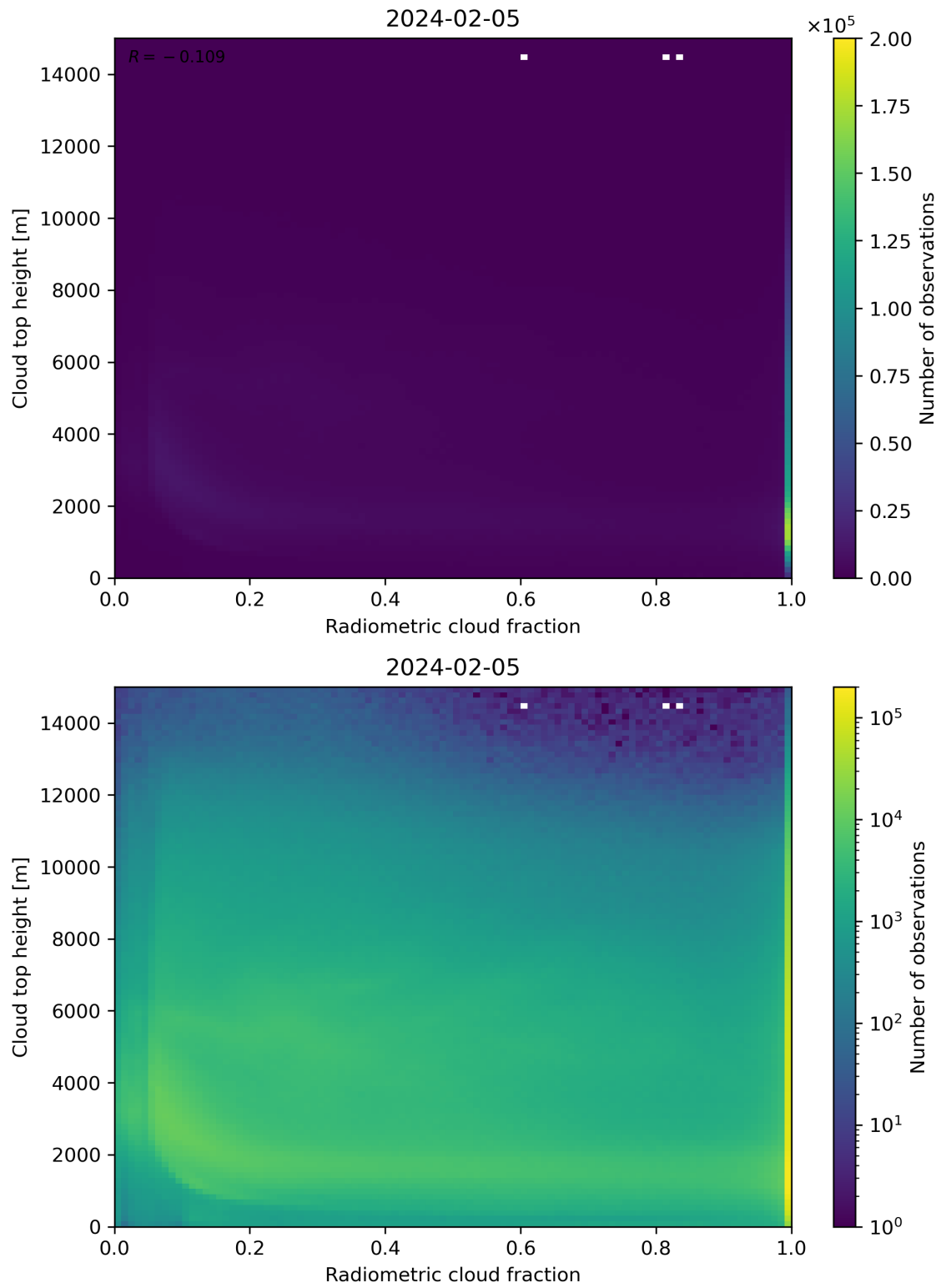
Figure 76: Scatter density plot of “Radiometric cloud fraction” against “Cloud top height” for 2024-02-04 to 2024-02-06.
