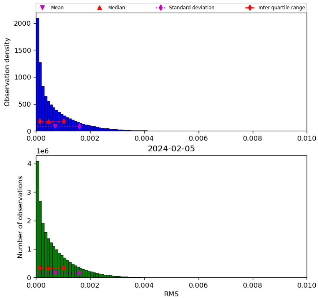
Figure 47: Histogram of “RMS” for 2024-02-04 to 2024-02-06
