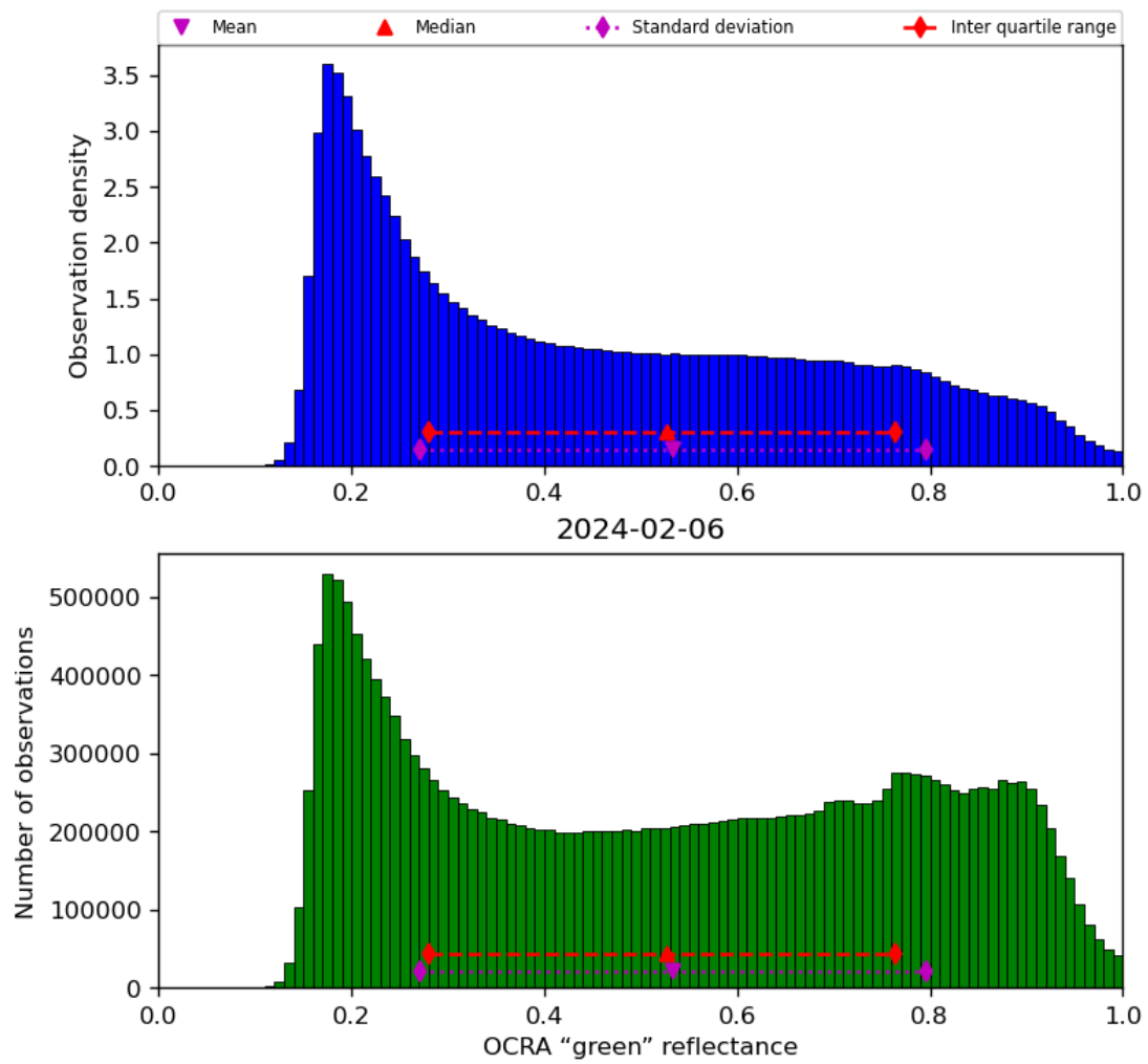
Figure 52: Histogram of “OCRA “green” reflectance” for 2024-02-06 to 2024-02-07
