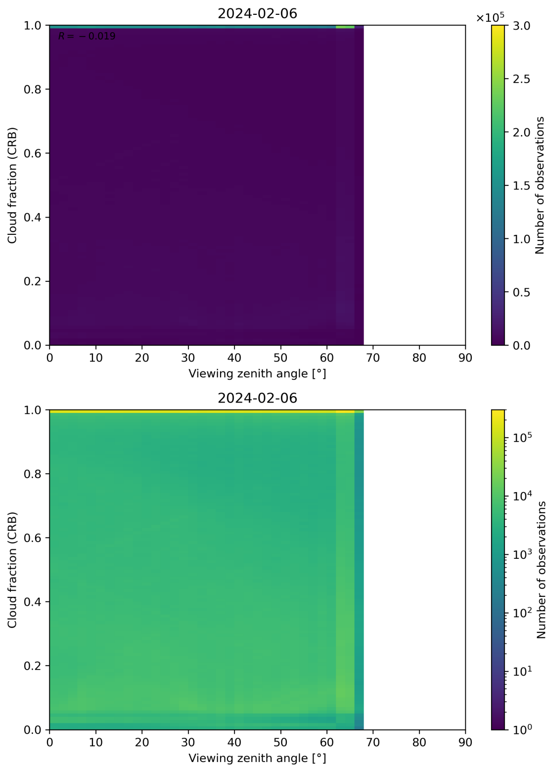
Figure 109: Scatter density plot of “Viewing zenith angle” against “Cloud fraction (CRB)” for 2024-02-06 to 2024-02-07.
