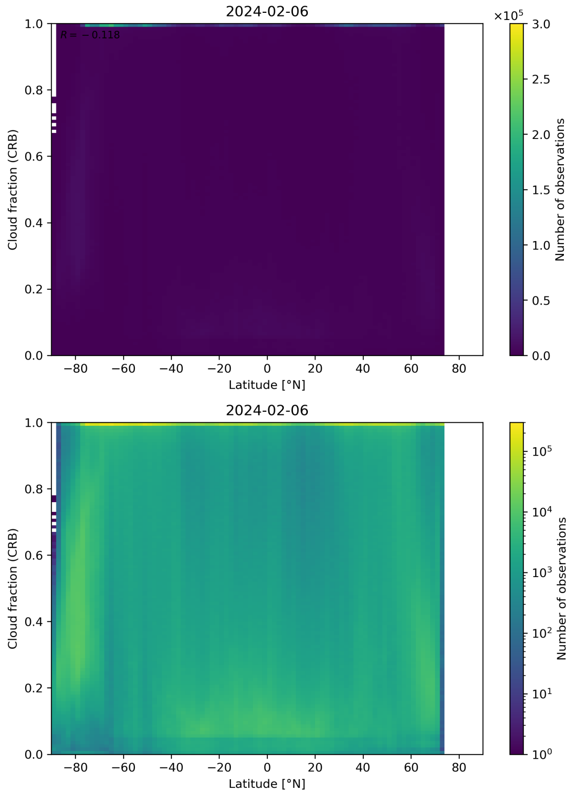
Figure 94: Scatter density plot of “Latitude” against “Cloud fraction (CRB)” for 2024-02-06 to 2024-02-07.
