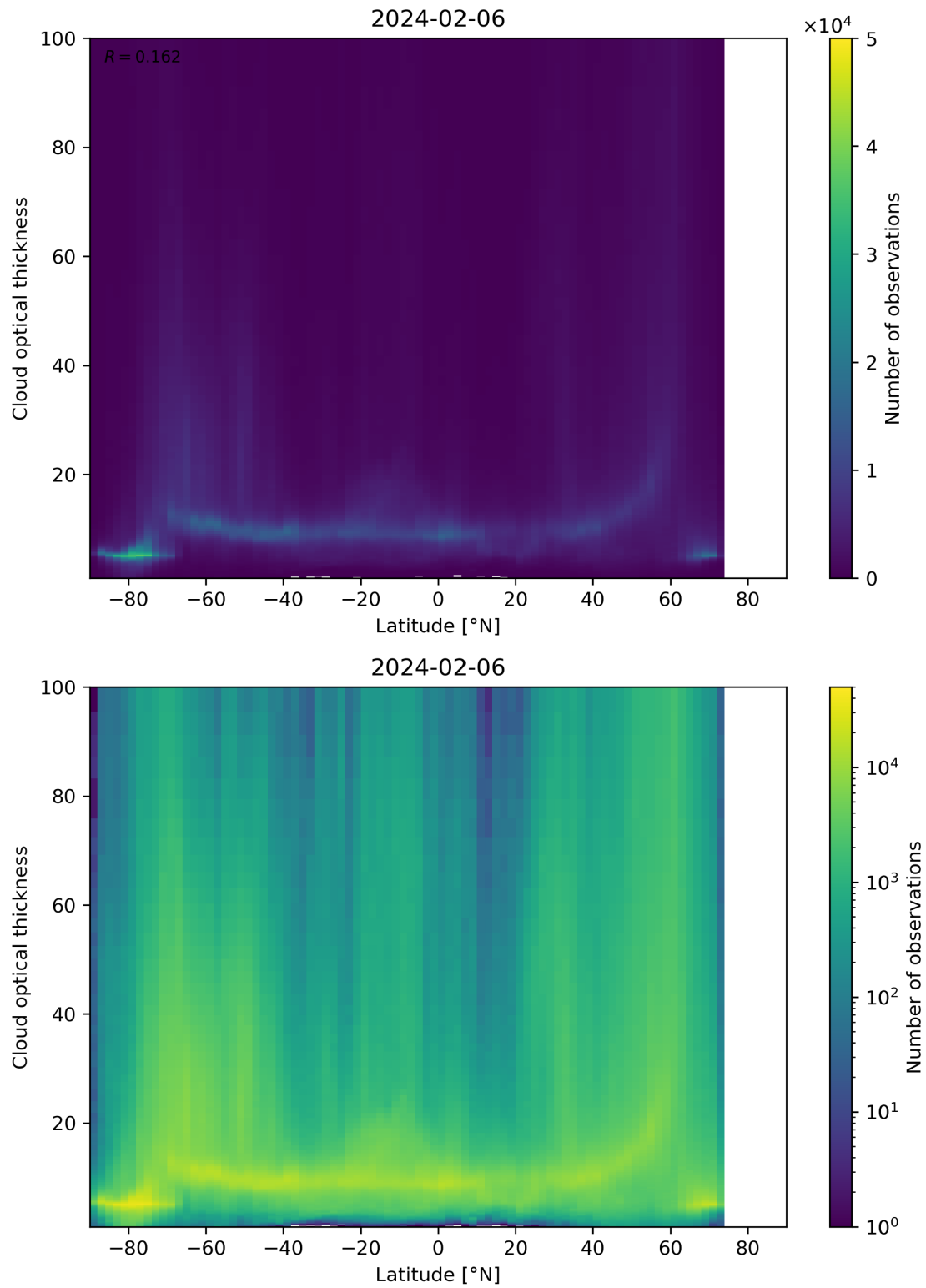
Figure 96: Scatter density plot of “Latitude” against “Cloud optical thickness” for 2024-02-06 to 2024-02-07.
