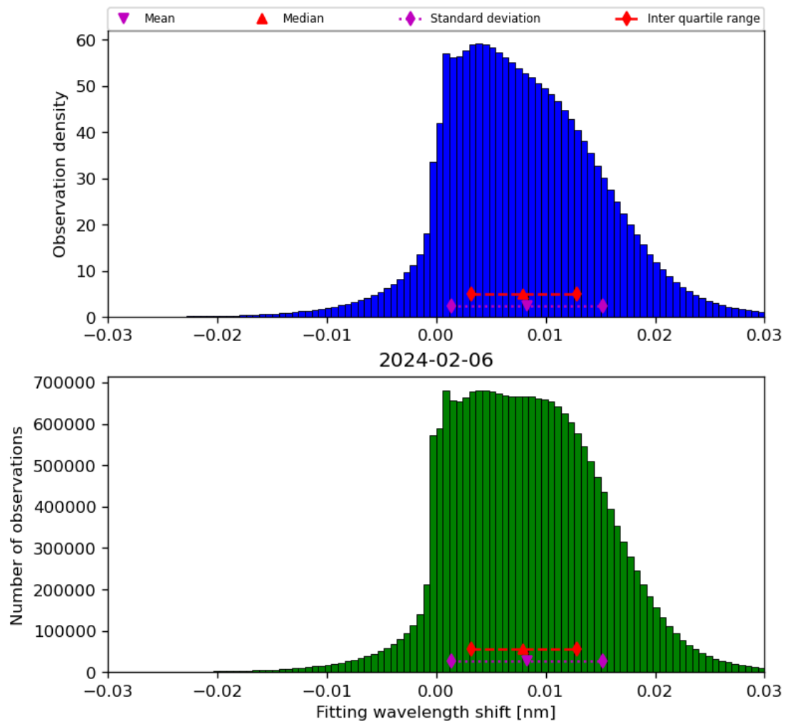
Figure 49: Histogram of “Fitting wavelength shift” for 2024-02-06 to 2024-02-07
