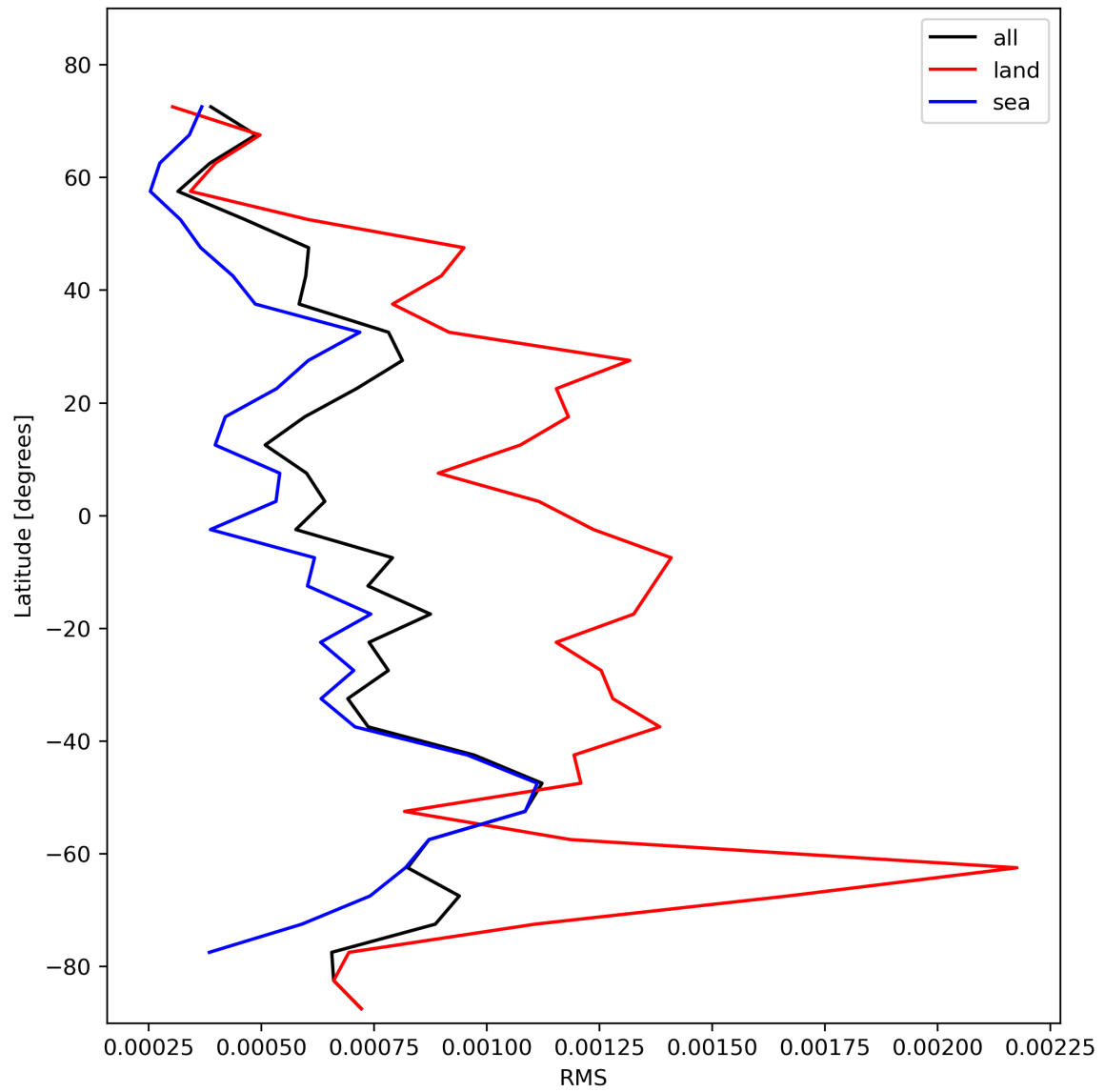
Figure 31: Zonal average of “RMS” for 2024-02-06 to 2024-02-07.
