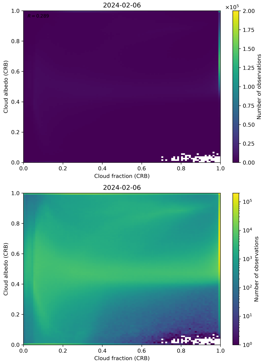
Figure 77: Scatter density plot of “Cloud fraction (CRB)” against “Cloud albedo (CRB)” for 2024-02-06 to 2024-02-07.
