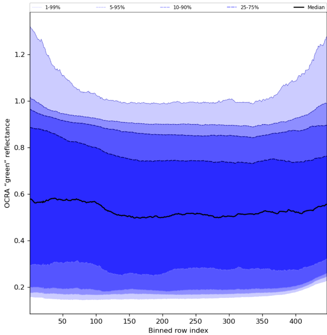
Figure 68: Along track statistics of "OCRA "green" reflectance" for 2024-02-06 to 2024-02-07
