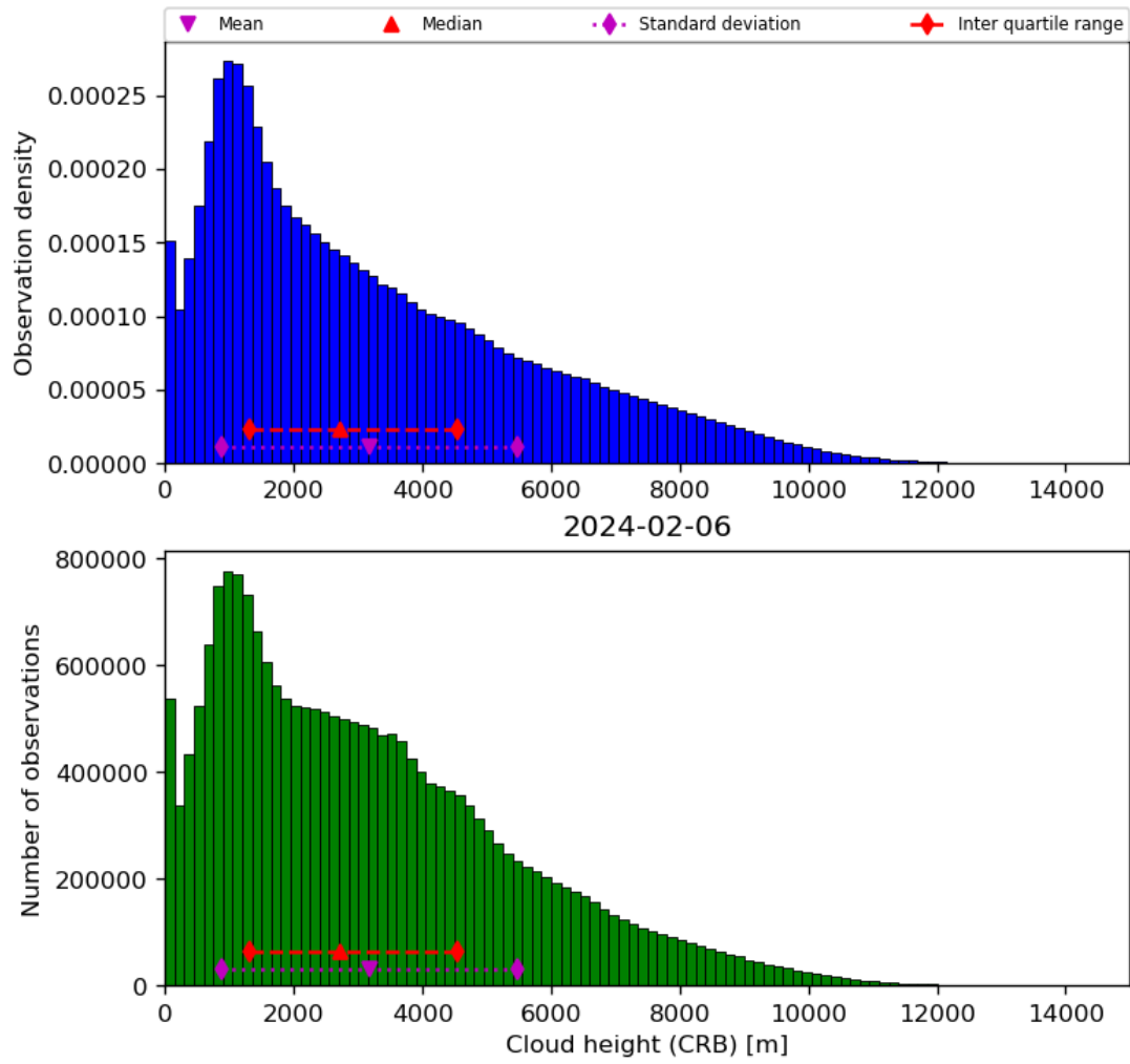
Figure 43: Histogram of “Cloud height (CRB)” for 2024-02-06 to 2024-02-07
