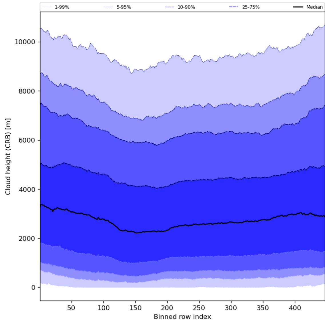
Figure 59: Along track statistics of “Cloud height (CRB)” for 2024-02-06 to 2024-02-07
