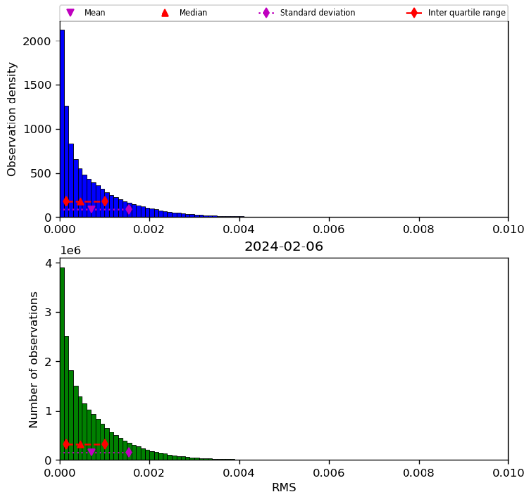
Figure 47: Histogram of “RMS” for 2024-02-06 to 2024-02-07
