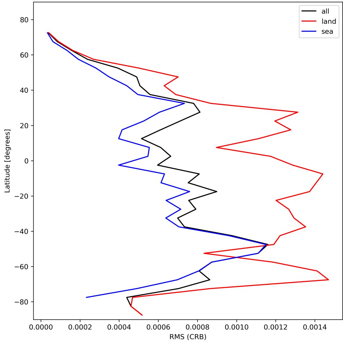
Figure 32: Zonal average of “RMS (CRB)” for 2024-02-06 to 2024-02-07.
