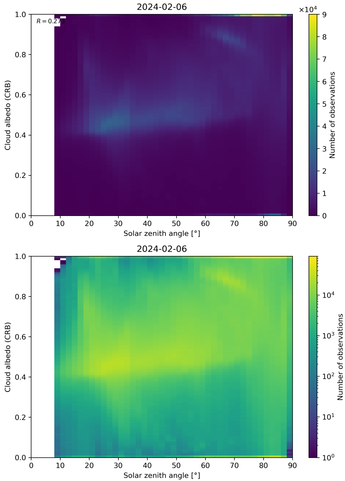
Figure 98: Scatter density plot of “Solar zenith angle” against “Cloud albedo (CRB)” for 2024-02-06 to 2024-02-07.
