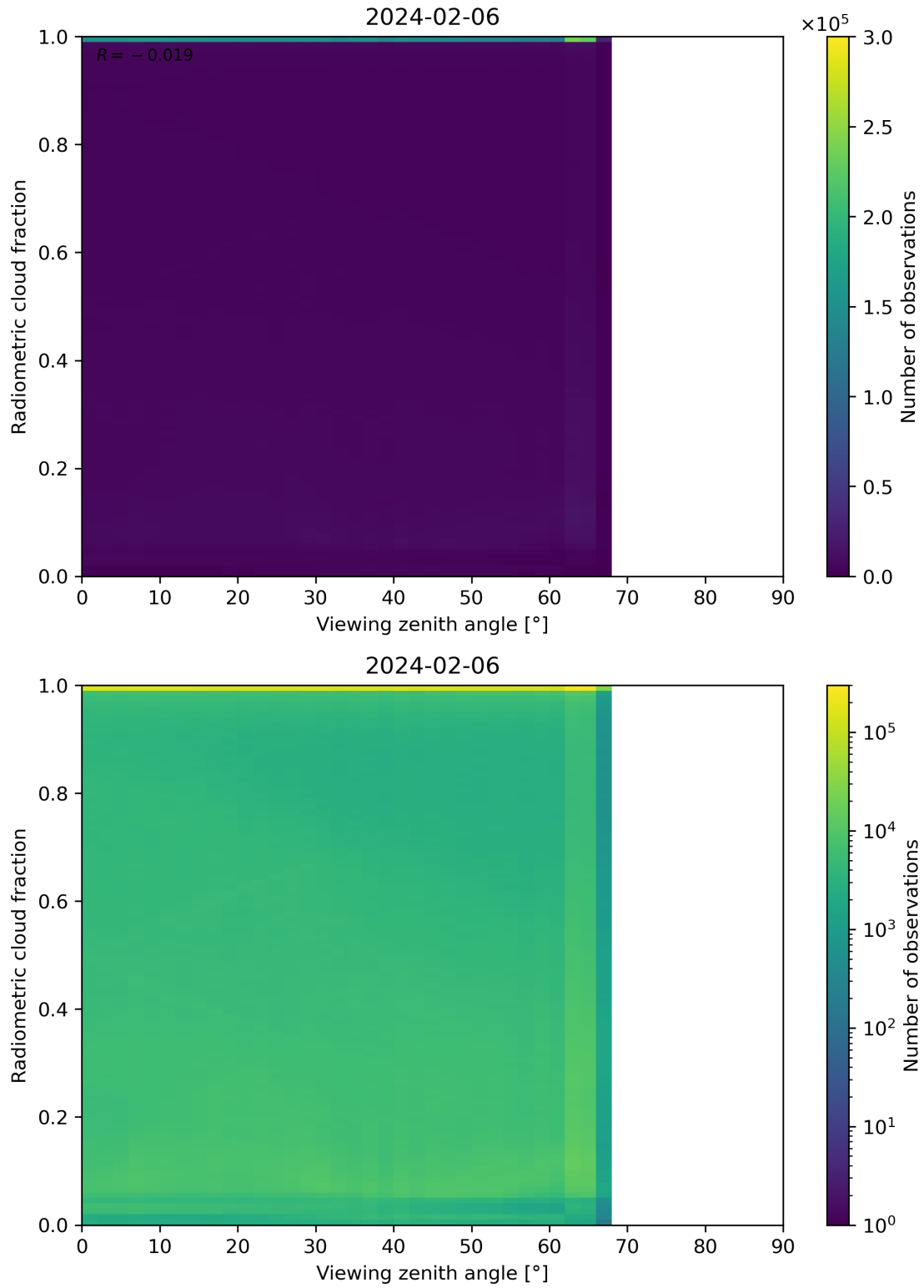
Figure 107: Scatter density plot of “Viewing zenith angle” against “Radiometric cloud fraction” for 2024-02-06 to 2024-02-07.
