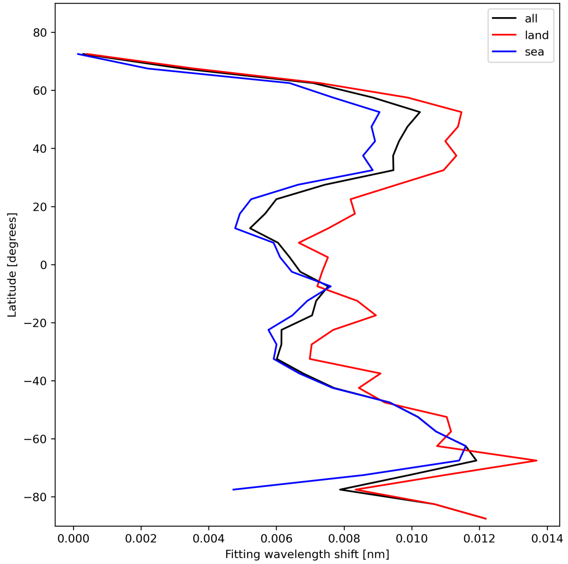
Figure 33: Zonal average of “Fitting wavelength shift” for 2024-02-06 to 2024-02-07.
