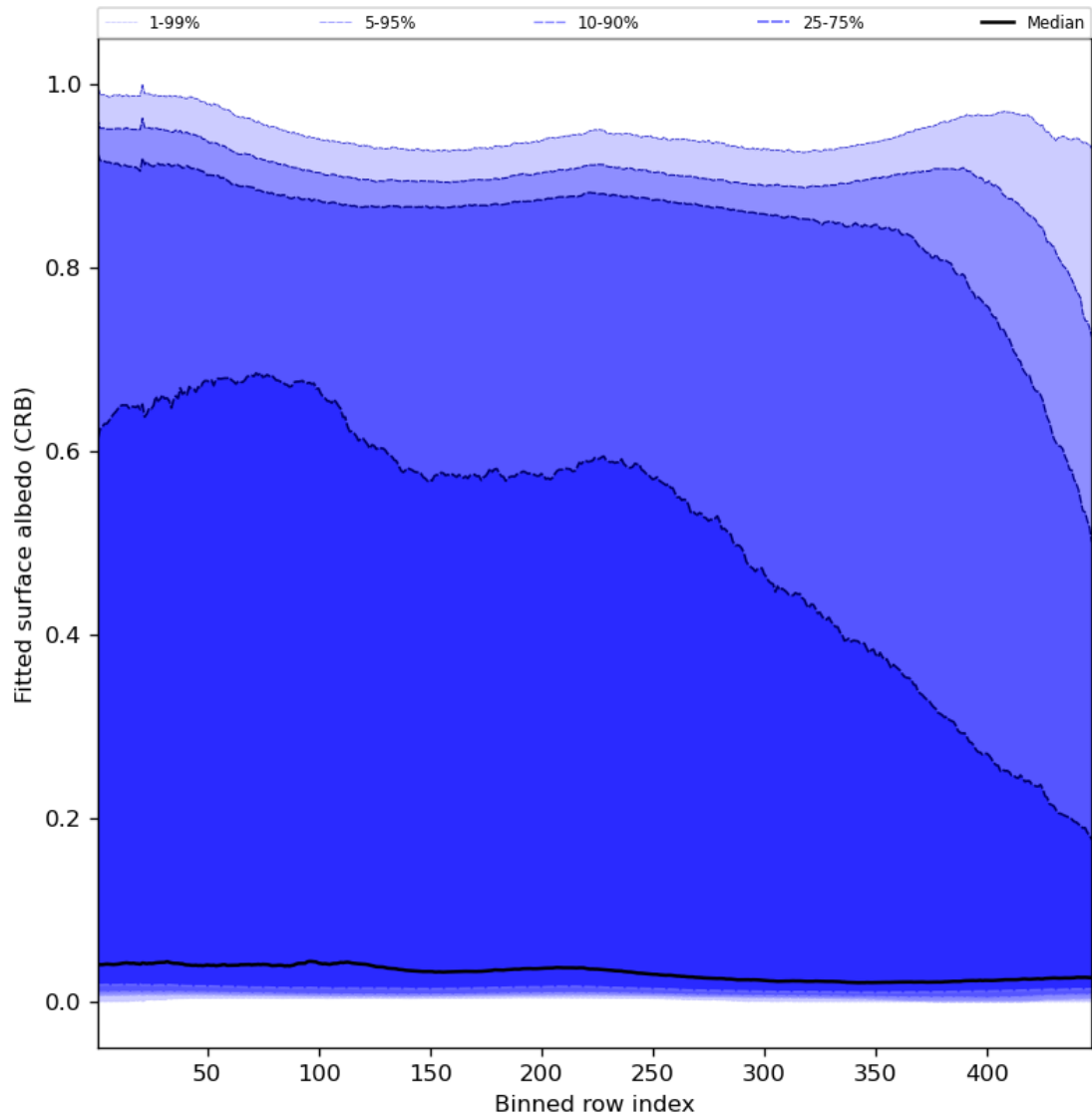
Figure 62: Along track statistics of “Fitted surface albedo (CRB)” for 2024-02-06 to 2024-02-07
