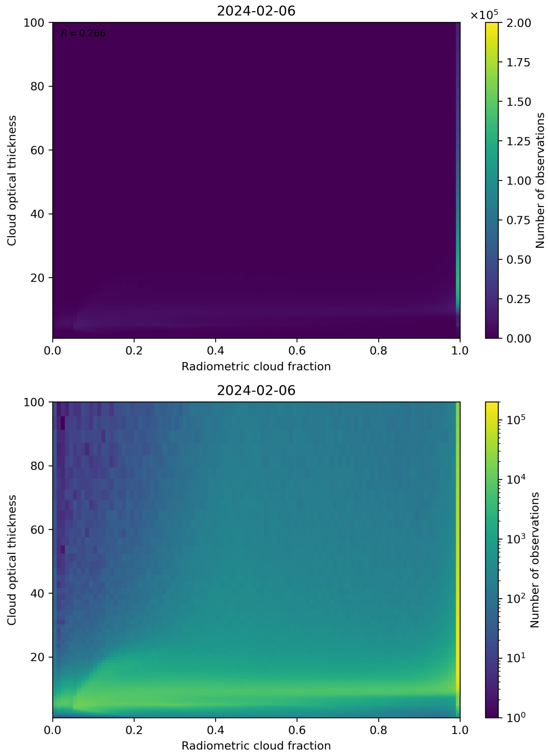
Figure 75: Scatter density plot of “Radiometric cloud fraction” against “Cloud optical thickness” for 2024-02-06 to 2024-02-07.
