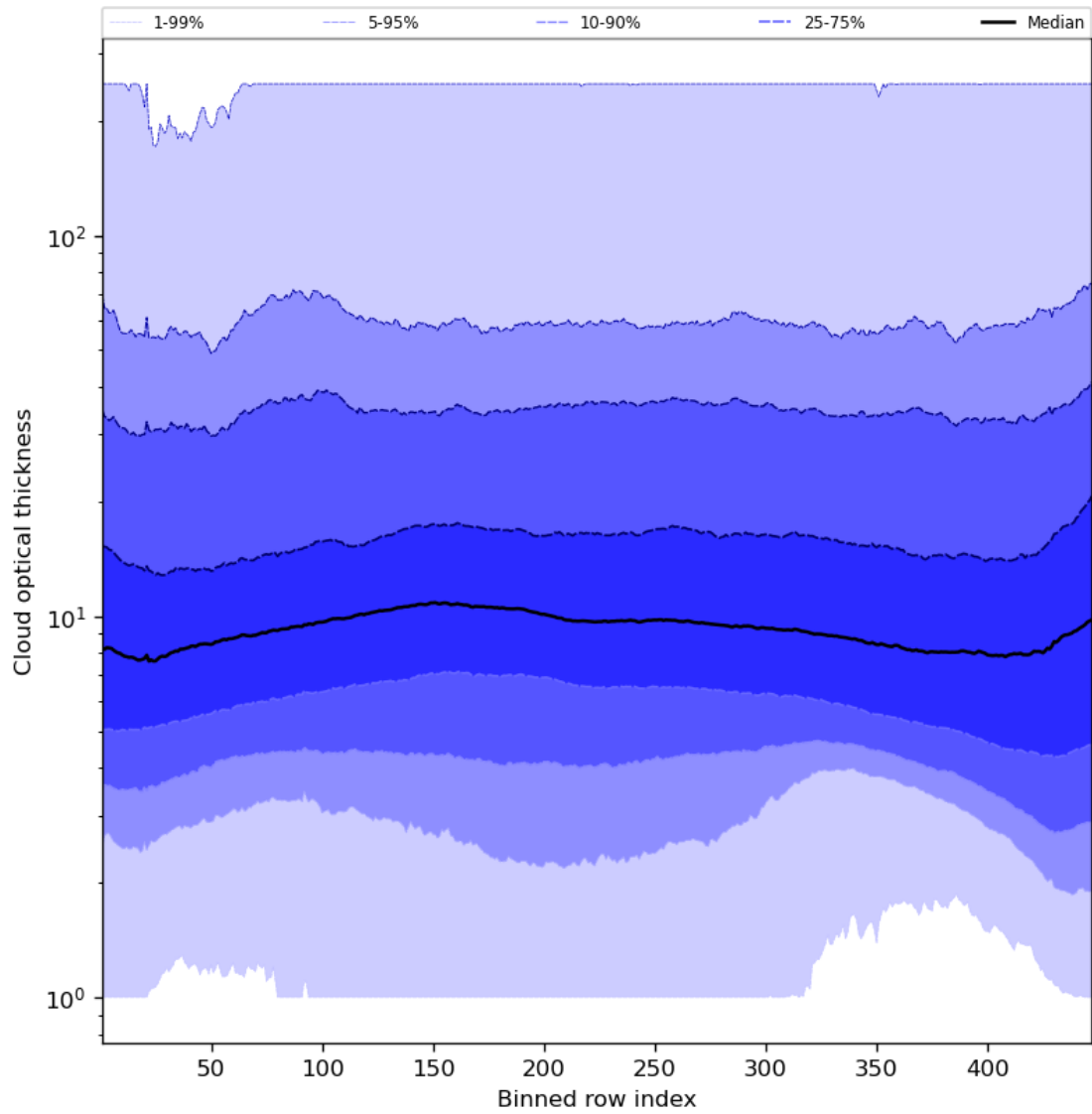
Figure 57: Along track statistics of “Cloud optical thickness” for 2024-02-06 to 2024-02-07
