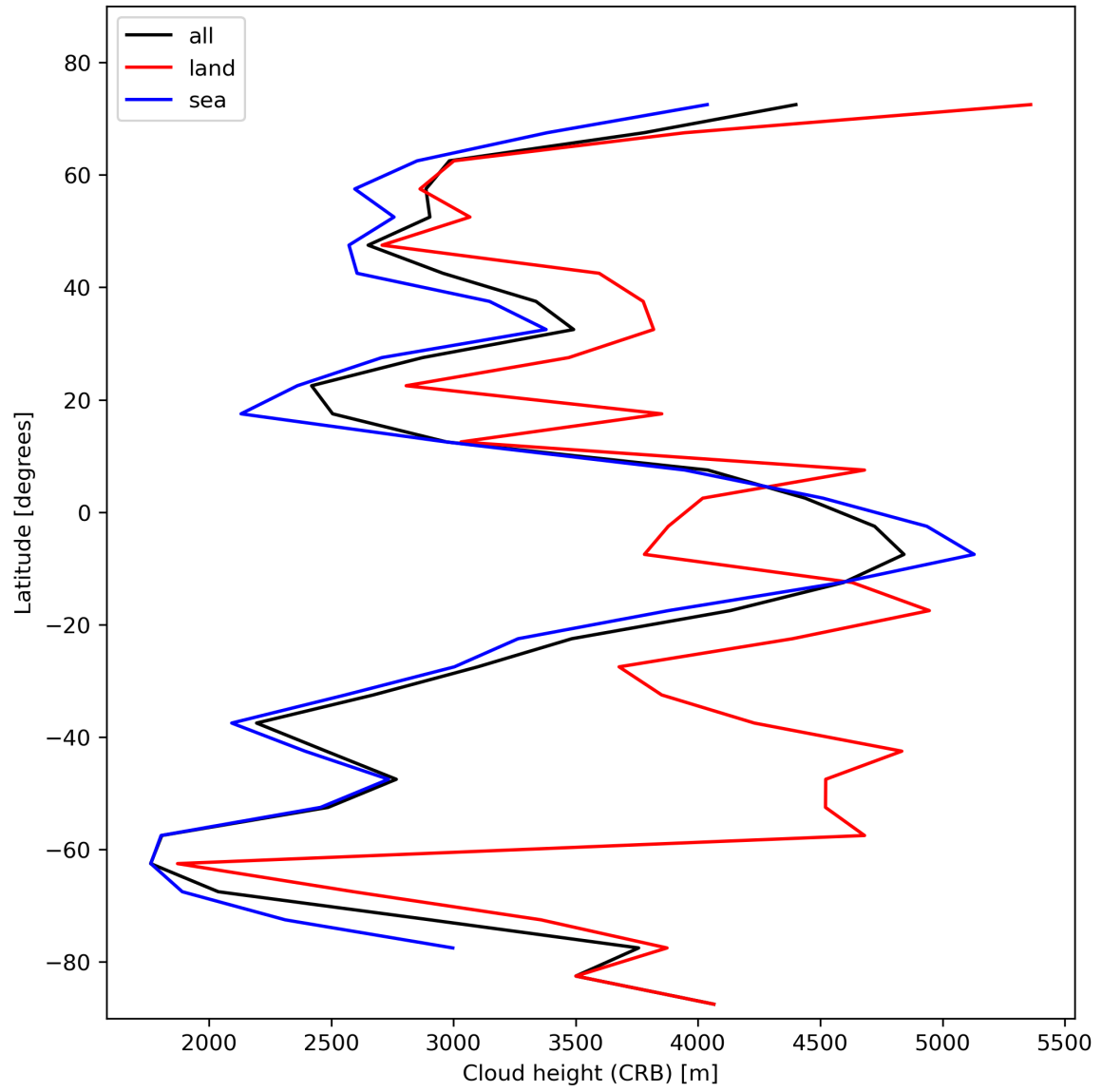
Figure 27: Zonal average of “Cloud height (CRB)” for 2024-02-06 to 2024-02-07.
