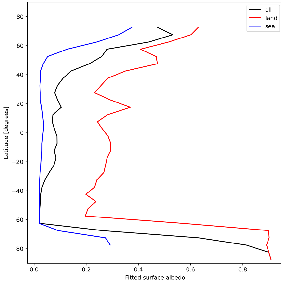
Figure 29: Zonal average of “Fitted surface albedo” for 2024-02-06 to 2024-02-07.
