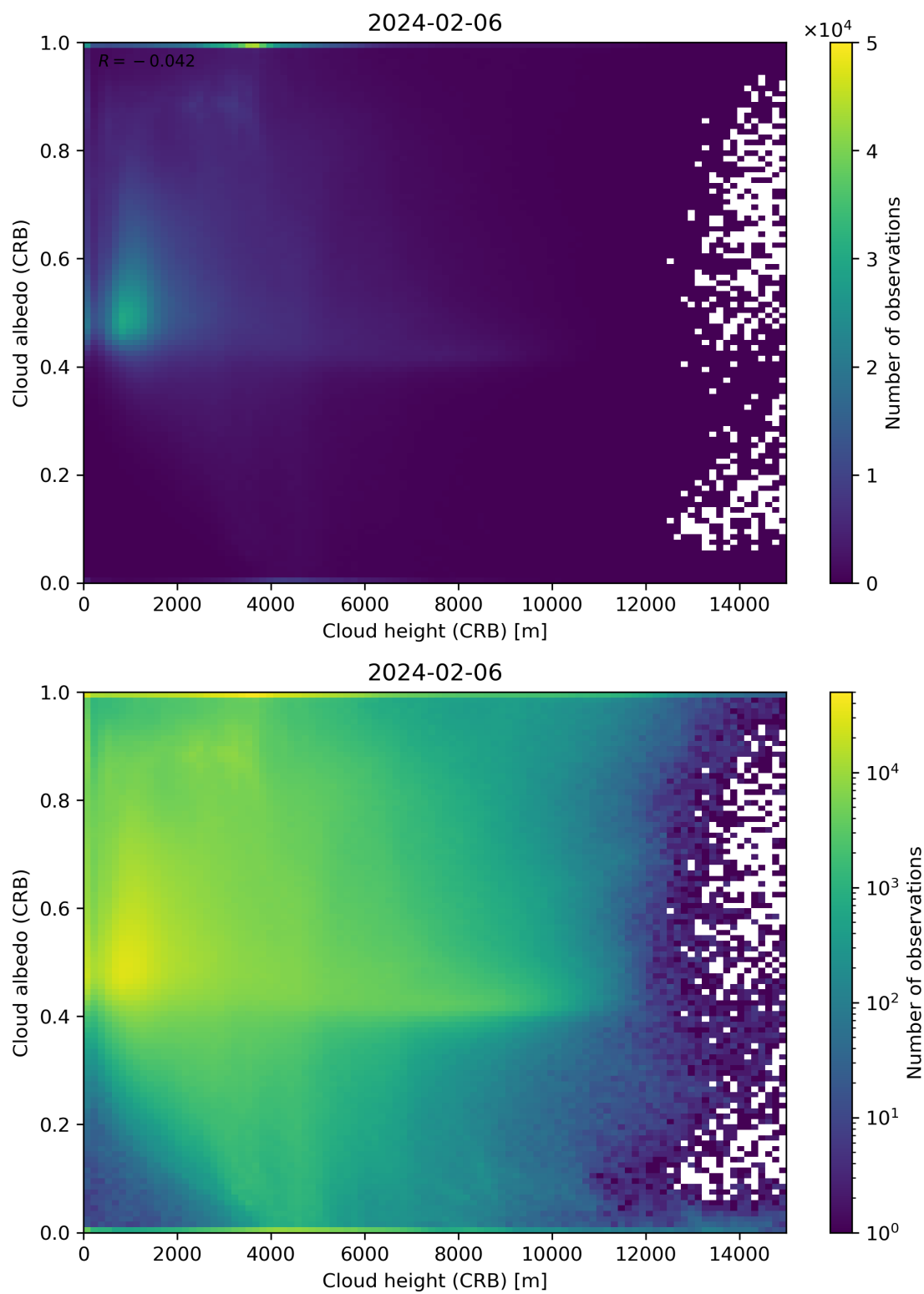
Figure 80: Scatter density plot of “Cloud height (CRB)” against “Cloud albedo (CRB)” for 2024-02-06 to 2024-02-07.
