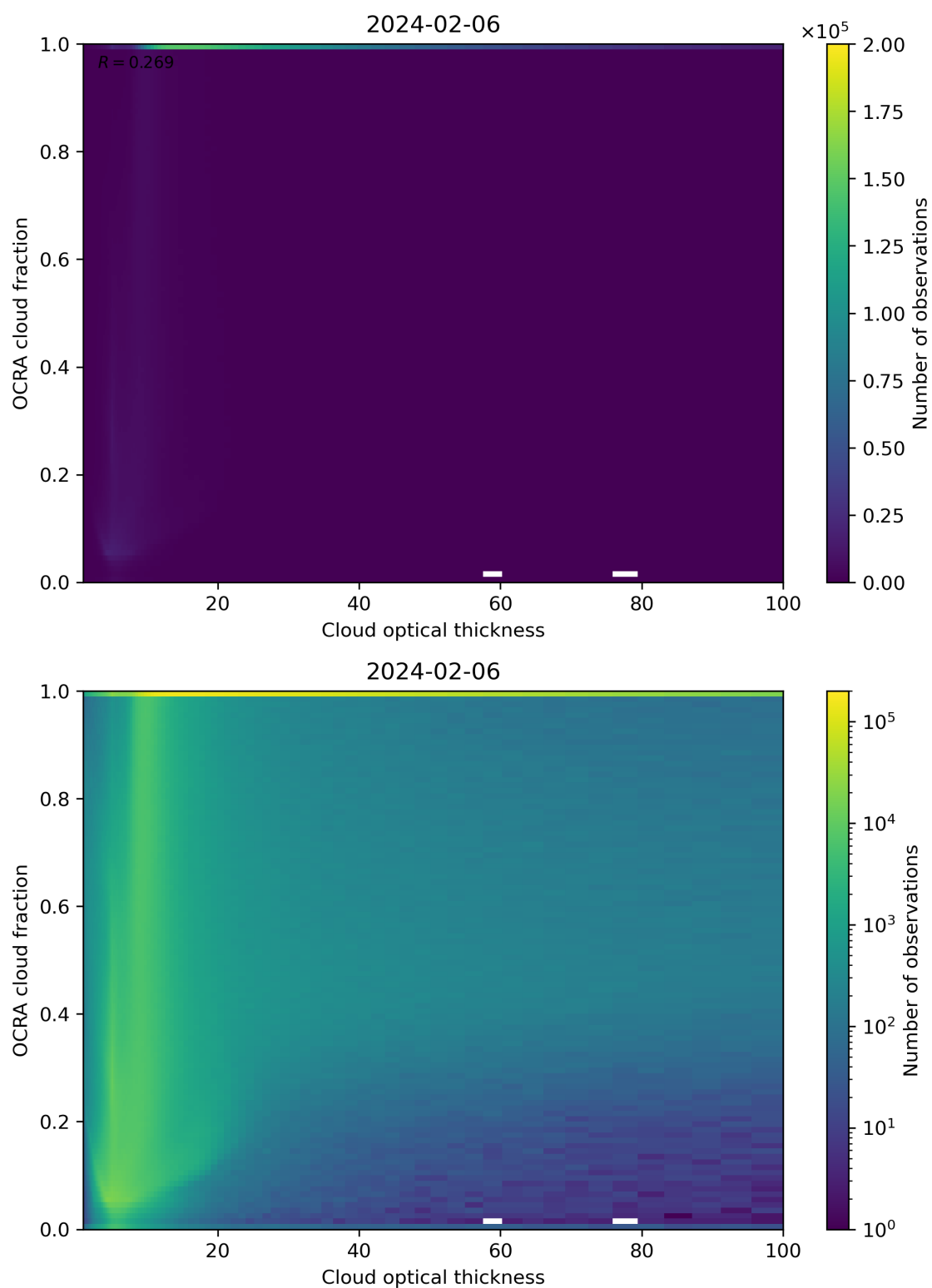
Figure 83: Scatter density plot of “Cloud optical thickness” against “OCRA cloud fraction” for 2024-02-06 to 2024-02-07.
