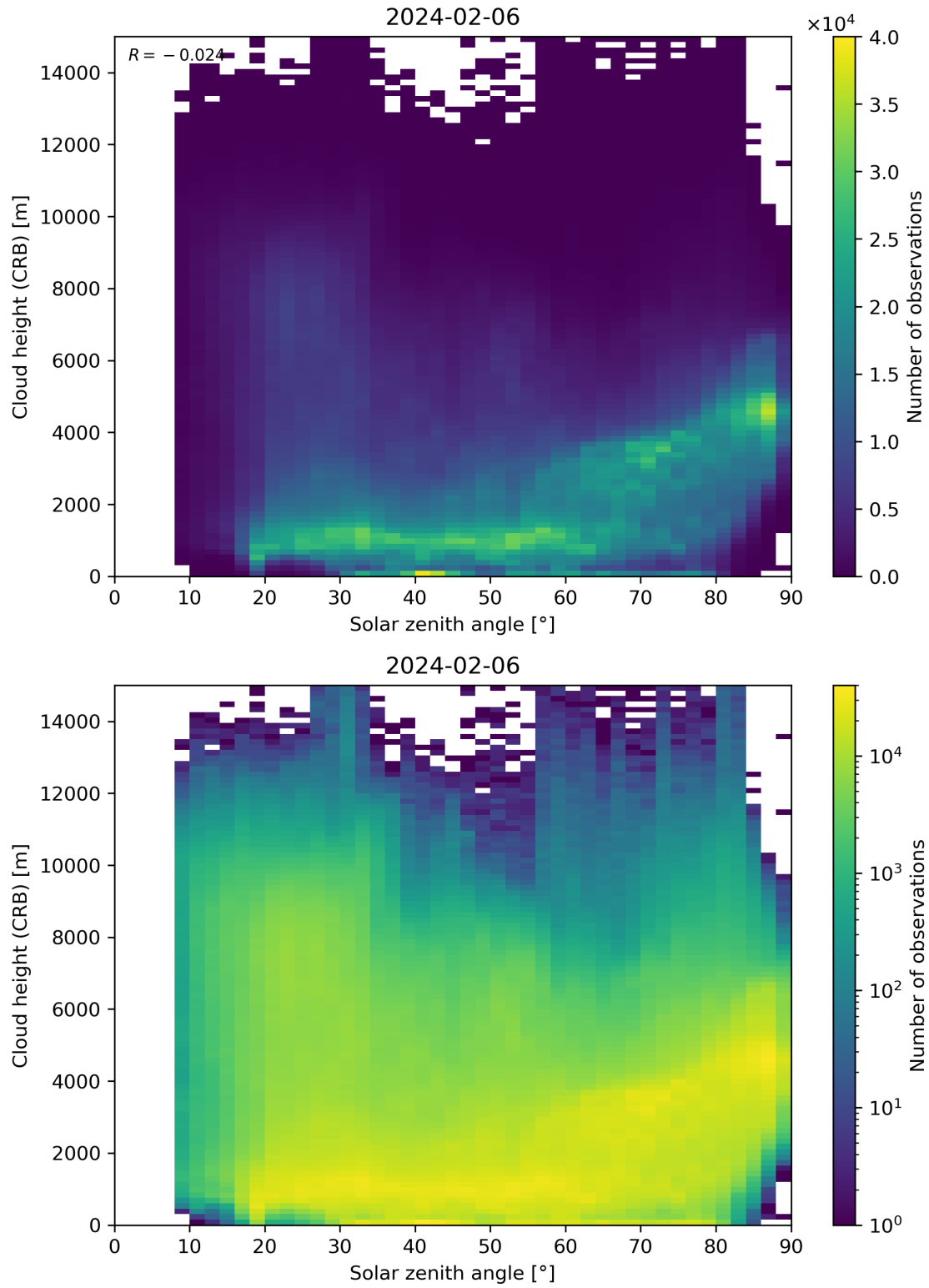
Figure 102: Scatter density plot of “Solar zenith angle” against “Cloud height (CRB)” for 2024-02-06 to 2024-02-07.
