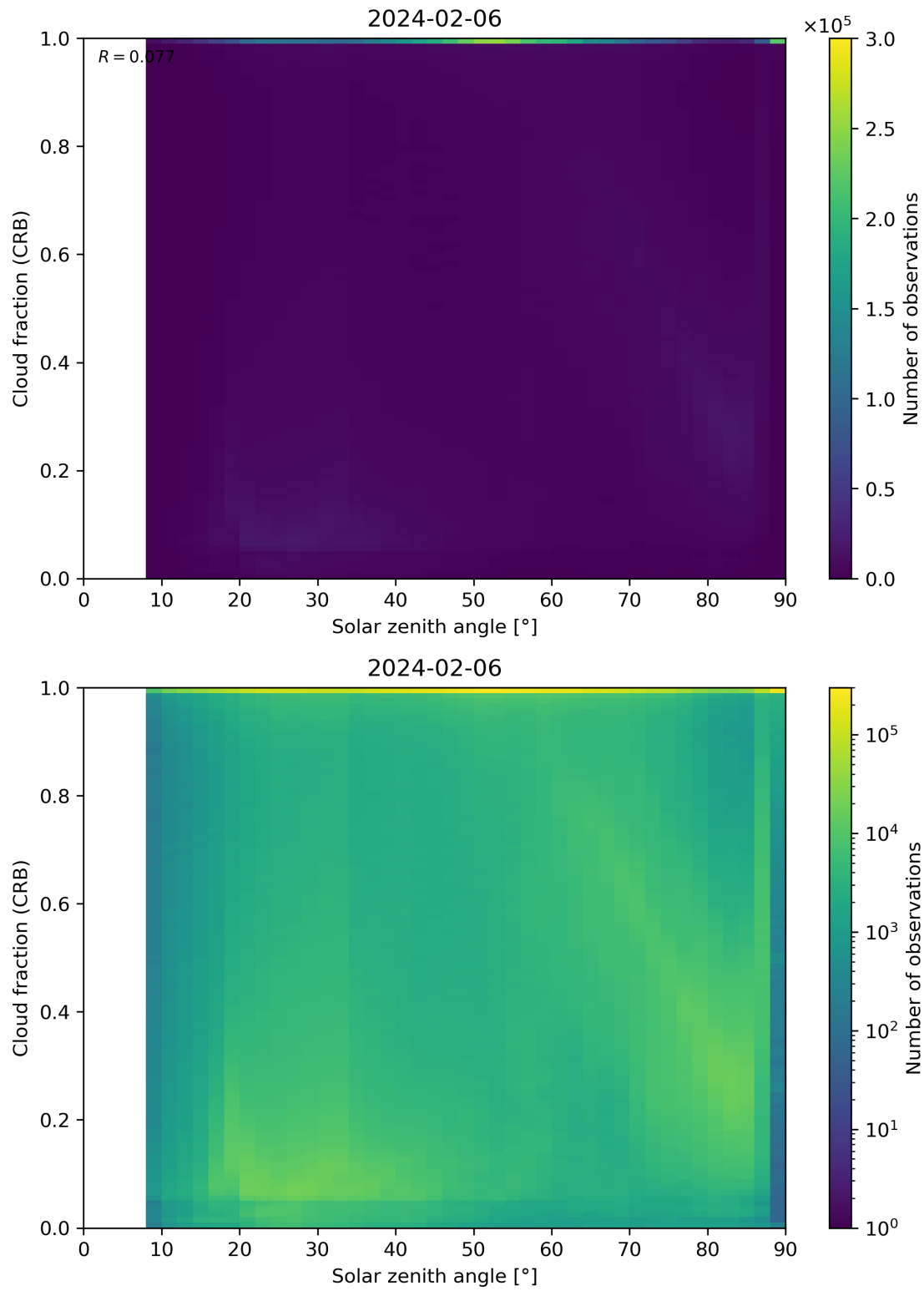
Figure 101: Scatter density plot of “Solar zenith angle” against “Cloud fraction (CRB)” for 2024-02-06 to 2024-02-07.
