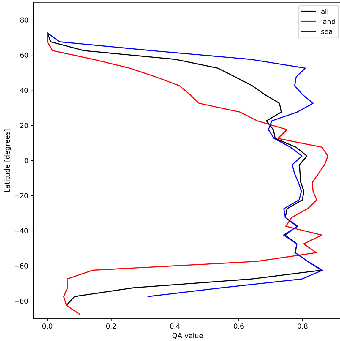
Figure 22: Zonal average of “QA value” for 2024-02-06 to 2024-02-07.
