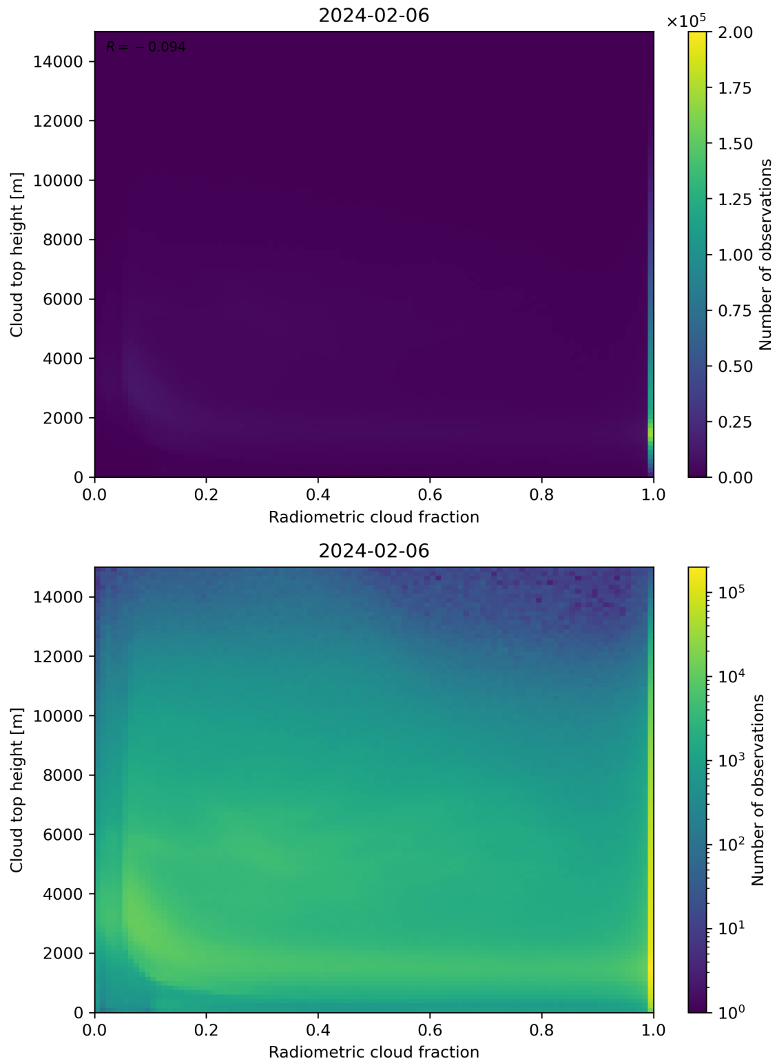
Figure 76: Scatter density plot of “Radiometric cloud fraction” against “Cloud top height” for 2024-02-06 to 2024-02-07.
