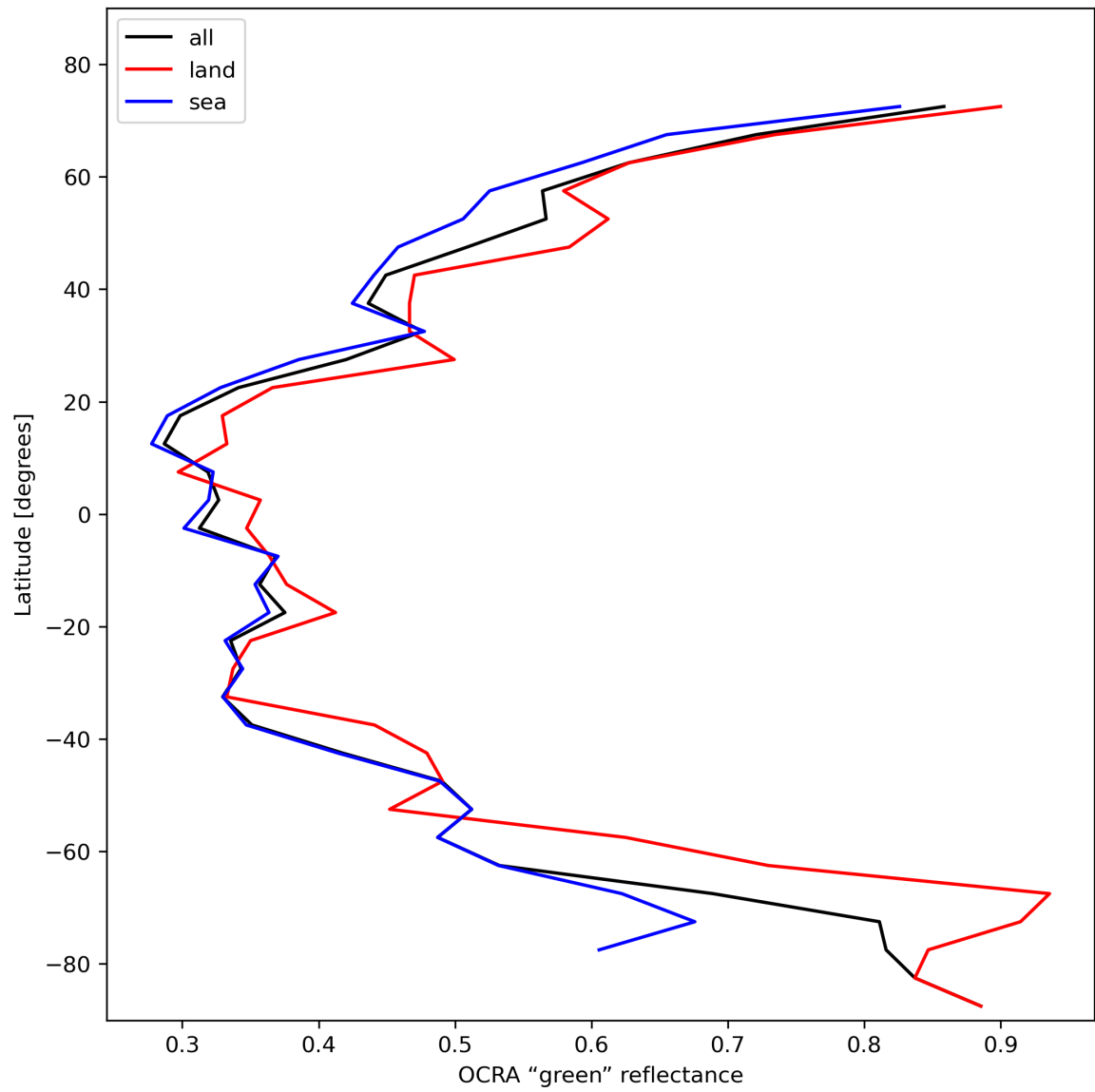
Figure 36: Zonal average of “OCRA “green” reflectance” for 2024-02-06 to 2024-02-07.
