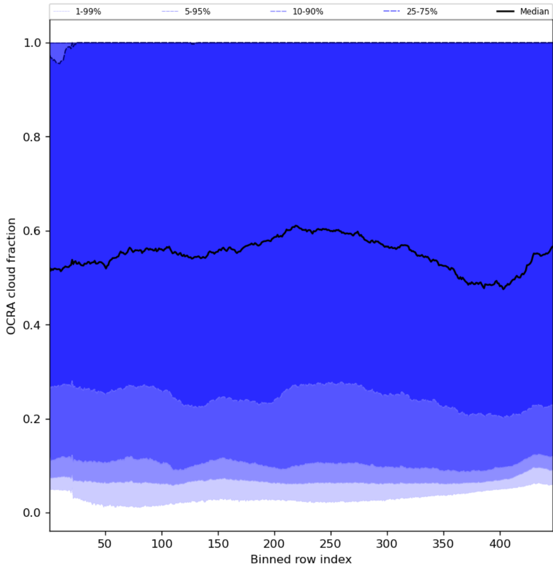
Figure 66: Along track statistics of “OCRA cloud fraction” for 2024-02-06 to 2024-02-07
