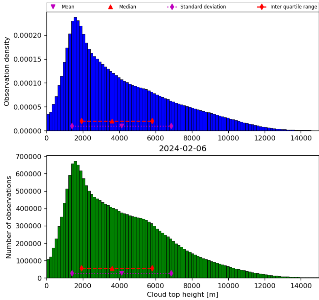
Figure 40: Histogram of “Cloud top height” for 2024-02-06 to 2024-02-07
