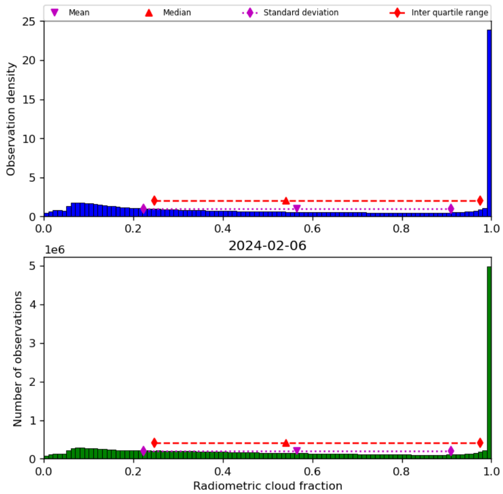
Figure 39: Histogram of “Radiometric cloud fraction” for 2024-02-06 to 2024-02-07
