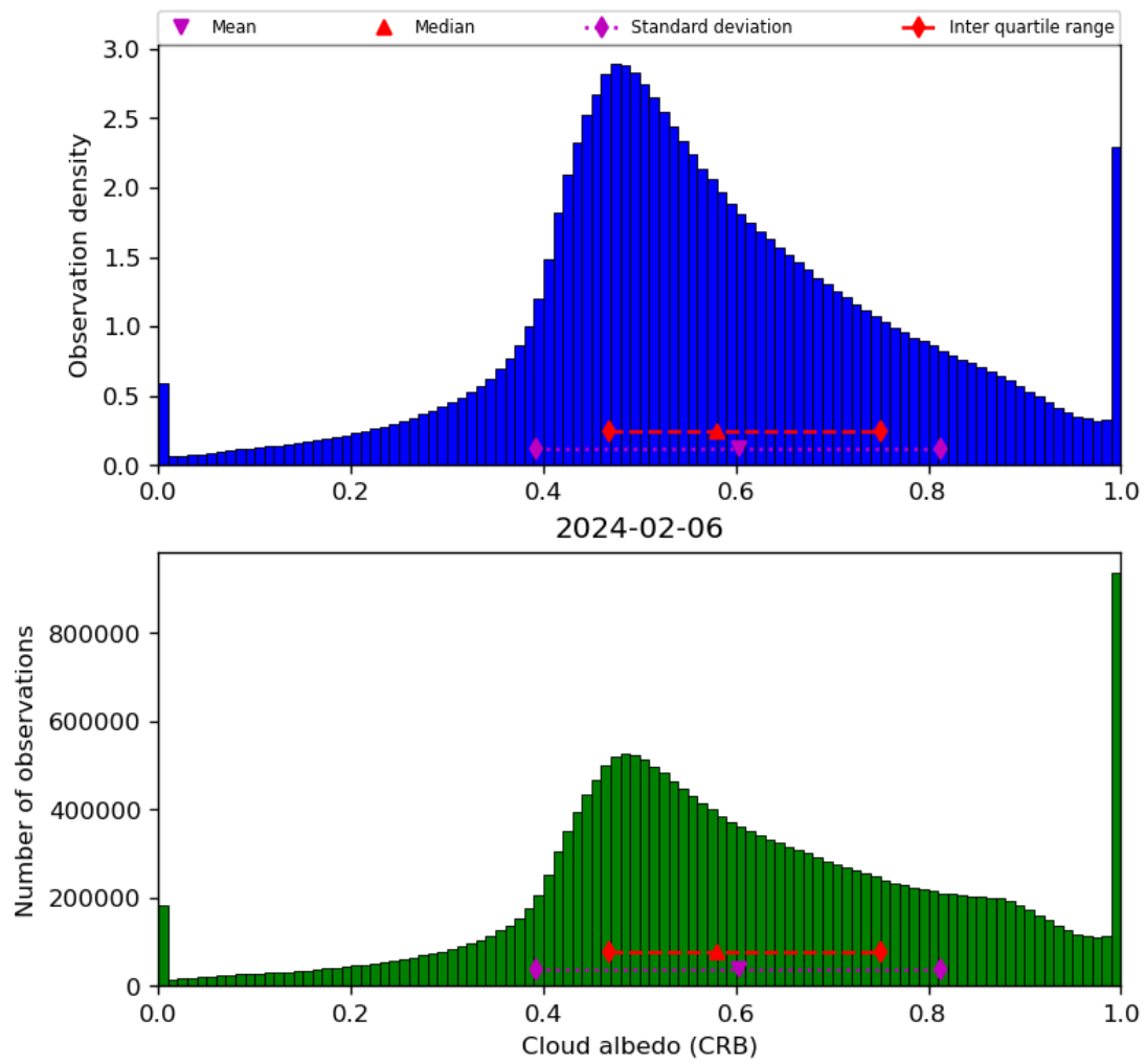
Figure 44: Histogram of “Cloud albedo (CRB)” for 2024-02-06 to 2024-02-07
