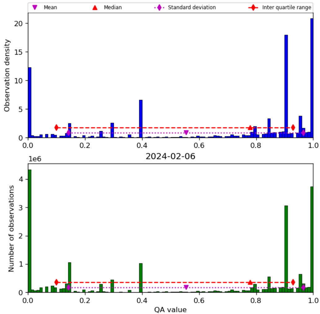
Figure 38: Histogram of “QA value” for 2024-02-06 to 2024-02-07
