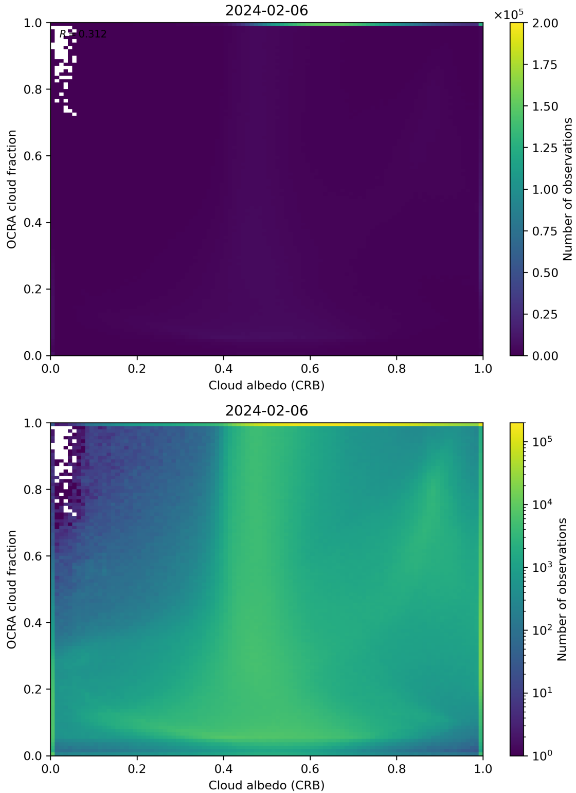
Figure 70: Scatter density plot of “Cloud albedo (CRB)” against “OCRA cloud fraction” for 2024-02-06 to 2024-02-07.
