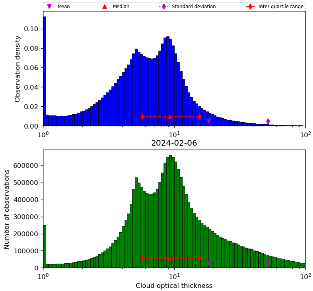
Figure 41: Histogram of “Cloud optical thickness” for 2024-02-06 to 2024-02-07
