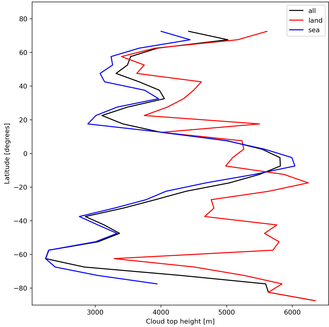
Figure 24: Zonal average of “Cloud top height” for 2024-02-06 to 2024-02-07.
