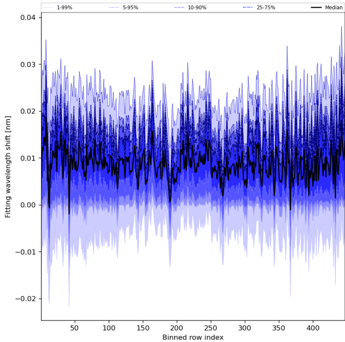
Figure 65: Along track statistics of “Fitting wavelength shift” for 2024-02-06 to 2024-02-07
