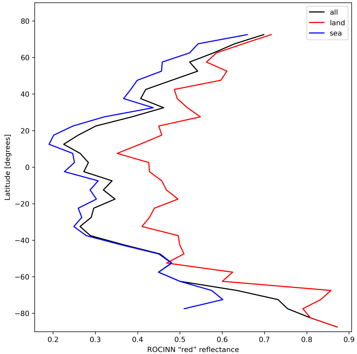
Figure 37: Zonal average of “ROCINN “red” reflectance” for 2024-02-06 to 2024-02-07.
