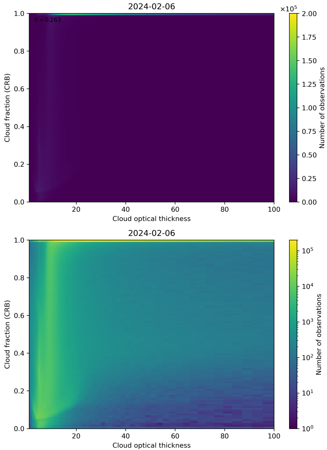
Figure 84: Scatter density plot of “Cloud optical thickness” against “Cloud fraction (CRB)” for 2024-02-06 to 2024-02-07.
