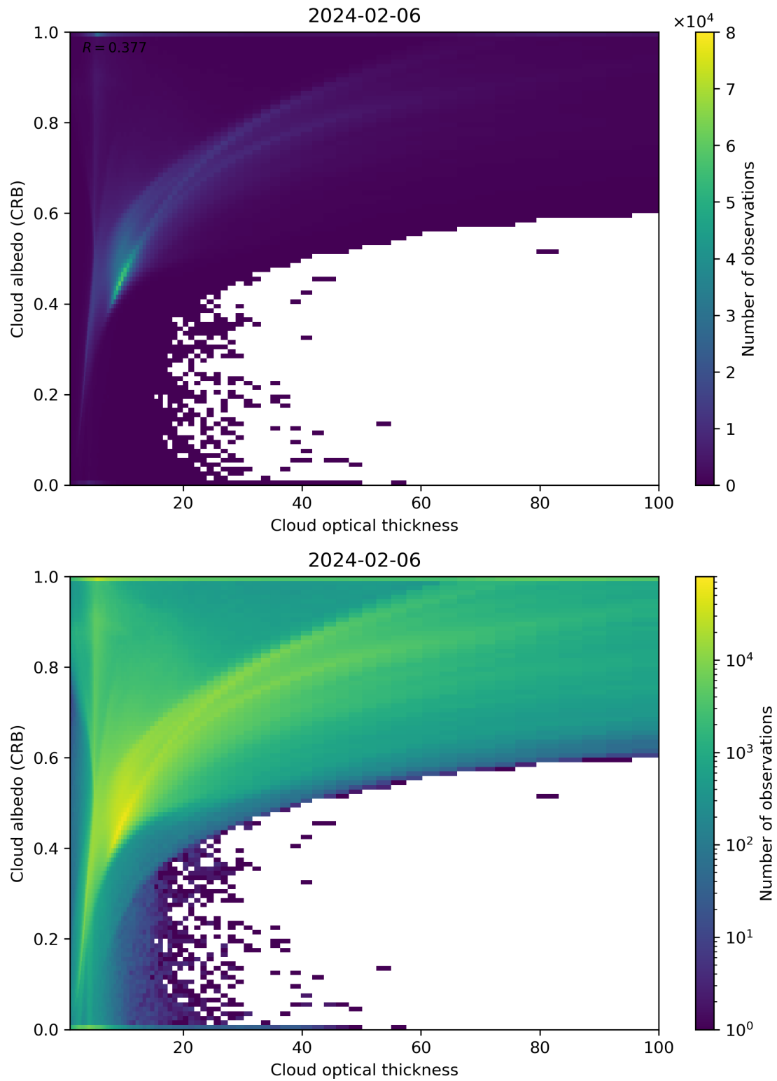
Figure 82: Scatter density plot of “Cloud optical thickness” against “Cloud albedo (CRB)” for 2024-02-06 to 2024-02-07.
