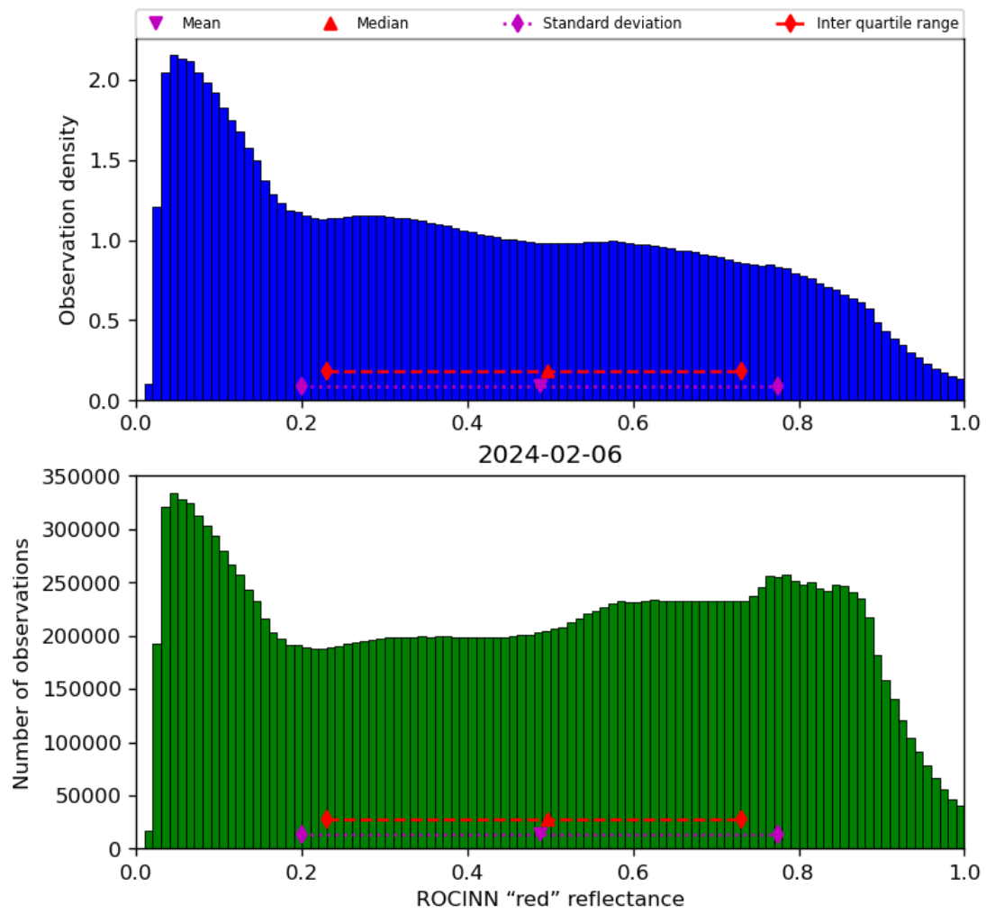
Figure 53: Histogram of “ROCINN “red” reflectance” for 2024-02-06 to 2024-02-07
