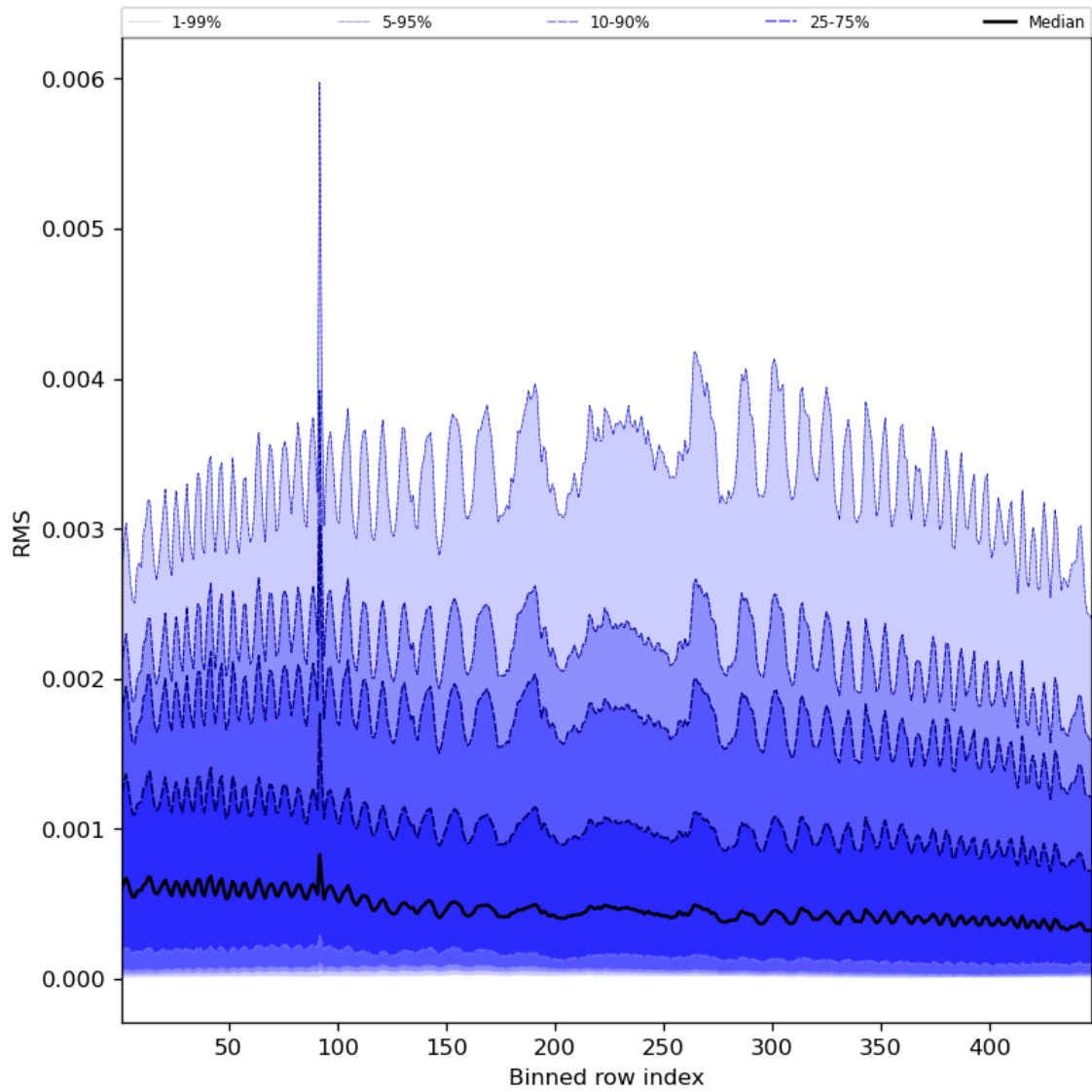
Figure 63: Along track statistics of “RMS” for 2024-02-06 to 2024-02-07
