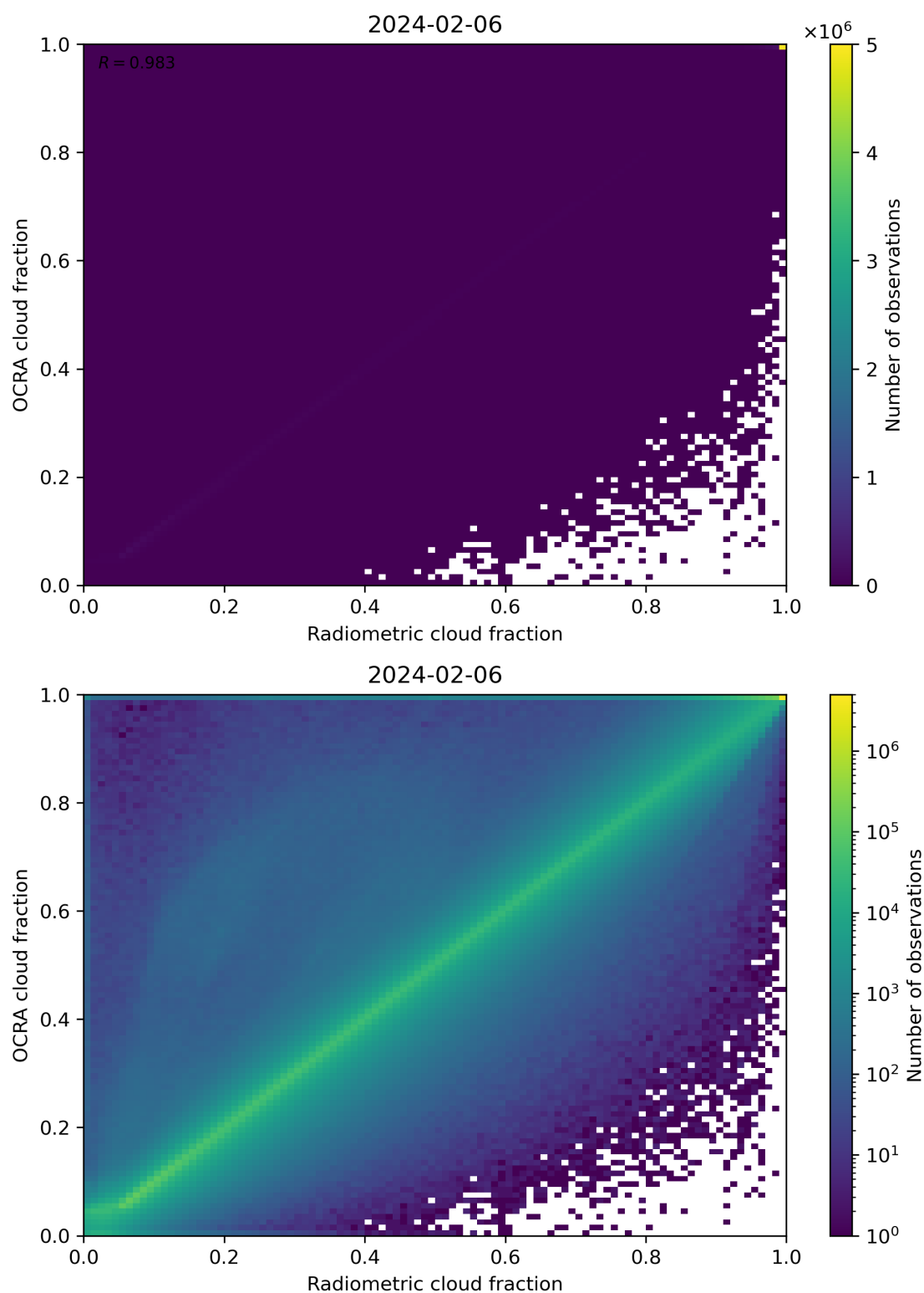
Figure 72: Scatter density plot of “Radiometric cloud fraction” against “OCRA cloud fraction” for 2024-02-06 to 2024-02-07.
