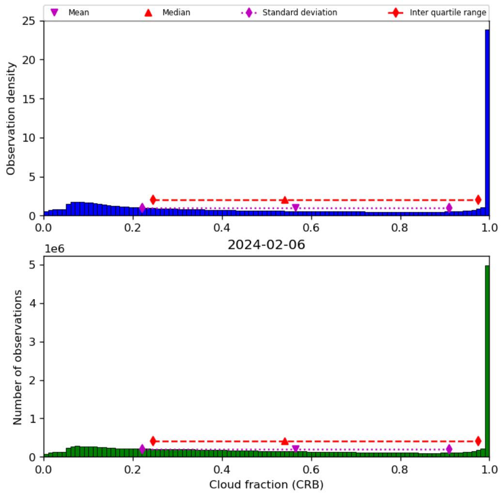
Figure 42: Histogram of “Cloud fraction (CRB)” for 2024-02-06 to 2024-02-07
