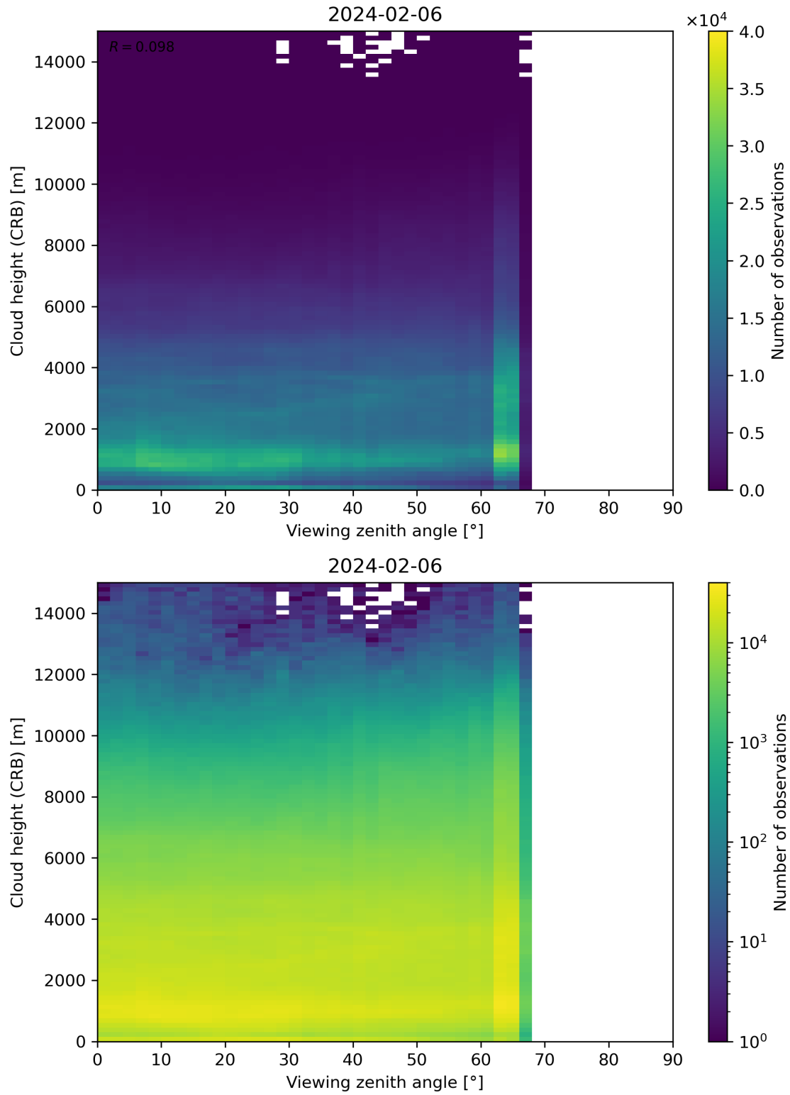
Figure 110: Scatter density plot of “Viewing zenith angle” against “Cloud height (CRB)” for 2024-02-06 to 2024-02-07.
