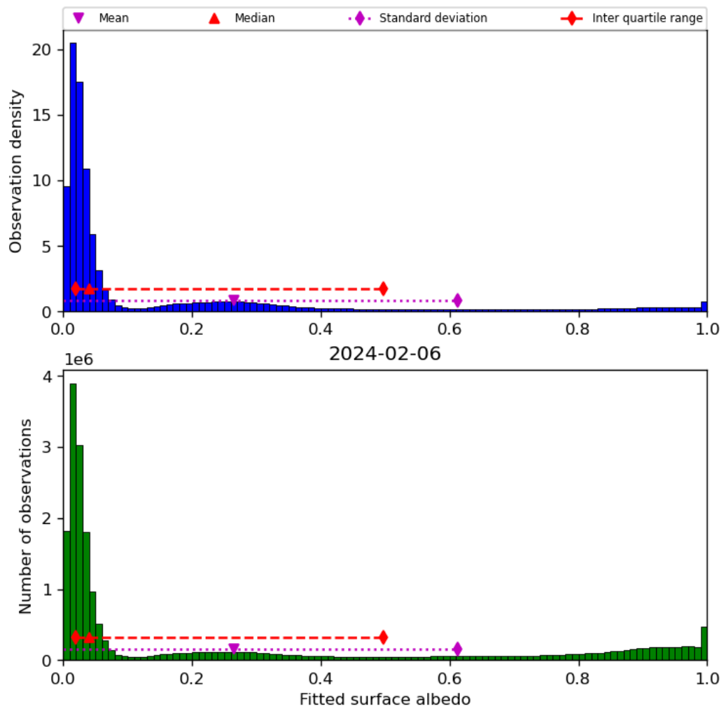
Figure 45: Histogram of “Fitted surface albedo” for 2024-02-06 to 2024-02-07
