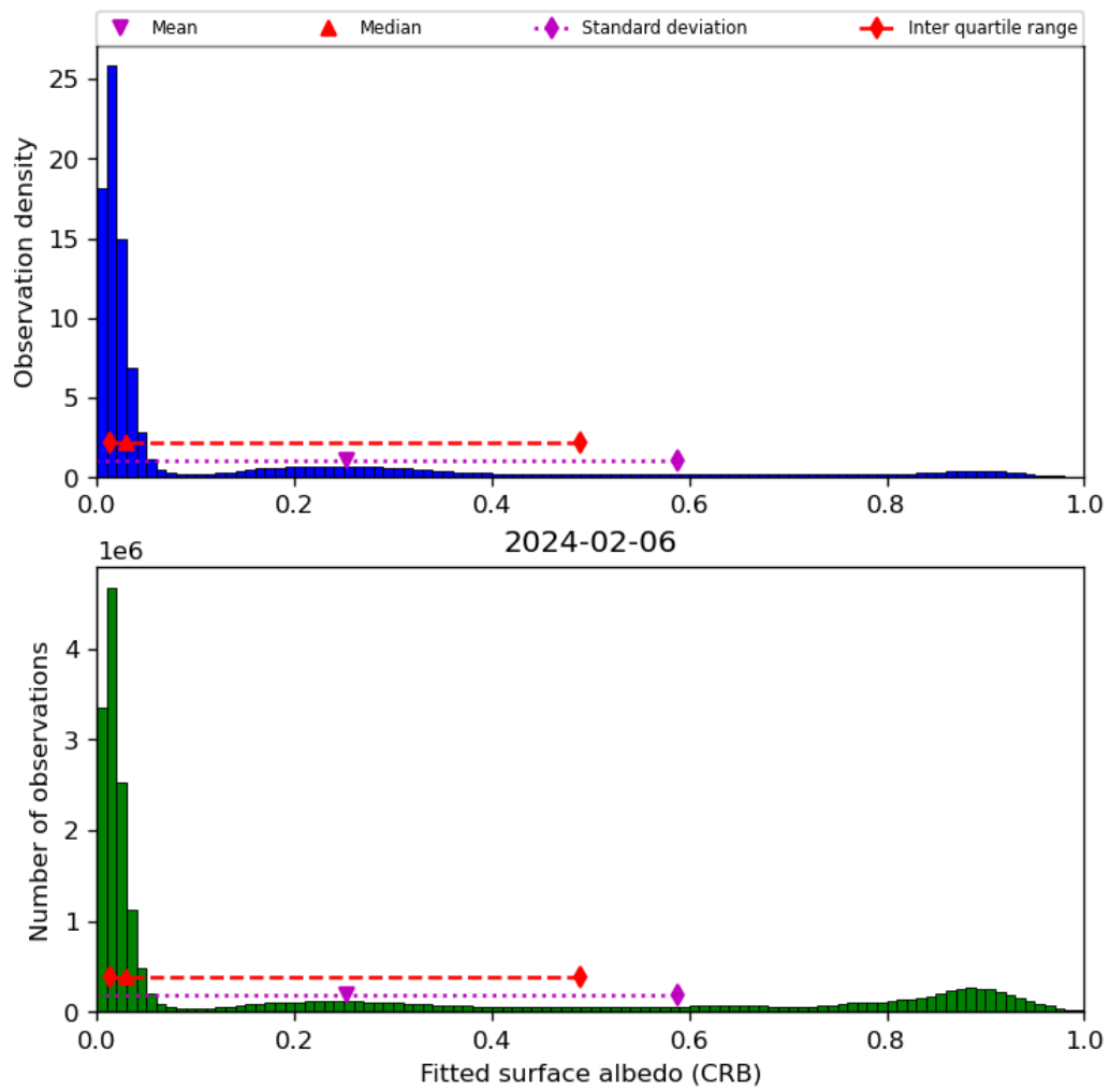
Figure 46: Histogram of “Fitted surface albedo (CRB)” for 2024-02-06 to 2024-02-07
