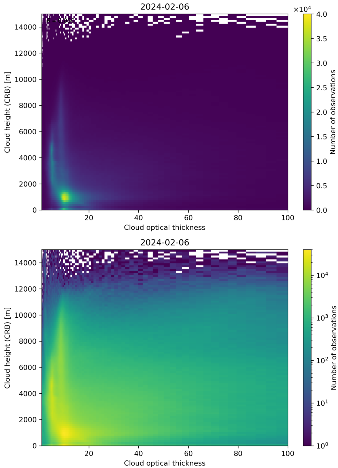
Figure 85: Scatter density plot of “Cloud optical thickness” against “Cloud height (CRB)” for 2024-02-06 to 2024-02-07.
