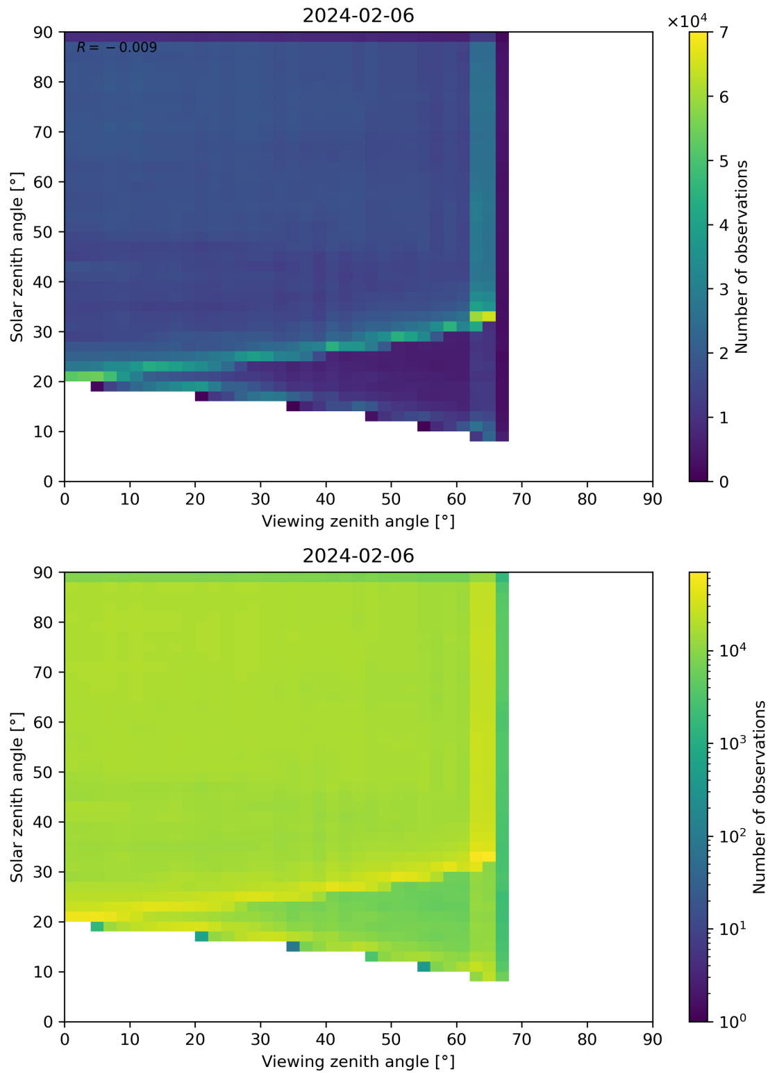
Figure 114: Scatter density plot of “Viewing zenith angle” against “Solar zenith angle” for 2024-02-06 to 2024-02-07.
