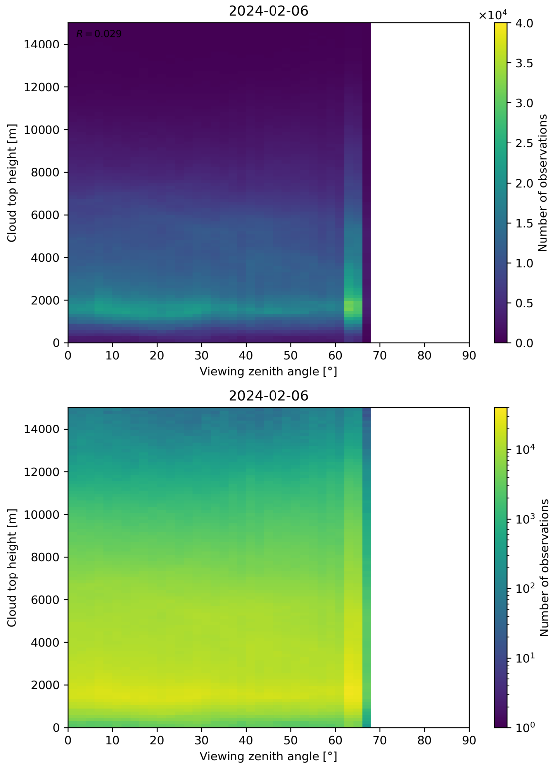
Figure 112: Scatter density plot of “Viewing zenith angle” against “Cloud top height” for 2024-02-06 to 2024-02-07.
