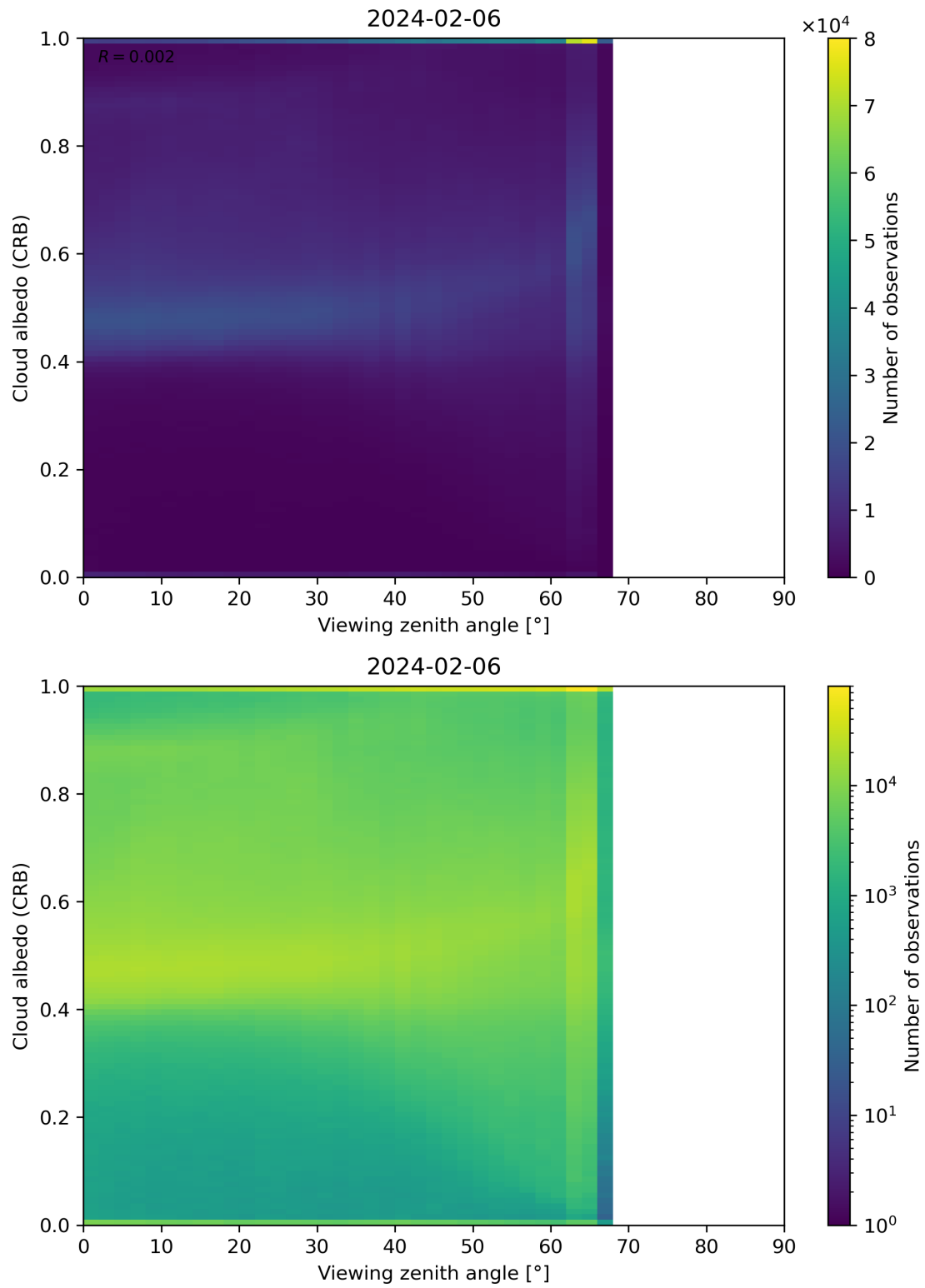
Figure 106: Scatter density plot of “Viewing zenith angle” against “Cloud albedo (CRB)” for 2024-02-06 to 2024-02-07.
