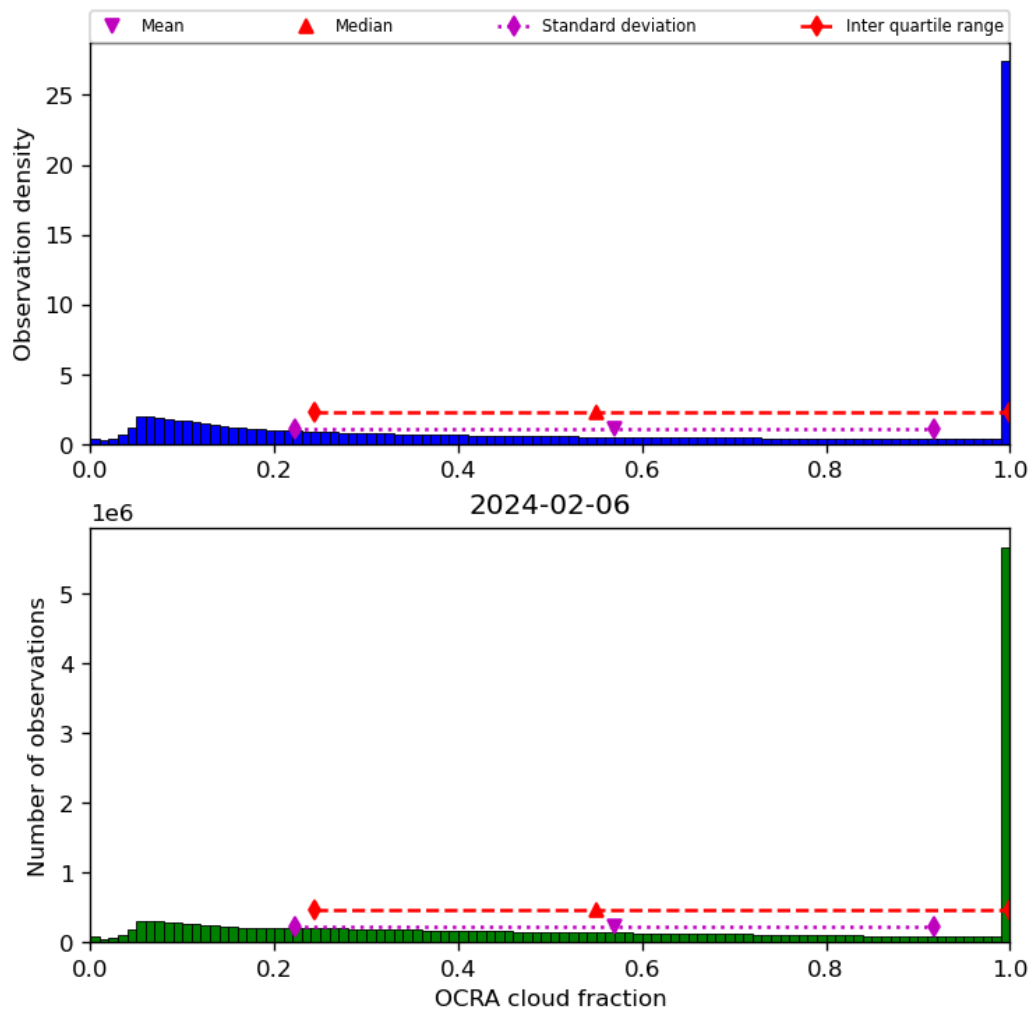
Figure 50: Histogram of “OCRA cloud fraction” for 2024-02-06 to 2024-02-07
