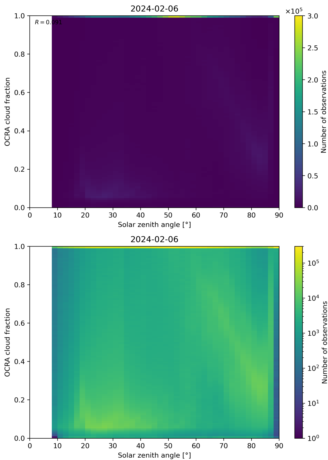
Figure 100: Scatter density plot of “Solar zenith angle” against “OCRA cloud fraction” for 2024-02-06 to 2024-02-07.
