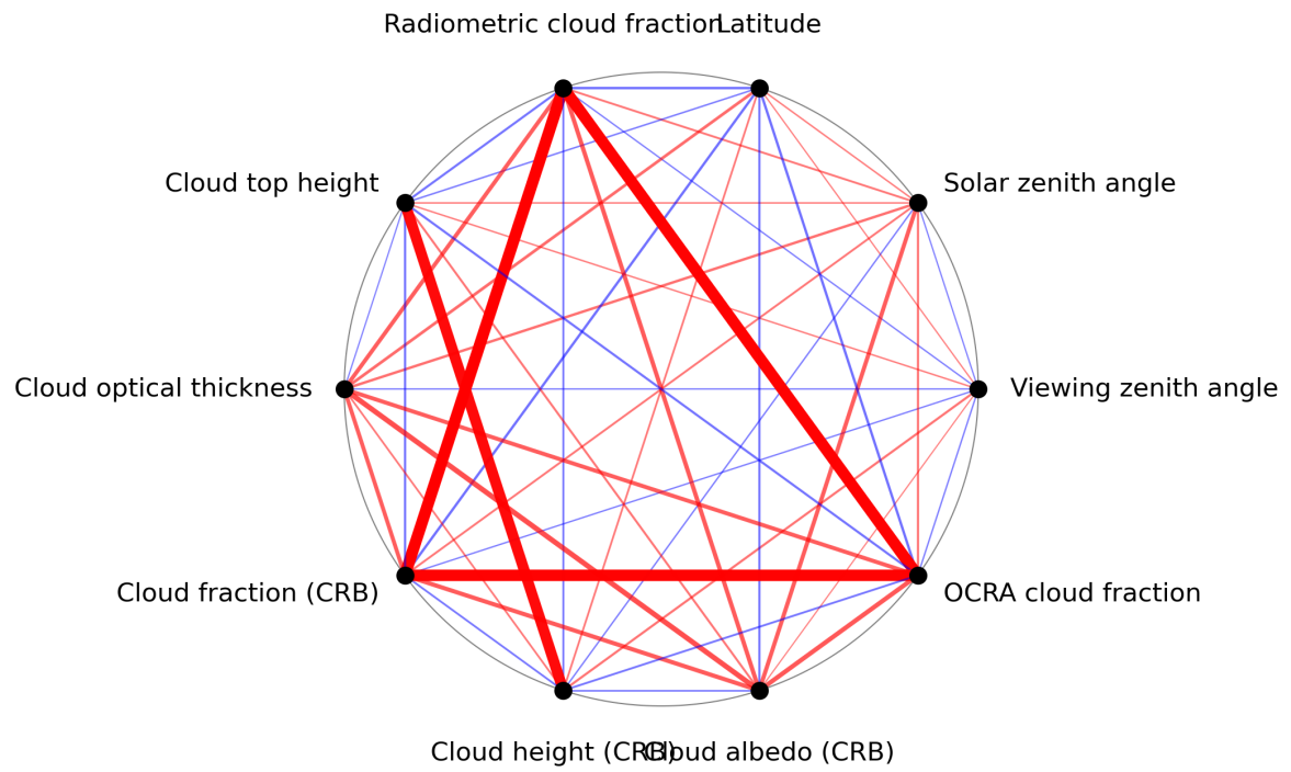
Figure 1: Map of correlation graph for 2024-02-06 to 2024-02-07.
