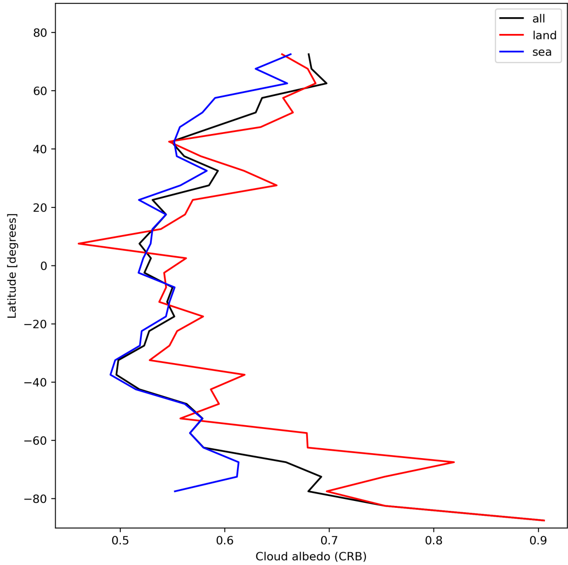
Figure 28: Zonal average of “Cloud albedo (CRB)” for 2024-02-06 to 2024-02-07.
