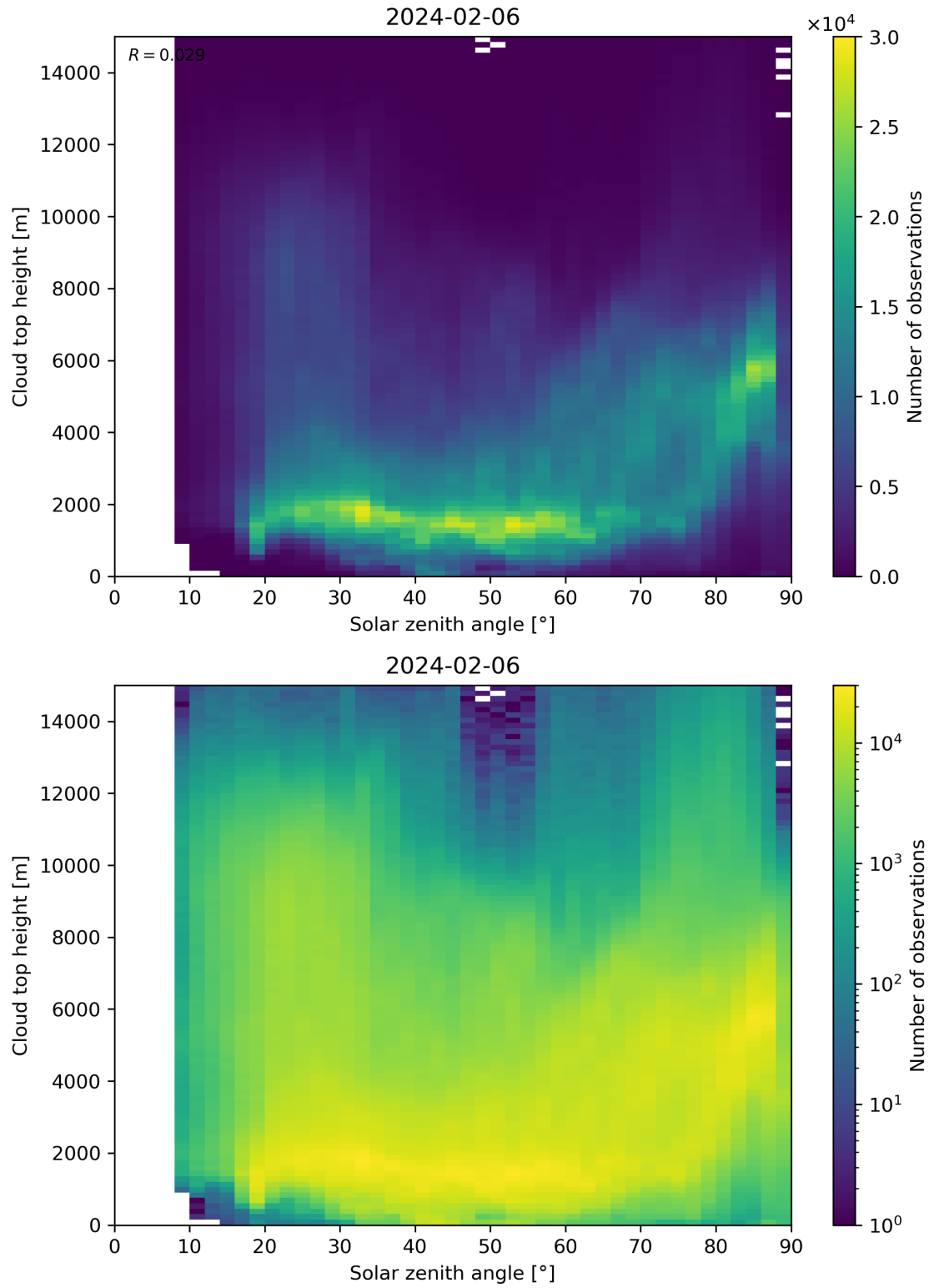
Figure 104: Scatter density plot of “Solar zenith angle” against “Cloud top height” for 2024-02-06 to 2024-02-07.
