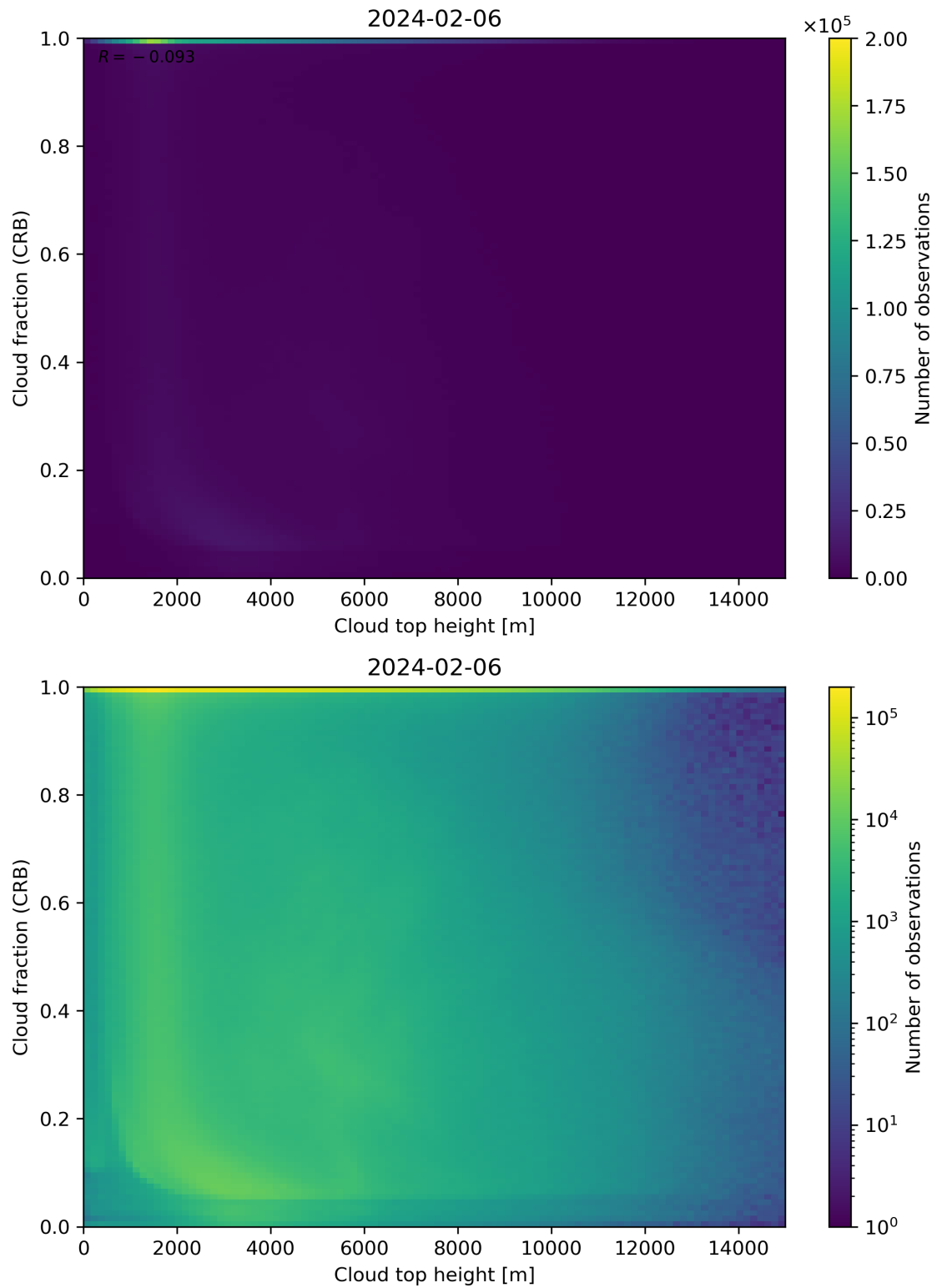
Figure 88: Scatter density plot of “Cloud top height” against “Cloud fraction (CRB)” for 2024-02-06 to 2024-02-07.
