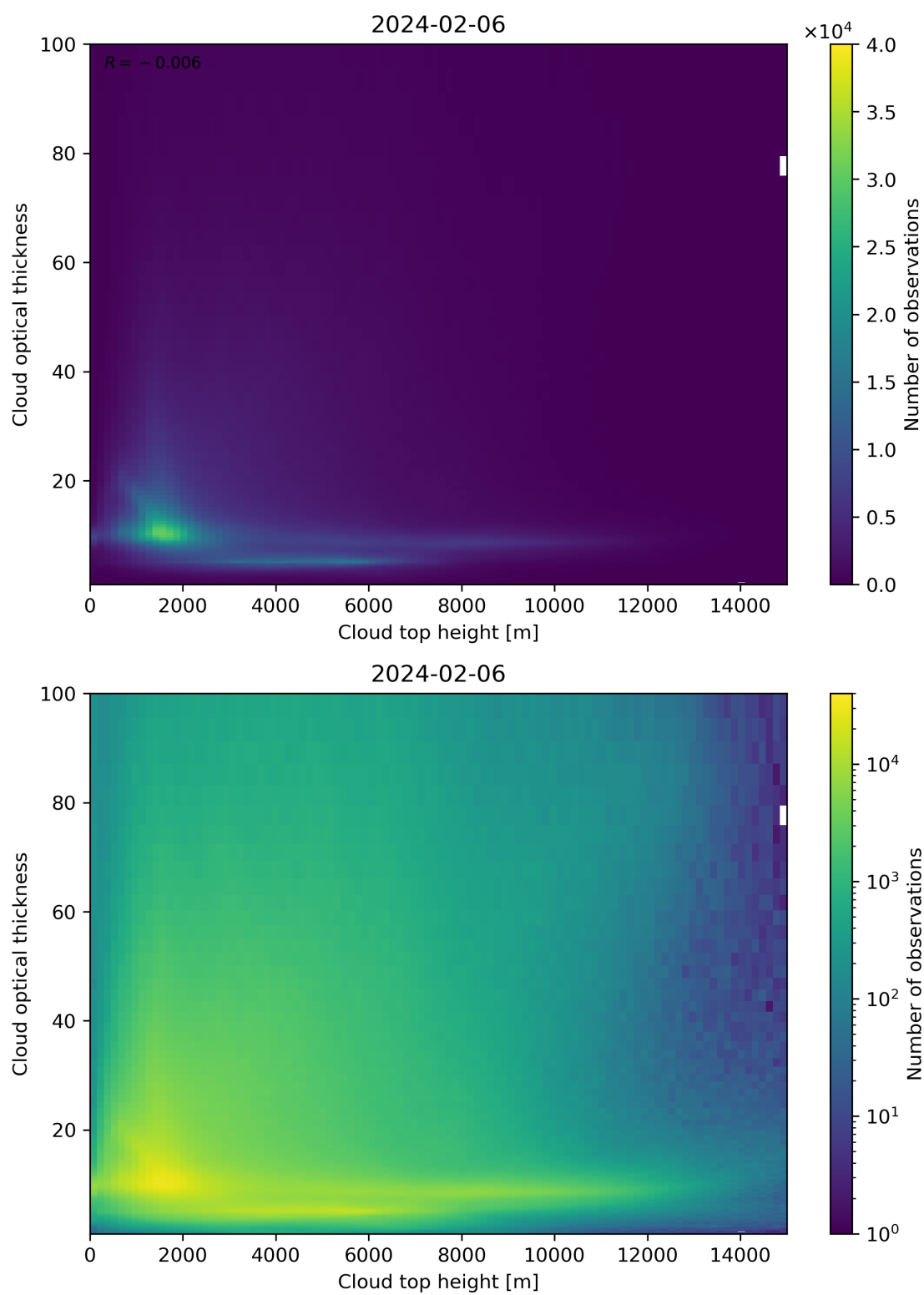
Figure 90: Scatter density plot of “Cloud top height” against “Cloud optical thickness” for 2024-02-06 to 2024-02-07.
