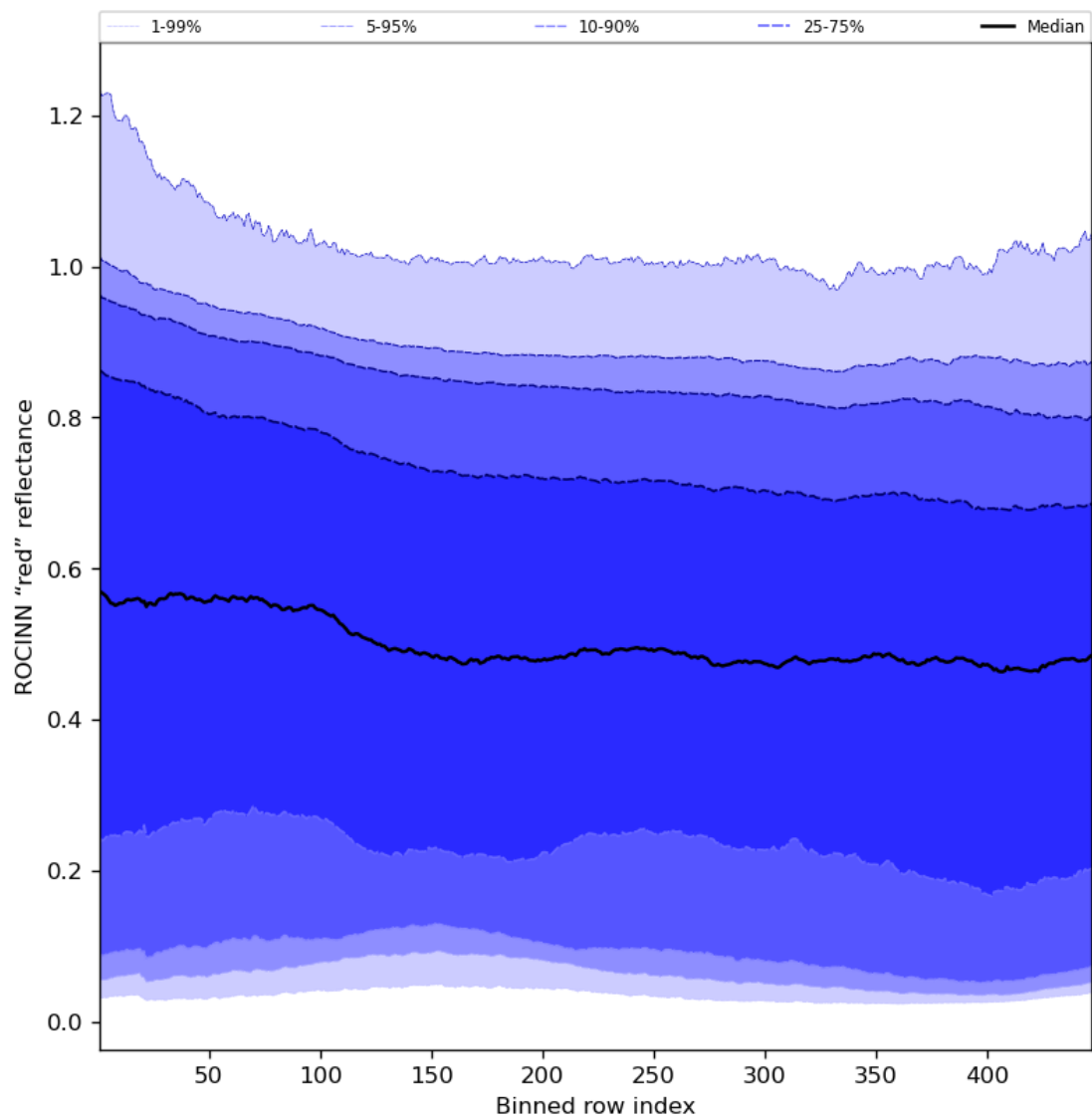
Figure 69: Along track statistics of “ROCINN “red” reflectance” for 2024-02-06 to 2024-02-07
