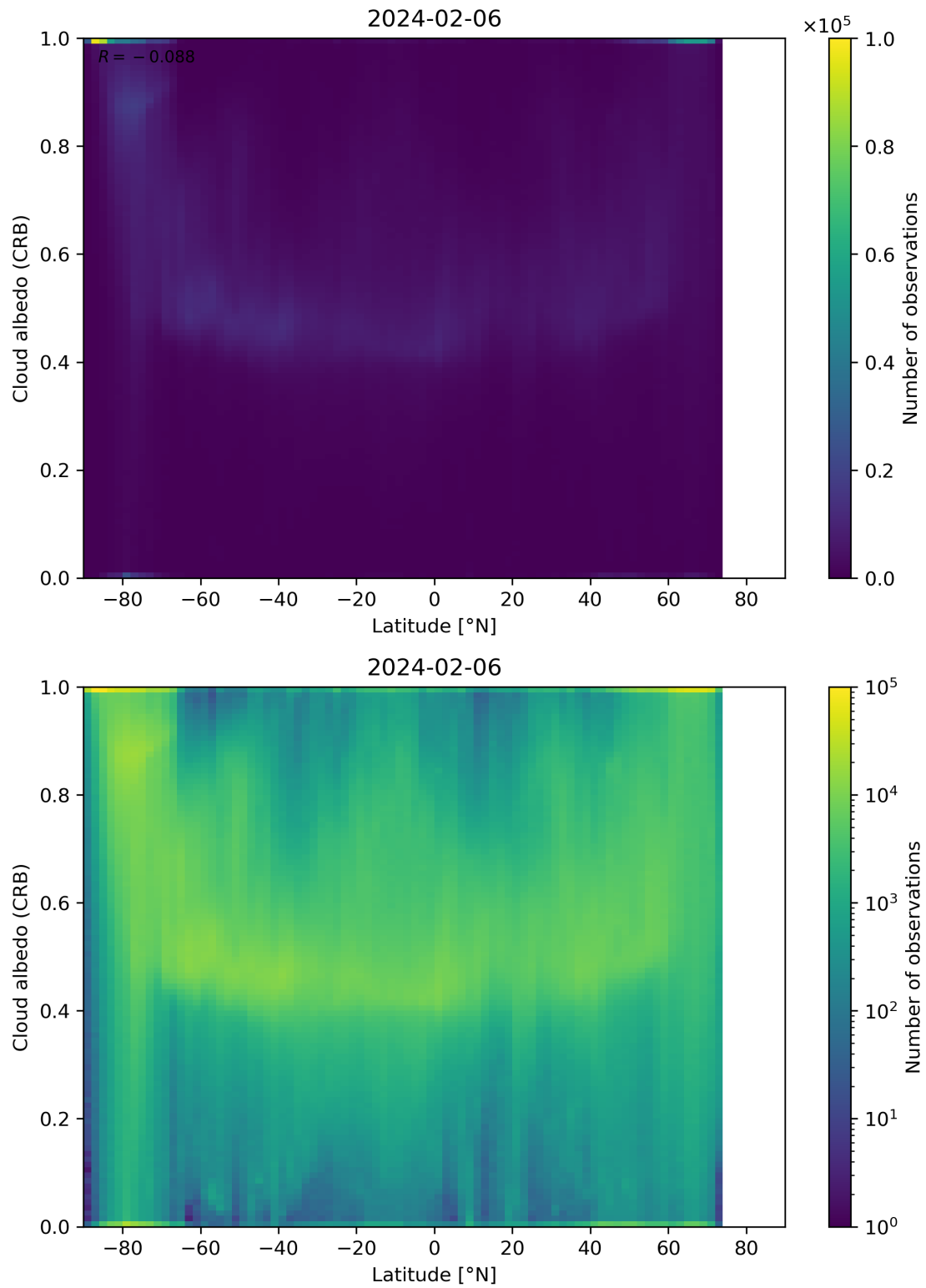
Figure 91: Scatter density plot of “Latitude” against “Cloud albedo (CRB)” for 2024-02-06 to 2024-02-07.
