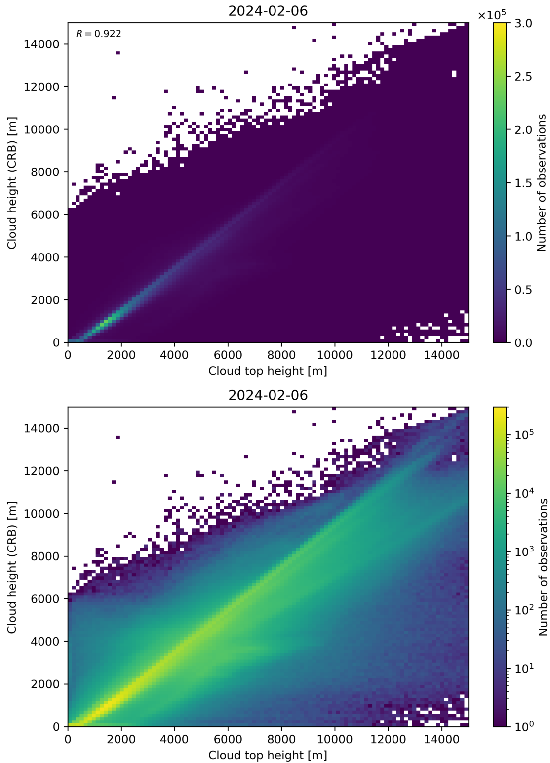
Figure 89: Scatter density plot of “Cloud top height” against “Cloud height (CRB)” for 2024-02-06 to 2024-02-07.
