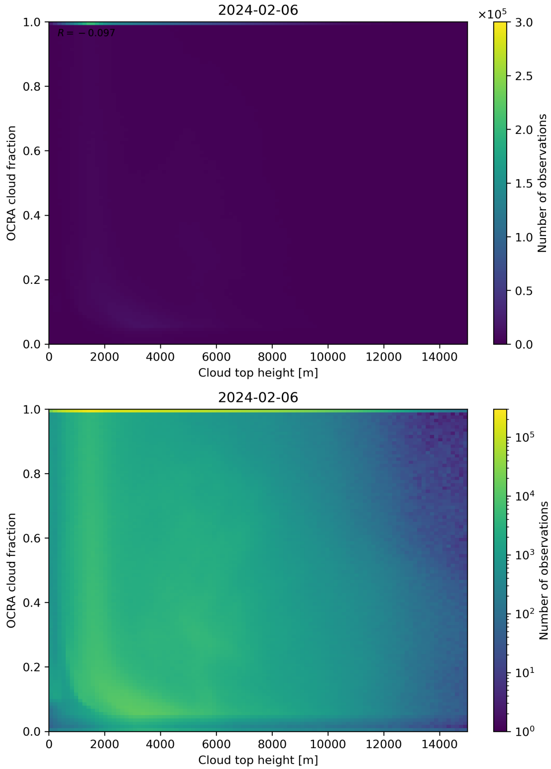
Figure 87: Scatter density plot of “Cloud top height” against “OCRA cloud fraction” for 2024-02-06 to 2024-02-07.
