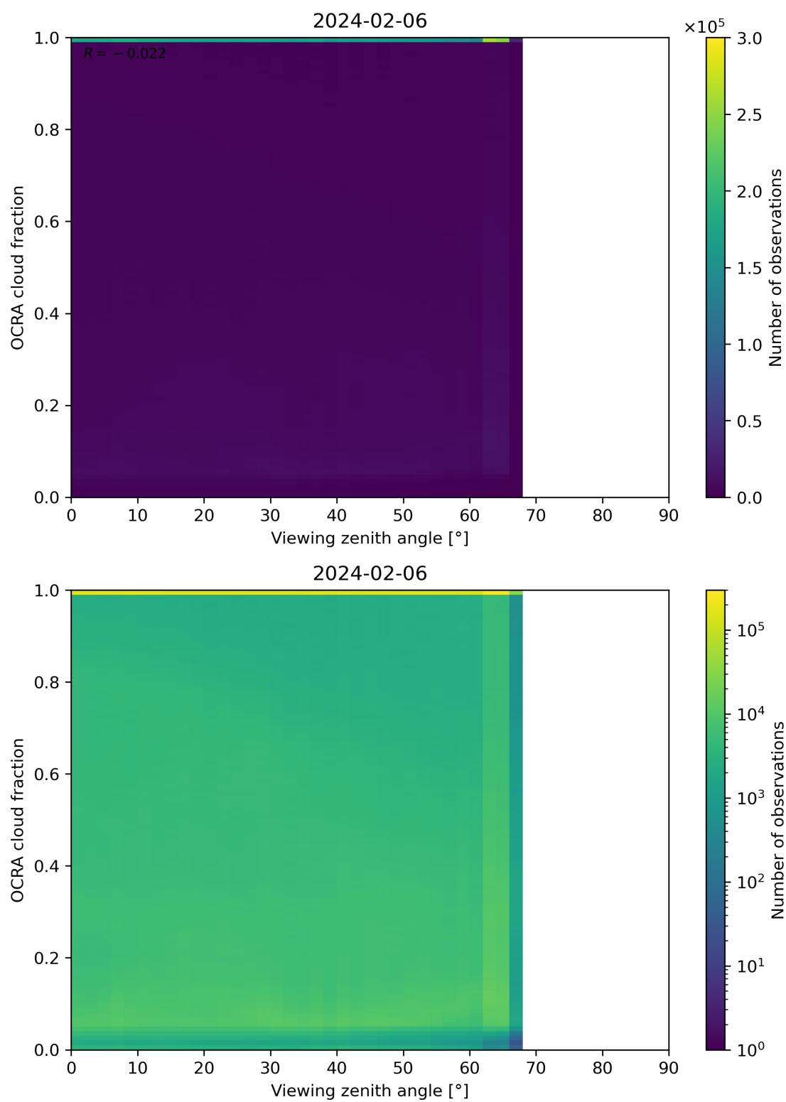
Figure 108: Scatter density plot of “Viewing zenith angle” against “OCRA cloud fraction” for 2024-02-06 to 2024-02-07.
