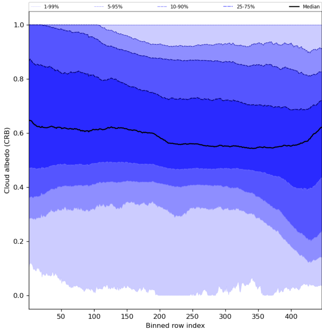
Figure 60: Along track statistics of “Cloud albedo (CRB)” for 2024-02-06 to 2024-02-07
