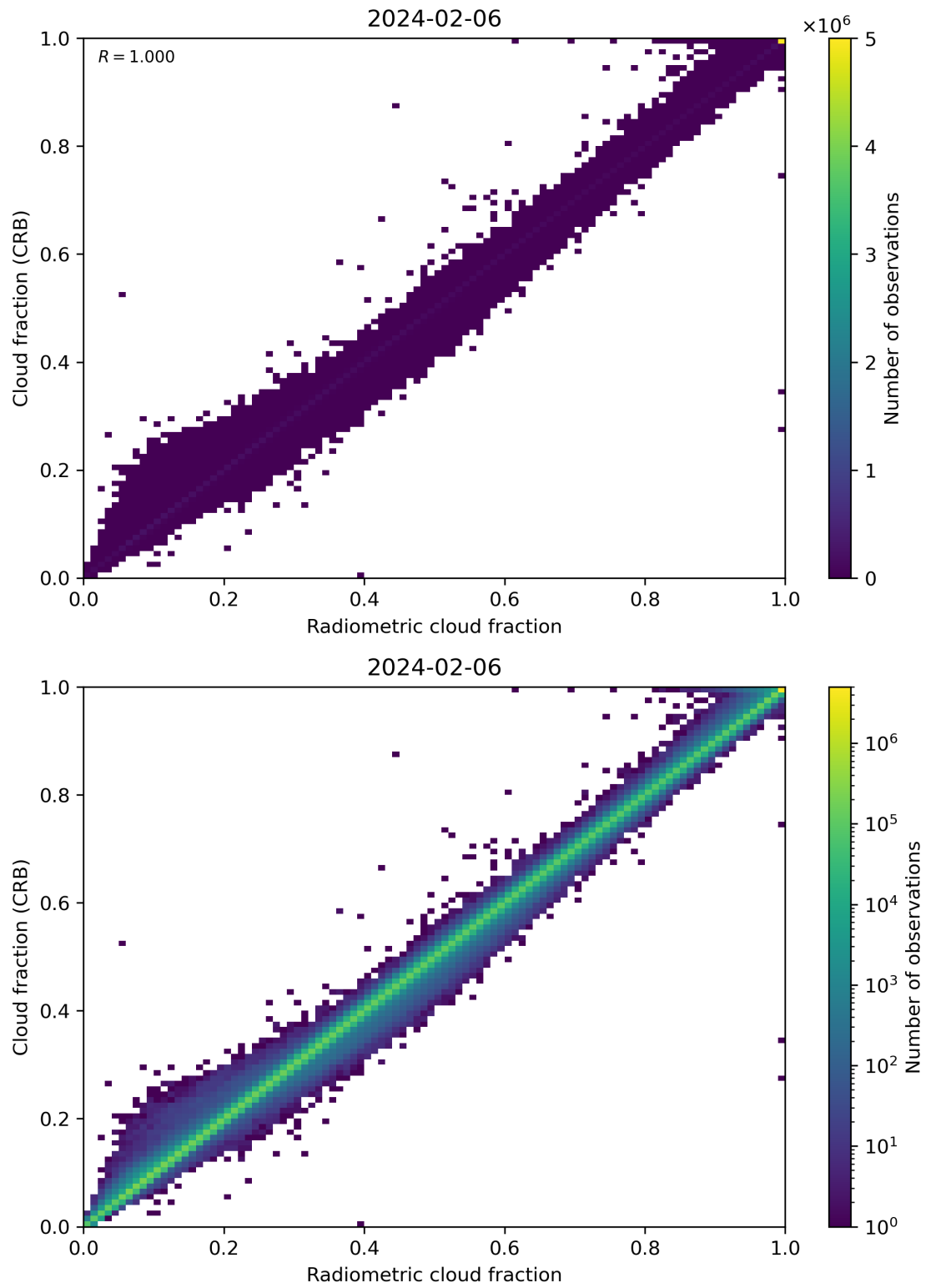
Figure 73: Scatter density plot of “Radiometric cloud fraction” against “Cloud fraction (CRB)” for 2024-02-06 to 2024-02-07.
