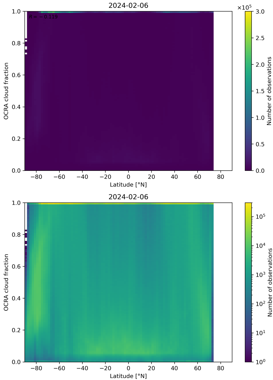
Figure 93: Scatter density plot of “Latitude” against “OCRA cloud fraction” for 2024-02-06 to 2024-02-07.
