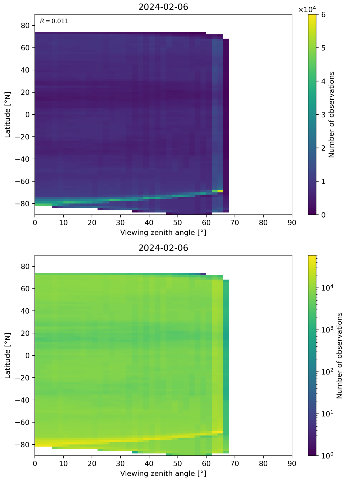
Figure 113: Scatter density plot of “Viewing zenith angle” against “Latitude” for 2024-02-06 to 2024-02-07.
