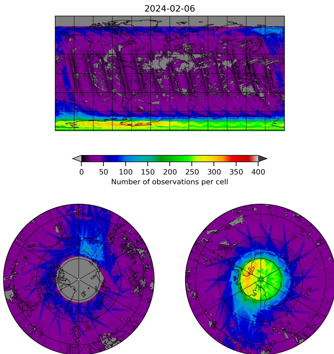
Figure 21: Map of the number of observations for 2024-02-06 to 2024-02-07
