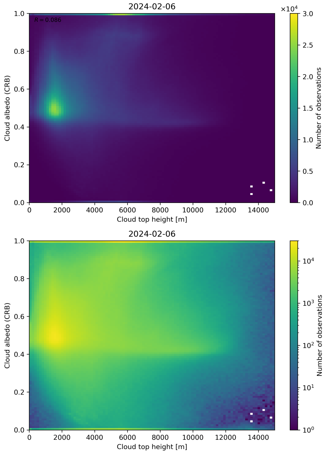
Figure 86: Scatter density plot of “Cloud top height” against “Cloud albedo (CRB)” for 2024-02-06 to 2024-02-07.
