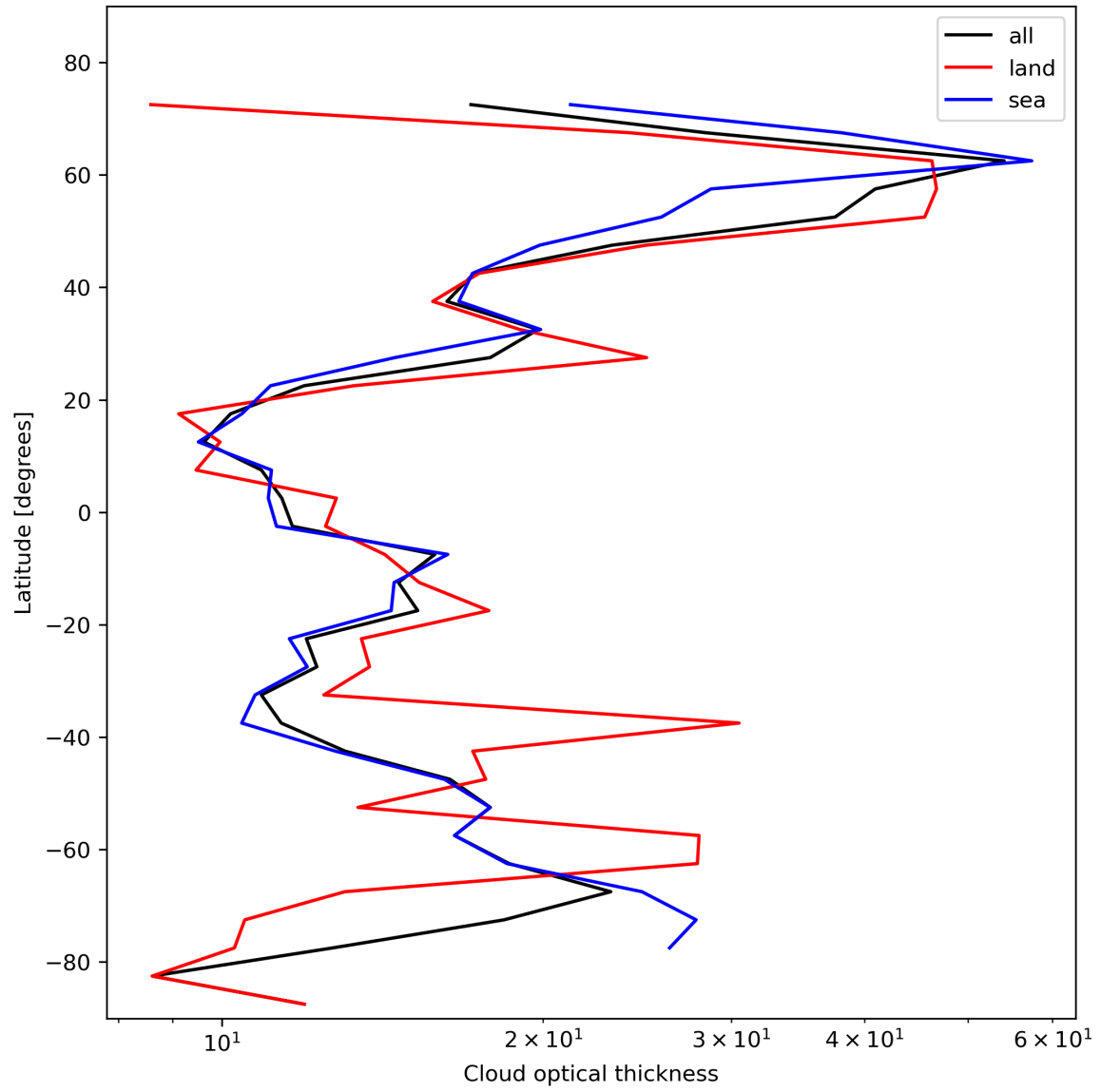
Figure 25: Zonal average of “Cloud optical thickness” for 2024-02-06 to 2024-02-07.
