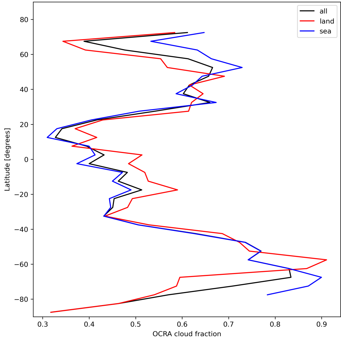
Figure 34: Zonal average of “OCRA cloud fraction” for 2024-02-06 to 2024-02-07.
