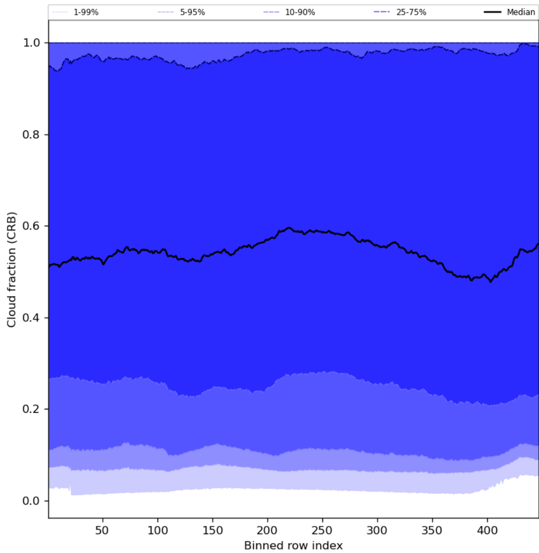
Figure 58: Along track statistics of “Cloud fraction (CRB)” for 2024-02-06 to 2024-02-07
