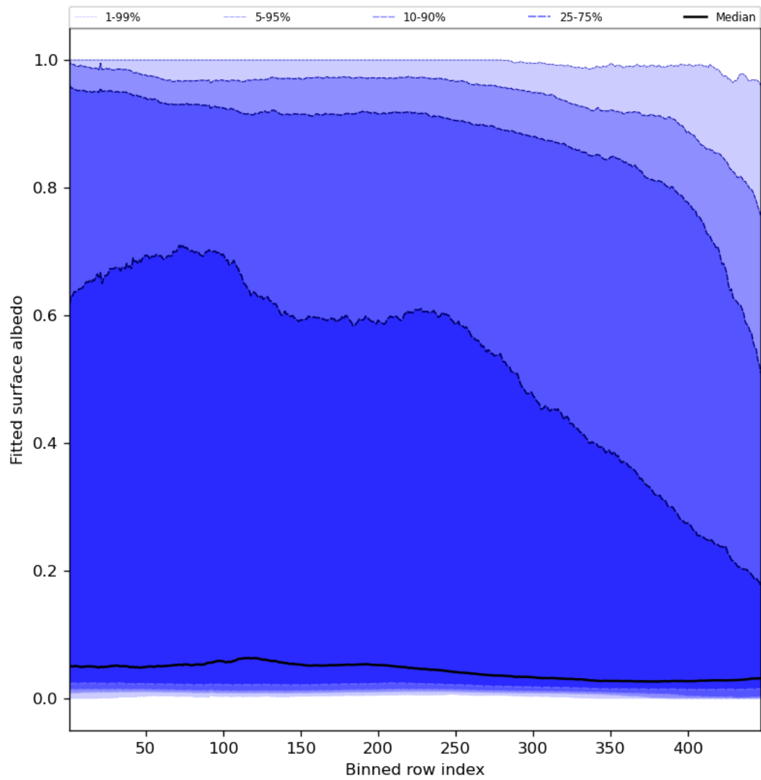
Figure 61: Along track statistics of “Fitted surface albedo” for 2024-02-06 to 2024-02-07
