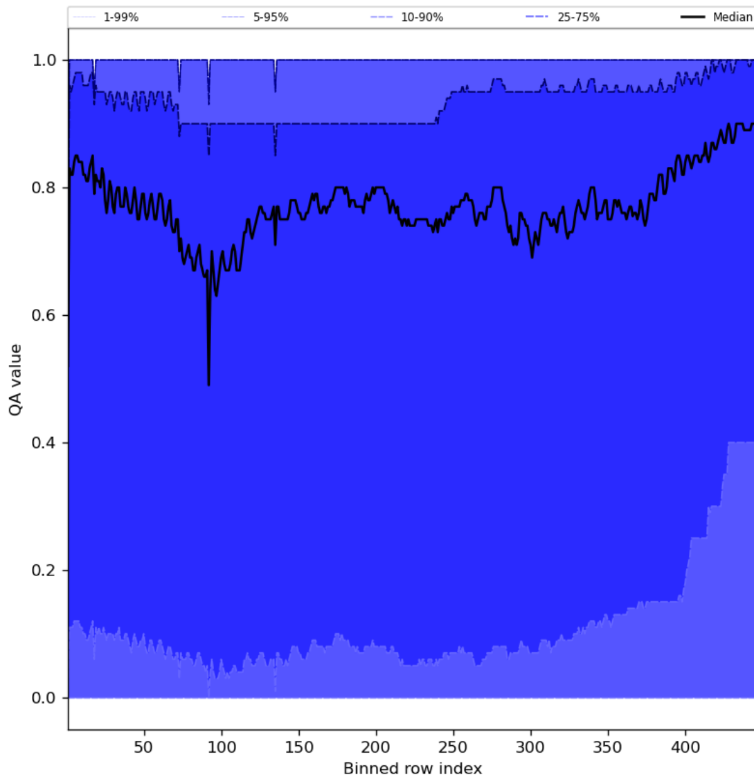
Figure 54: Along track statistics of “QA value” for 2024-02-06 to 2024-02-07
