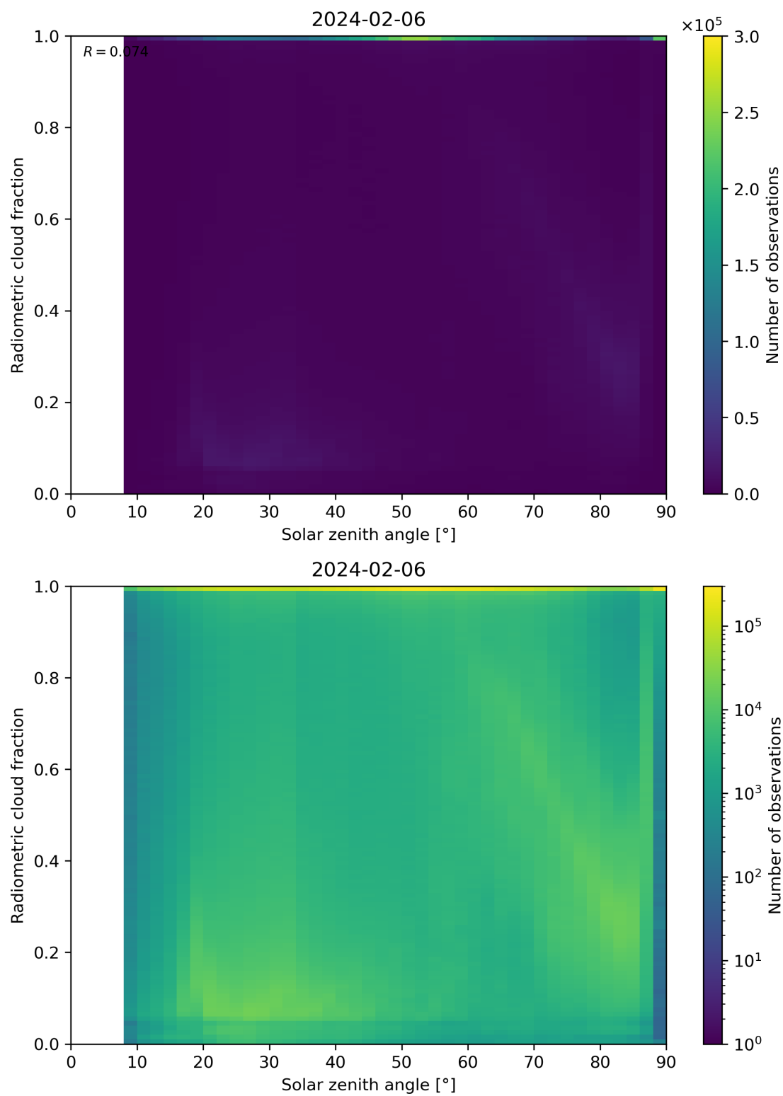
Figure 99: Scatter density plot of “Solar zenith angle” against “Radiometric cloud fraction” for 2024-02-06 to 2024-02-07.
