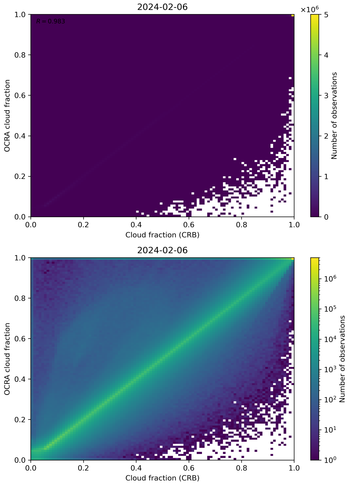
Figure 78: Scatter density plot of “Cloud fraction (CRB)” against “OCRA cloud fraction” for 2024-02-06 to 2024-02-07.
