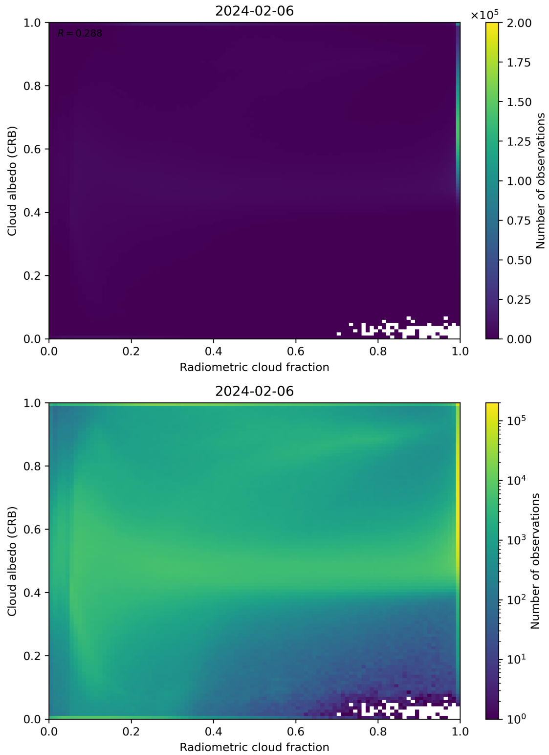
Figure 71: Scatter density plot of “Radiometric cloud fraction” against “Cloud albedo (CRB)” for 2024-02-06 to 2024-02-07.
