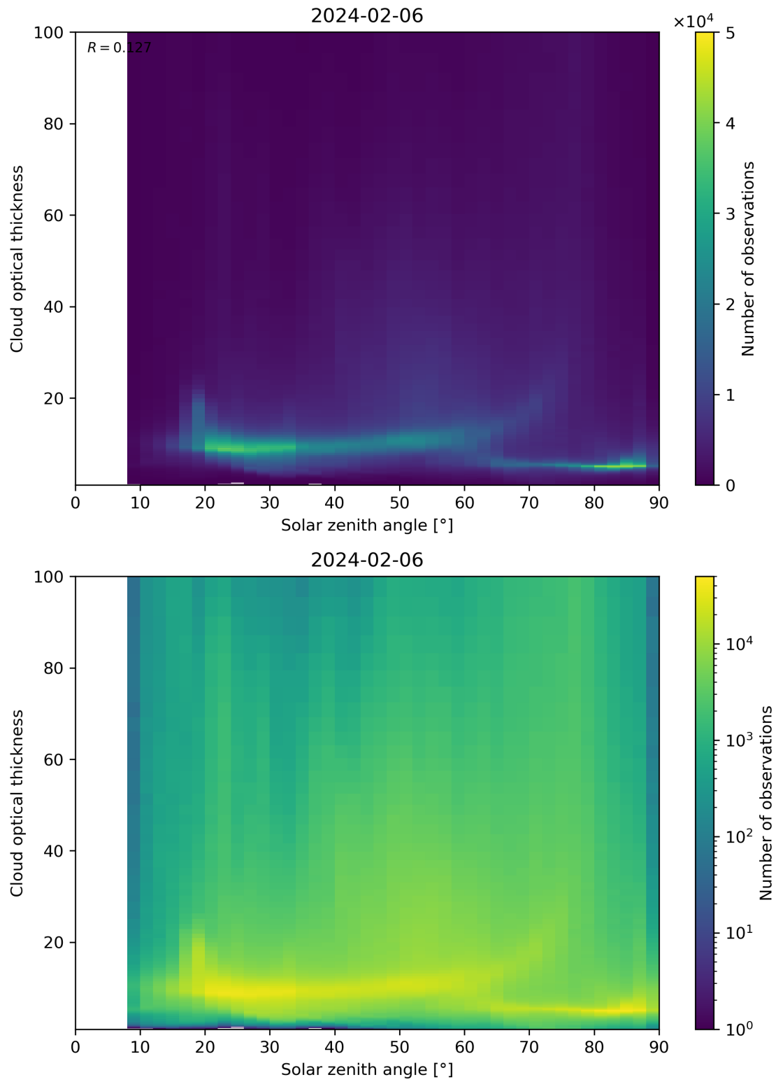
Figure 103: Scatter density plot of “Solar zenith angle” against “Cloud optical thickness” for 2024-02-06 to 2024-02-07.
