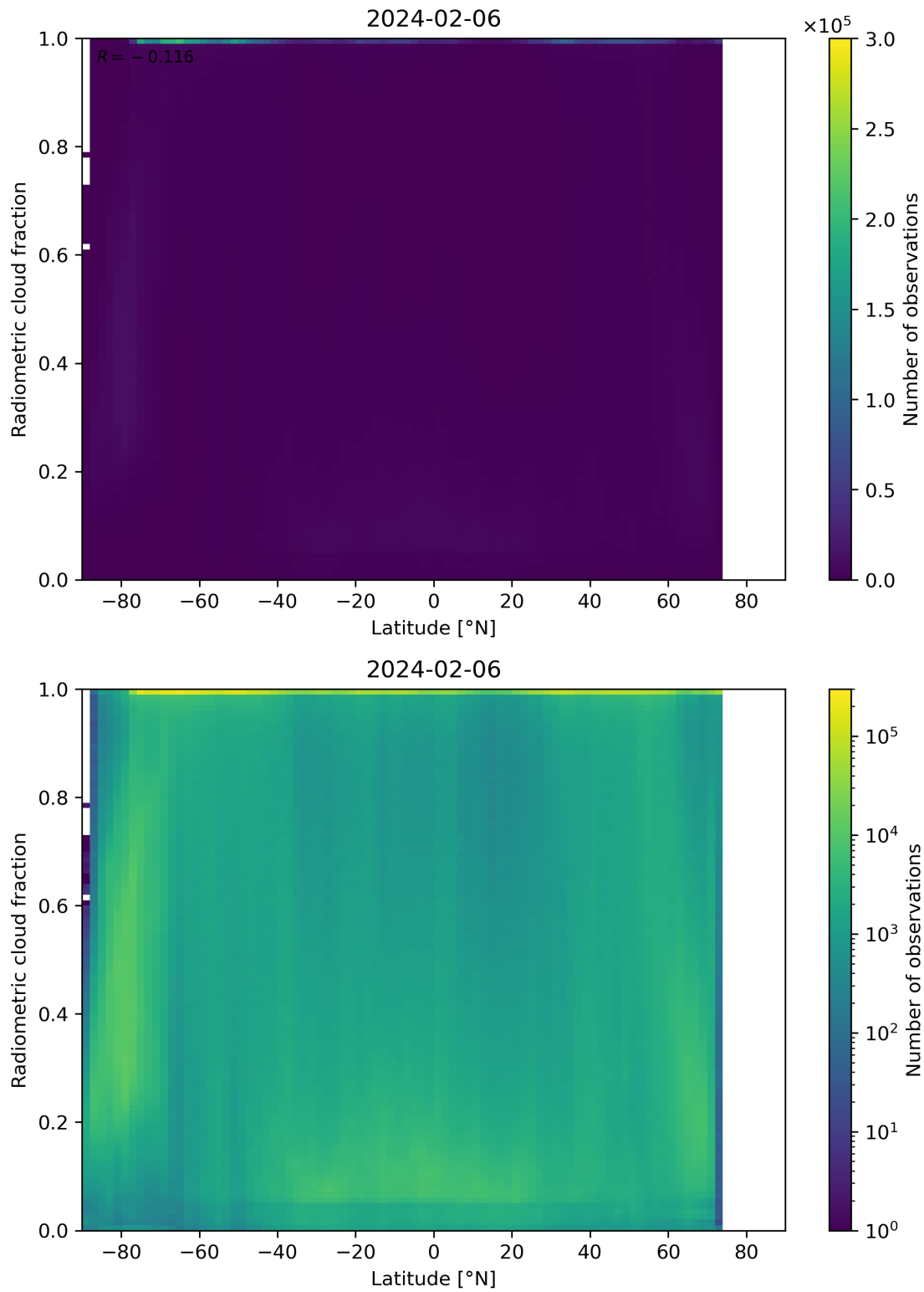
Figure 92: Scatter density plot of “Latitude” against “Radiometric cloud fraction” for 2024-02-06 to 2024-02-07.
