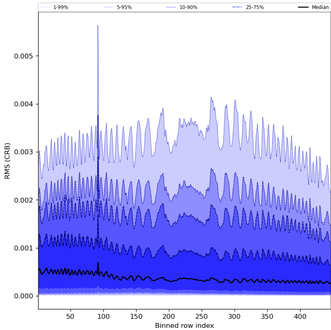
Figure 64: Along track statistics of “RMS (CRB)” for 2024-02-06 to 2024-02-07
