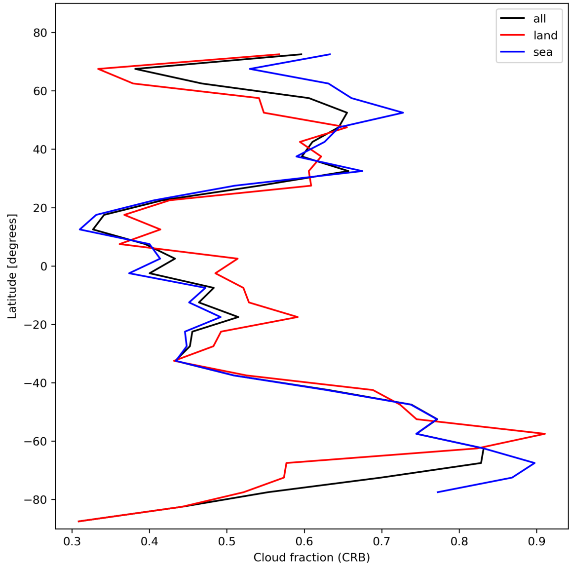
Figure 26: Zonal average of “Cloud fraction (CRB)” for 2024-02-06 to 2024-02-07.
