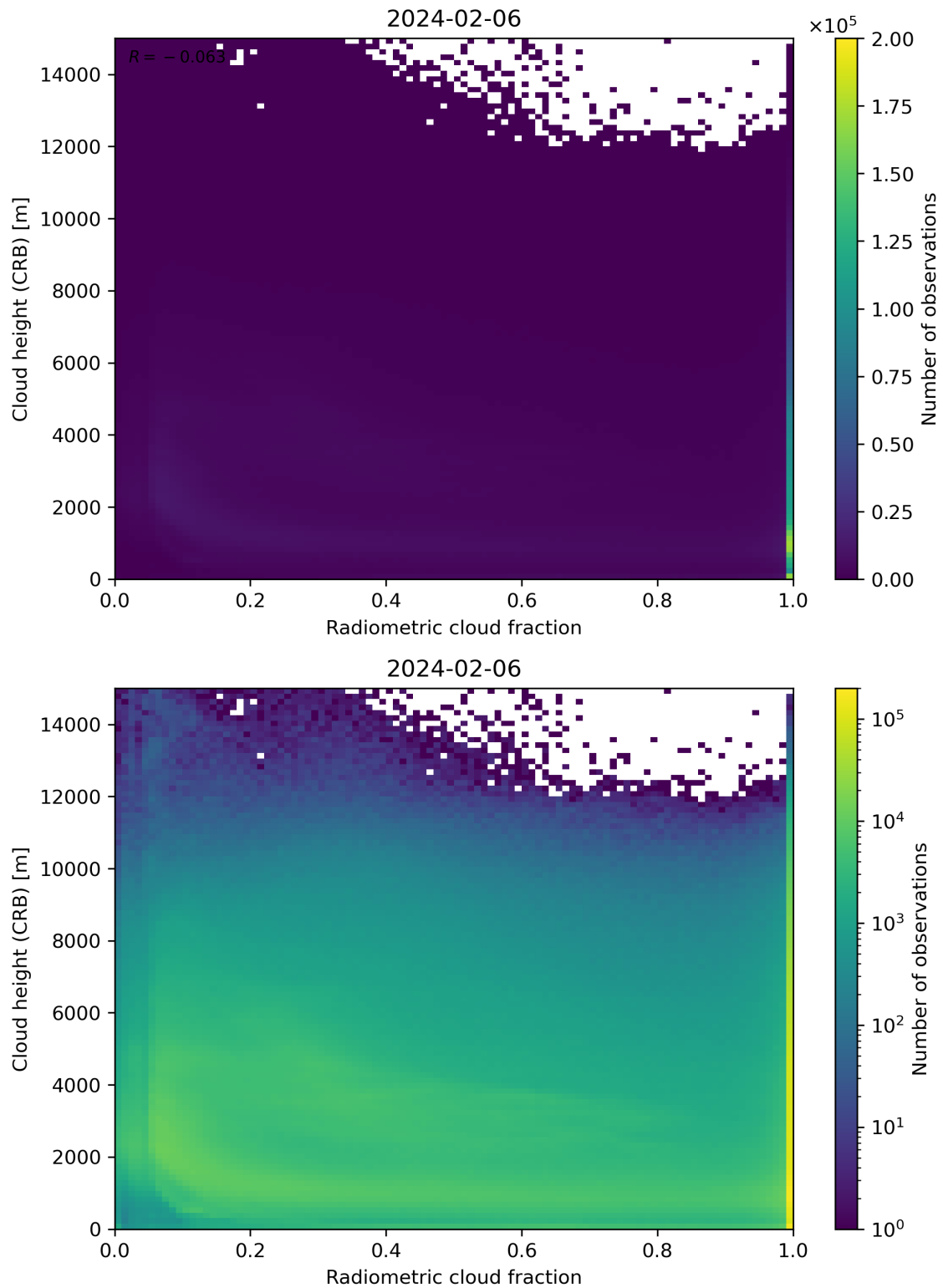
Figure 74: Scatter density plot of “Radiometric cloud fraction” against “Cloud height (CRB)” for 2024-02-06 to 2024-02-07.
