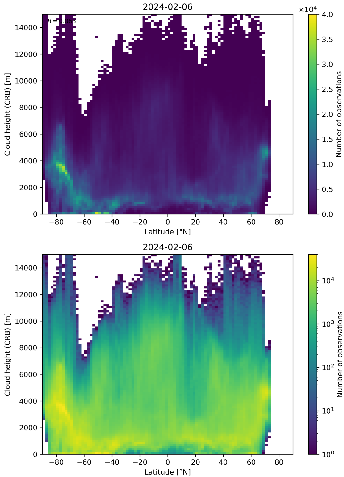
Figure 95: Scatter density plot of “Latitude” against “Cloud height (CRB)” for 2024-02-06 to 2024-02-07.
