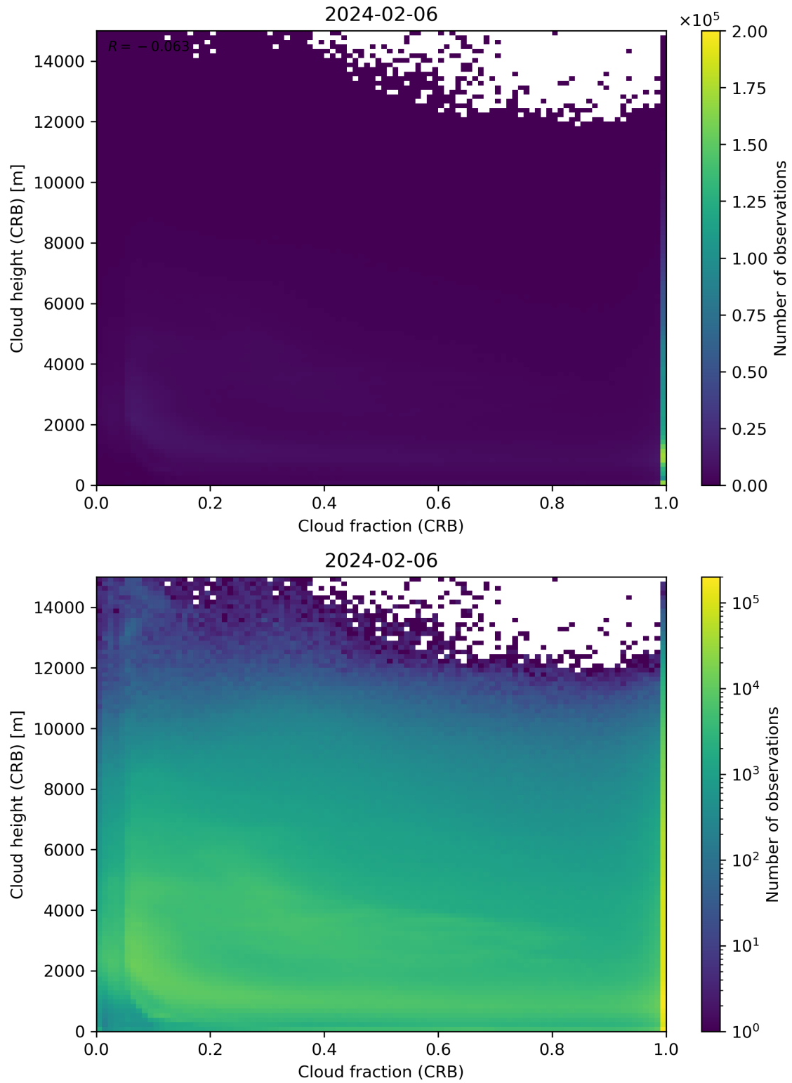
Figure 79: Scatter density plot of “Cloud fraction (CRB)” against “Cloud height (CRB)” for 2024-02-06 to 2024-02-07.
