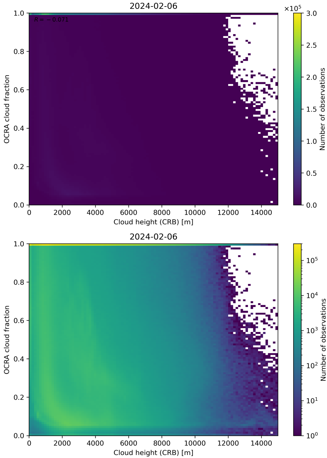
Figure 81: Scatter density plot of “Cloud height (CRB)” against “OCRA cloud fraction” for 2024-02-06 to 2024-02-07.
