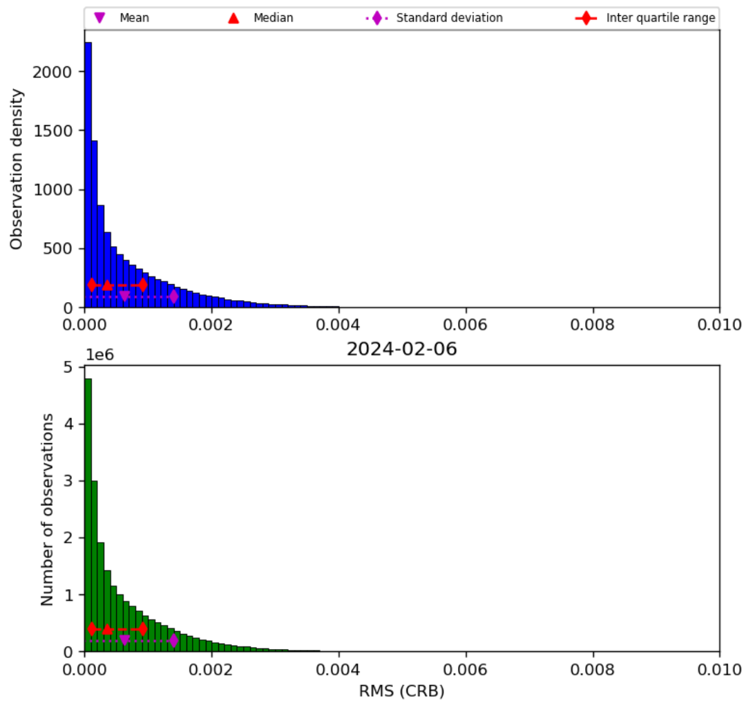
Figure 48: Histogram of "RMS (CRB)" for 2024-02-06 to 2024-02-07
