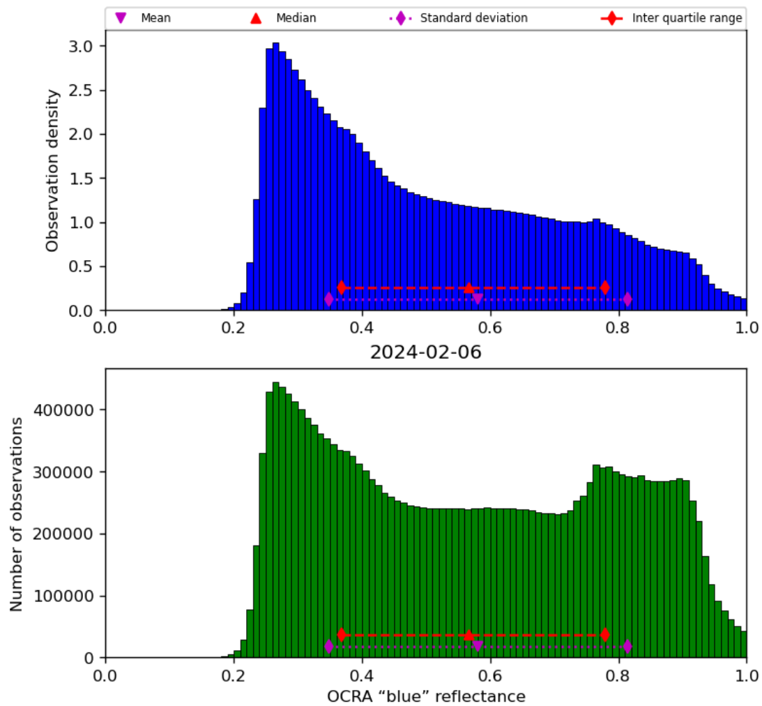
Figure 51: Histogram of “OCRA “blue” reflectance” for 2024-02-06 to 2024-02-07
