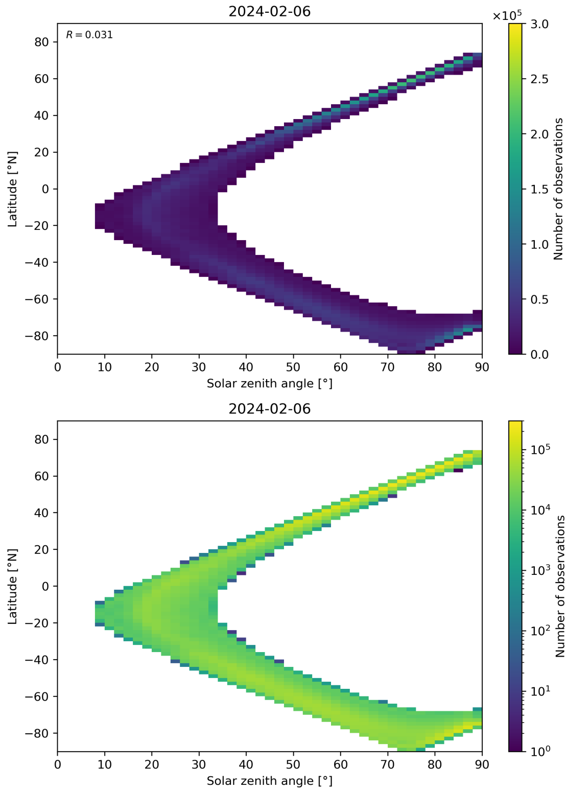
Figure 105: Scatter density plot of “Solar zenith angle” against “Latitude” for 2024-02-06 to 2024-02-07.
