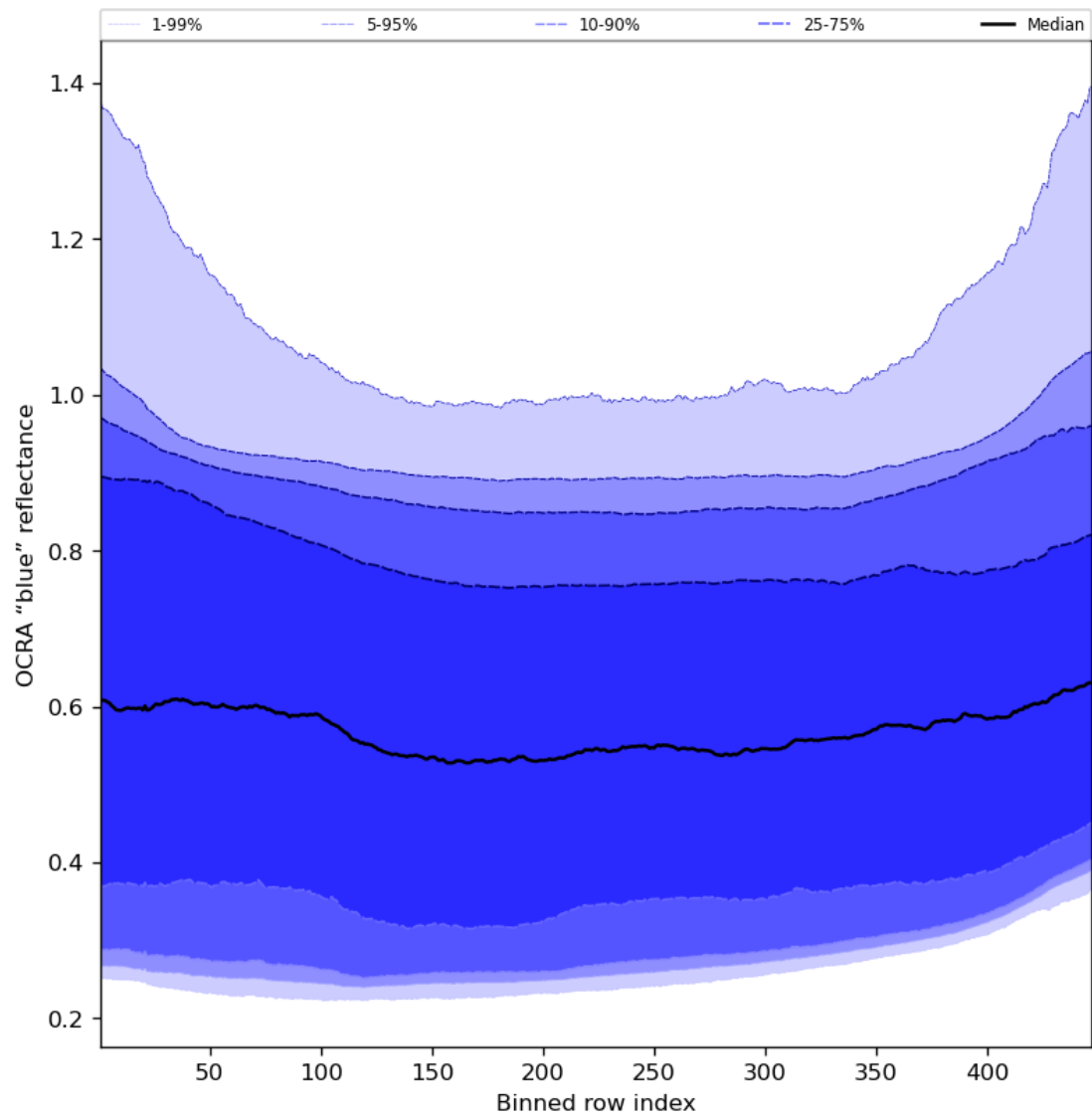
Figure 67: Along track statistics of “OCRA “blue” reflectance” for 2024-02-06 to 2024-02-07
