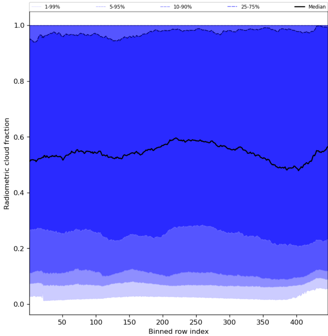
Figure 55: Along track statistics of “Radiometric cloud fraction” for 2024-02-06 to 2024-02-07
