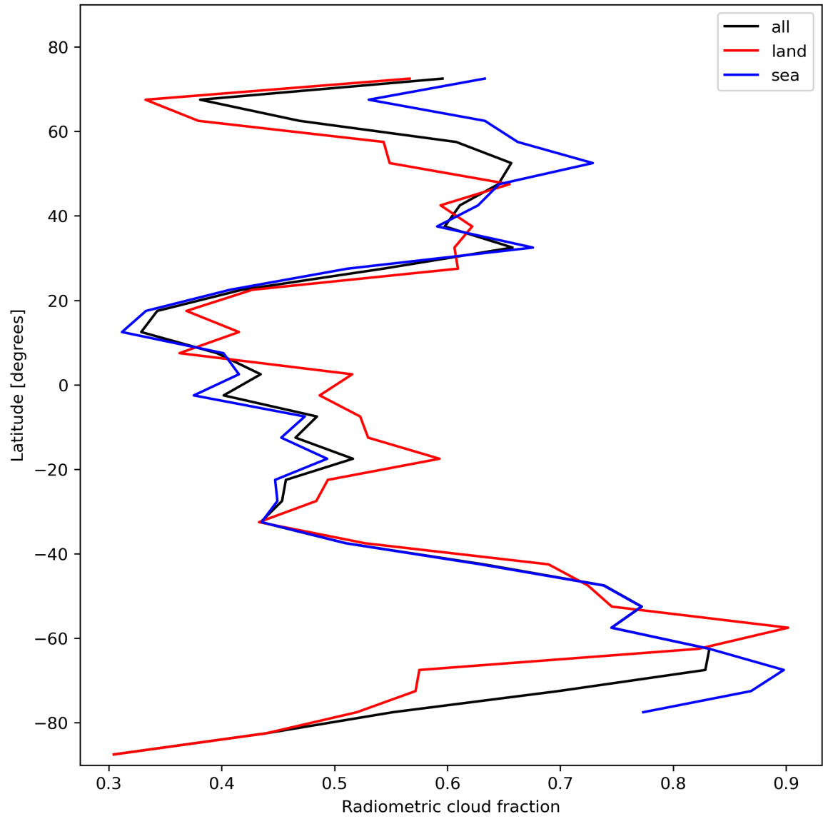
Figure 23: Zonal average of “Radiometric cloud fraction” for 2024-02-06 to 2024-02-07.
