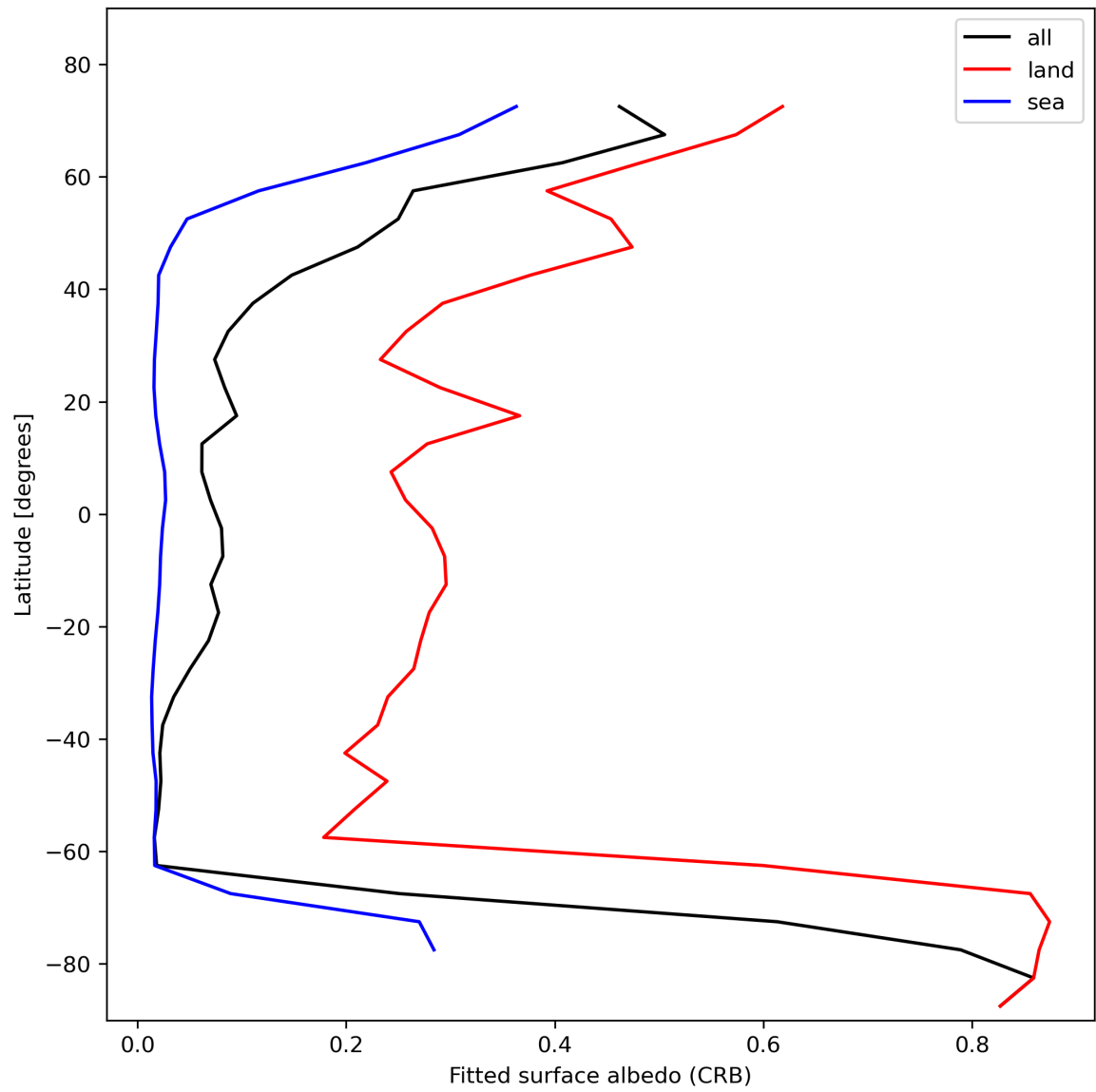
Figure 30: Zonal average of “Fitted surface albedo (CRB)” for 2024-02-06 to 2024-02-07.
