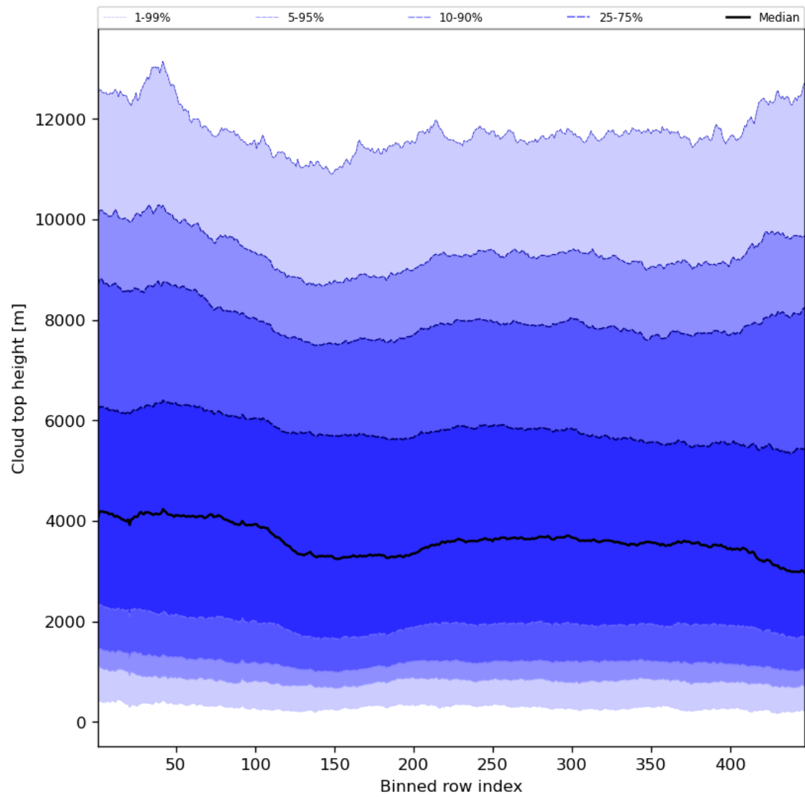
Figure 56: Along track statistics of “Cloud top height” for 2024-02-06 to 2024-02-07
