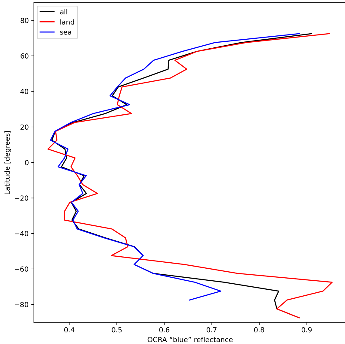
Figure 35: Zonal average of “OCRA “blue” reflectance” for 2024-02-06 to 2024-02-07.
