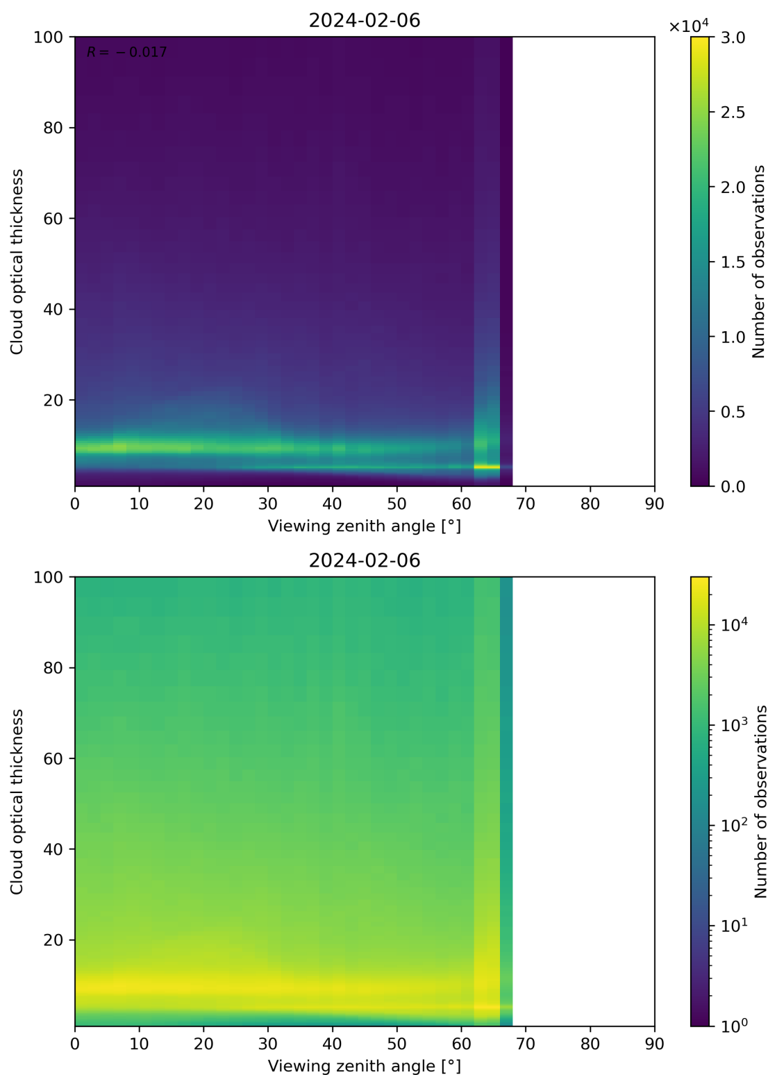
Figure 111: Scatter density plot of “Viewing zenith angle” against “Cloud optical thickness” for 2024-02-06 to 2024-02-07.
