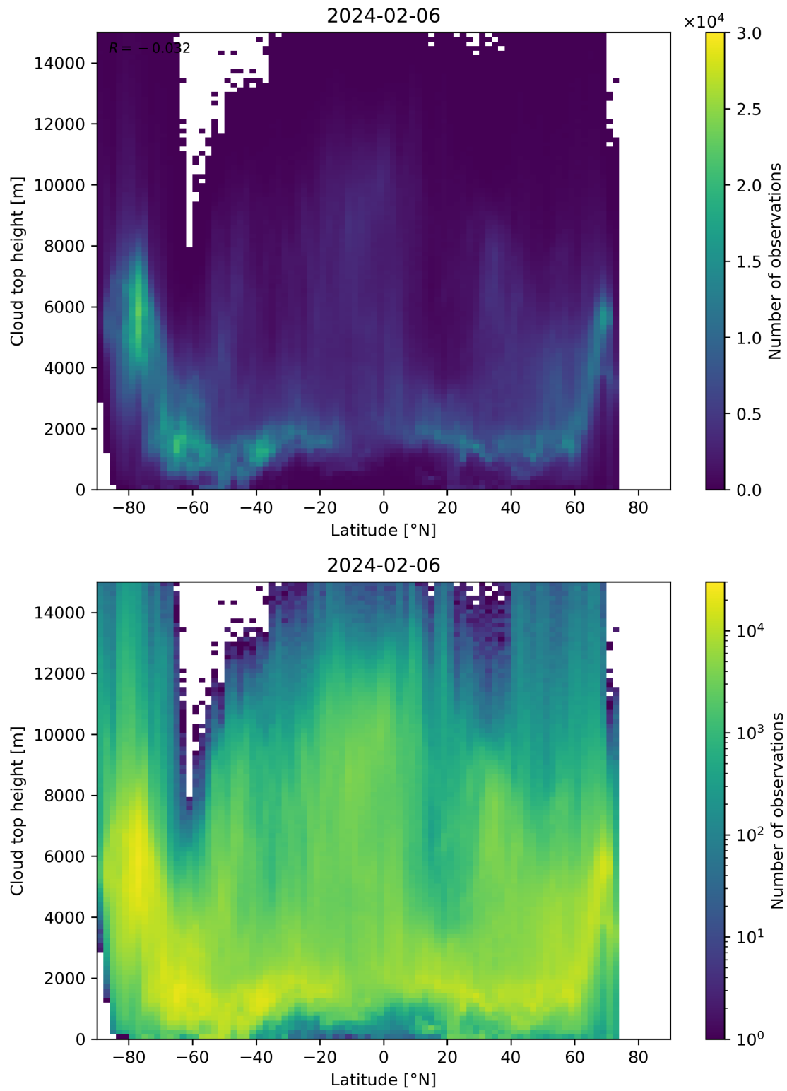
Figure 97: Scatter density plot of “Latitude” against “Cloud top height” for 2024-02-06 to 2024-02-07.
