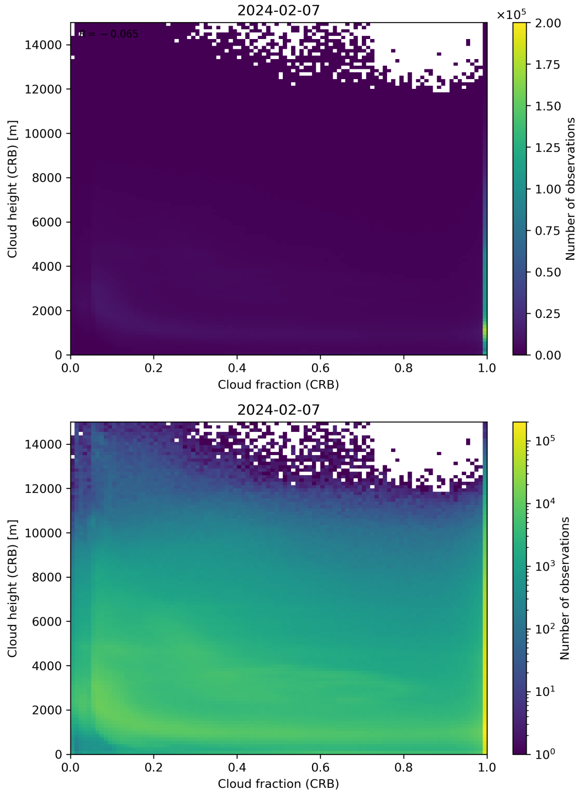
Figure 79: Scatter density plot of “Cloud fraction (CRB)” against “Cloud height (CRB)” for 2024-02-06 to 2024-02-08.
