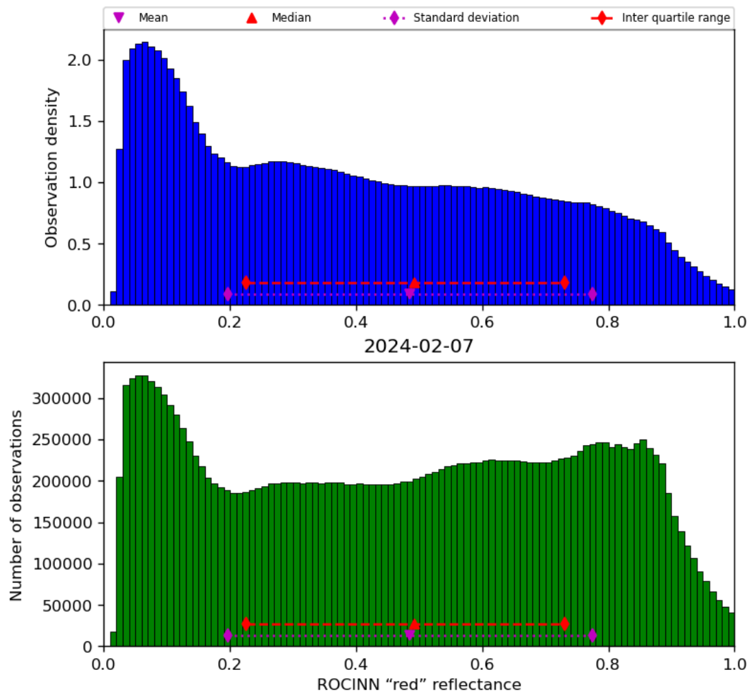
Figure 53: Histogram of “ROCINN “red” reflectance” for 2024-02-06 to 2024-02-08
