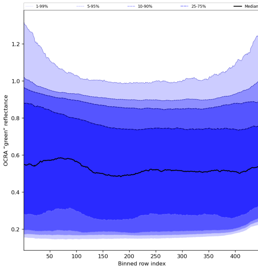
Figure 68: Along track statistics of "OCRA "green" reflectance" for 2024-02-06 to 2024-02-08
