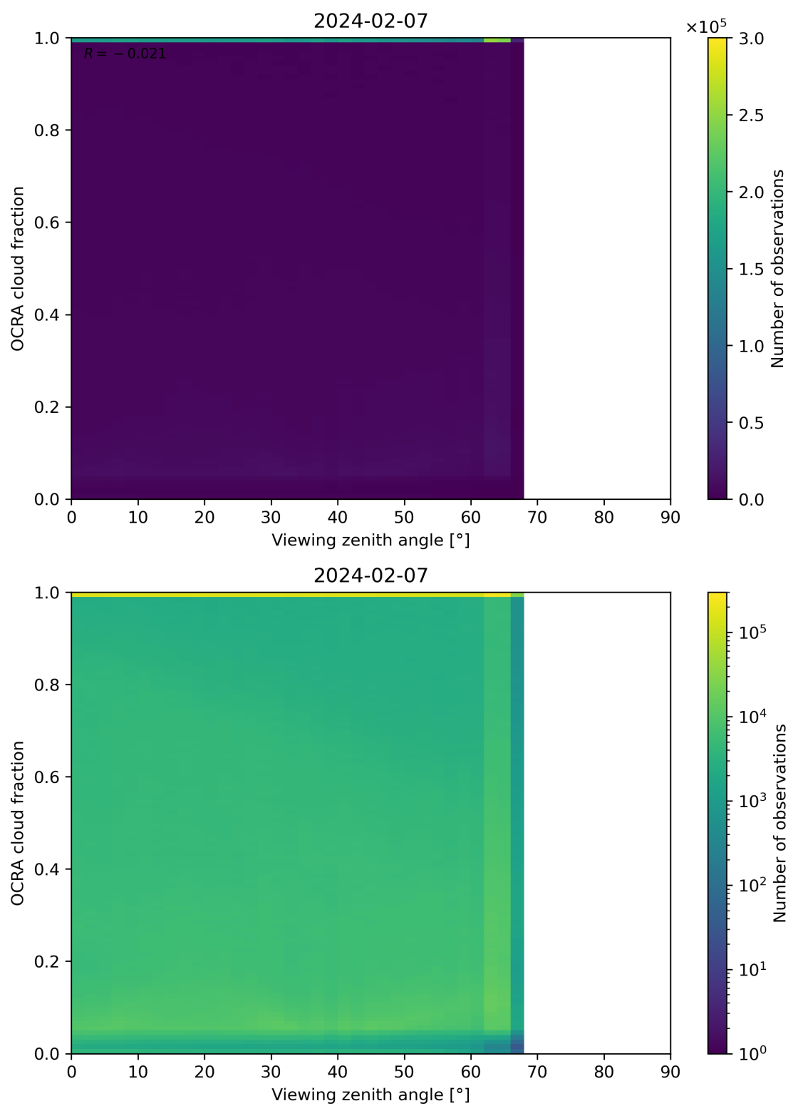
Figure 108: Scatter density plot of “Viewing zenith angle” against “OCRA cloud fraction” for 2024-02-06 to 2024-02-08.
