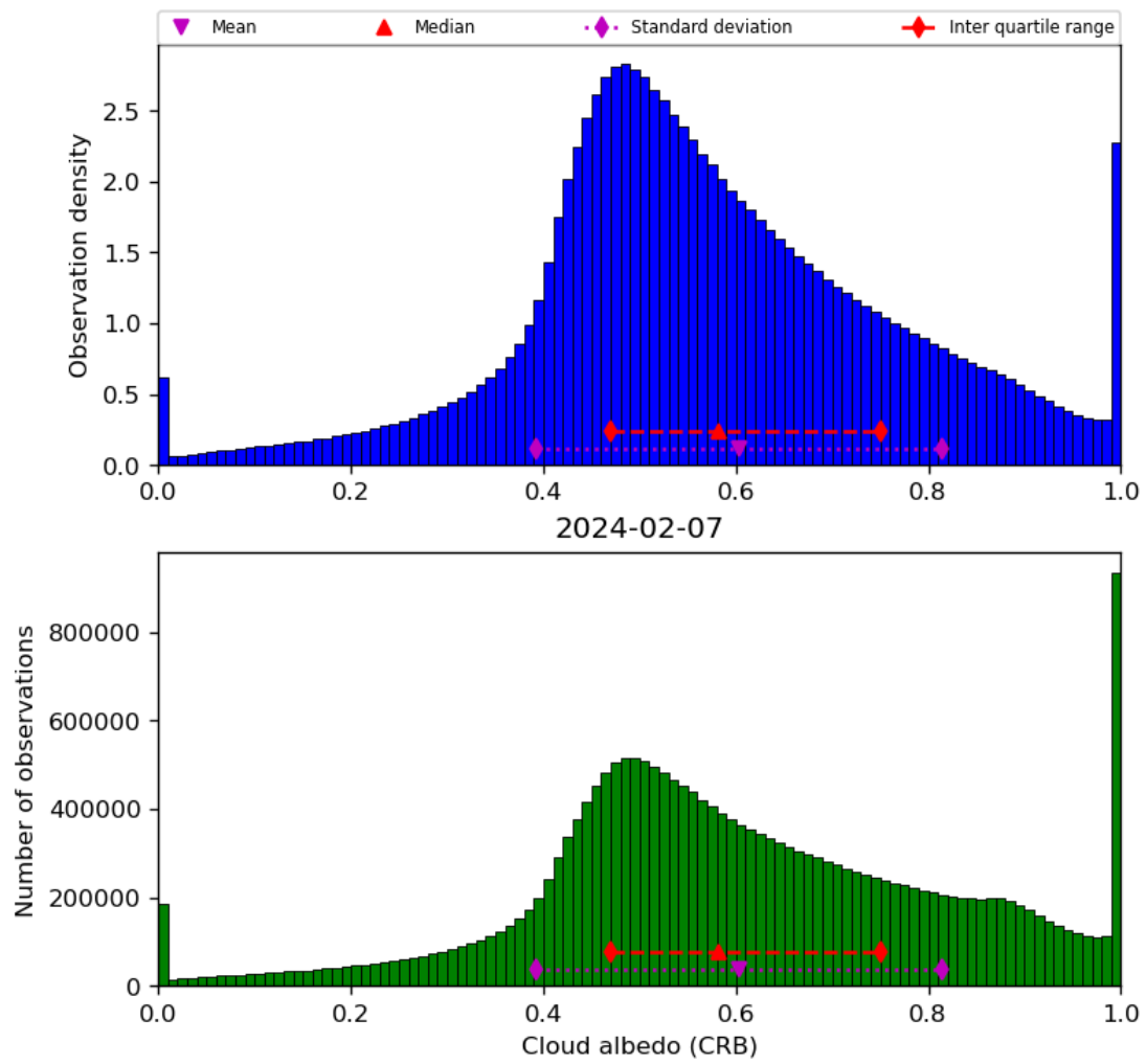
Figure 44: Histogram of “Cloud albedo (CRB)” for 2024-02-06 to 2024-02-08
