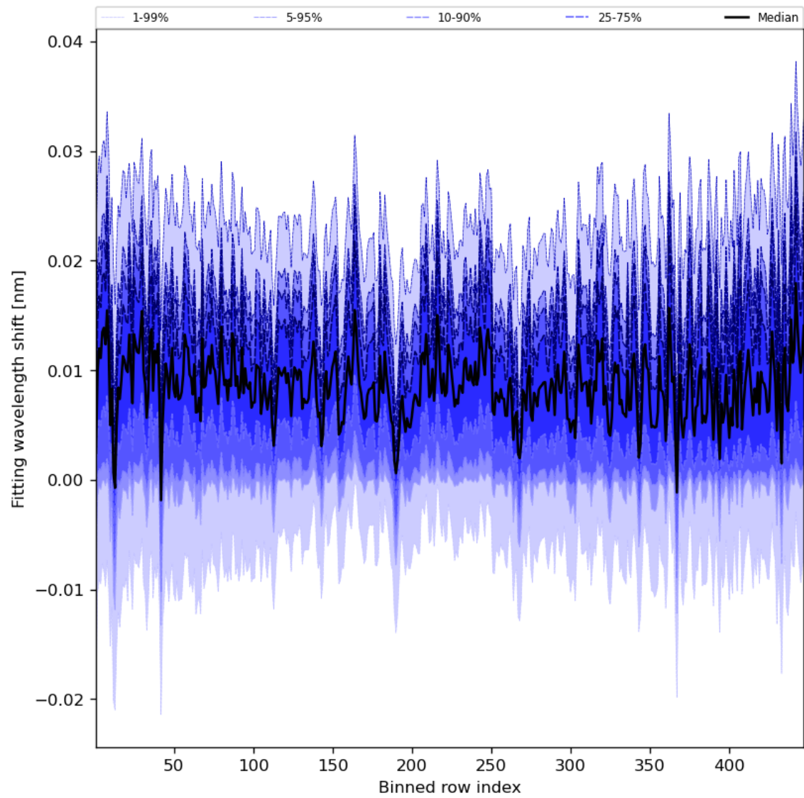
Figure 65: Along track statistics of “Fitting wavelength shift” for 2024-02-06 to 2024-02-08
