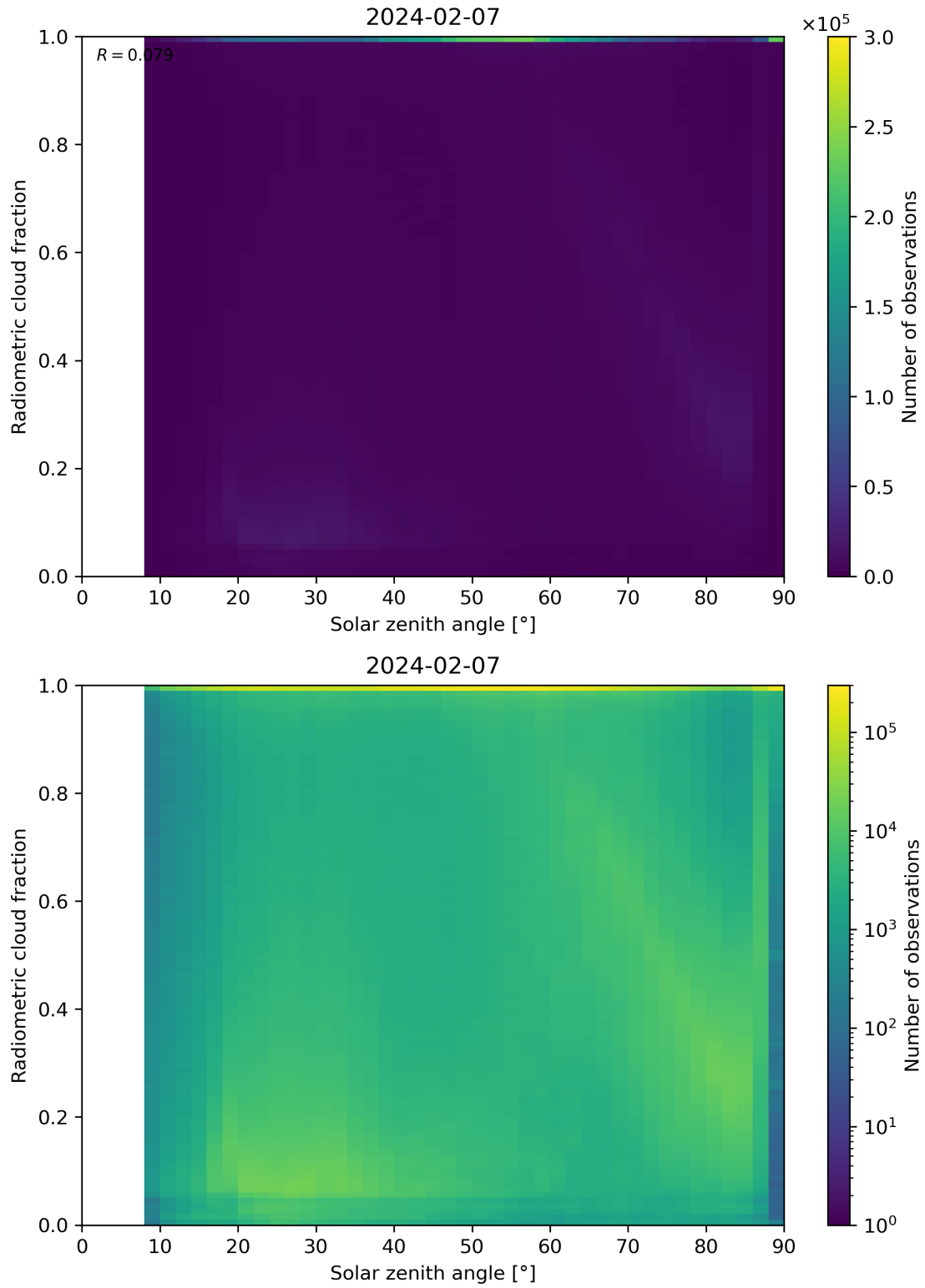
Figure 99: Scatter density plot of “Solar zenith angle” against “Radiometric cloud fraction” for 2024-02-06 to 2024-02-08.
