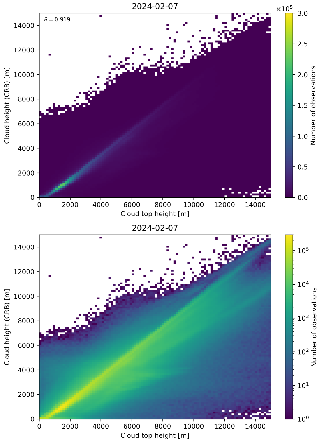
Figure 89: Scatter density plot of “Cloud top height” against “Cloud height (CRB)” for 2024-02-06 to 2024-02-08.
