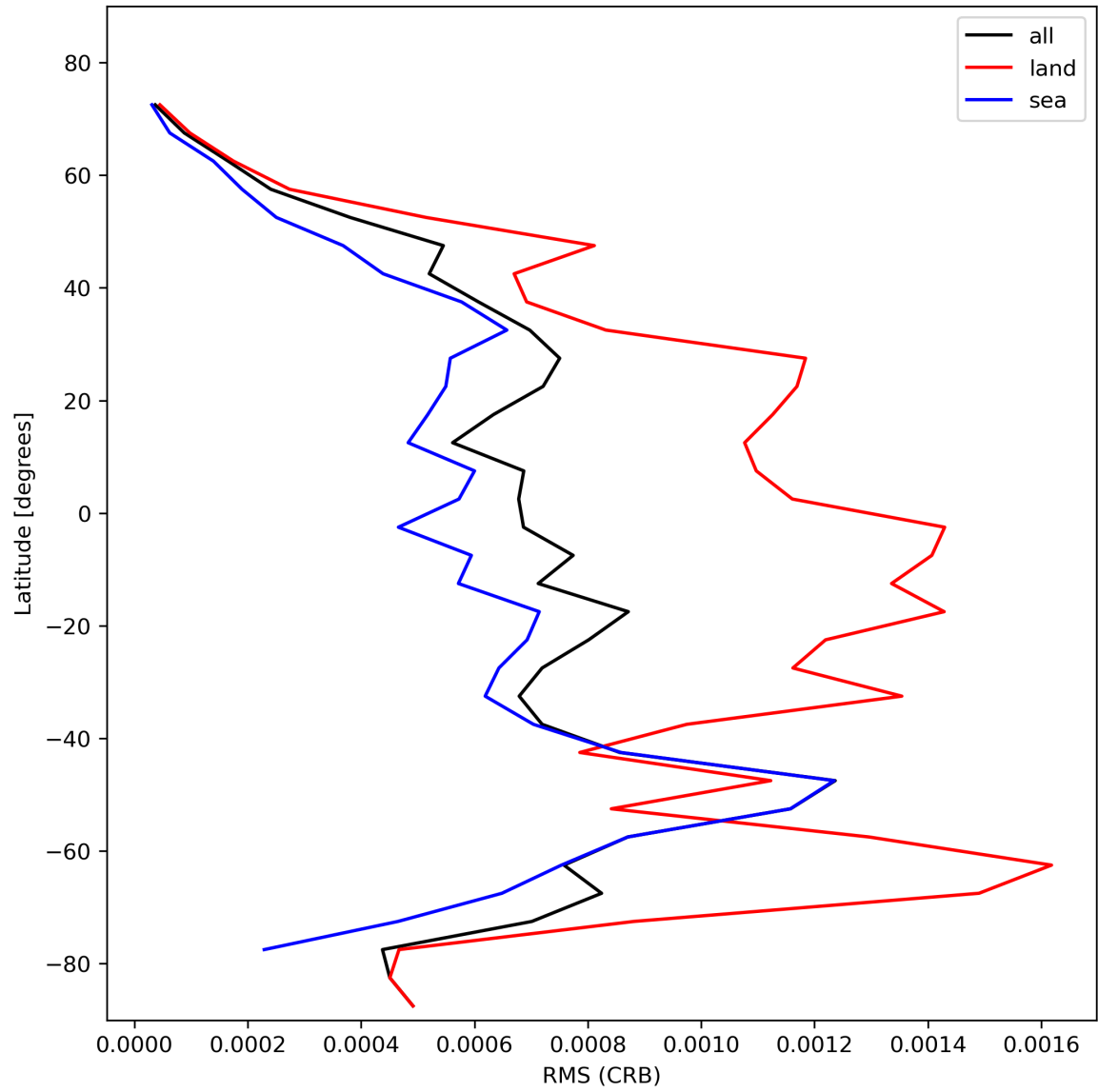
Figure 32: Zonal average of “RMS (CRB)” for 2024-02-06 to 2024-02-08.
