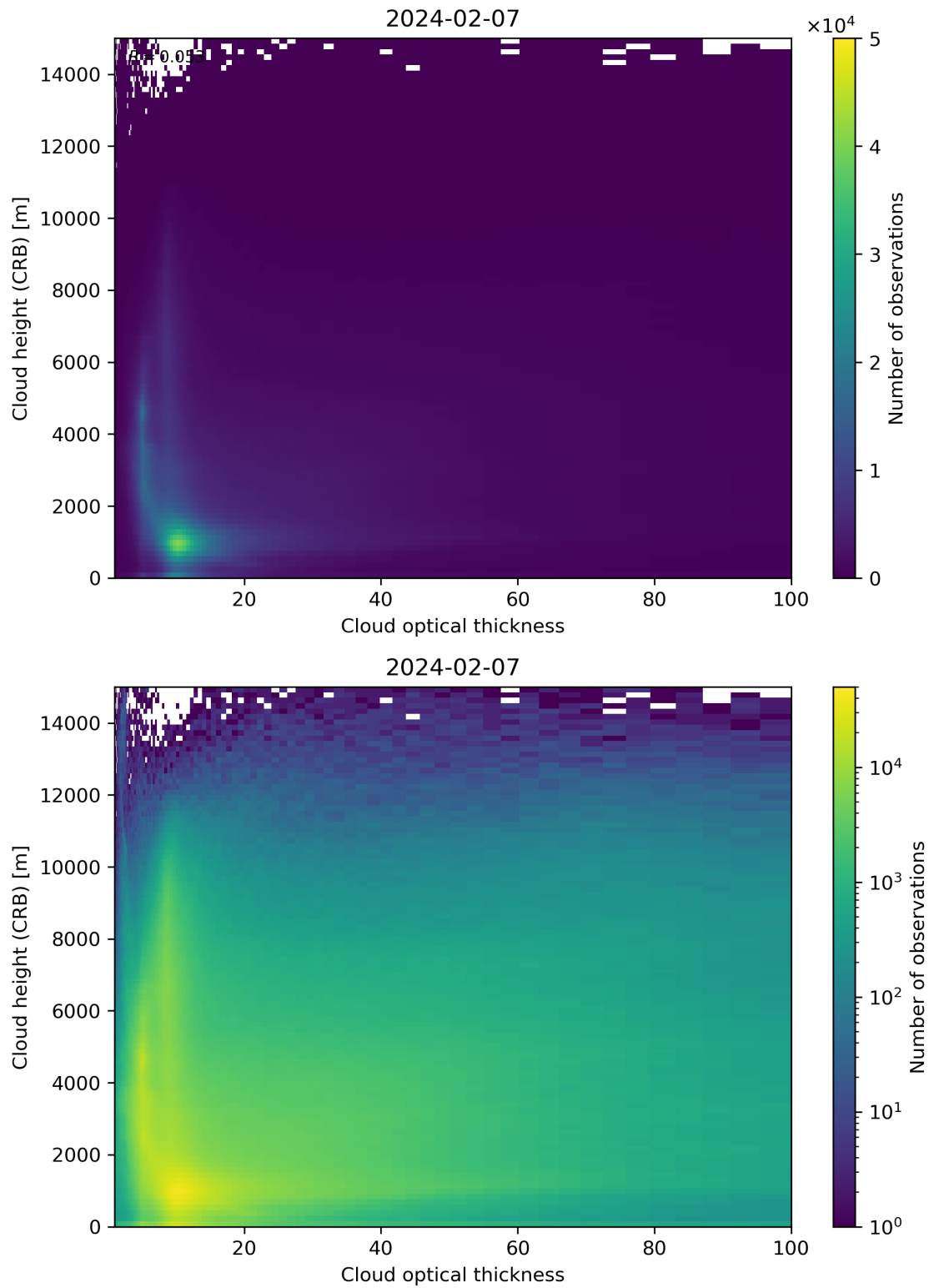
Figure 85: Scatter density plot of “Cloud optical thickness” against “Cloud height (CRB)” for 2024-02-06 to 2024-02-08.
