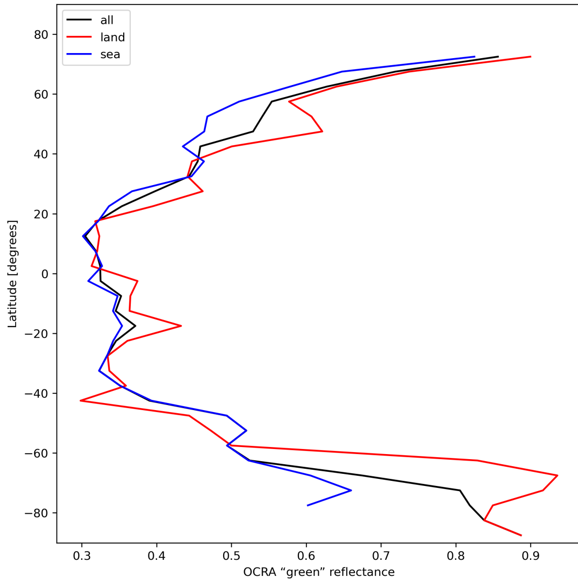
Figure 36: Zonal average of “OCRA “green” reflectance” for 2024-02-06 to 2024-02-08.
