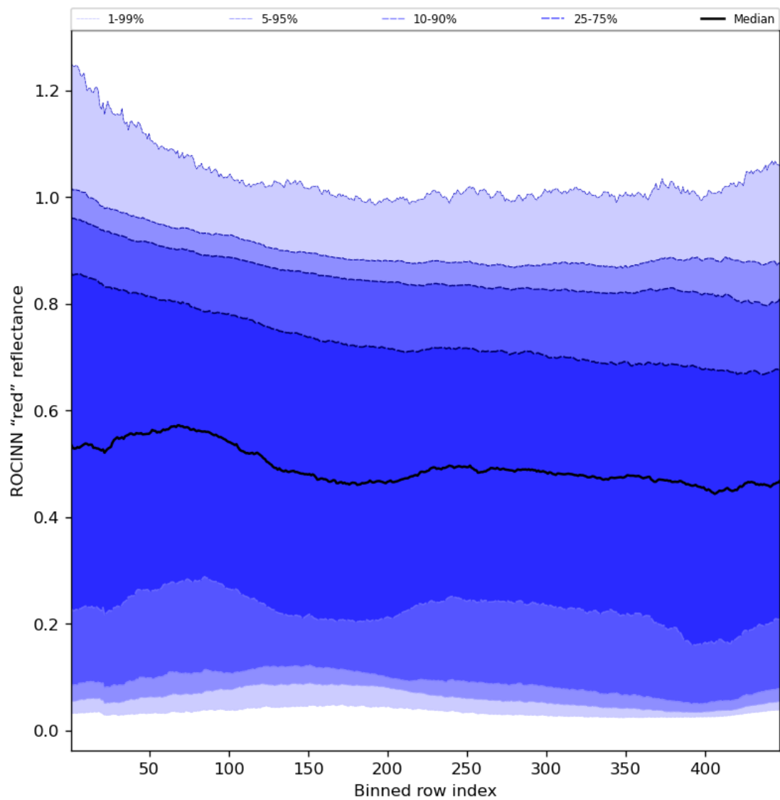
Figure 69: Along track statistics of “ROCINN “red” reflectance” for 2024-02-06 to 2024-02-08
