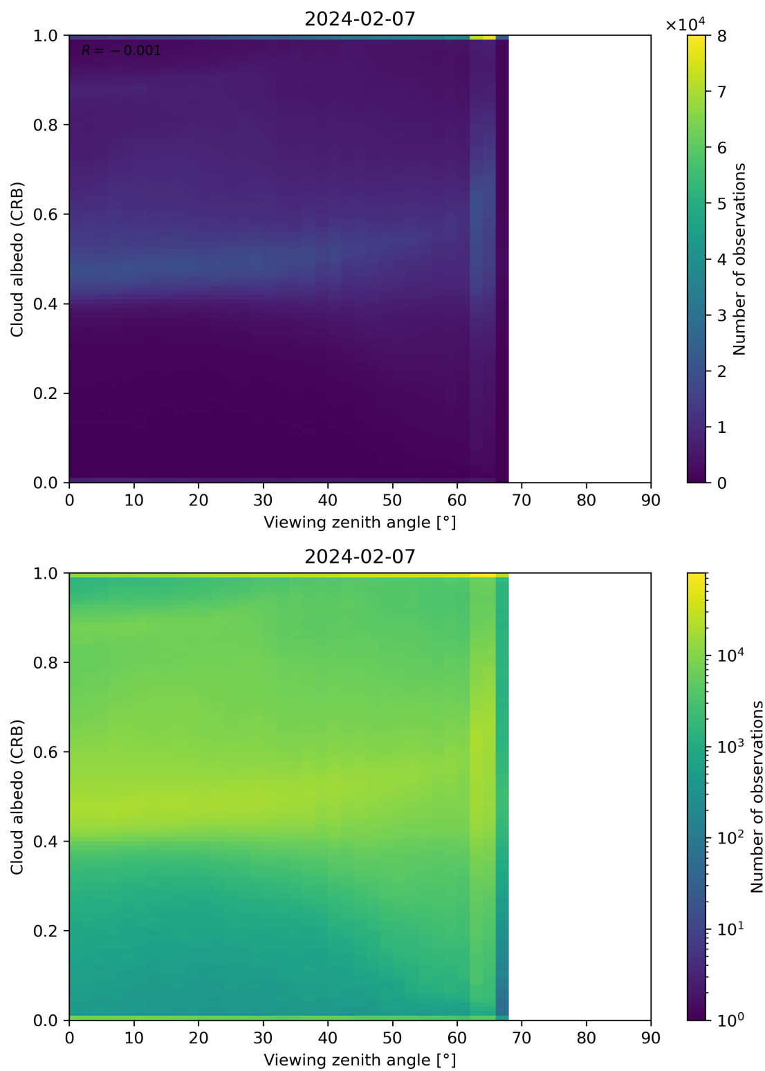
Figure 106: Scatter density plot of “Viewing zenith angle” against “Cloud albedo (CRB)” for 2024-02-06 to 2024-02-08.
