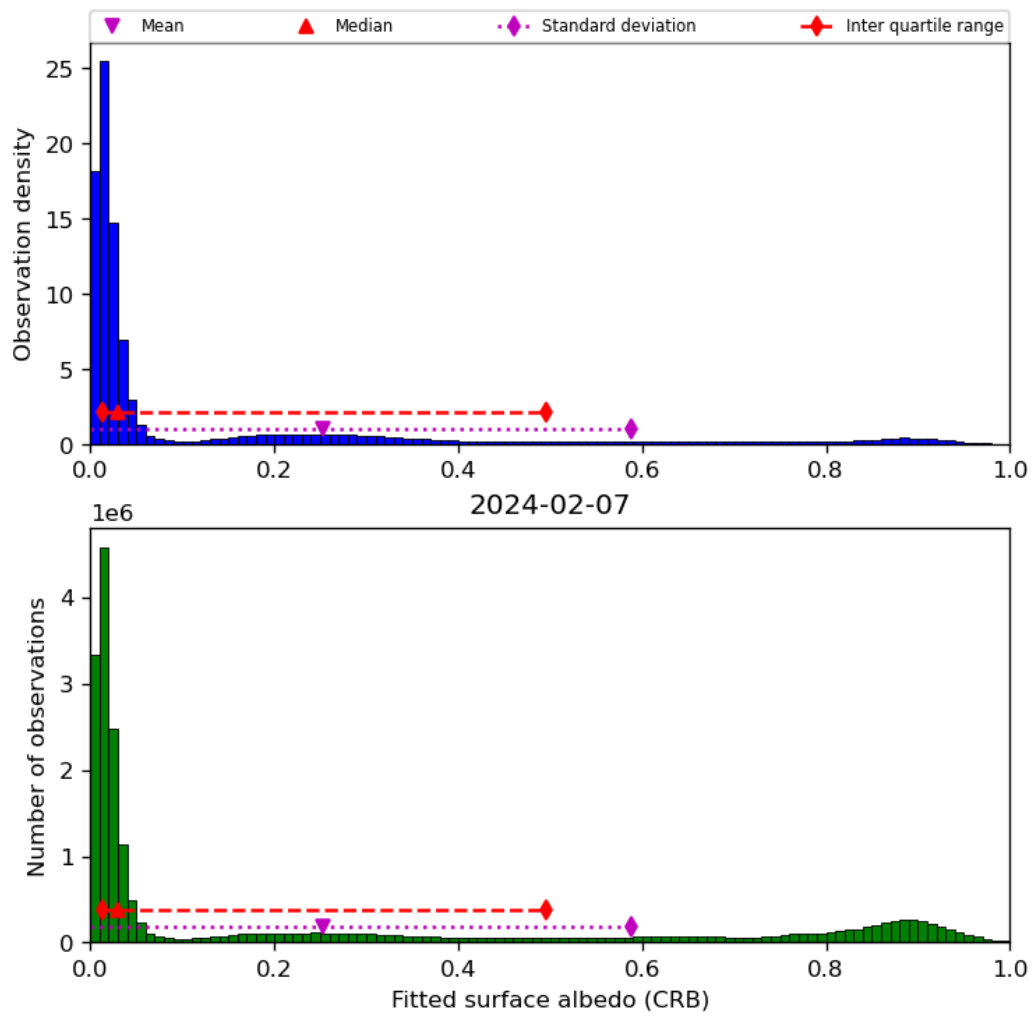
Figure 46: Histogram of “Fitted surface albedo (CRB)” for 2024-02-06 to 2024-02-08
