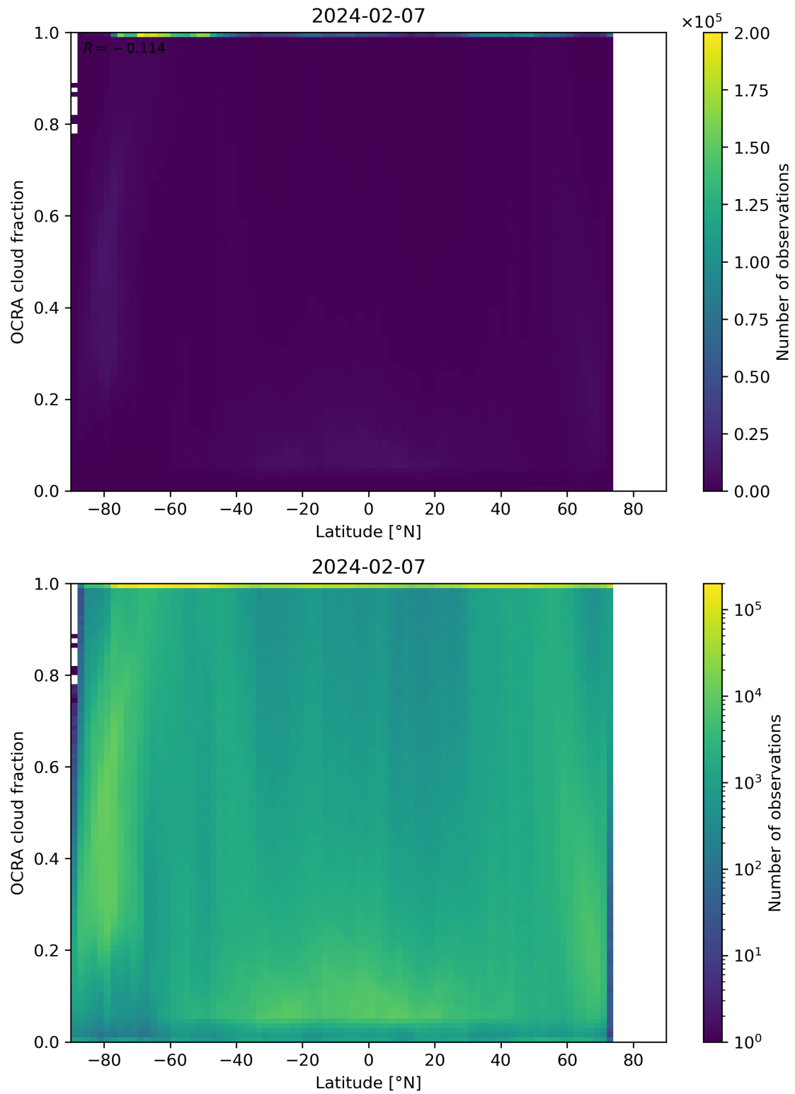
Figure 93: Scatter density plot of “Latitude” against “OCRA cloud fraction” for 2024-02-06 to 2024-02-08.
