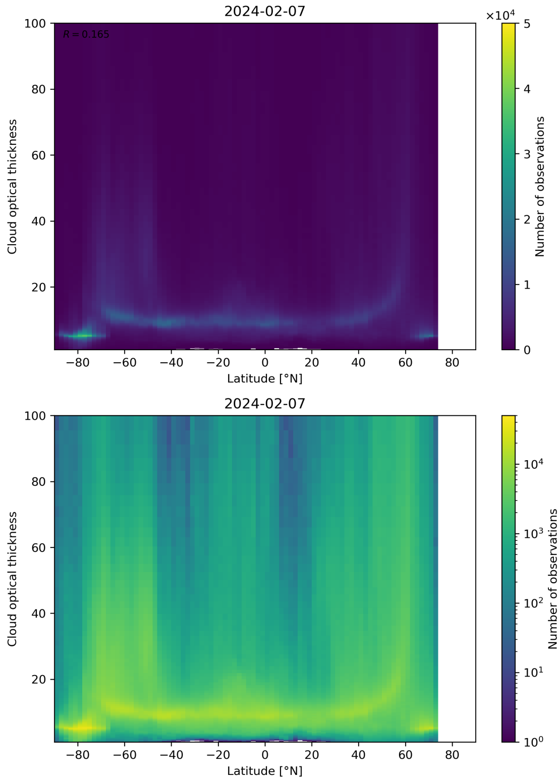
Figure 96: Scatter density plot of “Latitude” against “Cloud optical thickness” for 2024-02-06 to 2024-02-08.
