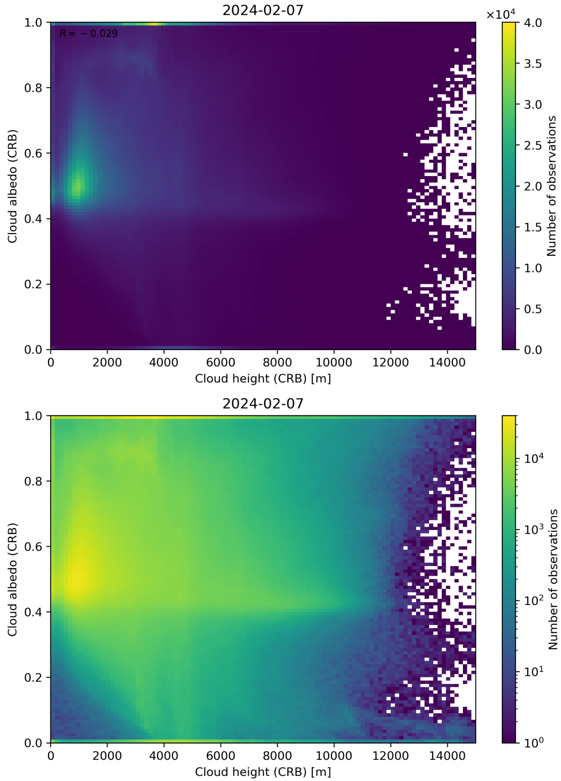
Figure 80: Scatter density plot of “Cloud height (CRB)” against “Cloud albedo (CRB)” for 2024-02-06 to 2024-02-08.
