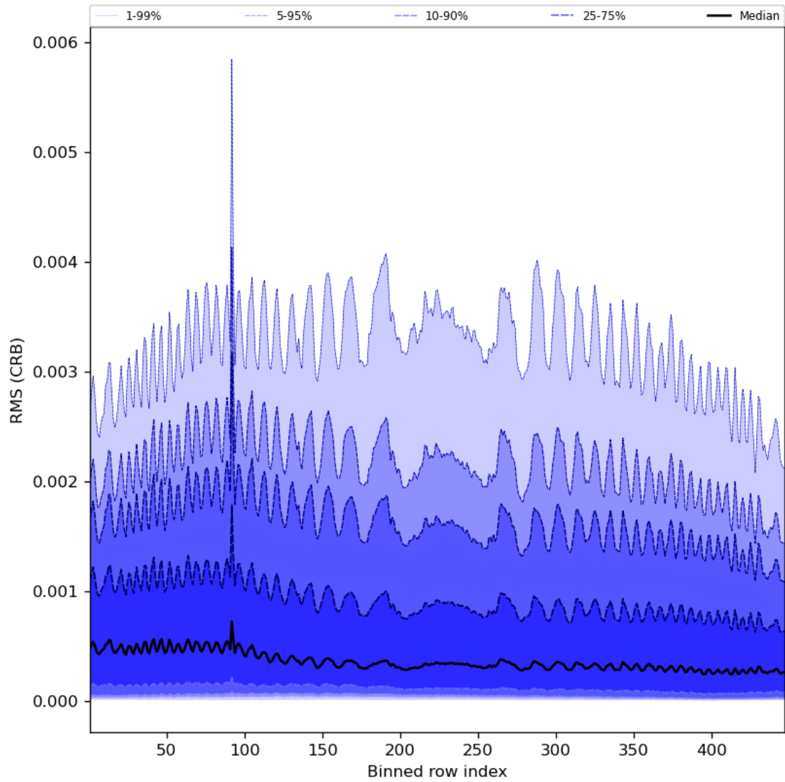
Figure 64: Along track statistics of “RMS (CRB)” for 2024-02-06 to 2024-02-08
