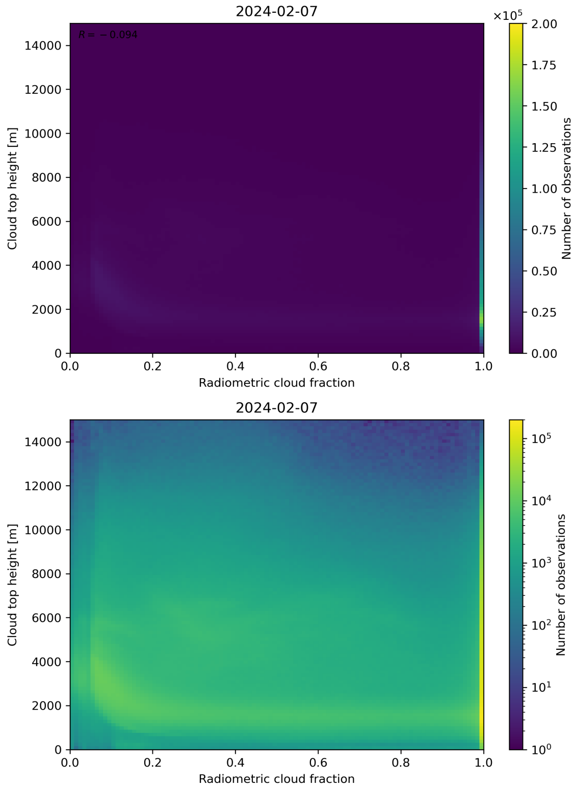
Figure 76: Scatter density plot of “Radiometric cloud fraction” against “Cloud top height” for 2024-02-06 to 2024-02-08.
