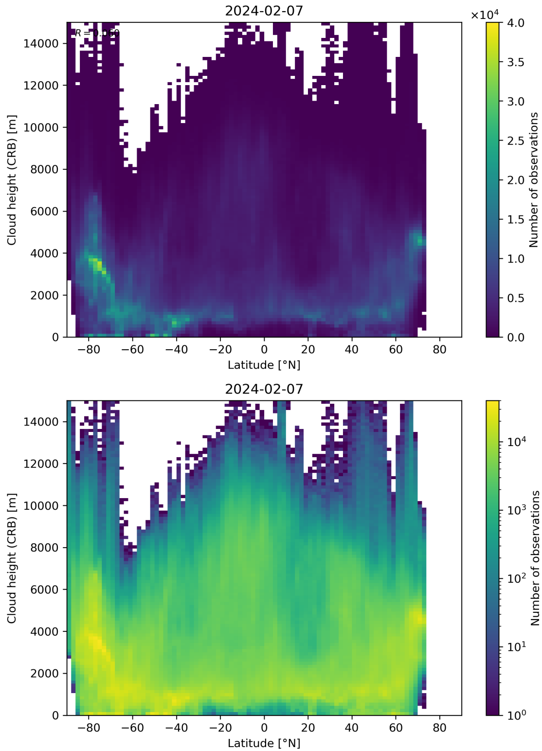
Figure 95: Scatter density plot of “Latitude” against “Cloud height (CRB)” for 2024-02-06 to 2024-02-08.
