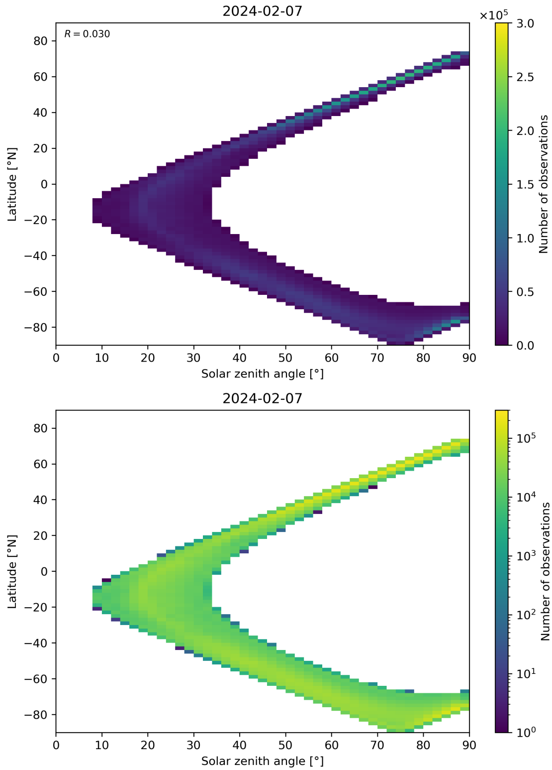
Figure 105: Scatter density plot of “Solar zenith angle” against “Latitude” for 2024-02-06 to 2024-02-08.
