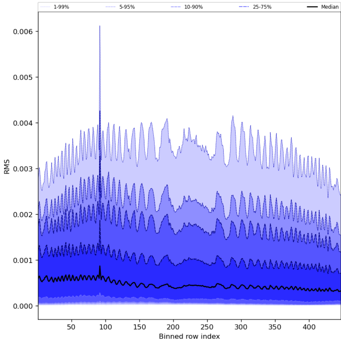
Figure 63: Along track statistics of “RMS” for 2024-02-06 to 2024-02-08
