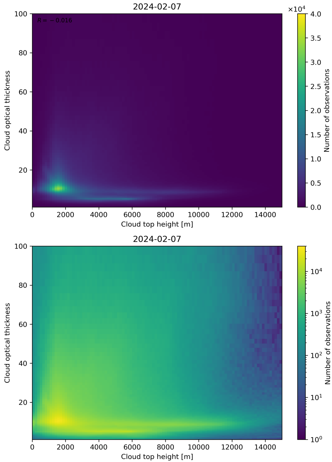
Figure 90: Scatter density plot of “Cloud top height” against “Cloud optical thickness” for 2024-02-06 to 2024-02-08.
