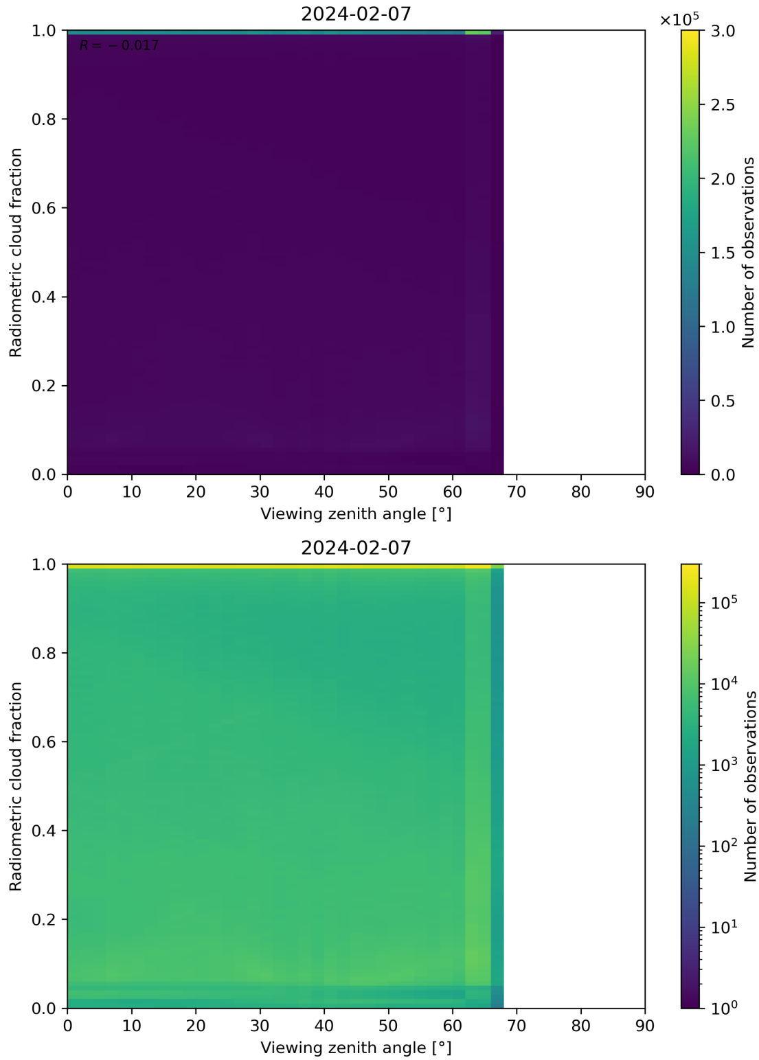
Figure 107: Scatter density plot of “Viewing zenith angle” against “Radiometric cloud fraction” for 2024-02-06 to 2024-02-08.
