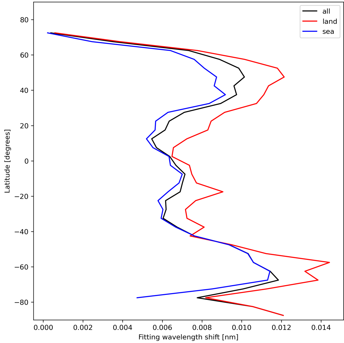
Figure 33: Zonal average of “Fitting wavelength shift” for 2024-02-06 to 2024-02-08.
