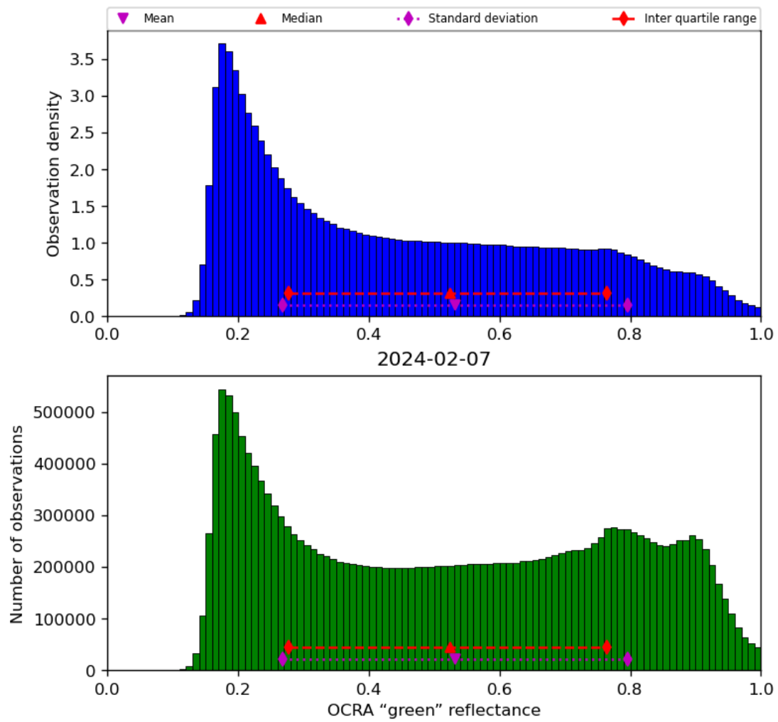
Figure 52: Histogram of “OCRA “green” reflectance” for 2024-02-06 to 2024-02-08
