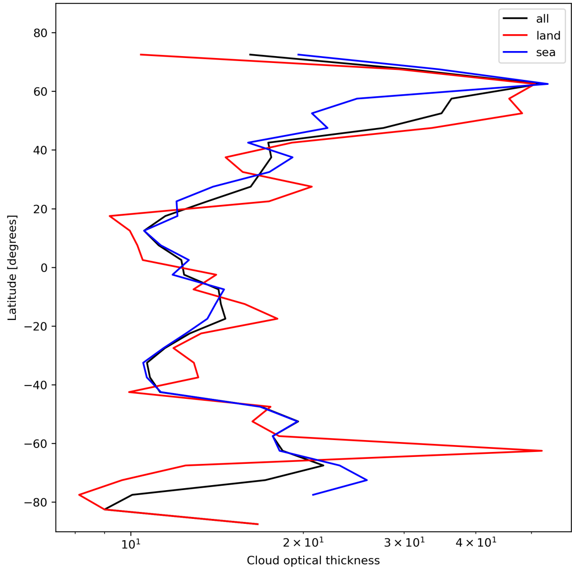
Figure 25: Zonal average of “Cloud optical thickness” for 2024-02-06 to 2024-02-08.
