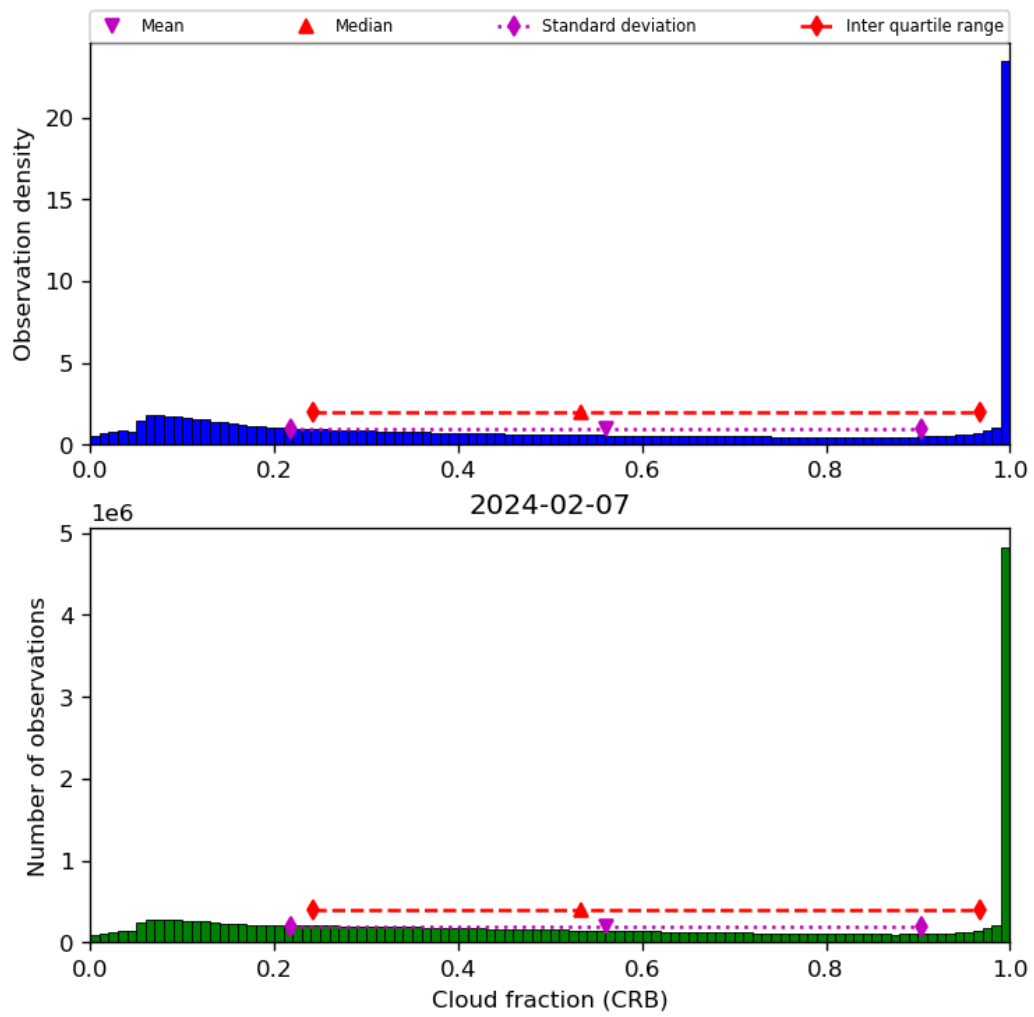
Figure 42: Histogram of “Cloud fraction (CRB)” for 2024-02-06 to 2024-02-08
