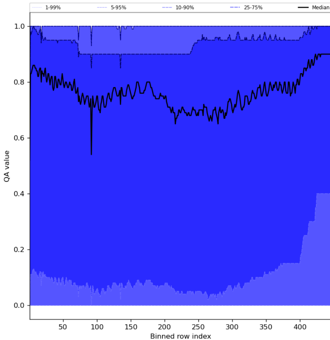
Figure 54: Along track statistics of “QA value” for 2024-02-06 to 2024-02-08
