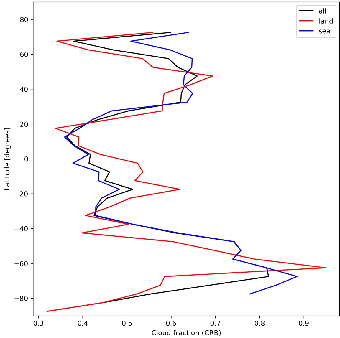
Figure 26: Zonal average of “Cloud fraction (CRB)” for 2024-02-06 to 2024-02-08.
