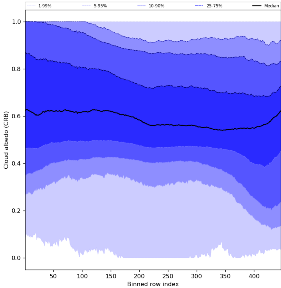
Figure 60: Along track statistics of “Cloud albedo (CRB)” for 2024-02-06 to 2024-02-08
