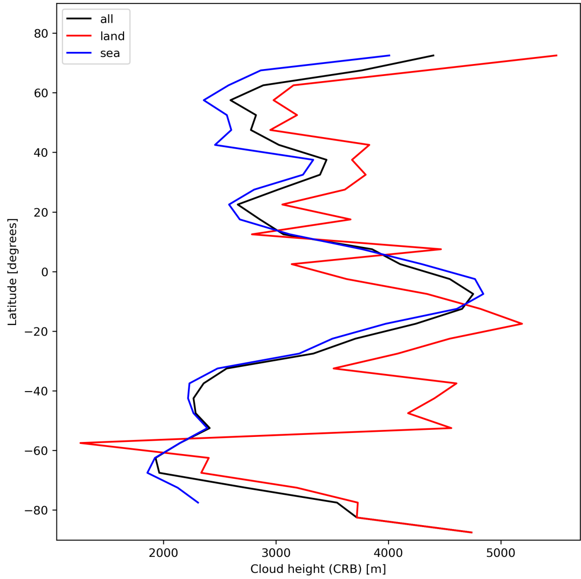
Figure 27: Zonal average of “Cloud height (CRB)” for 2024-02-06 to 2024-02-08.
