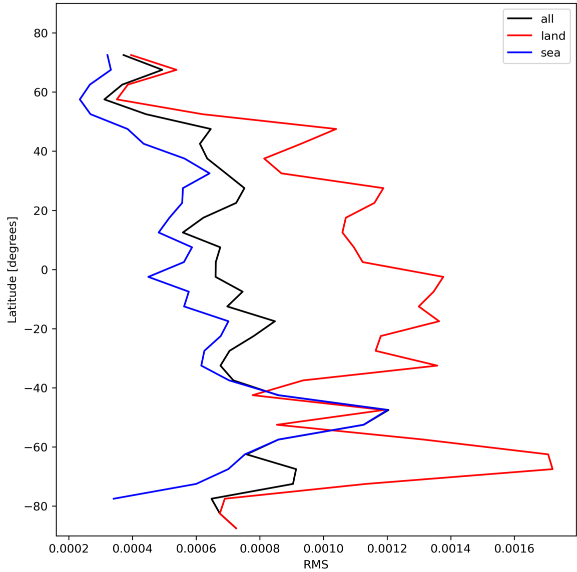
Figure 31: Zonal average of “RMS” for 2024-02-06 to 2024-02-08.
