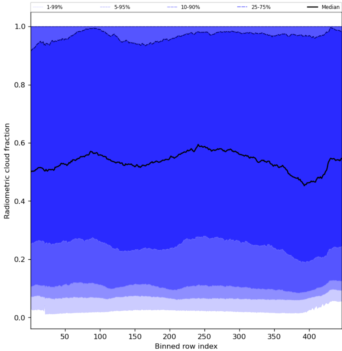
Figure 55: Along track statistics of “Radiometric cloud fraction” for 2024-02-06 to 2024-02-08
