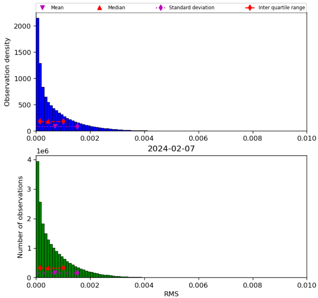
Figure 47: Histogram of “RMS” for 2024-02-06 to 2024-02-08
