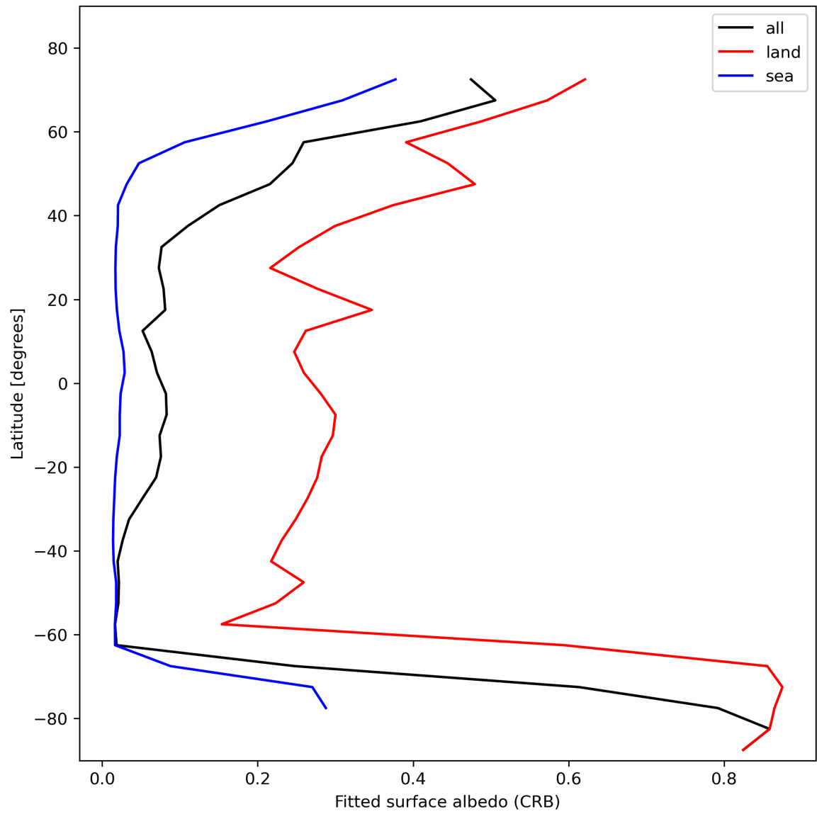
Figure 30: Zonal average of “Fitted surface albedo (CRB)” for 2024-02-06 to 2024-02-08.
