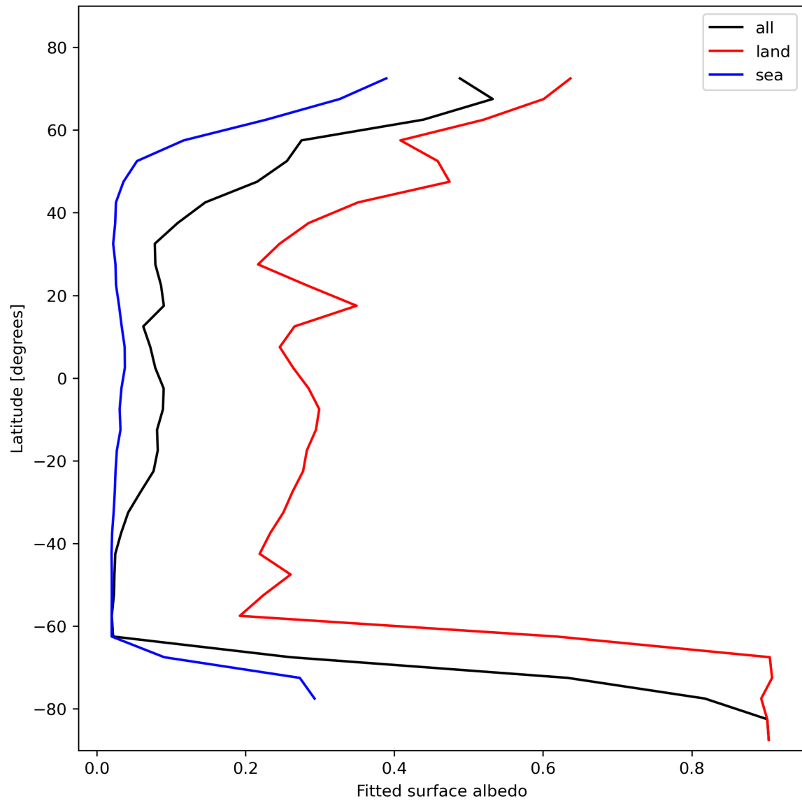
Figure 29: Zonal average of “Fitted surface albedo” for 2024-02-06 to 2024-02-08.
