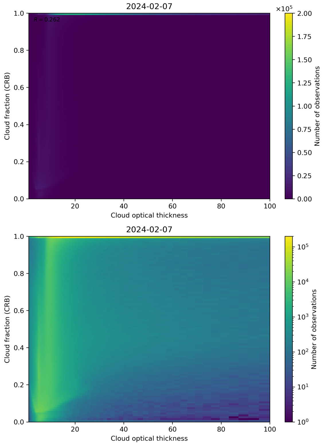
Figure 84: Scatter density plot of “Cloud optical thickness” against “Cloud fraction (CRB)” for 2024-02-06 to 2024-02-08.
