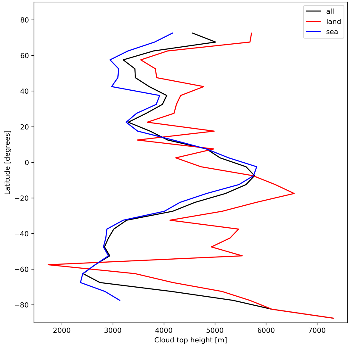
Figure 24: Zonal average of “Cloud top height” for 2024-02-06 to 2024-02-08.
