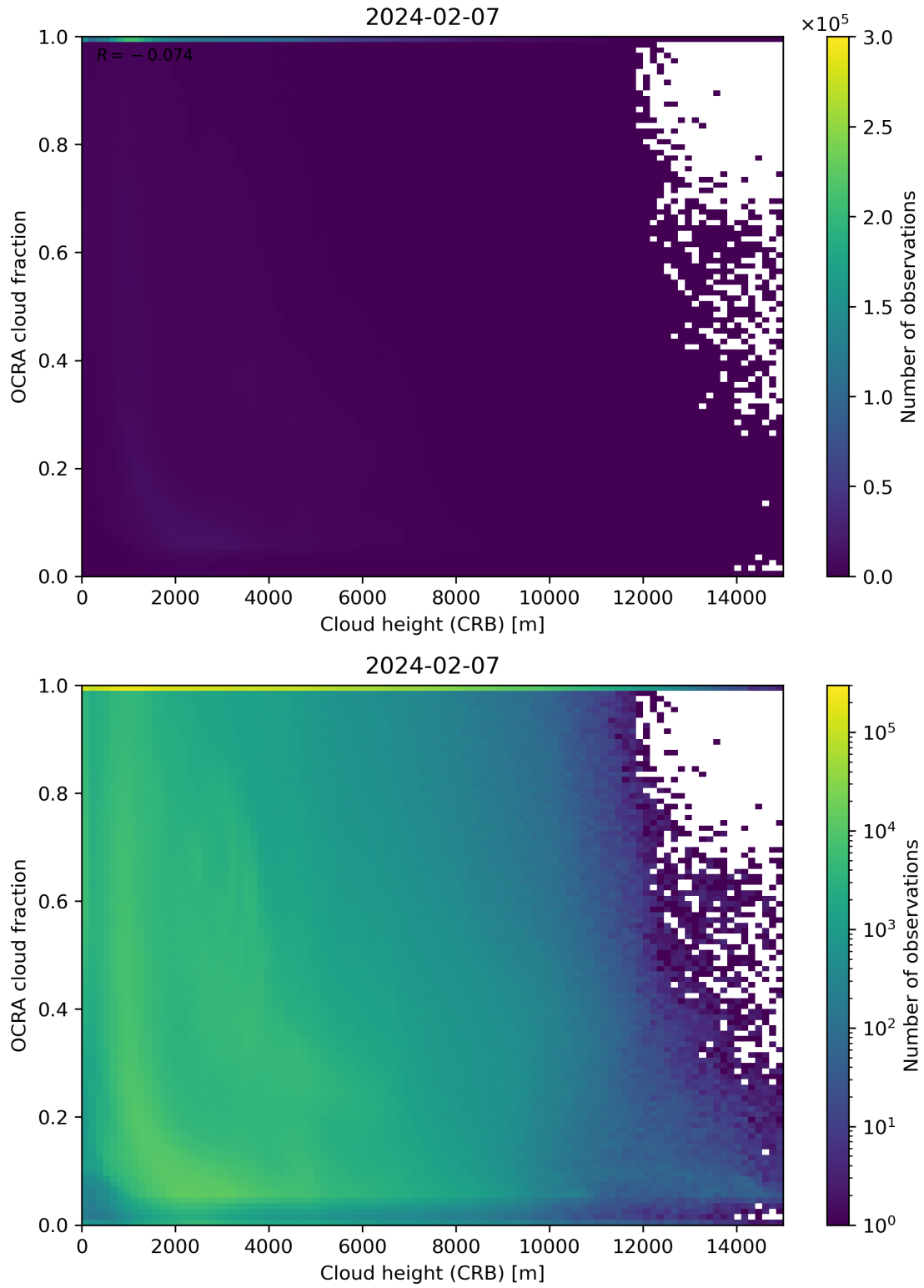
Figure 81: Scatter density plot of “Cloud height (CRB)” against “OCRA cloud fraction” for 2024-02-06 to 2024-02-08.
