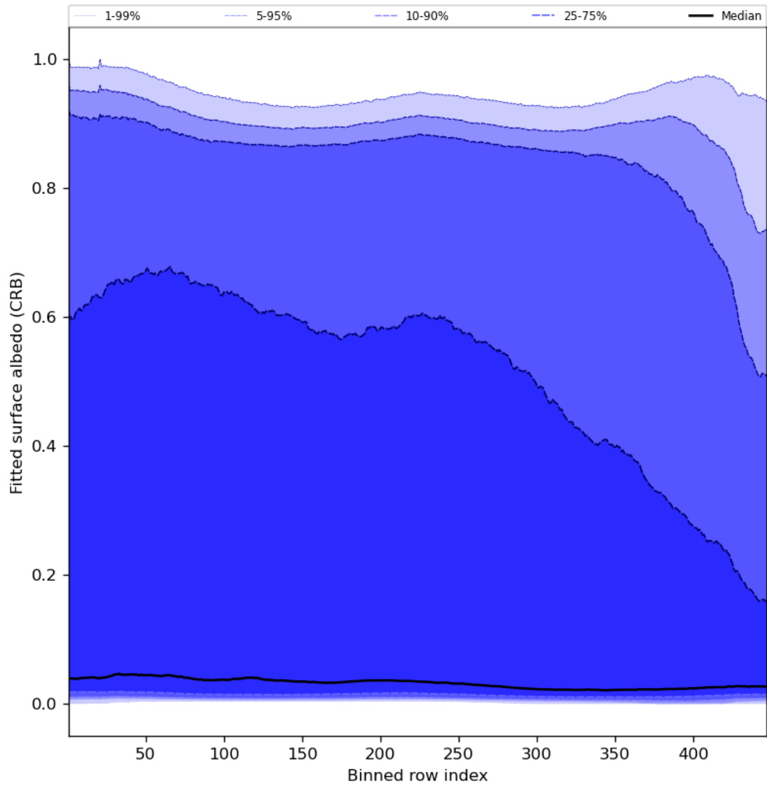
Figure 62: Along track statistics of “Fitted surface albedo (CRB)” for 2024-02-06 to 2024-02-08
