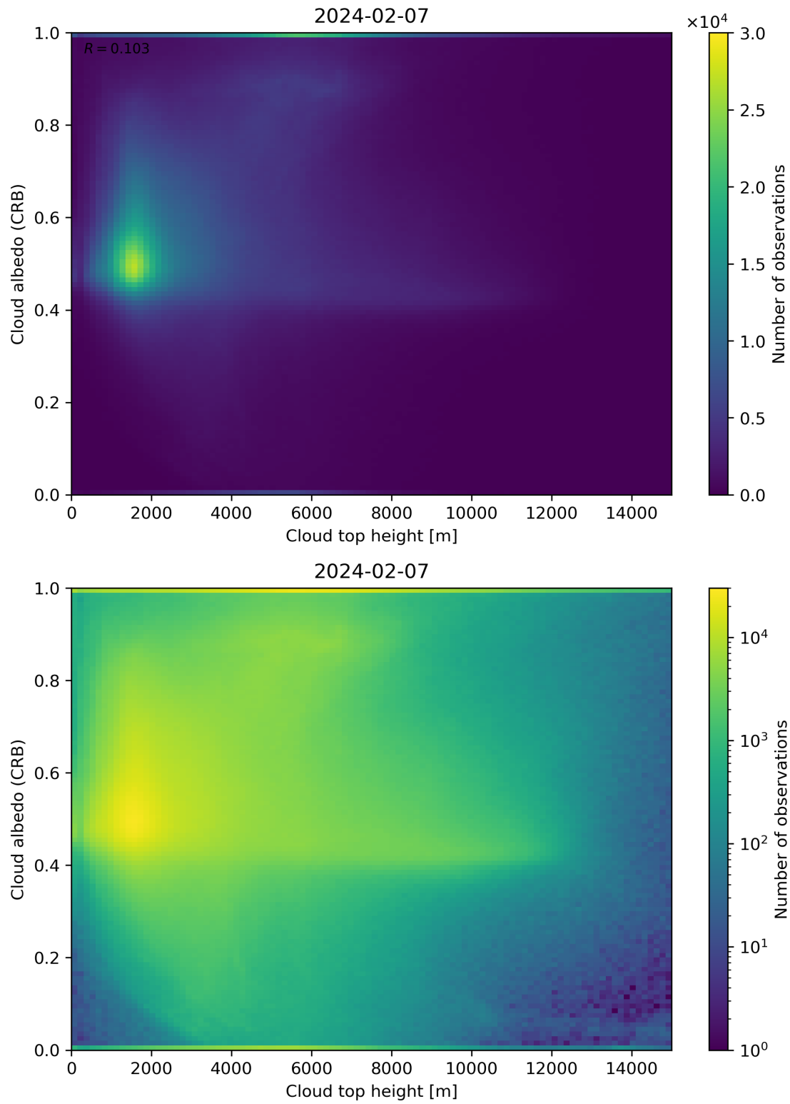
Figure 86: Scatter density plot of “Cloud top height” against “Cloud albedo (CRB)” for 2024-02-06 to 2024-02-08.
