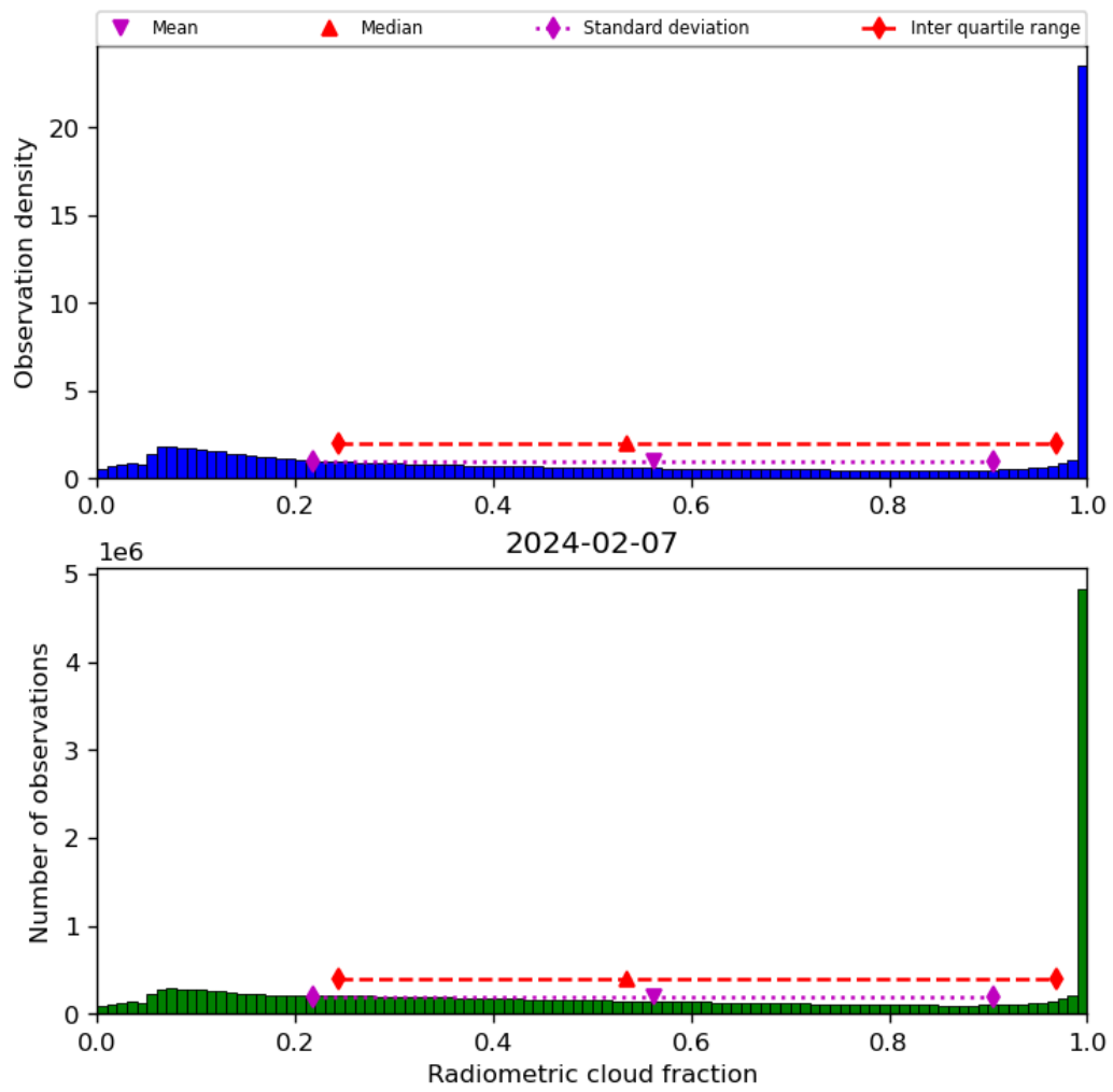
Figure 39: Histogram of “Radiometric cloud fraction” for 2024-02-06 to 2024-02-08
