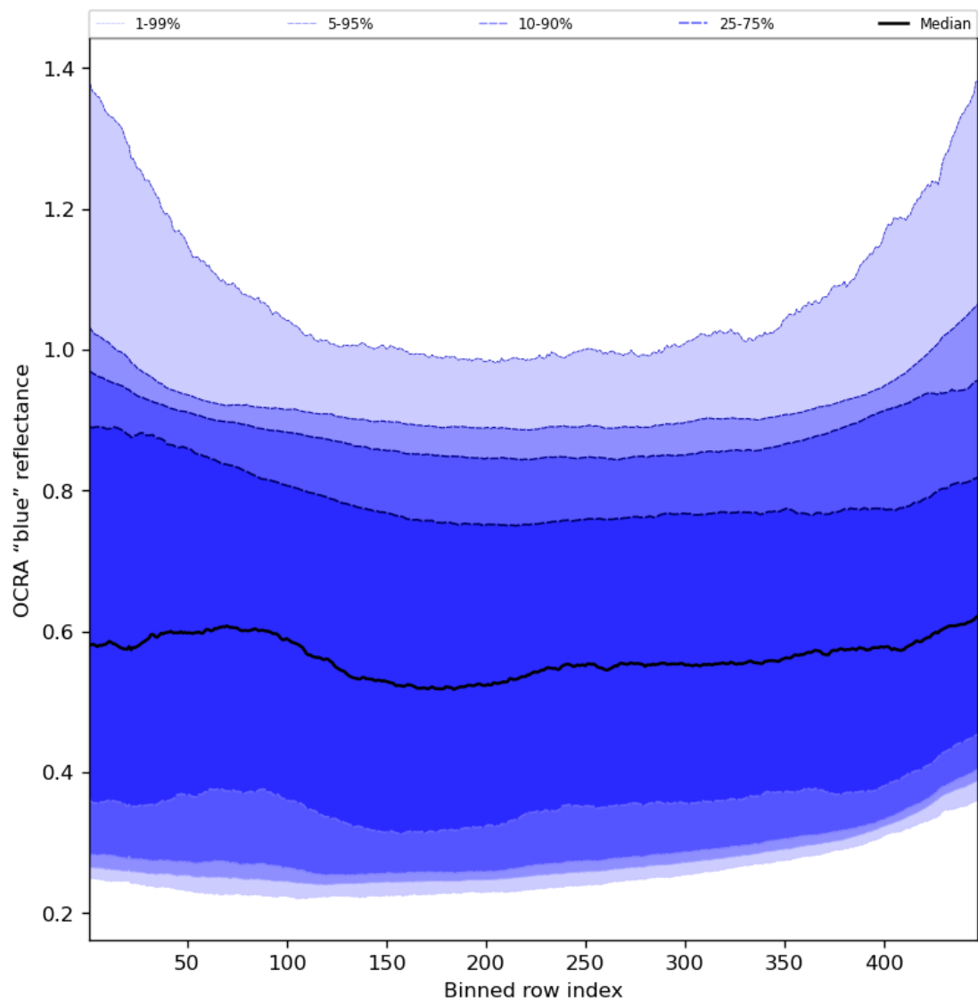
Figure 67: Along track statistics of “OCRA “blue” reflectance” for 2024-02-06 to 2024-02-08
