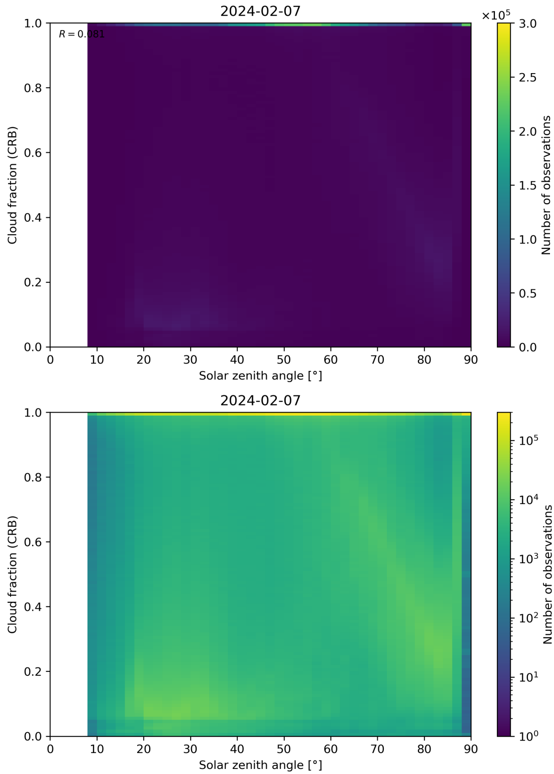
Figure 101: Scatter density plot of “Solar zenith angle” against “Cloud fraction (CRB)” for 2024-02-06 to 2024-02-08.
