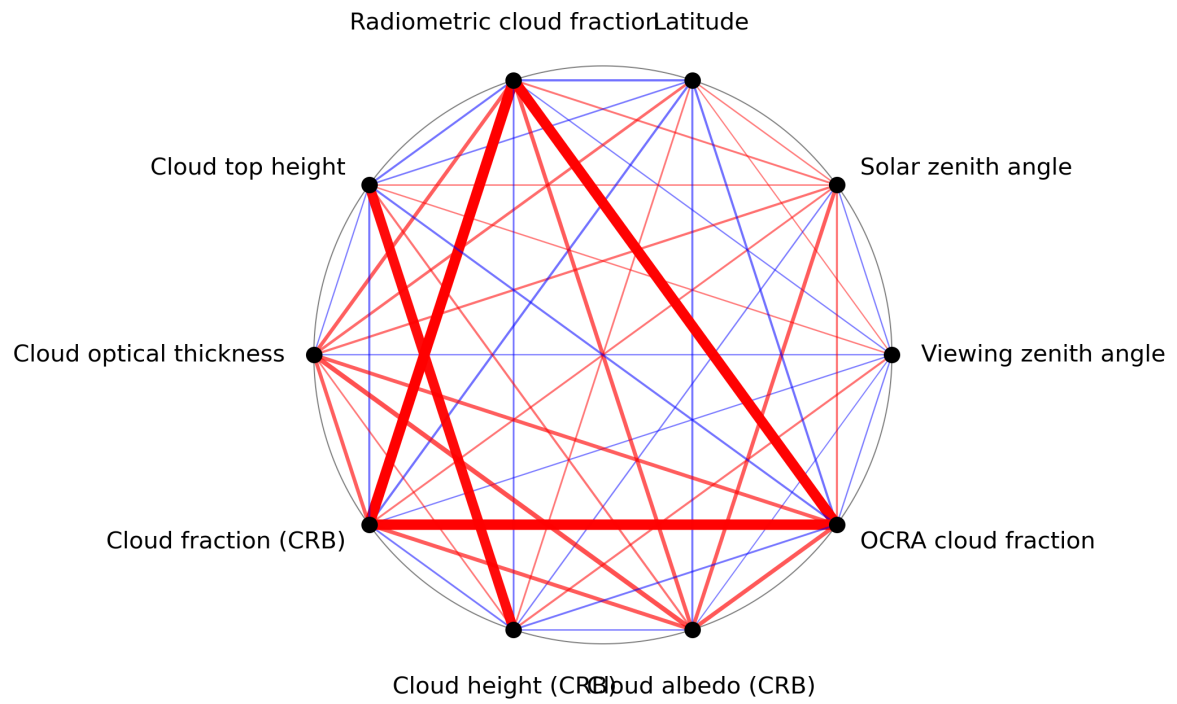
Figure 1: Map of correlation graph for 2024-02-06 to 2024-02-08.
