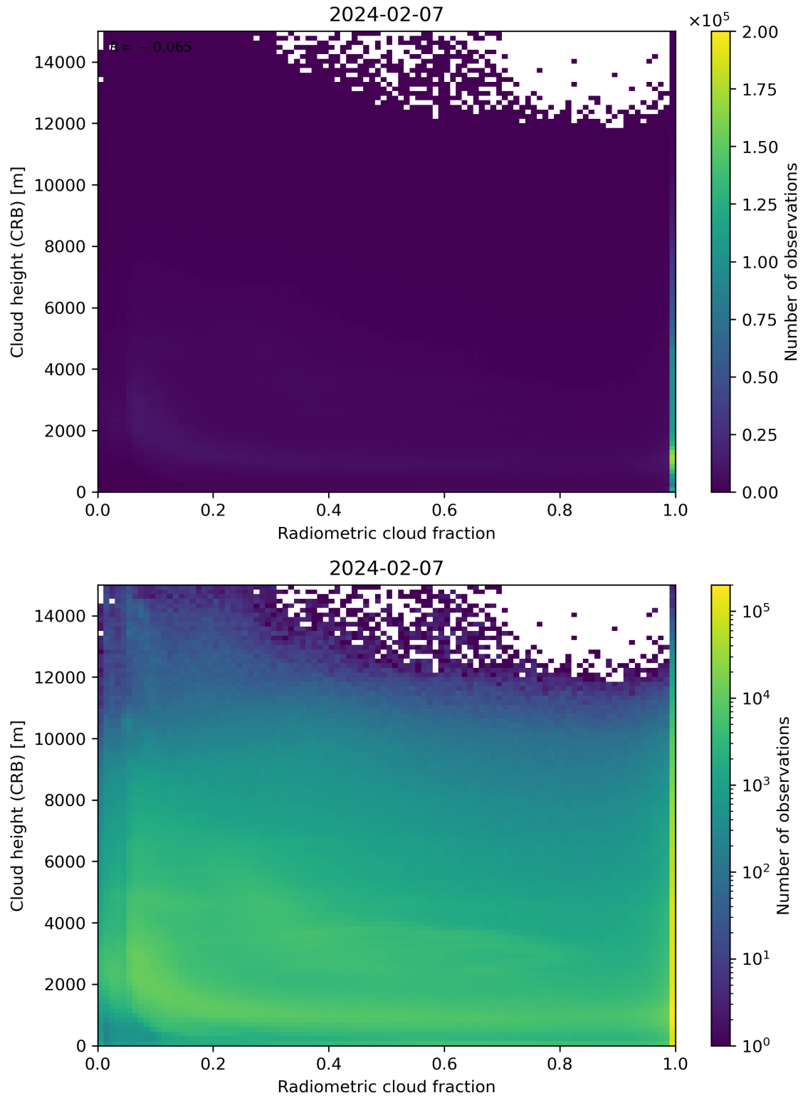
Figure 74: Scatter density plot of “Radiometric cloud fraction” against “Cloud height (CRB)” for 2024-02-06 to 2024-02-08.
