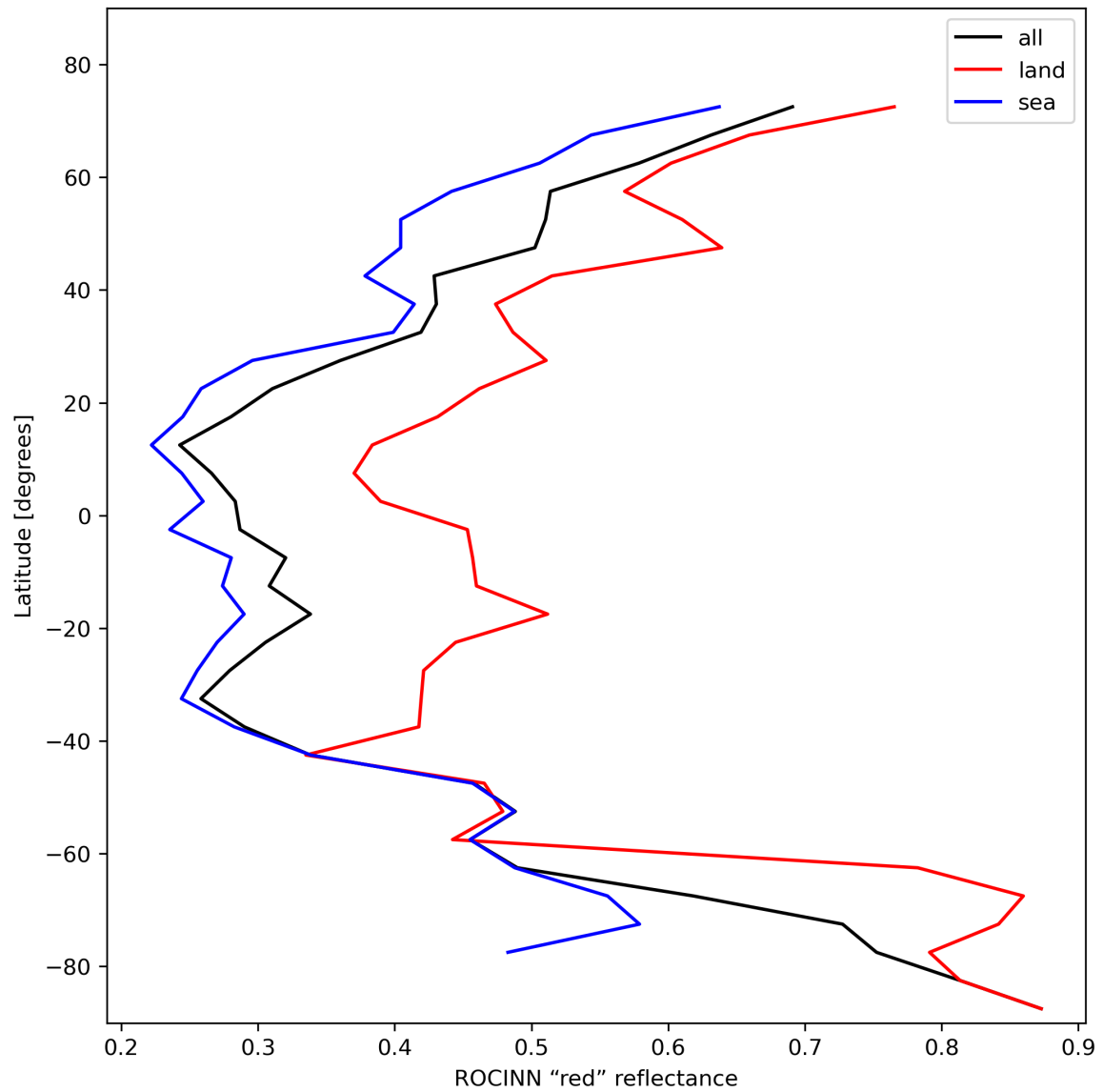
Figure 37: Zonal average of “ROCINN “red” reflectance” for 2024-02-06 to 2024-02-08.
