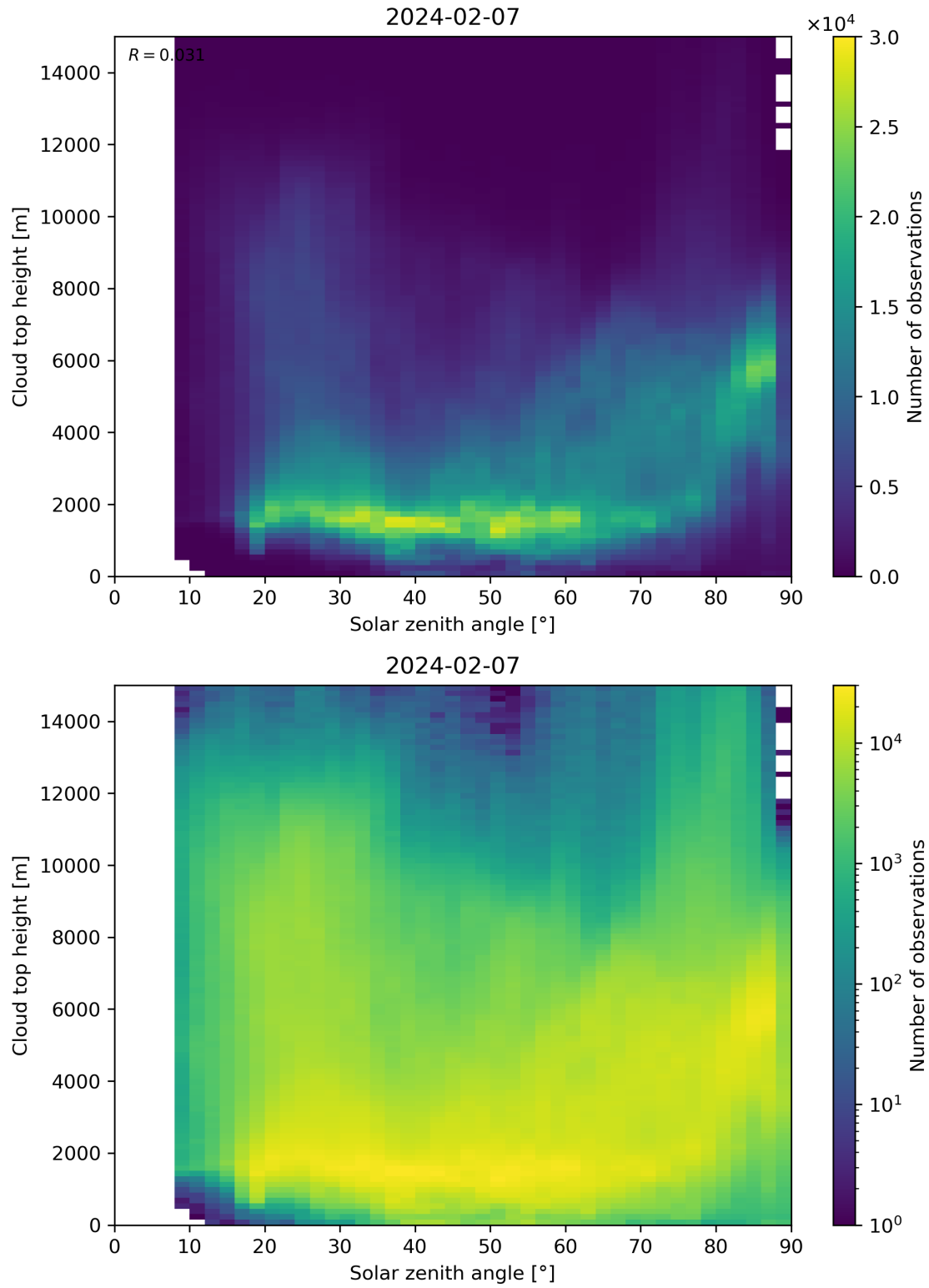
Figure 104: Scatter density plot of “Solar zenith angle” against “Cloud top height” for 2024-02-06 to 2024-02-08.
