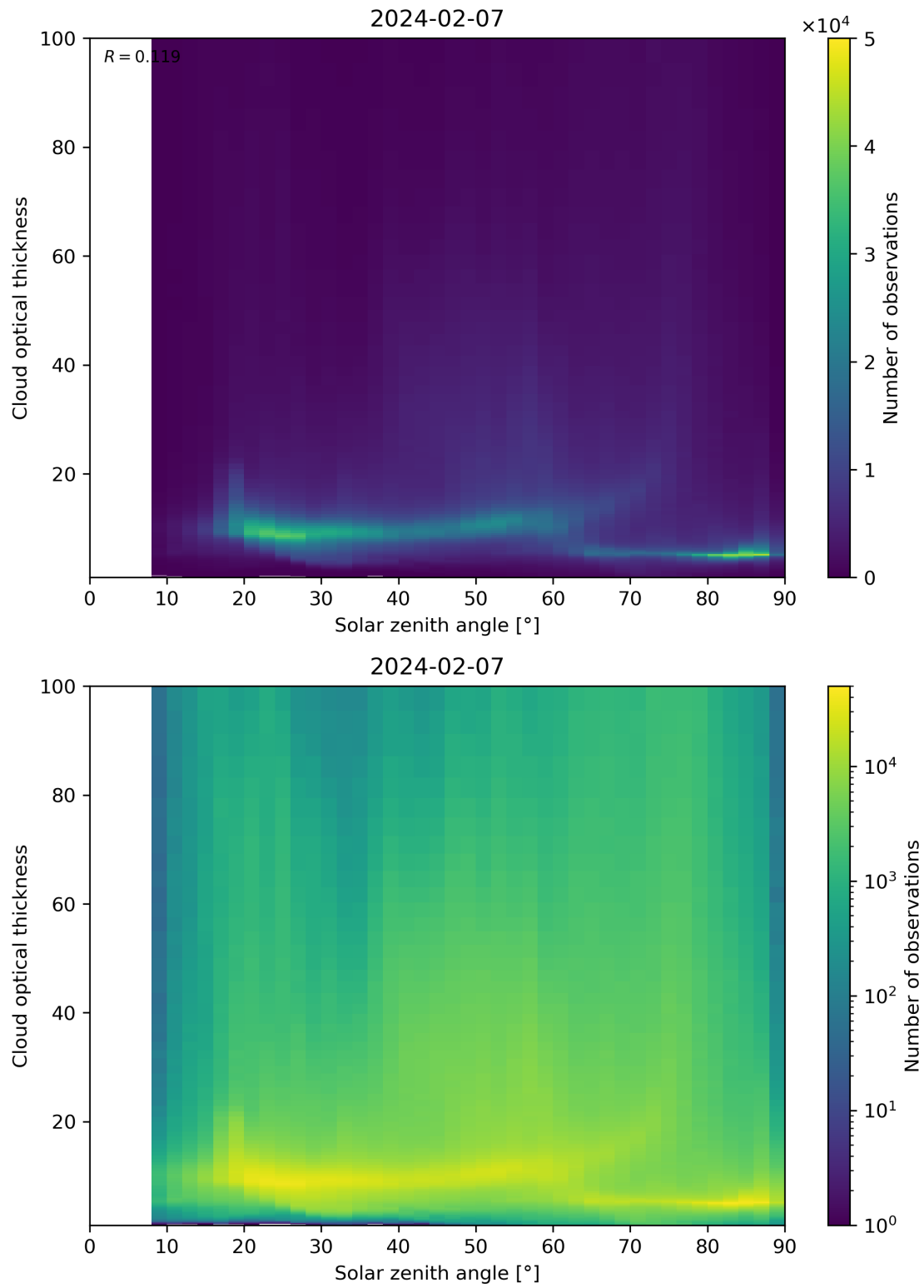
Figure 103: Scatter density plot of “Solar zenith angle” against “Cloud optical thickness” for 2024-02-06 to 2024-02-08.
