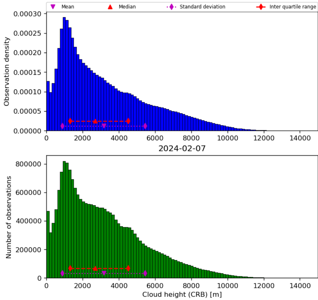
Figure 43: Histogram of “Cloud height (CRB)” for 2024-02-06 to 2024-02-08
