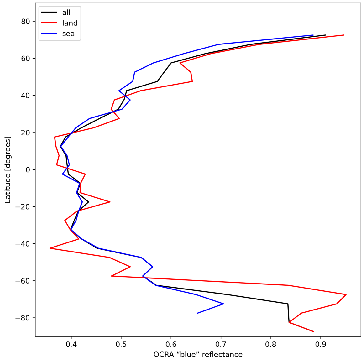
Figure 35: Zonal average of “OCRA “blue” reflectance” for 2024-02-06 to 2024-02-08.
