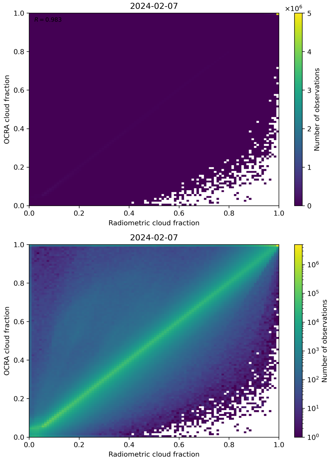
Figure 72: Scatter density plot of “Radiometric cloud fraction” against “OCRA cloud fraction” for 2024-02-06 to 2024-02-08.
