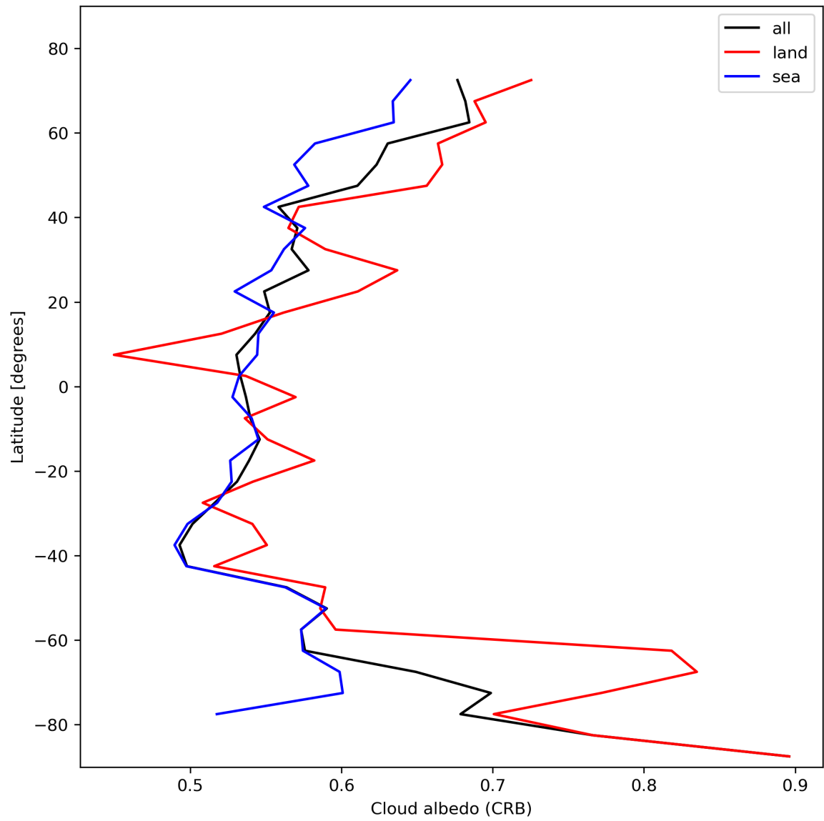
Figure 28: Zonal average of “Cloud albedo (CRB)” for 2024-02-06 to 2024-02-08.
