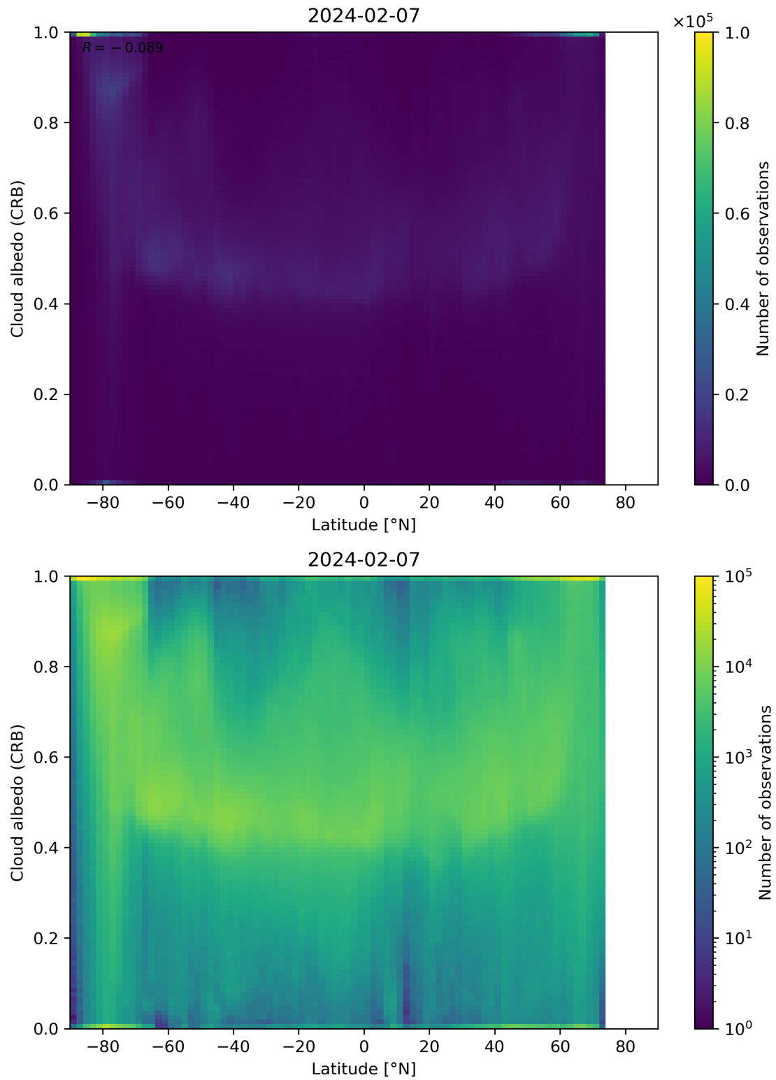
Figure 91: Scatter density plot of “Latitude” against “Cloud albedo (CRB)” for 2024-02-06 to 2024-02-08.
