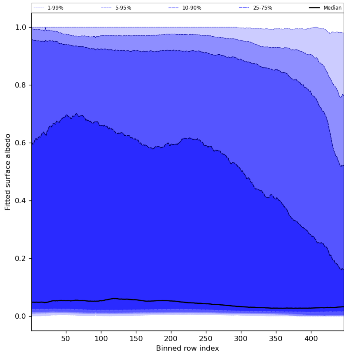
Figure 61: Along track statistics of “Fitted surface albedo” for 2024-02-06 to 2024-02-08
