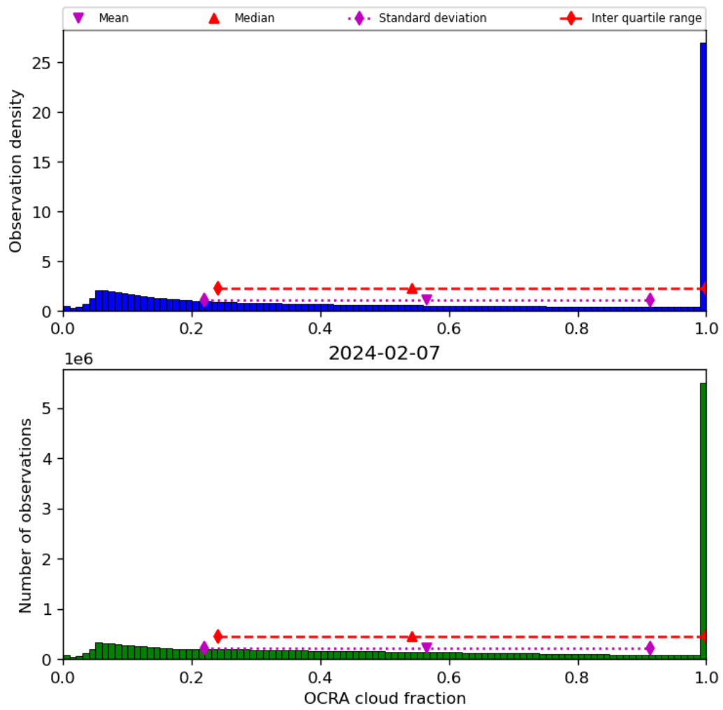
Figure 50: Histogram of “OCRA cloud fraction” for 2024-02-06 to 2024-02-08
