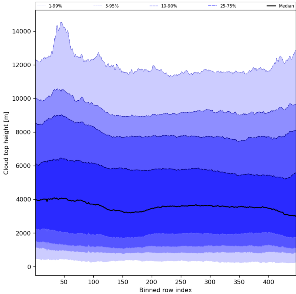
Figure 56: Along track statistics of “Cloud top height” for 2024-02-06 to 2024-02-08
