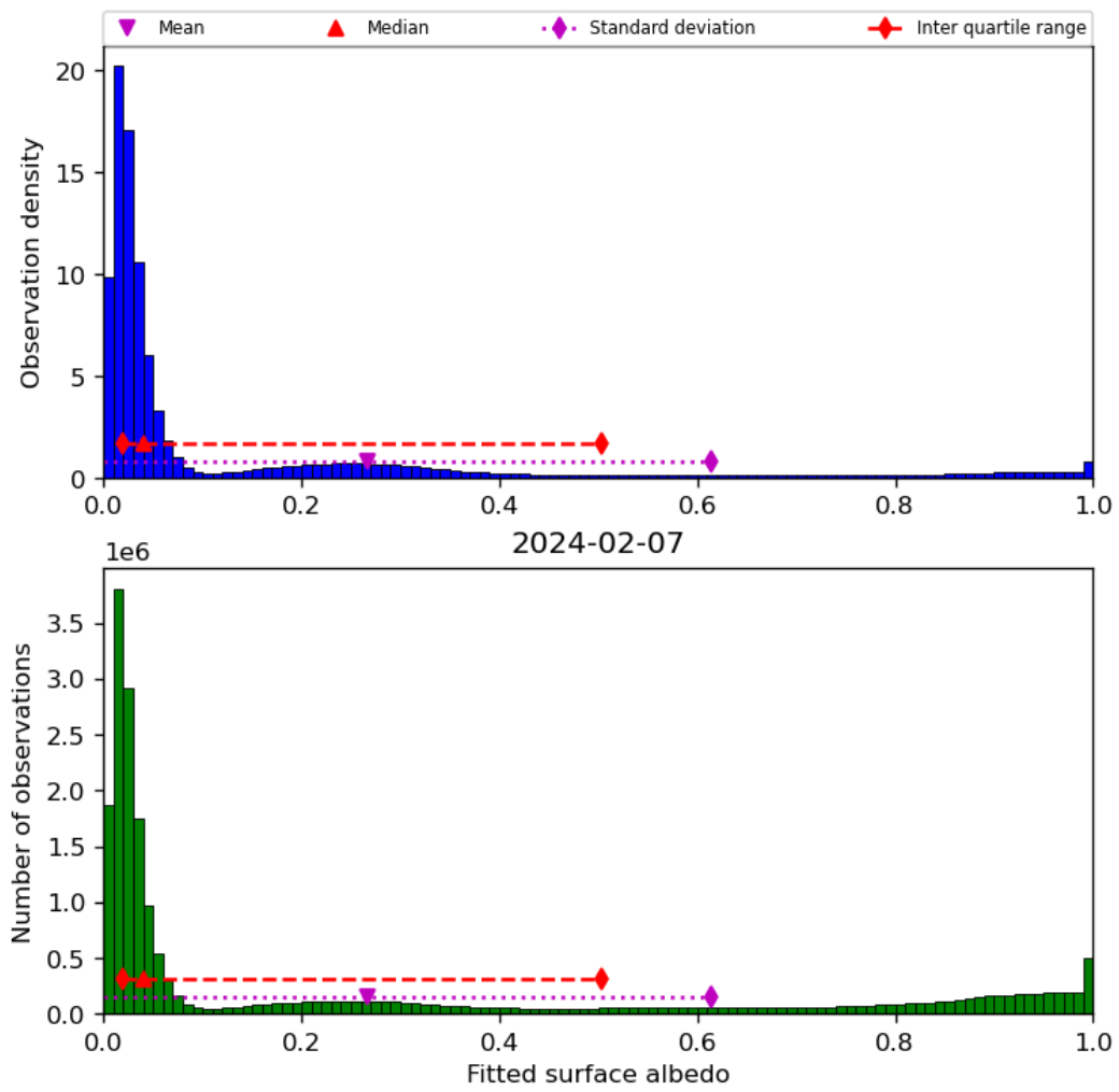
Figure 45: Histogram of “Fitted surface albedo” for 2024-02-06 to 2024-02-08
