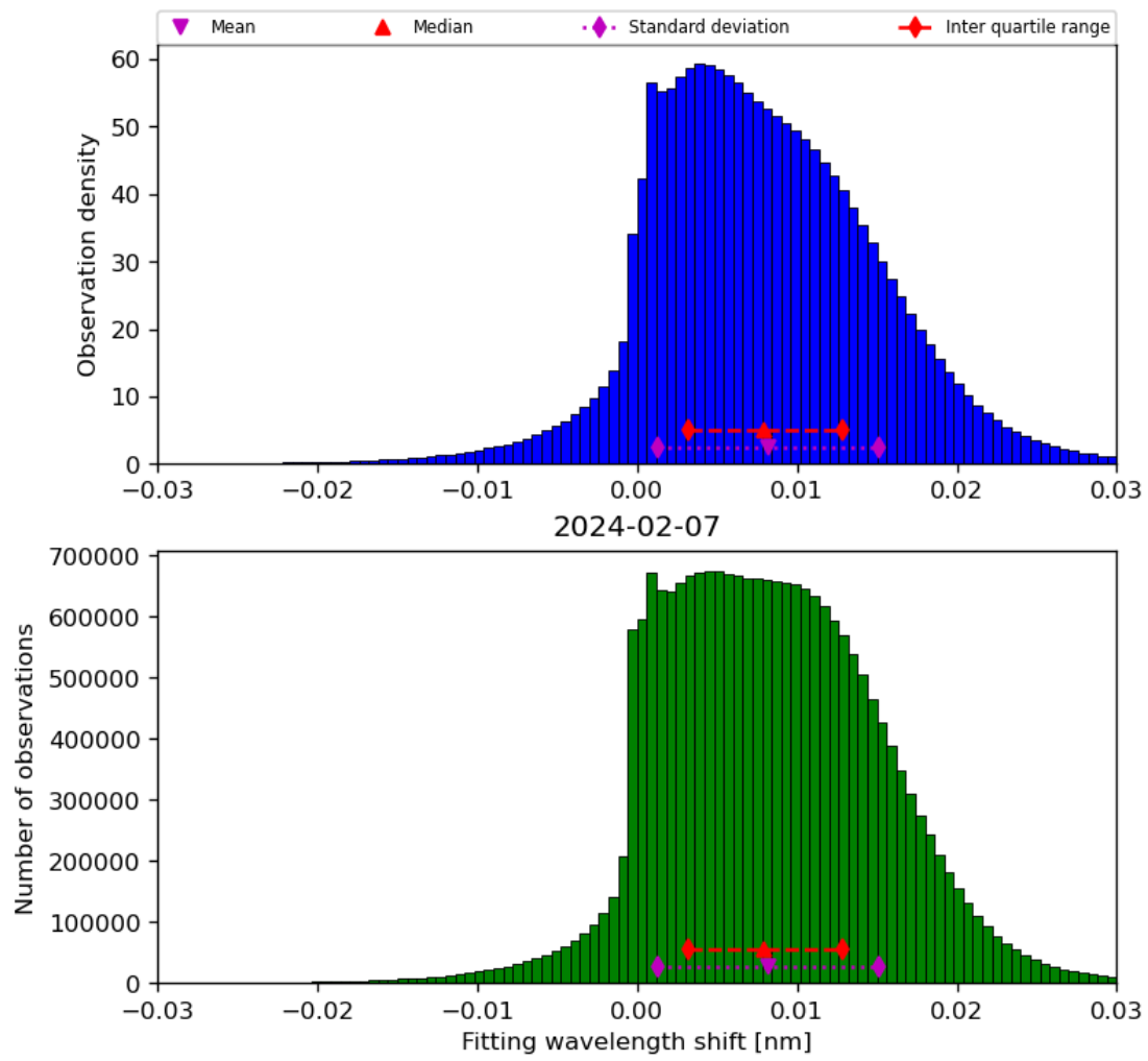
Figure 49: Histogram of “Fitting wavelength shift” for 2024-02-06 to 2024-02-08
