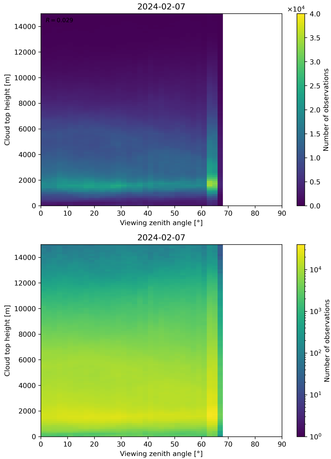
Figure 112: Scatter density plot of “Viewing zenith angle” against “Cloud top height” for 2024-02-06 to 2024-02-08.
