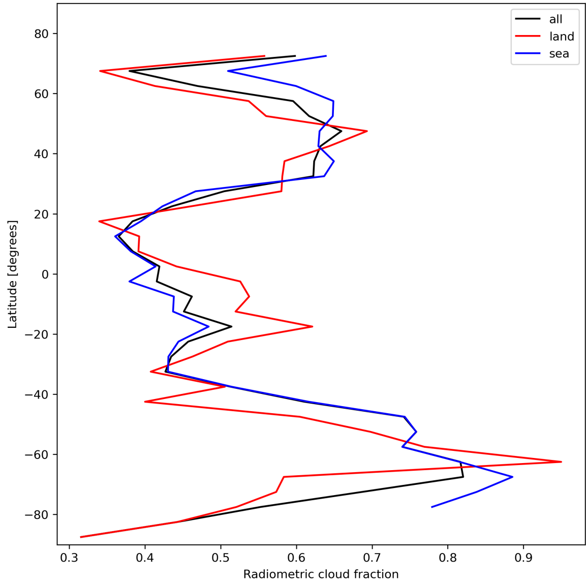
Figure 23: Zonal average of “Radiometric cloud fraction” for 2024-02-06 to 2024-02-08.
