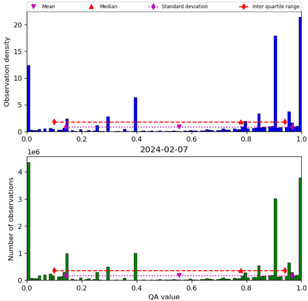
Figure 38: Histogram of “QA value” for 2024-02-06 to 2024-02-08
