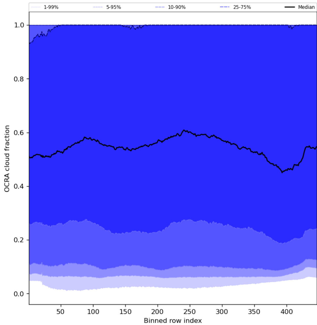
Figure 66: Along track statistics of “OCRA cloud fraction” for 2024-02-06 to 2024-02-08
