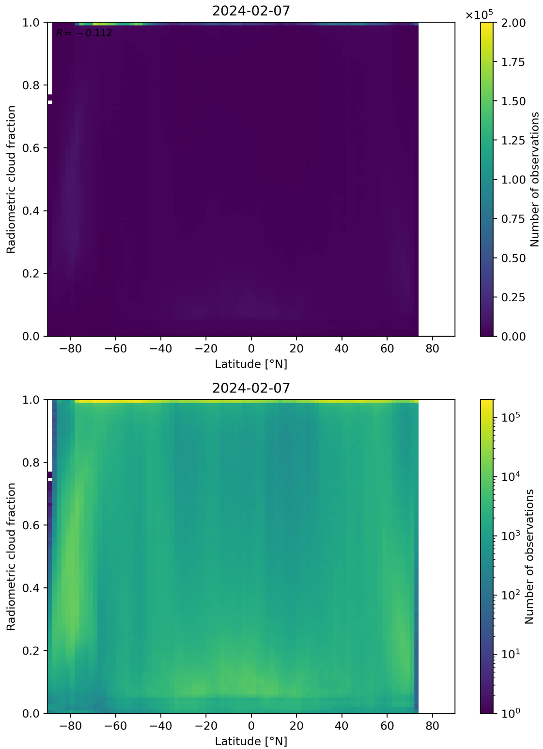
Figure 92: Scatter density plot of “Latitude” against “Radiometric cloud fraction” for 2024-02-06 to 2024-02-08.
