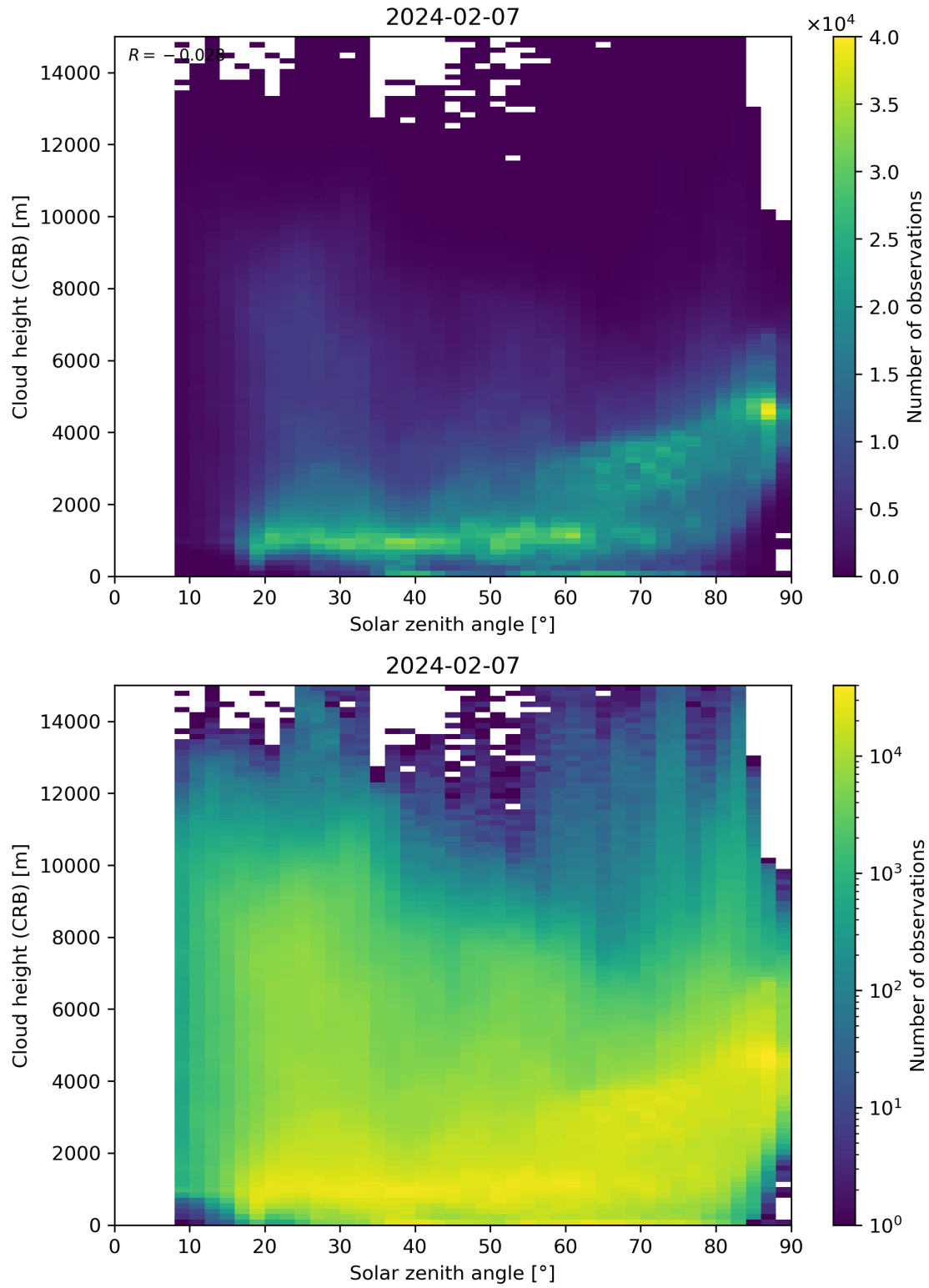
Figure 102: Scatter density plot of “Solar zenith angle” against “Cloud height (CRB)” for 2024-02-06 to 2024-02-08.
