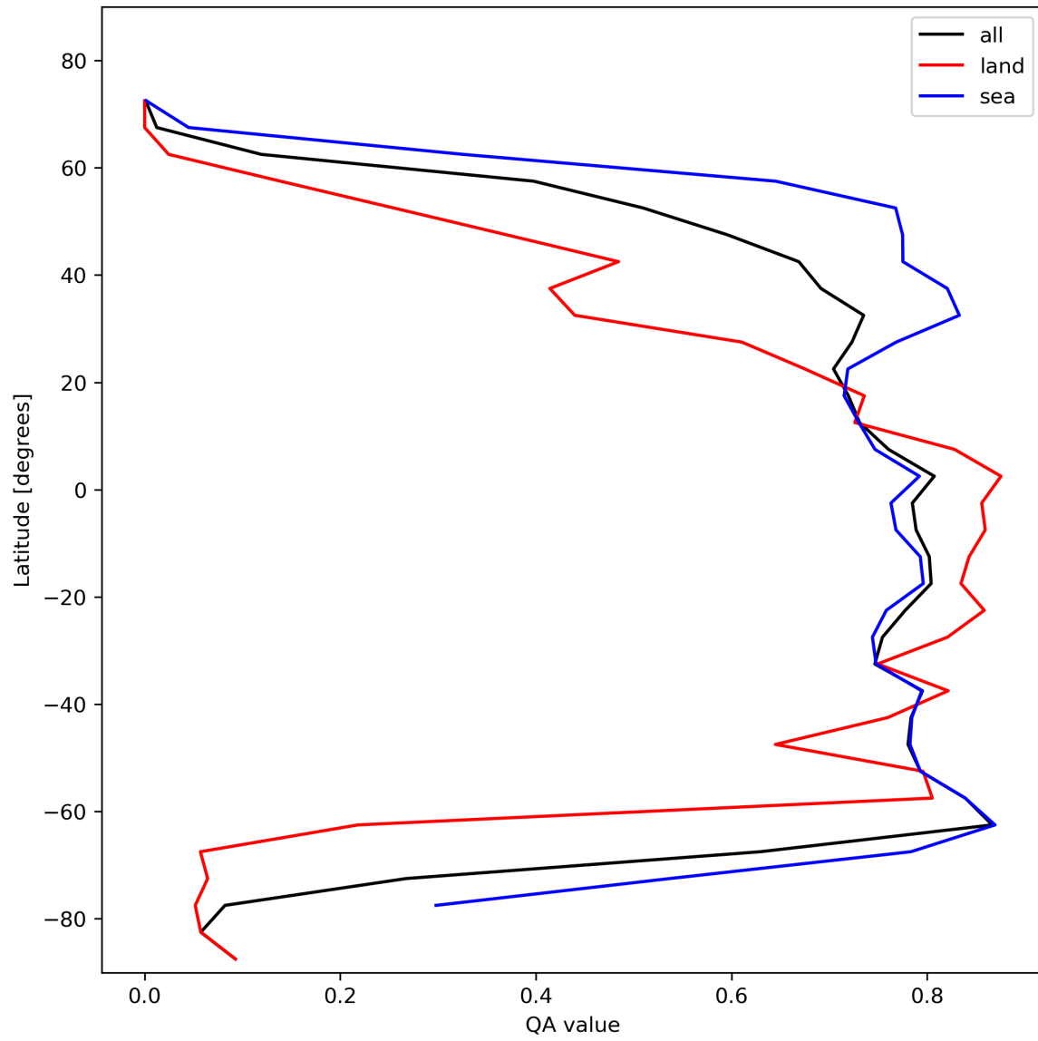
Figure 22: Zonal average of “QA value” for 2024-02-06 to 2024-02-08.
