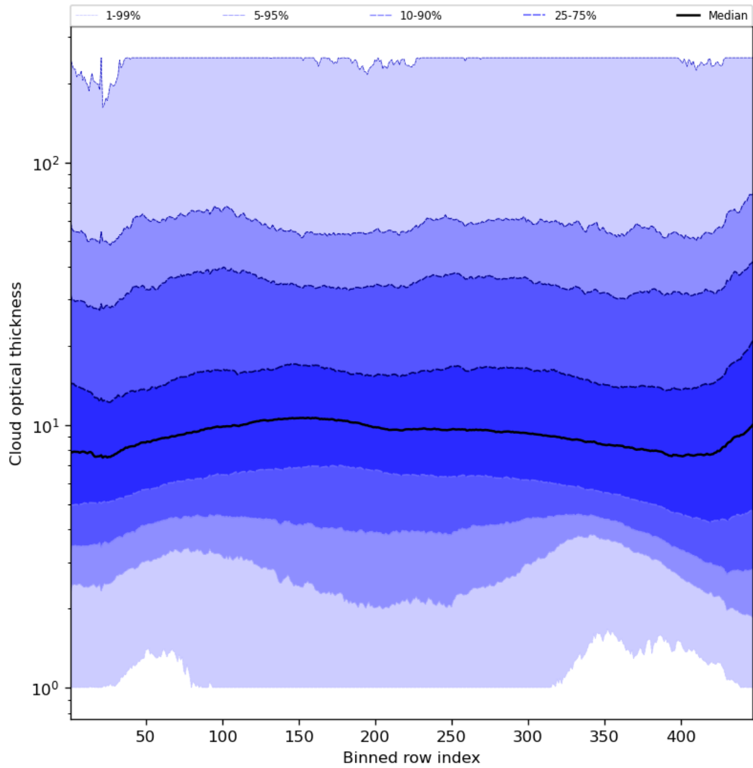
Figure 57: Along track statistics of “Cloud optical thickness” for 2024-02-06 to 2024-02-08
