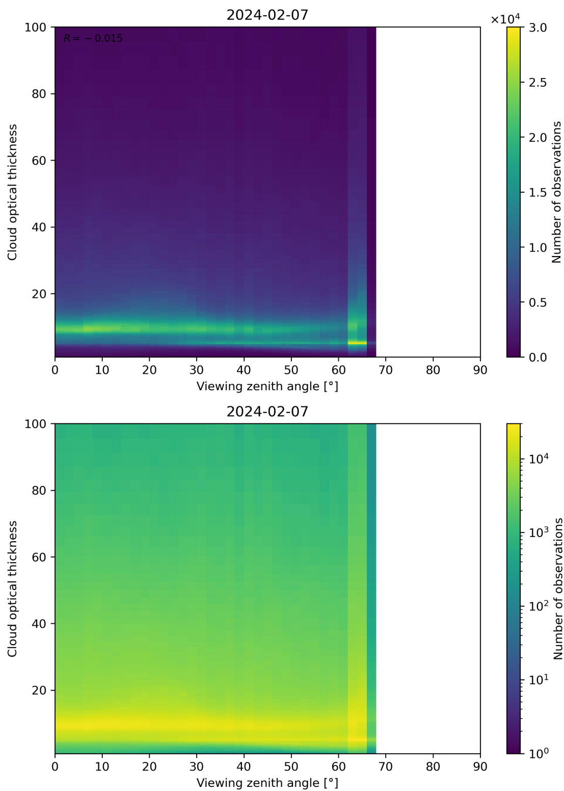
Figure 111: Scatter density plot of “Viewing zenith angle” against “Cloud optical thickness” for 2024-02-06 to 2024-02-08.
