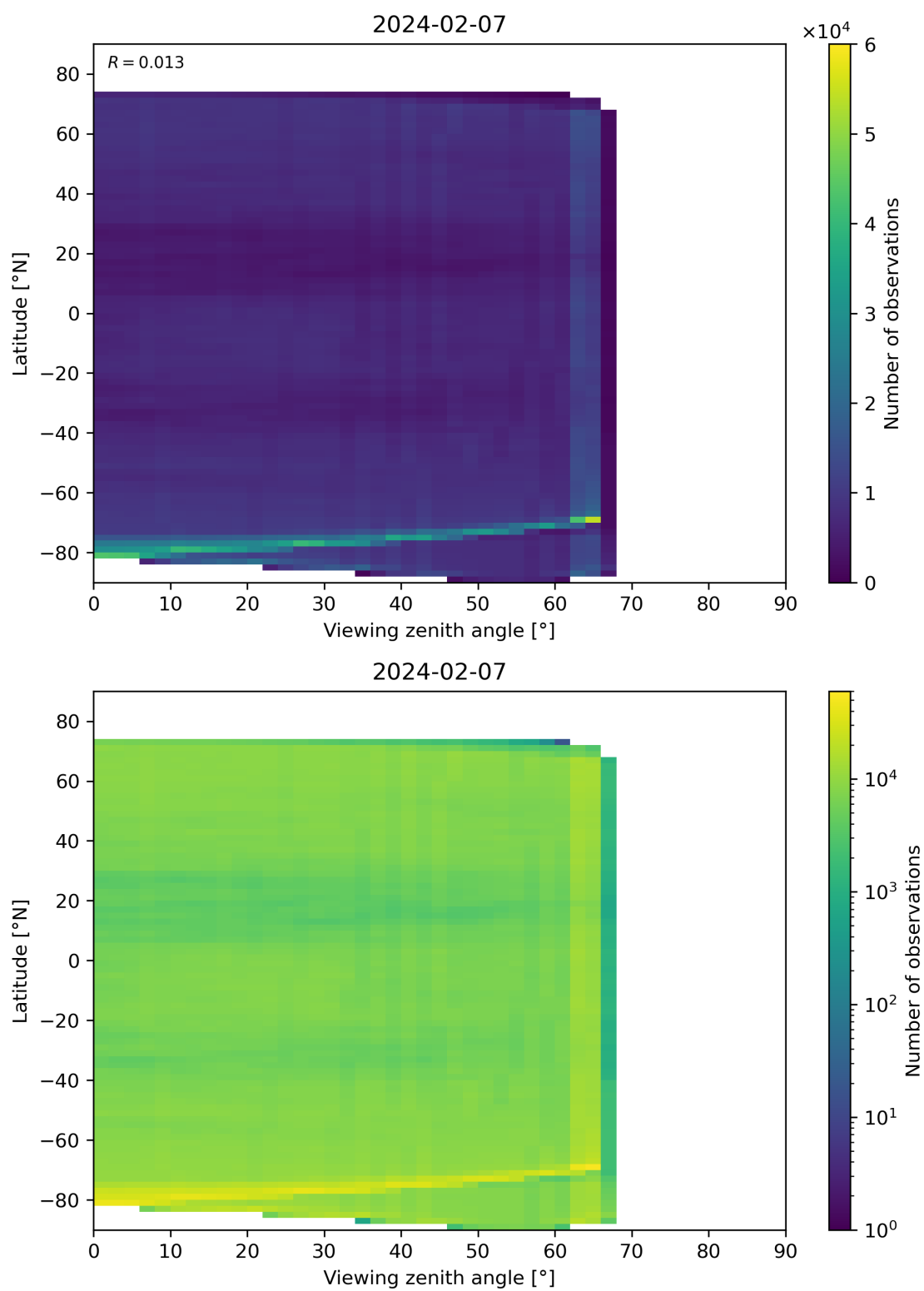
Figure 113: Scatter density plot of “Viewing zenith angle” against “Latitude” for 2024-02-06 to 2024-02-08.
