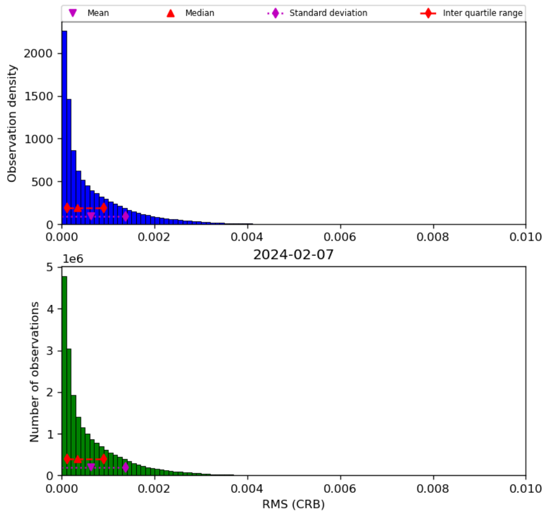
Figure 48: Histogram of “RMS (CRB)” for 2024-02-06 to 2024-02-08
