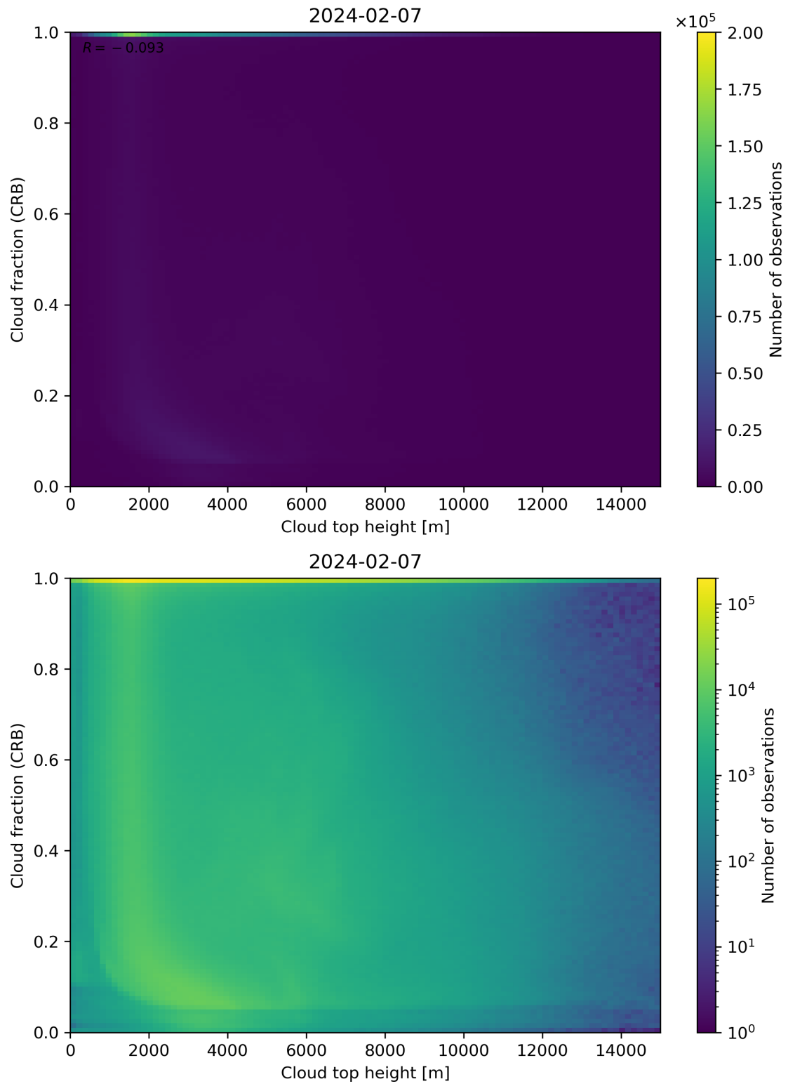
Figure 88: Scatter density plot of “Cloud top height” against “Cloud fraction (CRB)” for 2024-02-06 to 2024-02-08.
