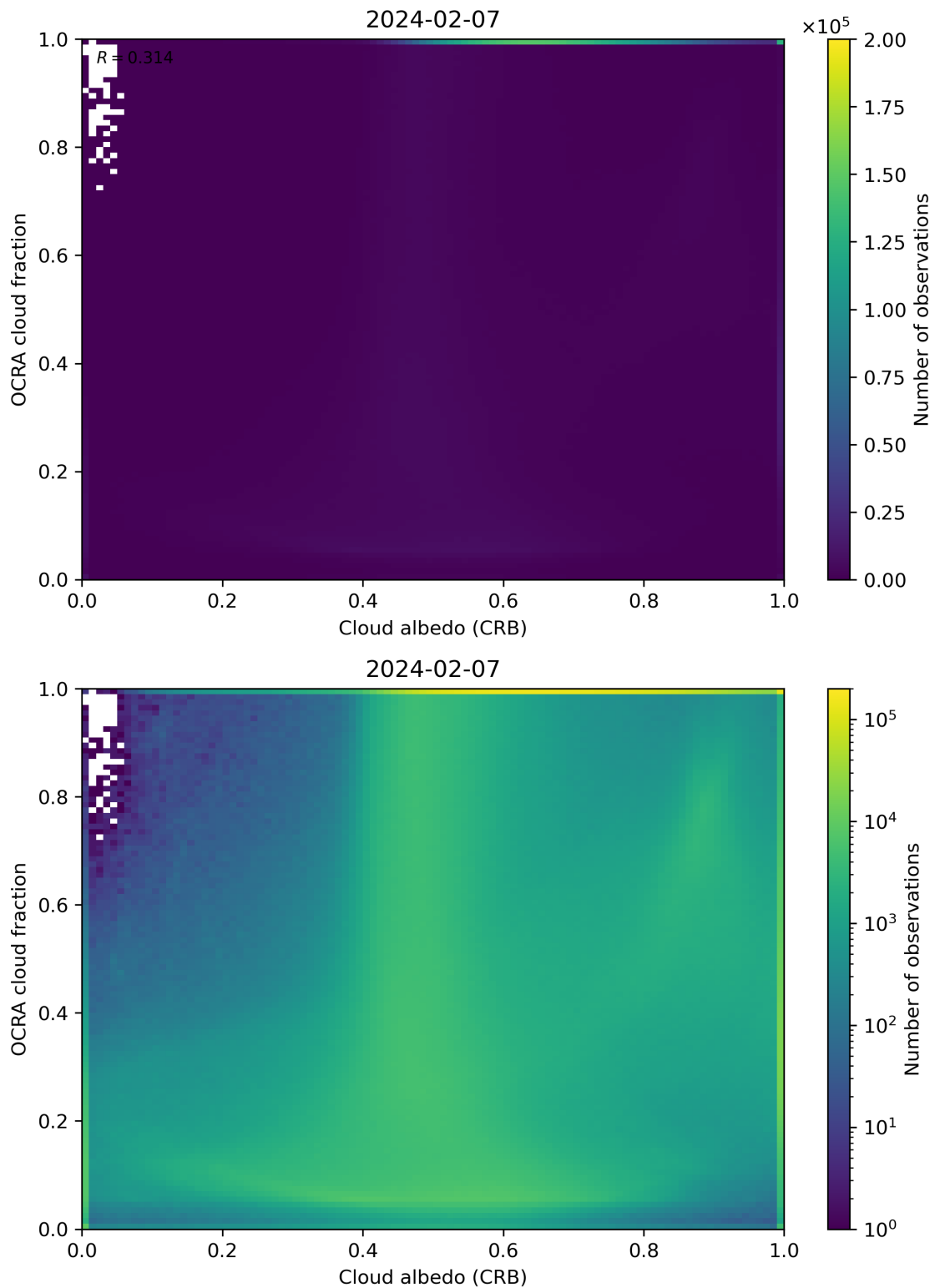
Figure 70: Scatter density plot of “Cloud albedo (CRB)” against “OCRA cloud fraction” for 2024-02-06 to 2024-02-08.
