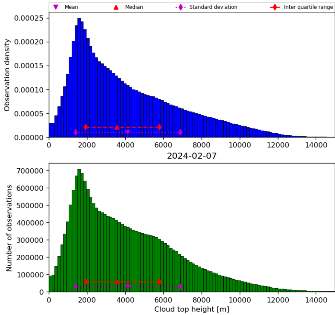
Figure 40: Histogram of “Cloud top height” for 2024-02-06 to 2024-02-08
