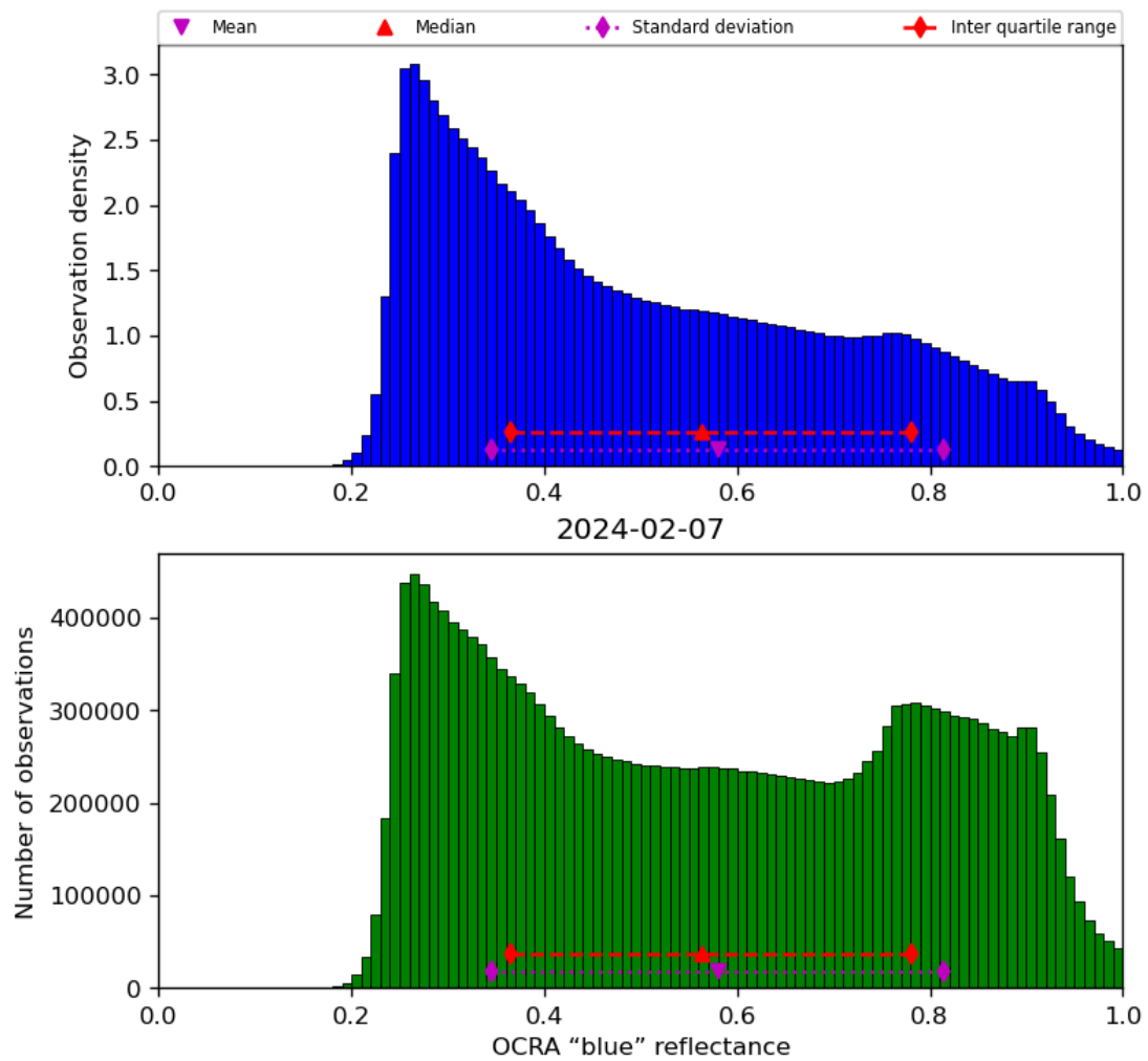
Figure 51: Histogram of “OCRA “blue” reflectance” for 2024-02-06 to 2024-02-08
