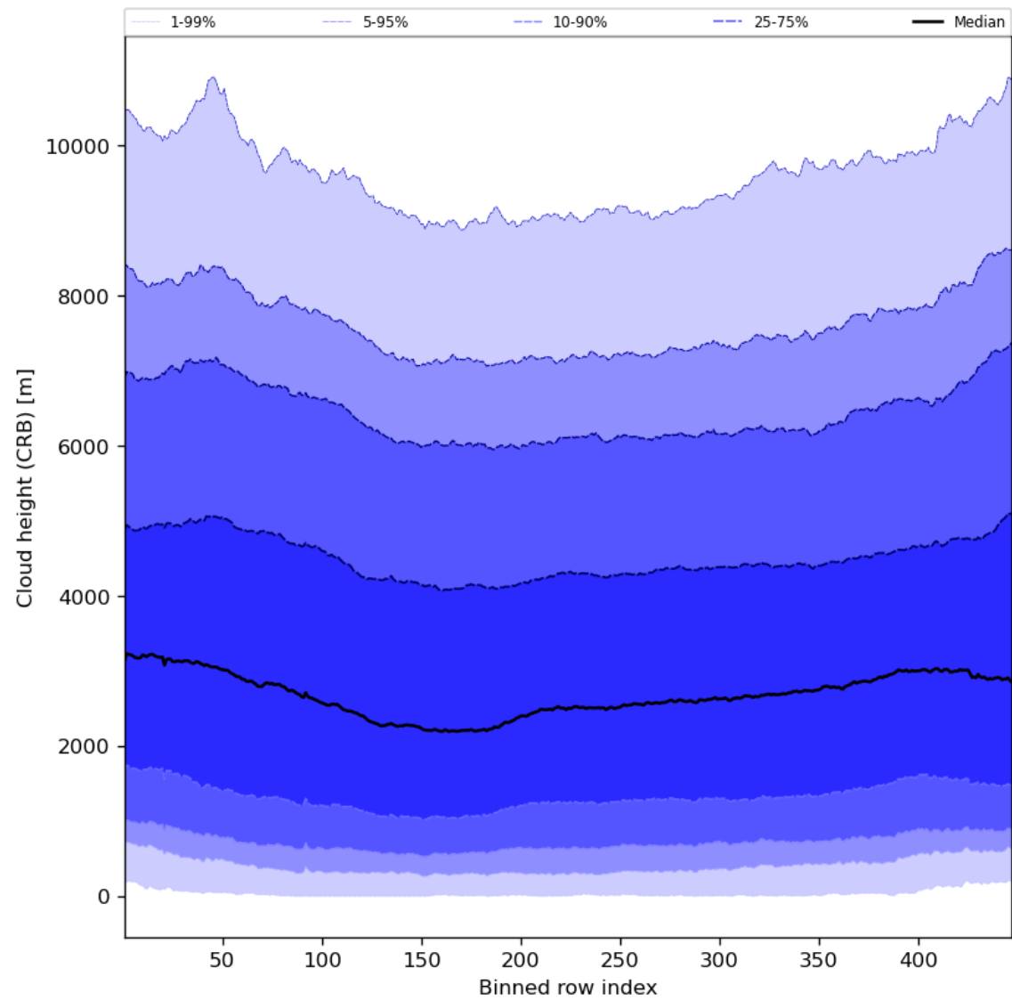
Figure 59: Along track statistics of “Cloud height (CRB)” for 2024-02-06 to 2024-02-08
