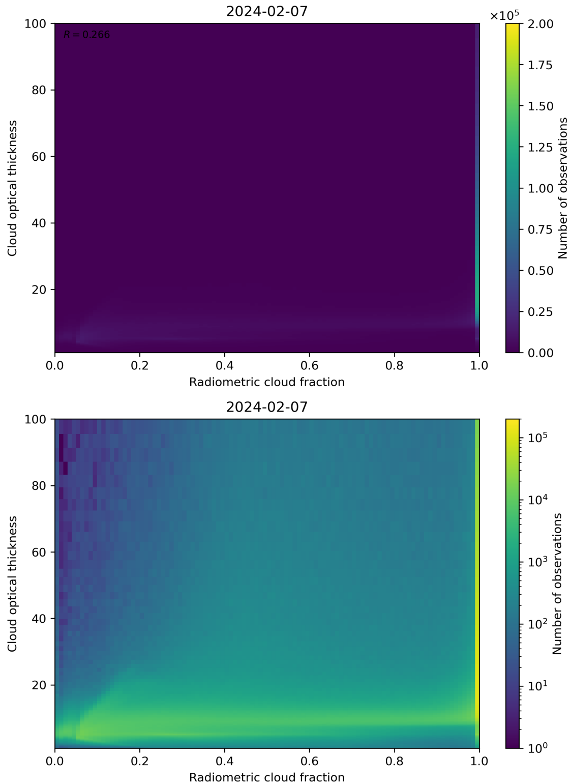
Figure 75: Scatter density plot of “Radiometric cloud fraction” against “Cloud optical thickness” for 2024-02-06 to 2024-02-08.
