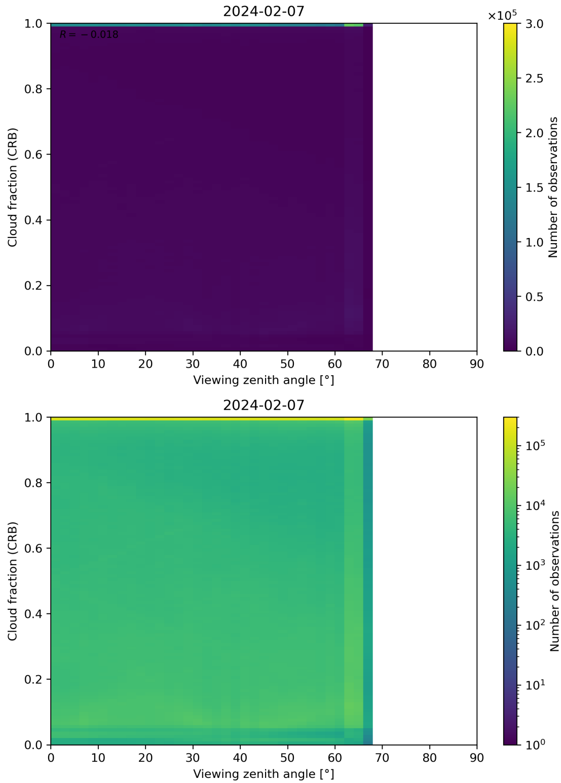
Figure 109: Scatter density plot of “Viewing zenith angle” against “Cloud fraction (CRB)” for 2024-02-06 to 2024-02-08.
