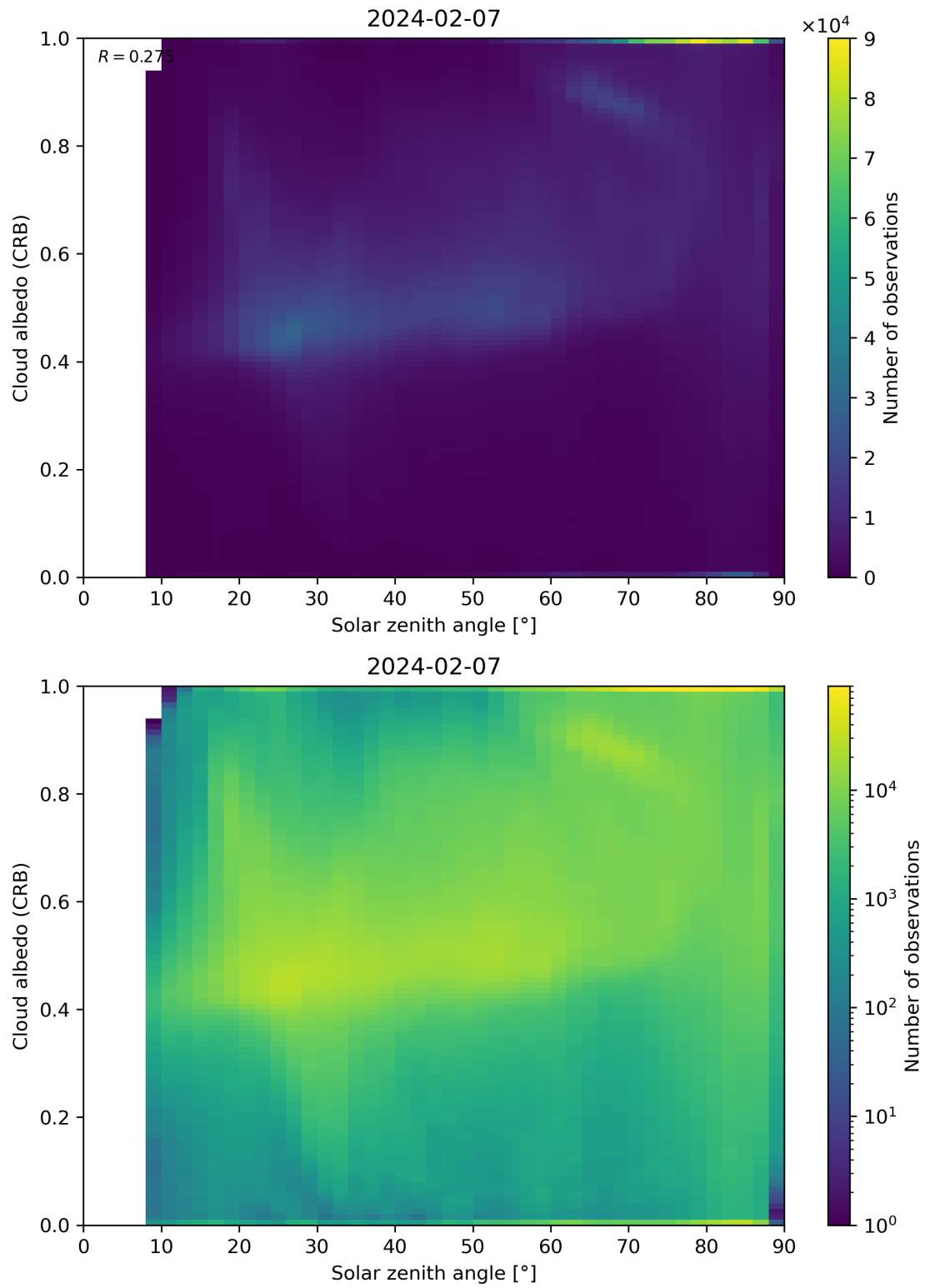
Figure 98: Scatter density plot of “Solar zenith angle” against “Cloud albedo (CRB)” for 2024-02-06 to 2024-02-08.
