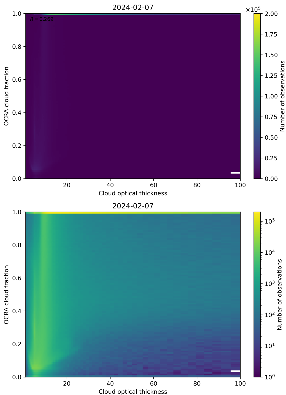
Figure 83: Scatter density plot of “Cloud optical thickness” against “OCRA cloud fraction” for 2024-02-06 to 2024-02-08.
