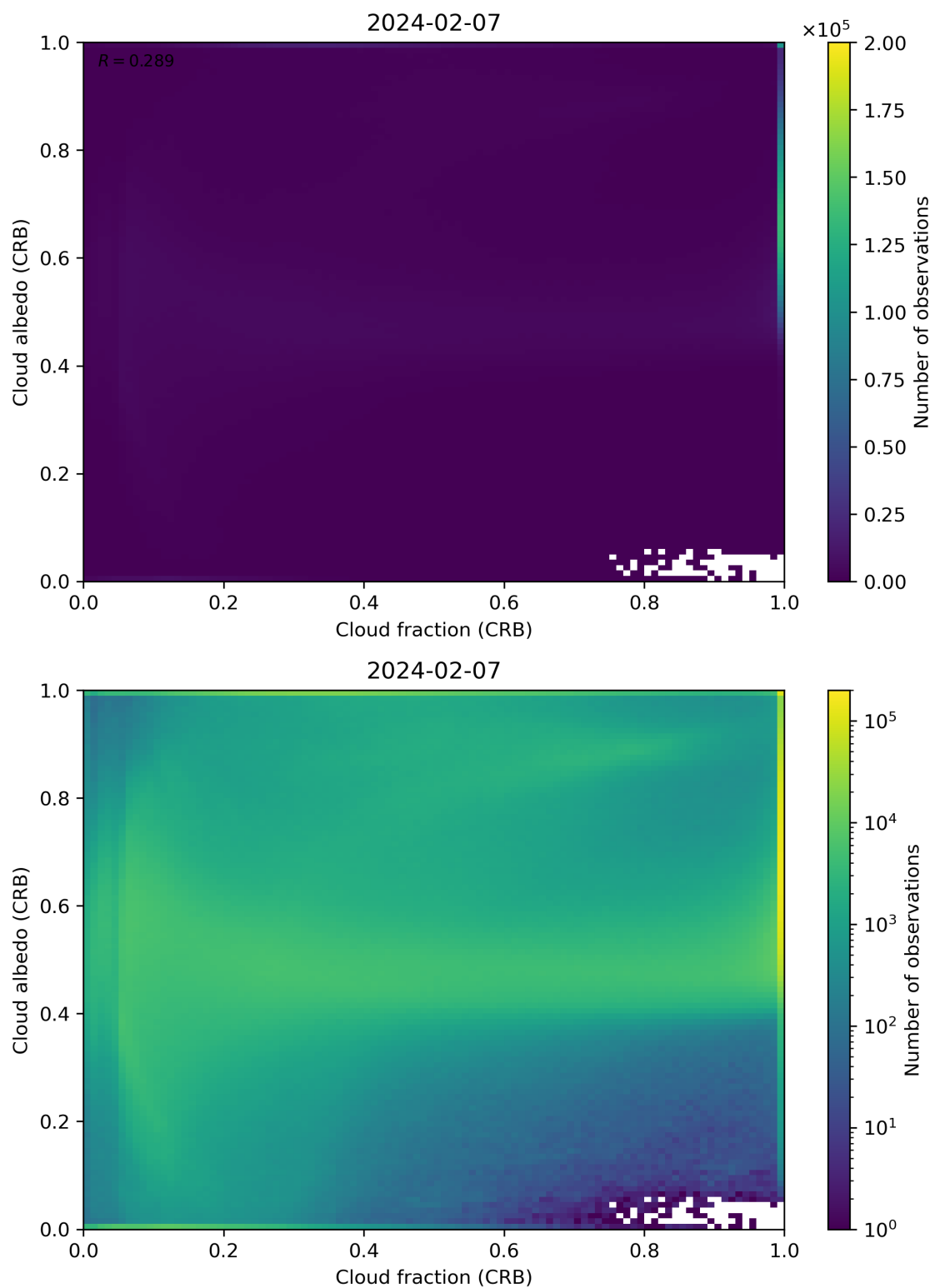
Figure 77: Scatter density plot of “Cloud fraction (CRB)” against “Cloud albedo (CRB)” for 2024-02-06 to 2024-02-08.
