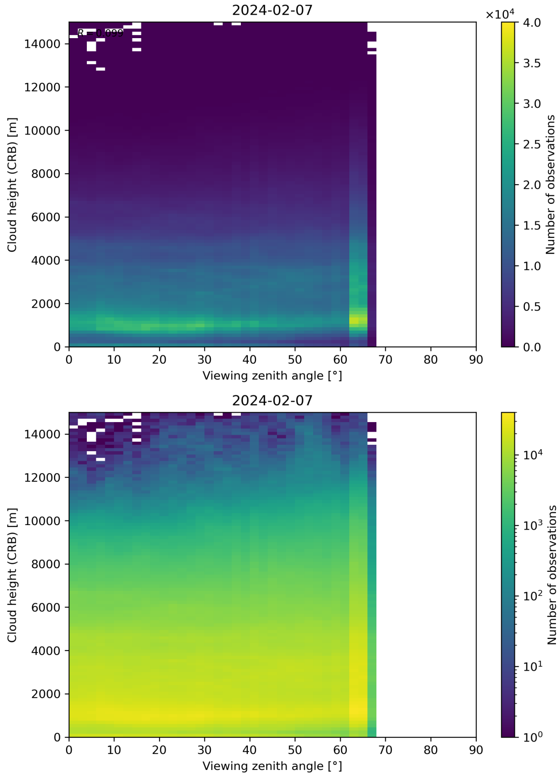
Figure 110: Scatter density plot of “Viewing zenith angle” against “Cloud height (CRB)” for 2024-02-06 to 2024-02-08.
