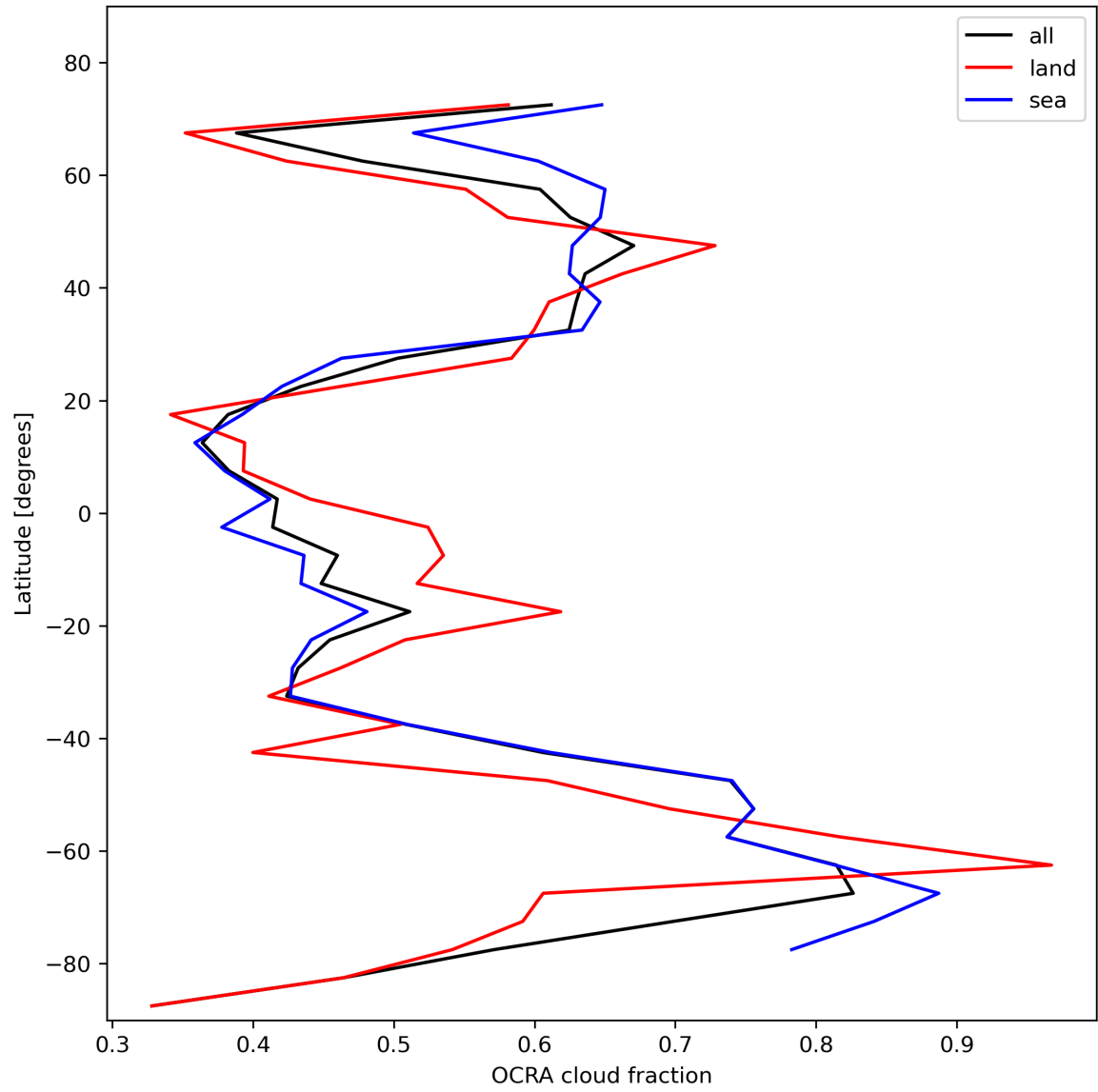
Figure 34: Zonal average of “OCRA cloud fraction” for 2024-02-06 to 2024-02-08.
