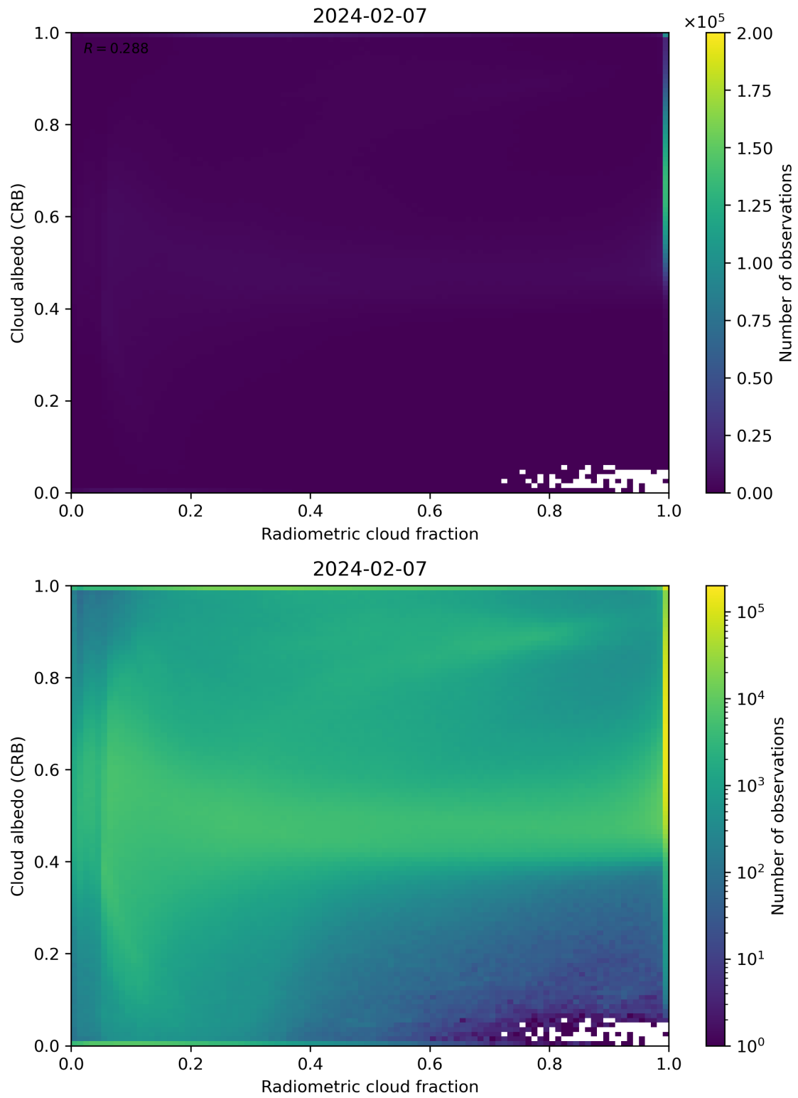
Figure 71: Scatter density plot of “Radiometric cloud fraction” against “Cloud albedo (CRB)” for 2024-02-06 to 2024-02-08.
