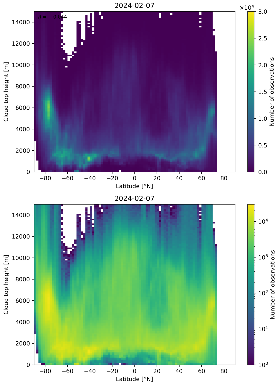
Figure 97: Scatter density plot of “Latitude” against “Cloud top height” for 2024-02-06 to 2024-02-08.
