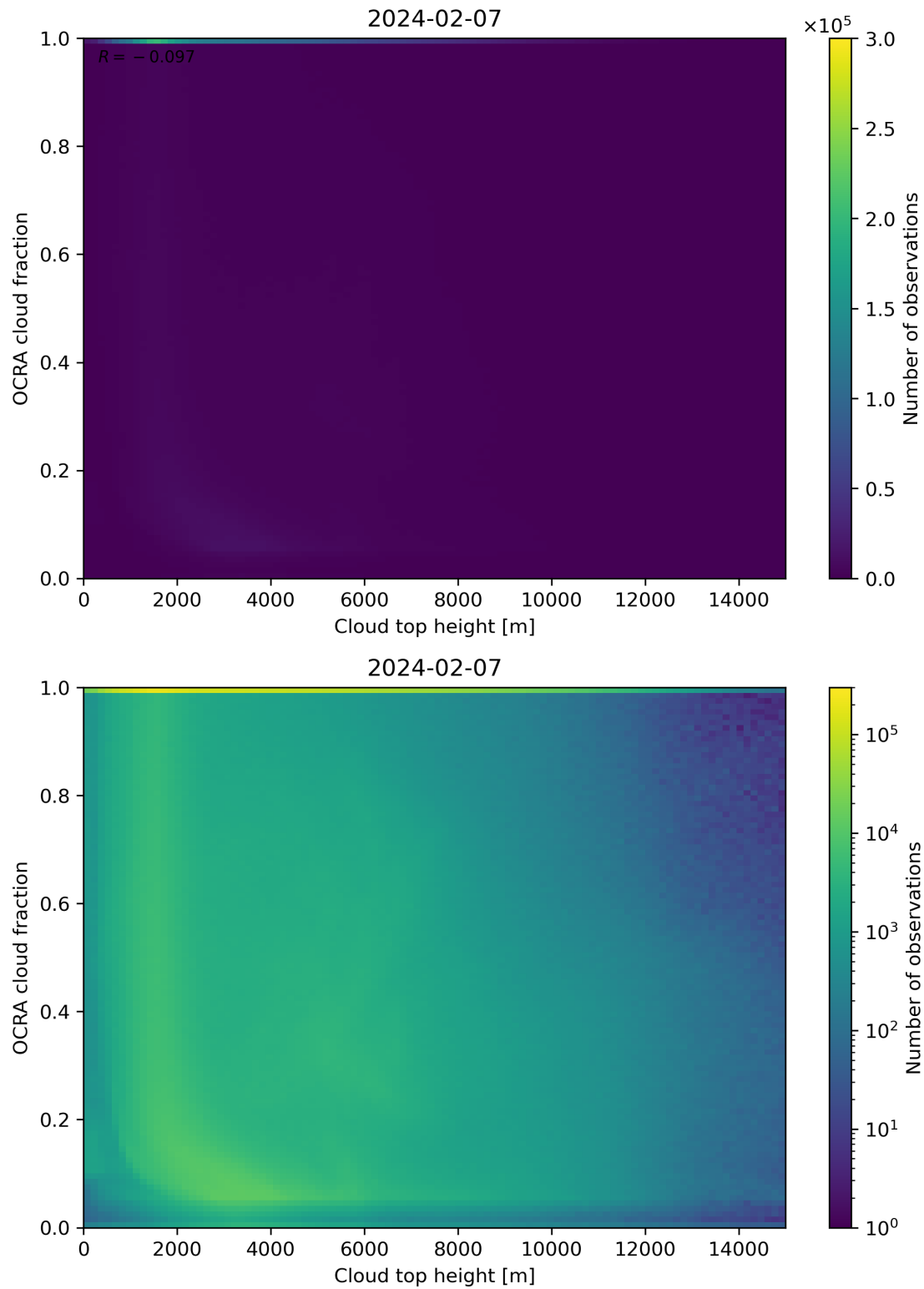
Figure 87: Scatter density plot of “Cloud top height” against “OCRA cloud fraction” for 2024-02-06 to 2024-02-08.
