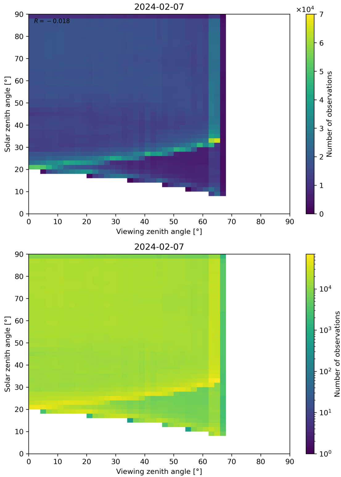
Figure 114: Scatter density plot of “Viewing zenith angle” against “Solar zenith angle” for 2024-02-06 to 2024-02-08.
