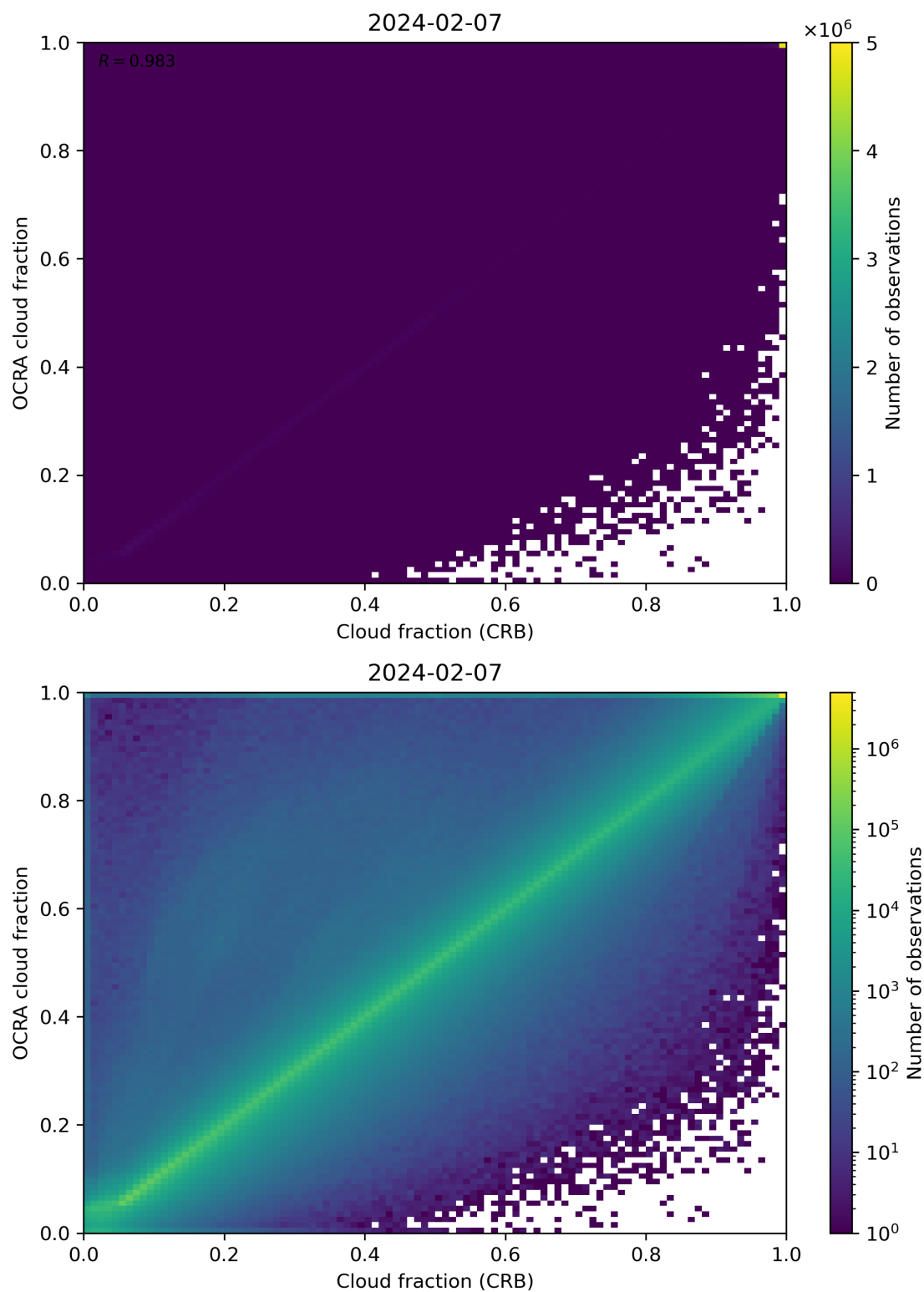
Figure 78: Scatter density plot of “Cloud fraction (CRB)” against “OCRA cloud fraction” for 2024-02-06 to 2024-02-08.
