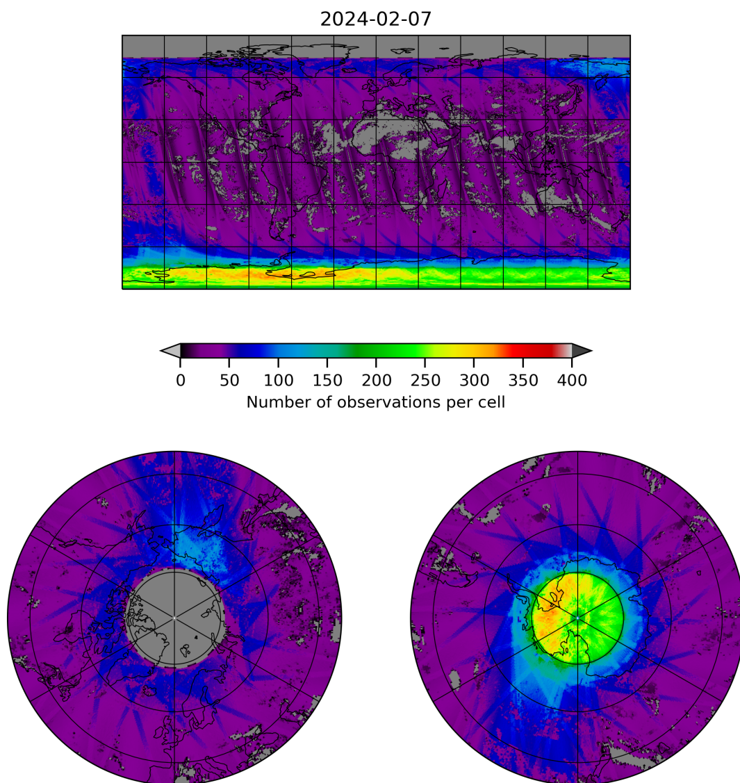
Figure 21: Map of the number of observations for 2024-02-06 to 2024-02-08
