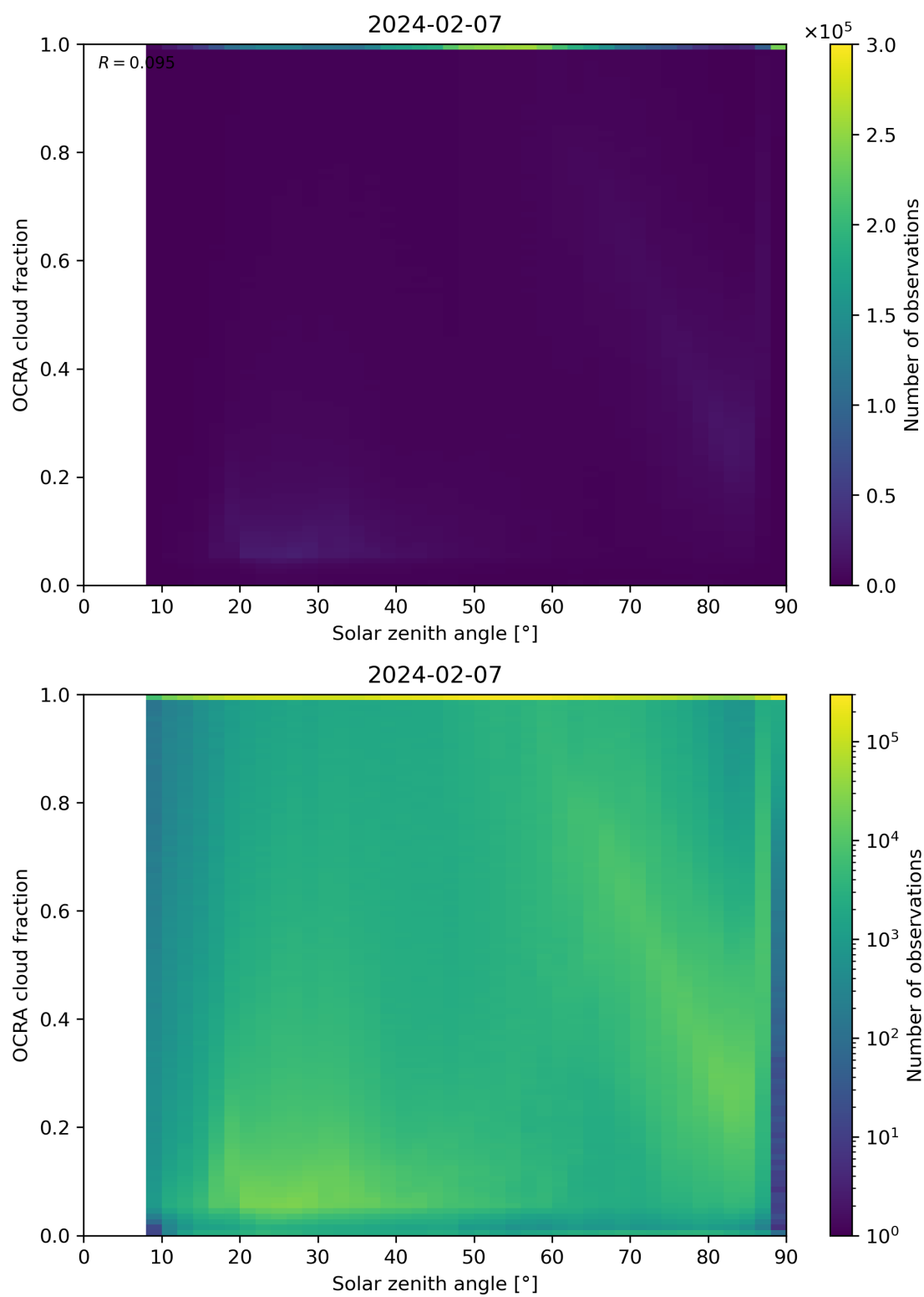
Figure 100: Scatter density plot of “Solar zenith angle” against “OCRA cloud fraction” for 2024-02-06 to 2024-02-08.
