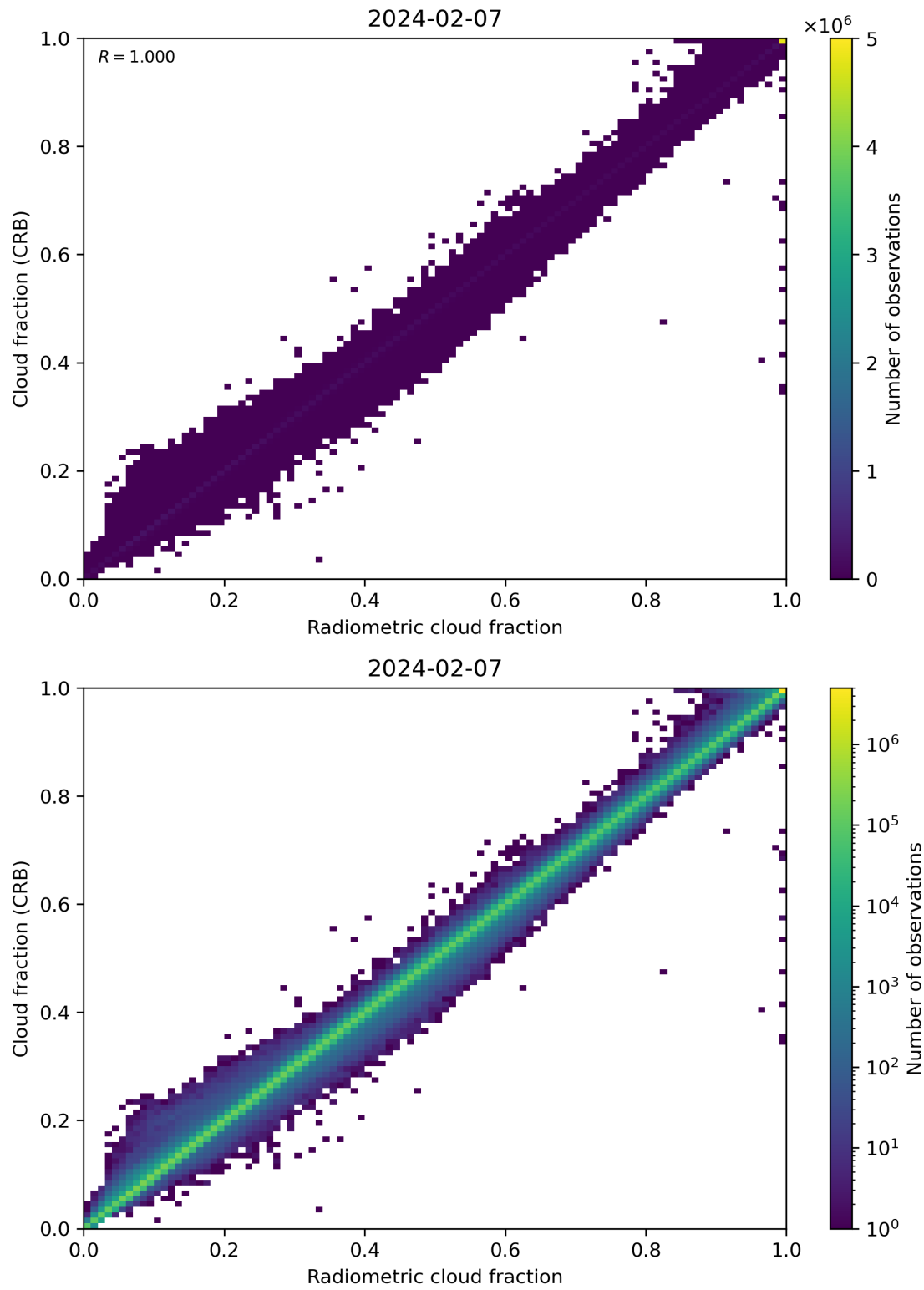
Figure 73: Scatter density plot of “Radiometric cloud fraction” against “Cloud fraction (CRB)” for 2024-02-06 to 2024-02-08.
