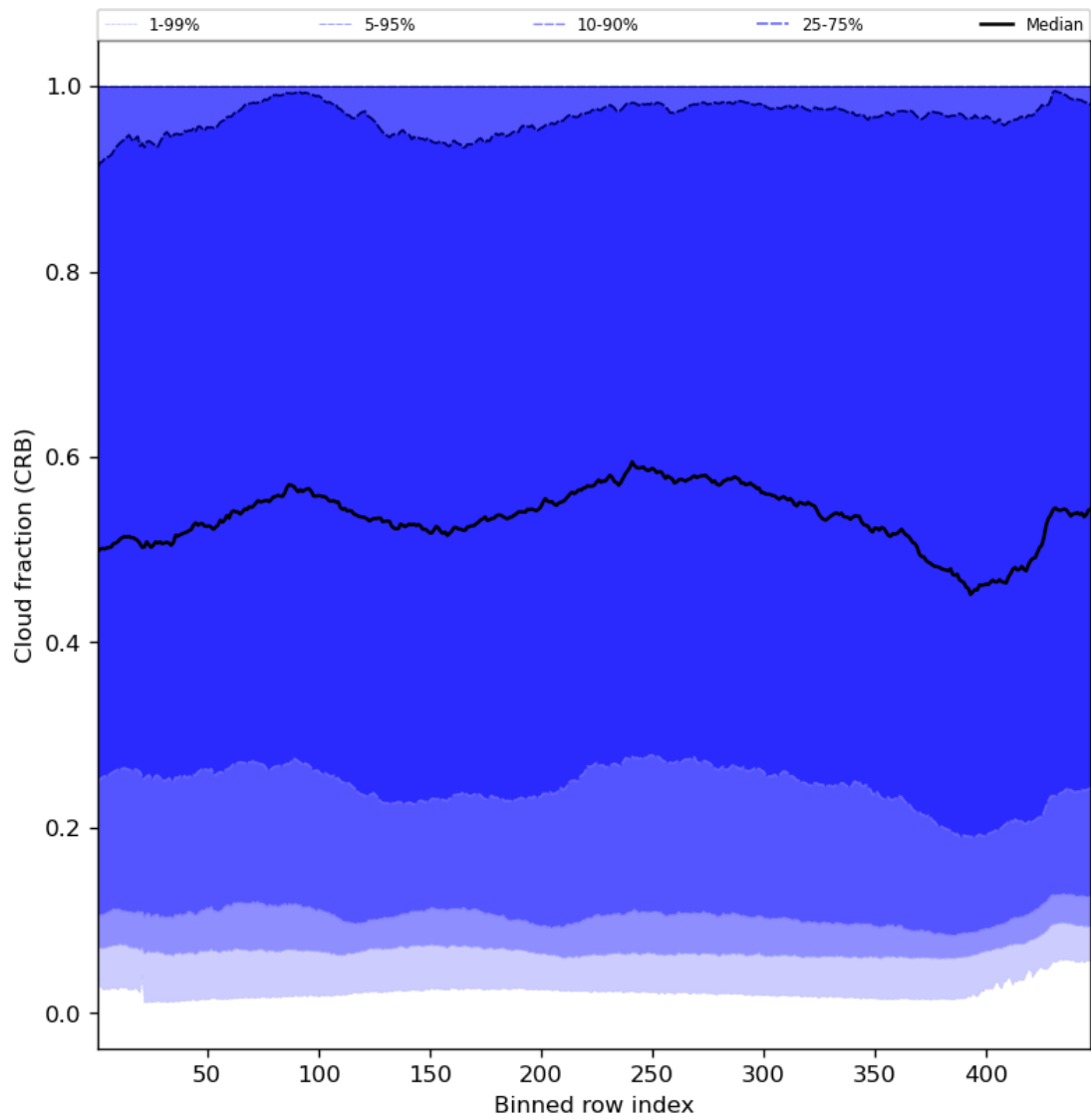
Figure 58: Along track statistics of “Cloud fraction (CRB)” for 2024-02-06 to 2024-02-08
