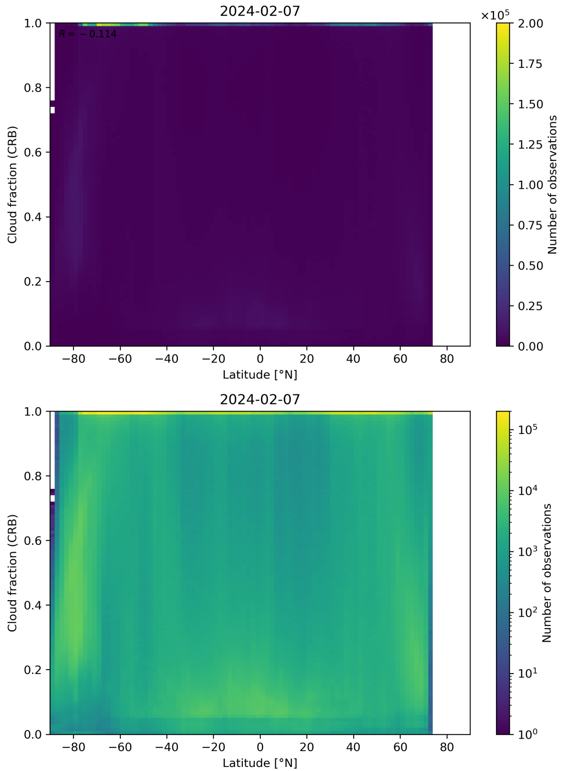
Figure 94: Scatter density plot of “Latitude” against “Cloud fraction (CRB)” for 2024-02-06 to 2024-02-08.
