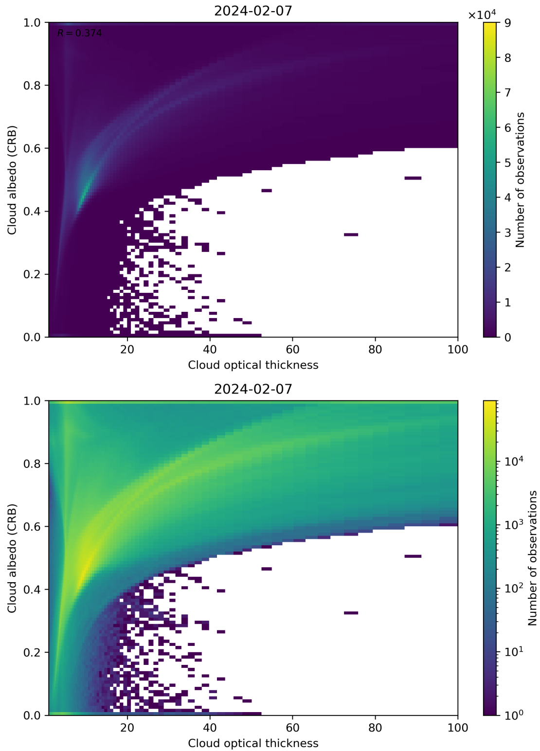
Figure 82: Scatter density plot of “Cloud optical thickness” against “Cloud albedo (CRB)” for 2024-02-06 to 2024-02-08.
