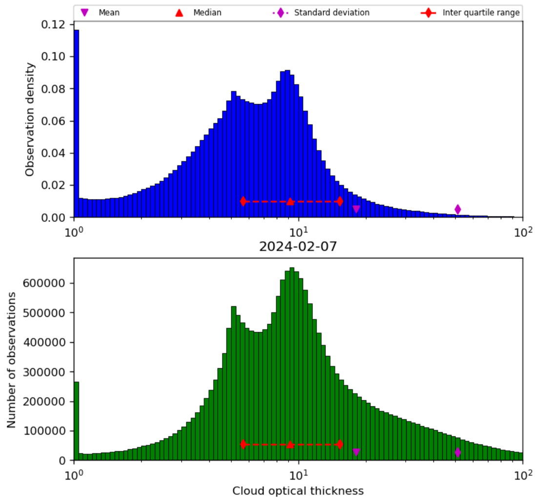
Figure 41: Histogram of “Cloud optical thickness” for 2024-02-06 to 2024-02-08
