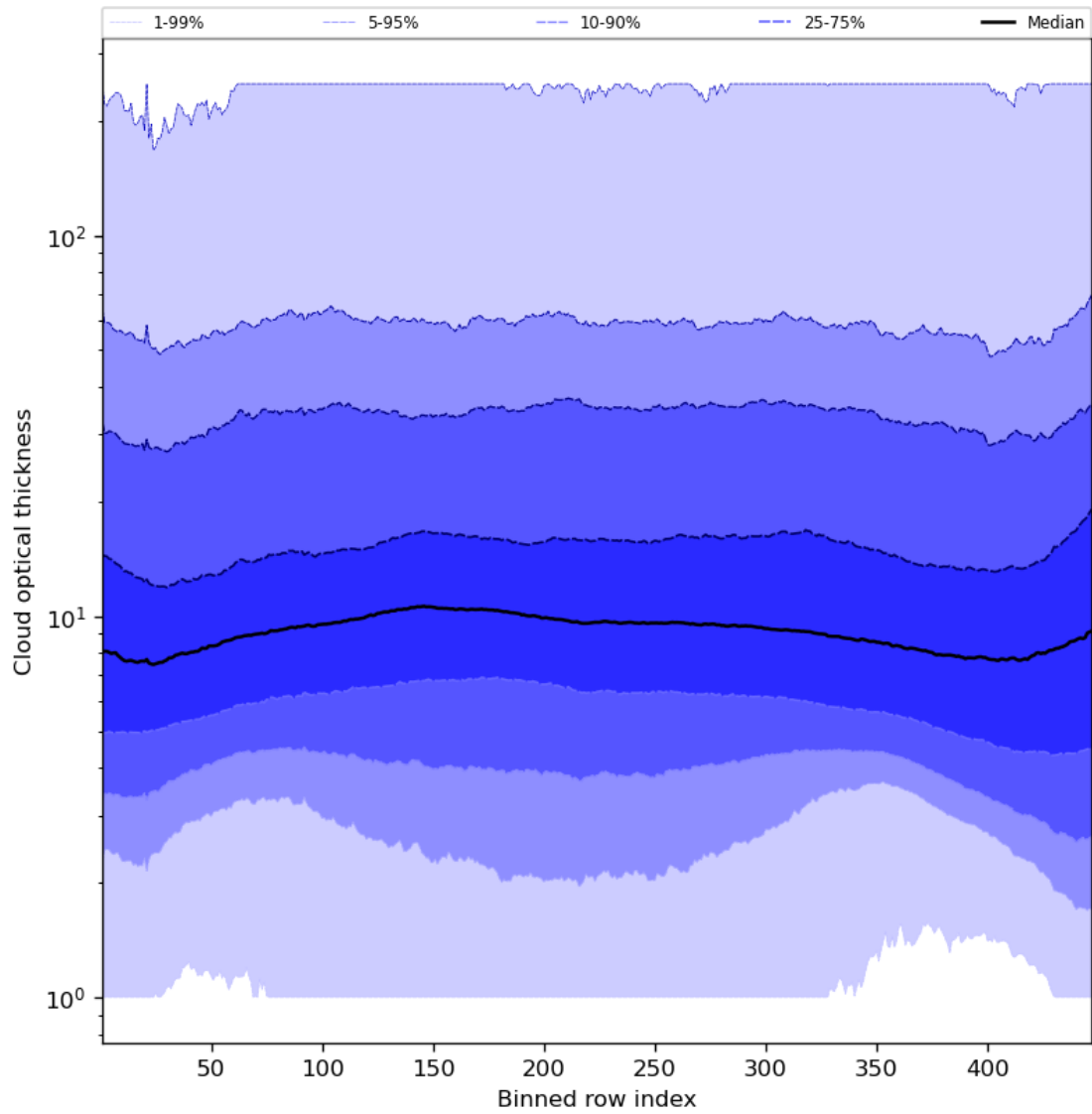
Figure 57: Along track statistics of “Cloud optical thickness” for 2024-02-07 to 2024-02-09
