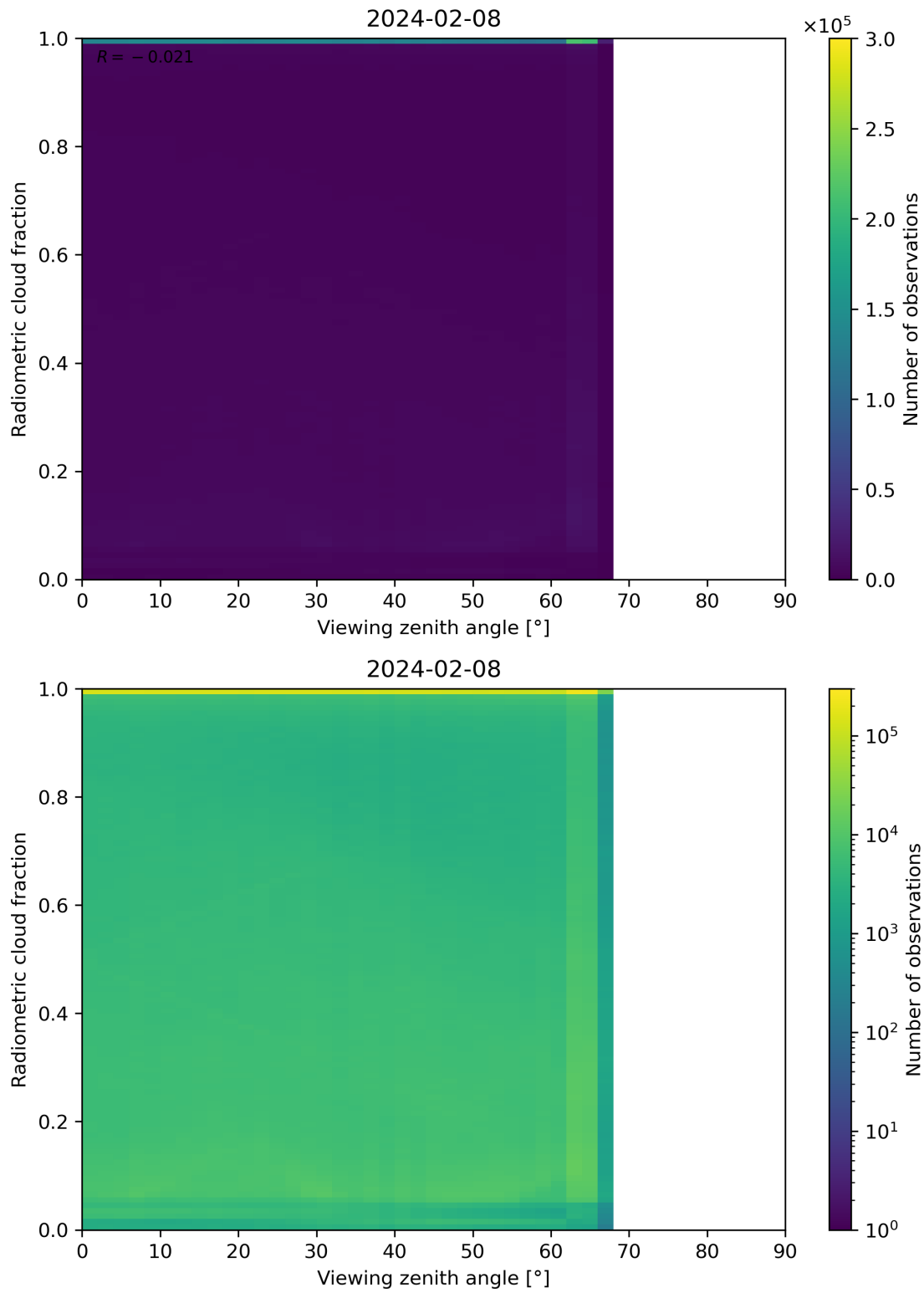
Figure 107: Scatter density plot of “Viewing zenith angle” against “Radiometric cloud fraction” for 2024-02-07 to 2024-02-09.
