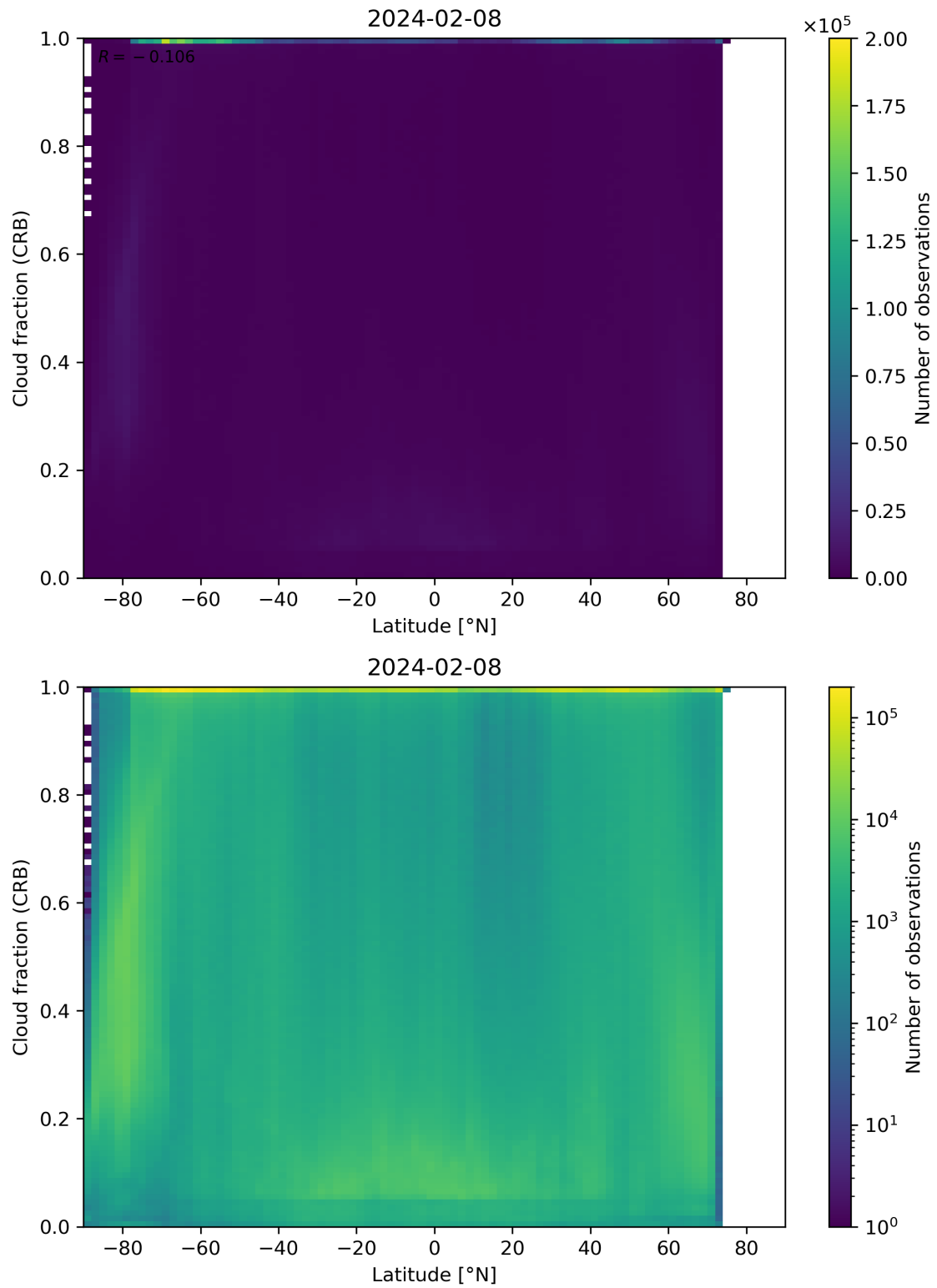
Figure 94: Scatter density plot of “Latitude” against “Cloud fraction (CRB)” for 2024-02-07 to 2024-02-09.
