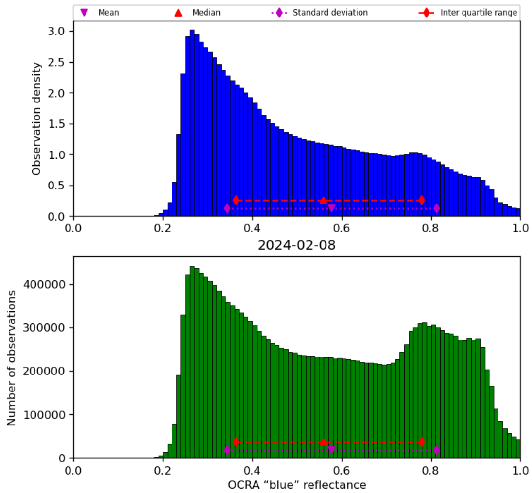
Figure 51: Histogram of “OCRA “blue” reflectance” for 2024-02-07 to 2024-02-09
