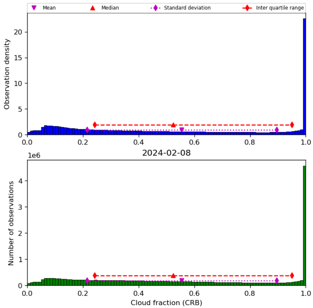
Figure 42: Histogram of “Cloud fraction (CRB)” for 2024-02-07 to 2024-02-09
