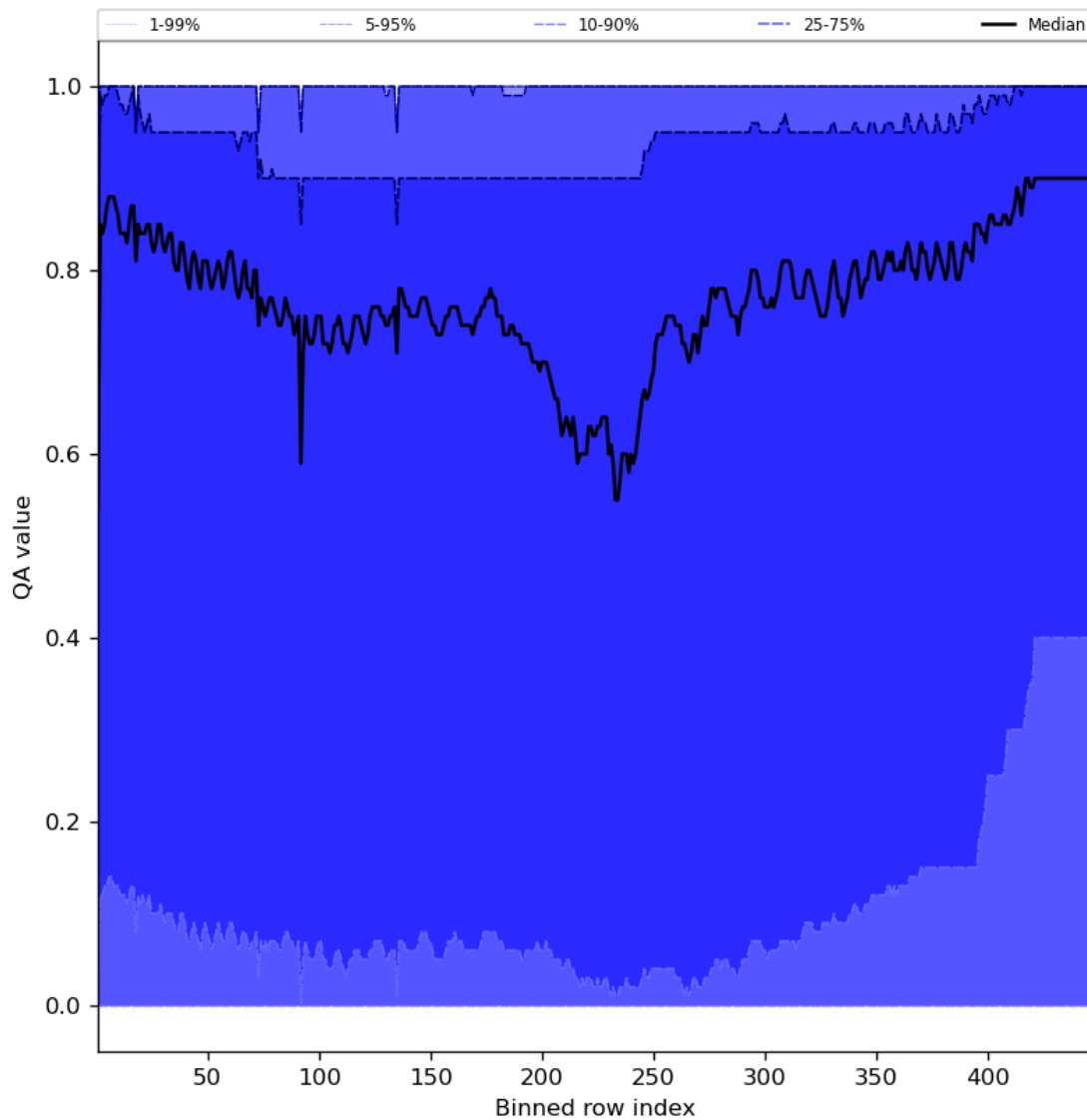
Figure 54: Along track statistics of “QA value” for 2024-02-07 to 2024-02-09
