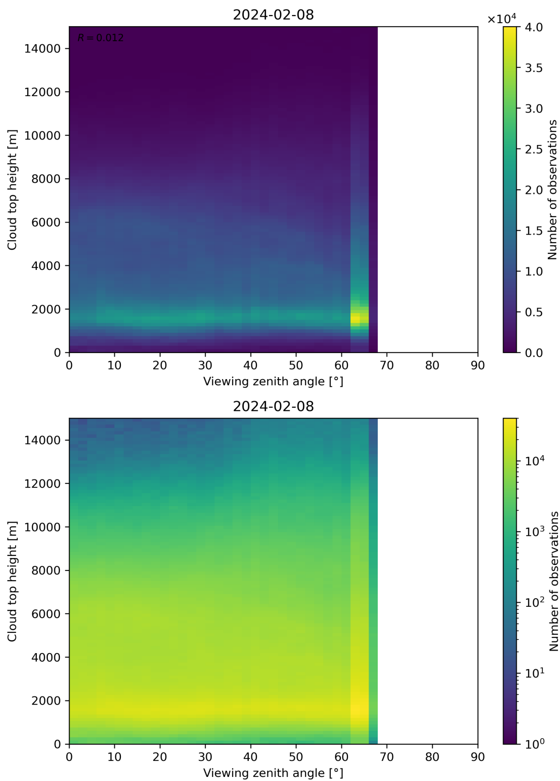
Figure 112: Scatter density plot of “Viewing zenith angle” against “Cloud top height” for 2024-02-07 to 2024-02-09.
