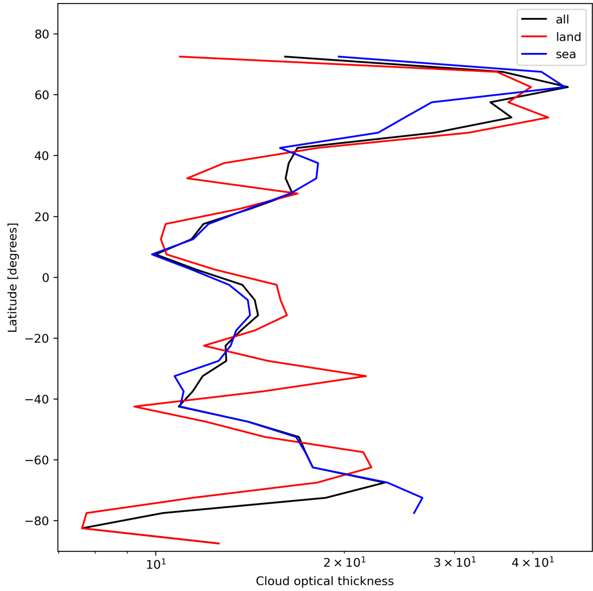
Figure 25: Zonal average of “Cloud optical thickness” for 2024-02-07 to 2024-02-09.
