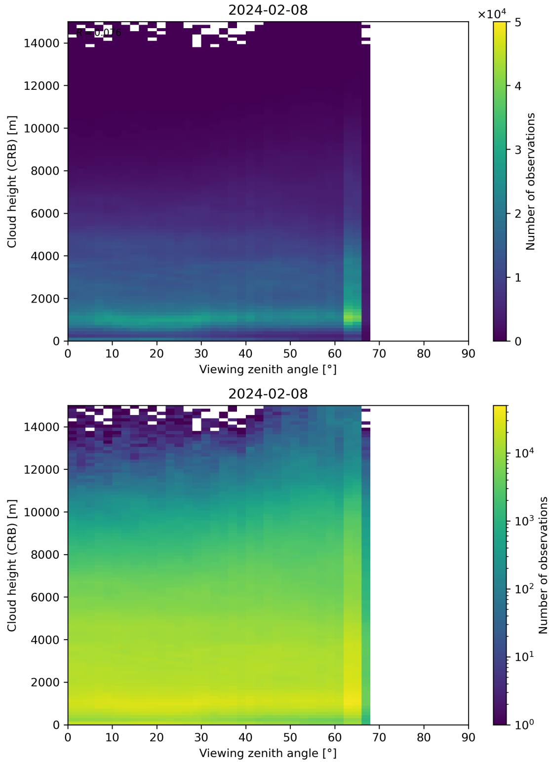
Figure 110: Scatter density plot of “Viewing zenith angle” against “Cloud height (CRB)” for 2024-02-07 to 2024-02-09.
