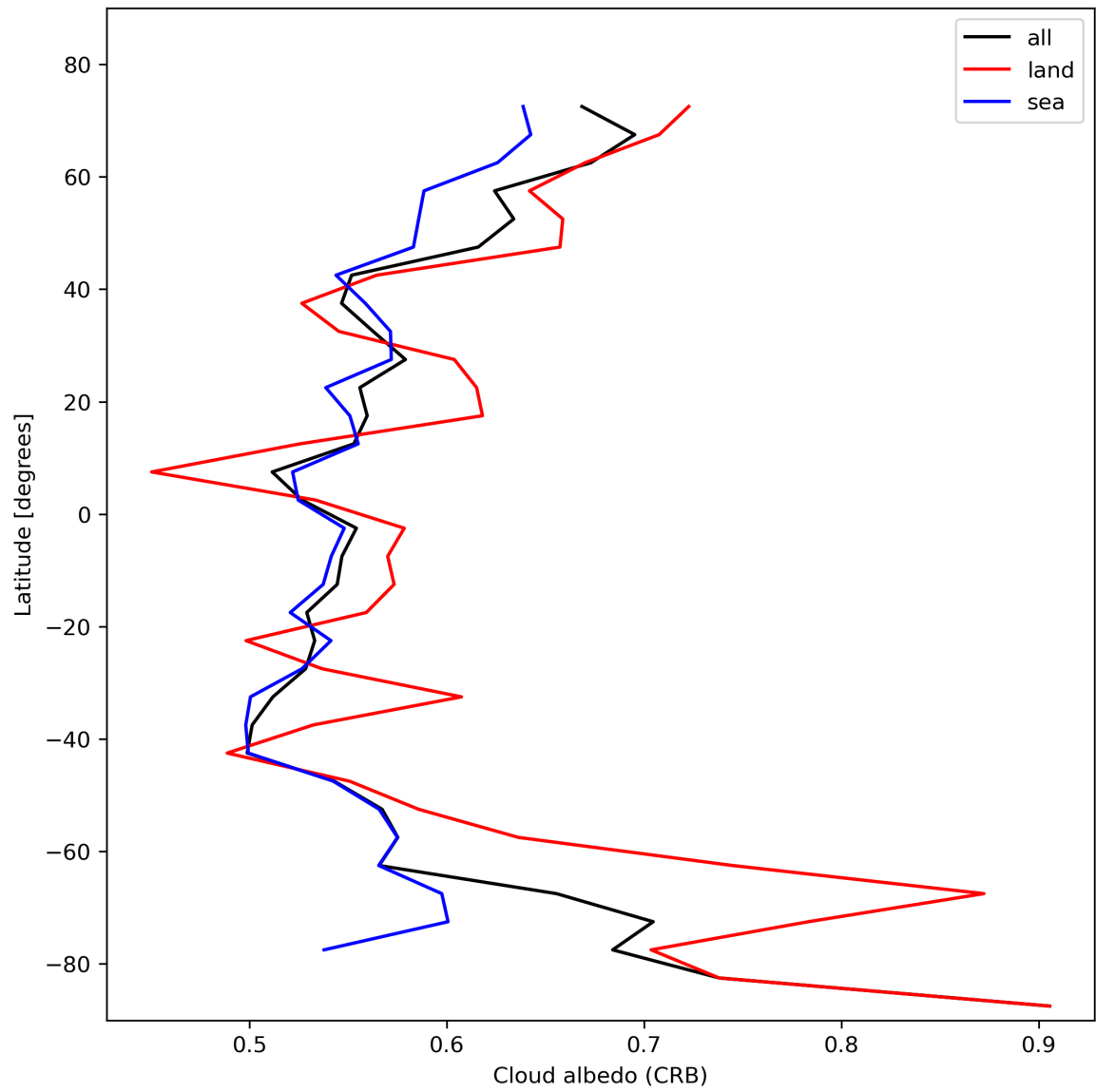
Figure 28: Zonal average of “Cloud albedo (CRB)” for 2024-02-07 to 2024-02-09.
