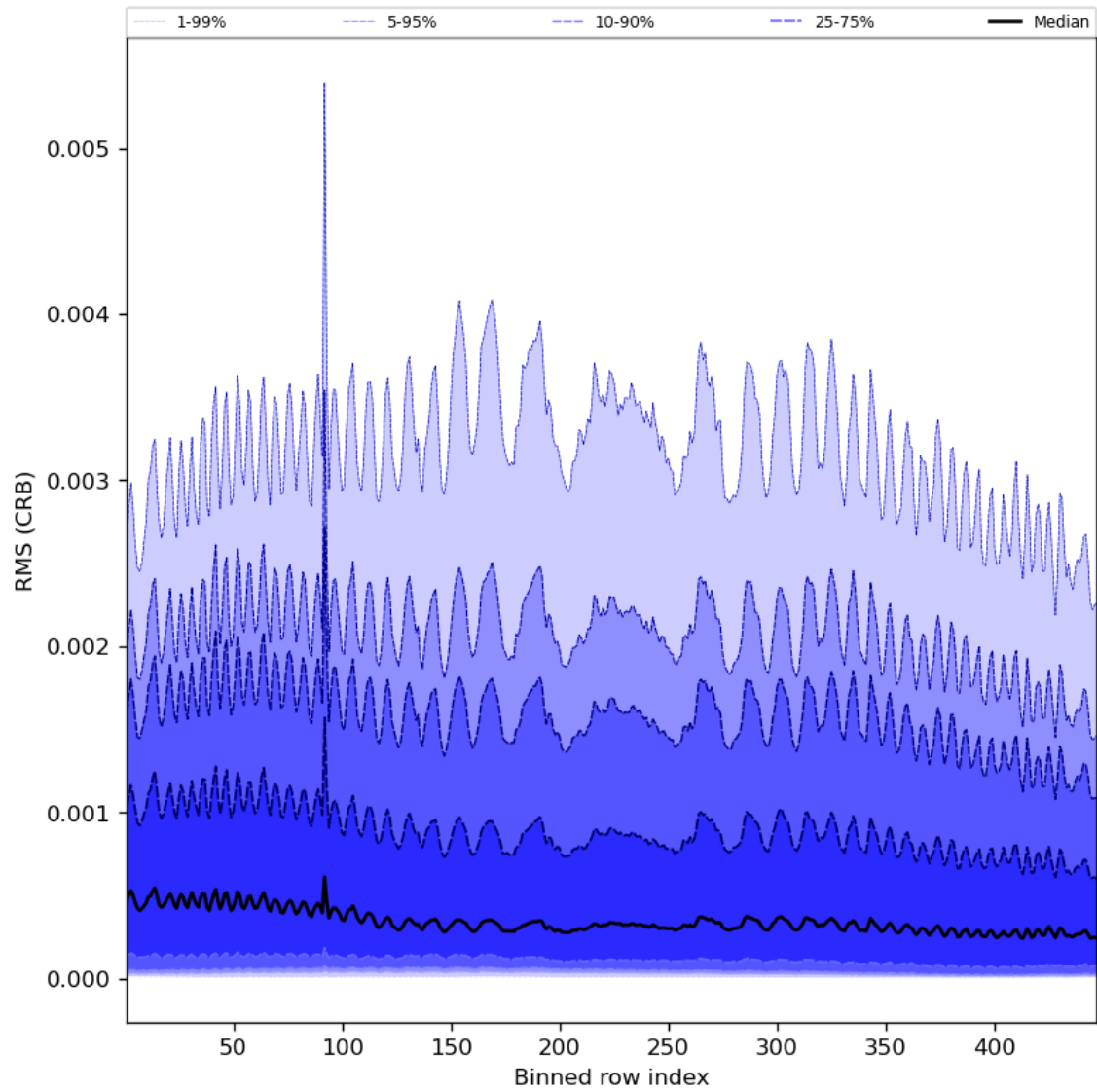
Figure 64: Along track statistics of “RMS (CRB)” for 2024-02-07 to 2024-02-09
