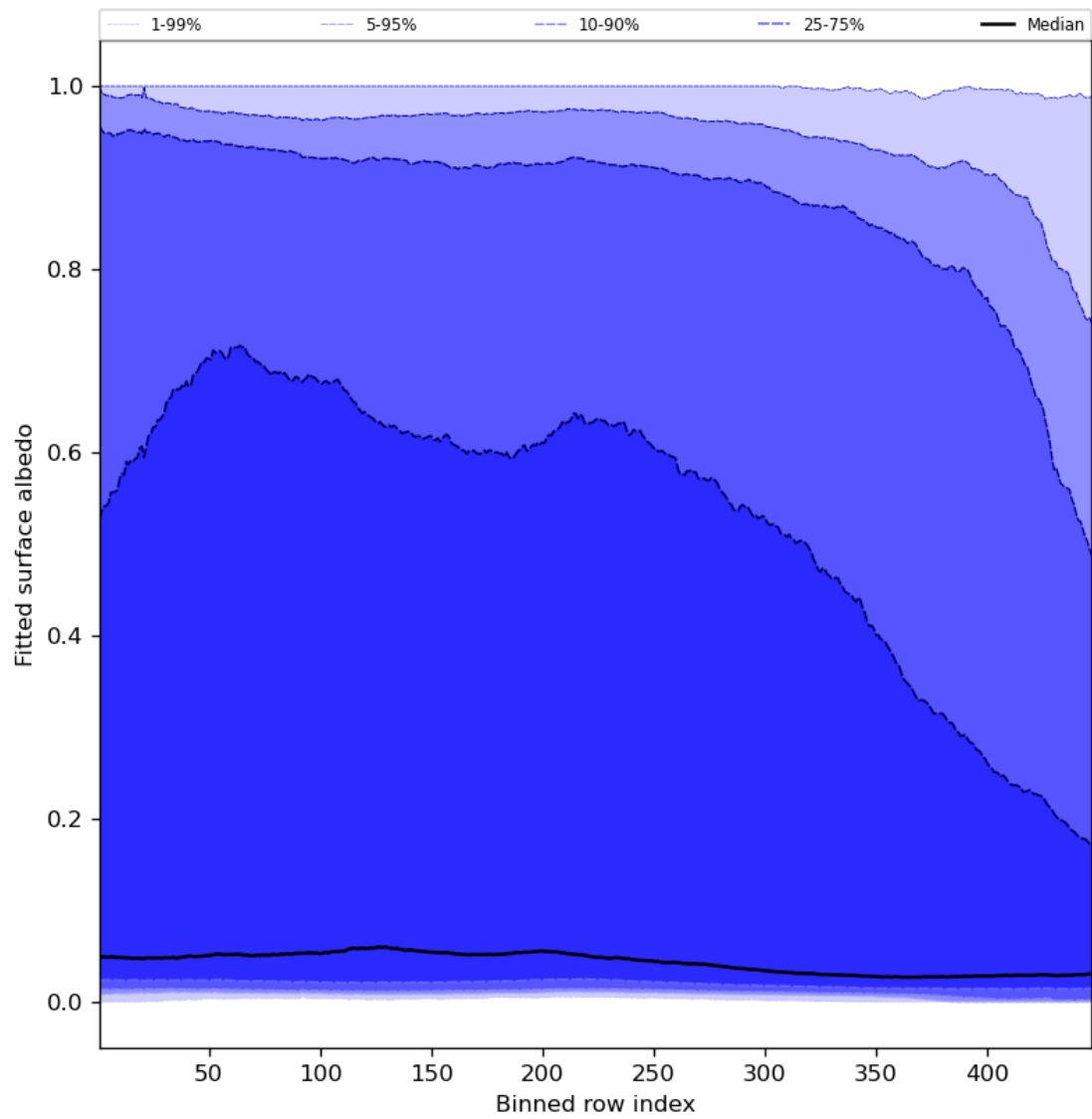
Figure 61: Along track statistics of “Fitted surface albedo” for 2024-02-07 to 2024-02-09
