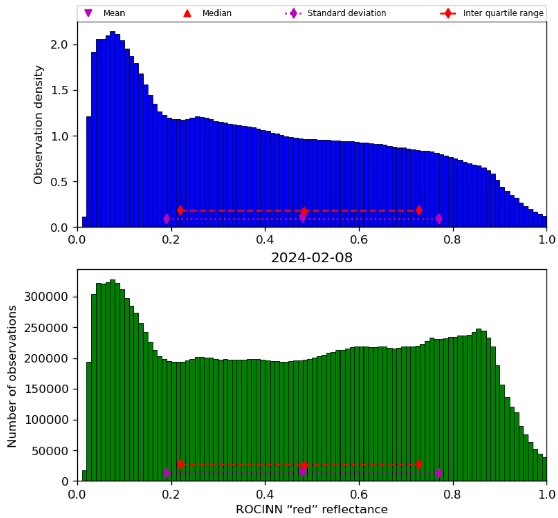
Figure 53: Histogram of “ROCINN “red” reflectance” for 2024-02-07 to 2024-02-09
