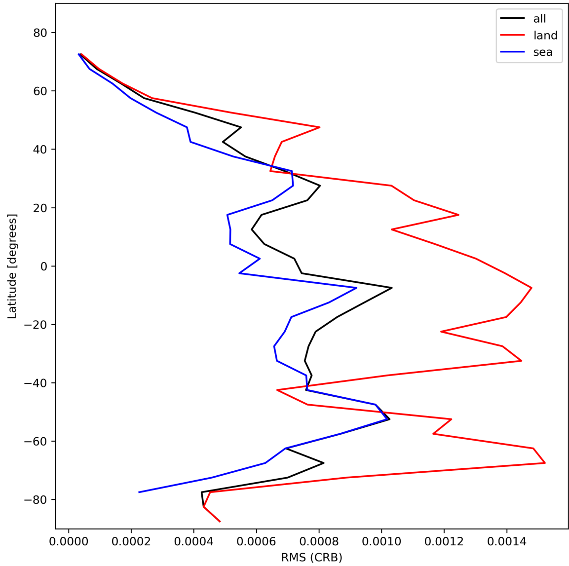
Figure 32: Zonal average of “RMS (CRB)” for 2024-02-07 to 2024-02-09.
