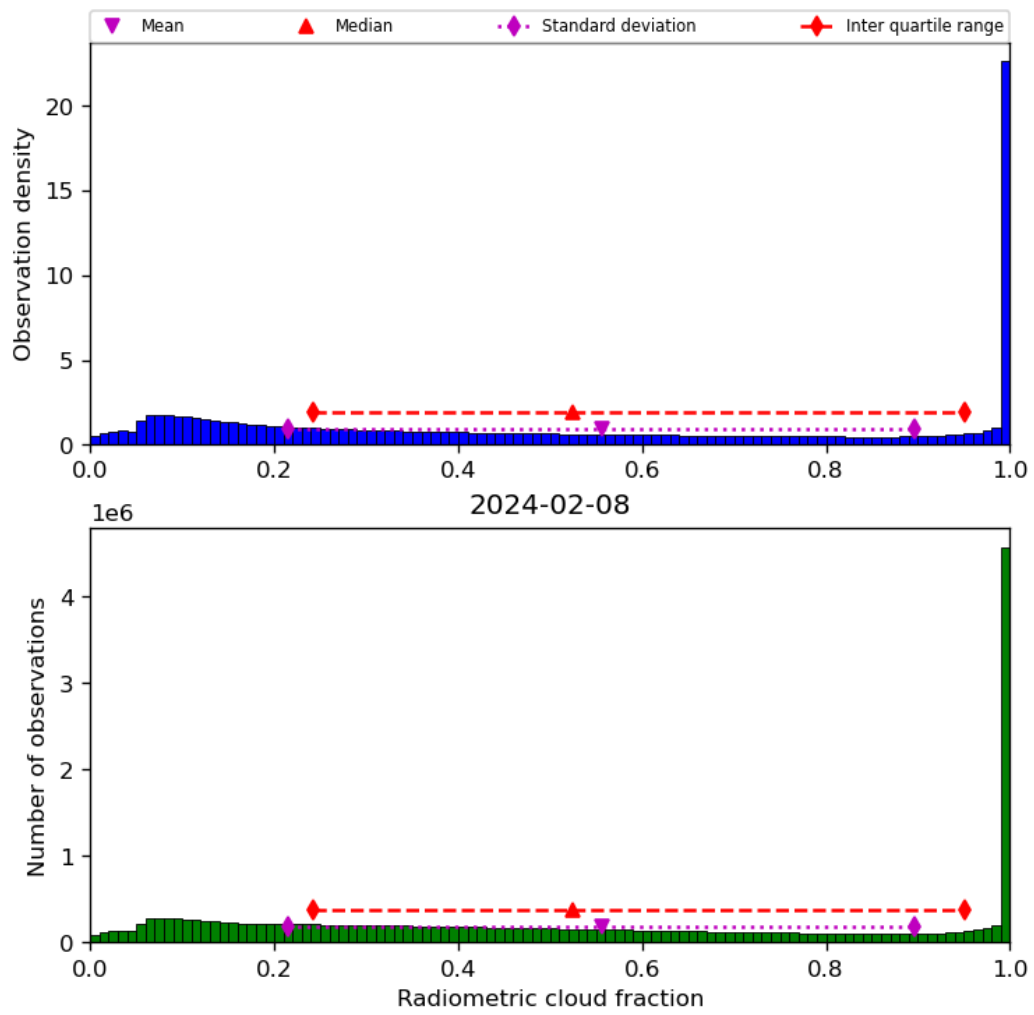
Figure 39: Histogram of “Radiometric cloud fraction” for 2024-02-07 to 2024-02-09
