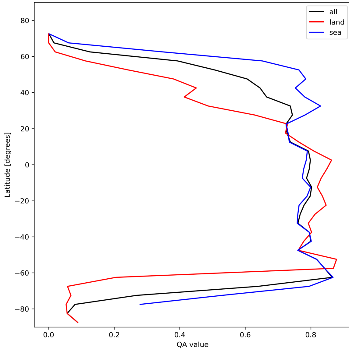
Figure 22: Zonal average of “QA value” for 2024-02-07 to 2024-02-09.
