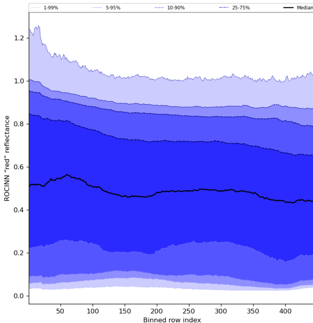
Figure 69: Along track statistics of “ROCINN “red” reflectance” for 2024-02-07 to 2024-02-09
