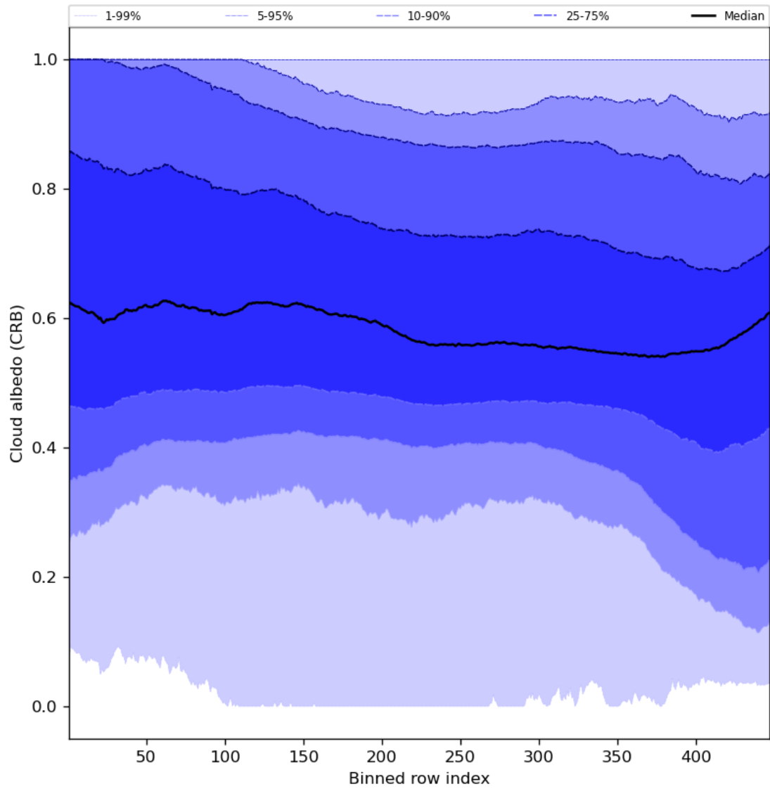
Figure 60: Along track statistics of “Cloud albedo (CRB)” for 2024-02-07 to 2024-02-09
