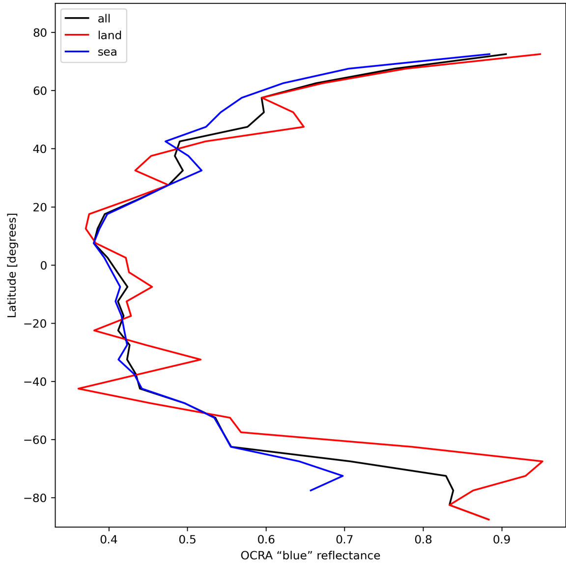
Figure 35: Zonal average of “OCRA “blue” reflectance” for 2024-02-07 to 2024-02-09.
