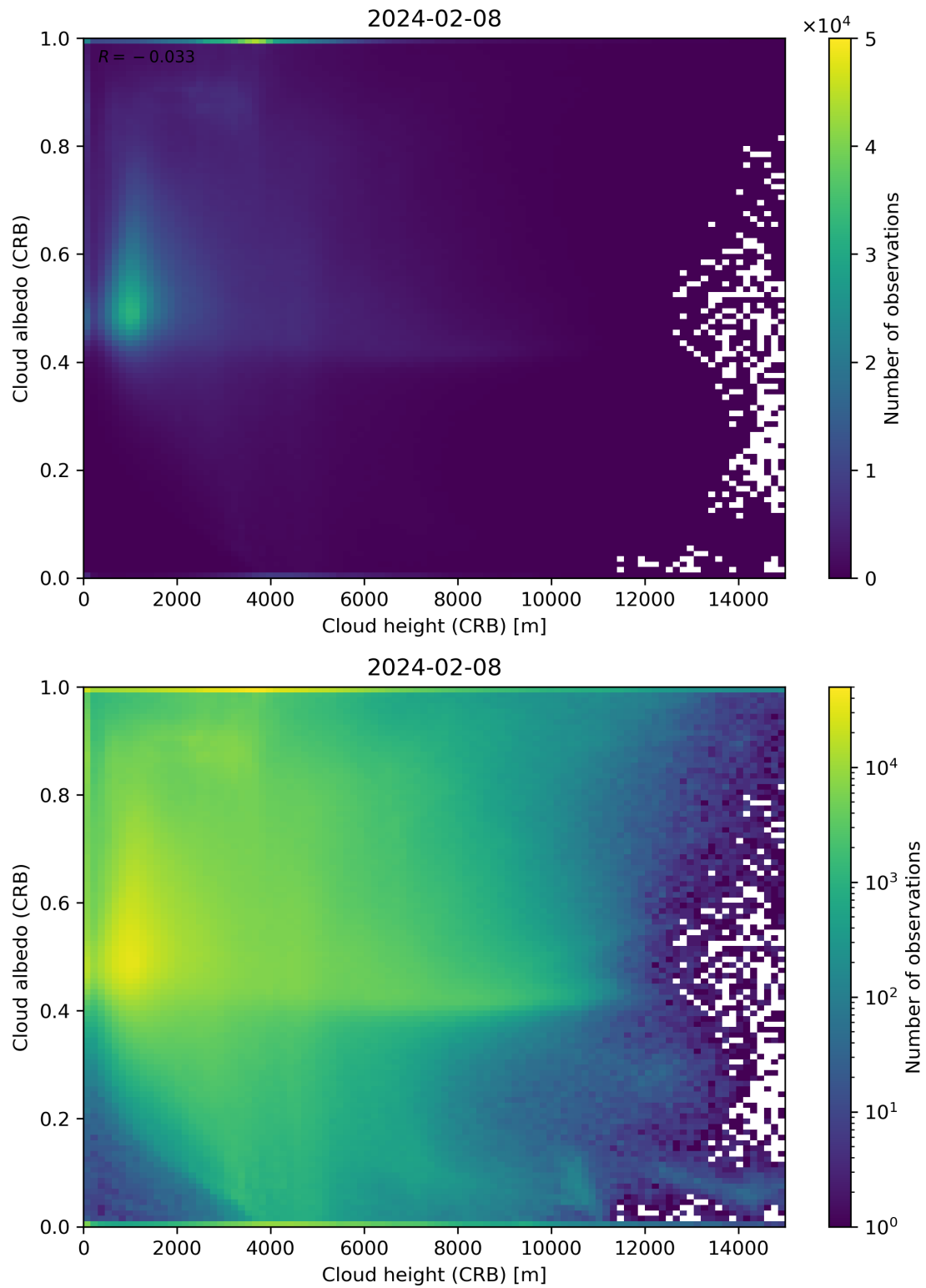
Figure 80: Scatter density plot of “Cloud height (CRB)” against “Cloud albedo (CRB)” for 2024-02-07 to 2024-02-09.
