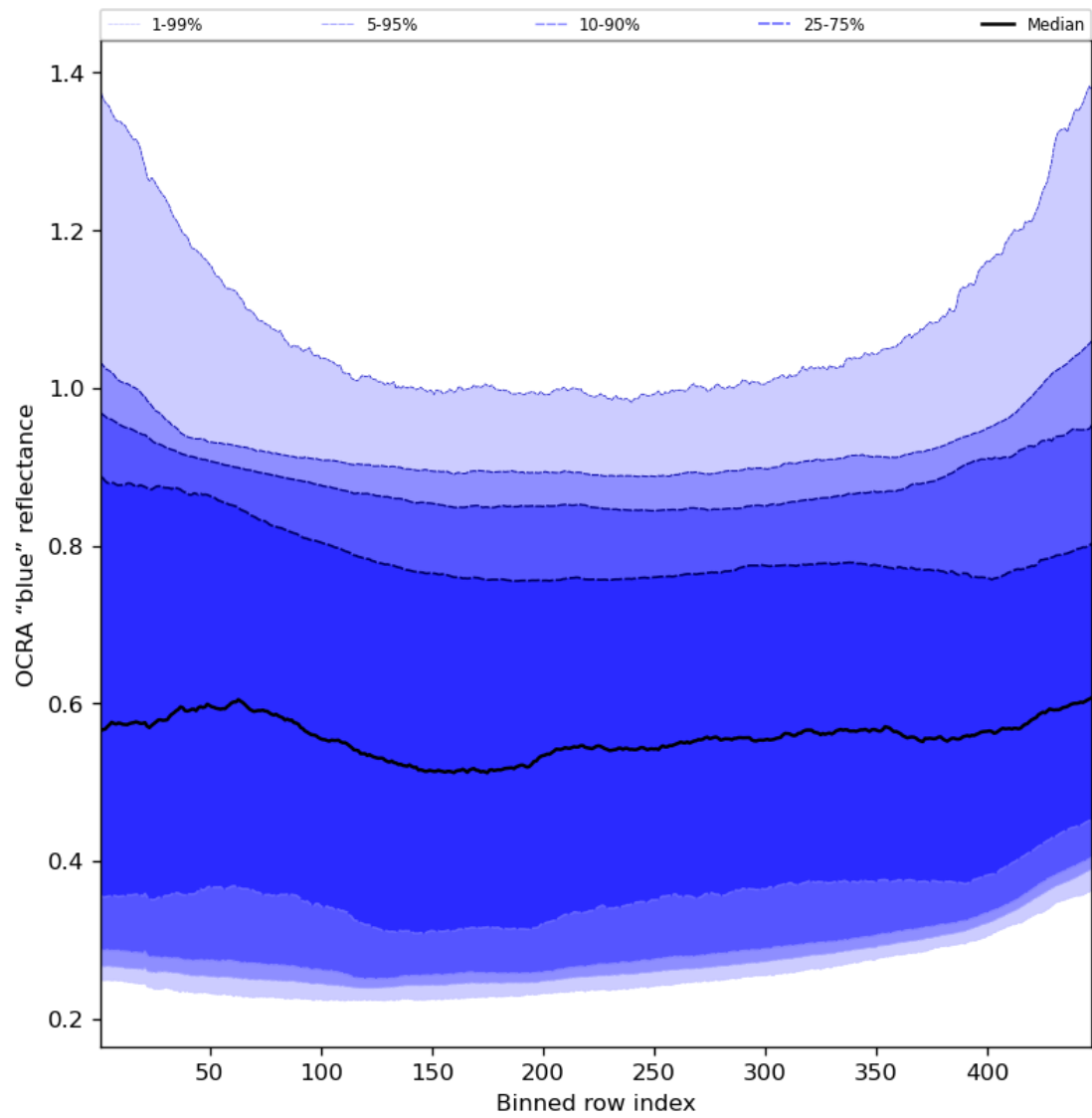
Figure 67: Along track statistics of “OCRA “blue” reflectance” for 2024-02-07 to 2024-02-09
