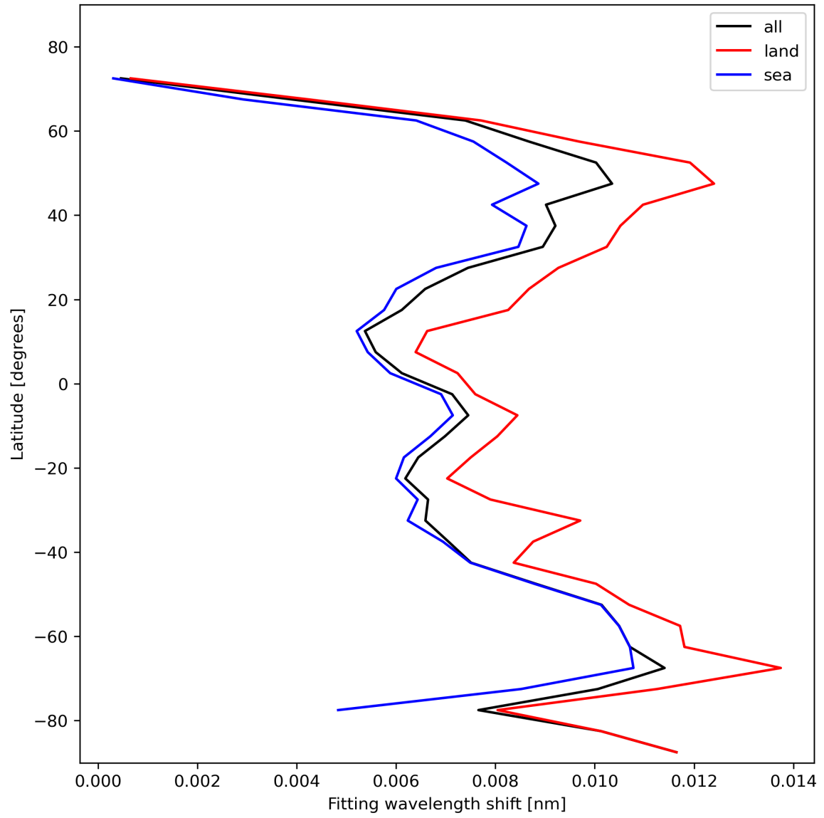
Figure 33: Zonal average of “Fitting wavelength shift” for 2024-02-07 to 2024-02-09.
