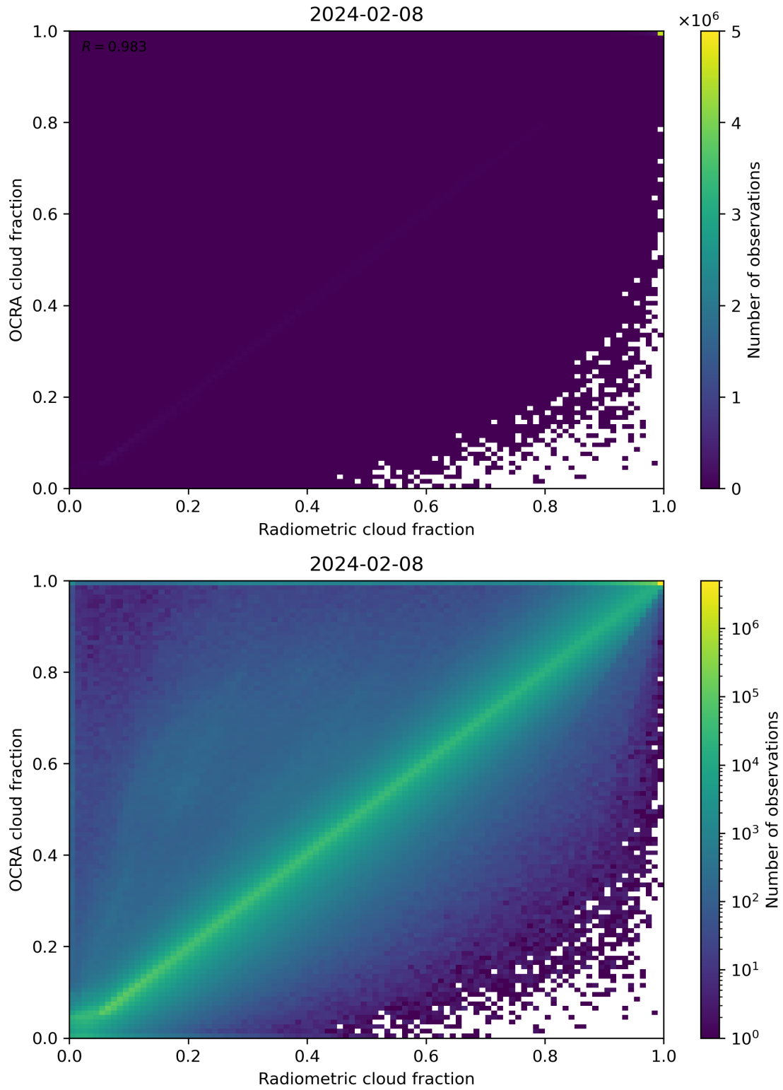
Figure 72: Scatter density plot of “Radiometric cloud fraction” against “OCRA cloud fraction” for 2024-02-07 to 2024-02-09.
