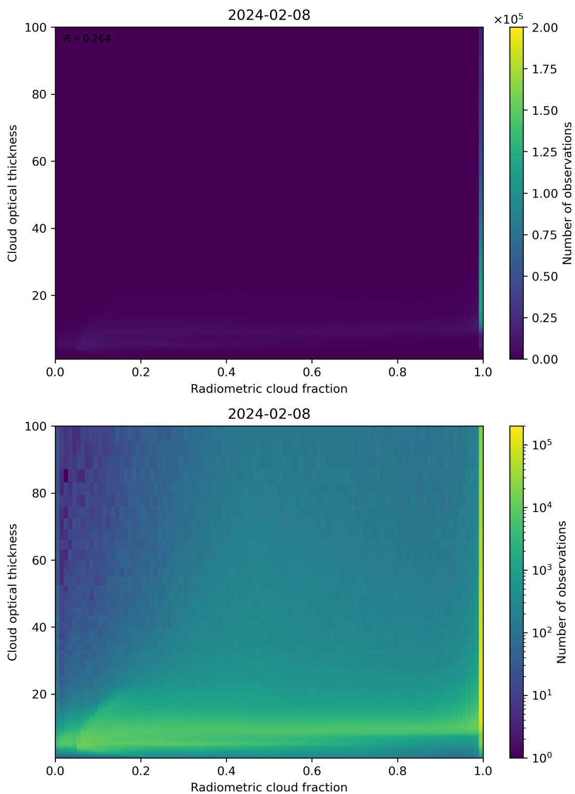
Figure 75: Scatter density plot of “Radiometric cloud fraction” against “Cloud optical thickness” for 2024-02-07 to 2024-02-09.
