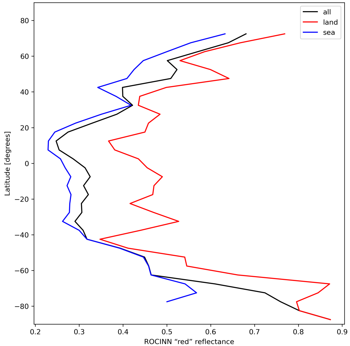
Figure 37: Zonal average of “ROCINN “red” reflectance” for 2024-02-07 to 2024-02-09.
