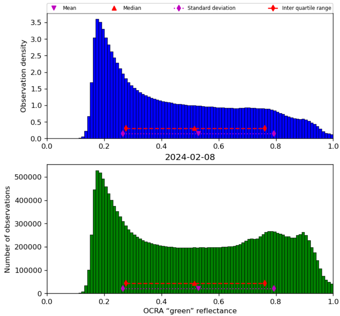
Figure 52: Histogram of “OCRA “green” reflectance” for 2024-02-07 to 2024-02-09
