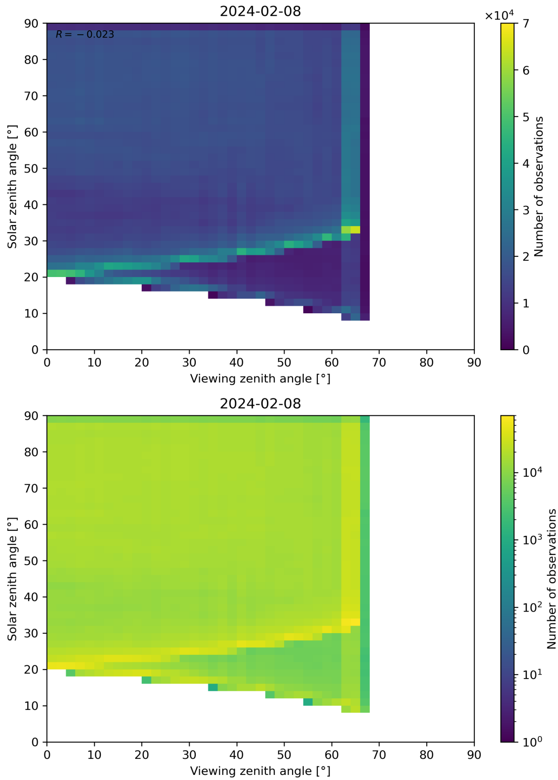
Figure 114: Scatter density plot of “Viewing zenith angle” against “Solar zenith angle” for 2024-02-07 to 2024-02-09.
