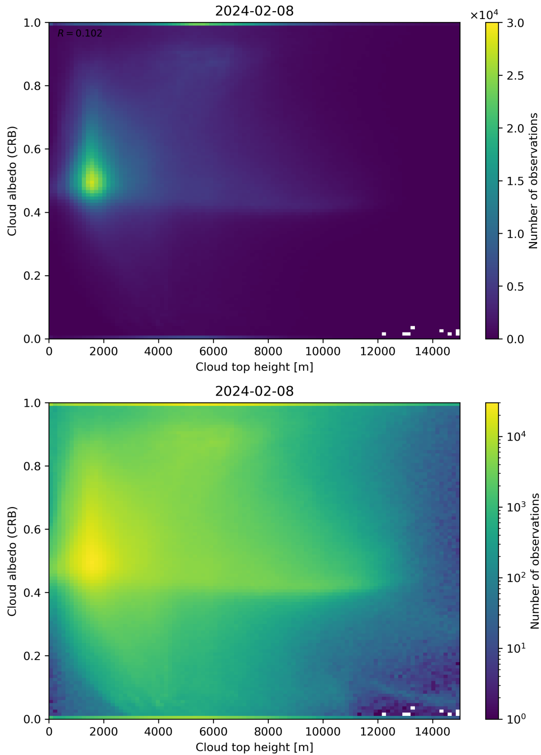
Figure 86: Scatter density plot of “Cloud top height” against “Cloud albedo (CRB)” for 2024-02-07 to 2024-02-09.
