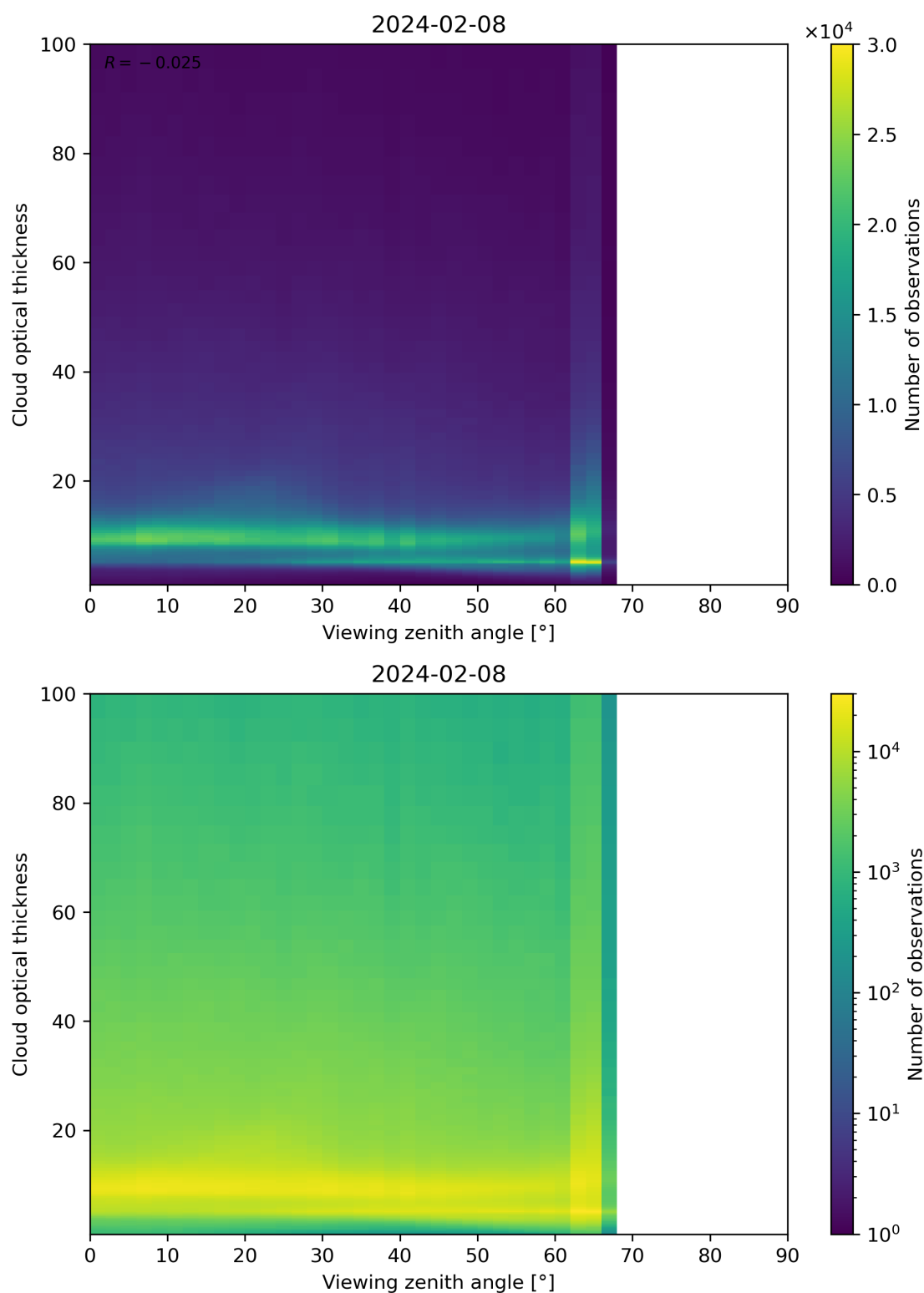
Figure 111: Scatter density plot of “Viewing zenith angle” against “Cloud optical thickness” for 2024-02-07 to 2024-02-09.
