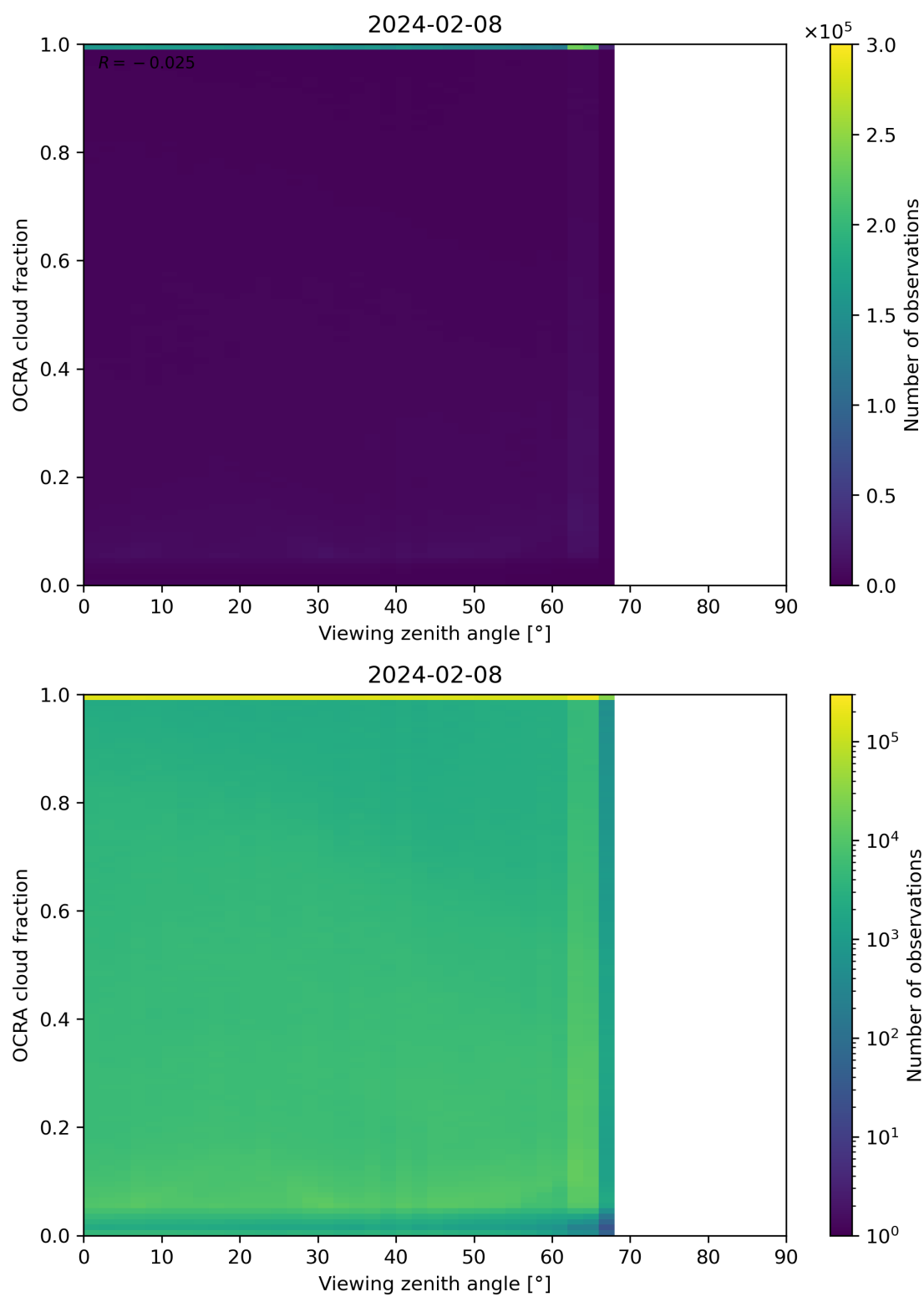
Figure 108: Scatter density plot of “Viewing zenith angle” against “OCRA cloud fraction” for 2024-02-07 to 2024-02-09.
