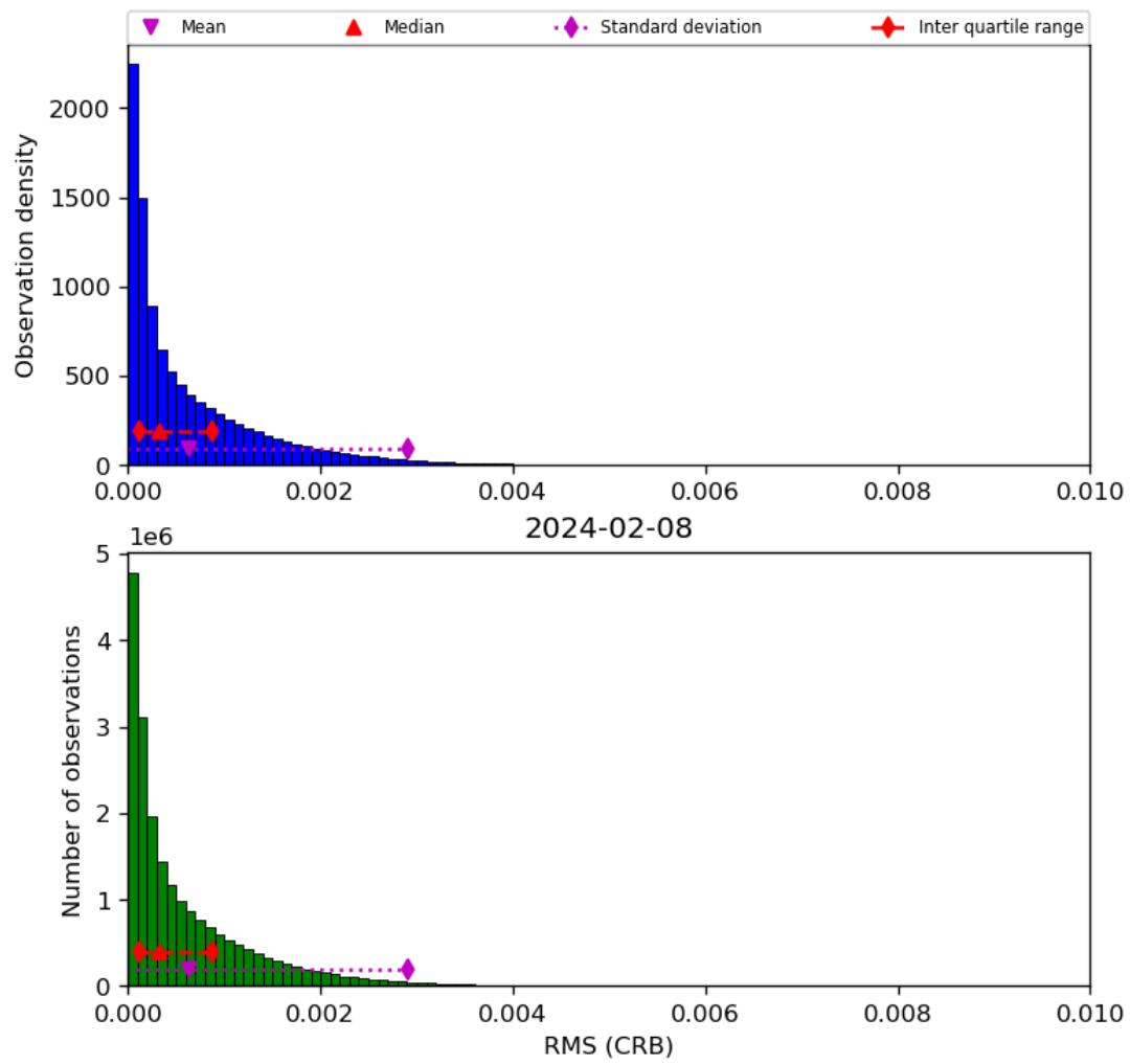
Figure 48: Histogram of “RMS (CRB)” for 2024-02-07 to 2024-02-09
