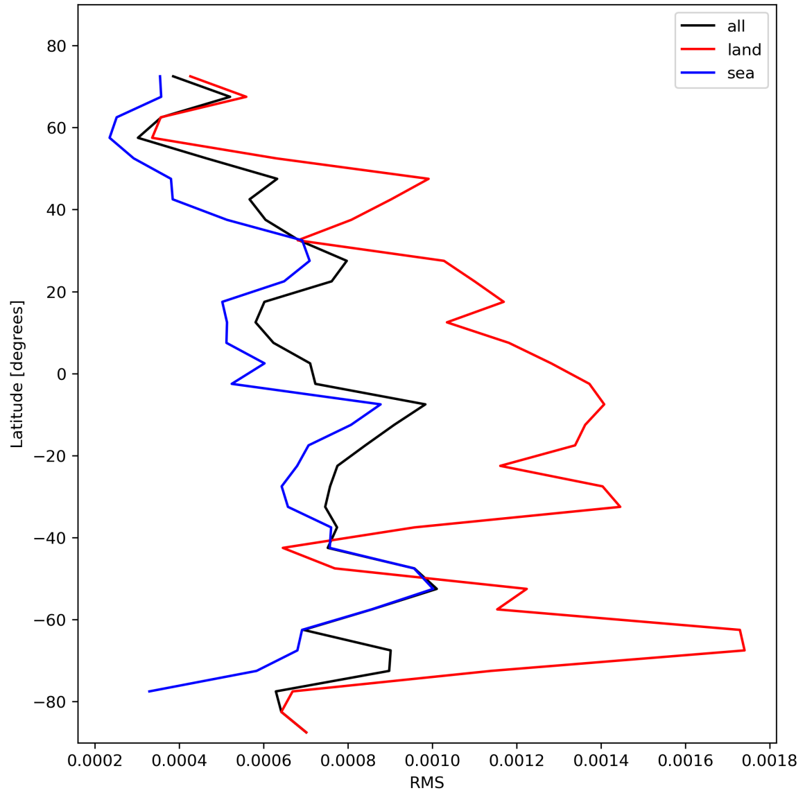
Figure 31: Zonal average of “RMS” for 2024-02-07 to 2024-02-09.
