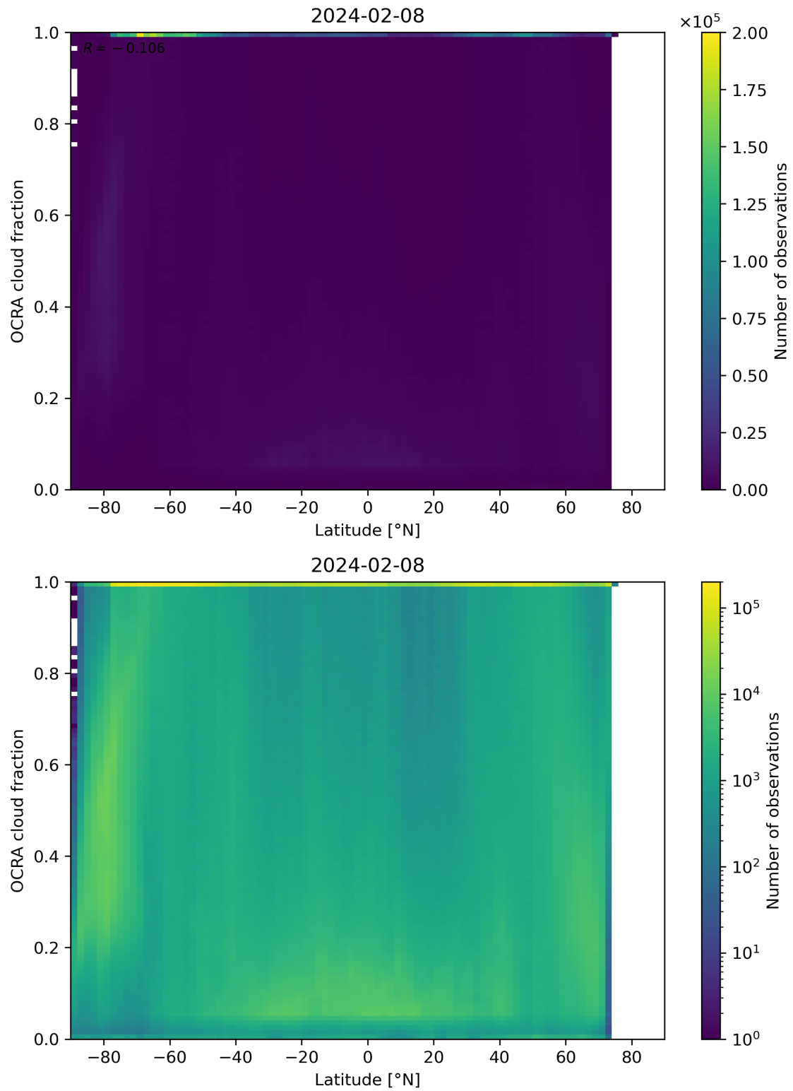
Figure 93: Scatter density plot of “Latitude” against “OCRA cloud fraction” for 2024-02-07 to 2024-02-09.
