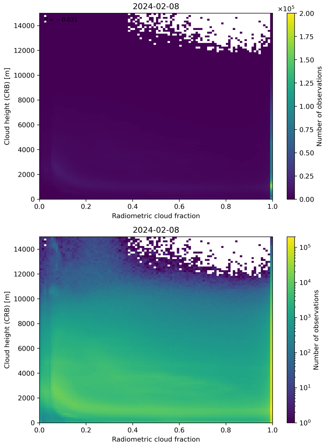
Figure 74: Scatter density plot of “Radiometric cloud fraction” against “Cloud height (CRB)” for 2024-02-07 to 2024-02-09.
