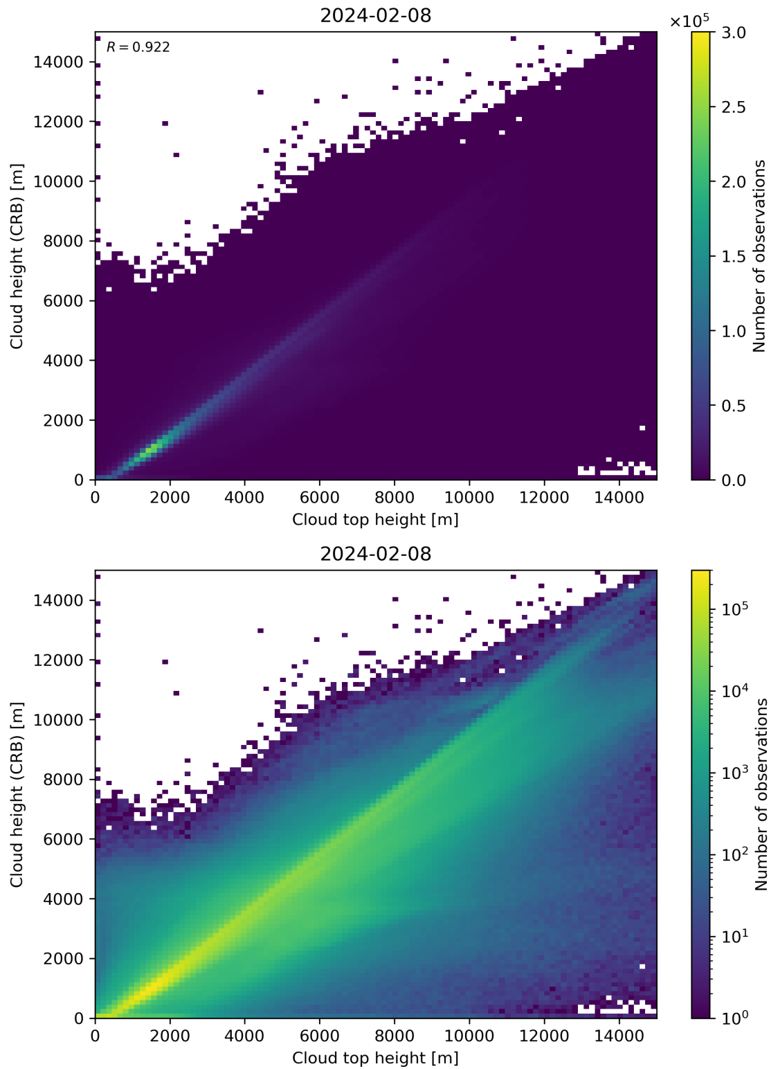
Figure 89: Scatter density plot of “Cloud top height” against “Cloud height (CRB)” for 2024-02-07 to 2024-02-09.
