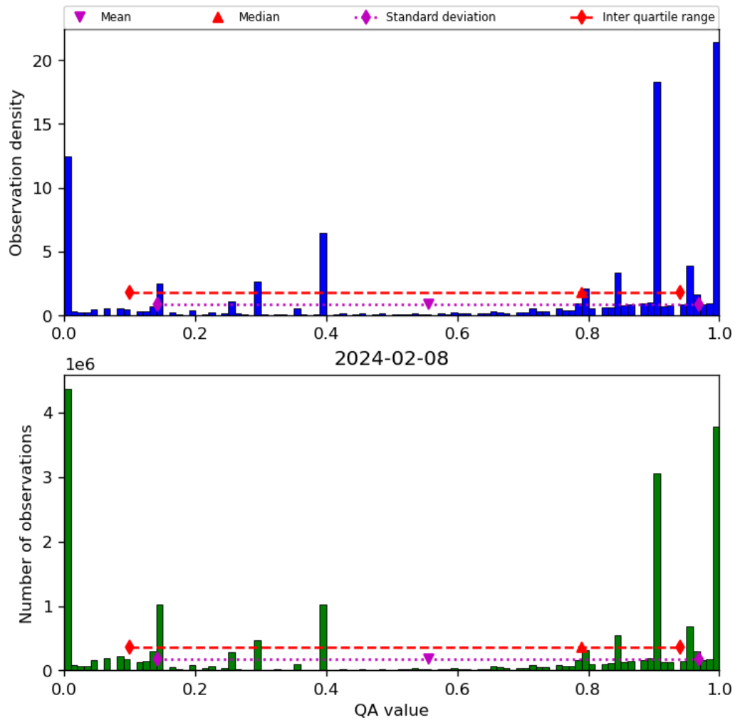
Figure 38: Histogram of “QA value” for 2024-02-07 to 2024-02-09
