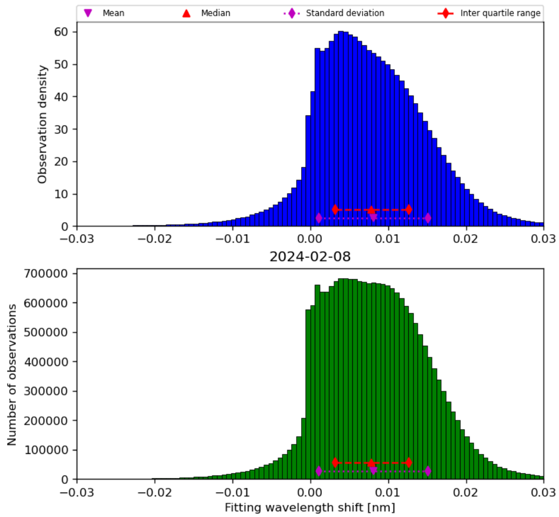
Figure 49: Histogram of “Fitting wavelength shift” for 2024-02-07 to 2024-02-09
