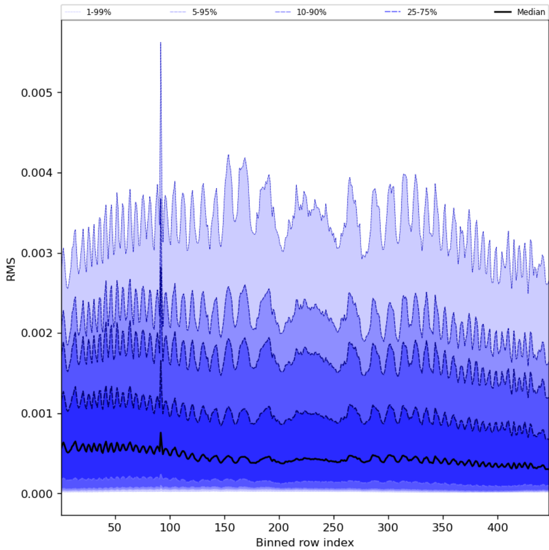
Figure 63: Along track statistics of “RMS” for 2024-02-07 to 2024-02-09
