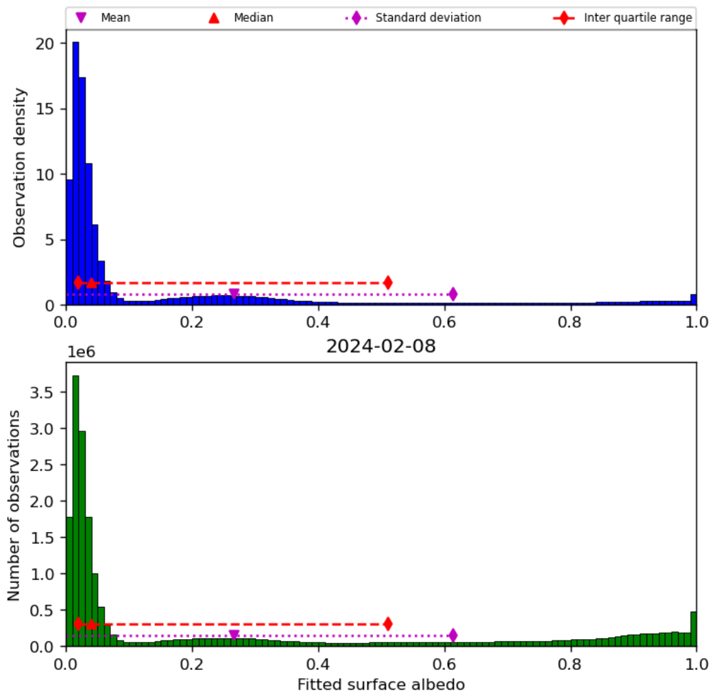
Figure 45: Histogram of “Fitted surface albedo” for 2024-02-07 to 2024-02-09
