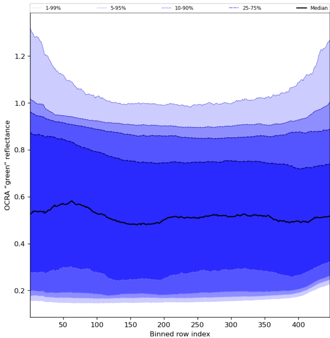
Figure 68: Along track statistics of “OCRA “green” reflectance” for 2024-02-07 to 2024-02-09
