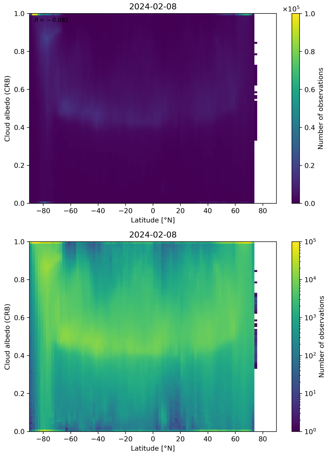
Figure 91: Scatter density plot of “Latitude” against “Cloud albedo (CRB)” for 2024-02-07 to 2024-02-09.
