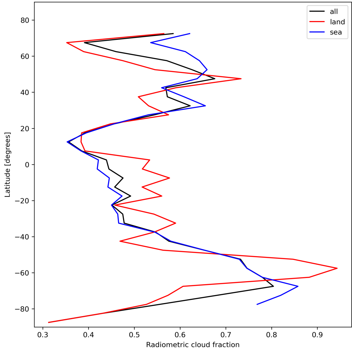
Figure 23: Zonal average of “Radiometric cloud fraction” for 2024-02-07 to 2024-02-09.
