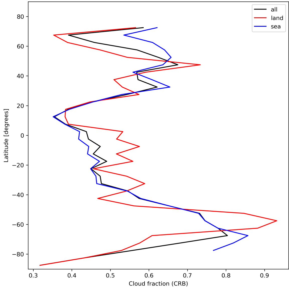
Figure 26: Zonal average of “Cloud fraction (CRB)” for 2024-02-07 to 2024-02-09.
