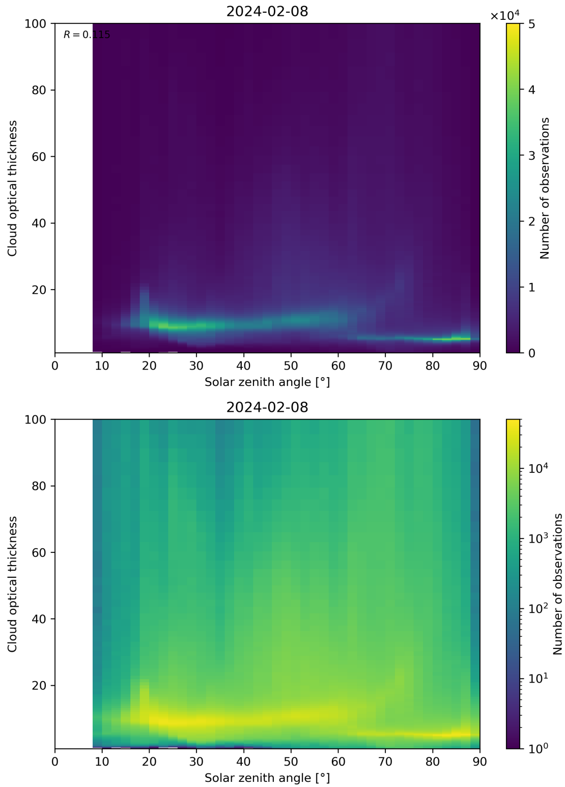
Figure 103: Scatter density plot of “Solar zenith angle” against “Cloud optical thickness” for 2024-02-07 to 2024-02-09.
