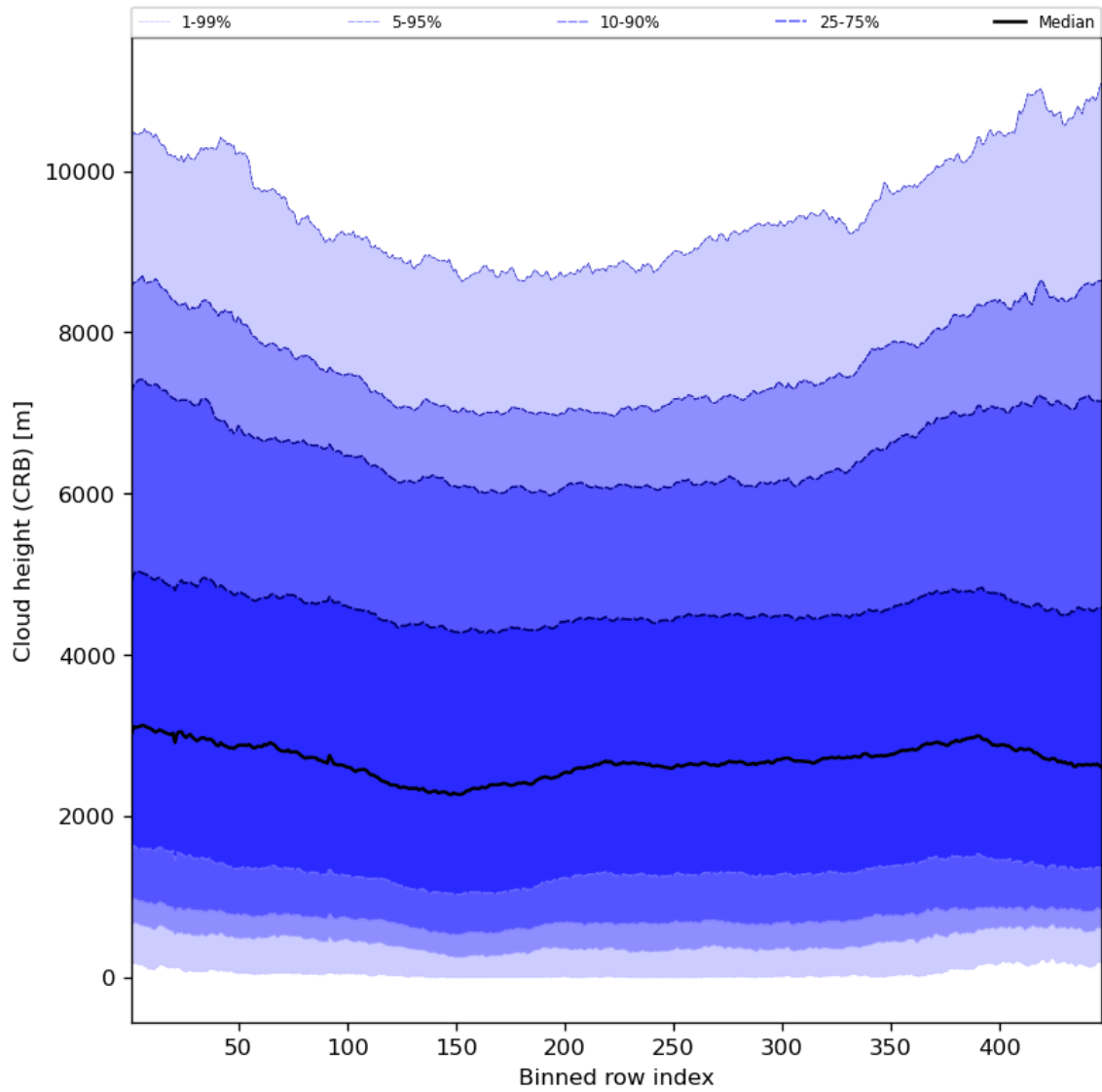
Figure 59: Along track statistics of “Cloud height (CRB)” for 2024-02-07 to 2024-02-09
