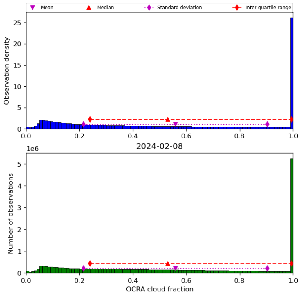
Figure 50: Histogram of “OCRA cloud fraction” for 2024-02-07 to 2024-02-09
