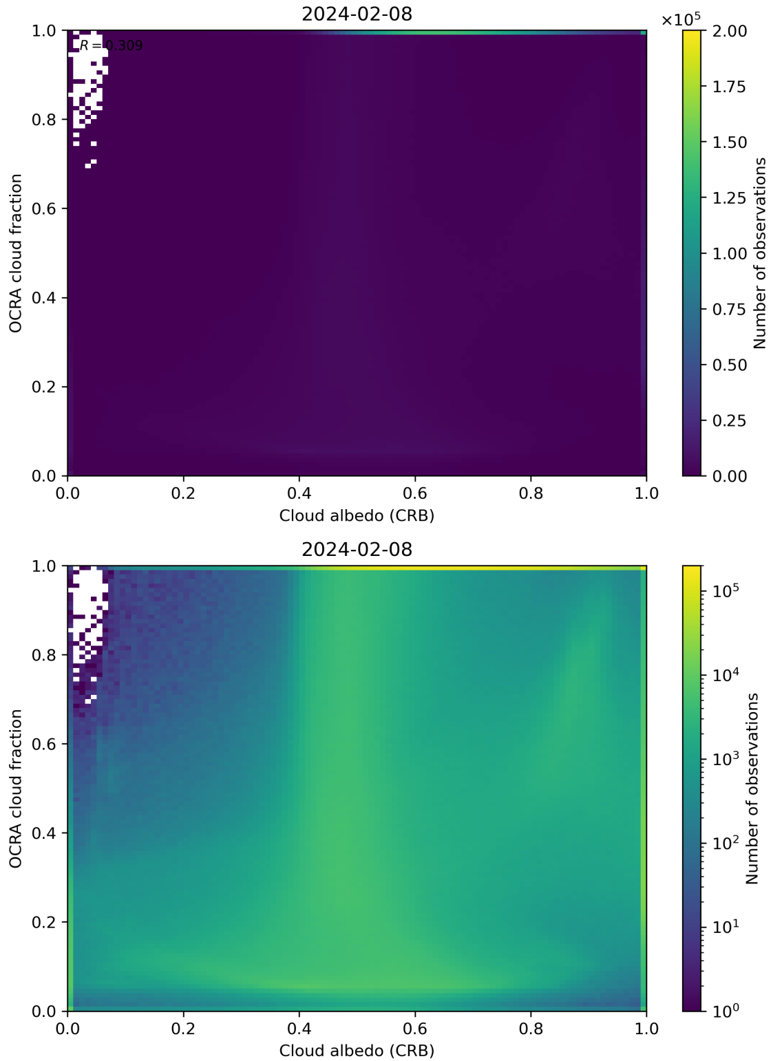
Figure 70: Scatter density plot of “Cloud albedo (CRB)” against “OCRA cloud fraction” for 2024-02-07 to 2024-02-09.
