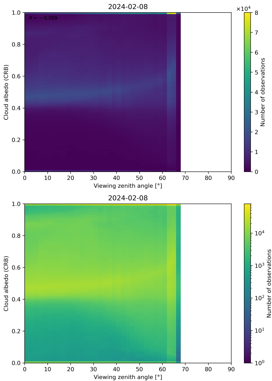
Figure 106: Scatter density plot of “Viewing zenith angle” against “Cloud albedo (CRB)” for 2024-02-07 to 2024-02-09.
