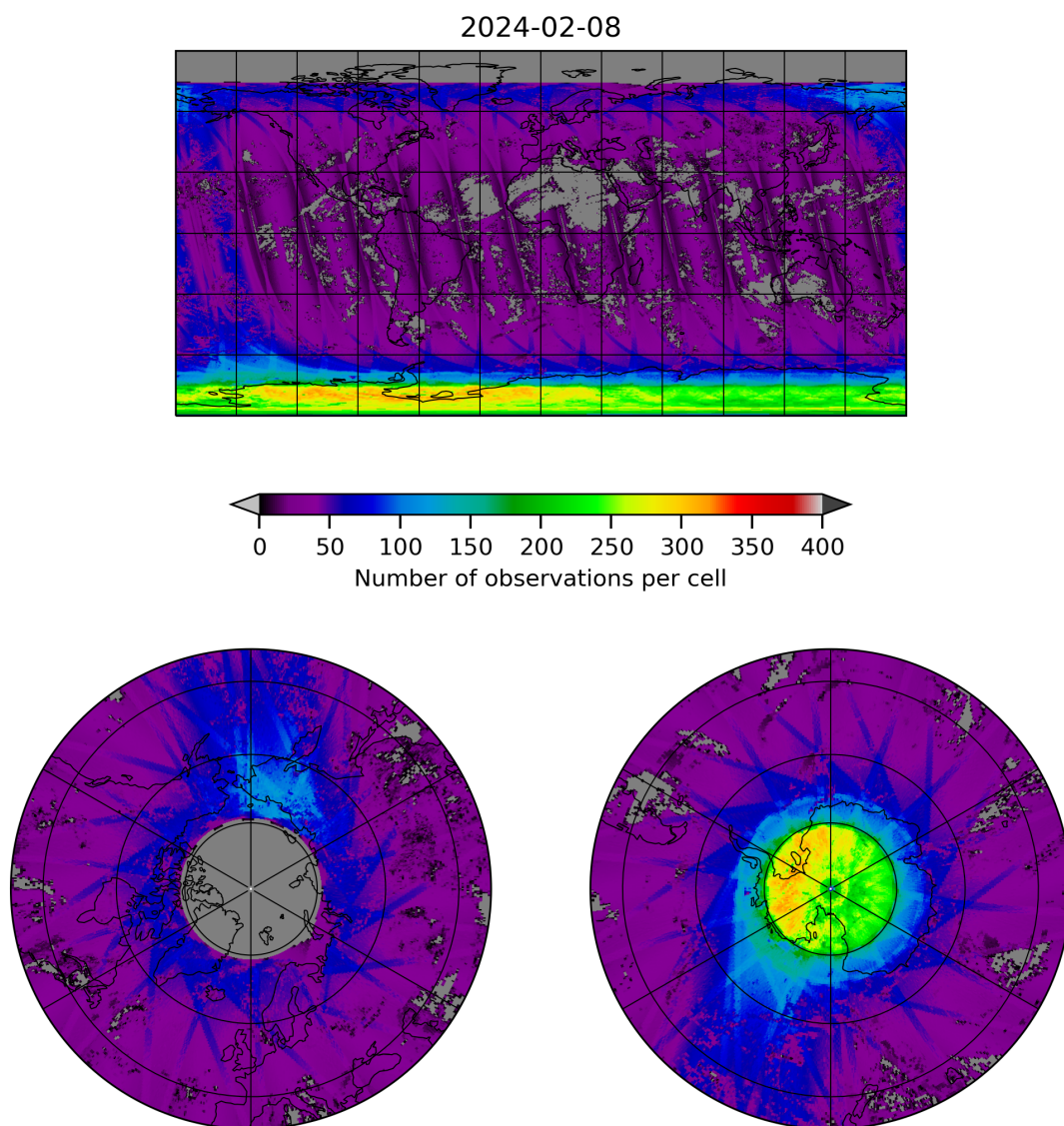
Figure 21: Map of the number of observations for 2024-02-07 to 2024-02-09
