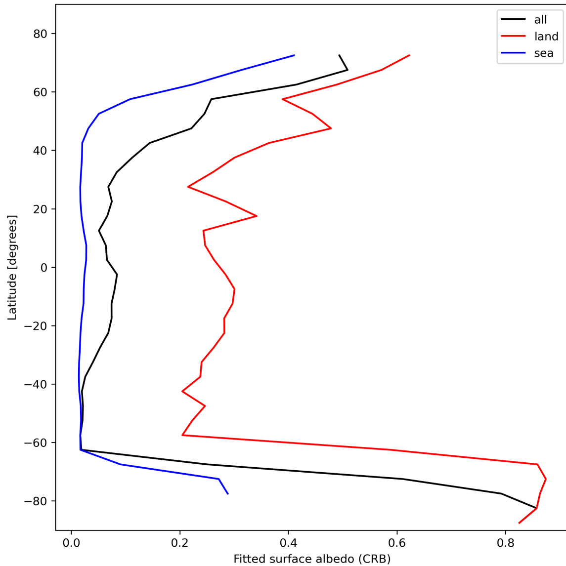
Figure 30: Zonal average of “Fitted surface albedo (CRB)” for 2024-02-07 to 2024-02-09.
