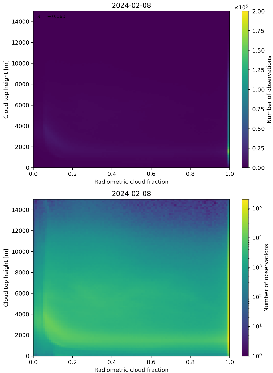
Figure 76: Scatter density plot of “Radiometric cloud fraction” against “Cloud top height” for 2024-02-07 to 2024-02-09.
