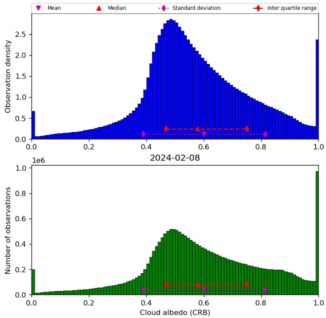
Figure 44: Histogram of “Cloud albedo (CRB)” for 2024-02-07 to 2024-02-09
