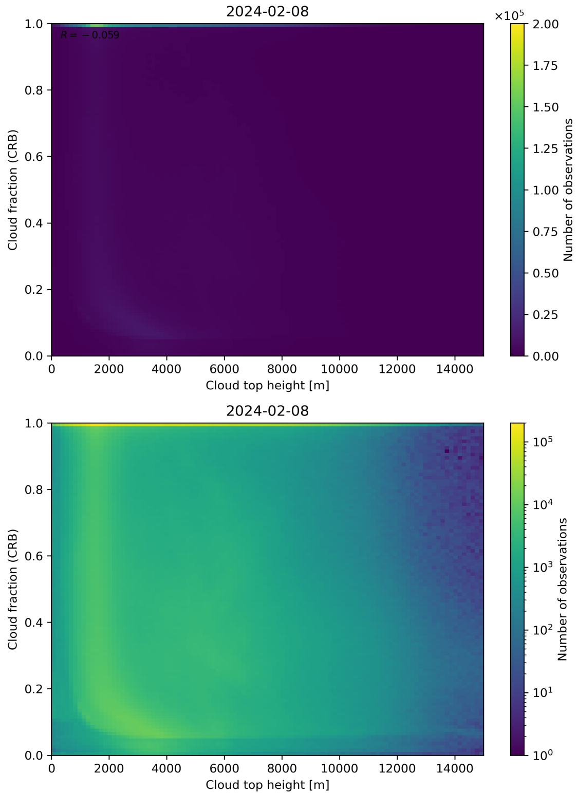
Figure 88: Scatter density plot of “Cloud top height” against “Cloud fraction (CRB)” for 2024-02-07 to 2024-02-09.
