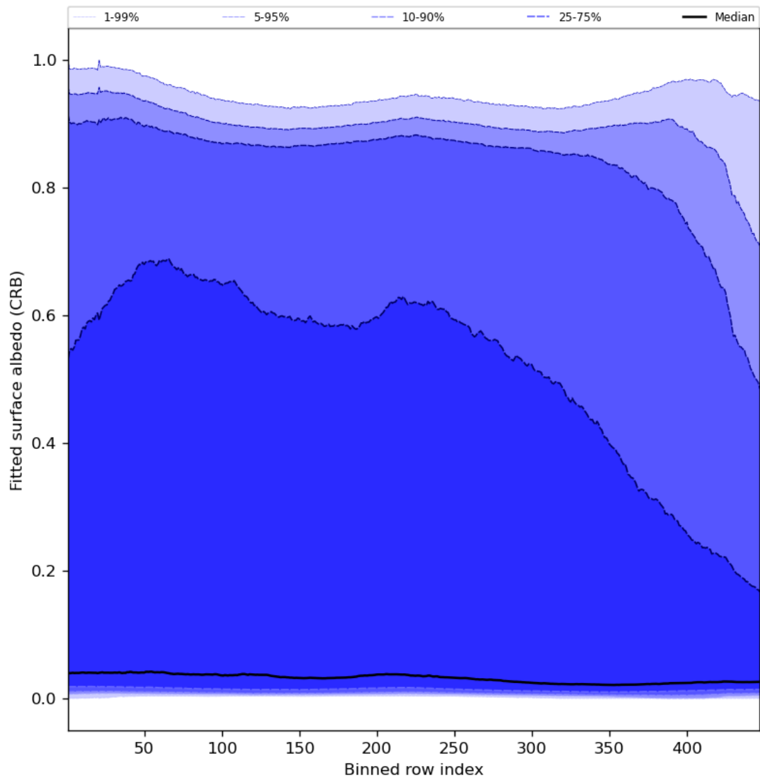
Figure 62: Along track statistics of “Fitted surface albedo (CRB)” for 2024-02-07 to 2024-02-09
