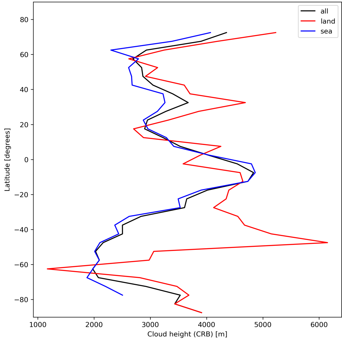
Figure 27: Zonal average of “Cloud height (CRB)” for 2024-02-07 to 2024-02-09.
