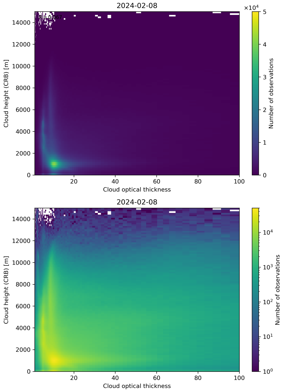
Figure 85: Scatter density plot of “Cloud optical thickness” against “Cloud height (CRB)” for 2024-02-07 to 2024-02-09.
