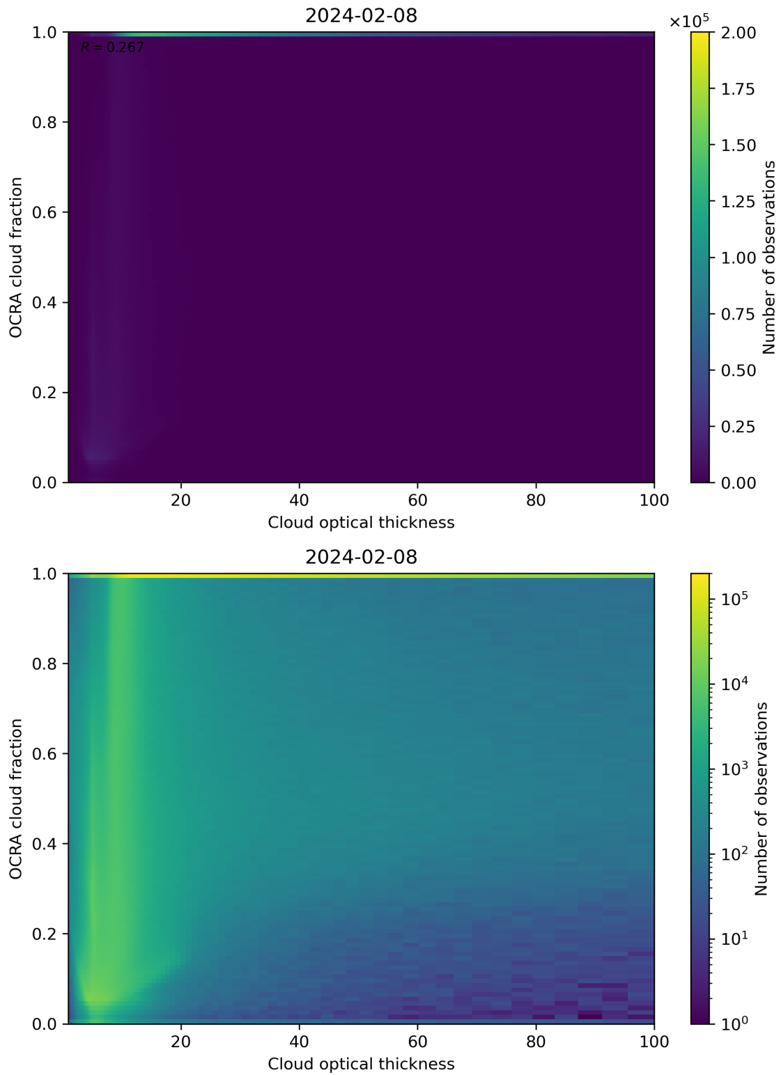
Figure 83: Scatter density plot of “Cloud optical thickness” against “OCRA cloud fraction” for 2024-02-07 to 2024-02-09.
