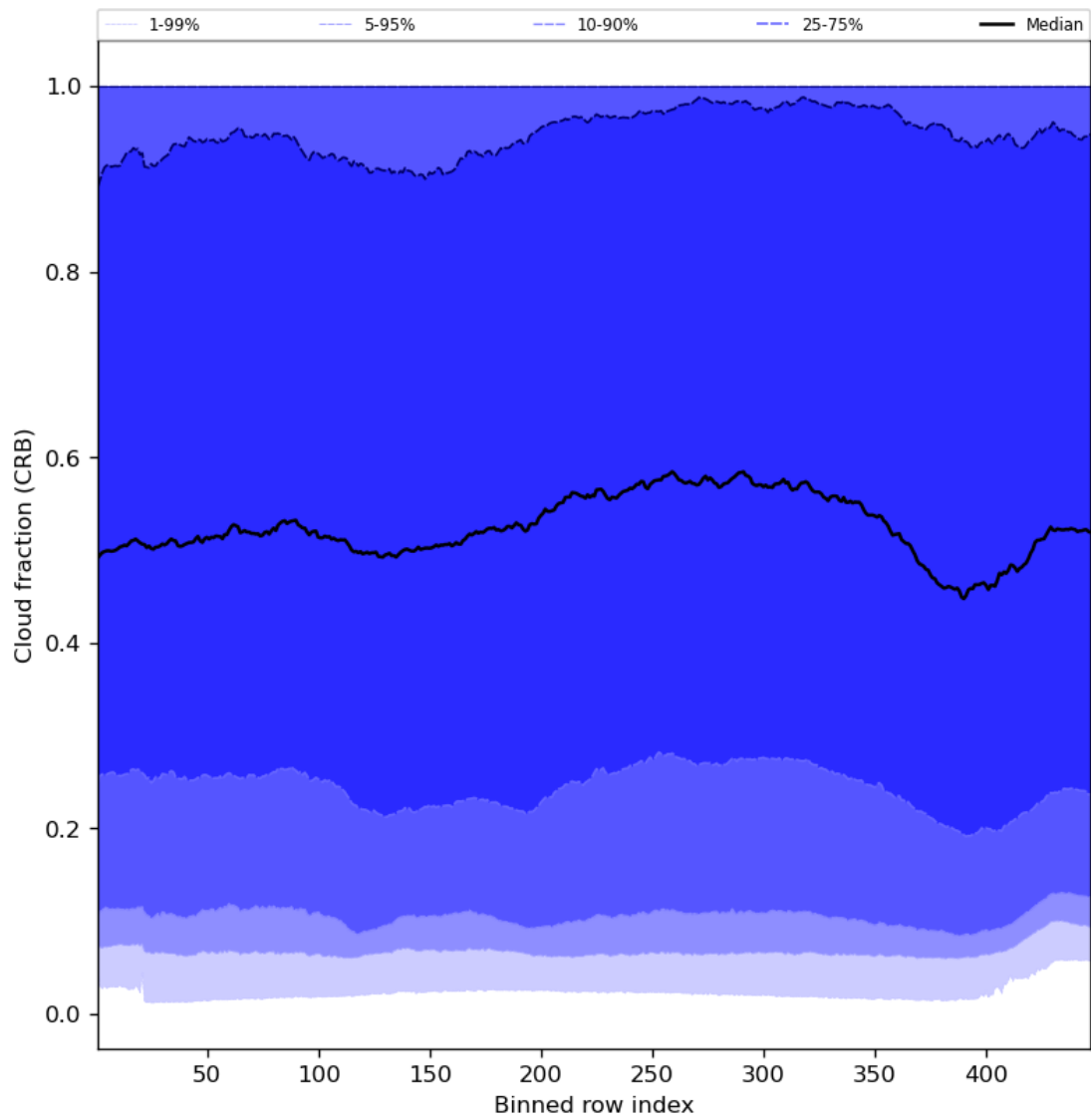
Figure 58: Along track statistics of “Cloud fraction (CRB)” for 2024-02-07 to 2024-02-09
