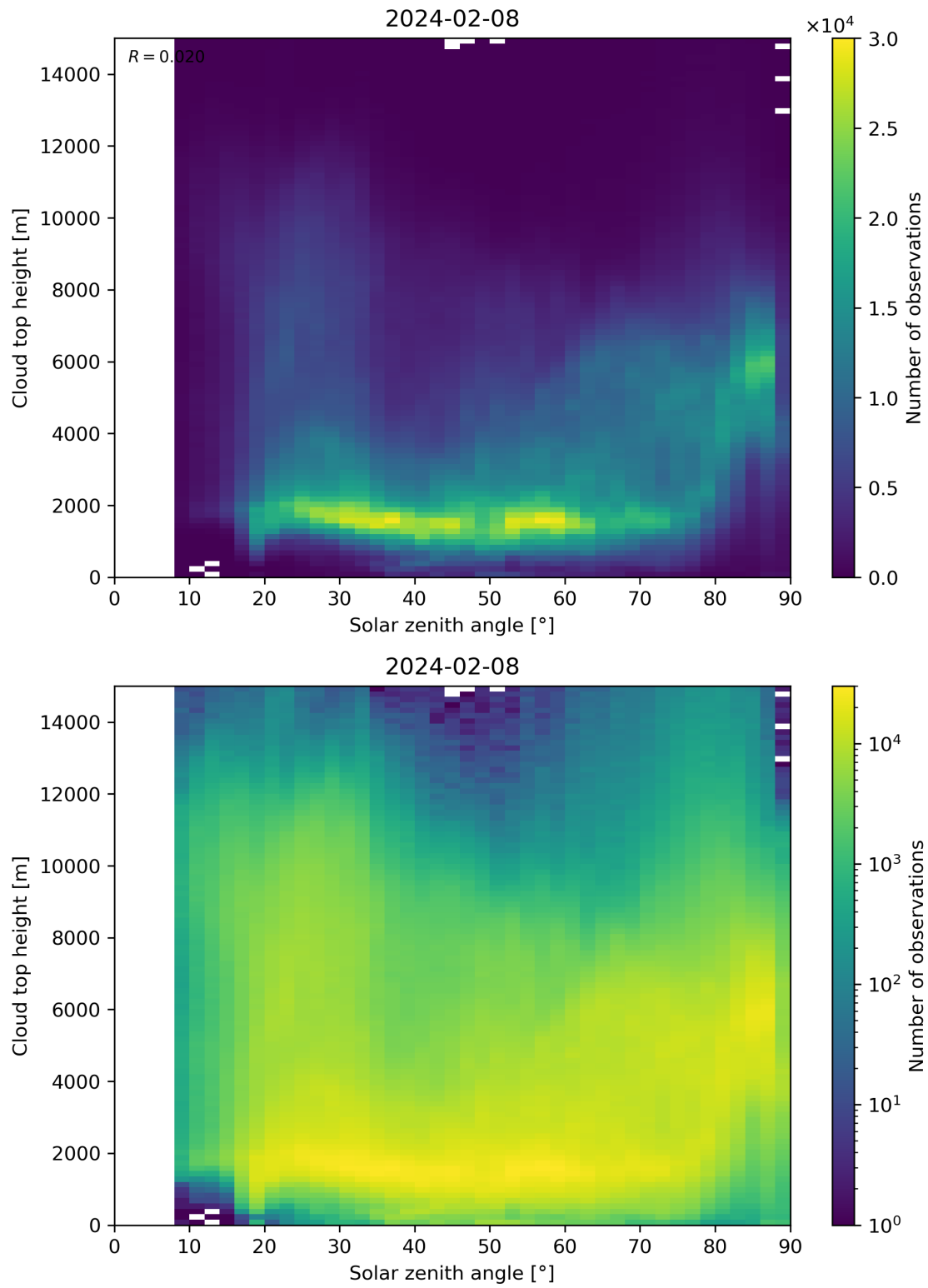
Figure 104: Scatter density plot of “Solar zenith angle” against “Cloud top height” for 2024-02-07 to 2024-02-09.
