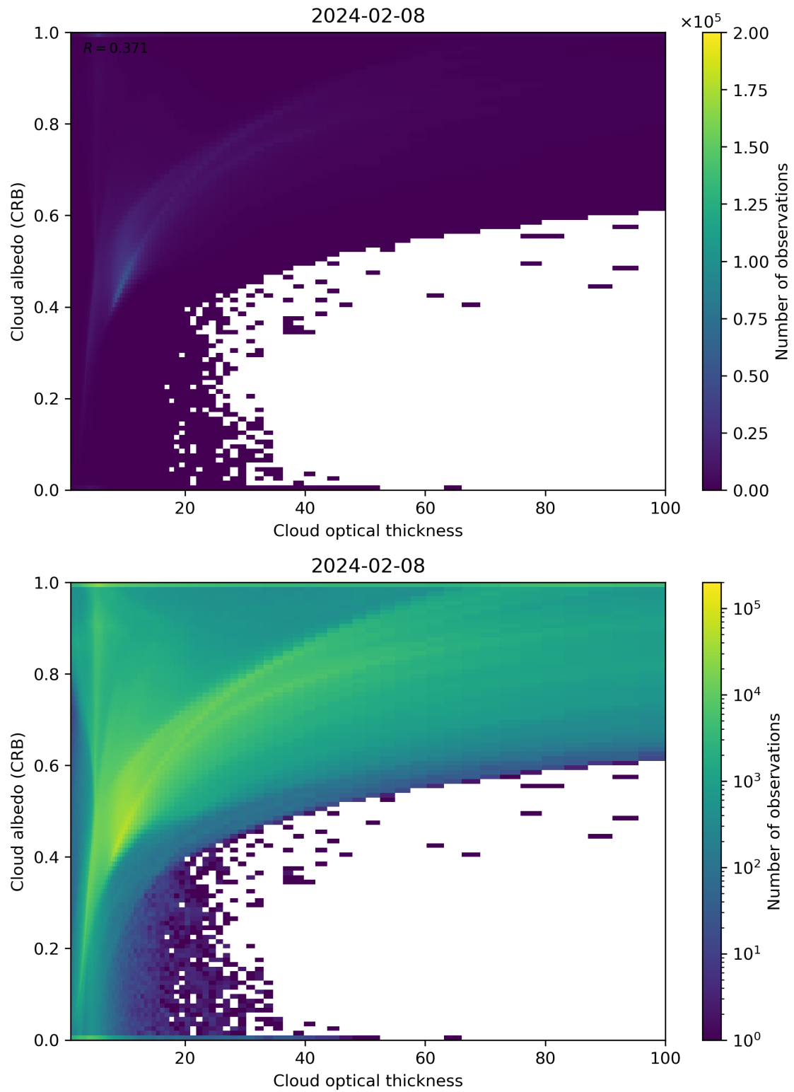
Figure 82: Scatter density plot of “Cloud optical thickness” against “Cloud albedo (CRB)” for 2024-02-07 to 2024-02-09.
