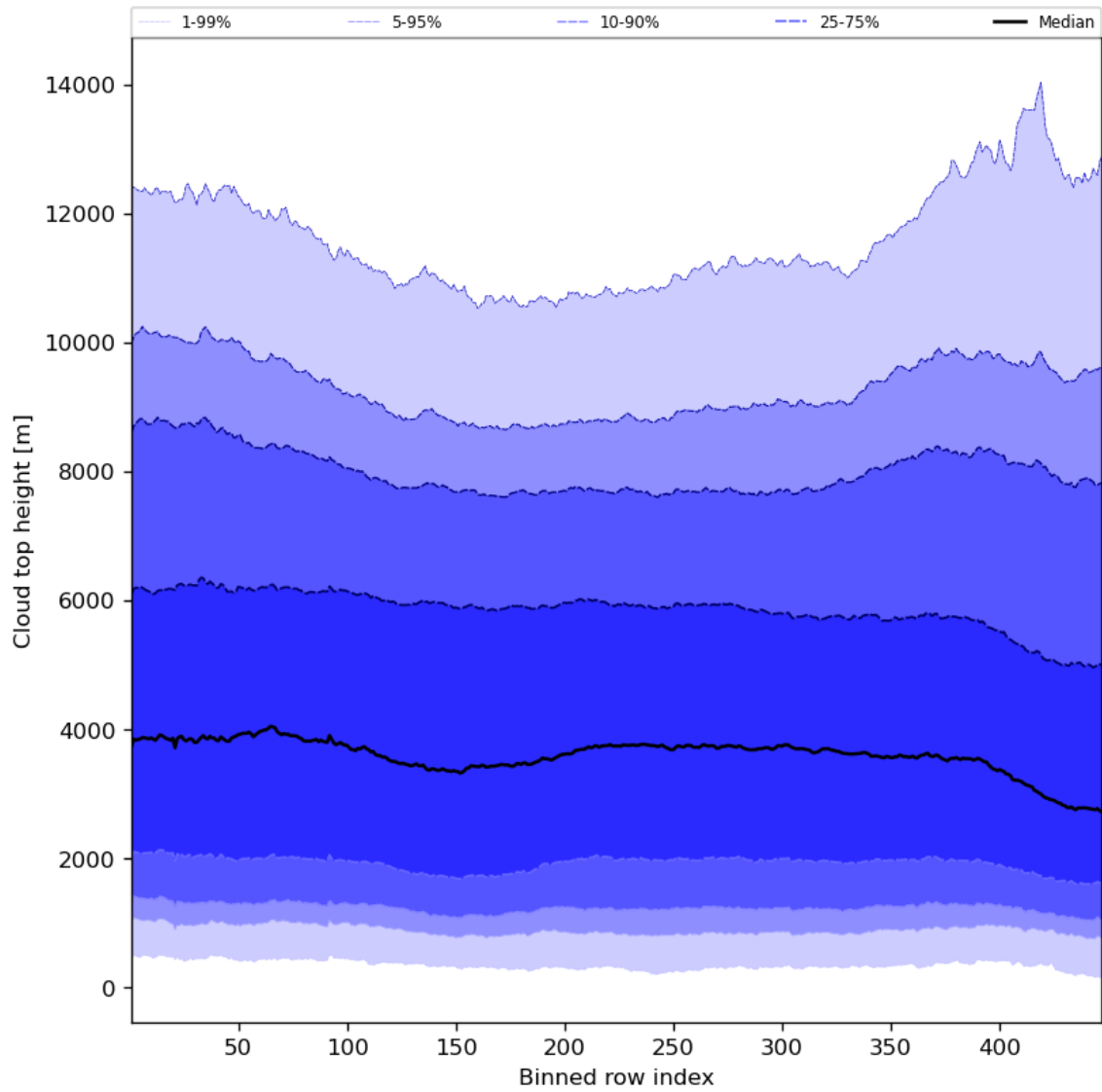
Figure 56: Along track statistics of “Cloud top height” for 2024-02-07 to 2024-02-09
