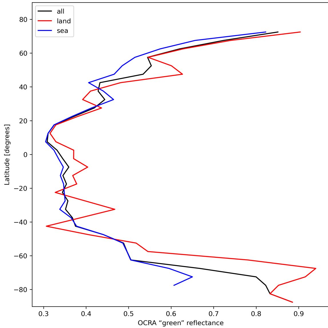
Figure 36: Zonal average of “OCRA “green” reflectance” for 2024-02-07 to 2024-02-09.
