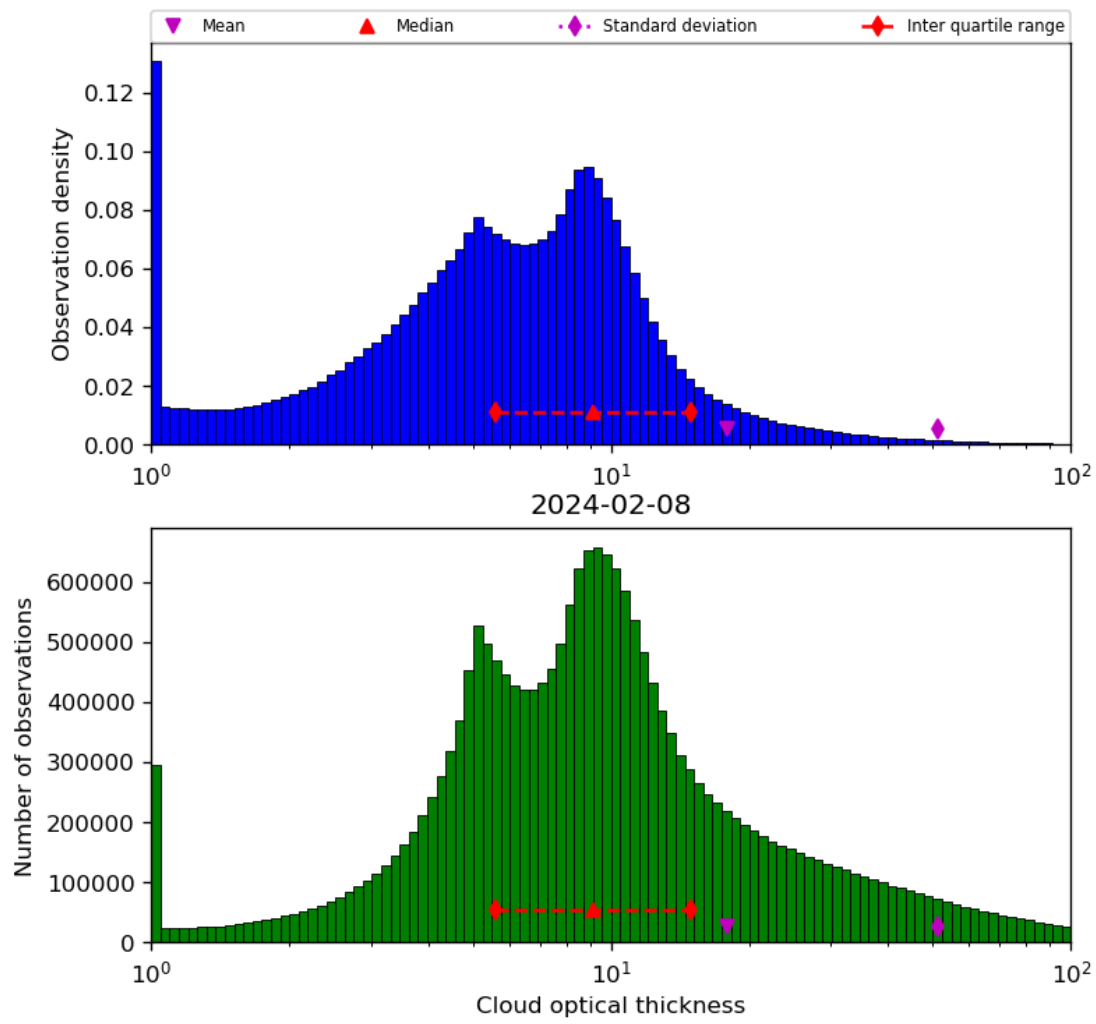
Figure 41: Histogram of “Cloud optical thickness” for 2024-02-07 to 2024-02-09
