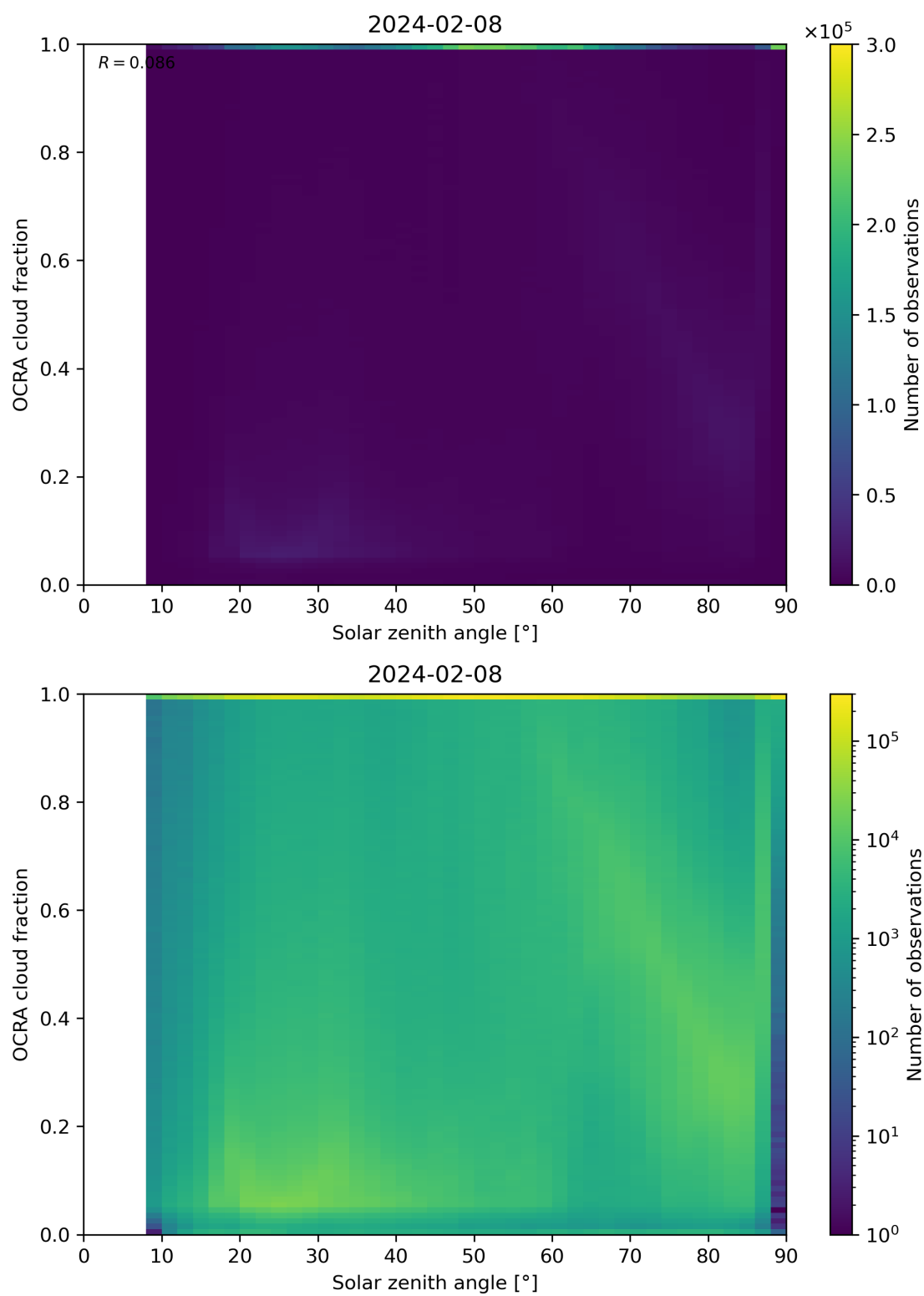
Figure 100: Scatter density plot of “Solar zenith angle” against “OCRA cloud fraction” for 2024-02-07 to 2024-02-09.
