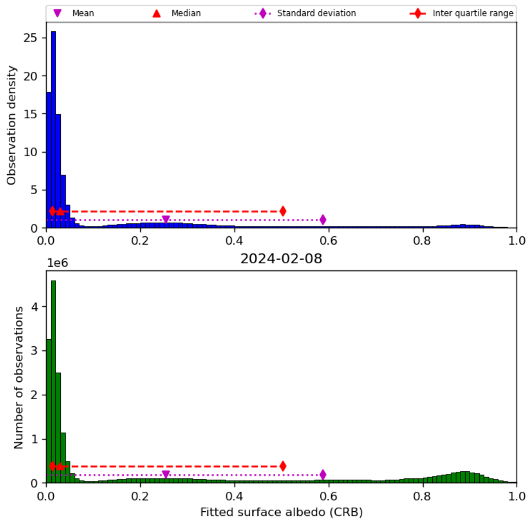
Figure 46: Histogram of “Fitted surface albedo (CRB)” for 2024-02-07 to 2024-02-09
