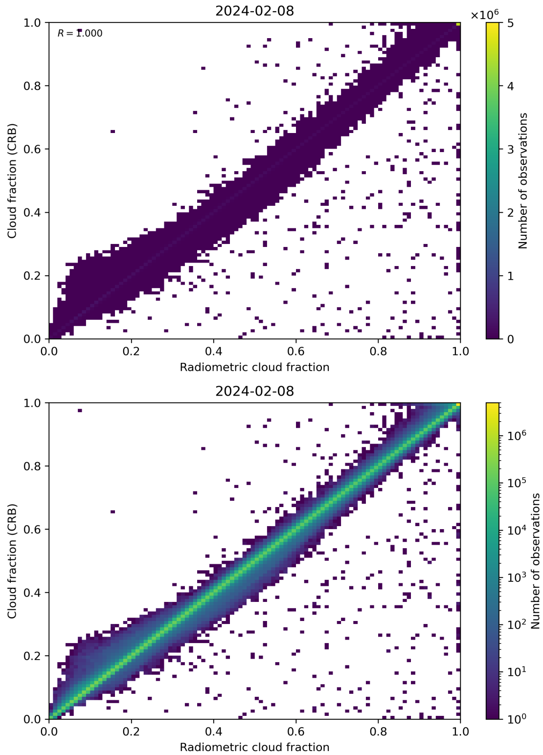
Figure 73: Scatter density plot of “Radiometric cloud fraction” against “Cloud fraction (CRB)” for 2024-02-07 to 2024-02-09.
