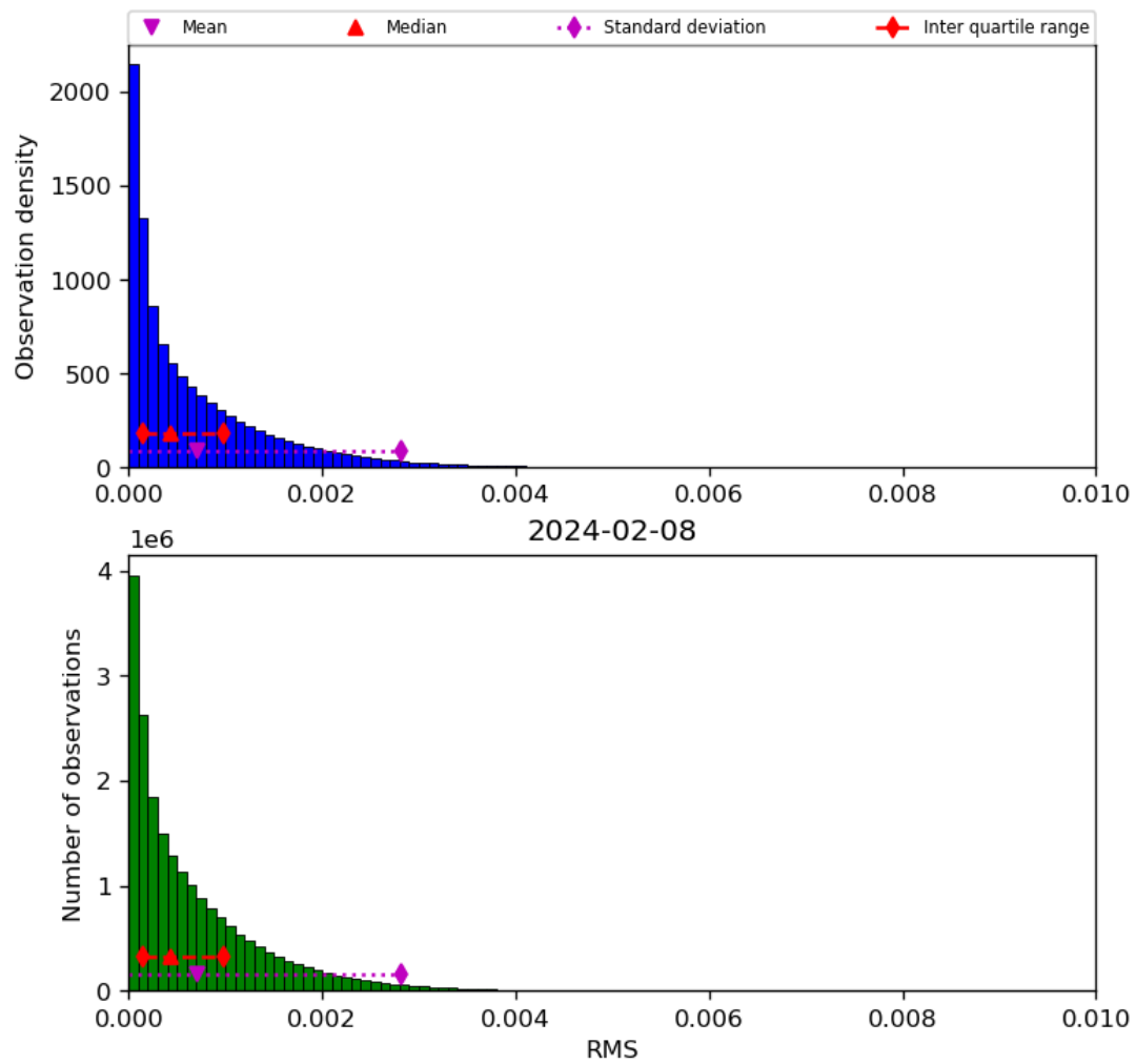
Figure 47: Histogram of “RMS” for 2024-02-07 to 2024-02-09
