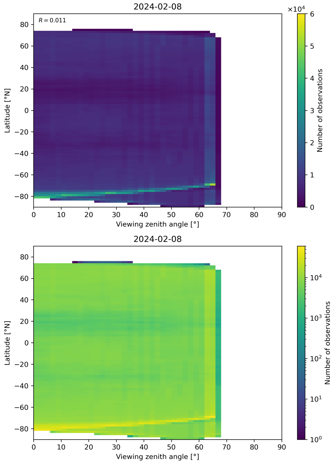
Figure 113: Scatter density plot of “Viewing zenith angle” against “Latitude” for 2024-02-07 to 2024-02-09.
