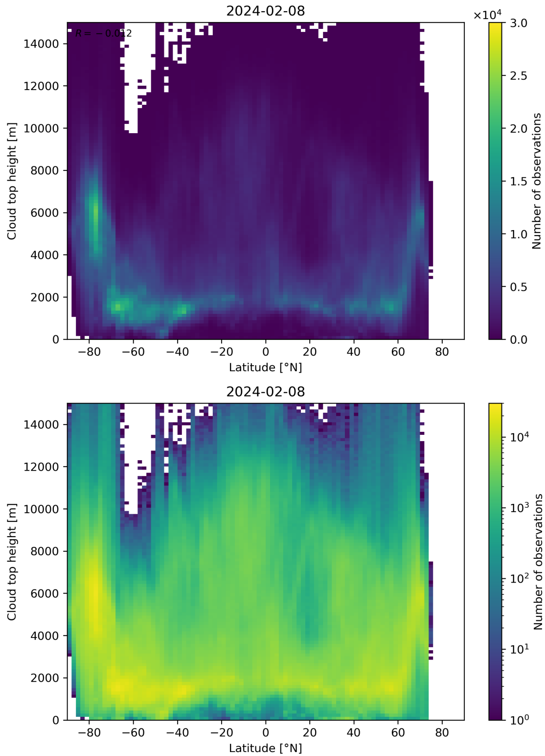
Figure 97: Scatter density plot of “Latitude” against “Cloud top height” for 2024-02-07 to 2024-02-09.
