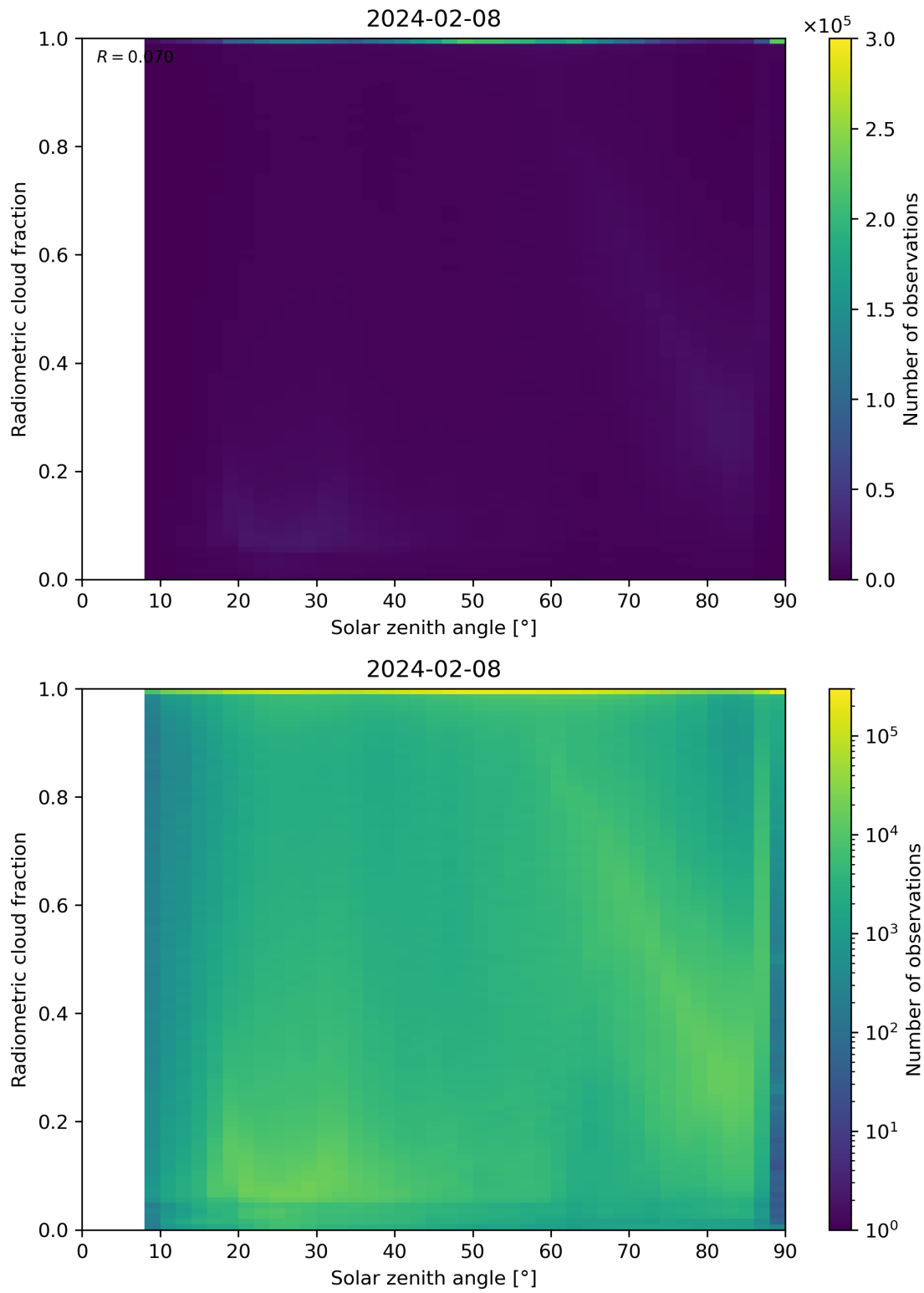
Figure 99: Scatter density plot of “Solar zenith angle” against “Radiometric cloud fraction” for 2024-02-07 to 2024-02-09.
