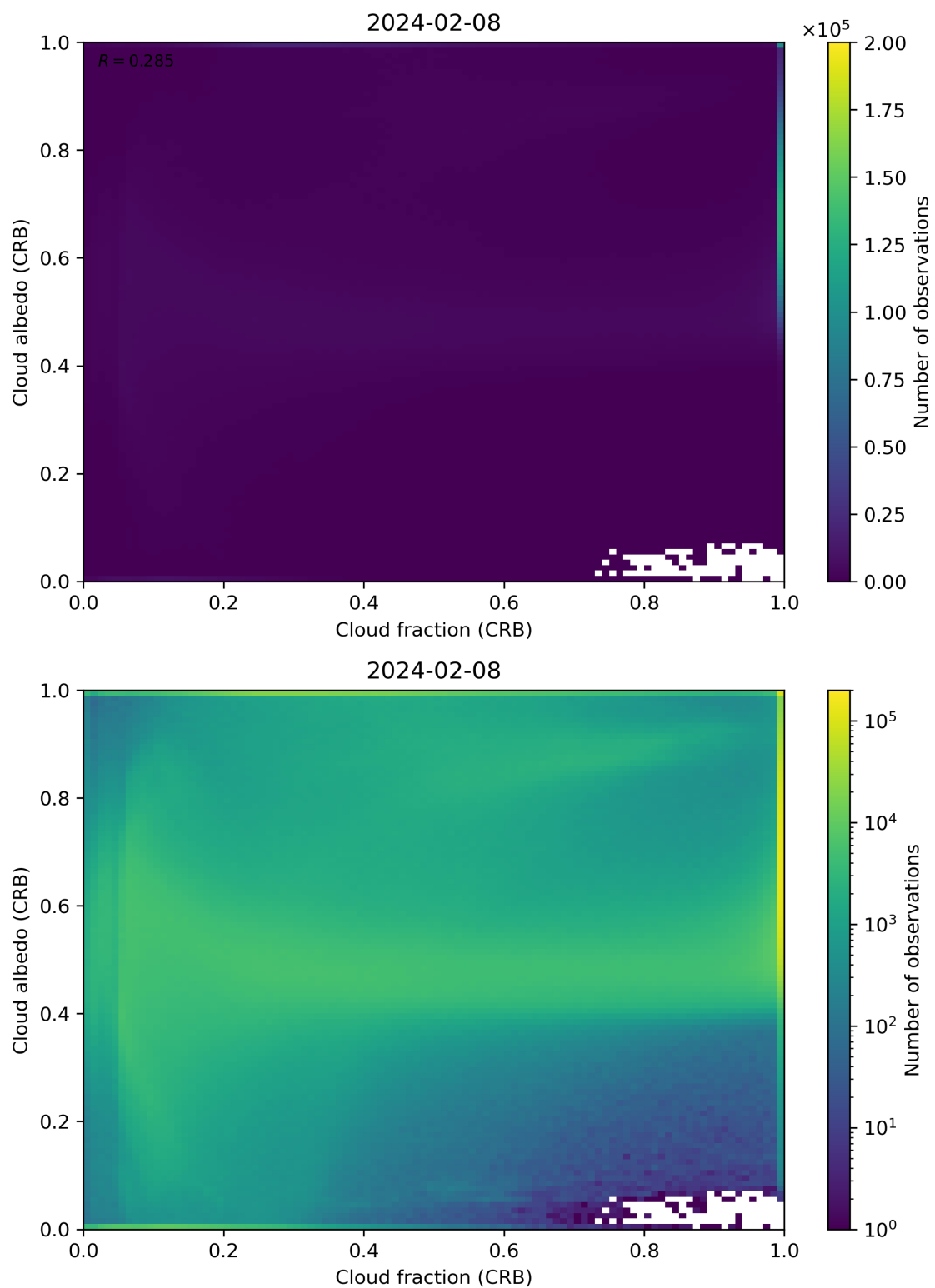
Figure 77: Scatter density plot of “Cloud fraction (CRB)” against “Cloud albedo (CRB)” for 2024-02-07 to 2024-02-09.
