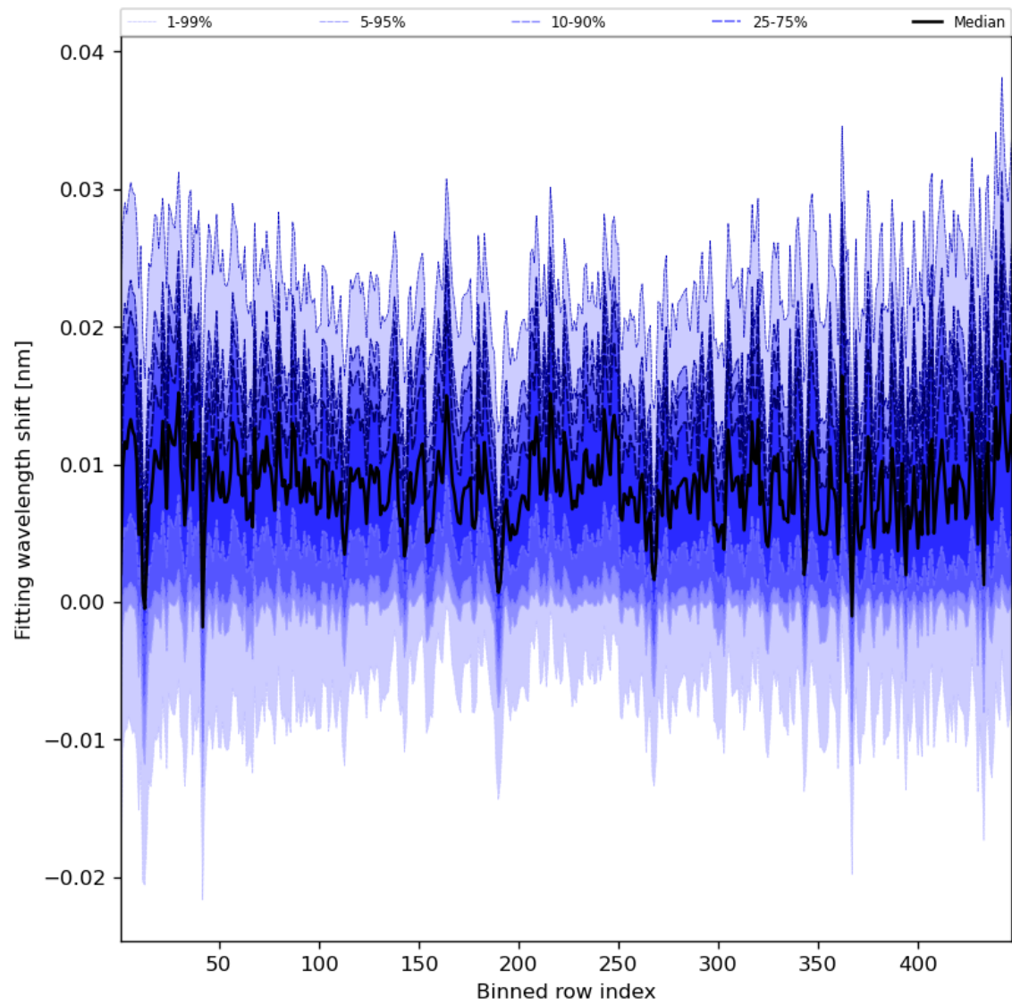
Figure 65: Along track statistics of “Fitting wavelength shift” for 2024-02-07 to 2024-02-09
