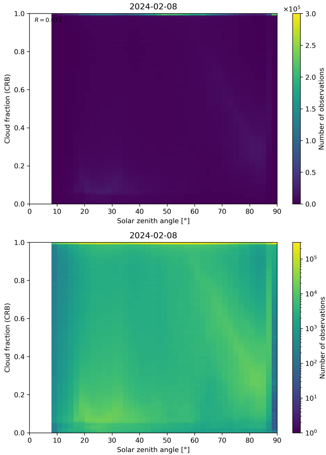
Figure 101: Scatter density plot of “Solar zenith angle” against “Cloud fraction (CRB)” for 2024-02-07 to 2024-02-09.
