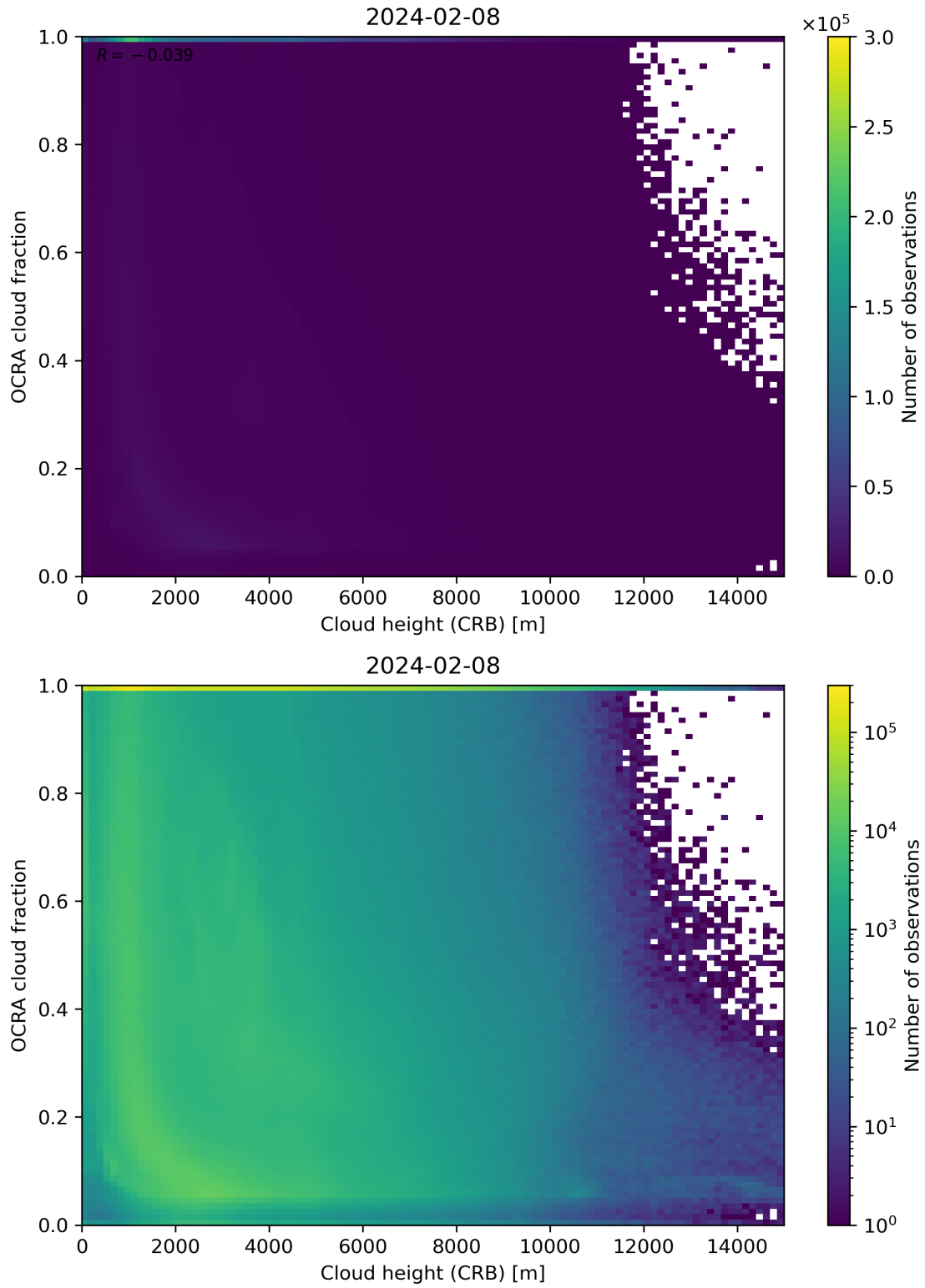
Figure 81: Scatter density plot of “Cloud height (CRB)” against “OCRA cloud fraction” for 2024-02-07 to 2024-02-09.
