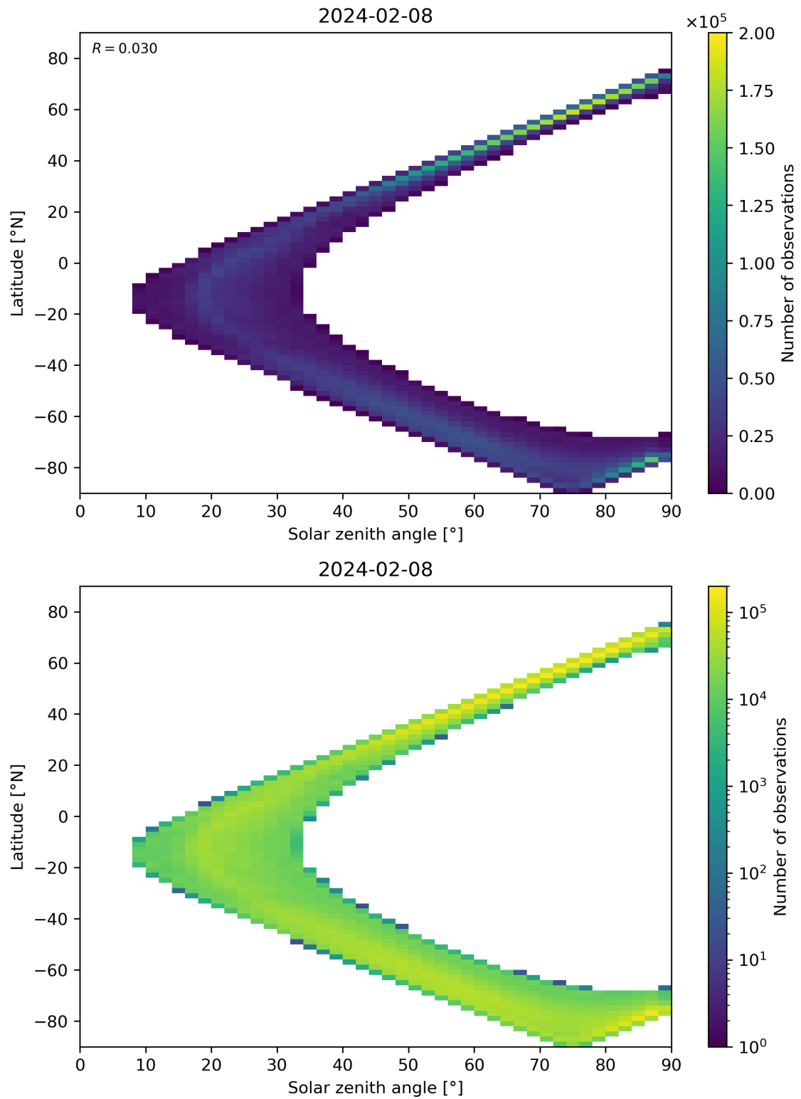
Figure 105: Scatter density plot of “Solar zenith angle” against “Latitude” for 2024-02-07 to 2024-02-09.
