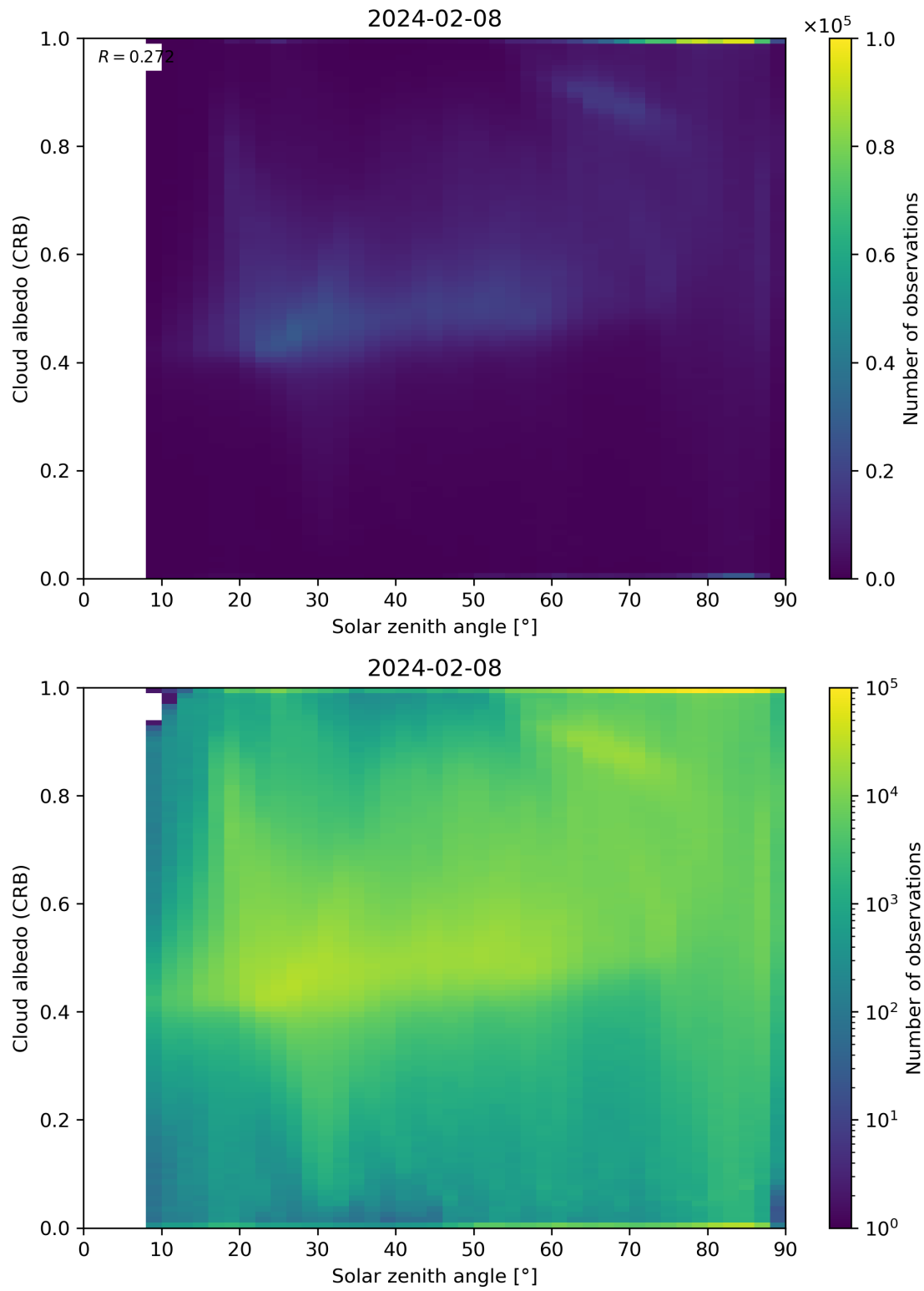
Figure 98: Scatter density plot of “Solar zenith angle” against “Cloud albedo (CRB)” for 2024-02-07 to 2024-02-09.
