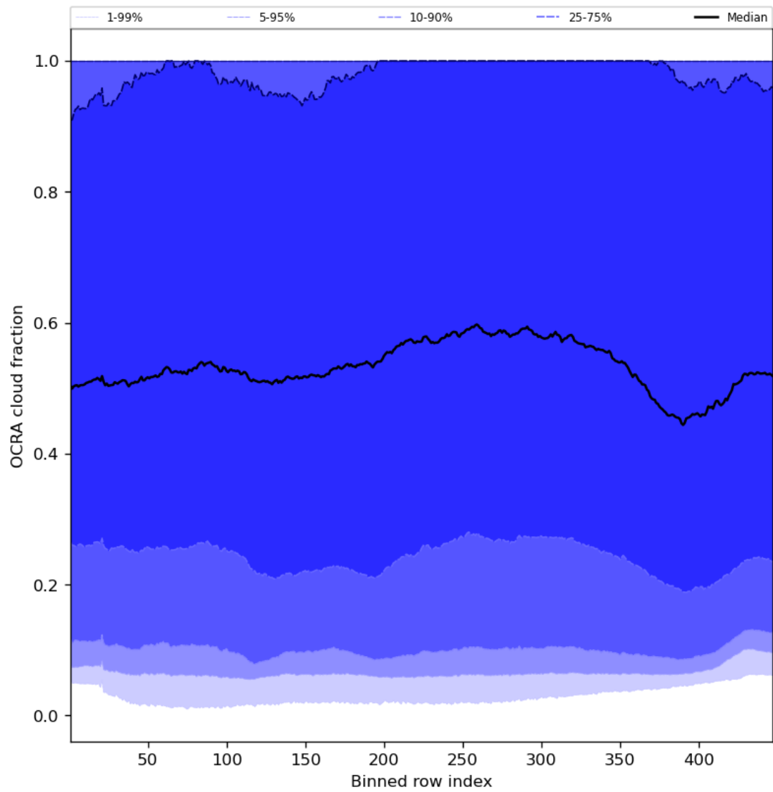
Figure 66: Along track statistics of “OCRA cloud fraction” for 2024-02-07 to 2024-02-09
