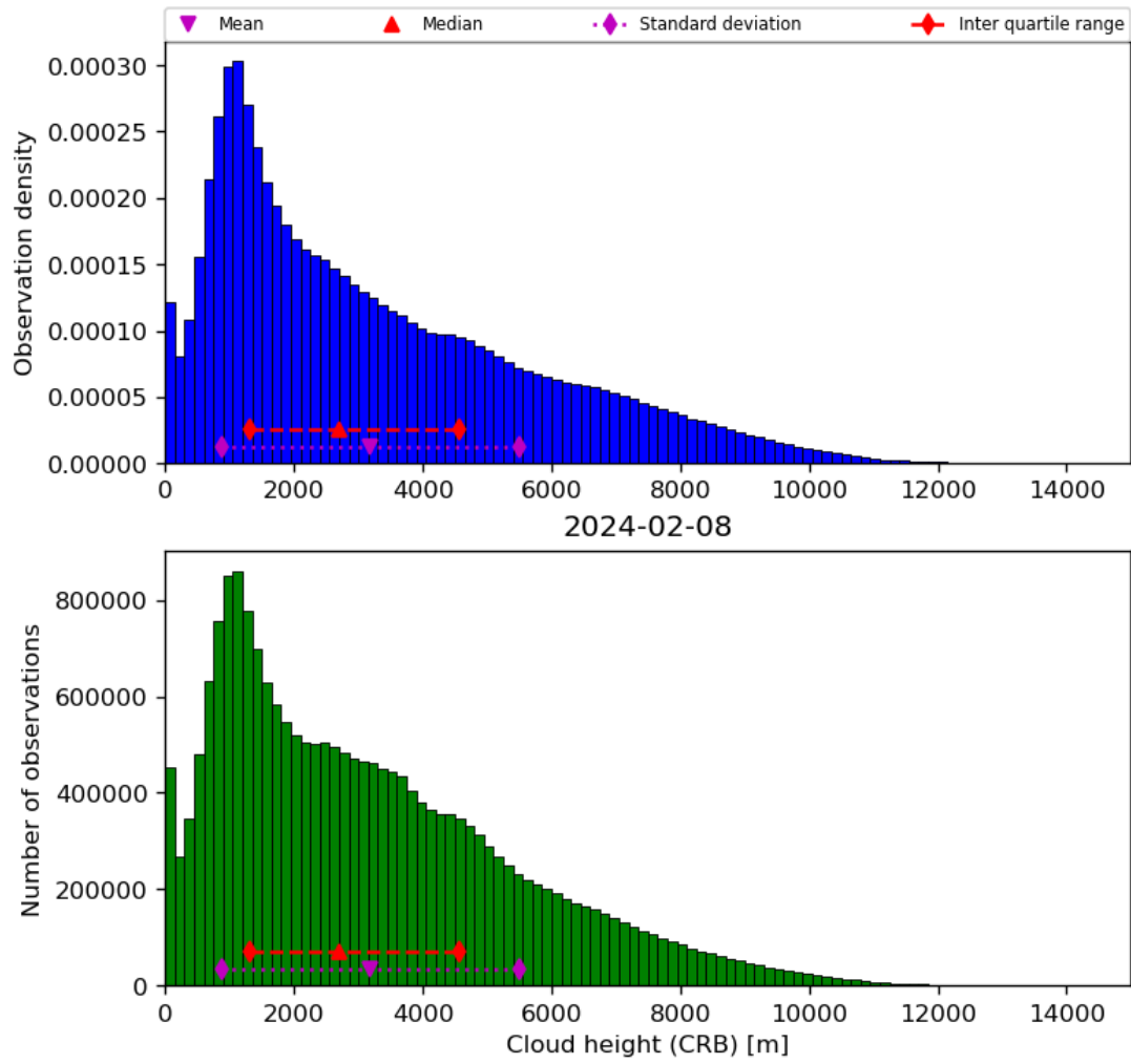
Figure 43: Histogram of “Cloud height (CRB)” for 2024-02-07 to 2024-02-09
