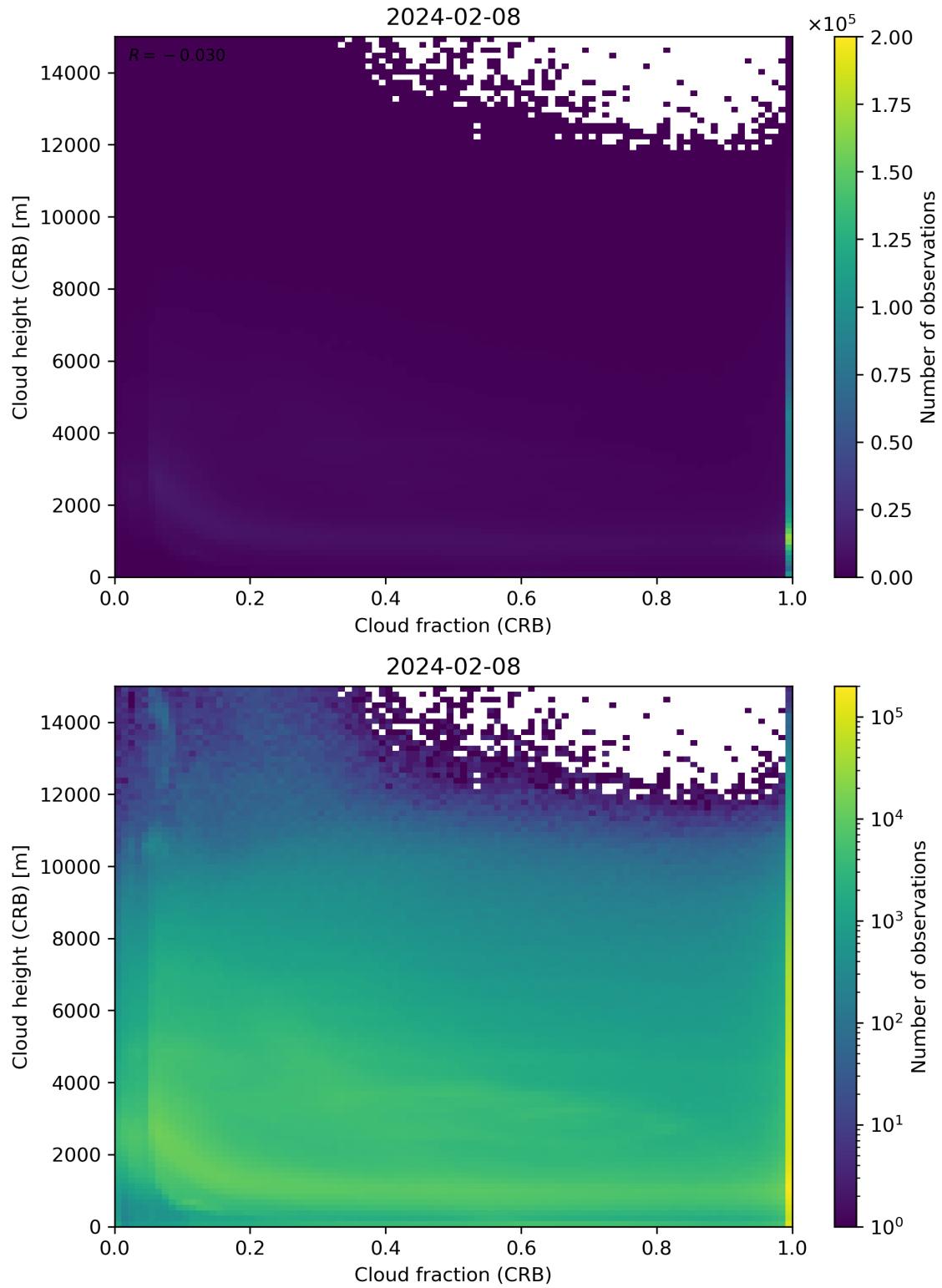
Figure 79: Scatter density plot of “Cloud fraction (CRB)” against “Cloud height (CRB)” for 2024-02-07 to 2024-02-09.
