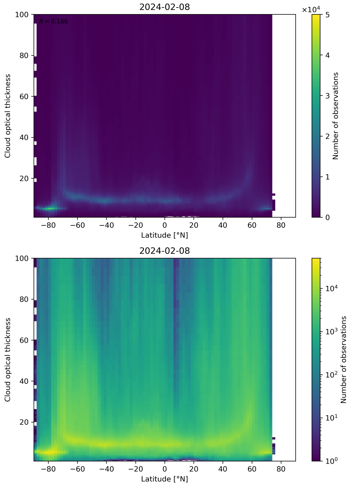
Figure 96: Scatter density plot of “Latitude” against “Cloud optical thickness” for 2024-02-07 to 2024-02-09.
