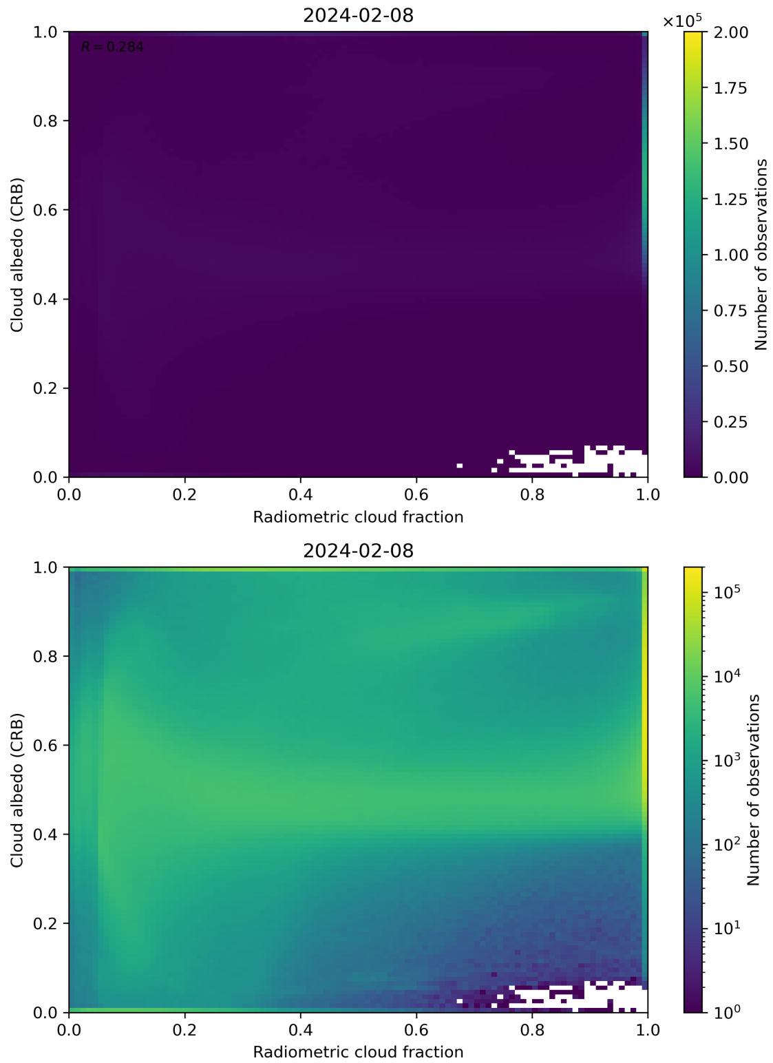
Figure 71: Scatter density plot of “Radiometric cloud fraction” against “Cloud albedo (CRB)” for 2024-02-07 to 2024-02-09.
