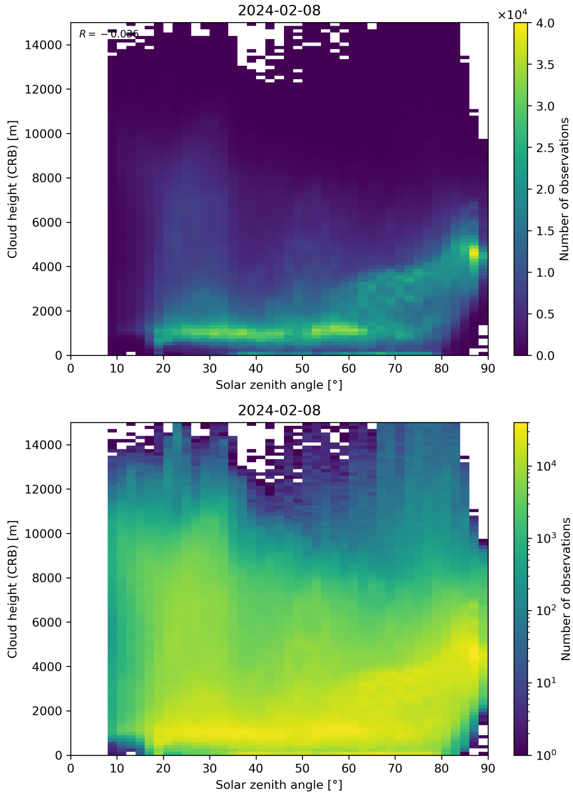
Figure 102: Scatter density plot of “Solar zenith angle” against “Cloud height (CRB)” for 2024-02-07 to 2024-02-09.
