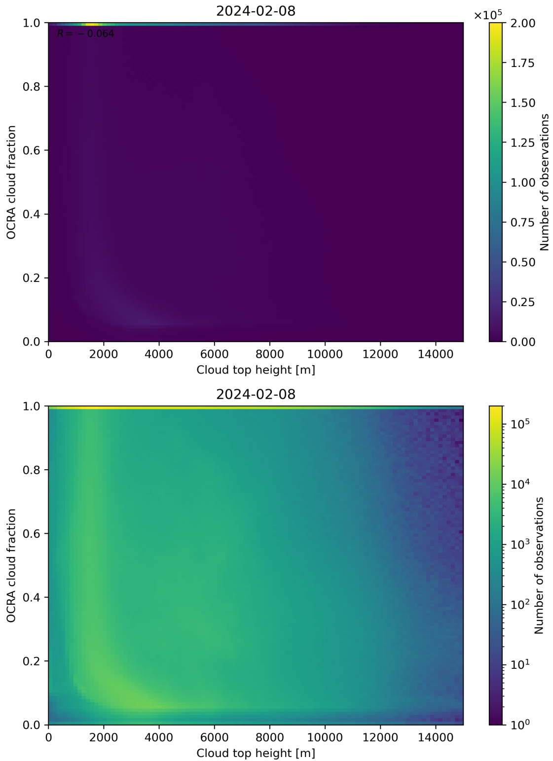
Figure 87: Scatter density plot of “Cloud top height” against “OCRA cloud fraction” for 2024-02-07 to 2024-02-09.
