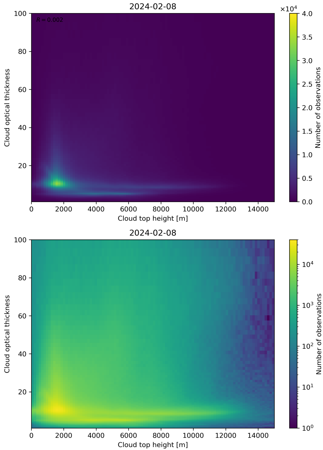
Figure 90: Scatter density plot of “Cloud top height” against “Cloud optical thickness” for 2024-02-07 to 2024-02-09.
