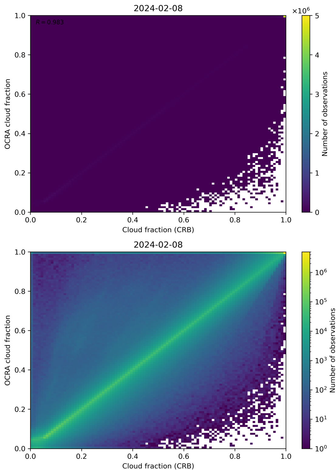
Figure 78: Scatter density plot of “Cloud fraction (CRB)” against “OCRA cloud fraction” for 2024-02-07 to 2024-02-09.
