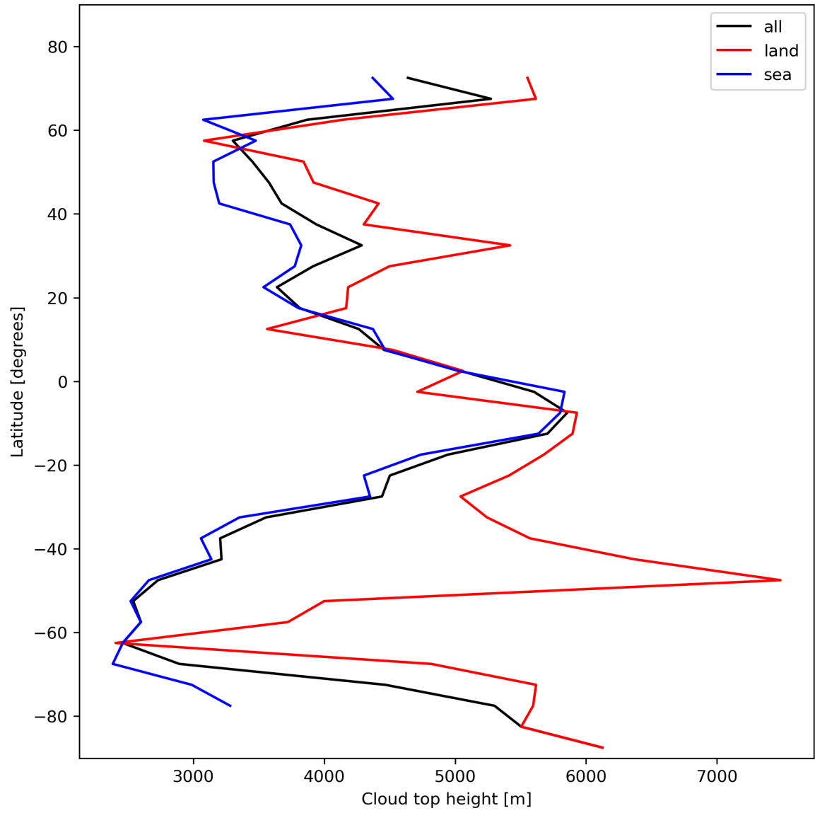
Figure 24: Zonal average of “Cloud top height” for 2024-02-07 to 2024-02-09.
