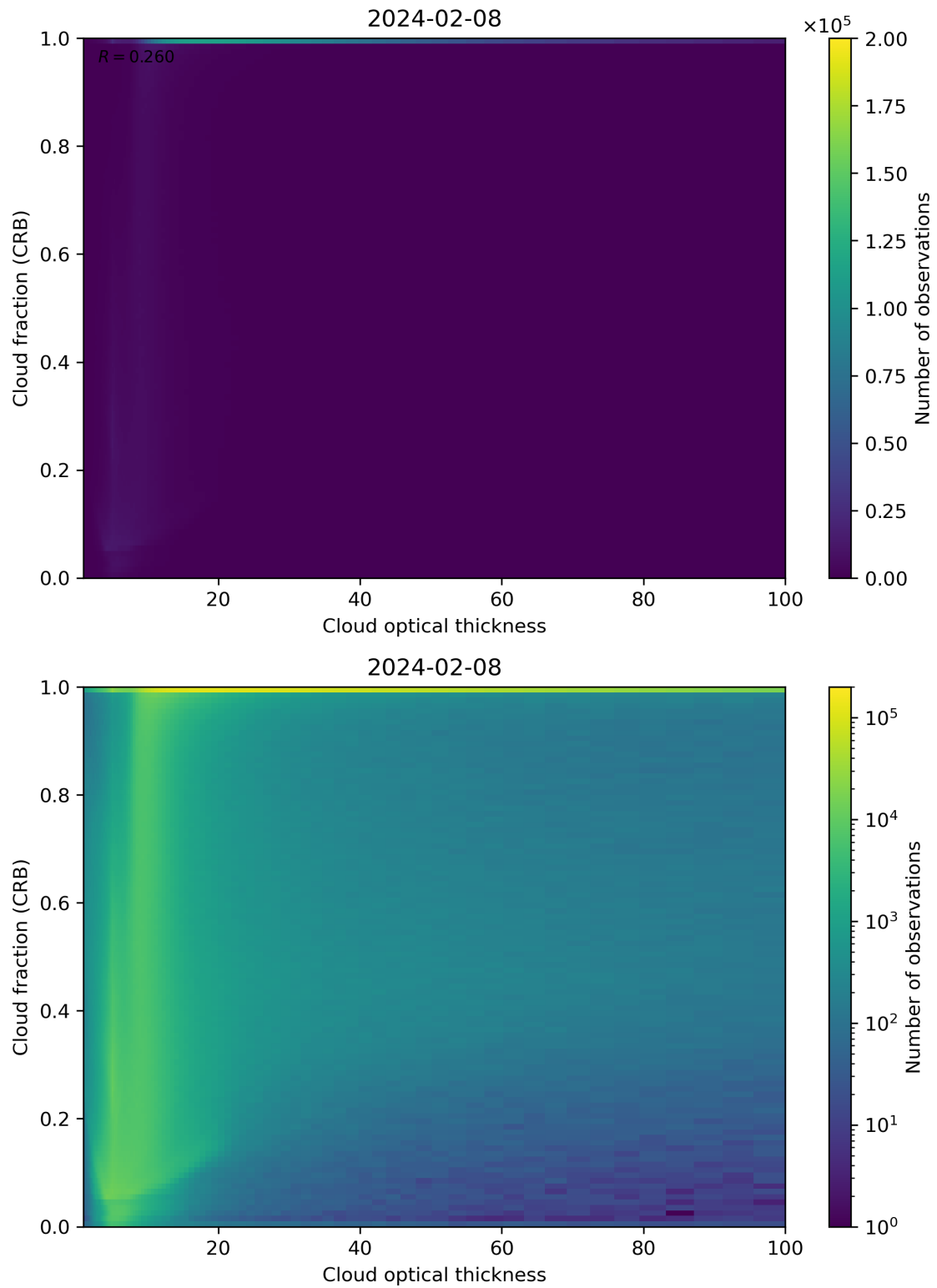
Figure 84: Scatter density plot of “Cloud optical thickness” against “Cloud fraction (CRB)” for 2024-02-07 to 2024-02-09.
