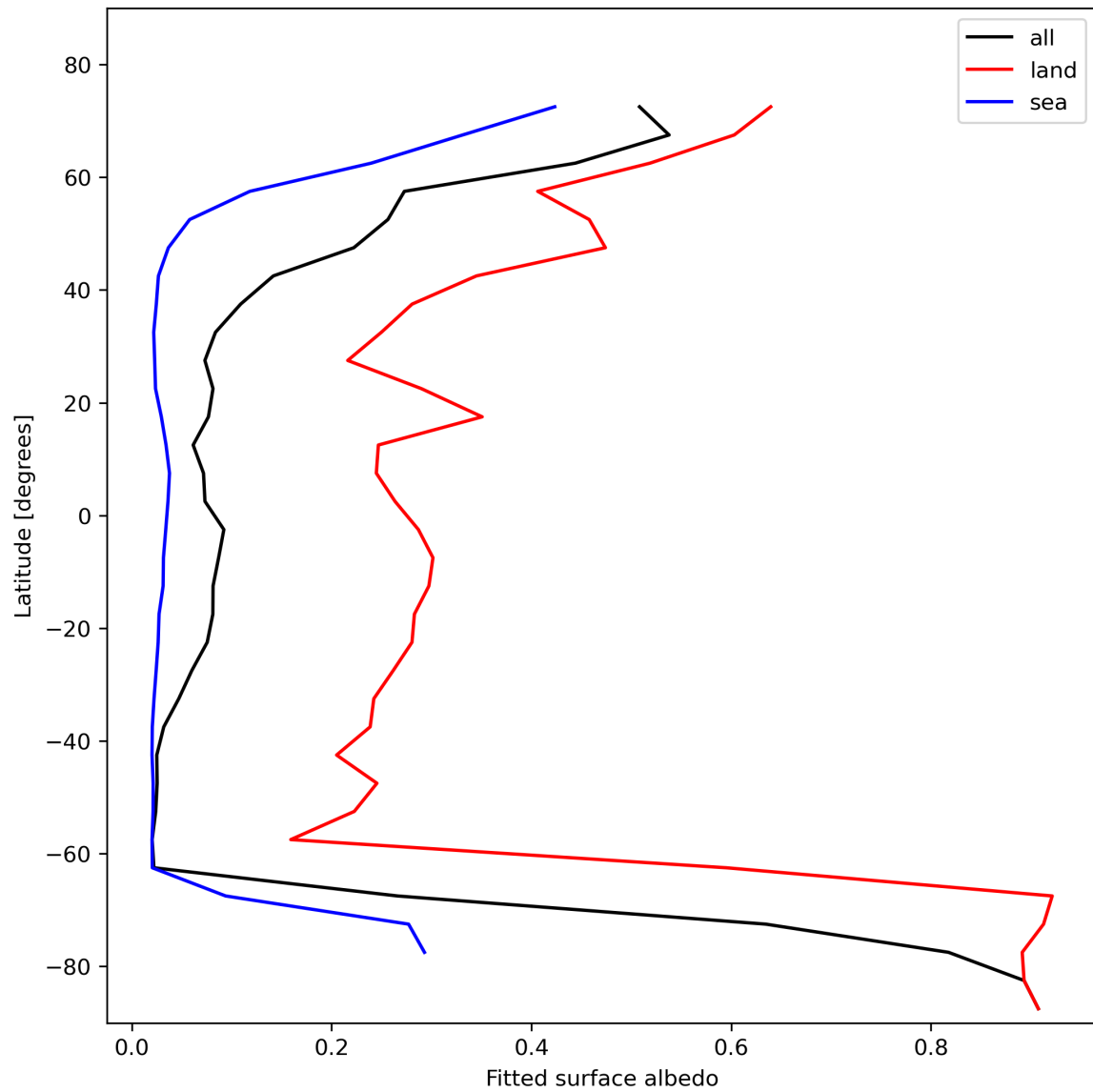
Figure 29: Zonal average of “Fitted surface albedo” for 2024-02-07 to 2024-02-09.
