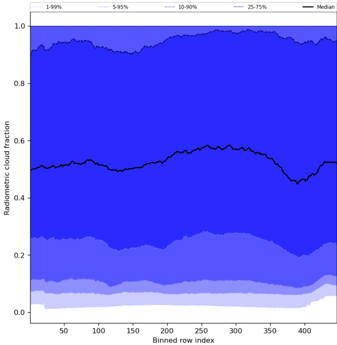
Figure 55: Along track statistics of “Radiometric cloud fraction” for 2024-02-07 to 2024-02-09
