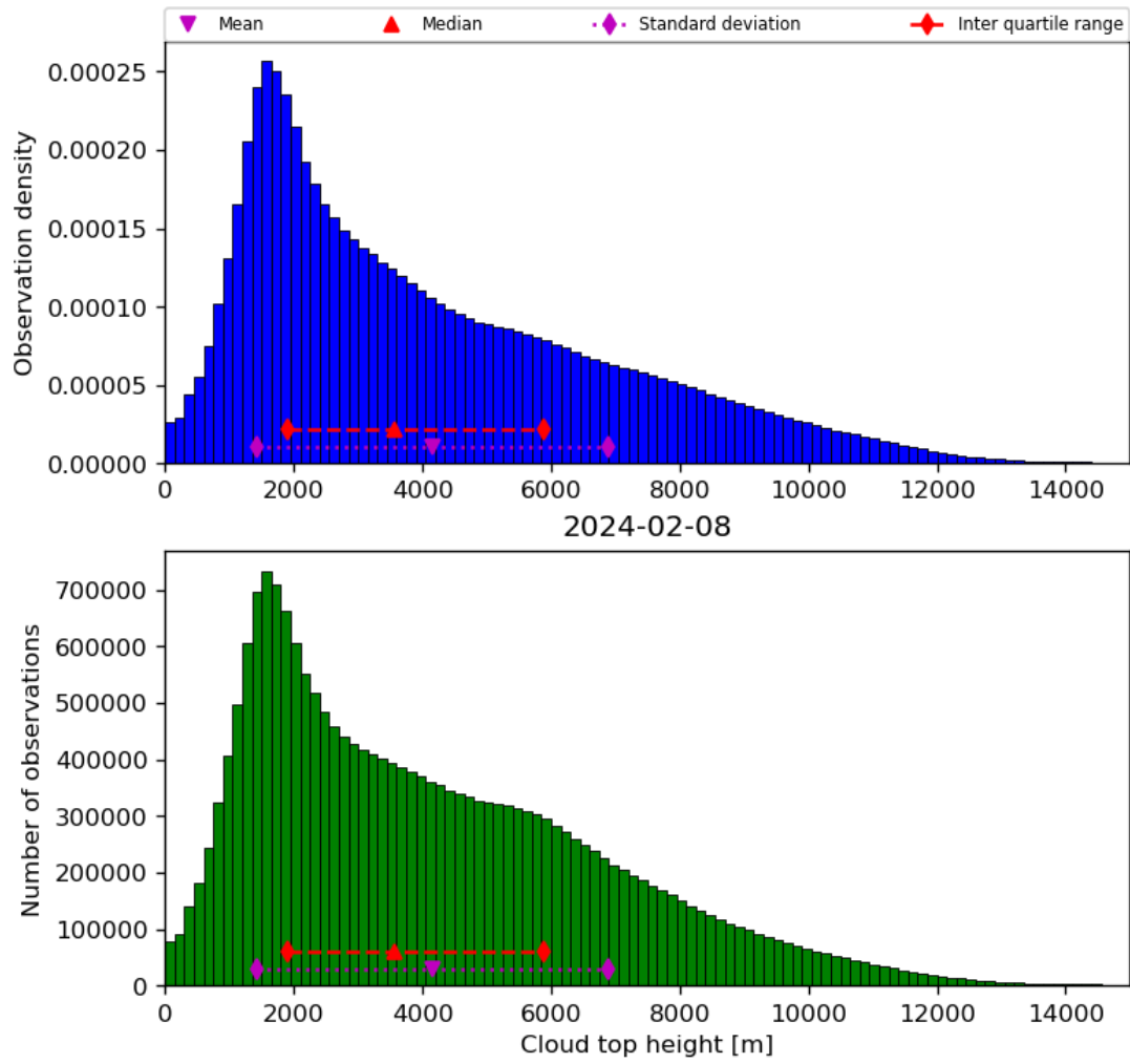
Figure 40: Histogram of “Cloud top height” for 2024-02-07 to 2024-02-09
