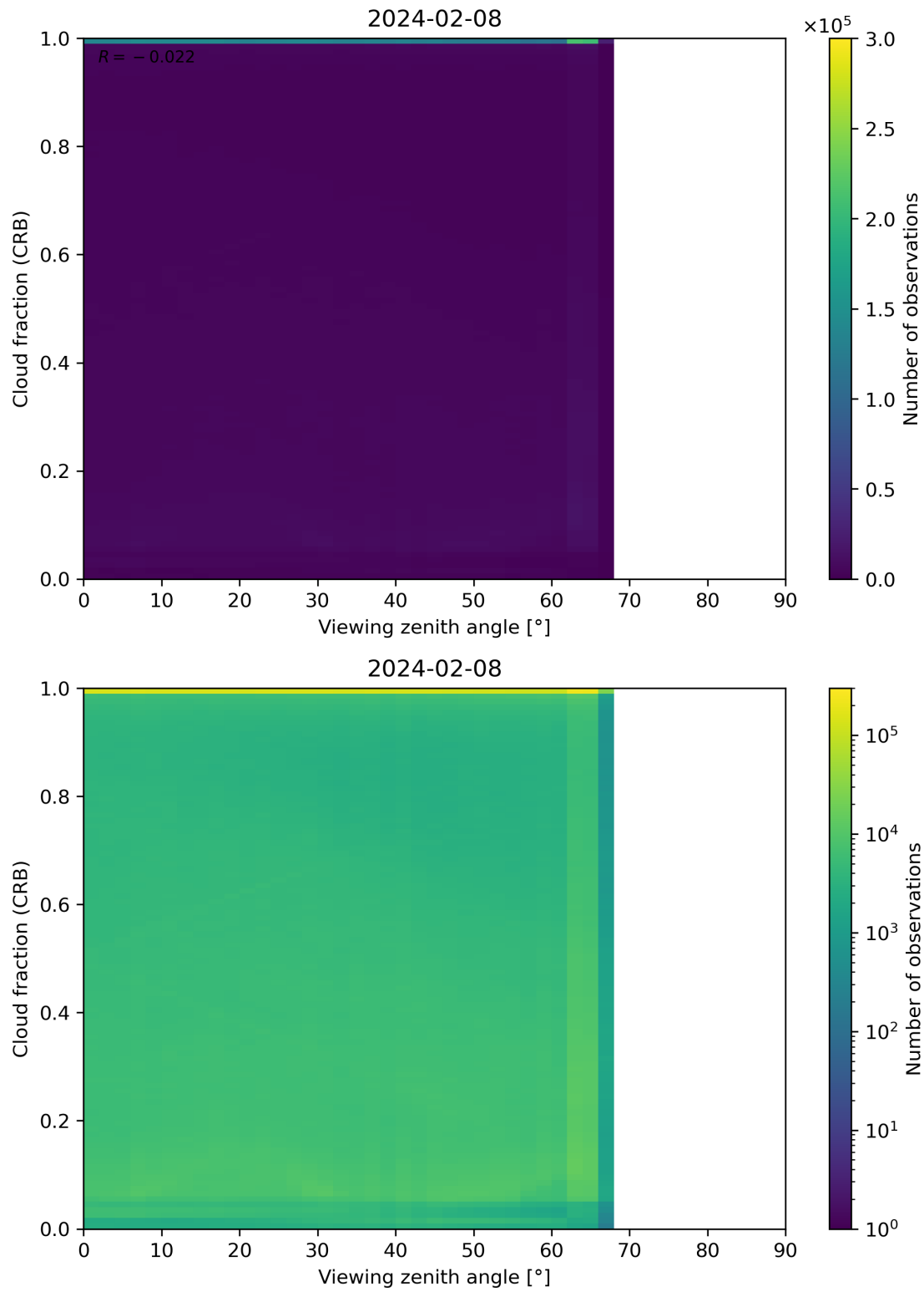
Figure 109: Scatter density plot of “Viewing zenith angle” against “Cloud fraction (CRB)” for 2024-02-07 to 2024-02-09.
