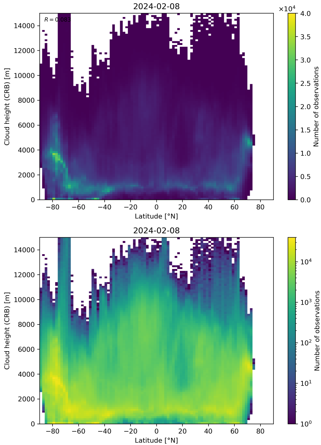
Figure 95: Scatter density plot of “Latitude” against “Cloud height (CRB)” for 2024-02-07 to 2024-02-09.
