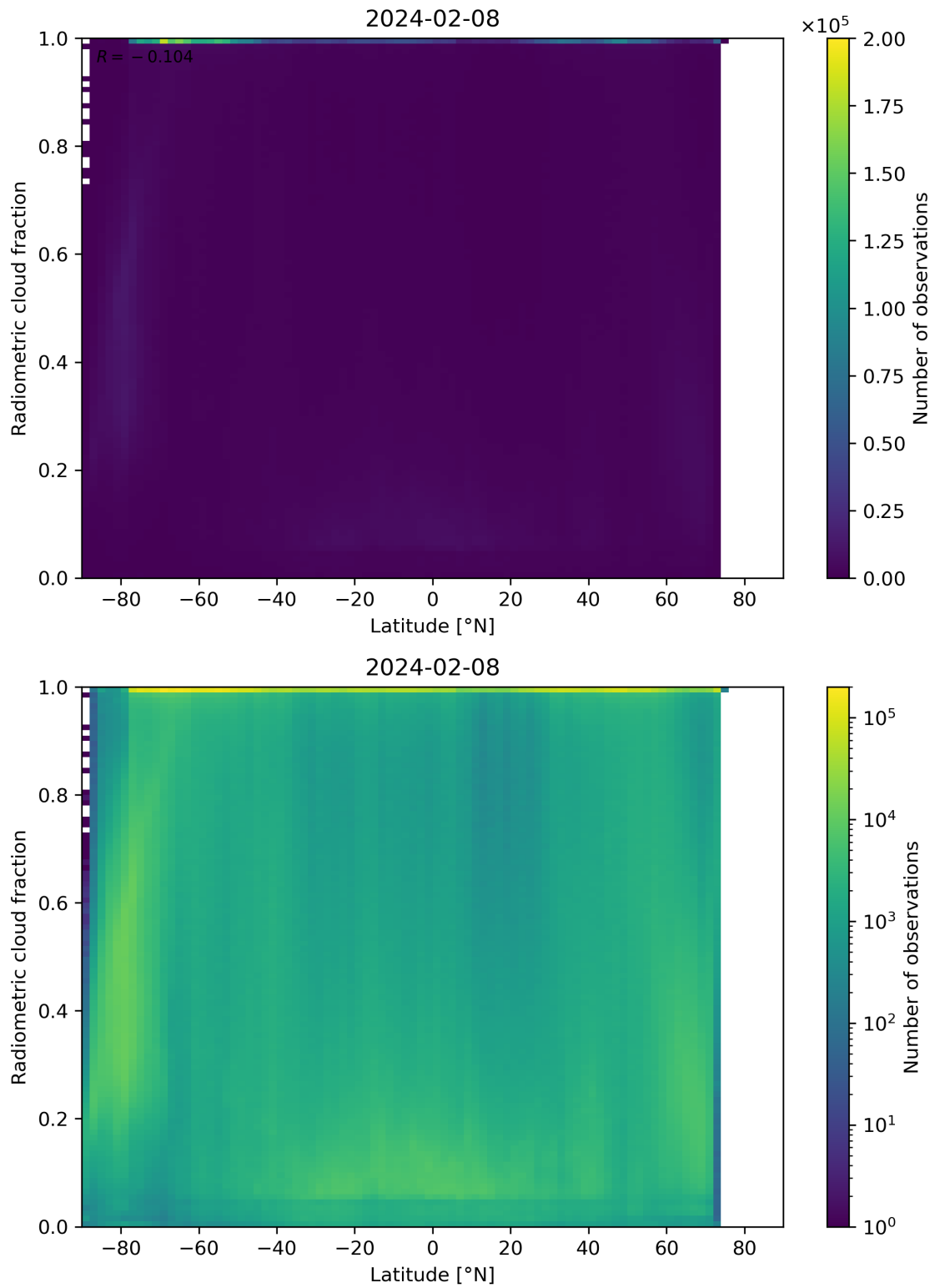
Figure 92: Scatter density plot of “Latitude” against “Radiometric cloud fraction” for 2024-02-07 to 2024-02-09.
