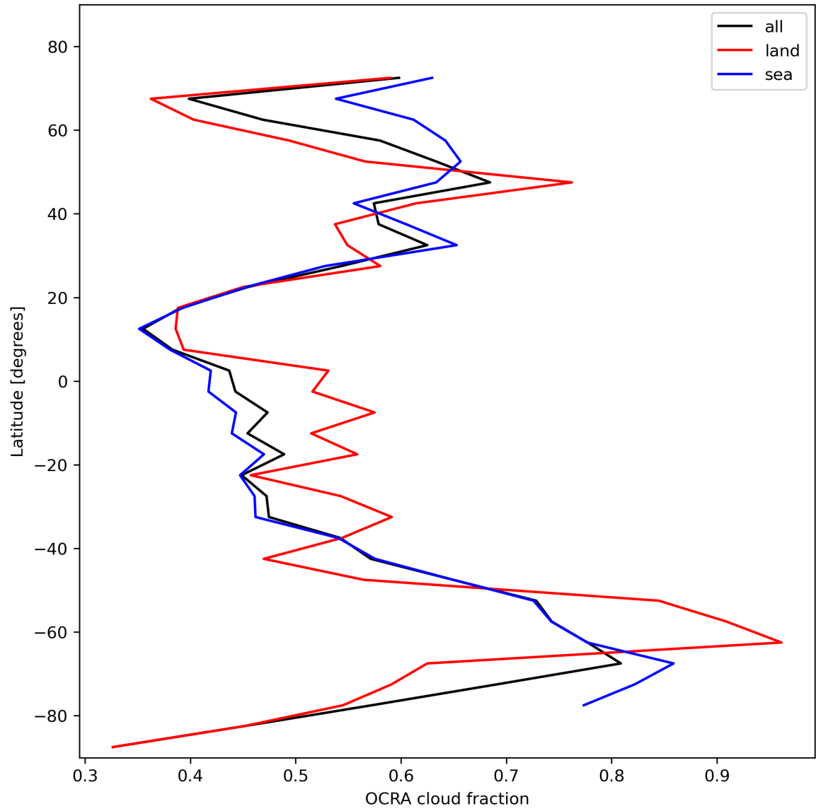
Figure 34: Zonal average of “OCRA cloud fraction” for 2024-02-07 to 2024-02-09.
