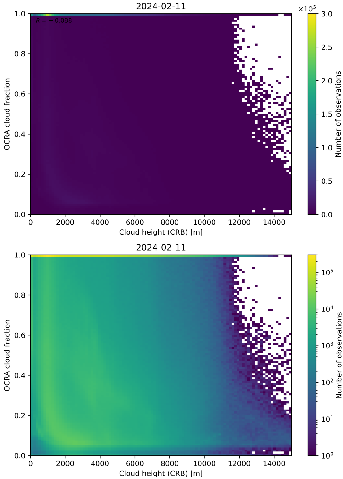
Figure 81: Scatter density plot of “Cloud height (CRB)” against “OCRA cloud fraction” for 2024-02-11 to 2024-02-12.
