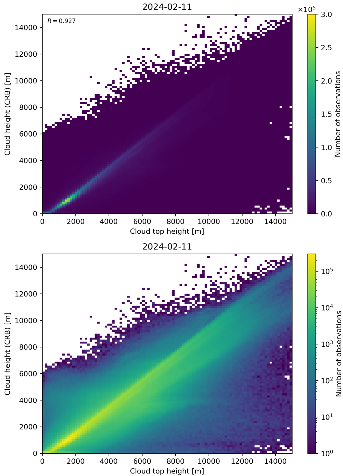
Figure 89: Scatter density plot of “Cloud top height” against “Cloud height (CRB)” for 2024-02-11 to 2024-02-12.
