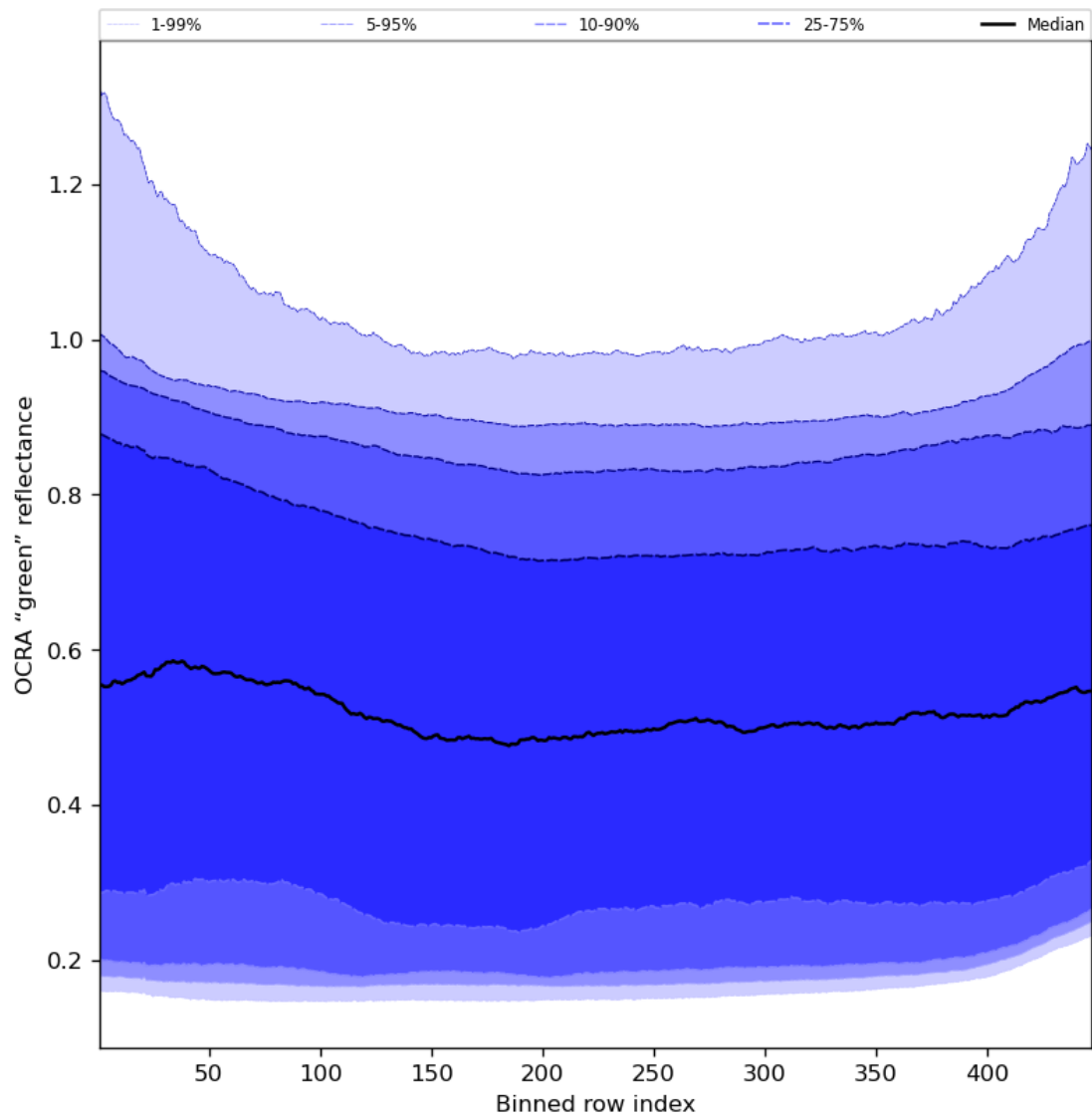
Figure 68: Along track statistics of “OCRA “green” reflectance” for 2024-02-11 to 2024-02-12
