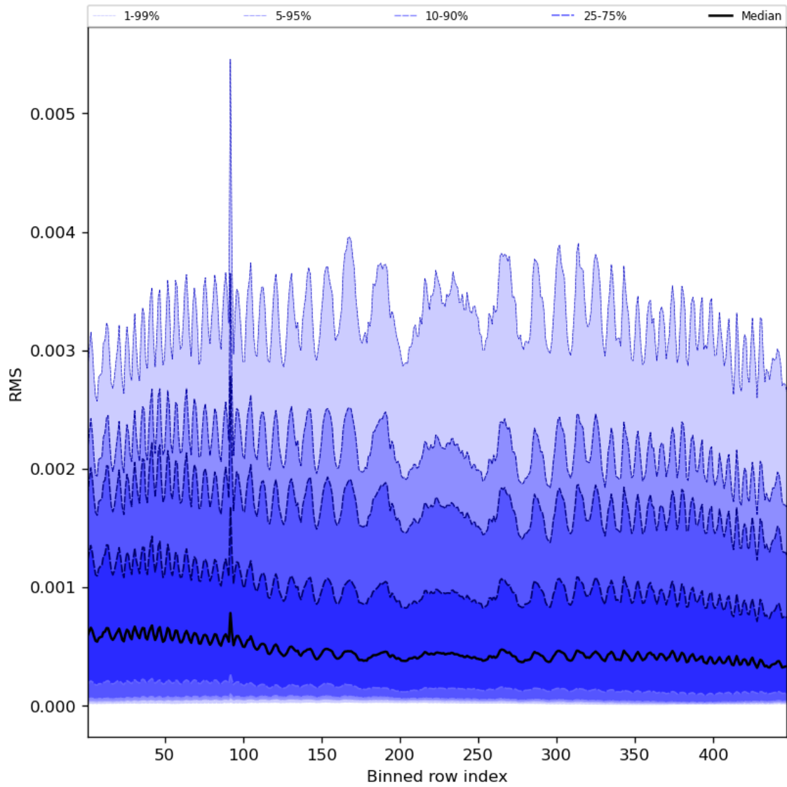
Figure 63: Along track statistics of “RMS” for 2024-02-11 to 2024-02-12
