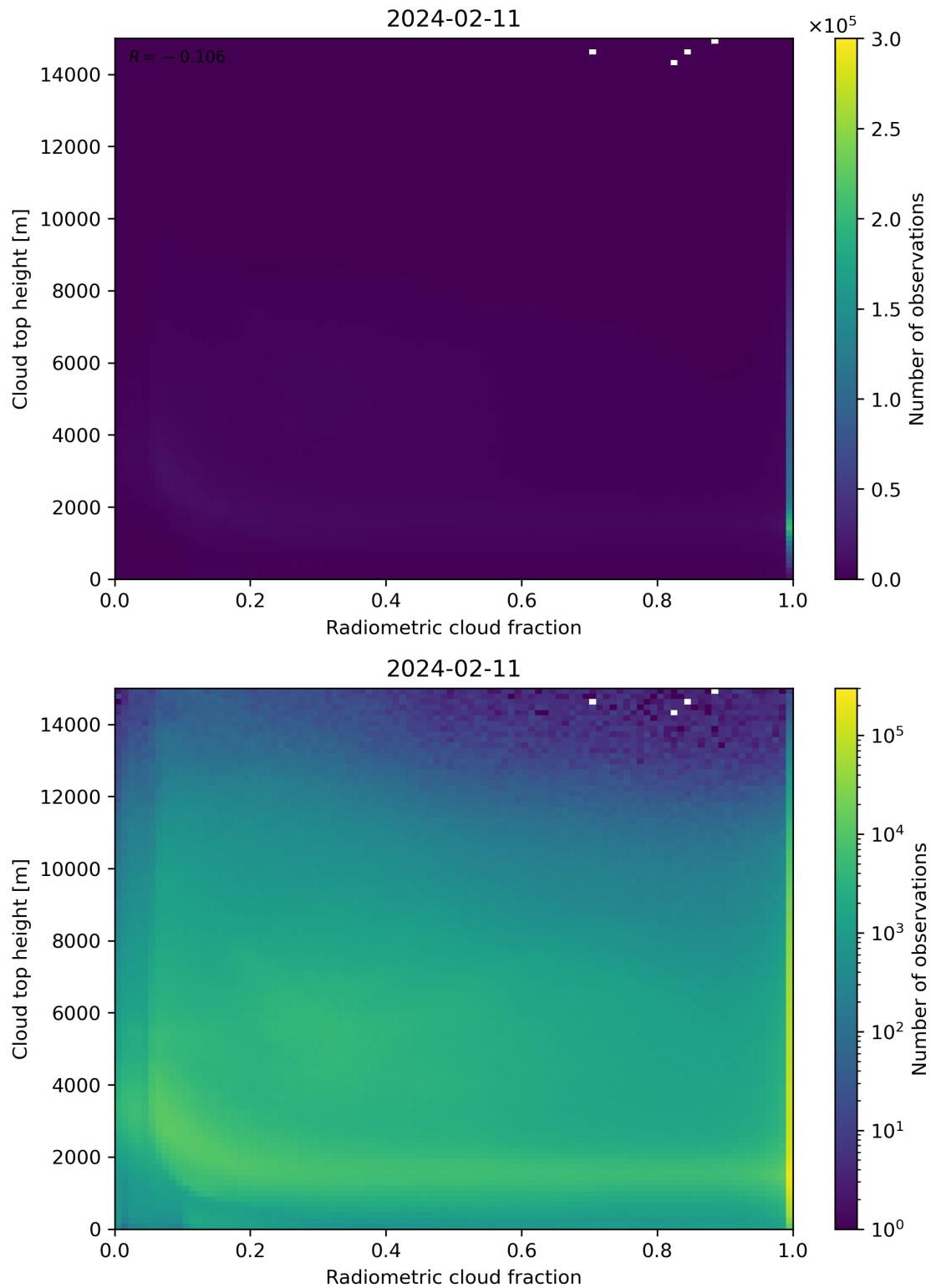
Figure 76: Scatter density plot of “Radiometric cloud fraction” against “Cloud top height” for 2024-02-11 to 2024-02-12.
