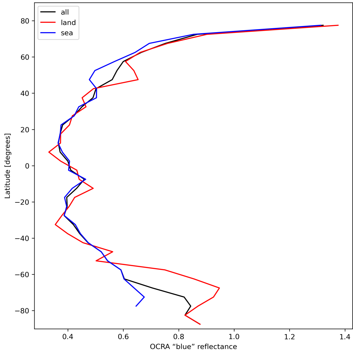
Figure 35: Zonal average of “OCRA “blue” reflectance” for 2024-02-11 to 2024-02-12.
