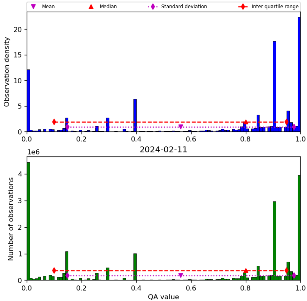
Figure 38: Histogram of “QA value” for 2024-02-11 to 2024-02-12
