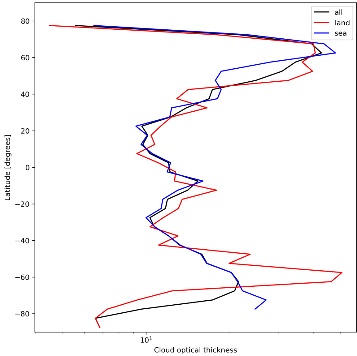
Figure 25: Zonal average of “Cloud optical thickness” for 2024-02-11 to 2024-02-12.
