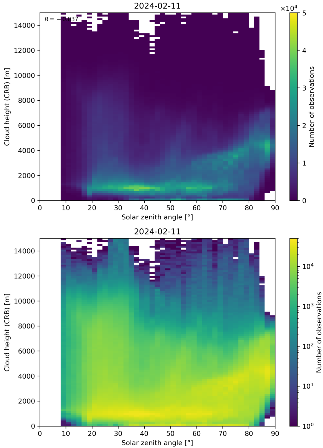
Figure 102: Scatter density plot of “Solar zenith angle” against “Cloud height (CRB)” for 2024-02-11 to 2024-02-12.
