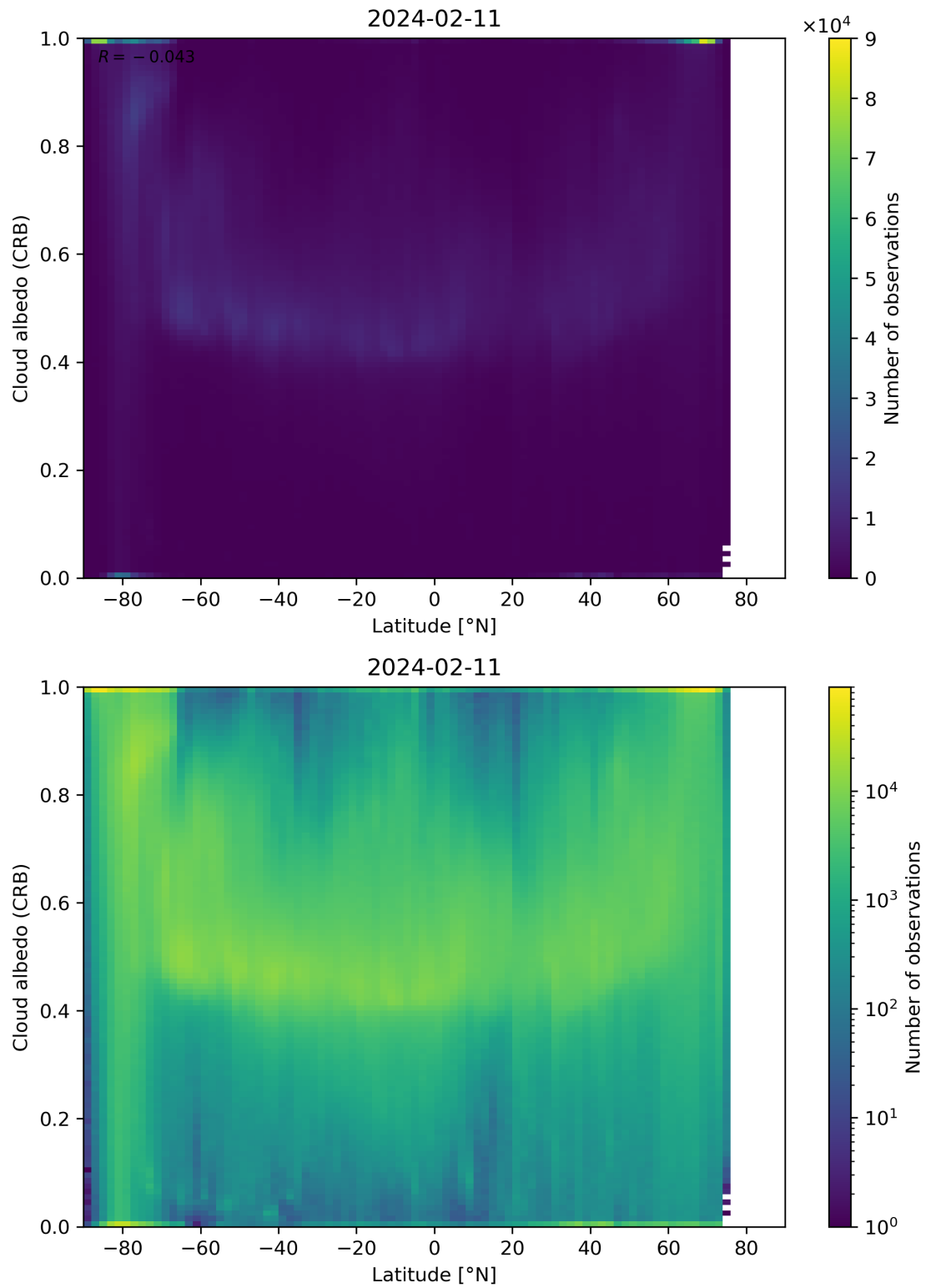
Figure 91: Scatter density plot of “Latitude” against “Cloud albedo (CRB)” for 2024-02-11 to 2024-02-12.
