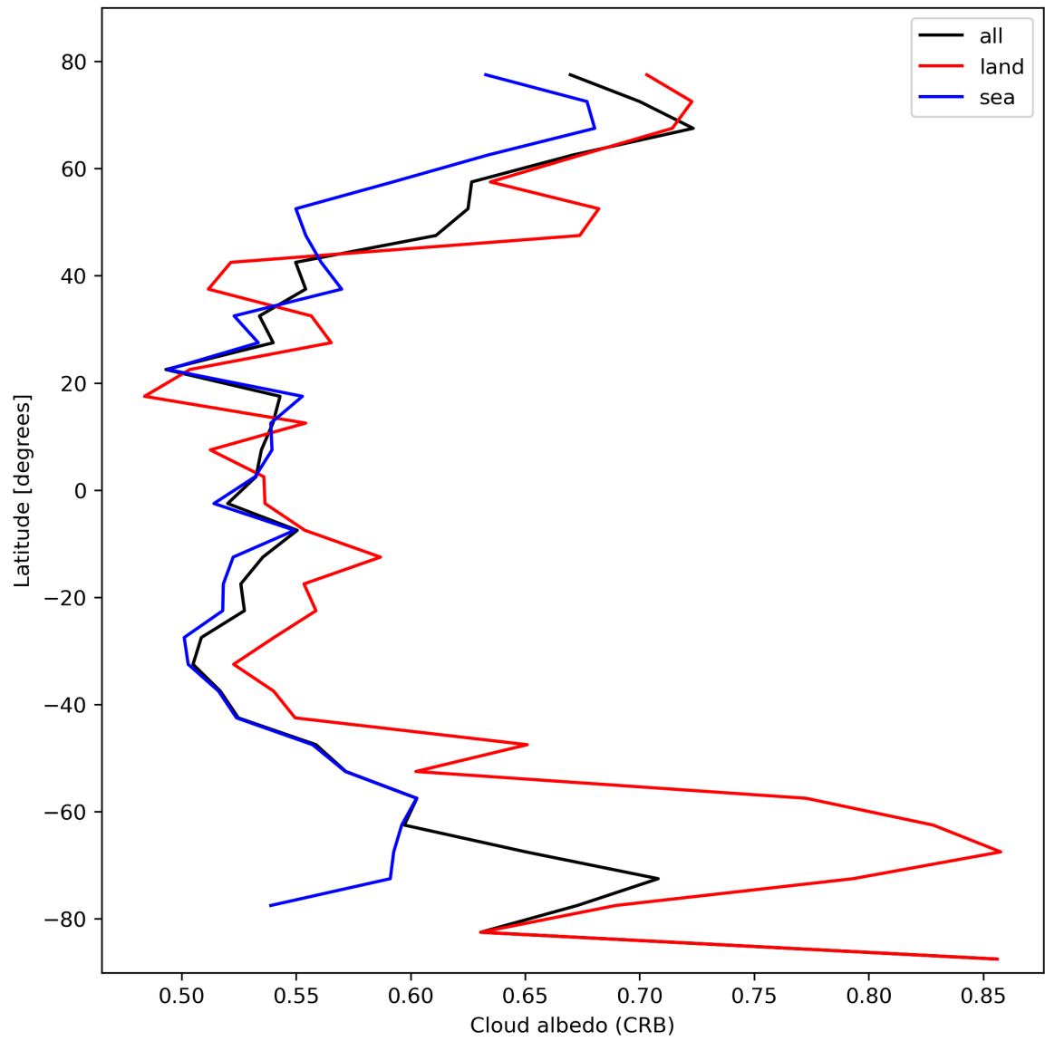
Figure 28: Zonal average of “Cloud albedo (CRB)” for 2024-02-11 to 2024-02-12.
