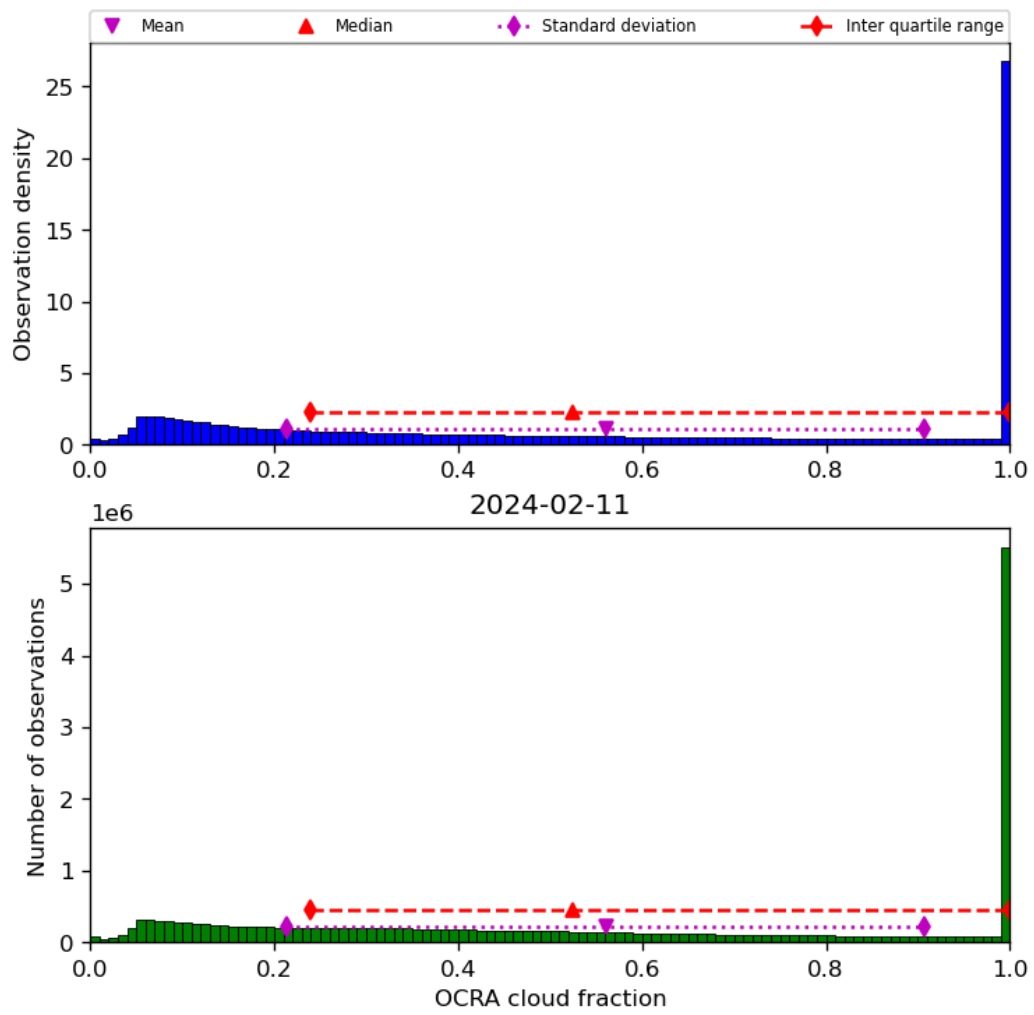
Figure 50: Histogram of “OCRA cloud fraction” for 2024-02-11 to 2024-02-12
