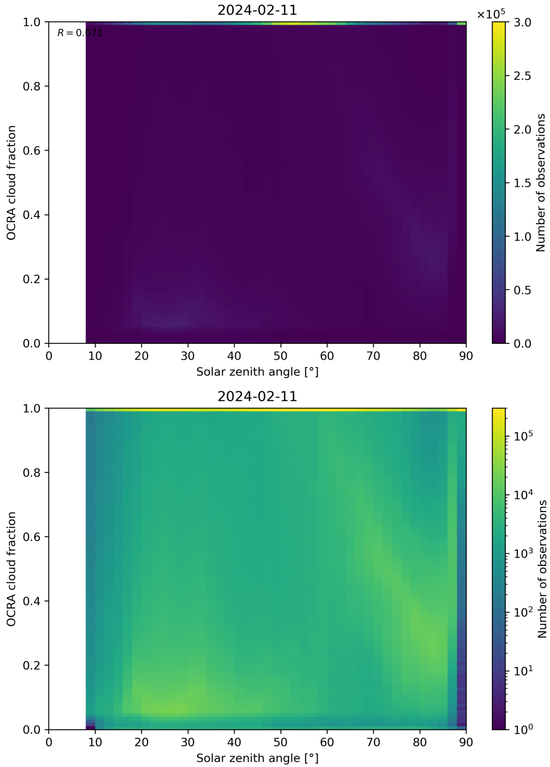
Figure 100: Scatter density plot of “Solar zenith angle” against “OCRA cloud fraction” for 2024-02-11 to 2024-02-12.
