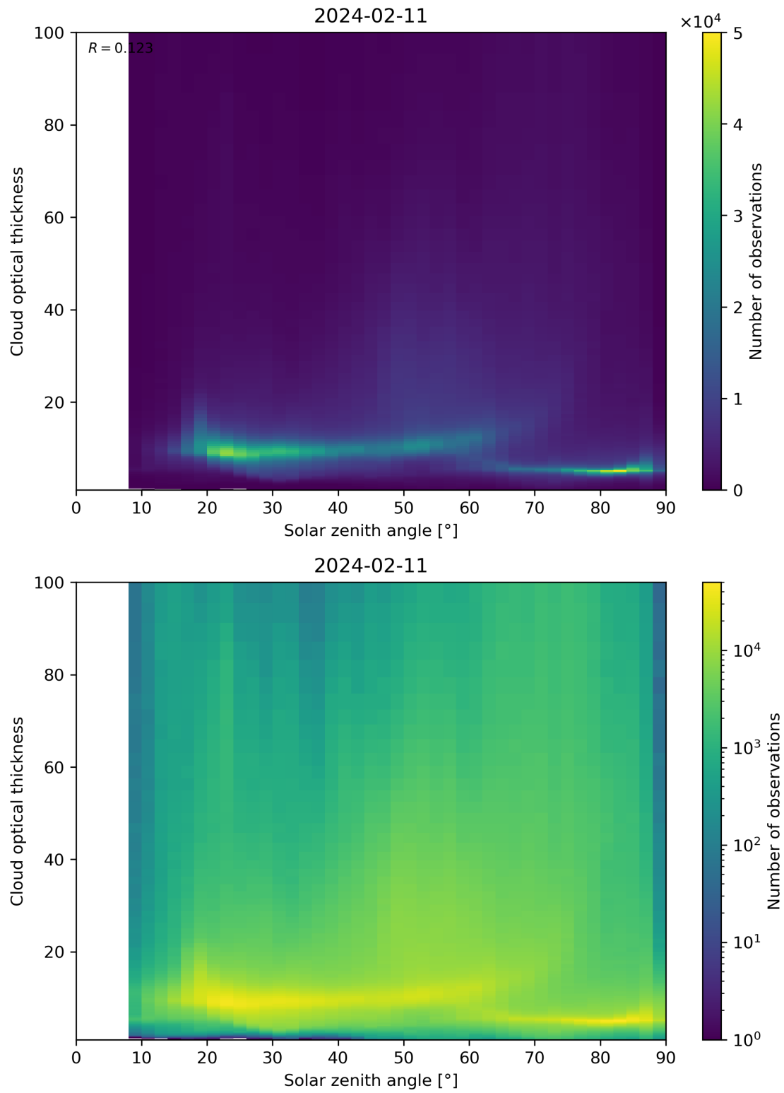
Figure 103: Scatter density plot of “Solar zenith angle” against “Cloud optical thickness” for 2024-02-11 to 2024-02-12.
