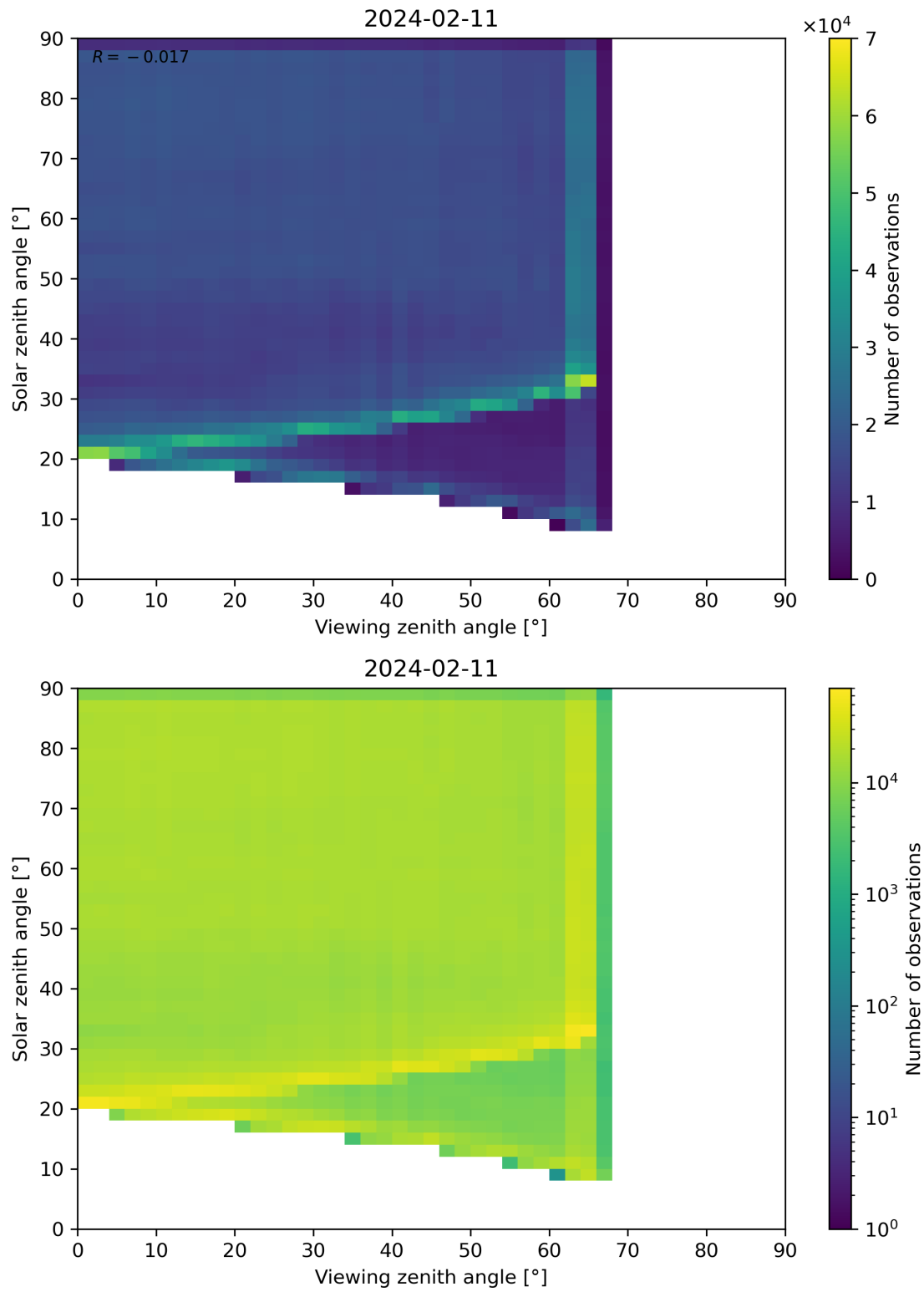
Figure 114: Scatter density plot of “Viewing zenith angle” against “Solar zenith angle” for 2024-02-11 to 2024-02-12.
