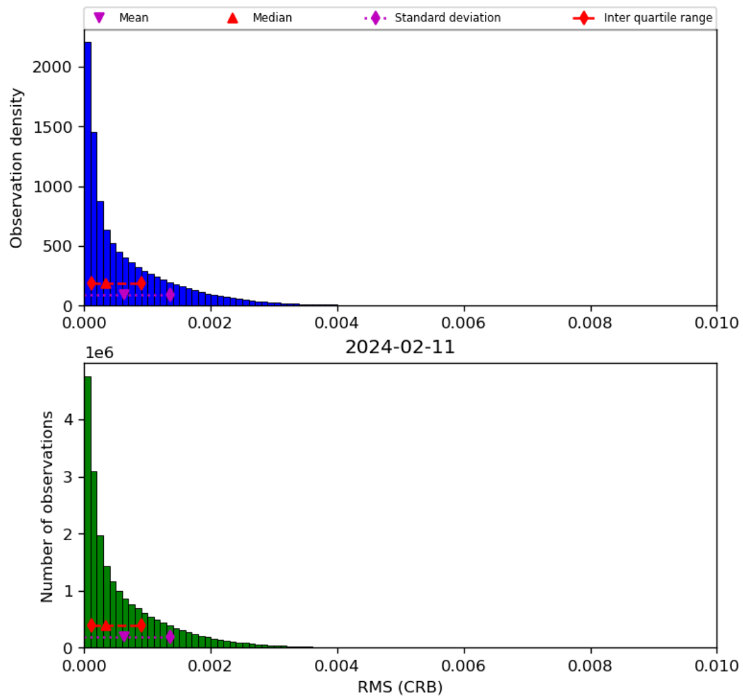
Figure 48: Histogram of “RMS (CRB)” for 2024-02-11 to 2024-02-12
