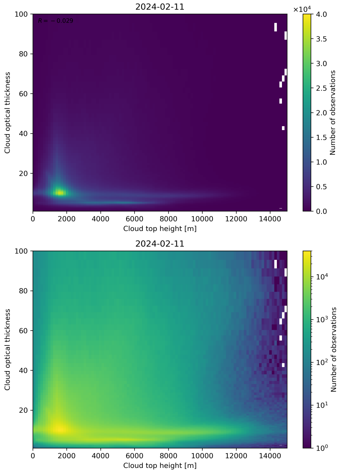
Figure 90: Scatter density plot of “Cloud top height” against “Cloud optical thickness” for 2024-02-11 to 2024-02-12.
