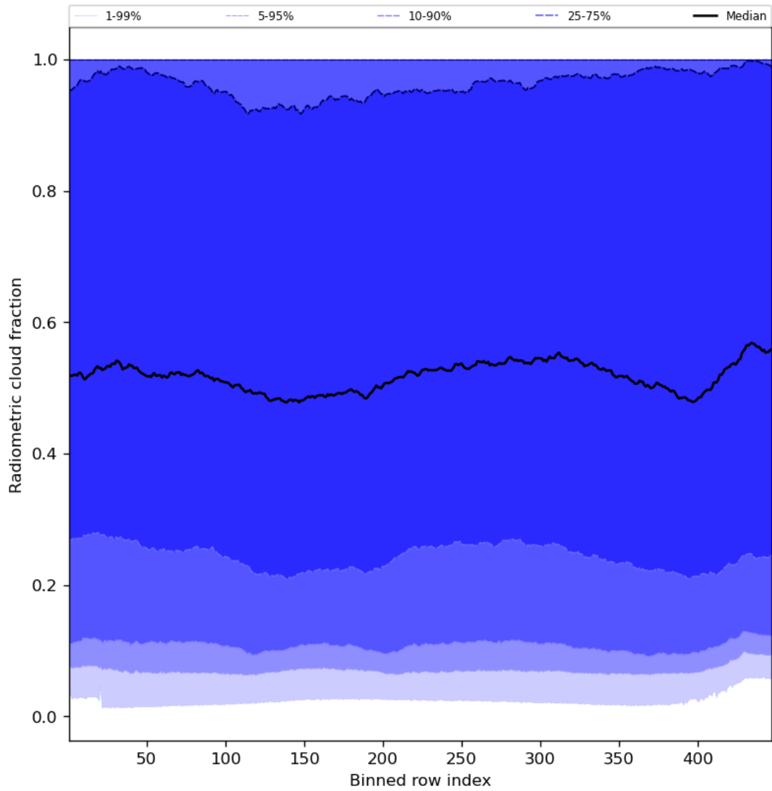
Figure 55: Along track statistics of “Radiometric cloud fraction” for 2024-02-11 to 2024-02-12
