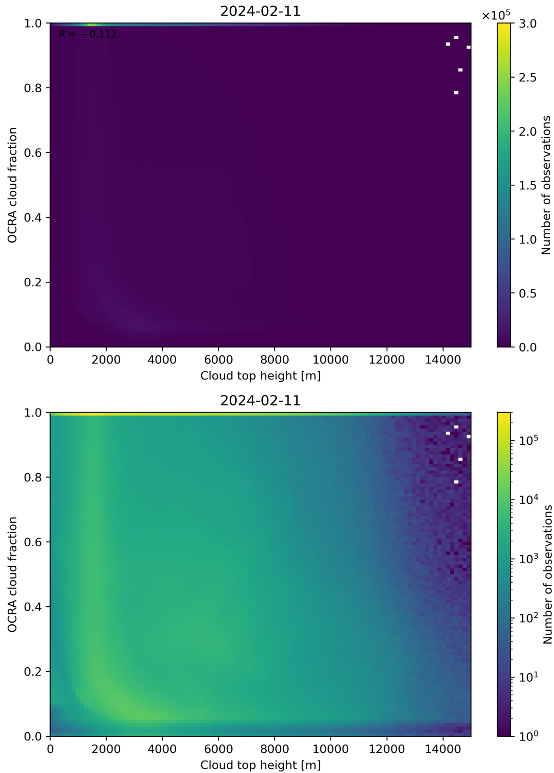
Figure 87: Scatter density plot of “Cloud top height” against “OCRA cloud fraction” for 2024-02-11 to 2024-02-12.
