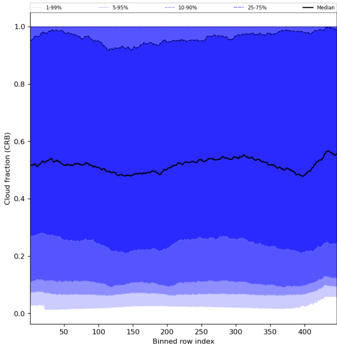
Figure 58: Along track statistics of “Cloud fraction (CRB)” for 2024-02-11 to 2024-02-12
