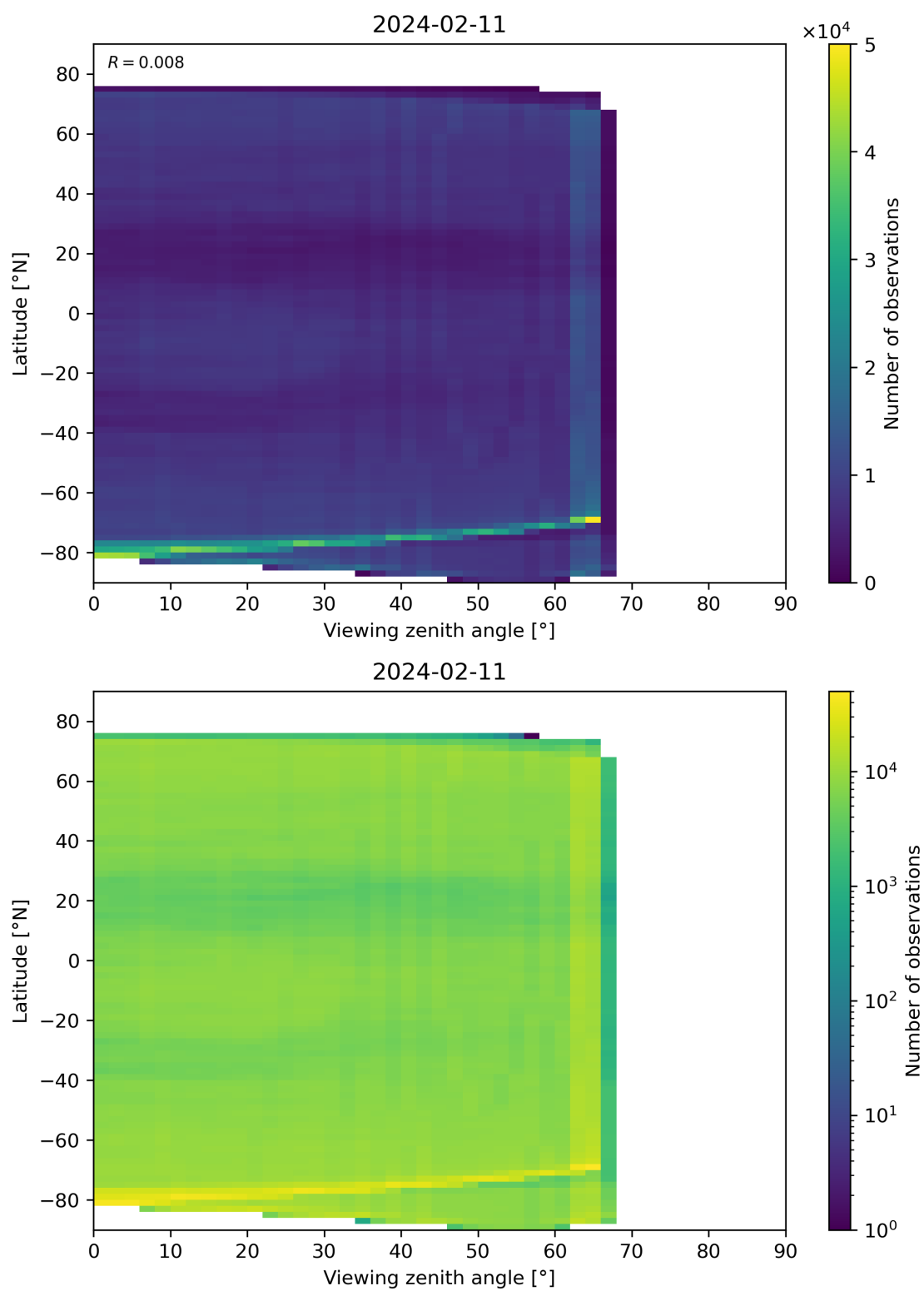
Figure 113: Scatter density plot of “Viewing zenith angle” against “Latitude” for 2024-02-11 to 2024-02-12.
