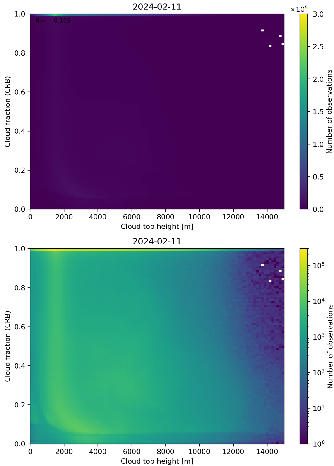
Figure 88: Scatter density plot of “Cloud top height” against “Cloud fraction (CRB)” for 2024-02-11 to 2024-02-12.
