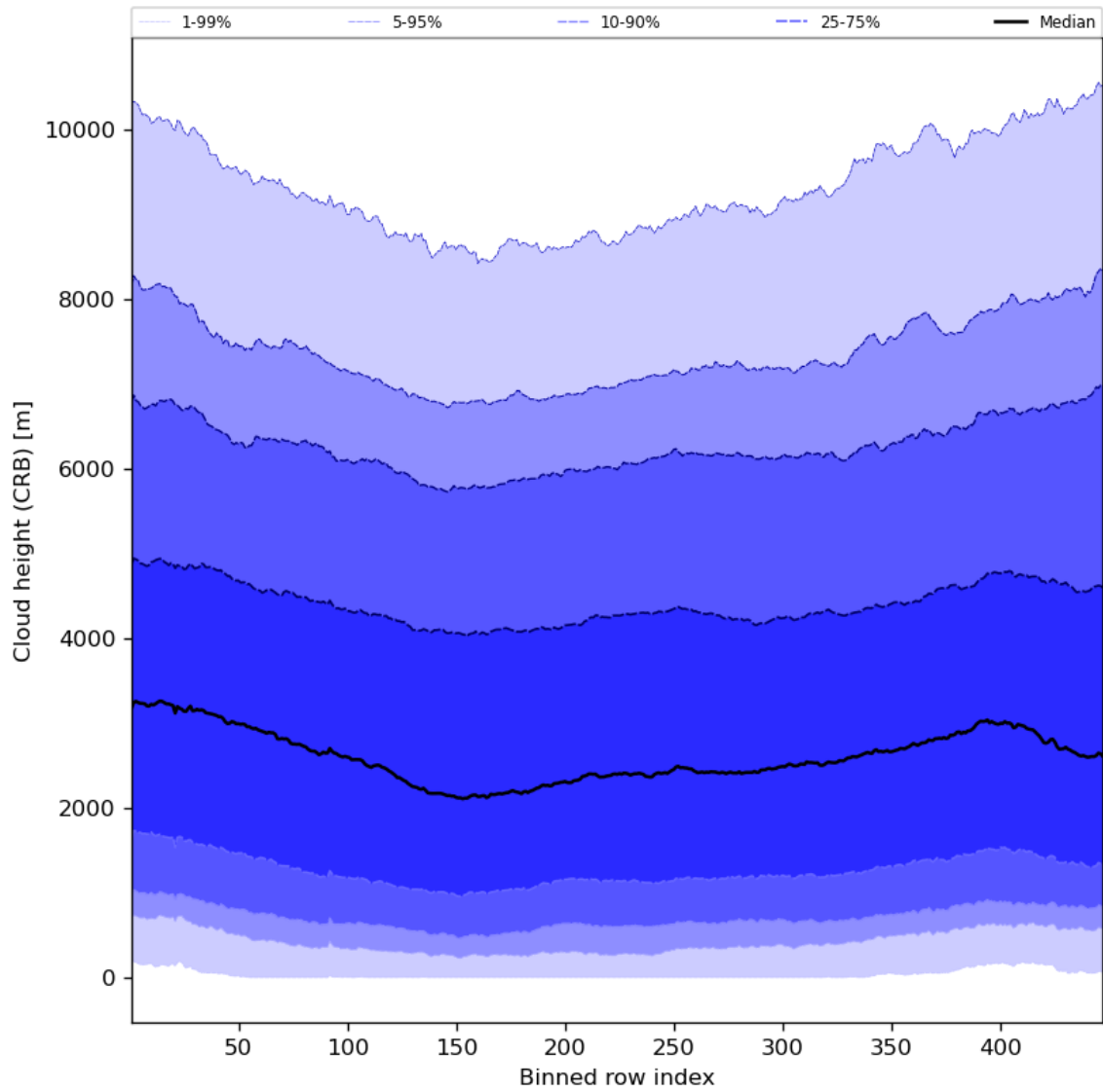
Figure 59: Along track statistics of “Cloud height (CRB)” for 2024-02-11 to 2024-02-12
