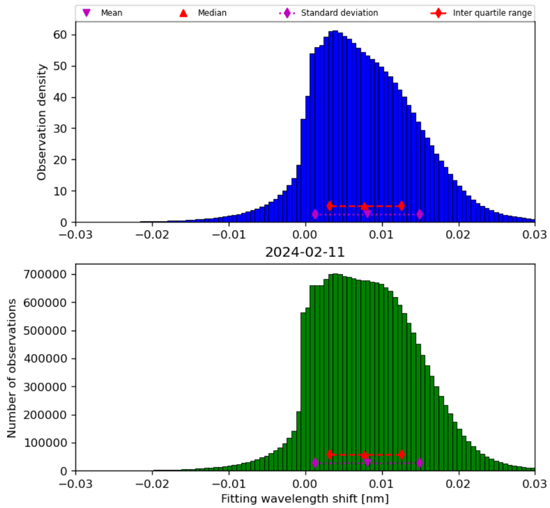
Figure 49: Histogram of “Fitting wavelength shift” for 2024-02-11 to 2024-02-12
