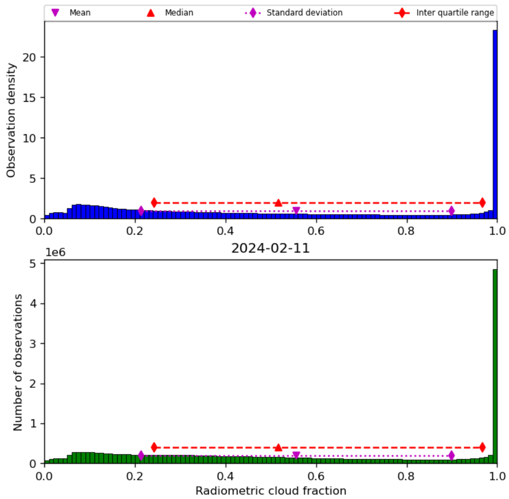
Figure 39: Histogram of “Radiometric cloud fraction” for 2024-02-11 to 2024-02-12
