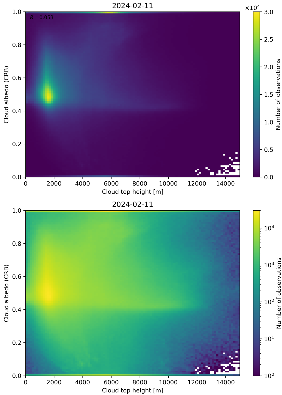
Figure 86: Scatter density plot of “Cloud top height” against “Cloud albedo (CRB)” for 2024-02-11 to 2024-02-12.
