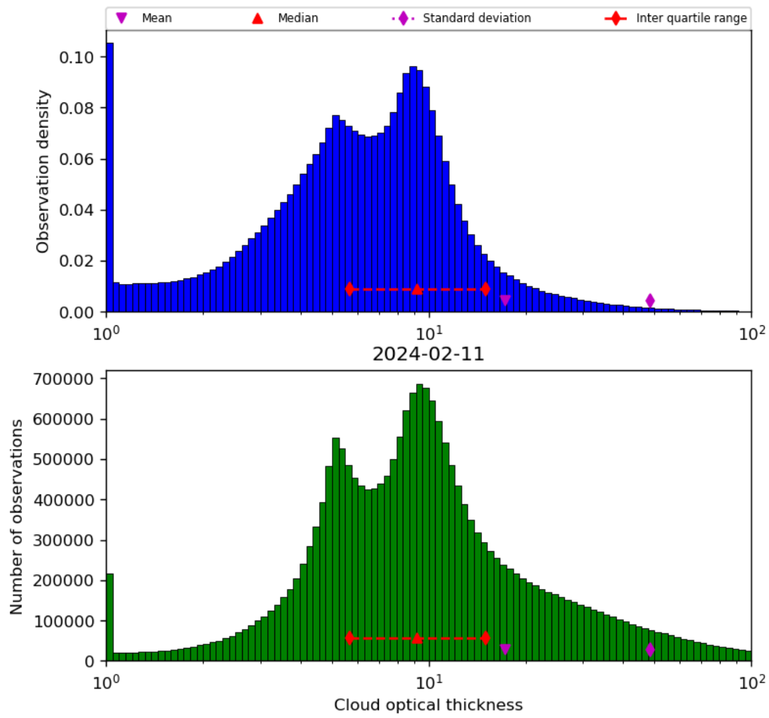
Figure 41: Histogram of “Cloud optical thickness” for 2024-02-11 to 2024-02-12
