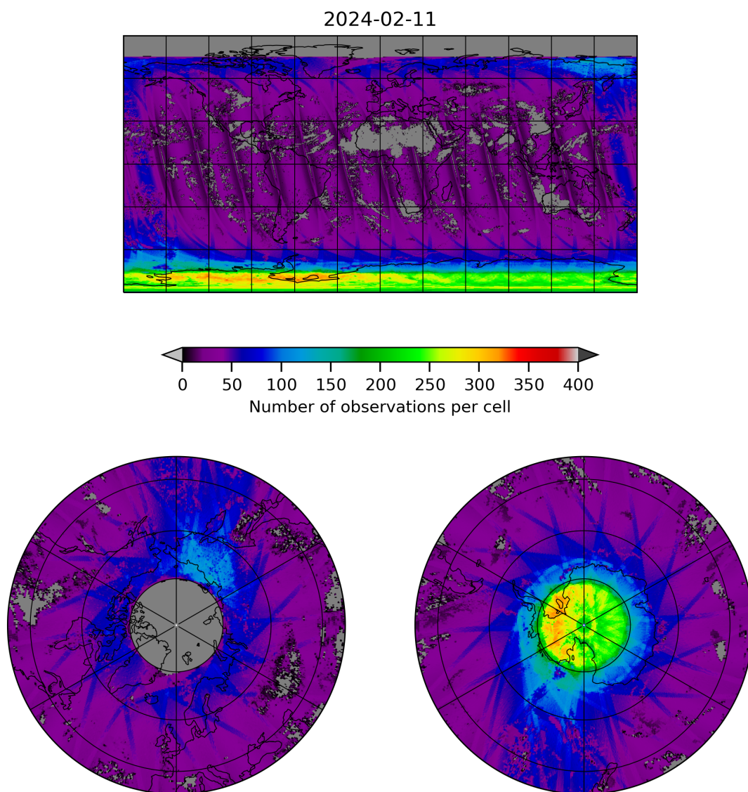
Figure 21: Map of the number of observations for 2024-02-11 to 2024-02-12
