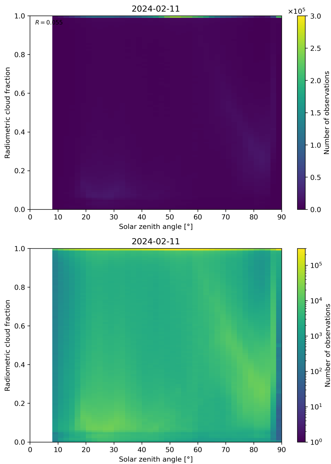
Figure 99: Scatter density plot of “Solar zenith angle” against “Radiometric cloud fraction” for 2024-02-11 to 2024-02-12.
