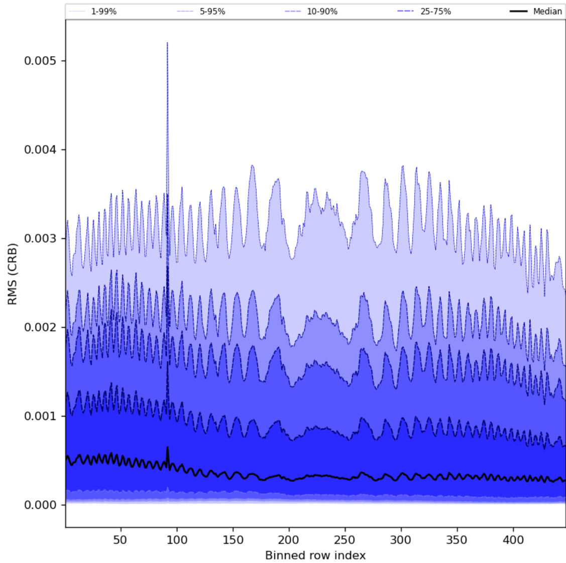
Figure 64: Along track statistics of “RMS (CRB)” for 2024-02-11 to 2024-02-12
