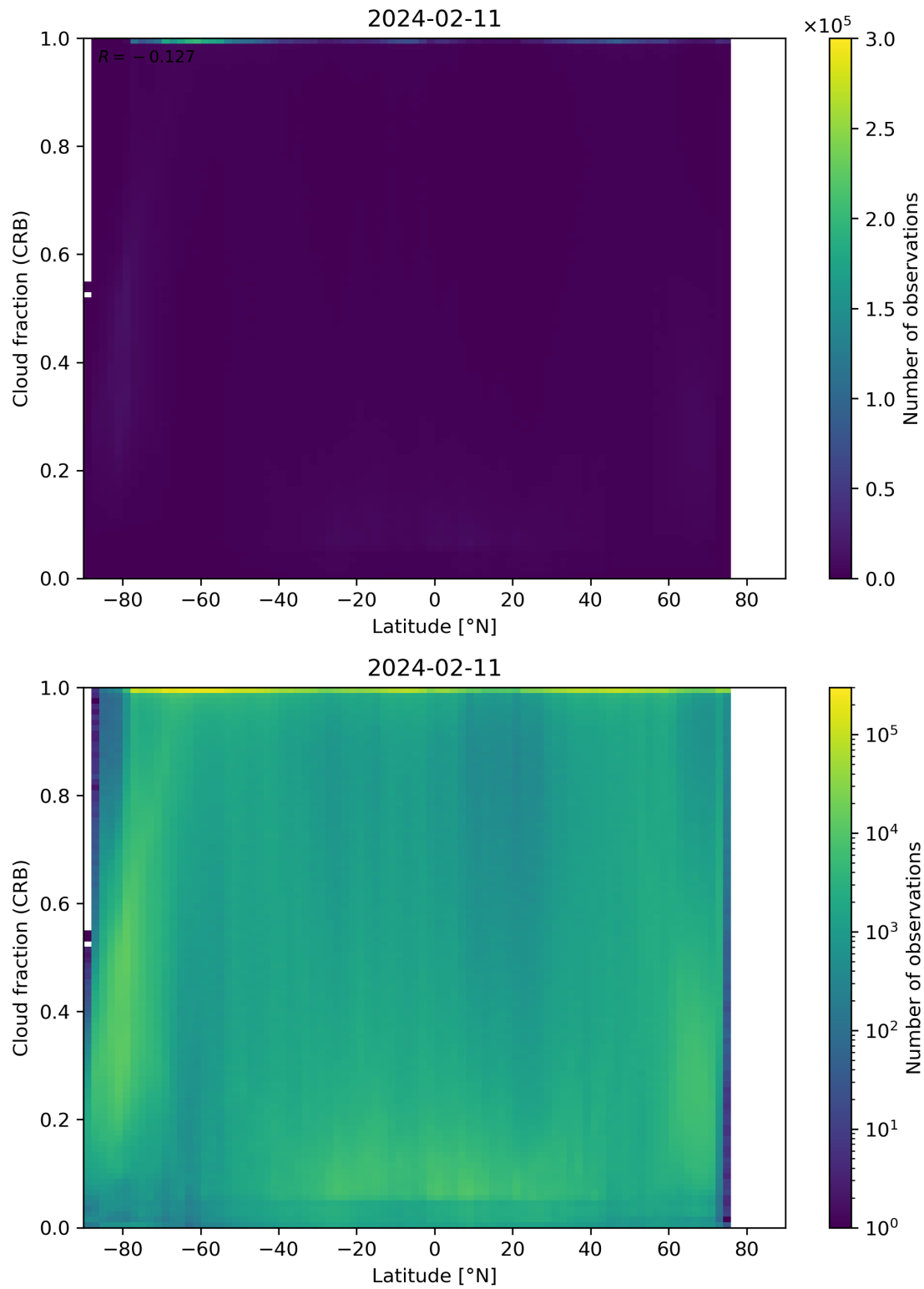
Figure 94: Scatter density plot of “Latitude” against “Cloud fraction (CRB)” for 2024-02-11 to 2024-02-12.
