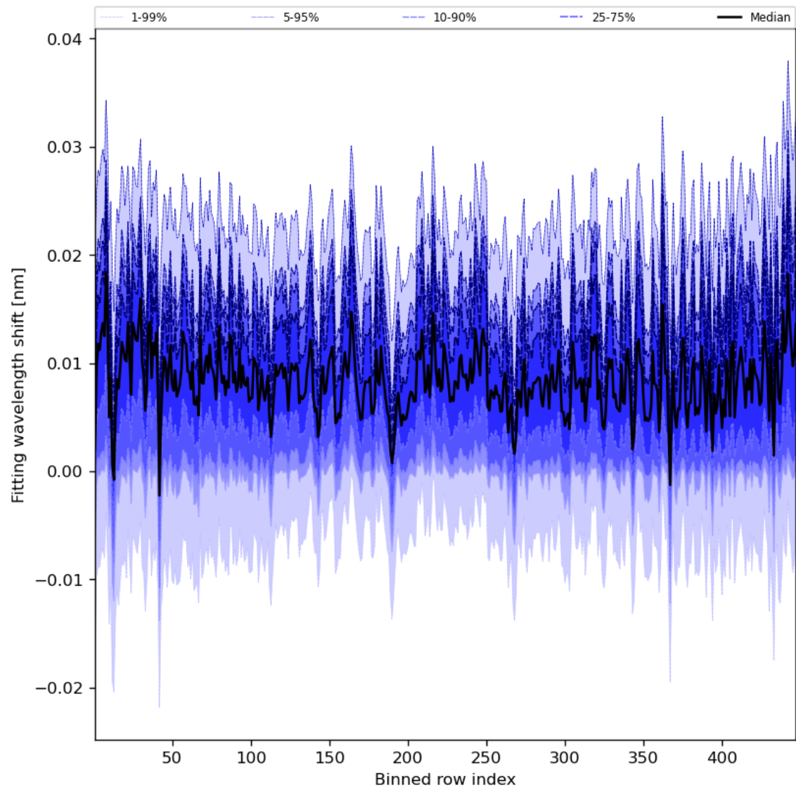
Figure 65: Along track statistics of “Fitting wavelength shift” for 2024-02-11 to 2024-02-12
