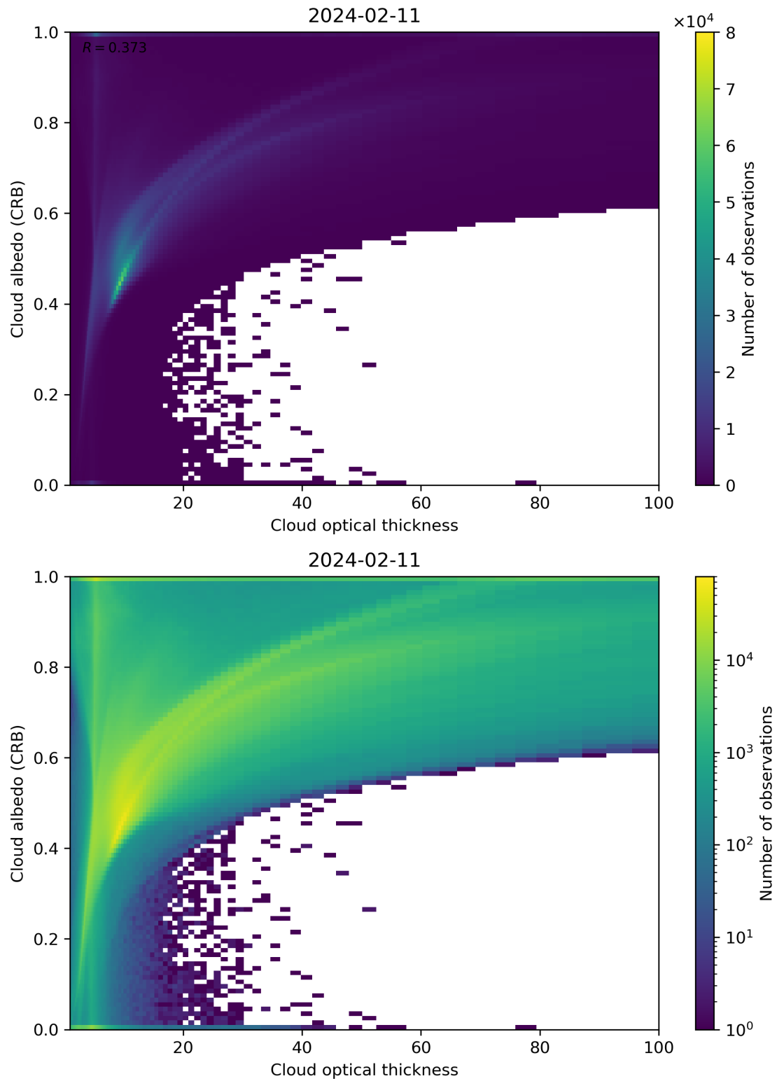
Figure 82: Scatter density plot of “Cloud optical thickness” against “Cloud albedo (CRB)” for 2024-02-11 to 2024-02-12.
