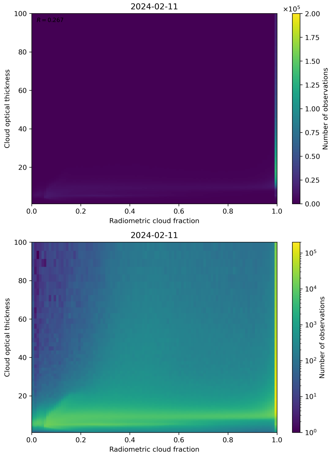
Figure 75: Scatter density plot of “Radiometric cloud fraction” against “Cloud optical thickness” for 2024-02-11 to 2024-02-12.
