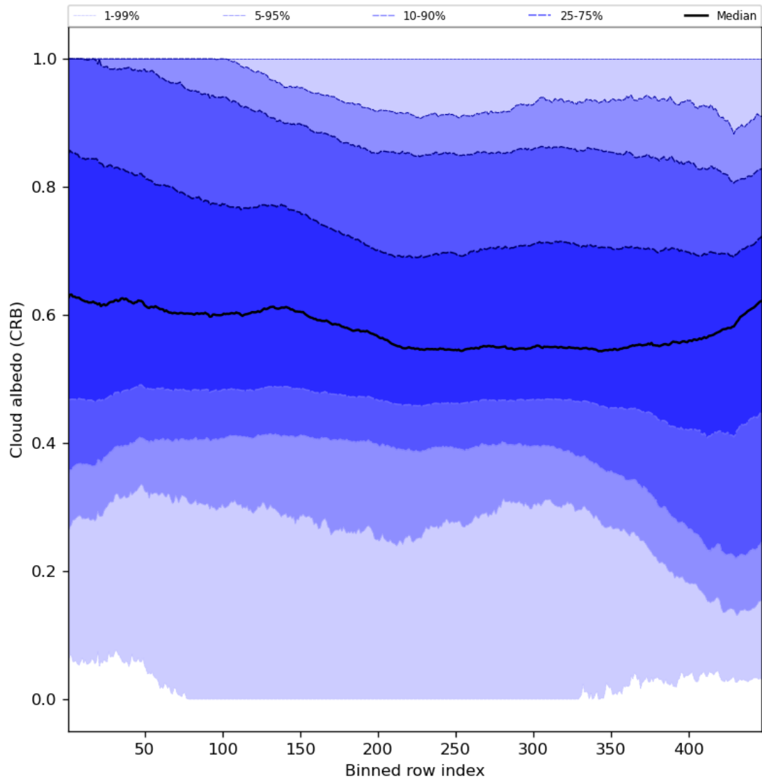
Figure 60: Along track statistics of “Cloud albedo (CRB)” for 2024-02-11 to 2024-02-12
