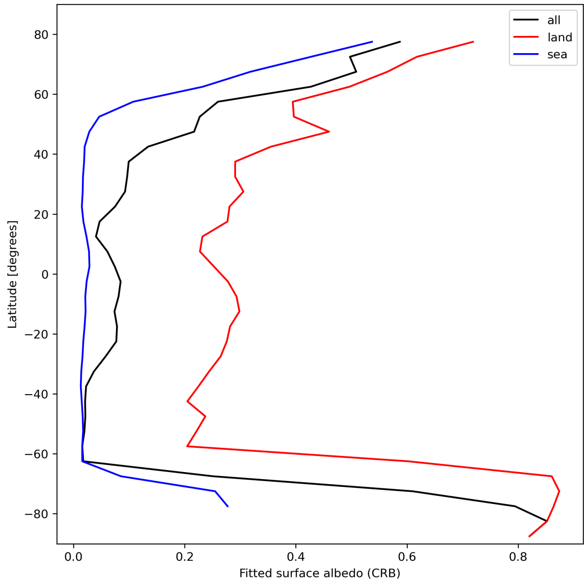
Figure 30: Zonal average of “Fitted surface albedo (CRB)” for 2024-02-11 to 2024-02-12.
