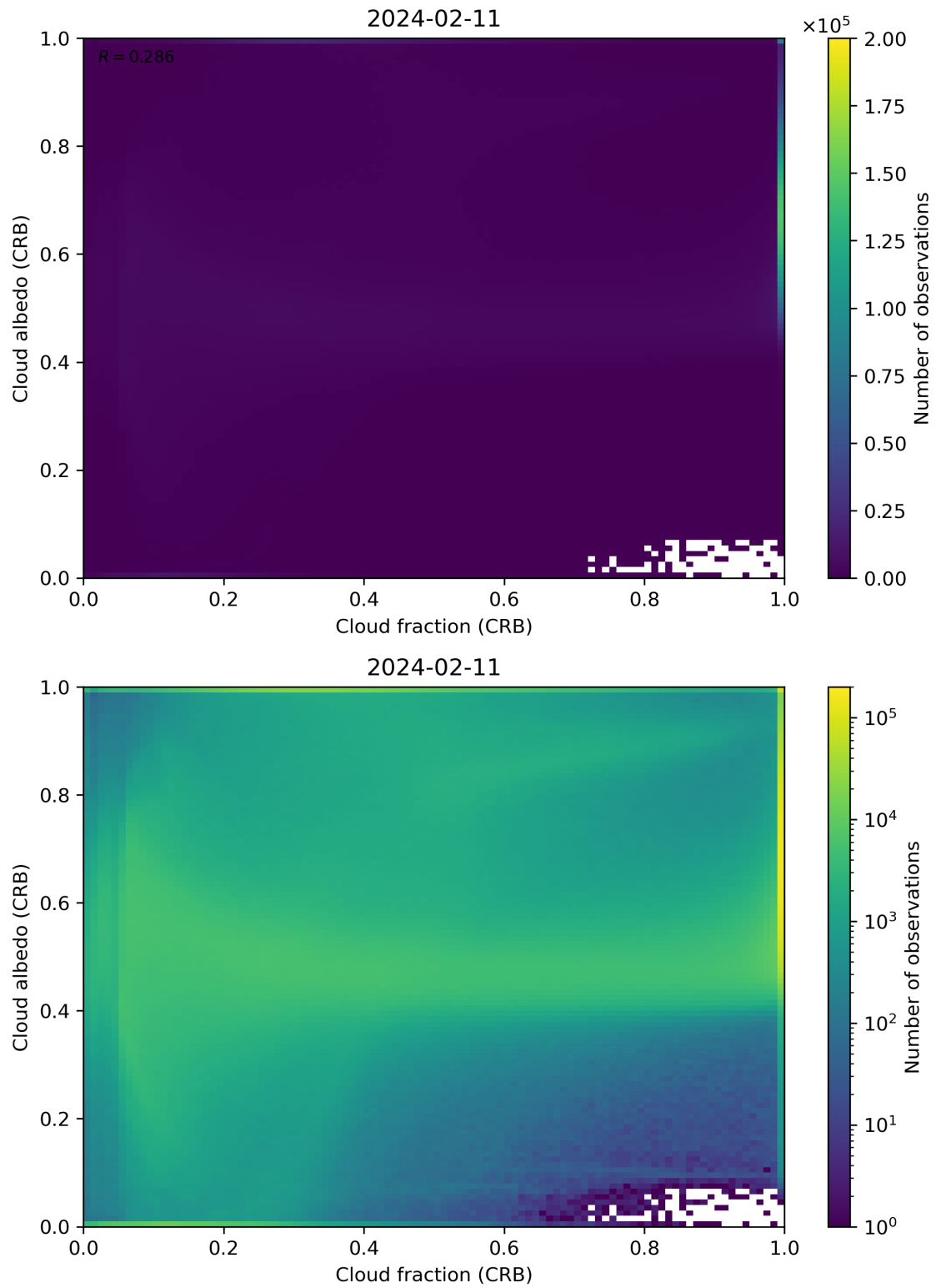
Figure 77: Scatter density plot of “Cloud fraction (CRB)” against “Cloud albedo (CRB)” for 2024-02-11 to 2024-02-12.
