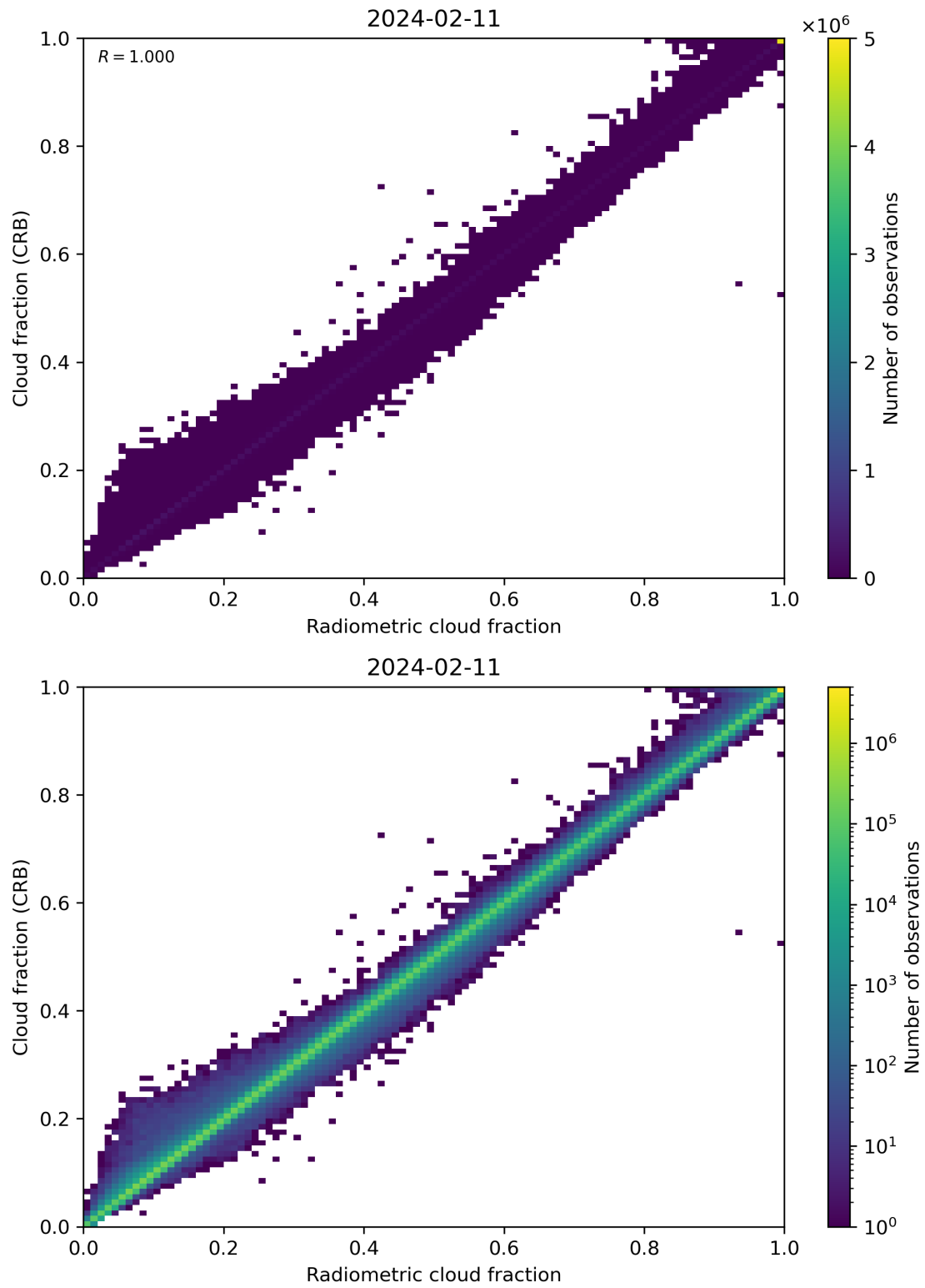
Figure 73: Scatter density plot of “Radiometric cloud fraction” against “Cloud fraction (CRB)” for 2024-02-11 to 2024-02-12.
