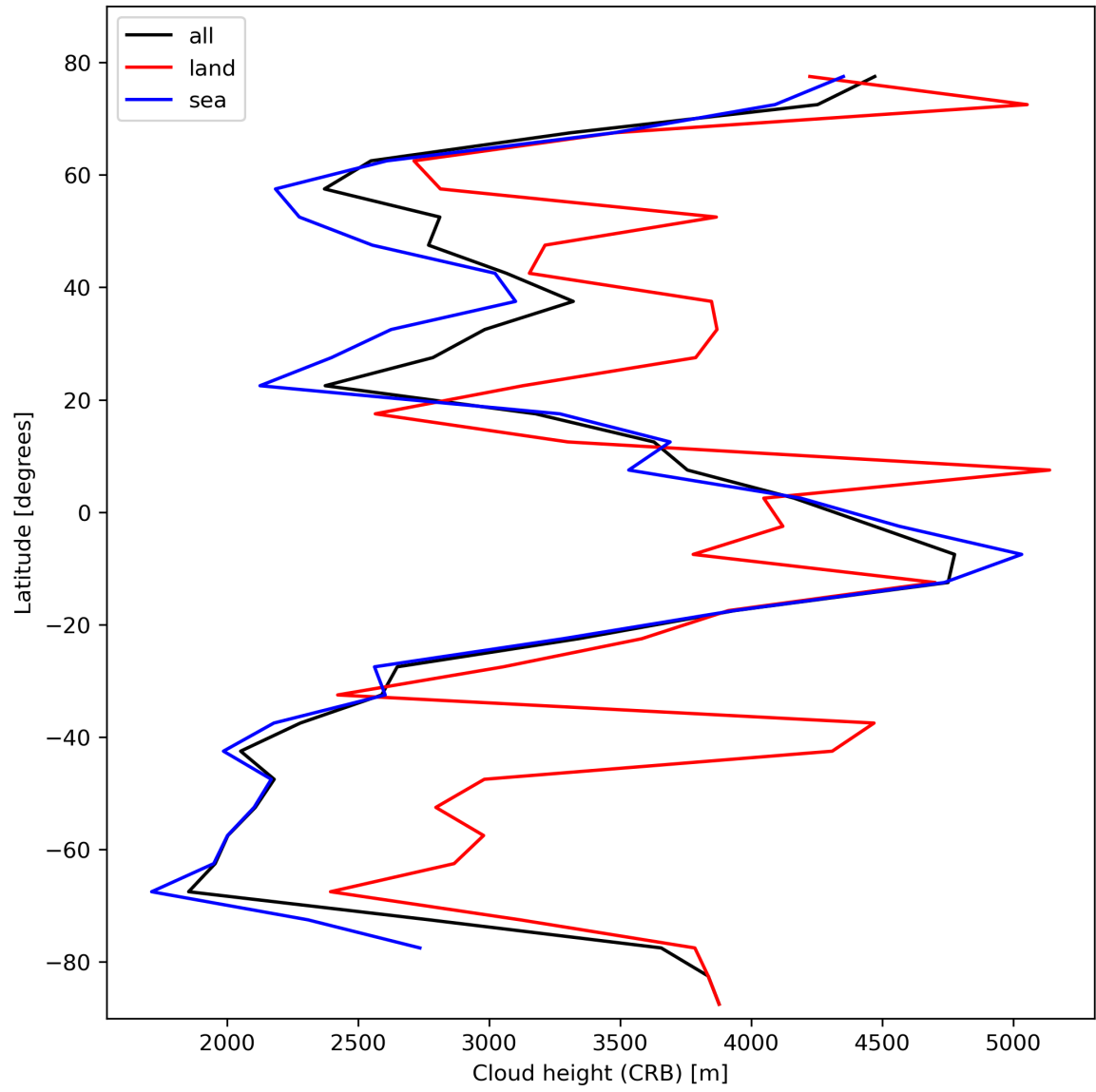
Figure 27: Zonal average of “Cloud height (CRB)” for 2024-02-11 to 2024-02-12.
