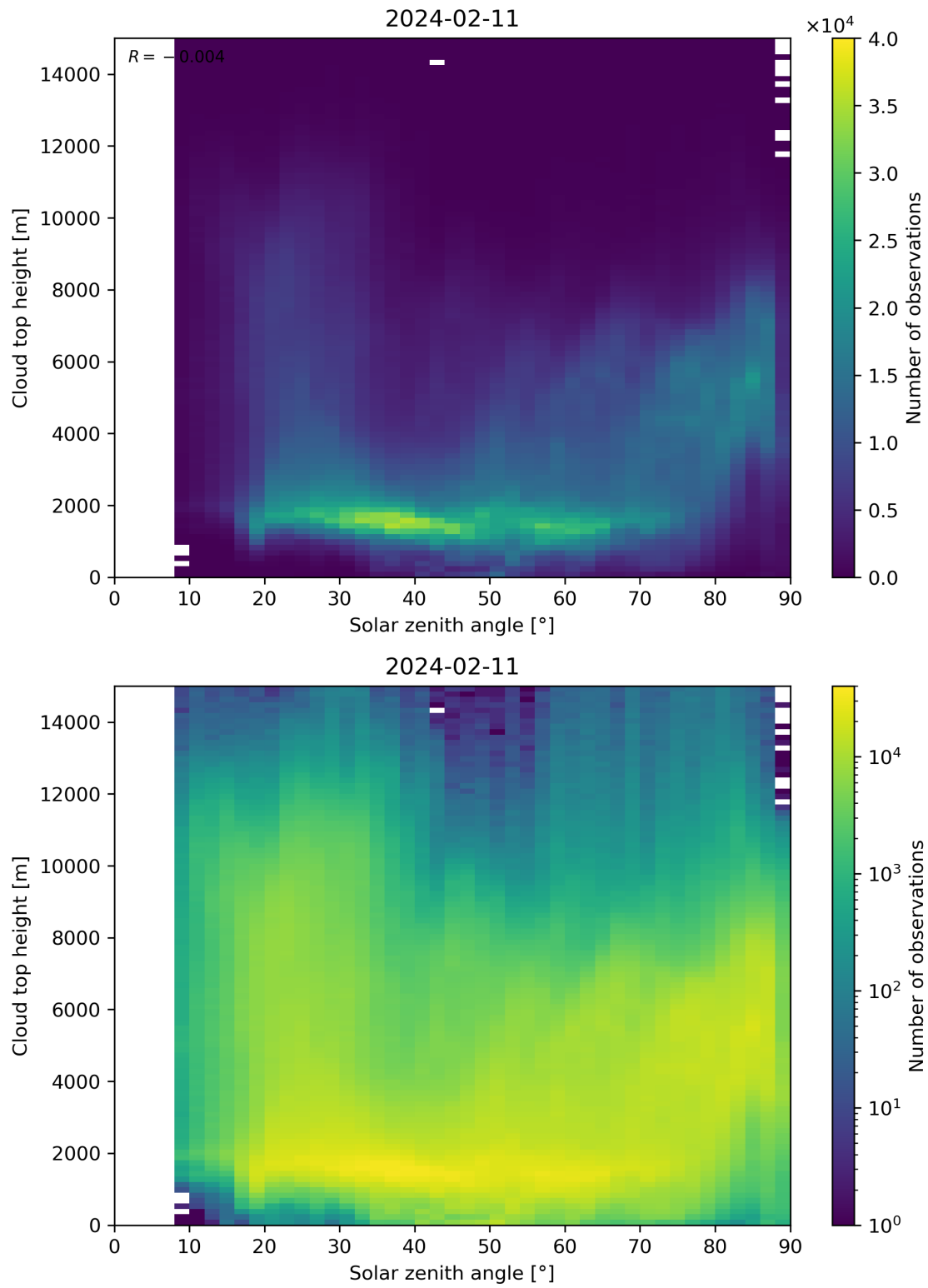
Figure 104: Scatter density plot of “Solar zenith angle” against “Cloud top height” for 2024-02-11 to 2024-02-12.
