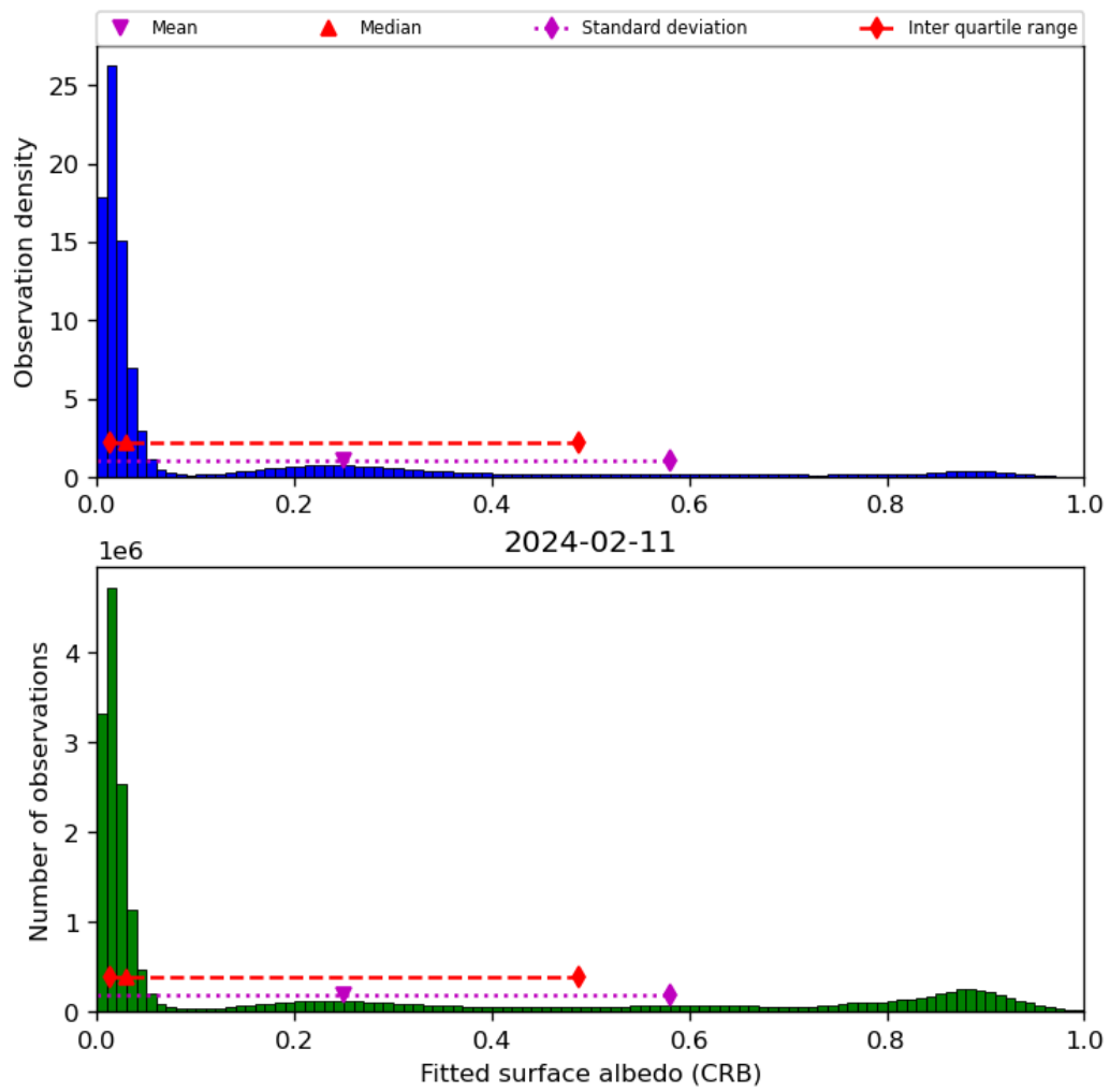
Figure 46: Histogram of “Fitted surface albedo (CRB)” for 2024-02-11 to 2024-02-12
