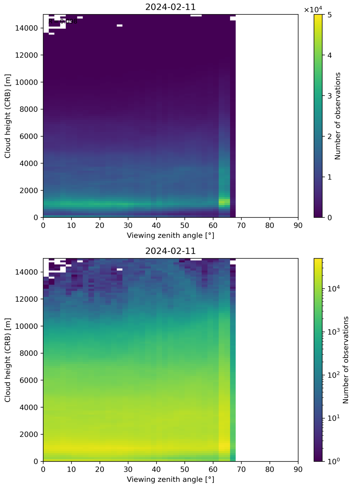
Figure 110: Scatter density plot of “Viewing zenith angle” against “Cloud height (CRB)” for 2024-02-11 to 2024-02-12.
