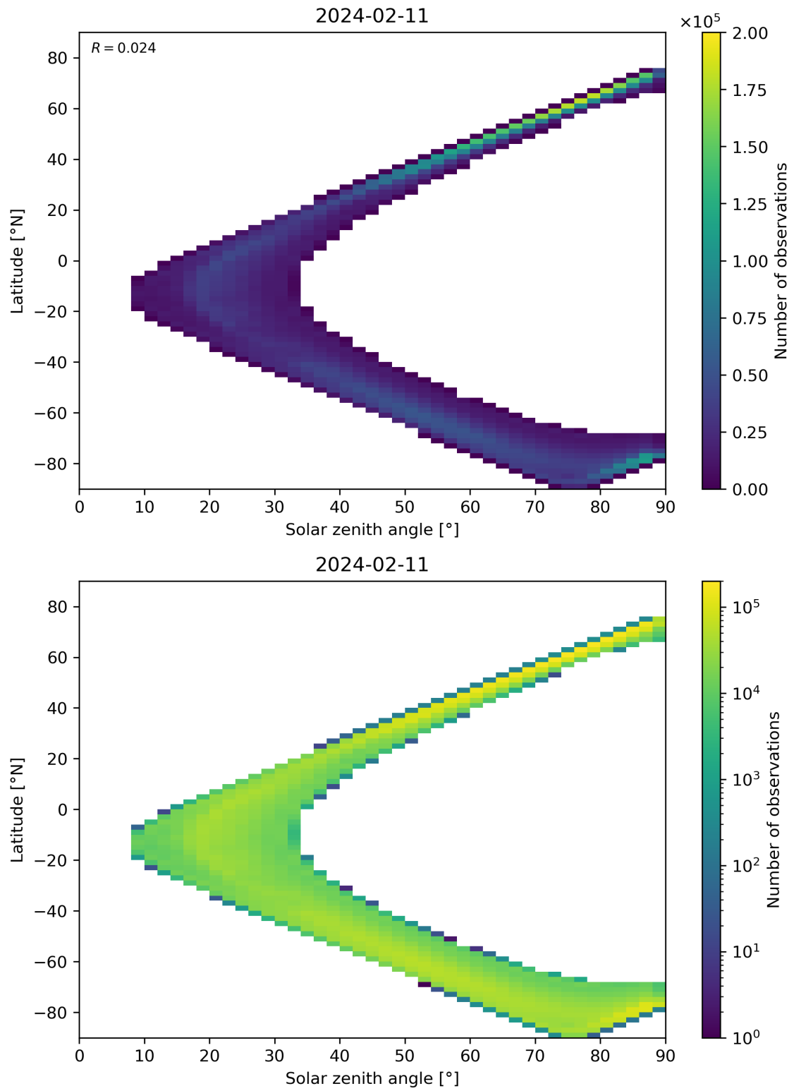
Figure 105: Scatter density plot of “Solar zenith angle” against “Latitude” for 2024-02-11 to 2024-02-12.
