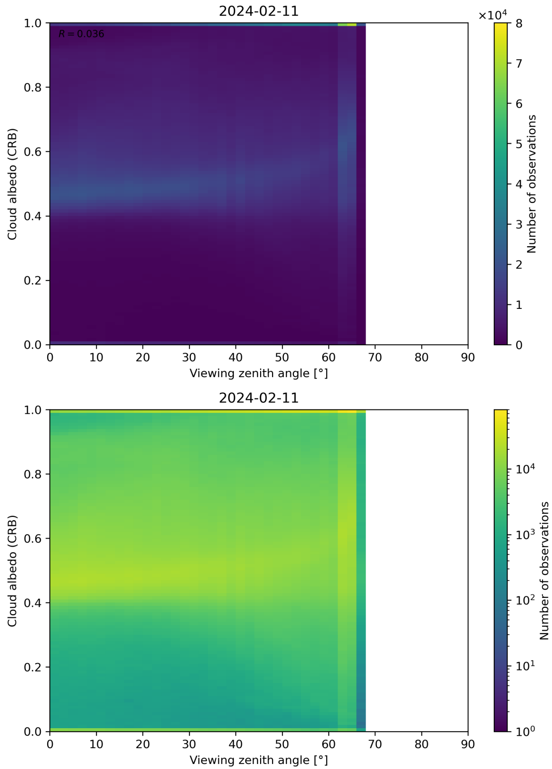
Figure 106: Scatter density plot of “Viewing zenith angle” against “Cloud albedo (CRB)” for 2024-02-11 to 2024-02-12.
