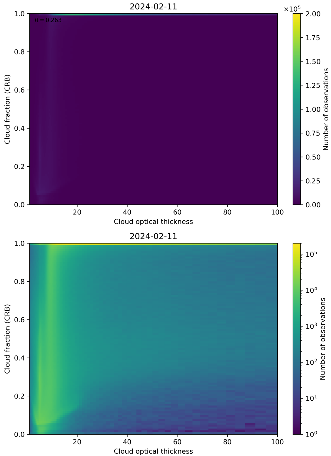
Figure 84: Scatter density plot of “Cloud optical thickness” against “Cloud fraction (CRB)” for 2024-02-11 to 2024-02-12.
