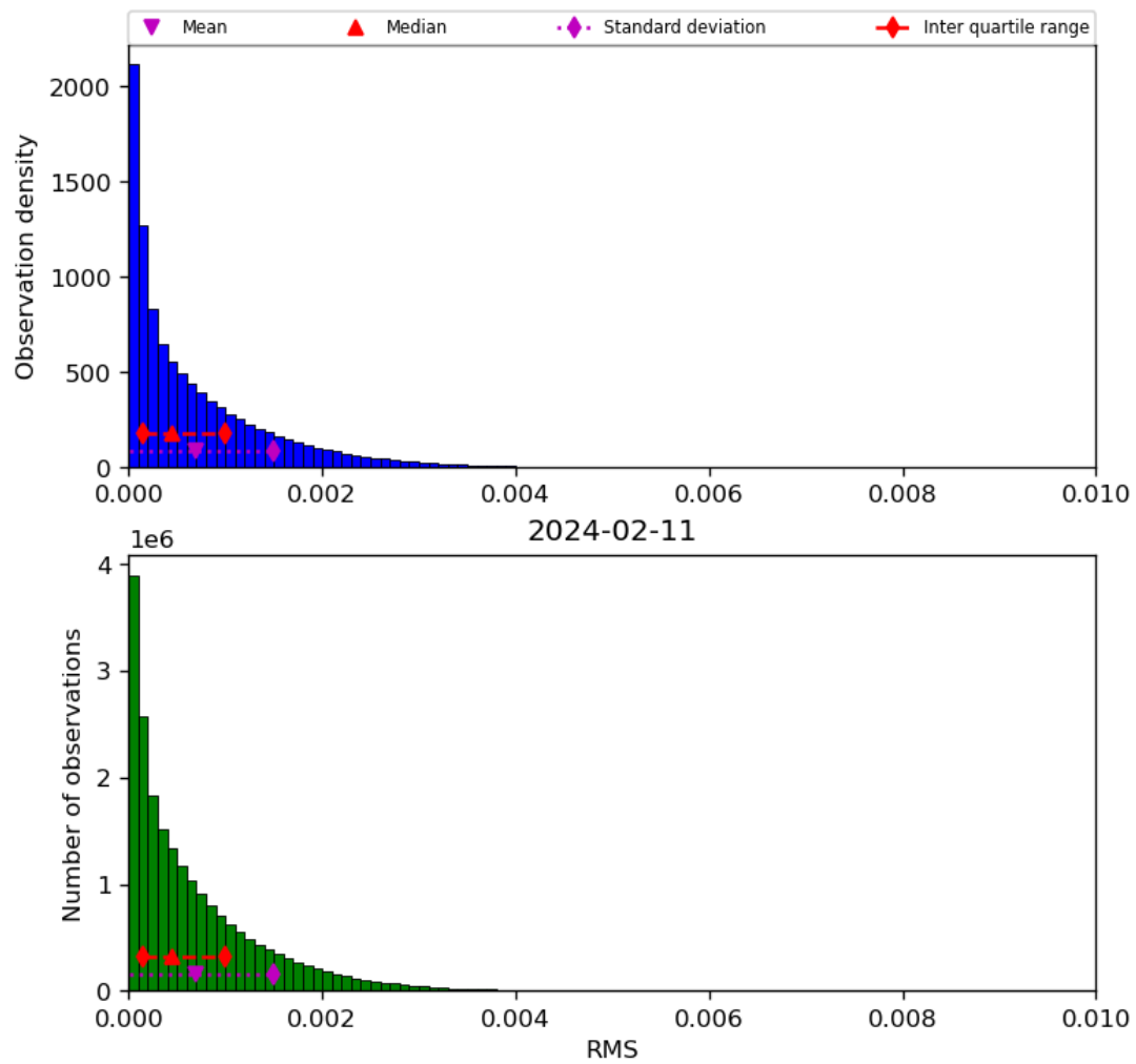
Figure 47: Histogram of “RMS” for 2024-02-11 to 2024-02-12
