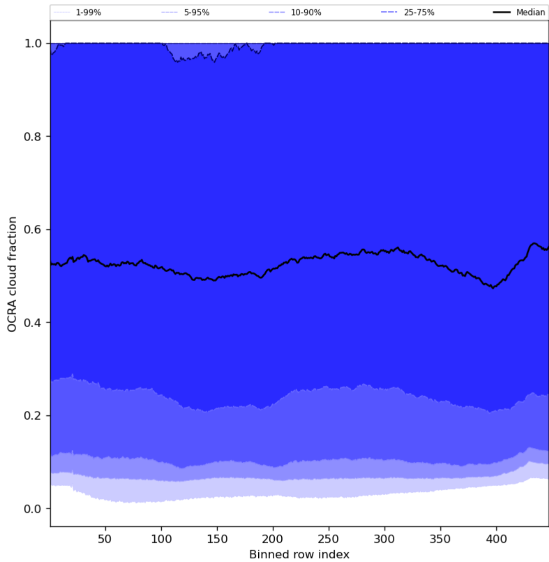
Figure 66: Along track statistics of “OCRA cloud fraction” for 2024-02-11 to 2024-02-12
