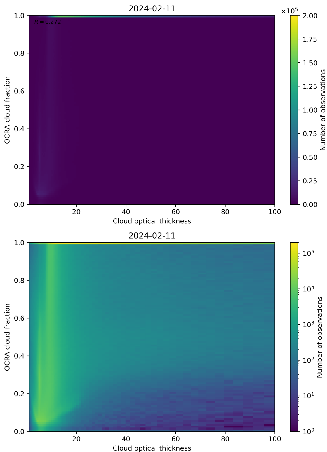
Figure 83: Scatter density plot of “Cloud optical thickness” against “OCRA cloud fraction” for 2024-02-11 to 2024-02-12.
