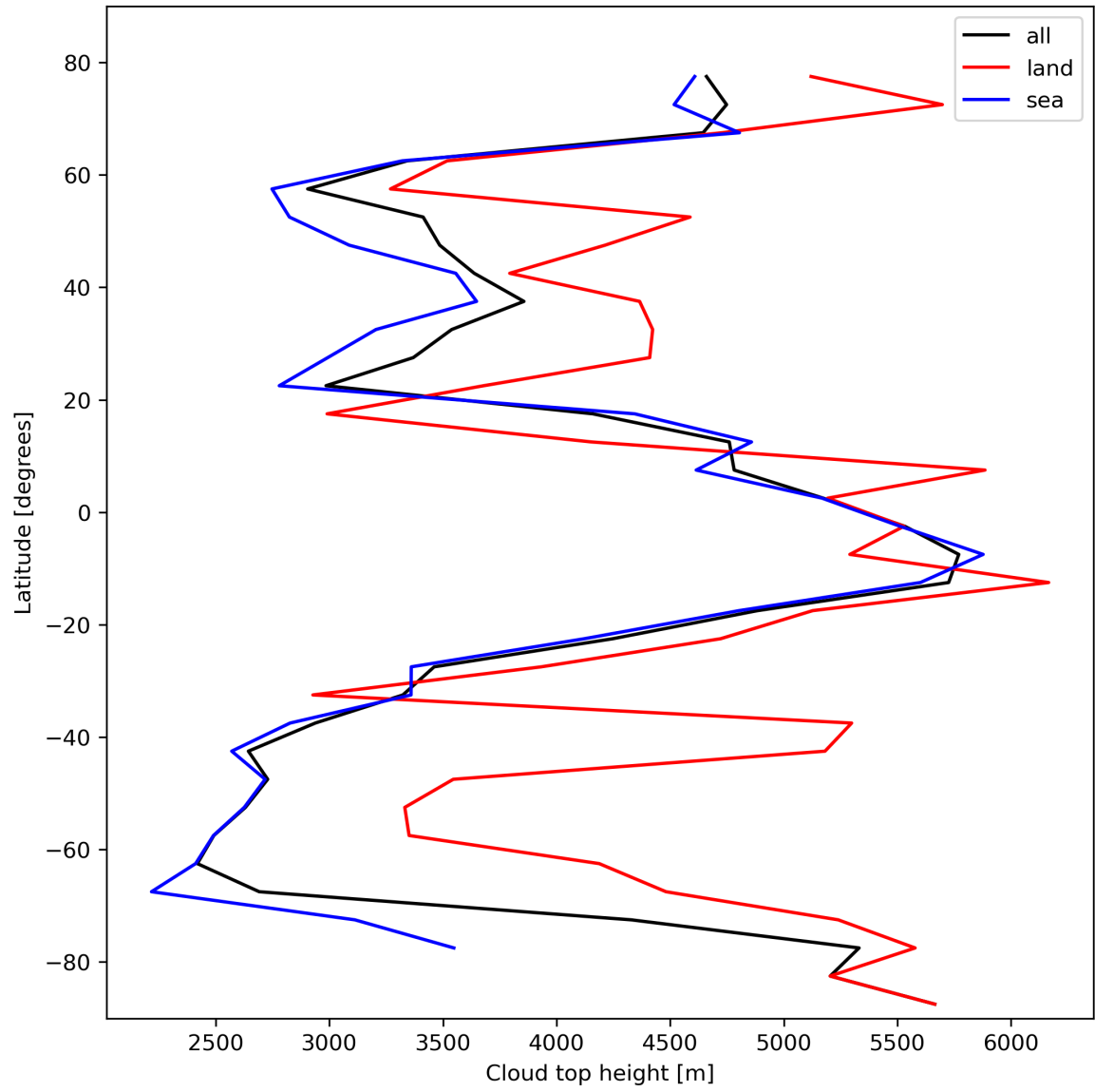
Figure 24: Zonal average of “Cloud top height” for 2024-02-11 to 2024-02-12.
