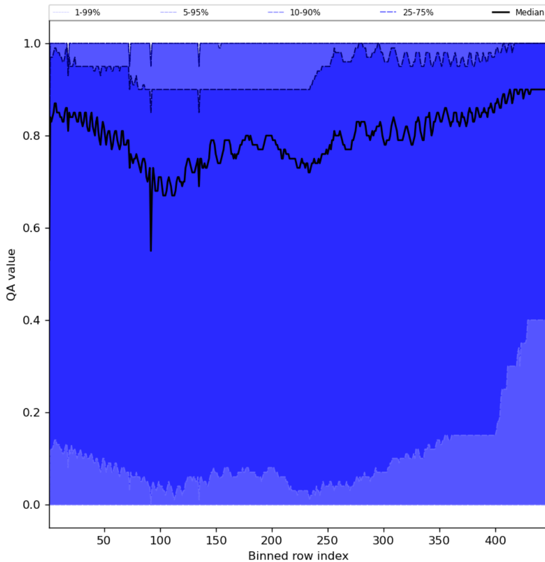
Figure 54: Along track statistics of “QA value” for 2024-02-11 to 2024-02-12
