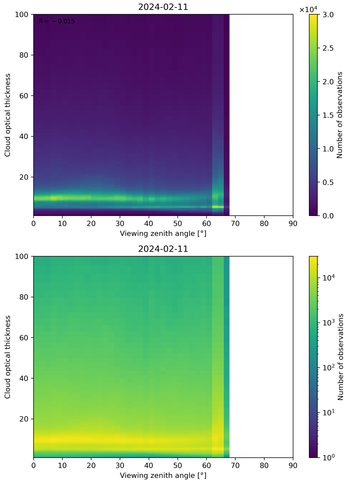
Figure 111: Scatter density plot of “Viewing zenith angle” against “Cloud optical thickness” for 2024-02-11 to 2024-02-12.
