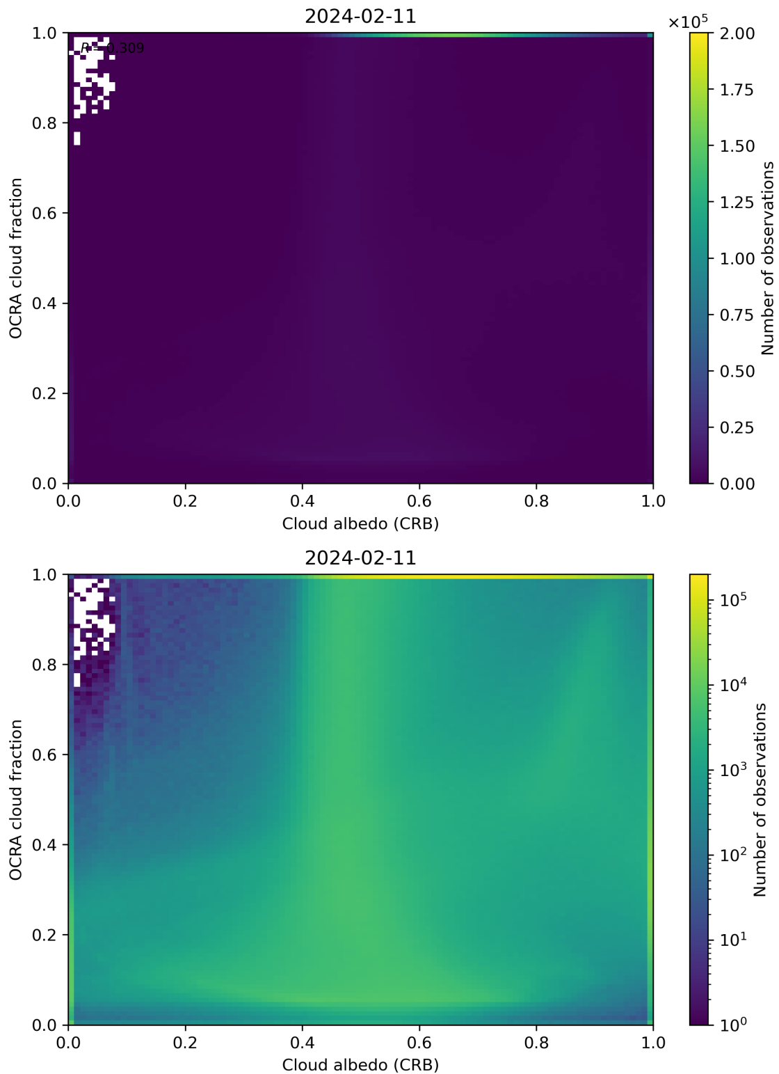
Figure 70: Scatter density plot of “Cloud albedo (CRB)” against “OCRA cloud fraction” for 2024-02-11 to 2024-02-12.
