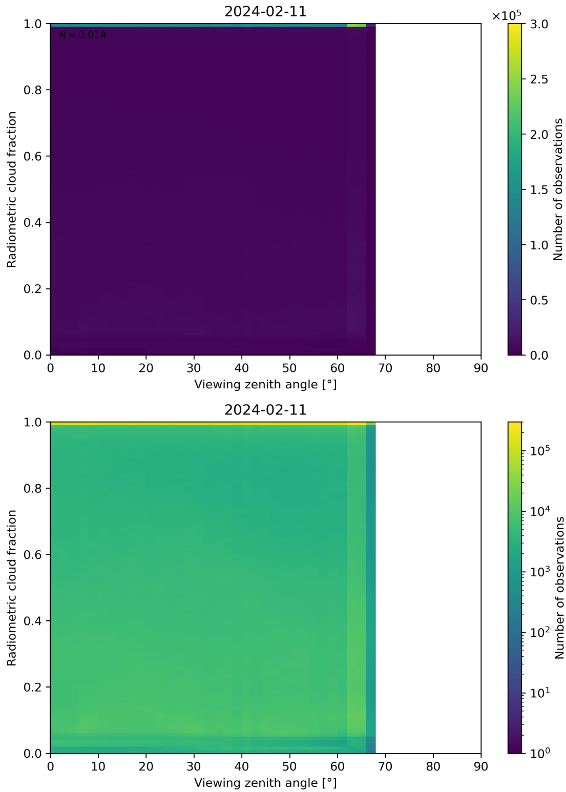
Figure 107: Scatter density plot of “Viewing zenith angle” against “Radiometric cloud fraction” for 2024-02-11 to 2024-02-12.
