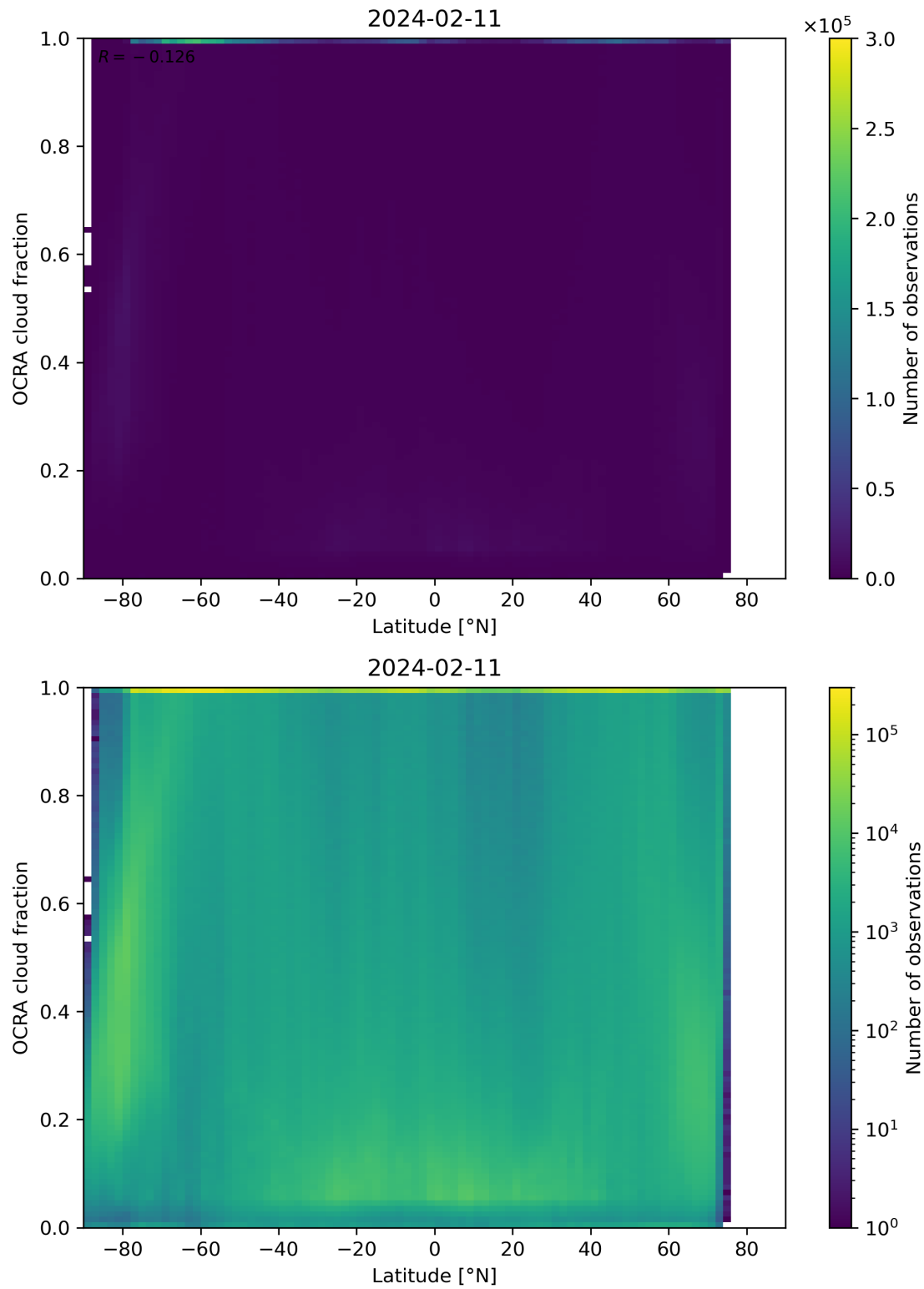
Figure 93: Scatter density plot of “Latitude” against “OCRA cloud fraction” for 2024-02-11 to 2024-02-12.
