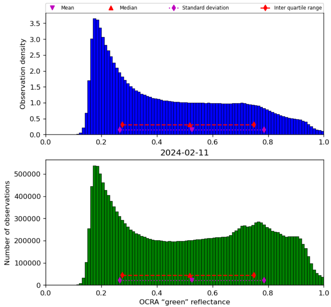
Figure 52: Histogram of “OCRA “green” reflectance” for 2024-02-11 to 2024-02-12
