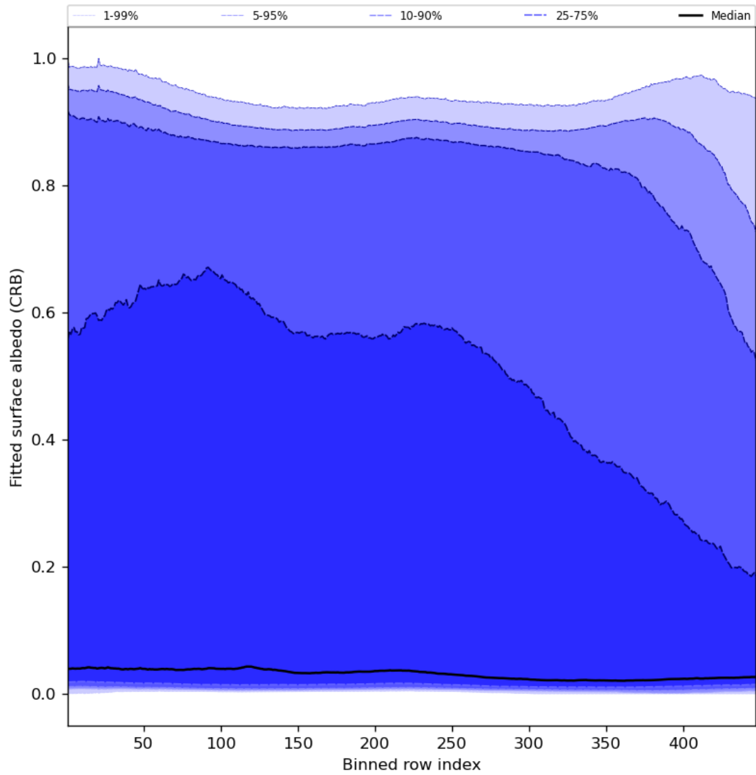
Figure 62: Along track statistics of “Fitted surface albedo (CRB)” for 2024-02-11 to 2024-02-12
