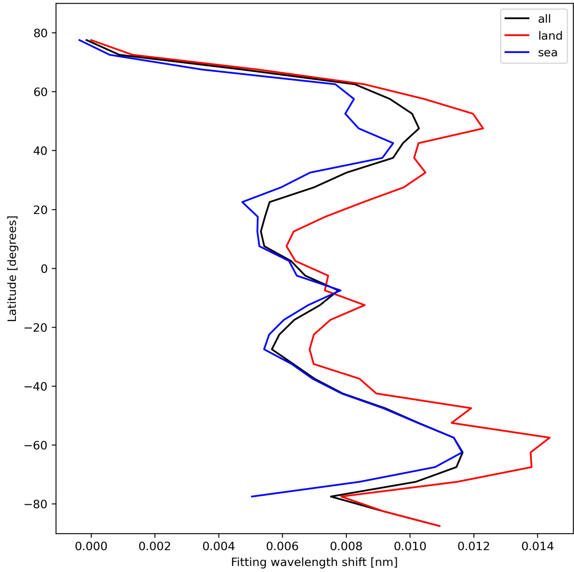
Figure 33: Zonal average of “Fitting wavelength shift” for 2024-02-11 to 2024-02-12.
