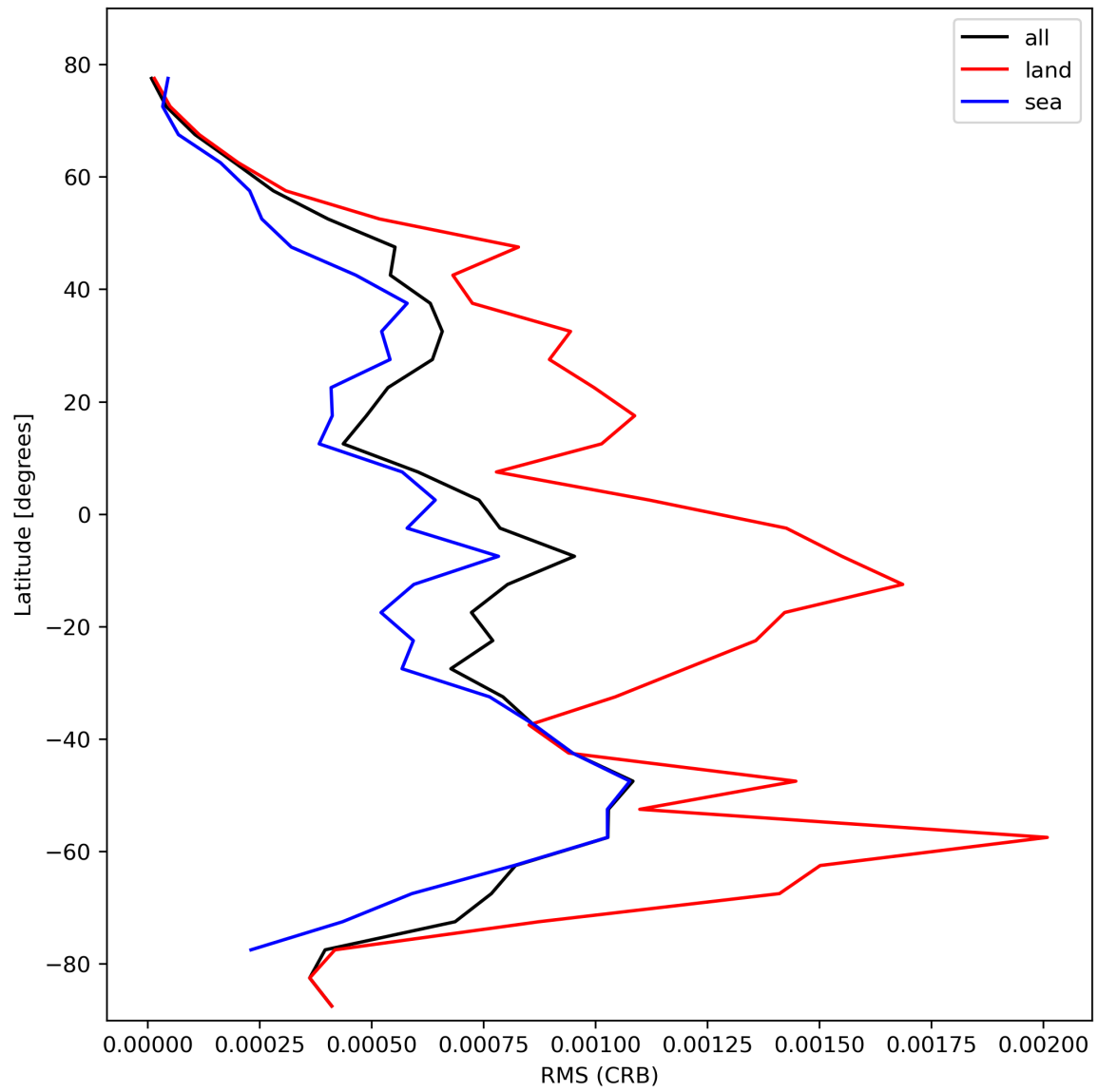
Figure 32: Zonal average of “RMS (CRB)” for 2024-02-11 to 2024-02-12.
