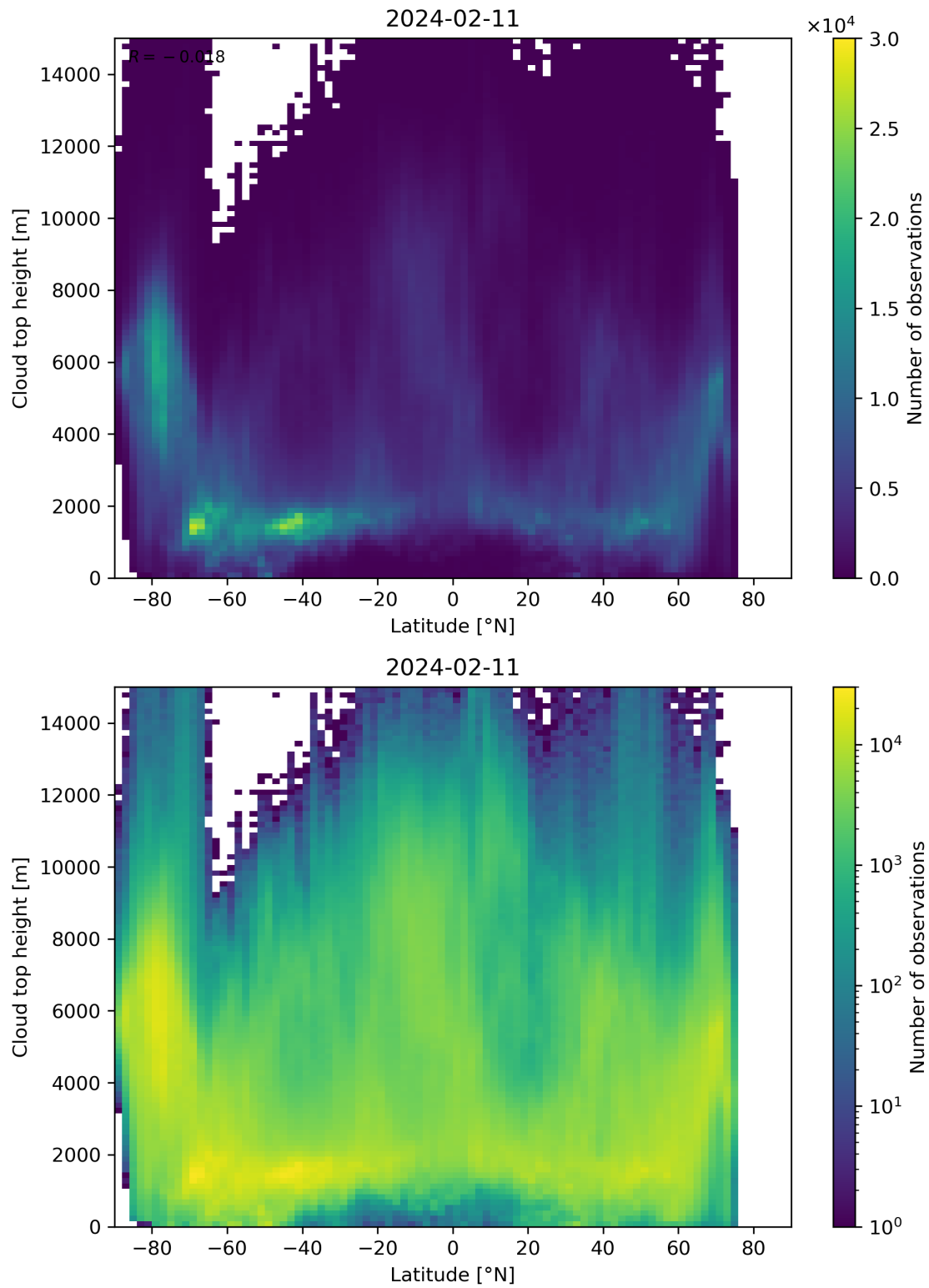
Figure 97: Scatter density plot of “Latitude” against “Cloud top height” for 2024-02-11 to 2024-02-12.
