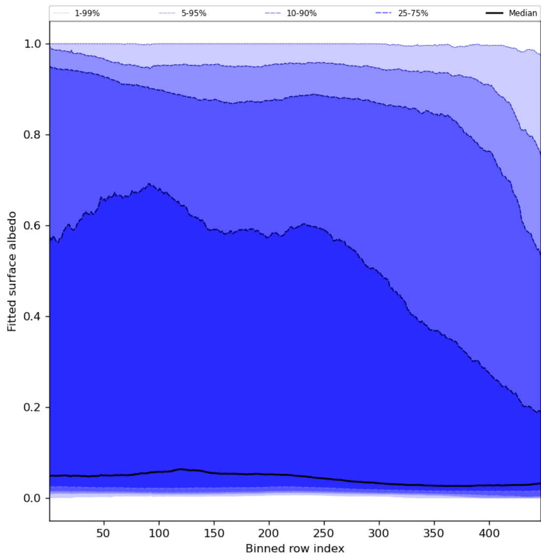
Figure 61: Along track statistics of “Fitted surface albedo” for 2024-02-11 to 2024-02-12
