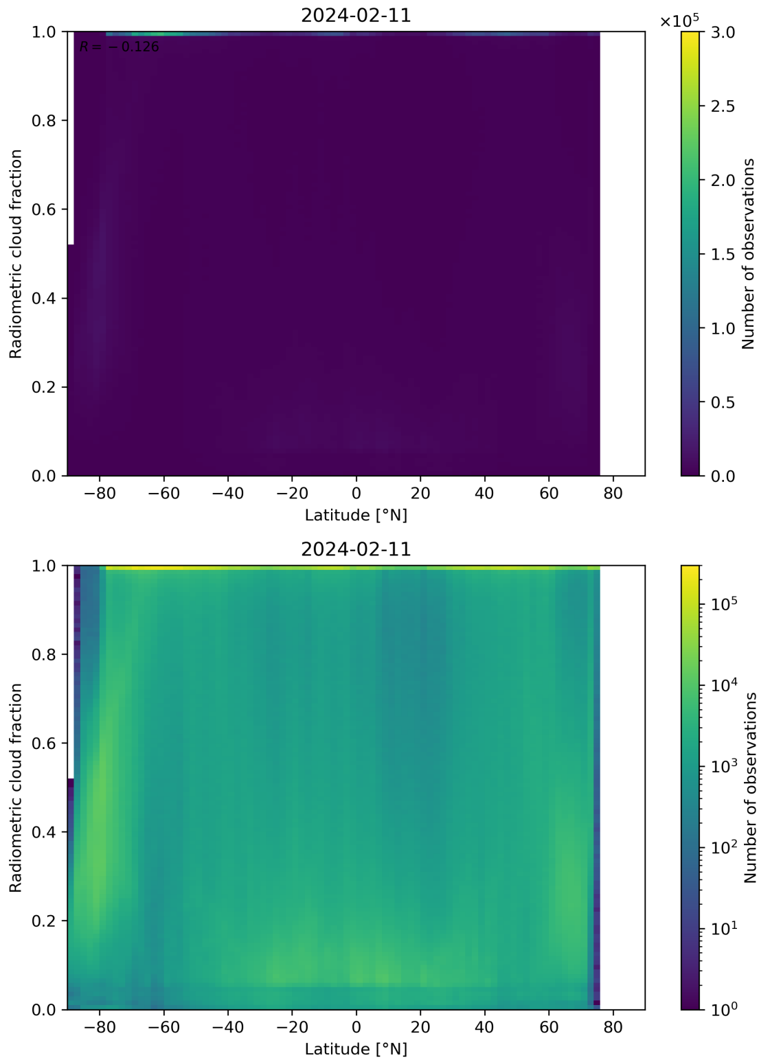
Figure 92: Scatter density plot of “Latitude” against “Radiometric cloud fraction” for 2024-02-11 to 2024-02-12.
