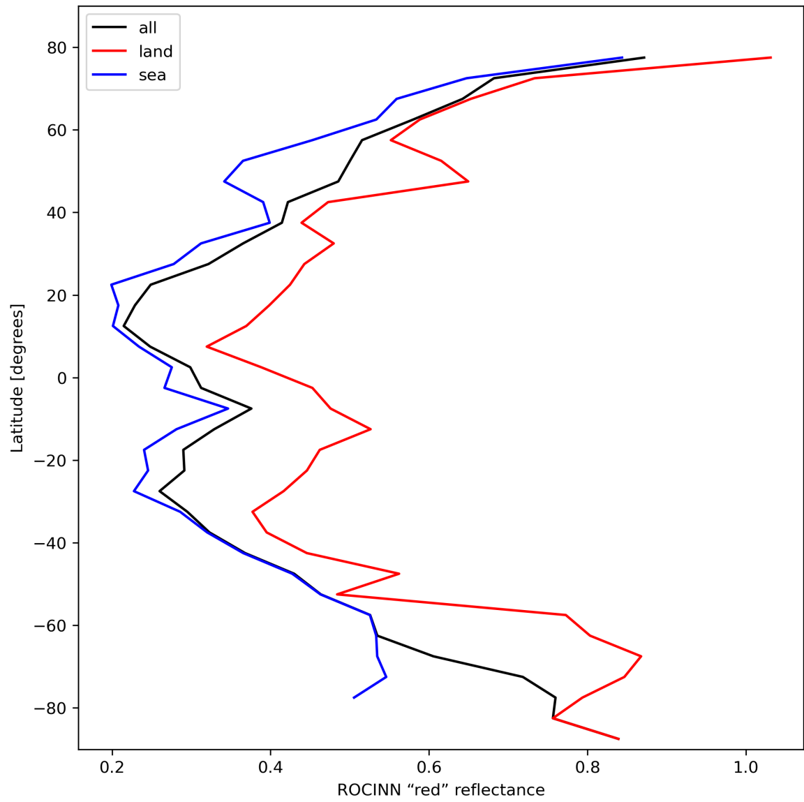
Figure 37: Zonal average of "ROCINN "red" reflectance" for 2024-02-11 to 2024-02-12.
