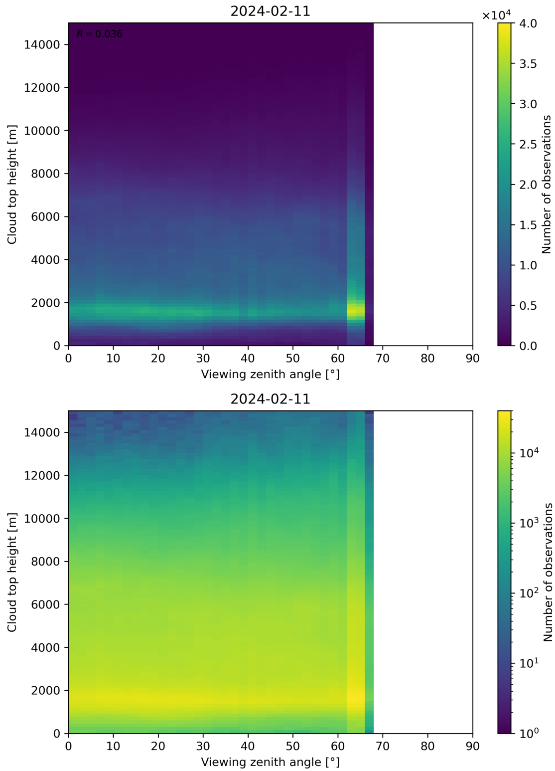
Figure 112: Scatter density plot of “Viewing zenith angle” against “Cloud top height” for 2024-02-11 to 2024-02-12.
