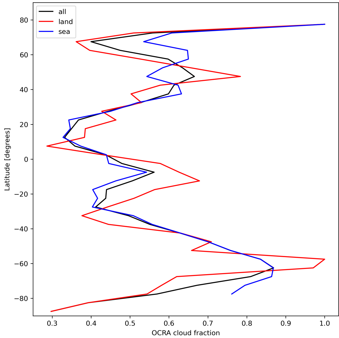
Figure 34: Zonal average of “OCRA cloud fraction” for 2024-02-11 to 2024-02-12.
