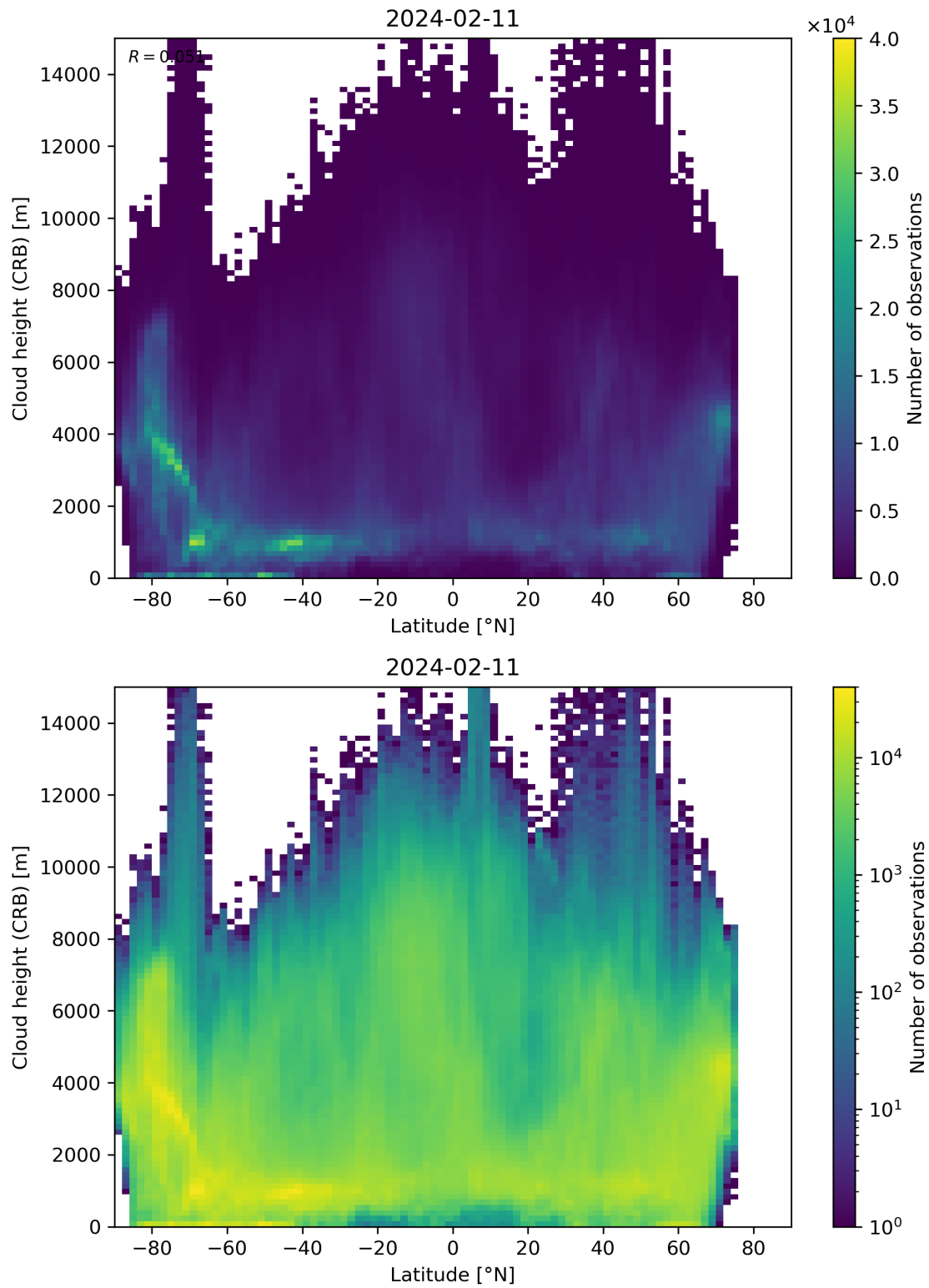
Figure 95: Scatter density plot of “Latitude” against “Cloud height (CRB)” for 2024-02-11 to 2024-02-12.
