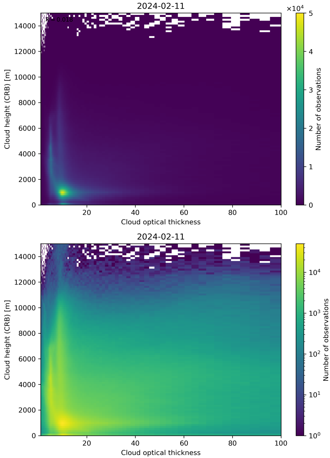
Figure 85: Scatter density plot of “Cloud optical thickness” against “Cloud height (CRB)” for 2024-02-11 to 2024-02-12.
