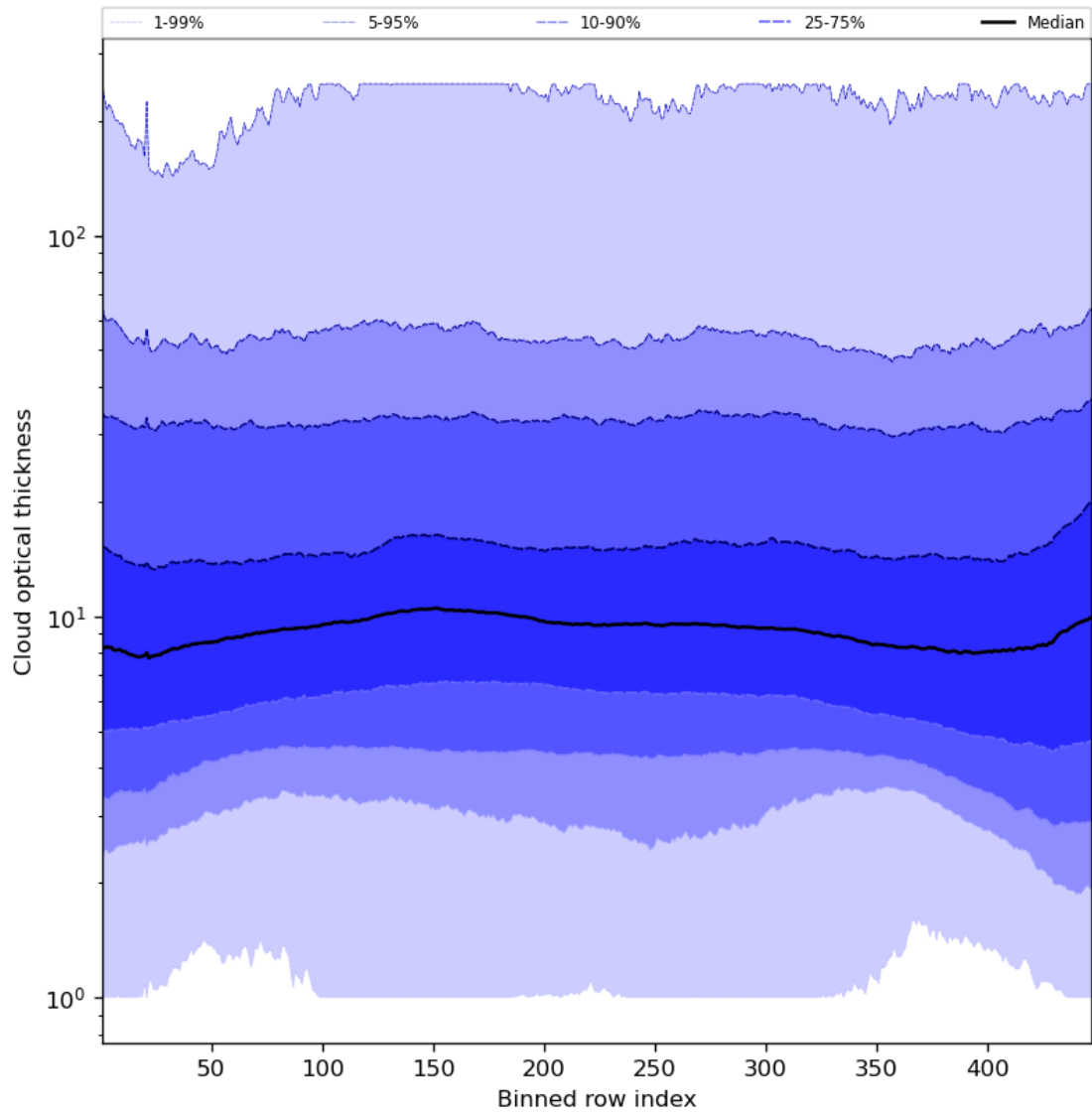
Figure 57: Along track statistics of “Cloud optical thickness” for 2024-02-11 to 2024-02-12
