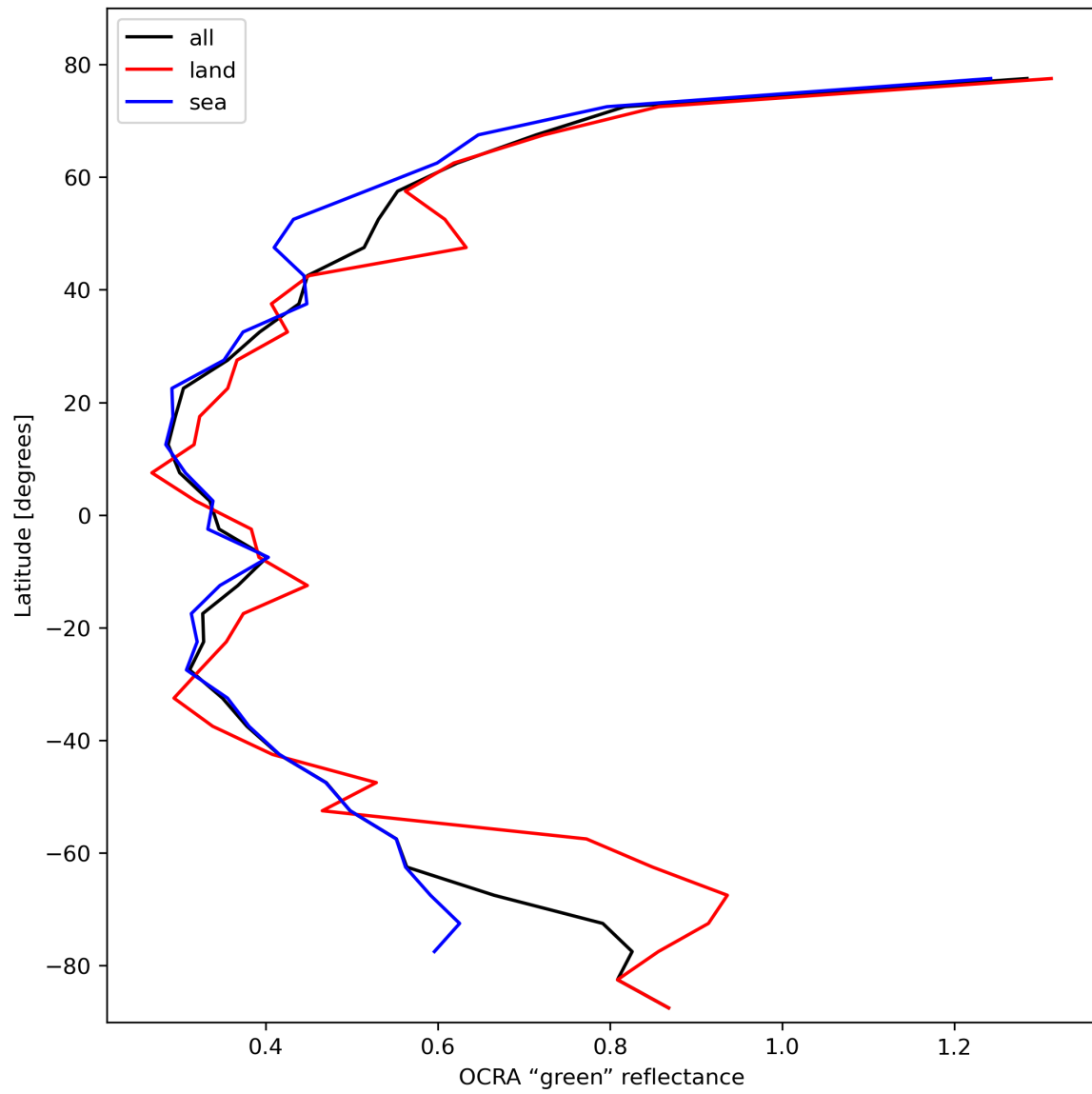
Figure 36: Zonal average of “OCRA “green” reflectance” for 2024-02-11 to 2024-02-12.
