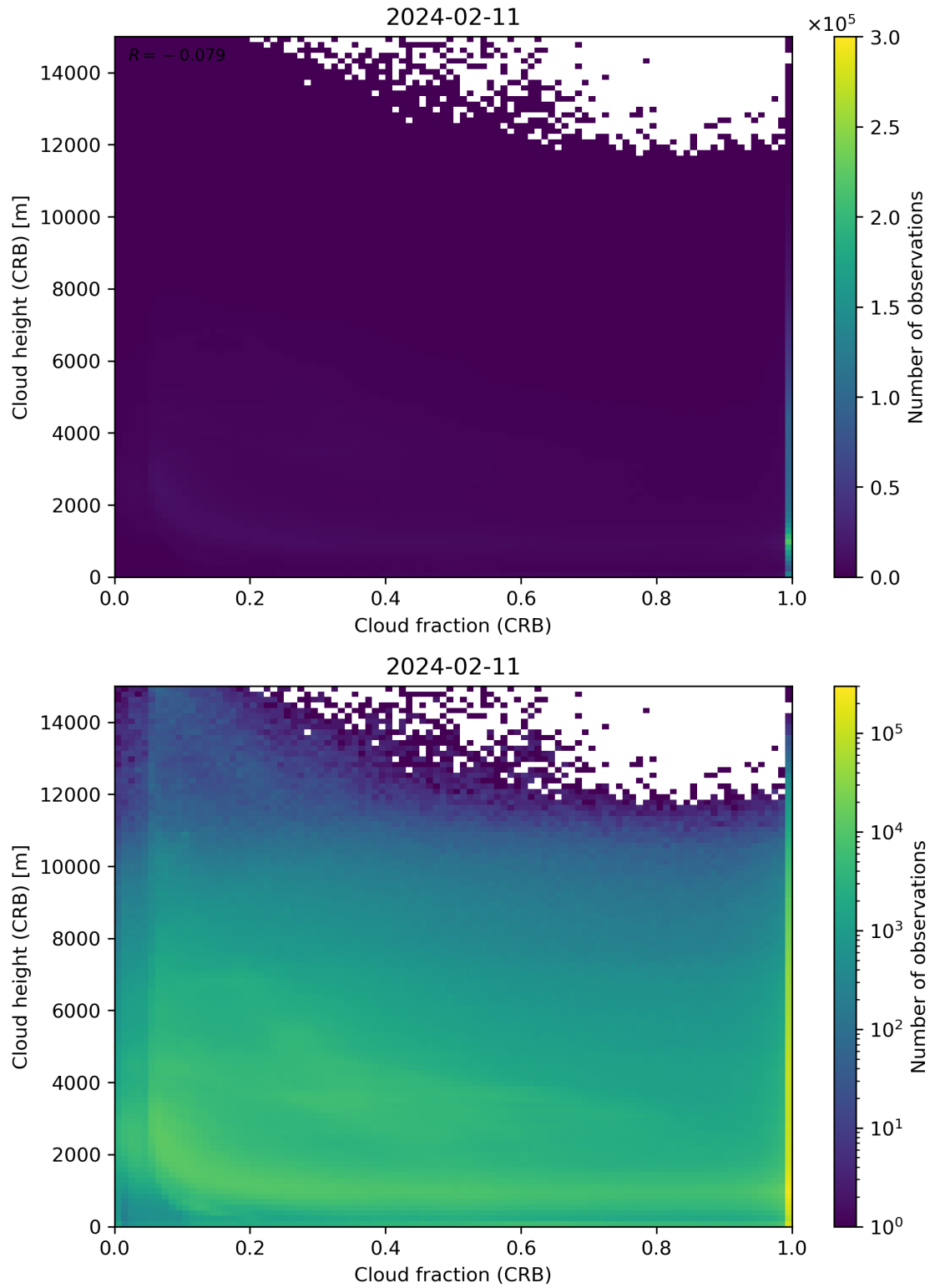
Figure 79: Scatter density plot of “Cloud fraction (CRB)” against “Cloud height (CRB)” for 2024-02-11 to 2024-02-12.
