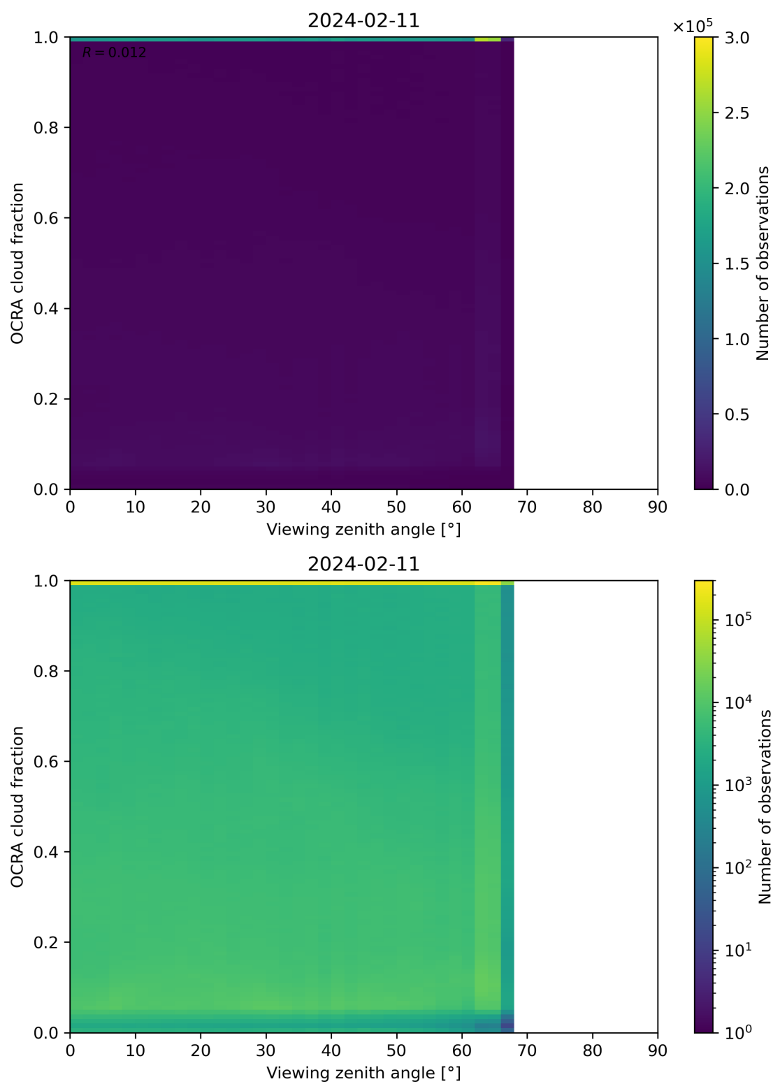
Figure 108: Scatter density plot of “Viewing zenith angle” against “OCRA cloud fraction” for 2024-02-11 to 2024-02-12.
