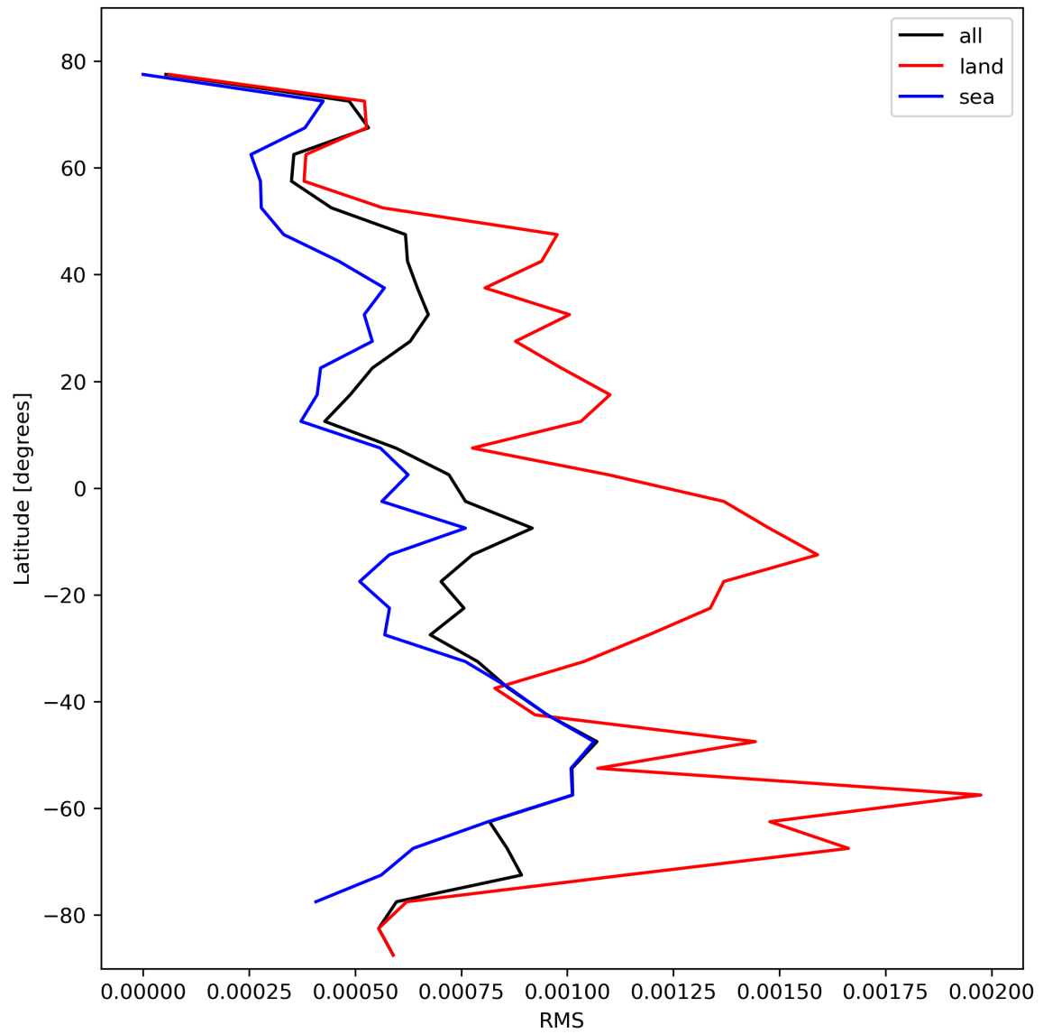
Figure 31: Zonal average of “RMS” for 2024-02-11 to 2024-02-12.
