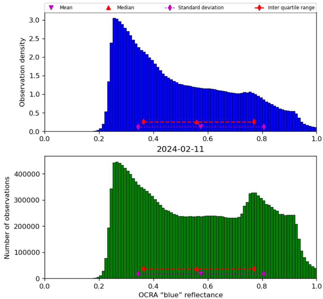
Figure 51: Histogram of “OCRA “blue” reflectance” for 2024-02-11 to 2024-02-12
