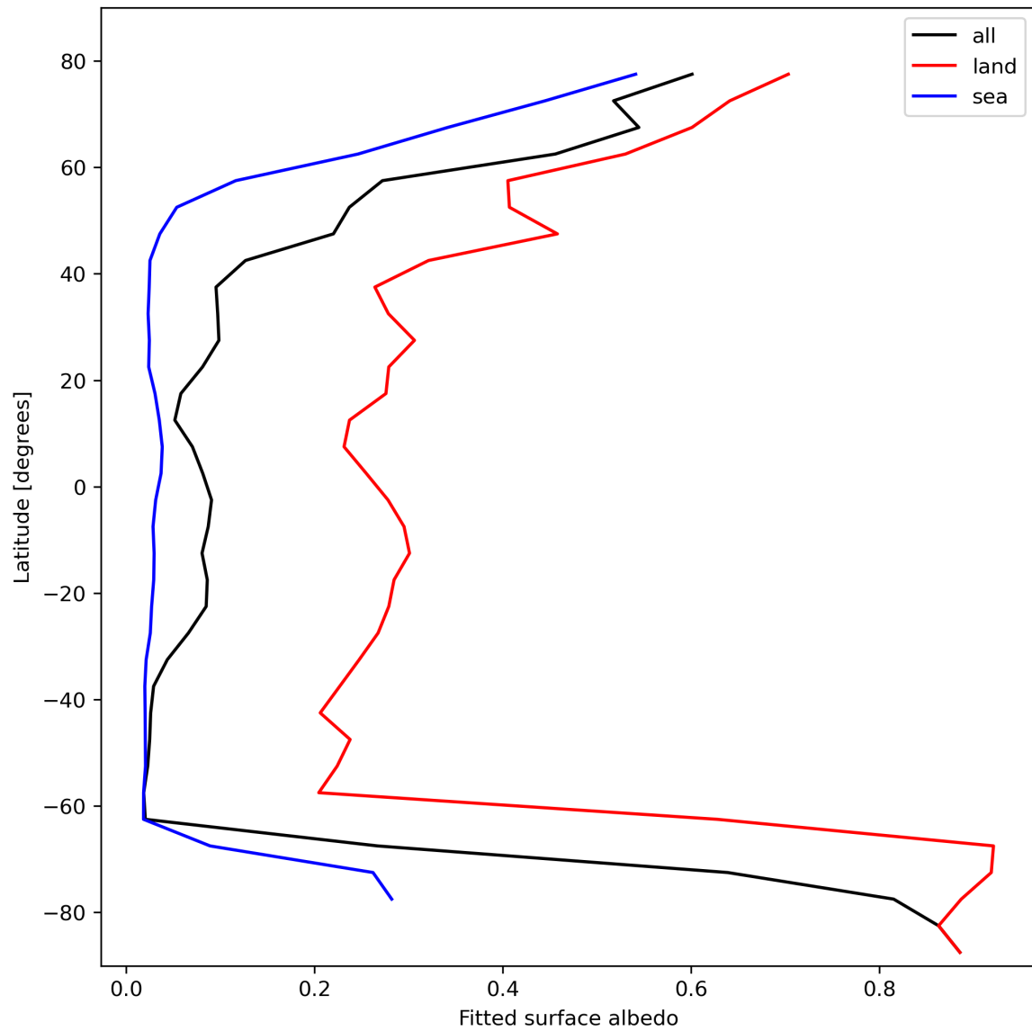
Figure 29: Zonal average of “Fitted surface albedo” for 2024-02-11 to 2024-02-12.
