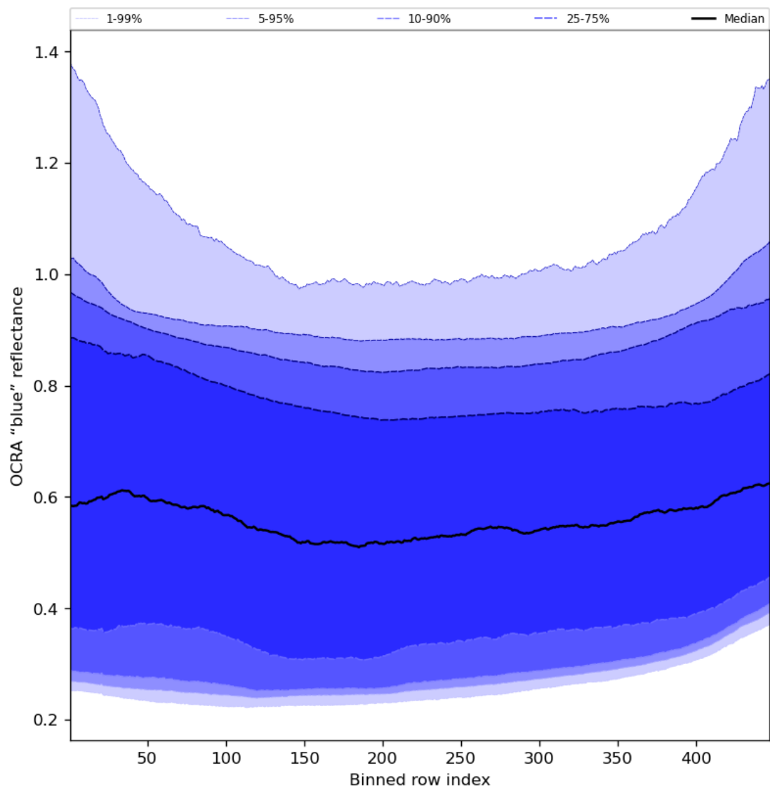
Figure 67: Along track statistics of “OCRA “blue” reflectance” for 2024-02-11 to 2024-02-12
