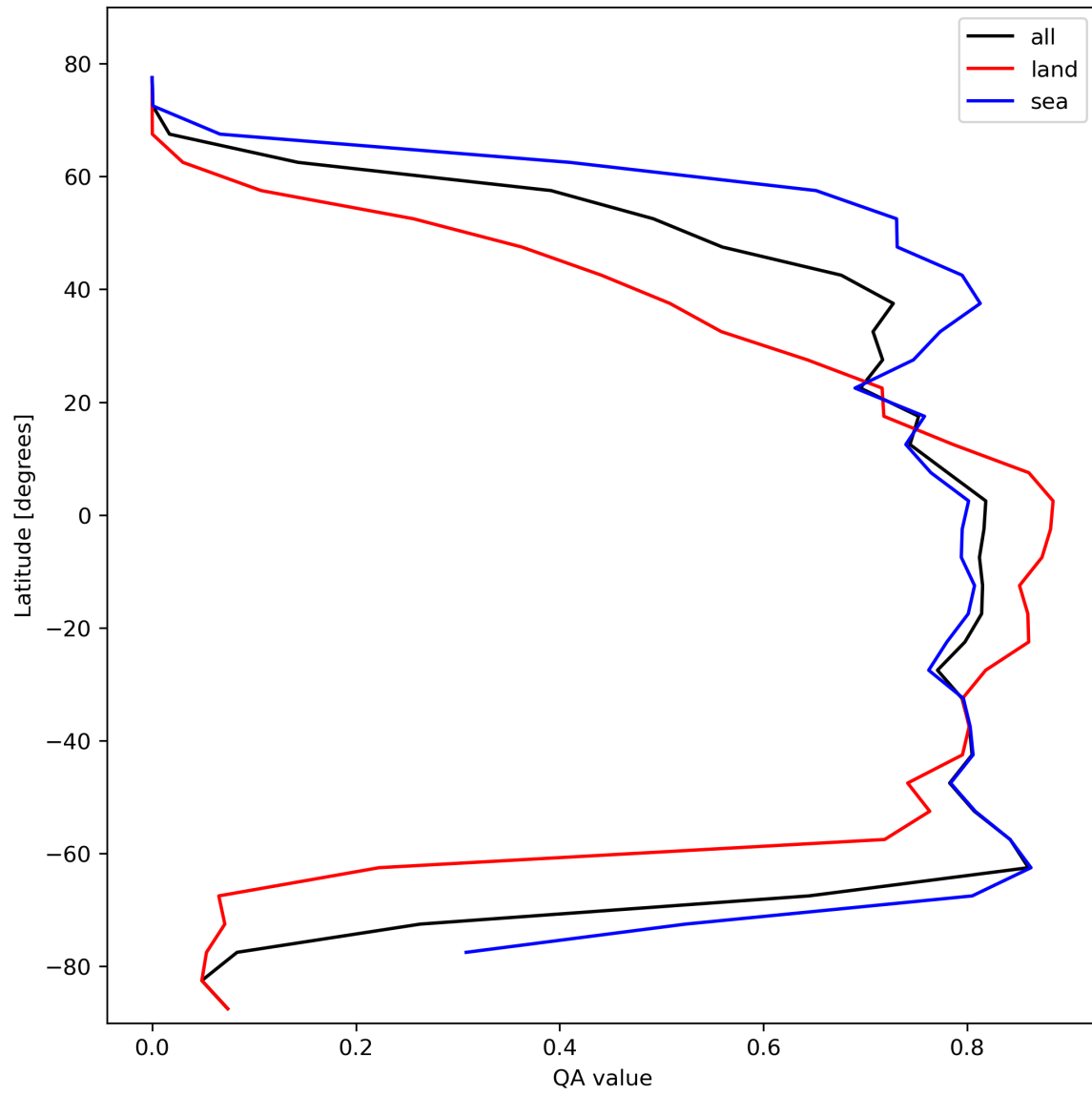
Figure 22: Zonal average of “QA value” for 2024-02-11 to 2024-02-12.
