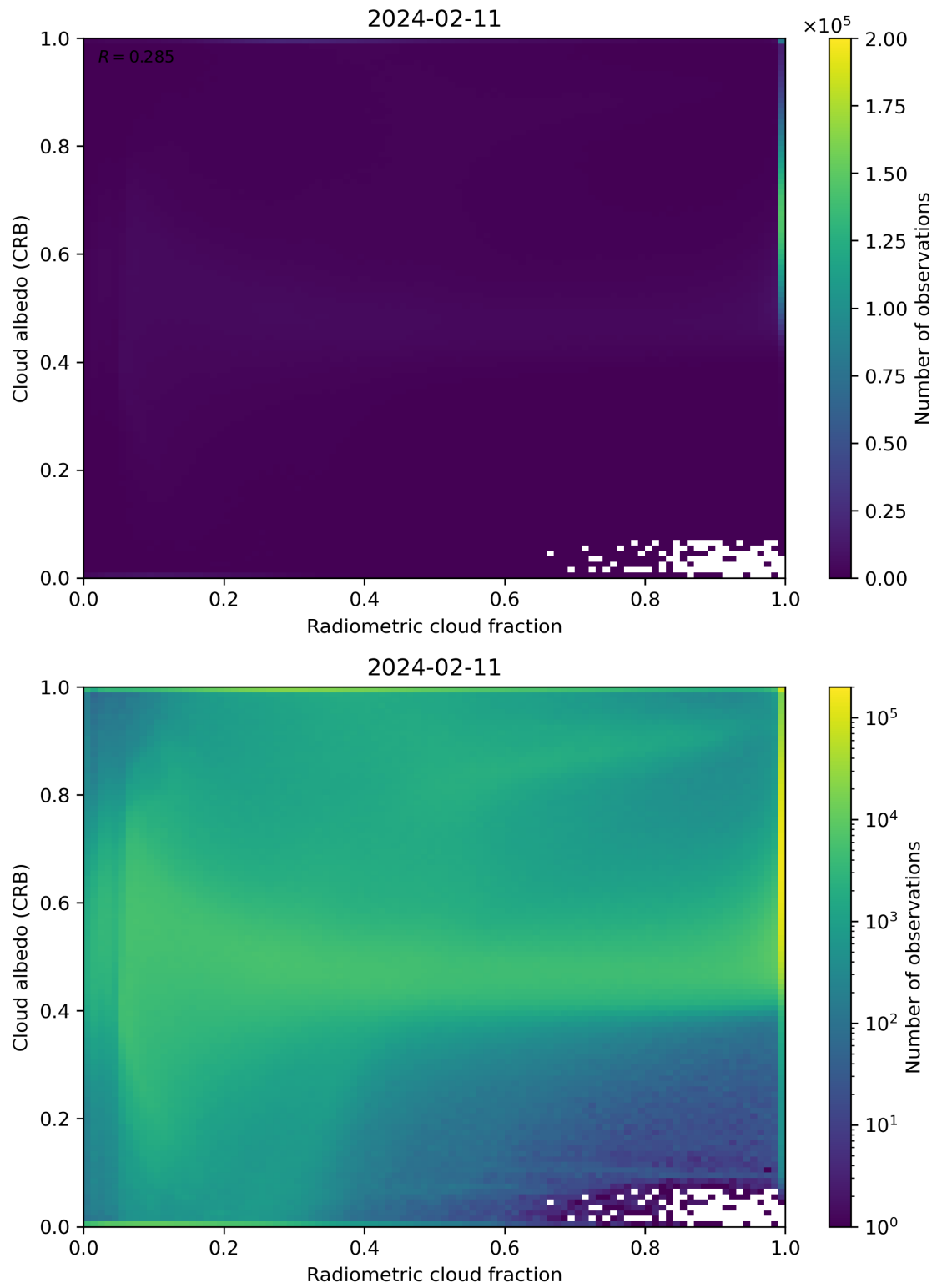
Figure 71: Scatter density plot of “Radiometric cloud fraction” against “Cloud albedo (CRB)” for 2024-02-11 to 2024-02-12.
