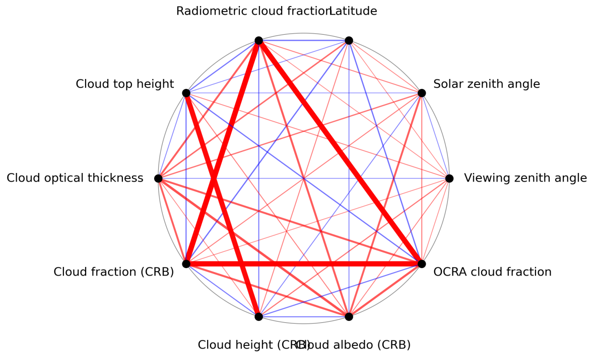
Figure 1: Map of correlation graph for 2024-02-11 to 2024-02-12.
