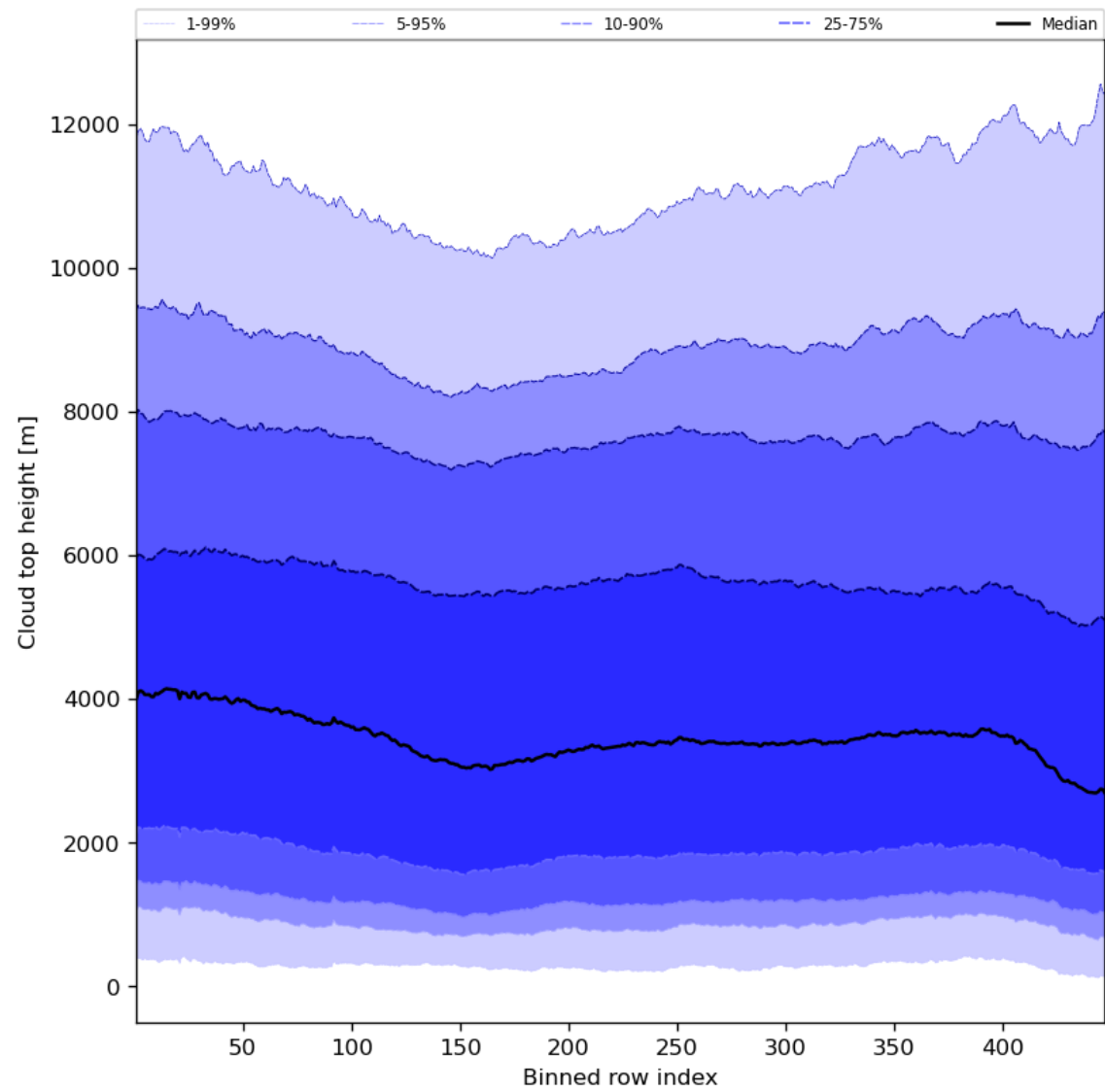
Figure 56: Along track statistics of “Cloud top height” for 2024-02-11 to 2024-02-12
