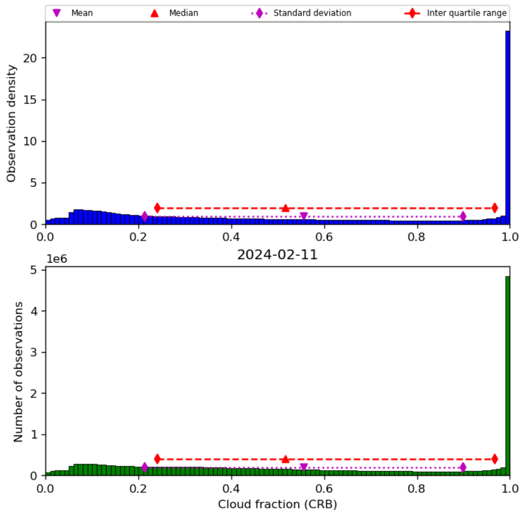
Figure 42: Histogram of “Cloud fraction (CRB)” for 2024-02-11 to 2024-02-12
