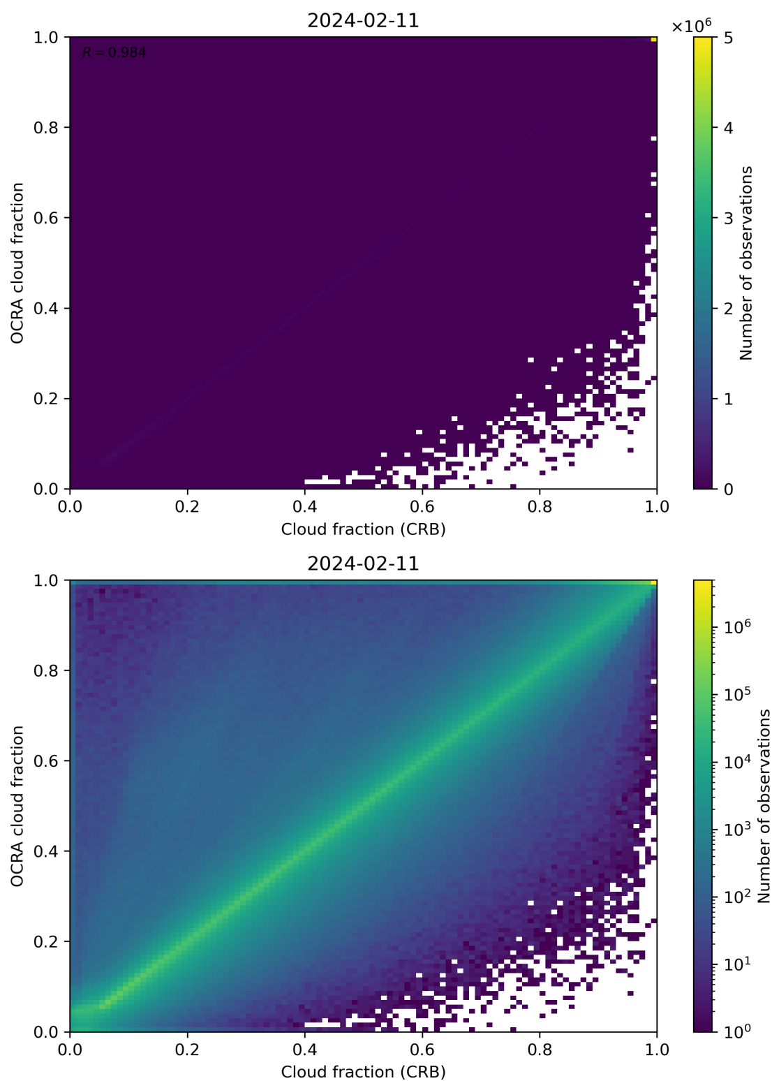
Figure 78: Scatter density plot of “Cloud fraction (CRB)” against “OCRA cloud fraction” for 2024-02-11 to 2024-02-12.
