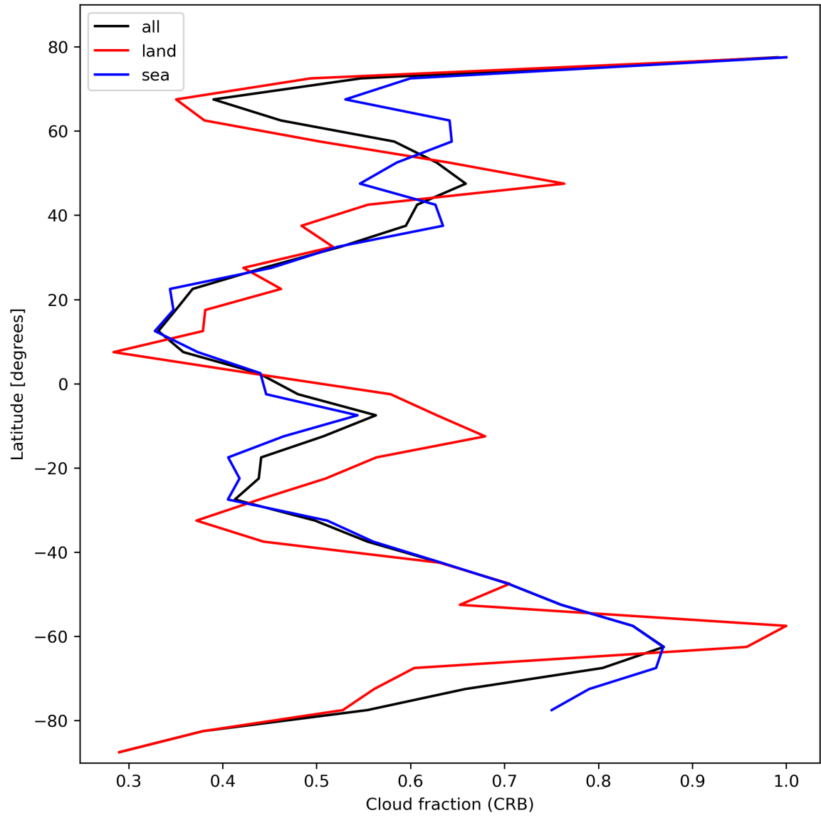
Figure 26: Zonal average of “Cloud fraction (CRB)” for 2024-02-11 to 2024-02-12.
