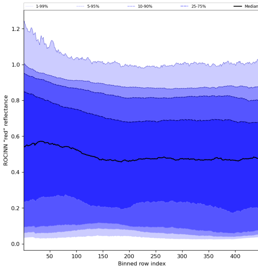
Figure 69: Along track statistics of “ROCINN “red” reflectance” for 2024-02-11 to 2024-02-12
