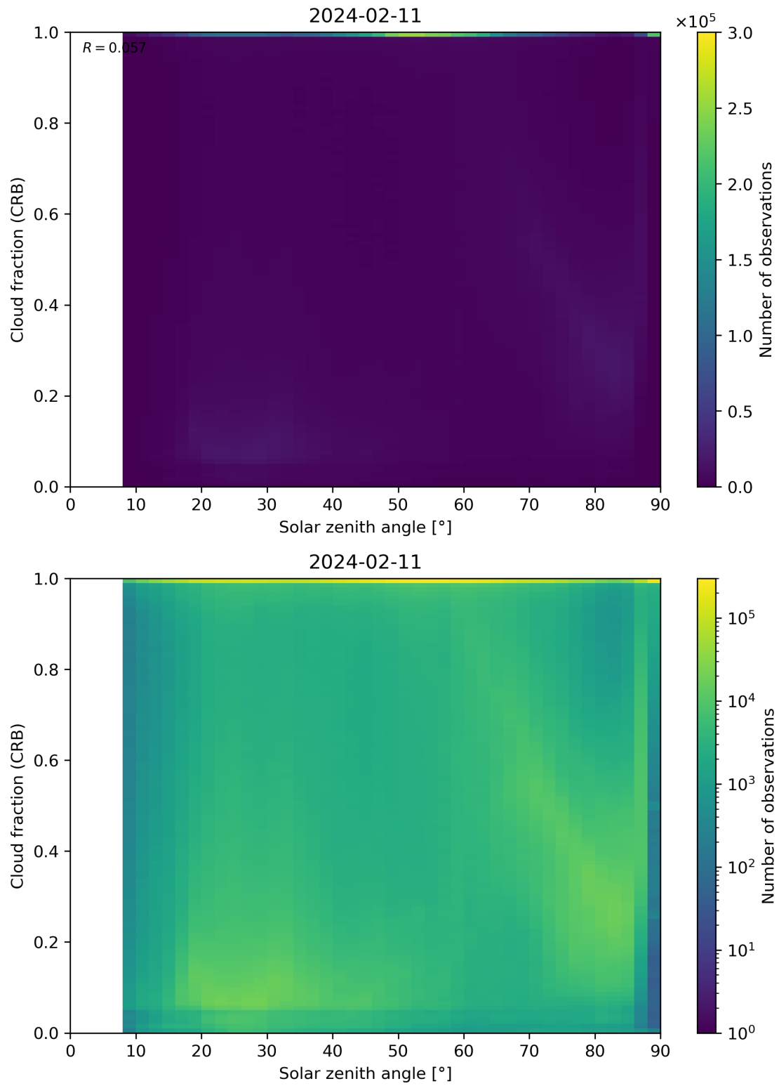
Figure 101: Scatter density plot of “Solar zenith angle” against “Cloud fraction (CRB)” for 2024-02-11 to 2024-02-12.
