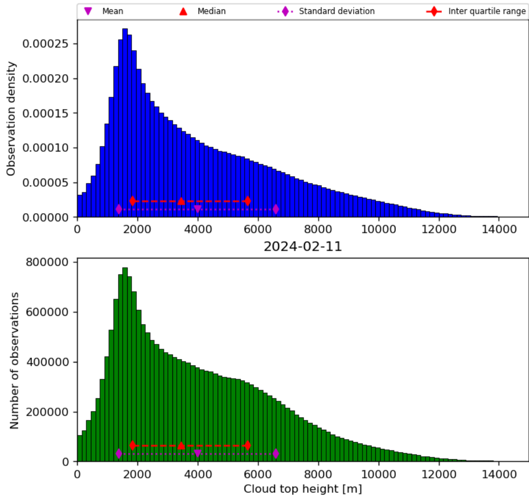
Figure 40: Histogram of “Cloud top height” for 2024-02-11 to 2024-02-12
