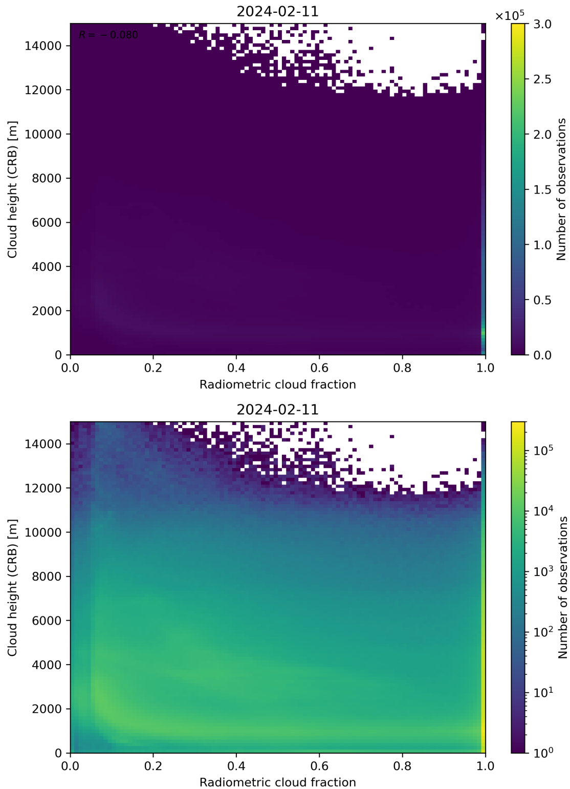
Figure 74: Scatter density plot of “Radiometric cloud fraction” against “Cloud height (CRB)” for 2024-02-11 to 2024-02-12.
