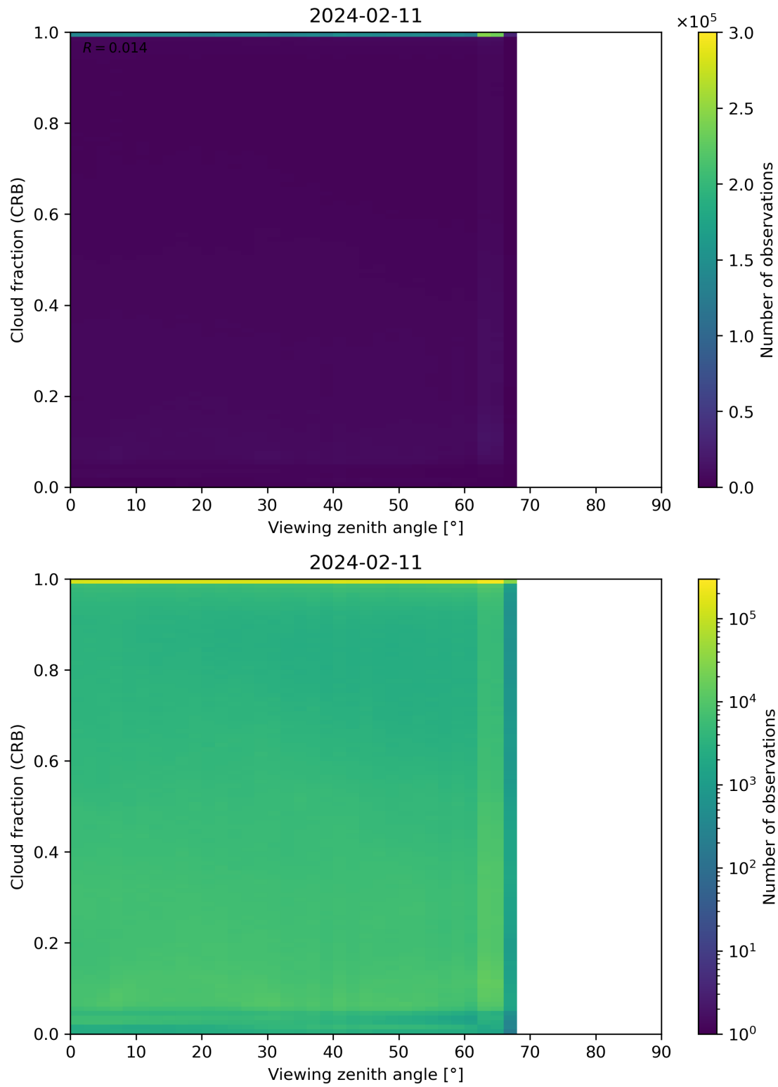
Figure 109: Scatter density plot of “Viewing zenith angle” against “Cloud fraction (CRB)” for 2024-02-11 to 2024-02-12.
