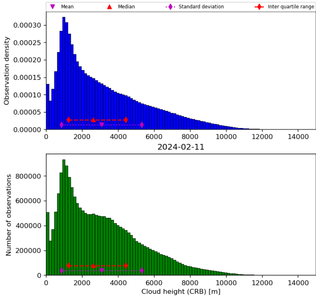
Figure 43: Histogram of “Cloud height (CRB)” for 2024-02-11 to 2024-02-12
