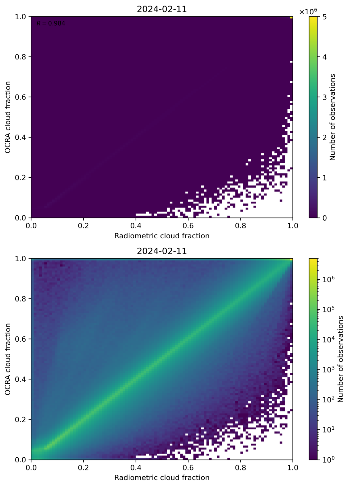
Figure 72: Scatter density plot of “Radiometric cloud fraction” against “OCRA cloud fraction” for 2024-02-11 to 2024-02-12.
