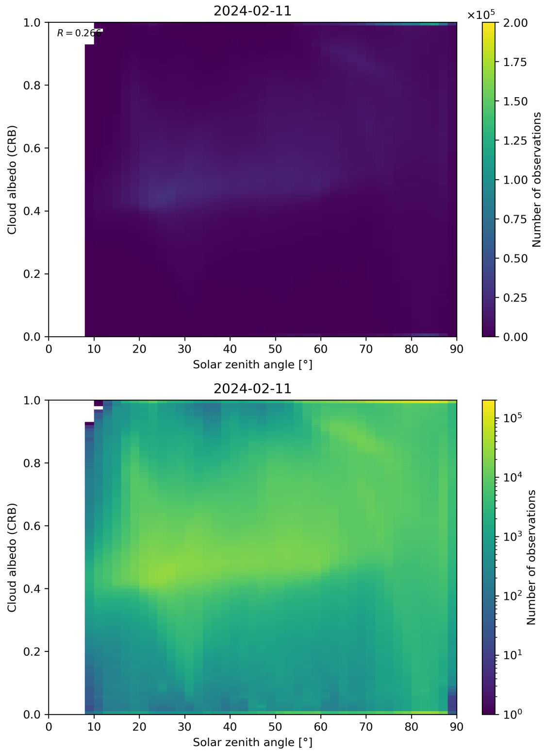
Figure 98: Scatter density plot of “Solar zenith angle” against “Cloud albedo (CRB)” for 2024-02-11 to 2024-02-12.
