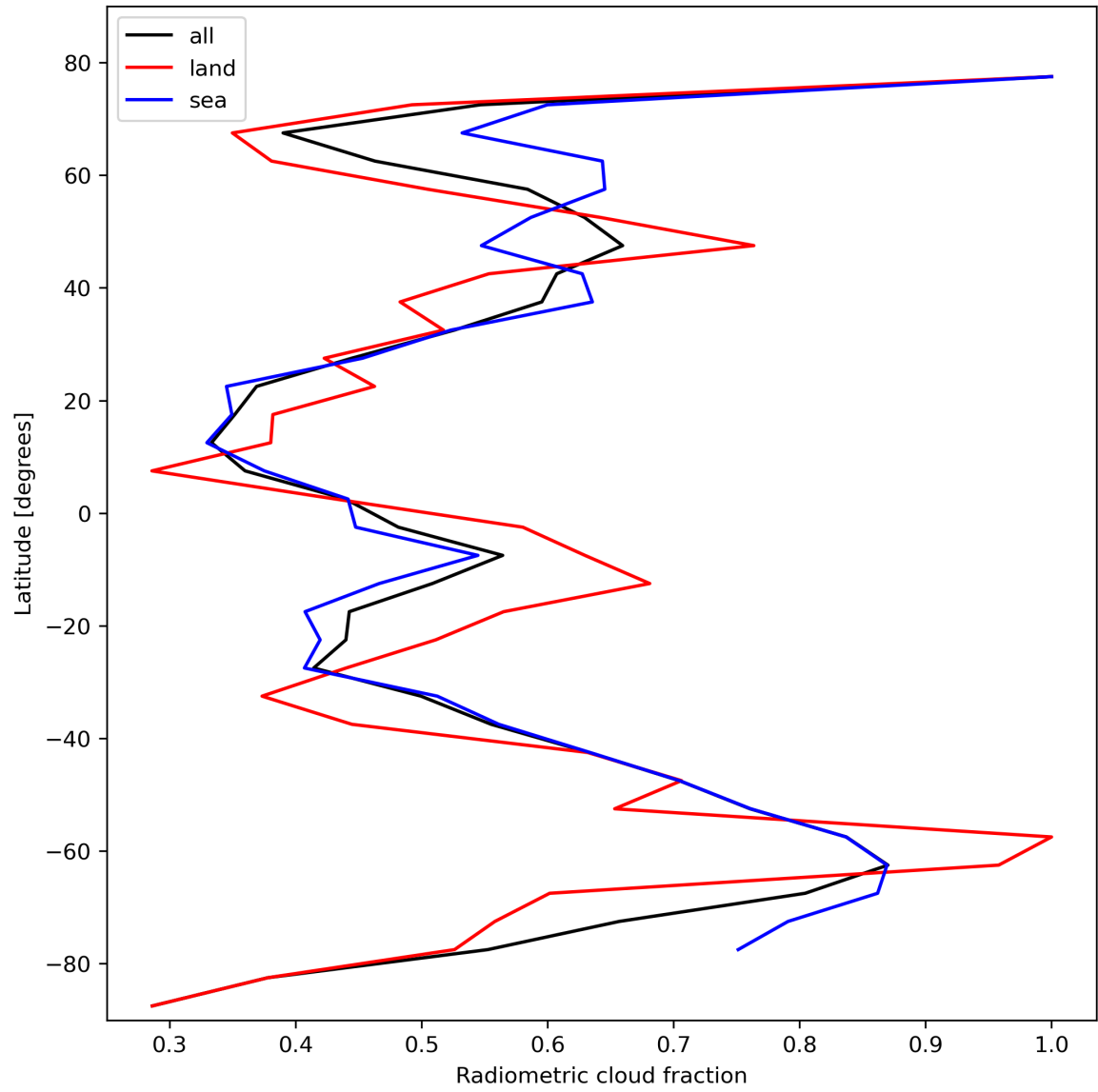
Figure 23: Zonal average of “Radiometric cloud fraction” for 2024-02-11 to 2024-02-12.
