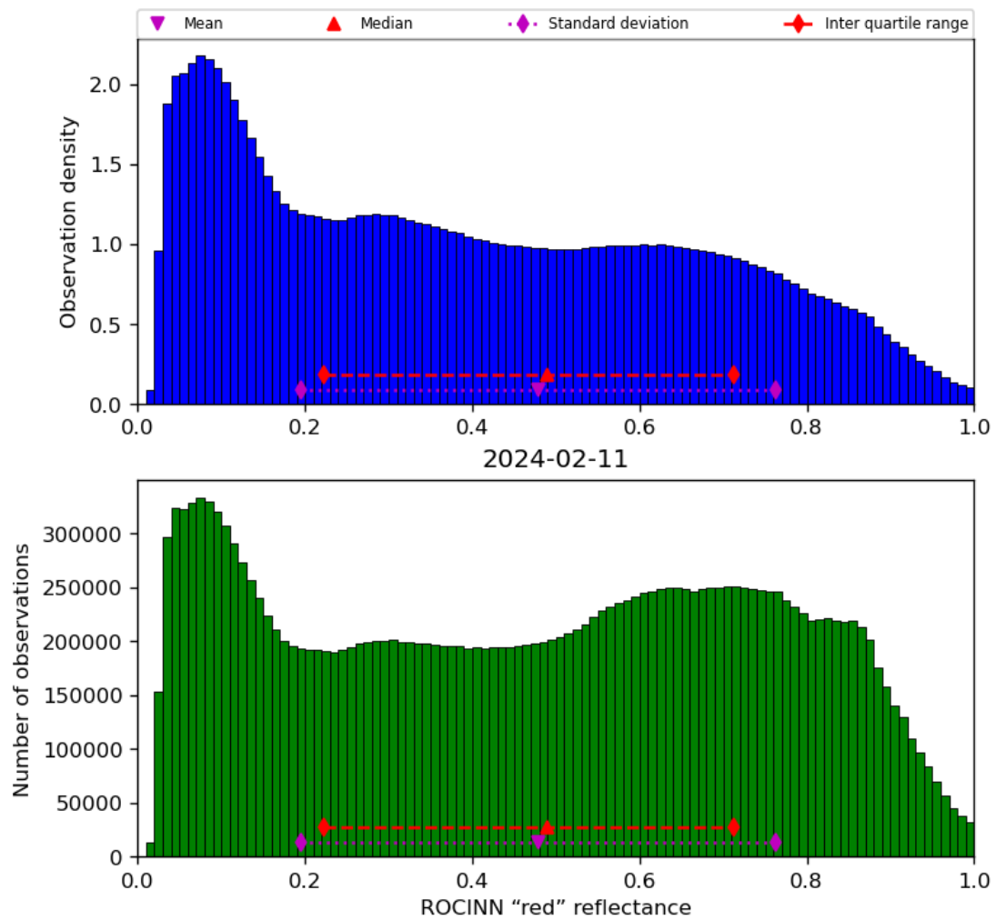
Figure 53: Histogram of “ROCINN “red” reflectance” for 2024-02-11 to 2024-02-12
