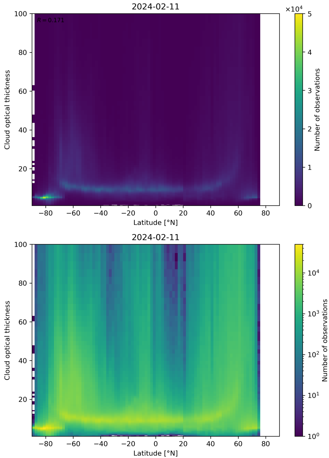
Figure 96: Scatter density plot of “Latitude” against “Cloud optical thickness” for 2024-02-11 to 2024-02-12.
