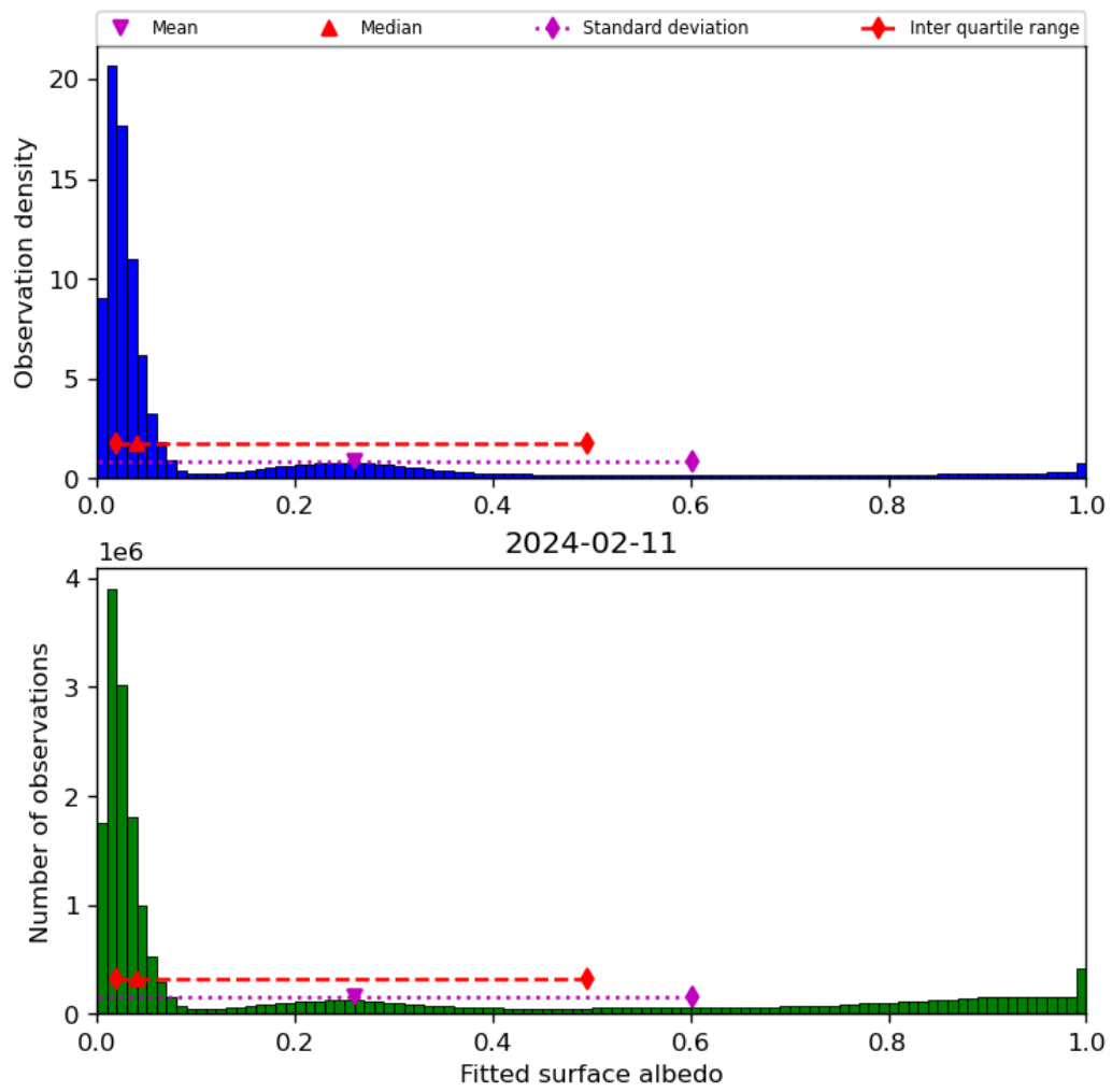
Figure 45: Histogram of “Fitted surface albedo” for 2024-02-11 to 2024-02-12
