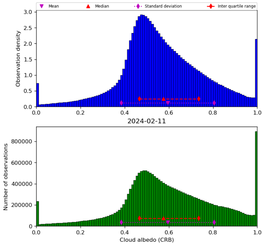
Figure 44: Histogram of “Cloud albedo (CRB)” for 2024-02-11 to 2024-02-12
