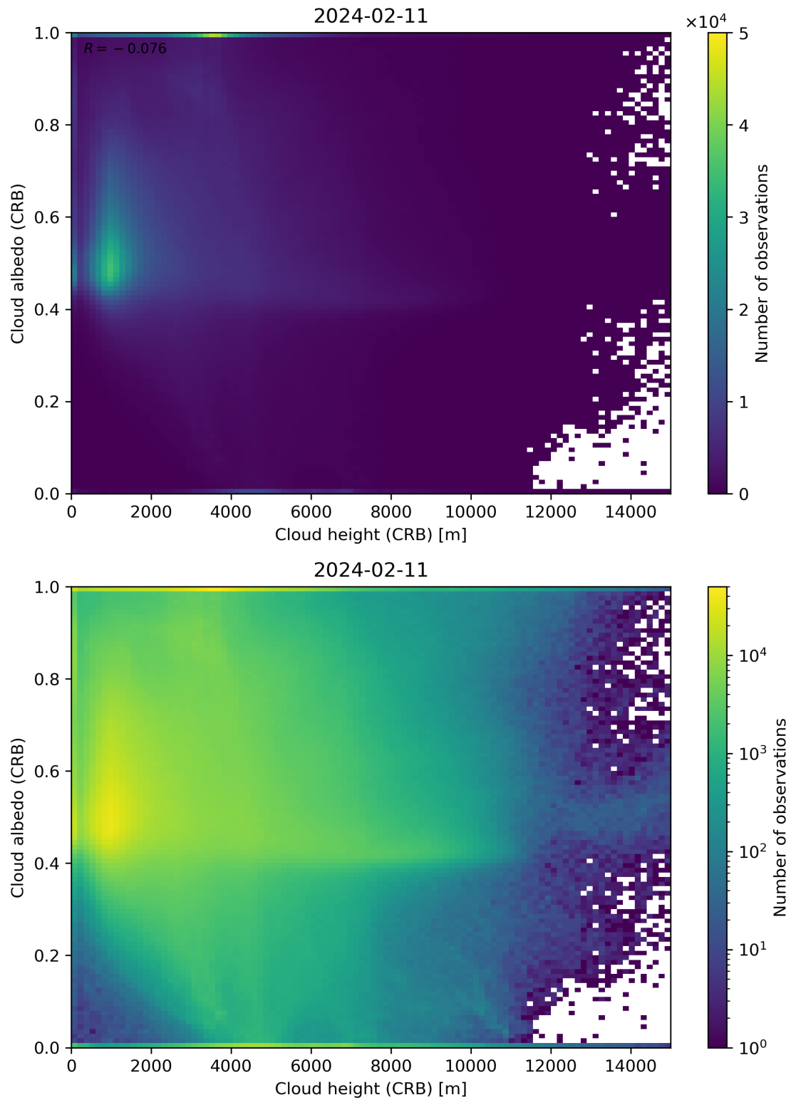
Figure 80: Scatter density plot of “Cloud height (CRB)” against “Cloud albedo (CRB)” for 2024-02-11 to 2024-02-12.
