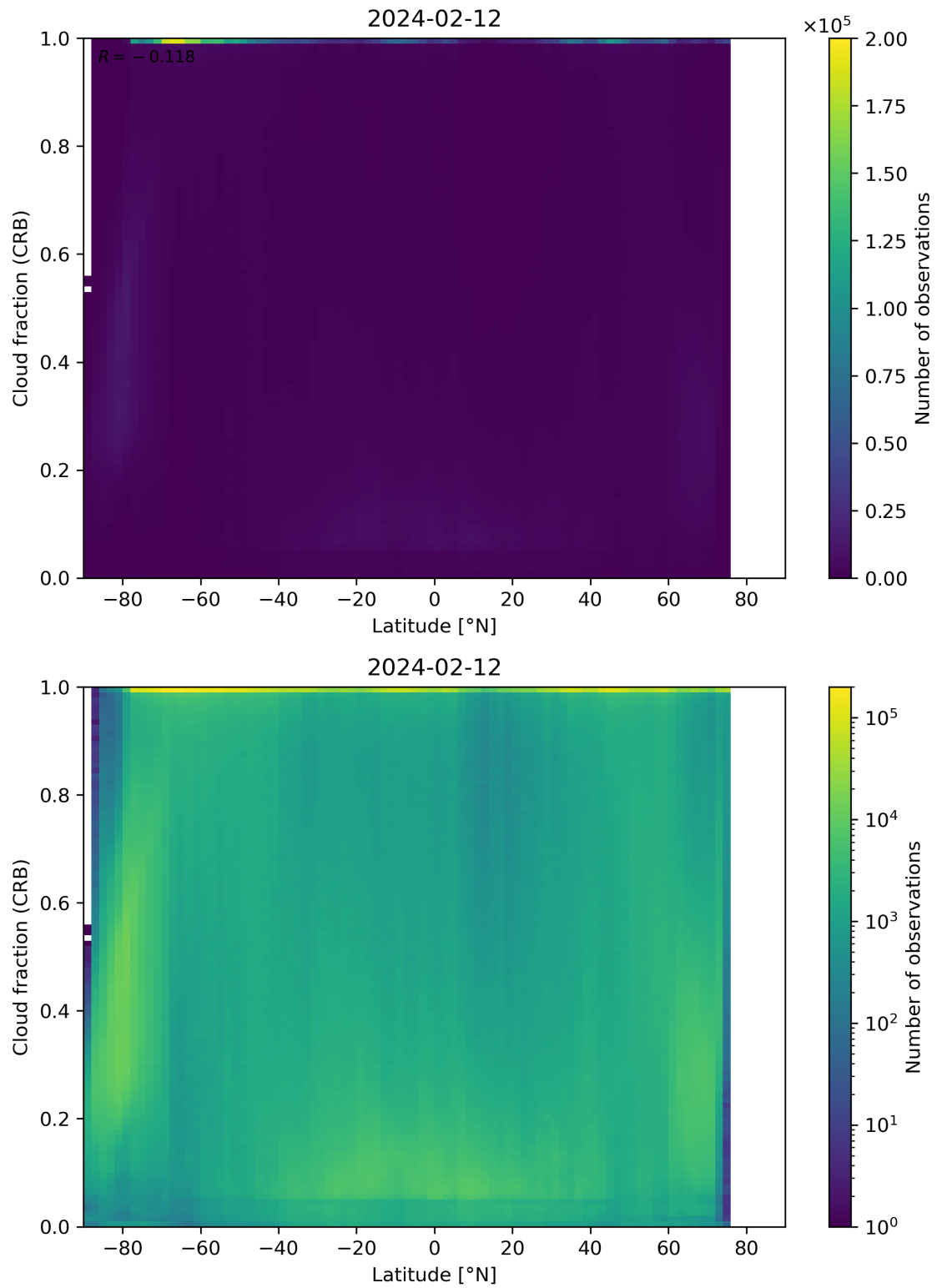
Figure 94: Scatter density plot of “Latitude” against “Cloud fraction (CRB)” for 2024-02-11 to 2024-02-13.
