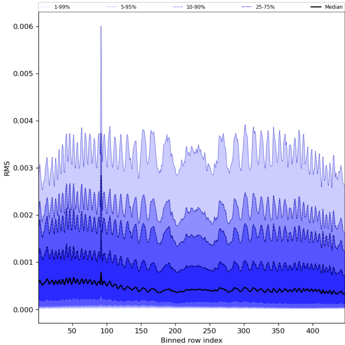
Figure 63: Along track statistics of “RMS” for 2024-02-11 to 2024-02-13
