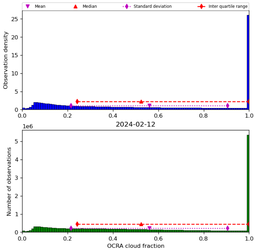
Figure 50: Histogram of “OCRA cloud fraction” for 2024-02-11 to 2024-02-13
