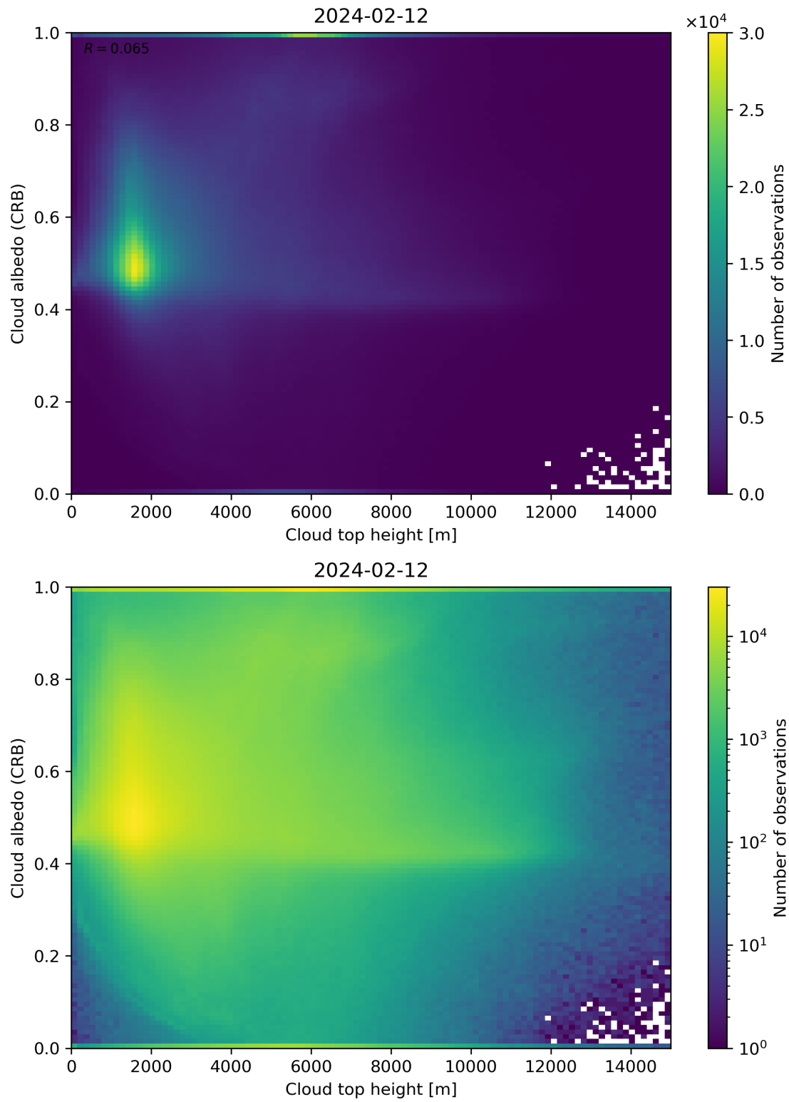
Figure 86: Scatter density plot of “Cloud top height” against “Cloud albedo (CRB)” for 2024-02-11 to 2024-02-13.
