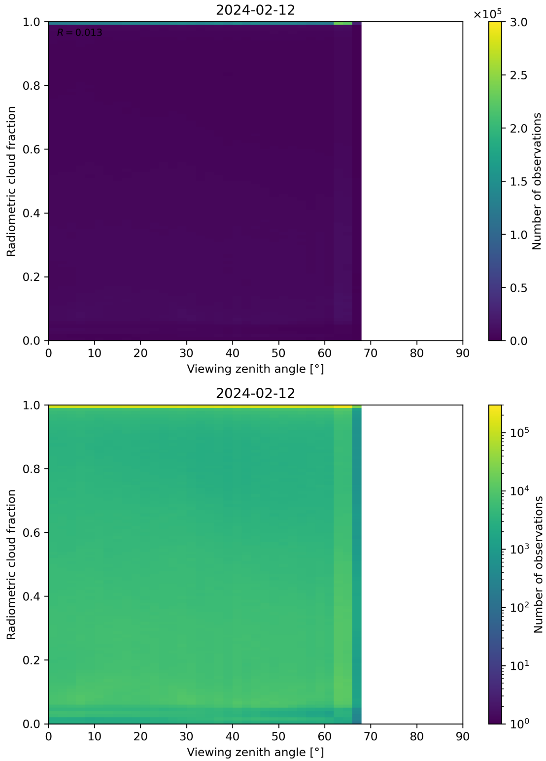
Figure 107: Scatter density plot of “Viewing zenith angle” against “Radiometric cloud fraction” for 2024-02-11 to 2024-02-13.
