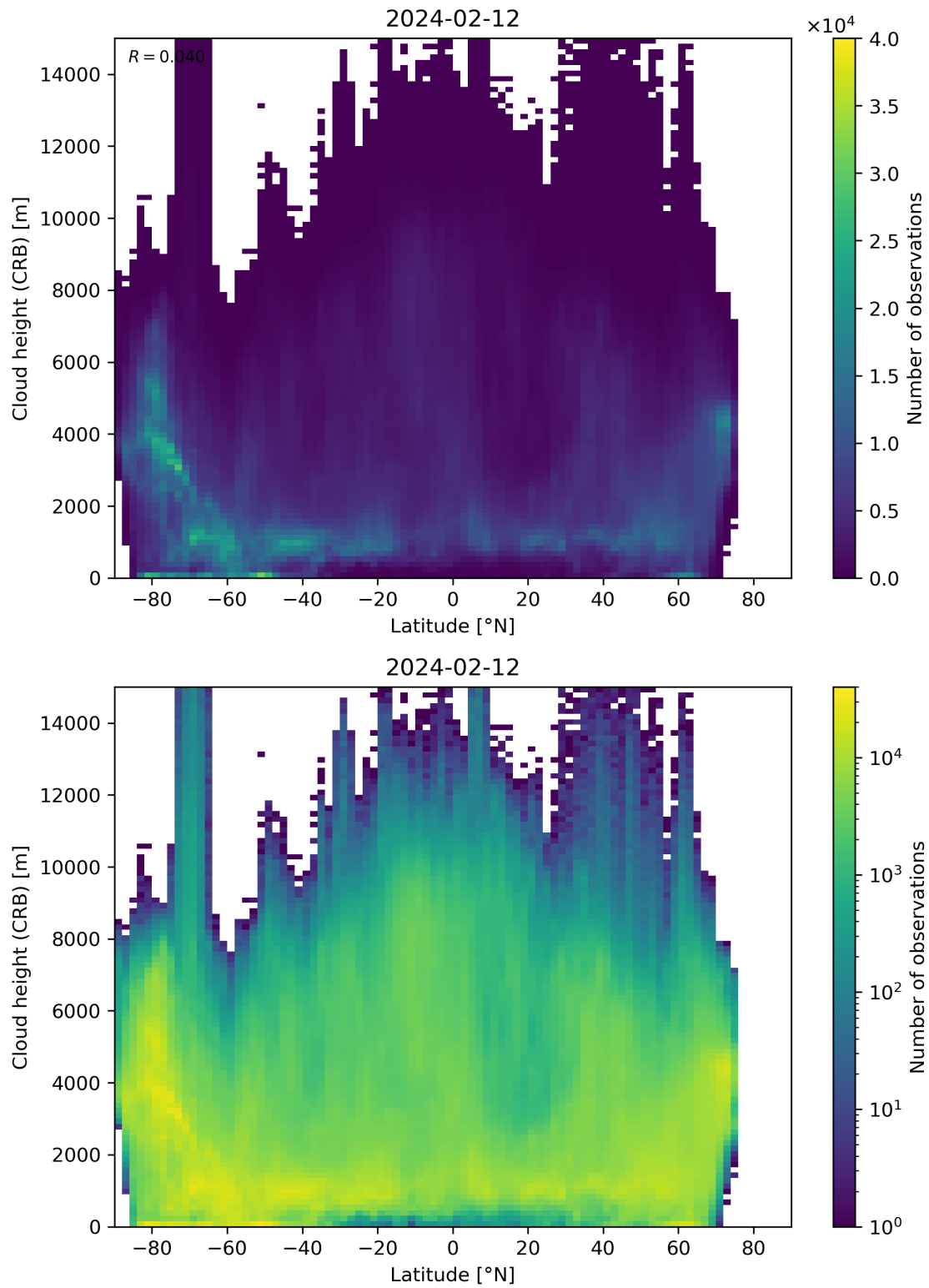
Figure 95: Scatter density plot of “Latitude” against “Cloud height (CRB)” for 2024-02-11 to 2024-02-13.
