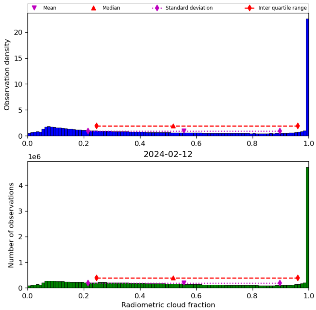
Figure 39: Histogram of “Radiometric cloud fraction” for 2024-02-11 to 2024-02-13
