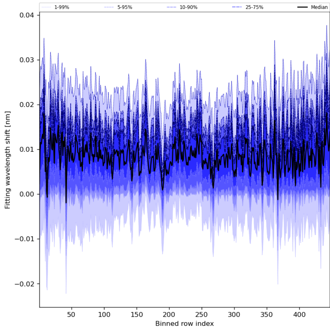
Figure 65: Along track statistics of “Fitting wavelength shift” for 2024-02-11 to 2024-02-13
