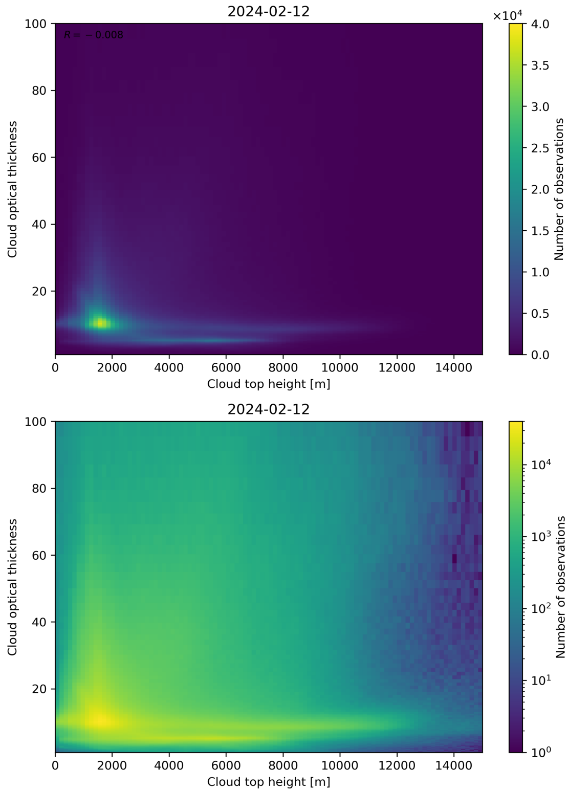
Figure 90: Scatter density plot of “Cloud top height” against “Cloud optical thickness” for 2024-02-11 to 2024-02-13.
