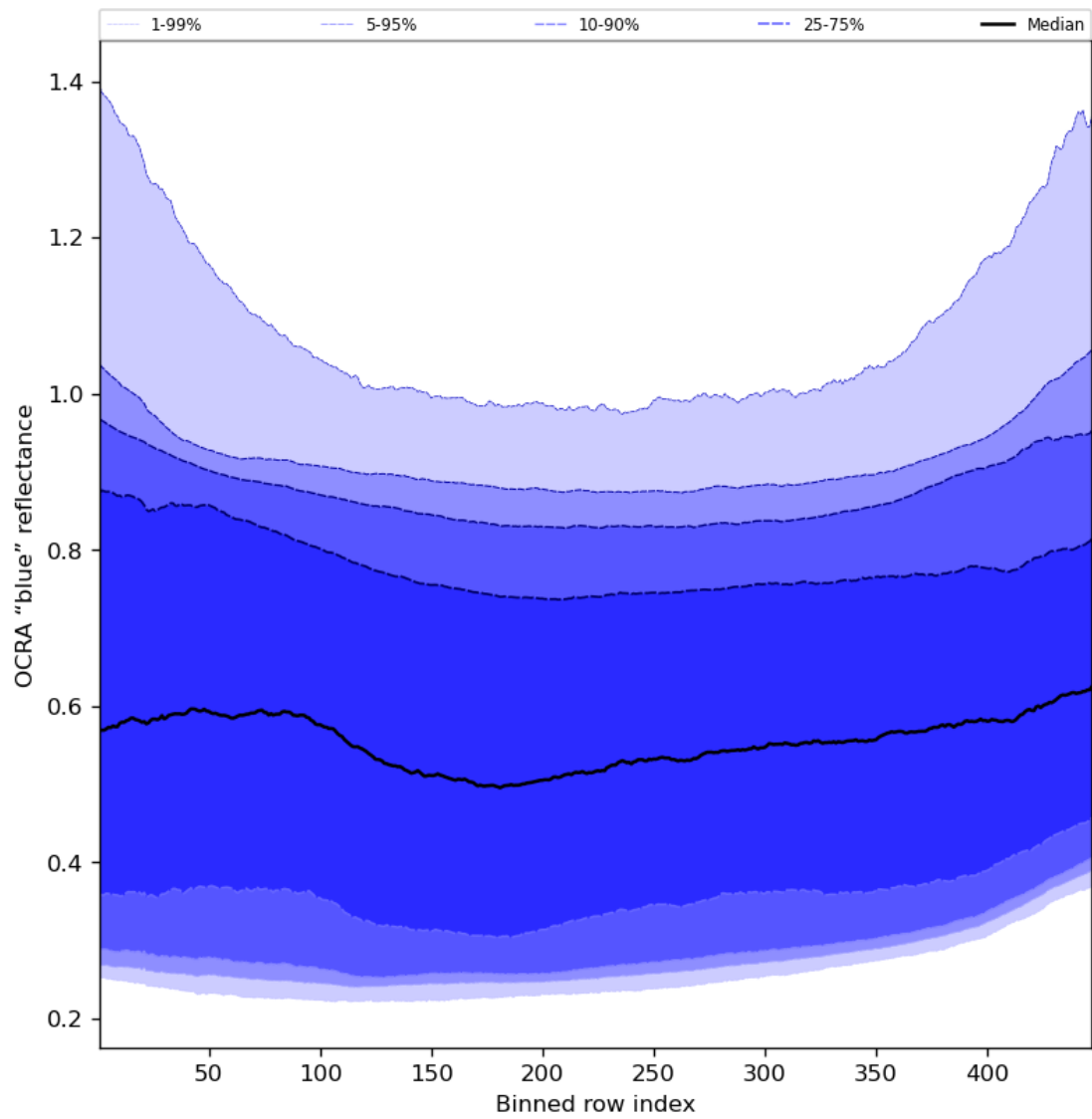
Figure 67: Along track statistics of “OCRA “blue” reflectance” for 2024-02-11 to 2024-02-13
