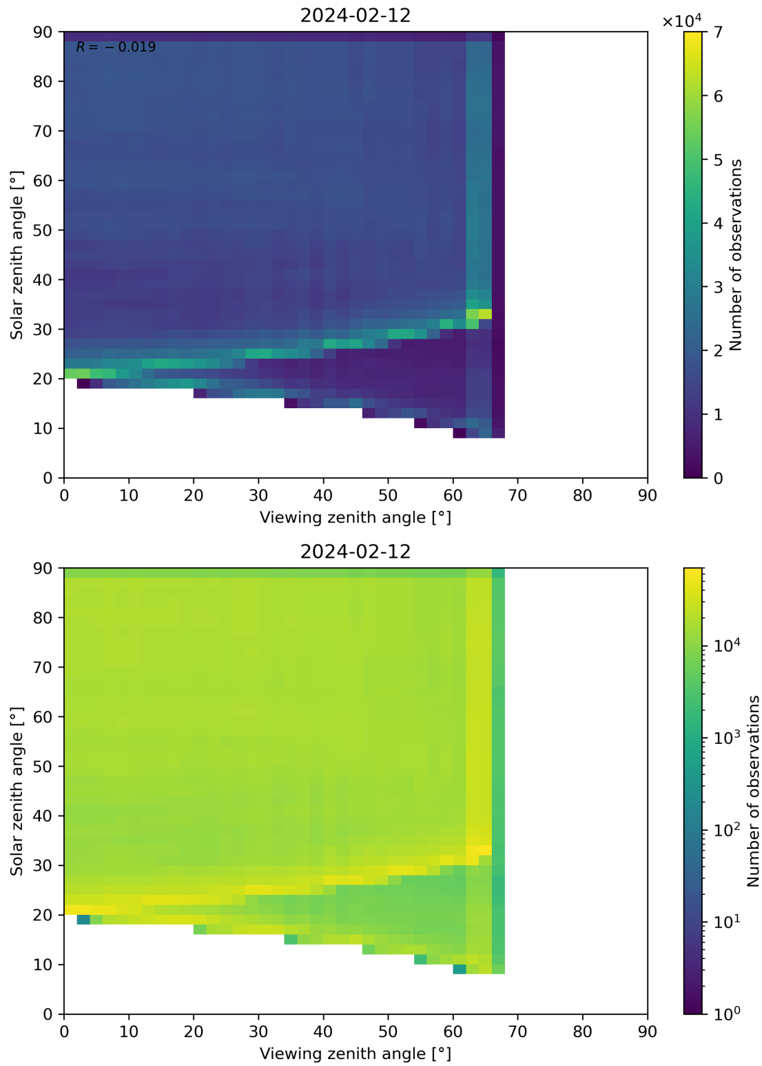
Figure 114: Scatter density plot of “Viewing zenith angle” against “Solar zenith angle” for 2024-02-11 to 2024-02-13.
