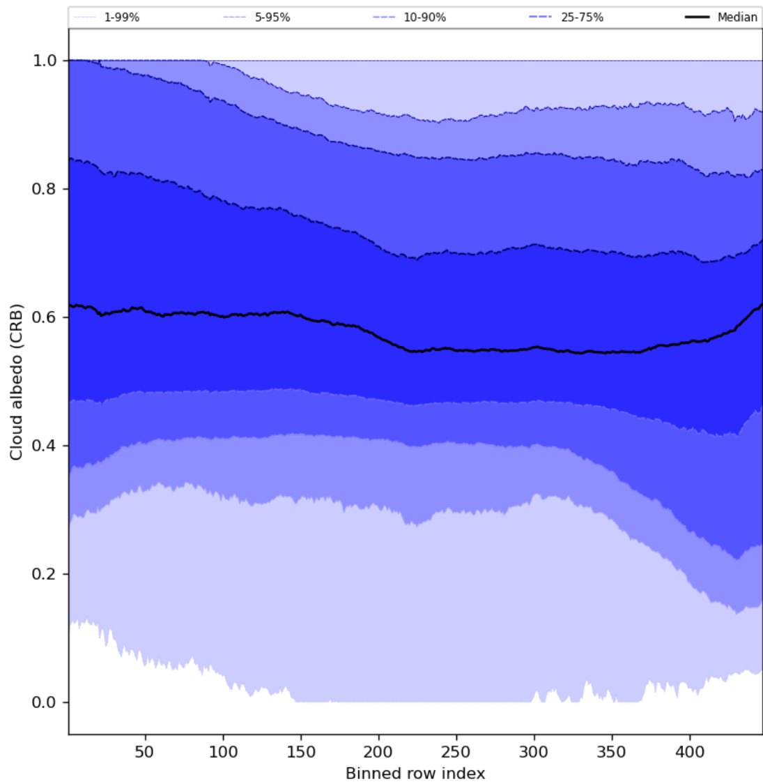
Figure 60: Along track statistics of “Cloud albedo (CRB)” for 2024-02-11 to 2024-02-13
