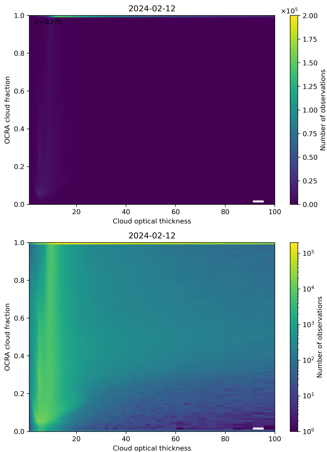
Figure 83: Scatter density plot of “Cloud optical thickness” against “OCRA cloud fraction” for 2024-02-11 to 2024-02-13.
