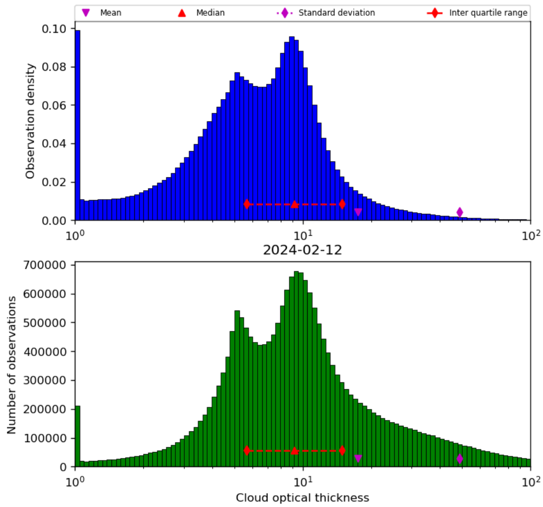
Figure 41: Histogram of “Cloud optical thickness” for 2024-02-11 to 2024-02-13
