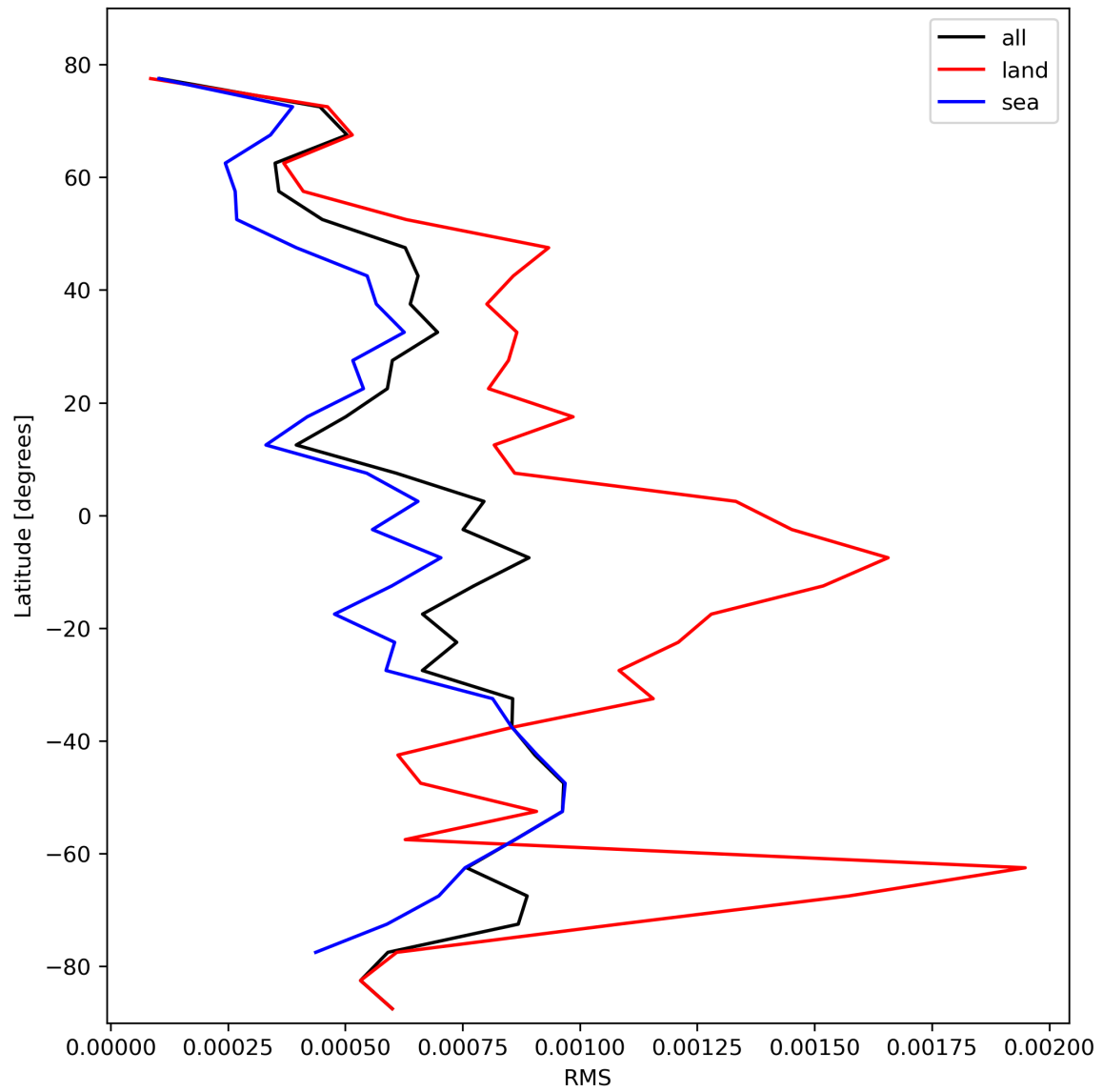
Figure 31: Zonal average of “RMS” for 2024-02-11 to 2024-02-13.
