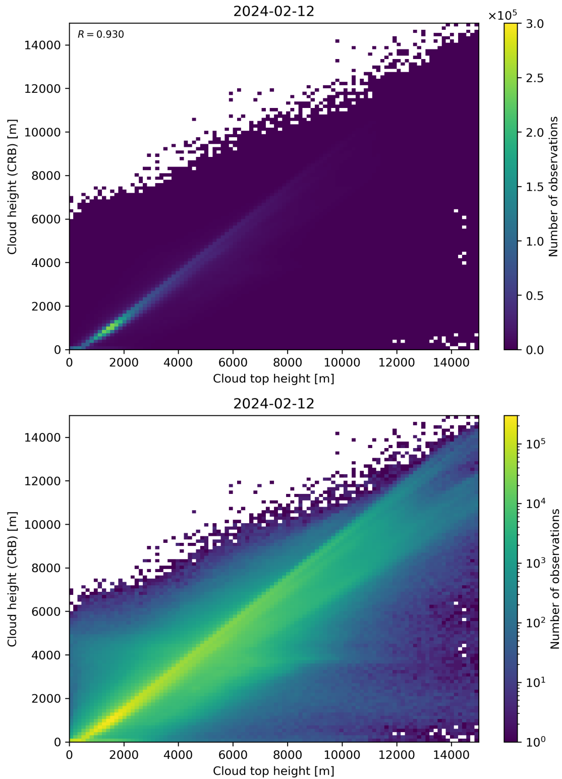
Figure 89: Scatter density plot of “Cloud top height” against “Cloud height (CRB)” for 2024-02-11 to 2024-02-13.
