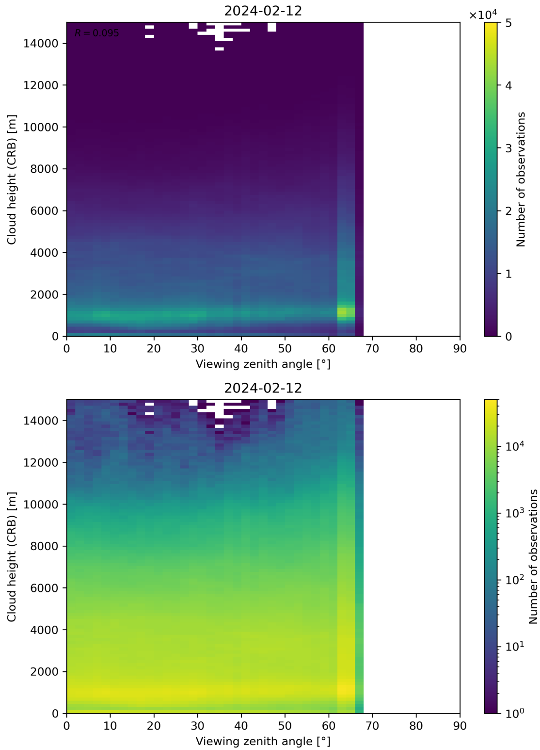
Figure 110: Scatter density plot of “Viewing zenith angle” against “Cloud height (CRB)” for 2024-02-11 to 2024-02-13.
