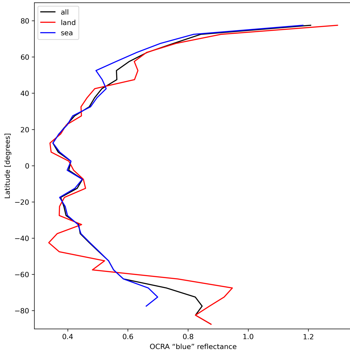
Figure 35: Zonal average of “OCRA “blue” reflectance” for 2024-02-11 to 2024-02-13.
