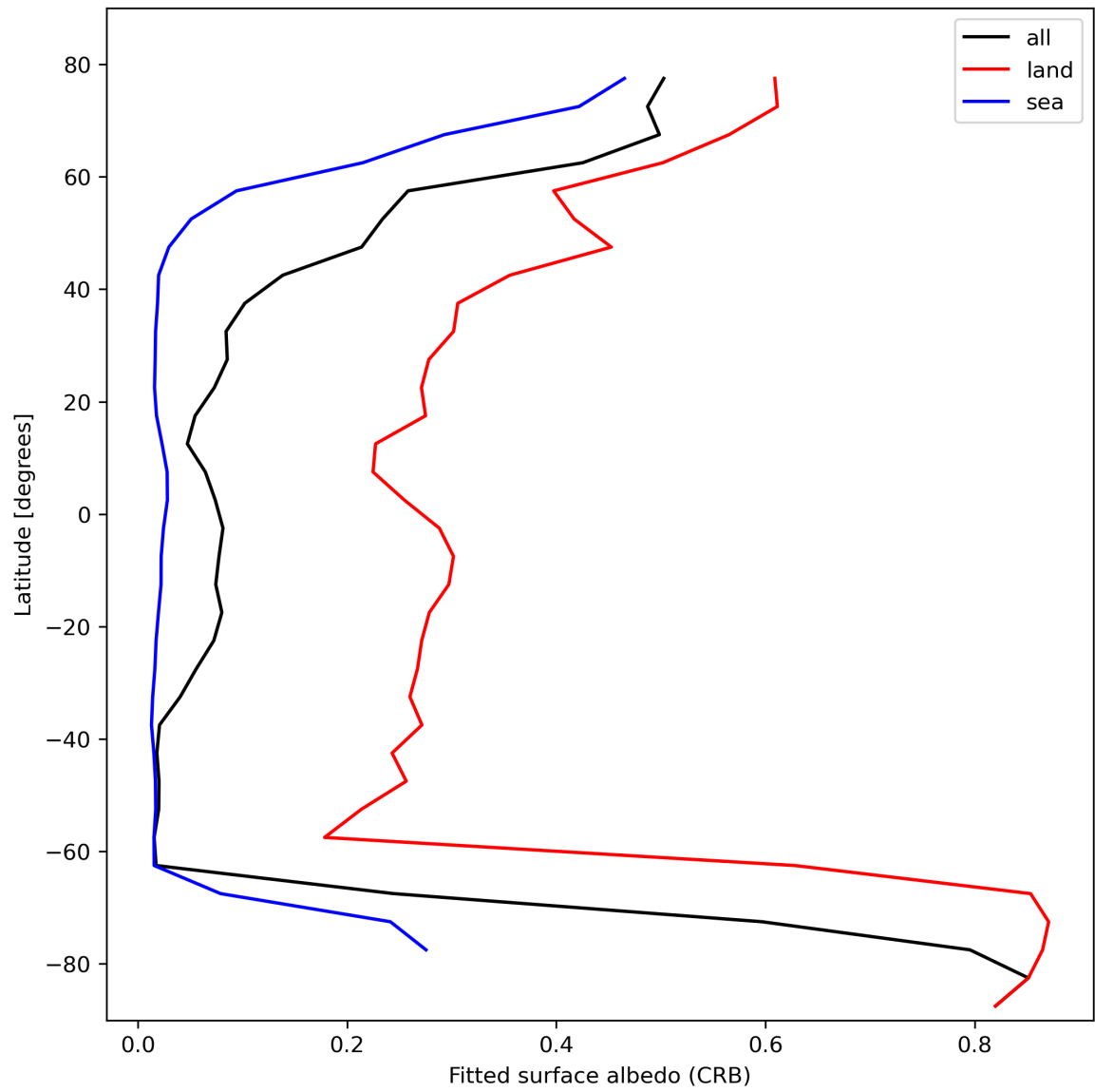
Figure 30: Zonal average of “Fitted surface albedo (CRB)” for 2024-02-11 to 2024-02-13.
