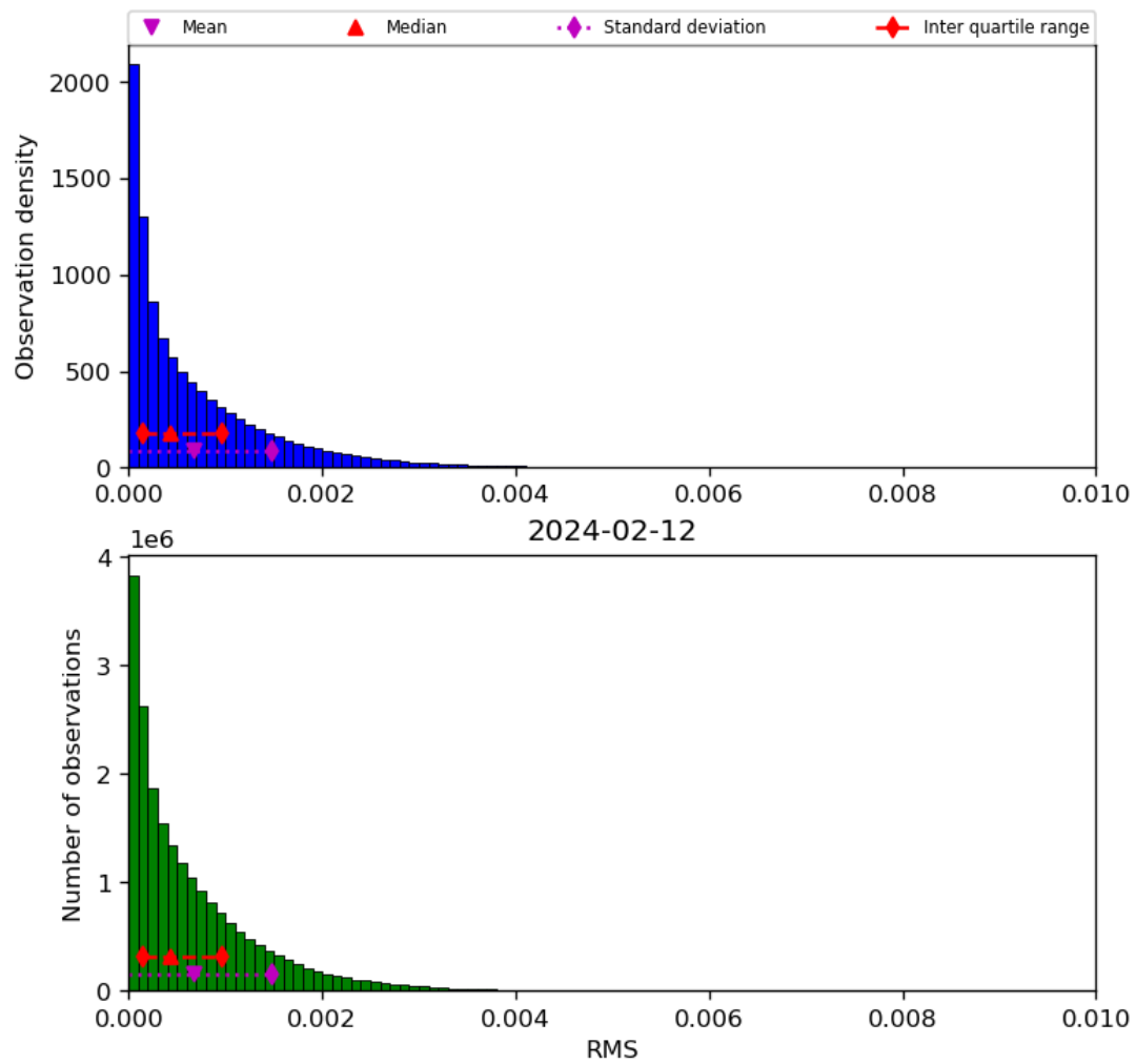
Figure 47: Histogram of “RMS” for 2024-02-11 to 2024-02-13
