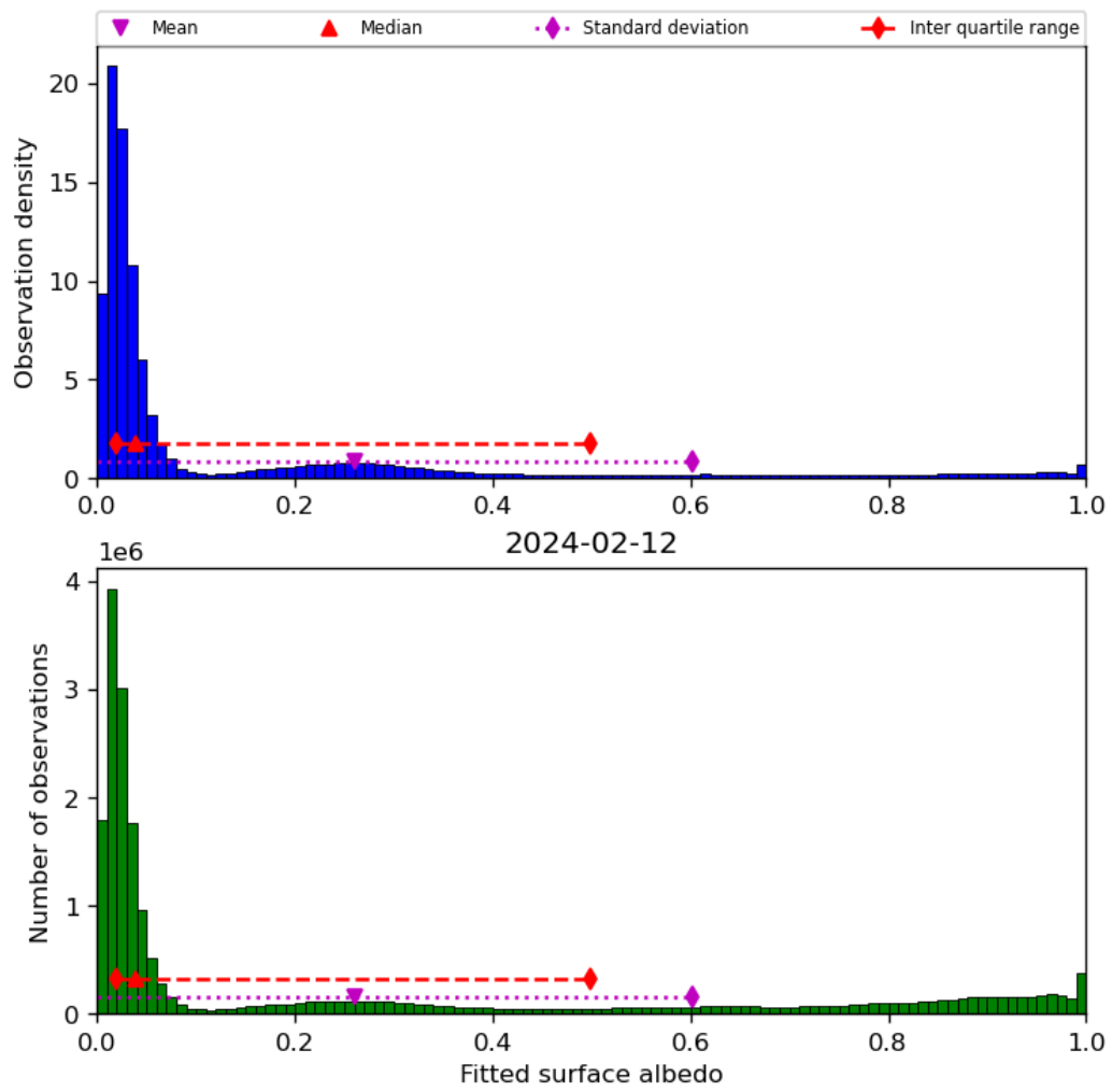
Figure 45: Histogram of “Fitted surface albedo” for 2024-02-11 to 2024-02-13
