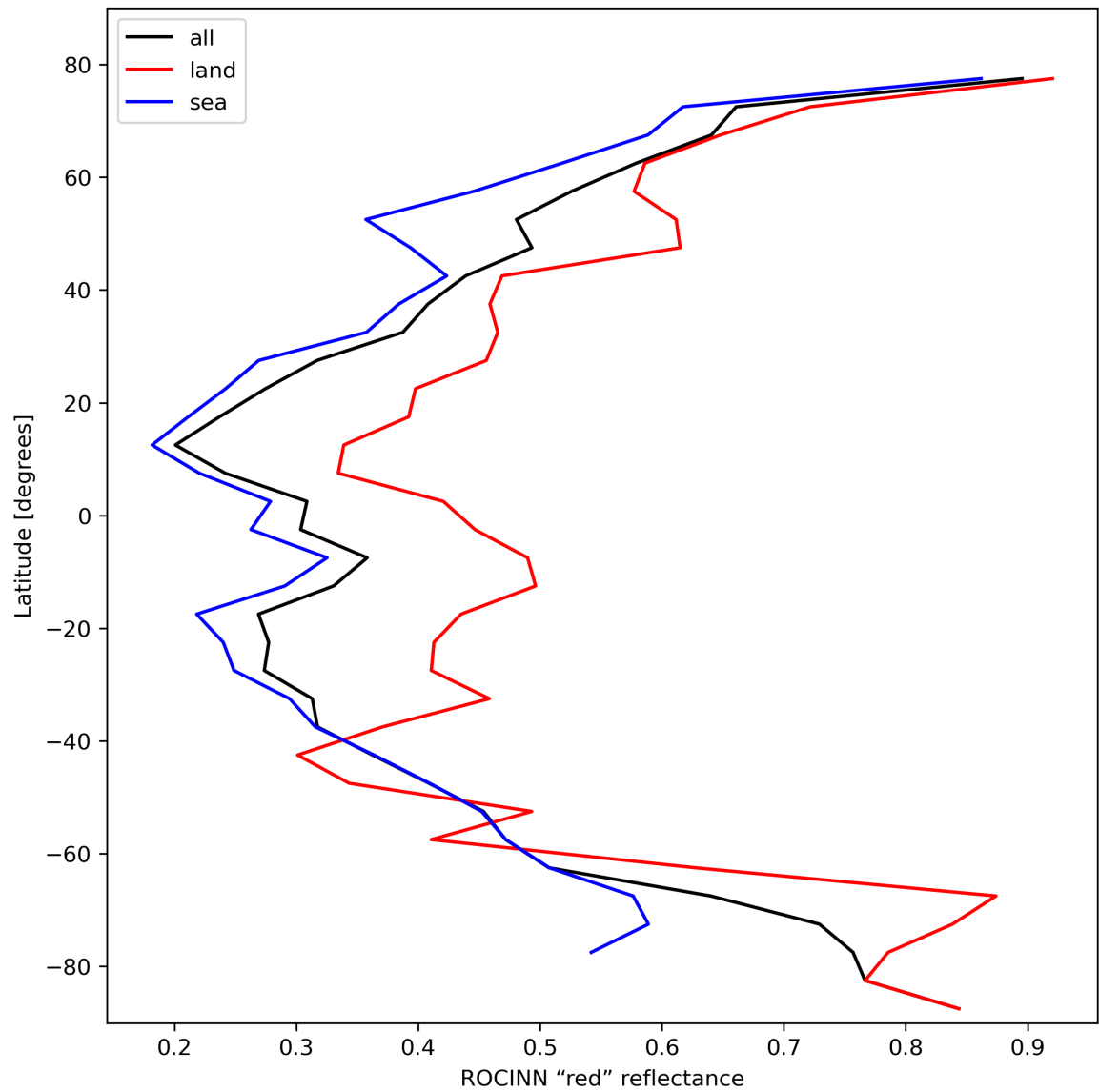
Figure 37: Zonal average of “ROCINN “red” reflectance” for 2024-02-11 to 2024-02-13.
