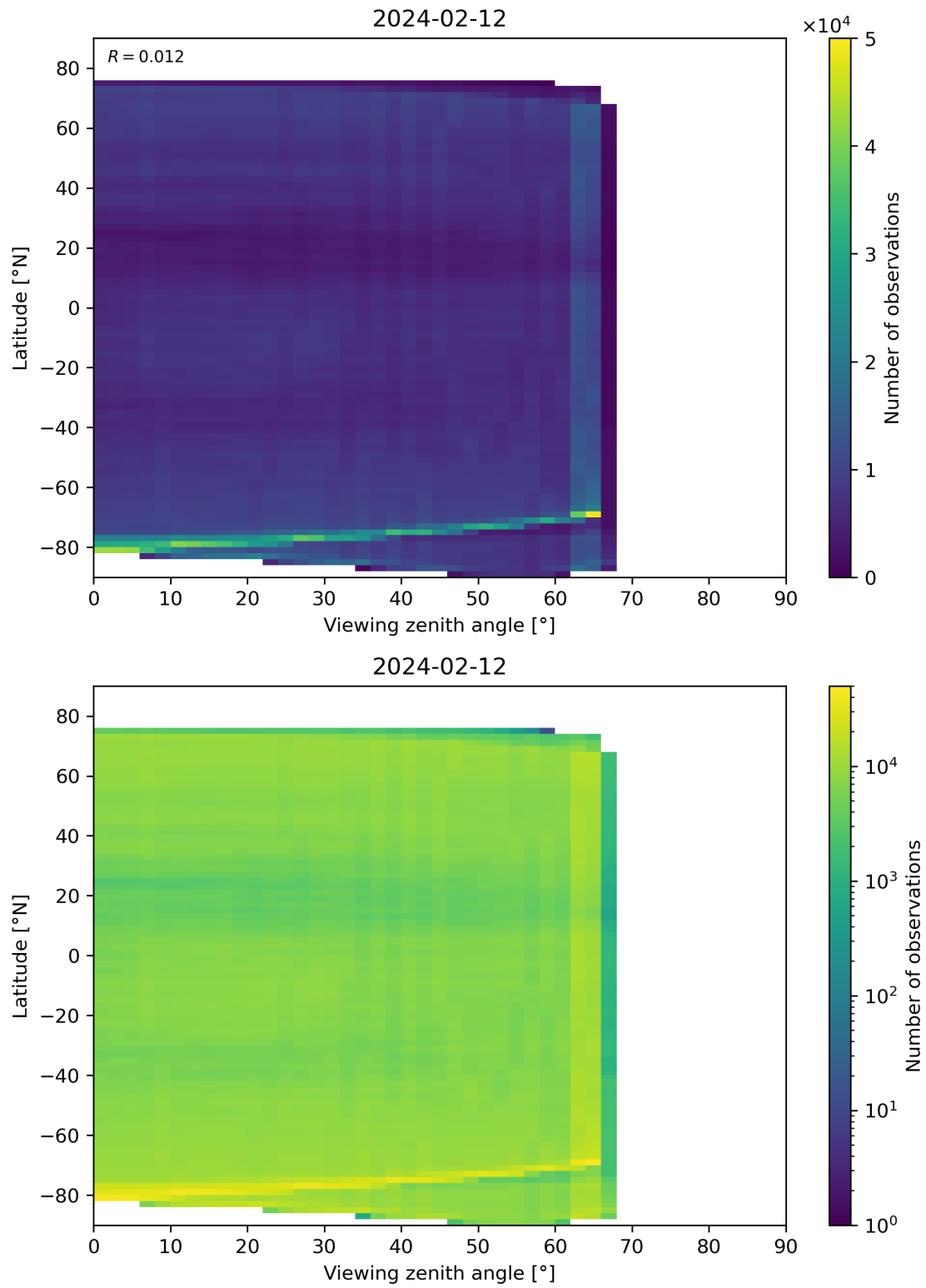
Figure 113: Scatter density plot of “Viewing zenith angle” against “Latitude” for 2024-02-11 to 2024-02-13.
