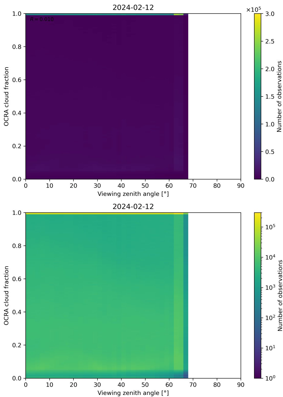
Figure 108: Scatter density plot of “Viewing zenith angle” against “OCRA cloud fraction” for 2024-02-11 to 2024-02-13.
