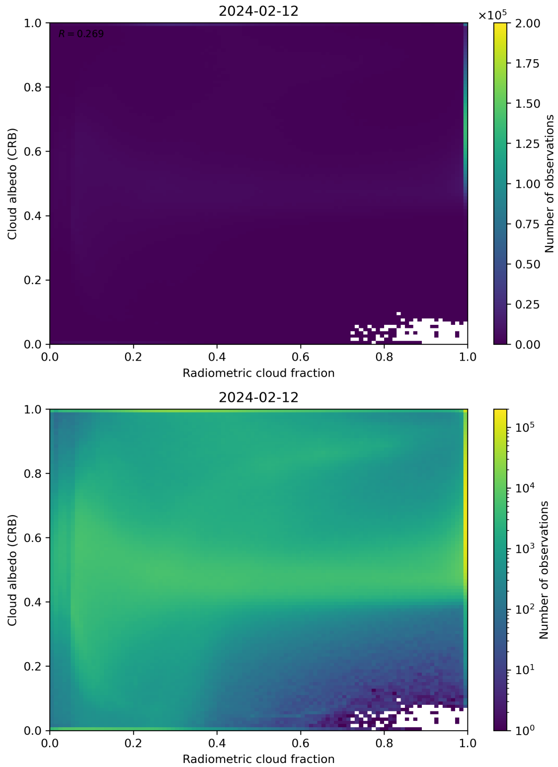
Figure 71: Scatter density plot of “Radiometric cloud fraction” against “Cloud albedo (CRB)” for 2024-02-11 to 2024-02-13.
