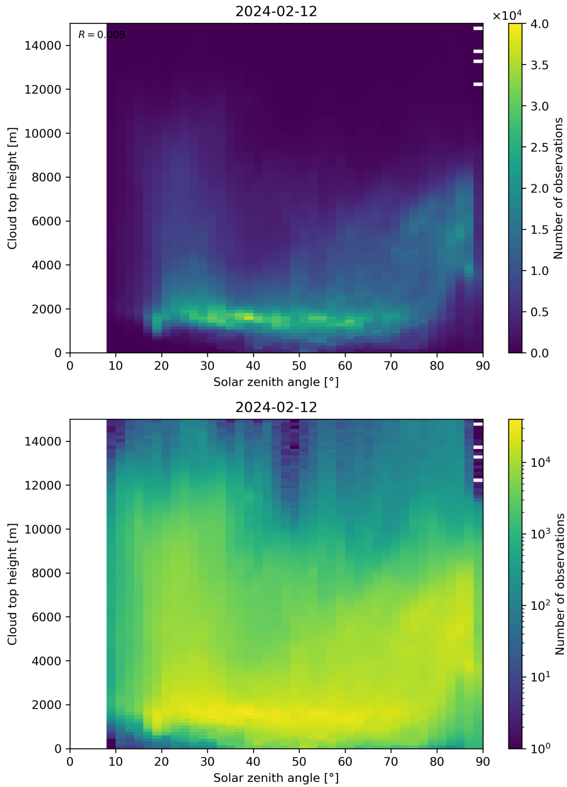
Figure 104: Scatter density plot of “Solar zenith angle” against “Cloud top height” for 2024-02-11 to 2024-02-13.
