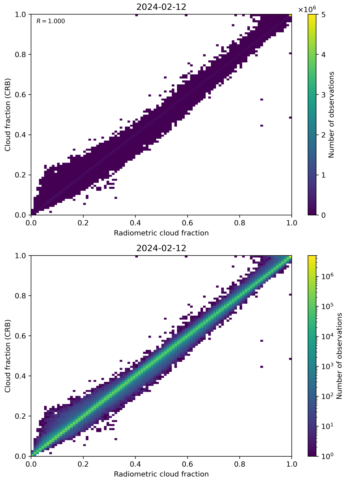
Figure 73: Scatter density plot of “Radiometric cloud fraction” against “Cloud fraction (CRB)” for 2024-02-11 to 2024-02-13.
