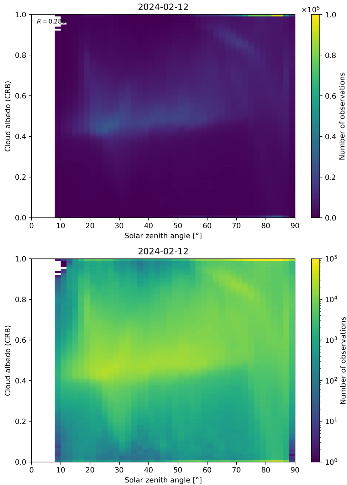
Figure 98: Scatter density plot of “Solar zenith angle” against “Cloud albedo (CRB)” for 2024-02-11 to 2024-02-13.
