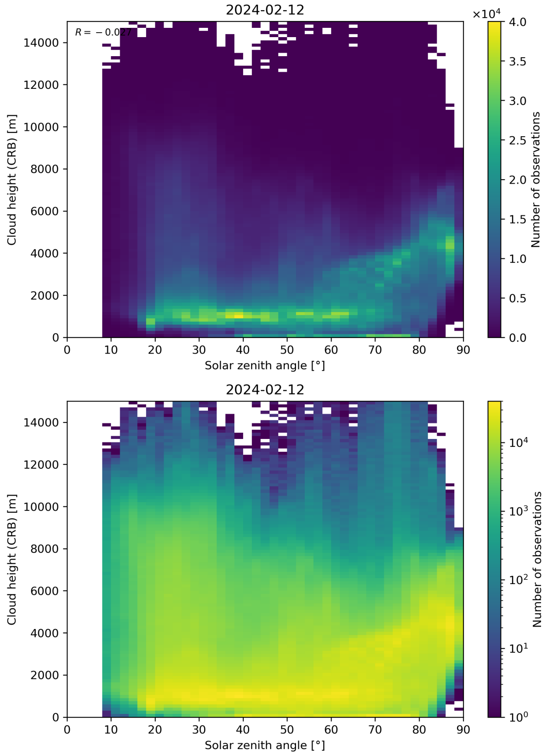
Figure 102: Scatter density plot of “Solar zenith angle” against “Cloud height (CRB)” for 2024-02-11 to 2024-02-13.
