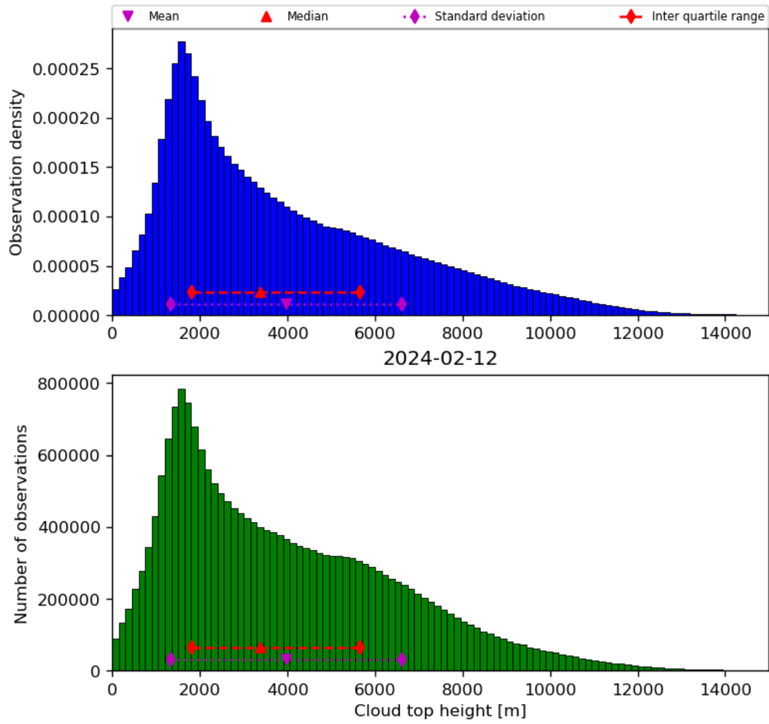
Figure 40: Histogram of “Cloud top height” for 2024-02-11 to 2024-02-13
