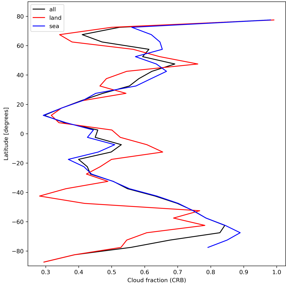
Figure 26: Zonal average of “Cloud fraction (CRB)” for 2024-02-11 to 2024-02-13.
