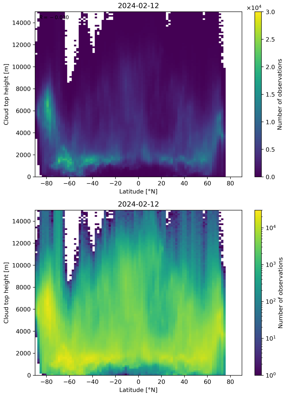
Figure 97: Scatter density plot of “Latitude” against “Cloud top height” for 2024-02-11 to 2024-02-13.
