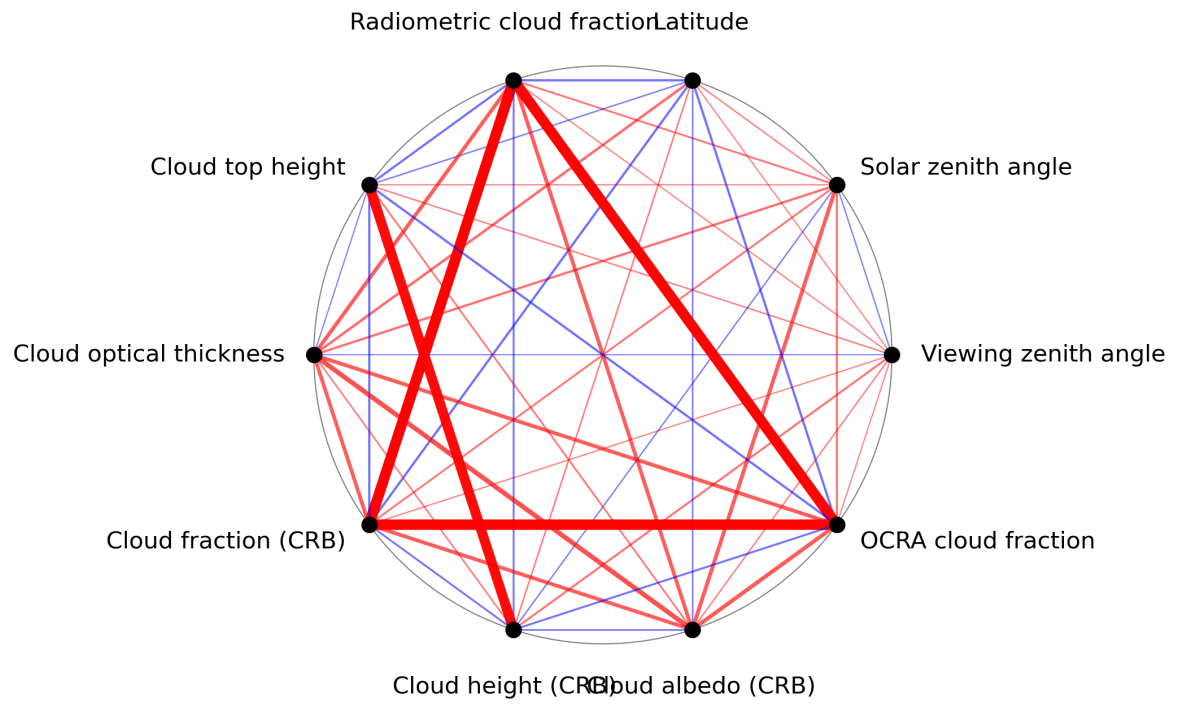
Figure 1: Map of correlation graph for 2024-02-11 to 2024-02-13.
