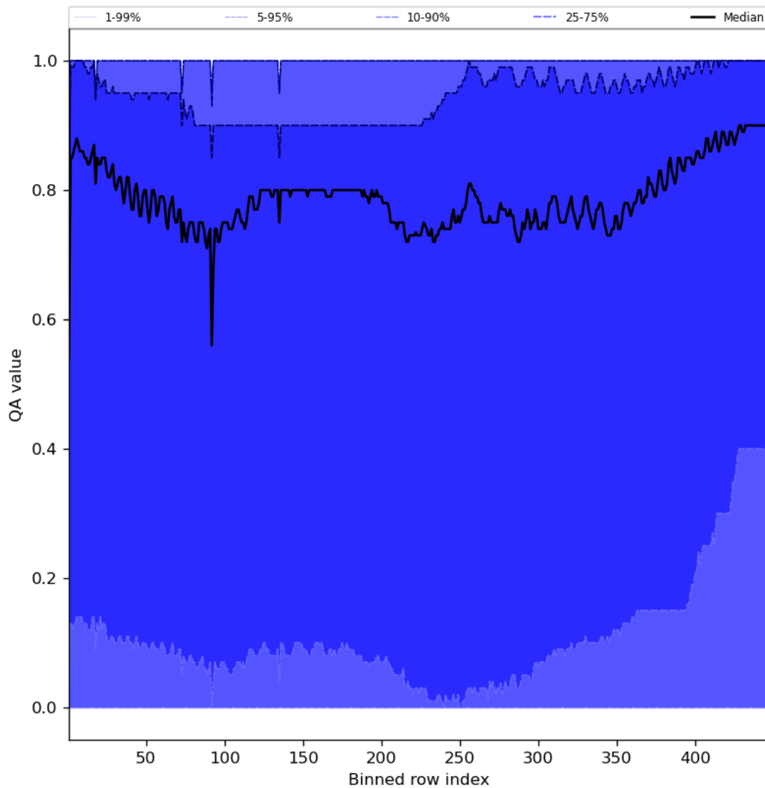
Figure 54: Along track statistics of “QA value” for 2024-02-11 to 2024-02-13
