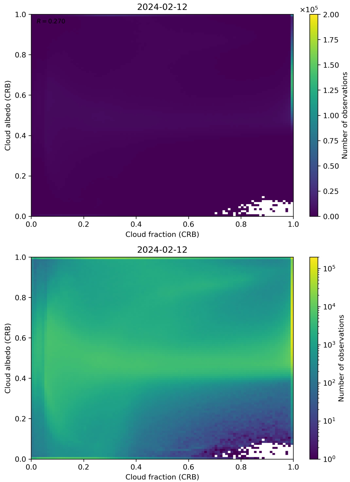
Figure 77: Scatter density plot of “Cloud fraction (CRB)” against “Cloud albedo (CRB)” for 2024-02-11 to 2024-02-13.
