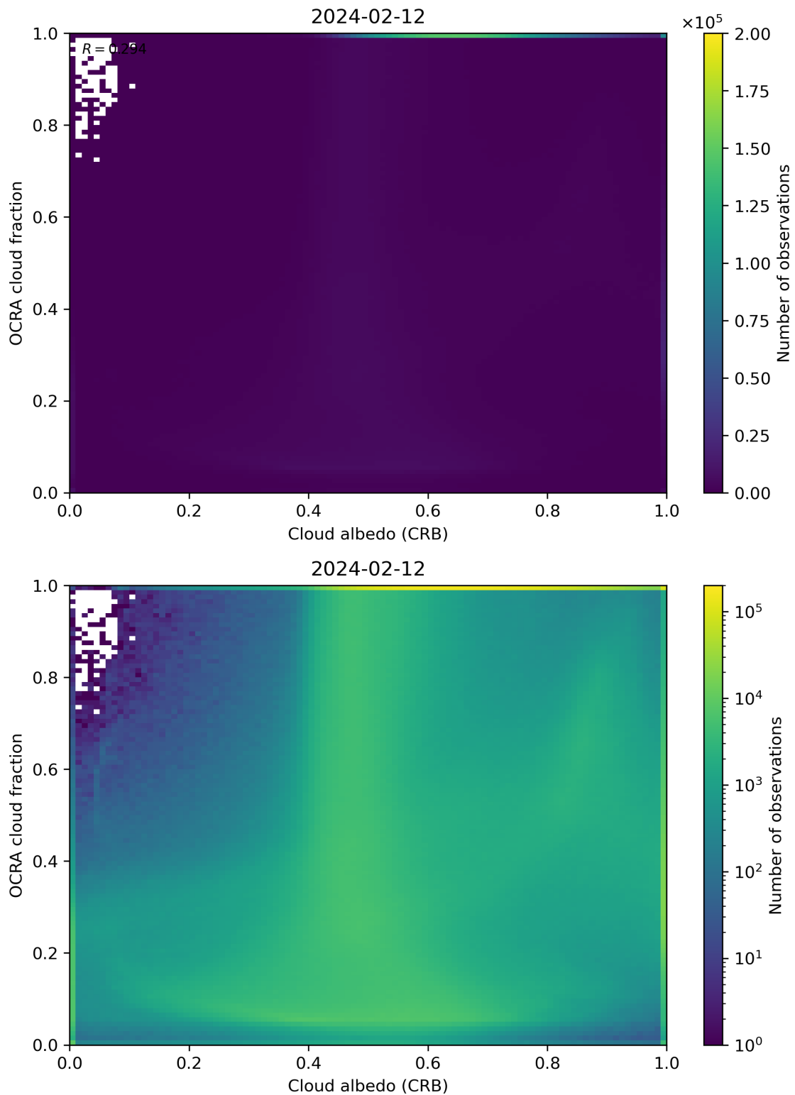
Figure 70: Scatter density plot of “Cloud albedo (CRB)” against “OCRA cloud fraction” for 2024-02-11 to 2024-02-13.
