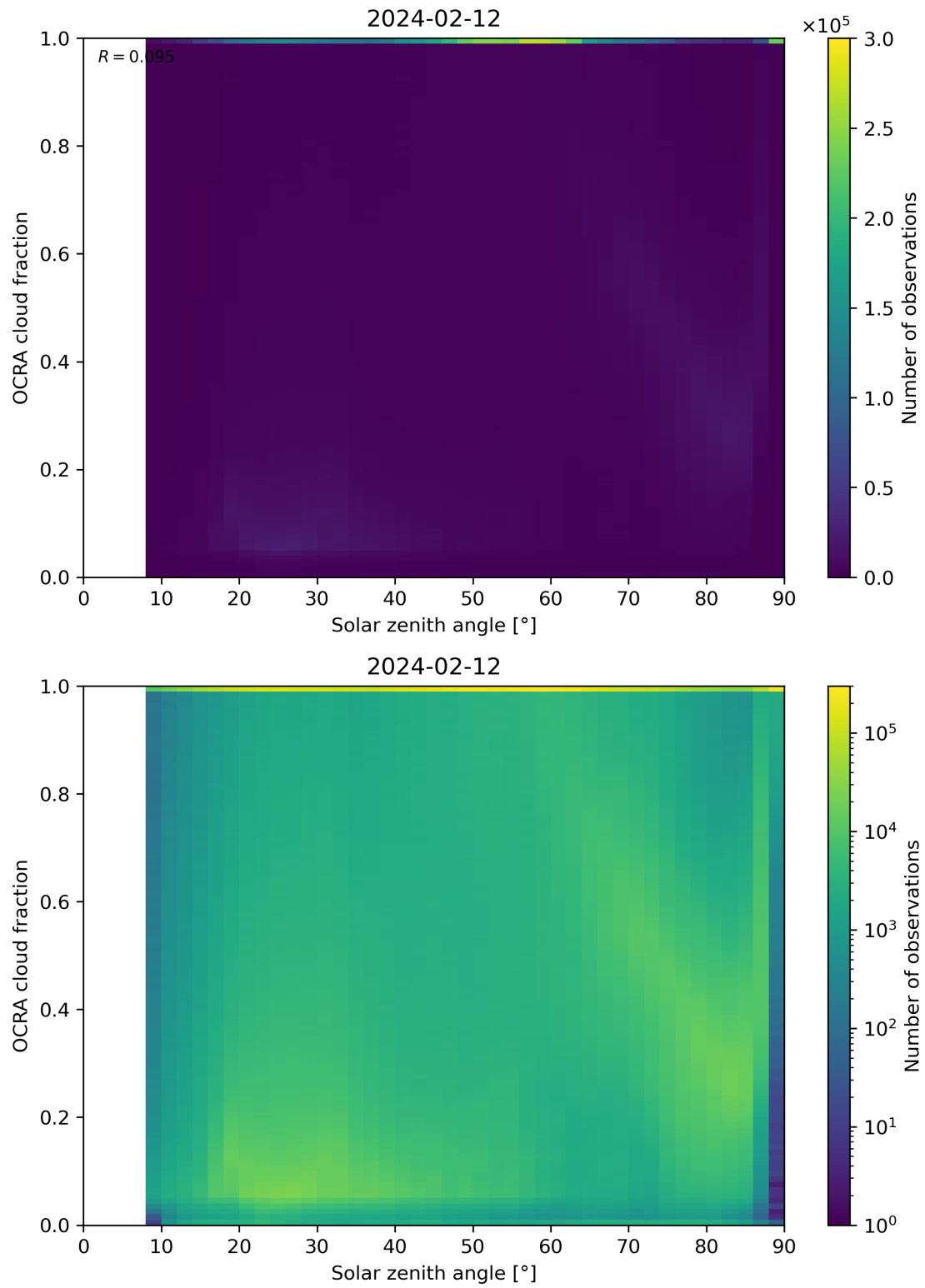
Figure 100: Scatter density plot of “Solar zenith angle” against “OCRA cloud fraction” for 2024-02-11 to 2024-02-13.
