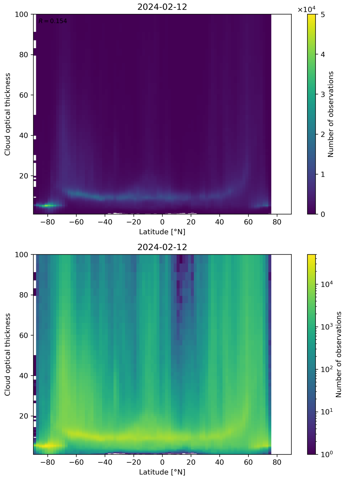
Figure 96: Scatter density plot of “Latitude” against “Cloud optical thickness” for 2024-02-11 to 2024-02-13.
