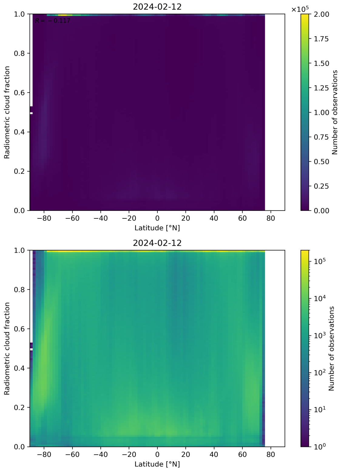
Figure 92: Scatter density plot of “Latitude” against “Radiometric cloud fraction” for 2024-02-11 to 2024-02-13.
