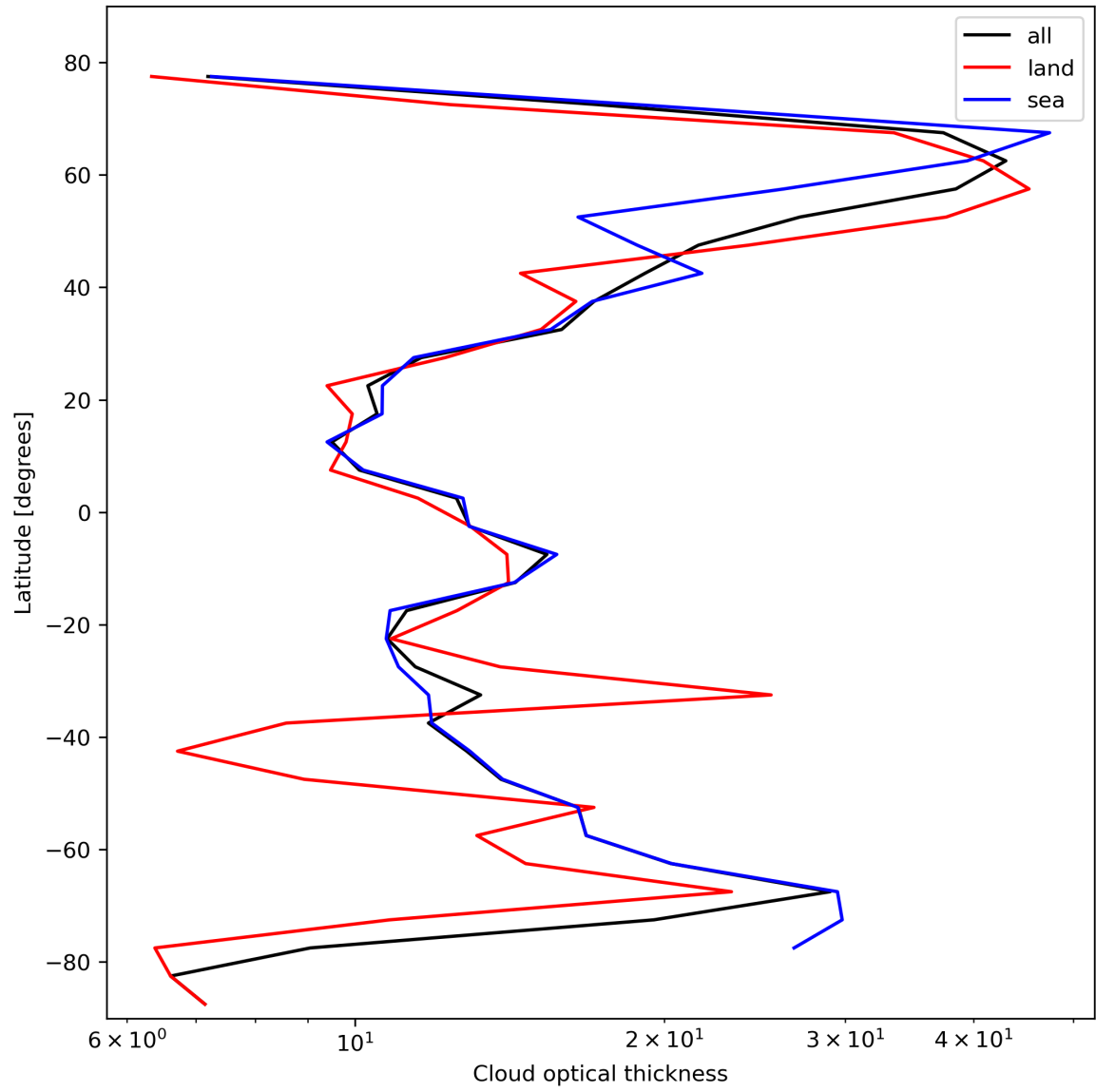
Figure 25: Zonal average of “Cloud optical thickness” for 2024-02-11 to 2024-02-13.
