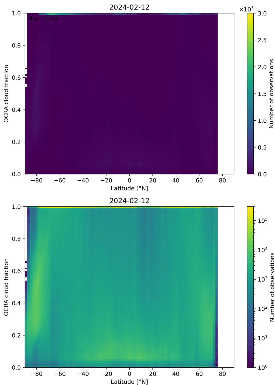
Figure 93: Scatter density plot of “Latitude” against “OCRA cloud fraction” for 2024-02-11 to 2024-02-13.
