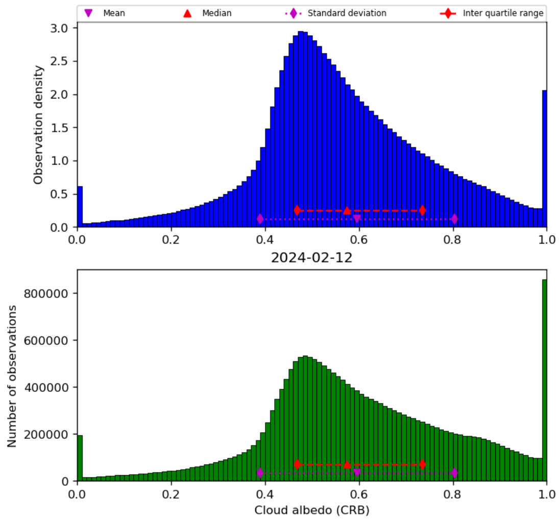
Figure 44: Histogram of “Cloud albedo (CRB)” for 2024-02-11 to 2024-02-13
