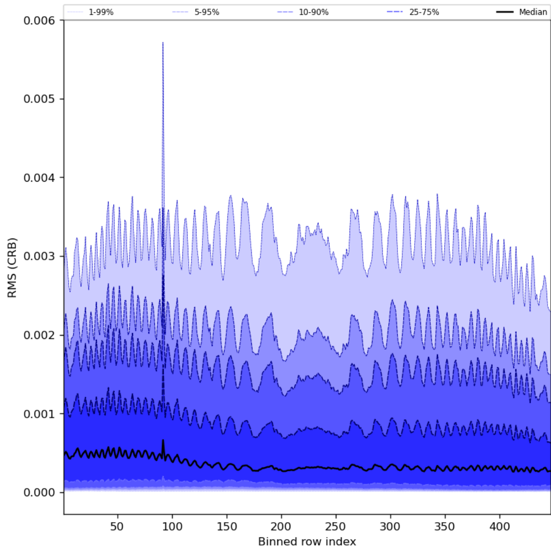
Figure 64: Along track statistics of “RMS (CRB)” for 2024-02-11 to 2024-02-13
