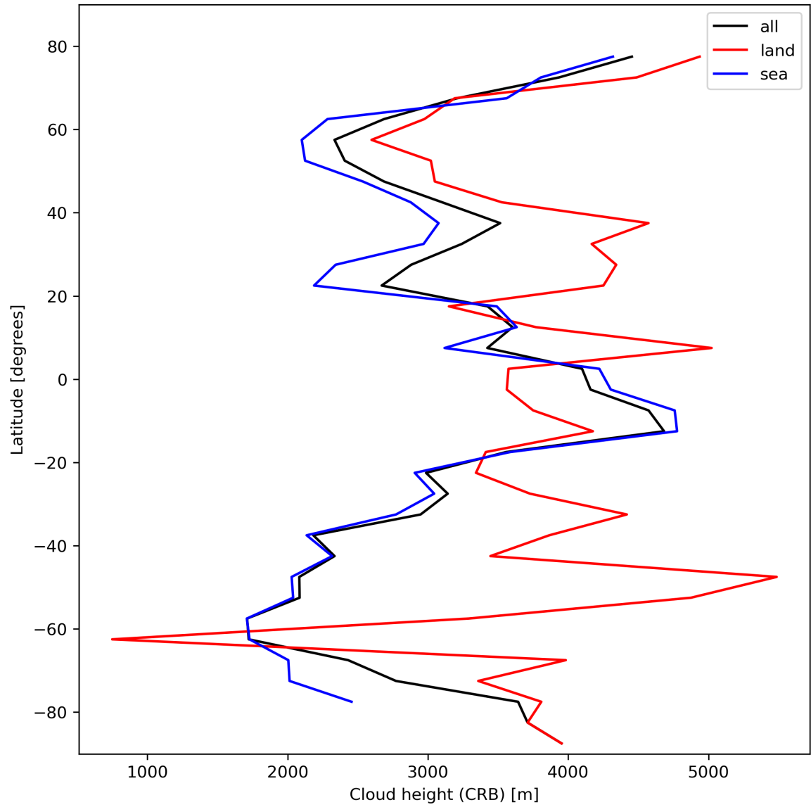
Figure 27: Zonal average of “Cloud height (CRB)” for 2024-02-11 to 2024-02-13.
