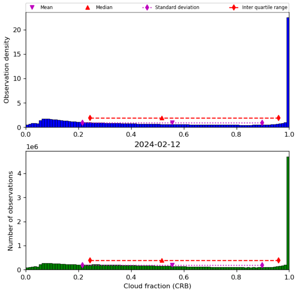
Figure 42: Histogram of “Cloud fraction (CRB)” for 2024-02-11 to 2024-02-13
