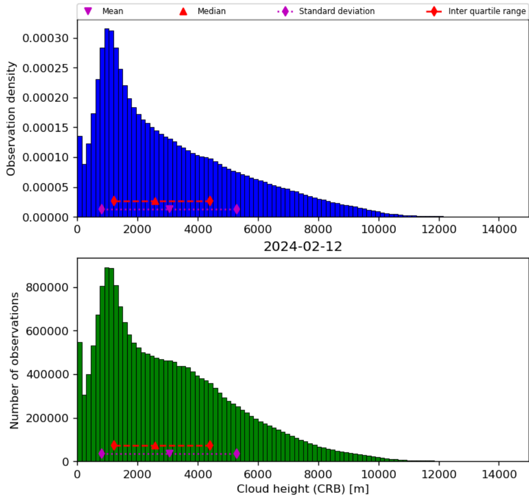
Figure 43: Histogram of “Cloud height (CRB)” for 2024-02-11 to 2024-02-13
