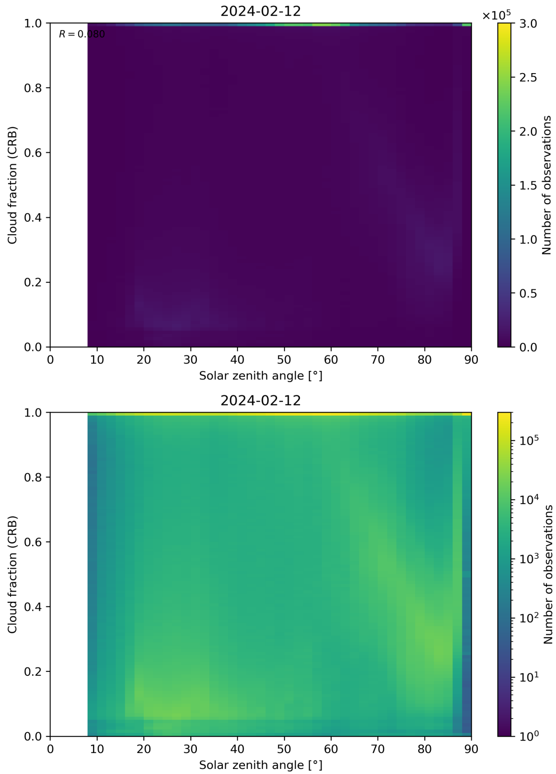
Figure 101: Scatter density plot of “Solar zenith angle” against “Cloud fraction (CRB)” for 2024-02-11 to 2024-02-13.
