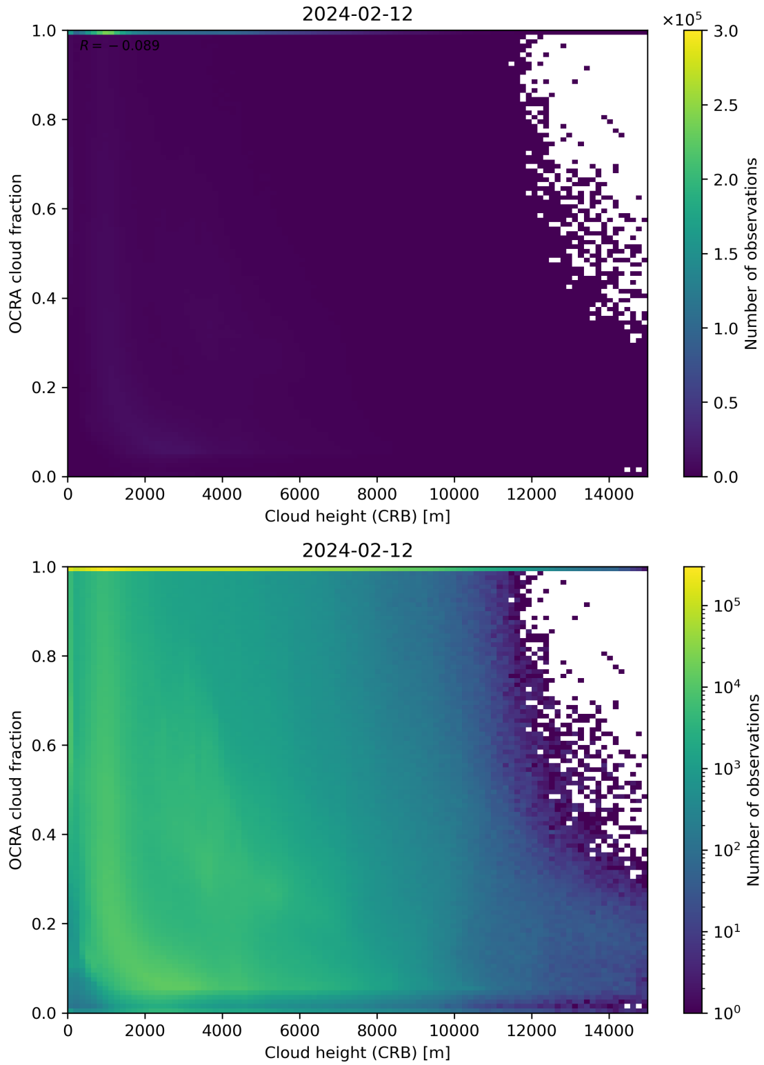
Figure 81: Scatter density plot of “Cloud height (CRB)” against “OCRA cloud fraction” for 2024-02-11 to 2024-02-13.
