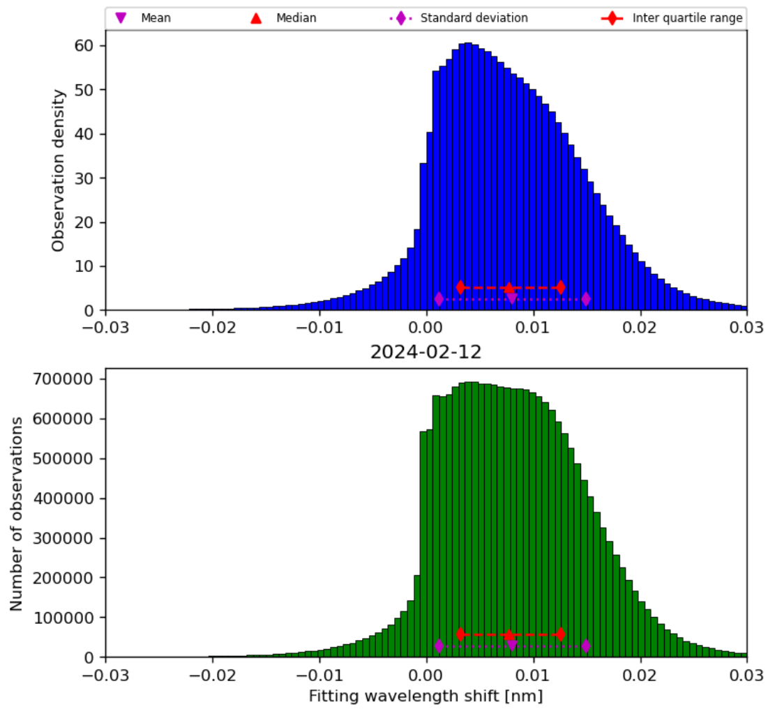
Figure 49: Histogram of “Fitting wavelength shift” for 2024-02-11 to 2024-02-13
