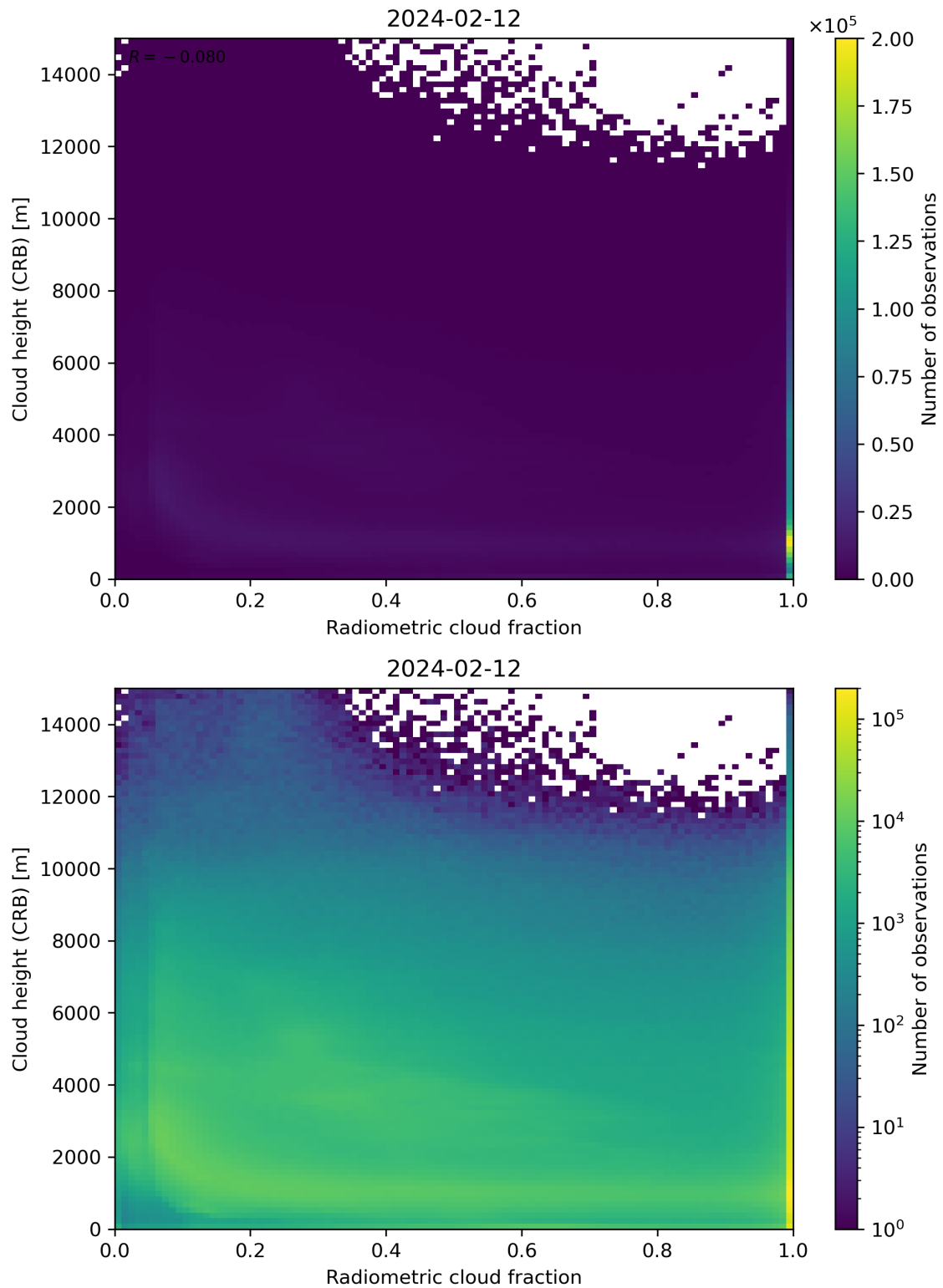
Figure 74: Scatter density plot of “Radiometric cloud fraction” against “Cloud height (CRB)” for 2024-02-11 to 2024-02-13.
