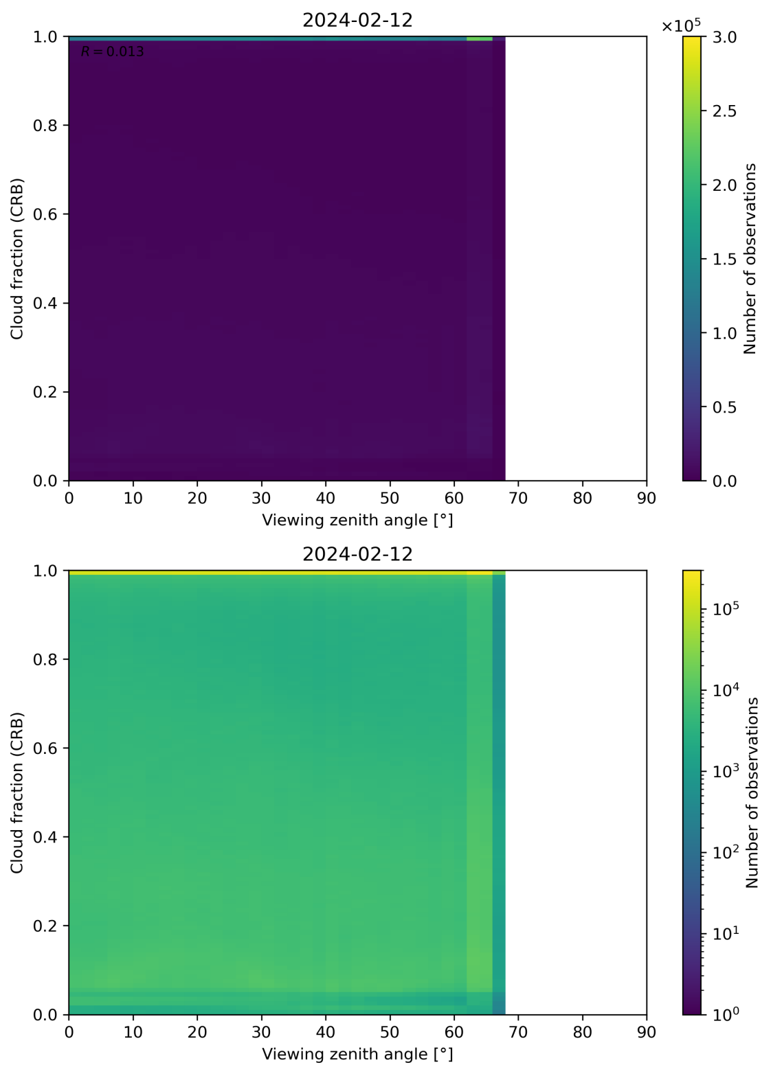
Figure 109: Scatter density plot of “Viewing zenith angle” against “Cloud fraction (CRB)” for 2024-02-11 to 2024-02-13.
