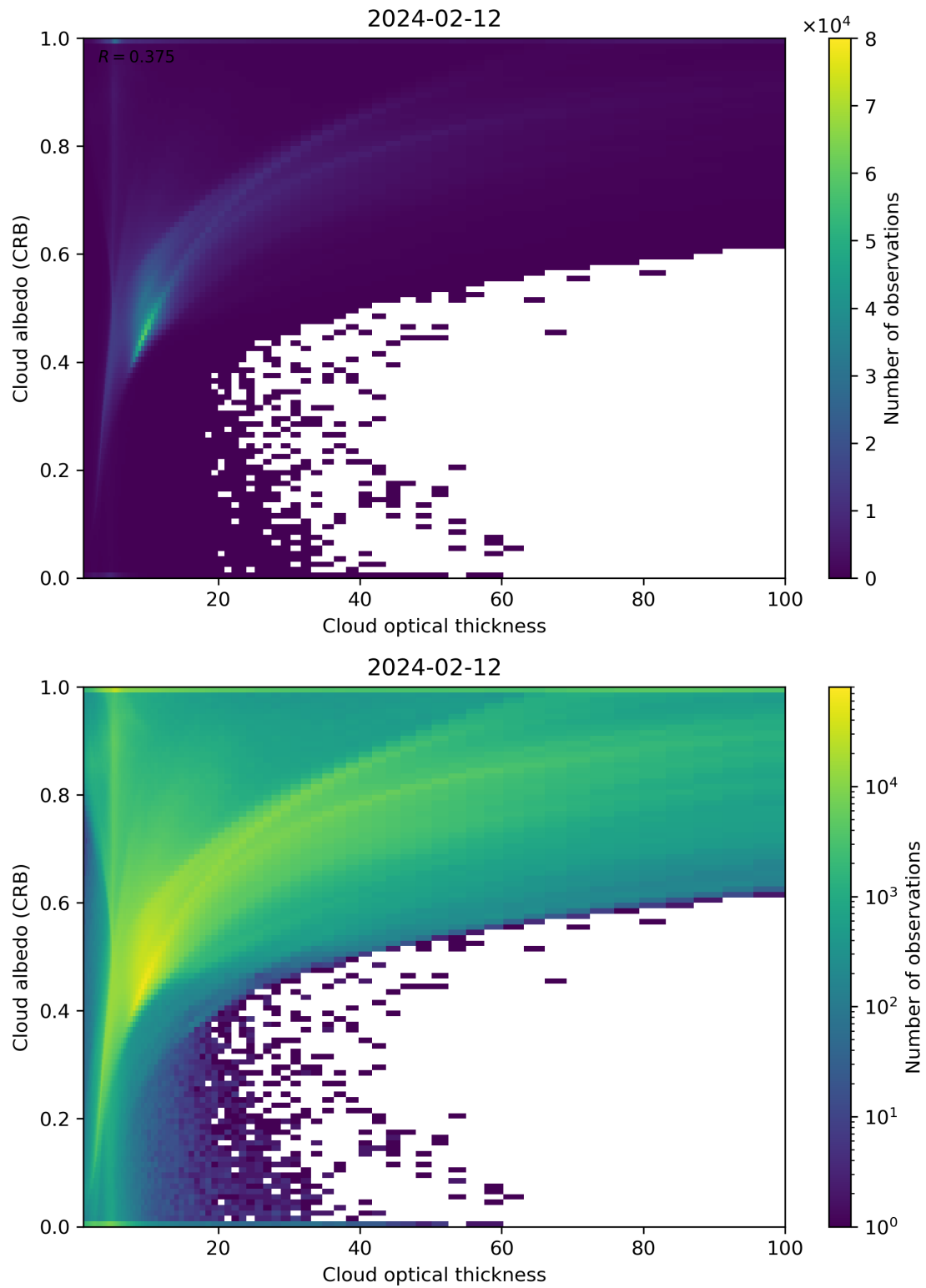
Figure 82: Scatter density plot of “Cloud optical thickness” against “Cloud albedo (CRB)” for 2024-02-11 to 2024-02-13.
