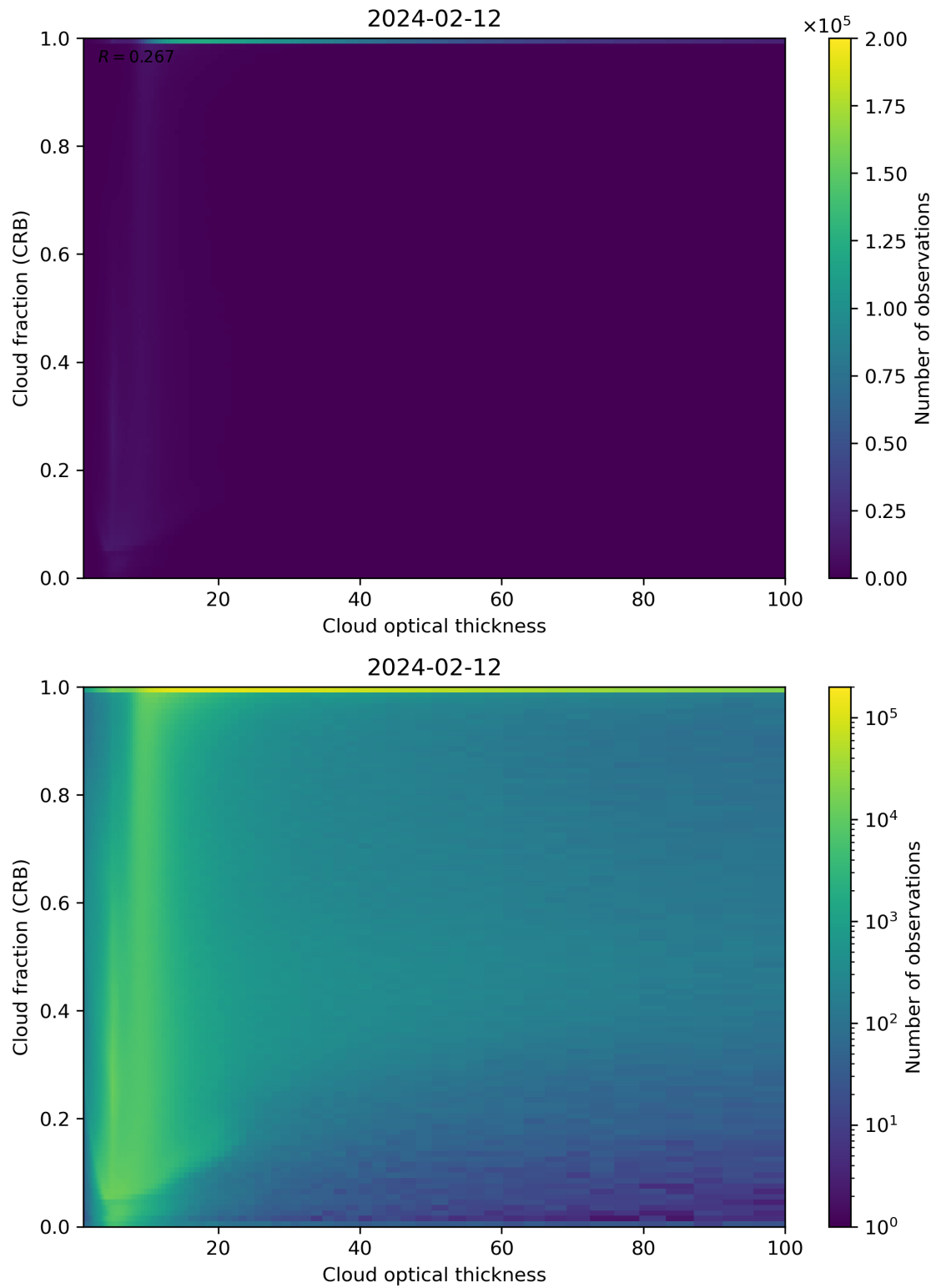
Figure 84: Scatter density plot of “Cloud optical thickness” against “Cloud fraction (CRB)” for 2024-02-11 to 2024-02-13.
