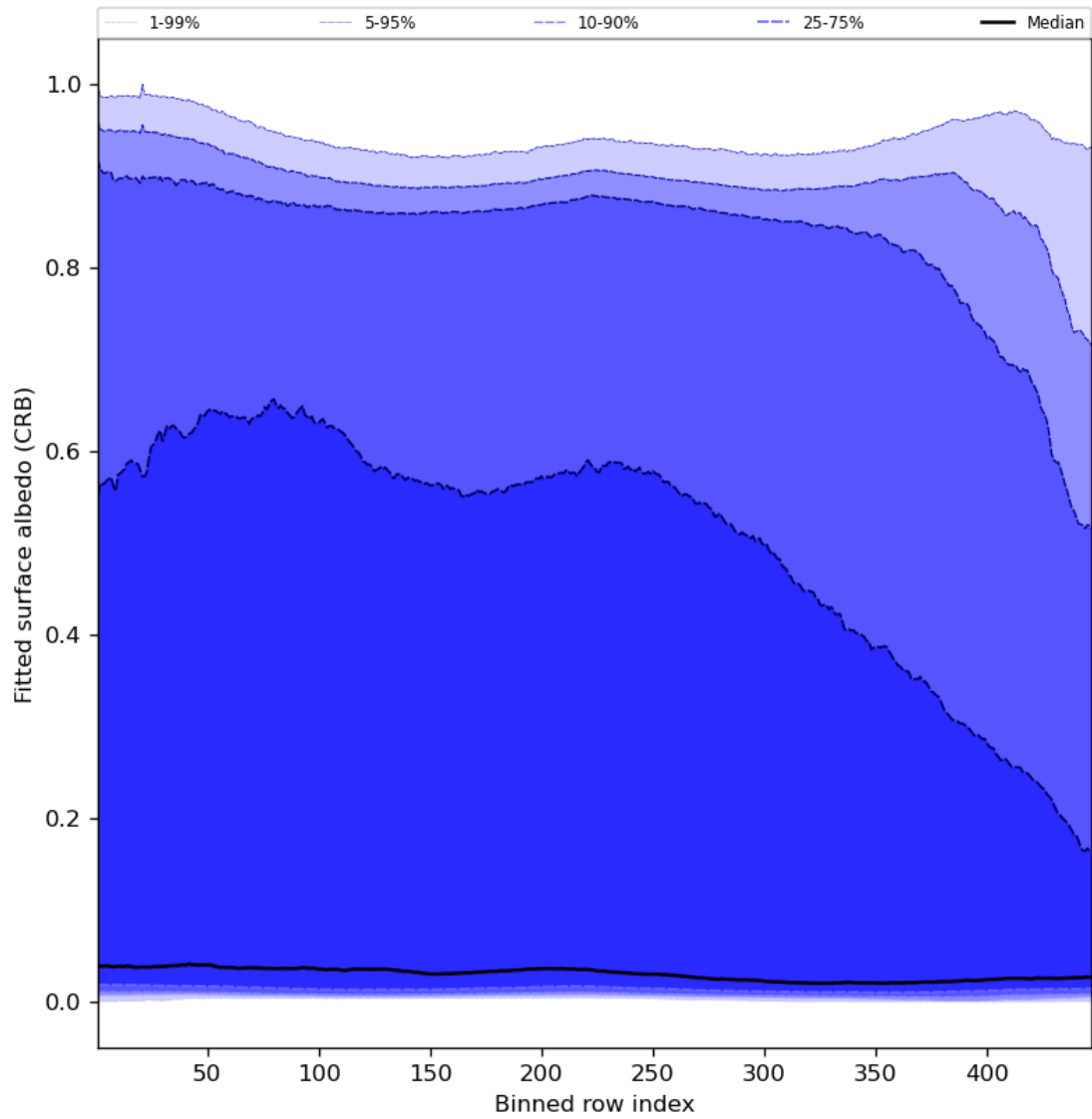
Figure 62: Along track statistics of “Fitted surface albedo (CRB)” for 2024-02-11 to 2024-02-13
