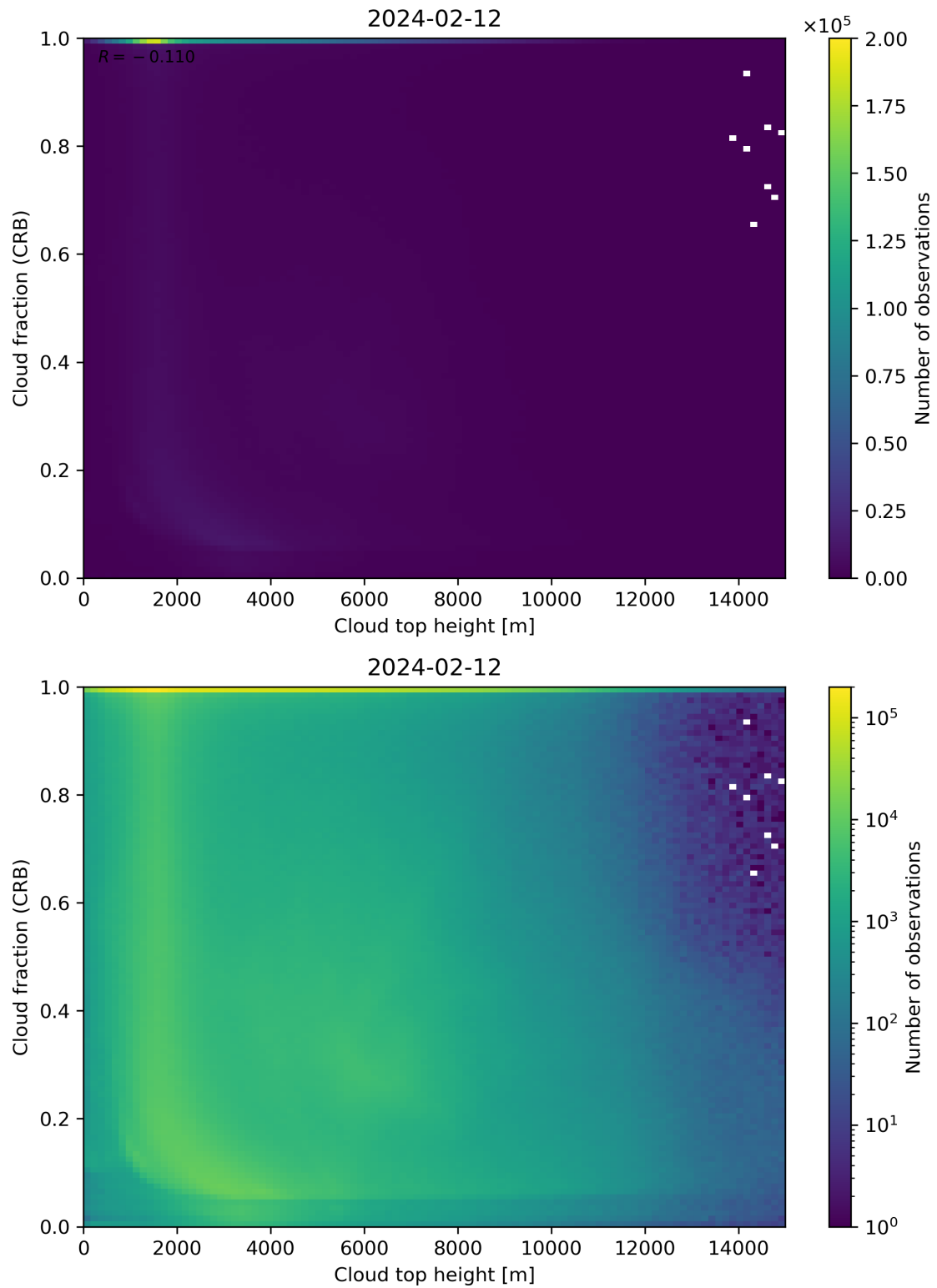
Figure 88: Scatter density plot of “Cloud top height” against “Cloud fraction (CRB)” for 2024-02-11 to 2024-02-13.
