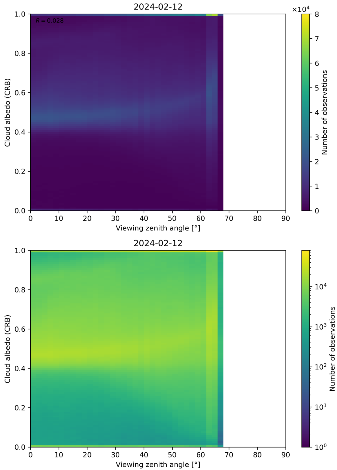
Figure 106: Scatter density plot of “Viewing zenith angle” against “Cloud albedo (CRB)” for 2024-02-11 to 2024-02-13.
