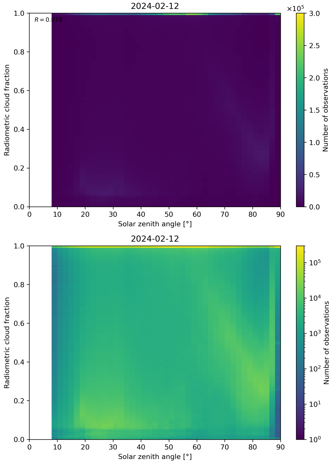
Figure 99: Scatter density plot of “Solar zenith angle” against “Radiometric cloud fraction” for 2024-02-11 to 2024-02-13.
