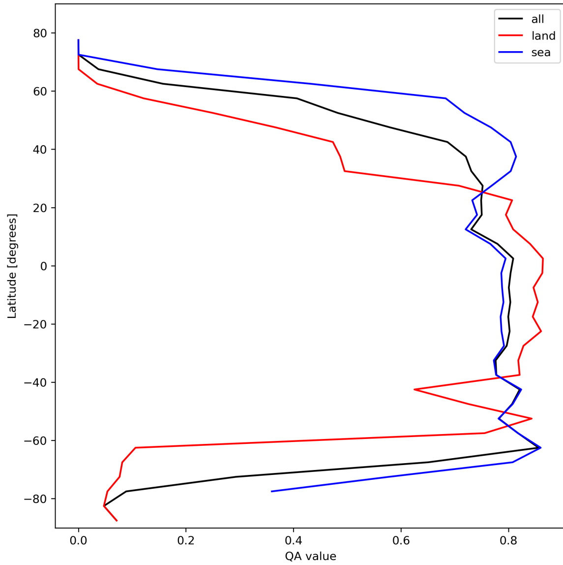
Figure 22: Zonal average of “QA value” for 2024-02-11 to 2024-02-13.
