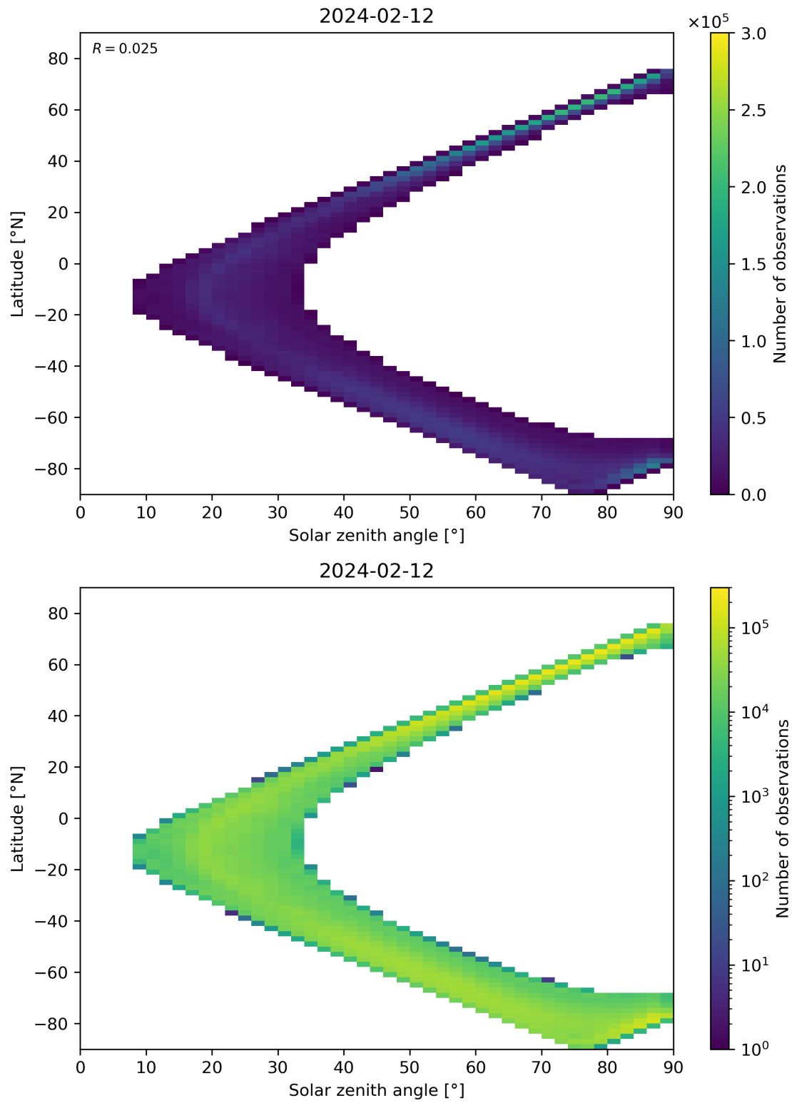
Figure 105: Scatter density plot of “Solar zenith angle” against “Latitude” for 2024-02-11 to 2024-02-13.
