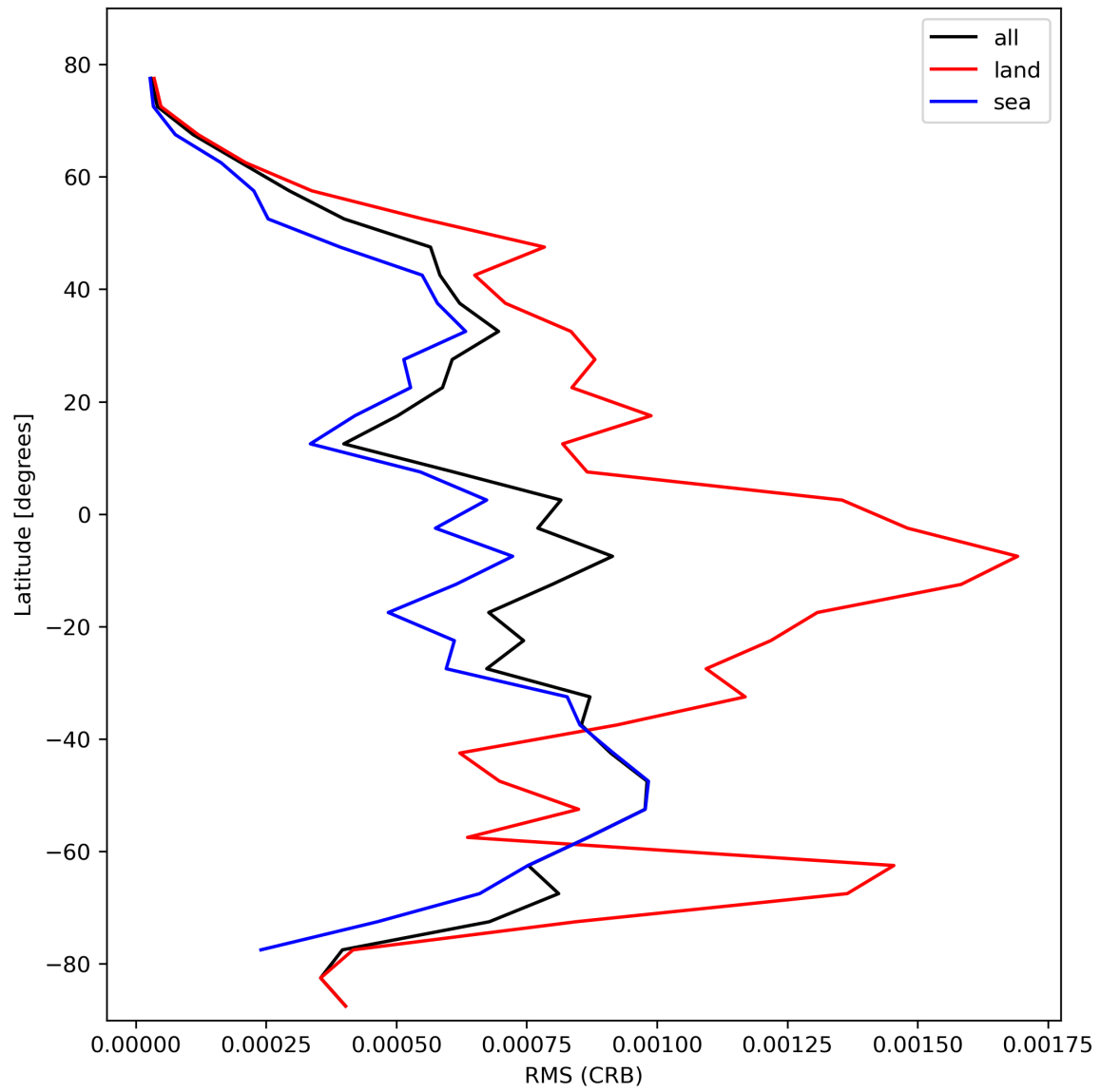
Figure 32: Zonal average of “RMS (CRB)” for 2024-02-11 to 2024-02-13.
