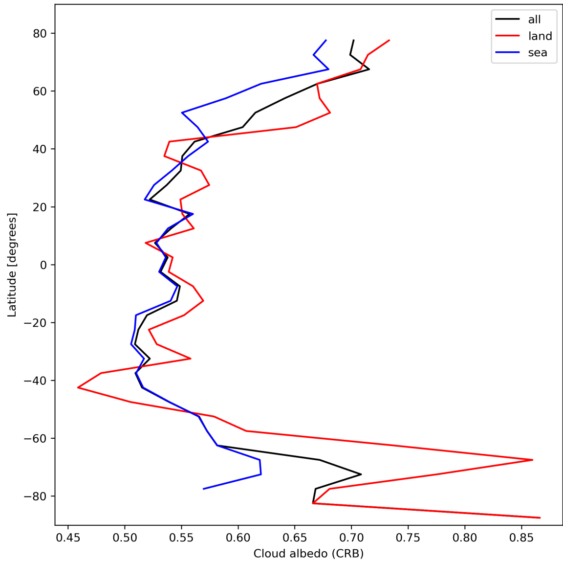
Figure 28: Zonal average of “Cloud albedo (CRB)” for 2024-02-11 to 2024-02-13.
