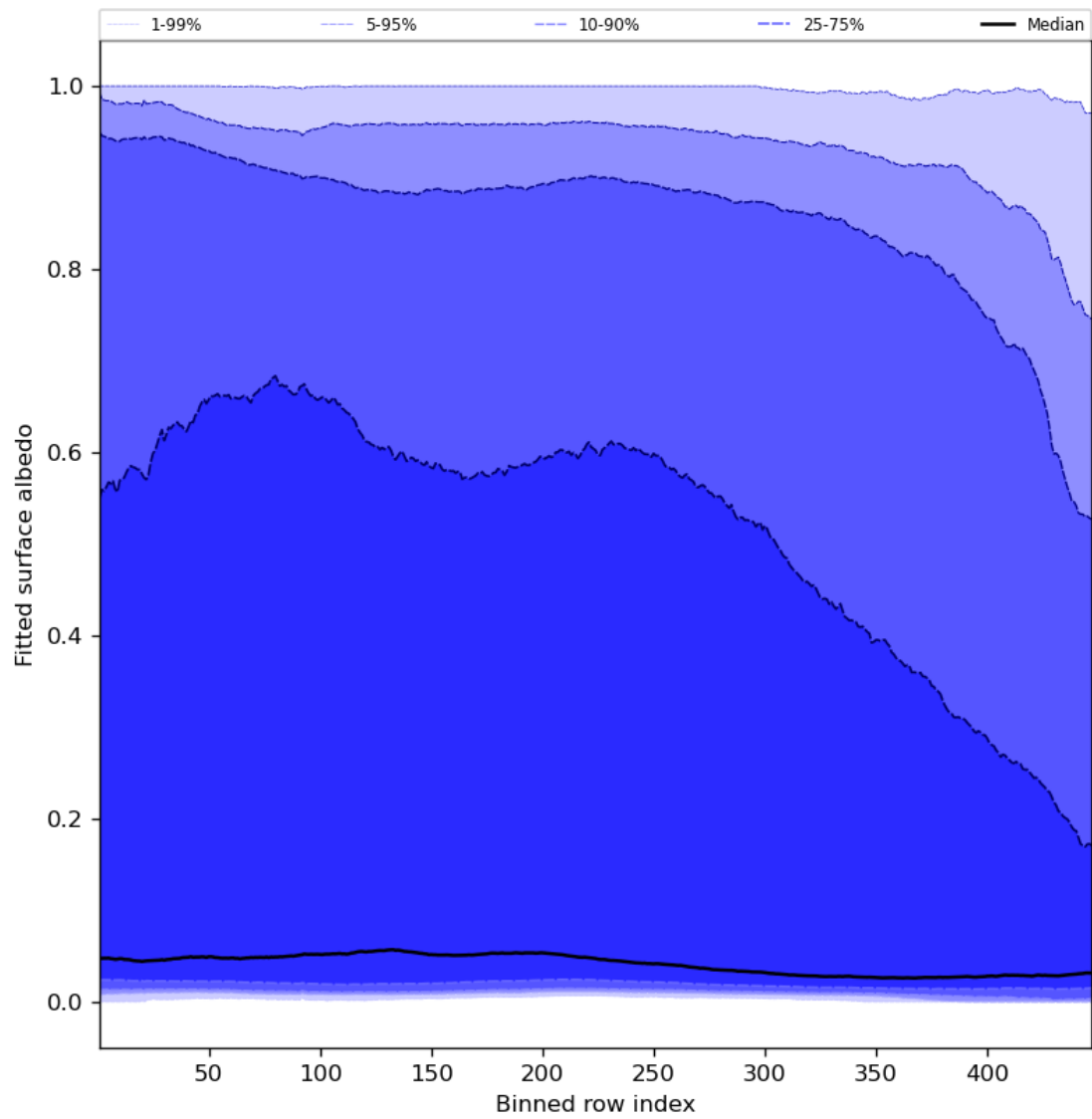
Figure 61: Along track statistics of “Fitted surface albedo” for 2024-02-11 to 2024-02-13
