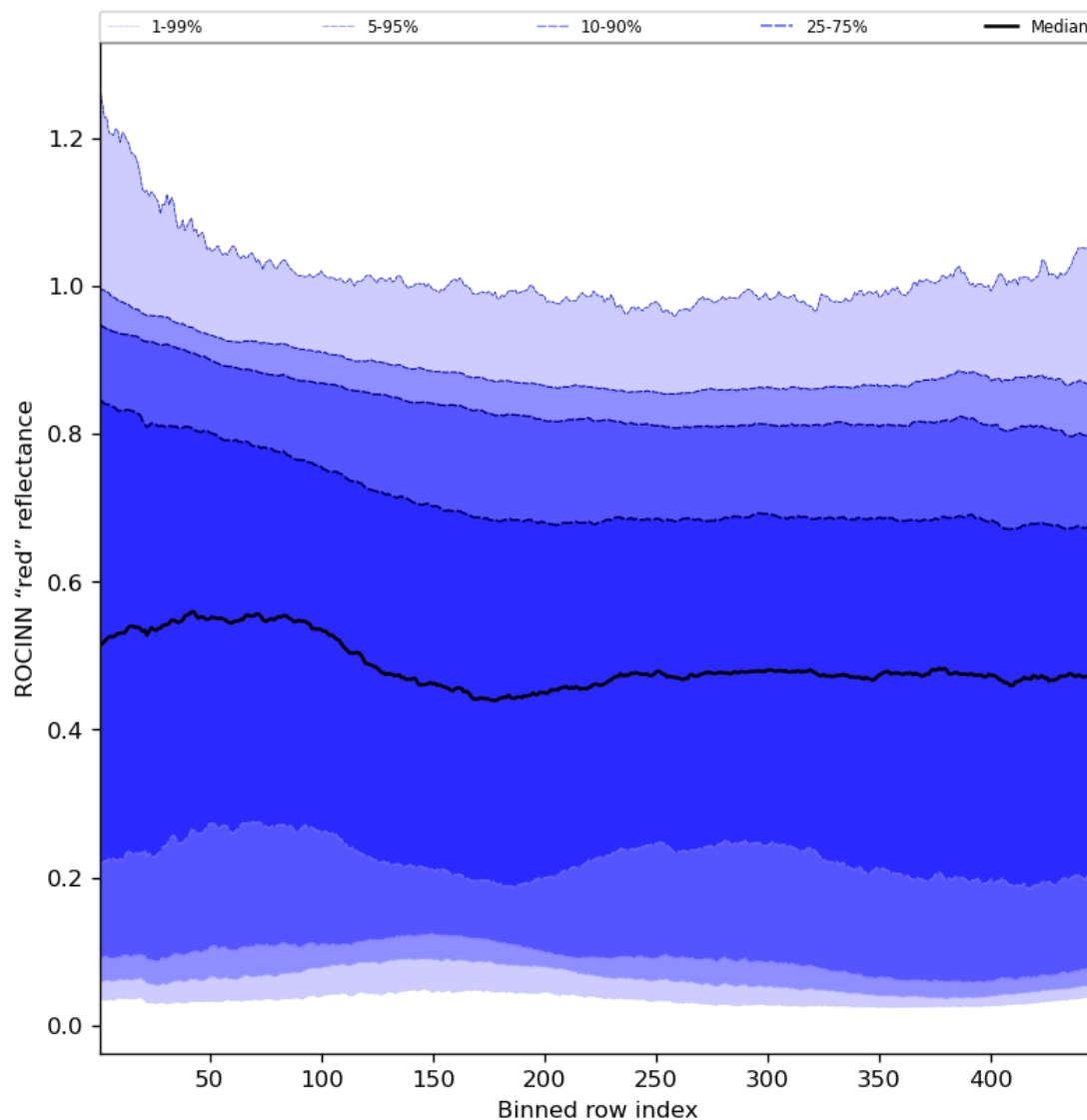
Figure 69: Along track statistics of “ROCINN “red” reflectance” for 2024-02-11 to 2024-02-13
