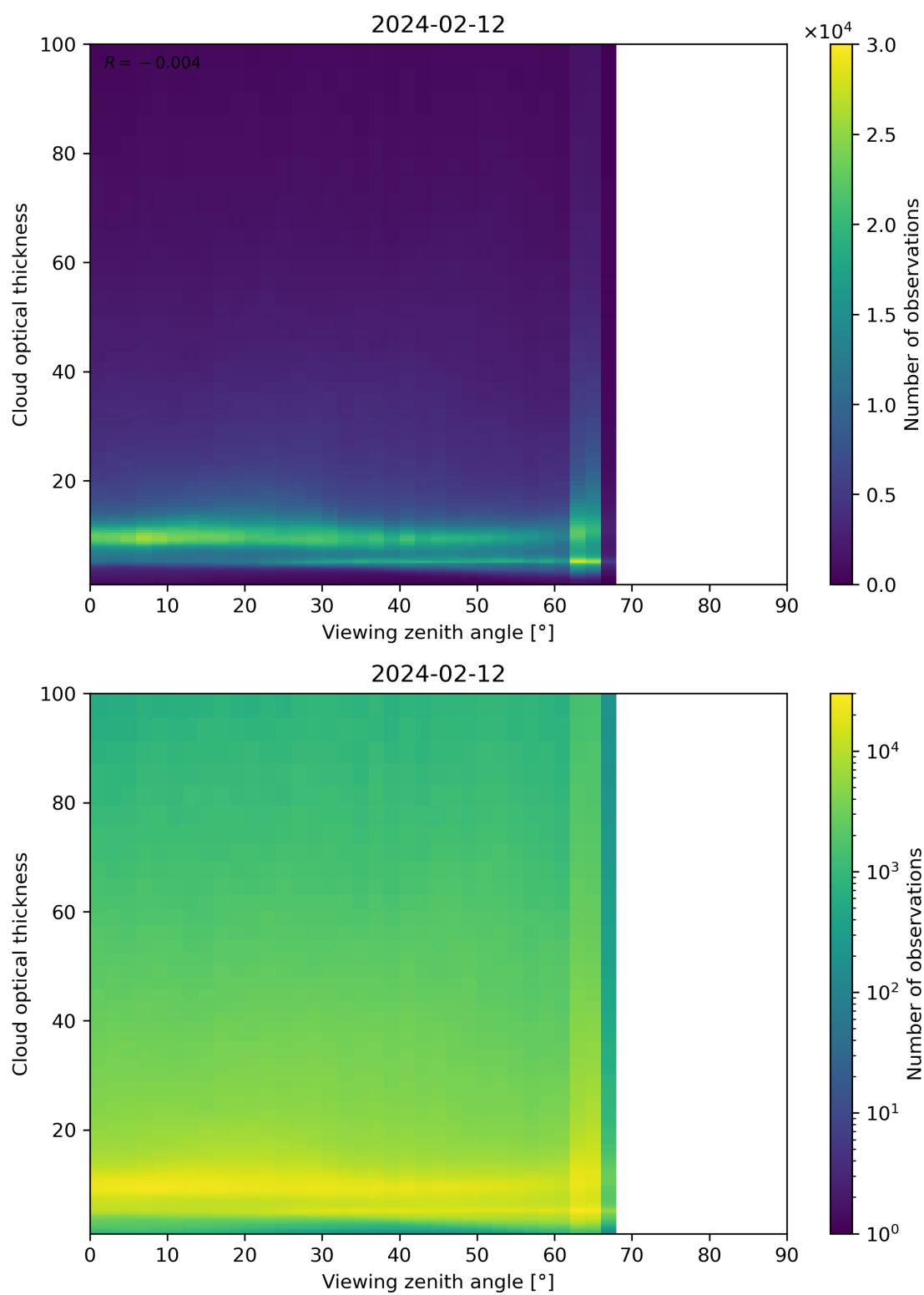
Figure 111: Scatter density plot of “Viewing zenith angle” against “Cloud optical thickness” for 2024-02-11 to 2024-02-13.
