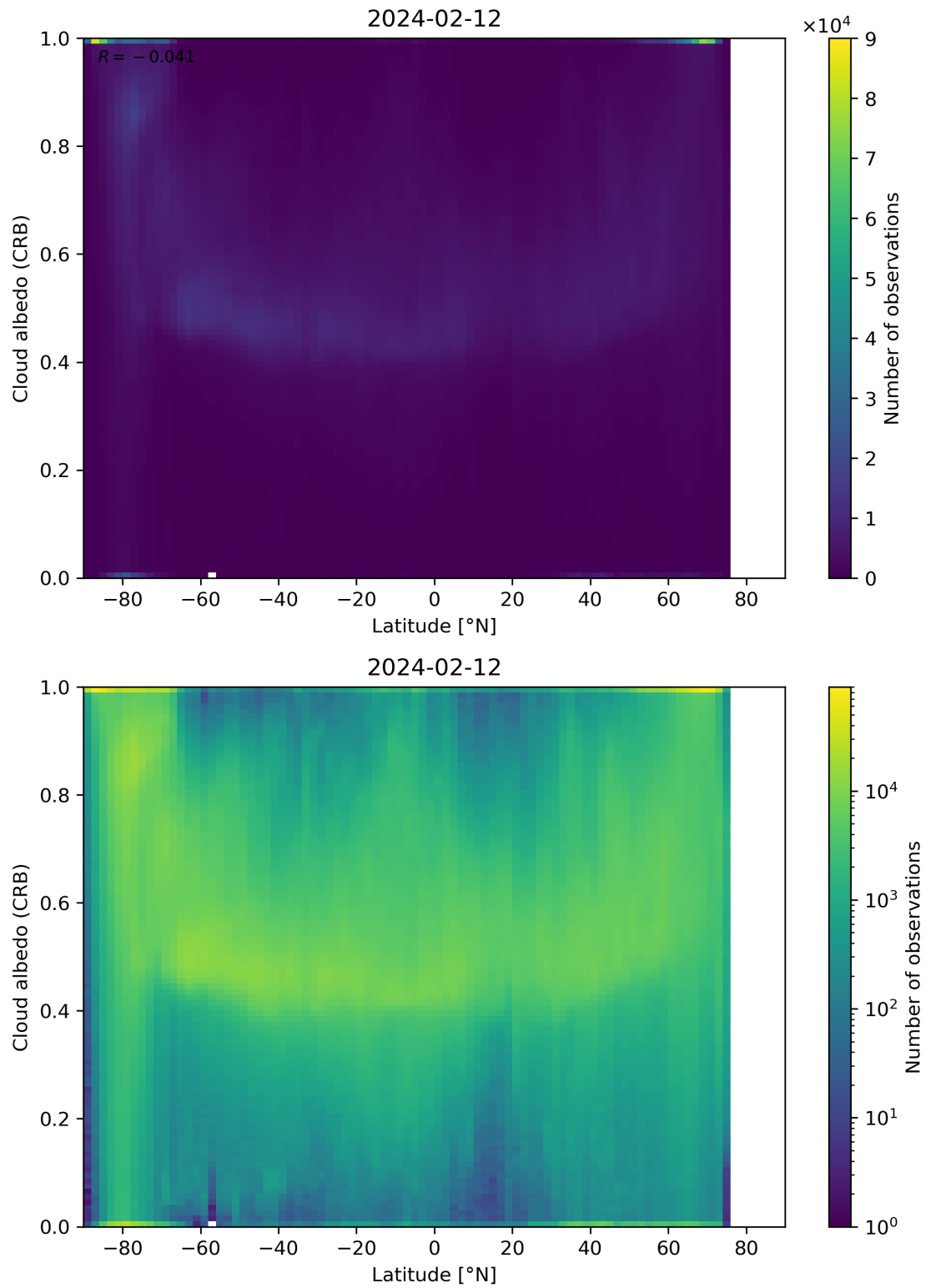
Figure 91: Scatter density plot of “Latitude” against “Cloud albedo (CRB)” for 2024-02-11 to 2024-02-13.
