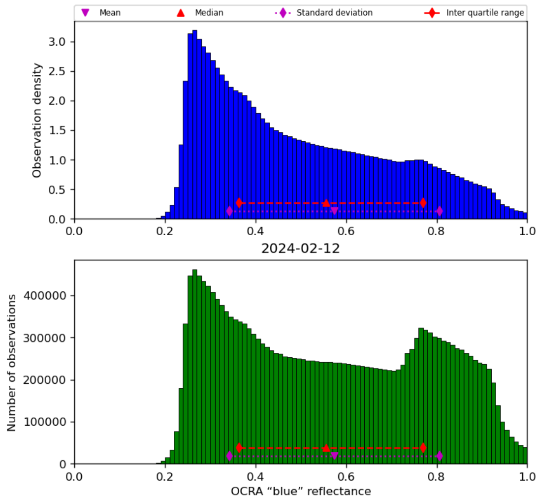
Figure 51: Histogram of “OCRA “blue” reflectance” for 2024-02-11 to 2024-02-13
