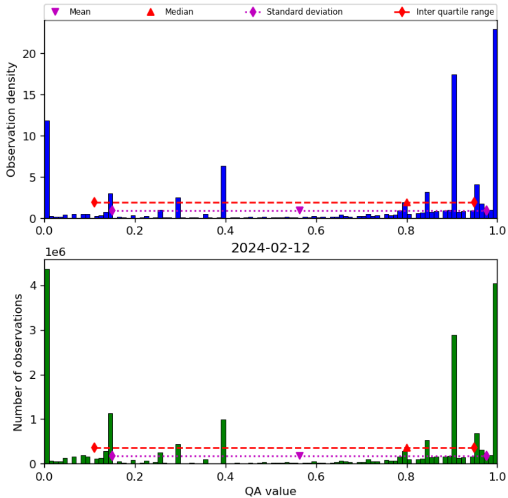
Figure 38: Histogram of “QA value” for 2024-02-11 to 2024-02-13
