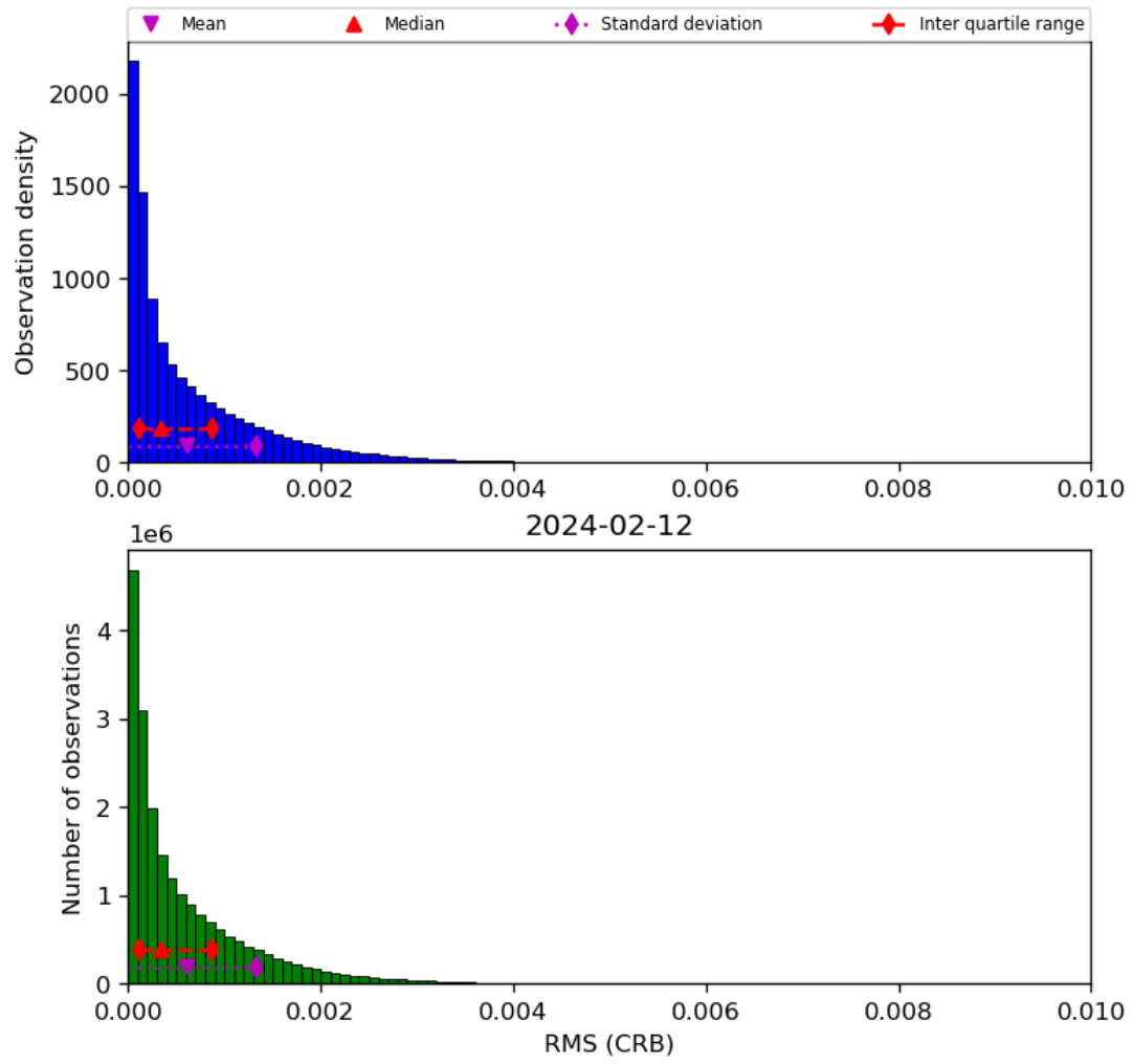
Figure 48: Histogram of “RMS (CRB)” for 2024-02-11 to 2024-02-13
