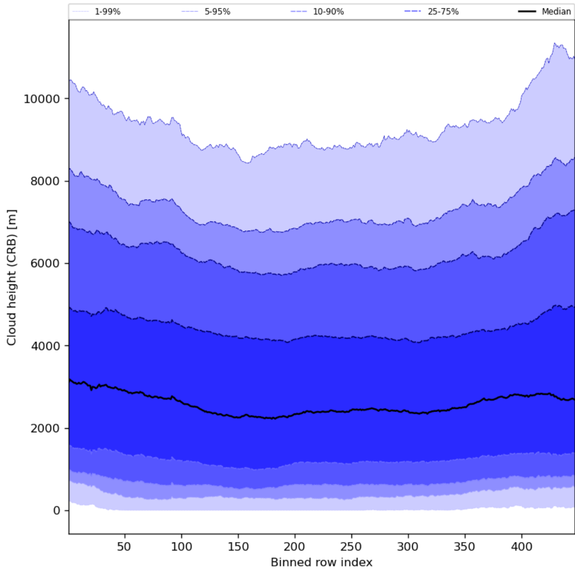
Figure 59: Along track statistics of “Cloud height (CRB)” for 2024-02-11 to 2024-02-13
