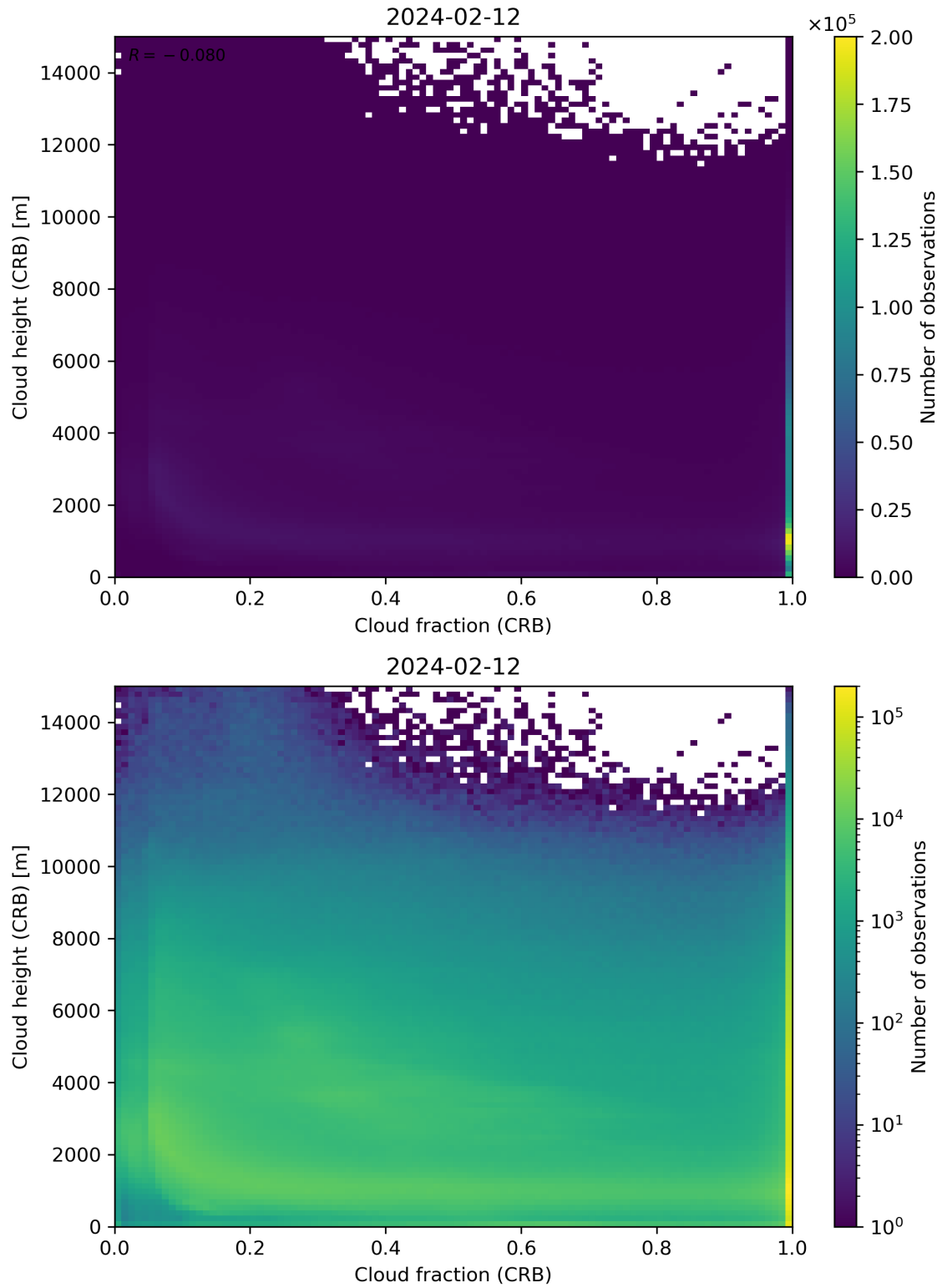
Figure 79: Scatter density plot of “Cloud fraction (CRB)” against “Cloud height (CRB)” for 2024-02-11 to 2024-02-13.
