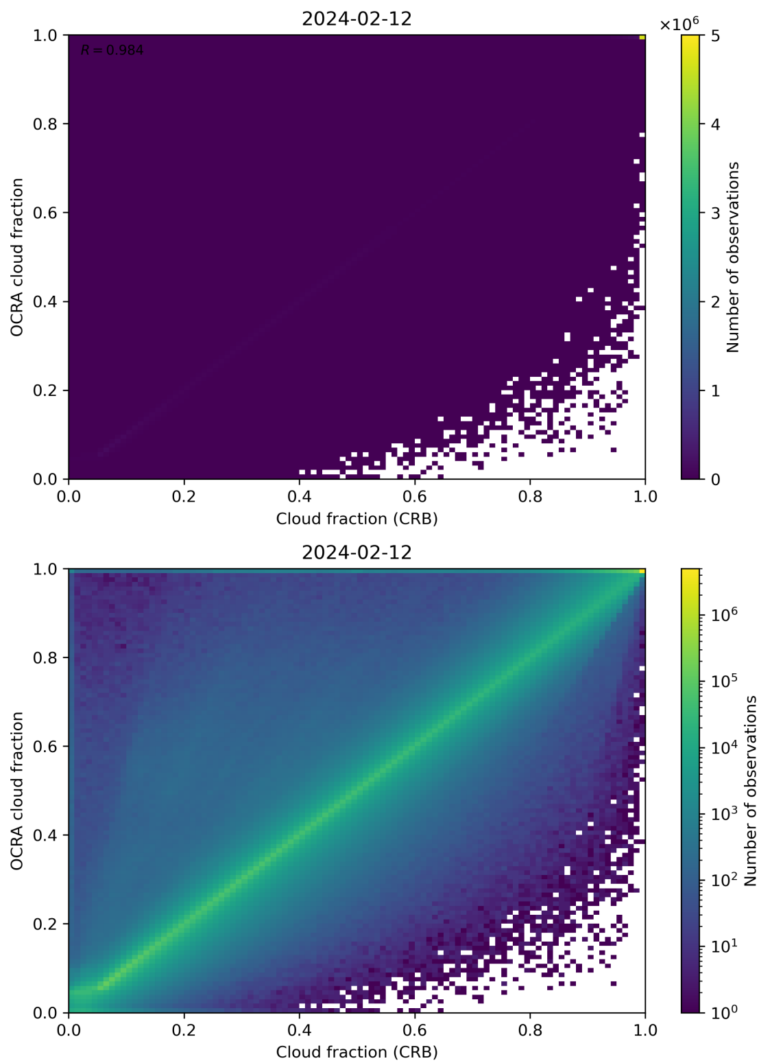
Figure 78: Scatter density plot of “Cloud fraction (CRB)” against “OCRA cloud fraction” for 2024-02-11 to 2024-02-13.
