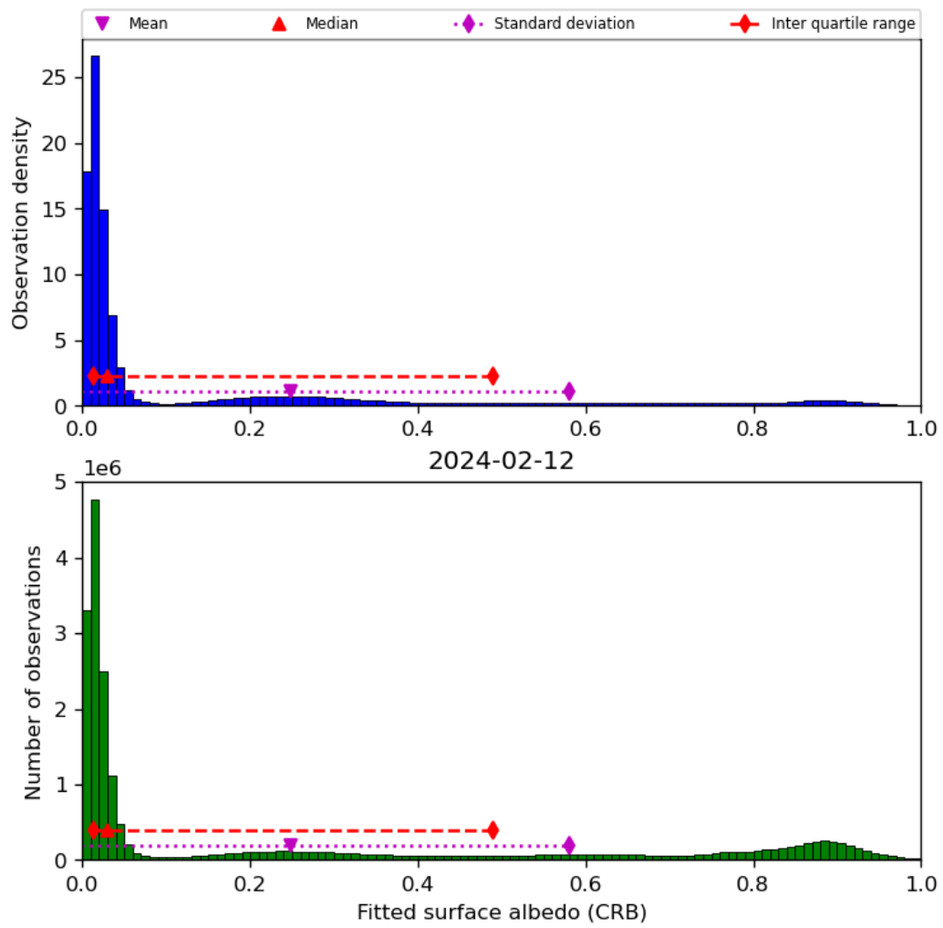
Figure 46: Histogram of “Fitted surface albedo (CRB)” for 2024-02-11 to 2024-02-13
