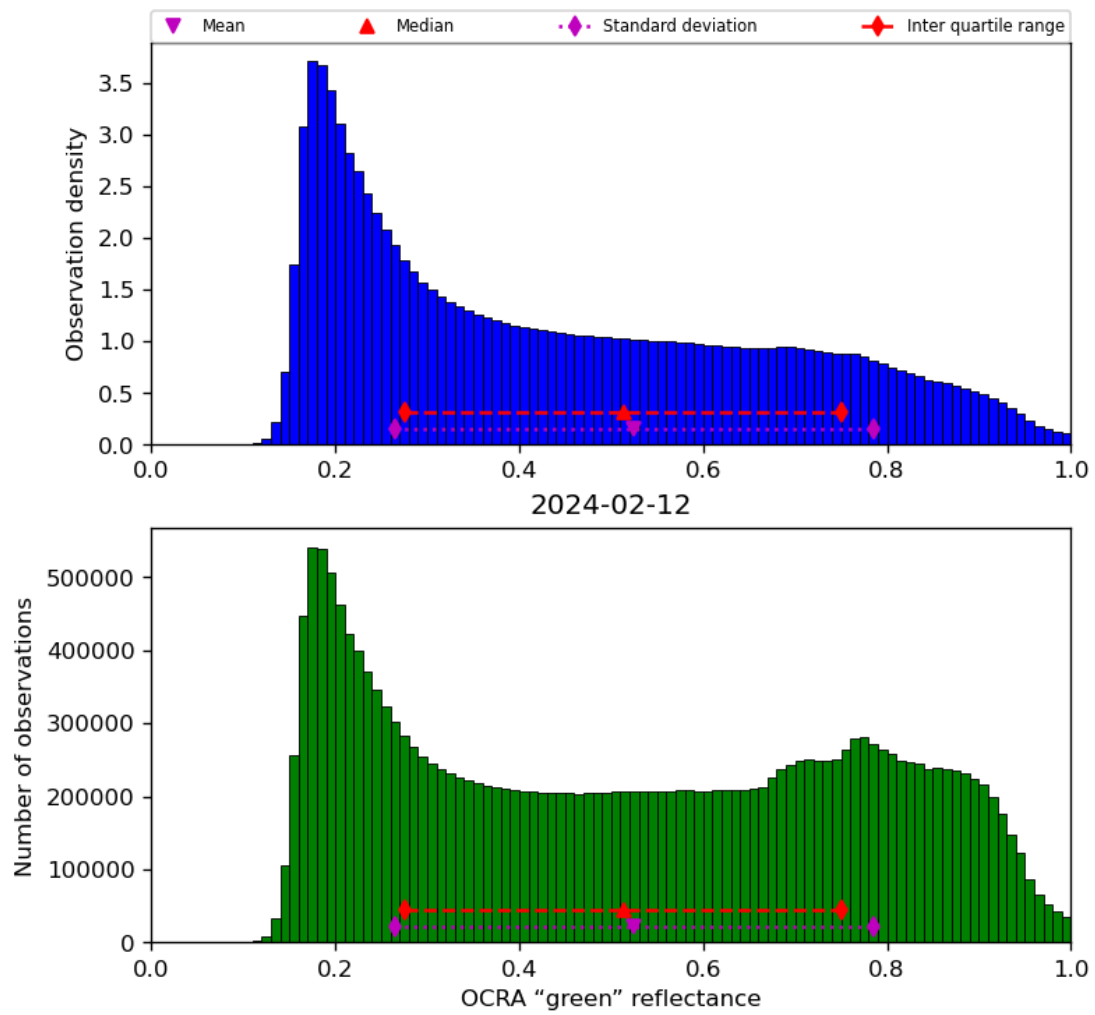
Figure 52: Histogram of “OCRA “green” reflectance” for 2024-02-11 to 2024-02-13
