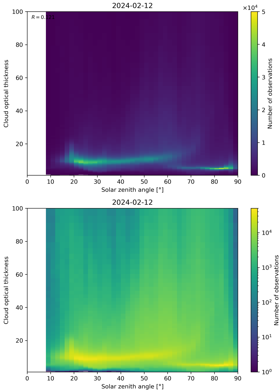
Figure 103: Scatter density plot of “Solar zenith angle” against “Cloud optical thickness” for 2024-02-11 to 2024-02-13.
