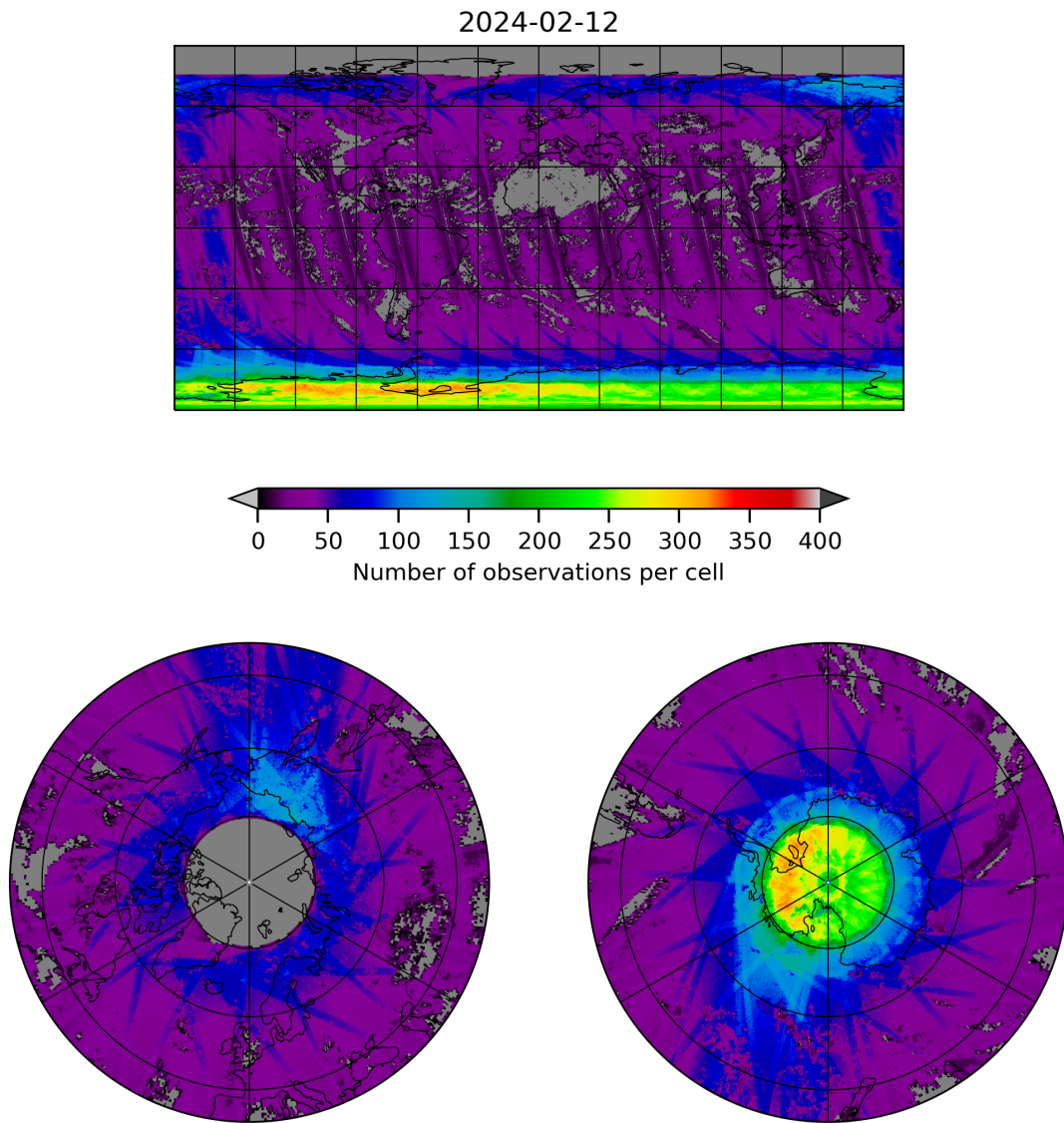
Figure 21: Map of the number of observations for 2024-02-11 to 2024-02-13
