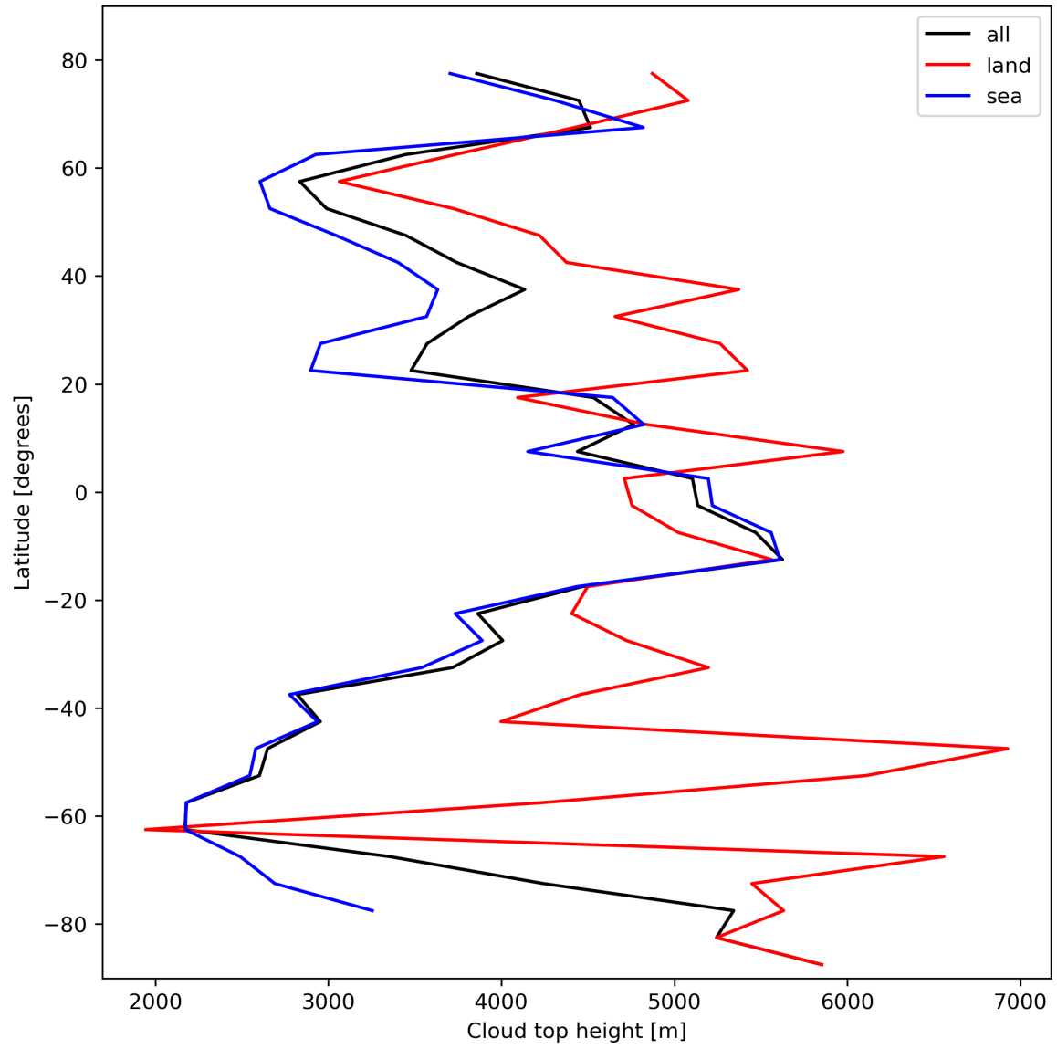
Figure 24: Zonal average of “Cloud top height” for 2024-02-11 to 2024-02-13.
