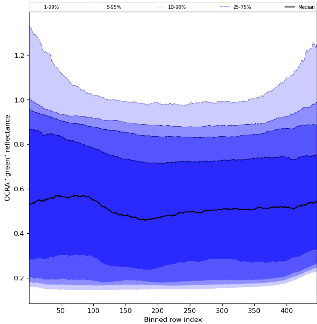
Figure 68: Along track statistics of "OCRA "green" reflectance" for 2024-02-11 to 2024-02-13
