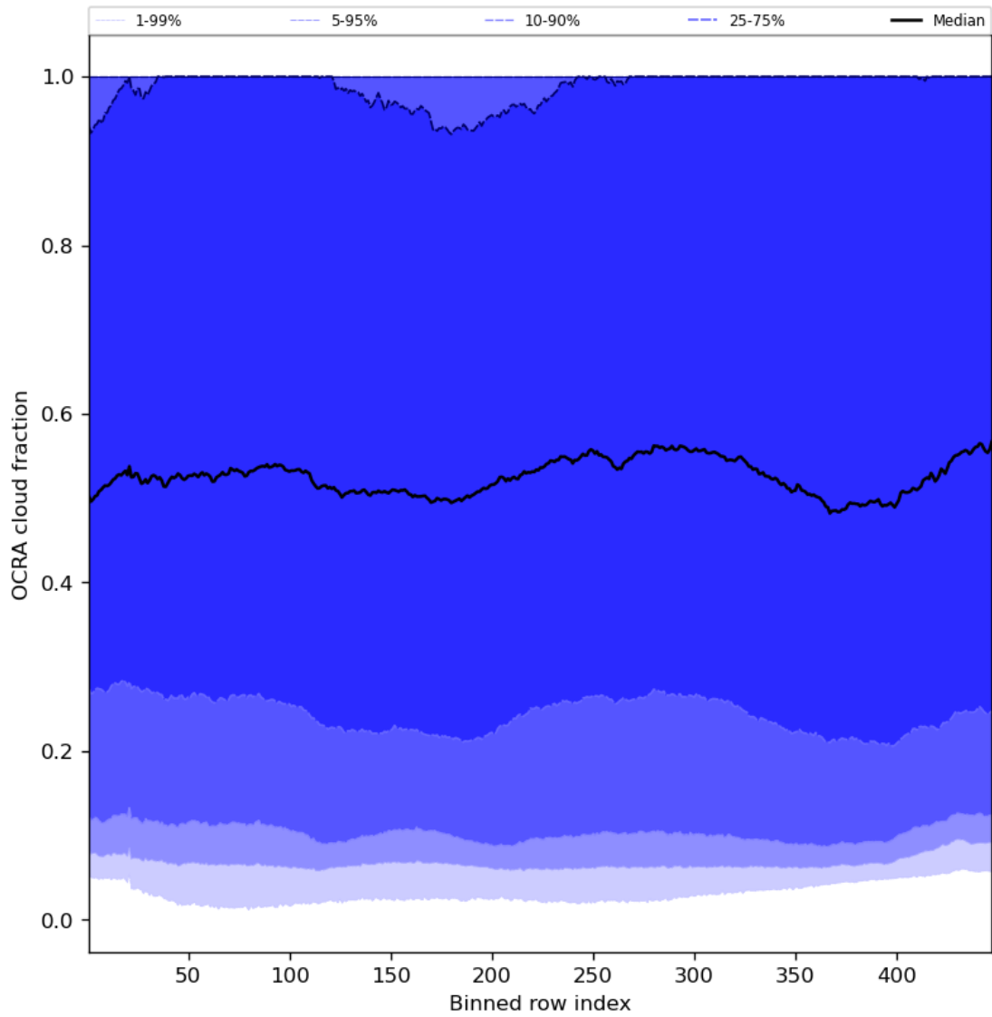
Figure 66: Along track statistics of “OCRA cloud fraction” for 2024-02-11 to 2024-02-13
