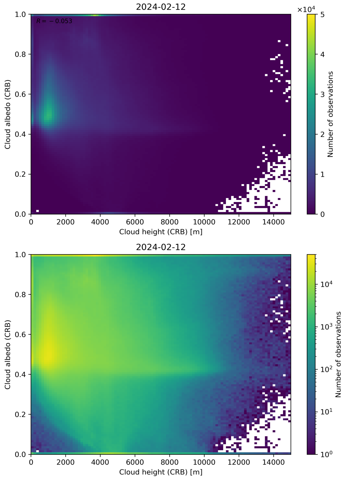
Figure 80: Scatter density plot of “Cloud height (CRB)” against “Cloud albedo (CRB)” for 2024-02-11 to 2024-02-13.
