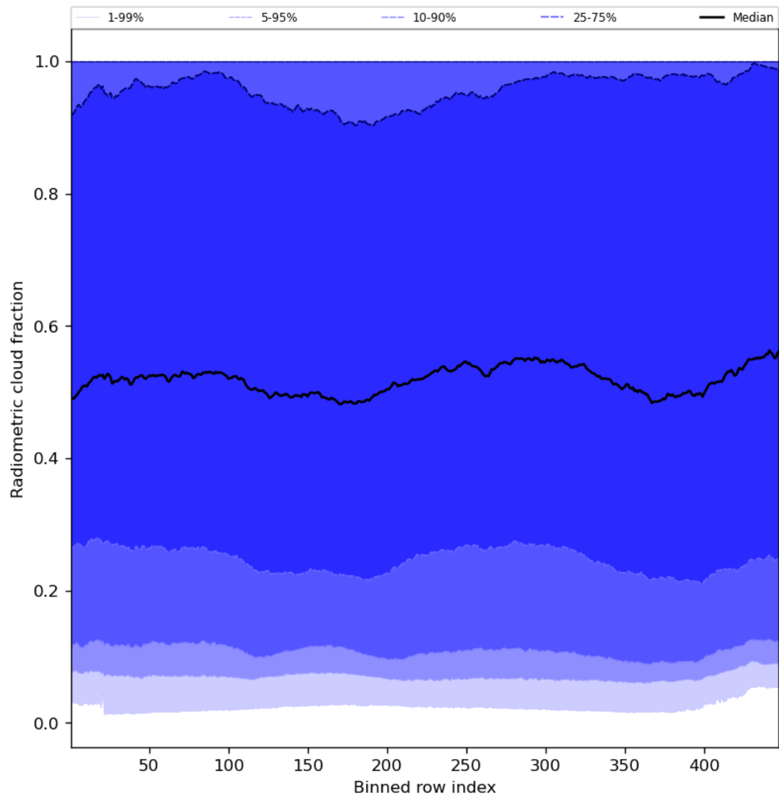
Figure 55: Along track statistics of “Radiometric cloud fraction” for 2024-02-11 to 2024-02-13
