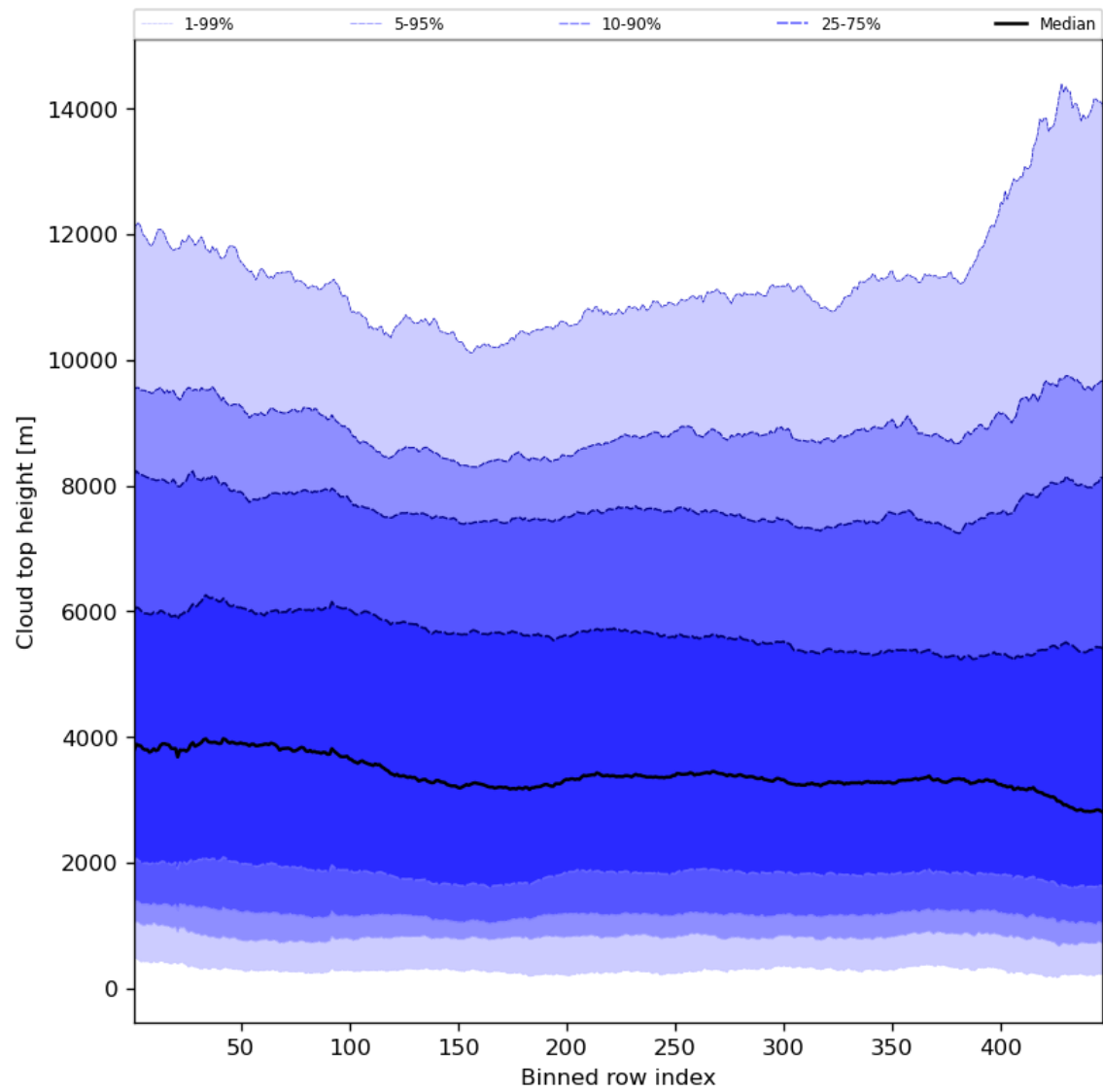
Figure 56: Along track statistics of “Cloud top height” for 2024-02-11 to 2024-02-13
