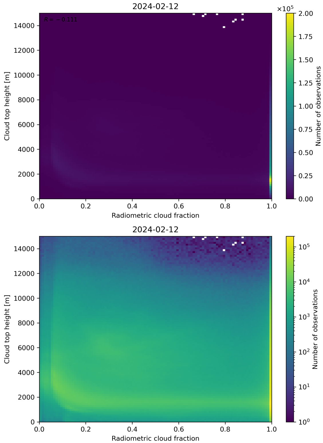
Figure 76: Scatter density plot of “Radiometric cloud fraction” against “Cloud top height” for 2024-02-11 to 2024-02-13.
