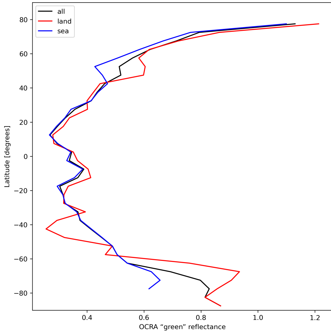
Figure 36: Zonal average of “OCRA “green” reflectance” for 2024-02-11 to 2024-02-13.
