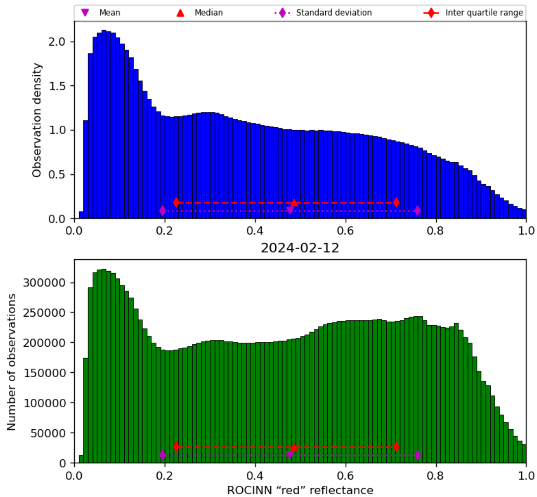
Figure 53: Histogram of “ROCINN “red” reflectance” for 2024-02-11 to 2024-02-13
