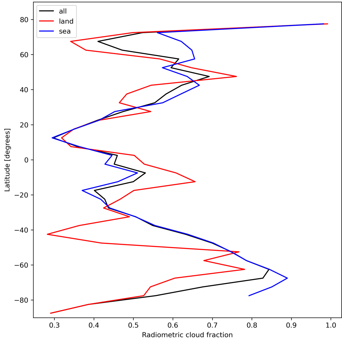
Figure 23: Zonal average of “Radiometric cloud fraction” for 2024-02-11 to 2024-02-13.
