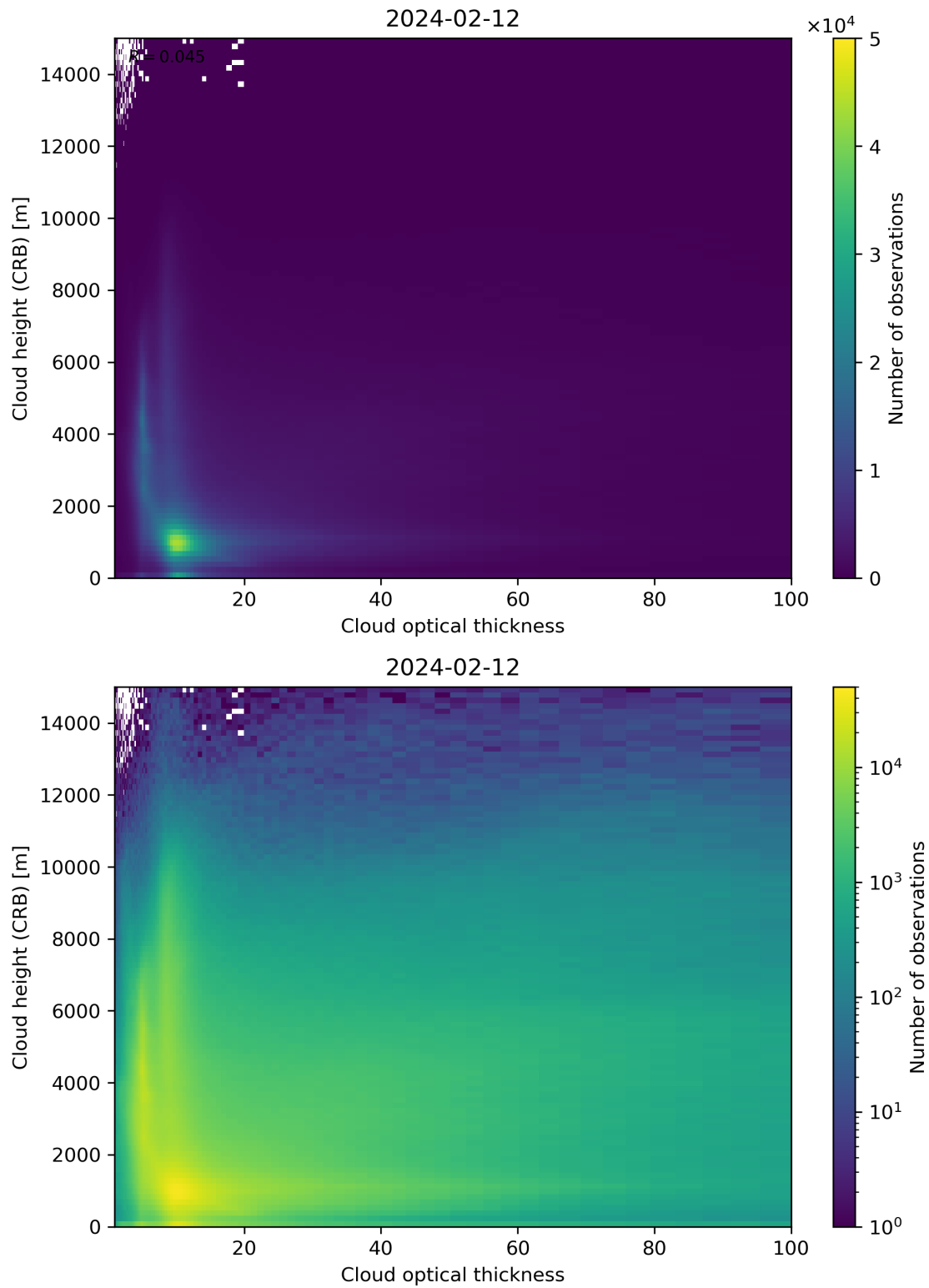
Figure 85: Scatter density plot of “Cloud optical thickness” against “Cloud height (CRB)” for 2024-02-11 to 2024-02-13.
