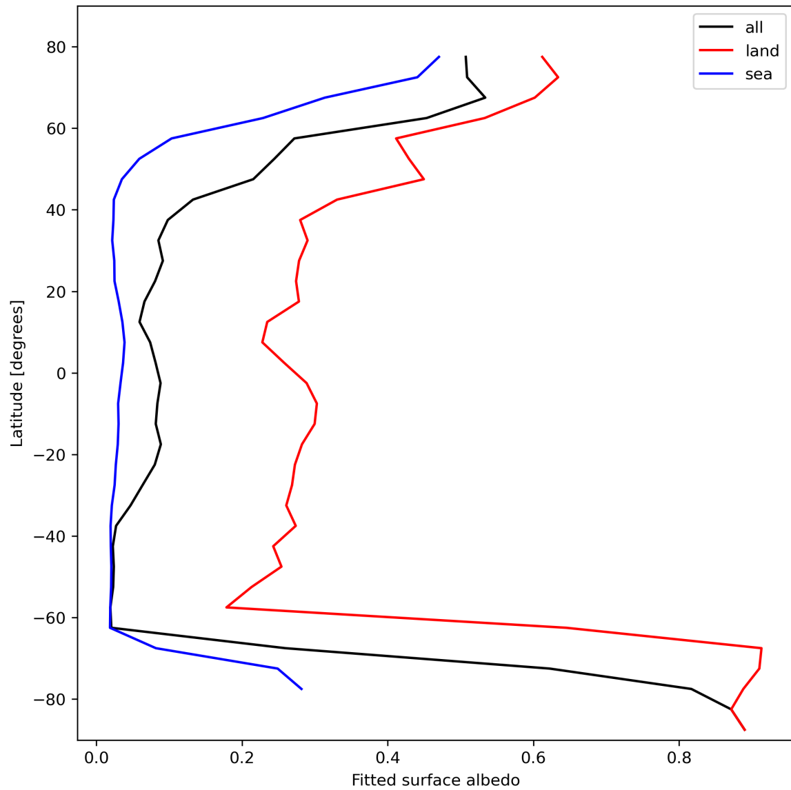
Figure 29: Zonal average of “Fitted surface albedo” for 2024-02-11 to 2024-02-13.
