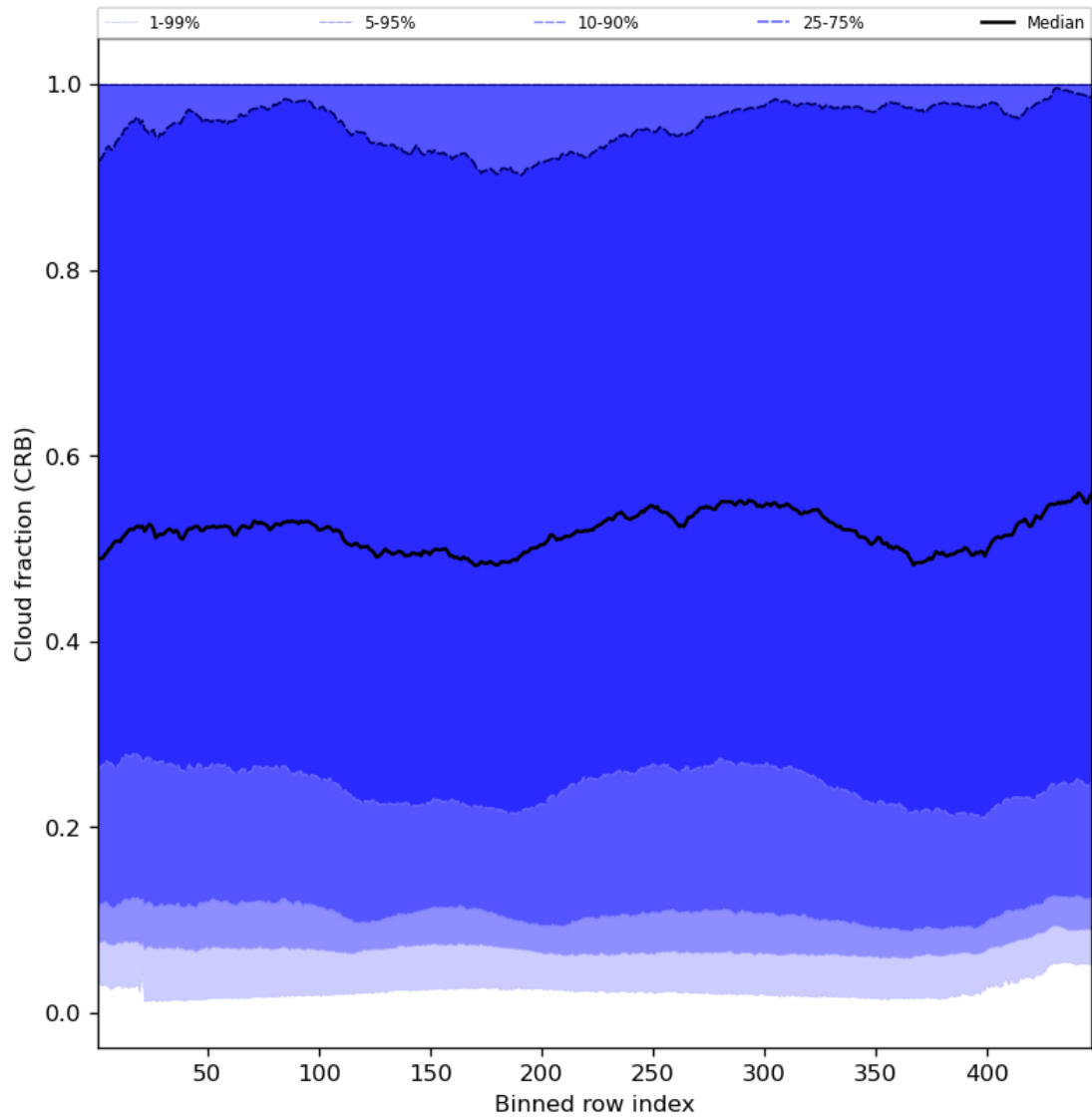
Figure 58: Along track statistics of “Cloud fraction (CRB)” for 2024-02-11 to 2024-02-13
