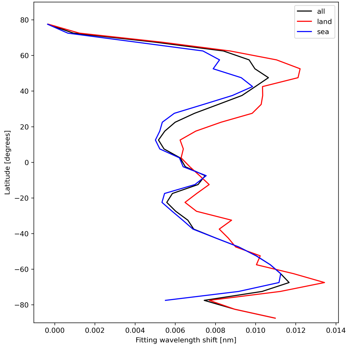
Figure 33: Zonal average of “Fitting wavelength shift” for 2024-02-11 to 2024-02-13.
