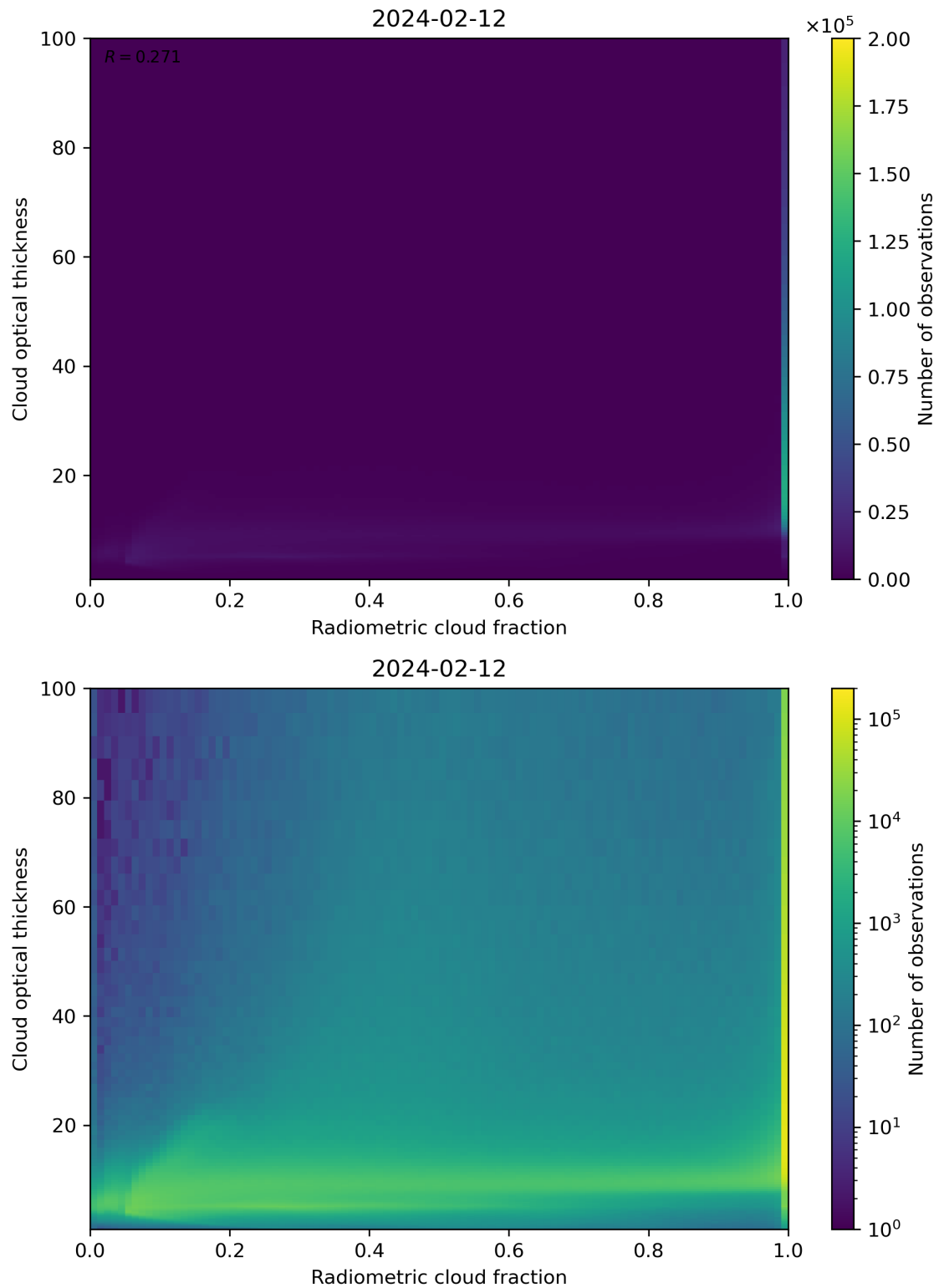
Figure 75: Scatter density plot of “Radiometric cloud fraction” against “Cloud optical thickness” for 2024-02-11 to 2024-02-13.
