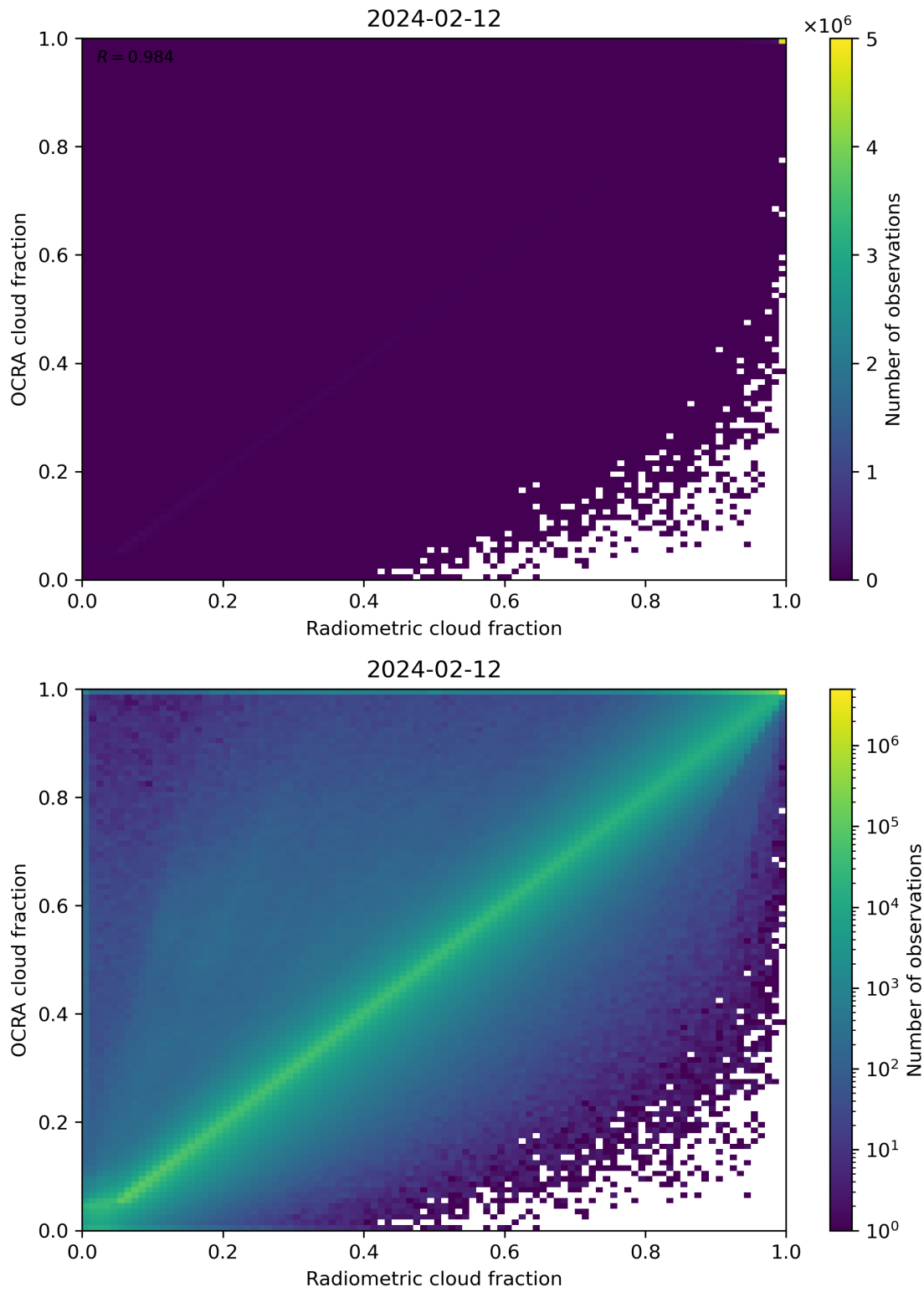
Figure 72: Scatter density plot of “Radiometric cloud fraction” against “OCRA cloud fraction” for 2024-02-11 to 2024-02-13.
