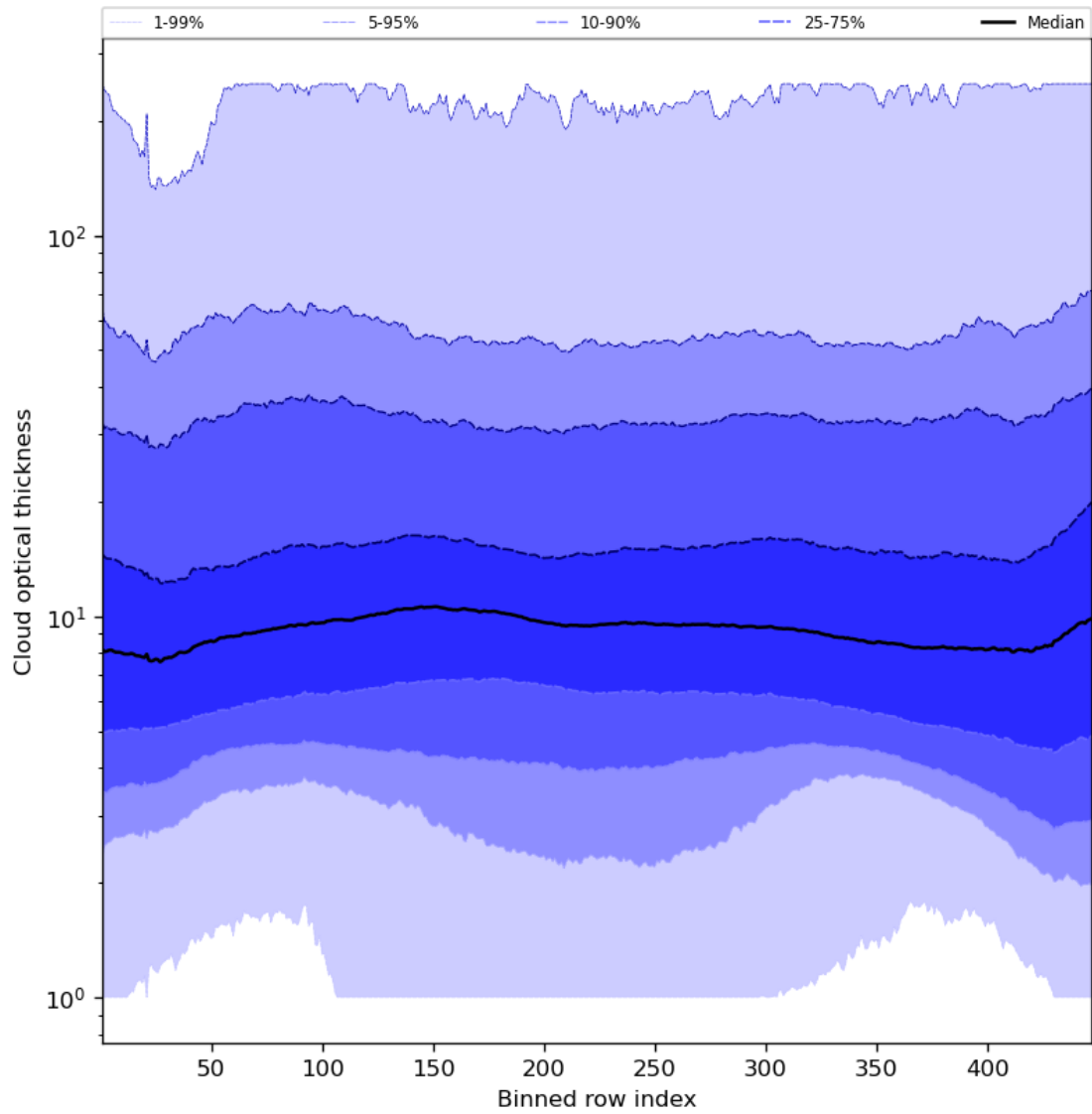
Figure 57: Along track statistics of “Cloud optical thickness” for 2024-02-11 to 2024-02-13
