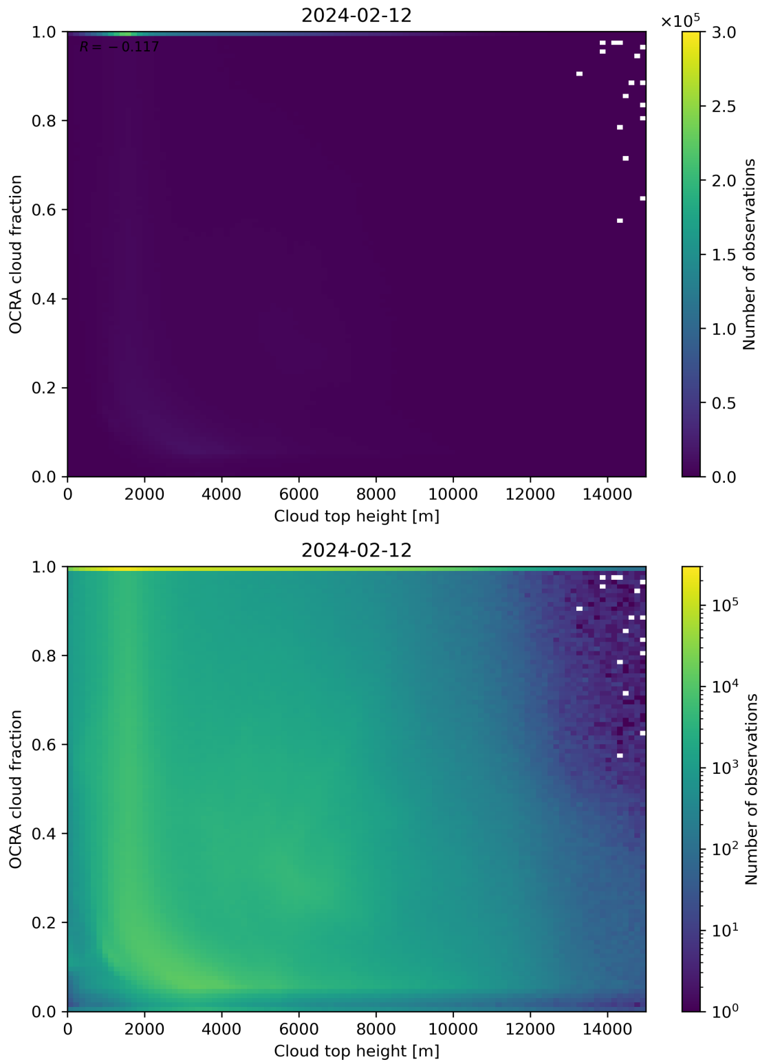
Figure 87: Scatter density plot of “Cloud top height” against “OCRA cloud fraction” for 2024-02-11 to 2024-02-13.
