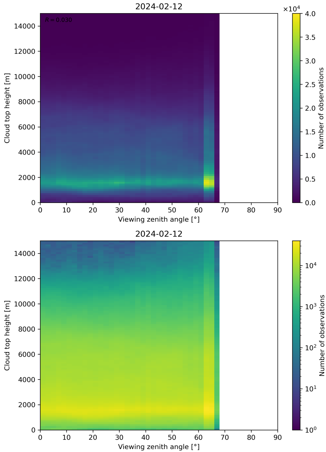
Figure 112: Scatter density plot of “Viewing zenith angle” against “Cloud top height” for 2024-02-11 to 2024-02-13.
