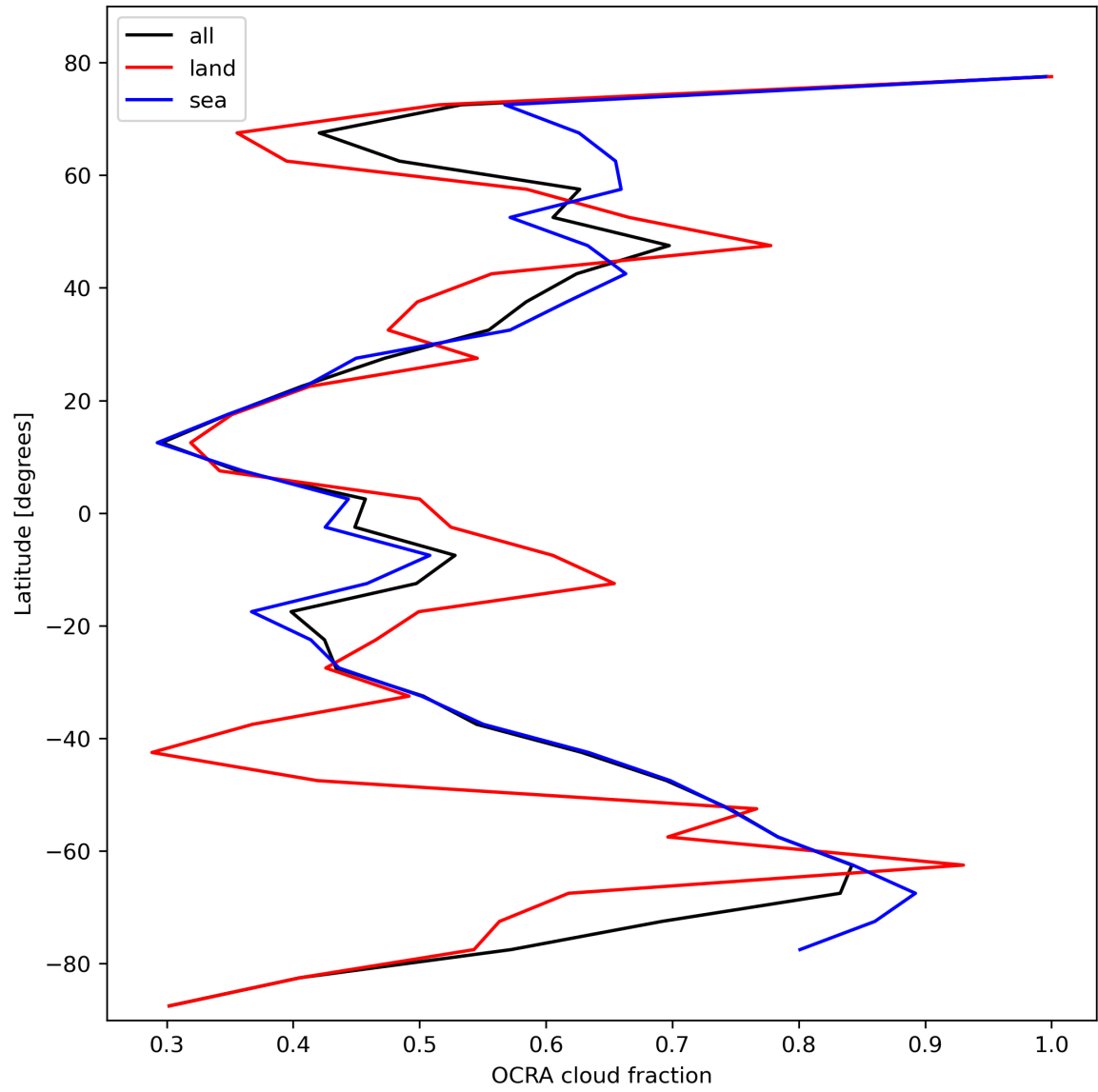
Figure 34: Zonal average of “OCRA cloud fraction” for 2024-02-11 to 2024-02-13.
