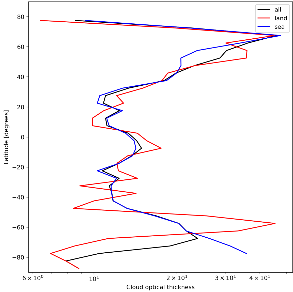
Figure 25: Zonal average of “Cloud optical thickness” for 2024-02-13 to 2024-02-15.
