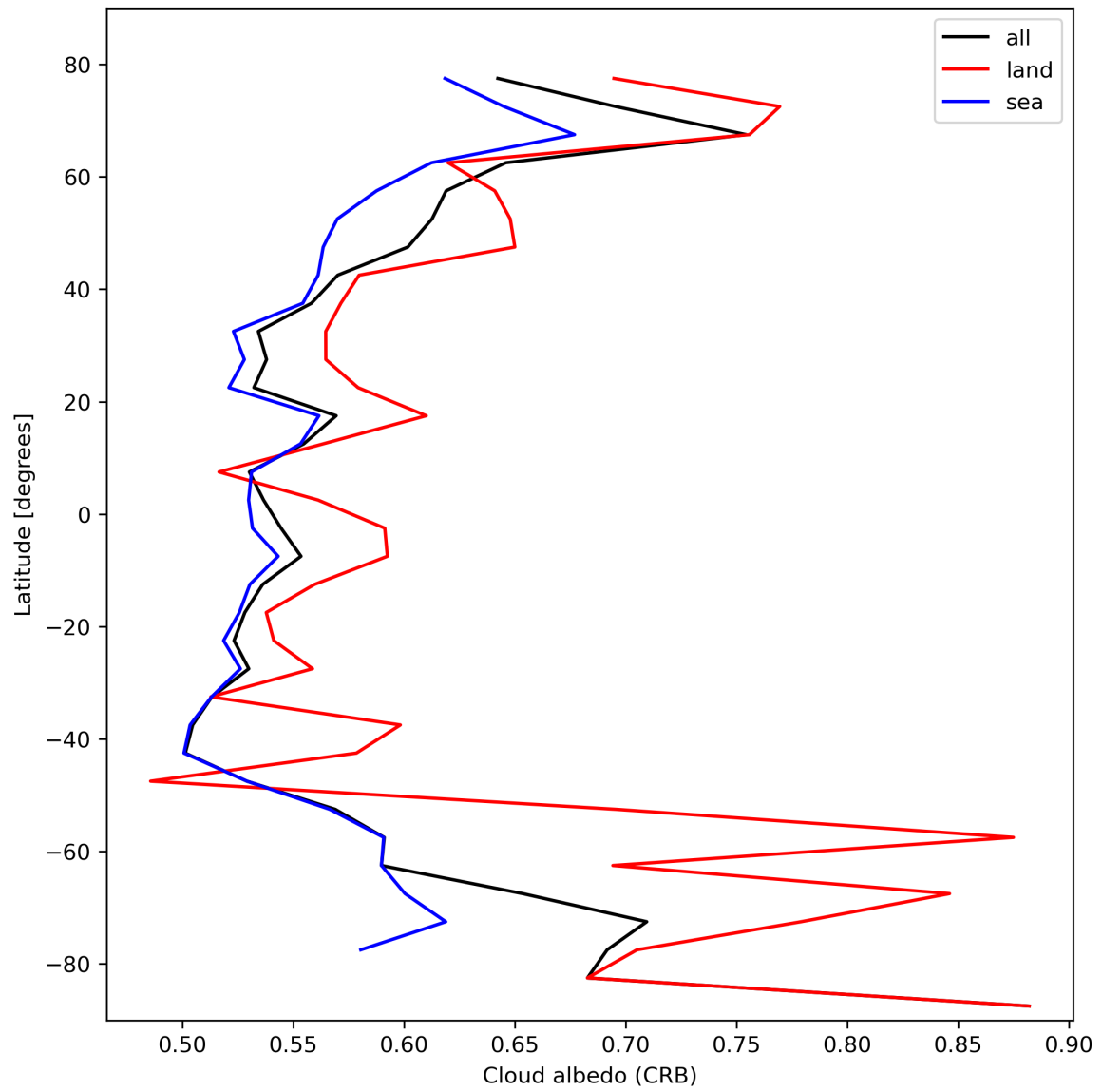
Figure 28: Zonal average of “Cloud albedo (CRB)” for 2024-02-13 to 2024-02-15.
