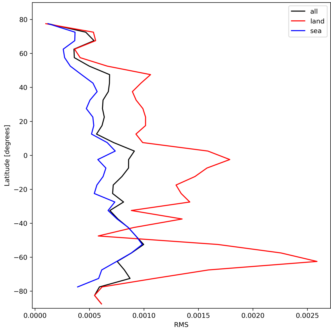
Figure 31: Zonal average of “RMS” for 2024-02-13 to 2024-02-15.
