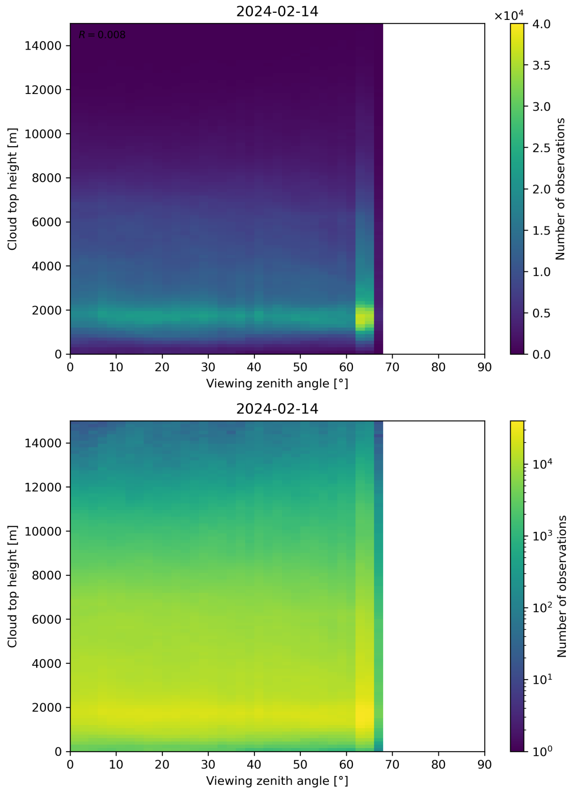
Figure 112: Scatter density plot of “Viewing zenith angle” against “Cloud top height” for 2024-02-13 to 2024-02-15.
