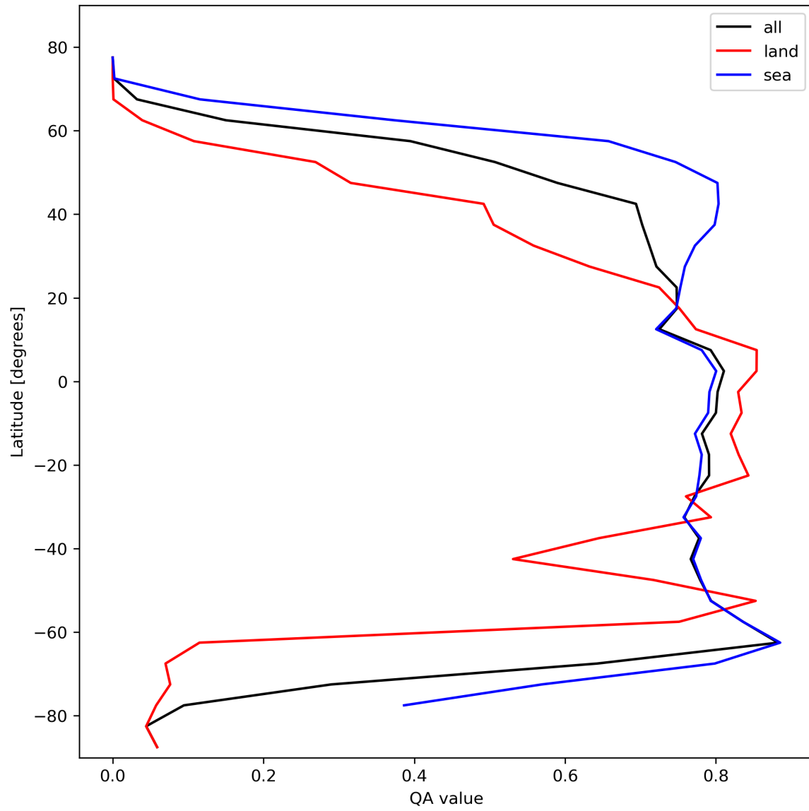
Figure 22: Zonal average of “QA value” for 2024-02-13 to 2024-02-15.
