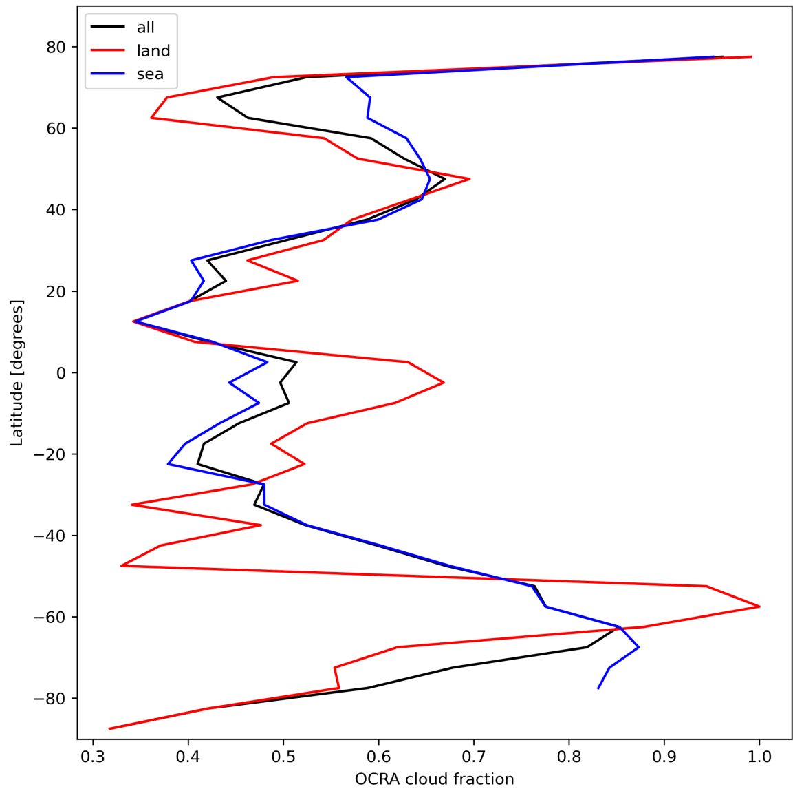
Figure 34: Zonal average of “OCRA cloud fraction” for 2024-02-13 to 2024-02-15.
