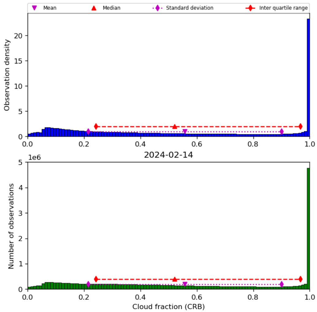
Figure 42: Histogram of “Cloud fraction (CRB)” for 2024-02-13 to 2024-02-15
