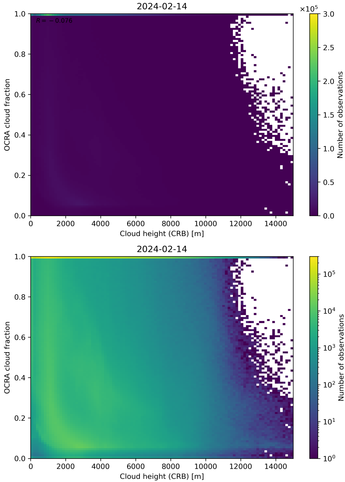
Figure 81: Scatter density plot of “Cloud height (CRB)” against “OCRA cloud fraction” for 2024-02-13 to 2024-02-15.
