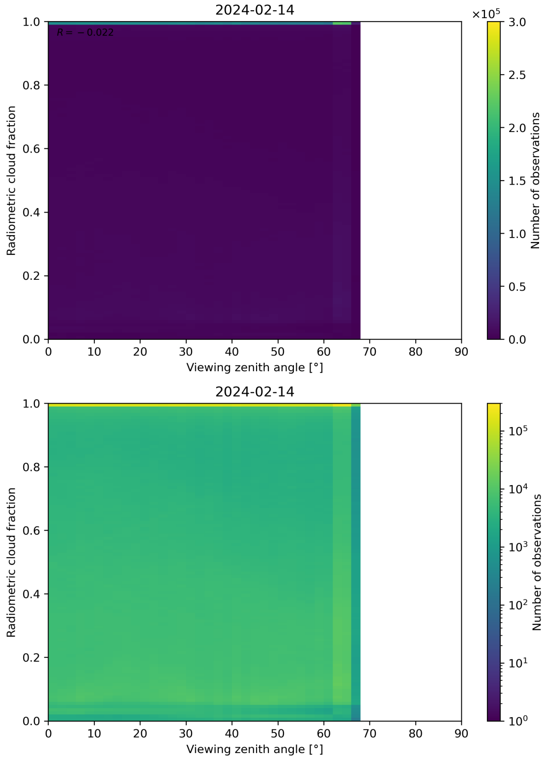
Figure 107: Scatter density plot of “Viewing zenith angle” against “Radiometric cloud fraction” for 2024-02-13 to 2024-02-15.
