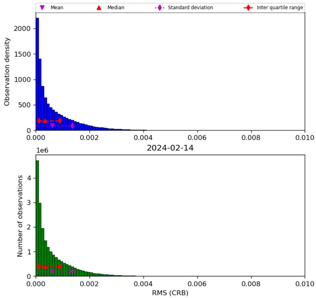
Figure 48: Histogram of “RMS (CRB)” for 2024-02-13 to 2024-02-15
