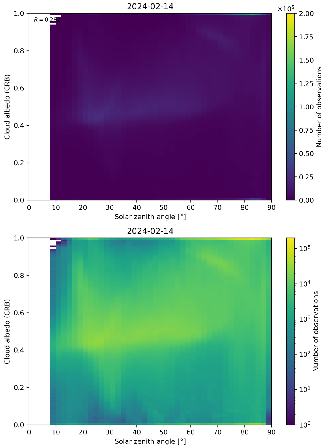
Figure 98: Scatter density plot of “Solar zenith angle” against “Cloud albedo (CRB)” for 2024-02-13 to 2024-02-15.
