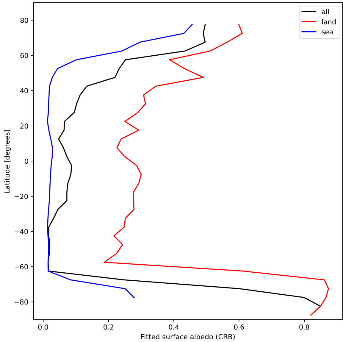
Figure 30: Zonal average of “Fitted surface albedo (CRB)” for 2024-02-13 to 2024-02-15.
