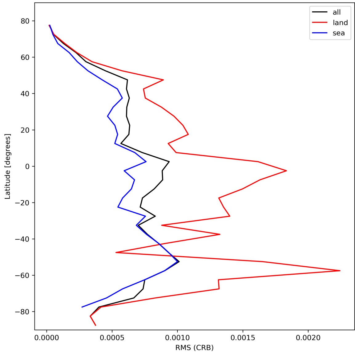
Figure 32: Zonal average of “RMS (CRB)” for 2024-02-13 to 2024-02-15.
