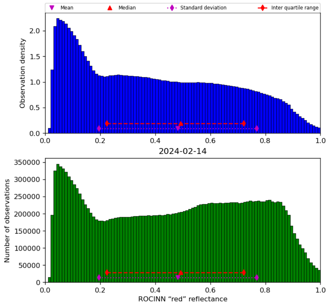
Figure 53: Histogram of “ROCINN “red” reflectance” for 2024-02-13 to 2024-02-15
