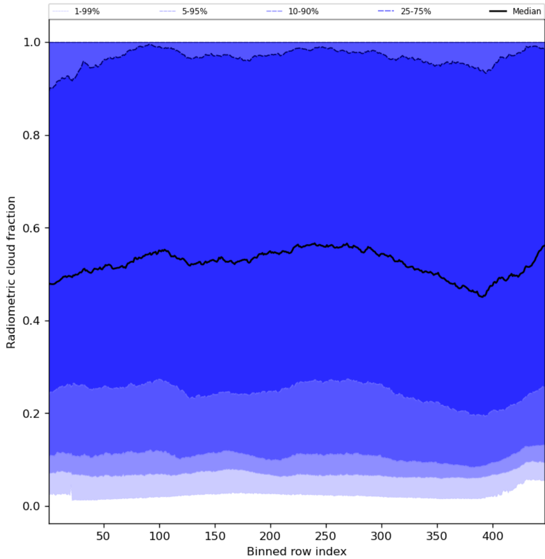
Figure 55: Along track statistics of “Radiometric cloud fraction” for 2024-02-13 to 2024-02-15
