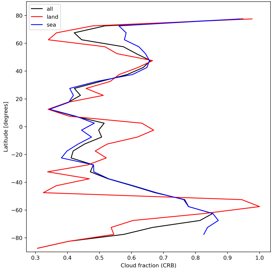
Figure 26: Zonal average of “Cloud fraction (CRB)” for 2024-02-13 to 2024-02-15.
