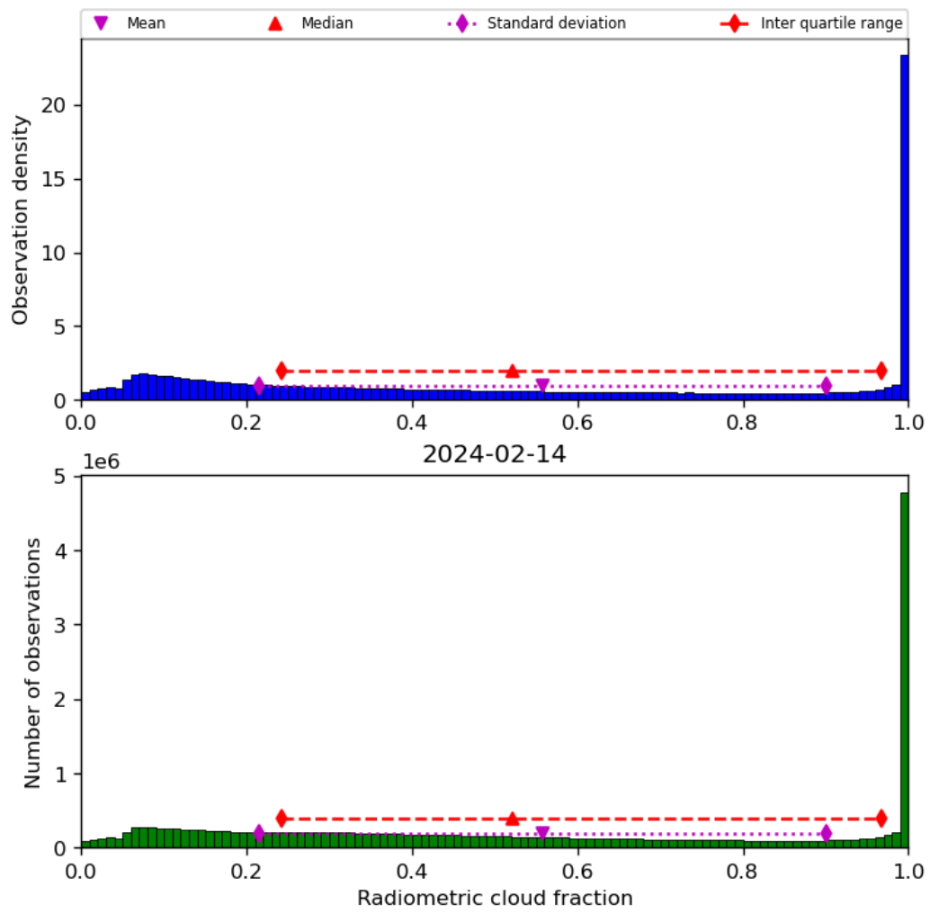
Figure 39: Histogram of “Radiometric cloud fraction” for 2024-02-13 to 2024-02-15
