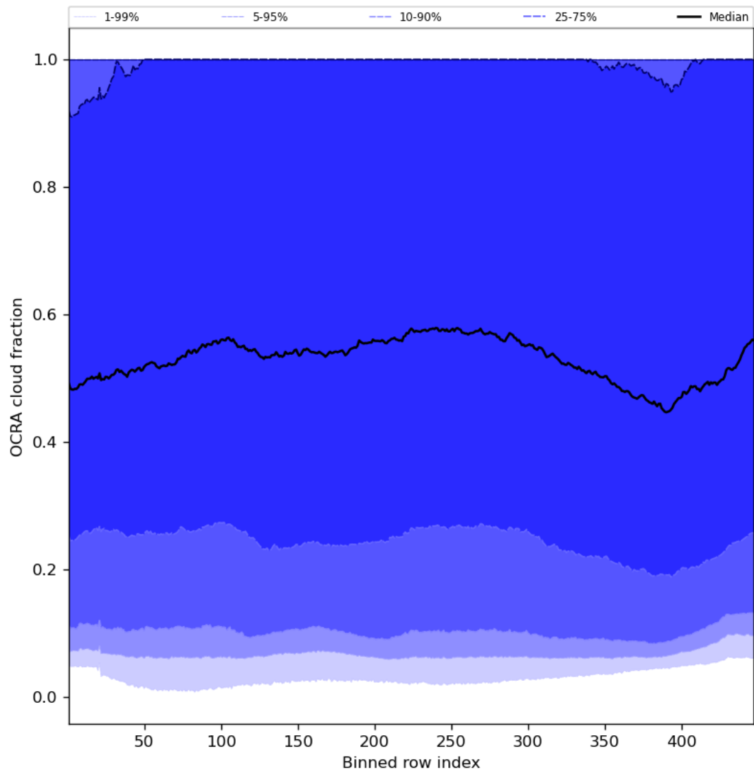
Figure 66: Along track statistics of “OCRA cloud fraction” for 2024-02-13 to 2024-02-15
