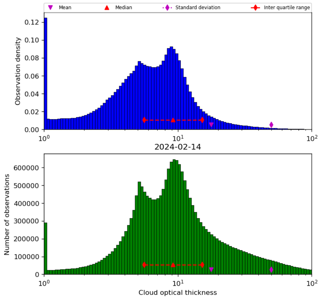
Figure 41: Histogram of “Cloud optical thickness” for 2024-02-13 to 2024-02-15
