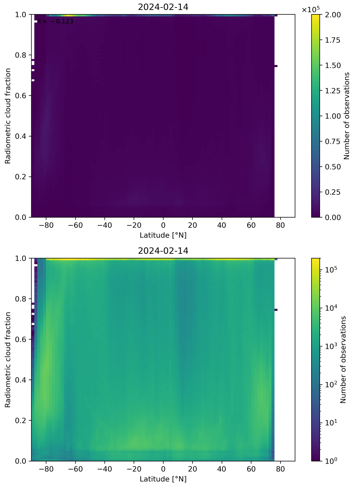
Figure 92: Scatter density plot of “Latitude” against “Radiometric cloud fraction” for 2024-02-13 to 2024-02-15.
