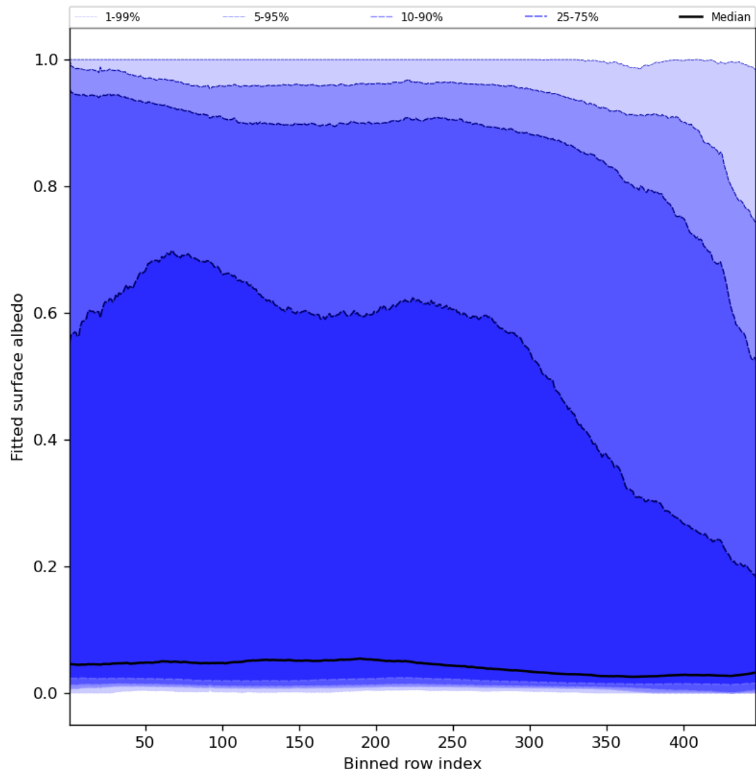
Figure 61: Along track statistics of “Fitted surface albedo” for 2024-02-13 to 2024-02-15
