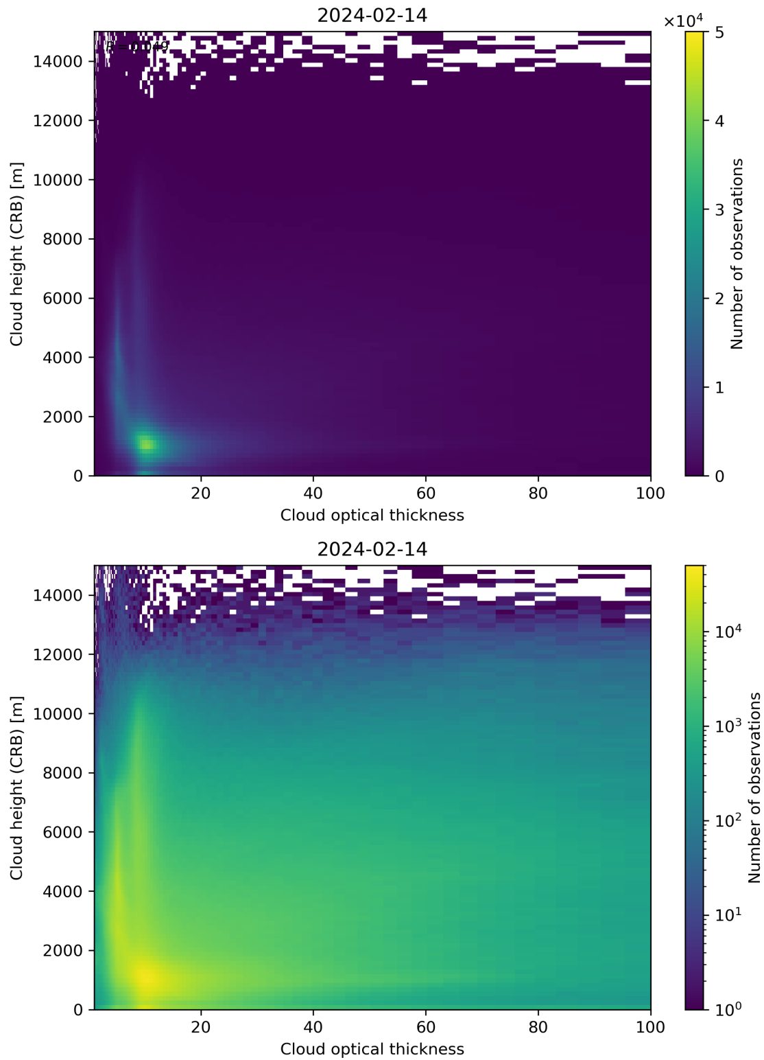
Figure 85: Scatter density plot of “Cloud optical thickness” against “Cloud height (CRB)” for 2024-02-13 to 2024-02-15.
