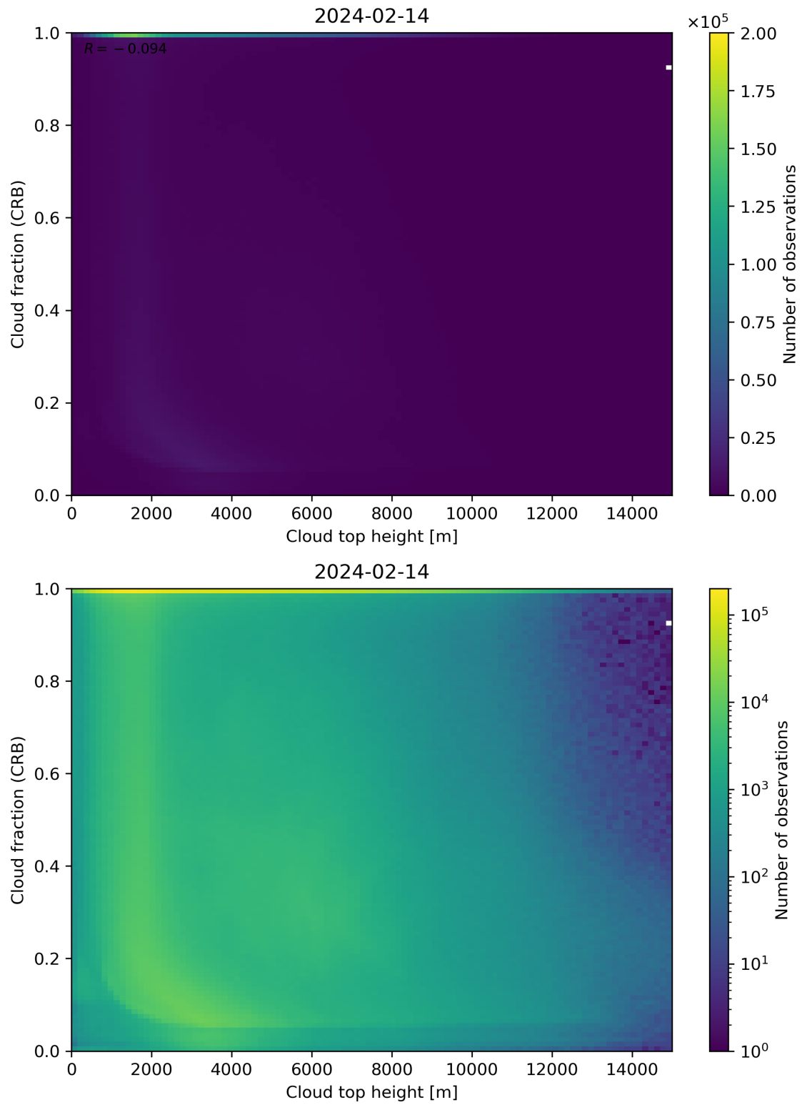
Figure 88: Scatter density plot of “Cloud top height” against “Cloud fraction (CRB)” for 2024-02-13 to 2024-02-15.
