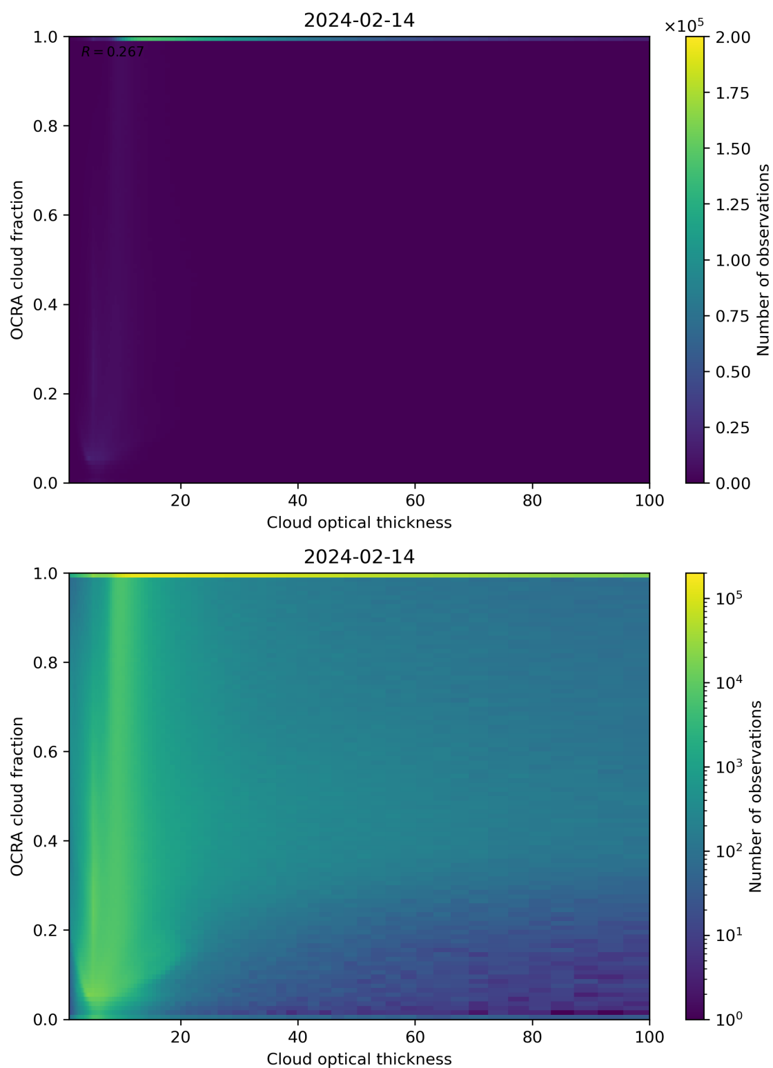
Figure 83: Scatter density plot of “Cloud optical thickness” against “OCRA cloud fraction” for 2024-02-13 to 2024-02-15.
