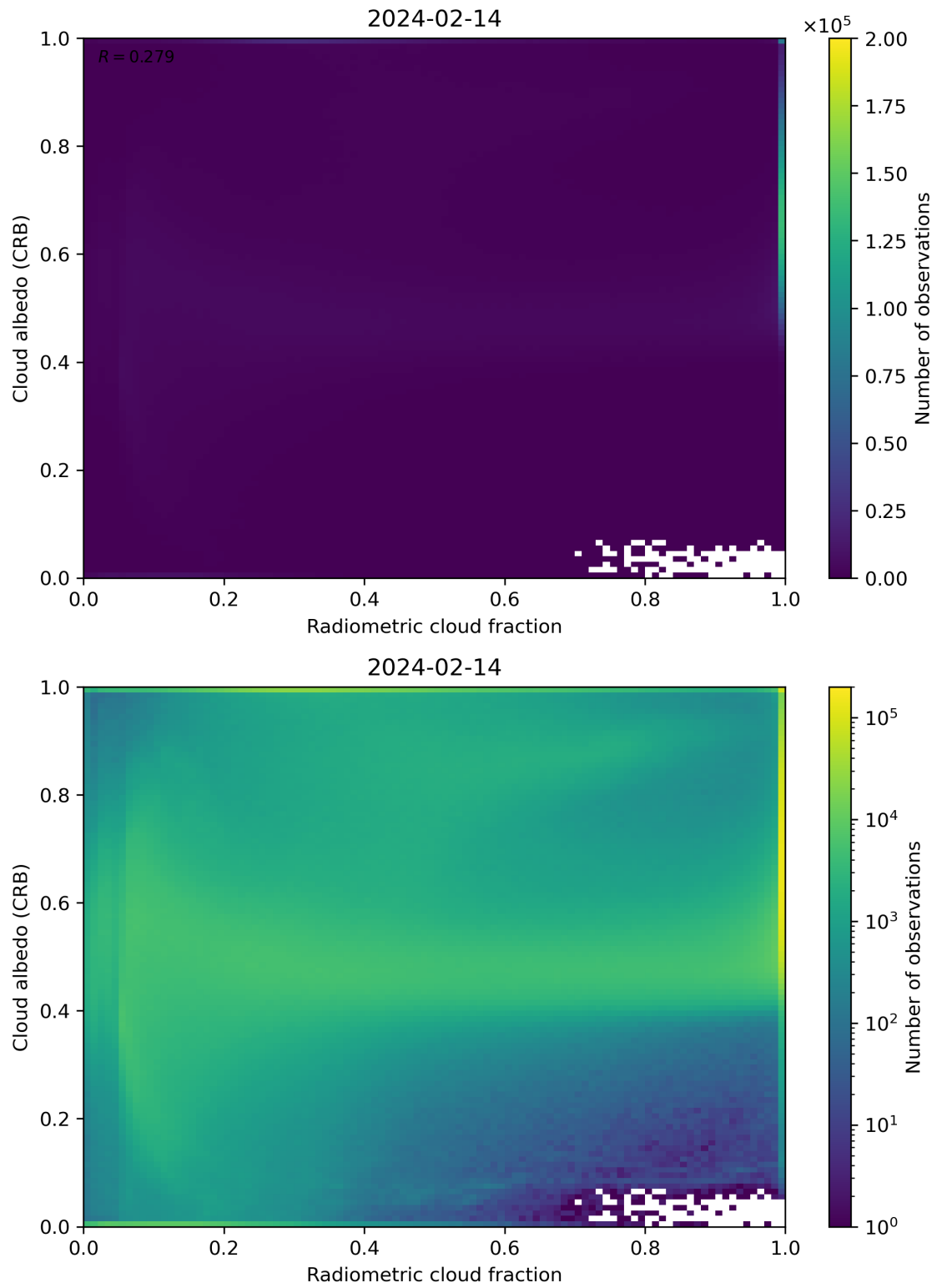
Figure 71: Scatter density plot of “Radiometric cloud fraction” against “Cloud albedo (CRB)” for 2024-02-13 to 2024-02-15.
