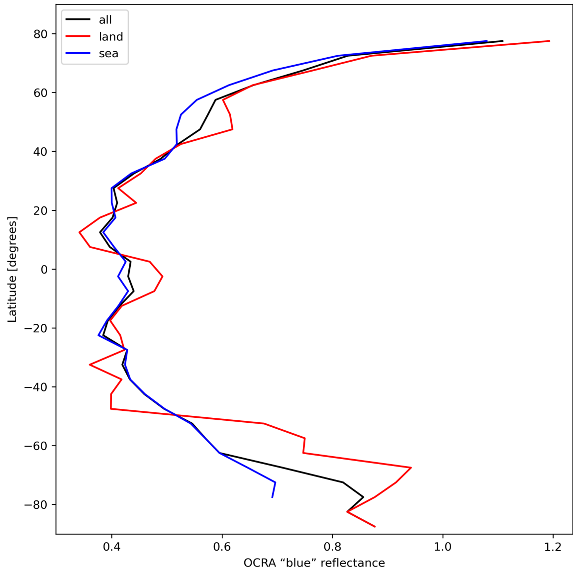
Figure 35: Zonal average of “OCRA “blue” reflectance” for 2024-02-13 to 2024-02-15.
