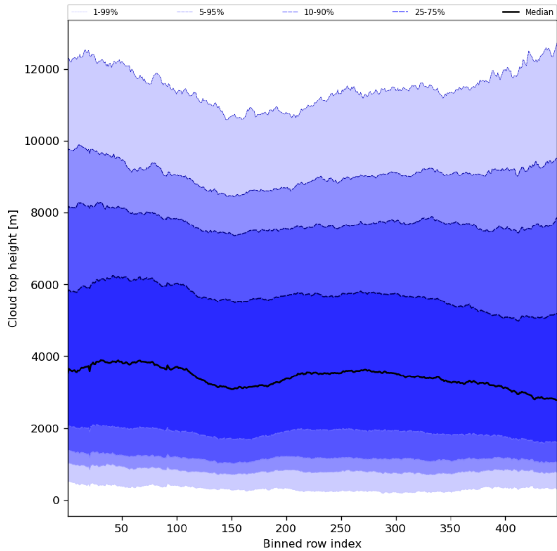
Figure 56: Along track statistics of “Cloud top height” for 2024-02-13 to 2024-02-15
