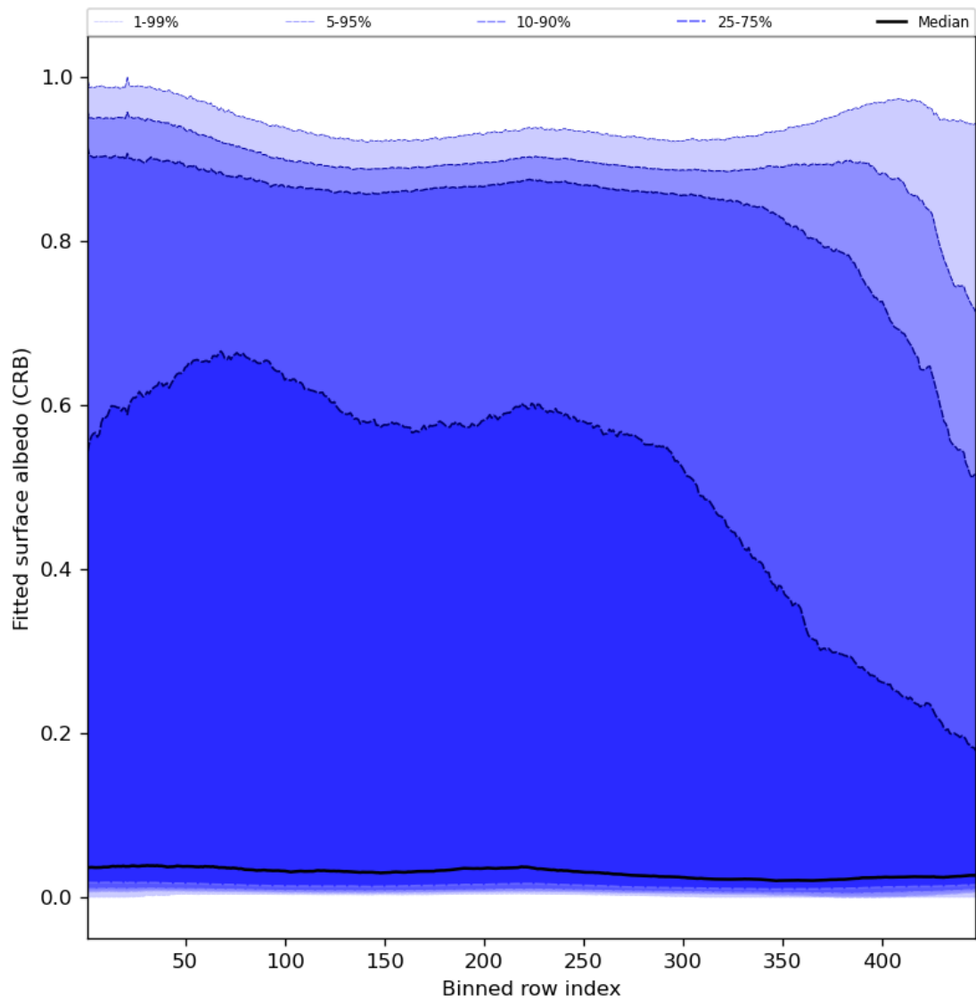
Figure 62: Along track statistics of “Fitted surface albedo (CRB)” for 2024-02-13 to 2024-02-15
