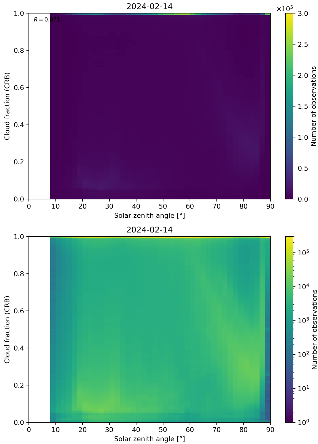
Figure 101: Scatter density plot of “Solar zenith angle” against “Cloud fraction (CRB)” for 2024-02-13 to 2024-02-15.
