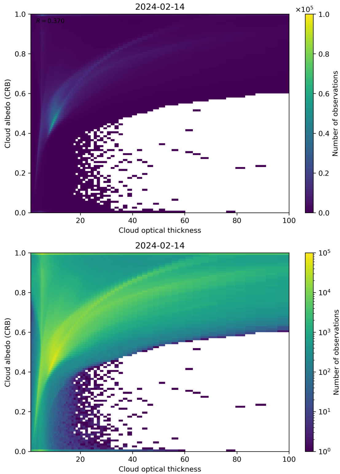
Figure 82: Scatter density plot of “Cloud optical thickness” against “Cloud albedo (CRB)” for 2024-02-13 to 2024-02-15.
