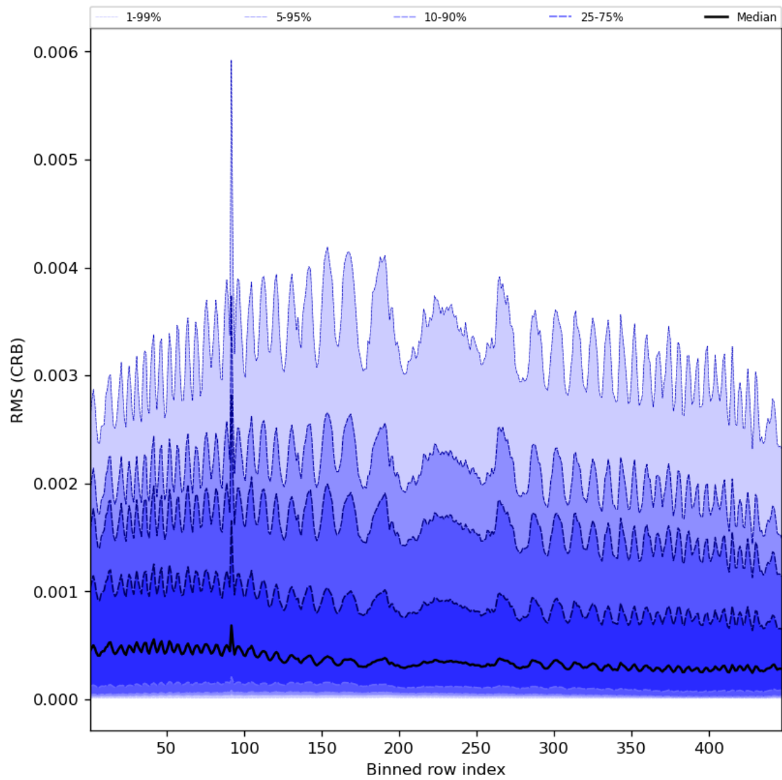
Figure 64: Along track statistics of “RMS (CRB)” for 2024-02-13 to 2024-02-15
