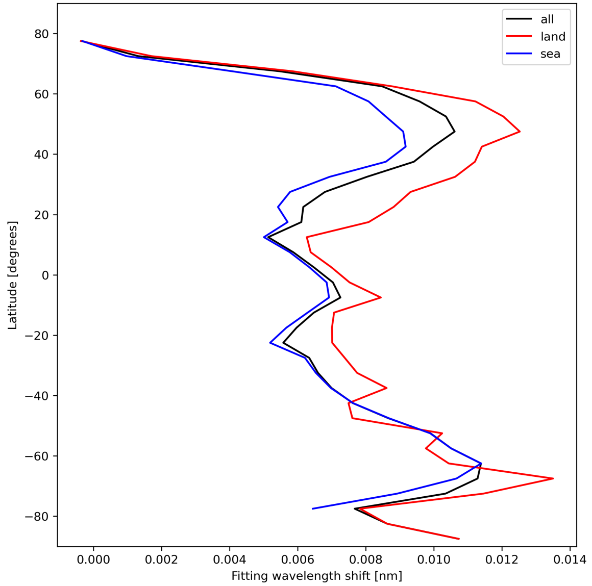
Figure 33: Zonal average of “Fitting wavelength shift” for 2024-02-13 to 2024-02-15.
