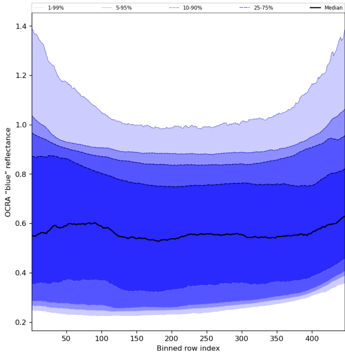
Figure 67: Along track statistics of “OCRA “blue” reflectance” for 2024-02-13 to 2024-02-15
