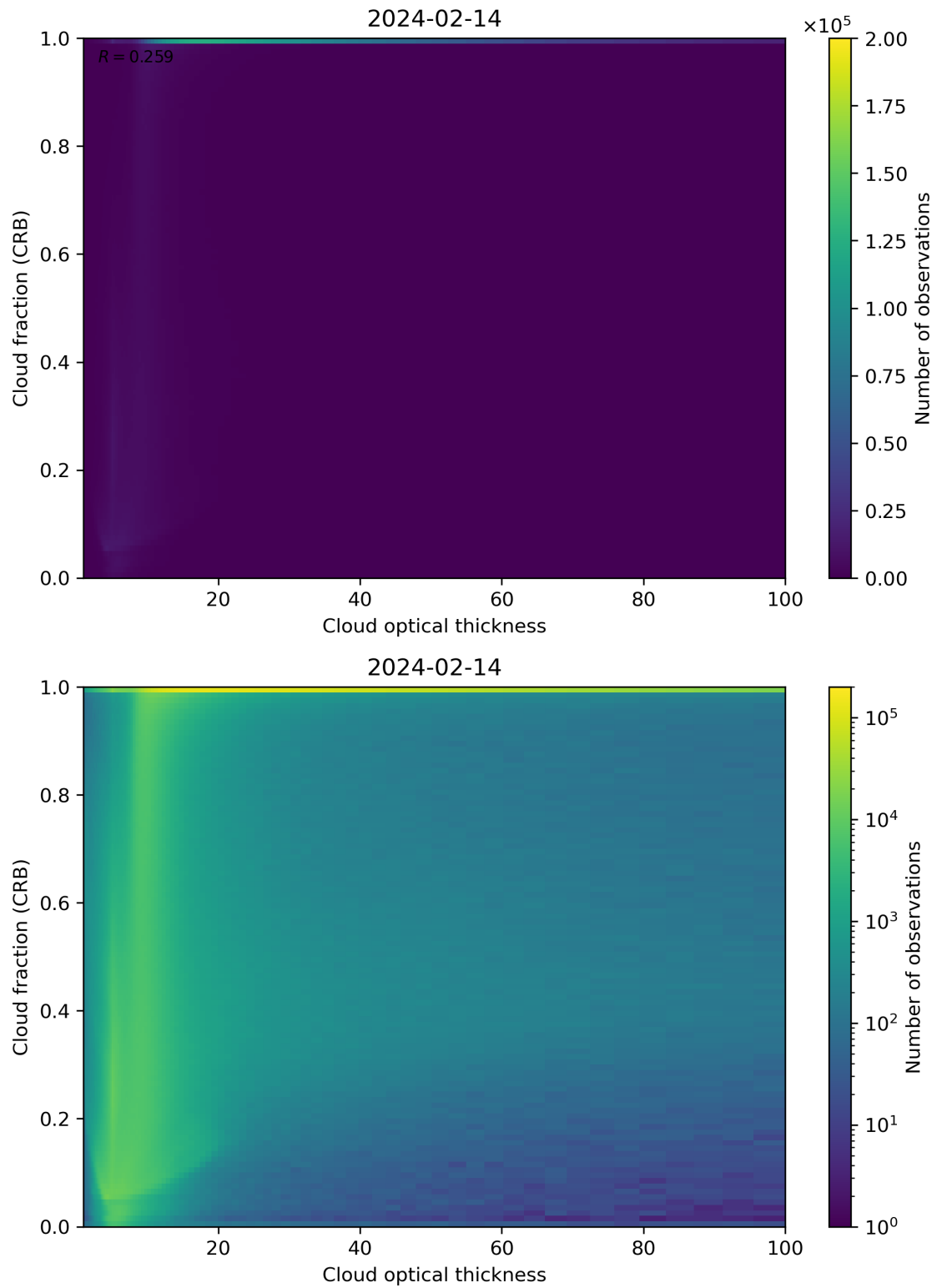
Figure 84: Scatter density plot of “Cloud optical thickness” against “Cloud fraction (CRB)” for 2024-02-13 to 2024-02-15.
