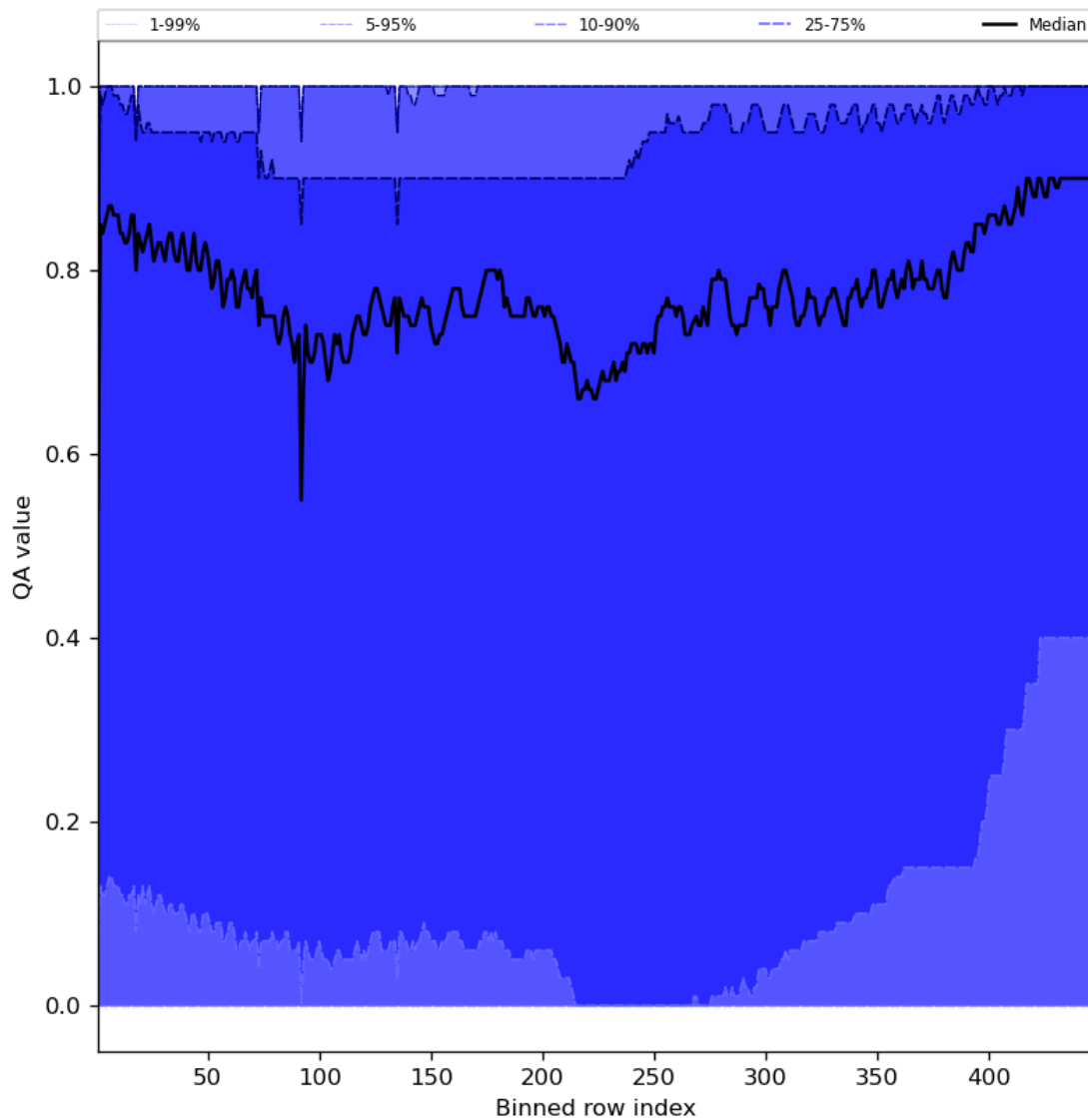
Figure 54: Along track statistics of “QA value” for 2024-02-13 to 2024-02-15
