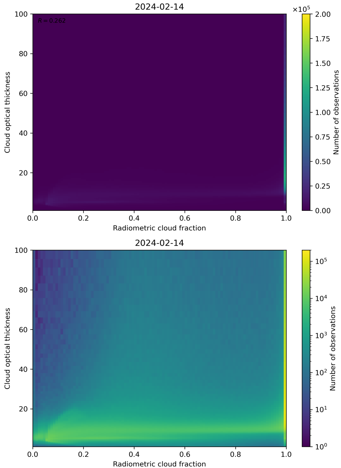
Figure 75: Scatter density plot of “Radiometric cloud fraction” against “Cloud optical thickness” for 2024-02-13 to 2024-02-15.
