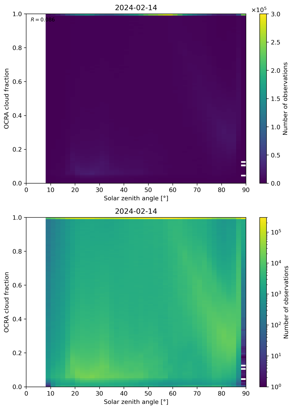
Figure 100: Scatter density plot of “Solar zenith angle” against “OCRA cloud fraction” for 2024-02-13 to 2024-02-15.
