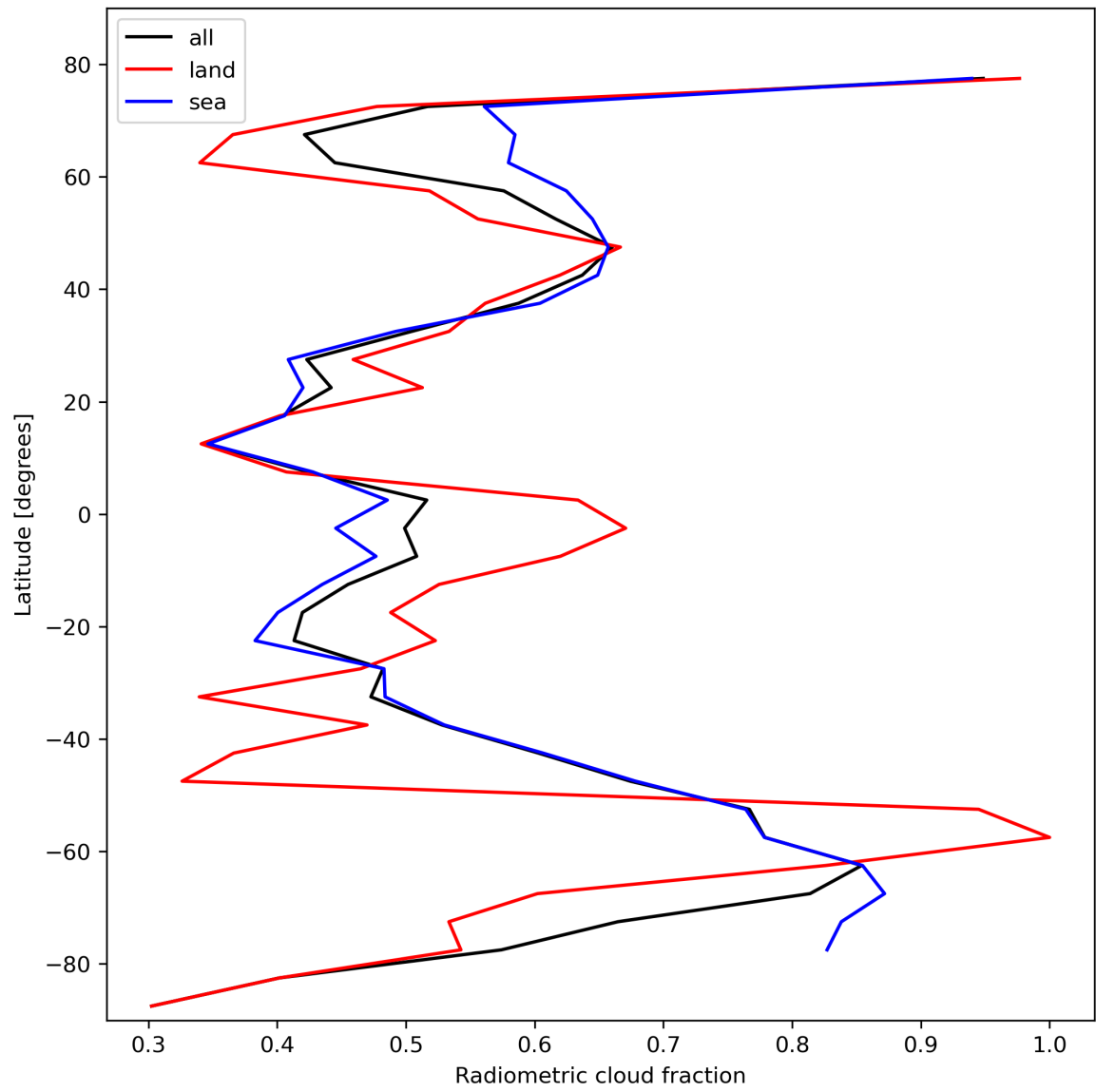
Figure 23: Zonal average of “Radiometric cloud fraction” for 2024-02-13 to 2024-02-15.
