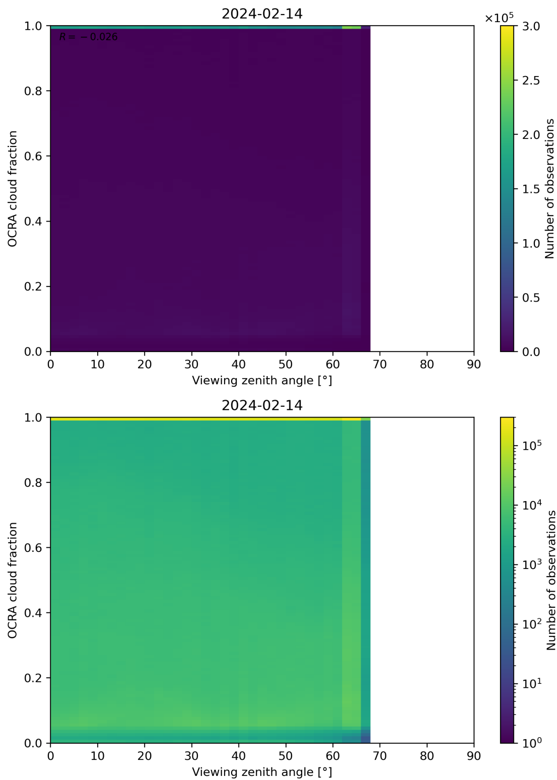
Figure 108: Scatter density plot of “Viewing zenith angle” against “OCRA cloud fraction” for 2024-02-13 to 2024-02-15.
