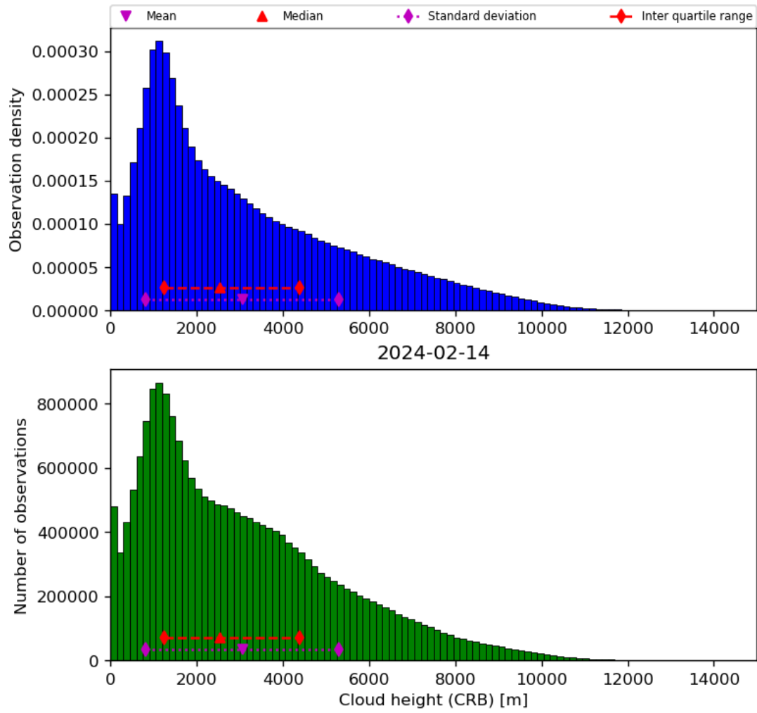
Figure 43: Histogram of “Cloud height (CRB)” for 2024-02-13 to 2024-02-15
