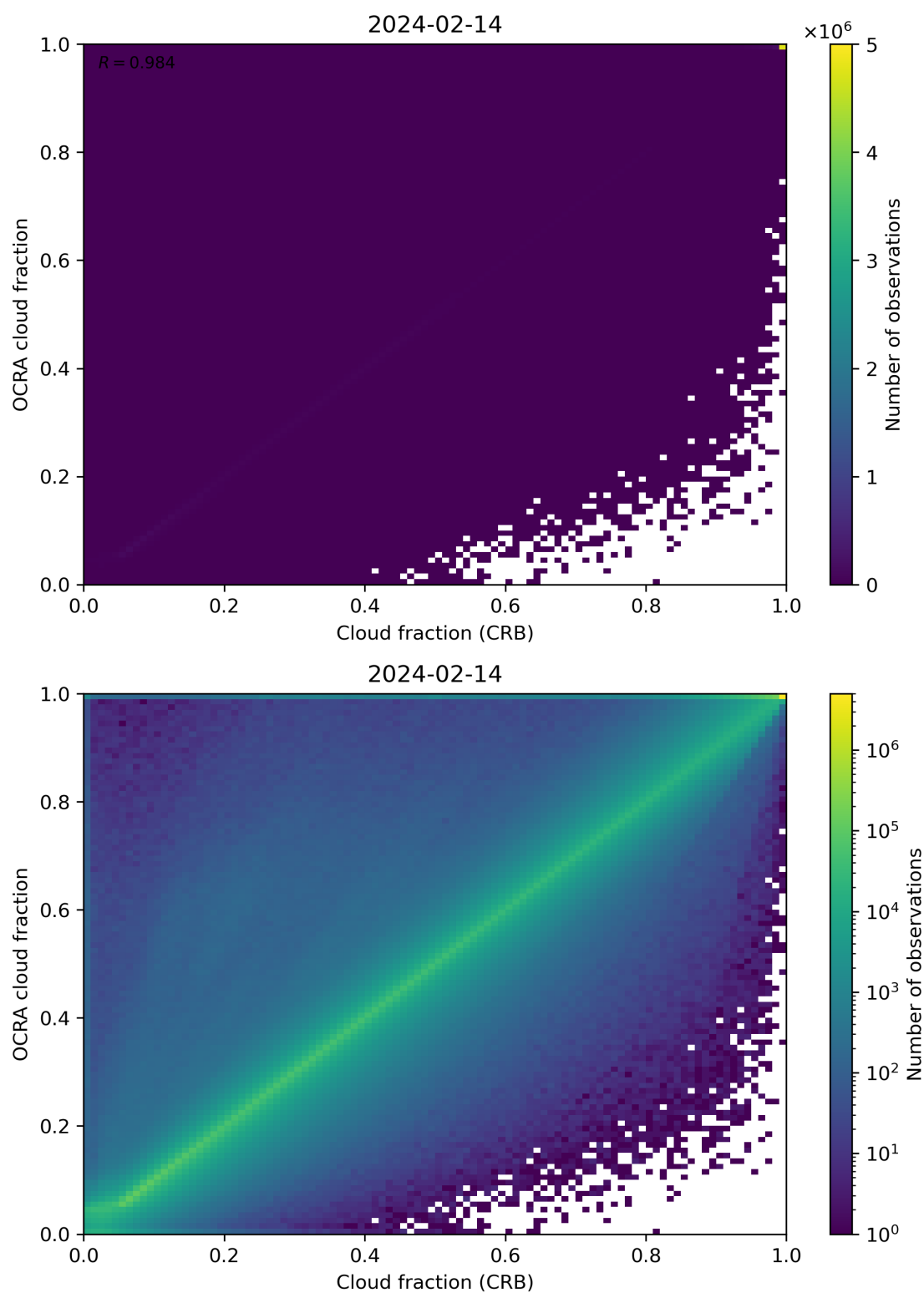
Figure 78: Scatter density plot of “Cloud fraction (CRB)” against “OCRA cloud fraction” for 2024-02-13 to 2024-02-15.
