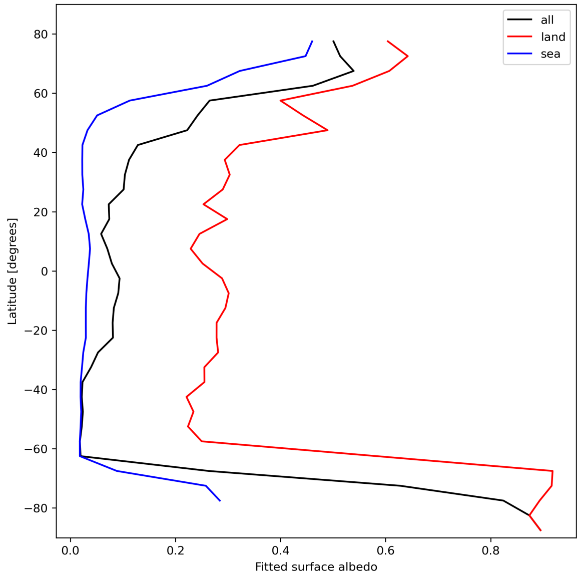
Figure 29: Zonal average of “Fitted surface albedo” for 2024-02-13 to 2024-02-15.
