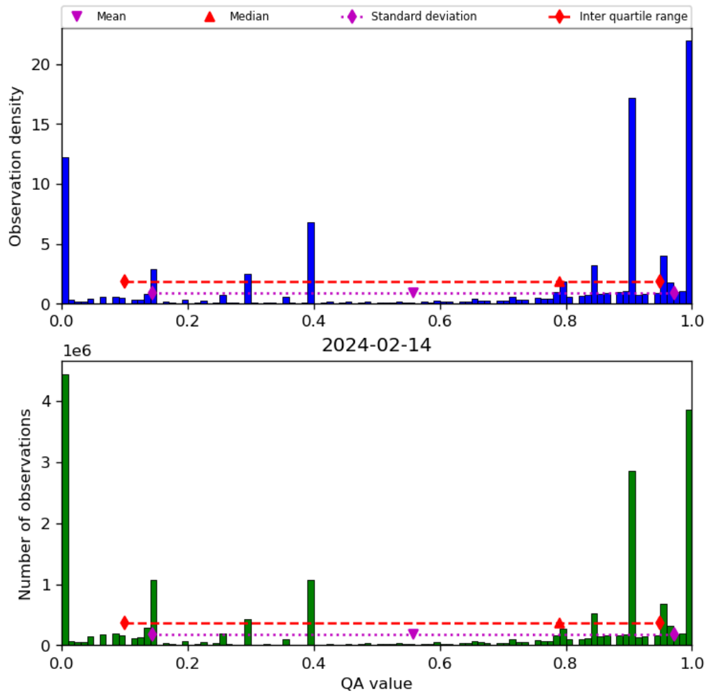
Figure 38: Histogram of “QA value” for 2024-02-13 to 2024-02-15
