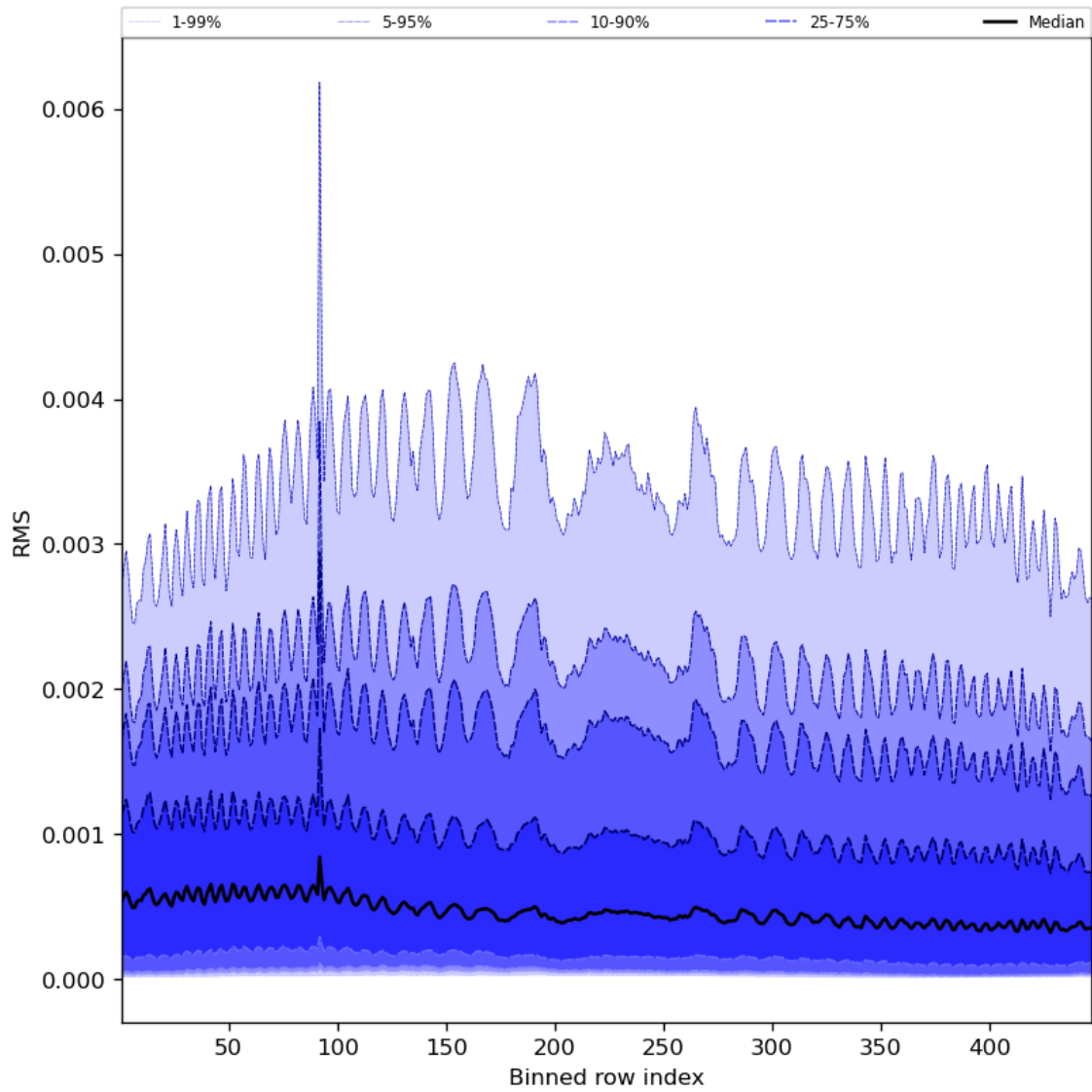
Figure 63: Along track statistics of “RMS” for 2024-02-13 to 2024-02-15
