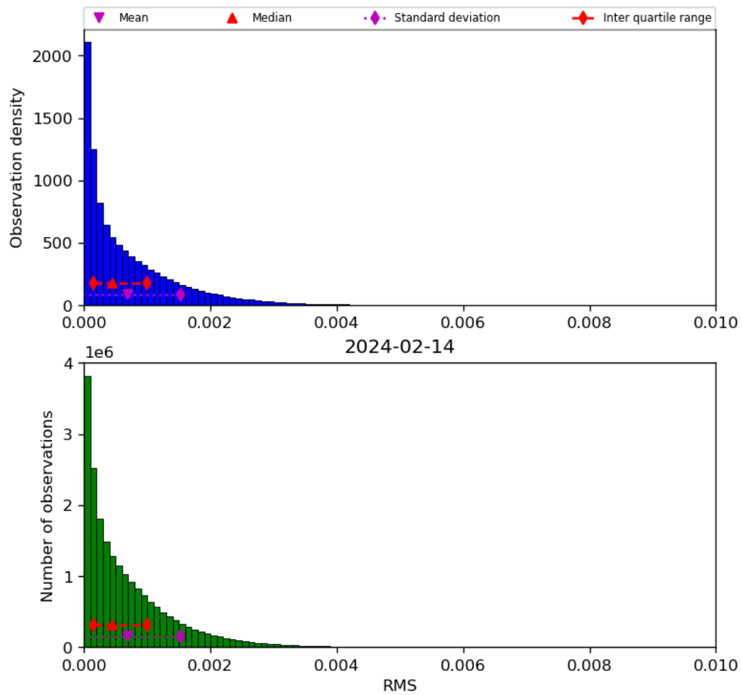
Figure 47: Histogram of “RMS” for 2024-02-13 to 2024-02-15
