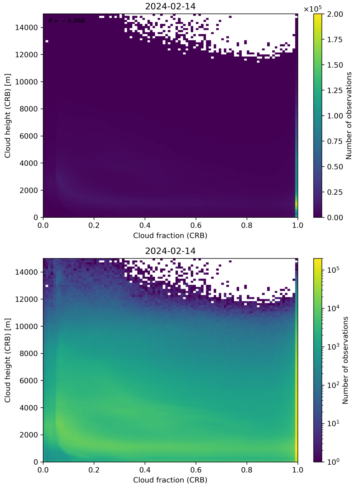
Figure 79: Scatter density plot of “Cloud fraction (CRB)” against “Cloud height (CRB)” for 2024-02-13 to 2024-02-15.
