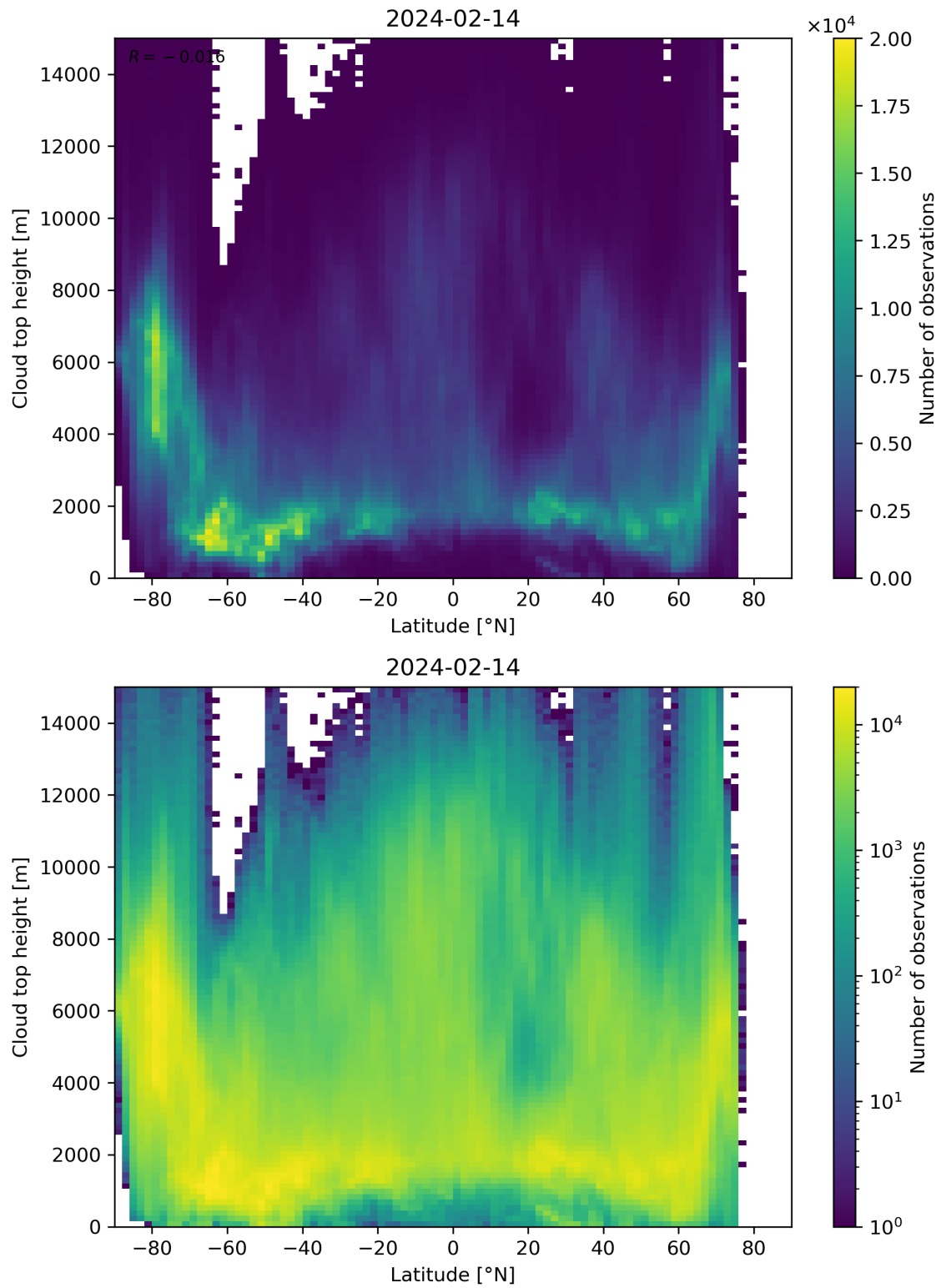
Figure 97: Scatter density plot of “Latitude” against “Cloud top height” for 2024-02-13 to 2024-02-15.
