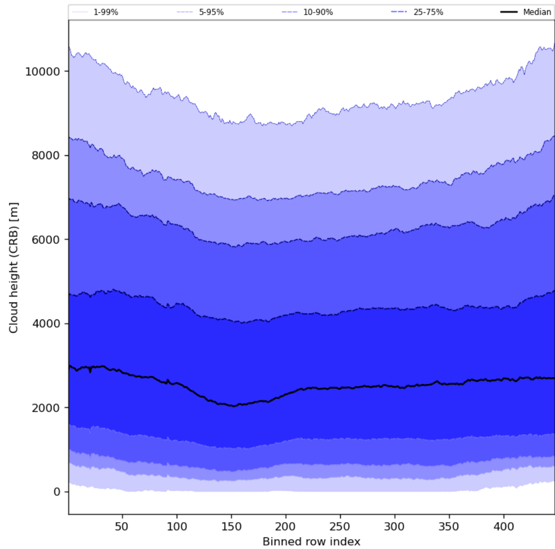
Figure 59: Along track statistics of “Cloud height (CRB)” for 2024-02-13 to 2024-02-15
