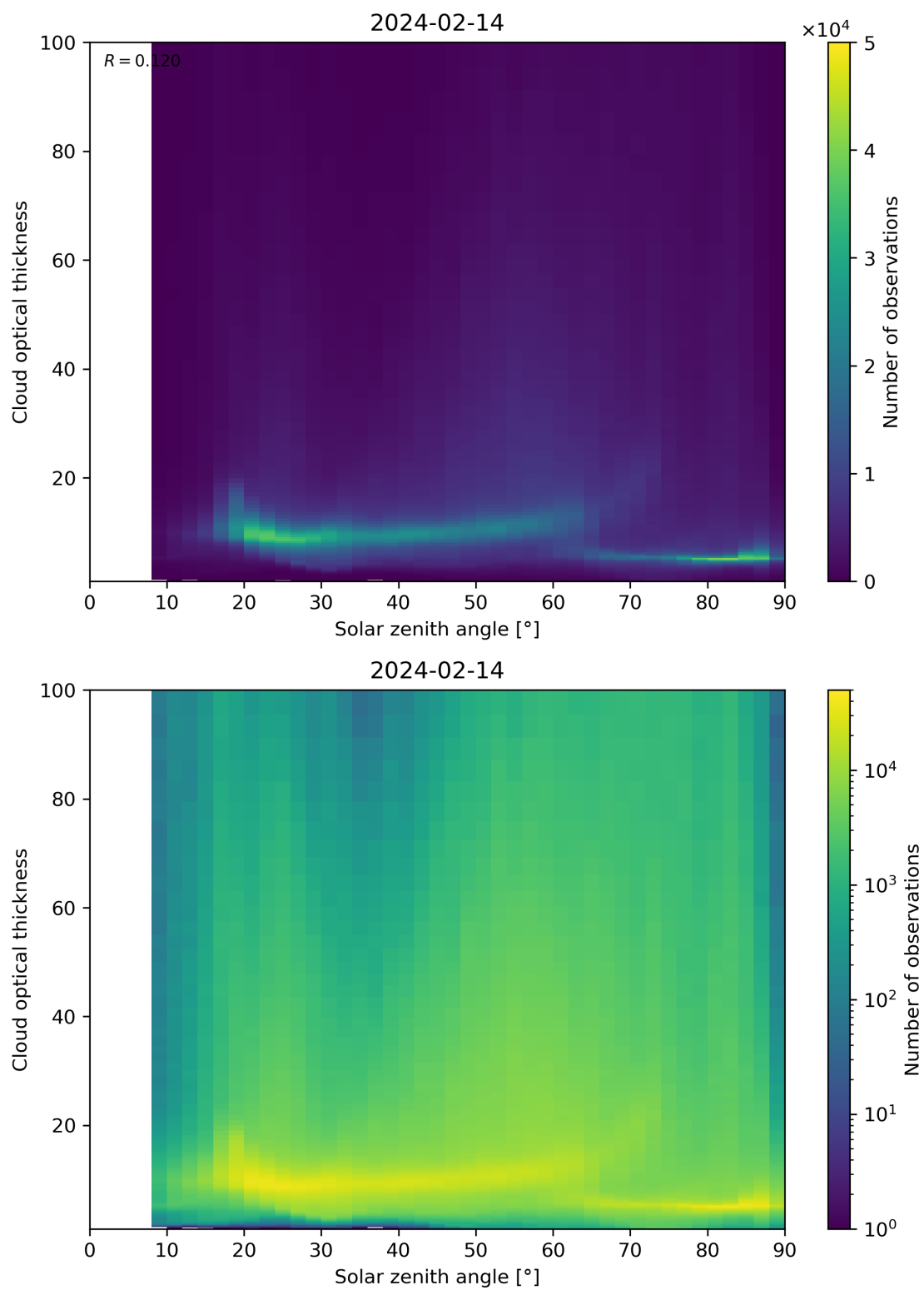
Figure 103: Scatter density plot of “Solar zenith angle” against “Cloud optical thickness” for 2024-02-13 to 2024-02-15.
