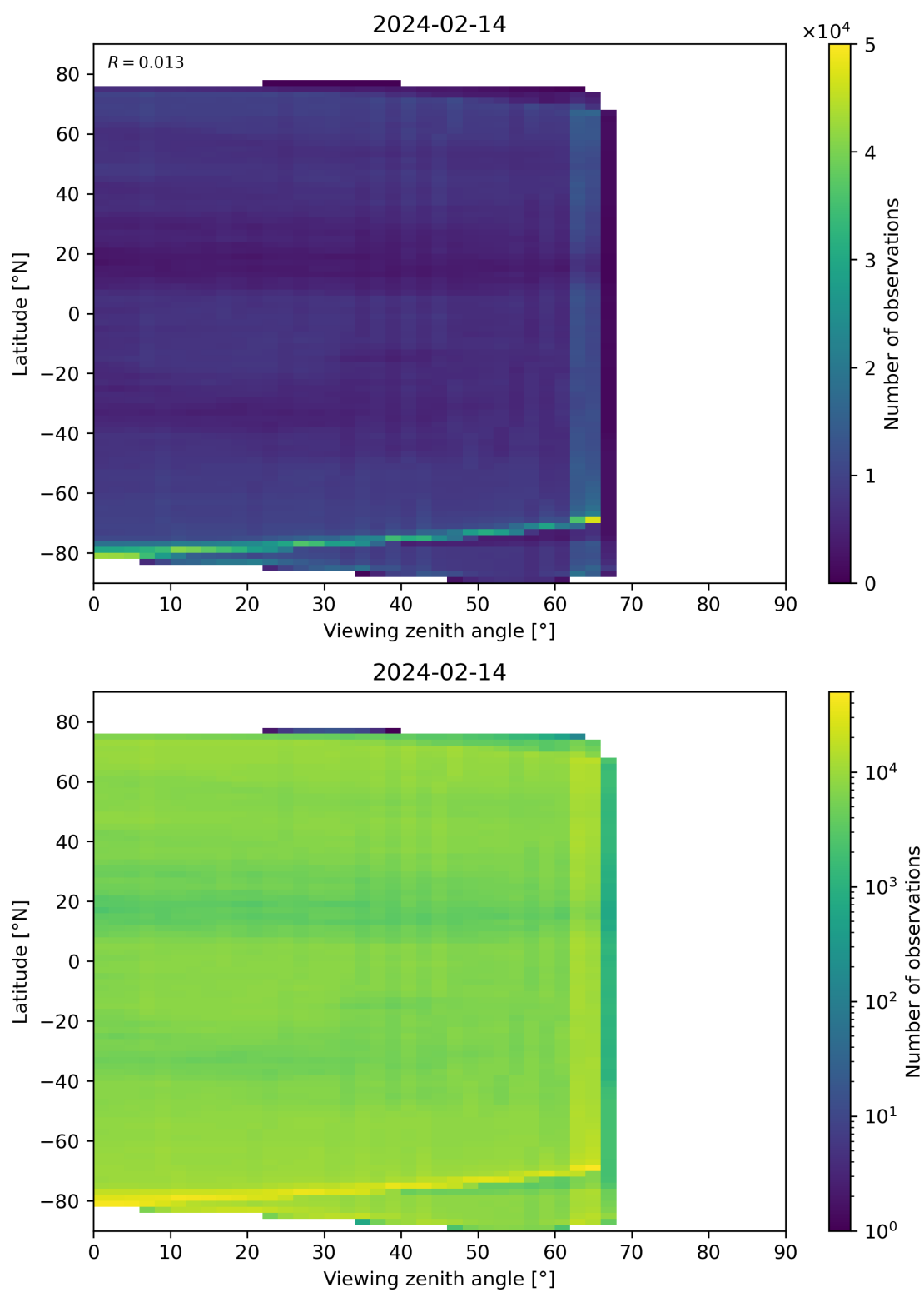
Figure 113: Scatter density plot of “Viewing zenith angle” against “Latitude” for 2024-02-13 to 2024-02-15.
