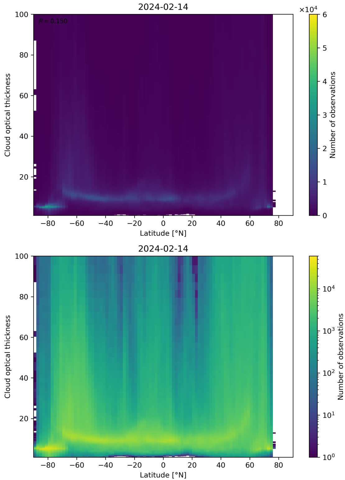
Figure 96: Scatter density plot of “Latitude” against “Cloud optical thickness” for 2024-02-13 to 2024-02-15.
