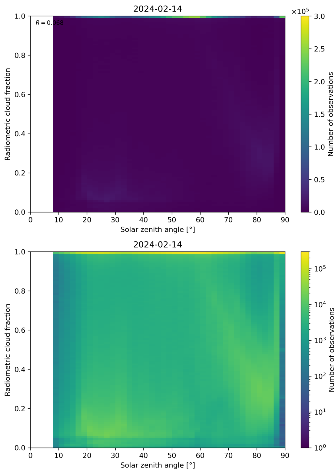
Figure 99: Scatter density plot of “Solar zenith angle” against “Radiometric cloud fraction” for 2024-02-13 to 2024-02-15.
