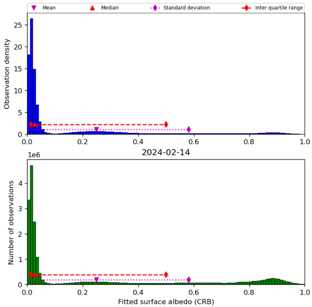
Figure 46: Histogram of “Fitted surface albedo (CRB)” for 2024-02-13 to 2024-02-15
