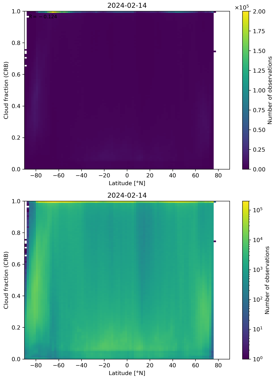
Figure 94: Scatter density plot of “Latitude” against “Cloud fraction (CRB)” for 2024-02-13 to 2024-02-15.
