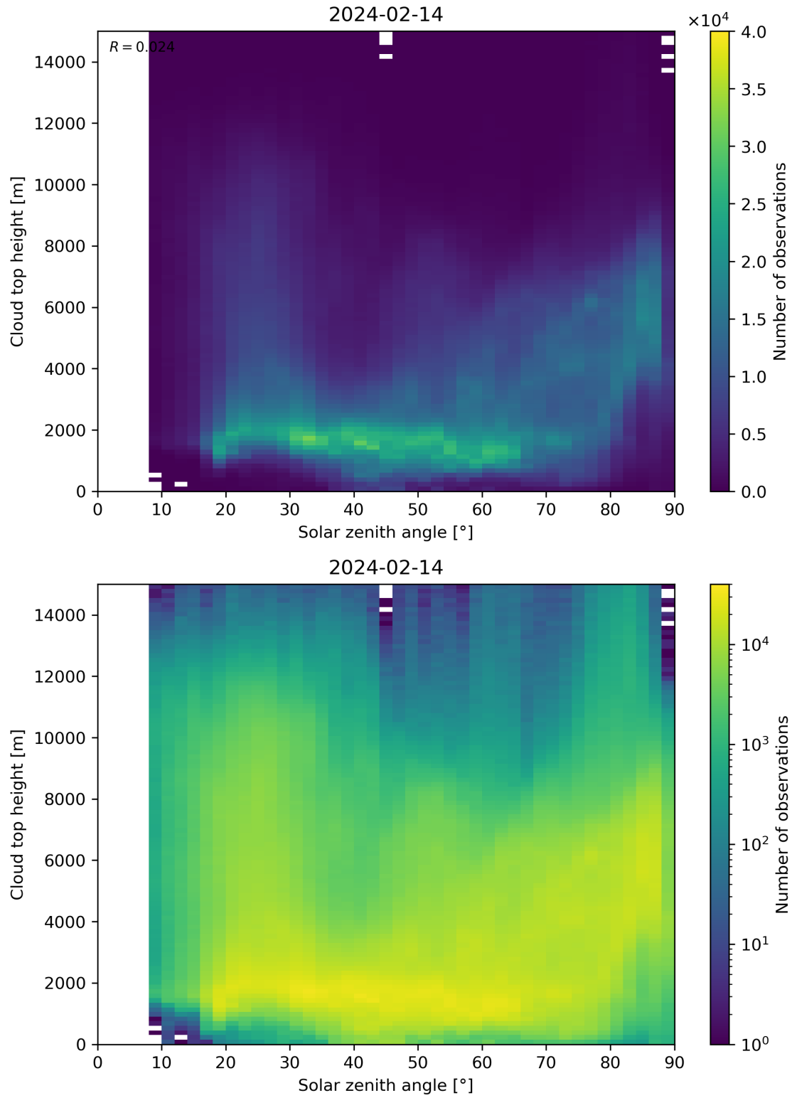
Figure 104: Scatter density plot of “Solar zenith angle” against “Cloud top height” for 2024-02-13 to 2024-02-15.
