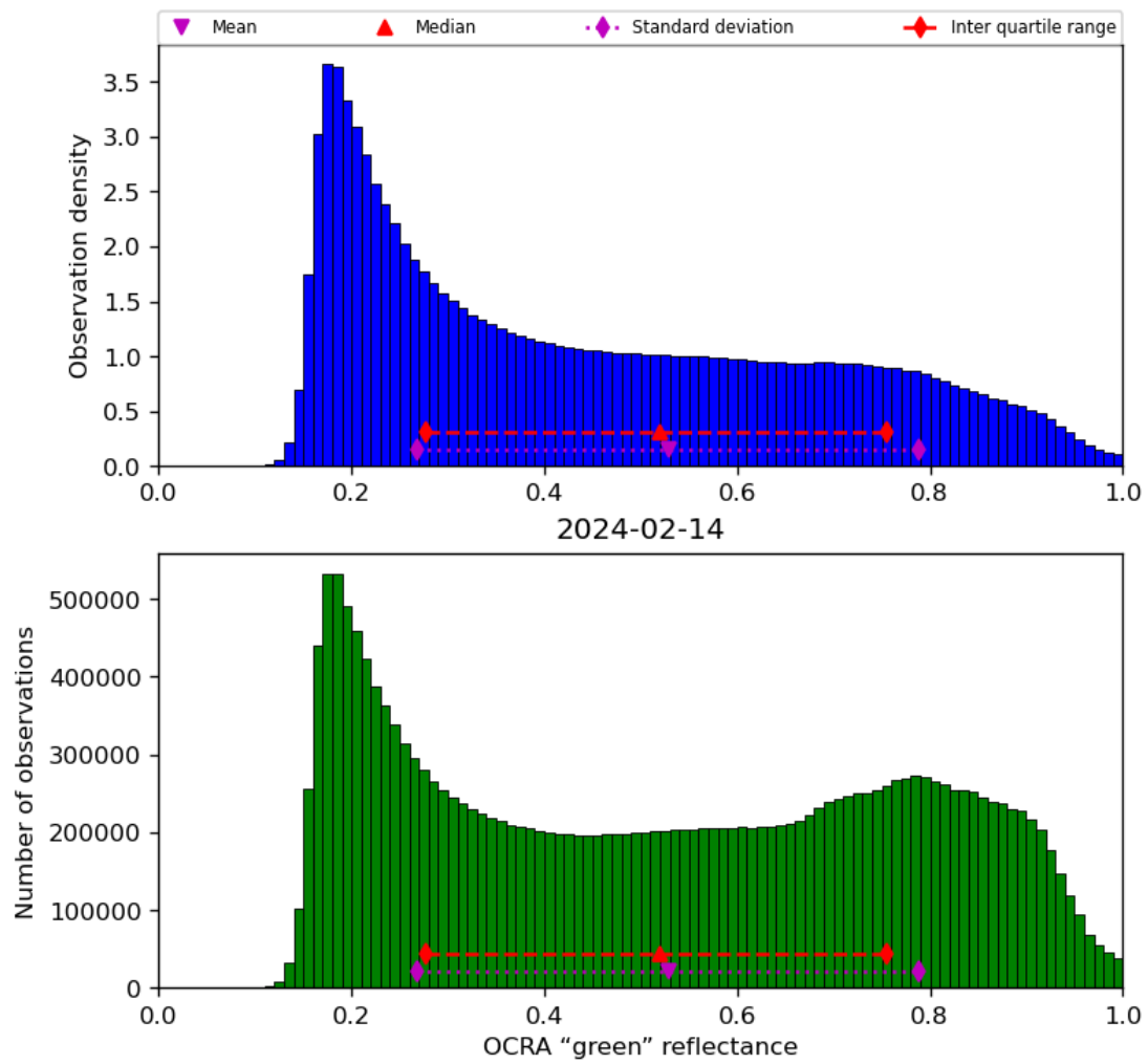
Figure 52: Histogram of “OCRA “green” reflectance” for 2024-02-13 to 2024-02-15
