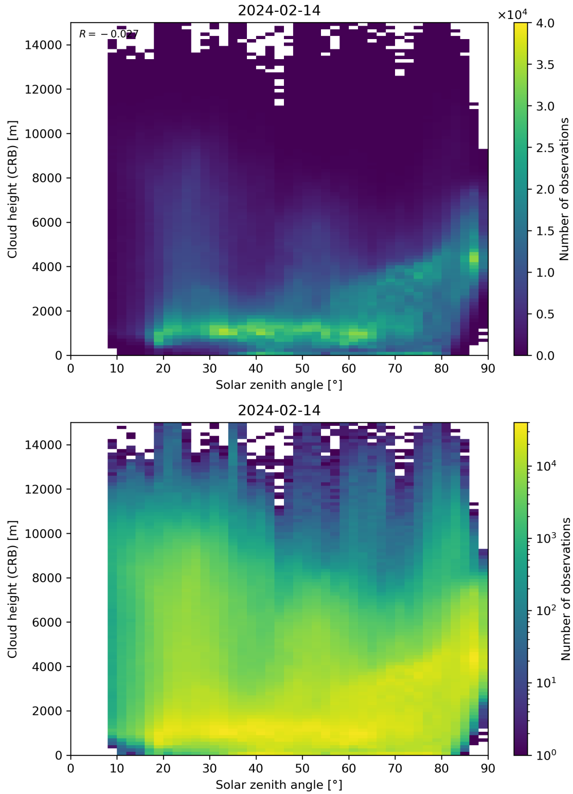
Figure 102: Scatter density plot of “Solar zenith angle” against “Cloud height (CRB)” for 2024-02-13 to 2024-02-15.
