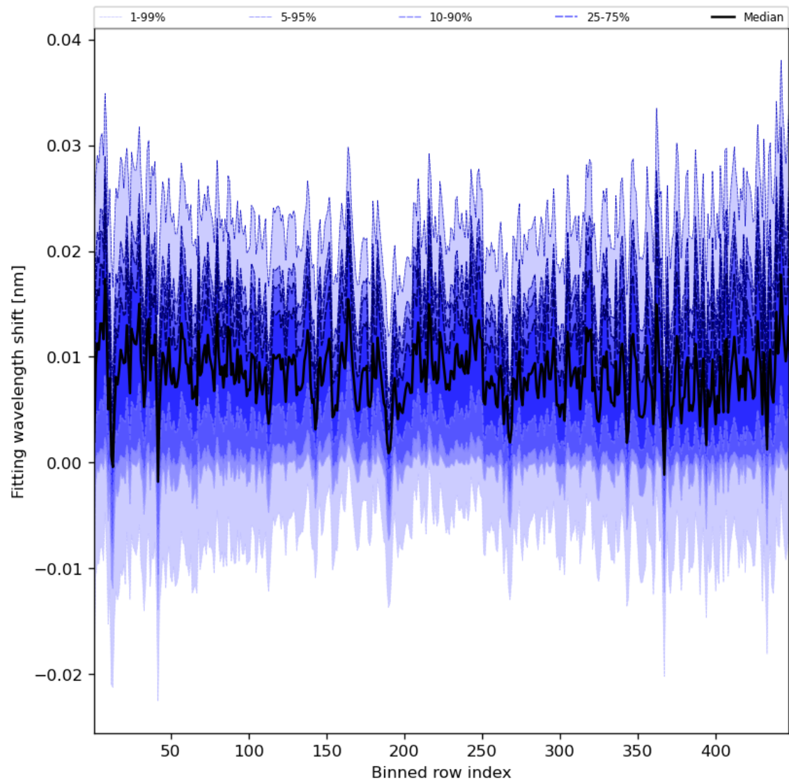
Figure 65: Along track statistics of “Fitting wavelength shift” for 2024-02-13 to 2024-02-15
