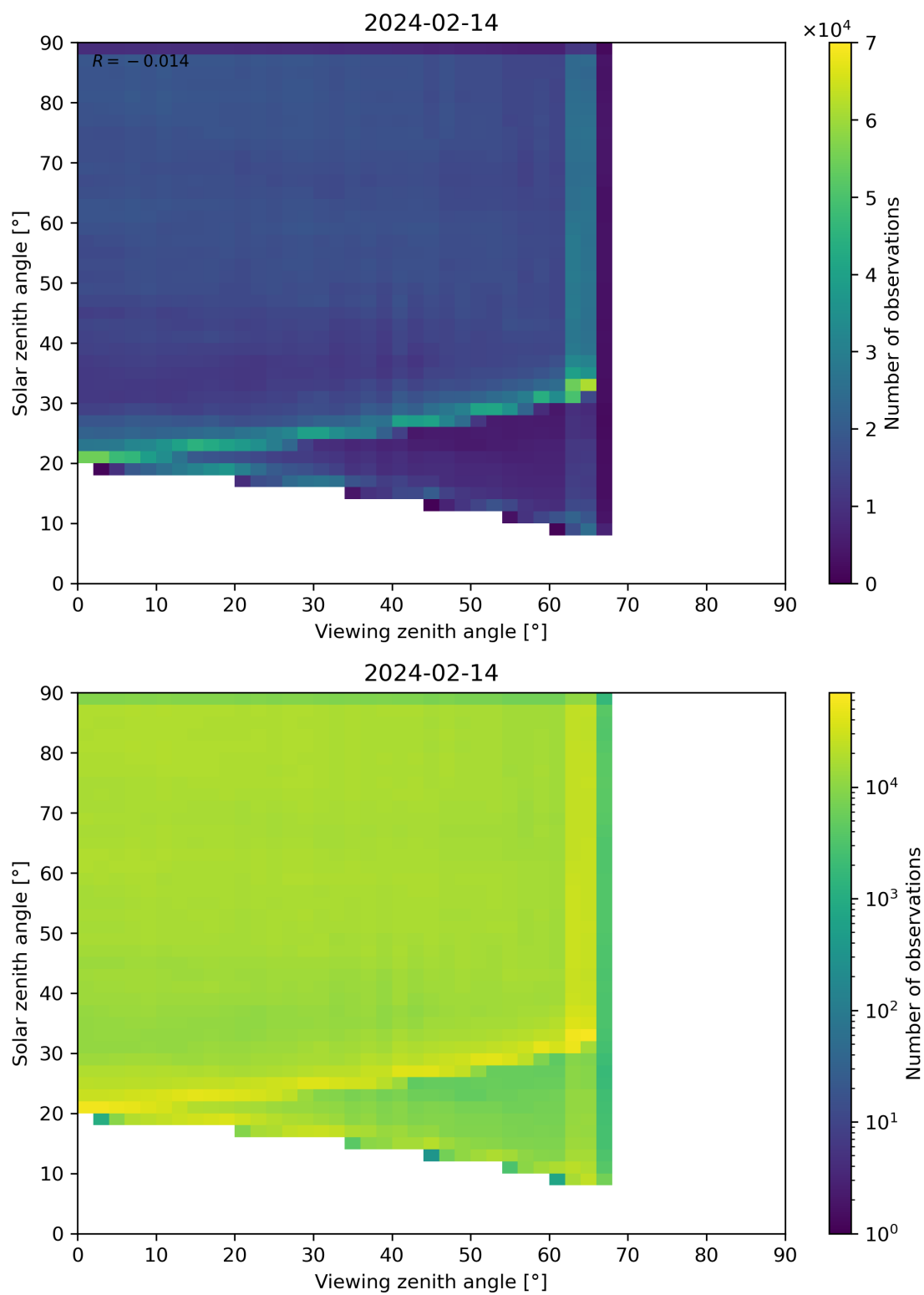
Figure 114: Scatter density plot of “Viewing zenith angle” against “Solar zenith angle” for 2024-02-13 to 2024-02-15.
