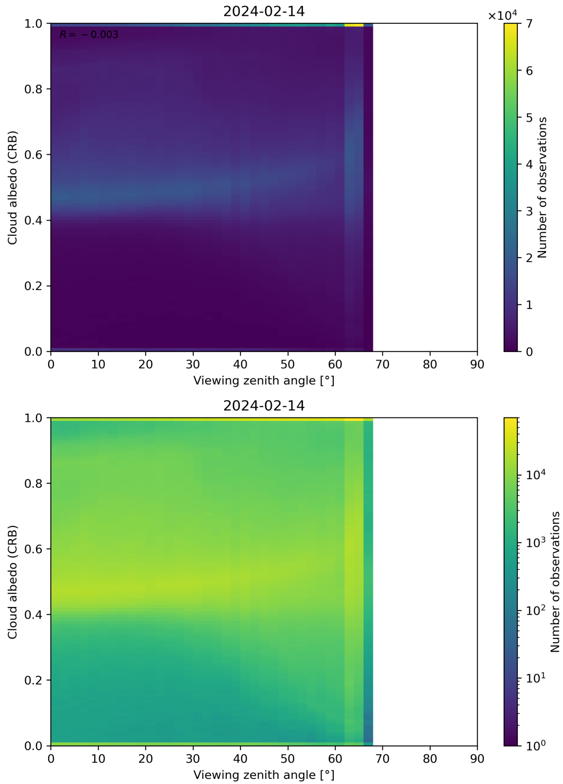
Figure 106: Scatter density plot of “Viewing zenith angle” against “Cloud albedo (CRB)” for 2024-02-13 to 2024-02-15.
