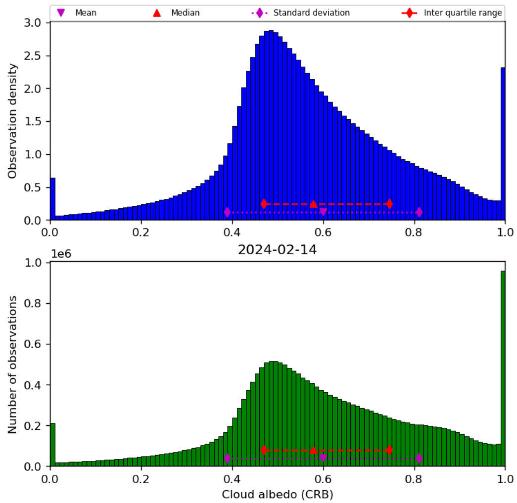
Figure 44: Histogram of “Cloud albedo (CRB)” for 2024-02-13 to 2024-02-15
