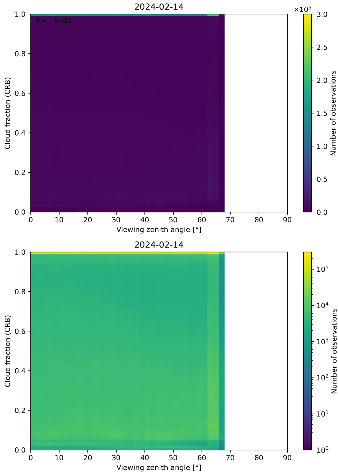
Figure 109: Scatter density plot of “Viewing zenith angle” against “Cloud fraction (CRB)” for 2024-02-13 to 2024-02-15.
