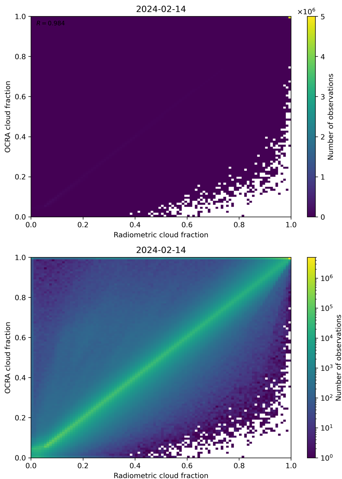
Figure 72: Scatter density plot of “Radiometric cloud fraction” against “OCRA cloud fraction” for 2024-02-13 to 2024-02-15.
