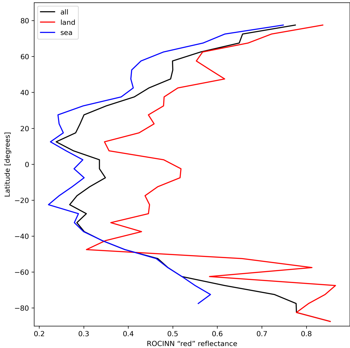
Figure 37: Zonal average of “ROCINN “red” reflectance” for 2024-02-13 to 2024-02-15.
