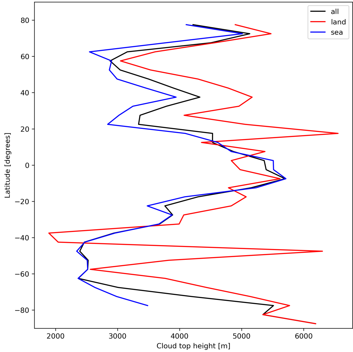
Figure 24: Zonal average of “Cloud top height” for 2024-02-13 to 2024-02-15.
