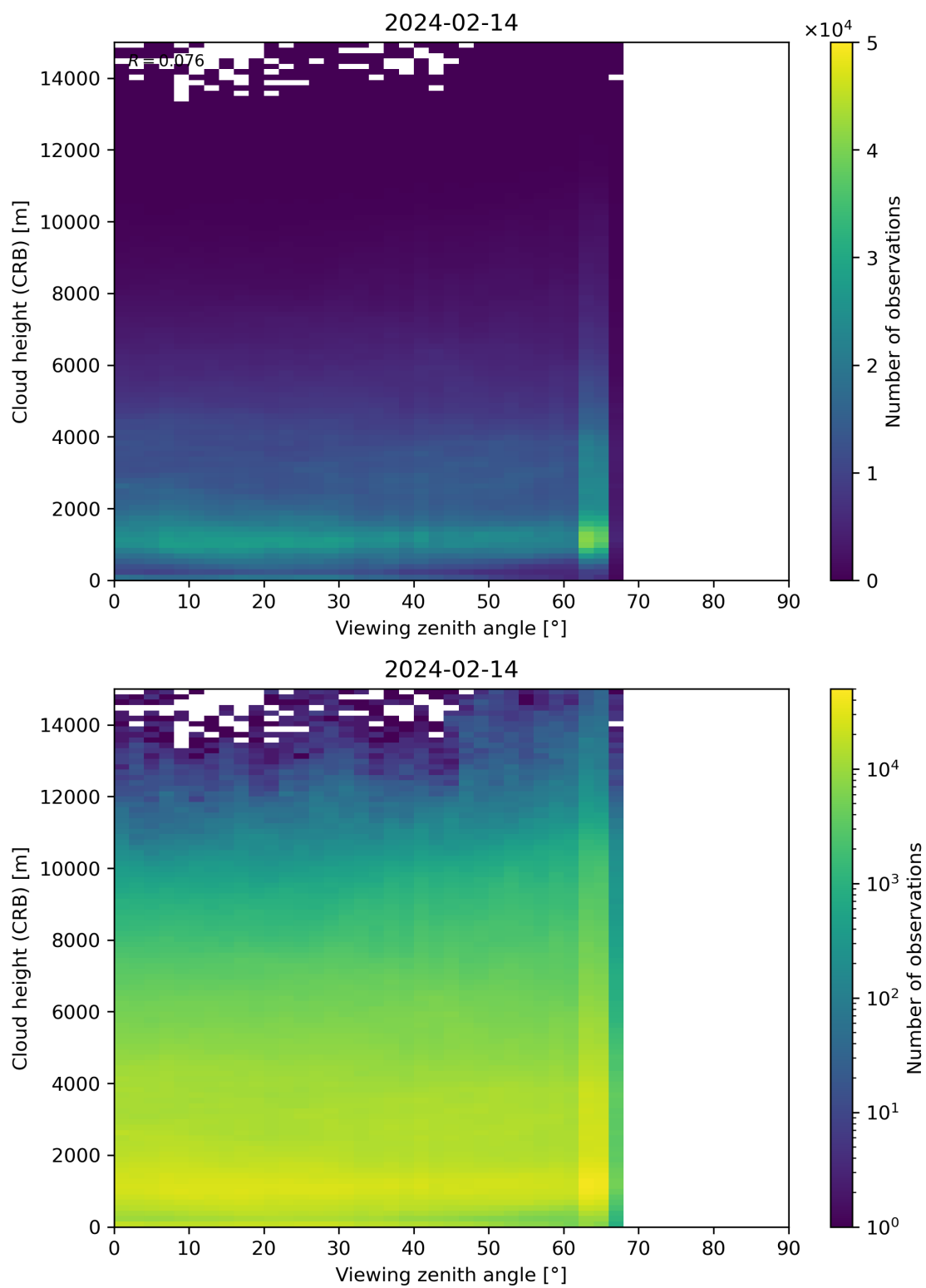
Figure 110: Scatter density plot of “Viewing zenith angle” against “Cloud height (CRB)” for 2024-02-13 to 2024-02-15.
