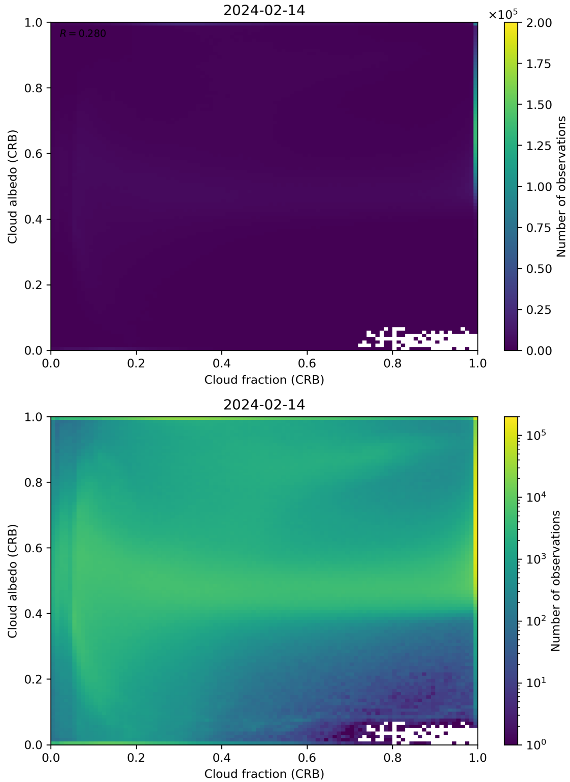
Figure 77: Scatter density plot of “Cloud fraction (CRB)” against “Cloud albedo (CRB)” for 2024-02-13 to 2024-02-15.
