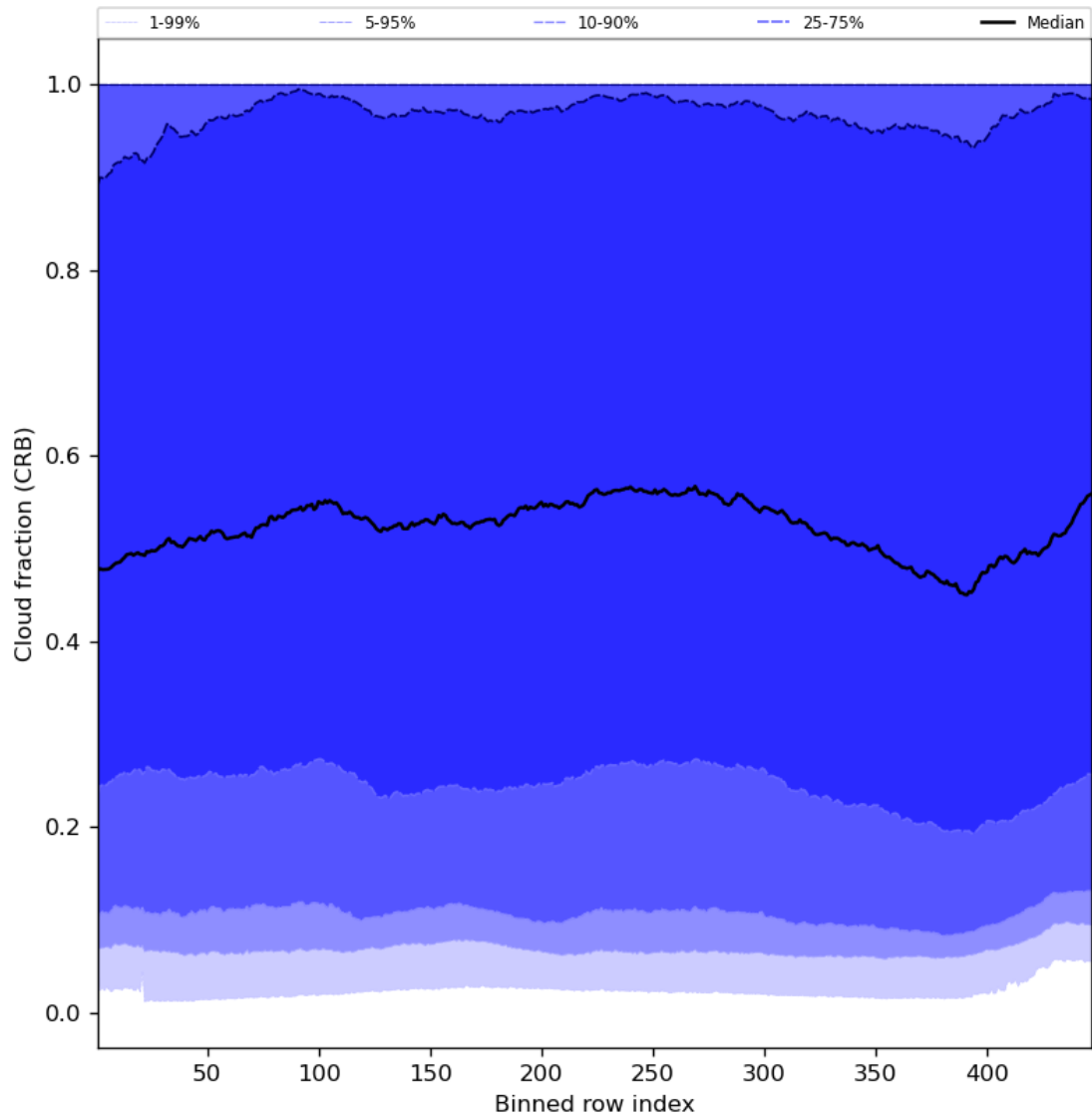
Figure 58: Along track statistics of “Cloud fraction (CRB)” for 2024-02-13 to 2024-02-15
