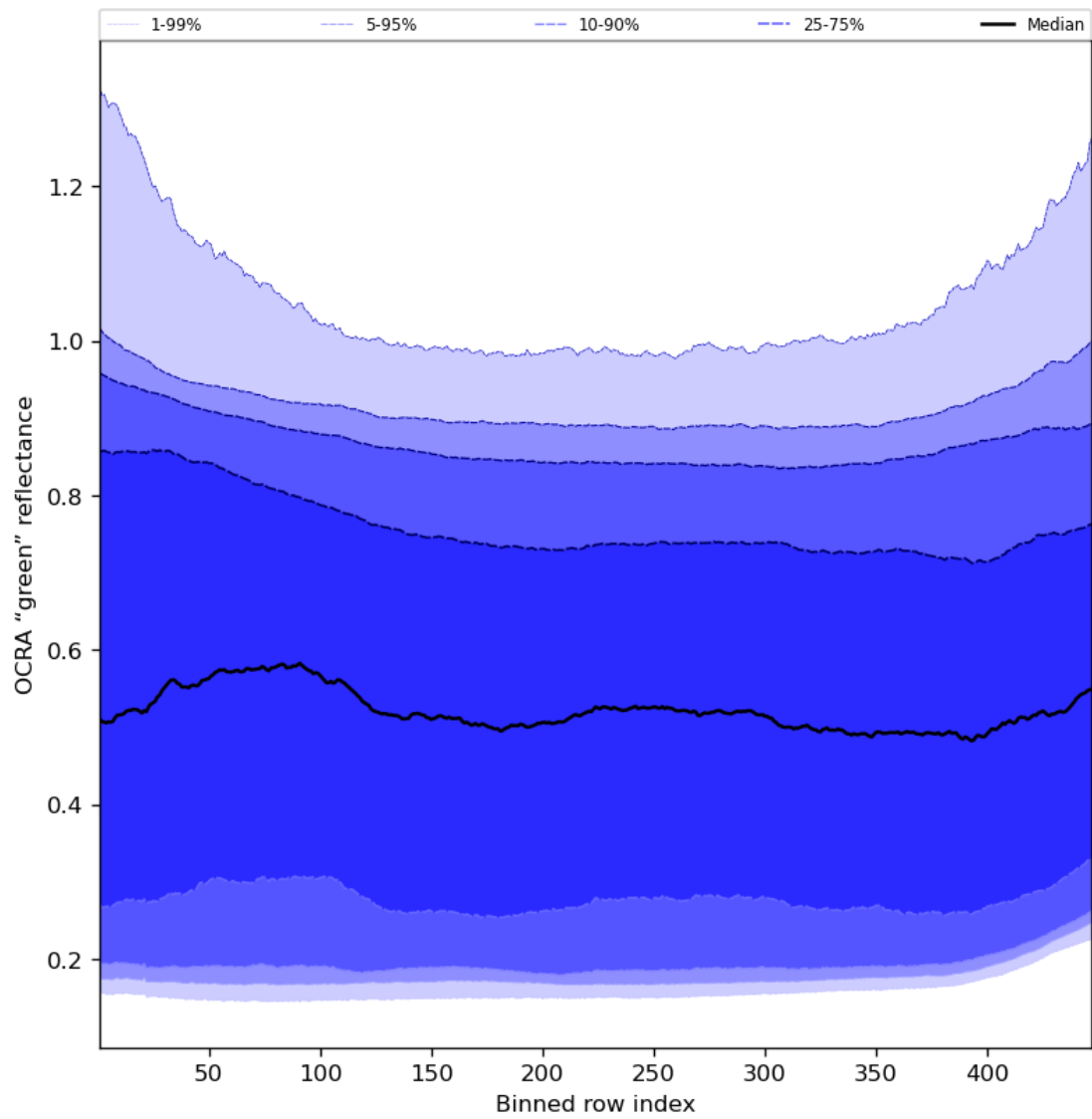
Figure 68: Along track statistics of “OCRA “green” reflectance” for 2024-02-13 to 2024-02-15
