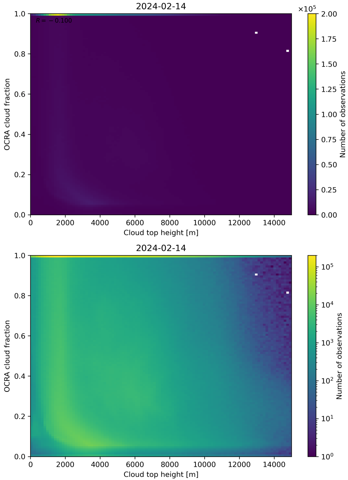
Figure 87: Scatter density plot of “Cloud top height” against “OCRA cloud fraction” for 2024-02-13 to 2024-02-15.
