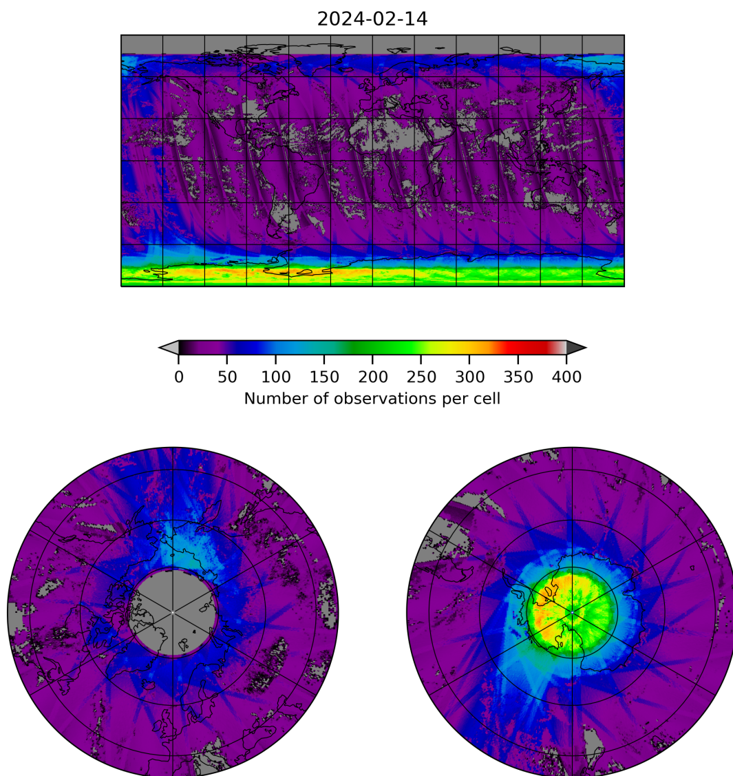
Figure 21: Map of the number of observations for 2024-02-13 to 2024-02-15
