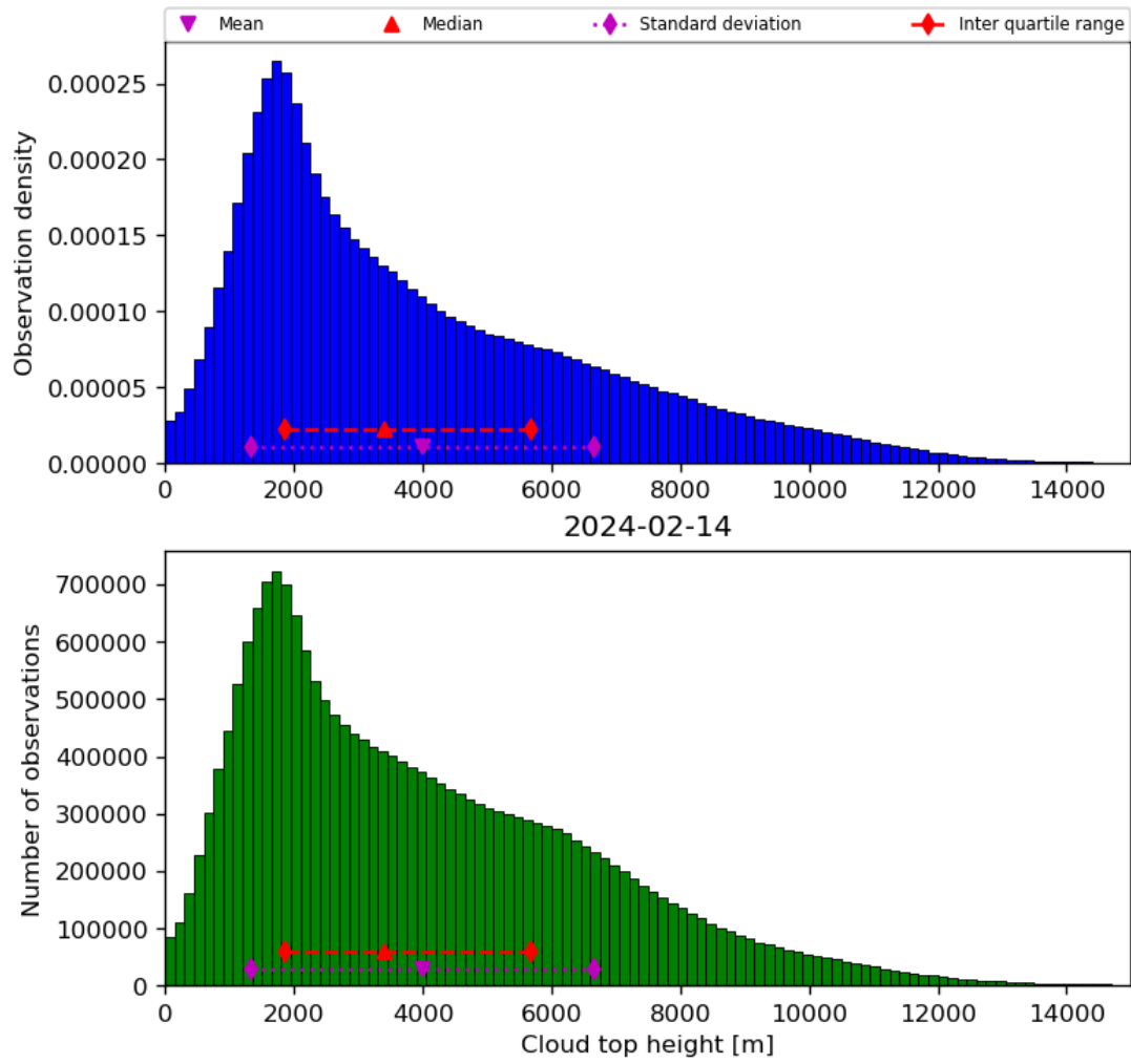
Figure 40: Histogram of “Cloud top height” for 2024-02-13 to 2024-02-15
