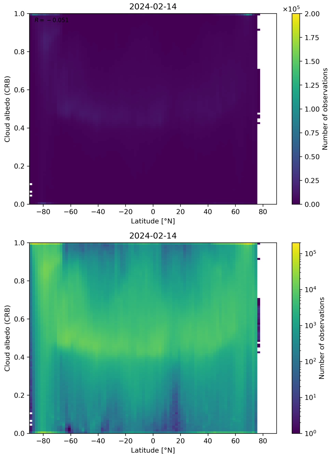
Figure 91: Scatter density plot of “Latitude” against “Cloud albedo (CRB)” for 2024-02-13 to 2024-02-15.
