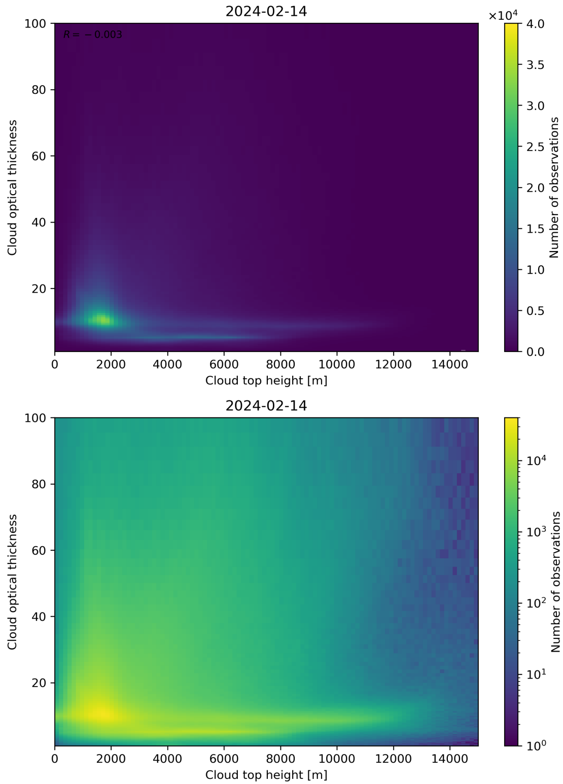
Figure 90: Scatter density plot of “Cloud top height” against “Cloud optical thickness” for 2024-02-13 to 2024-02-15.
