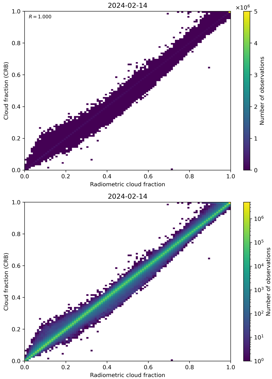
Figure 73: Scatter density plot of “Radiometric cloud fraction” against “Cloud fraction (CRB)” for 2024-02-13 to 2024-02-15.
