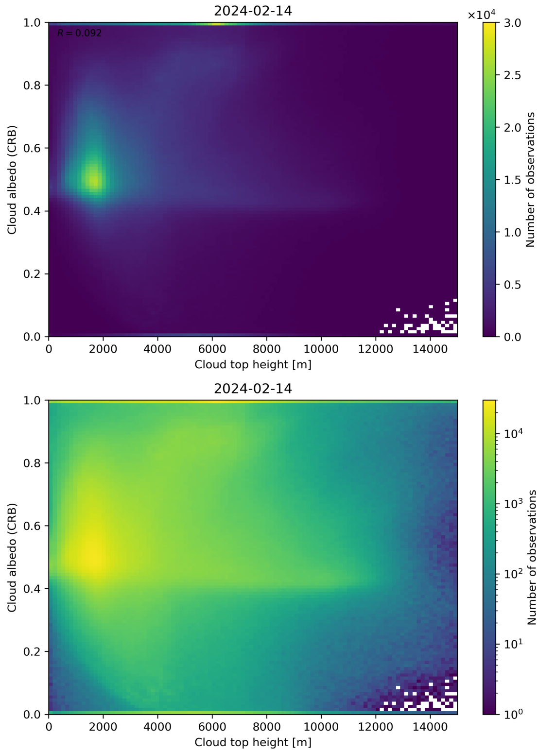
Figure 86: Scatter density plot of “Cloud top height” against “Cloud albedo (CRB)” for 2024-02-13 to 2024-02-15.
