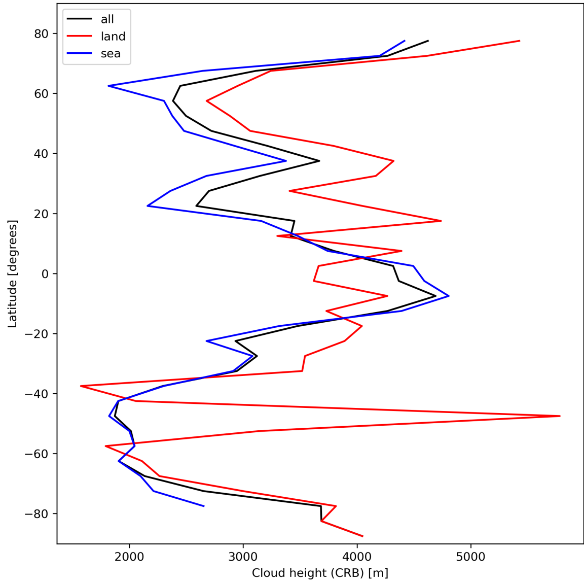
Figure 27: Zonal average of “Cloud height (CRB)” for 2024-02-13 to 2024-02-15.
