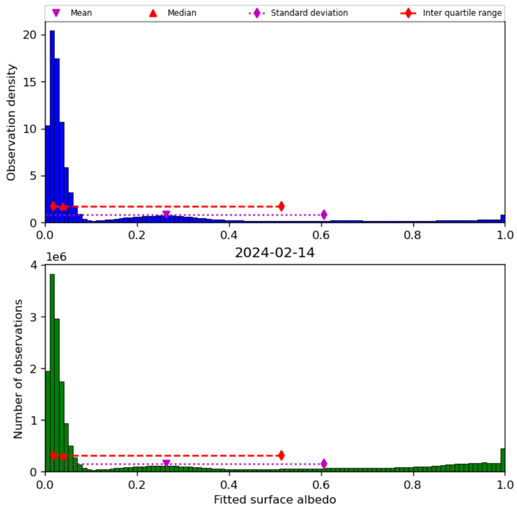
Figure 45: Histogram of “Fitted surface albedo” for 2024-02-13 to 2024-02-15
