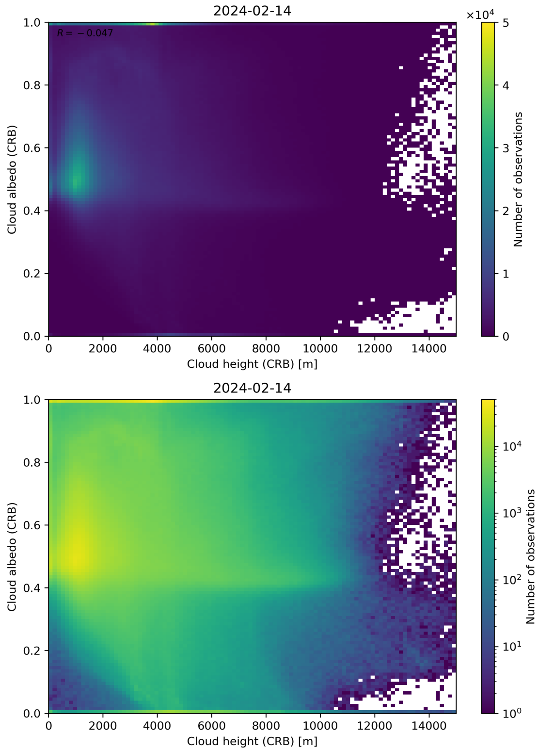
Figure 80: Scatter density plot of “Cloud height (CRB)” against “Cloud albedo (CRB)” for 2024-02-13 to 2024-02-15.
