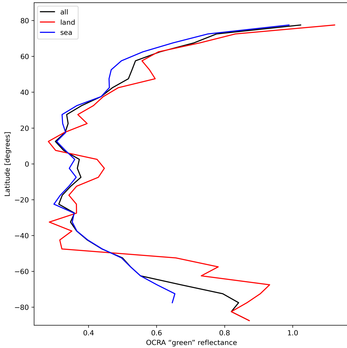
Figure 36: Zonal average of “OCRA “green” reflectance” for 2024-02-13 to 2024-02-15.
