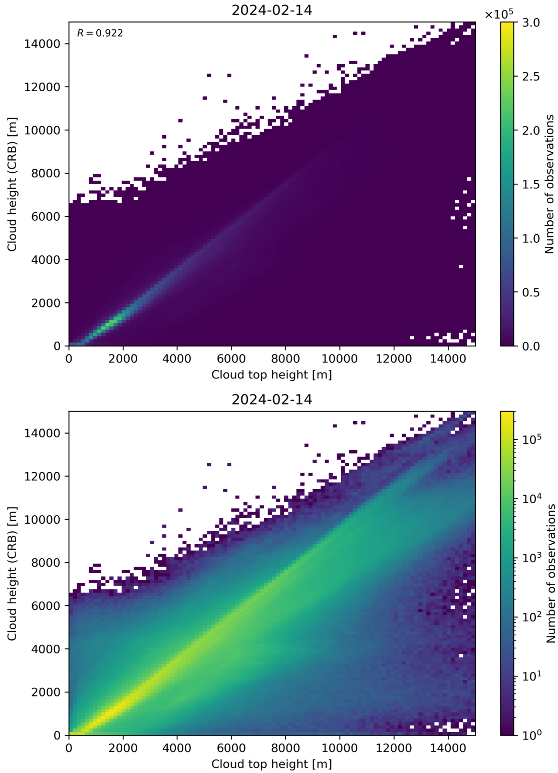
Figure 89: Scatter density plot of “Cloud top height” against “Cloud height (CRB)” for 2024-02-13 to 2024-02-15.
