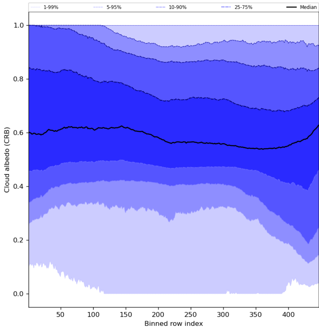
Figure 60: Along track statistics of “Cloud albedo (CRB)” for 2024-02-13 to 2024-02-15
