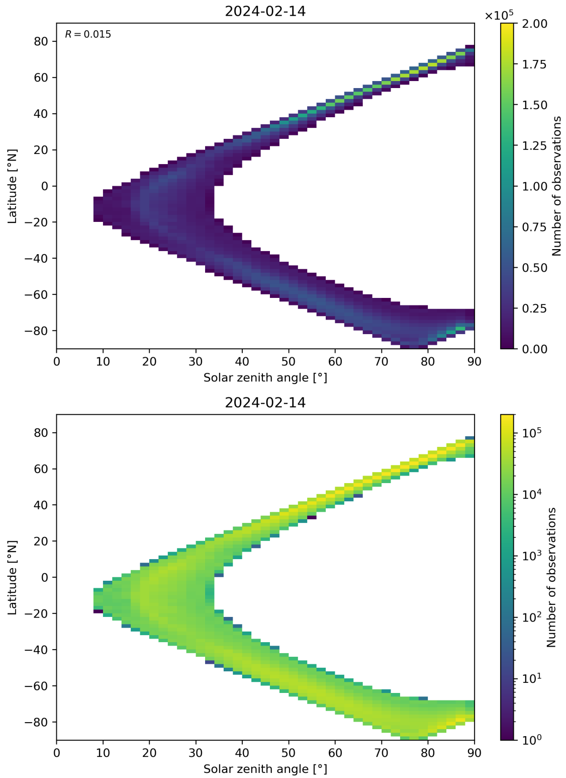
Figure 105: Scatter density plot of “Solar zenith angle” against “Latitude” for 2024-02-13 to 2024-02-15.
