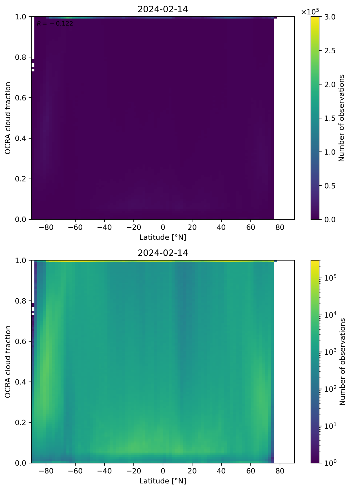
Figure 93: Scatter density plot of “Latitude” against “OCRA cloud fraction” for 2024-02-13 to 2024-02-15.
