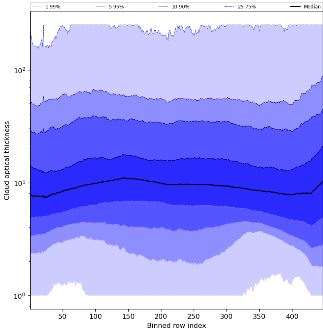
Figure 57: Along track statistics of “Cloud optical thickness” for 2024-02-13 to 2024-02-15
