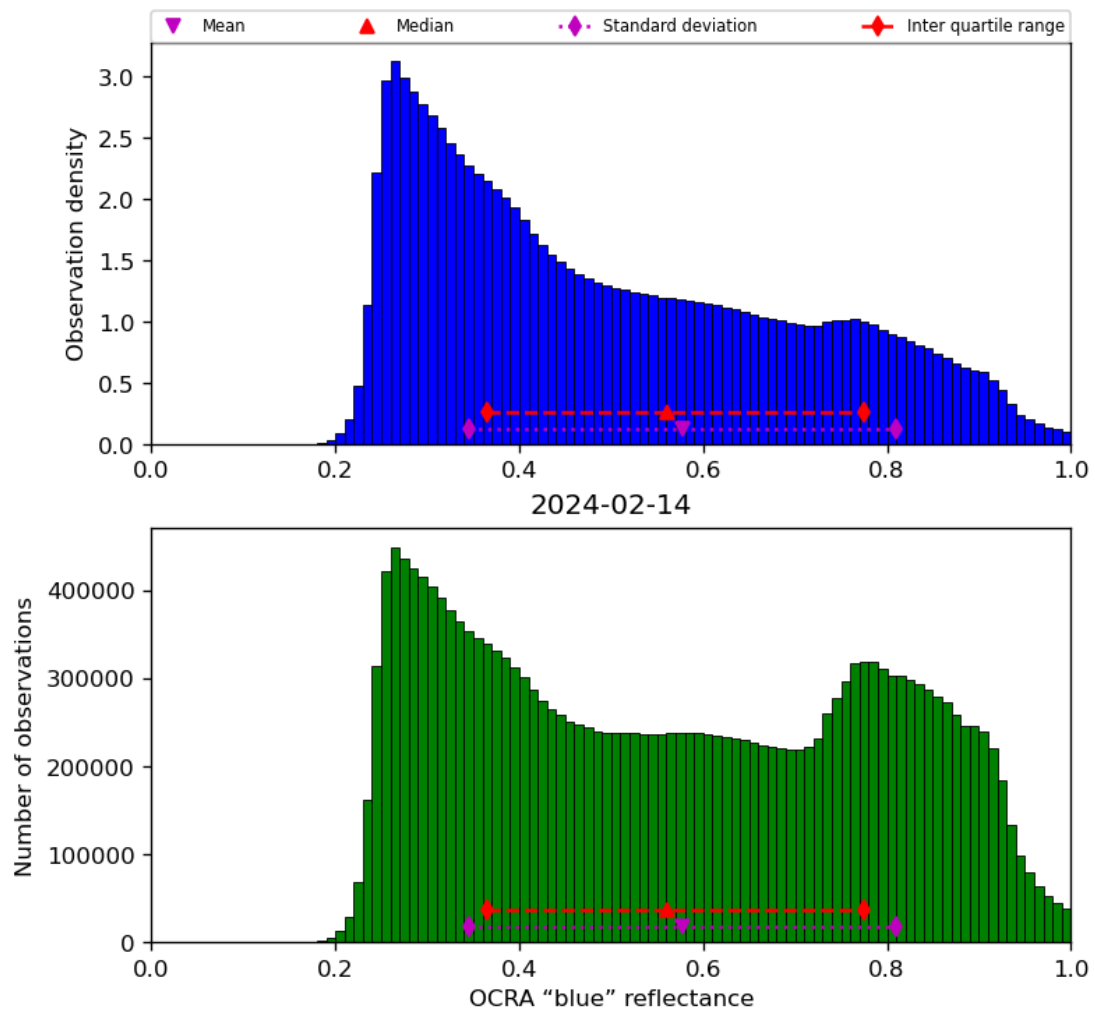
Figure 51: Histogram of “OCRA “blue” reflectance” for 2024-02-13 to 2024-02-15
