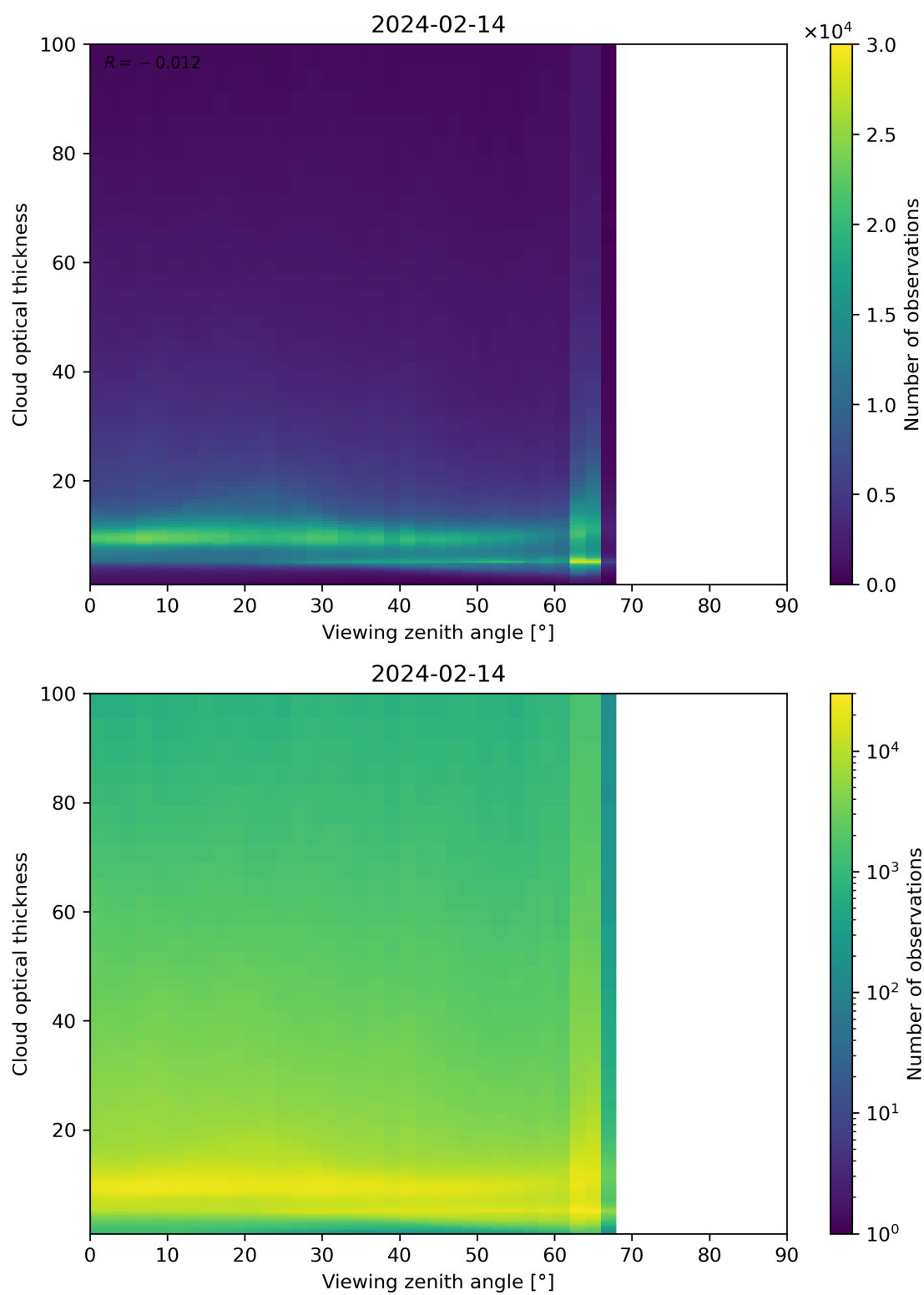
Figure 111: Scatter density plot of “Viewing zenith angle” against “Cloud optical thickness” for 2024-02-13 to 2024-02-15.
