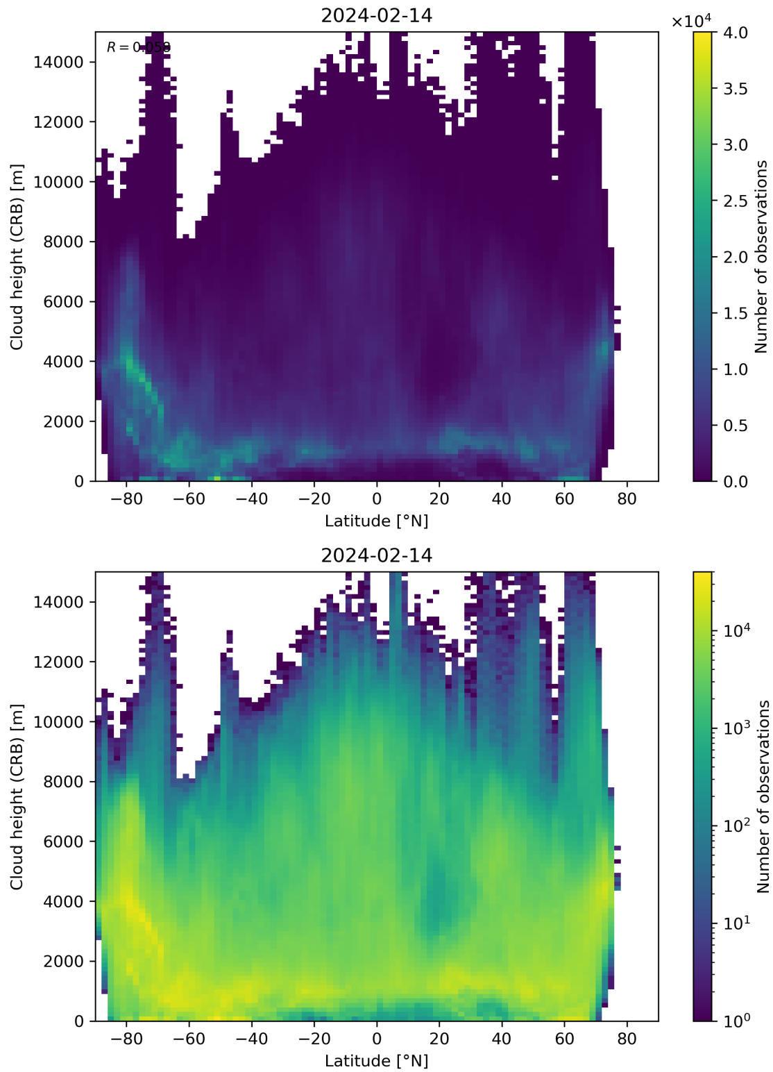
Figure 95: Scatter density plot of “Latitude” against “Cloud height (CRB)” for 2024-02-13 to 2024-02-15.
