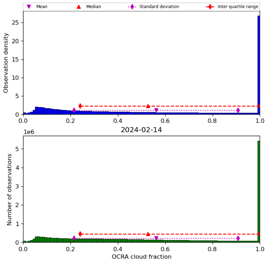
Figure 50: Histogram of “OCRA cloud fraction” for 2024-02-13 to 2024-02-15
