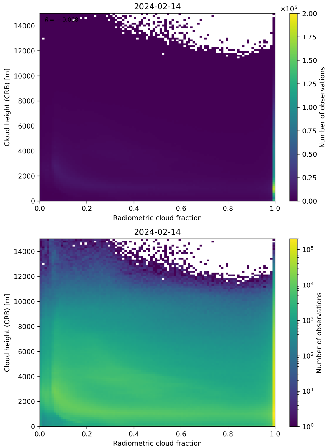
Figure 74: Scatter density plot of “Radiometric cloud fraction” against “Cloud height (CRB)” for 2024-02-13 to 2024-02-15.
