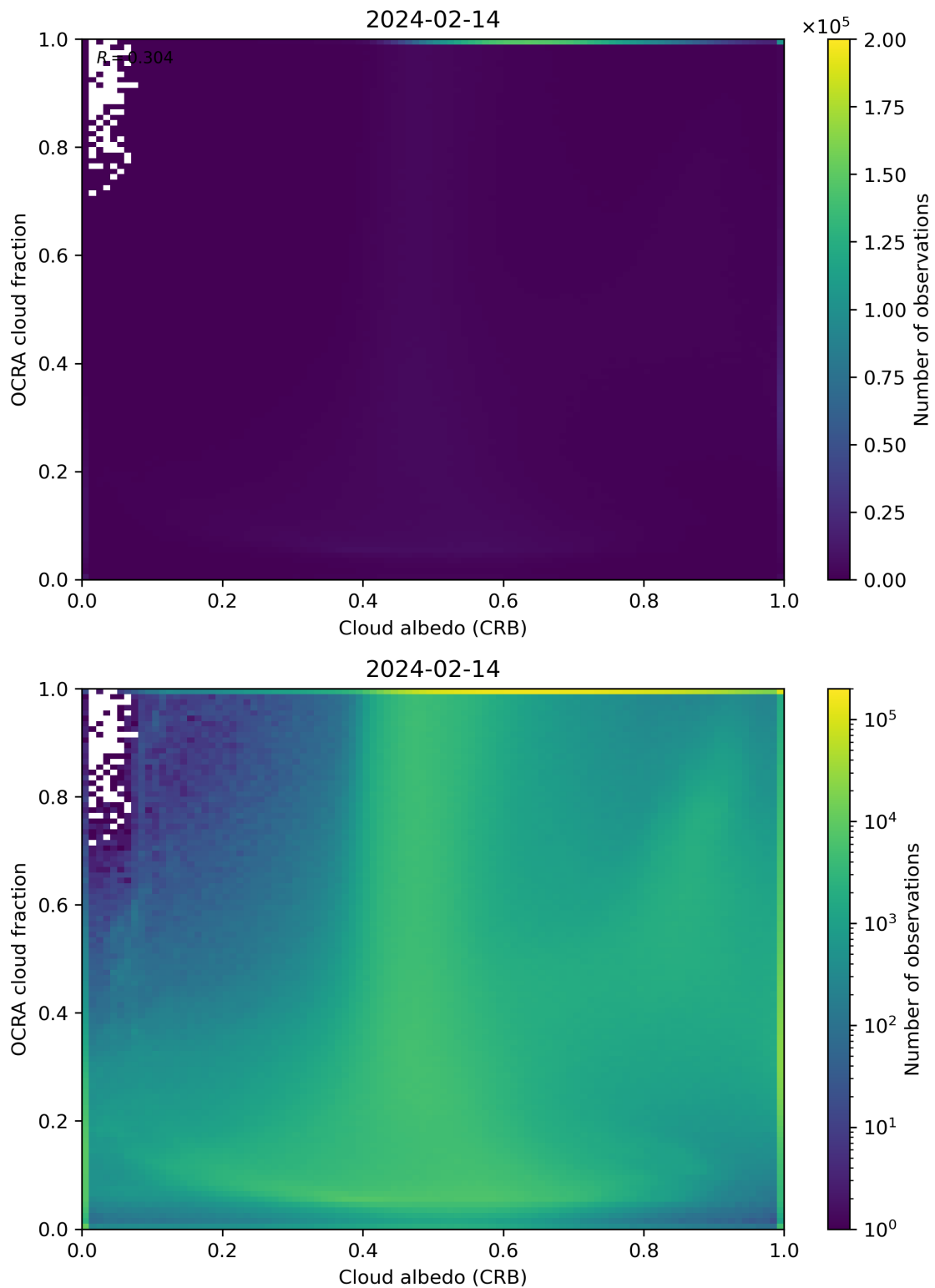
Figure 70: Scatter density plot of “Cloud albedo (CRB)” against “OCRA cloud fraction” for 2024-02-13 to 2024-02-15.
