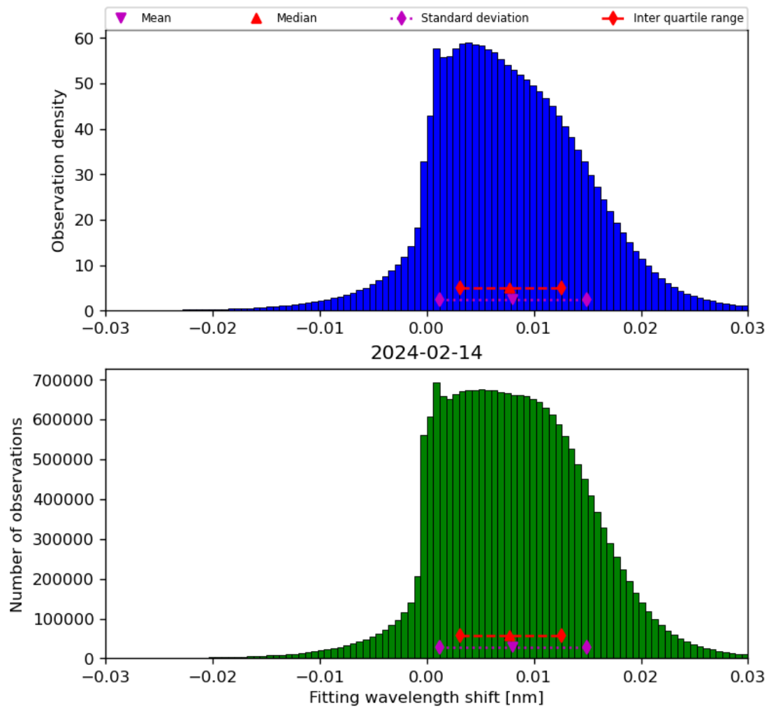
Figure 49: Histogram of “Fitting wavelength shift” for 2024-02-13 to 2024-02-15
