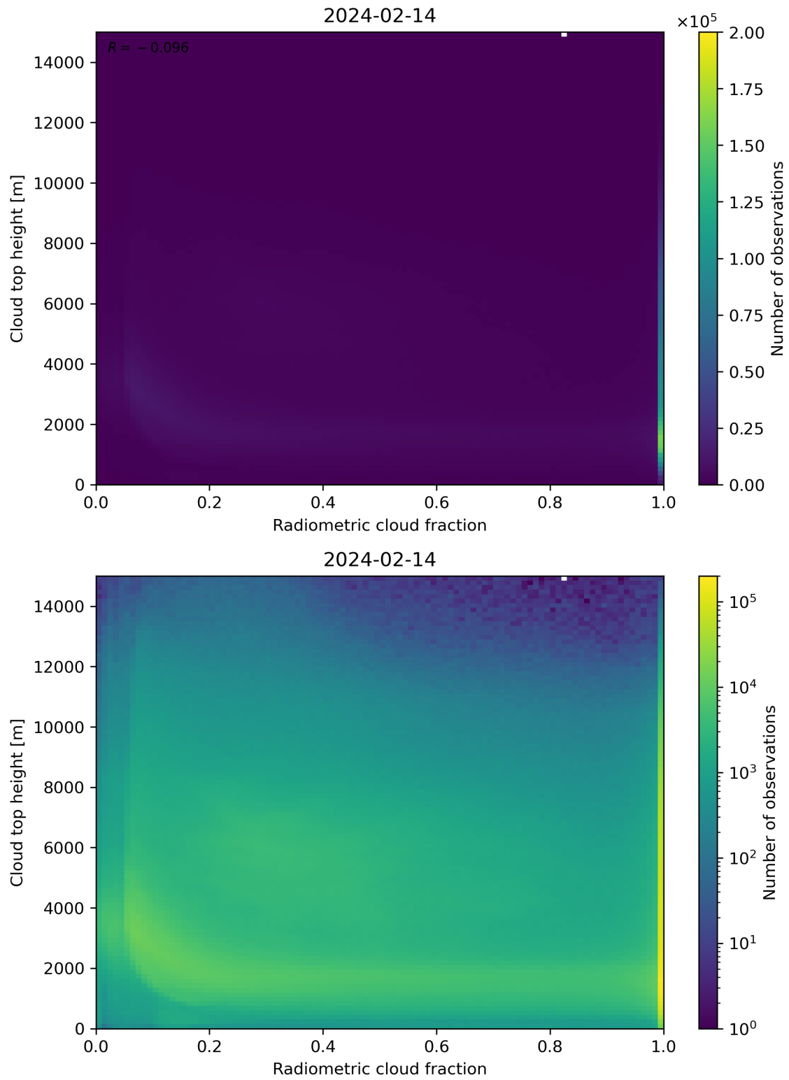
Figure 76: Scatter density plot of “Radiometric cloud fraction” against “Cloud top height” for 2024-02-13 to 2024-02-15.
