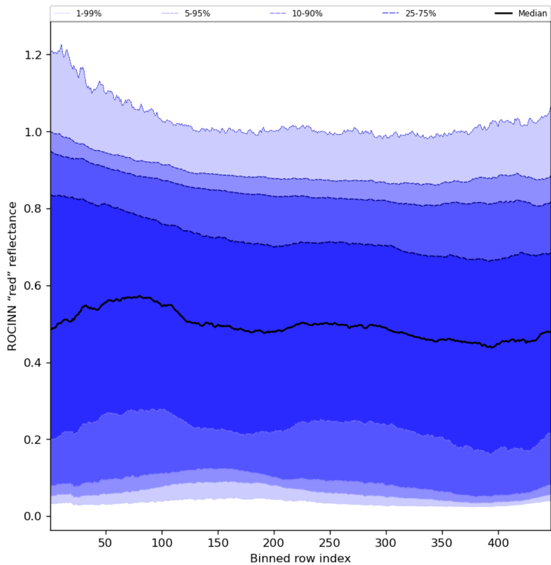
Figure 69: Along track statistics of "ROCINN "red" reflectance" for 2024-02-13 to 2024-02-15
