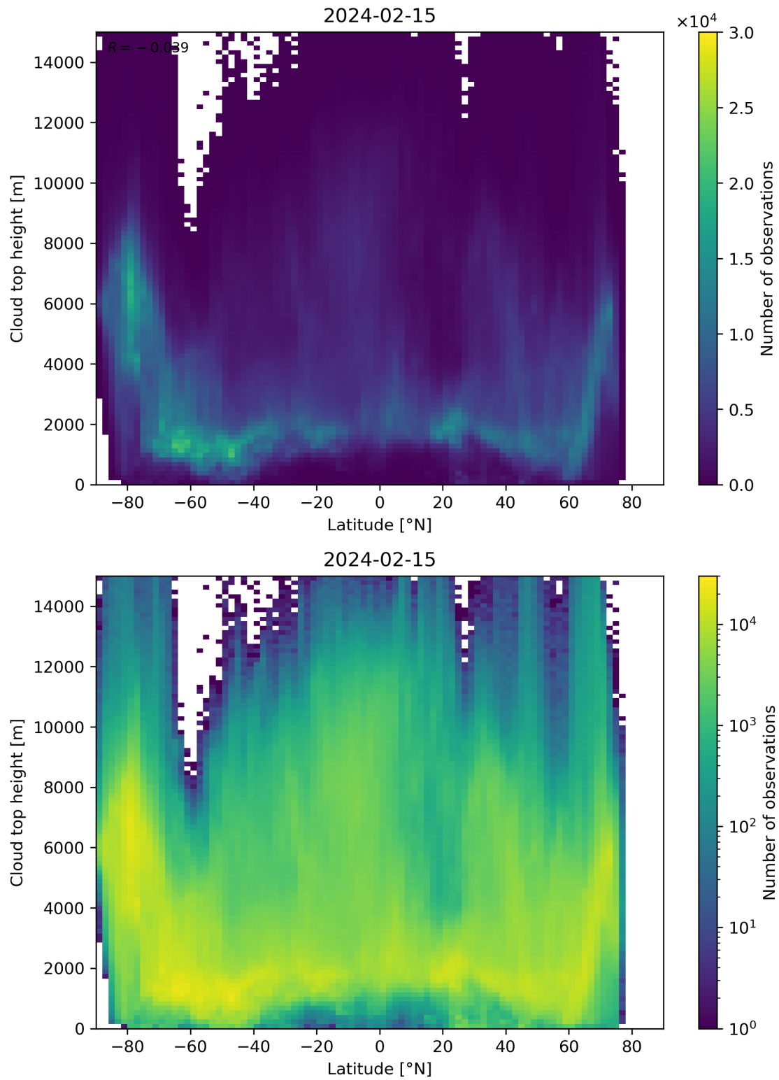
Figure 97: Scatter density plot of “Latitude” against “Cloud top height” for 2024-02-14 to 2024-02-16.
