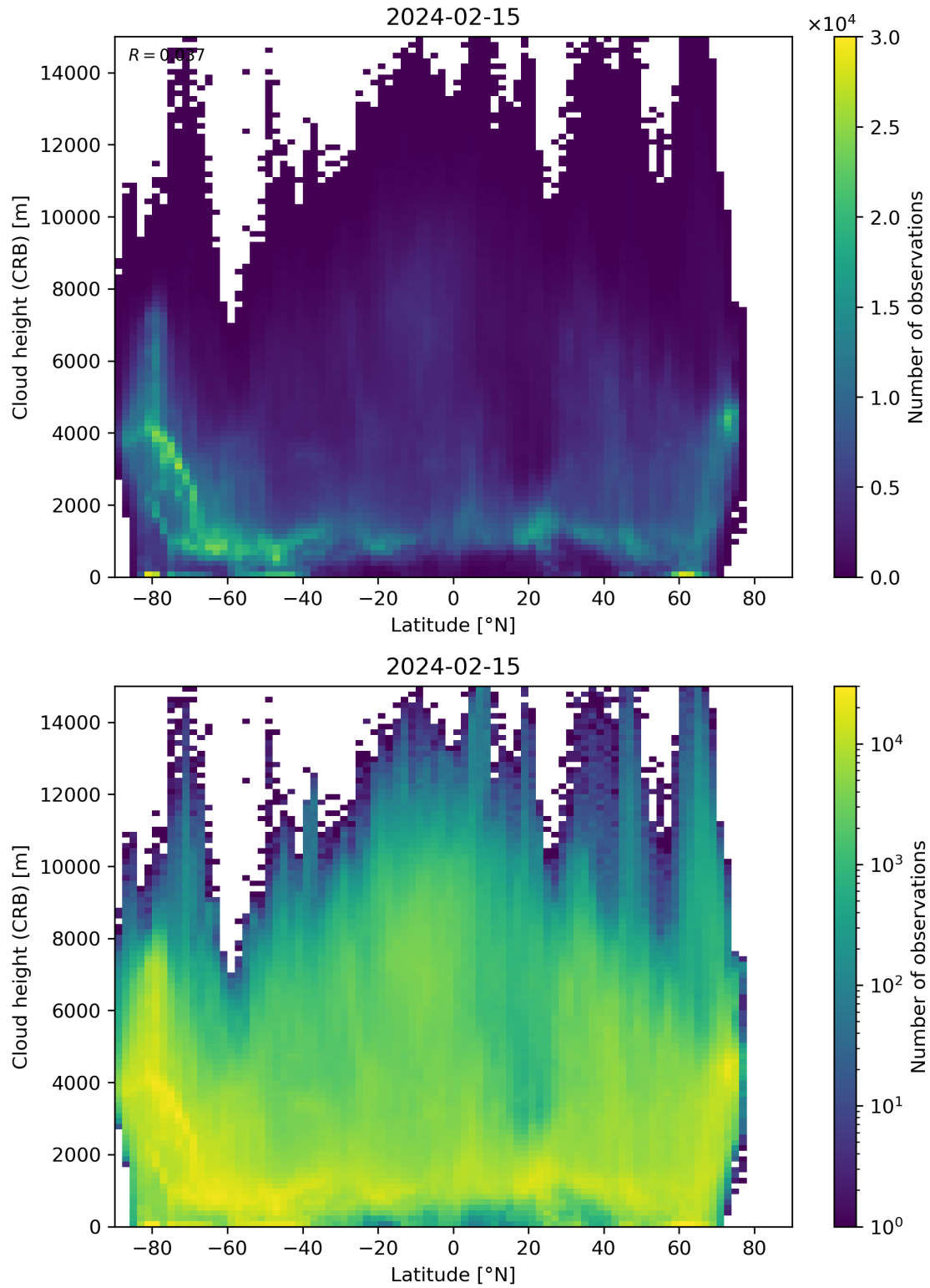
Figure 95: Scatter density plot of “Latitude” against “Cloud height (CRB)” for 2024-02-14 to 2024-02-16.
