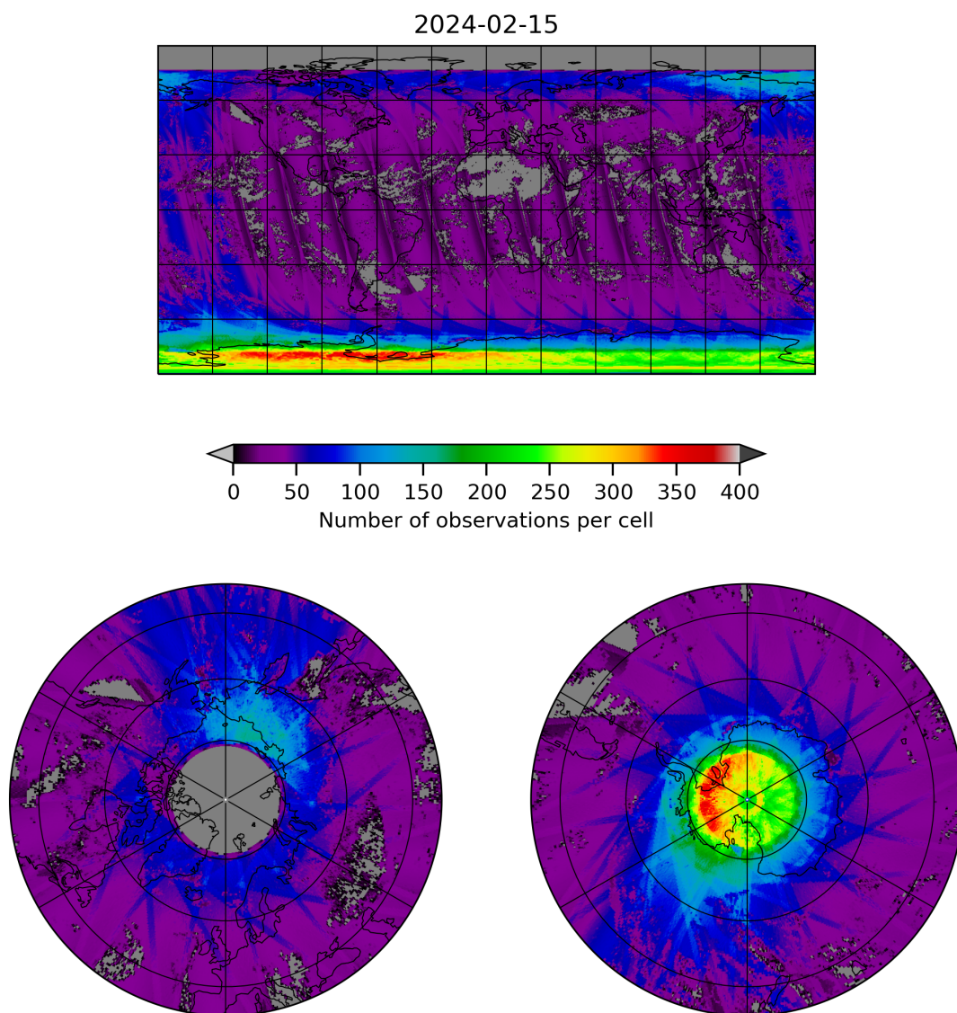
Figure 21: Map of the number of observations for 2024-02-14 to 2024-02-16
