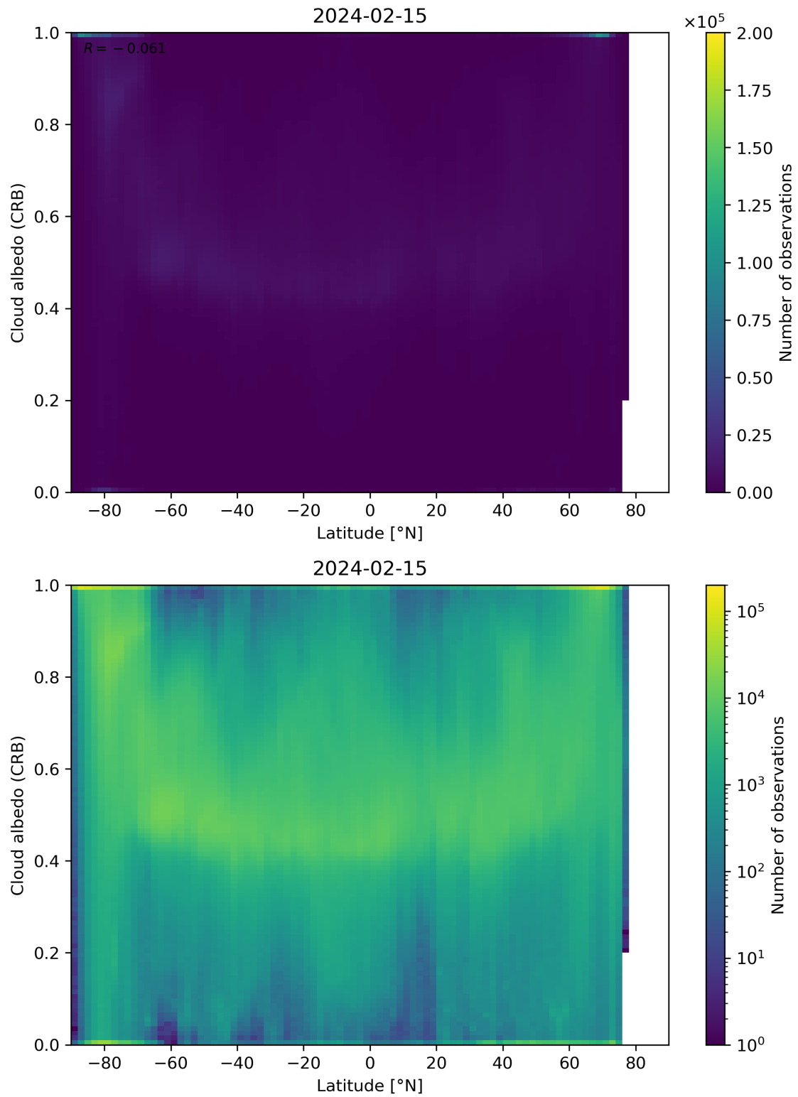
Figure 91: Scatter density plot of “Latitude” against “Cloud albedo (CRB)” for 2024-02-14 to 2024-02-16.
