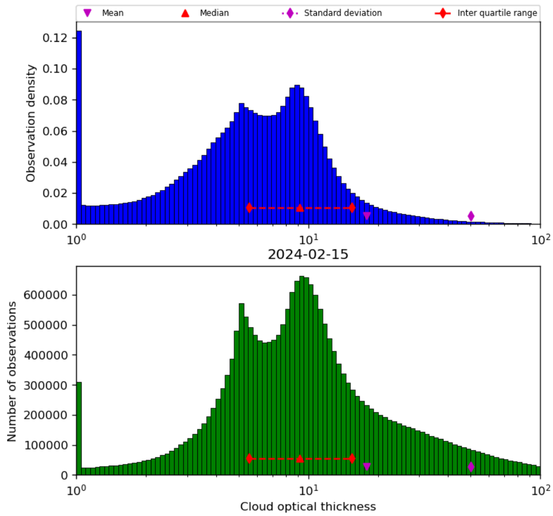
Figure 41: Histogram of “Cloud optical thickness” for 2024-02-14 to 2024-02-16
