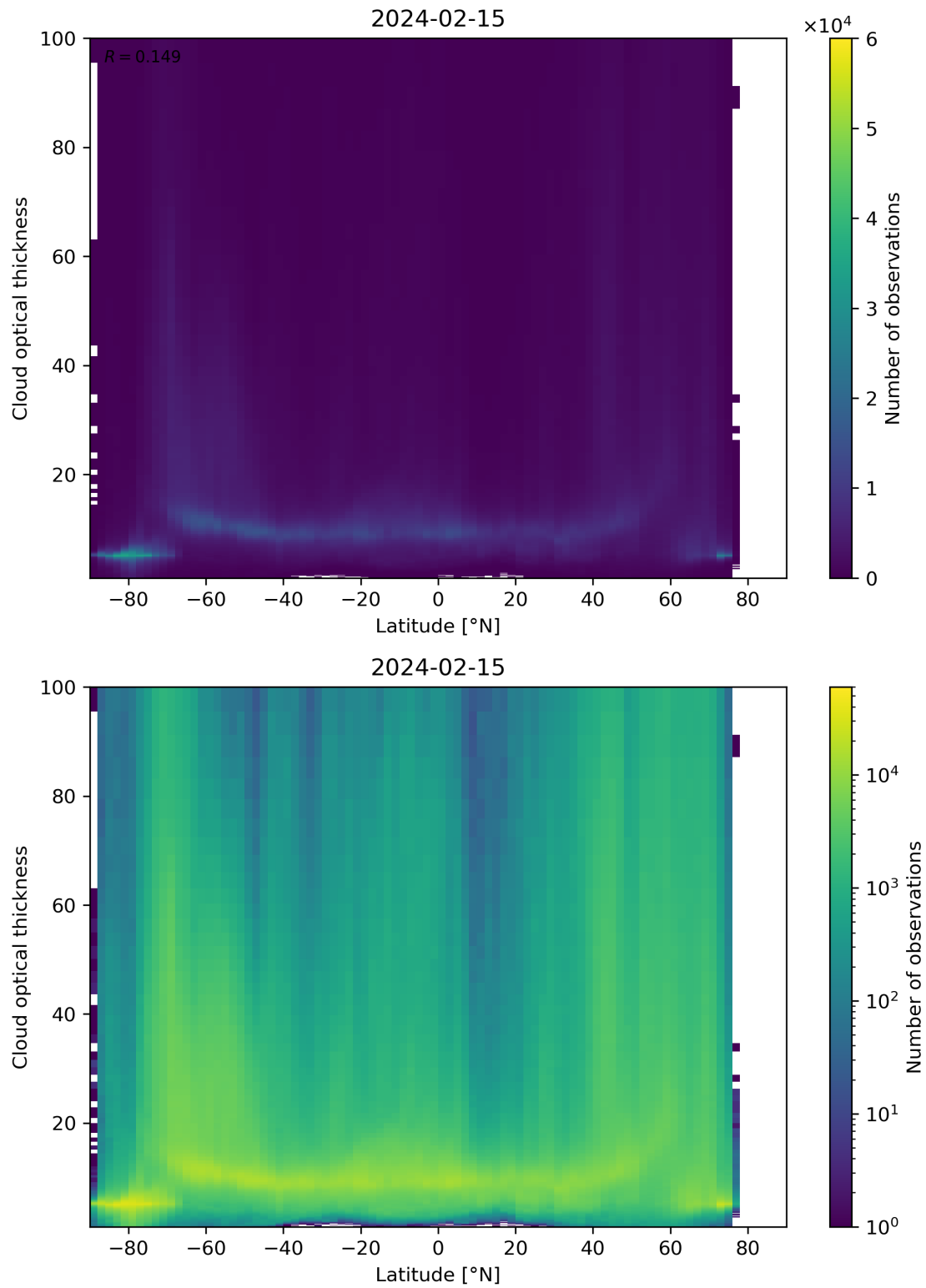
Figure 96: Scatter density plot of “Latitude” against “Cloud optical thickness” for 2024-02-14 to 2024-02-16.
