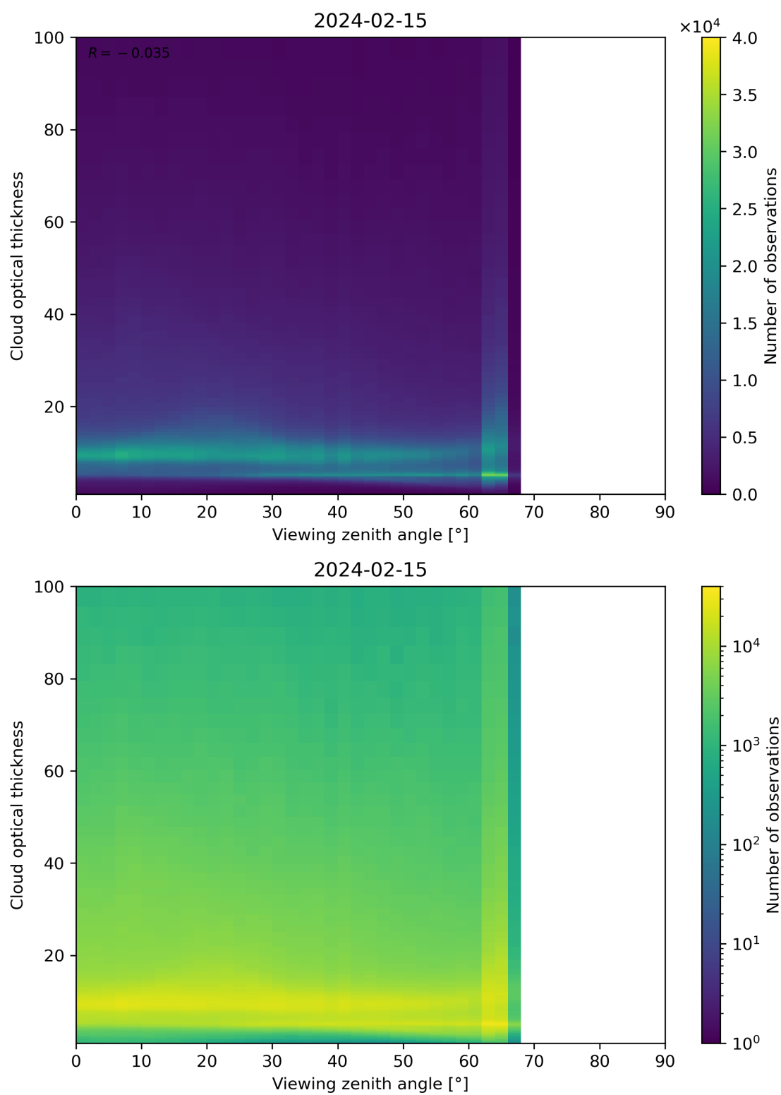
Figure 111: Scatter density plot of “Viewing zenith angle” against “Cloud optical thickness” for 2024-02-14 to 2024-02-16.
