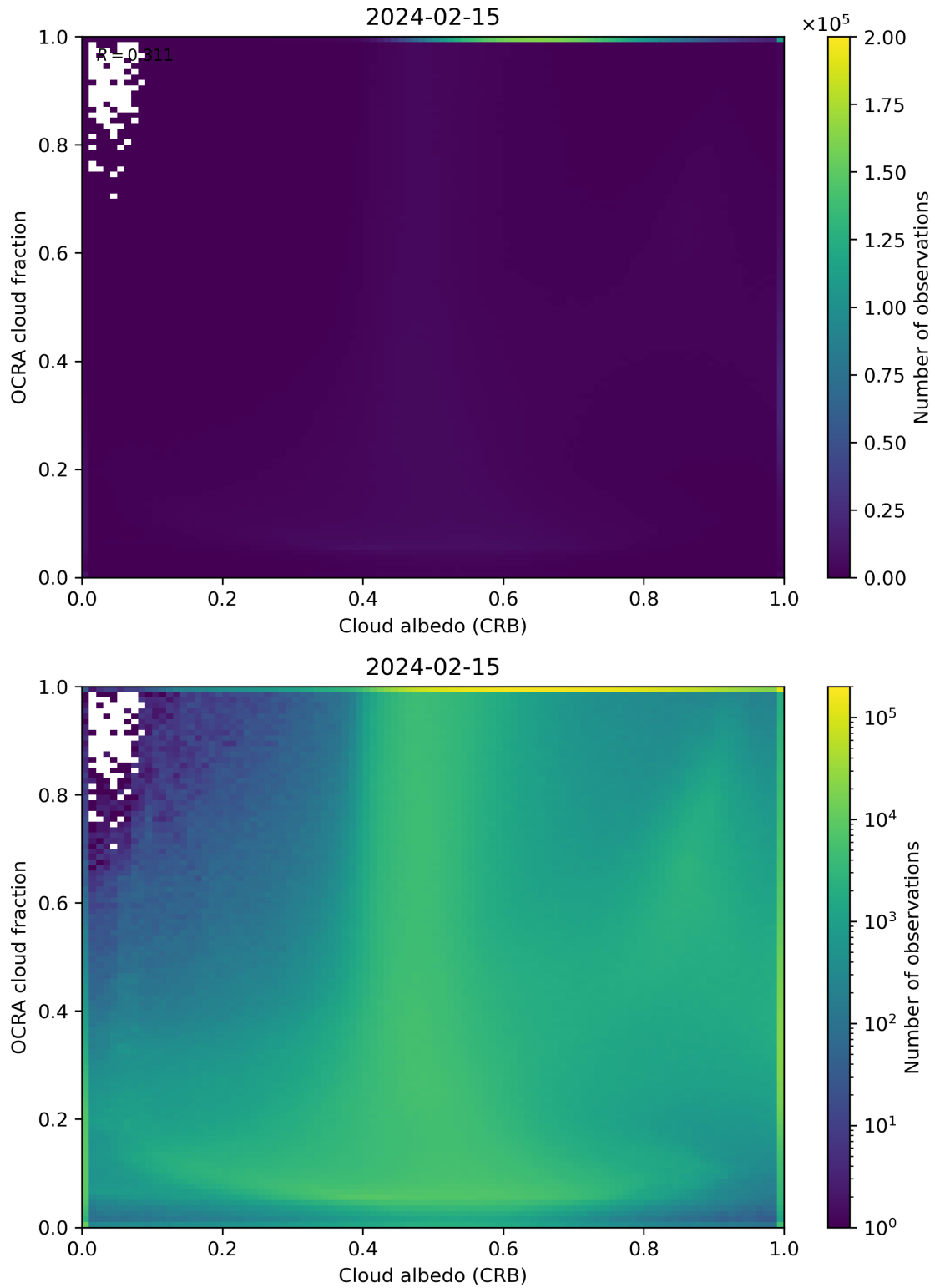
Figure 70: Scatter density plot of “Cloud albedo (CRB)” against “OCRA cloud fraction” for 2024-02-14 to 2024-02-16.
