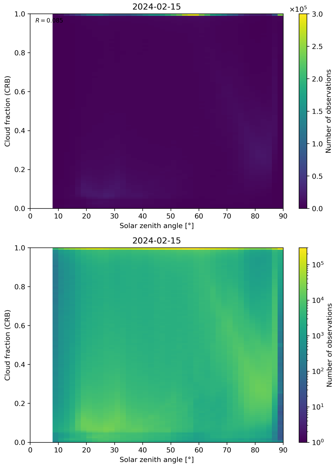
Figure 101: Scatter density plot of “Solar zenith angle” against “Cloud fraction (CRB)” for 2024-02-14 to 2024-02-16.
