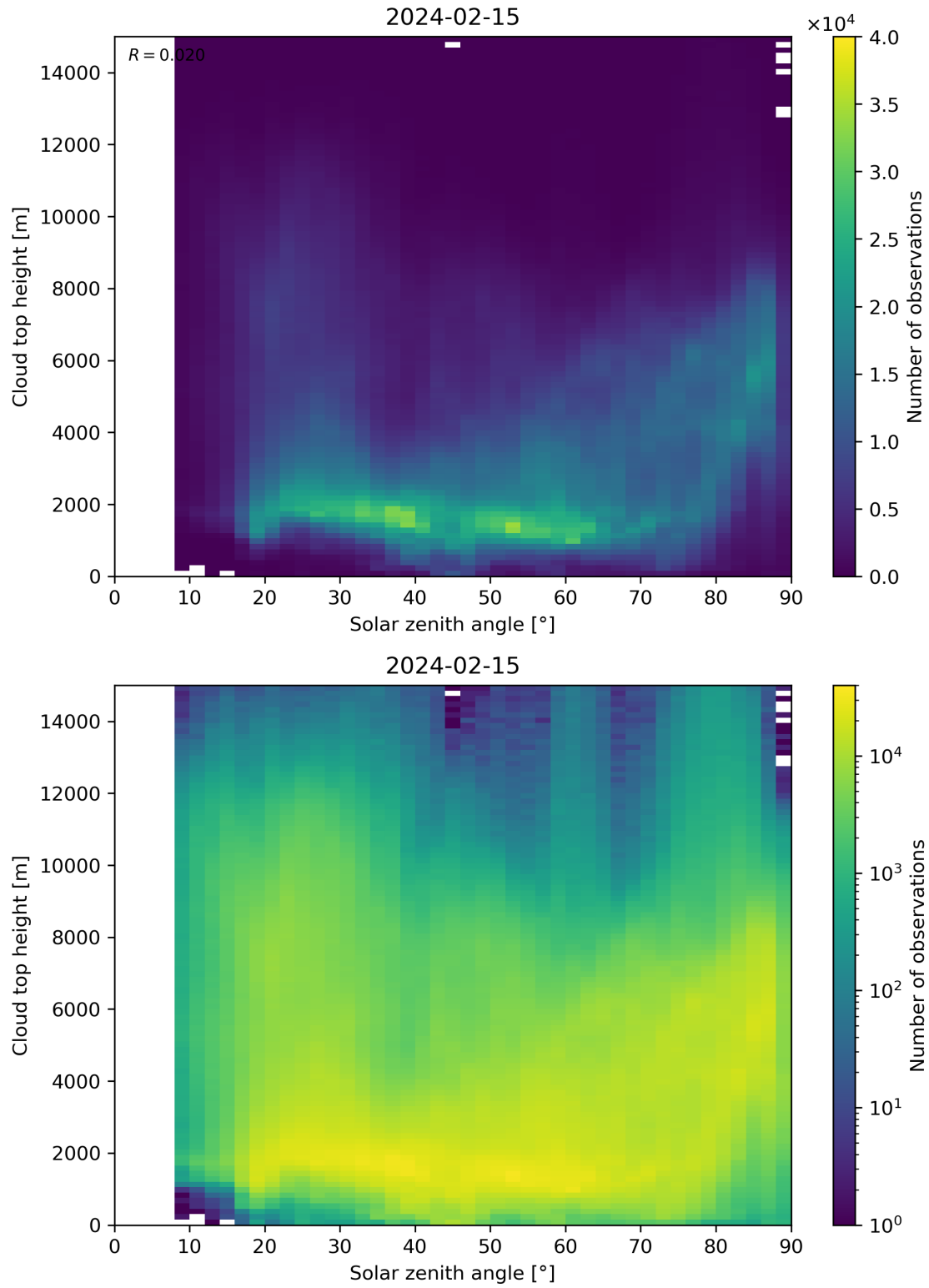
Figure 104: Scatter density plot of “Solar zenith angle” against “Cloud top height” for 2024-02-14 to 2024-02-16.
