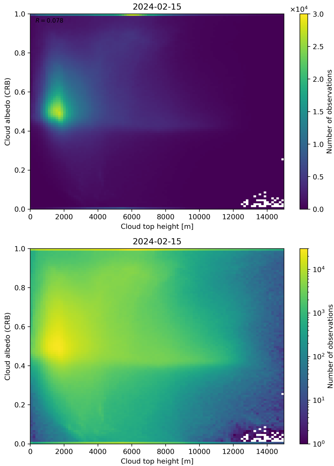
Figure 86: Scatter density plot of “Cloud top height” against “Cloud albedo (CRB)” for 2024-02-14 to 2024-02-16.
