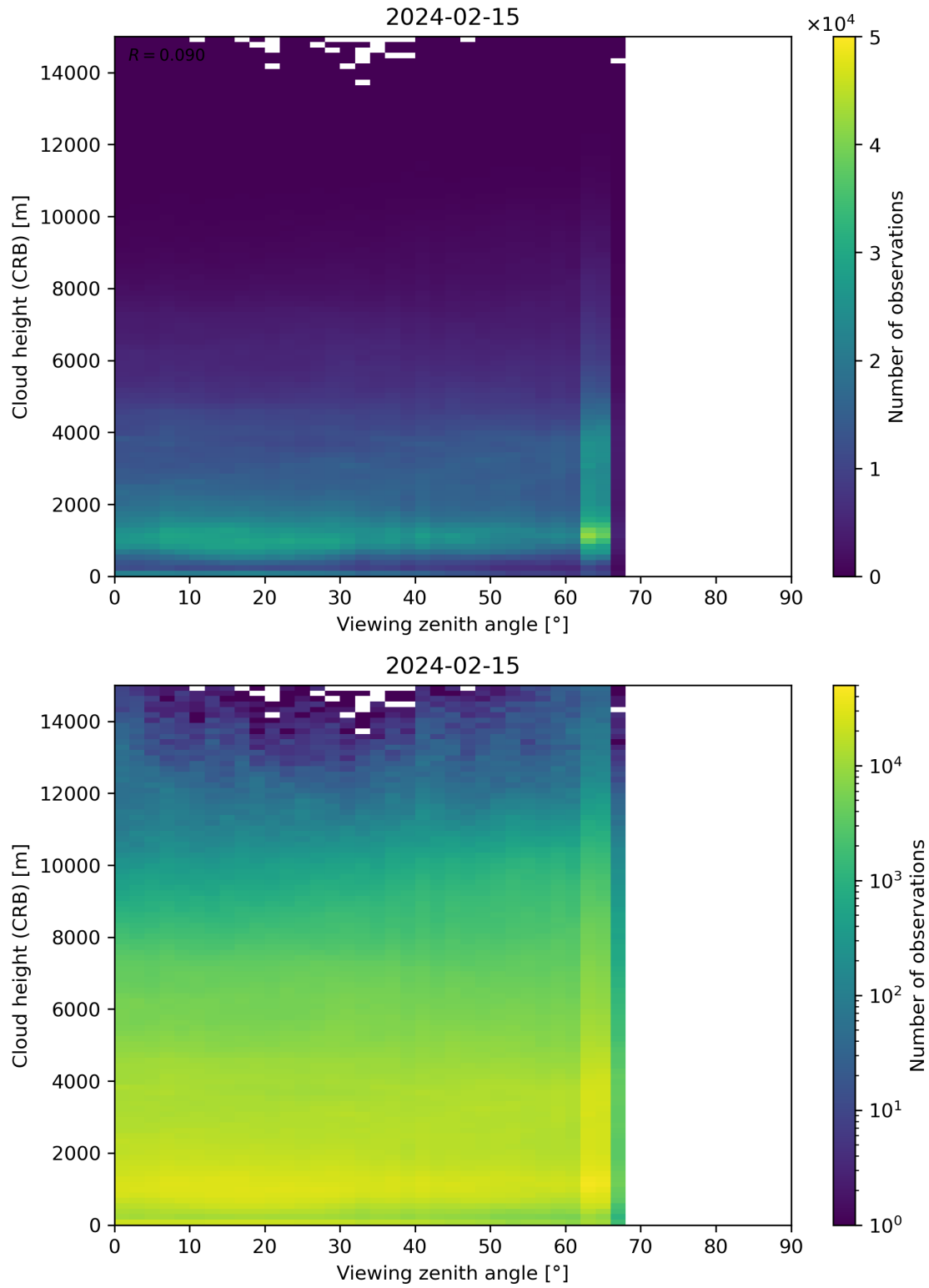
Figure 110: Scatter density plot of “Viewing zenith angle” against “Cloud height (CRB)” for 2024-02-14 to 2024-02-16.
