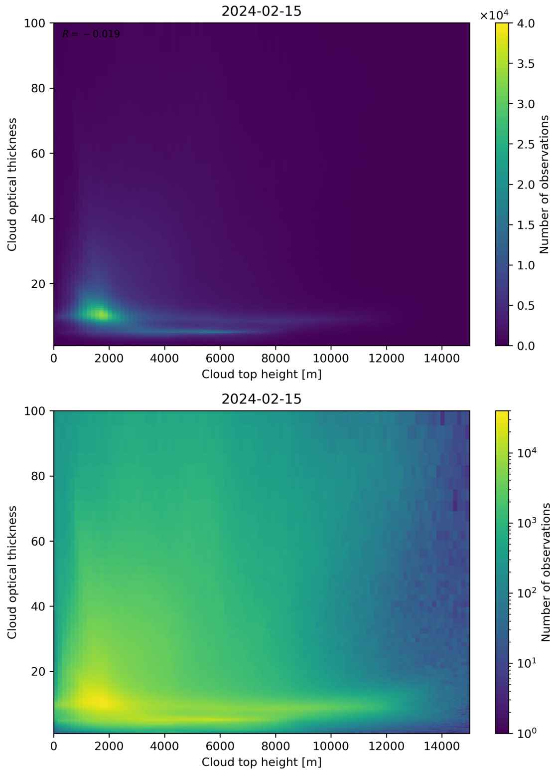
Figure 90: Scatter density plot of “Cloud top height” against “Cloud optical thickness” for 2024-02-14 to 2024-02-16.
