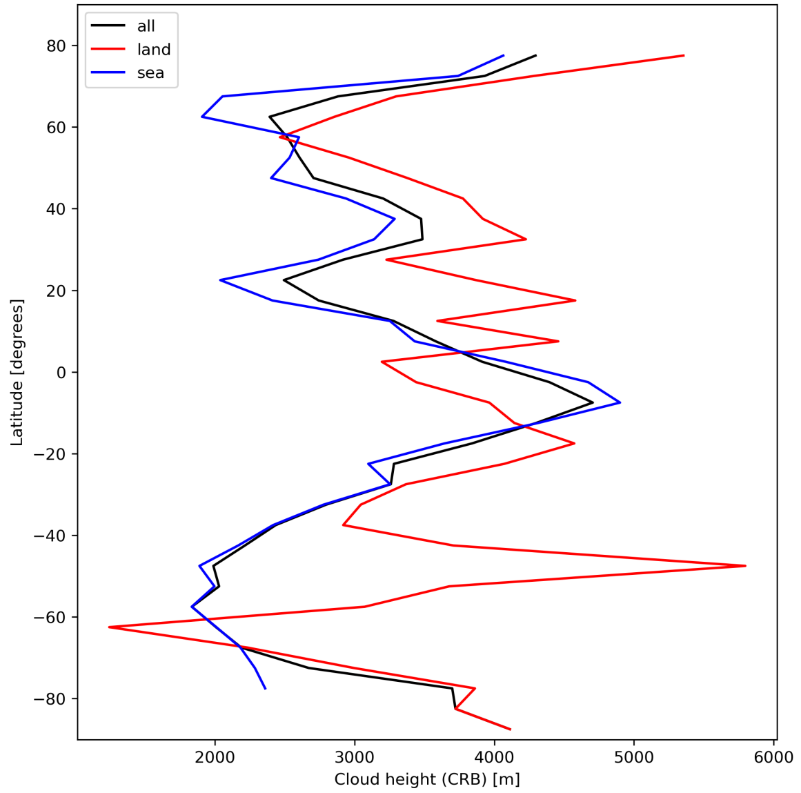
Figure 27: Zonal average of “Cloud height (CRB)” for 2024-02-14 to 2024-02-16.
