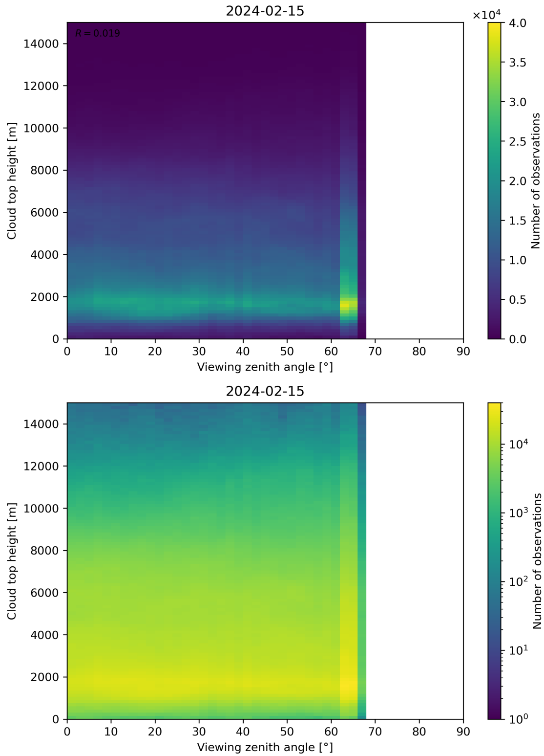
Figure 112: Scatter density plot of “Viewing zenith angle” against “Cloud top height” for 2024-02-14 to 2024-02-16.
