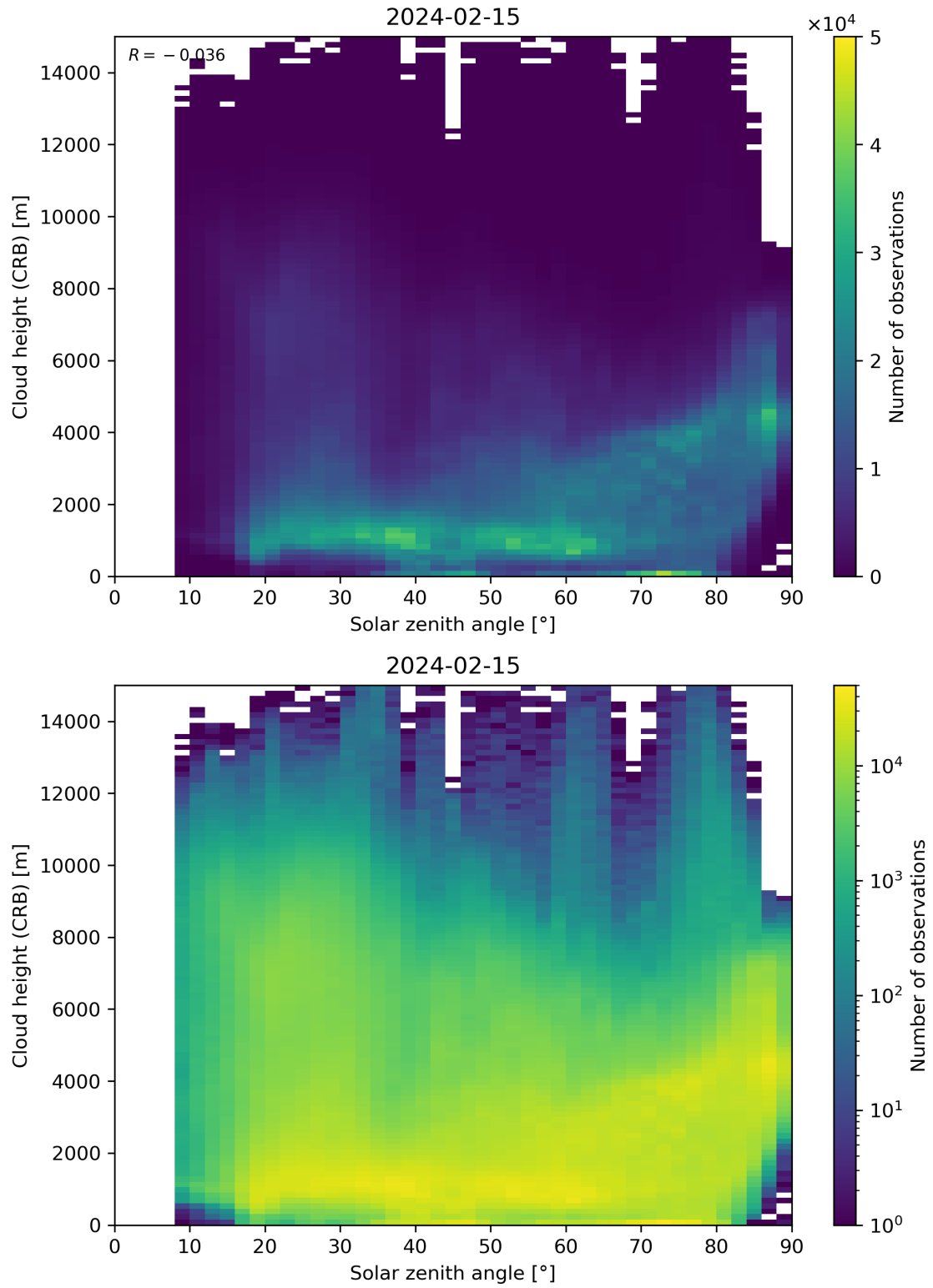
Figure 102: Scatter density plot of “Solar zenith angle” against “Cloud height (CRB)” for 2024-02-14 to 2024-02-16.
