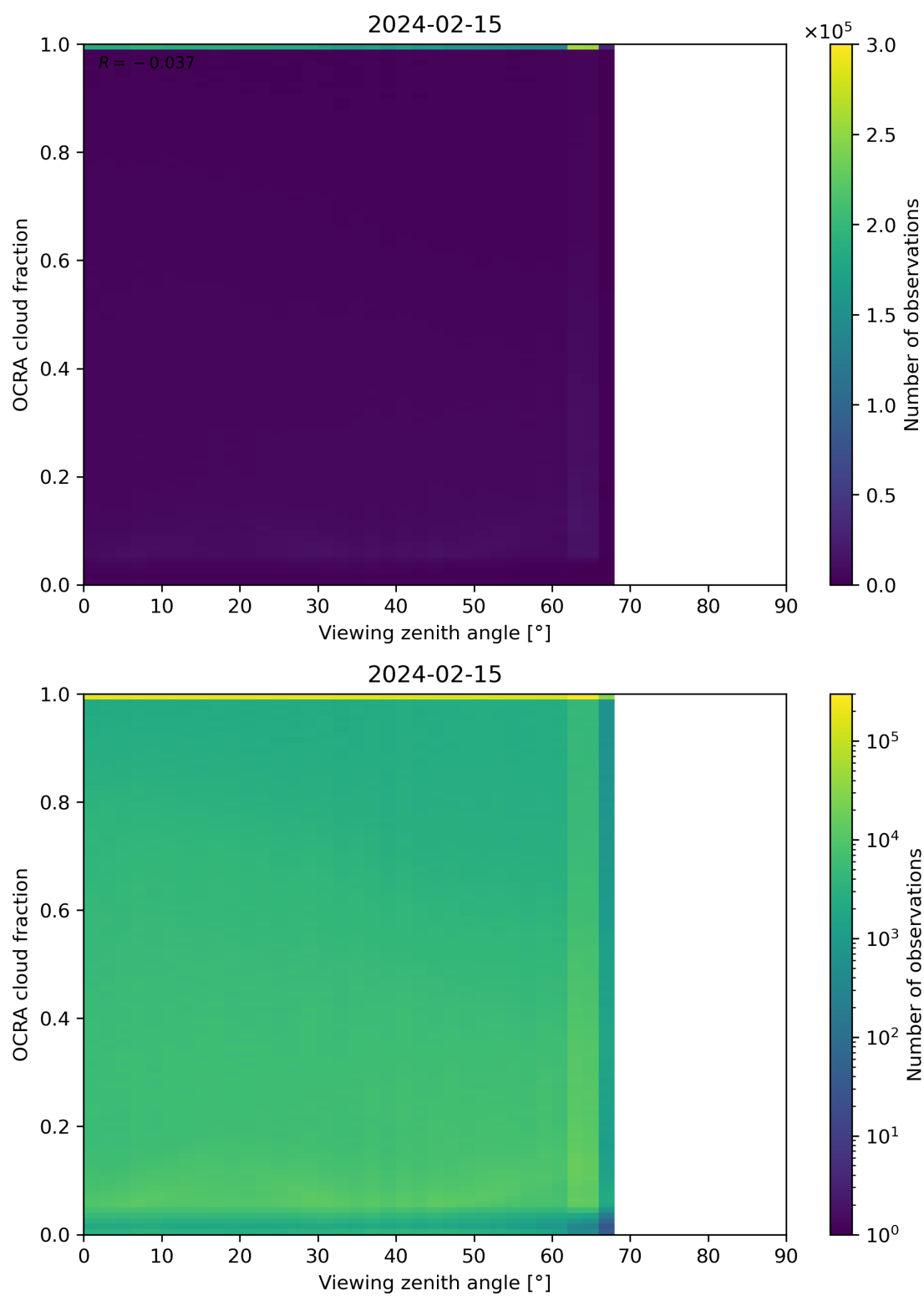
Figure 108: Scatter density plot of “Viewing zenith angle” against “OCRA cloud fraction” for 2024-02-14 to 2024-02-16.
