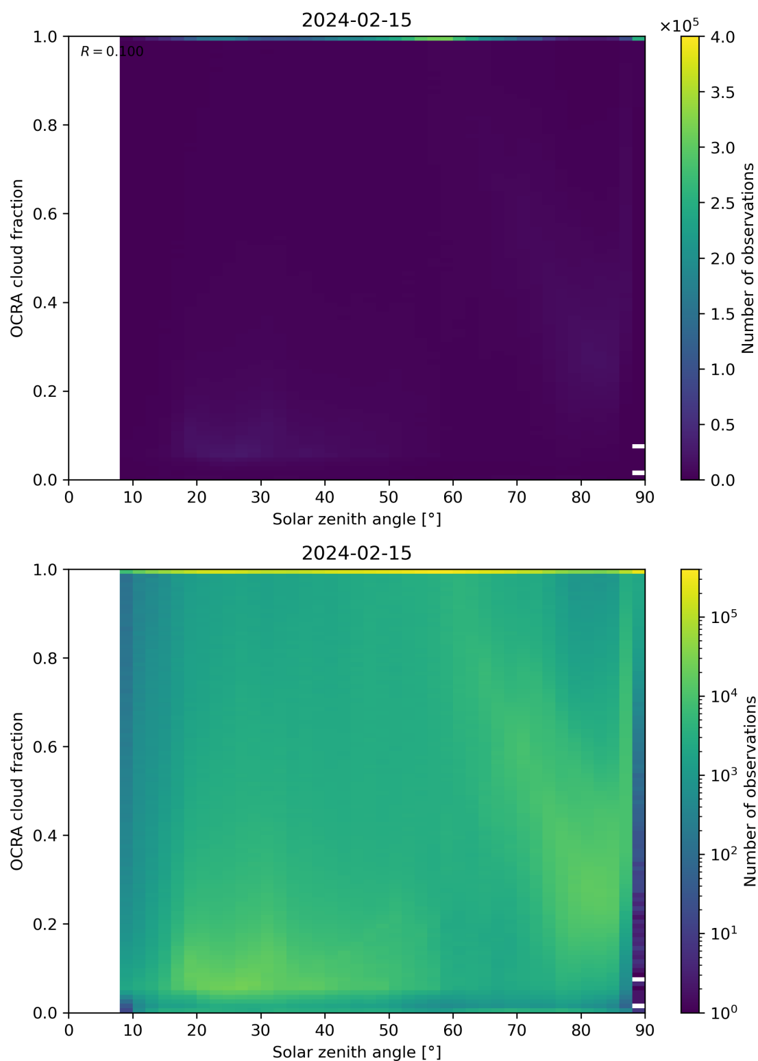
Figure 100: Scatter density plot of “Solar zenith angle” against “OCRA cloud fraction” for 2024-02-14 to 2024-02-16.
