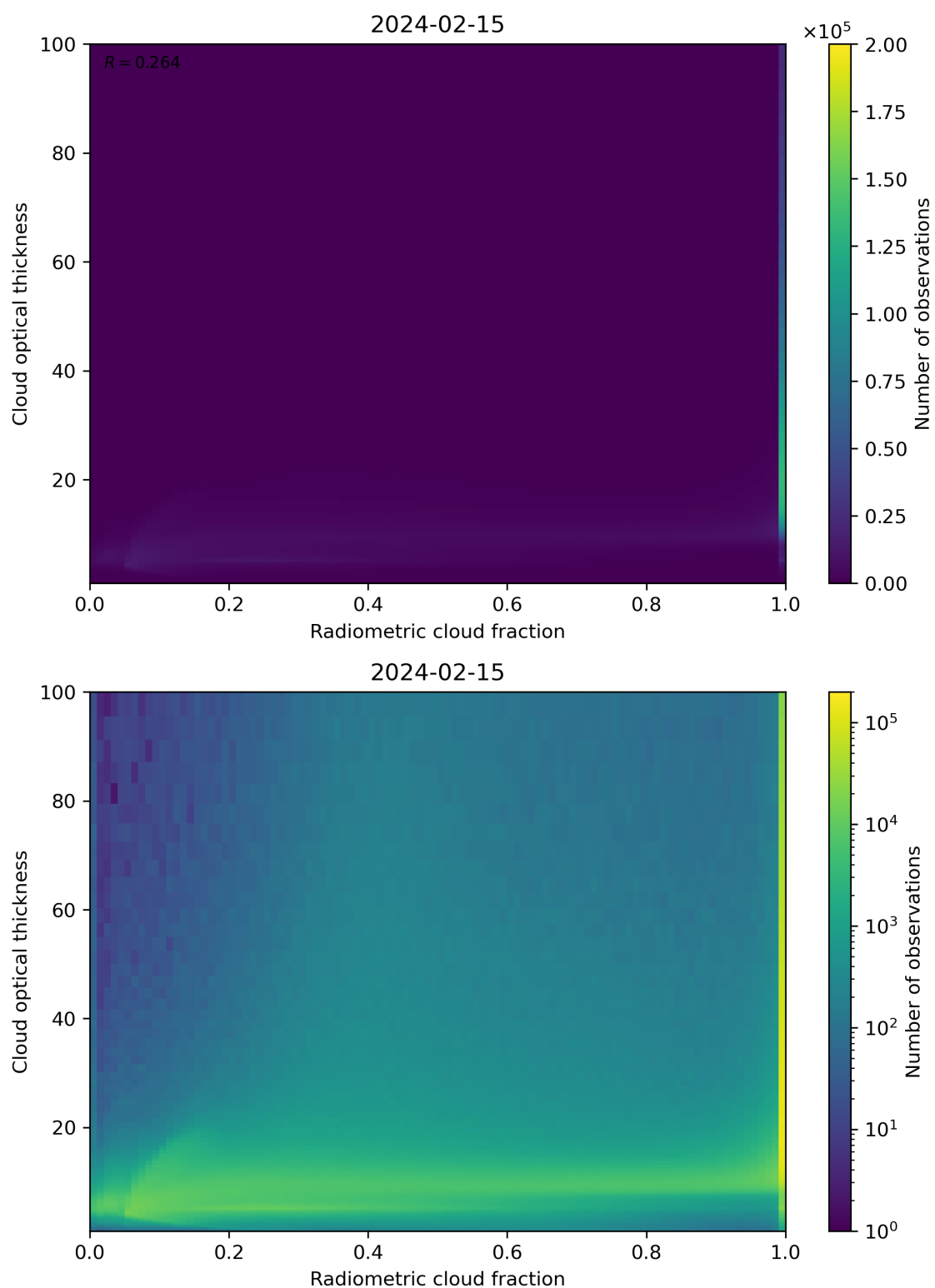
Figure 75: Scatter density plot of “Radiometric cloud fraction” against “Cloud optical thickness” for 2024-02-14 to 2024-02-16.
