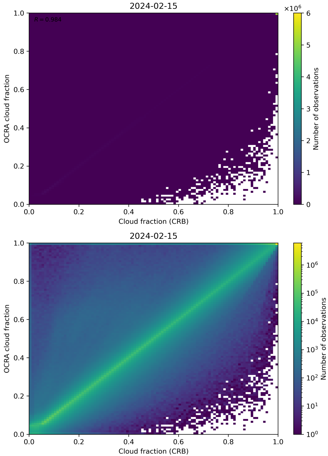
Figure 78: Scatter density plot of “Cloud fraction (CRB)” against “OCRA cloud fraction” for 2024-02-14 to 2024-02-16.
