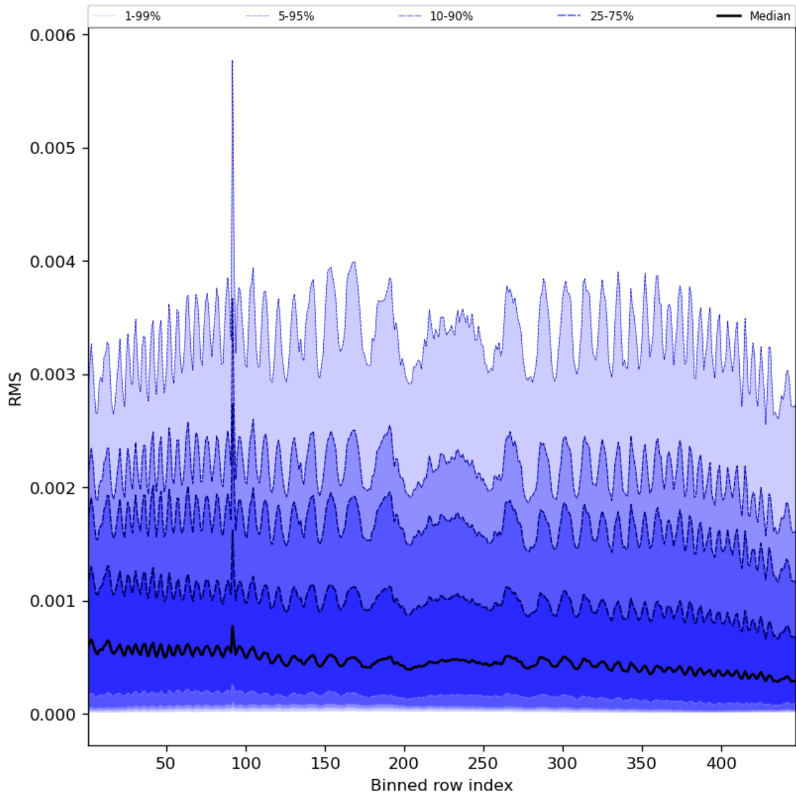
Figure 63: Along track statistics of “RMS” for 2024-02-14 to 2024-02-16
