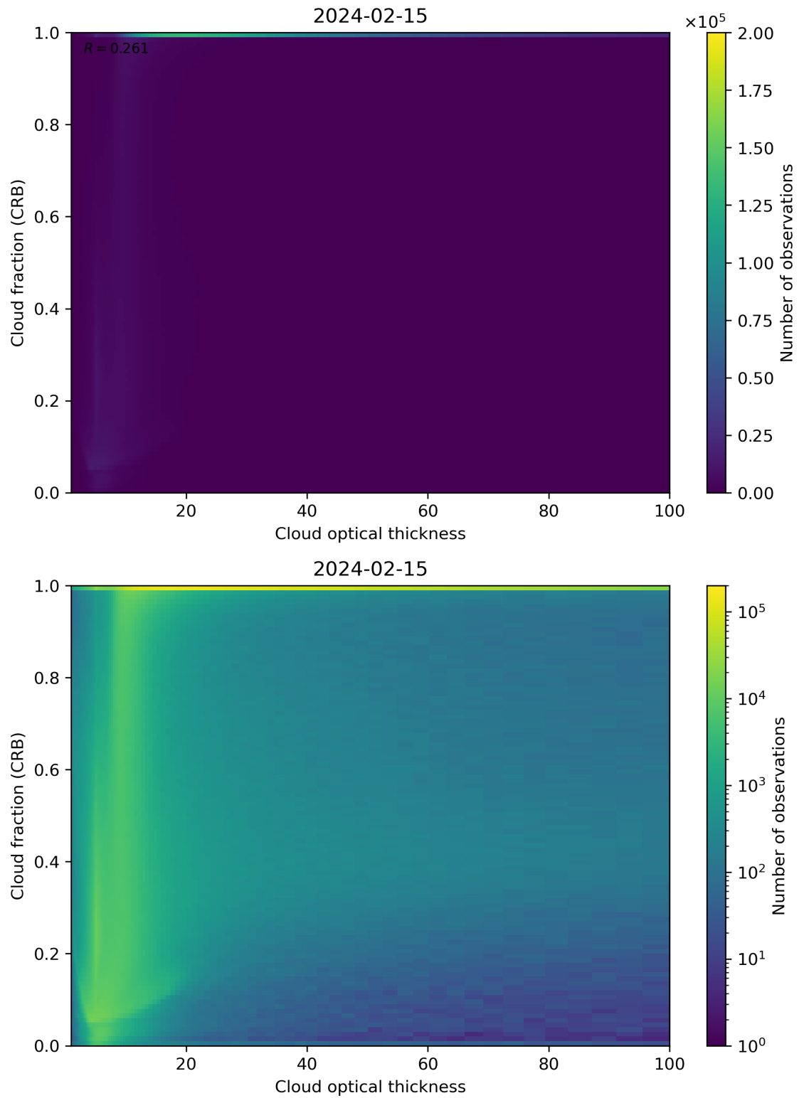
Figure 84: Scatter density plot of “Cloud optical thickness” against “Cloud fraction (CRB)” for 2024-02-14 to 2024-02-16.
