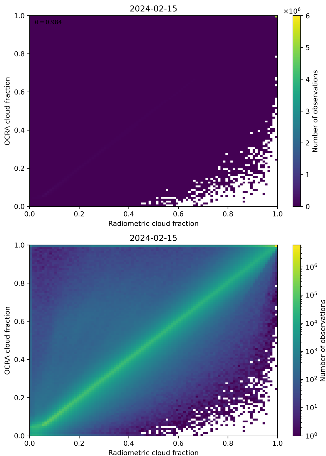
Figure 72: Scatter density plot of “Radiometric cloud fraction” against “OCRA cloud fraction” for 2024-02-14 to 2024-02-16.
