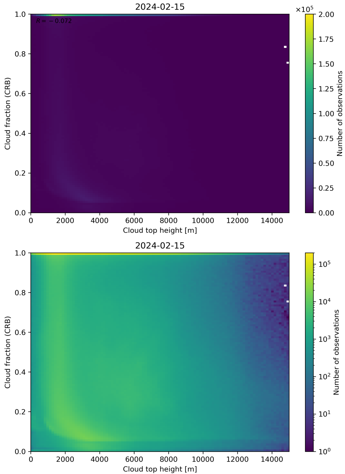
Figure 88: Scatter density plot of “Cloud top height” against “Cloud fraction (CRB)” for 2024-02-14 to 2024-02-16.
