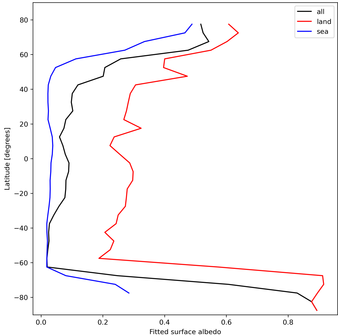
Figure 29: Zonal average of “Fitted surface albedo” for 2024-02-14 to 2024-02-16.
