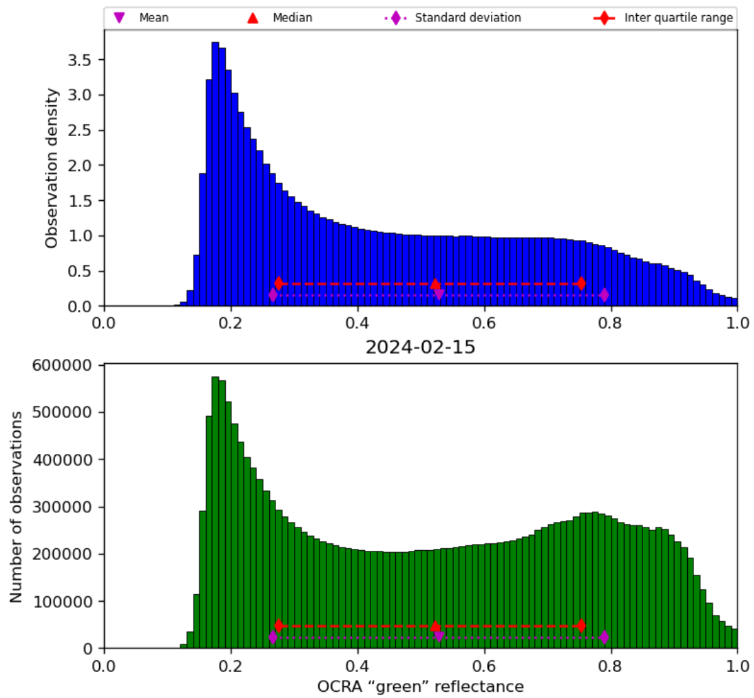
Figure 52: Histogram of “OCRA “green” reflectance” for 2024-02-14 to 2024-02-16
