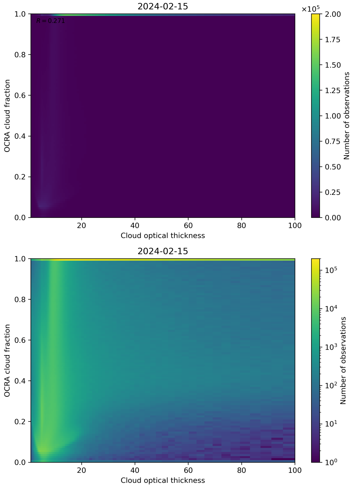
Figure 83: Scatter density plot of “Cloud optical thickness” against “OCRA cloud fraction” for 2024-02-14 to 2024-02-16.
