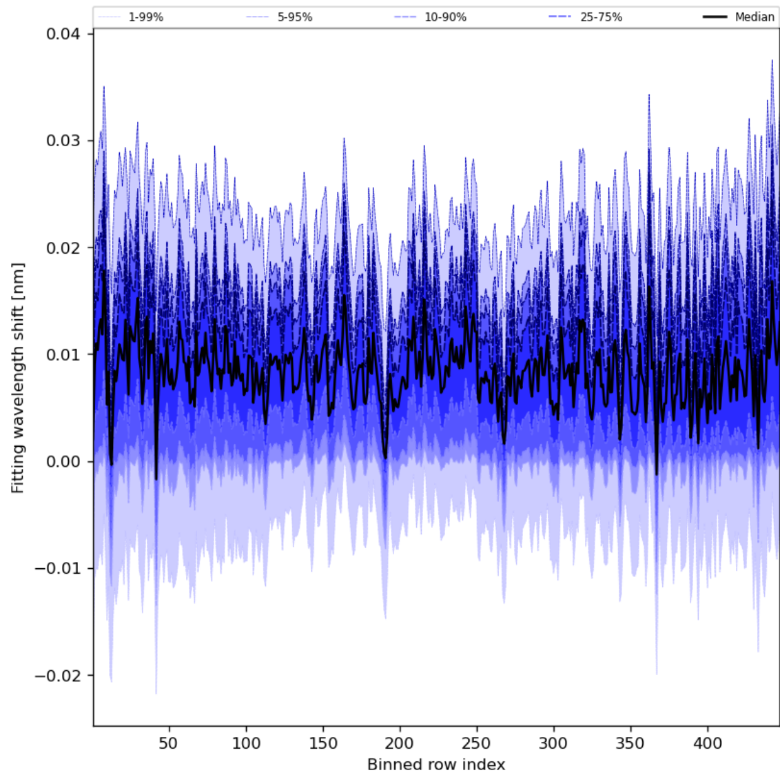
Figure 65: Along track statistics of “Fitting wavelength shift” for 2024-02-14 to 2024-02-16
