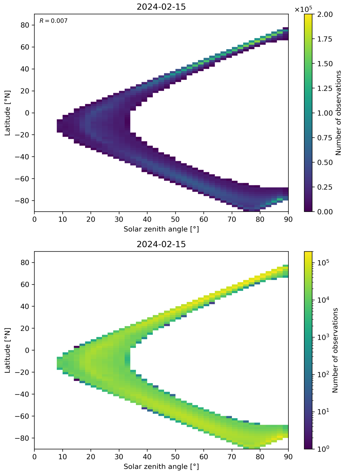
Figure 105: Scatter density plot of “Solar zenith angle” against “Latitude” for 2024-02-14 to 2024-02-16.
