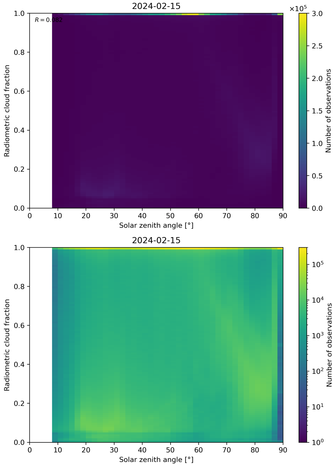
Figure 99: Scatter density plot of “Solar zenith angle” against “Radiometric cloud fraction” for 2024-02-14 to 2024-02-16.
