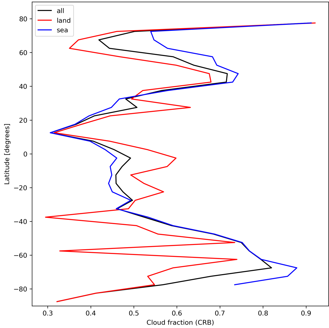
Figure 26: Zonal average of “Cloud fraction (CRB)” for 2024-02-14 to 2024-02-16.
