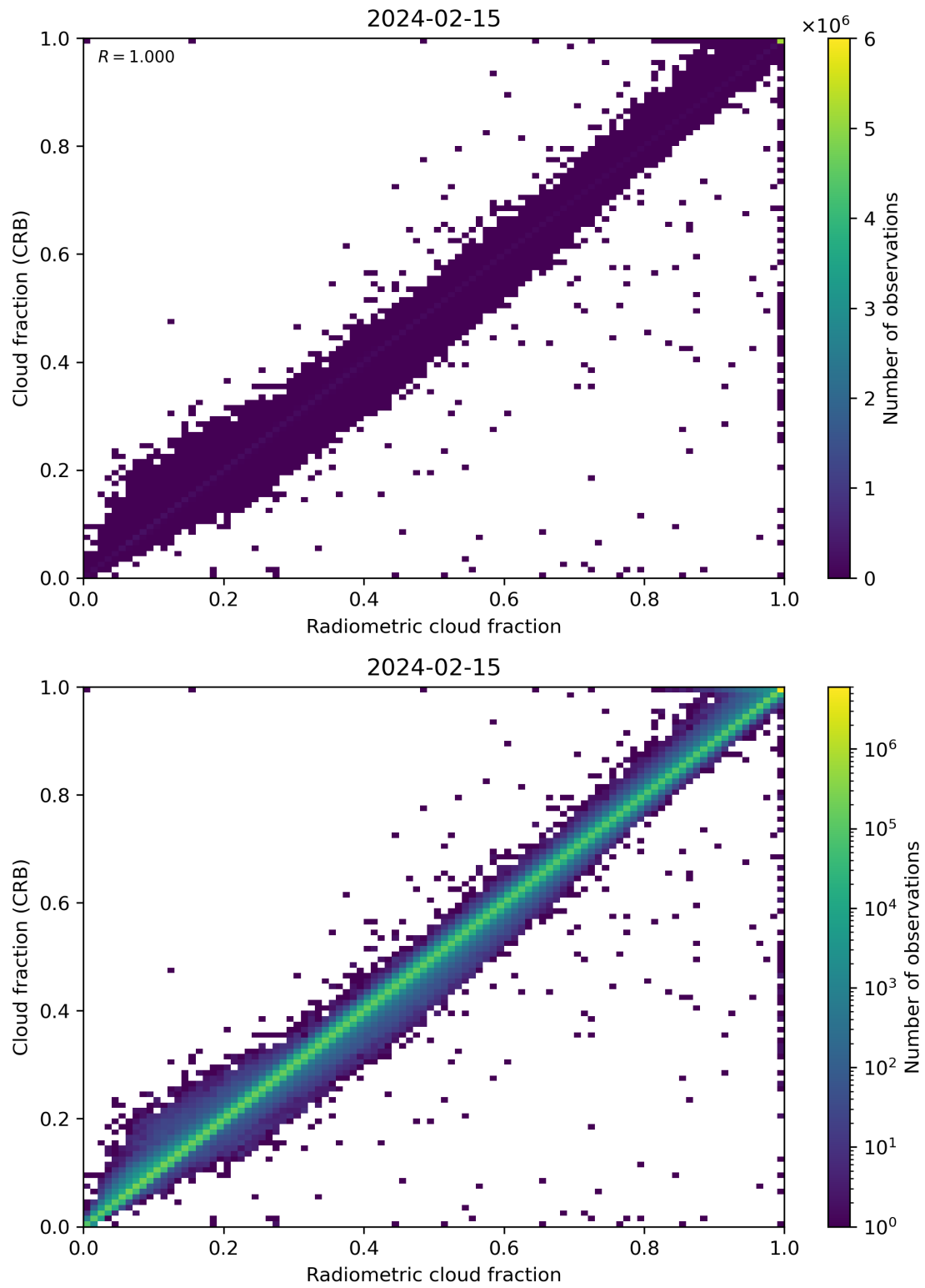
Figure 73: Scatter density plot of “Radiometric cloud fraction” against “Cloud fraction (CRB)” for 2024-02-14 to 2024-02-16.
