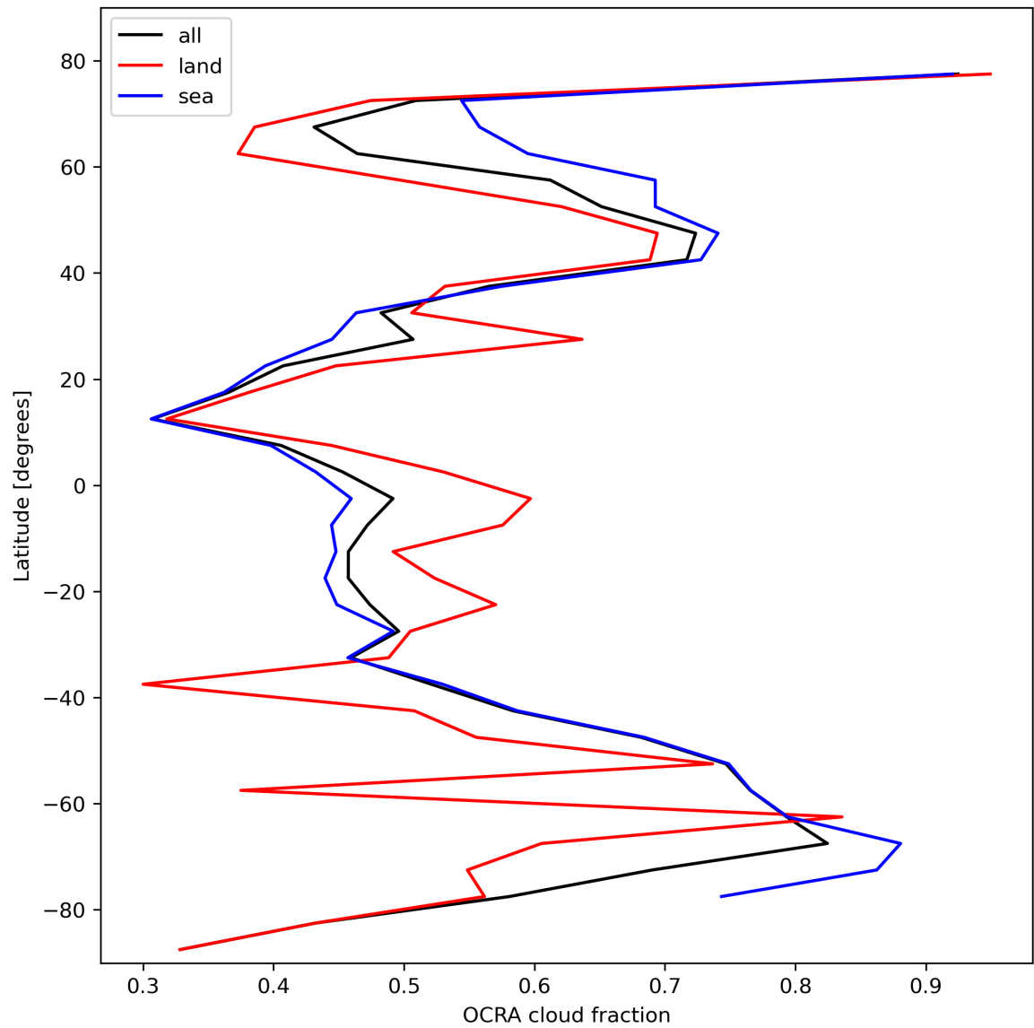
Figure 34: Zonal average of “OCRA cloud fraction” for 2024-02-14 to 2024-02-16.
