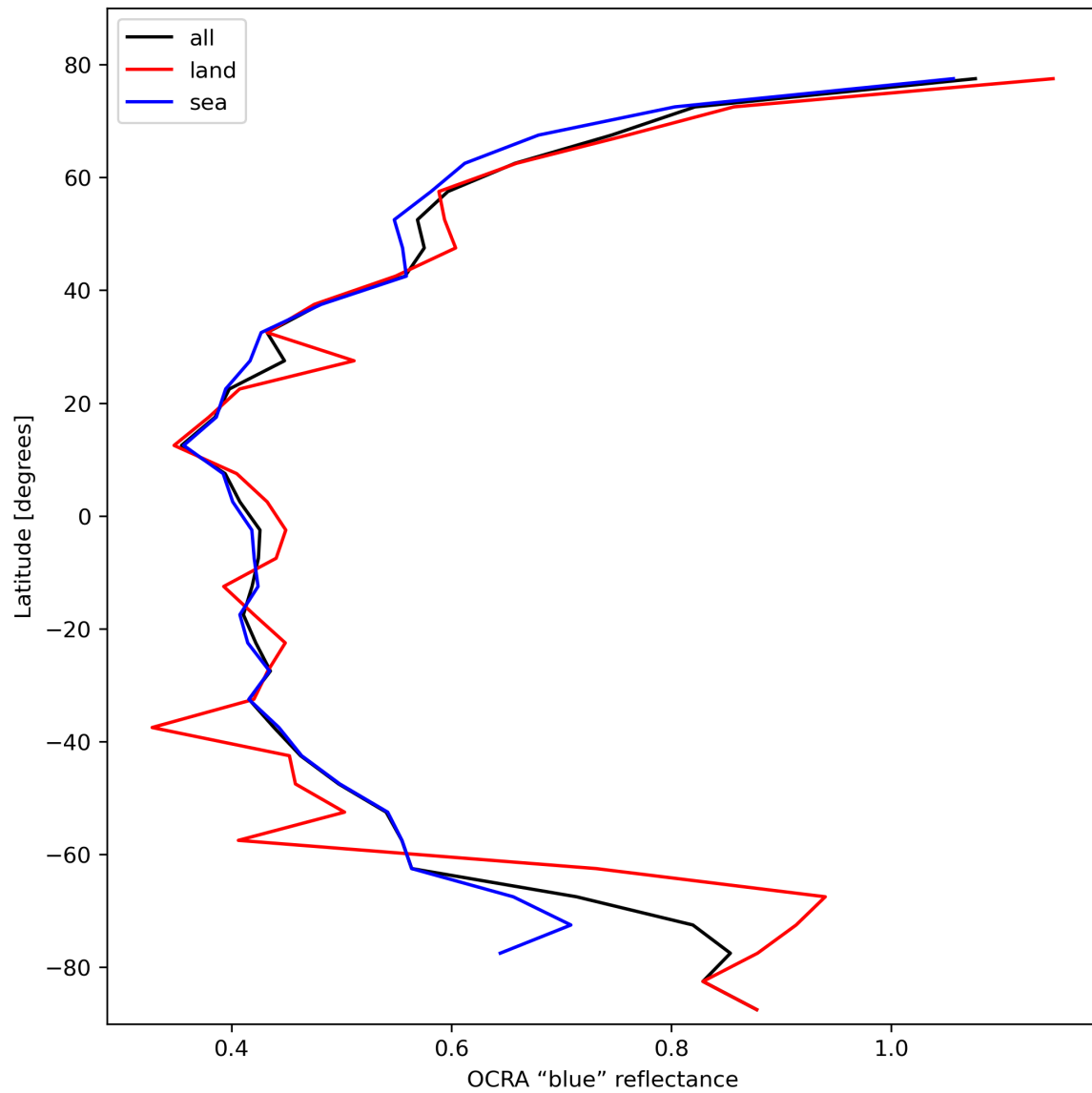
Figure 35: Zonal average of “OCRA “blue” reflectance” for 2024-02-14 to 2024-02-16.
