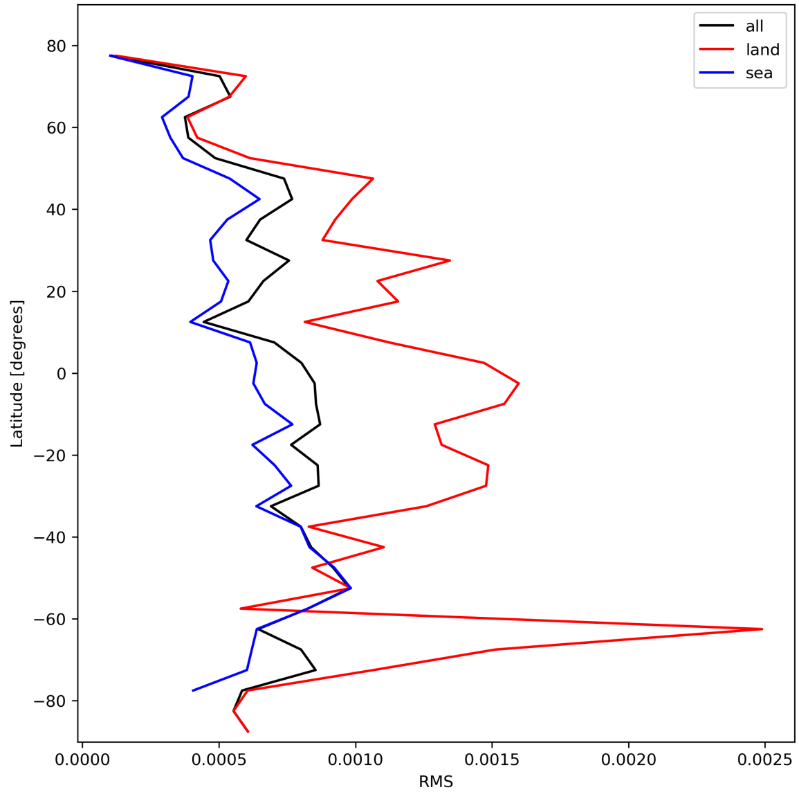
Figure 31: Zonal average of “RMS” for 2024-02-14 to 2024-02-16.
