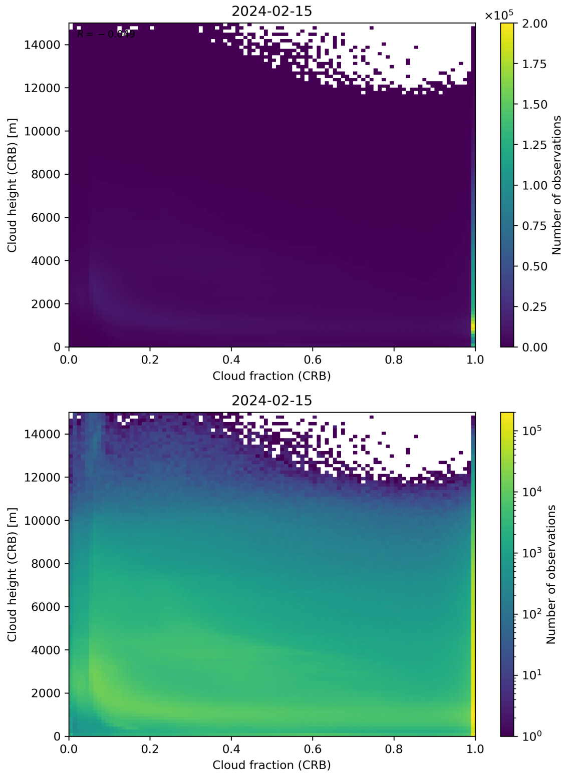
Figure 79: Scatter density plot of “Cloud fraction (CRB)” against “Cloud height (CRB)” for 2024-02-14 to 2024-02-16.
