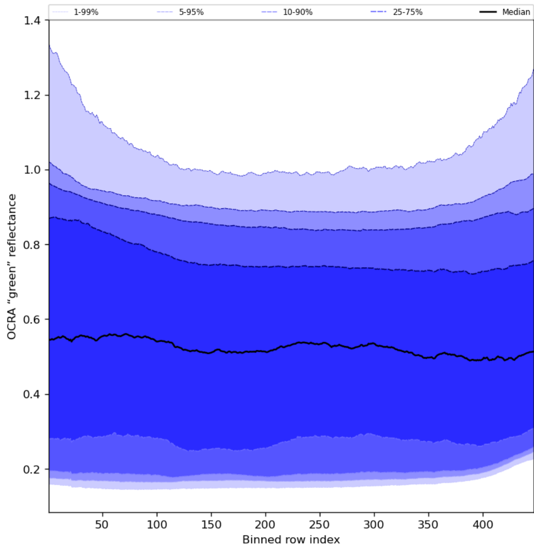
Figure 68: Along track statistics of “OCRA “green” reflectance” for 2024-02-14 to 2024-02-16
