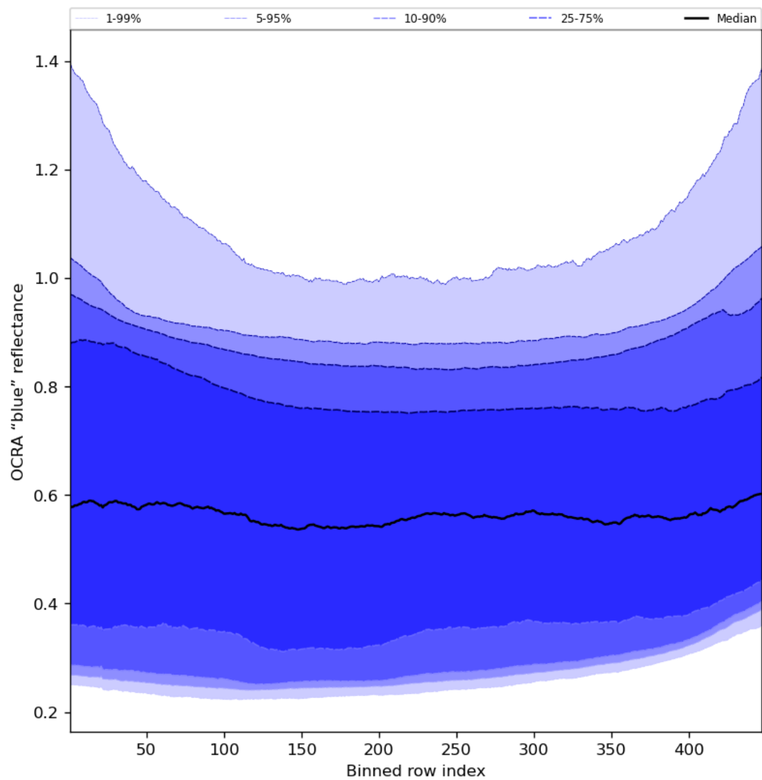
Figure 67: Along track statistics of “OCRA “blue” reflectance” for 2024-02-14 to 2024-02-16
