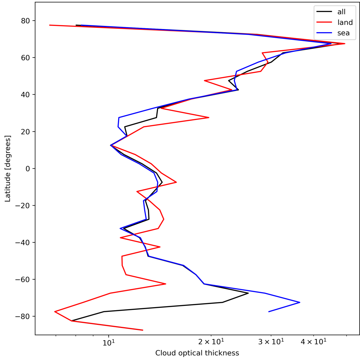
Figure 25: Zonal average of “Cloud optical thickness” for 2024-02-14 to 2024-02-16.
