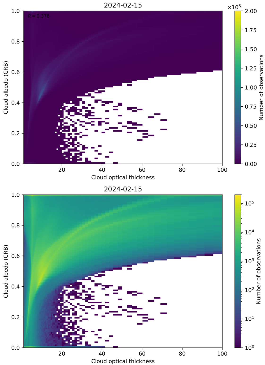
Figure 82: Scatter density plot of “Cloud optical thickness” against “Cloud albedo (CRB)” for 2024-02-14 to 2024-02-16.
