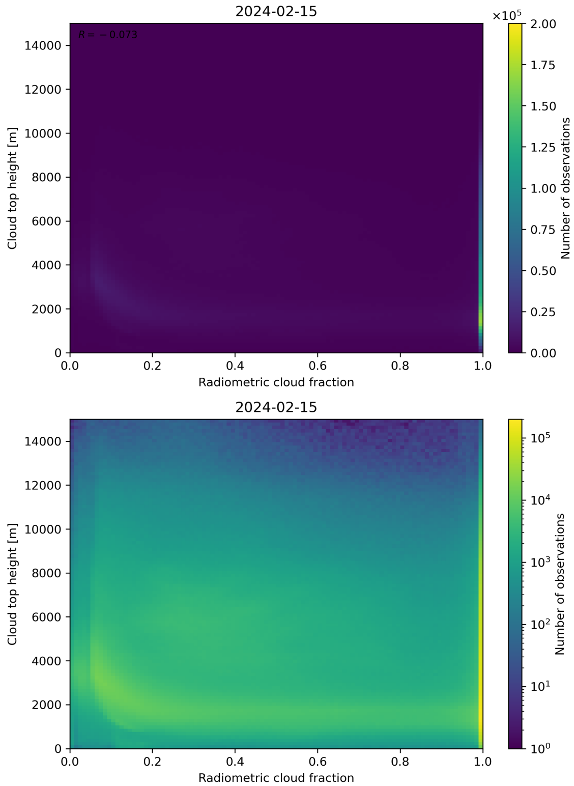
Figure 76: Scatter density plot of “Radiometric cloud fraction” against “Cloud top height” for 2024-02-14 to 2024-02-16.
