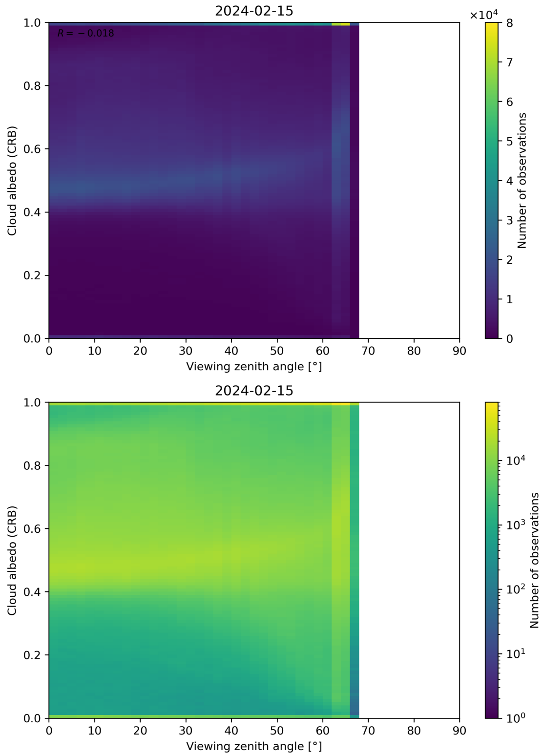
Figure 106: Scatter density plot of “Viewing zenith angle” against “Cloud albedo (CRB)” for 2024-02-14 to 2024-02-16.
