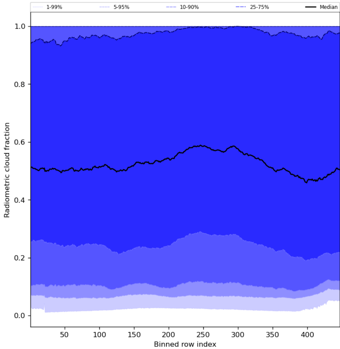
Figure 55: Along track statistics of “Radiometric cloud fraction” for 2024-02-14 to 2024-02-16
