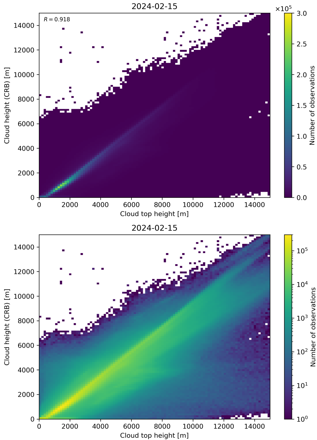
Figure 89: Scatter density plot of “Cloud top height” against “Cloud height (CRB)” for 2024-02-14 to 2024-02-16.
