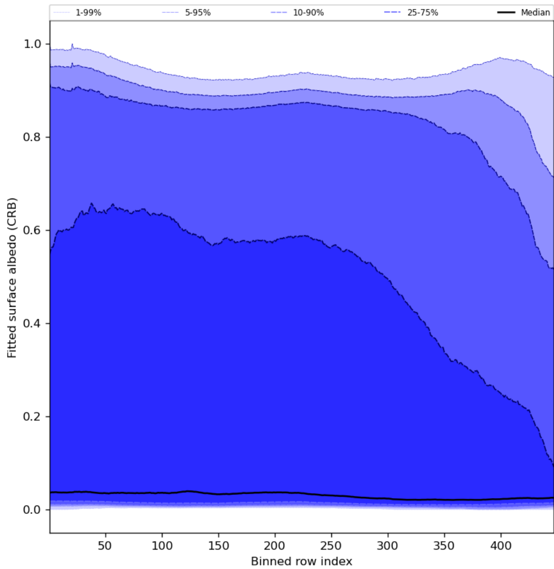
Figure 62: Along track statistics of “Fitted surface albedo (CRB)” for 2024-02-14 to 2024-02-16
