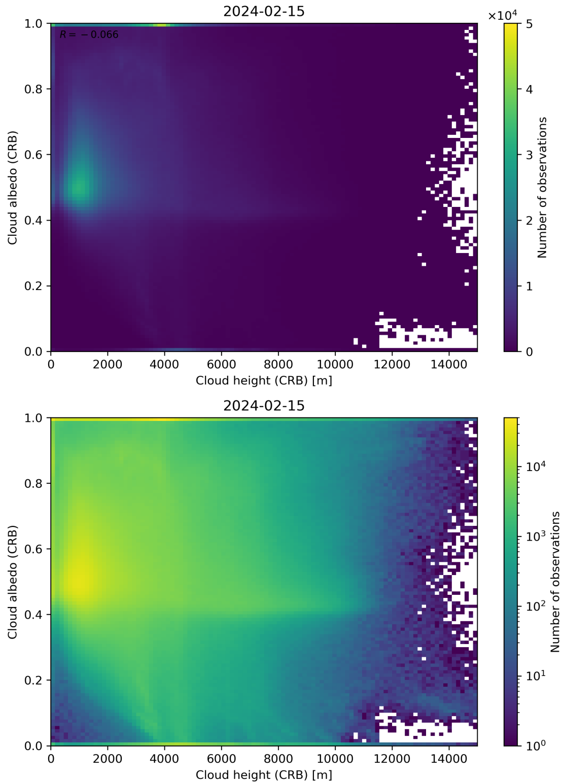
Figure 80: Scatter density plot of “Cloud height (CRB)” against “Cloud albedo (CRB)” for 2024-02-14 to 2024-02-16.
