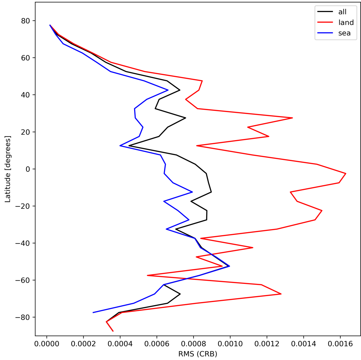
Figure 32: Zonal average of “RMS (CRB)” for 2024-02-14 to 2024-02-16.
