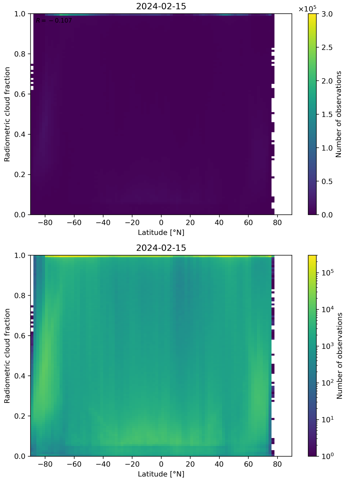
Figure 92: Scatter density plot of “Latitude” against “Radiometric cloud fraction” for 2024-02-14 to 2024-02-16.
