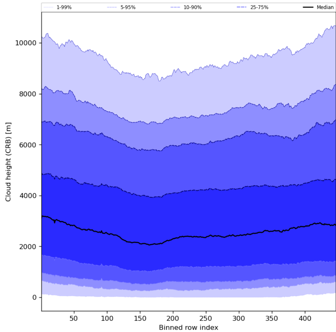
Figure 59: Along track statistics of “Cloud height (CRB)” for 2024-02-14 to 2024-02-16
