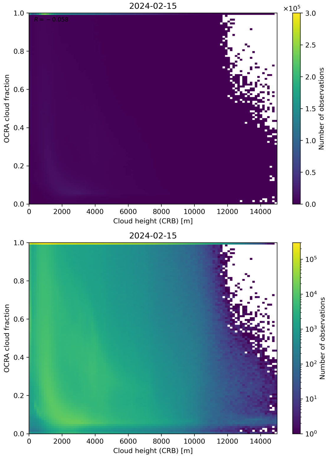
Figure 81: Scatter density plot of “Cloud height (CRB)” against “OCRA cloud fraction” for 2024-02-14 to 2024-02-16.
