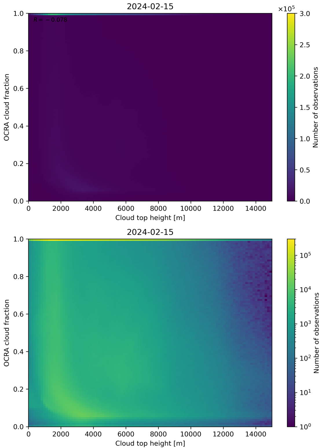
Figure 87: Scatter density plot of “Cloud top height” against “OCRA cloud fraction” for 2024-02-14 to 2024-02-16.
