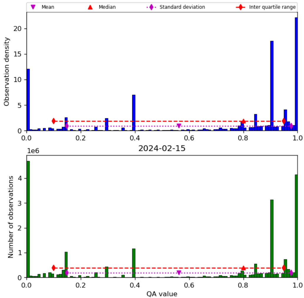
Figure 38: Histogram of “QA value” for 2024-02-14 to 2024-02-16
