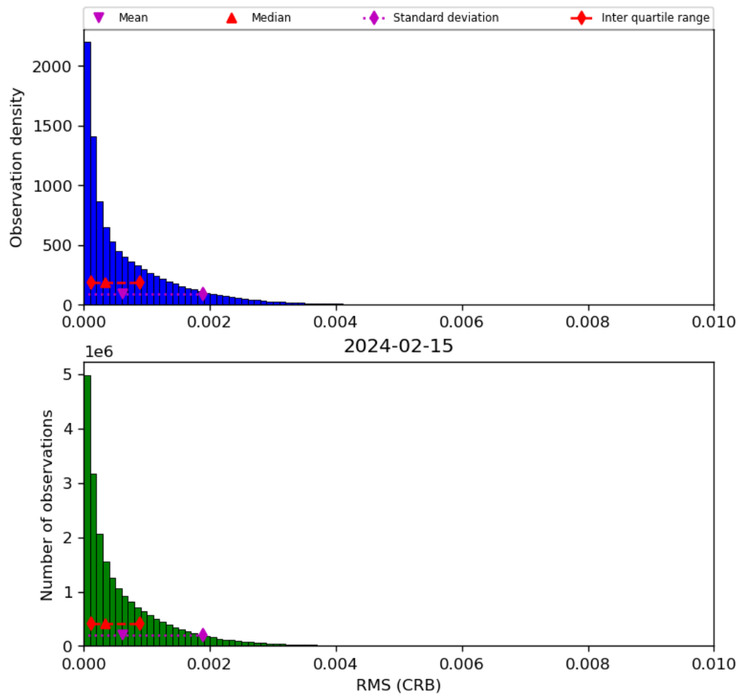
Figure 48: Histogram of “RMS (CRB)” for 2024-02-14 to 2024-02-16
