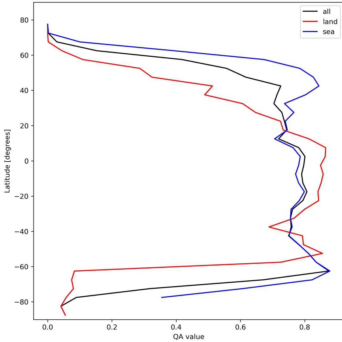
Figure 22: Zonal average of “QA value” for 2024-02-14 to 2024-02-16.
