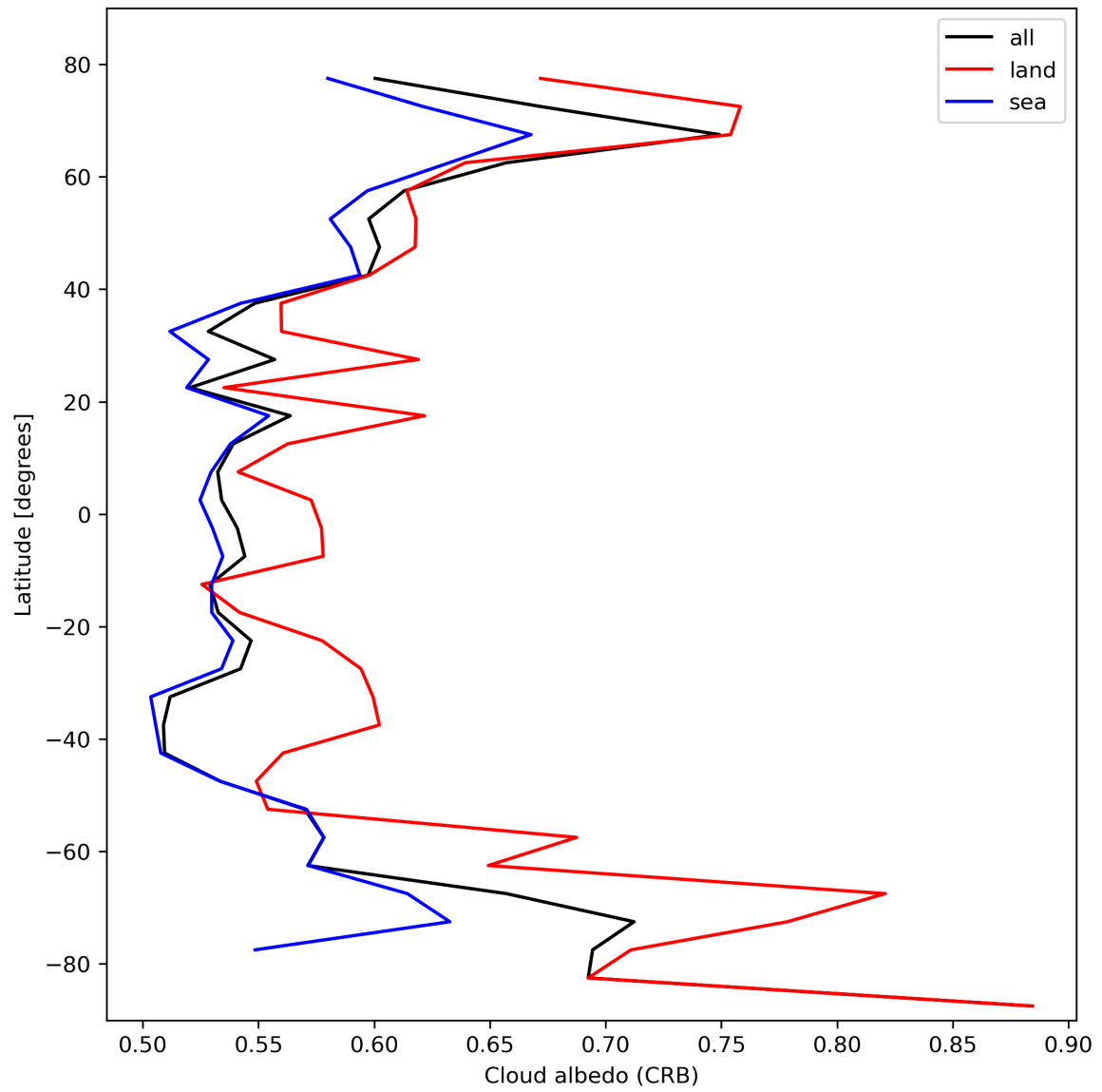
Figure 28: Zonal average of “Cloud albedo (CRB)” for 2024-02-14 to 2024-02-16.
