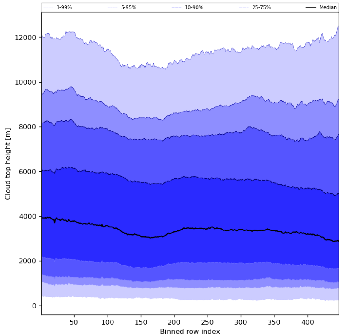
Figure 56: Along track statistics of “Cloud top height” for 2024-02-14 to 2024-02-16
