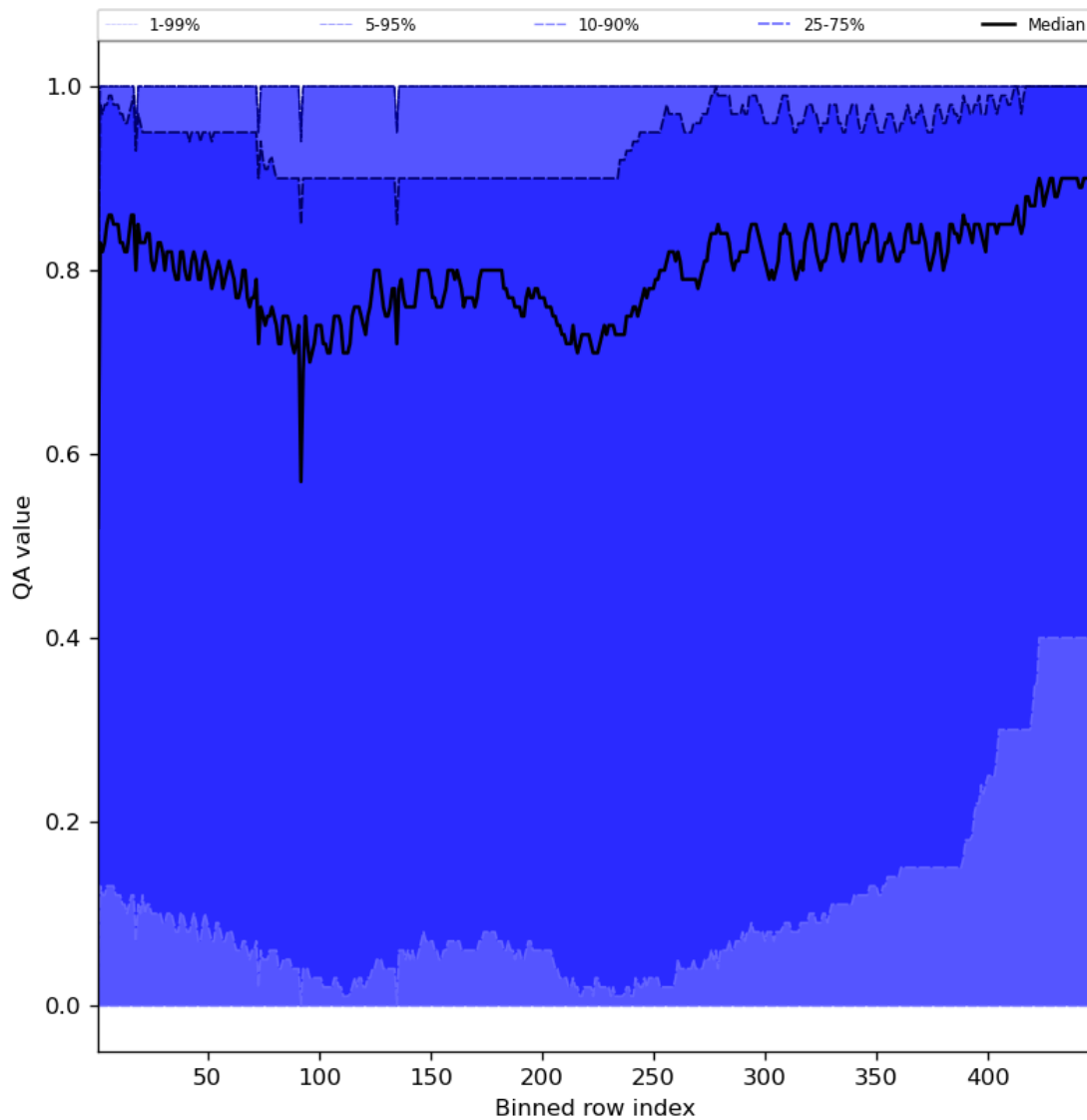
Figure 54: Along track statistics of “QA value” for 2024-02-14 to 2024-02-16
