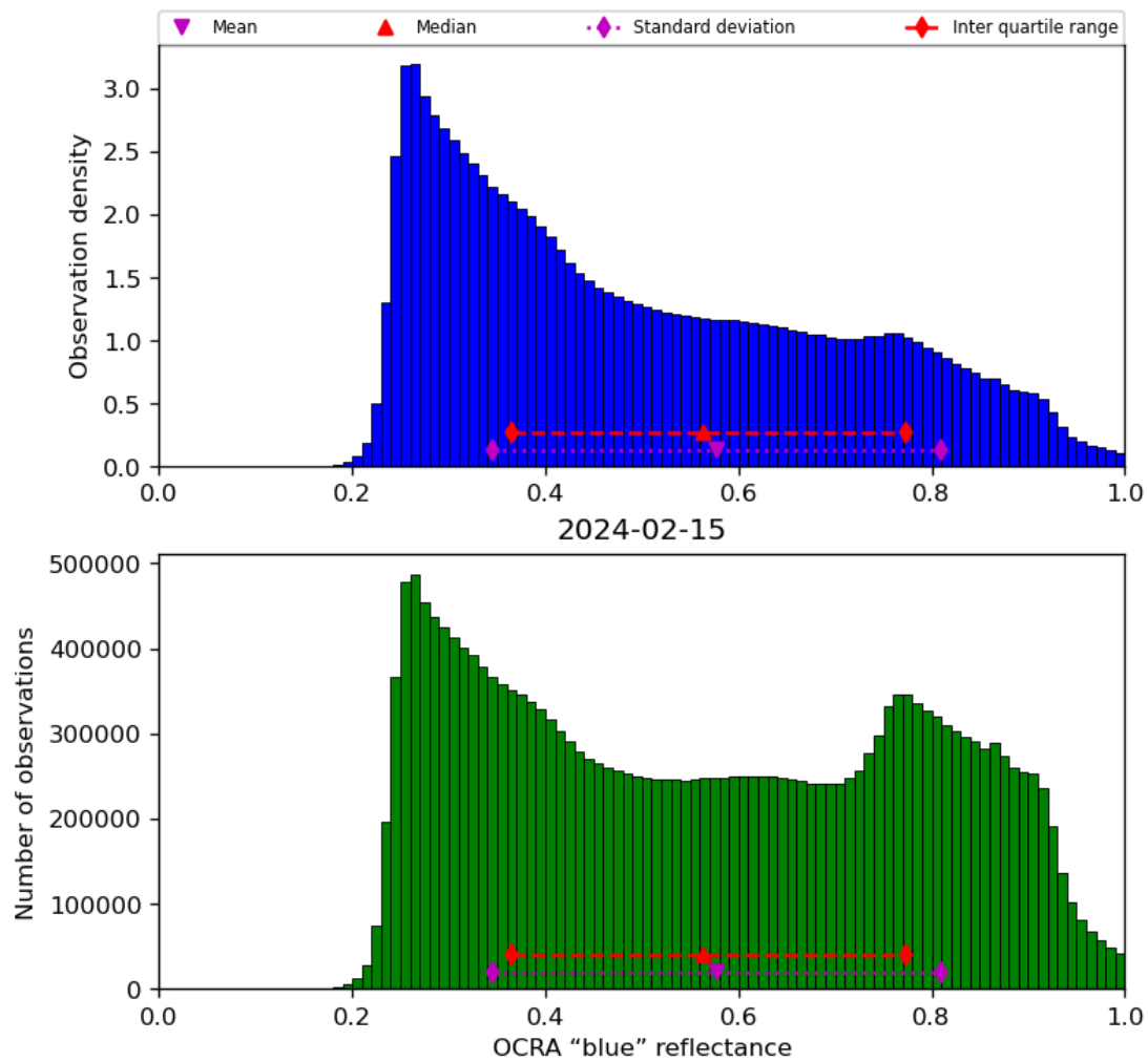
Figure 51: Histogram of “OCRA “blue” reflectance” for 2024-02-14 to 2024-02-16
