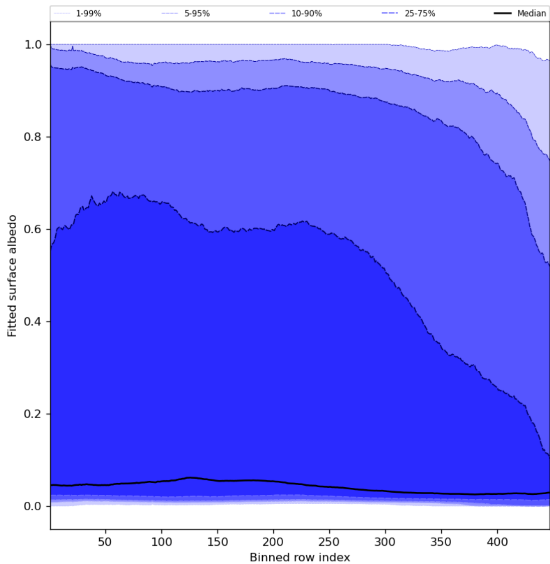
Figure 61: Along track statistics of “Fitted surface albedo” for 2024-02-14 to 2024-02-16
