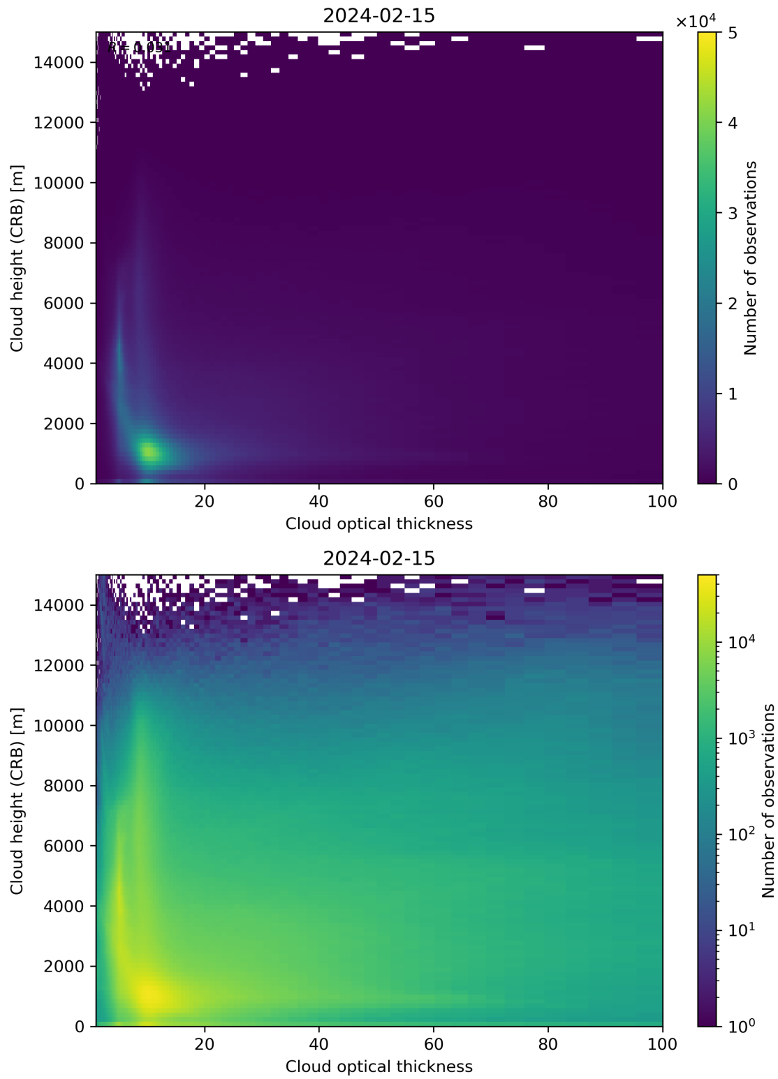
Figure 85: Scatter density plot of “Cloud optical thickness” against “Cloud height (CRB)” for 2024-02-14 to 2024-02-16.
