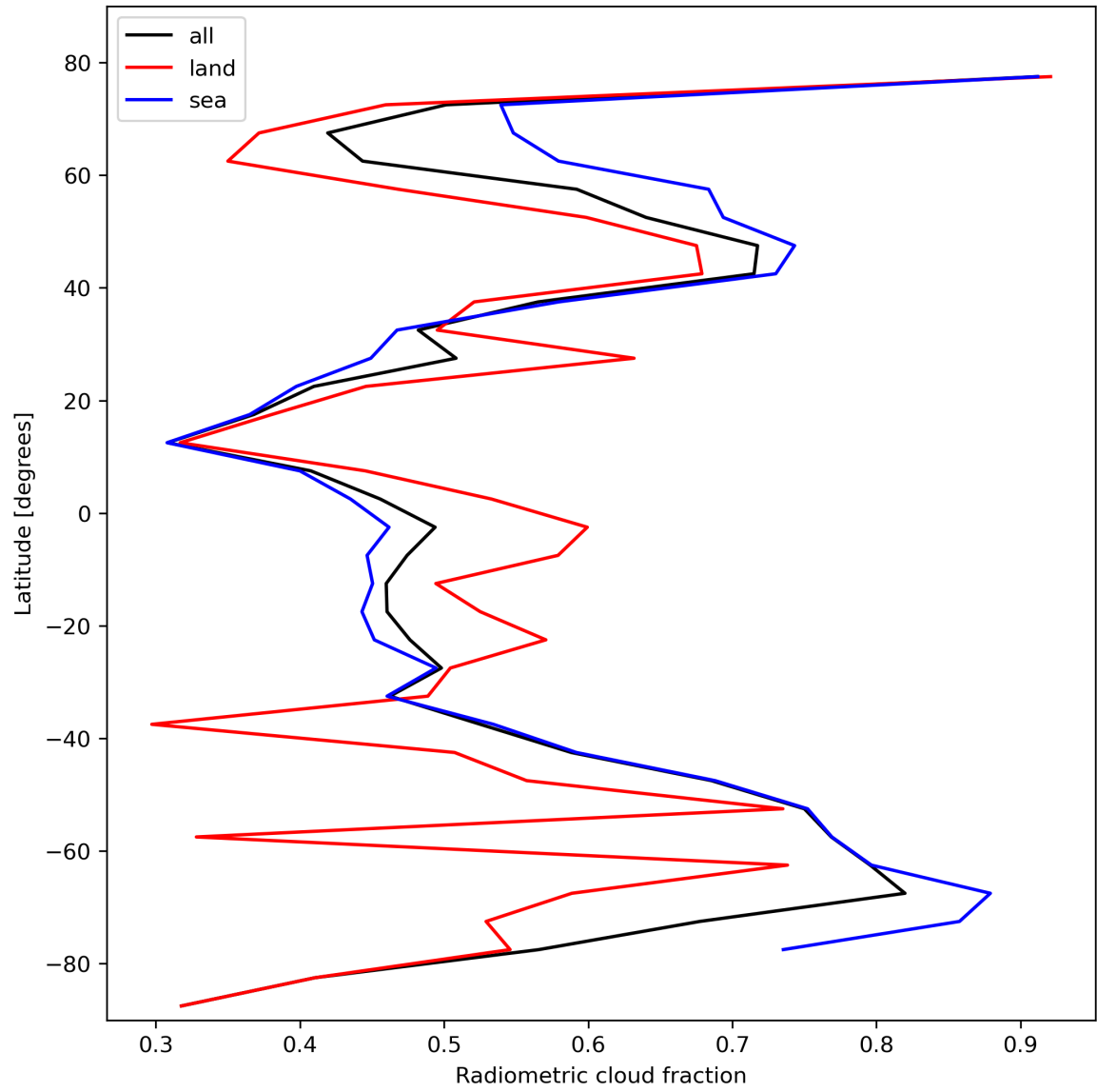
Figure 23: Zonal average of “Radiometric cloud fraction” for 2024-02-14 to 2024-02-16.
