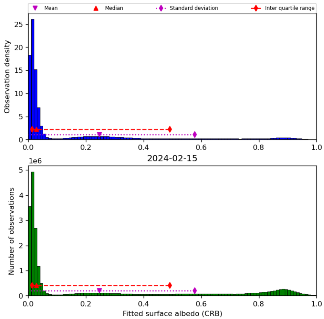
Figure 46: Histogram of “Fitted surface albedo (CRB)” for 2024-02-14 to 2024-02-16
