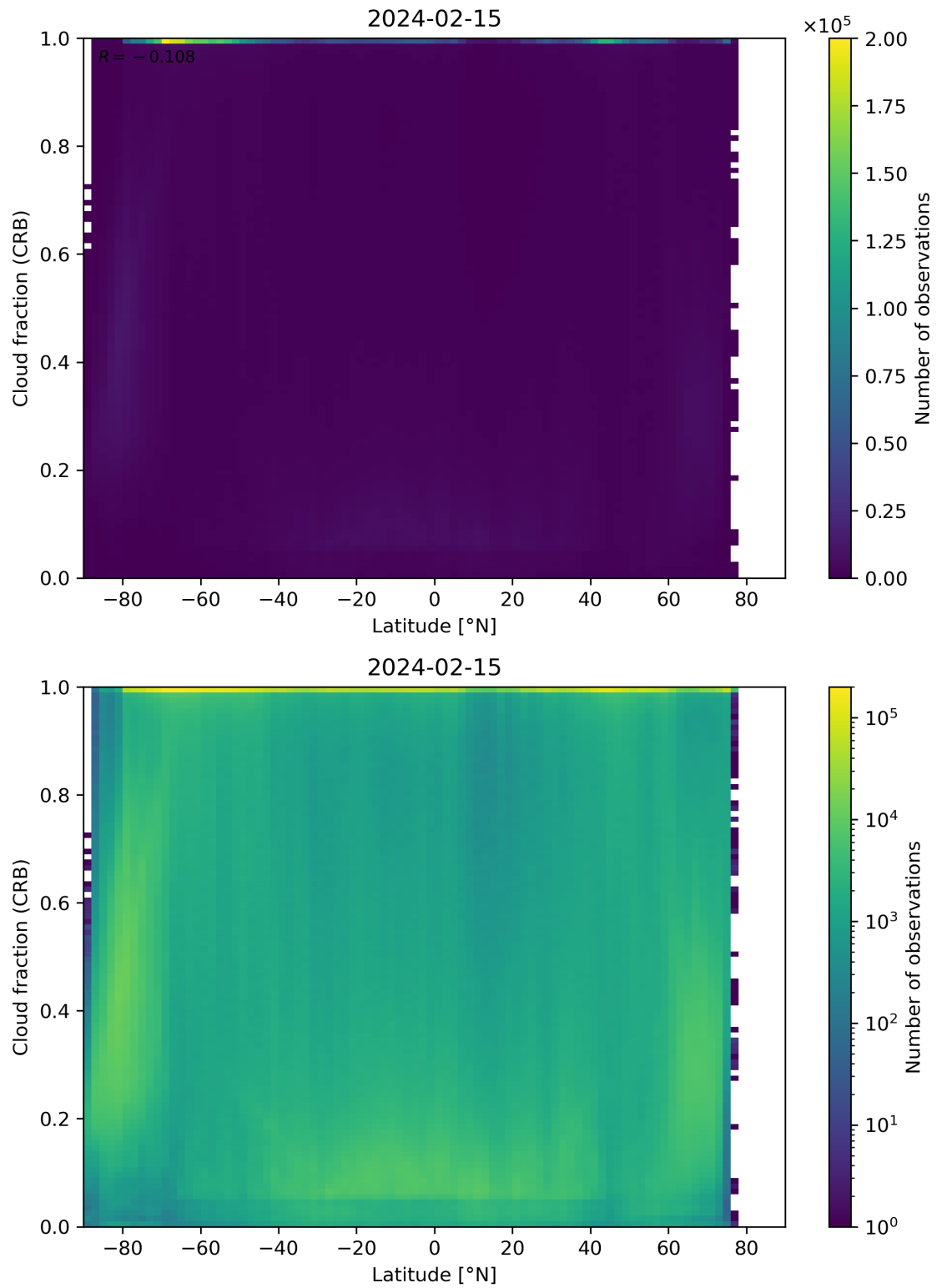
Figure 94: Scatter density plot of “Latitude” against “Cloud fraction (CRB)” for 2024-02-14 to 2024-02-16.
