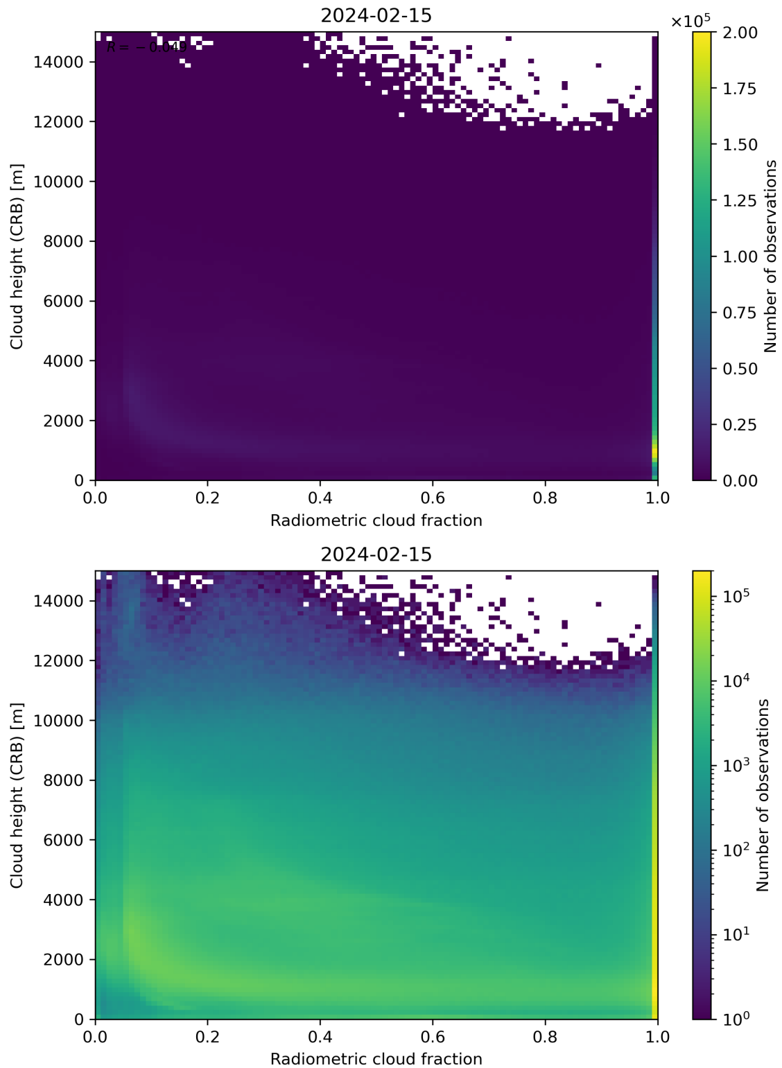
Figure 74: Scatter density plot of “Radiometric cloud fraction” against “Cloud height (CRB)” for 2024-02-14 to 2024-02-16.
