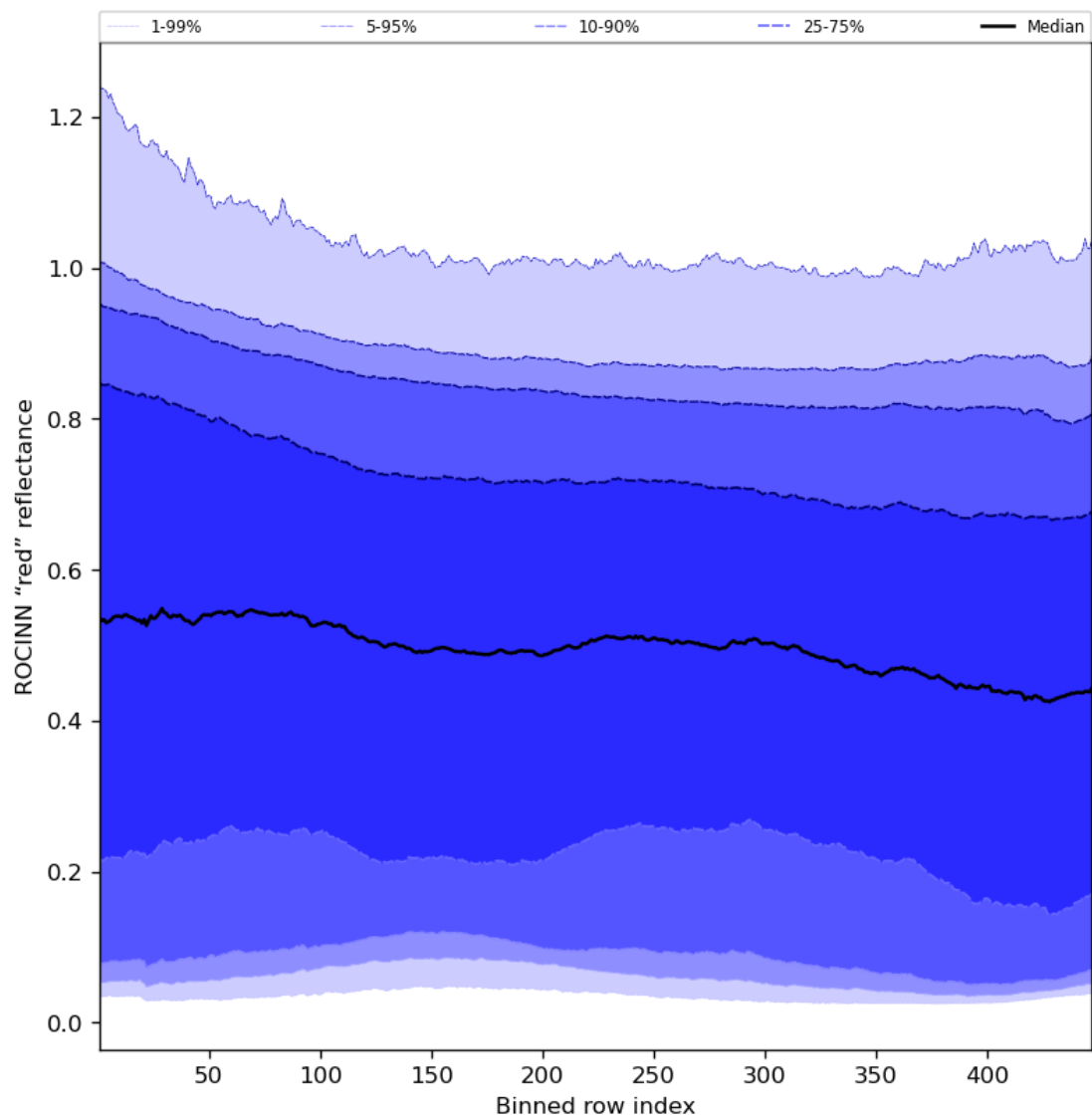
Figure 69: Along track statistics of “ROCINN “red” reflectance” for 2024-02-14 to 2024-02-16
