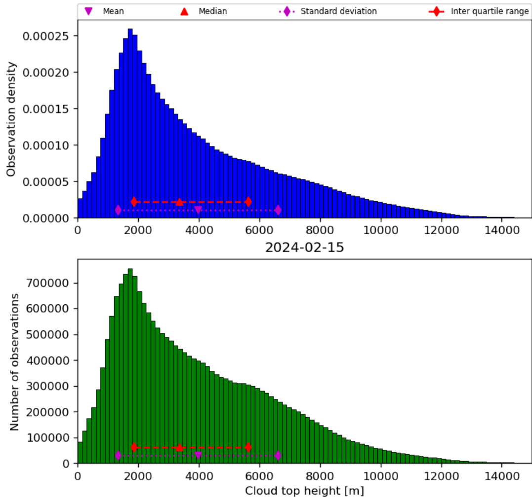
Figure 40: Histogram of “Cloud top height” for 2024-02-14 to 2024-02-16
