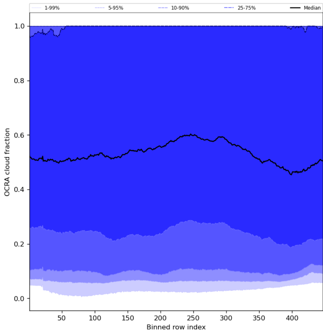
Figure 66: Along track statistics of “OCRA cloud fraction” for 2024-02-14 to 2024-02-16
