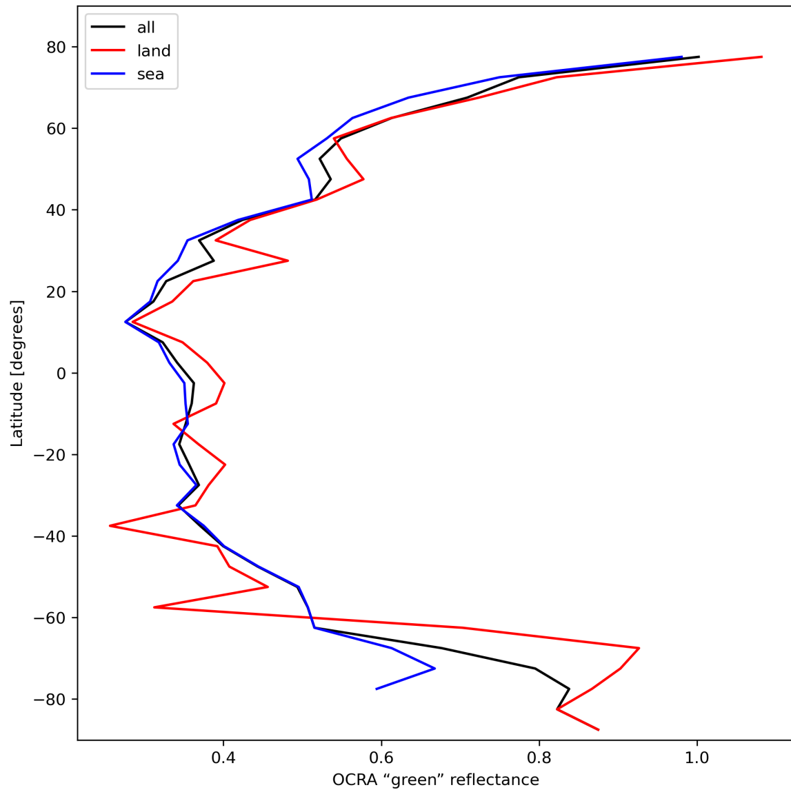
Figure 36: Zonal average of “OCRA “green” reflectance” for 2024-02-14 to 2024-02-16.
