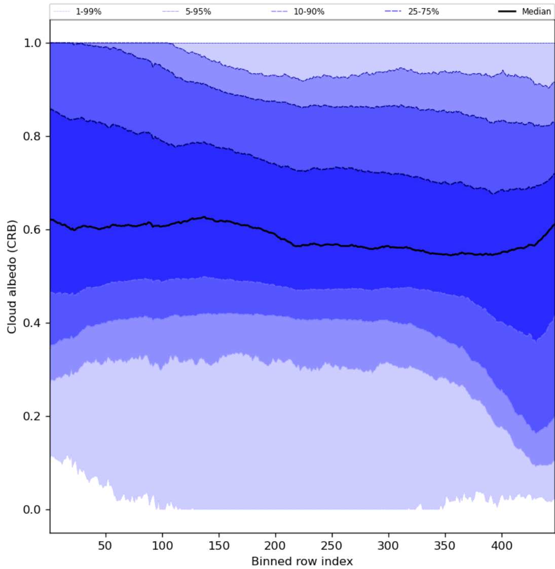
Figure 60: Along track statistics of “Cloud albedo (CRB)” for 2024-02-14 to 2024-02-16
