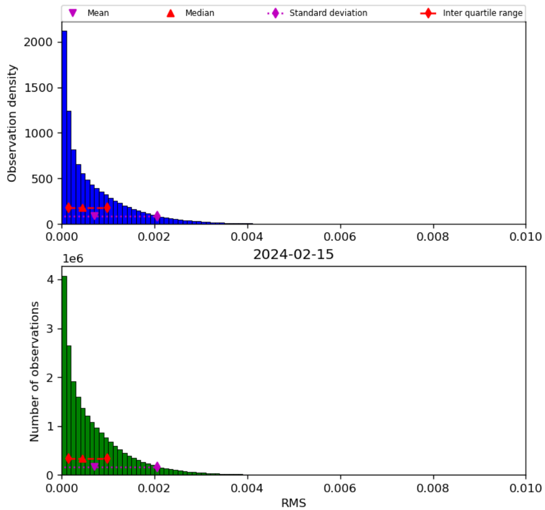
Figure 47: Histogram of “RMS” for 2024-02-14 to 2024-02-16
