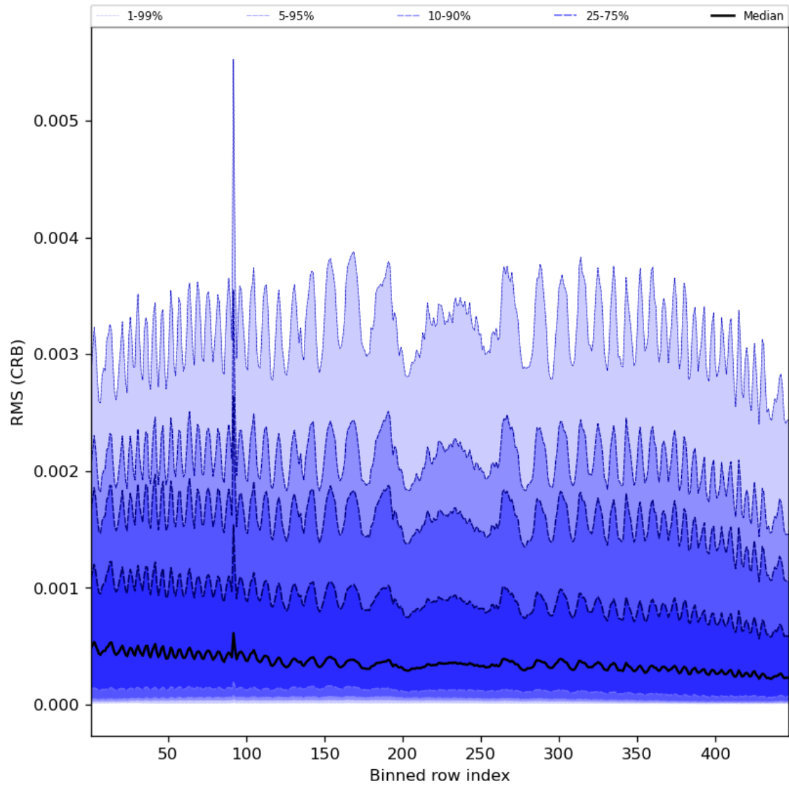
Figure 64: Along track statistics of "RMS (CRB)" for 2024-02-14 to 2024-02-16
