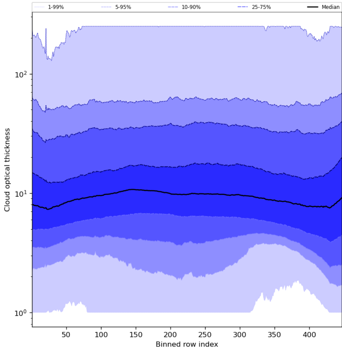
Figure 57: Along track statistics of “Cloud optical thickness” for 2024-02-14 to 2024-02-16
