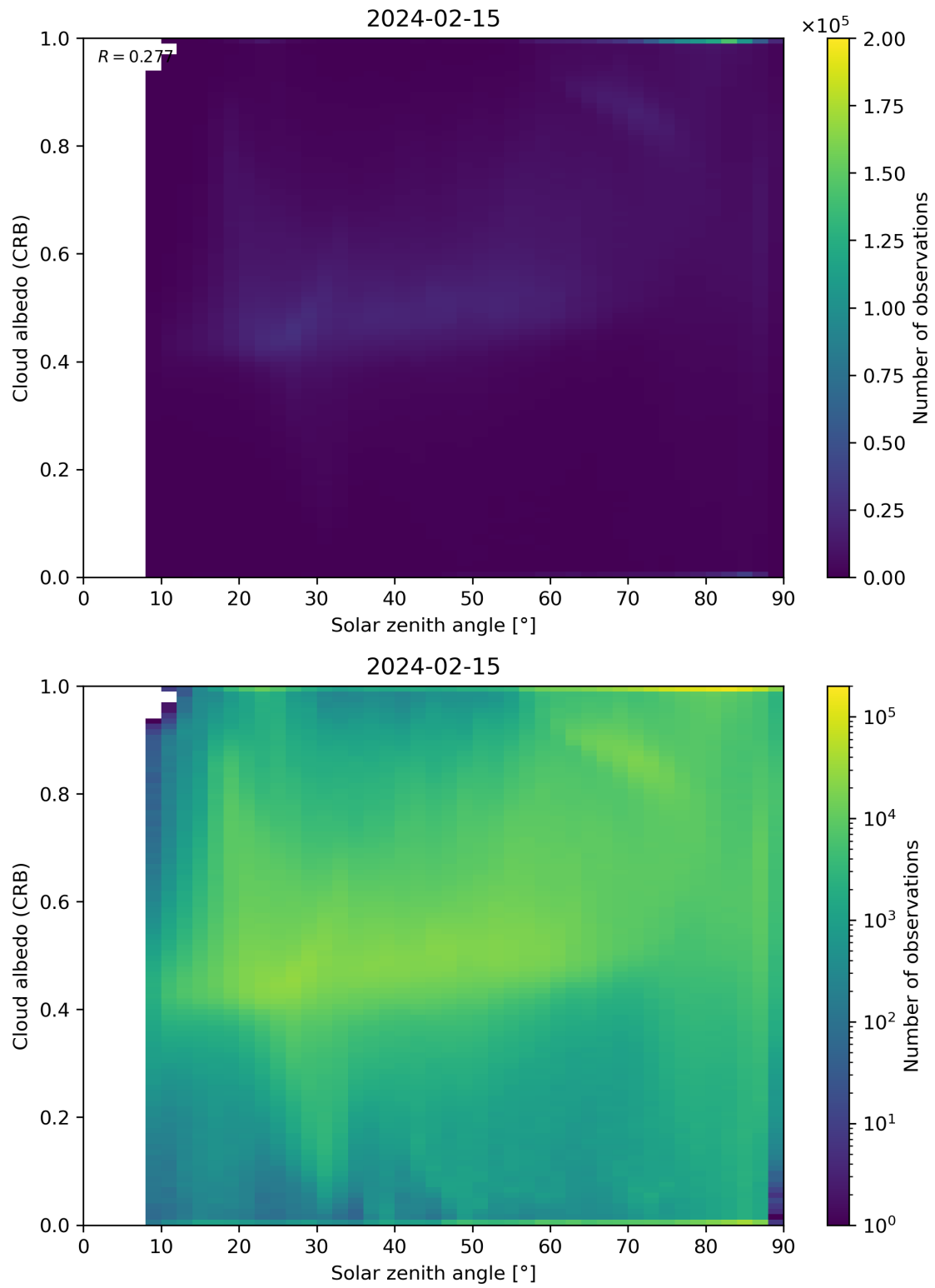
Figure 98: Scatter density plot of “Solar zenith angle” against “Cloud albedo (CRB)” for 2024-02-14 to 2024-02-16.
