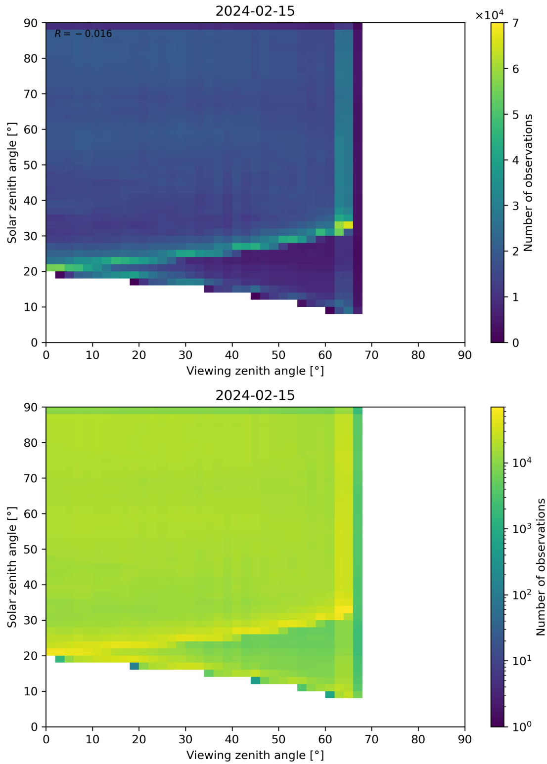
Figure 114: Scatter density plot of “Viewing zenith angle” against “Solar zenith angle” for 2024-02-14 to 2024-02-16.
