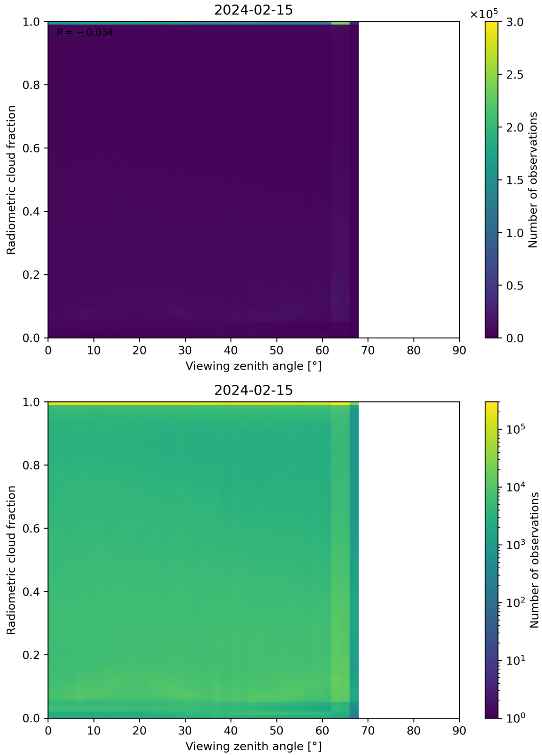
Figure 107: Scatter density plot of “Viewing zenith angle” against “Radiometric cloud fraction” for 2024-02-14 to 2024-02-16.
