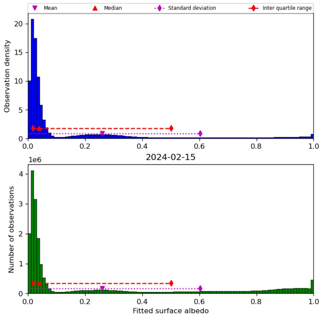
Figure 45: Histogram of “Fitted surface albedo” for 2024-02-14 to 2024-02-16
