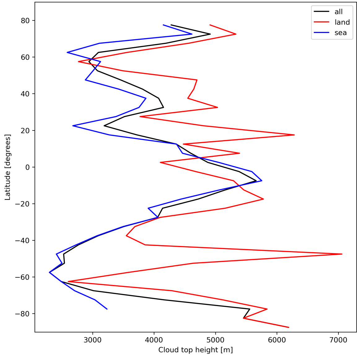
Figure 24: Zonal average of “Cloud top height” for 2024-02-14 to 2024-02-16.
