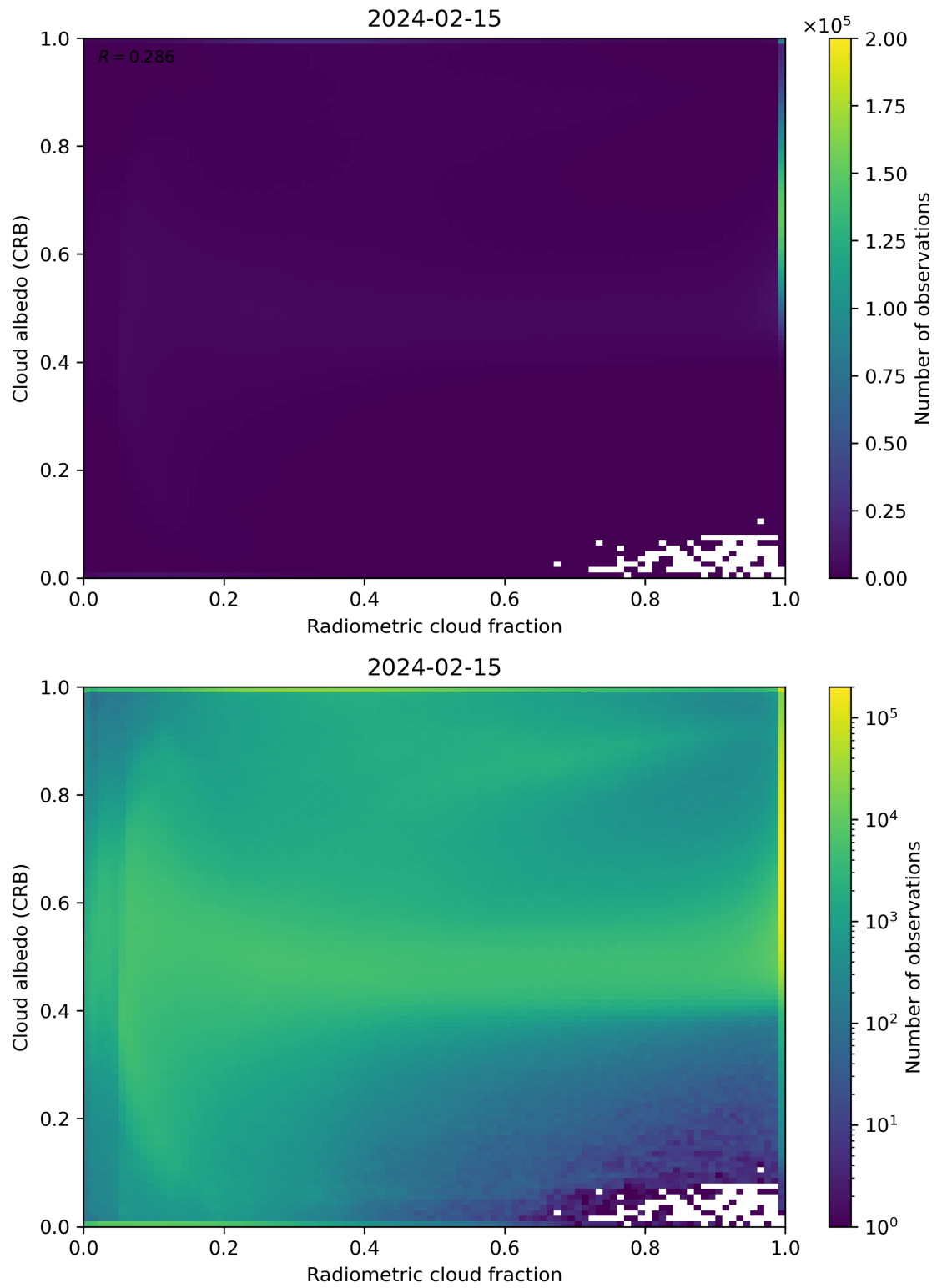
Figure 71: Scatter density plot of “Radiometric cloud fraction” against “Cloud albedo (CRB)” for 2024-02-14 to 2024-02-16.
