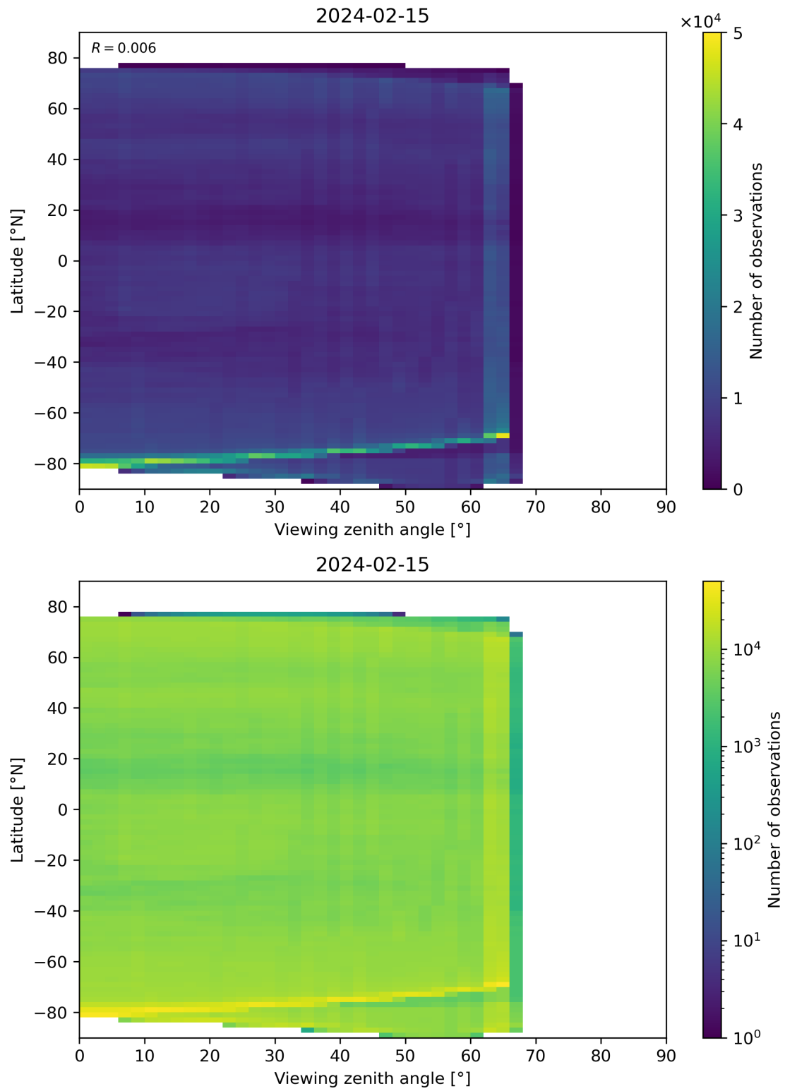
Figure 113: Scatter density plot of “Viewing zenith angle” against “Latitude” for 2024-02-14 to 2024-02-16.
