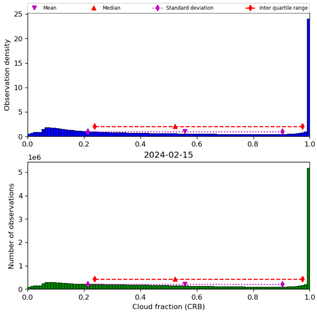
Figure 42: Histogram of “Cloud fraction (CRB)” for 2024-02-14 to 2024-02-16
