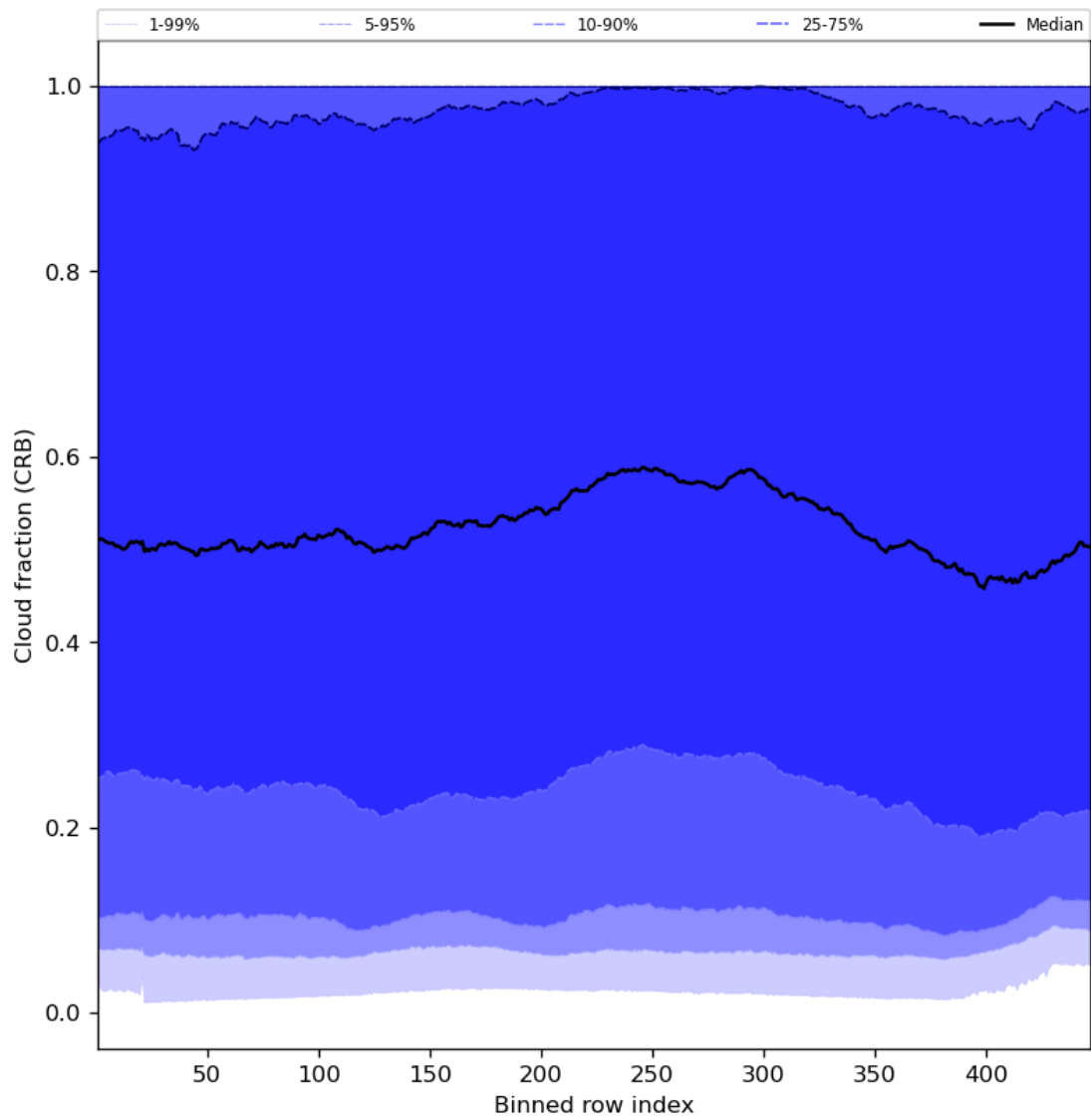
Figure 58: Along track statistics of “Cloud fraction (CRB)” for 2024-02-14 to 2024-02-16
