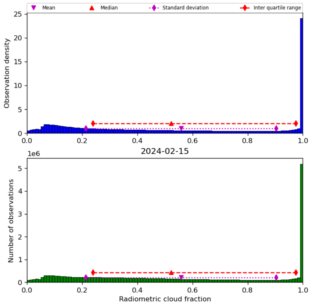
Figure 39: Histogram of “Radiometric cloud fraction” for 2024-02-14 to 2024-02-16
