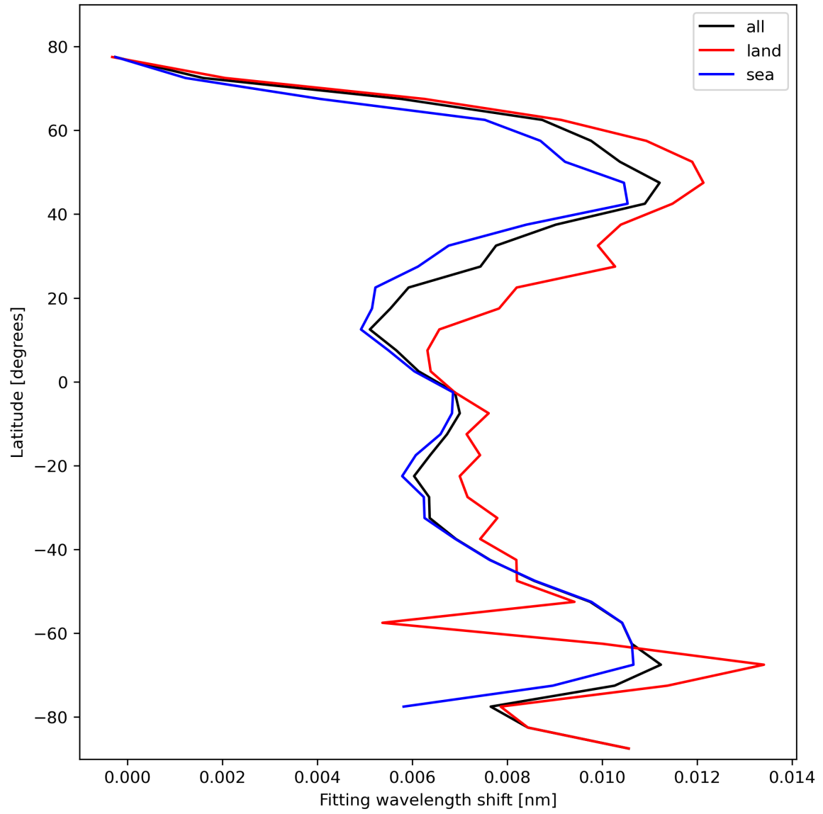
Figure 33: Zonal average of “Fitting wavelength shift” for 2024-02-14 to 2024-02-16.
