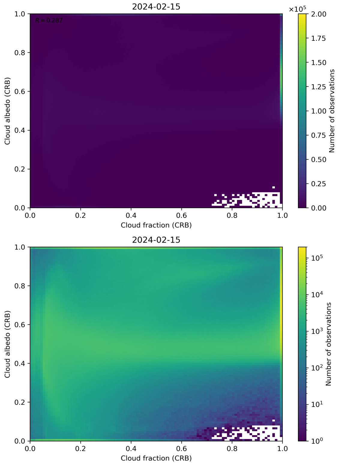
Figure 77: Scatter density plot of “Cloud fraction (CRB)” against “Cloud albedo (CRB)” for 2024-02-14 to 2024-02-16.
