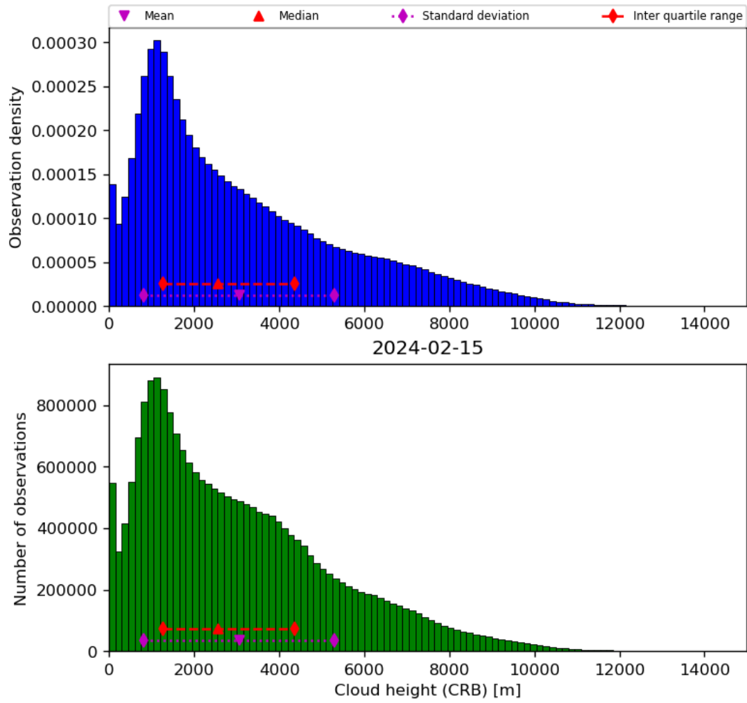
Figure 43: Histogram of “Cloud height (CRB)” for 2024-02-14 to 2024-02-16
