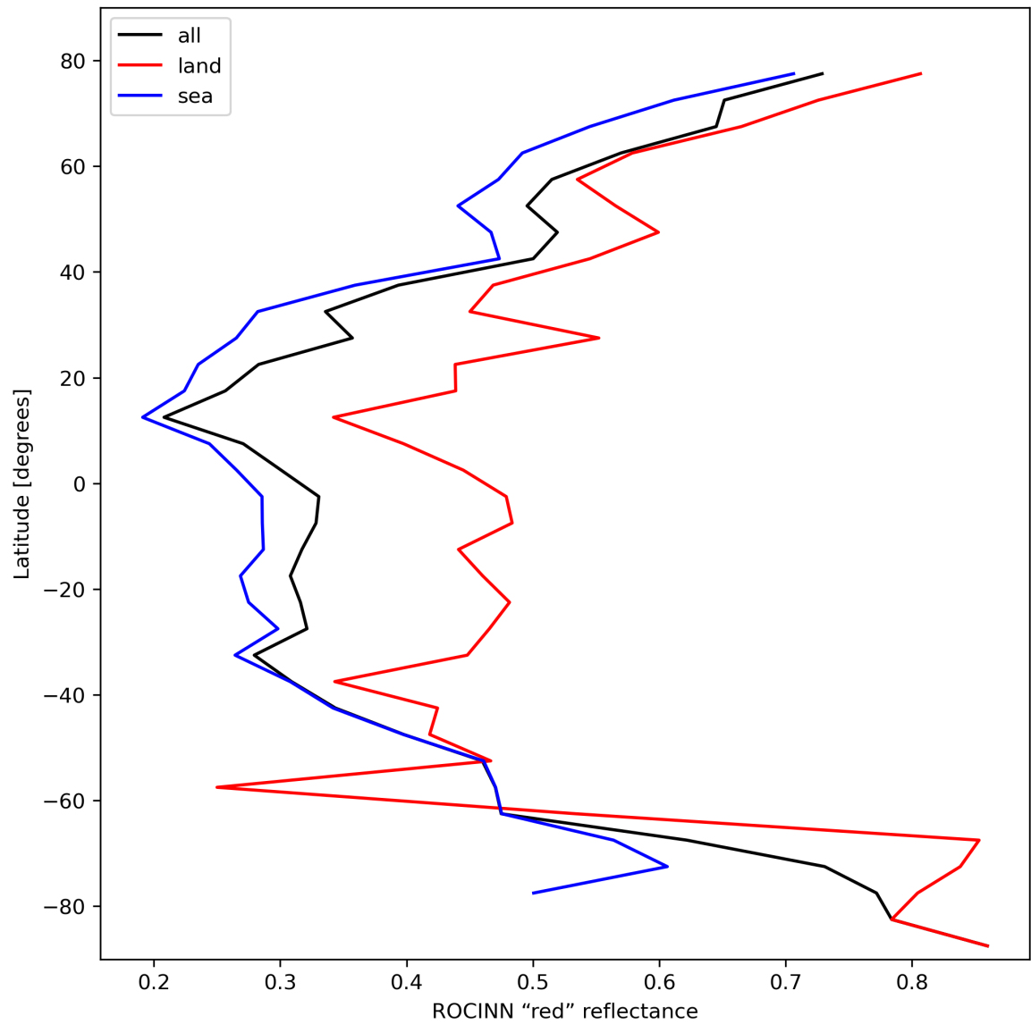
Figure 37: Zonal average of "ROCINN "red" reflectance" for 2024-02-14 to 2024-02-16.
