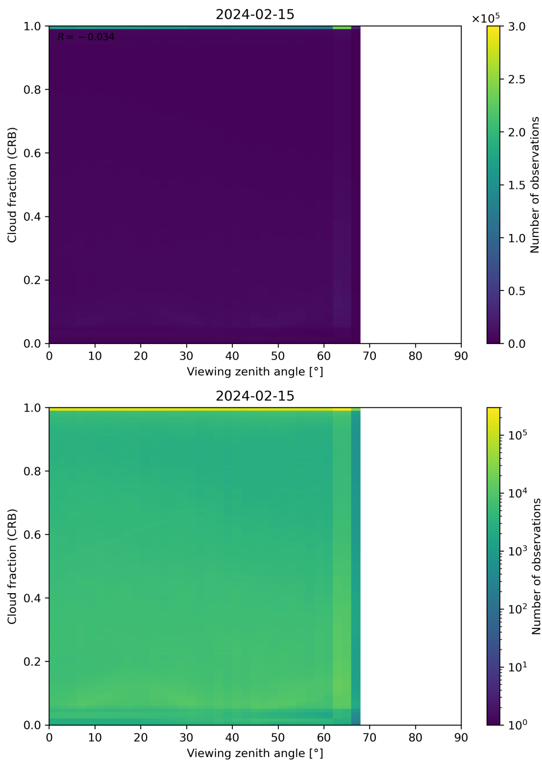
Figure 109: Scatter density plot of “Viewing zenith angle” against “Cloud fraction (CRB)” for 2024-02-14 to 2024-02-16.
