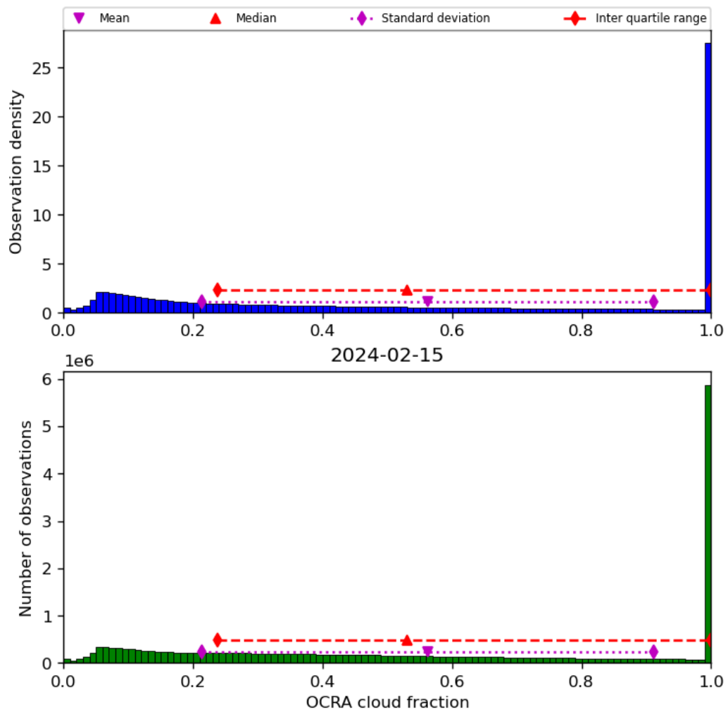
Figure 50: Histogram of “OCRA cloud fraction” for 2024-02-14 to 2024-02-16
