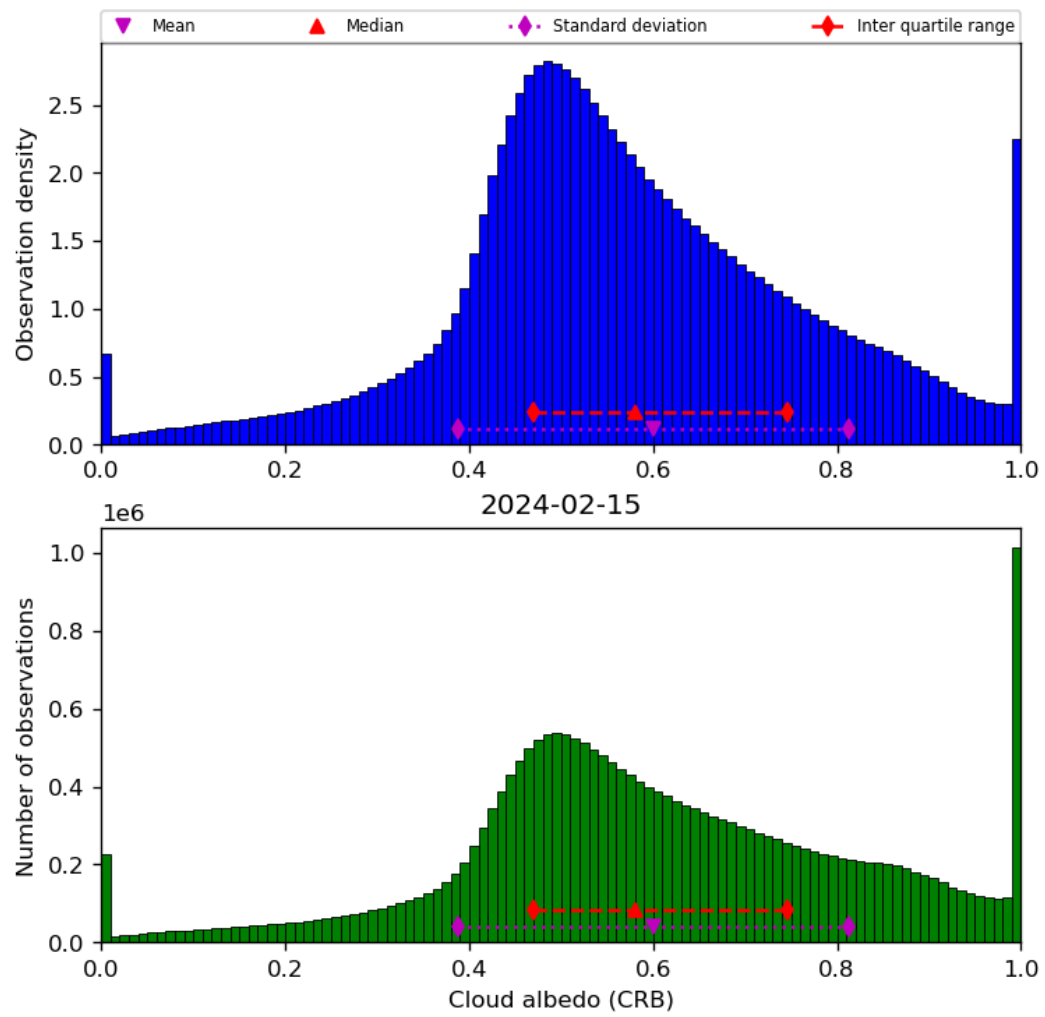
Figure 44: Histogram of “Cloud albedo (CRB)” for 2024-02-14 to 2024-02-16
