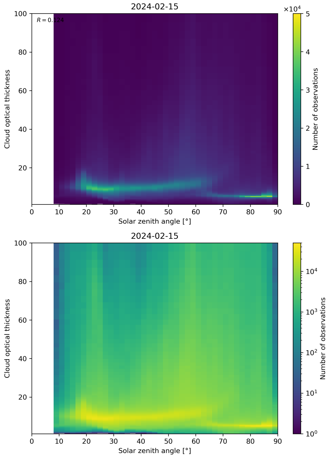
Figure 103: Scatter density plot of “Solar zenith angle” against “Cloud optical thickness” for 2024-02-14 to 2024-02-16.
