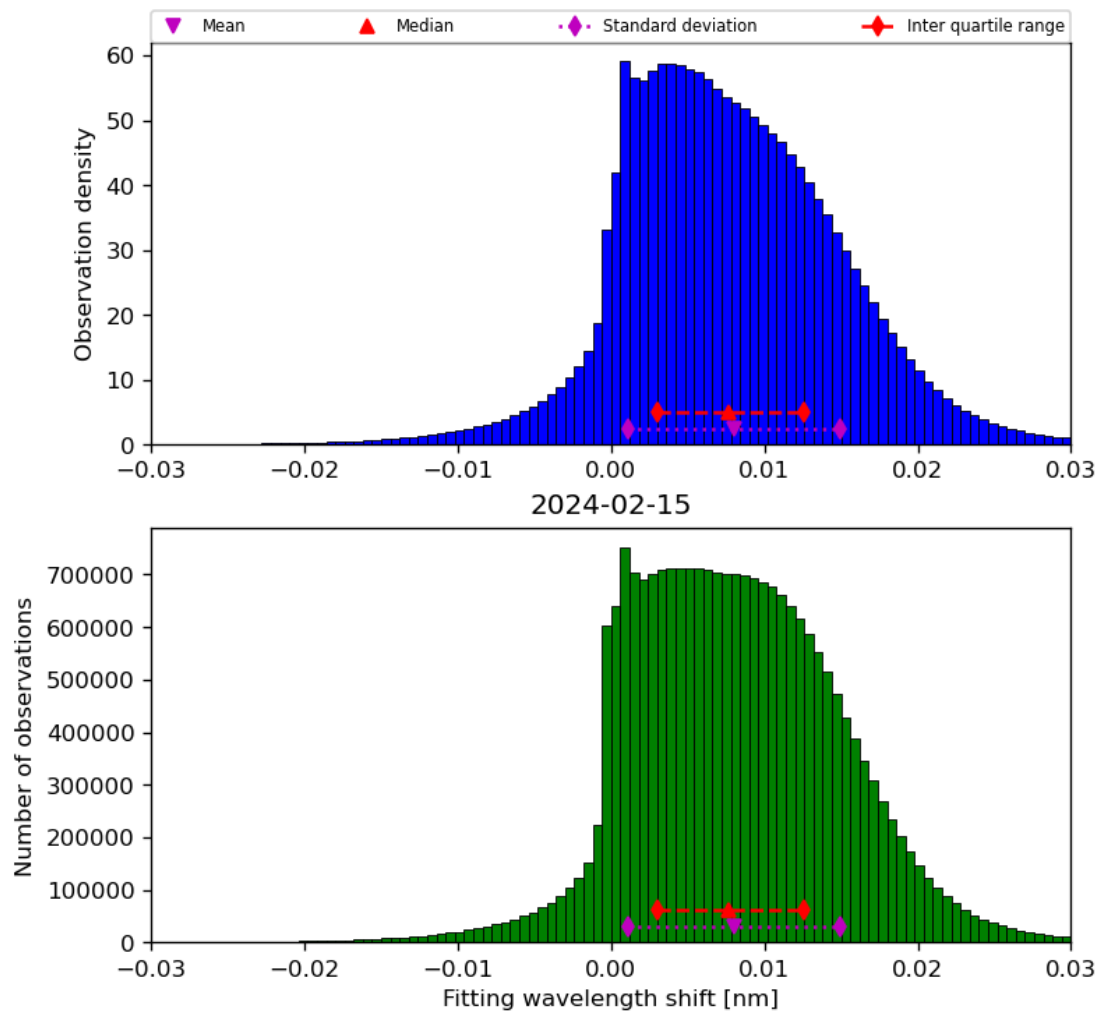
Figure 49: Histogram of “Fitting wavelength shift” for 2024-02-14 to 2024-02-16
