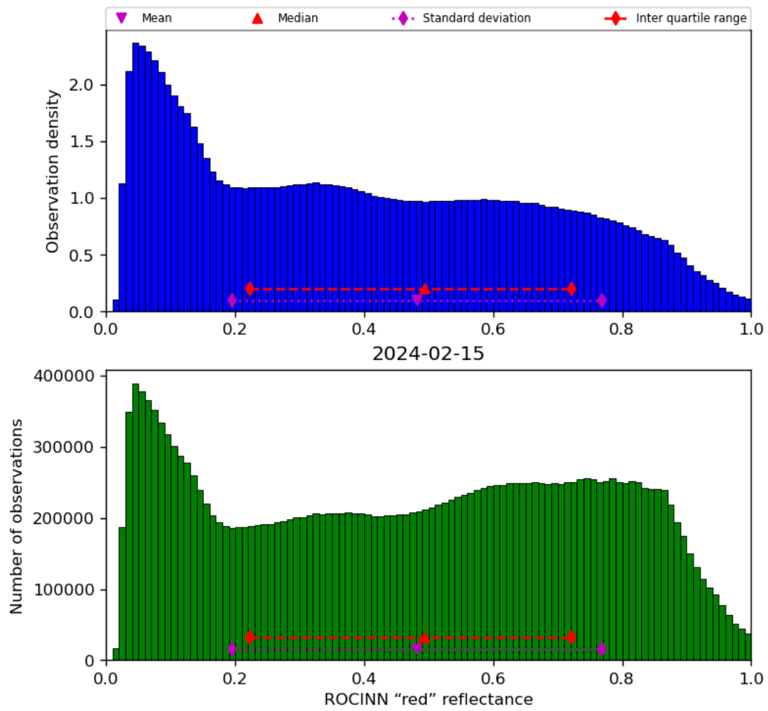
Figure 53: Histogram of “ROCINN “red” reflectance” for 2024-02-14 to 2024-02-16
