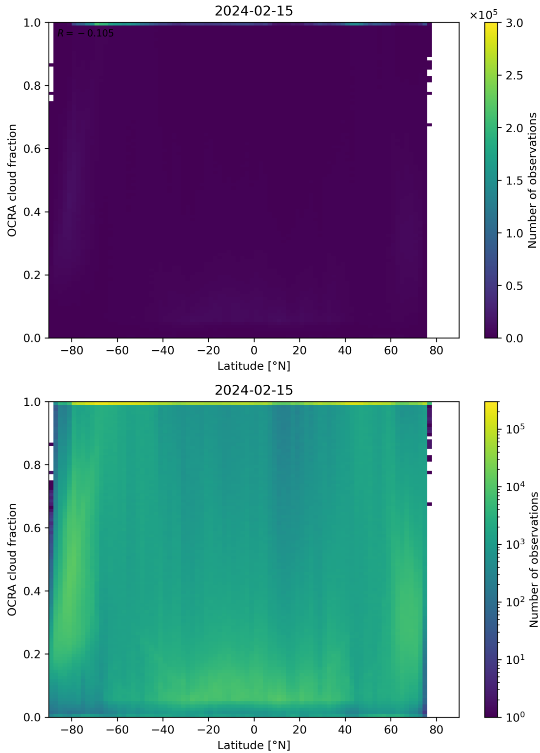
Figure 93: Scatter density plot of “Latitude” against “OCRA cloud fraction” for 2024-02-14 to 2024-02-16.
