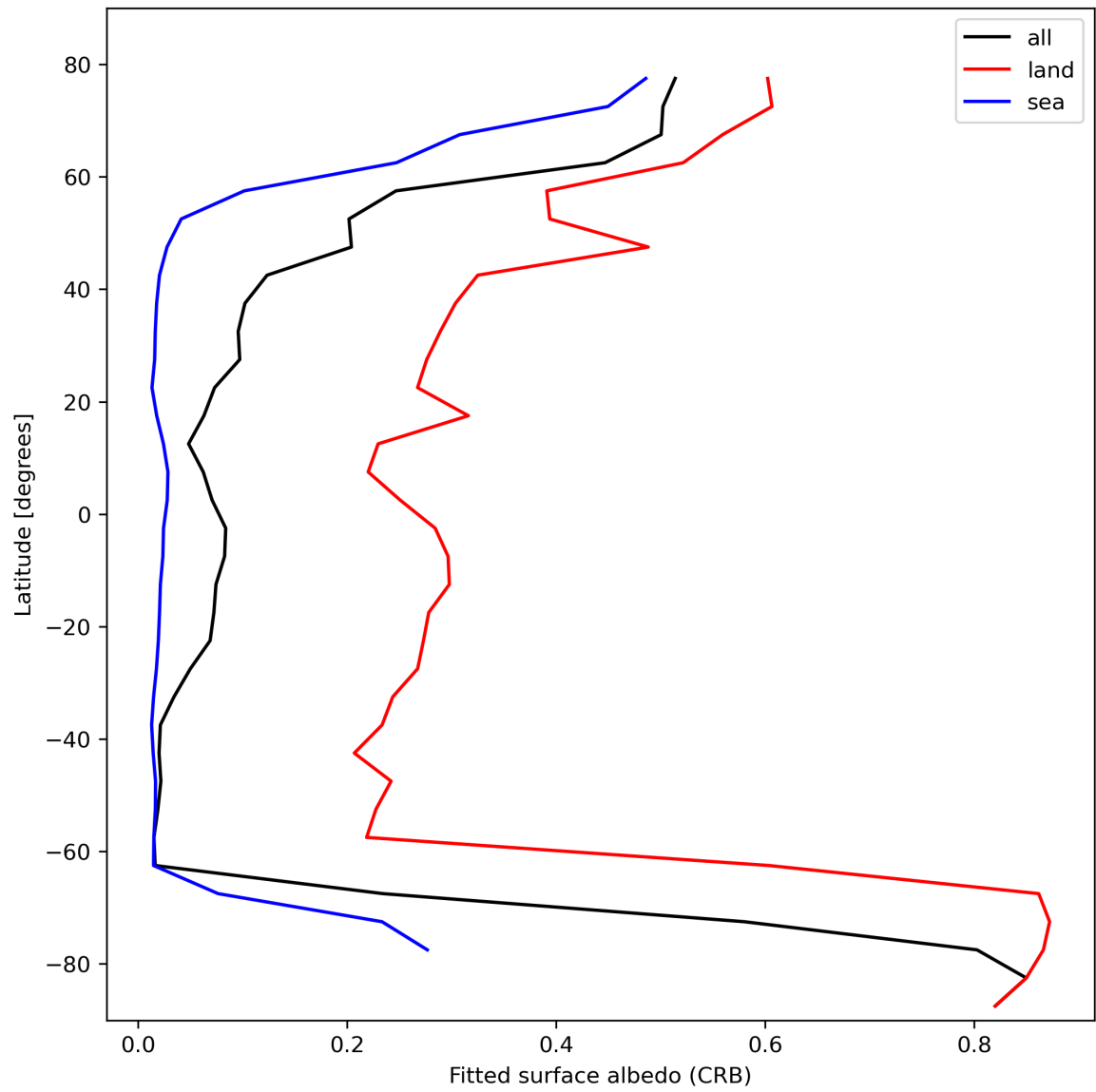
Figure 30: Zonal average of “Fitted surface albedo (CRB)” for 2024-02-14 to 2024-02-16.
