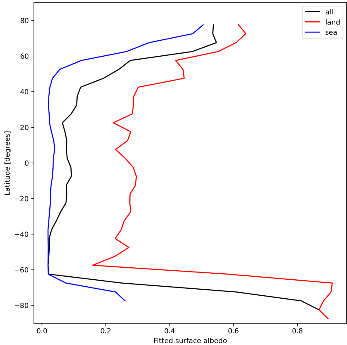
Figure 29: Zonal average of “Fitted surface albedo” for 2024-02-17 to 2024-02-18.
