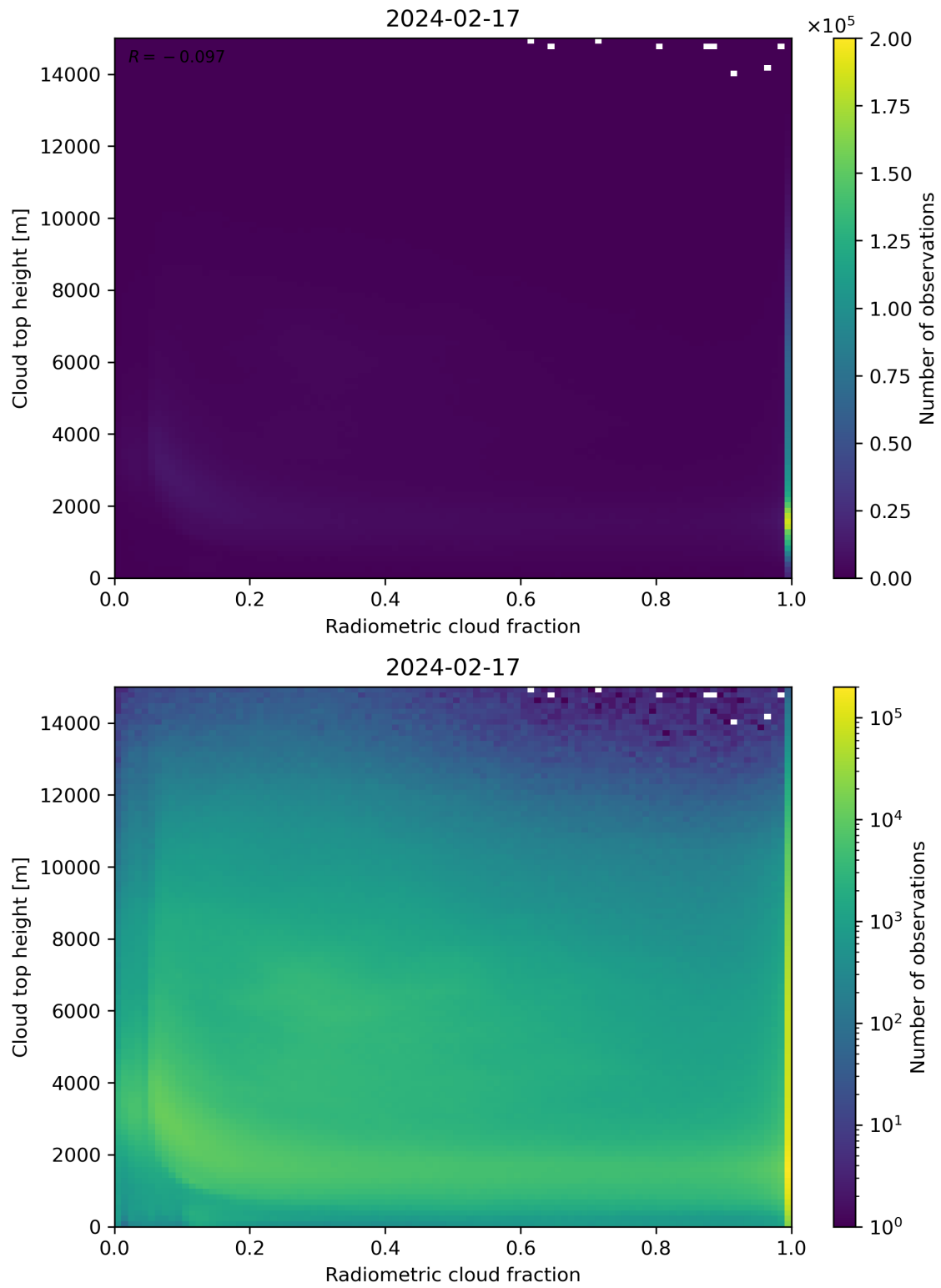
Figure 76: Scatter density plot of “Radiometric cloud fraction” against “Cloud top height” for 2024-02-17 to 2024-02-18.
