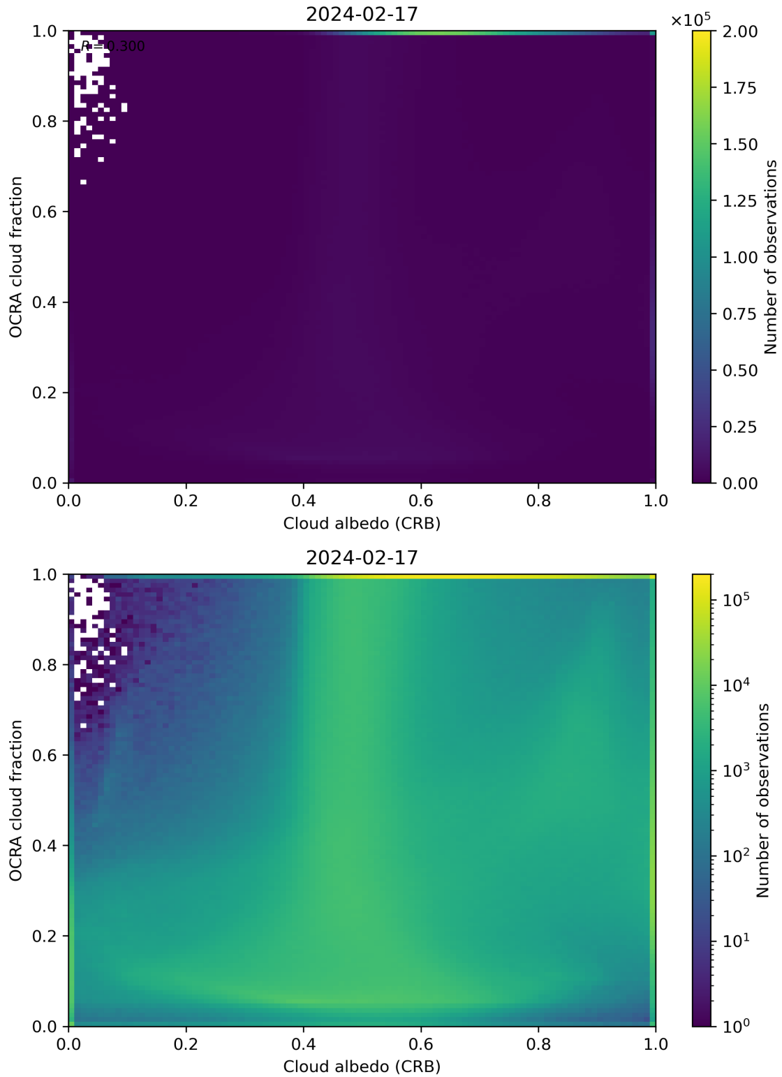
Figure 70: Scatter density plot of “Cloud albedo (CRB)” against “OCRA cloud fraction” for 2024-02-17 to 2024-02-18.
