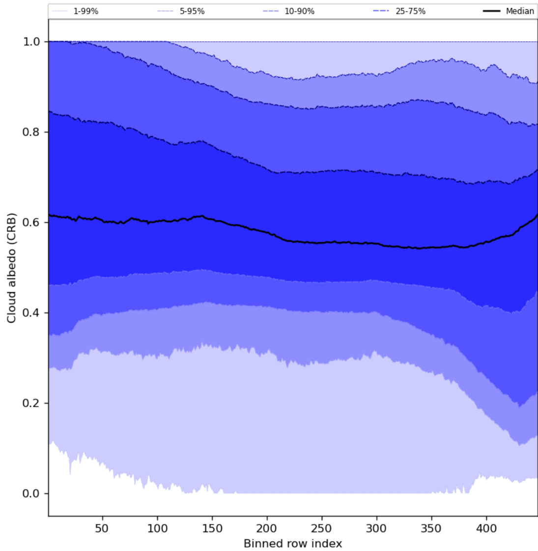
Figure 60: Along track statistics of “Cloud albedo (CRB)” for 2024-02-17 to 2024-02-18
