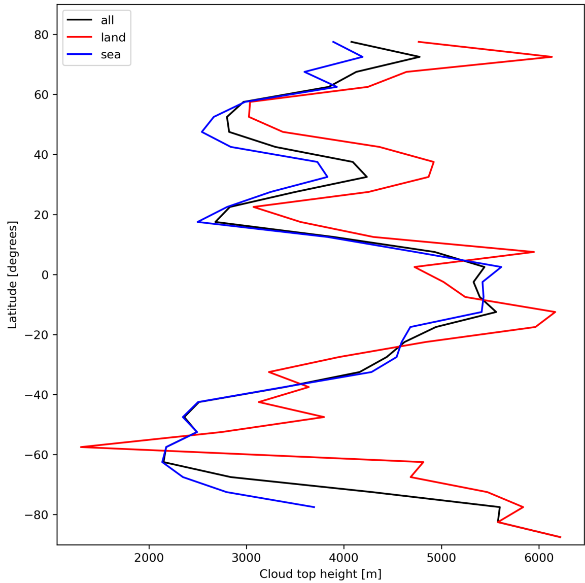
Figure 24: Zonal average of “Cloud top height” for 2024-02-17 to 2024-02-18.
