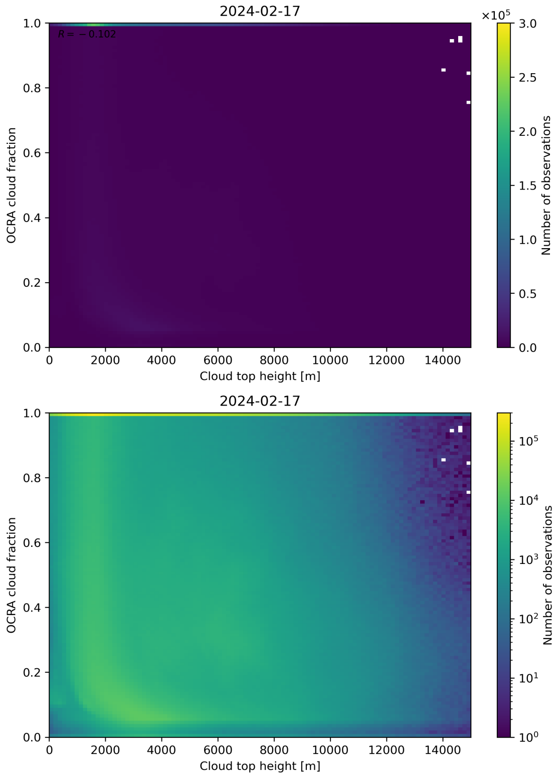
Figure 87: Scatter density plot of “Cloud top height” against “OCRA cloud fraction” for 2024-02-17 to 2024-02-18.
