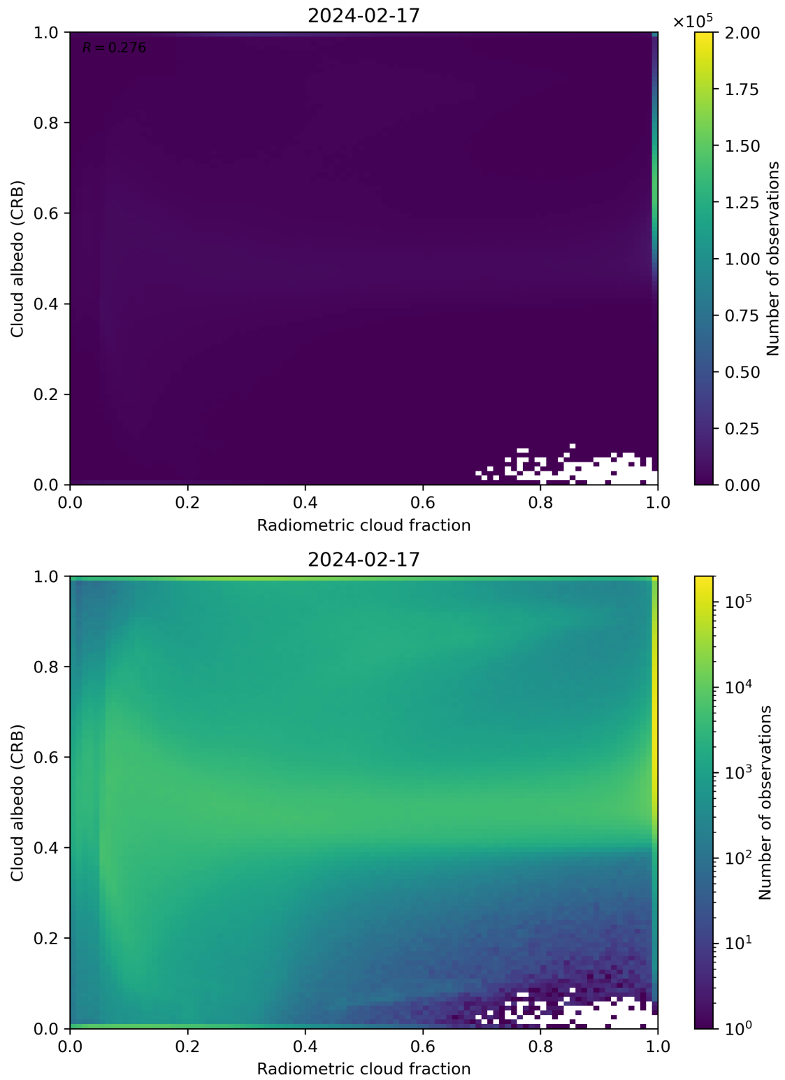
Figure 71: Scatter density plot of “Radiometric cloud fraction” against “Cloud albedo (CRB)” for 2024-02-17 to 2024-02-18.
