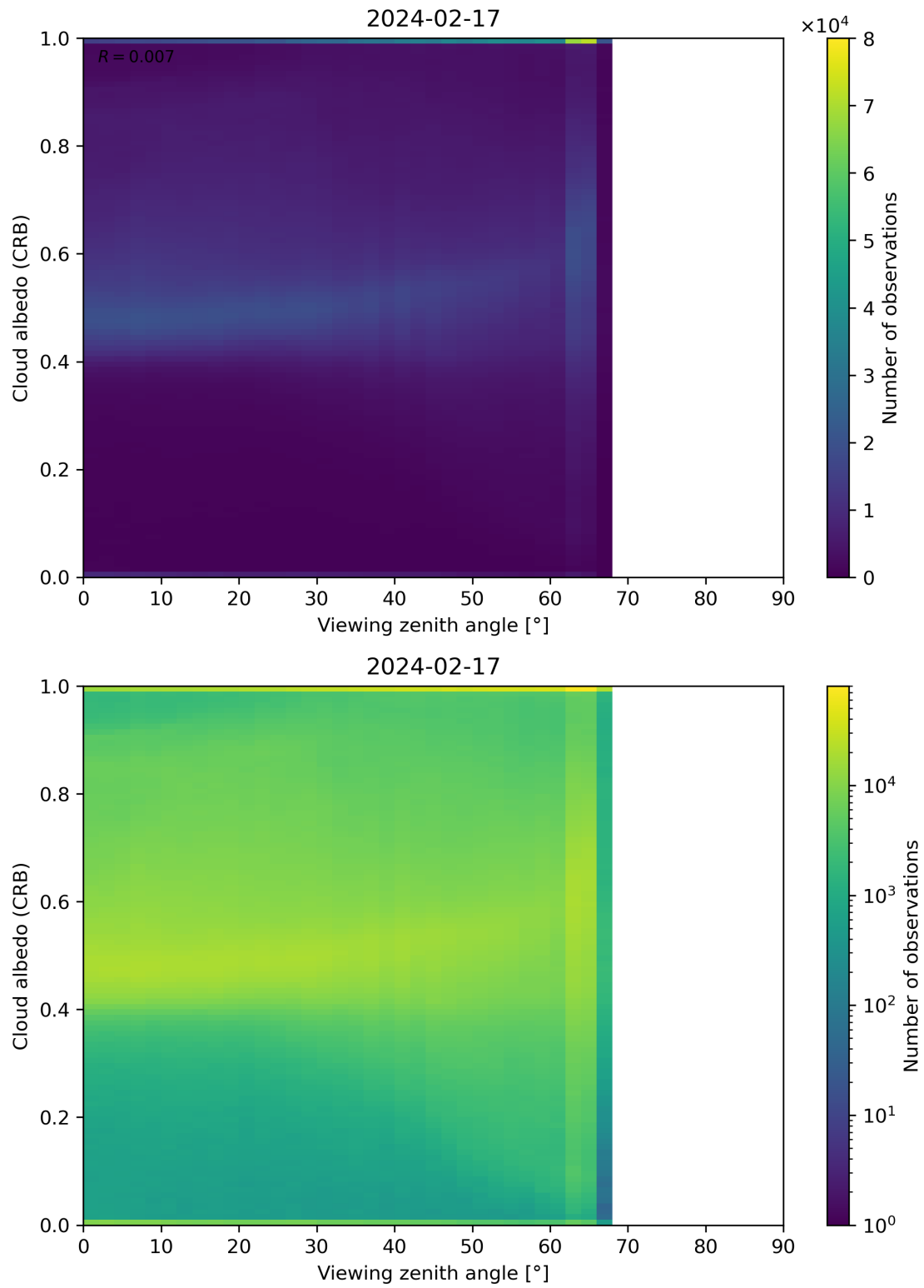
Figure 106: Scatter density plot of “Viewing zenith angle” against “Cloud albedo (CRB)” for 2024-02-17 to 2024-02-18.
