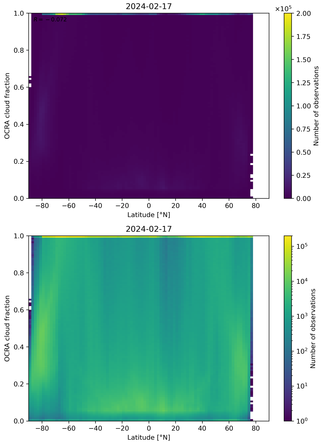
Figure 93: Scatter density plot of “Latitude” against “OCRA cloud fraction” for 2024-02-17 to 2024-02-18.
