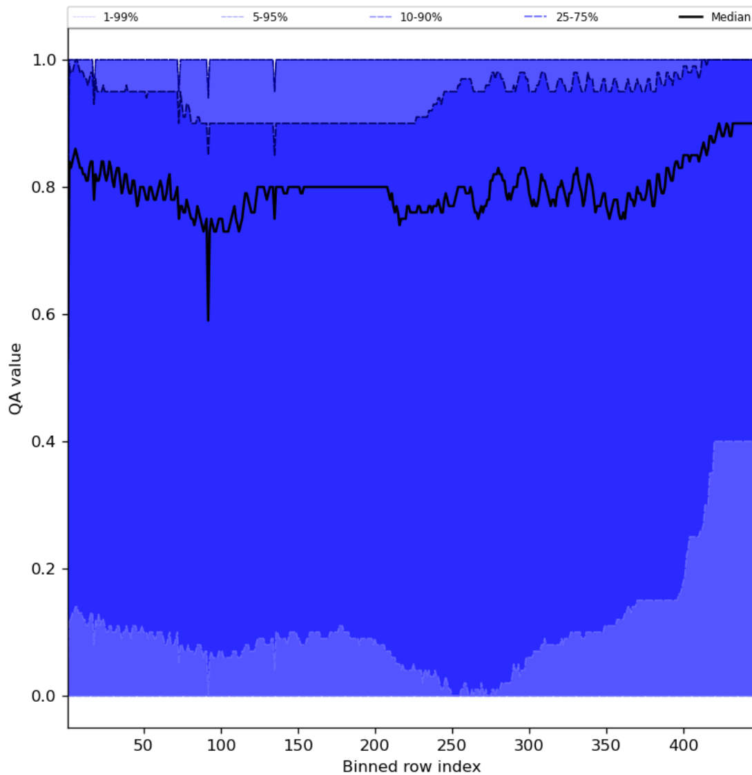
Figure 54: Along track statistics of “QA value” for 2024-02-17 to 2024-02-18
