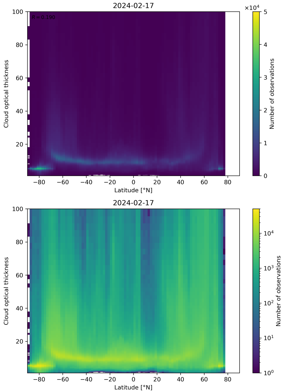
Figure 96: Scatter density plot of “Latitude” against “Cloud optical thickness” for 2024-02-17 to 2024-02-18.
