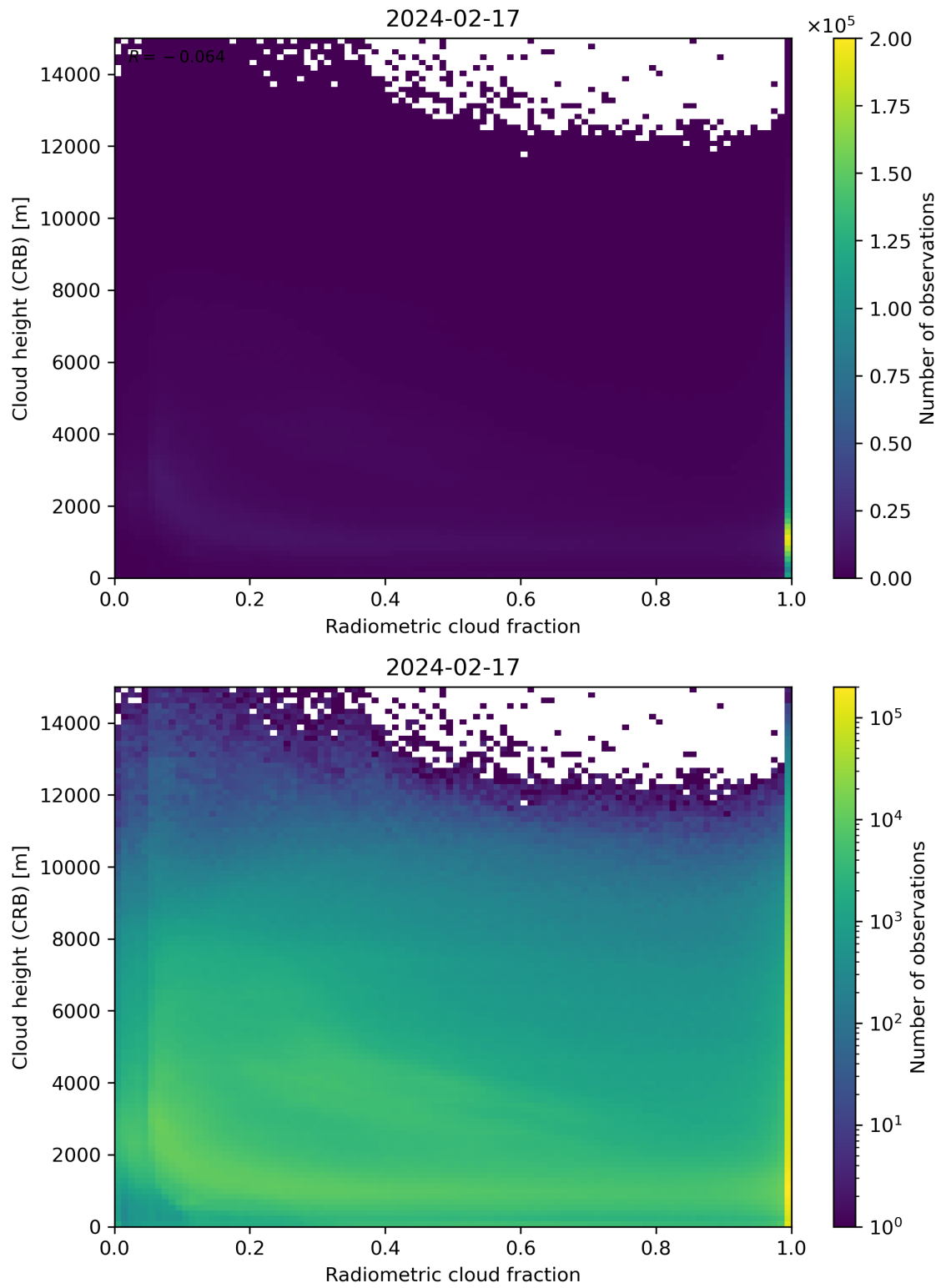
Figure 74: Scatter density plot of “Radiometric cloud fraction” against “Cloud height (CRB)” for 2024-02-17 to 2024-02-18.
