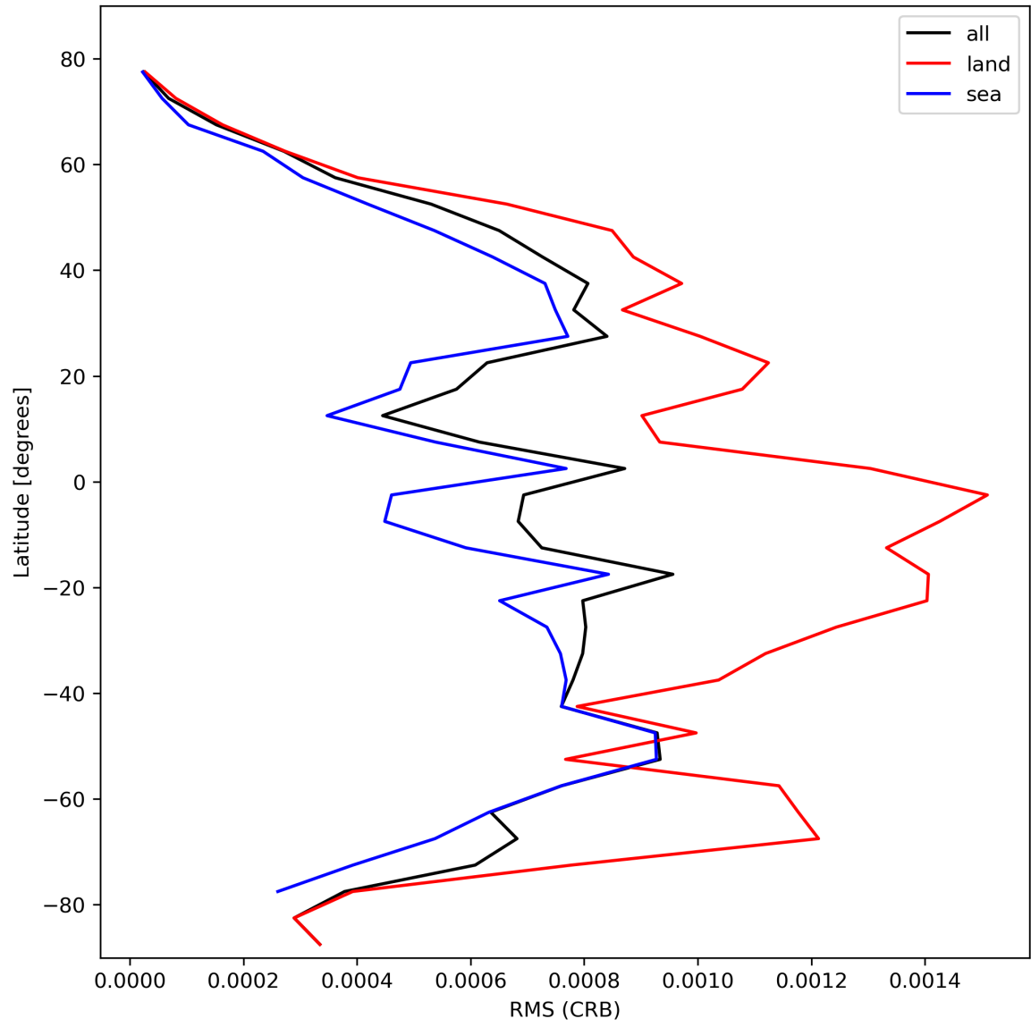
Figure 32: Zonal average of “RMS (CRB)” for 2024-02-17 to 2024-02-18.
