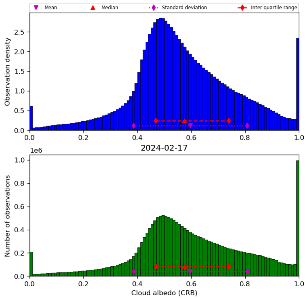
Figure 44: Histogram of “Cloud albedo (CRB)” for 2024-02-17 to 2024-02-18
