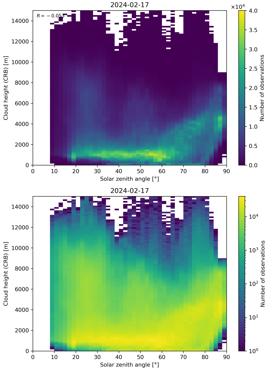
Figure 102: Scatter density plot of “Solar zenith angle” against “Cloud height (CRB)” for 2024-02-17 to 2024-02-18.
