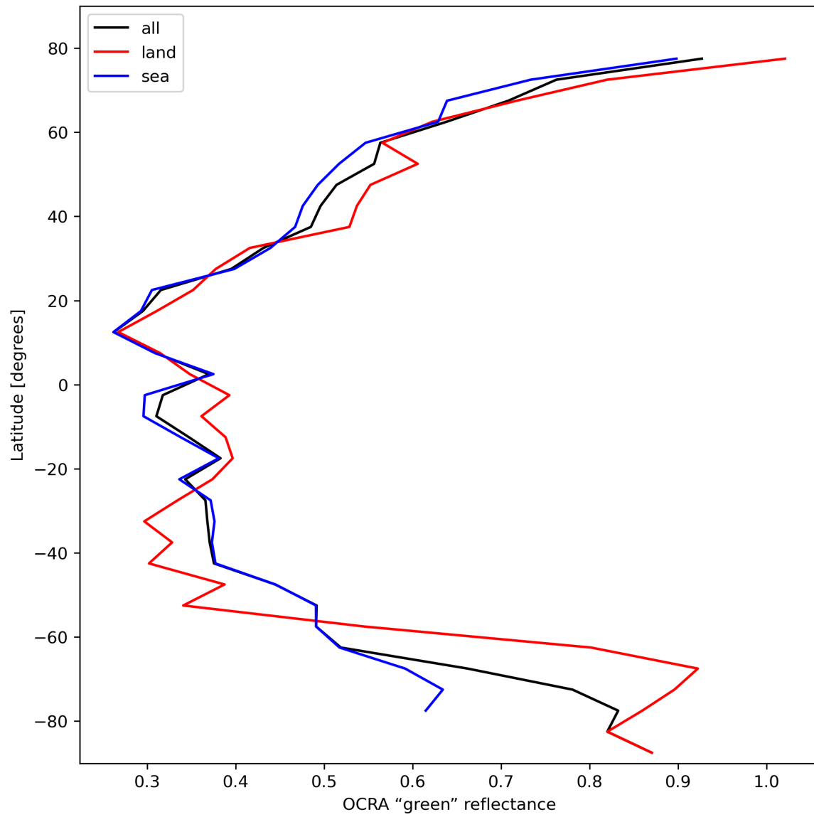
Figure 36: Zonal average of “OCRA “green” reflectance” for 2024-02-17 to 2024-02-18.
