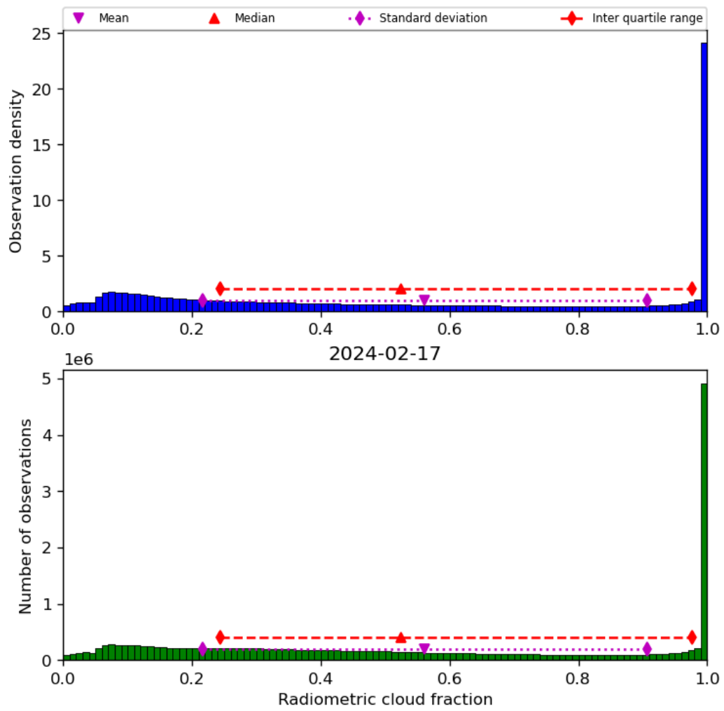
Figure 39: Histogram of “Radiometric cloud fraction” for 2024-02-17 to 2024-02-18
