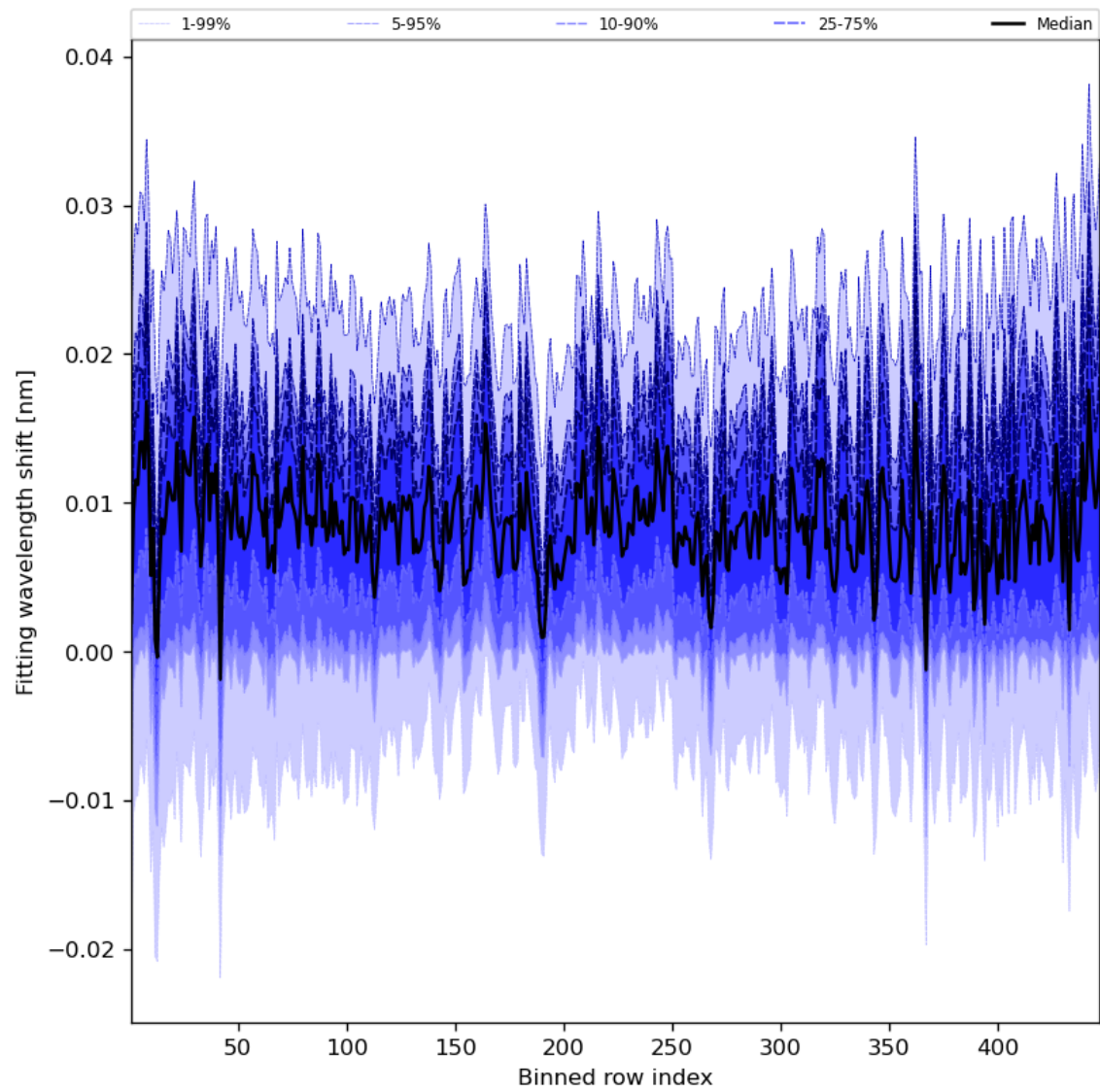
Figure 65: Along track statistics of “Fitting wavelength shift” for 2024-02-17 to 2024-02-18
