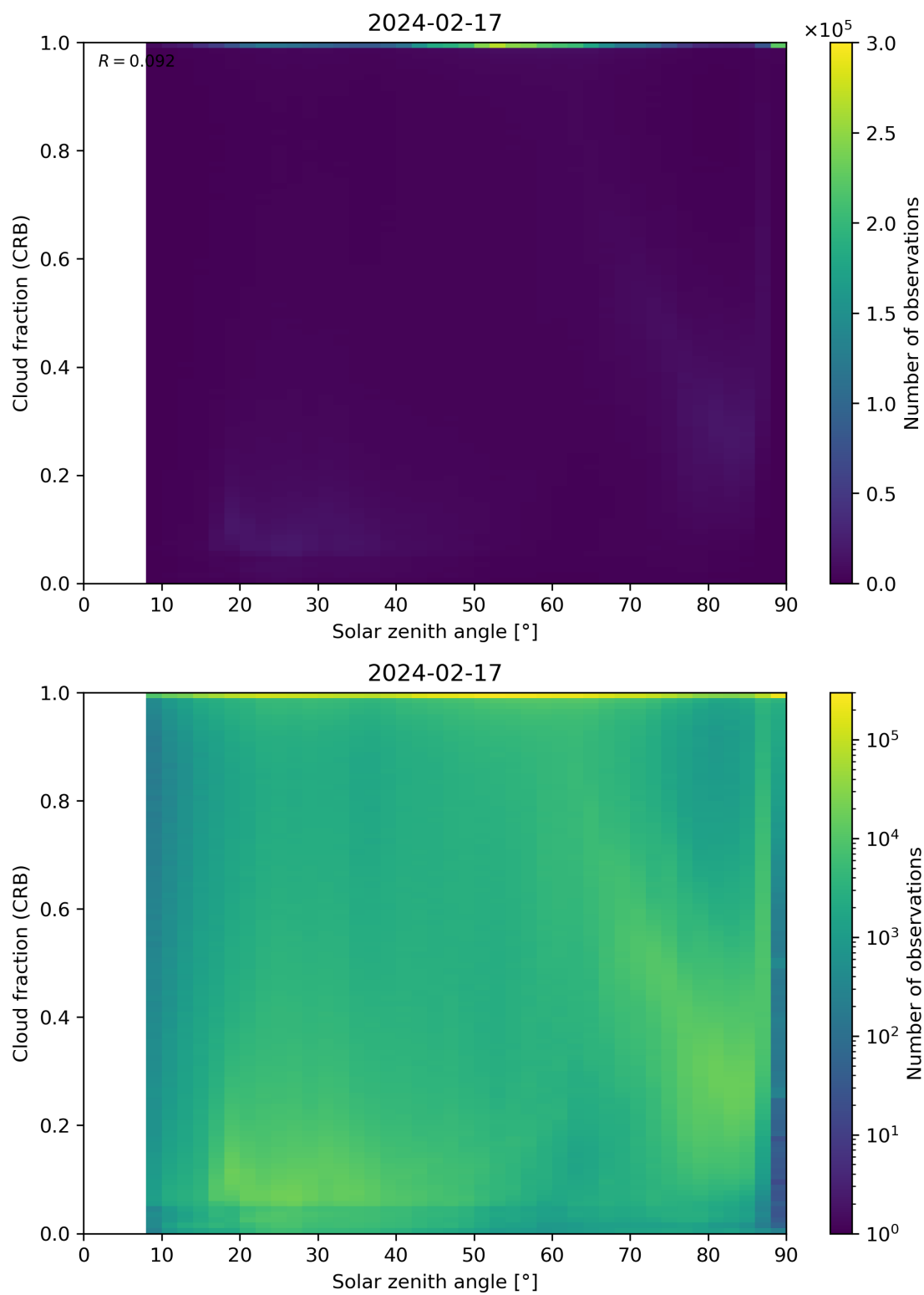
Figure 101: Scatter density plot of “Solar zenith angle” against “Cloud fraction (CRB)” for 2024-02-17 to 2024-02-18.
