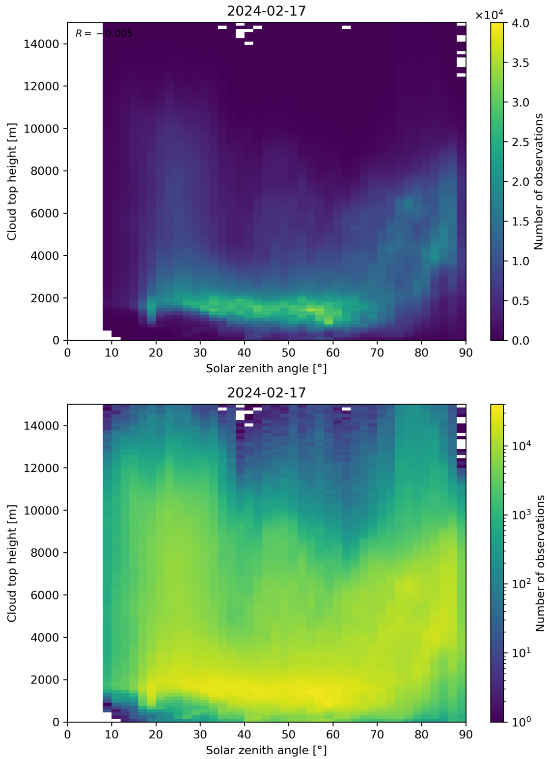
Figure 104: Scatter density plot of “Solar zenith angle” against “Cloud top height” for 2024-02-17 to 2024-02-18.
