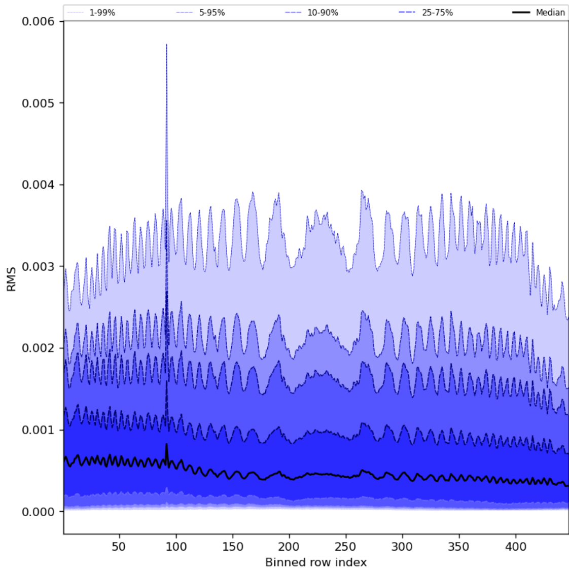
Figure 63: Along track statistics of “RMS” for 2024-02-17 to 2024-02-18
