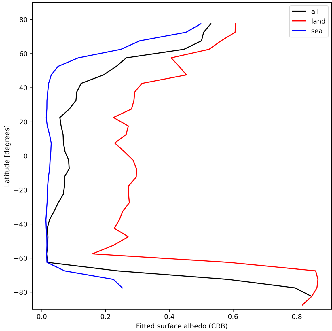
Figure 30: Zonal average of “Fitted surface albedo (CRB)” for 2024-02-17 to 2024-02-18.
