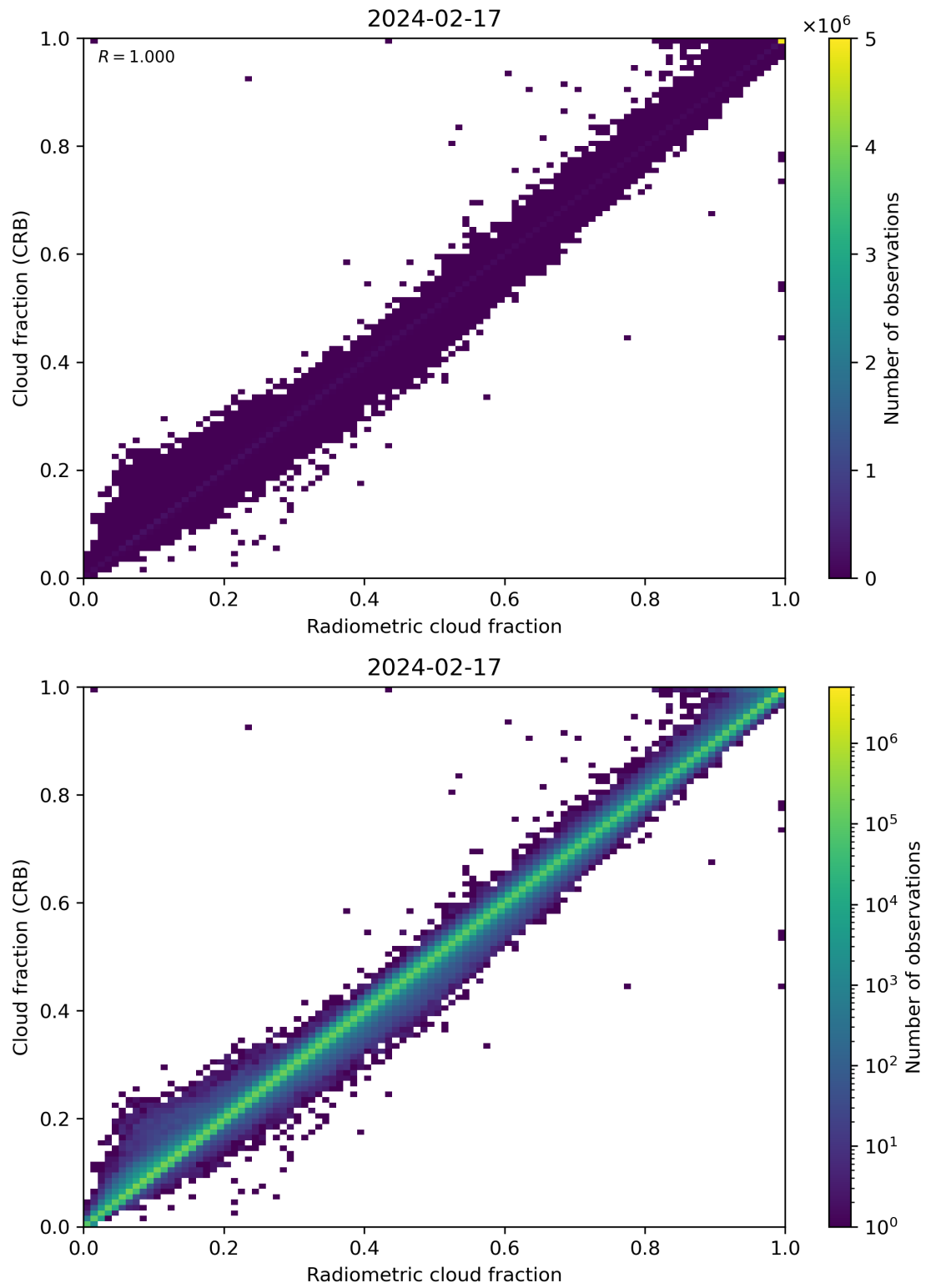
Figure 73: Scatter density plot of “Radiometric cloud fraction” against “Cloud fraction (CRB)” for 2024-02-17 to 2024-02-18.
