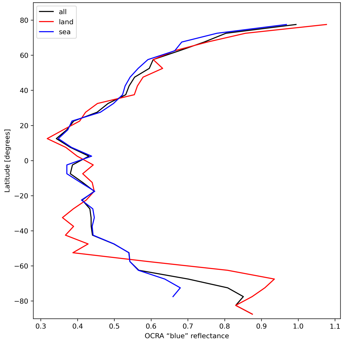
Figure 35: Zonal average of “OCRA “blue” reflectance” for 2024-02-17 to 2024-02-18.
