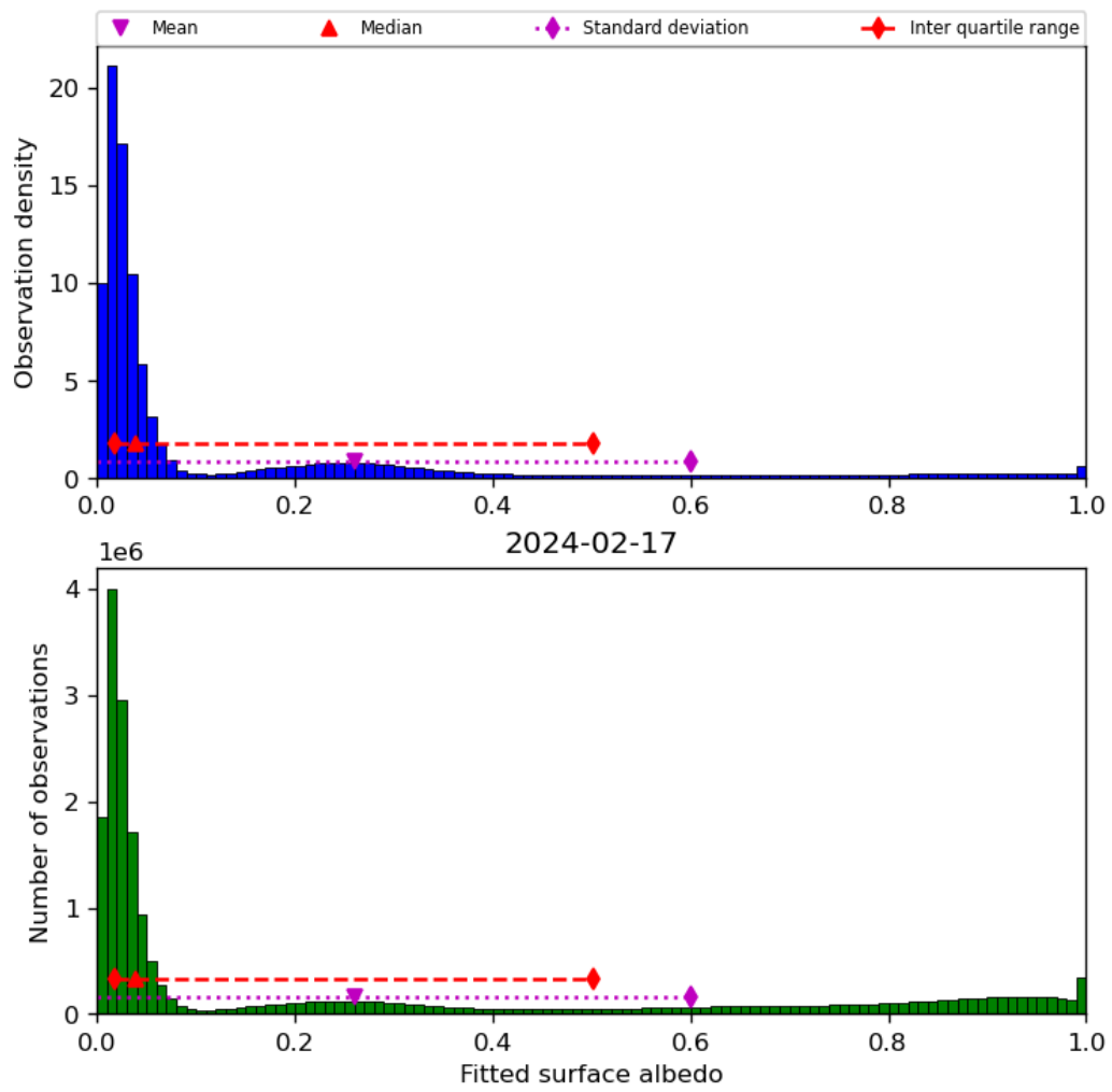
Figure 45: Histogram of “Fitted surface albedo” for 2024-02-17 to 2024-02-18
