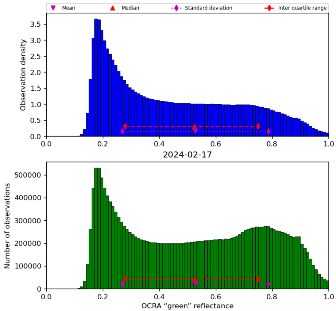
Figure 52: Histogram of “OCRA “green” reflectance” for 2024-02-17 to 2024-02-18
