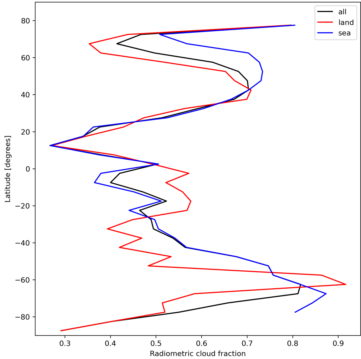
Figure 23: Zonal average of “Radiometric cloud fraction” for 2024-02-17 to 2024-02-18.
