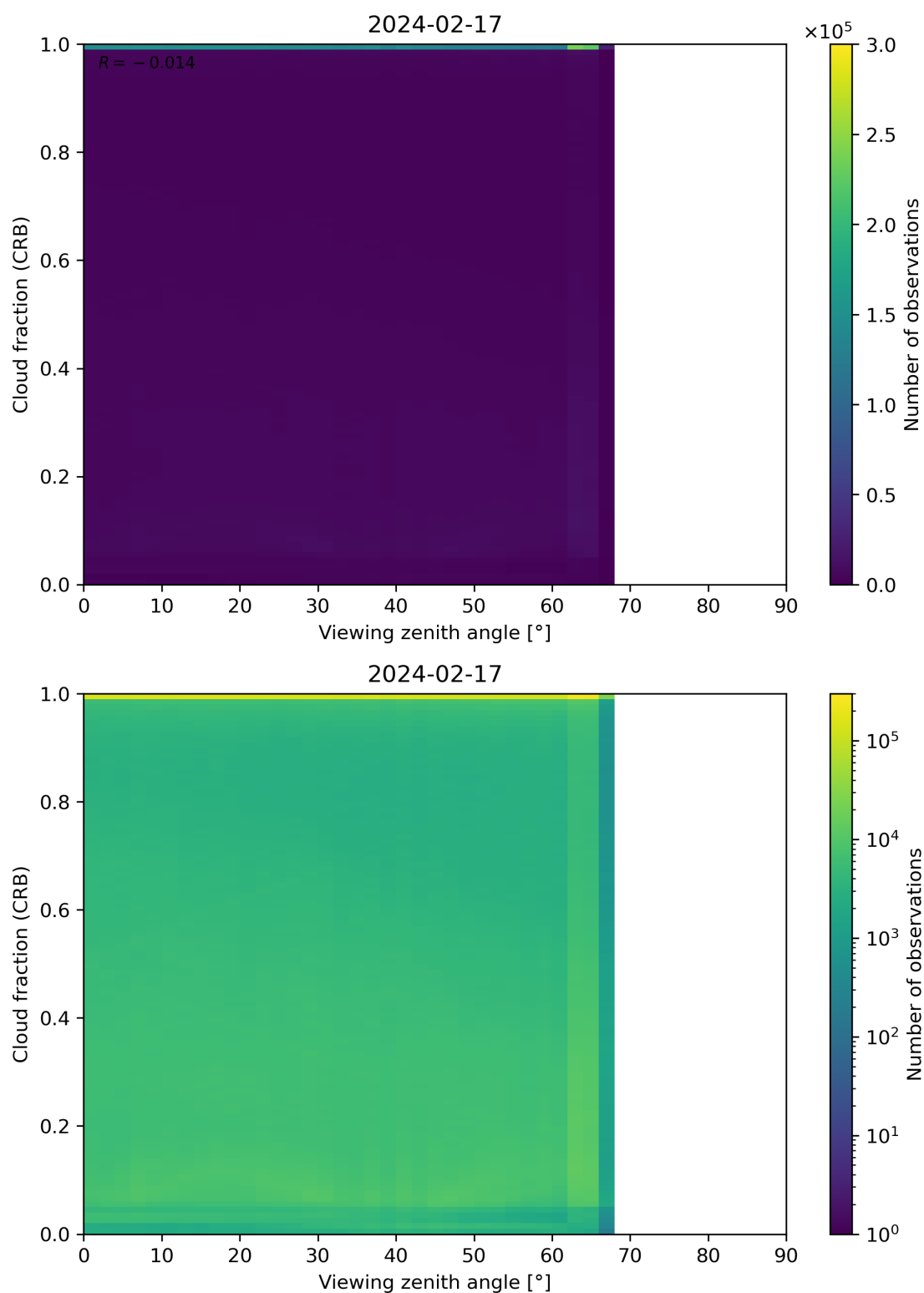
Figure 109: Scatter density plot of “Viewing zenith angle” against “Cloud fraction (CRB)” for 2024-02-17 to 2024-02-18.
