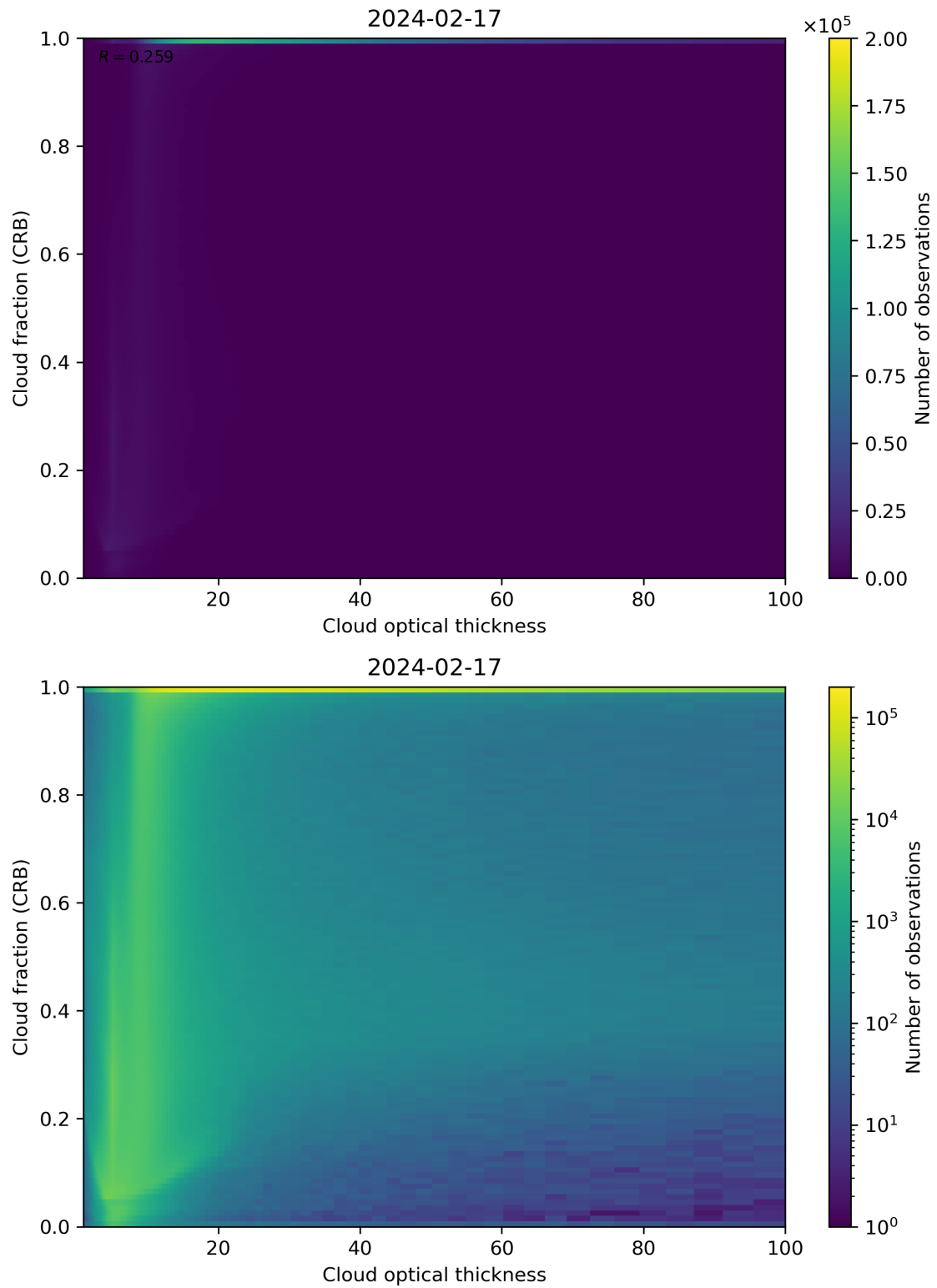
Figure 84: Scatter density plot of “Cloud optical thickness” against “Cloud fraction (CRB)” for 2024-02-17 to 2024-02-18.
