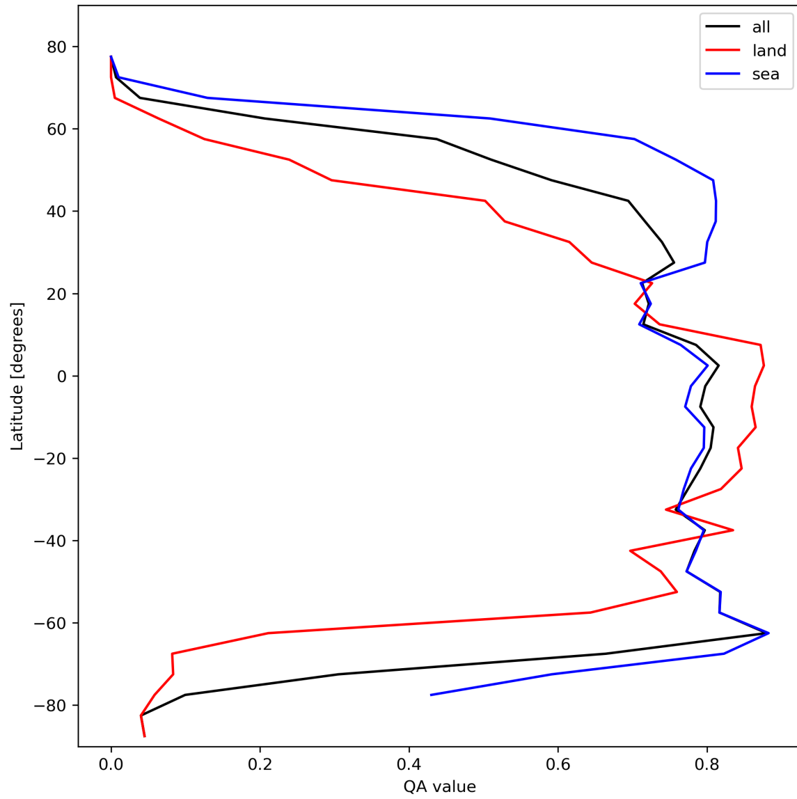
Figure 22: Zonal average of “QA value” for 2024-02-17 to 2024-02-18.
