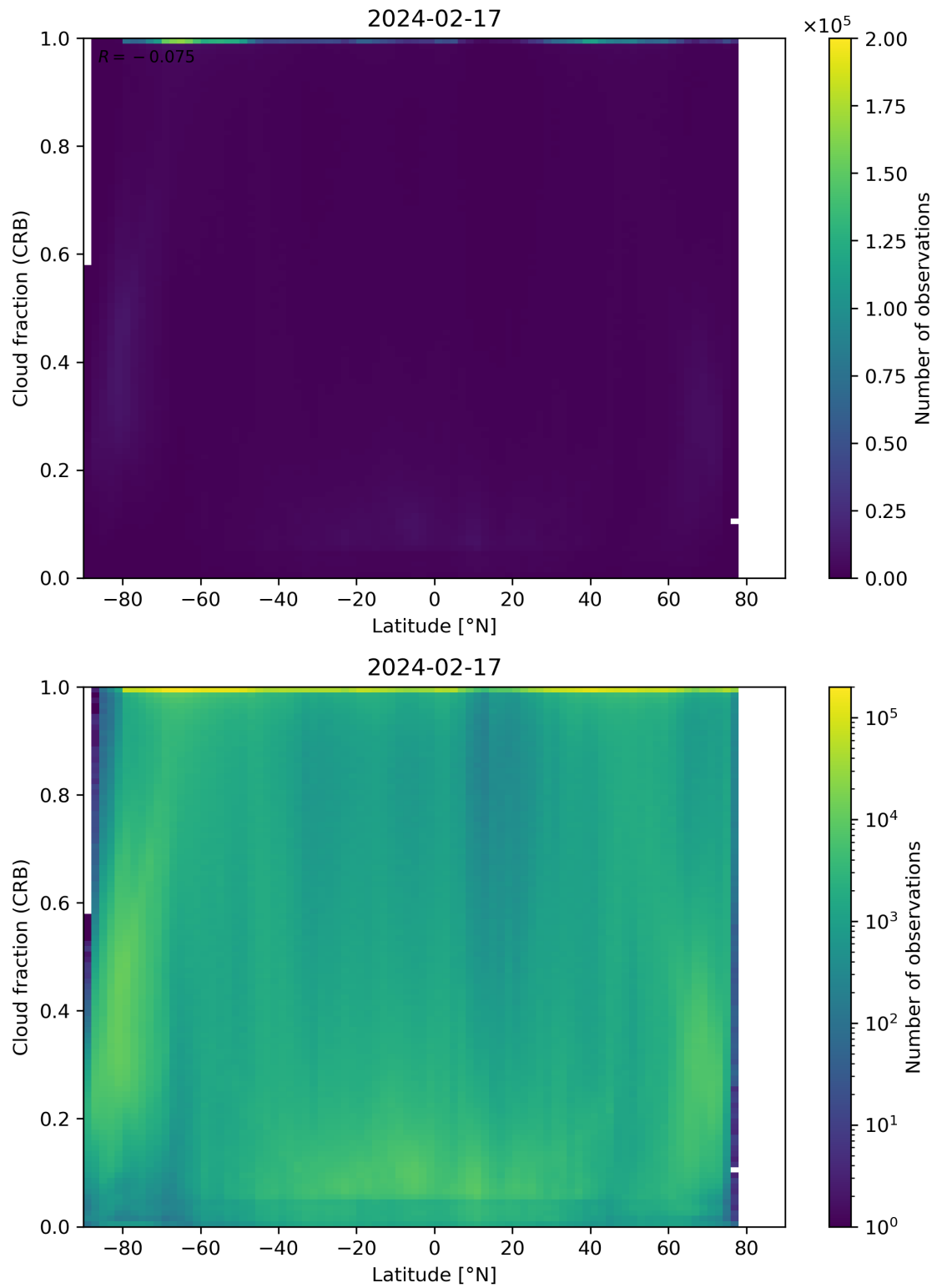
Figure 94: Scatter density plot of “Latitude” against “Cloud fraction (CRB)” for 2024-02-17 to 2024-02-18.
