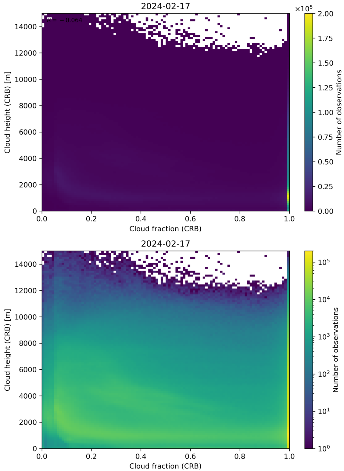
Figure 79: Scatter density plot of “Cloud fraction (CRB)” against “Cloud height (CRB)” for 2024-02-17 to 2024-02-18.
