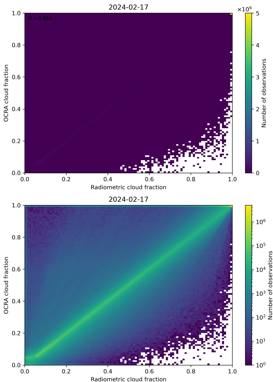
Figure 72: Scatter density plot of “Radiometric cloud fraction” against “OCRA cloud fraction” for 2024-02-17 to 2024-02-18.
