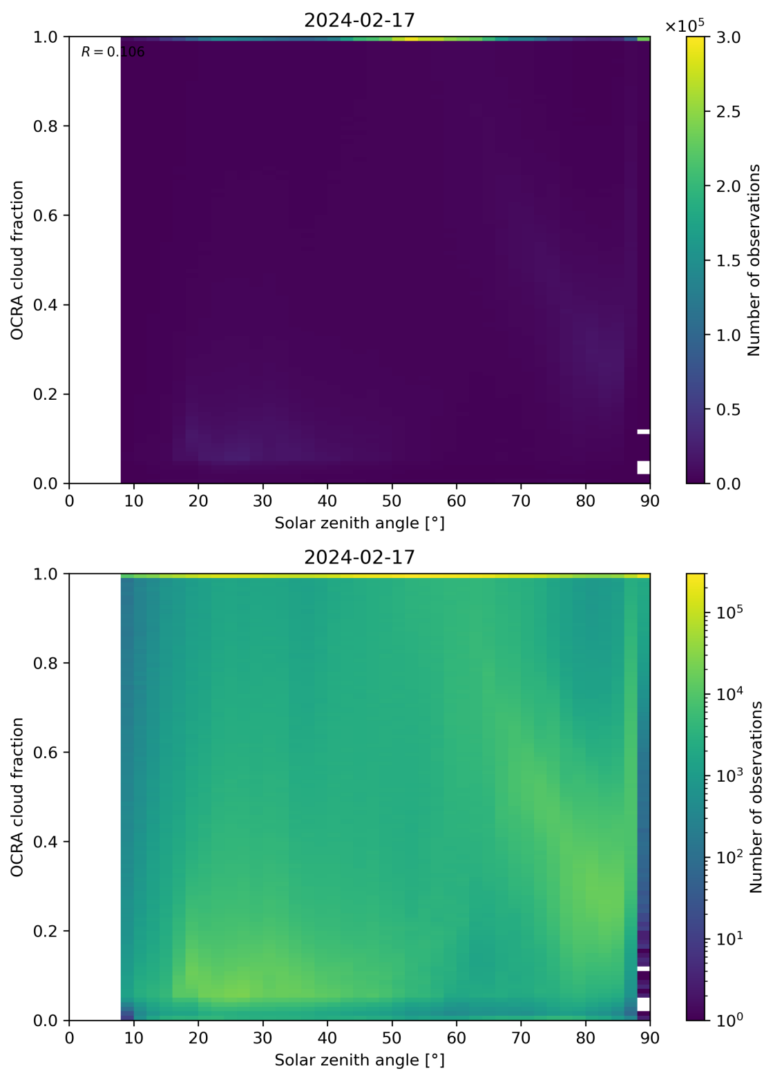
Figure 100: Scatter density plot of “Solar zenith angle” against “OCRA cloud fraction” for 2024-02-17 to 2024-02-18.
