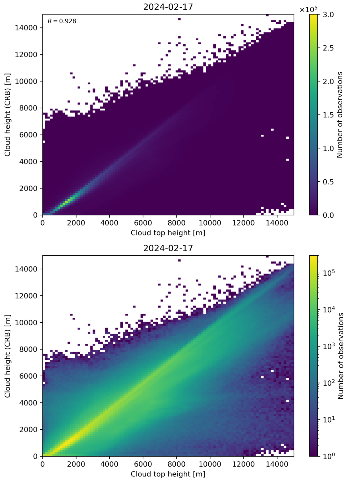
Figure 89: Scatter density plot of “Cloud top height” against “Cloud height (CRB)” for 2024-02-17 to 2024-02-18.
