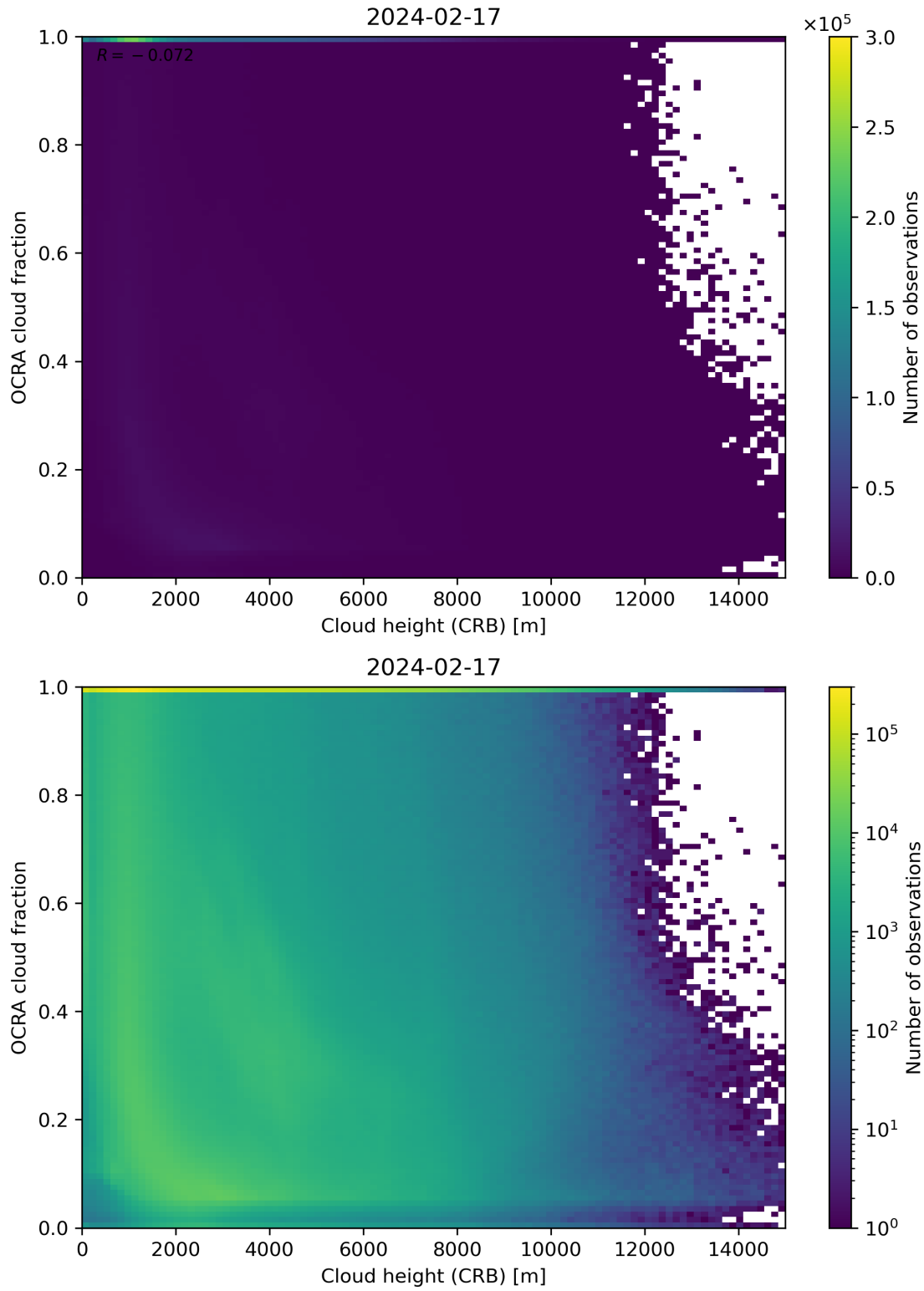
Figure 81: Scatter density plot of “Cloud height (CRB)” against “OCRA cloud fraction” for 2024-02-17 to 2024-02-18.
