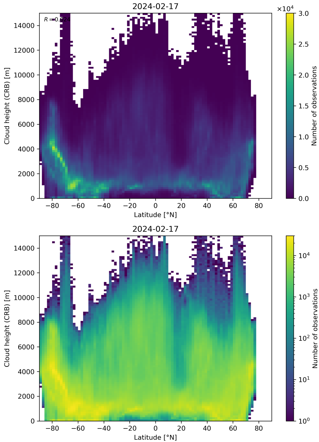
Figure 95: Scatter density plot of “Latitude” against “Cloud height (CRB)” for 2024-02-17 to 2024-02-18.
