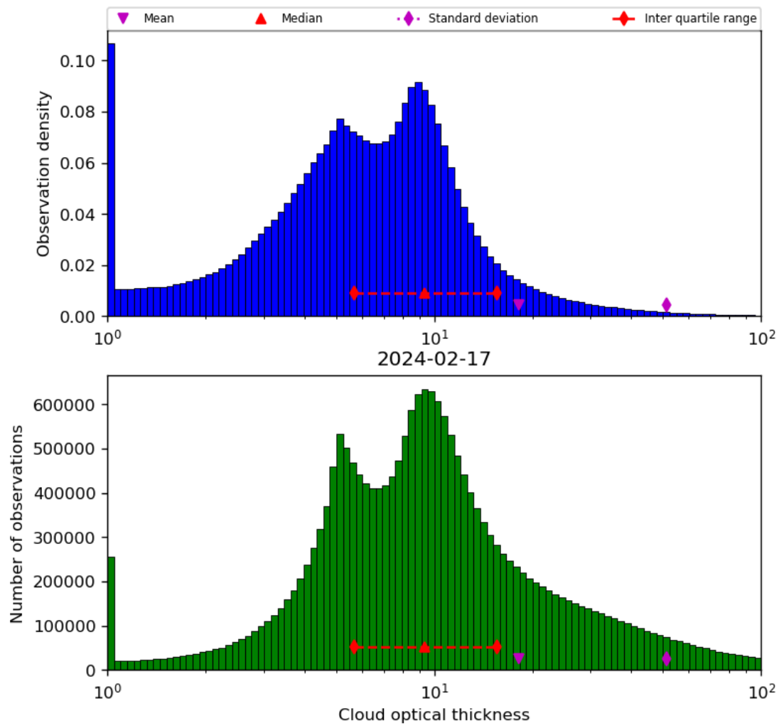
Figure 41: Histogram of “Cloud optical thickness” for 2024-02-17 to 2024-02-18
