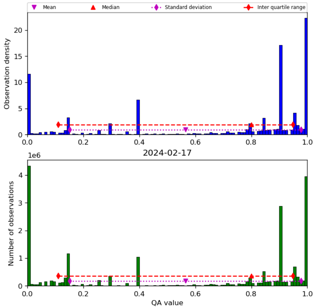
Figure 38: Histogram of “QA value” for 2024-02-17 to 2024-02-18
