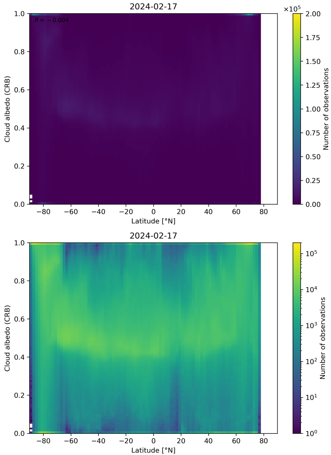
Figure 91: Scatter density plot of “Latitude” against “Cloud albedo (CRB)” for 2024-02-17 to 2024-02-18.
