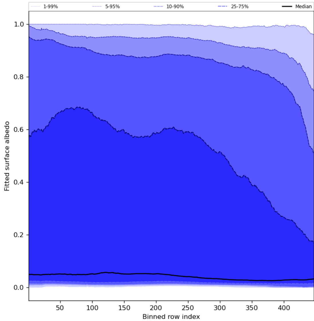
Figure 61: Along track statistics of “Fitted surface albedo” for 2024-02-17 to 2024-02-18
