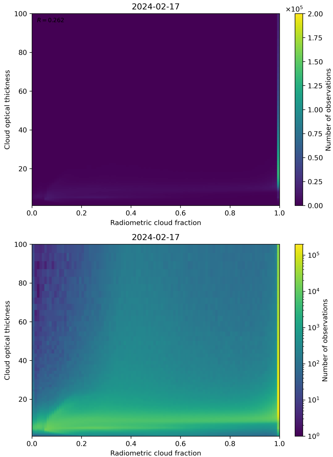
Figure 75: Scatter density plot of “Radiometric cloud fraction” against “Cloud optical thickness” for 2024-02-17 to 2024-02-18.
