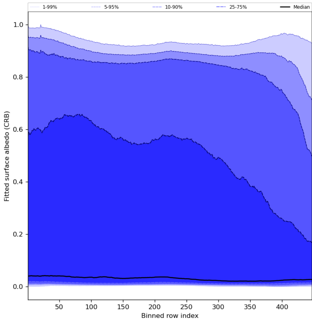
Figure 62: Along track statistics of “Fitted surface albedo (CRB)” for 2024-02-17 to 2024-02-18
