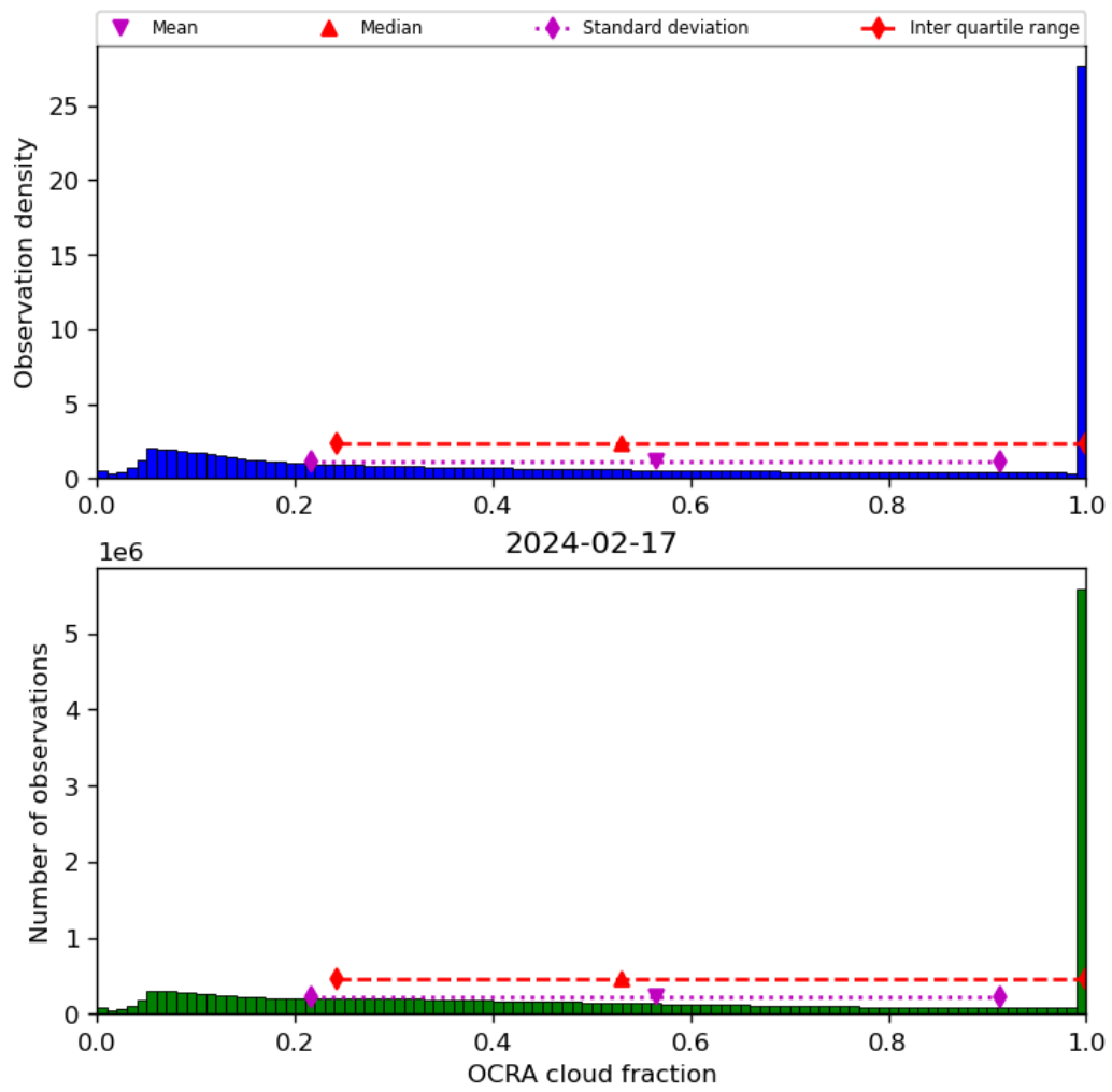
Figure 50: Histogram of “OCRA cloud fraction” for 2024-02-17 to 2024-02-18
