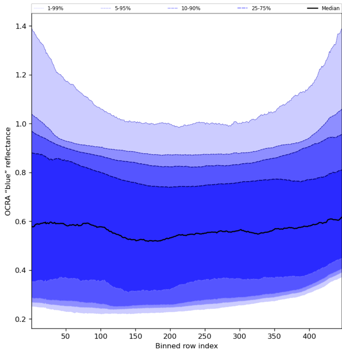
Figure 67: Along track statistics of “OCRA “blue” reflectance” for 2024-02-17 to 2024-02-18
