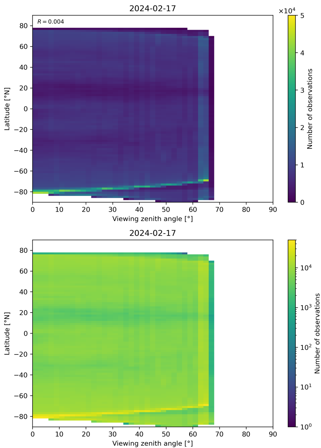
Figure 113: Scatter density plot of “Viewing zenith angle” against “Latitude” for 2024-02-17 to 2024-02-18.
