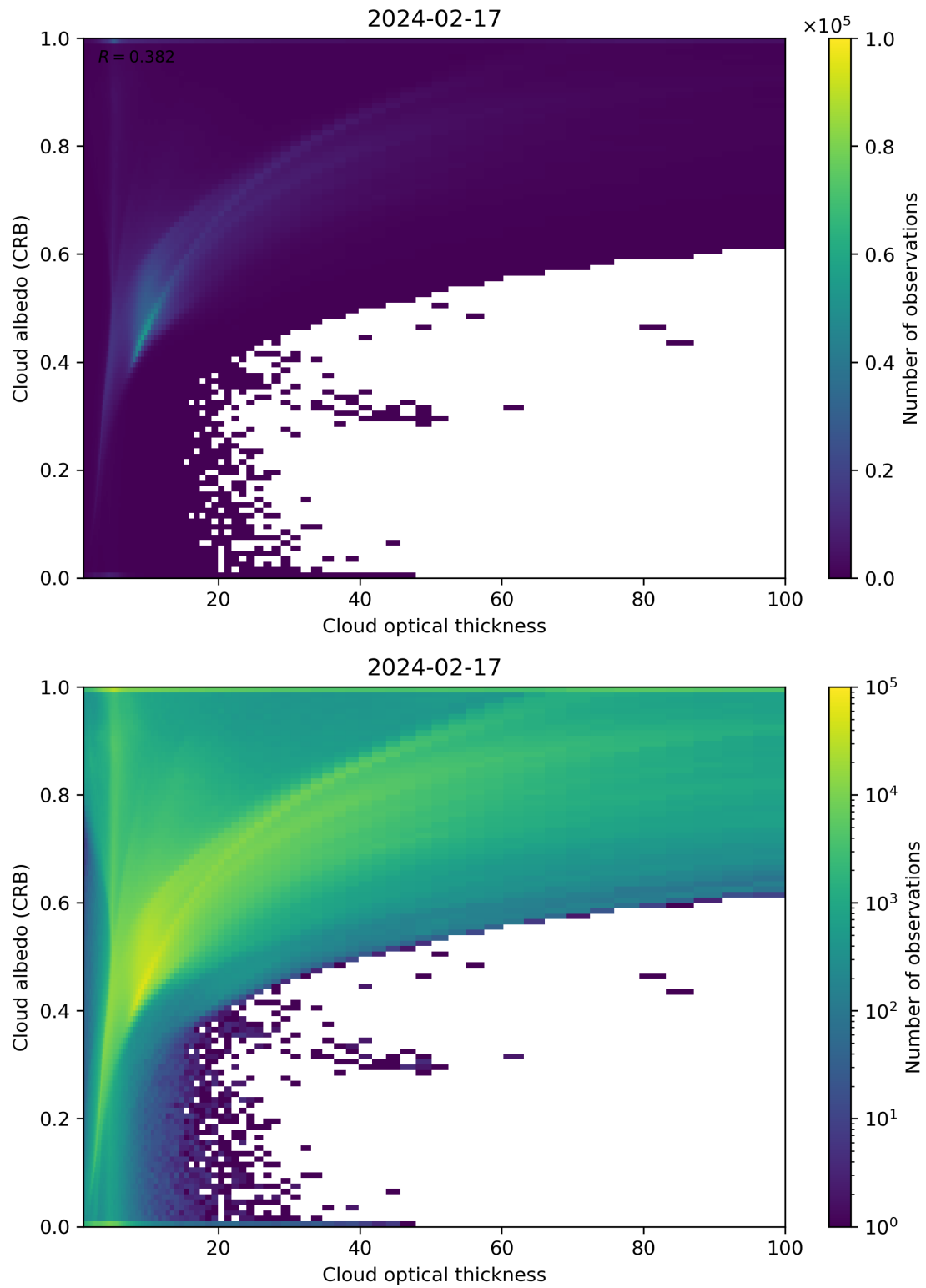
Figure 82: Scatter density plot of “Cloud optical thickness” against “Cloud albedo (CRB)” for 2024-02-17 to 2024-02-18.
