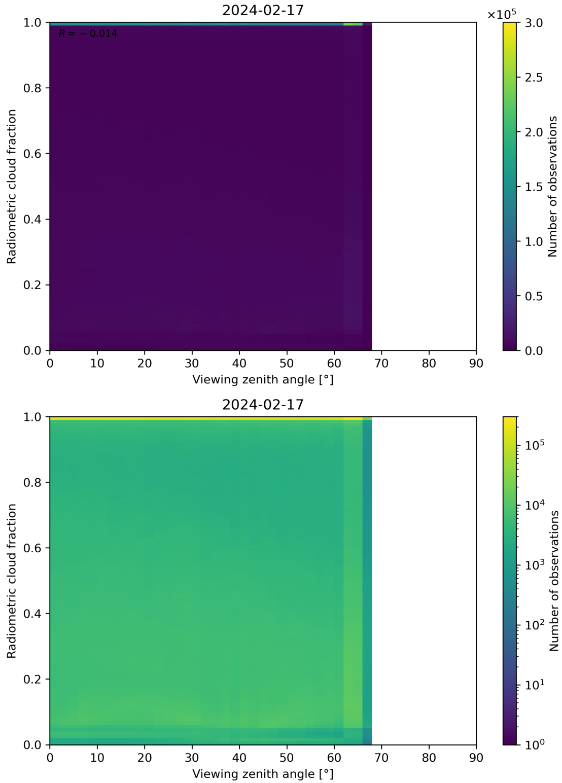
Figure 107: Scatter density plot of “Viewing zenith angle” against “Radiometric cloud fraction” for 2024-02-17 to 2024-02-18.
