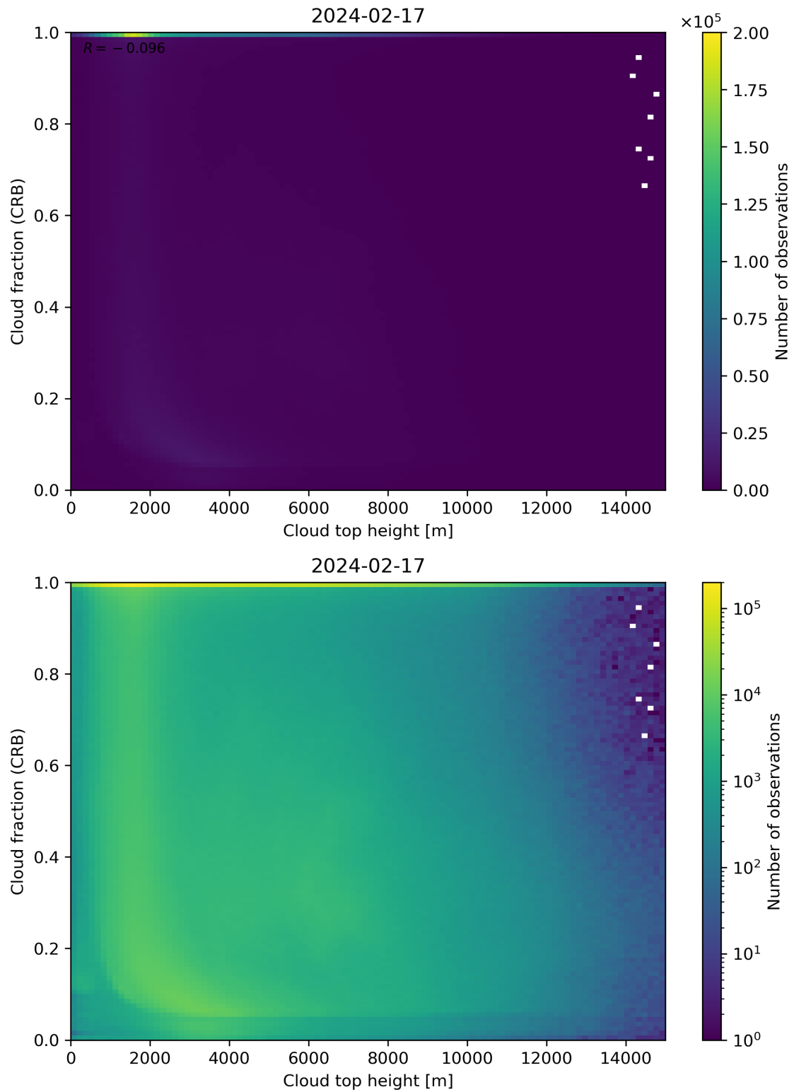
Figure 88: Scatter density plot of “Cloud top height” against “Cloud fraction (CRB)” for 2024-02-17 to 2024-02-18.
