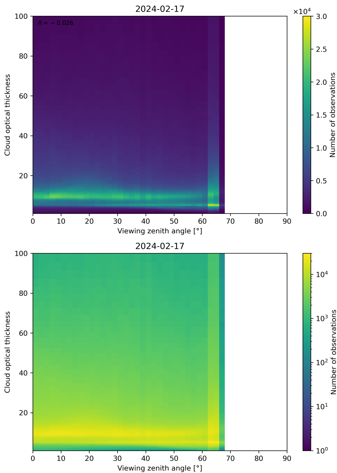
Figure 111: Scatter density plot of “Viewing zenith angle” against “Cloud optical thickness” for 2024-02-17 to 2024-02-18.
