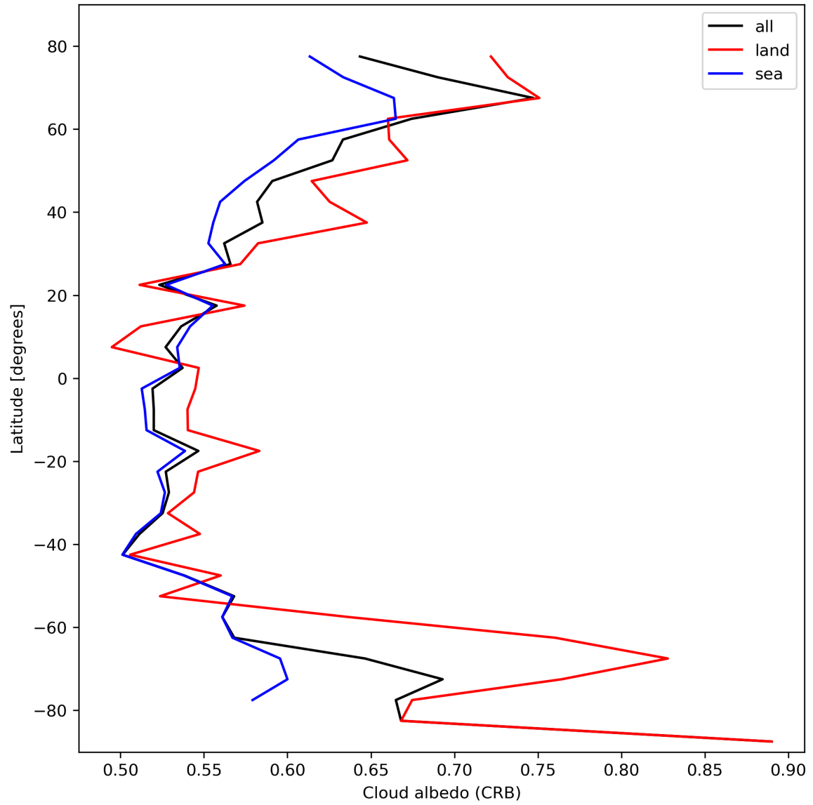
Figure 28: Zonal average of “Cloud albedo (CRB)” for 2024-02-17 to 2024-02-18.
