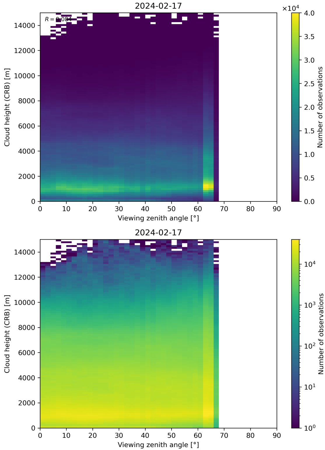
Figure 110: Scatter density plot of “Viewing zenith angle” against “Cloud height (CRB)” for 2024-02-17 to 2024-02-18.
