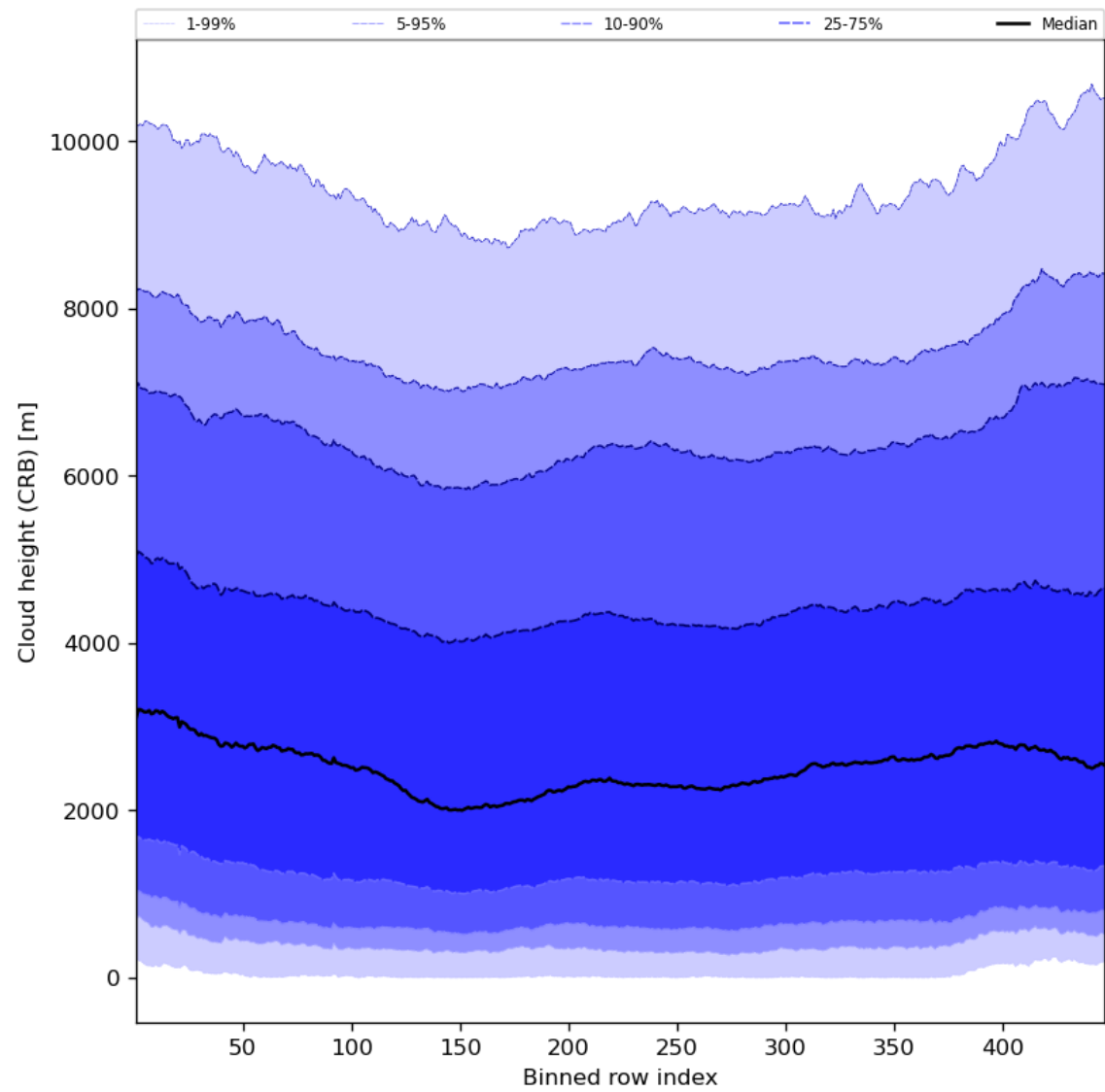
Figure 59: Along track statistics of “Cloud height (CRB)” for 2024-02-17 to 2024-02-18
