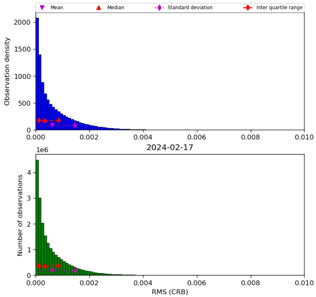
Figure 48: Histogram of “RMS (CRB)” for 2024-02-17 to 2024-02-18
