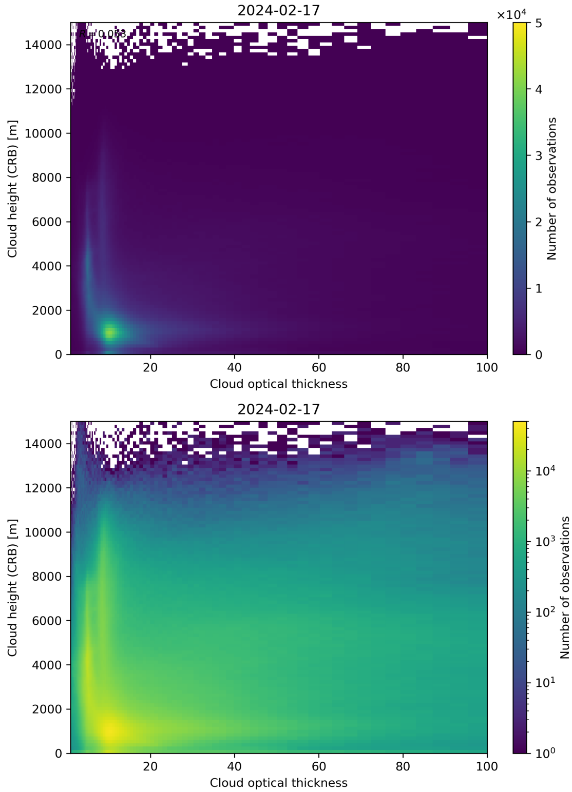
Figure 85: Scatter density plot of “Cloud optical thickness” against “Cloud height (CRB)” for 2024-02-17 to 2024-02-18.
