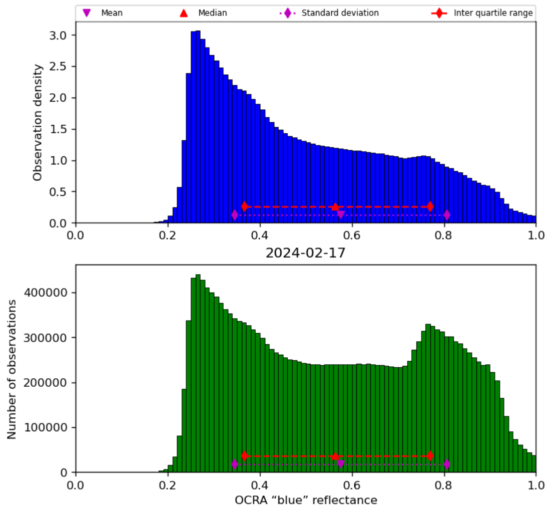
Figure 51: Histogram of “OCRA “blue” reflectance” for 2024-02-17 to 2024-02-18
