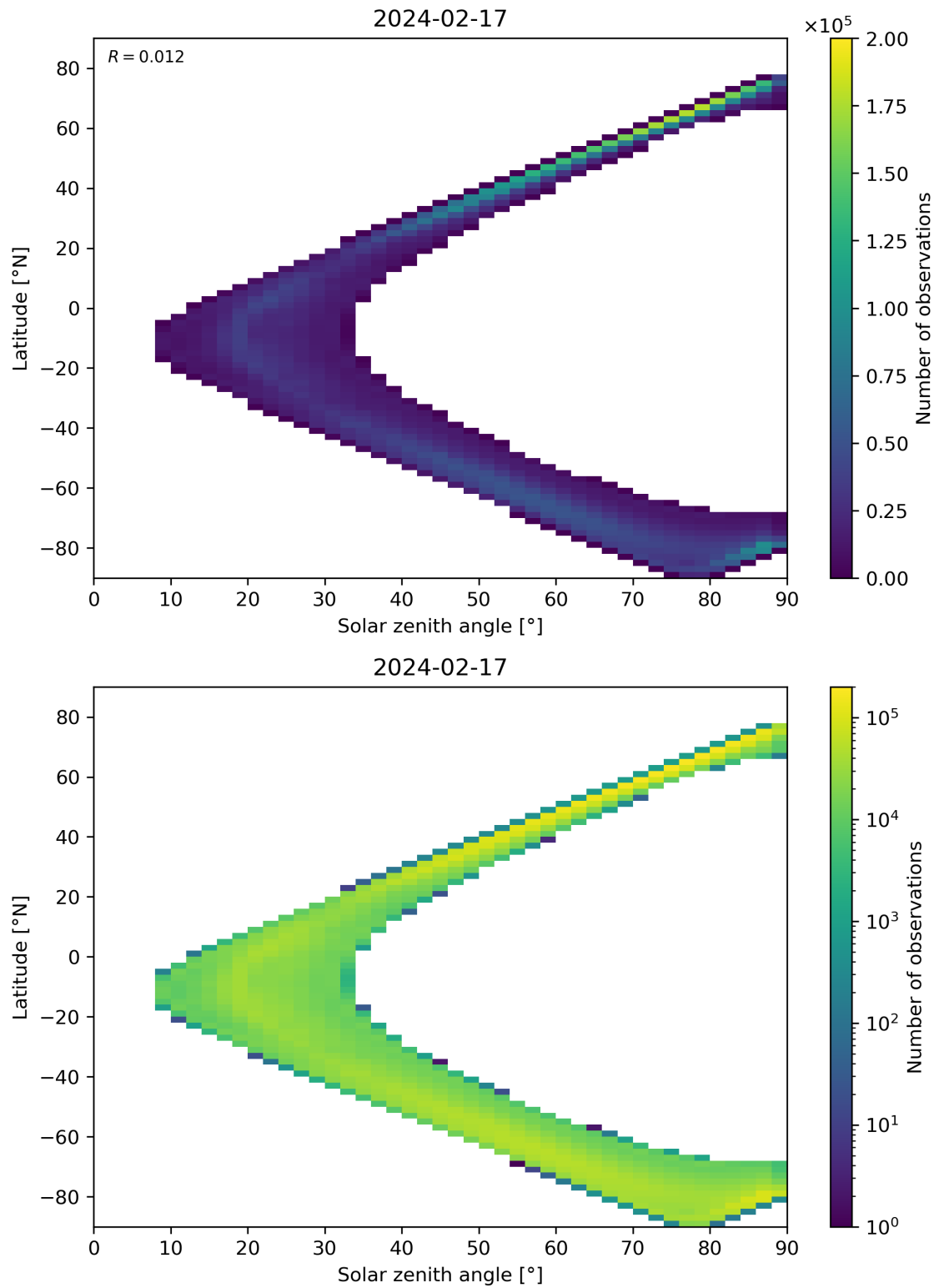
Figure 105: Scatter density plot of “Solar zenith angle” against “Latitude” for 2024-02-17 to 2024-02-18.
