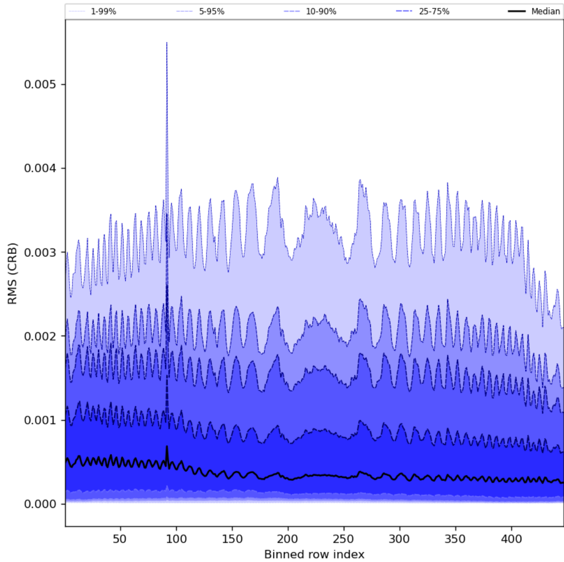
Figure 64: Along track statistics of “RMS (CRB)” for 2024-02-17 to 2024-02-18
