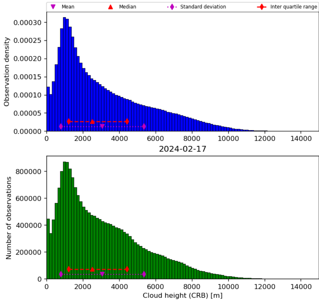
Figure 43: Histogram of “Cloud height (CRB)” for 2024-02-17 to 2024-02-18
