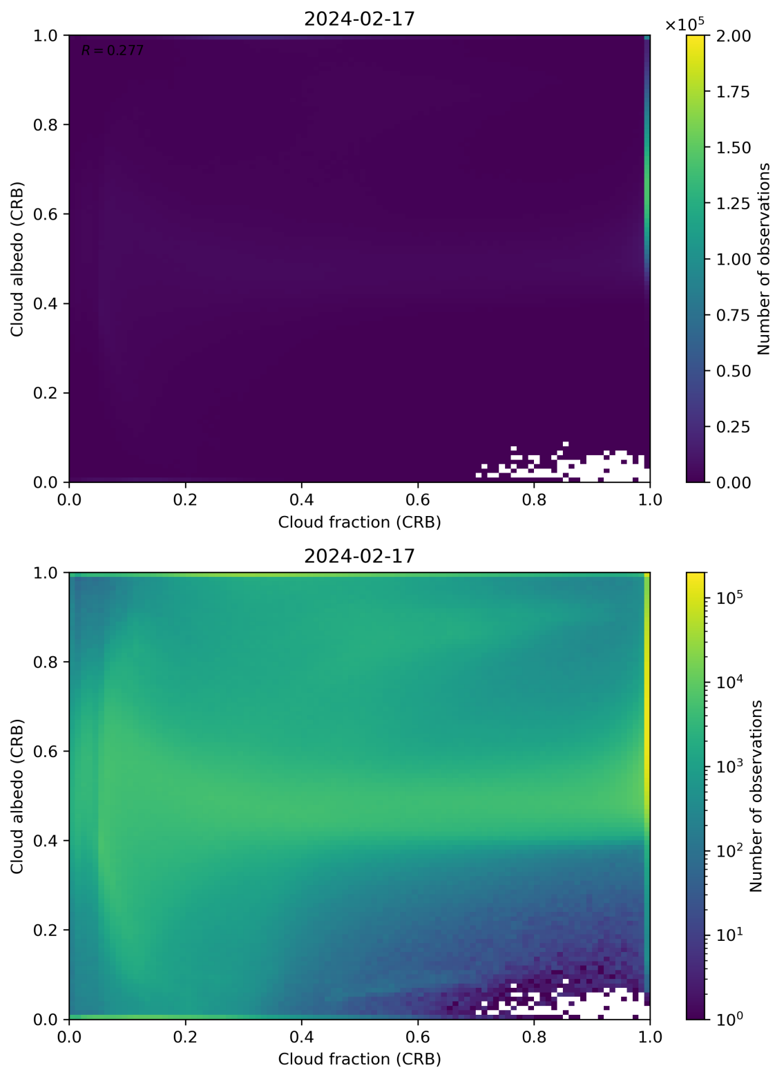
Figure 77: Scatter density plot of “Cloud fraction (CRB)” against “Cloud albedo (CRB)” for 2024-02-17 to 2024-02-18.
