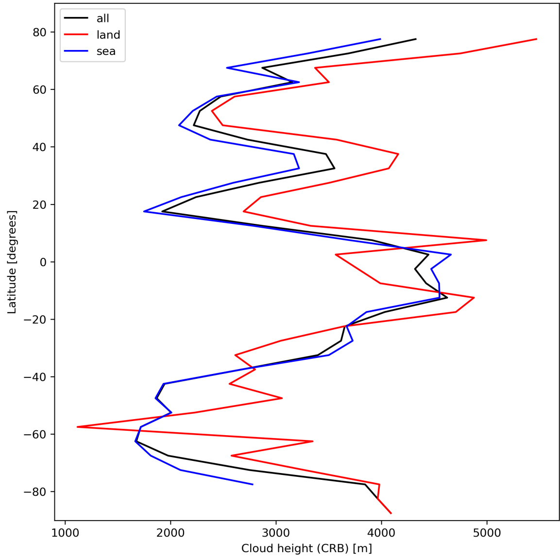
Figure 27: Zonal average of “Cloud height (CRB)” for 2024-02-17 to 2024-02-18.
