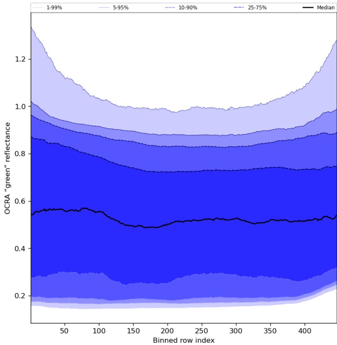
Figure 68: Along track statistics of "OCRA "green" reflectance" for 2024-02-17 to 2024-02-18
