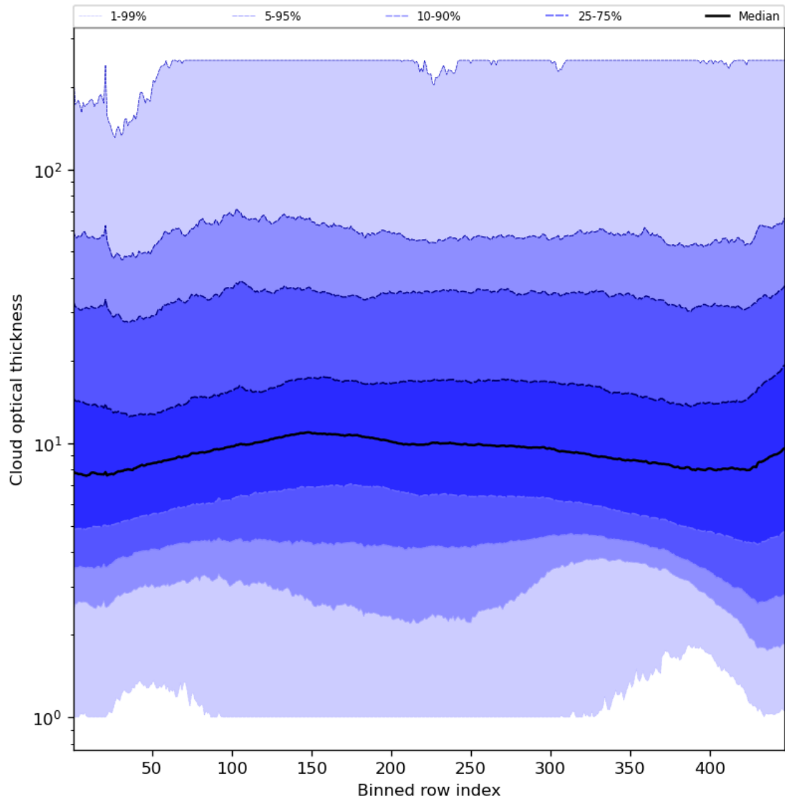
Figure 57: Along track statistics of “Cloud optical thickness” for 2024-02-17 to 2024-02-18
