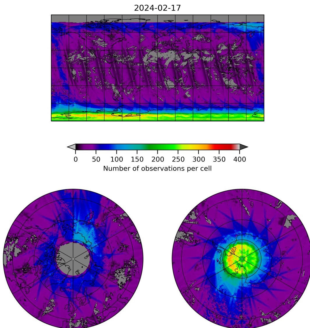
Figure 21: Map of the number of observations for 2024-02-17 to 2024-02-18
