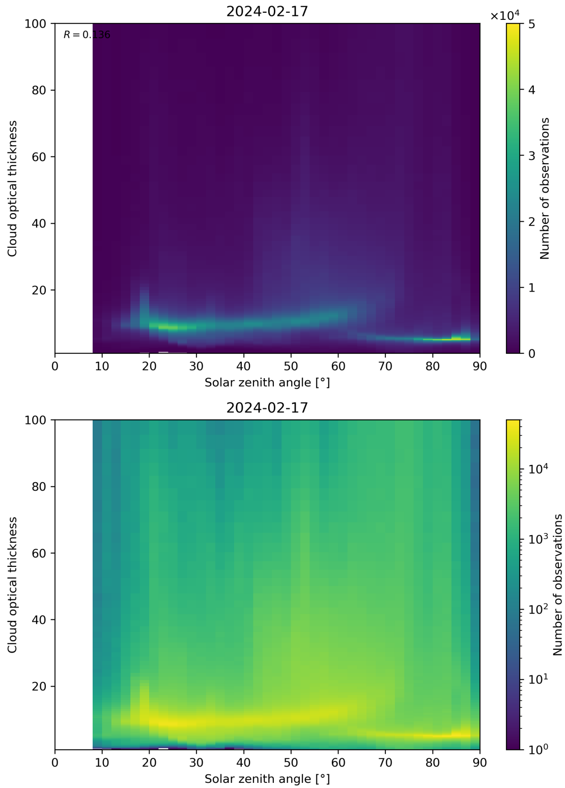
Figure 103: Scatter density plot of “Solar zenith angle” against “Cloud optical thickness” for 2024-02-17 to 2024-02-18.
