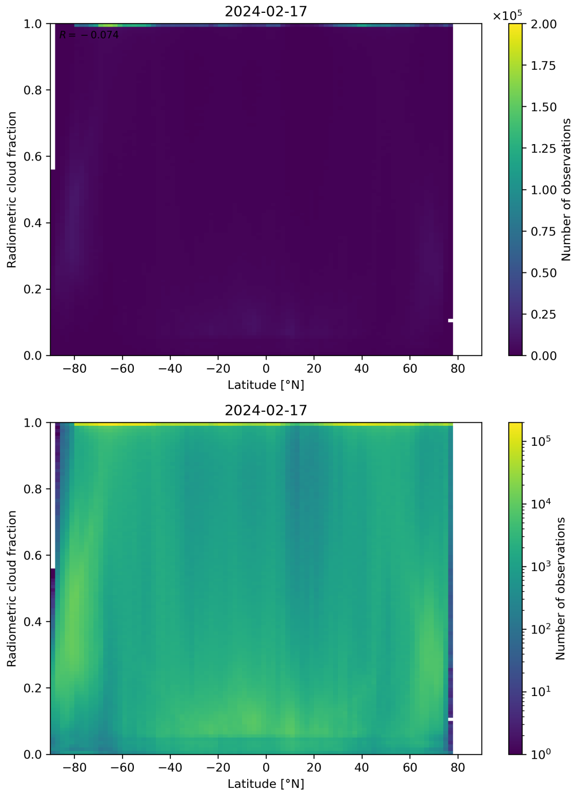
Figure 92: Scatter density plot of “Latitude” against “Radiometric cloud fraction” for 2024-02-17 to 2024-02-18.
