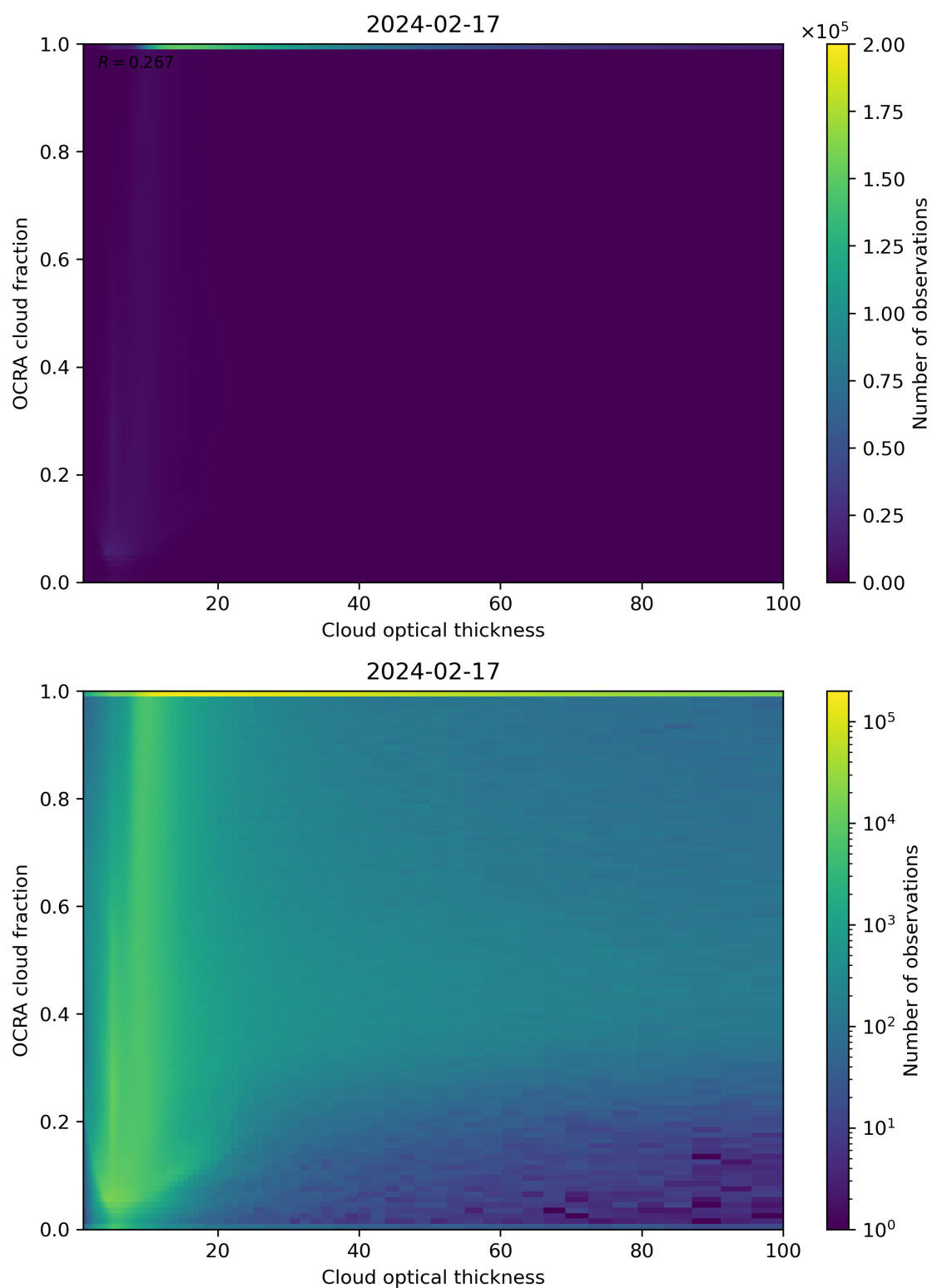
Figure 83: Scatter density plot of “Cloud optical thickness” against “OCRA cloud fraction” for 2024-02-17 to 2024-02-18.
