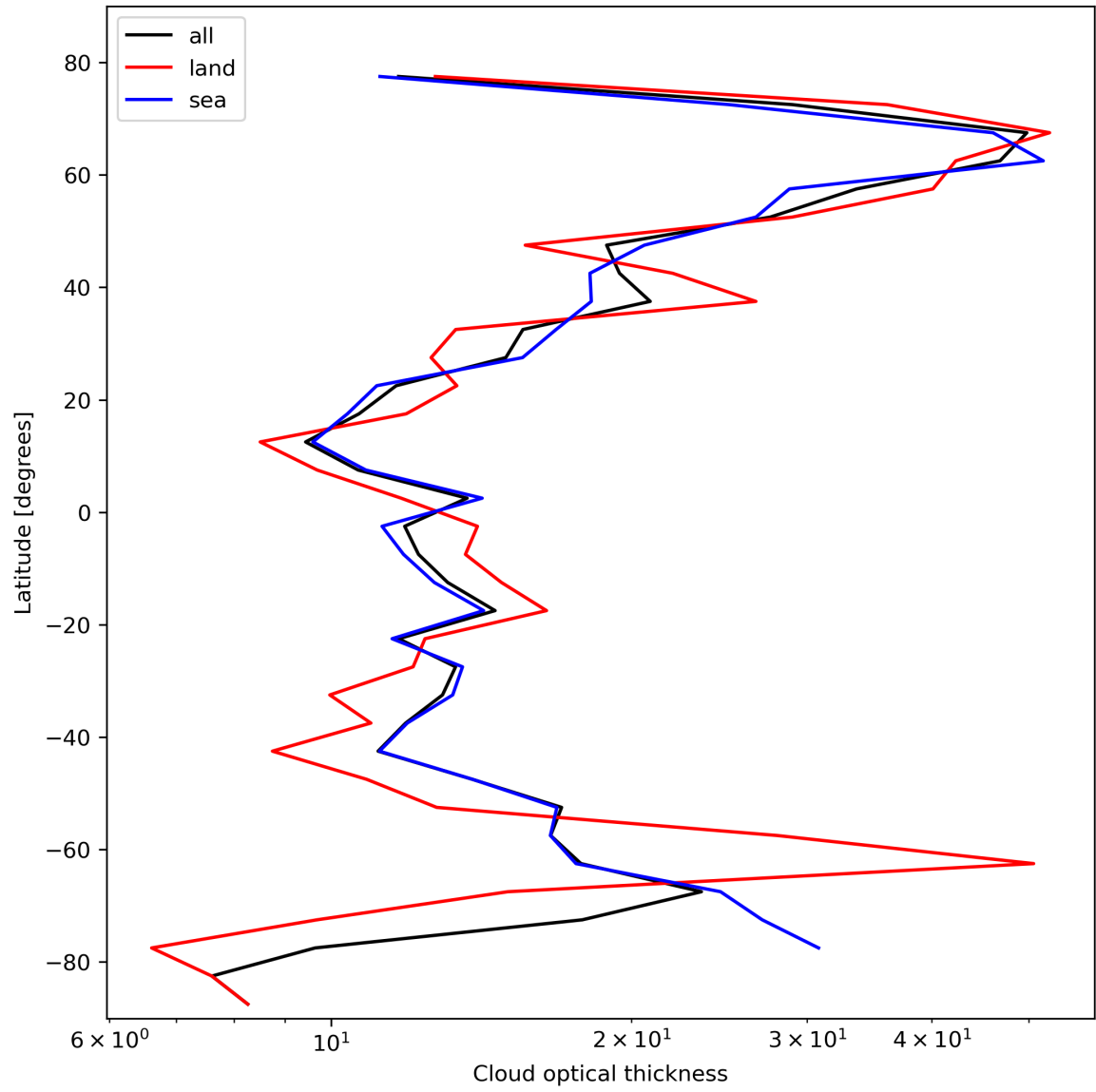
Figure 25: Zonal average of “Cloud optical thickness” for 2024-02-17 to 2024-02-18.
