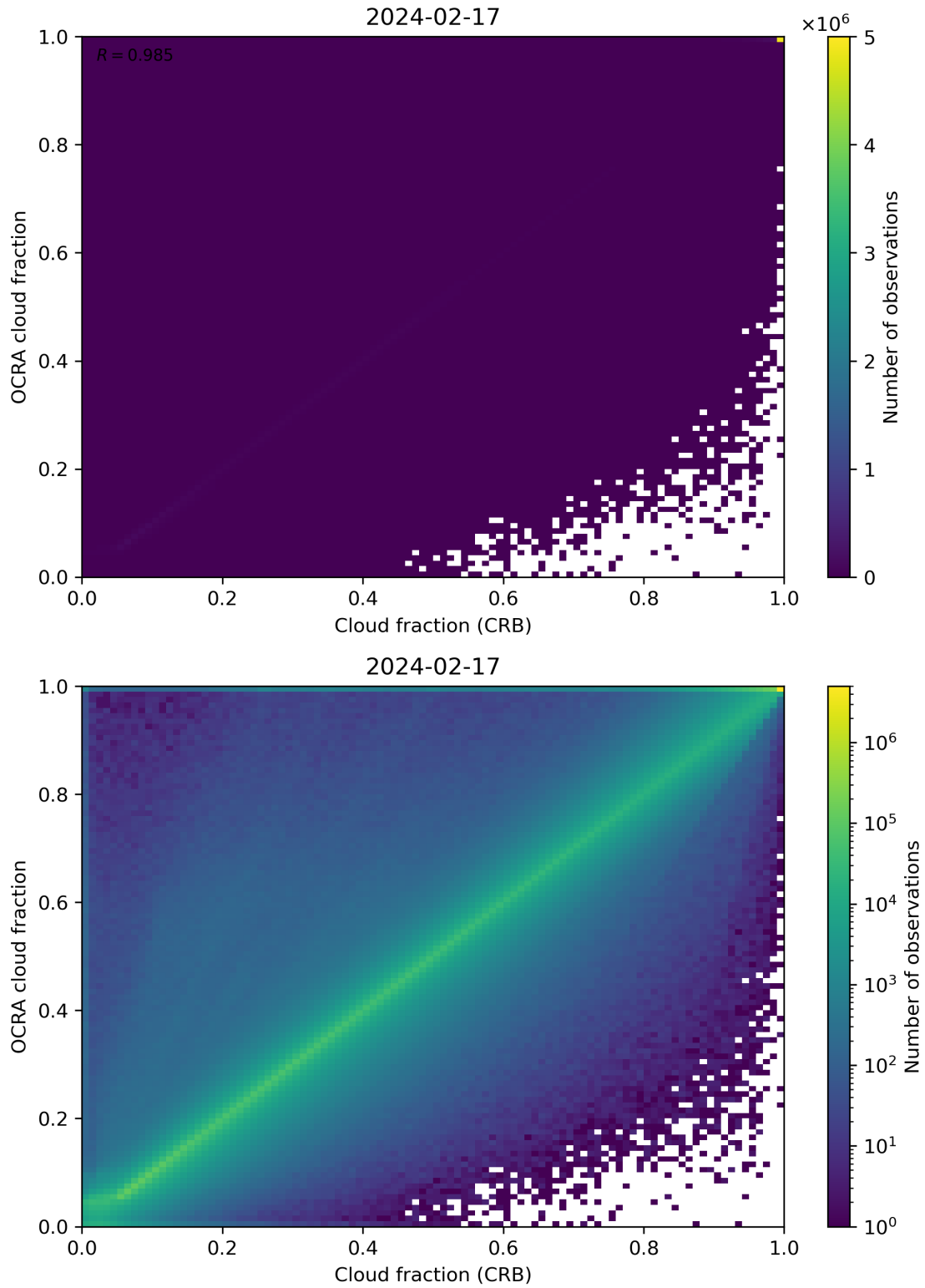
Figure 78: Scatter density plot of “Cloud fraction (CRB)” against “OCRA cloud fraction” for 2024-02-17 to 2024-02-18.
