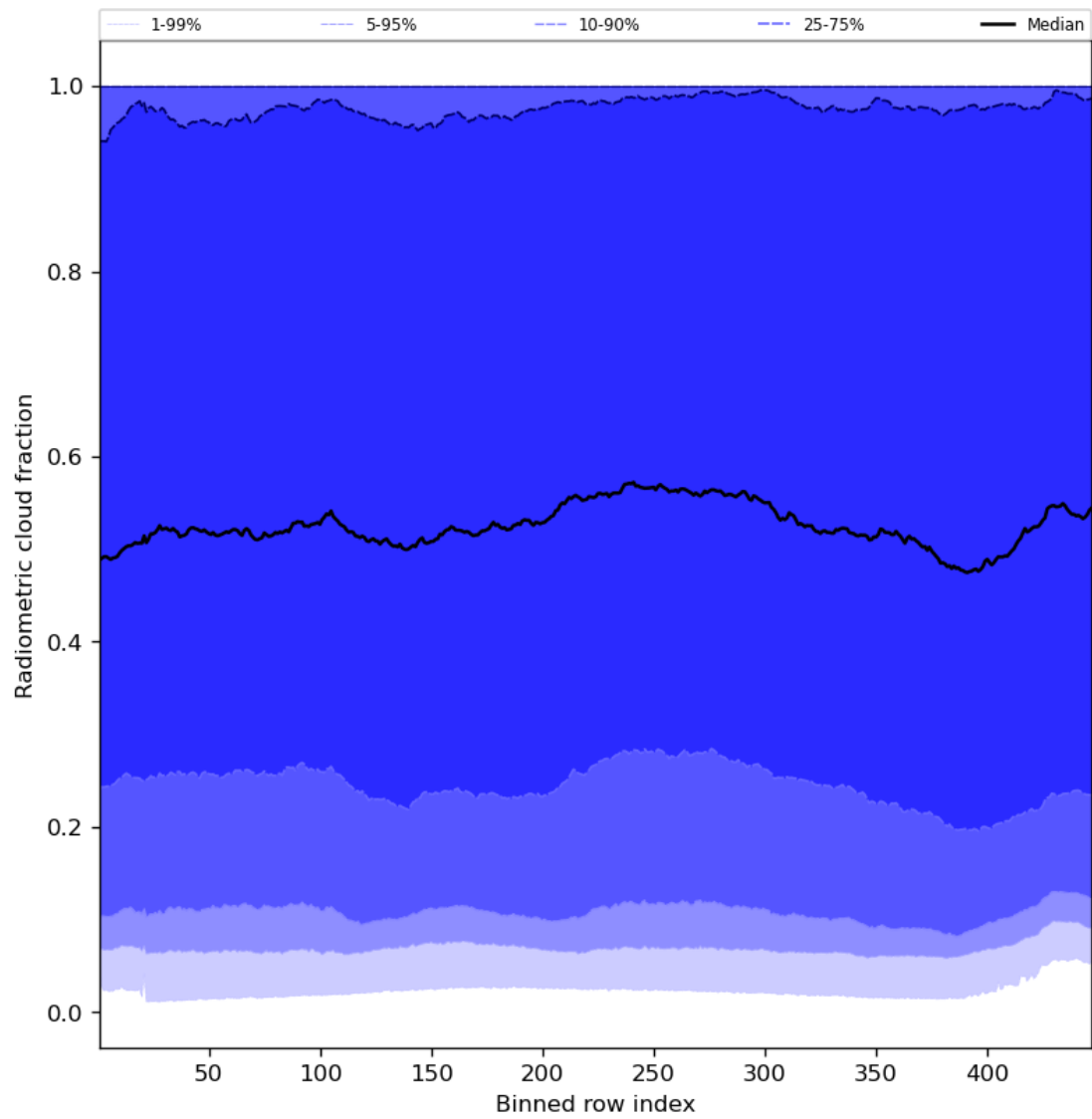
Figure 55: Along track statistics of “Radiometric cloud fraction” for 2024-02-17 to 2024-02-18
