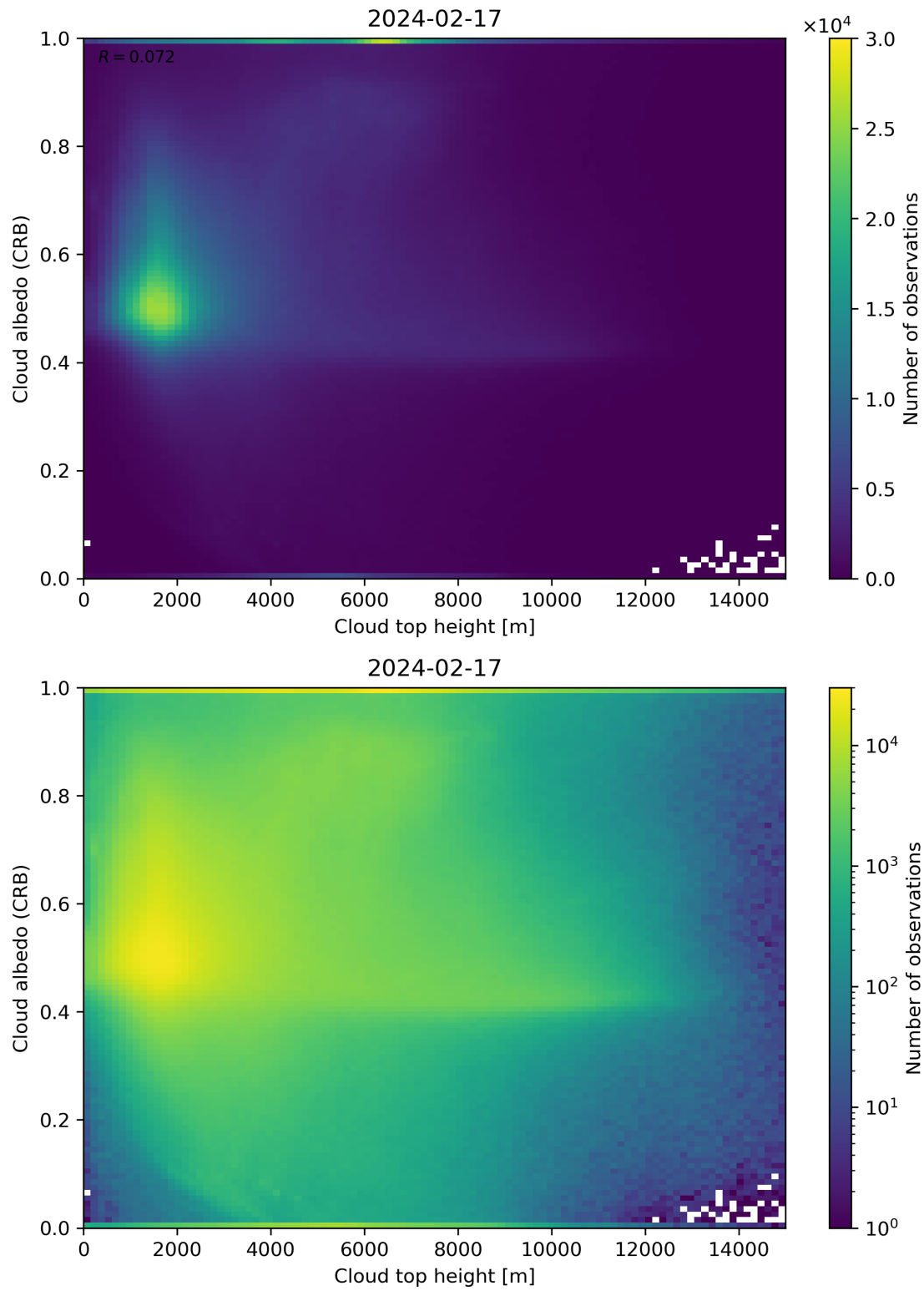
Figure 86: Scatter density plot of “Cloud top height” against “Cloud albedo (CRB)” for 2024-02-17 to 2024-02-18.
