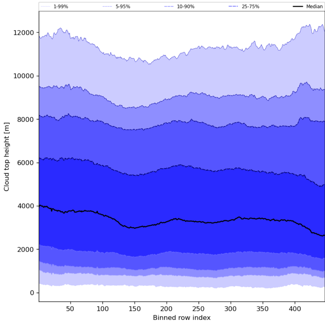
Figure 56: Along track statistics of “Cloud top height” for 2024-02-17 to 2024-02-18
