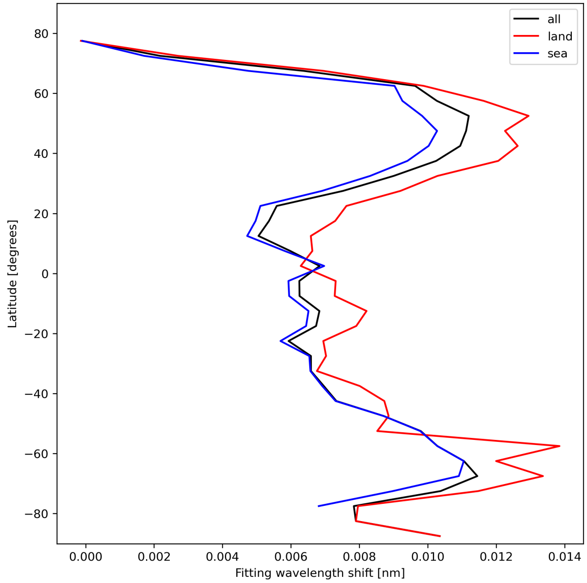
Figure 33: Zonal average of “Fitting wavelength shift” for 2024-02-17 to 2024-02-18.
