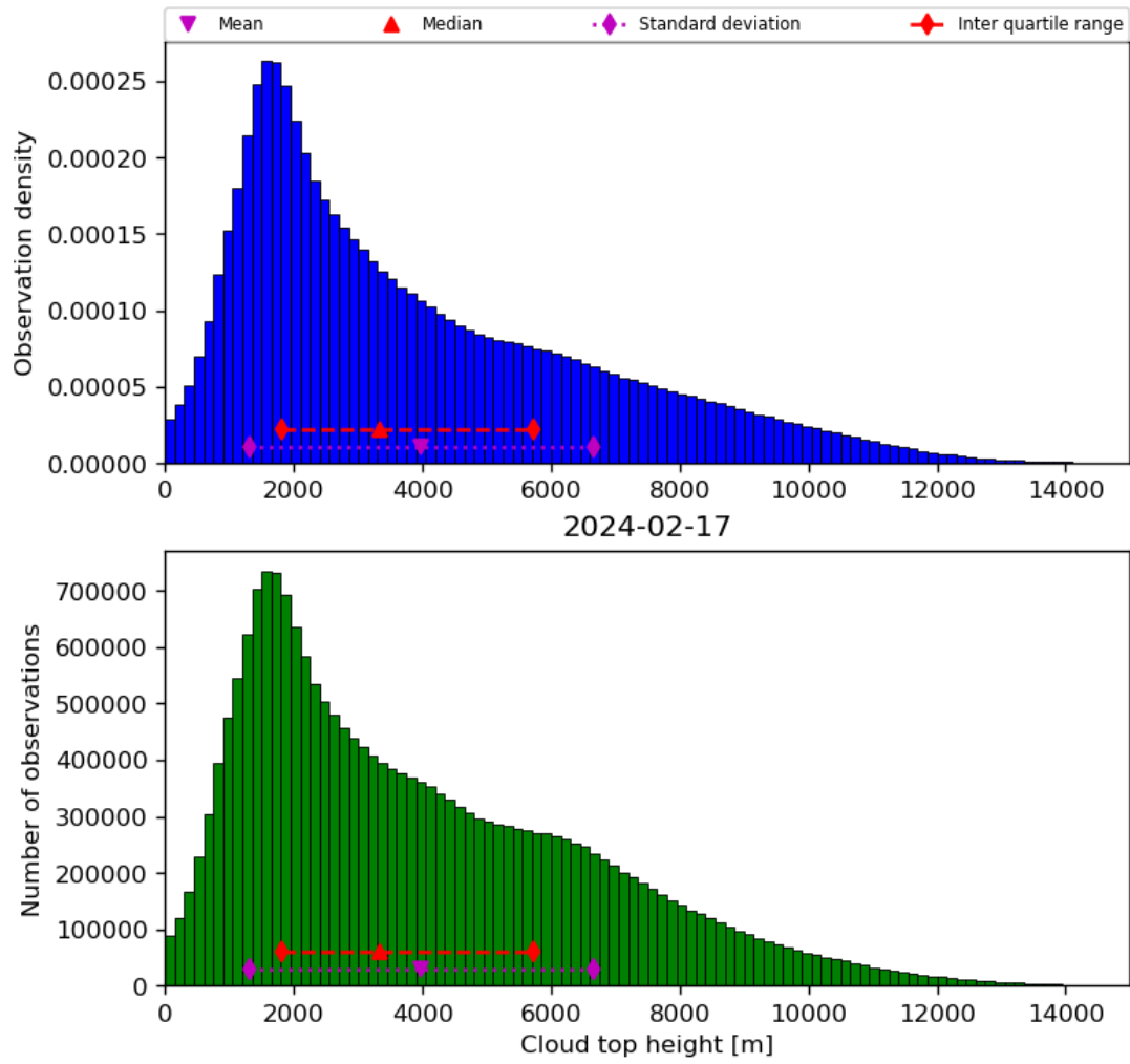
Figure 40: Histogram of “Cloud top height” for 2024-02-17 to 2024-02-18
