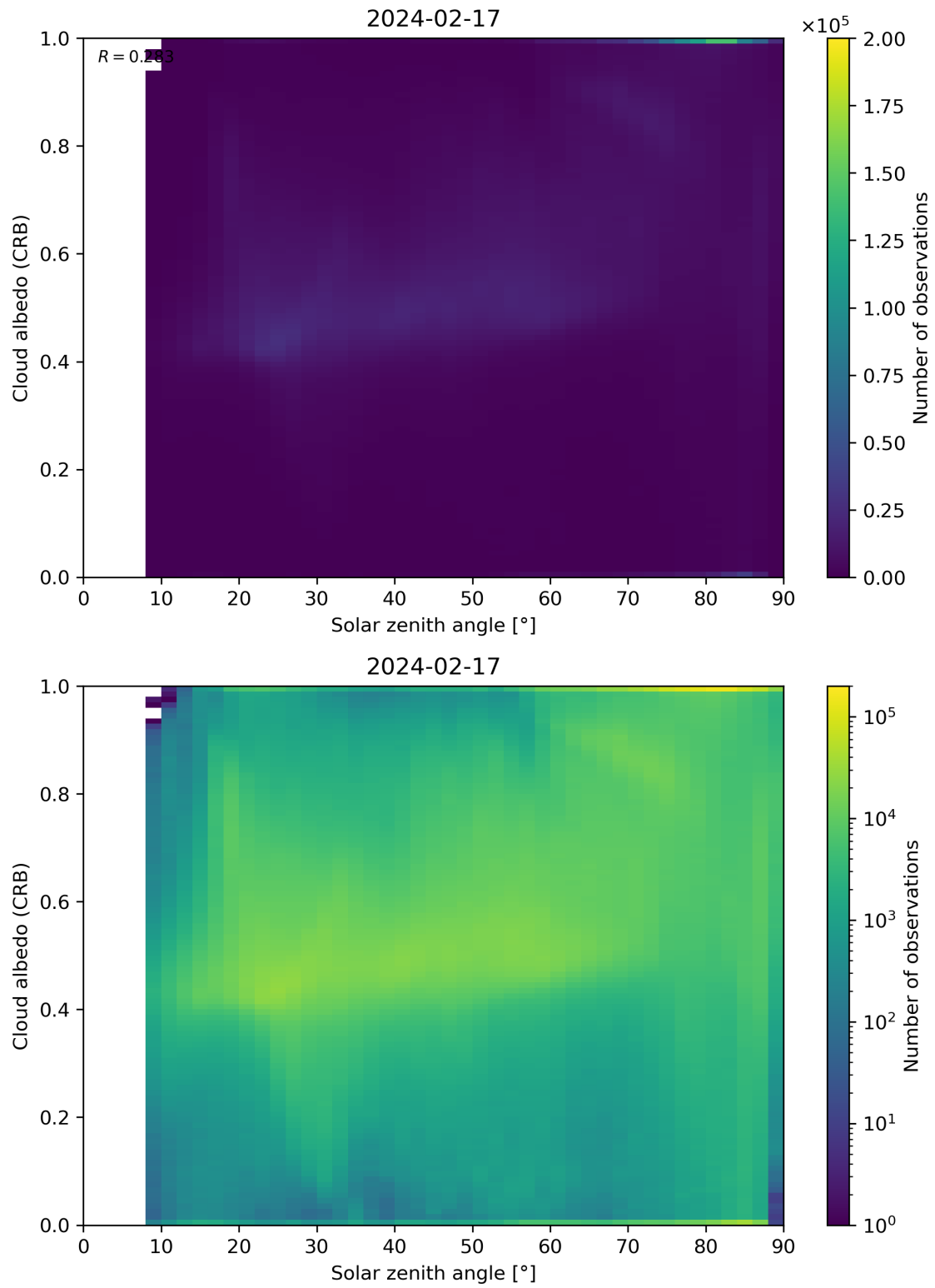
Figure 98: Scatter density plot of “Solar zenith angle” against “Cloud albedo (CRB)” for 2024-02-17 to 2024-02-18.
