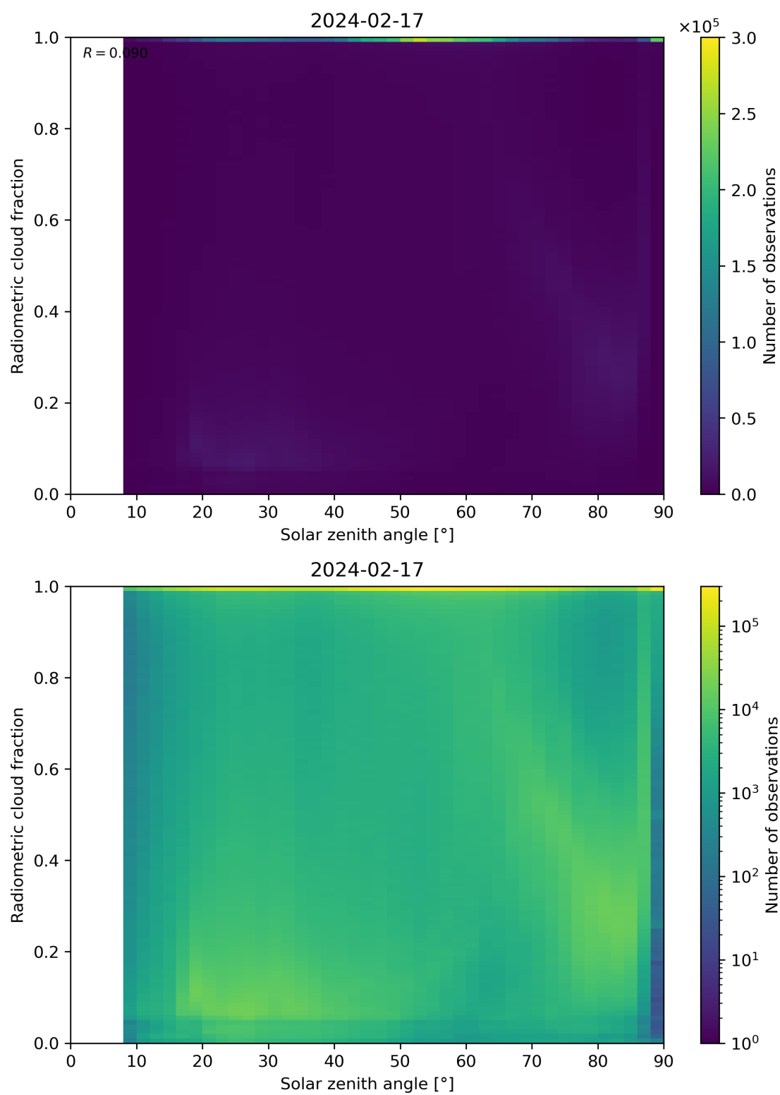
Figure 99: Scatter density plot of “Solar zenith angle” against “Radiometric cloud fraction” for 2024-02-17 to 2024-02-18.
