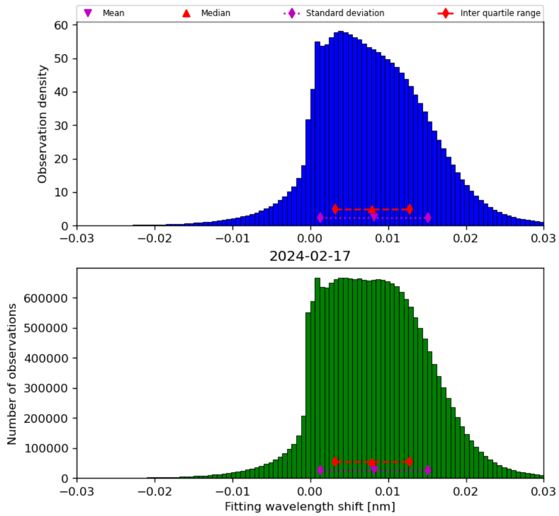
Figure 49: Histogram of “Fitting wavelength shift” for 2024-02-17 to 2024-02-18
