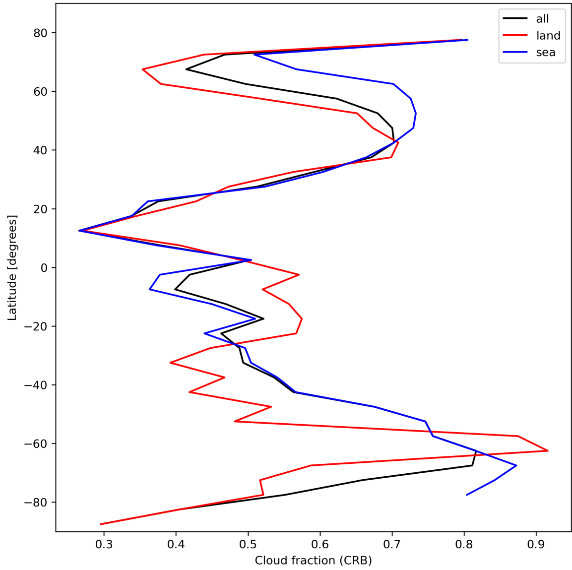
Figure 26: Zonal average of “Cloud fraction (CRB)” for 2024-02-17 to 2024-02-18.
