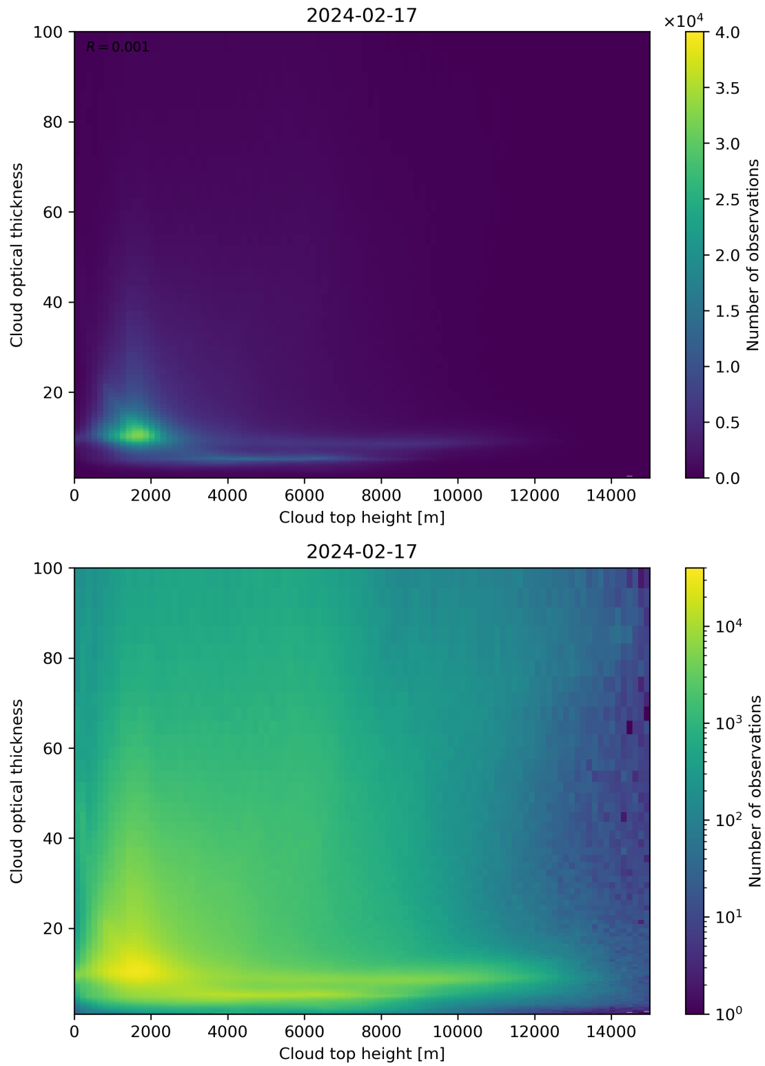
Figure 90: Scatter density plot of “Cloud top height” against “Cloud optical thickness” for 2024-02-17 to 2024-02-18.
