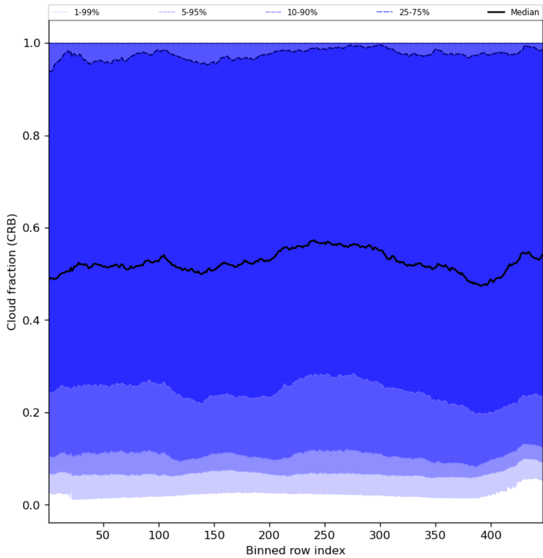
Figure 58: Along track statistics of “Cloud fraction (CRB)” for 2024-02-17 to 2024-02-18
