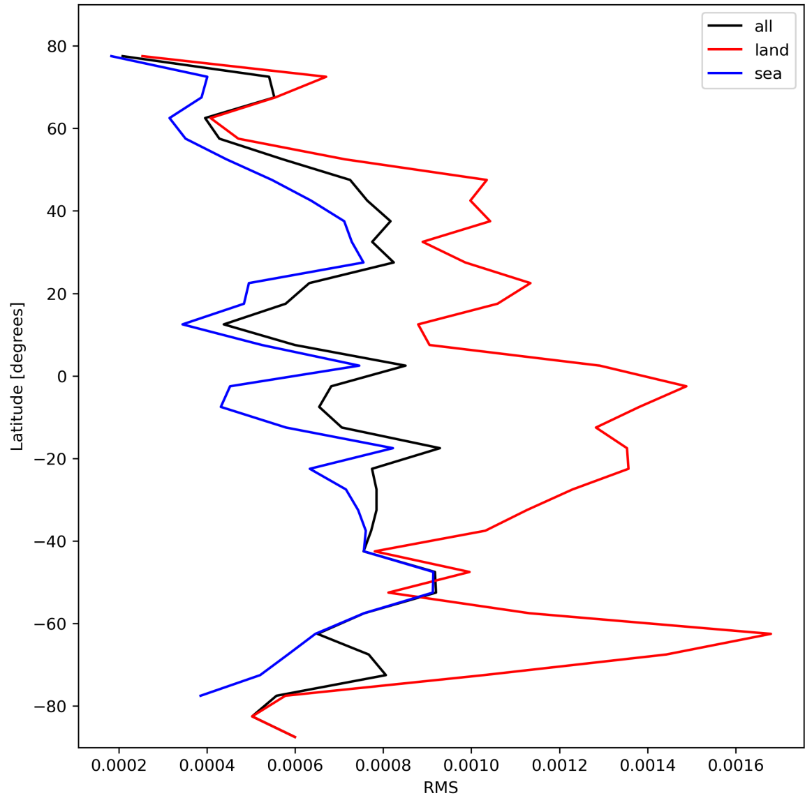
Figure 31: Zonal average of “RMS” for 2024-02-17 to 2024-02-18.
