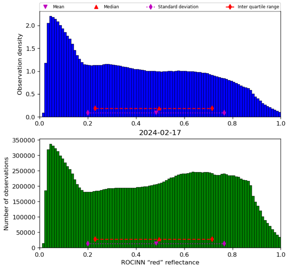
Figure 53: Histogram of “ROCINN “red” reflectance” for 2024-02-17 to 2024-02-18
