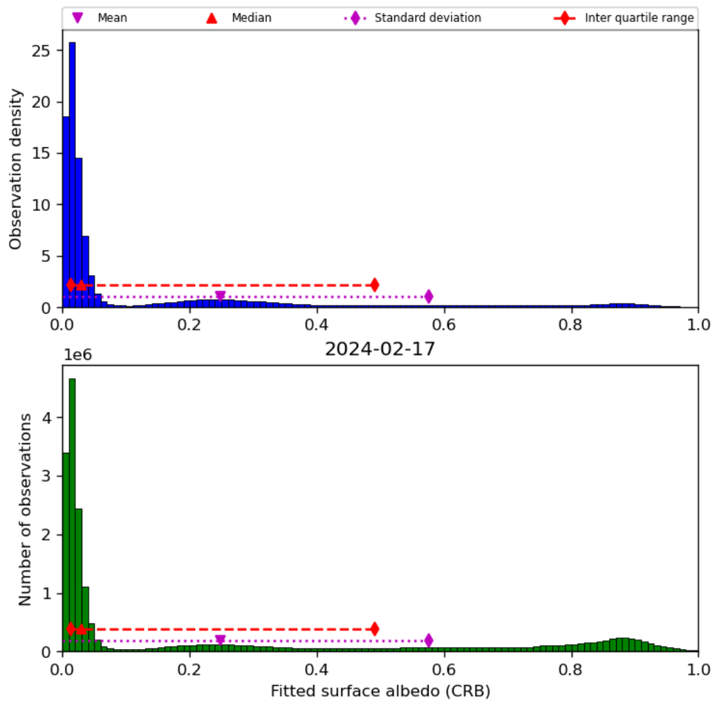
Figure 46: Histogram of “Fitted surface albedo (CRB)” for 2024-02-17 to 2024-02-18
