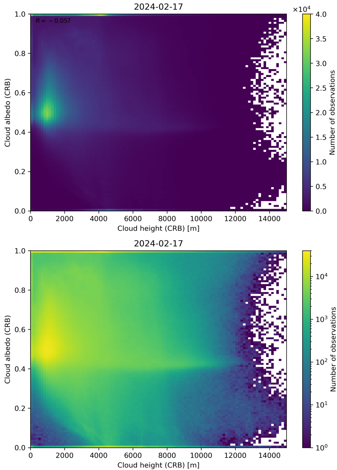
Figure 80: Scatter density plot of “Cloud height (CRB)” against “Cloud albedo (CRB)” for 2024-02-17 to 2024-02-18.
