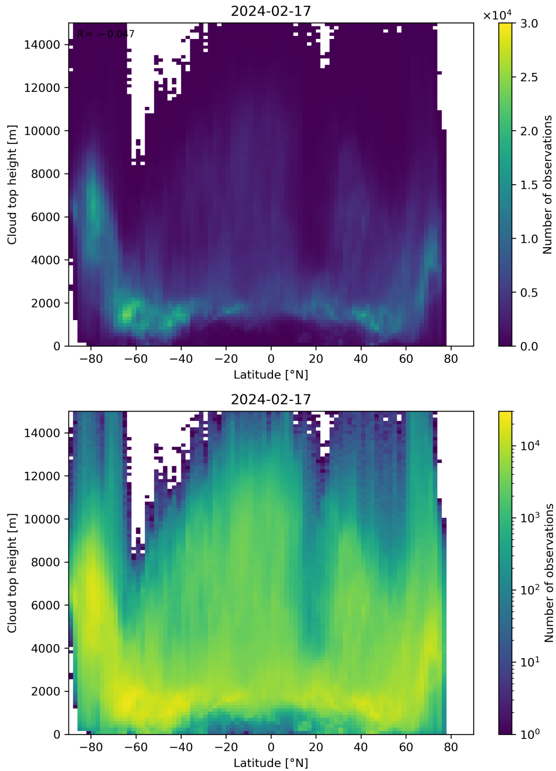
Figure 97: Scatter density plot of “Latitude” against “Cloud top height” for 2024-02-17 to 2024-02-18.
