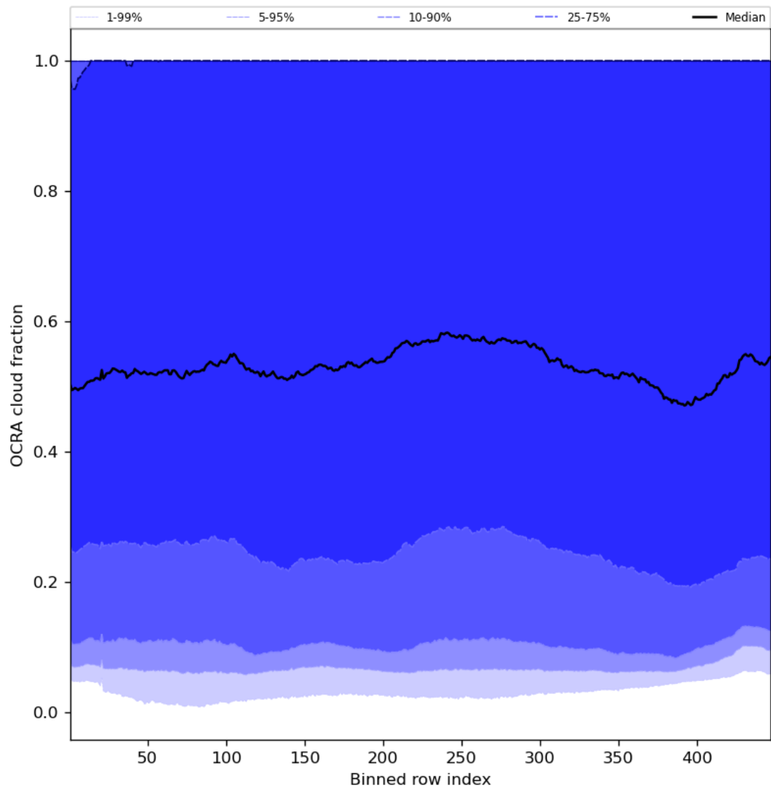
Figure 66: Along track statistics of “OCRA cloud fraction” for 2024-02-17 to 2024-02-18
