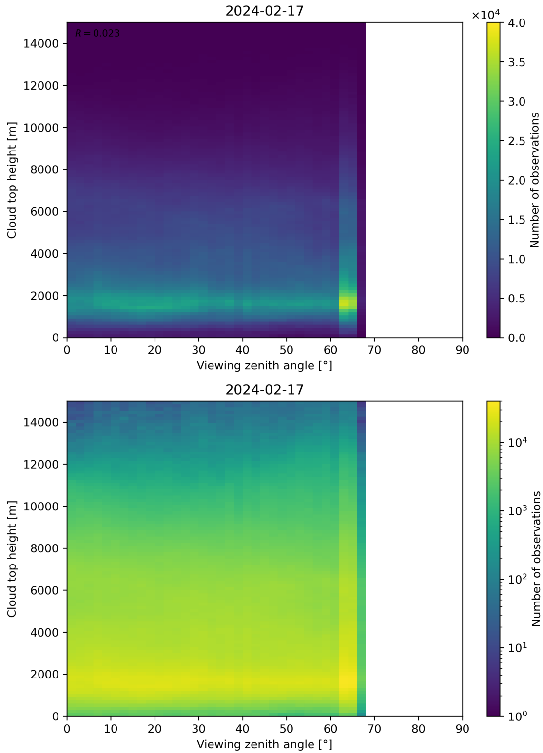
Figure 112: Scatter density plot of “Viewing zenith angle” against “Cloud top height” for 2024-02-17 to 2024-02-18.
