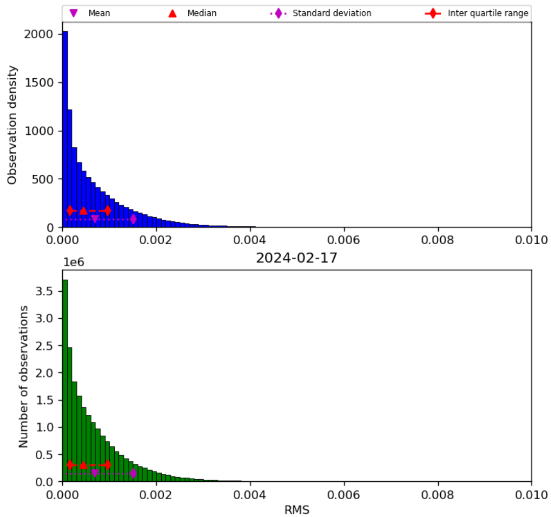
Figure 47: Histogram of “RMS” for 2024-02-17 to 2024-02-18
