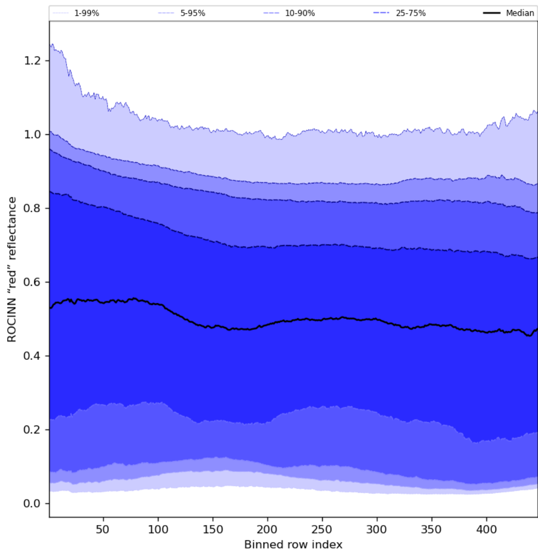
Figure 69: Along track statistics of “ROCINN “red” reflectance” for 2024-02-17 to 2024-02-18
