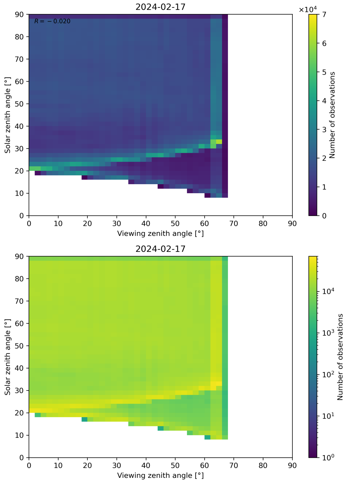
Figure 114: Scatter density plot of “Viewing zenith angle” against “Solar zenith angle” for 2024-02-17 to 2024-02-18.
