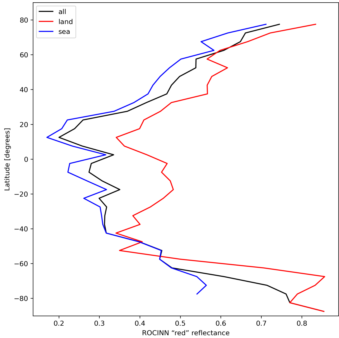
Figure 37: Zonal average of "ROCINN "red" reflectance" for 2024-02-17 to 2024-02-18.
