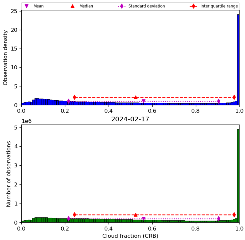
Figure 42: Histogram of “Cloud fraction (CRB)” for 2024-02-17 to 2024-02-18
