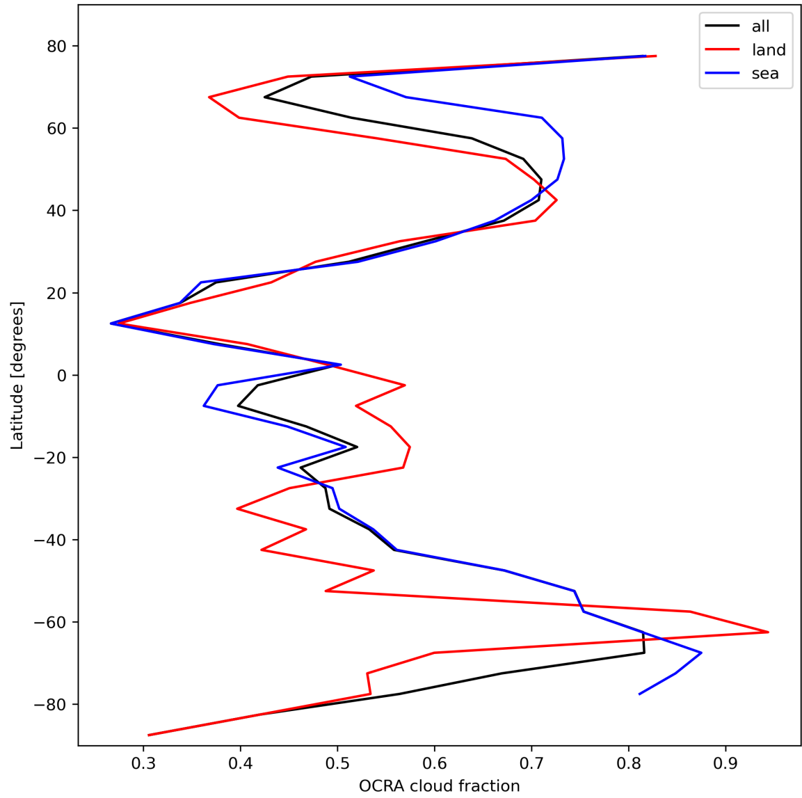
Figure 34: Zonal average of “OCRA cloud fraction” for 2024-02-17 to 2024-02-18.
