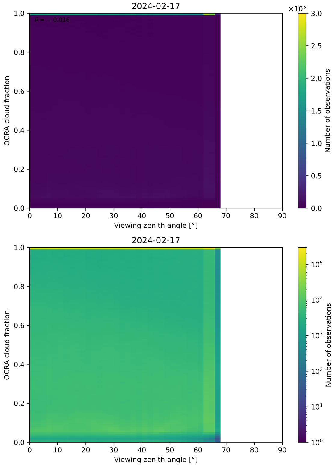
Figure 108: Scatter density plot of “Viewing zenith angle” against “OCRA cloud fraction” for 2024-02-17 to 2024-02-18.
