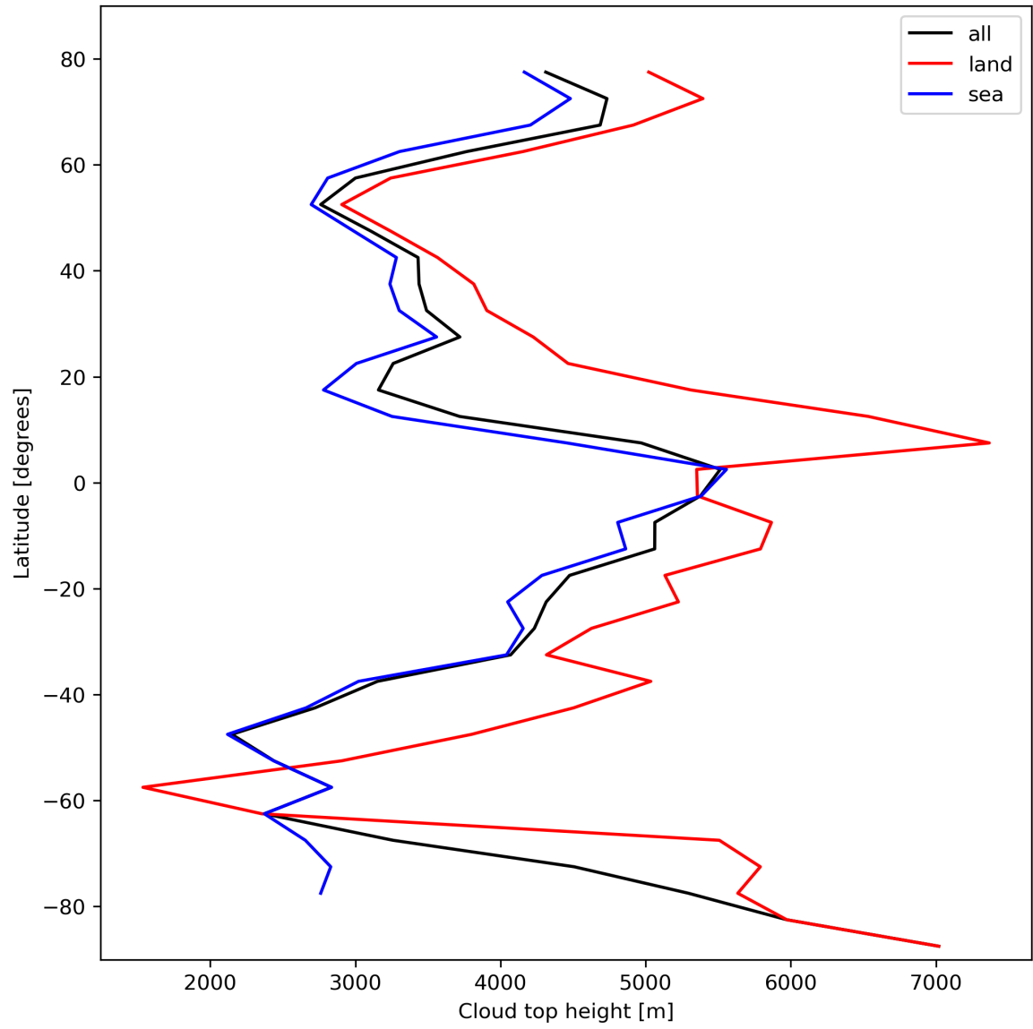
Figure 24: Zonal average of “Cloud top height” for 2024-02-22 to 2024-02-23.
