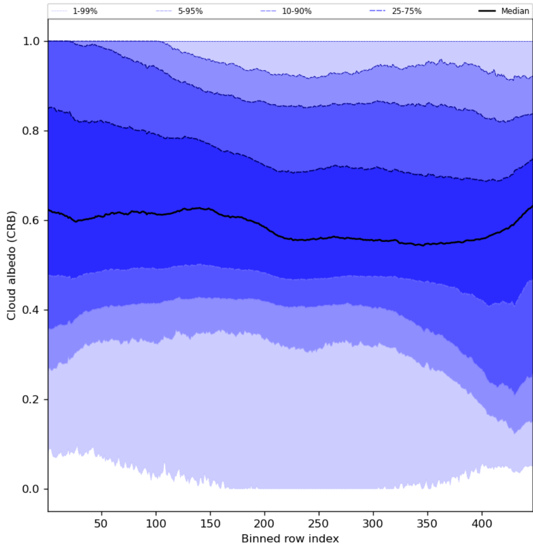
Figure 60: Along track statistics of “Cloud albedo (CRB)” for 2024-02-22 to 2024-02-23
