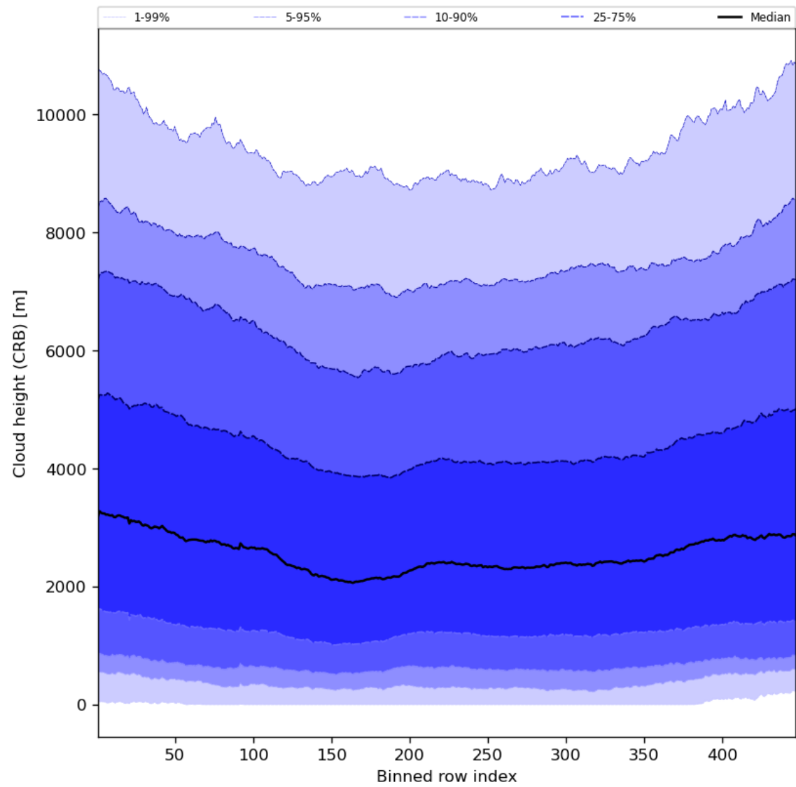
Figure 59: Along track statistics of “Cloud height (CRB)” for 2024-02-22 to 2024-02-23
