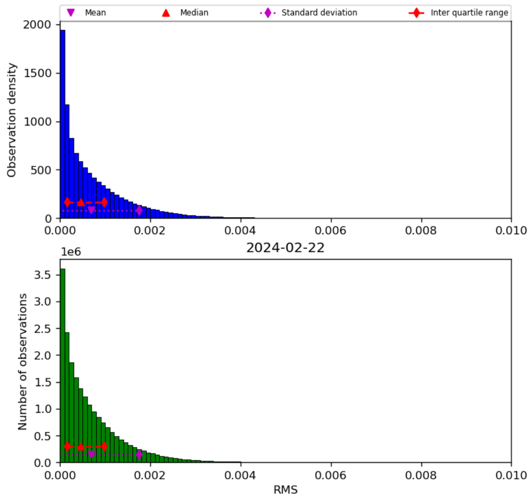
Figure 47: Histogram of “RMS” for 2024-02-22 to 2024-02-23
