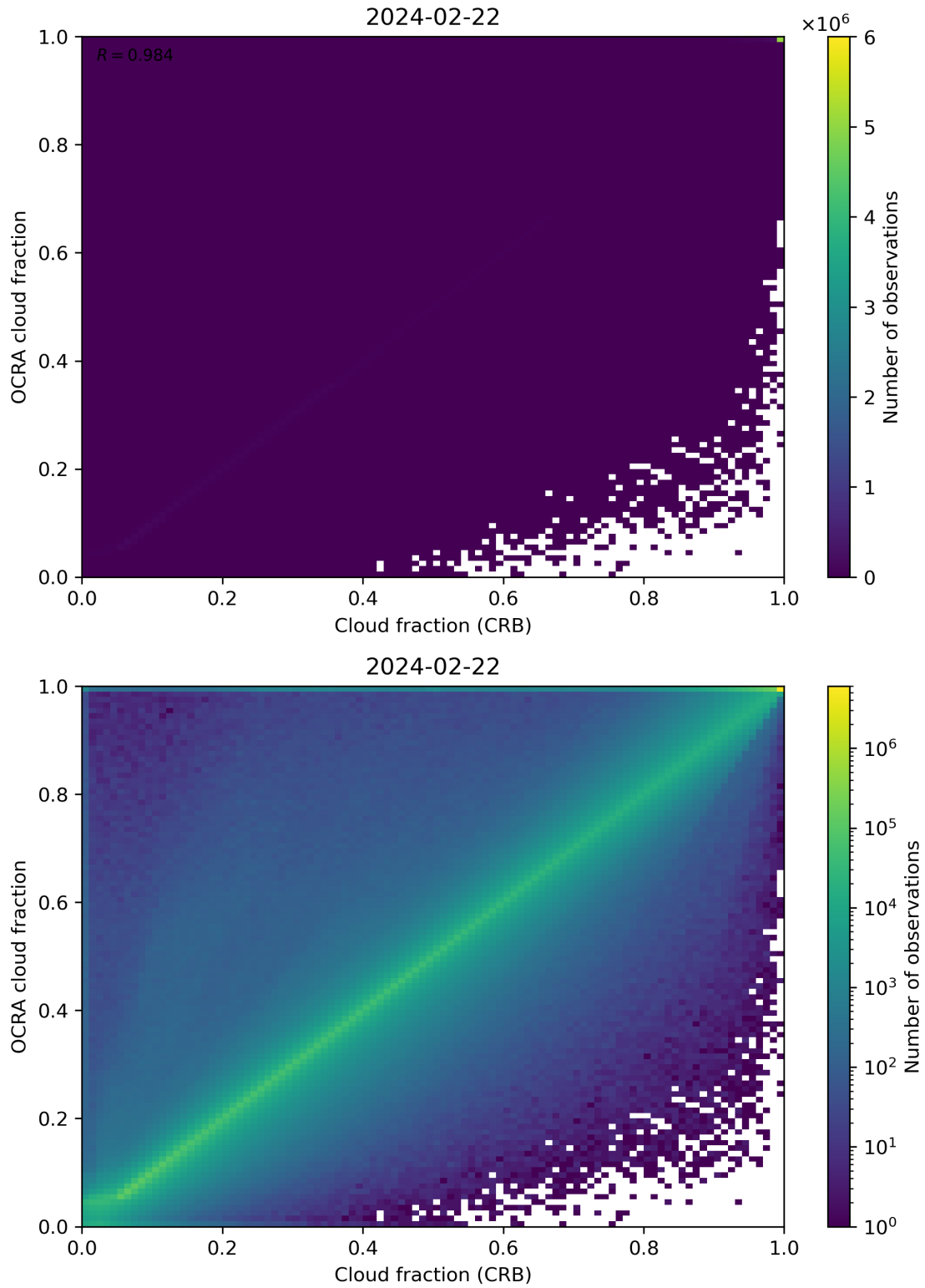
Figure 78: Scatter density plot of “Cloud fraction (CRB)” against “OCRA cloud fraction” for 2024-02-22 to 2024-02-23.
