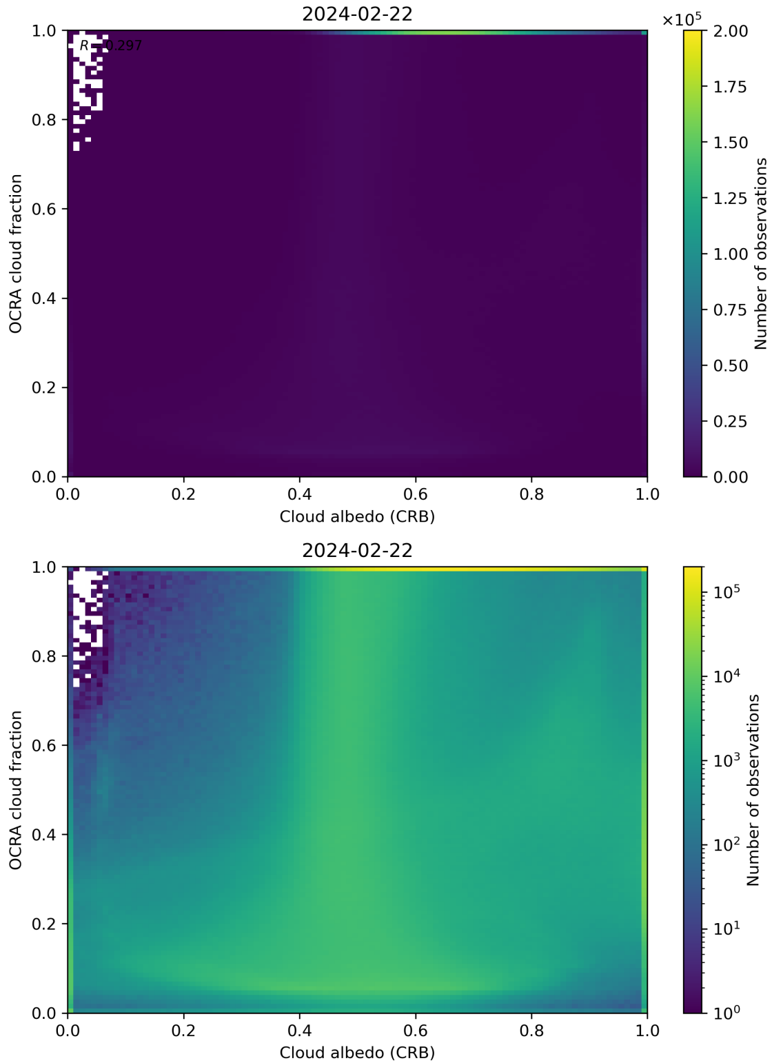
Figure 70: Scatter density plot of “Cloud albedo (CRB)” against “OCRA cloud fraction” for 2024-02-22 to 2024-02-23.
