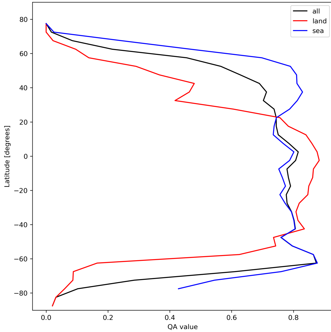
Figure 22: Zonal average of “QA value” for 2024-02-22 to 2024-02-23.
