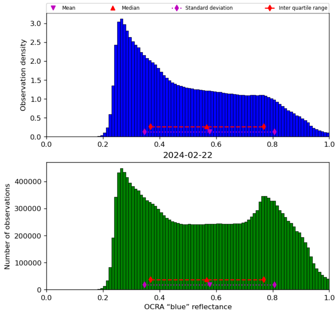
Figure 51: Histogram of “OCRA “blue” reflectance” for 2024-02-22 to 2024-02-23
