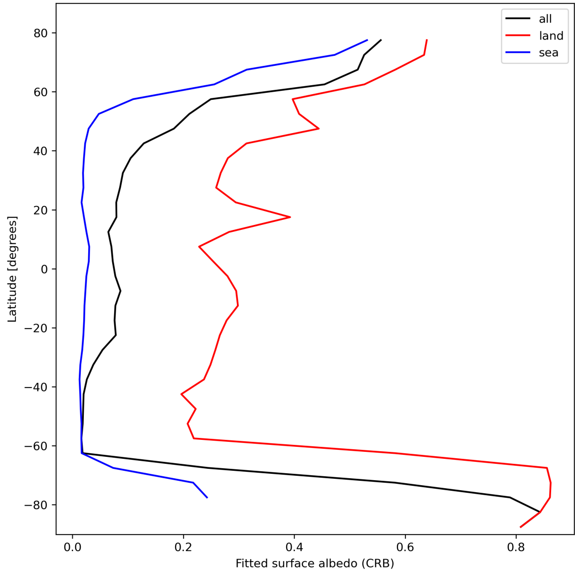
Figure 30: Zonal average of “Fitted surface albedo (CRB)” for 2024-02-22 to 2024-02-23.
