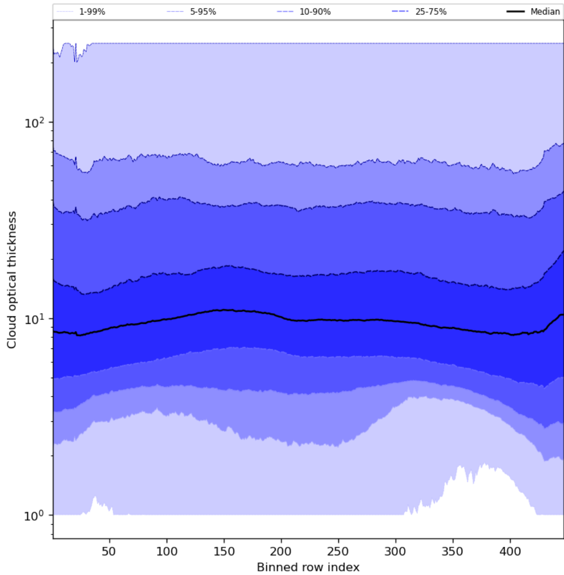
Figure 57: Along track statistics of “Cloud optical thickness” for 2024-02-22 to 2024-02-23
