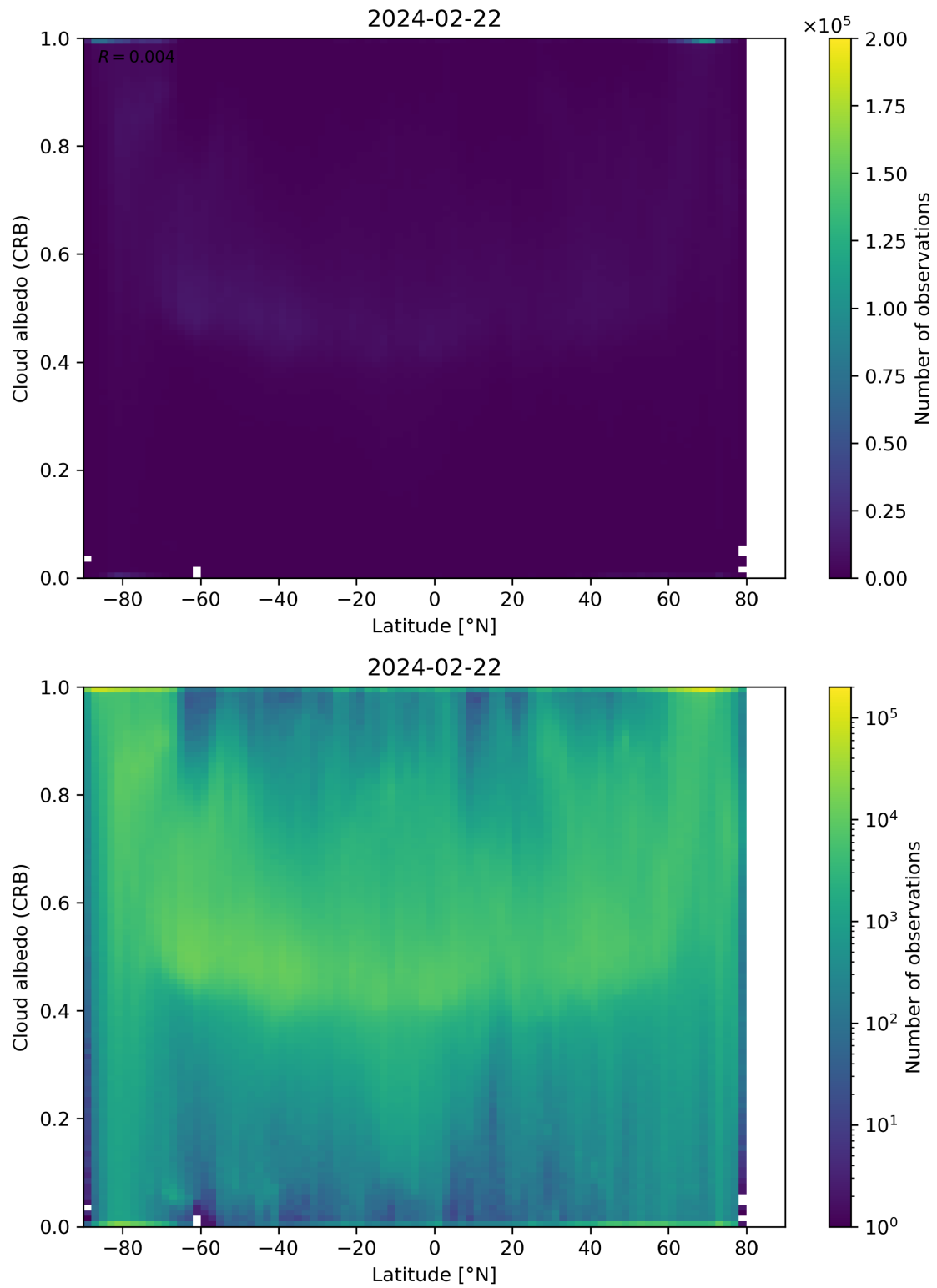
Figure 91: Scatter density plot of “Latitude” against “Cloud albedo (CRB)” for 2024-02-22 to 2024-02-23.
