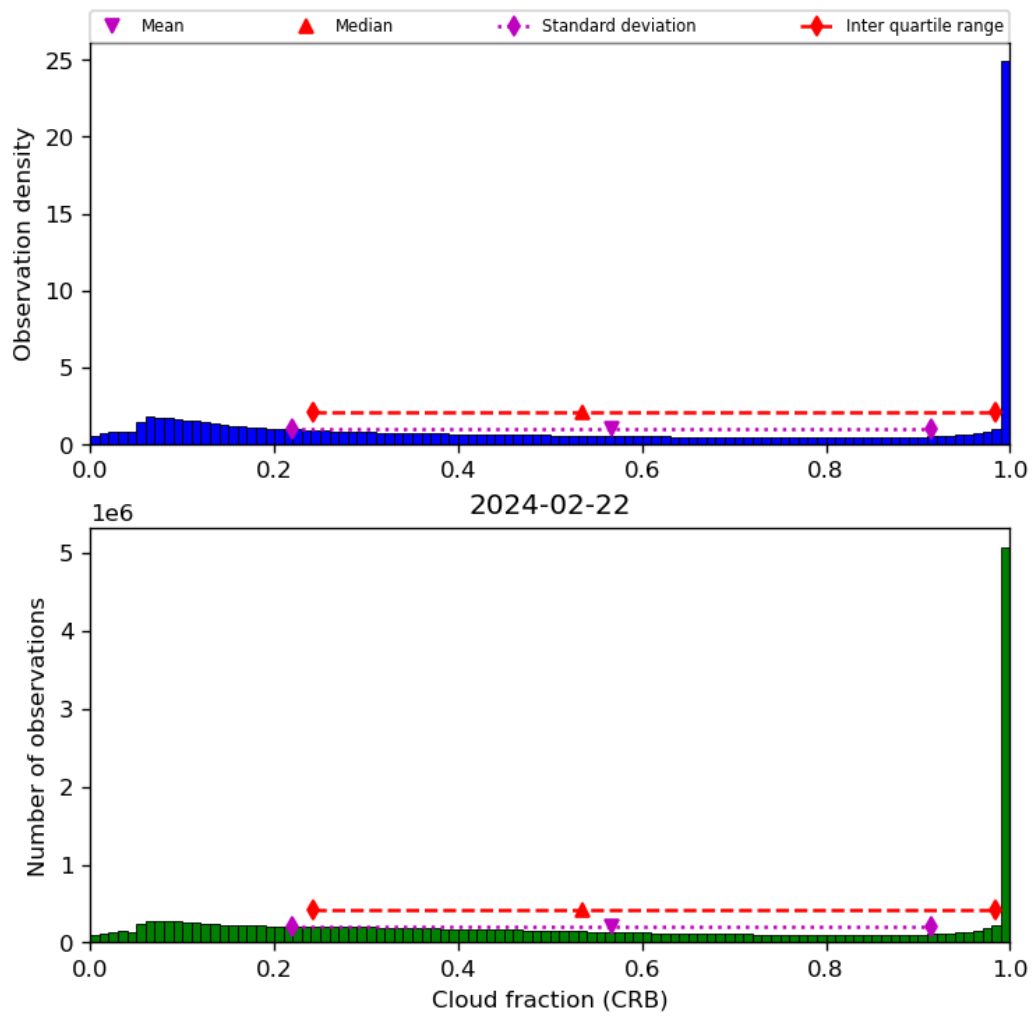
Figure 42: Histogram of “Cloud fraction (CRB)” for 2024-02-22 to 2024-02-23
