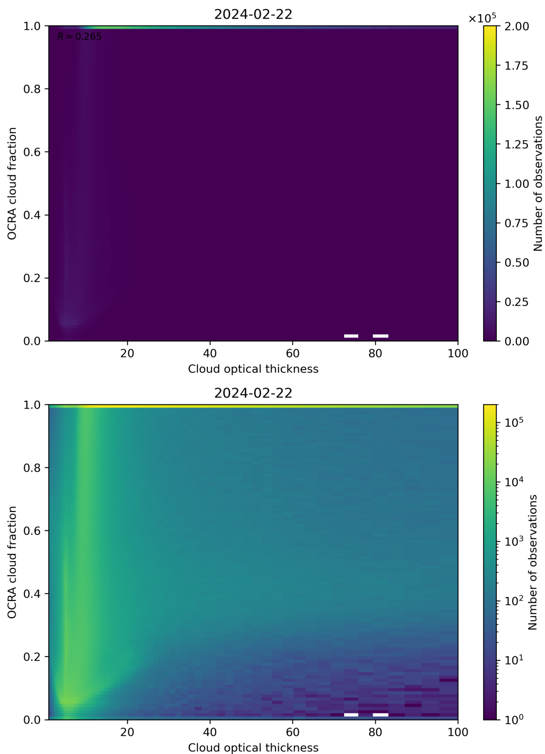
Figure 83: Scatter density plot of “Cloud optical thickness” against “OCRA cloud fraction” for 2024-02-22 to 2024-02-23.
