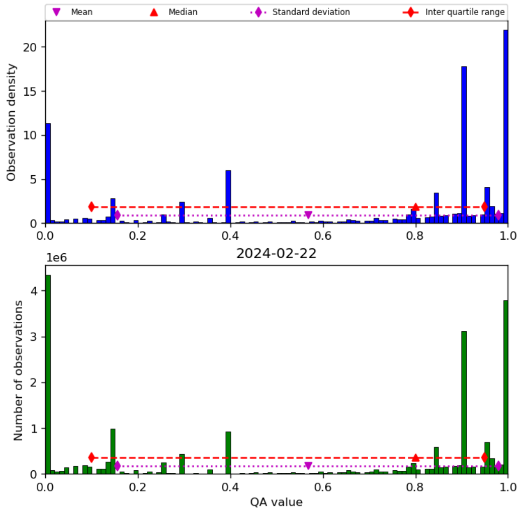
Figure 38: Histogram of “QA value” for 2024-02-22 to 2024-02-23
