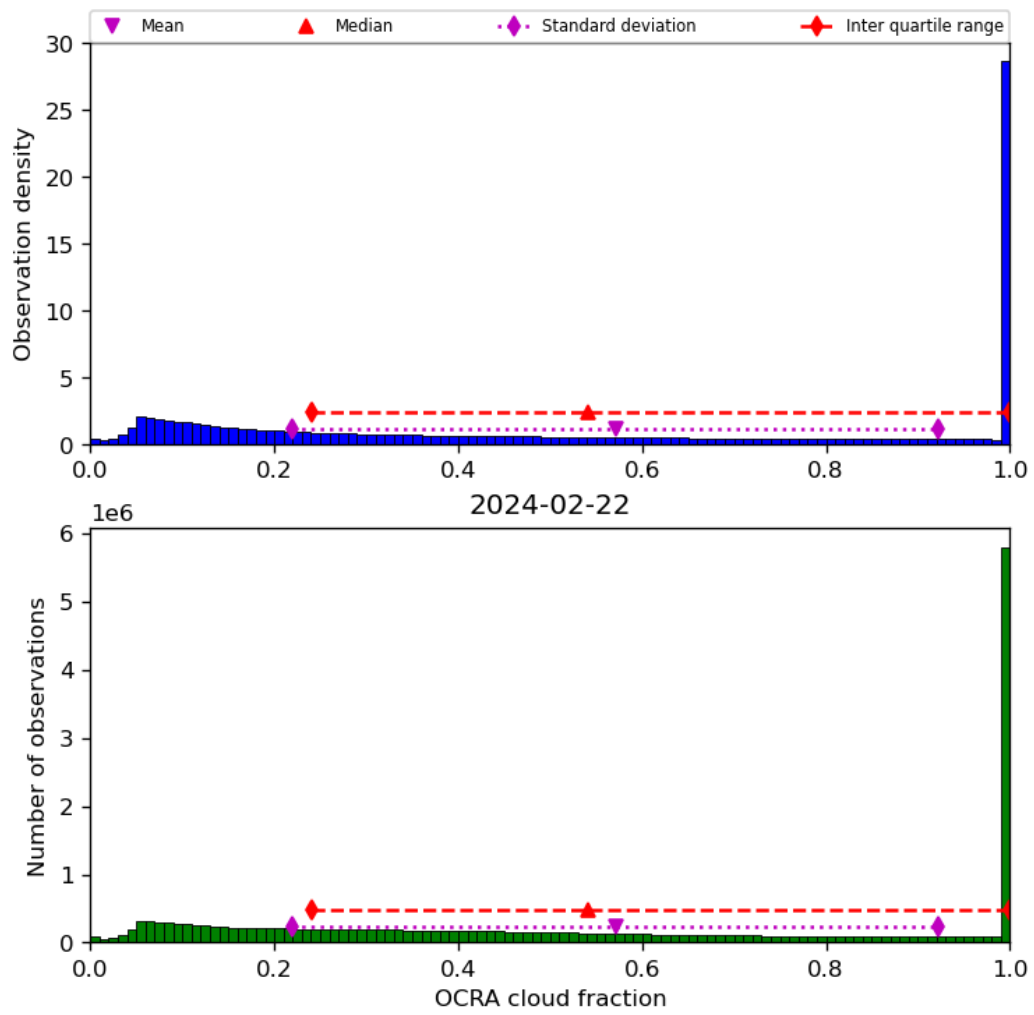
Figure 50: Histogram of “OCRA cloud fraction” for 2024-02-22 to 2024-02-23
