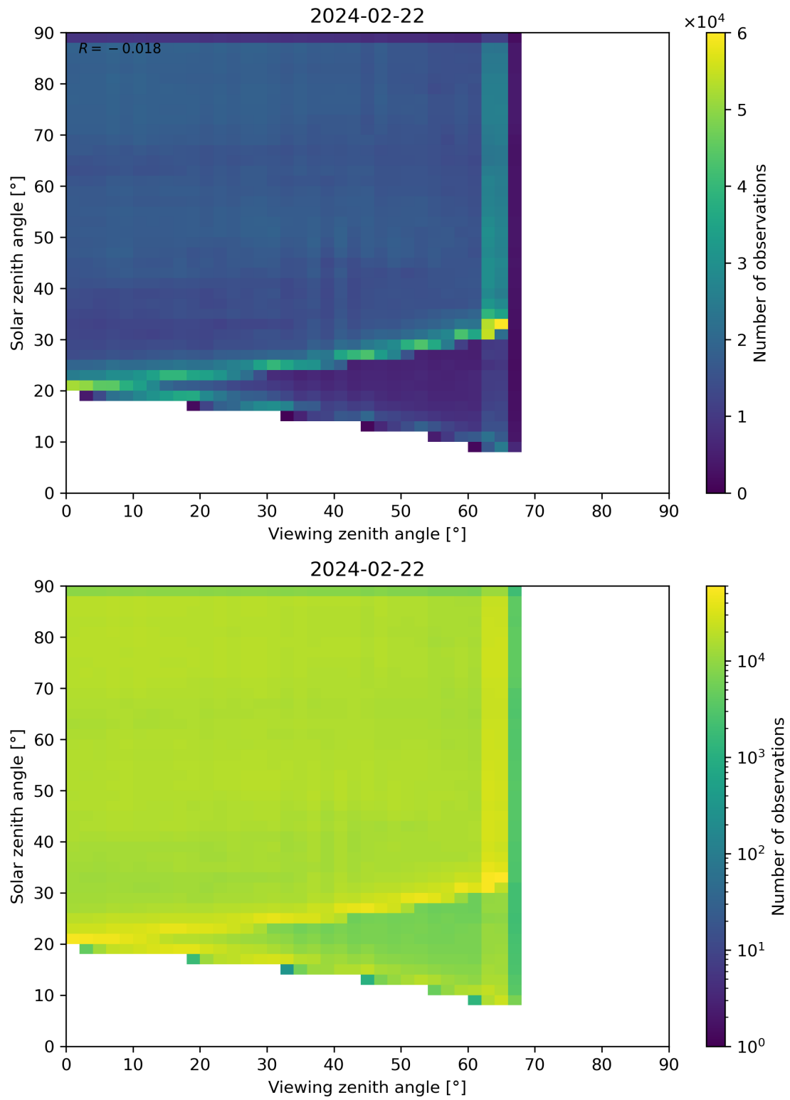
Figure 114: Scatter density plot of “Viewing zenith angle” against “Solar zenith angle” for 2024-02-22 to 2024-02-23.
