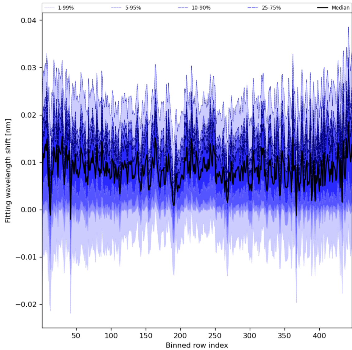
Figure 65: Along track statistics of “Fitting wavelength shift” for 2024-02-22 to 2024-02-23
