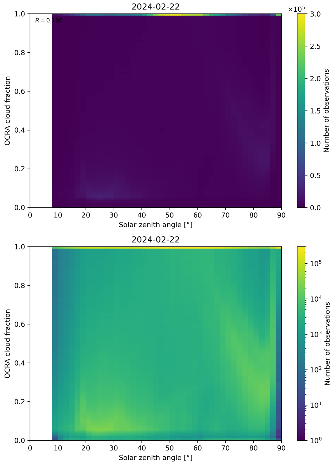
Figure 100: Scatter density plot of “Solar zenith angle” against “OCRA cloud fraction” for 2024-02-22 to 2024-02-23.
