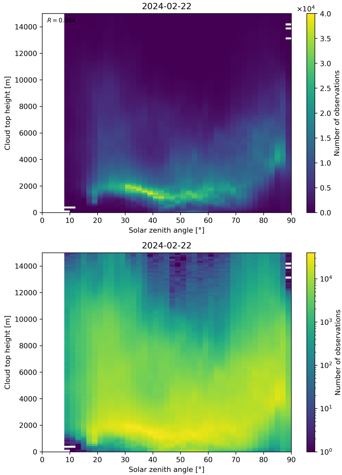
Figure 104: Scatter density plot of “Solar zenith angle” against “Cloud top height” for 2024-02-22 to 2024-02-23.
