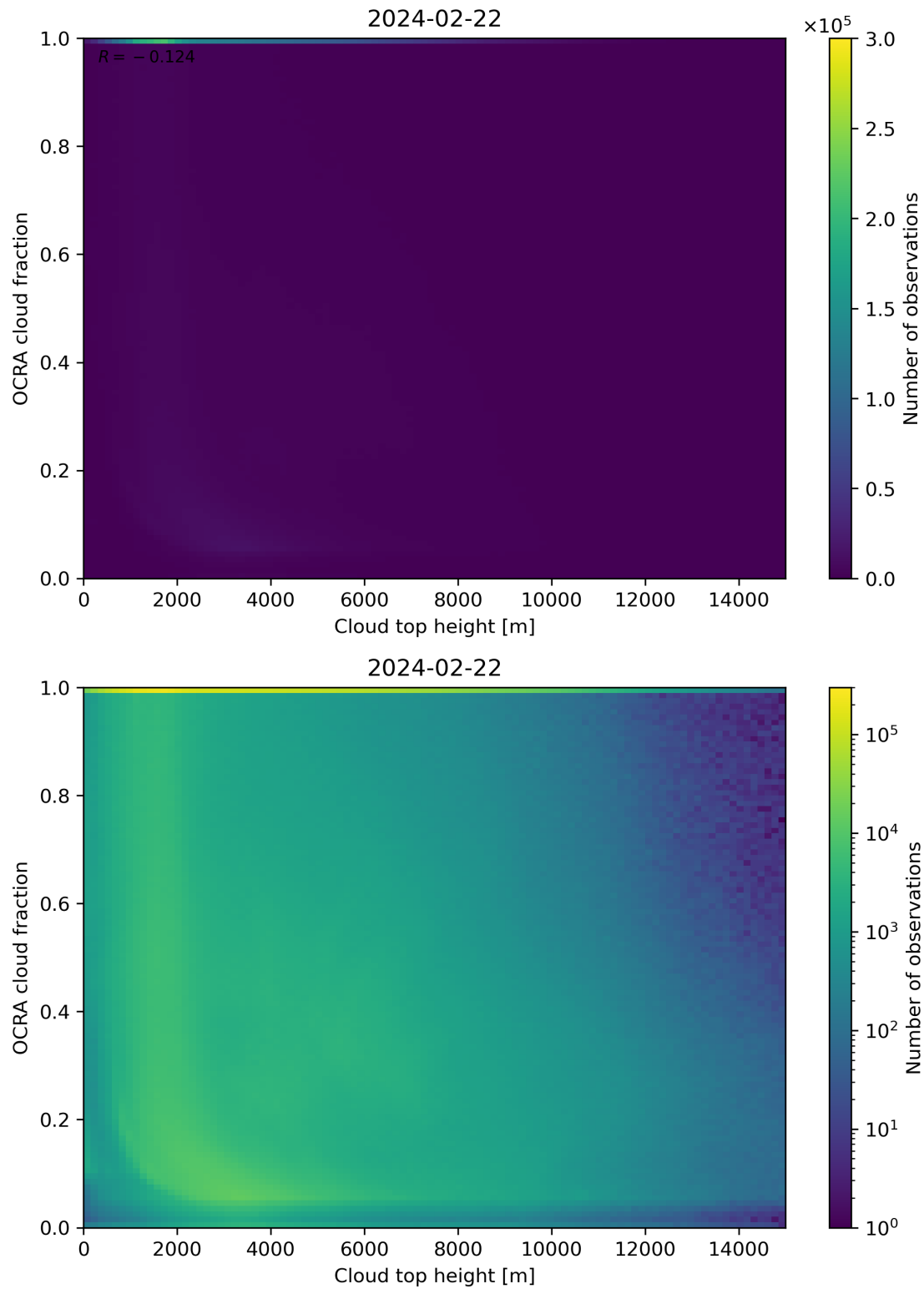
Figure 87: Scatter density plot of “Cloud top height” against “OCRA cloud fraction” for 2024-02-22 to 2024-02-23.
