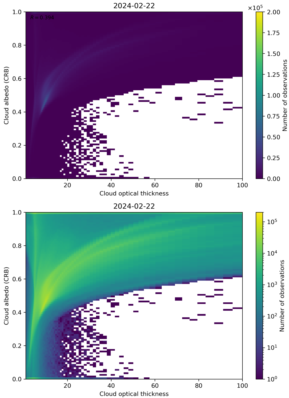
Figure 82: Scatter density plot of “Cloud optical thickness” against “Cloud albedo (CRB)” for 2024-02-22 to 2024-02-23.
