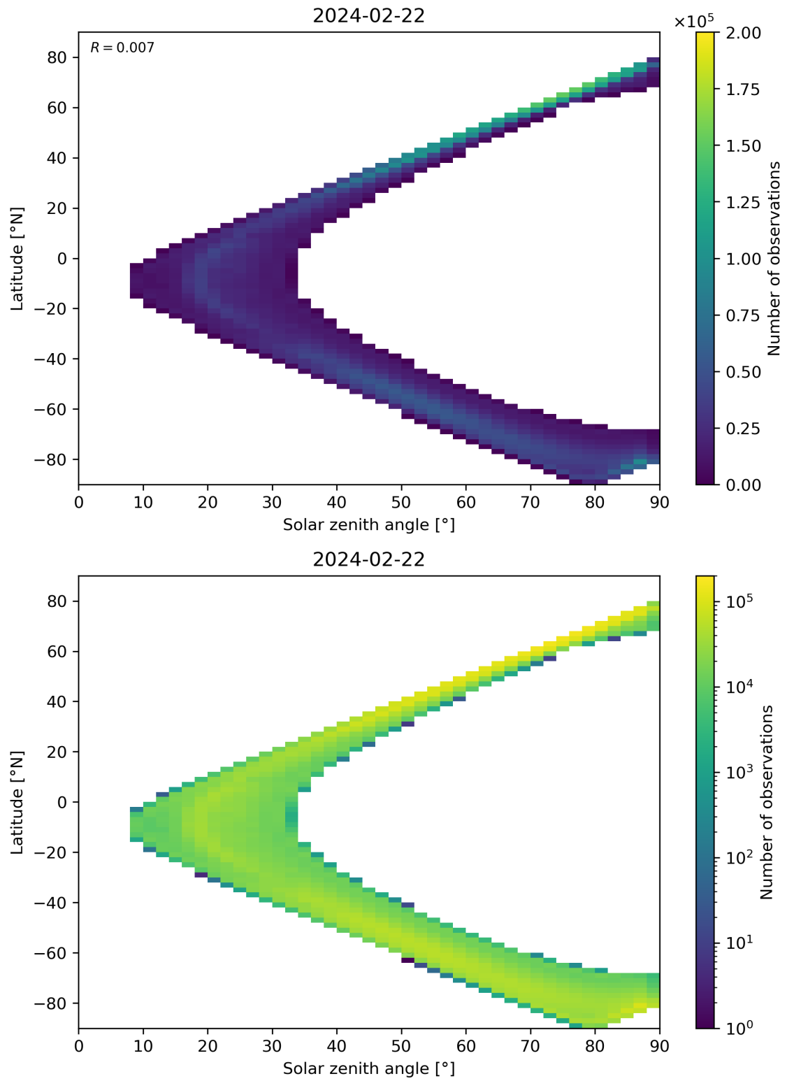
Figure 105: Scatter density plot of “Solar zenith angle” against “Latitude” for 2024-02-22 to 2024-02-23.
