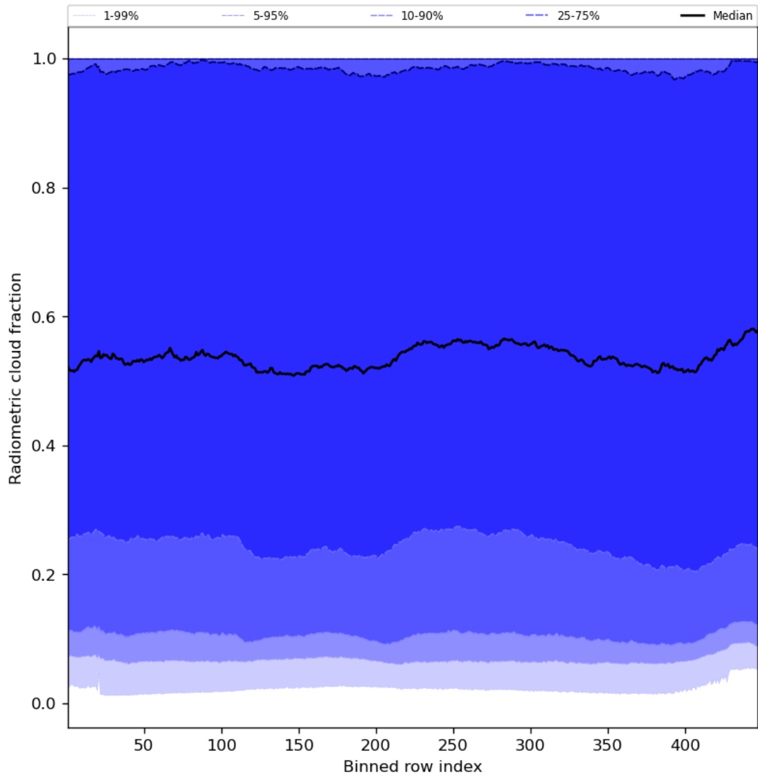
Figure 55: Along track statistics of “Radiometric cloud fraction” for 2024-02-22 to 2024-02-23
