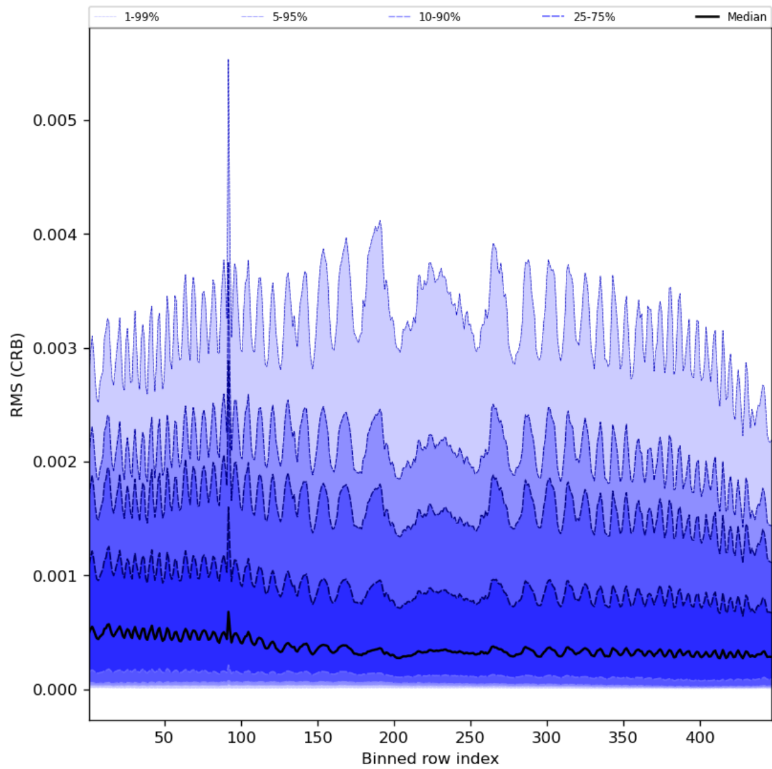
Figure 64: Along track statistics of “RMS (CRB)” for 2024-02-22 to 2024-02-23
