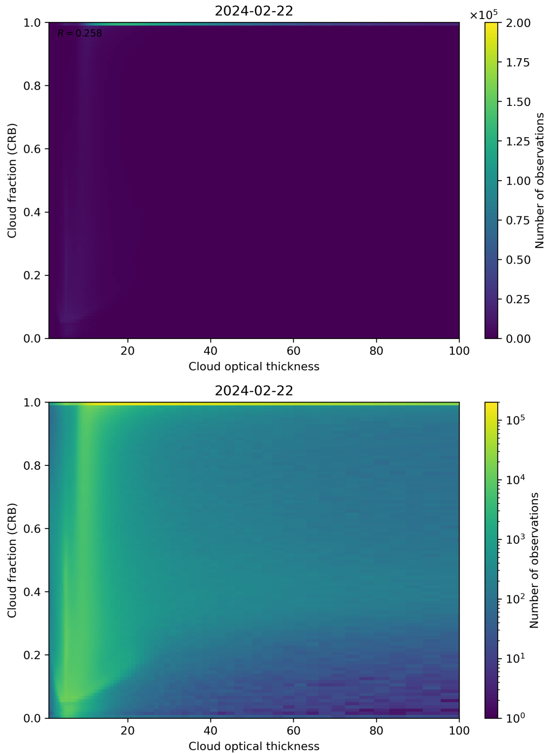
Figure 84: Scatter density plot of “Cloud optical thickness” against “Cloud fraction (CRB)” for 2024-02-22 to 2024-02-23.
