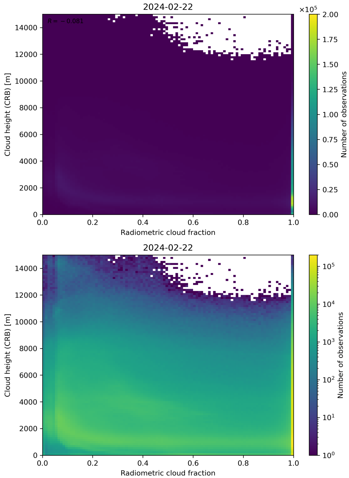
Figure 74: Scatter density plot of “Radiometric cloud fraction” against “Cloud height (CRB)” for 2024-02-22 to 2024-02-23.
