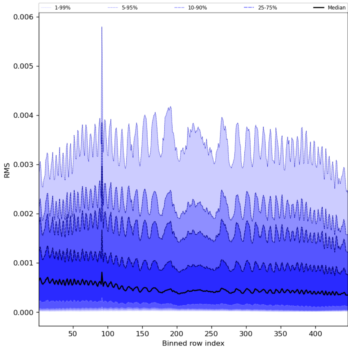
Figure 63: Along track statistics of “RMS” for 2024-02-22 to 2024-02-23
