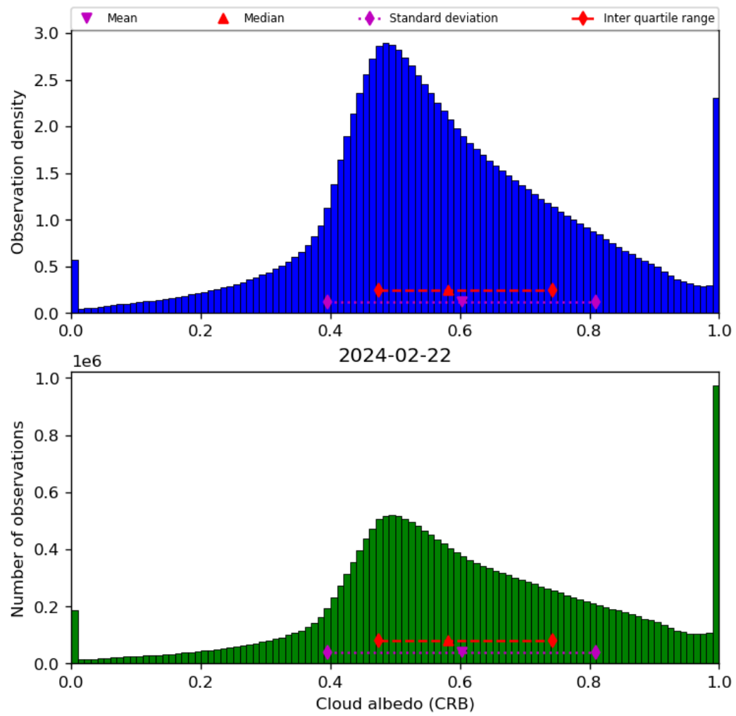
Figure 44: Histogram of “Cloud albedo (CRB)” for 2024-02-22 to 2024-02-23
