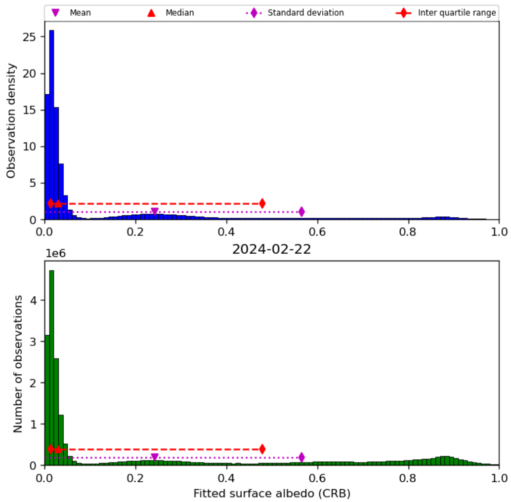
Figure 46: Histogram of “Fitted surface albedo (CRB)” for 2024-02-22 to 2024-02-23
