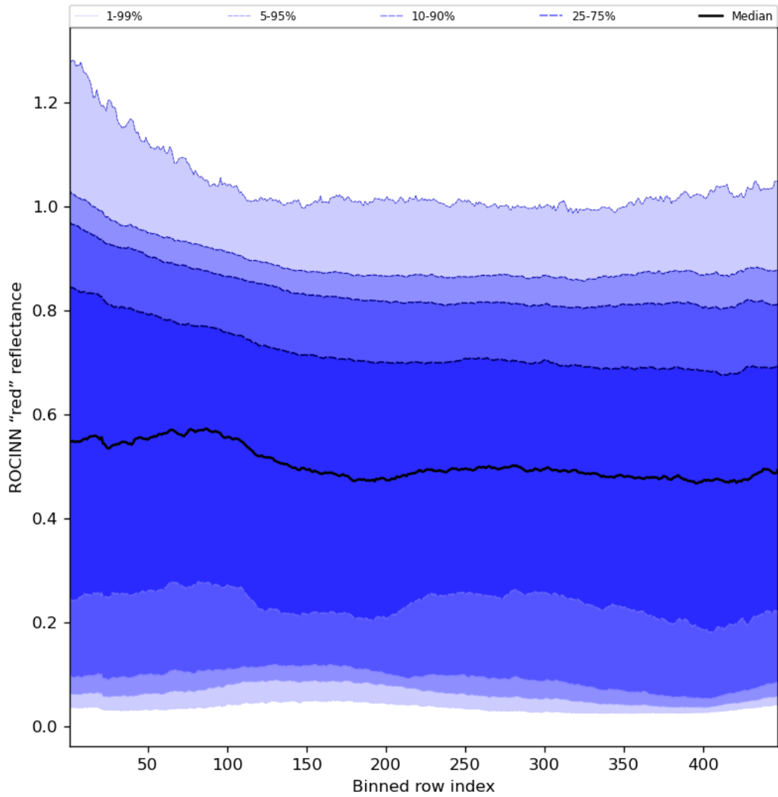
Figure 69: Along track statistics of “ROCINN “red” reflectance” for 2024-02-22 to 2024-02-23
