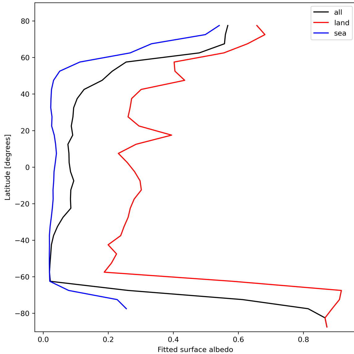
Figure 29: Zonal average of “Fitted surface albedo” for 2024-02-22 to 2024-02-23.
