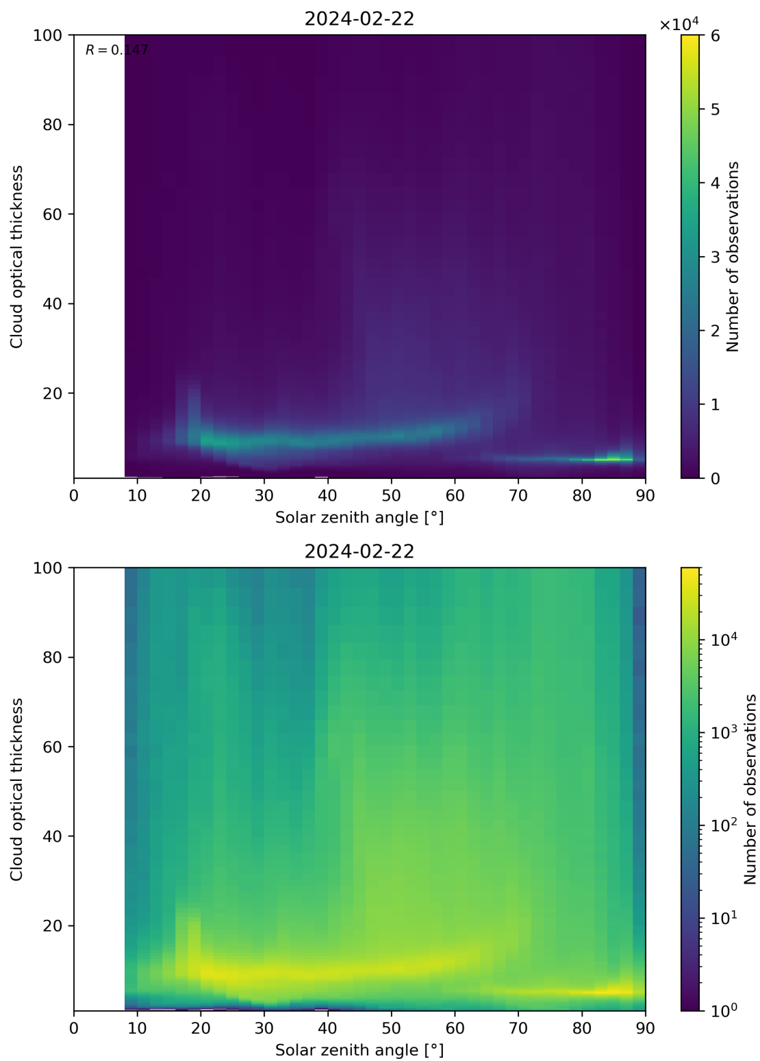
Figure 103: Scatter density plot of “Solar zenith angle” against “Cloud optical thickness” for 2024-02-22 to 2024-02-23.
