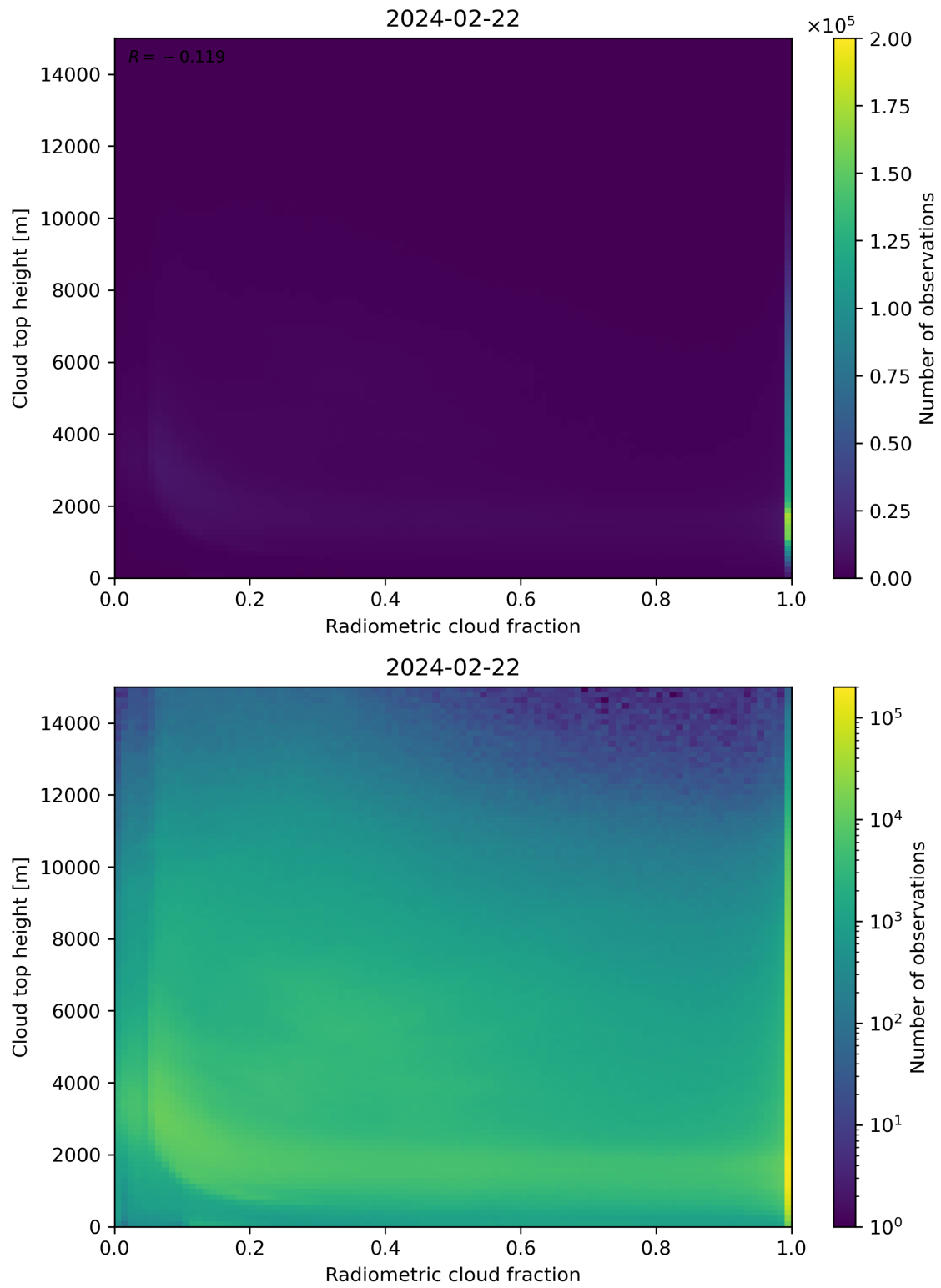
Figure 76: Scatter density plot of “Radiometric cloud fraction” against “Cloud top height” for 2024-02-22 to 2024-02-23.
