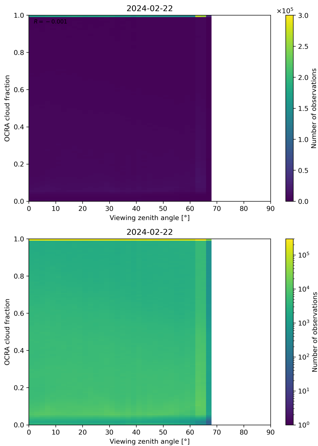
Figure 108: Scatter density plot of “Viewing zenith angle” against “OCRA cloud fraction” for 2024-02-22 to 2024-02-23.
