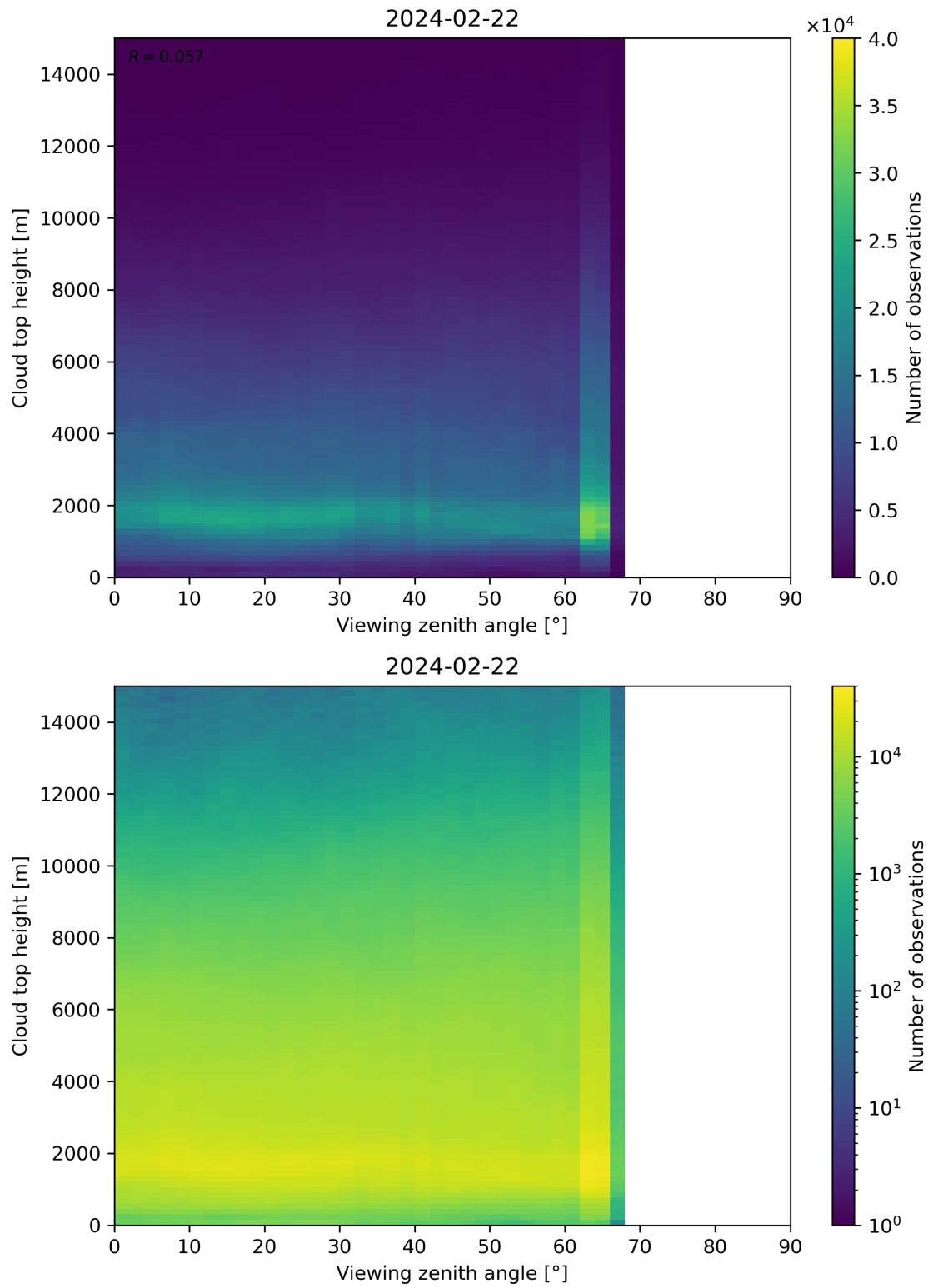
Figure 112: Scatter density plot of “Viewing zenith angle” against “Cloud top height” for 2024-02-22 to 2024-02-23.
