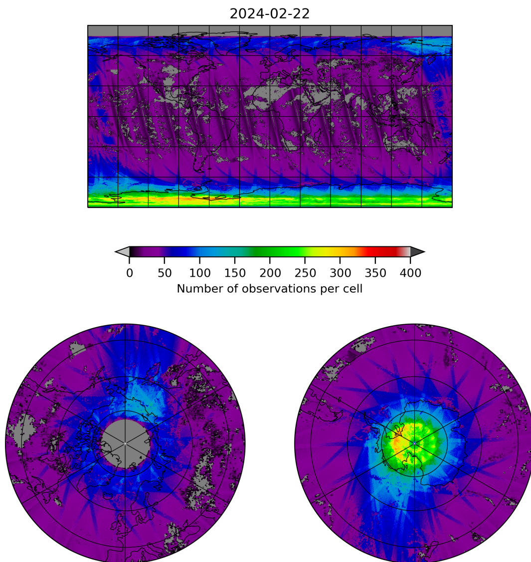
Figure 21: Map of the number of observations for 2024-02-22 to 2024-02-23
