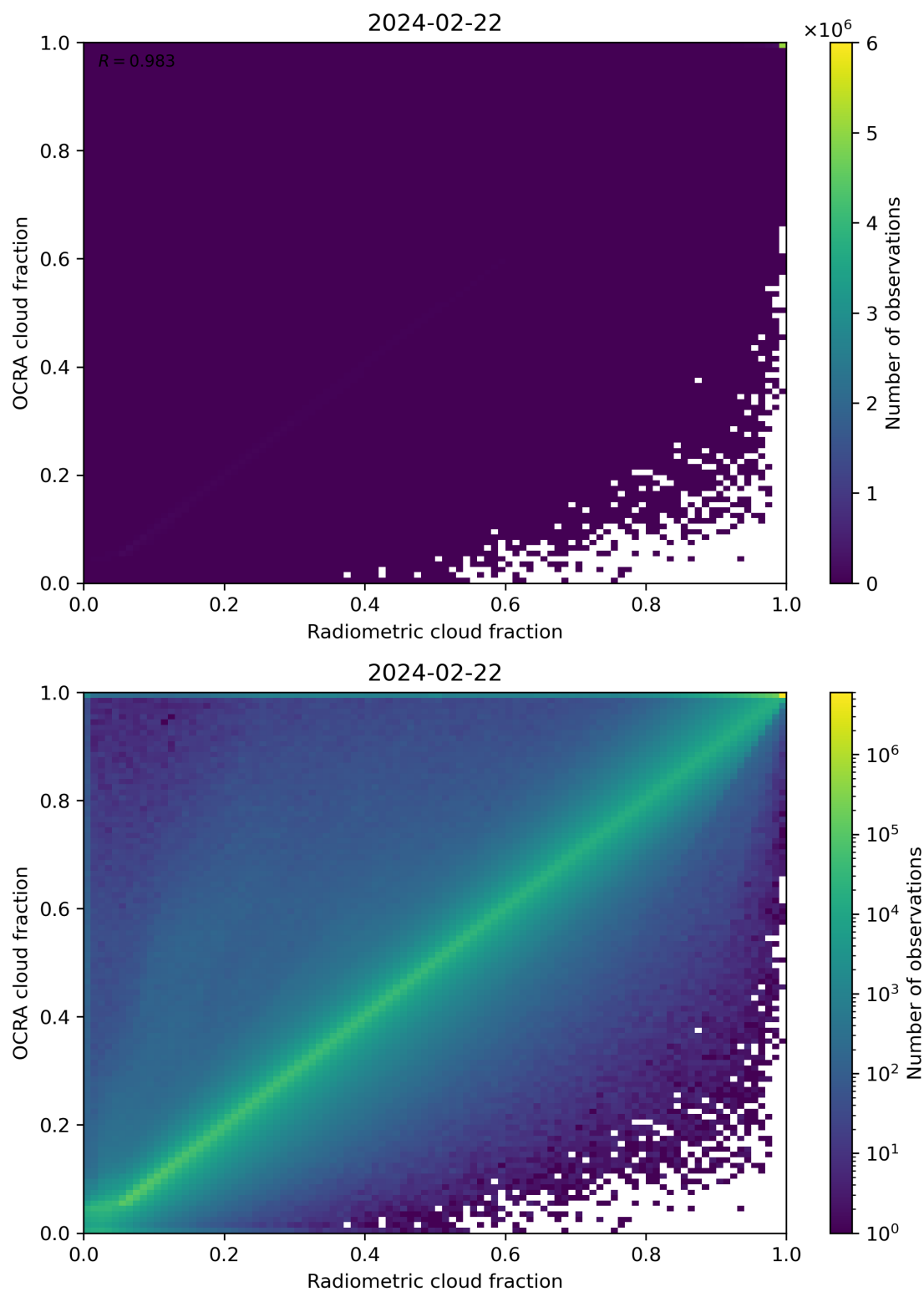
Figure 72: Scatter density plot of “Radiometric cloud fraction” against “OCRA cloud fraction” for 2024-02-22 to 2024-02-23.
