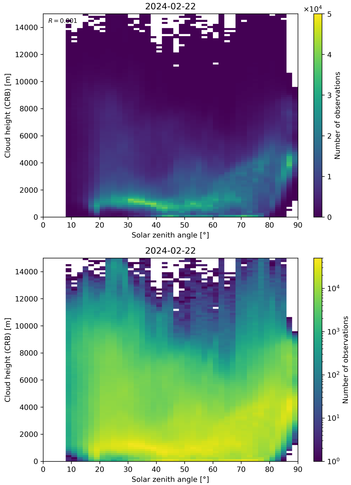
Figure 102: Scatter density plot of “Solar zenith angle” against “Cloud height (CRB)” for 2024-02-22 to 2024-02-23.
