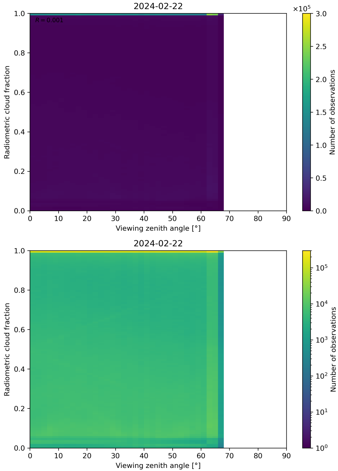
Figure 107: Scatter density plot of “Viewing zenith angle” against “Radiometric cloud fraction” for 2024-02-22 to 2024-02-23.
