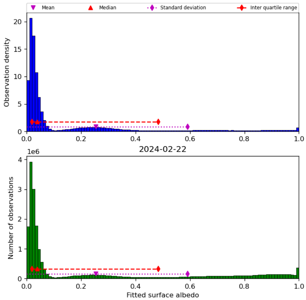
Figure 45: Histogram of “Fitted surface albedo” for 2024-02-22 to 2024-02-23
