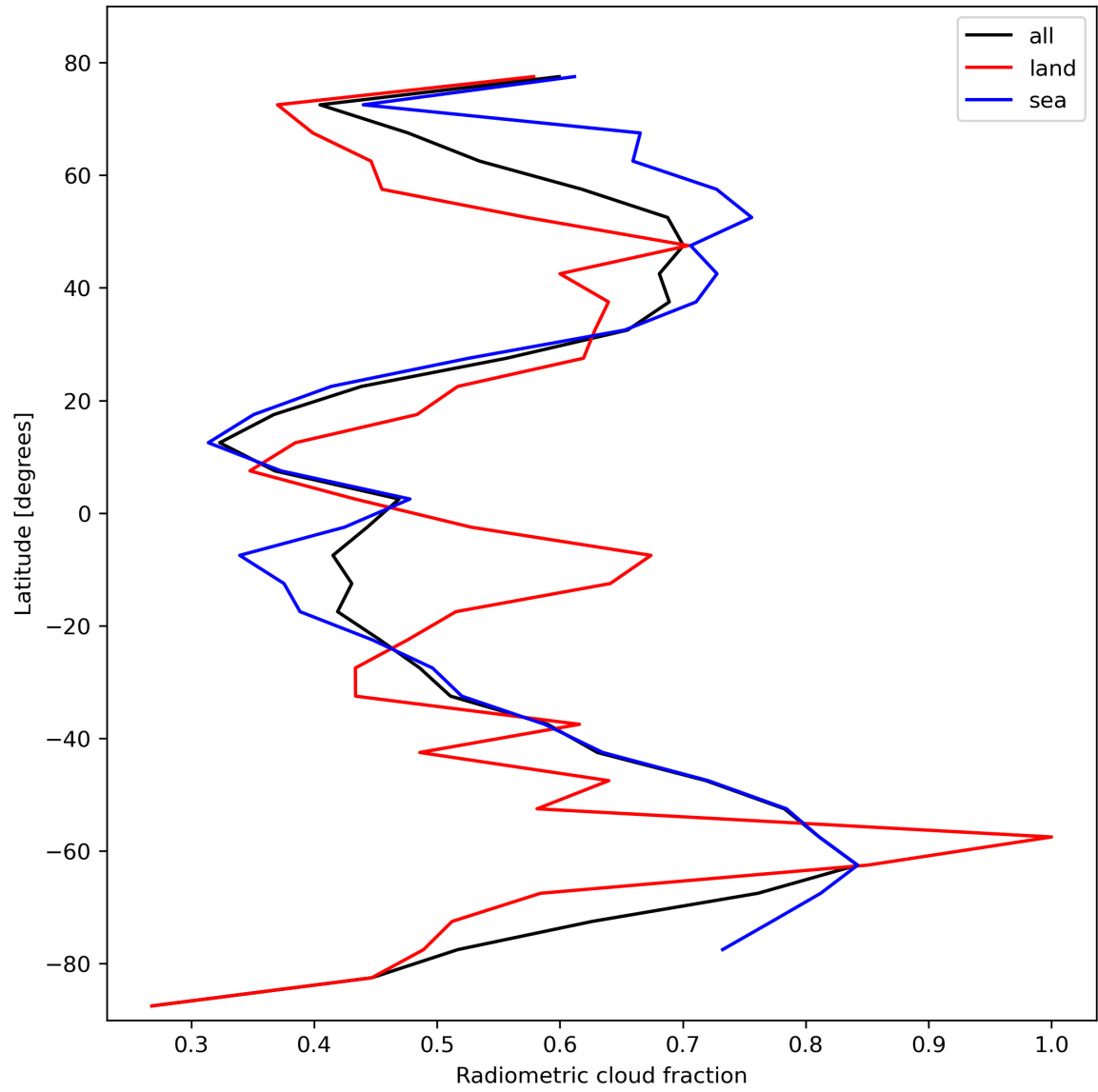
Figure 23: Zonal average of “Radiometric cloud fraction” for 2024-02-22 to 2024-02-23.
