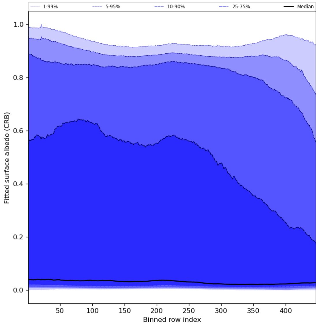
Figure 62: Along track statistics of “Fitted surface albedo (CRB)” for 2024-02-22 to 2024-02-23
