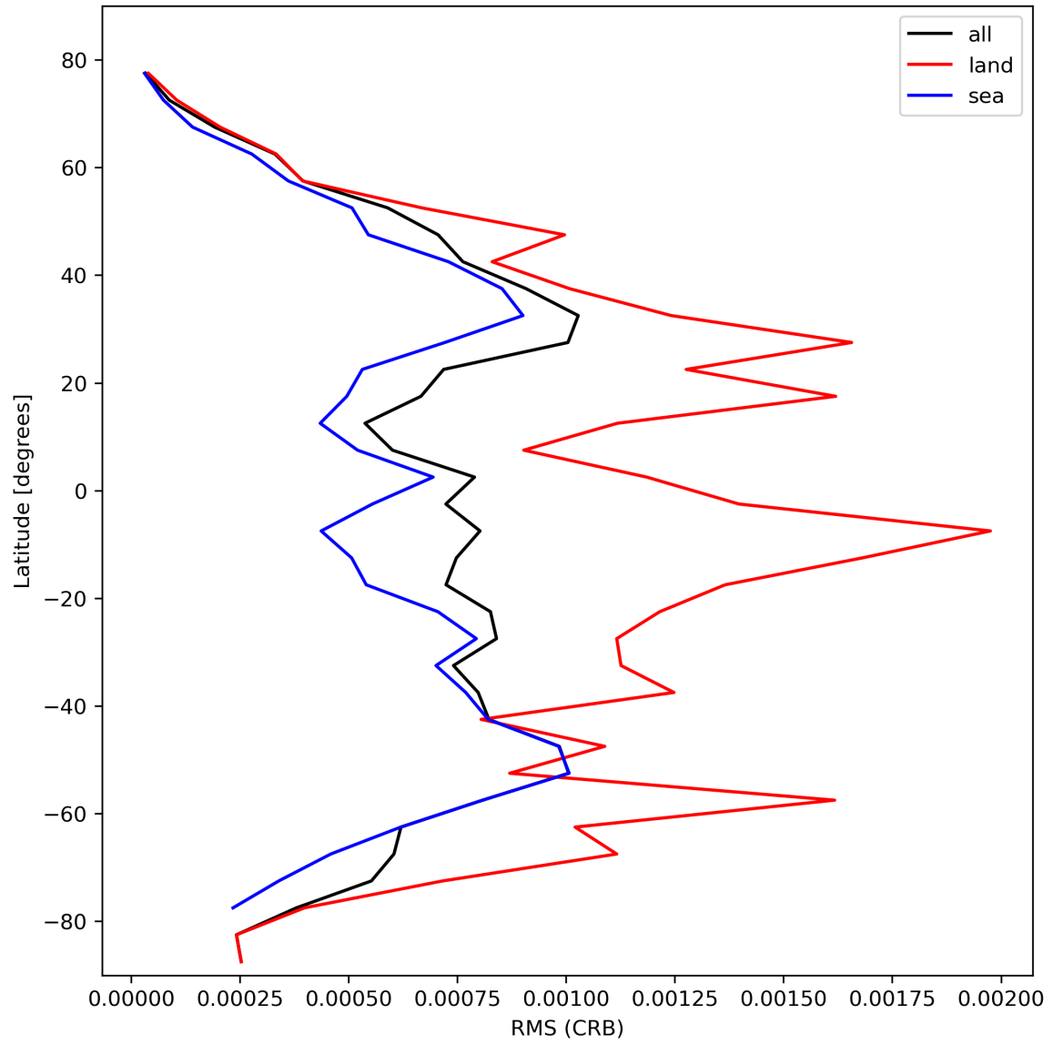
Figure 32: Zonal average of “RMS (CRB)” for 2024-02-22 to 2024-02-23.
