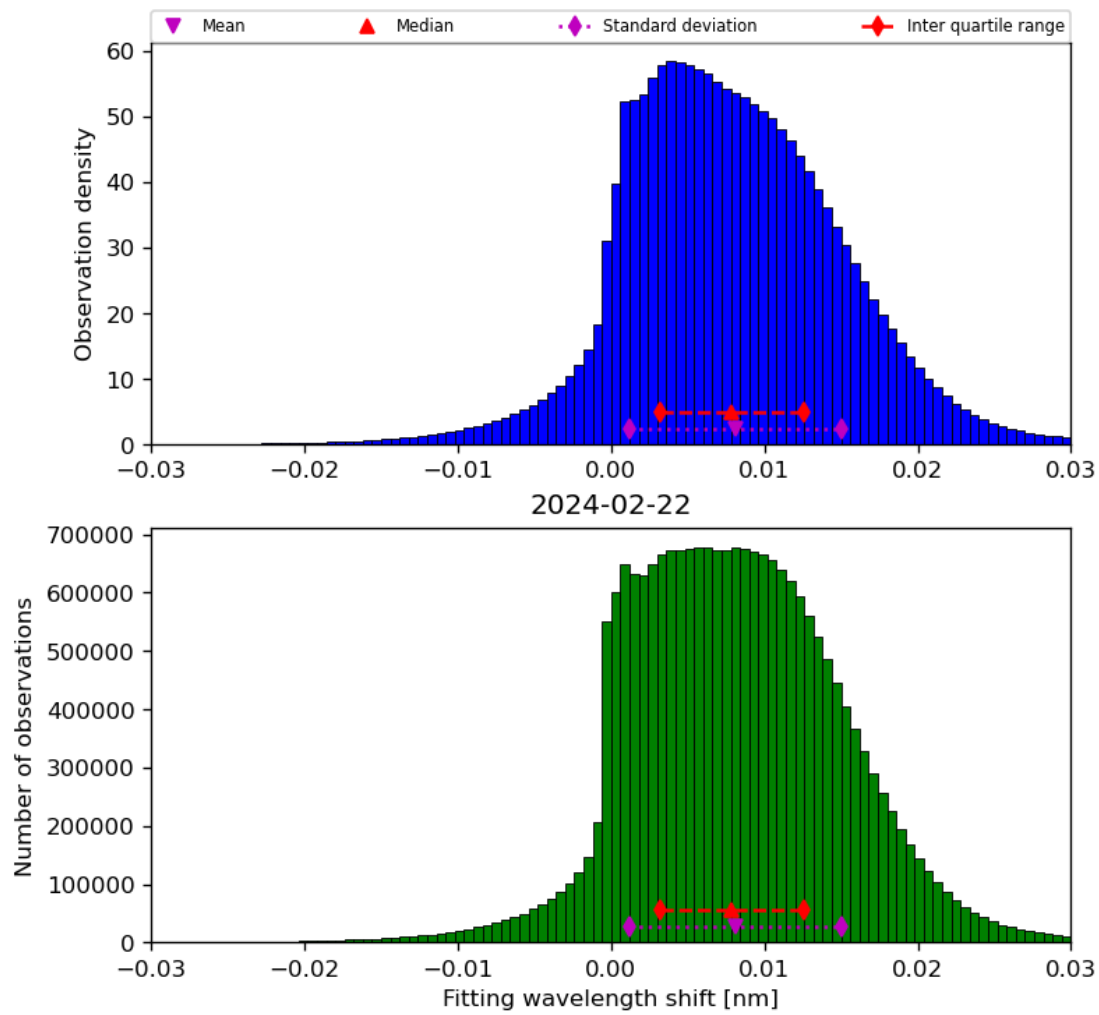
Figure 49: Histogram of “Fitting wavelength shift” for 2024-02-22 to 2024-02-23
