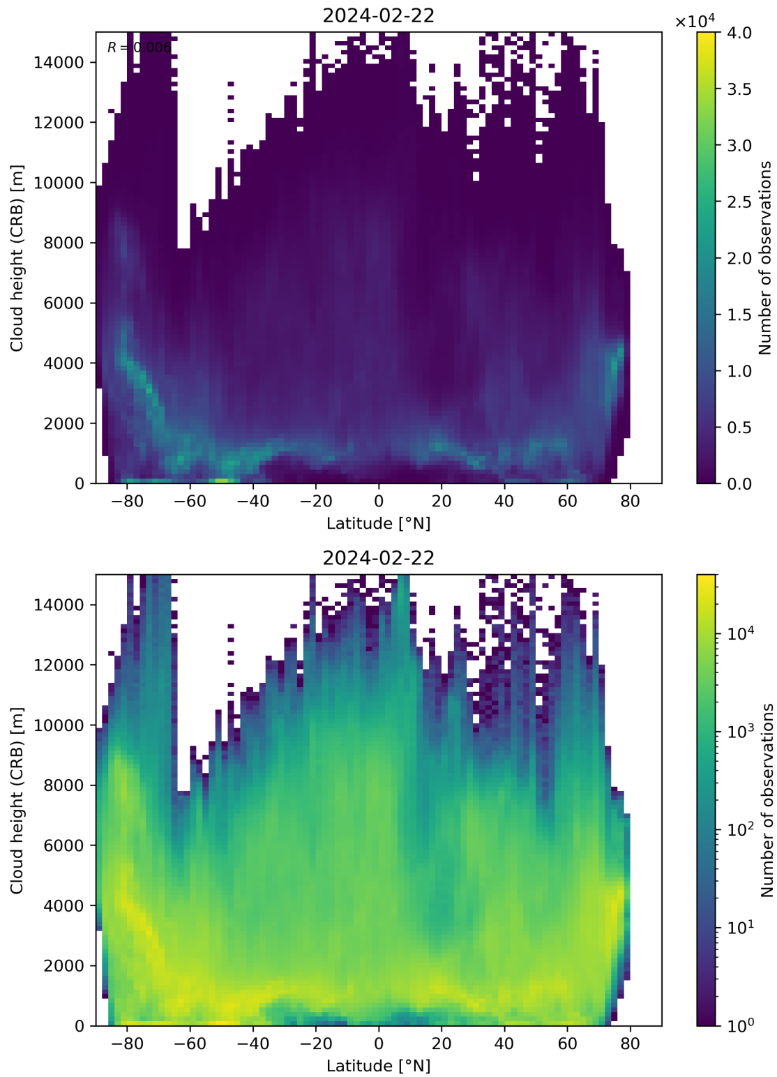
Figure 95: Scatter density plot of “Latitude” against “Cloud height (CRB)” for 2024-02-22 to 2024-02-23.
