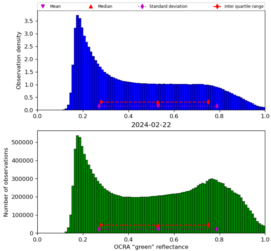
Figure 52: Histogram of “OCRA “green” reflectance” for 2024-02-22 to 2024-02-23
