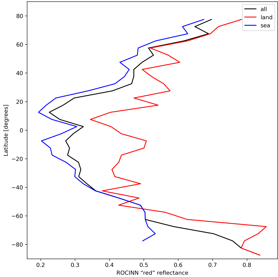
Figure 37: Zonal average of “ROCINN “red” reflectance” for 2024-02-22 to 2024-02-23.
