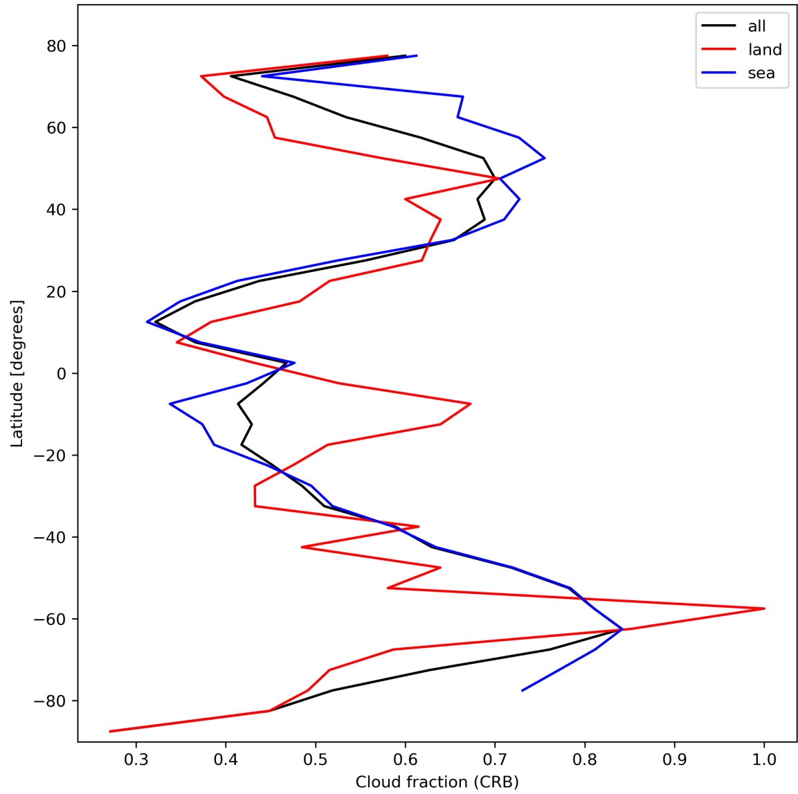
Figure 26: Zonal average of “Cloud fraction (CRB)” for 2024-02-22 to 2024-02-23.
