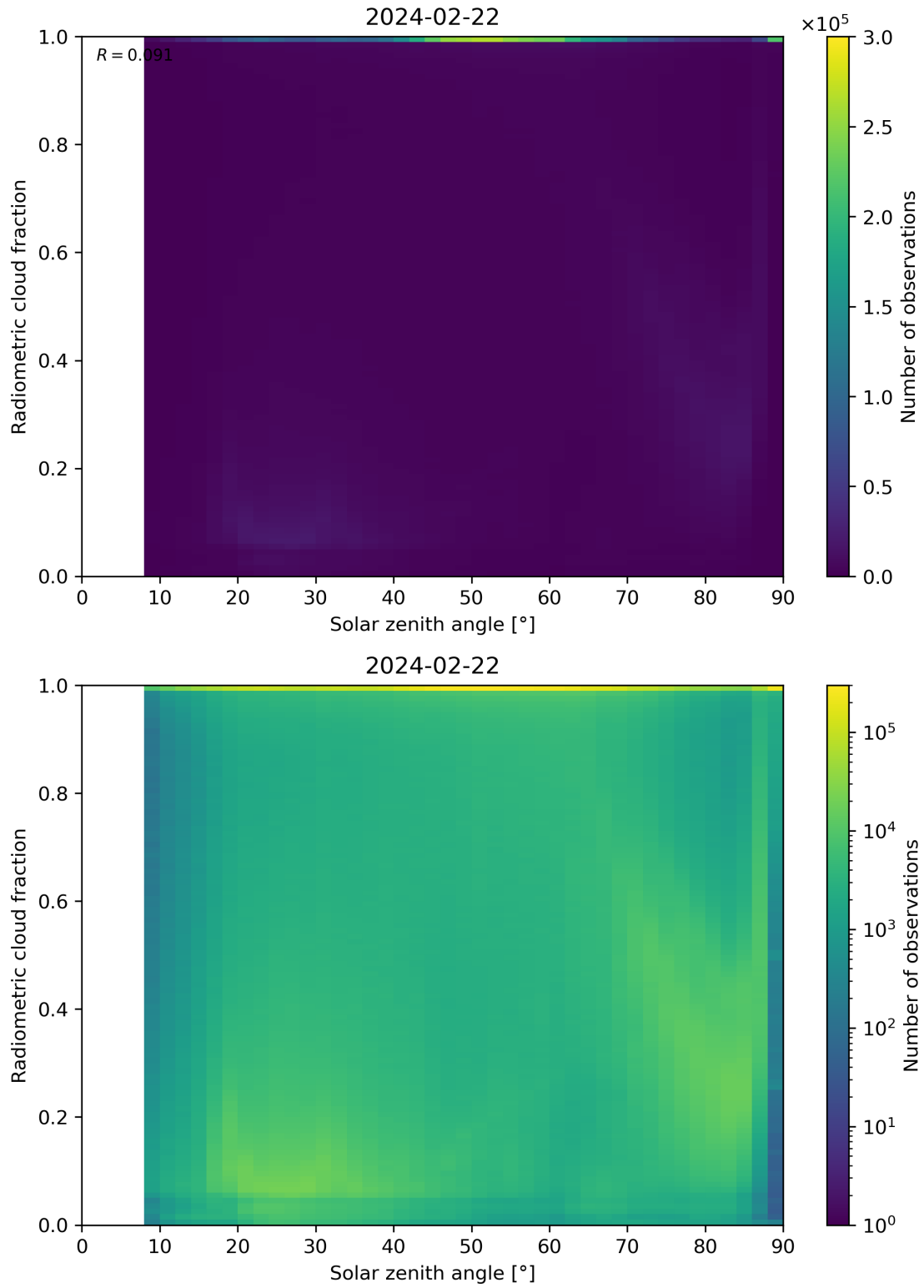
Figure 99: Scatter density plot of “Solar zenith angle” against “Radiometric cloud fraction” for 2024-02-22 to 2024-02-23.
