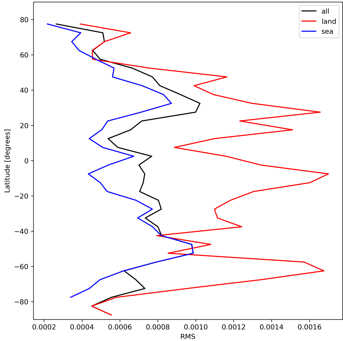
Figure 31: Zonal average of “RMS” for 2024-02-22 to 2024-02-23.
