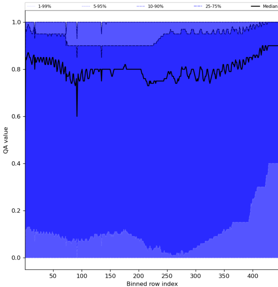
Figure 54: Along track statistics of “QA value” for 2024-02-22 to 2024-02-23
