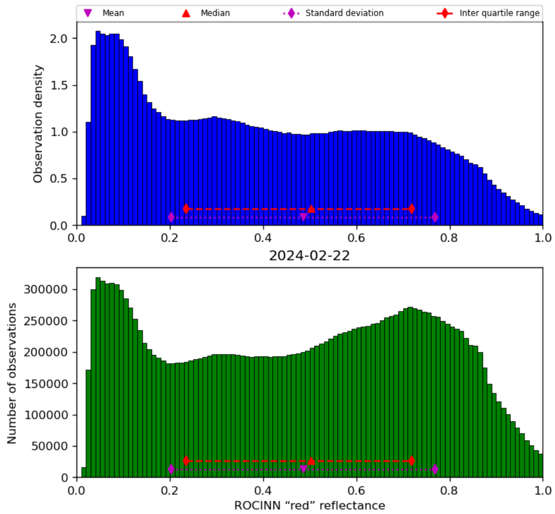
Figure 53: Histogram of “ROCINN “red” reflectance” for 2024-02-22 to 2024-02-23
