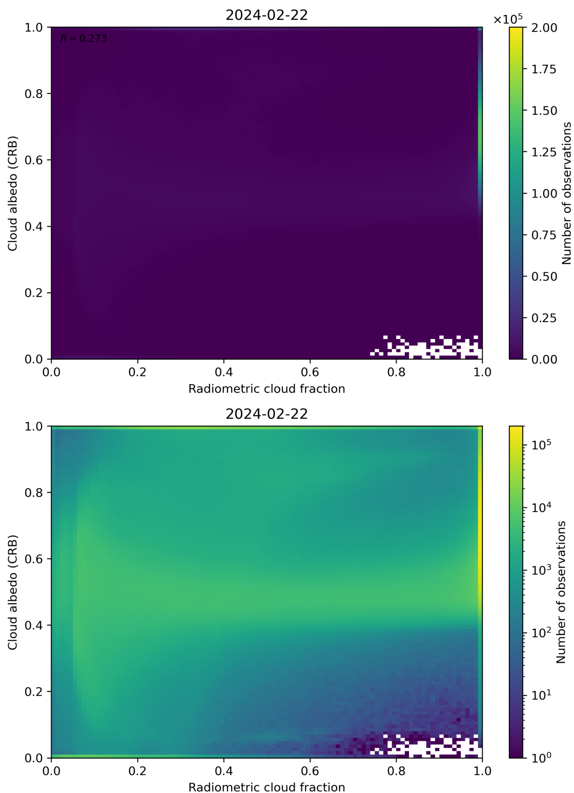
Figure 71: Scatter density plot of “Radiometric cloud fraction” against “Cloud albedo (CRB)” for 2024-02-22 to 2024-02-23.
