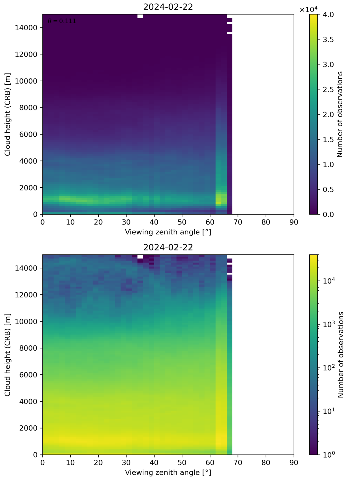
Figure 110: Scatter density plot of “Viewing zenith angle” against “Cloud height (CRB)” for 2024-02-22 to 2024-02-23.
