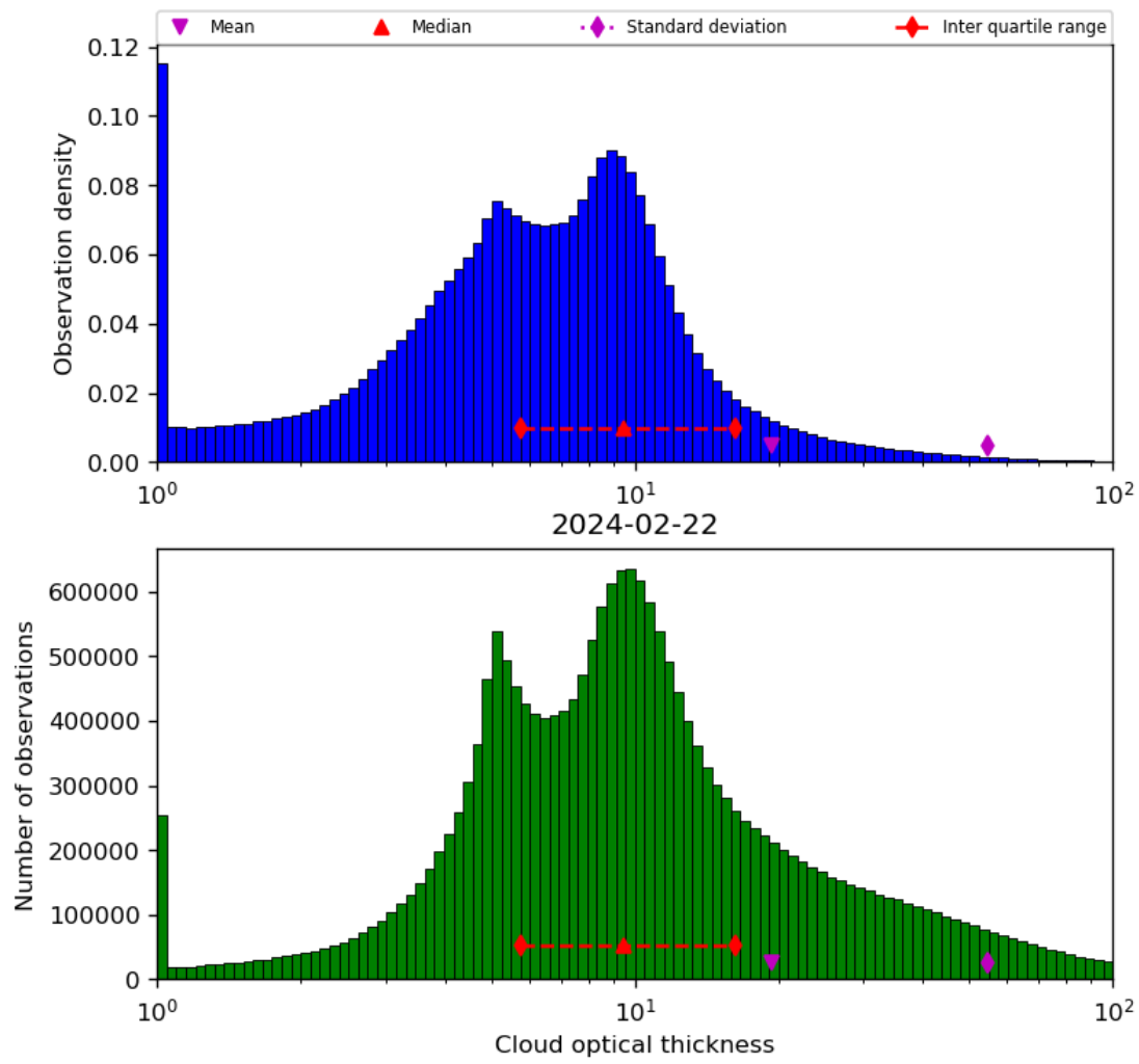
Figure 41: Histogram of “Cloud optical thickness” for 2024-02-22 to 2024-02-23
