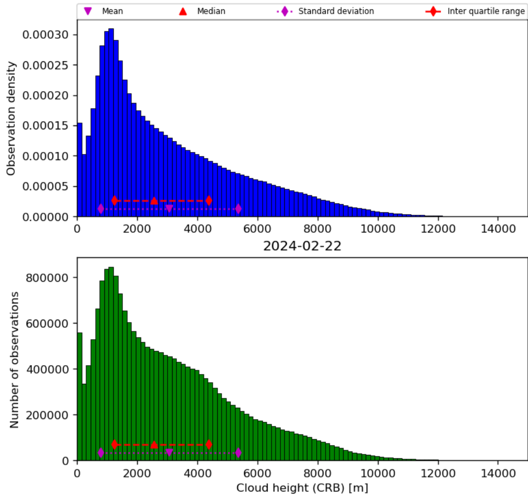
Figure 43: Histogram of “Cloud height (CRB)” for 2024-02-22 to 2024-02-23
