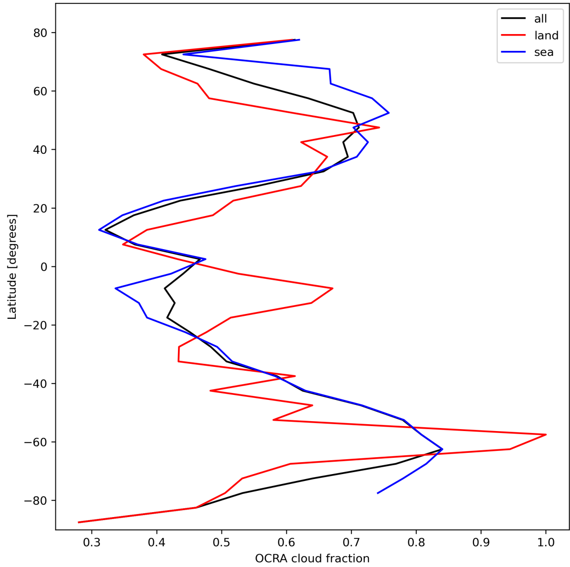
Figure 34: Zonal average of “OCRA cloud fraction” for 2024-02-22 to 2024-02-23.
