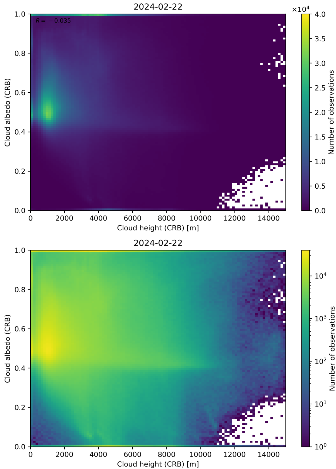
Figure 80: Scatter density plot of “Cloud height (CRB)” against “Cloud albedo (CRB)” for 2024-02-22 to 2024-02-23.
