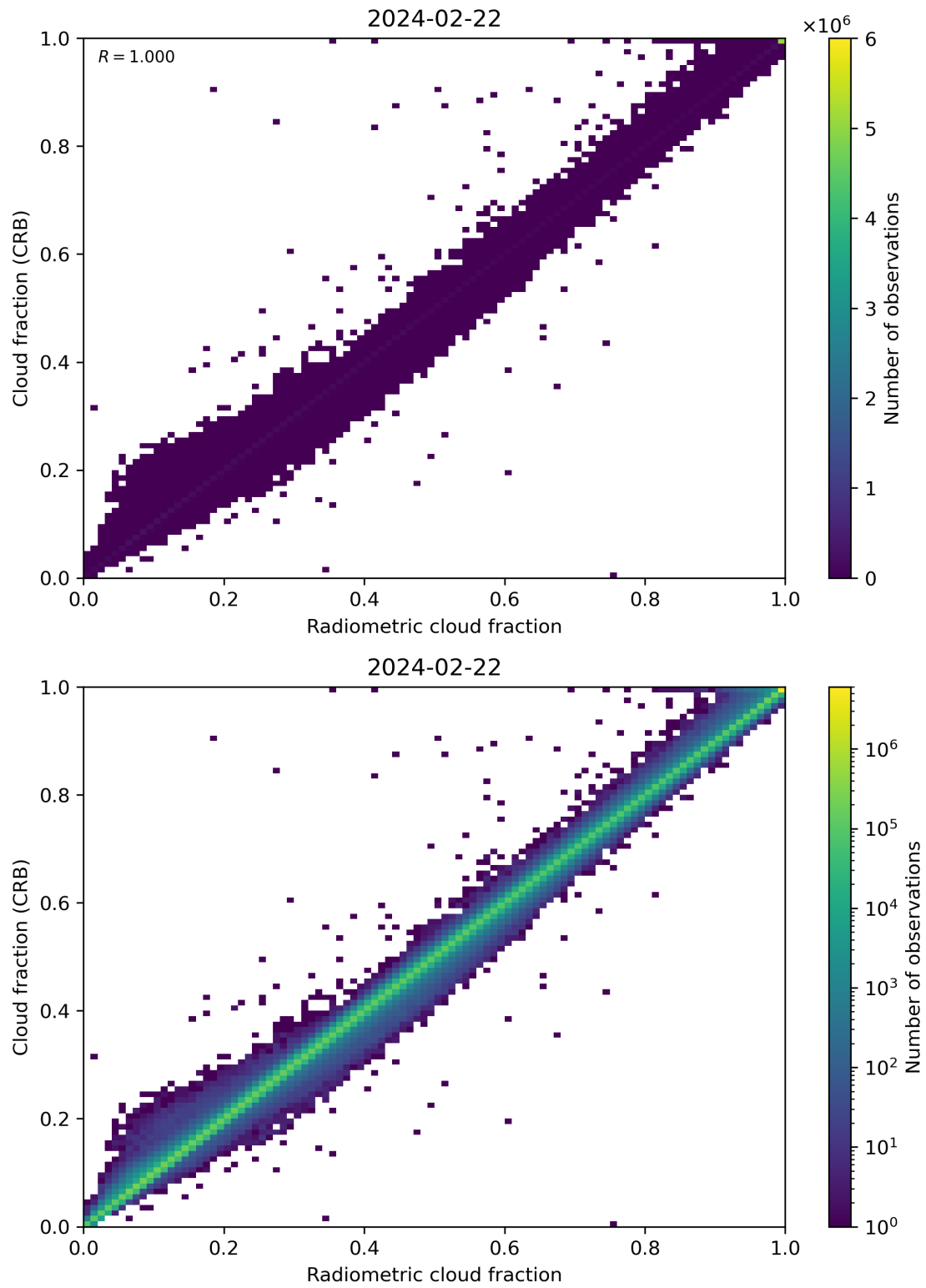
Figure 73: Scatter density plot of “Radiometric cloud fraction” against “Cloud fraction (CRB)” for 2024-02-22 to 2024-02-23.
