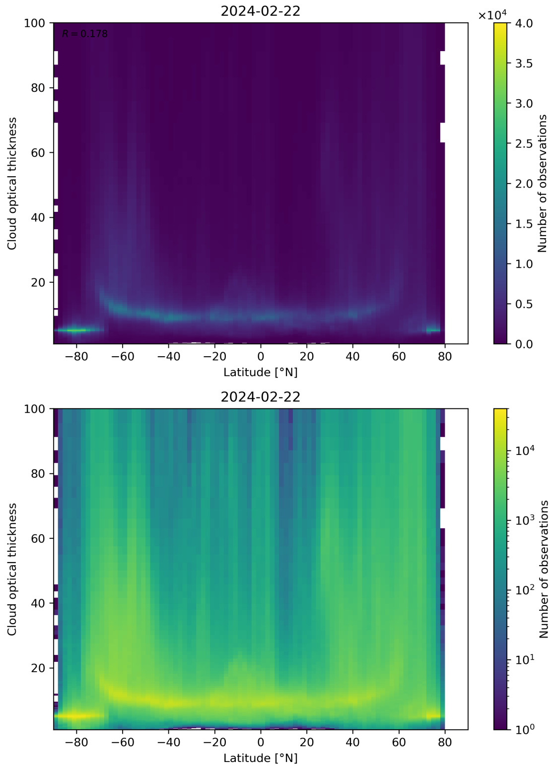
Figure 96: Scatter density plot of “Latitude” against “Cloud optical thickness” for 2024-02-22 to 2024-02-23.
