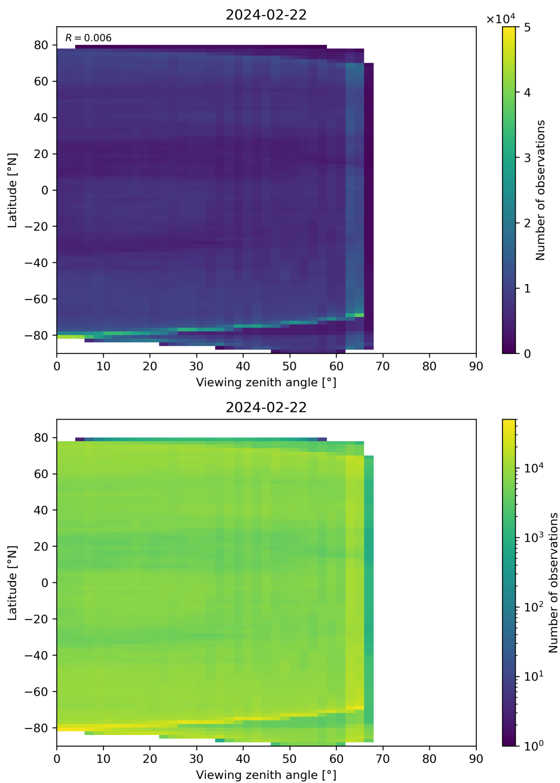
Figure 113: Scatter density plot of “Viewing zenith angle” against “Latitude” for 2024-02-22 to 2024-02-23.
