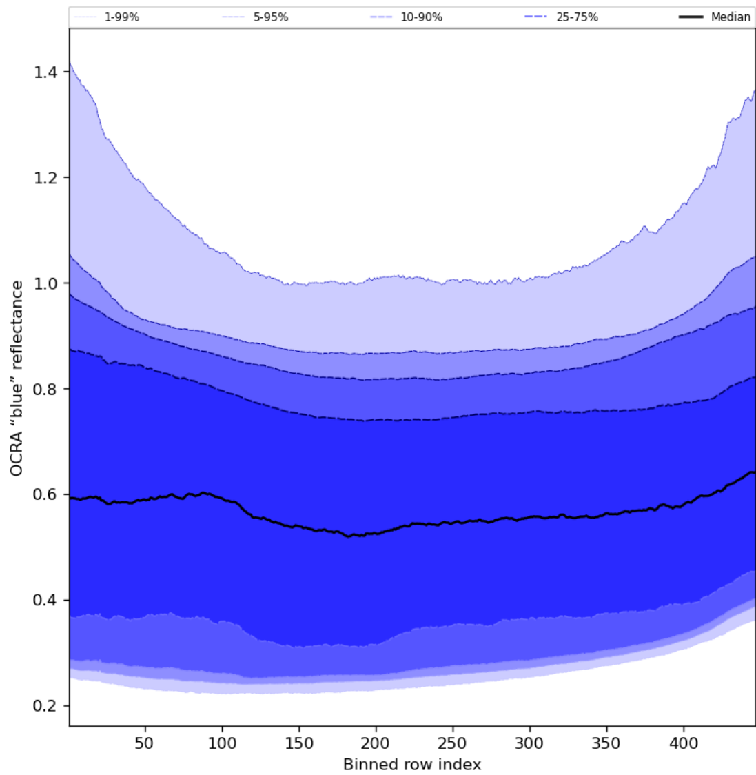
Figure 67: Along track statistics of “OCRA “blue” reflectance” for 2024-02-22 to 2024-02-23
