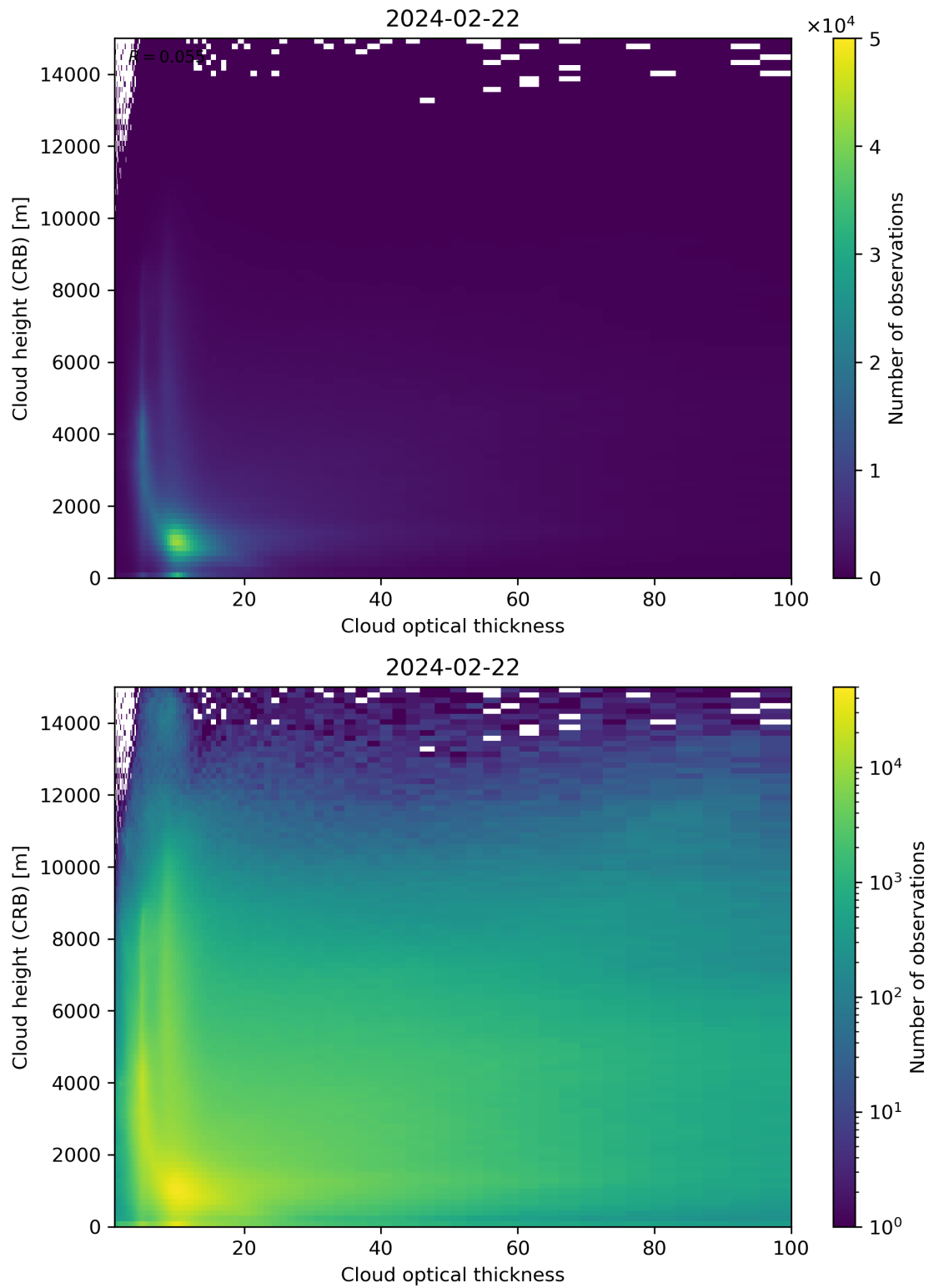
Figure 85: Scatter density plot of “Cloud optical thickness” against “Cloud height (CRB)” for 2024-02-22 to 2024-02-23.
