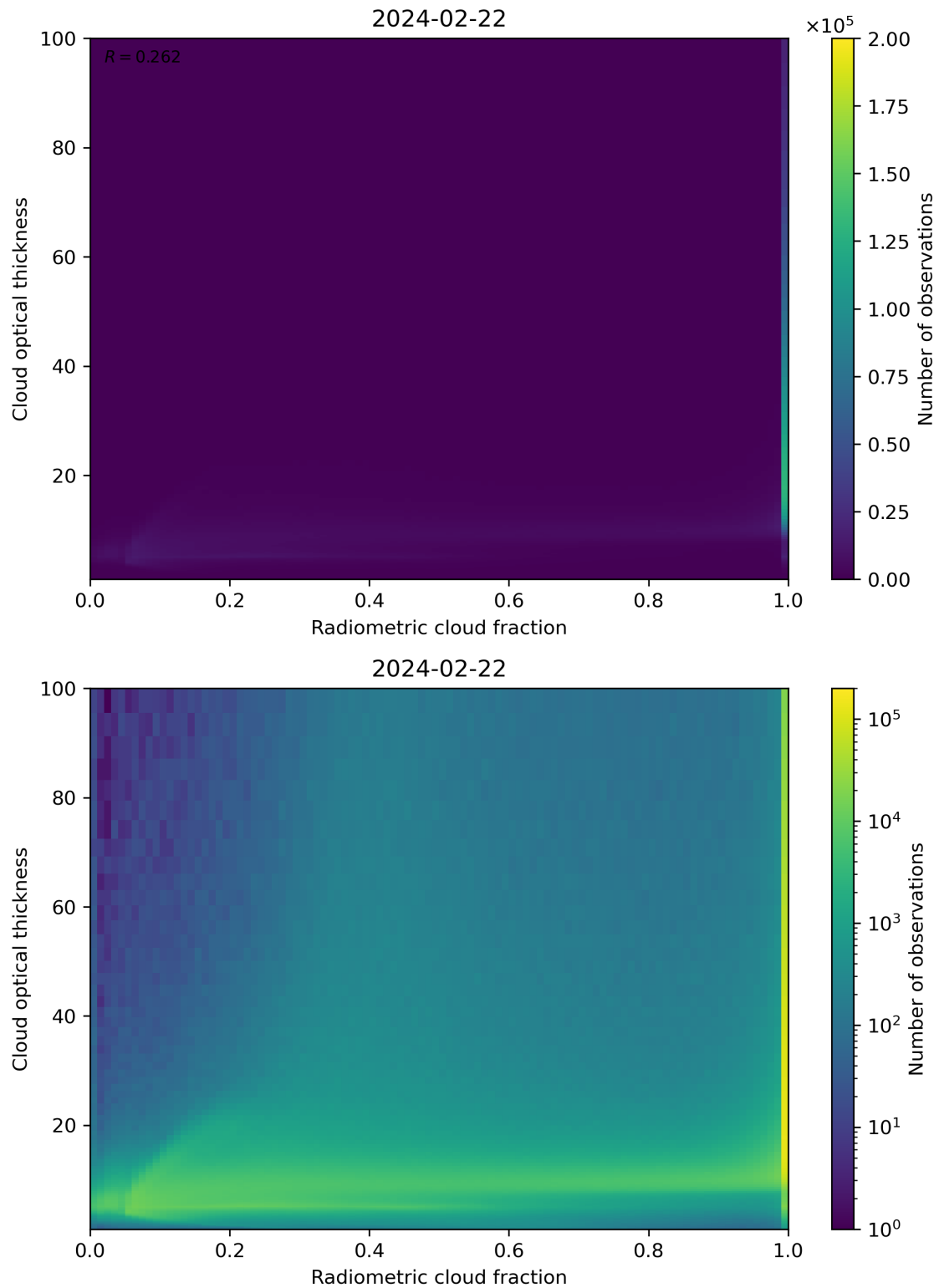
Figure 75: Scatter density plot of “Radiometric cloud fraction” against “Cloud optical thickness” for 2024-02-22 to 2024-02-23.
