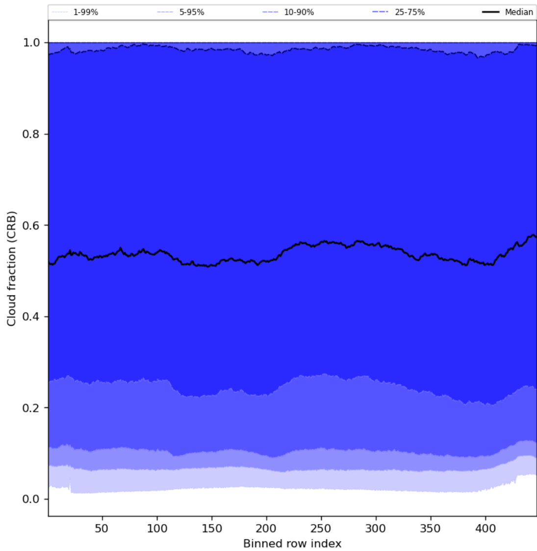
Figure 58: Along track statistics of “Cloud fraction (CRB)” for 2024-02-22 to 2024-02-23
