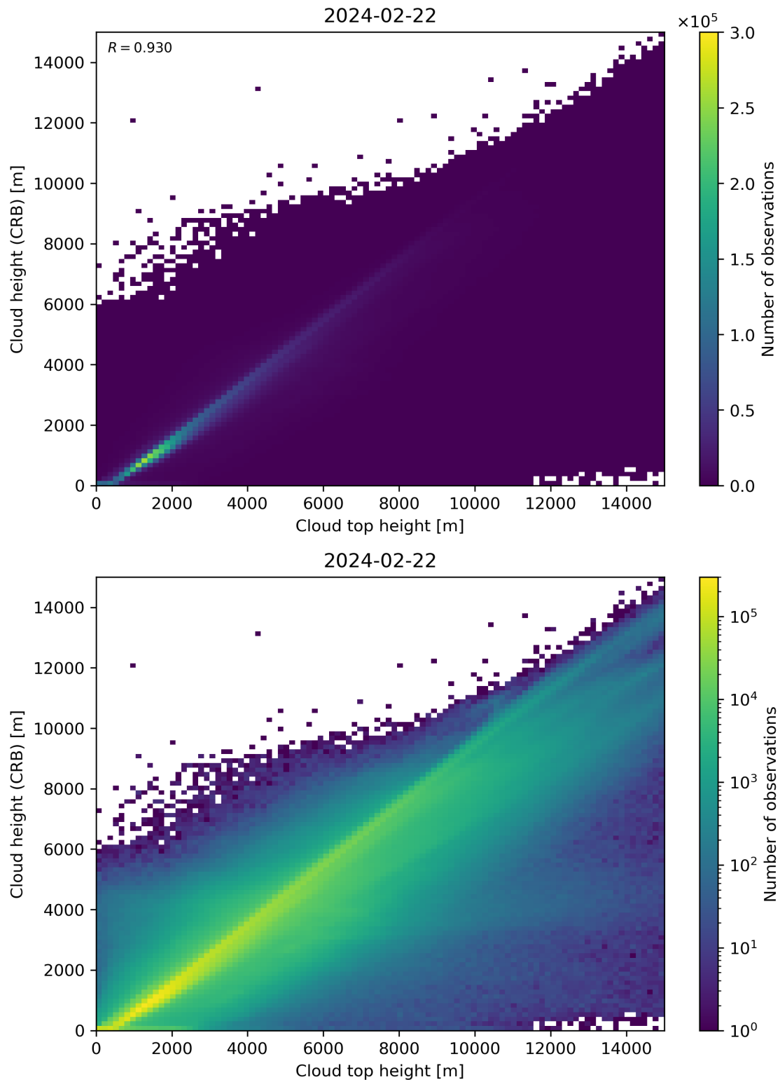
Figure 89: Scatter density plot of “Cloud top height” against “Cloud height (CRB)” for 2024-02-22 to 2024-02-23.
