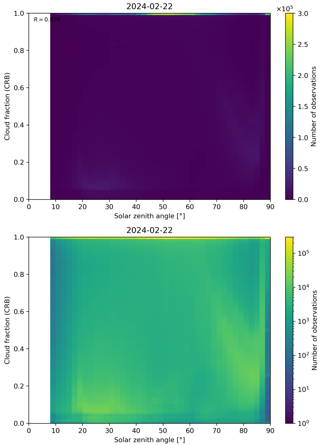
Figure 101: Scatter density plot of “Solar zenith angle” against “Cloud fraction (CRB)” for 2024-02-22 to 2024-02-23.
