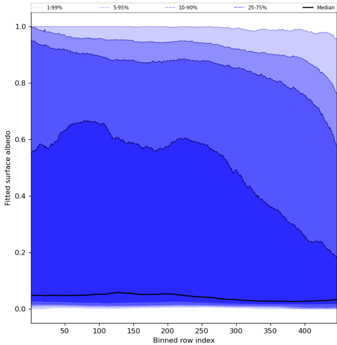
Figure 61: Along track statistics of “Fitted surface albedo” for 2024-02-22 to 2024-02-23
