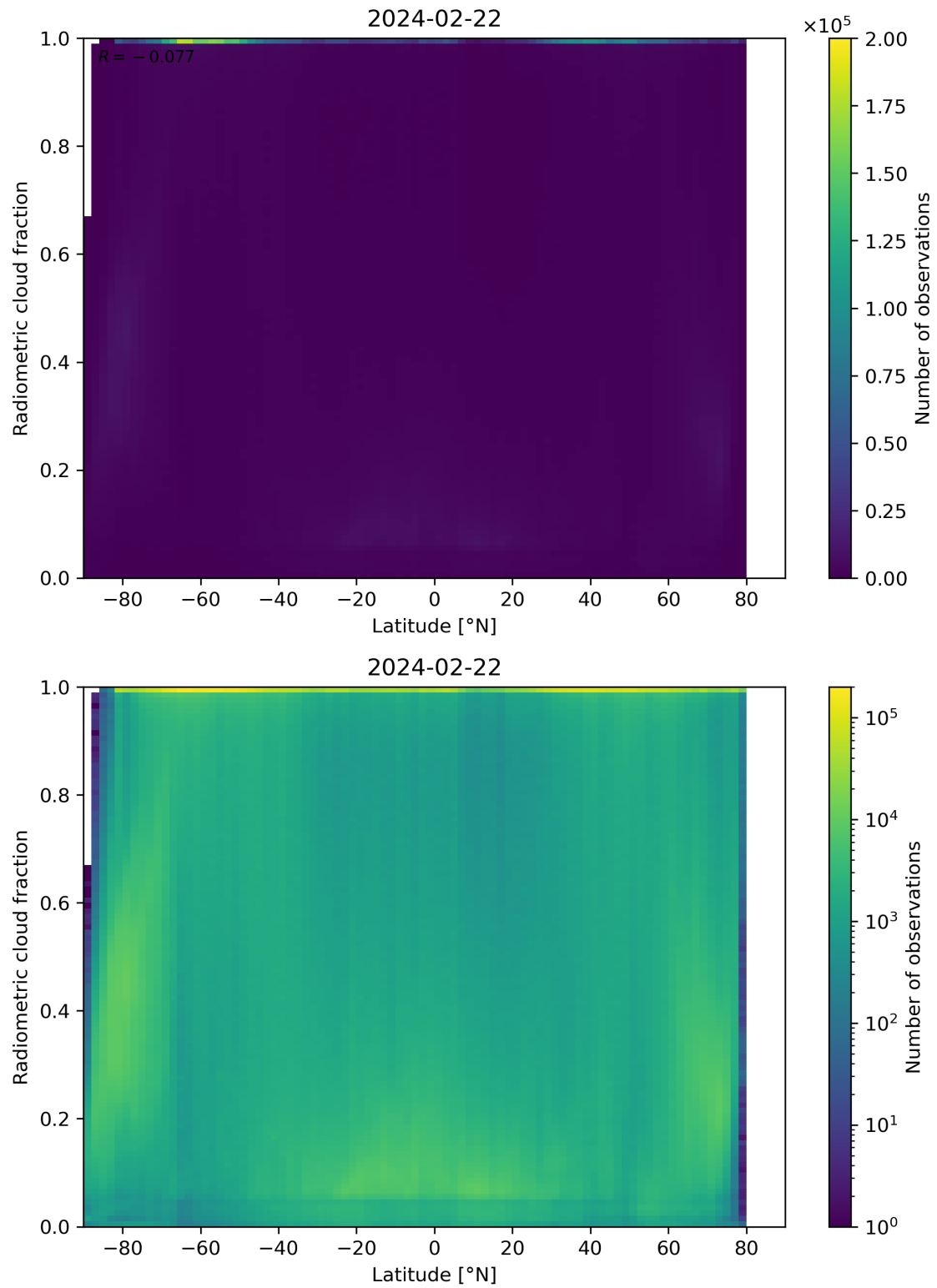
Figure 92: Scatter density plot of “Latitude” against “Radiometric cloud fraction” for 2024-02-22 to 2024-02-23.
