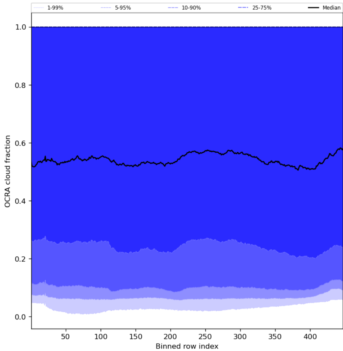
Figure 66: Along track statistics of “OCRA cloud fraction” for 2024-02-22 to 2024-02-23
