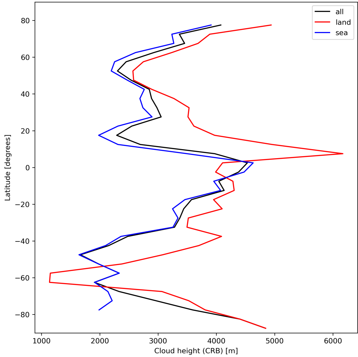
Figure 27: Zonal average of “Cloud height (CRB)” for 2024-02-22 to 2024-02-23.
