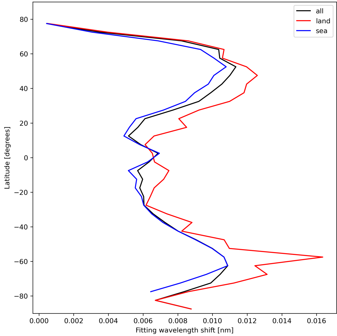
Figure 33: Zonal average of “Fitting wavelength shift” for 2024-02-22 to 2024-02-23.
