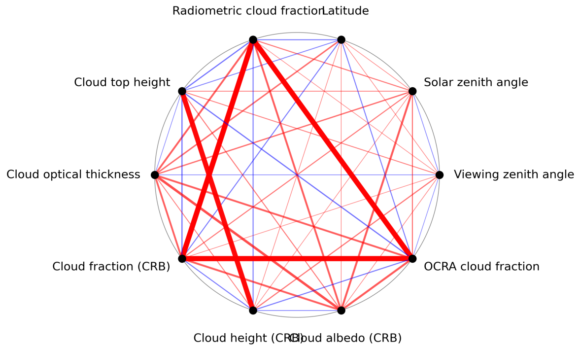
Figure 1: Map of correlation graph for 2024-02-22 to 2024-02-23.
