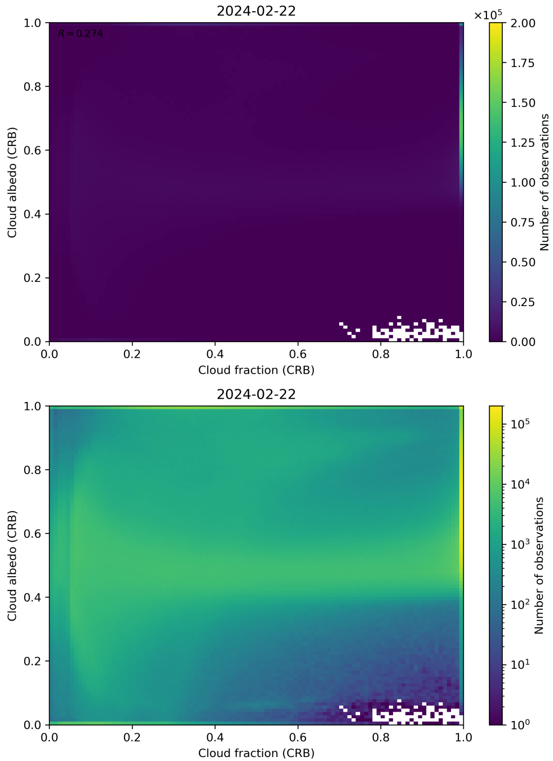
Figure 77: Scatter density plot of “Cloud fraction (CRB)” against “Cloud albedo (CRB)” for 2024-02-22 to 2024-02-23.
