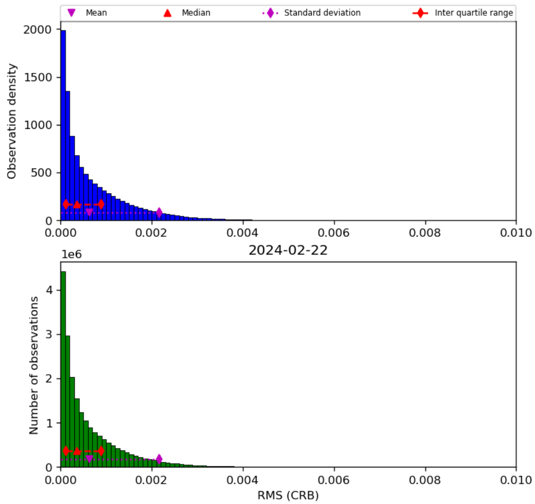
Figure 48: Histogram of “RMS (CRB)” for 2024-02-22 to 2024-02-23
