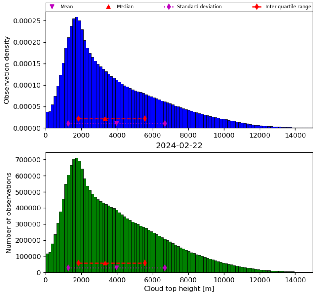
Figure 40: Histogram of “Cloud top height” for 2024-02-22 to 2024-02-23
