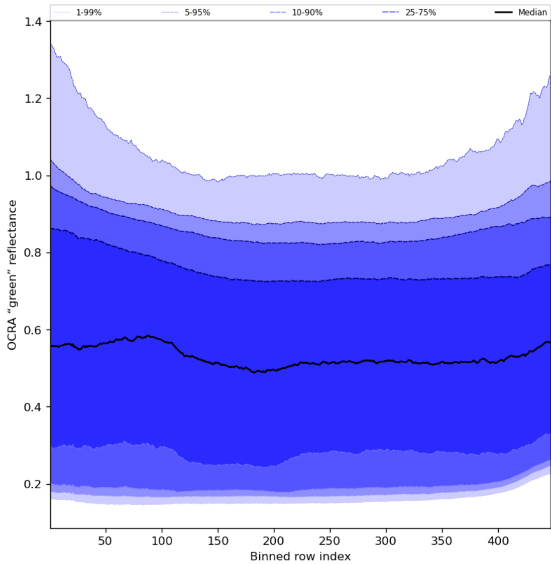
Figure 68: Along track statistics of “OCRA “green” reflectance” for 2024-02-22 to 2024-02-23
