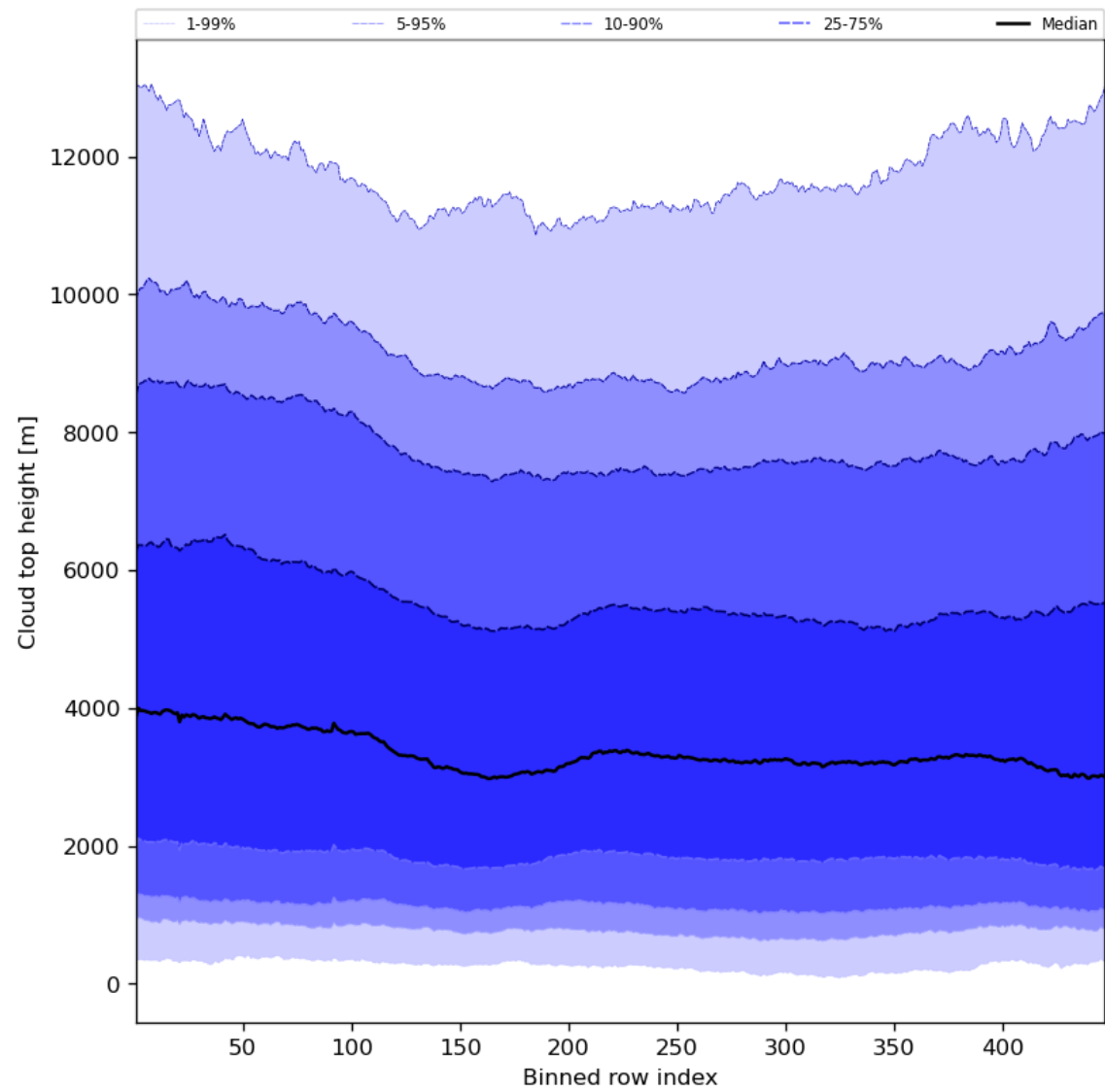
Figure 56: Along track statistics of “Cloud top height” for 2024-02-22 to 2024-02-23
