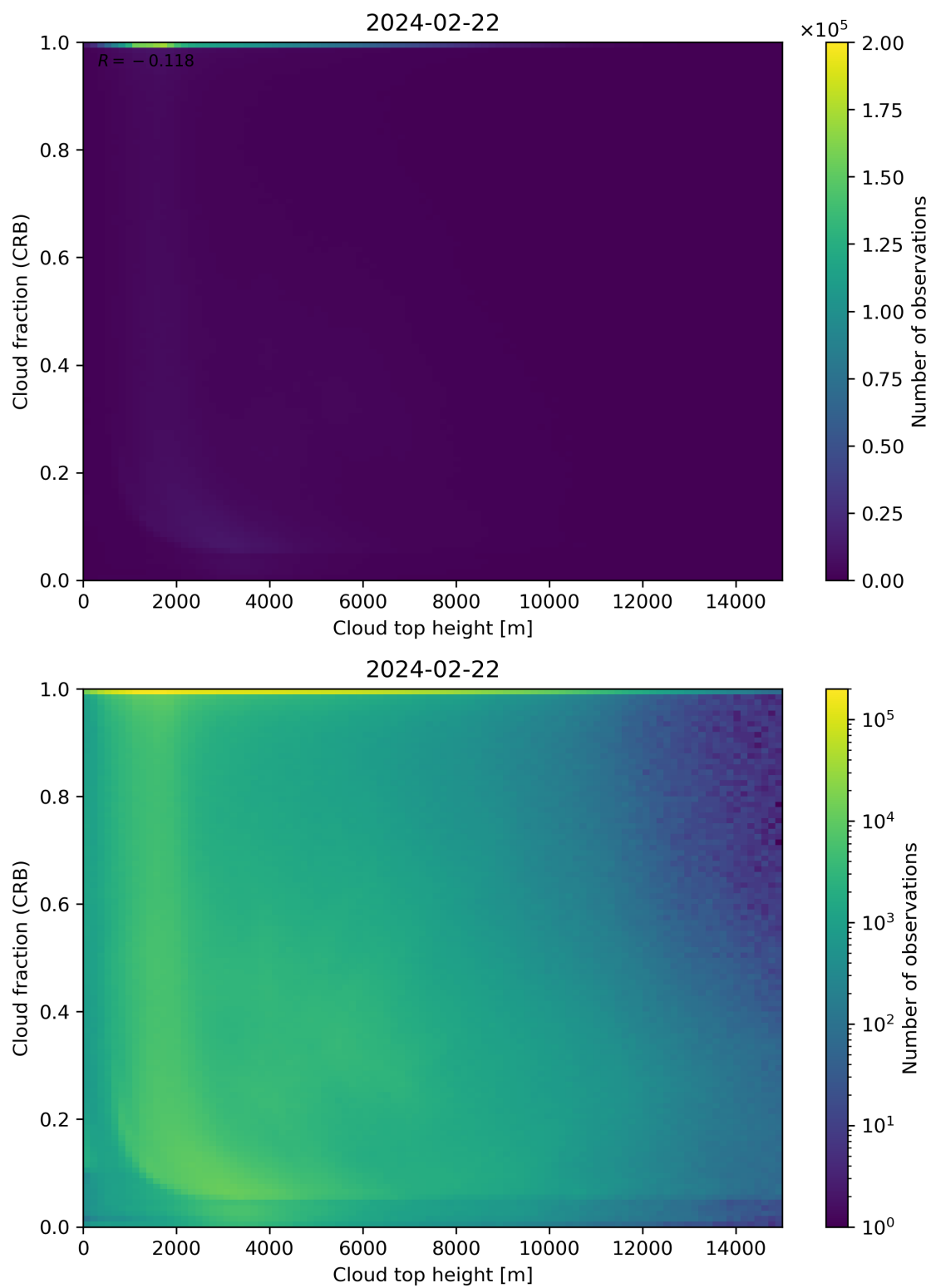
Figure 88: Scatter density plot of “Cloud top height” against “Cloud fraction (CRB)” for 2024-02-22 to 2024-02-23.
