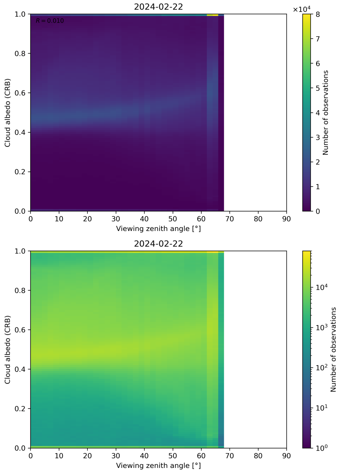
Figure 106: Scatter density plot of “Viewing zenith angle” against “Cloud albedo (CRB)” for 2024-02-22 to 2024-02-23.
