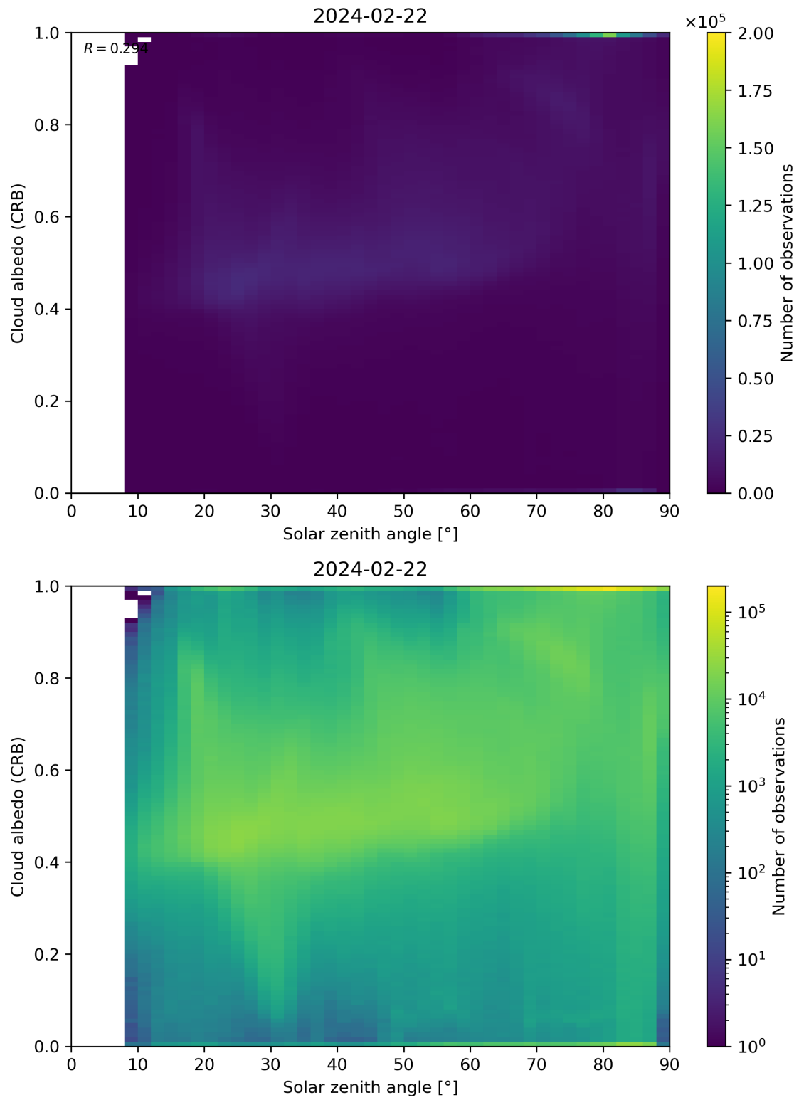
Figure 98: Scatter density plot of “Solar zenith angle” against “Cloud albedo (CRB)” for 2024-02-22 to 2024-02-23.
