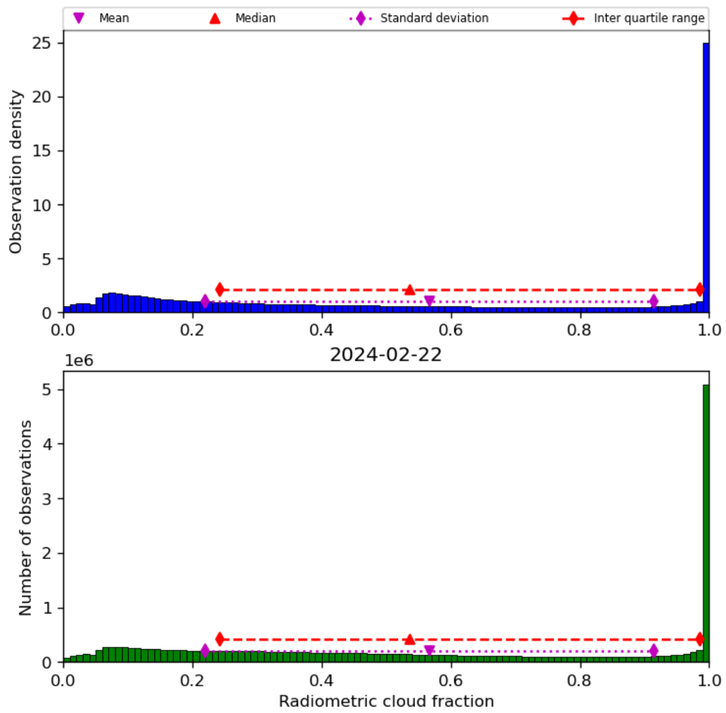
Figure 39: Histogram of “Radiometric cloud fraction” for 2024-02-22 to 2024-02-23
