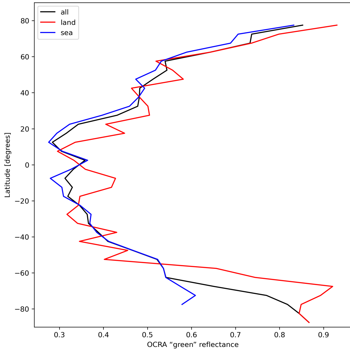
Figure 36: Zonal average of “OCRA “green” reflectance” for 2024-02-22 to 2024-02-23.
