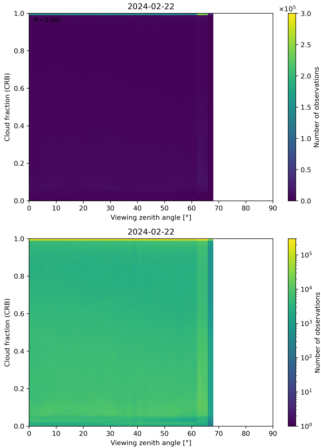
Figure 109: Scatter density plot of “Viewing zenith angle” against “Cloud fraction (CRB)” for 2024-02-22 to 2024-02-23.
