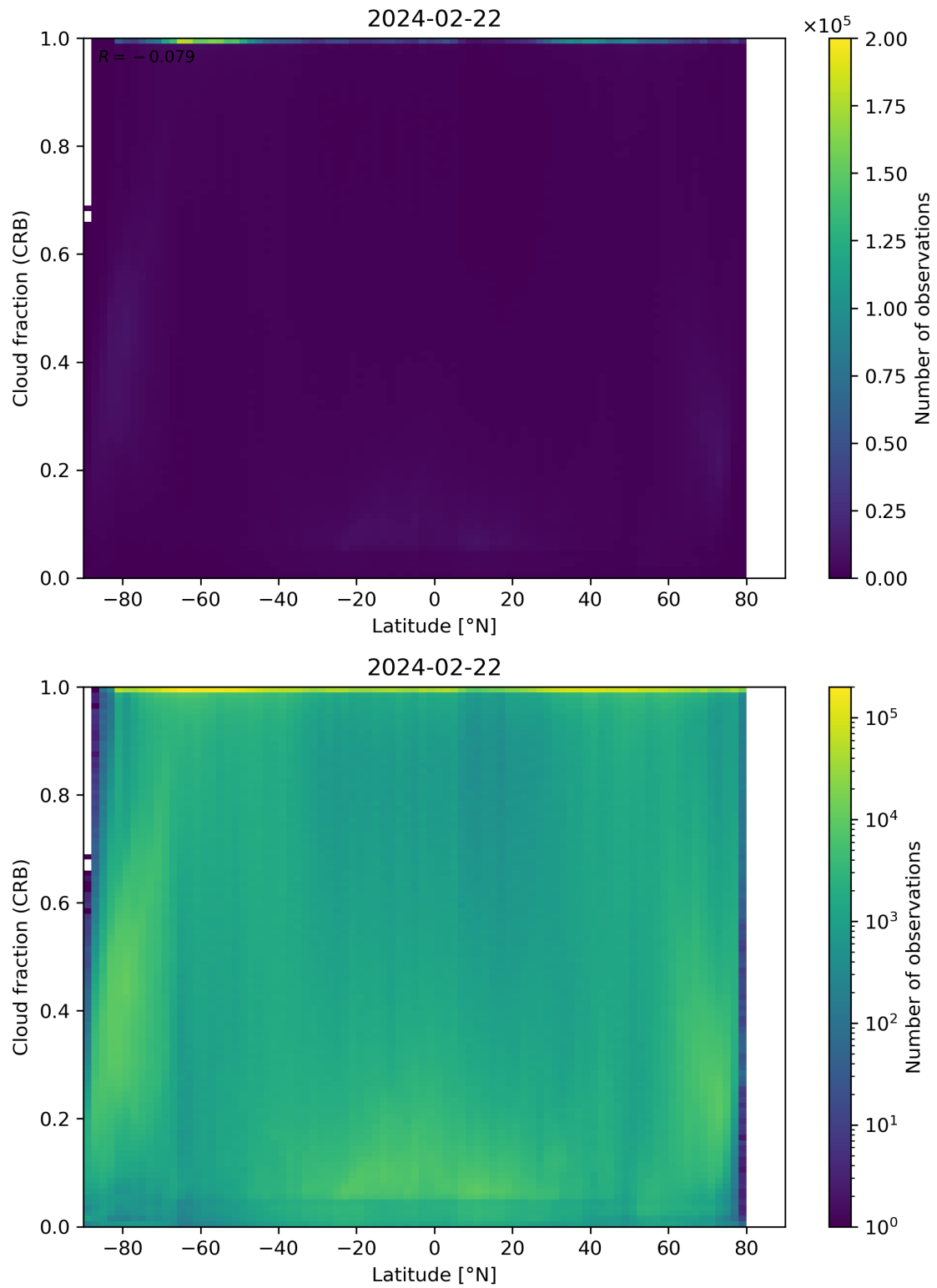
Figure 94: Scatter density plot of “Latitude” against “Cloud fraction (CRB)” for 2024-02-22 to 2024-02-23.
