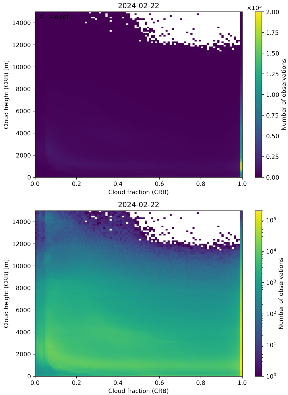
Figure 79: Scatter density plot of “Cloud fraction (CRB)” against “Cloud height (CRB)” for 2024-02-22 to 2024-02-23.
