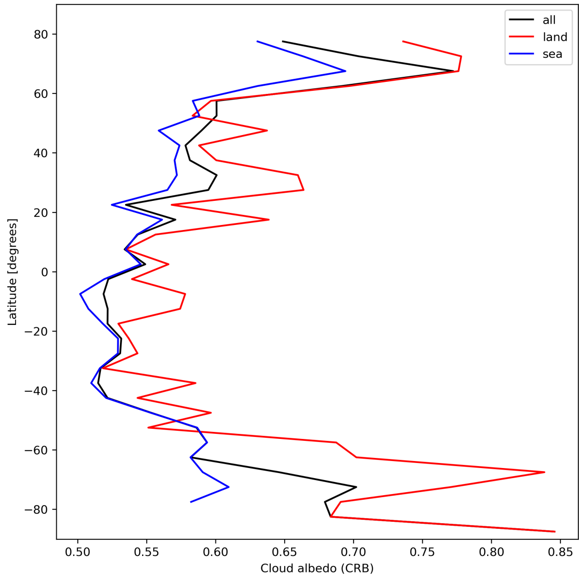
Figure 28: Zonal average of “Cloud albedo (CRB)” for 2024-02-22 to 2024-02-23.
