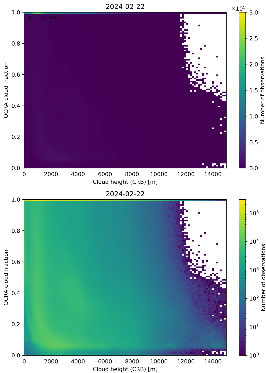
Figure 81: Scatter density plot of “Cloud height (CRB)” against “OCRA cloud fraction” for 2024-02-22 to 2024-02-23.
