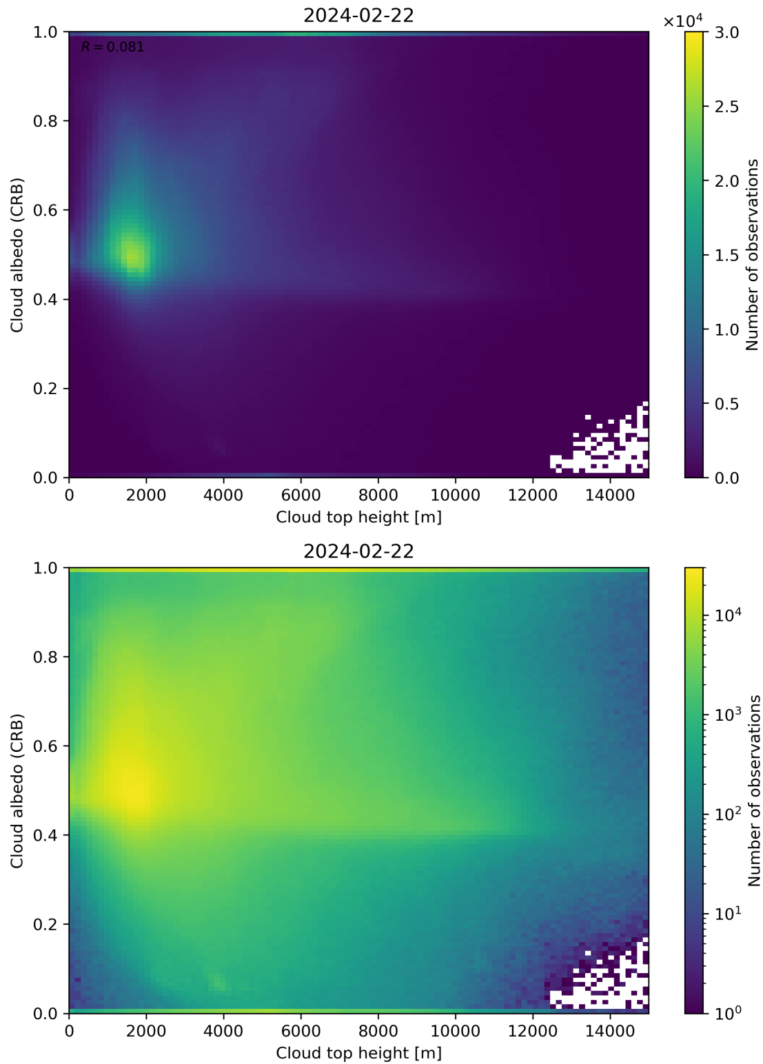
Figure 86: Scatter density plot of “Cloud top height” against “Cloud albedo (CRB)” for 2024-02-22 to 2024-02-23.
