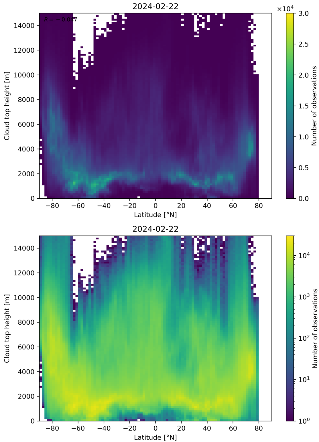
Figure 97: Scatter density plot of “Latitude” against “Cloud top height” for 2024-02-22 to 2024-02-23.
