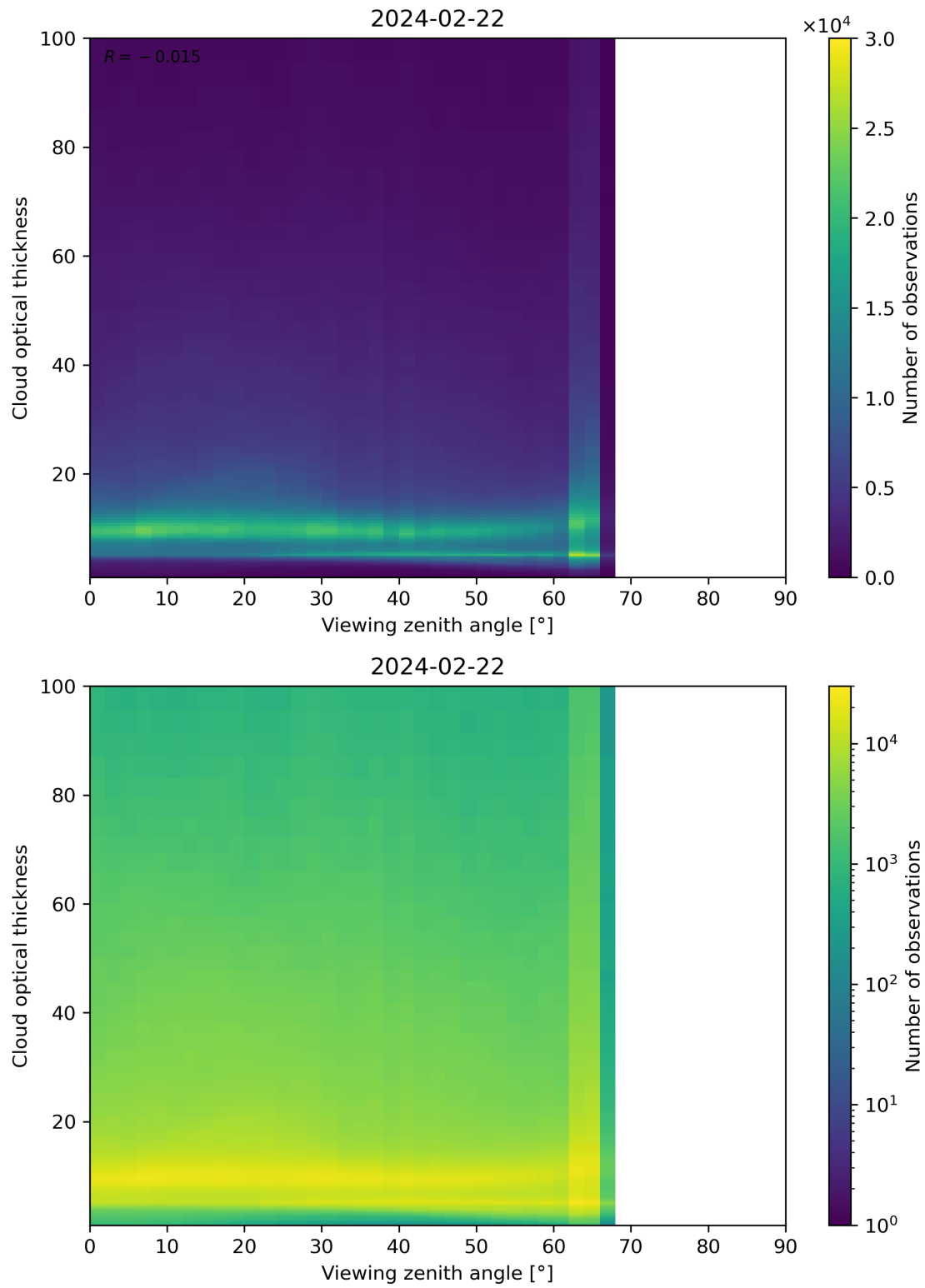
Figure 111: Scatter density plot of “Viewing zenith angle” against “Cloud optical thickness” for 2024-02-22 to 2024-02-23.
