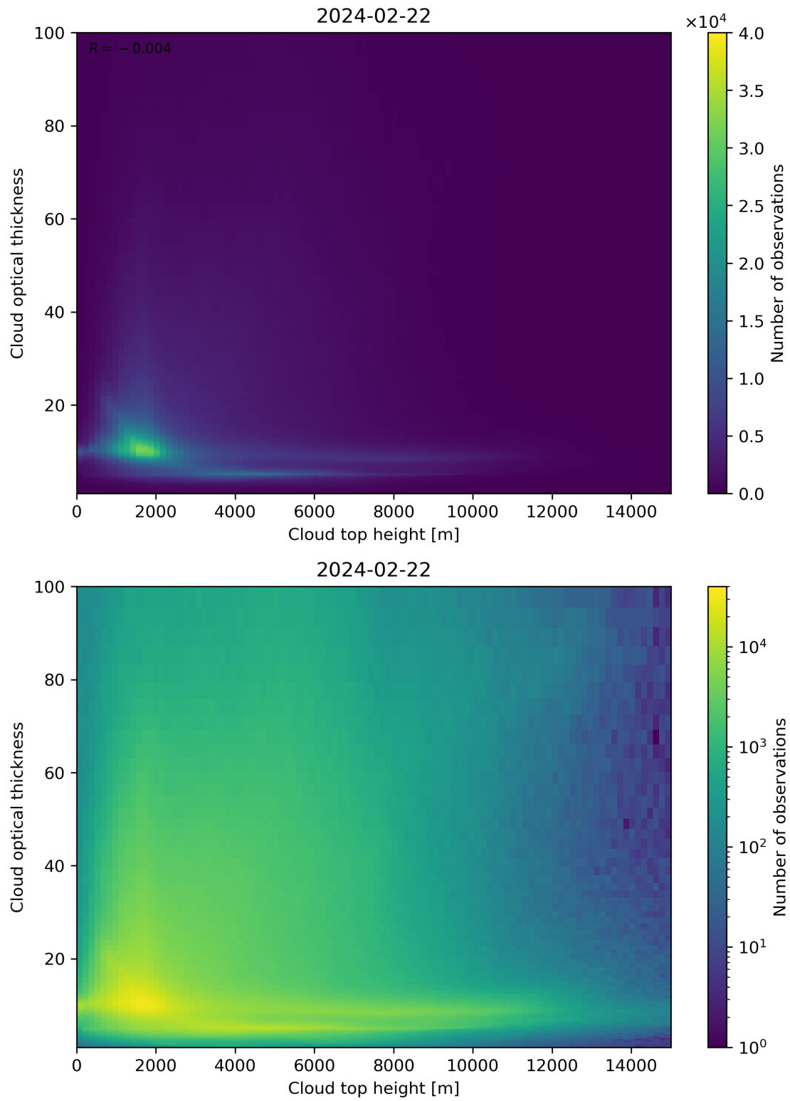
Figure 90: Scatter density plot of “Cloud top height” against “Cloud optical thickness” for 2024-02-22 to 2024-02-23.
