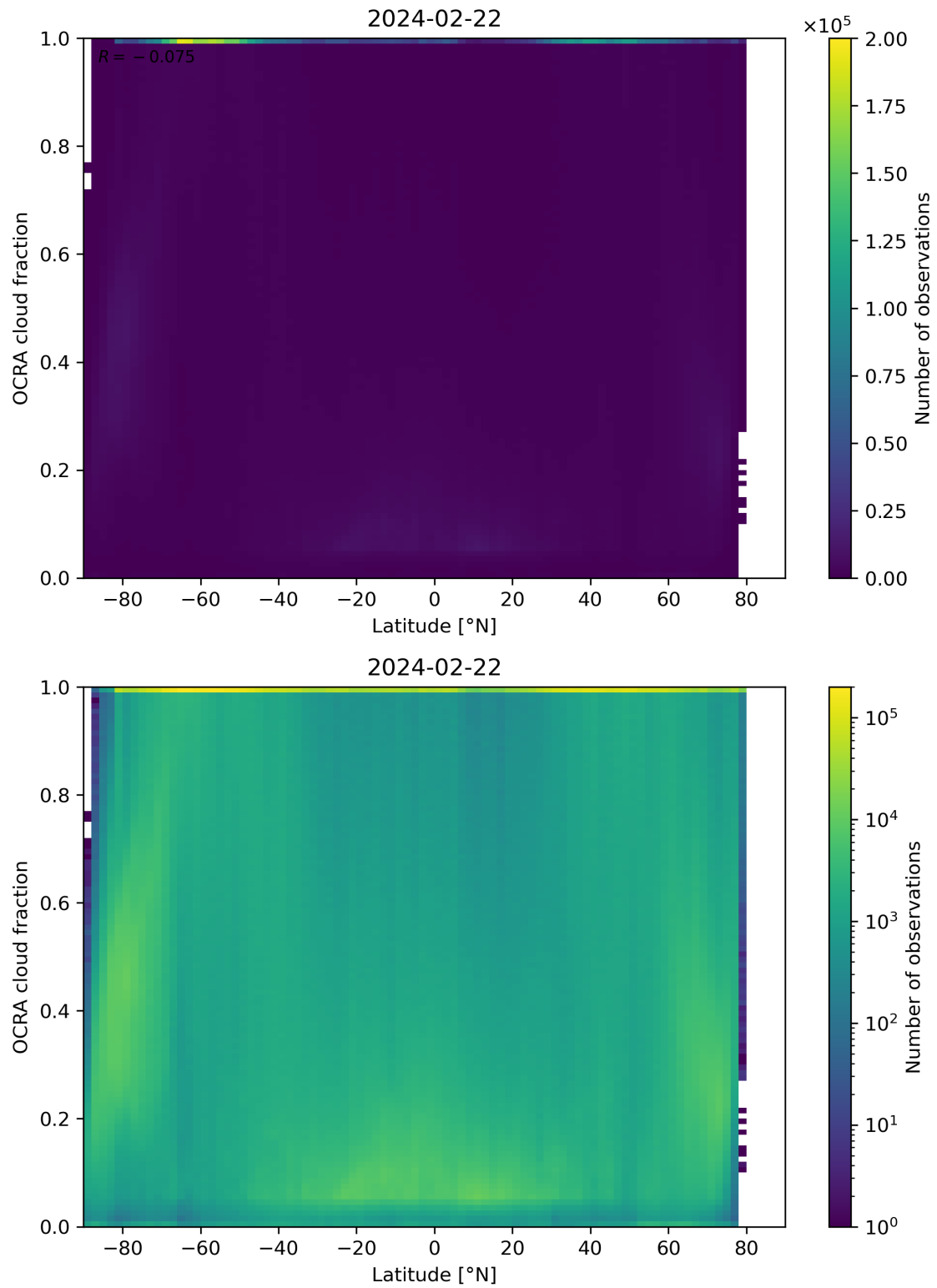
Figure 93: Scatter density plot of “Latitude” against “OCRA cloud fraction” for 2024-02-22 to 2024-02-23.
