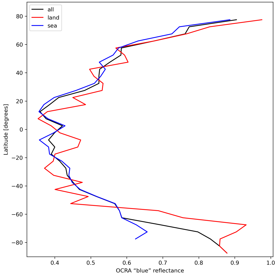
Figure 35: Zonal average of “OCRA “blue” reflectance” for 2024-02-22 to 2024-02-23.
