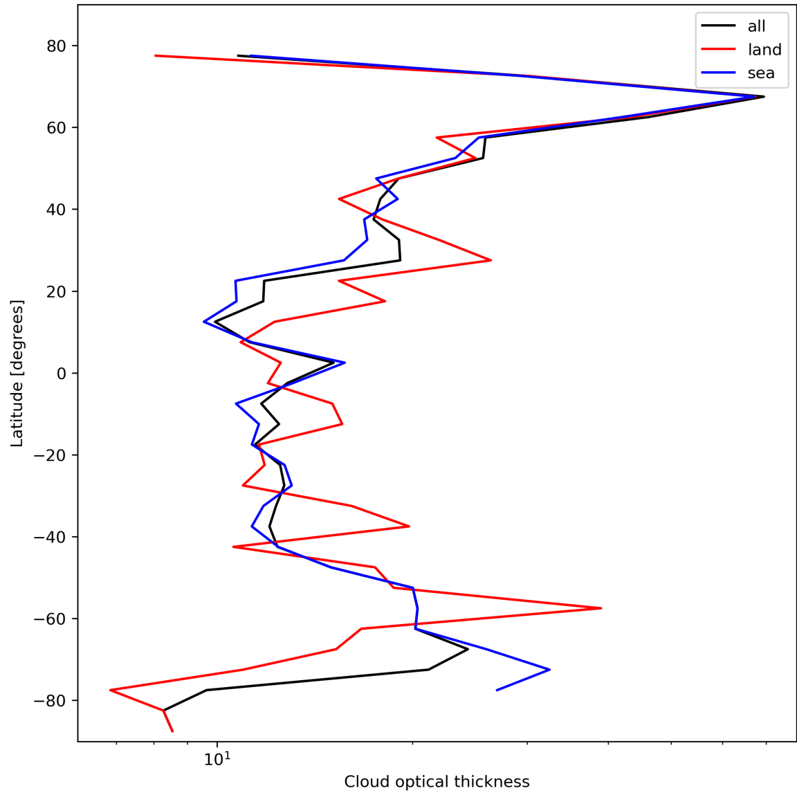
Figure 25: Zonal average of “Cloud optical thickness” for 2024-02-22 to 2024-02-23.
