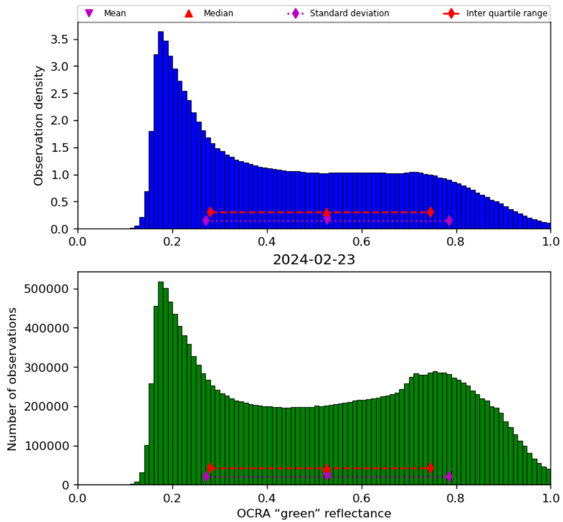
Figure 52: Histogram of “OCRA “green” reflectance” for 2024-02-22 to 2024-02-24
