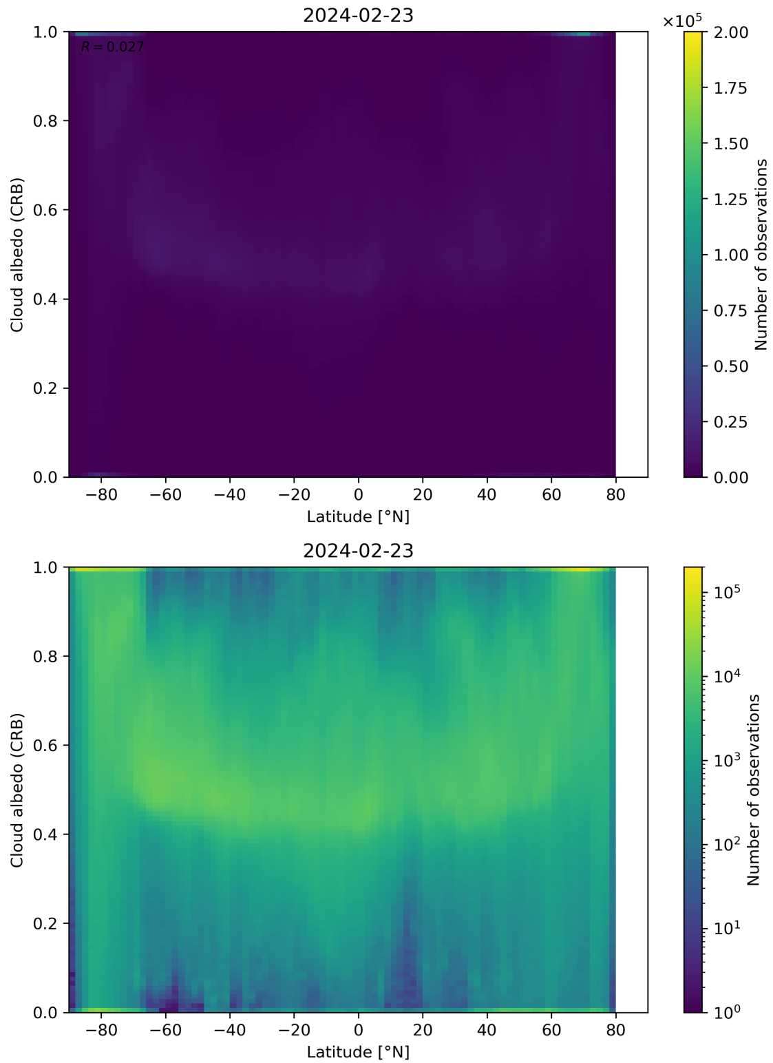
Figure 91: Scatter density plot of “Latitude” against “Cloud albedo (CRB)” for 2024-02-22 to 2024-02-24.
