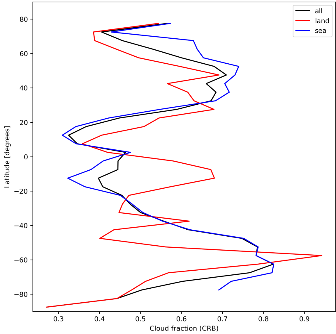
Figure 26: Zonal average of “Cloud fraction (CRB)” for 2024-02-22 to 2024-02-24.
