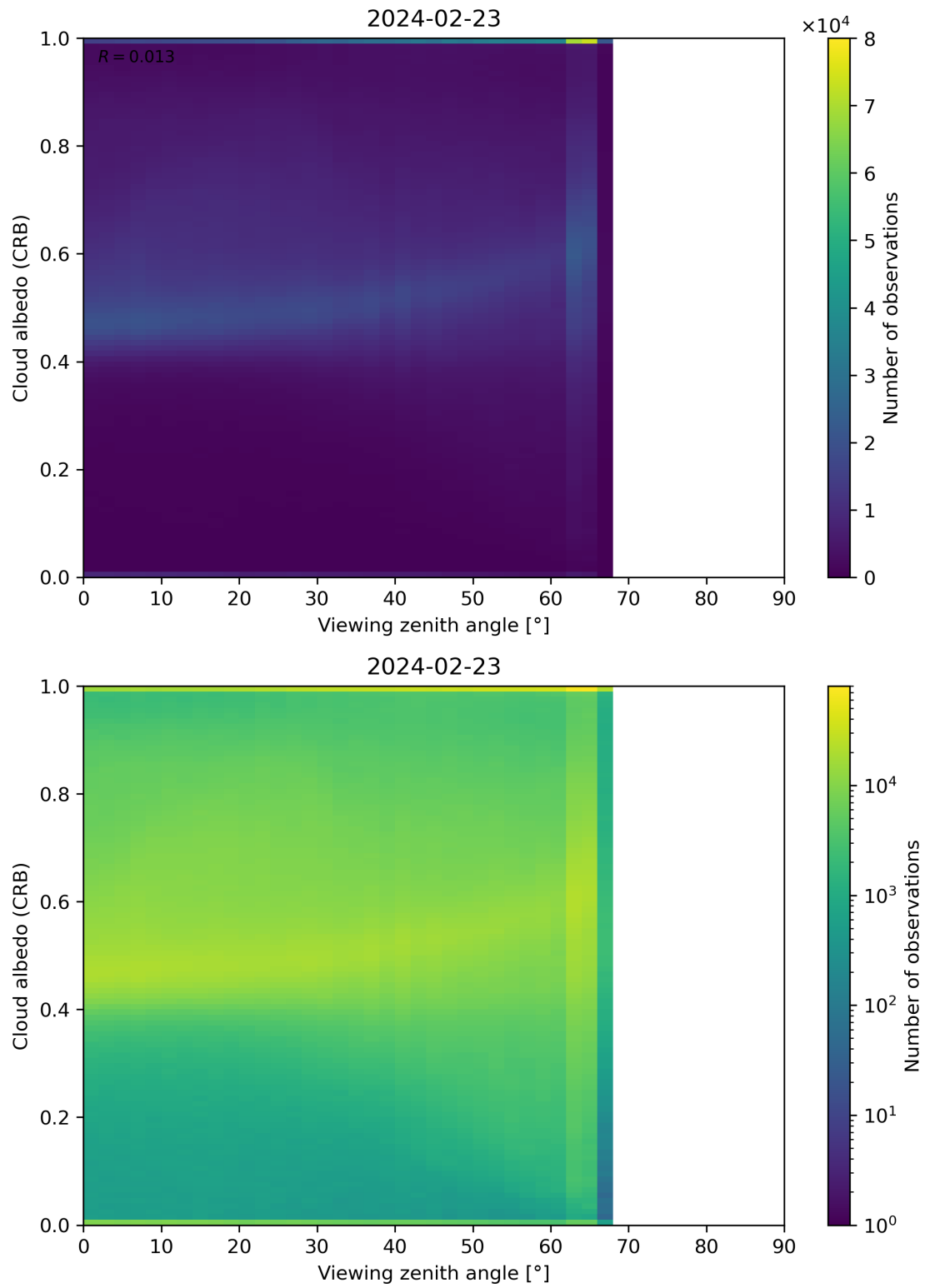
Figure 106: Scatter density plot of “Viewing zenith angle” against “Cloud albedo (CRB)” for 2024-02-22 to 2024-02-24.
