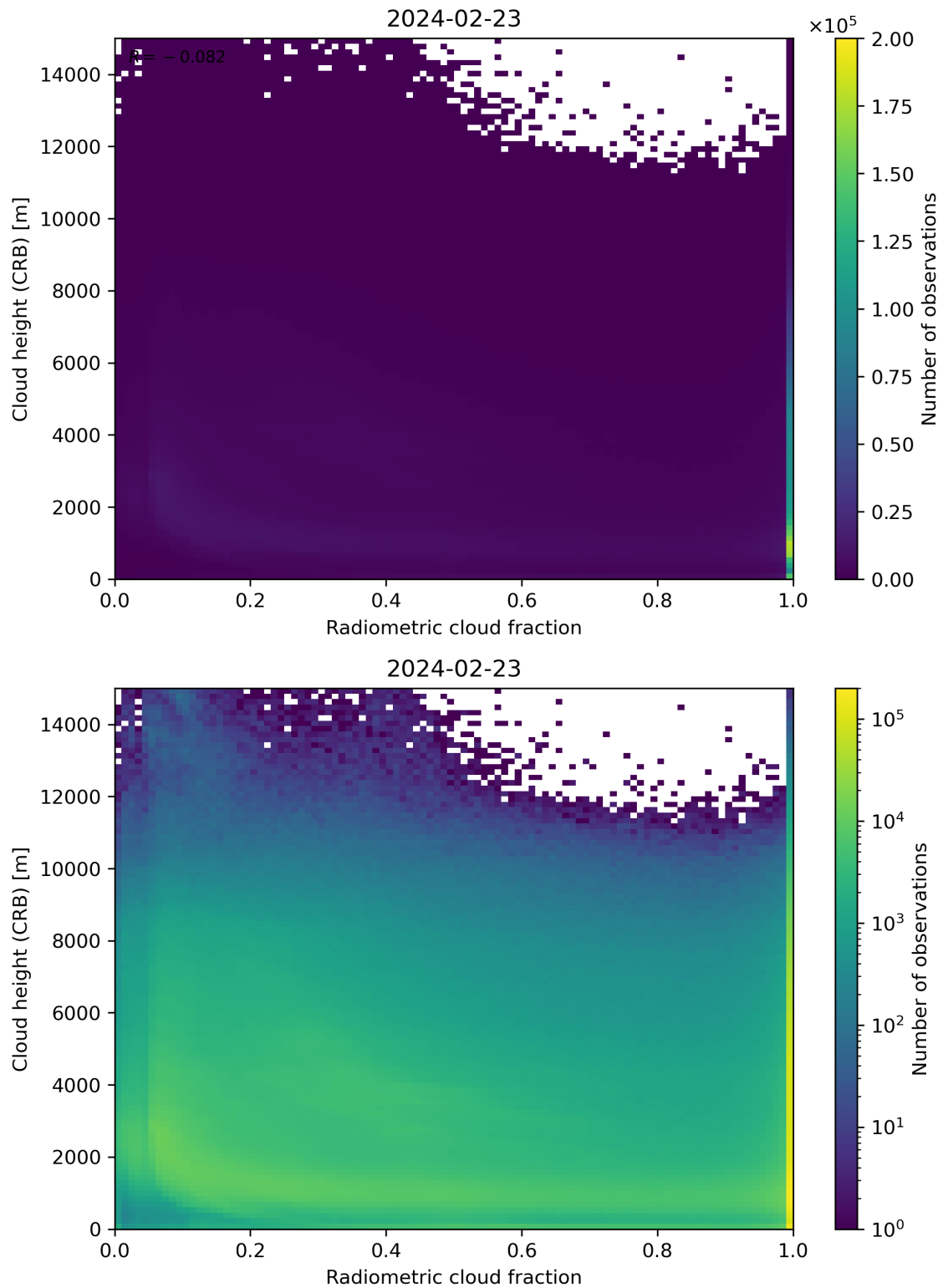
Figure 74: Scatter density plot of “Radiometric cloud fraction” against “Cloud height (CRB)” for 2024-02-22 to 2024-02-24.
