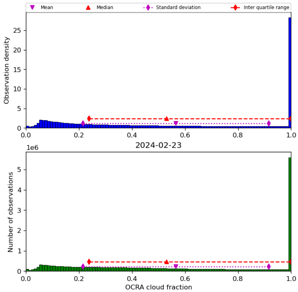
Figure 50: Histogram of “OCRA cloud fraction” for 2024-02-22 to 2024-02-24
