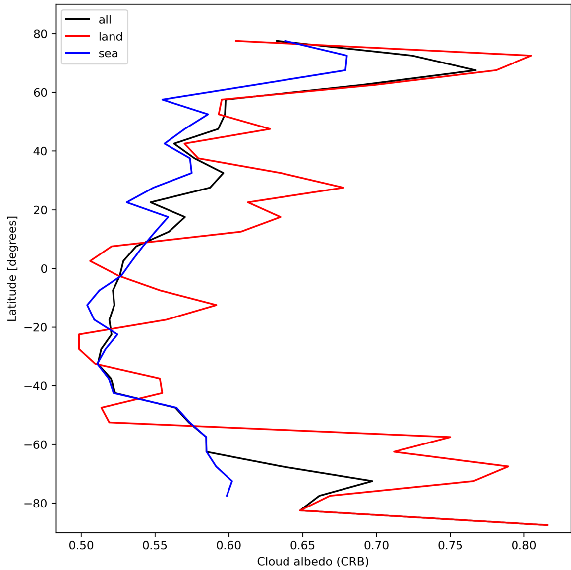
Figure 28: Zonal average of “Cloud albedo (CRB)” for 2024-02-22 to 2024-02-24.
