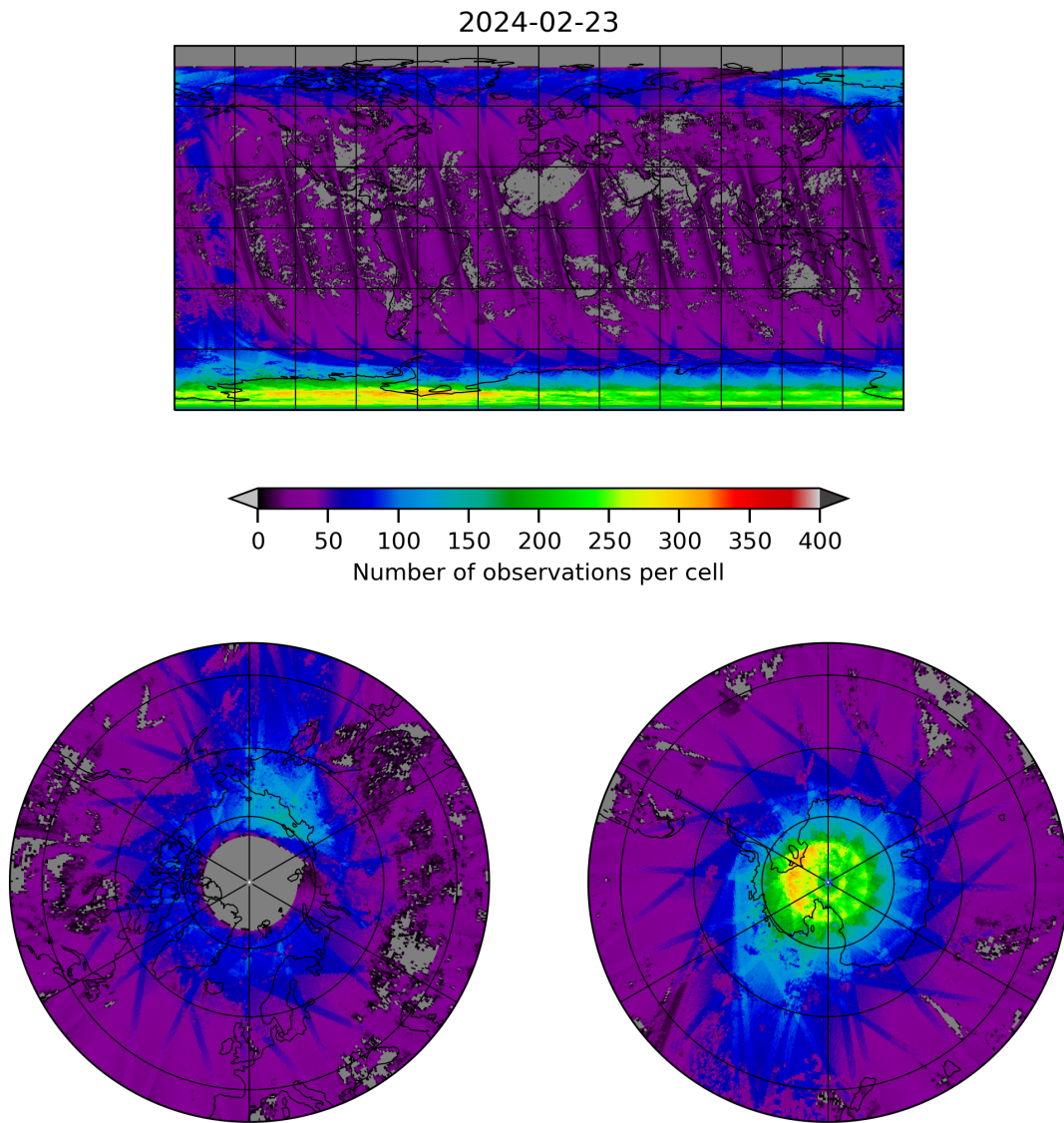
Figure 21: Map of the number of observations for 2024-02-22 to 2024-02-24
