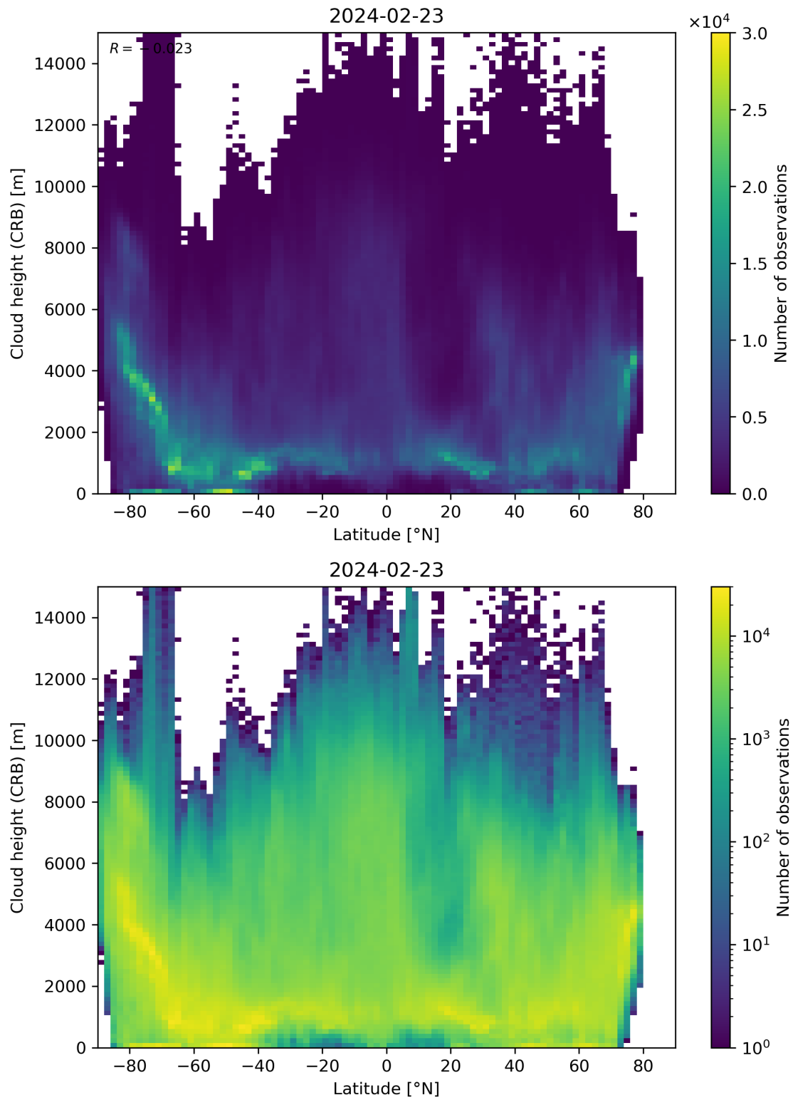
Figure 95: Scatter density plot of “Latitude” against “Cloud height (CRB)” for 2024-02-22 to 2024-02-24.
