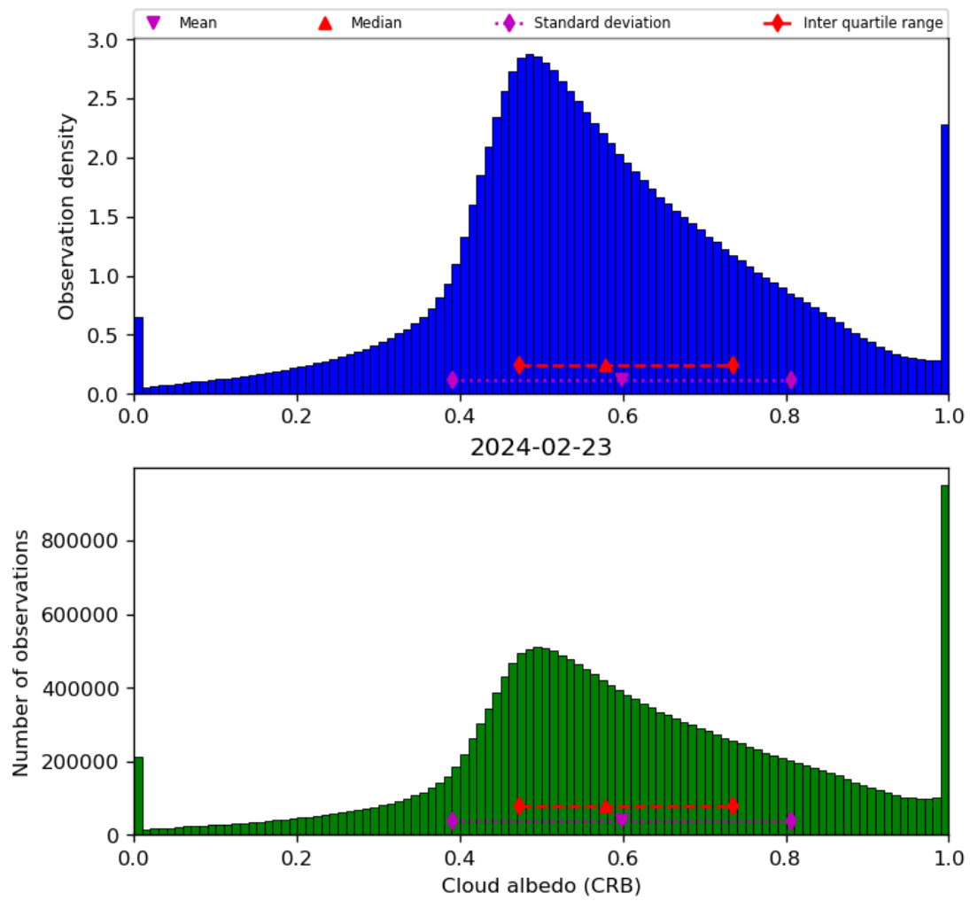
Figure 44: Histogram of “Cloud albedo (CRB)” for 2024-02-22 to 2024-02-24
