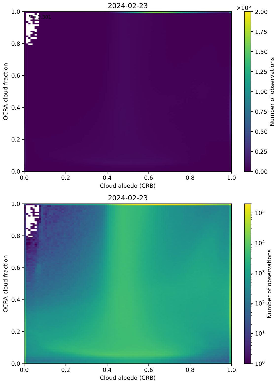
Figure 70: Scatter density plot of “Cloud albedo (CRB)” against “OCRA cloud fraction” for 2024-02-22 to 2024-02-24.
