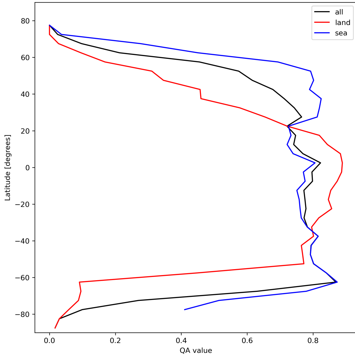
Figure 22: Zonal average of “QA value” for 2024-02-22 to 2024-02-24.
