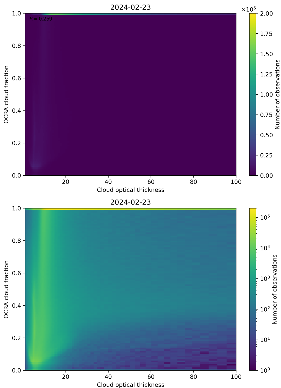
Figure 83: Scatter density plot of “Cloud optical thickness” against “OCRA cloud fraction” for 2024-02-22 to 2024-02-24.
