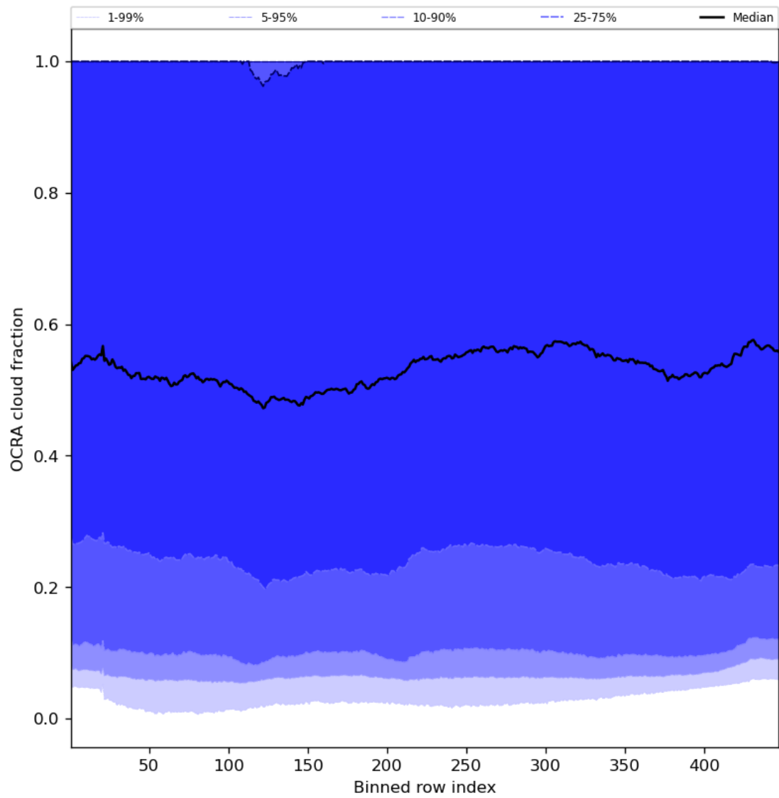
Figure 66: Along track statistics of “OCRA cloud fraction” for 2024-02-22 to 2024-02-24
