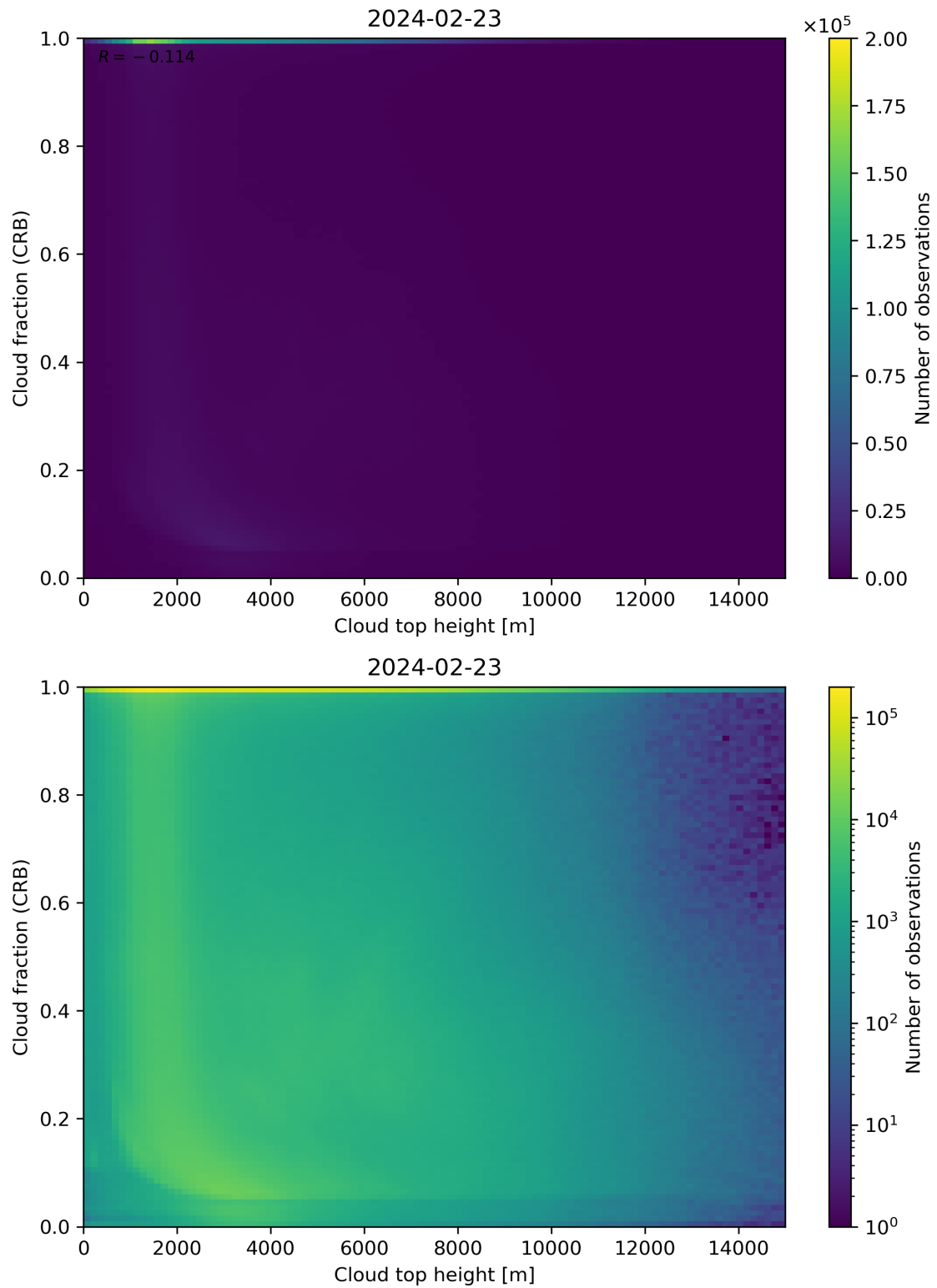
Figure 88: Scatter density plot of “Cloud top height” against “Cloud fraction (CRB)” for 2024-02-22 to 2024-02-24.
