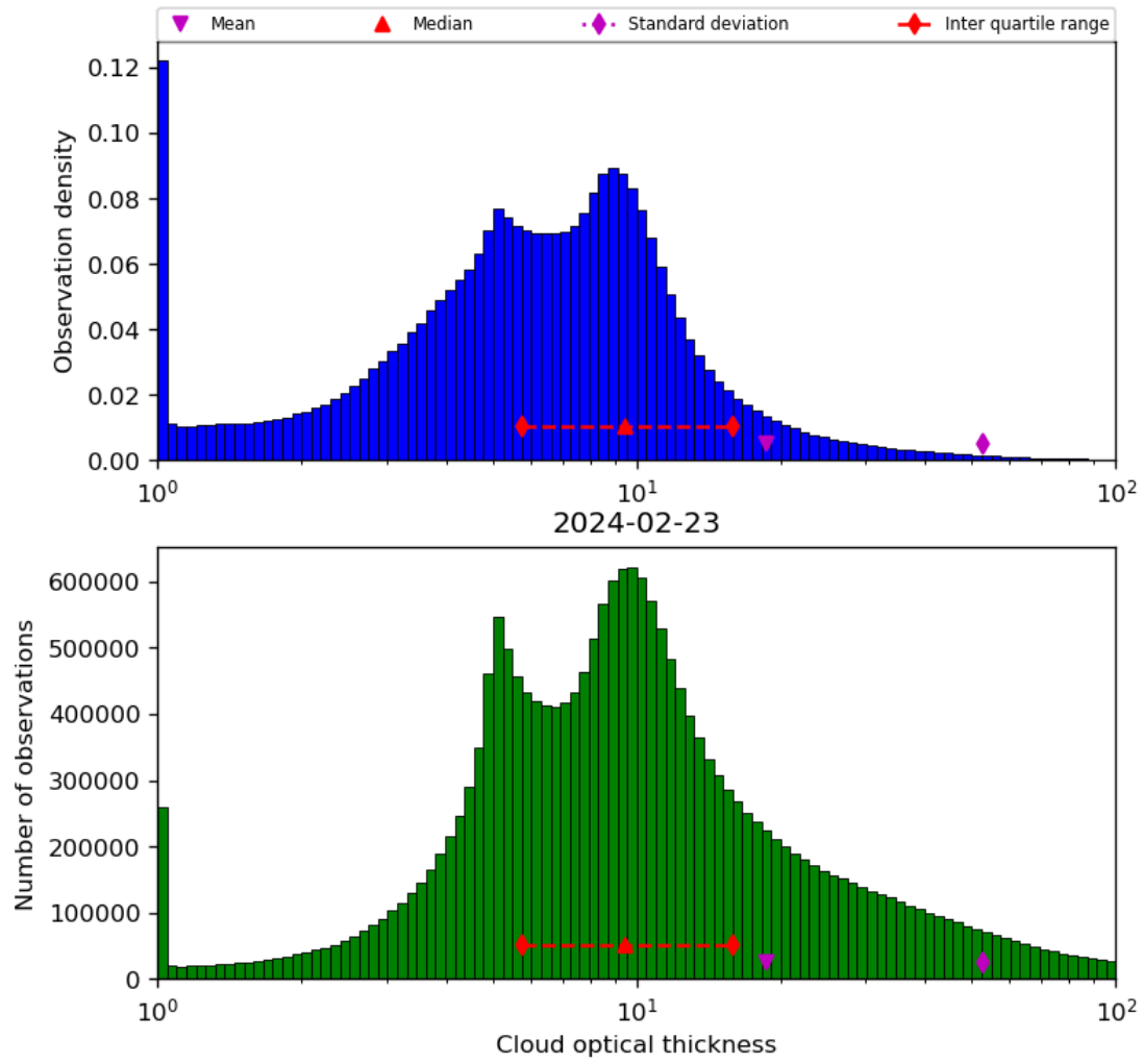
Figure 41: Histogram of “Cloud optical thickness” for 2024-02-22 to 2024-02-24
