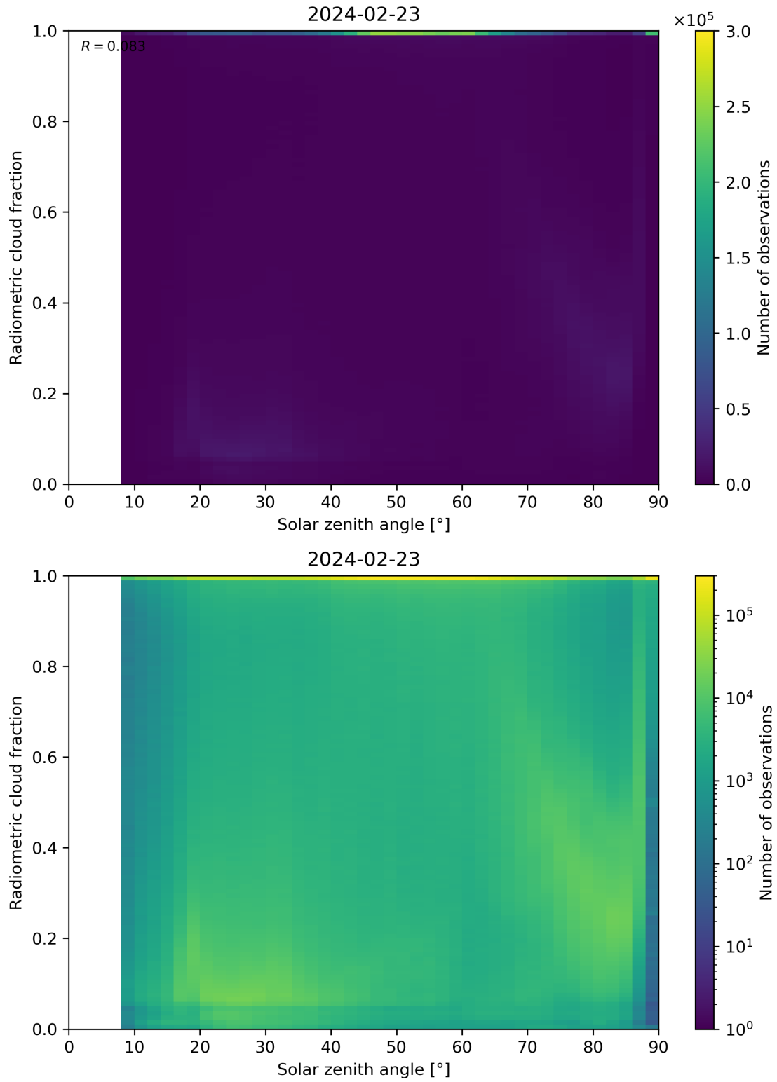
Figure 99: Scatter density plot of “Solar zenith angle” against “Radiometric cloud fraction” for 2024-02-22 to 2024-02-24.
