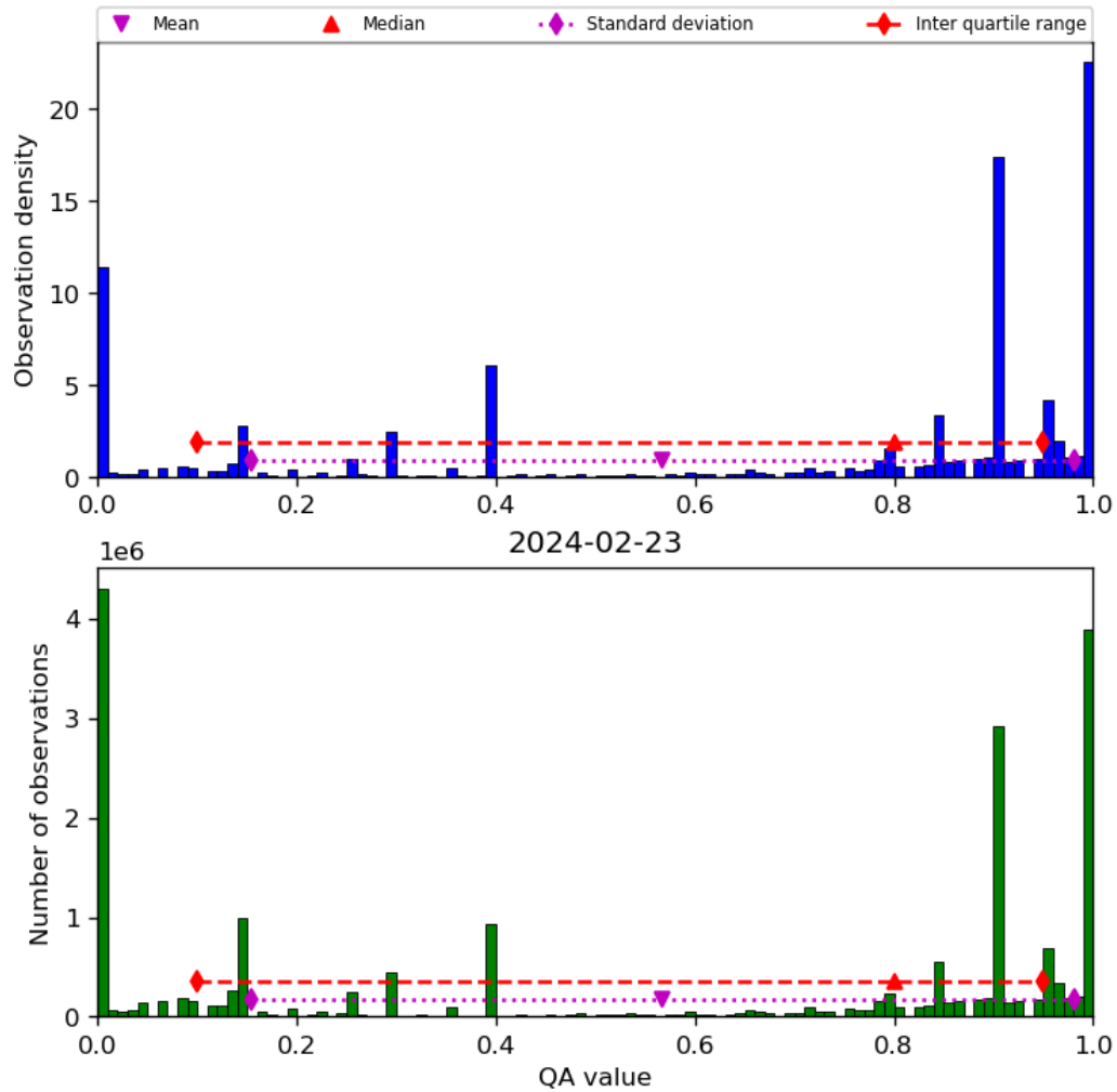
Figure 38: Histogram of “QA value” for 2024-02-22 to 2024-02-24
