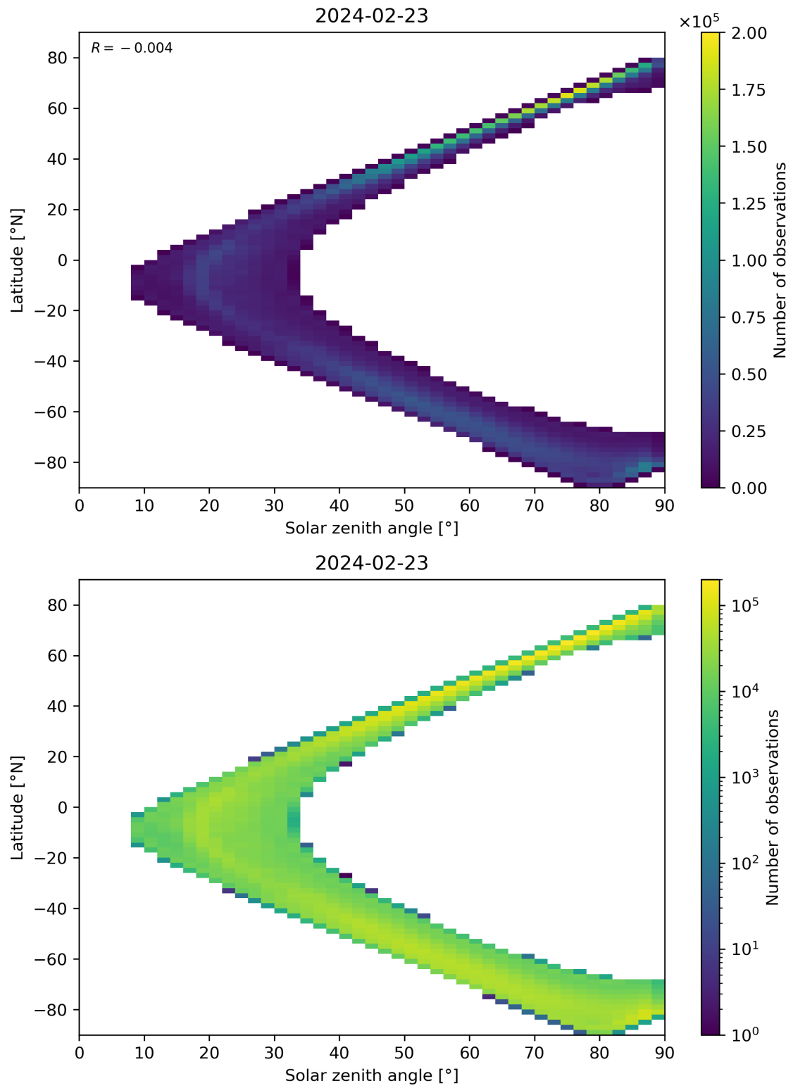
Figure 105: Scatter density plot of “Solar zenith angle” against “Latitude” for 2024-02-22 to 2024-02-24.
