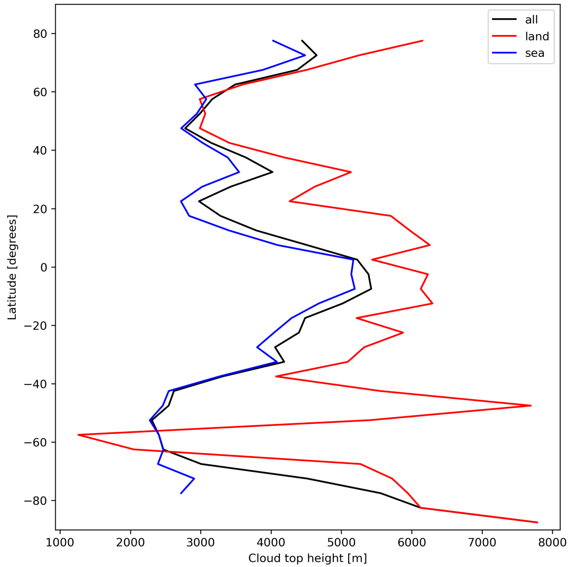
Figure 24: Zonal average of “Cloud top height” for 2024-02-22 to 2024-02-24.
