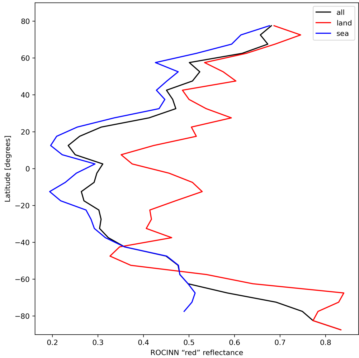
Figure 37: Zonal average of "ROCINN "red" reflectance" for 2024-02-22 to 2024-02-24.
