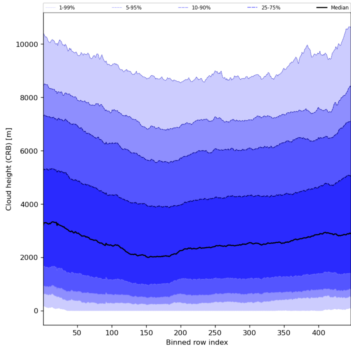
Figure 59: Along track statistics of “Cloud height (CRB)” for 2024-02-22 to 2024-02-24
