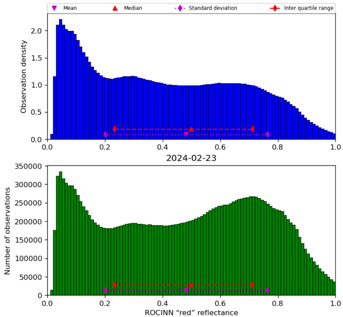
Figure 53: Histogram of “ROCINN “red” reflectance” for 2024-02-22 to 2024-02-24
