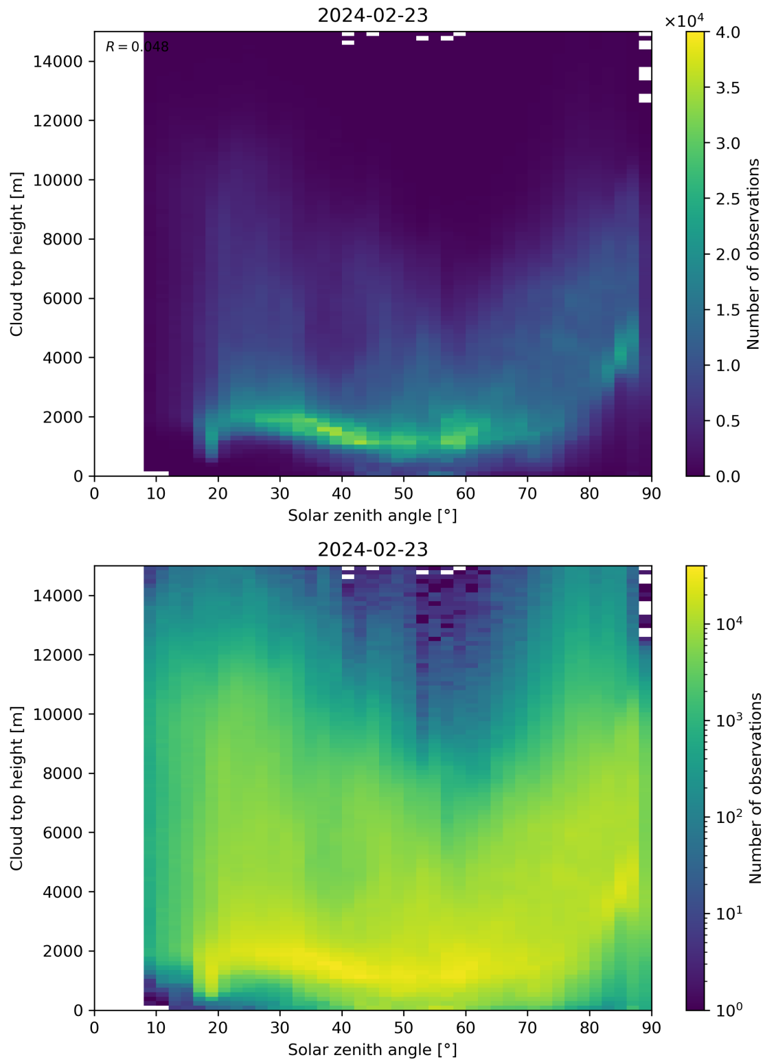
Figure 104: Scatter density plot of “Solar zenith angle” against “Cloud top height” for 2024-02-22 to 2024-02-24.
