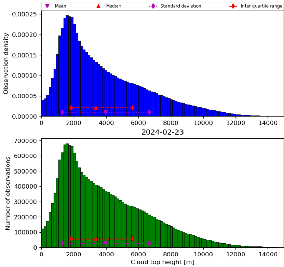
Figure 40: Histogram of “Cloud top height” for 2024-02-22 to 2024-02-24
