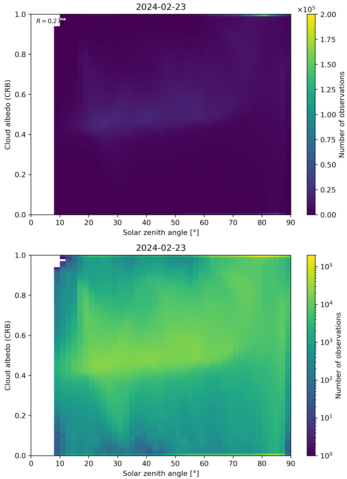
Figure 98: Scatter density plot of “Solar zenith angle” against “Cloud albedo (CRB)” for 2024-02-22 to 2024-02-24.
