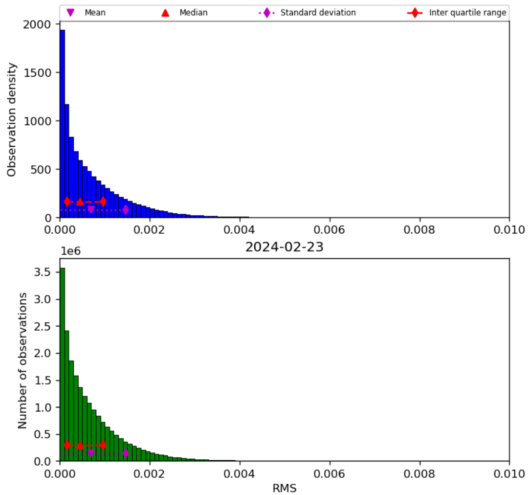
Figure 47: Histogram of “RMS” for 2024-02-22 to 2024-02-24
