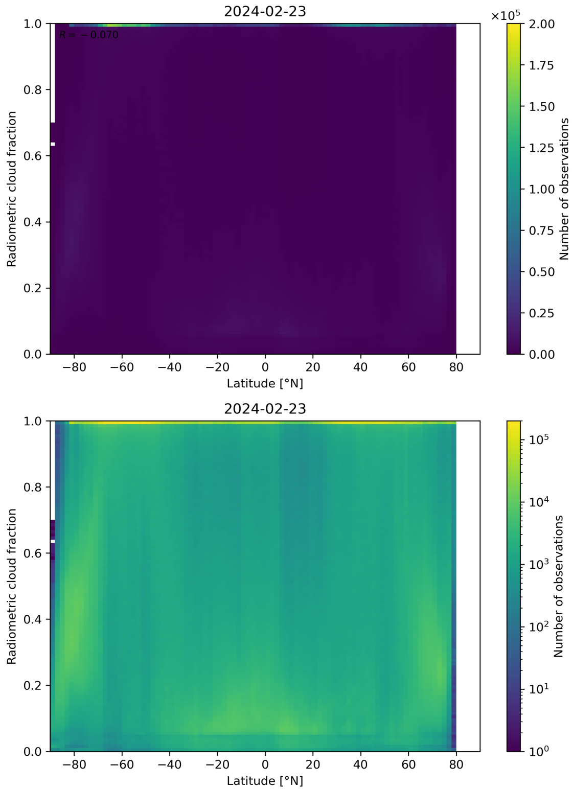
Figure 92: Scatter density plot of “Latitude” against “Radiometric cloud fraction” for 2024-02-22 to 2024-02-24.
