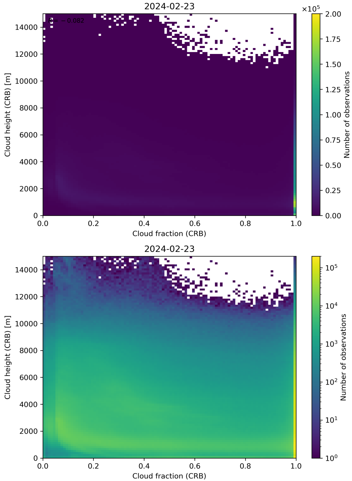
Figure 79: Scatter density plot of “Cloud fraction (CRB)” against “Cloud height (CRB)” for 2024-02-22 to 2024-02-24.
