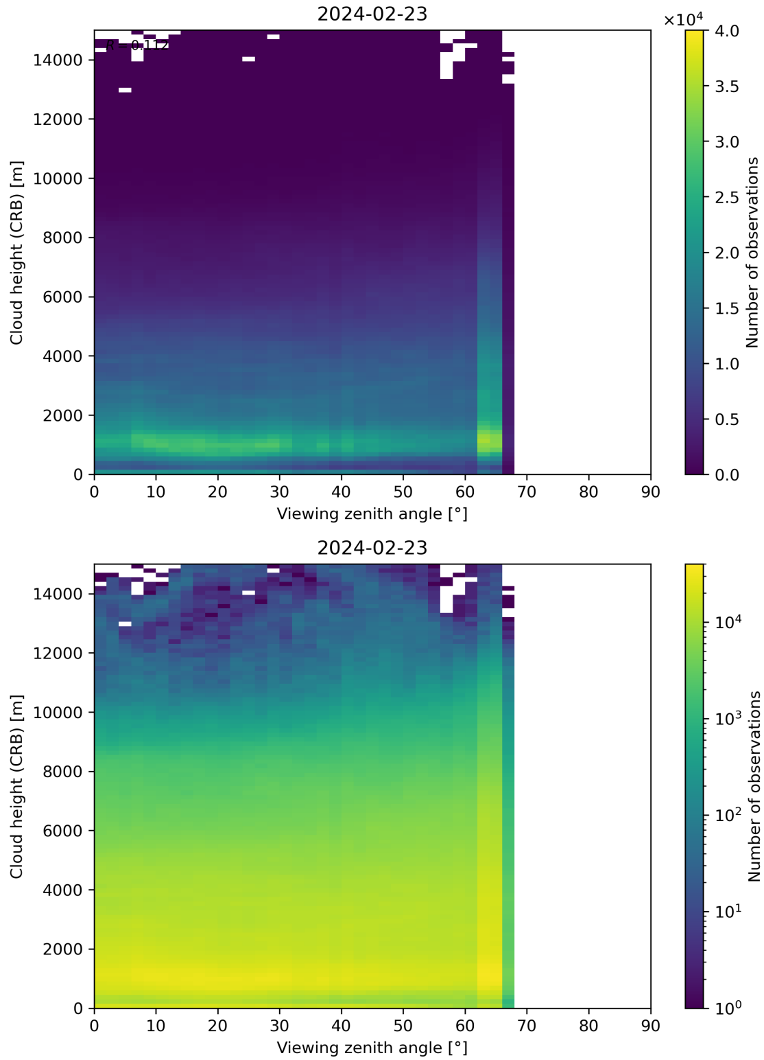
Figure 110: Scatter density plot of “Viewing zenith angle” against “Cloud height (CRB)” for 2024-02-22 to 2024-02-24.
