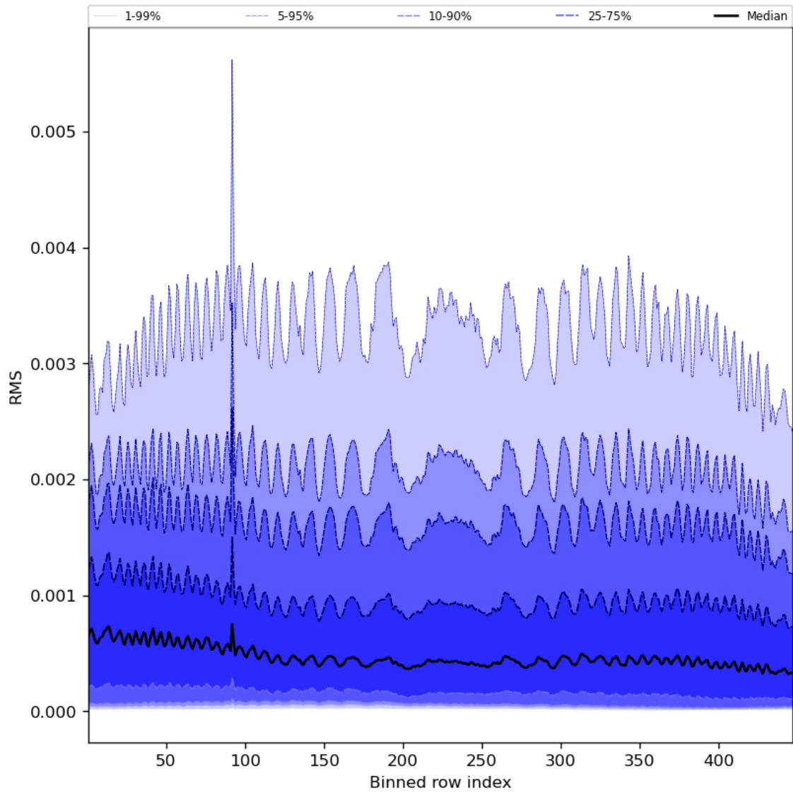
Figure 63: Along track statistics of “RMS” for 2024-02-22 to 2024-02-24
