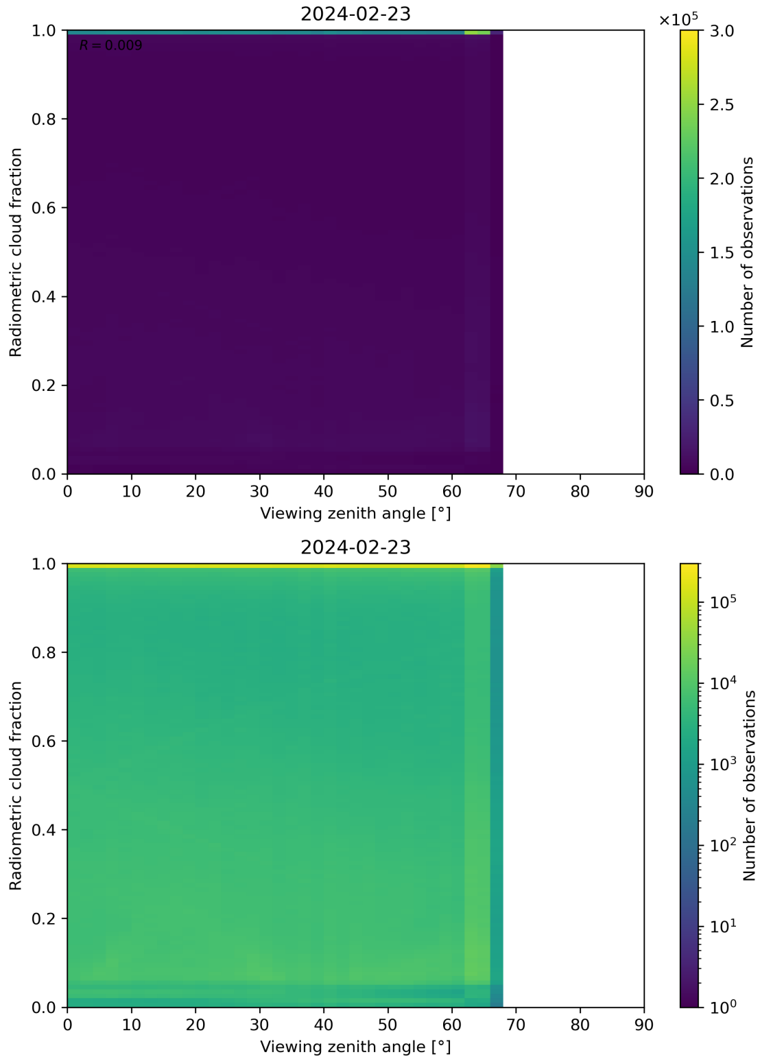
Figure 107: Scatter density plot of “Viewing zenith angle” against “Radiometric cloud fraction” for 2024-02-22 to 2024-02-24.
