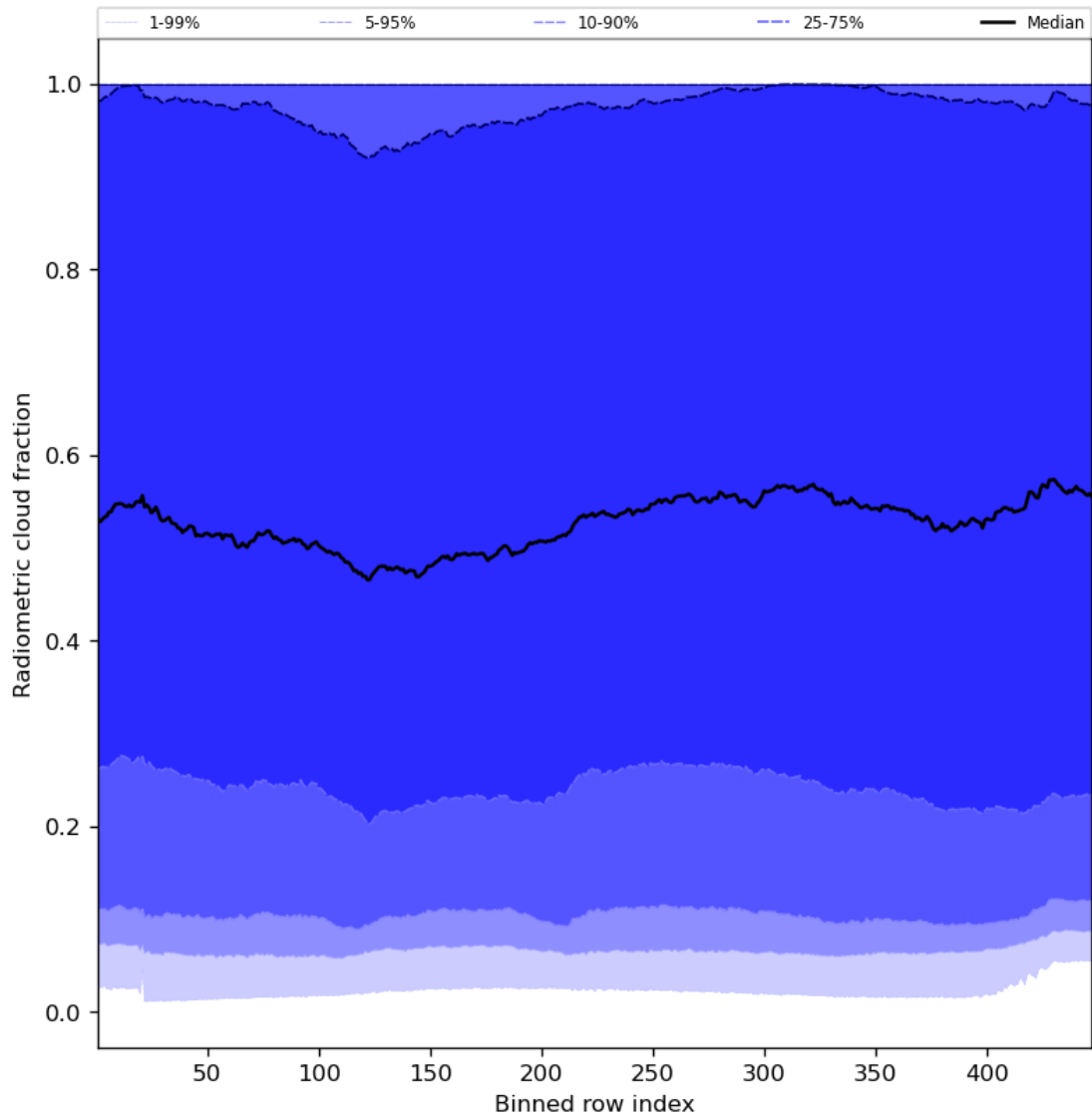
Figure 55: Along track statistics of “Radiometric cloud fraction” for 2024-02-22 to 2024-02-24
