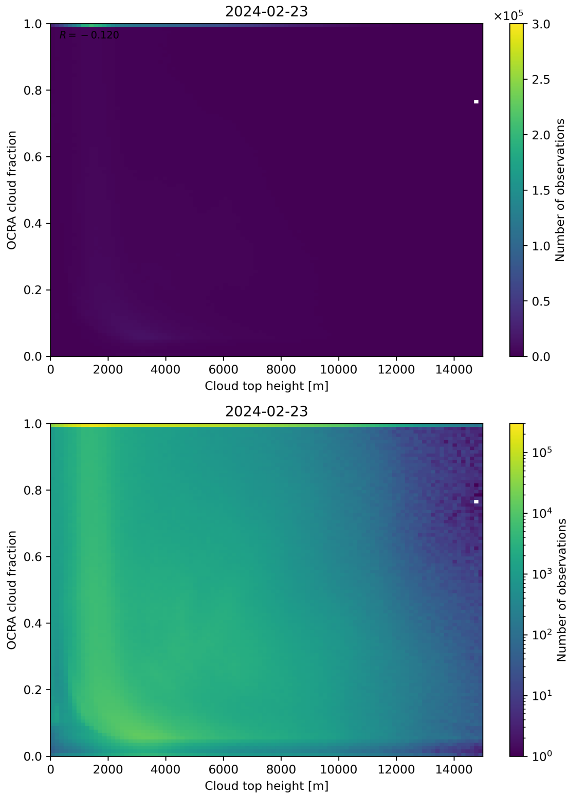
Figure 87: Scatter density plot of “Cloud top height” against “OCRA cloud fraction” for 2024-02-22 to 2024-02-24.
