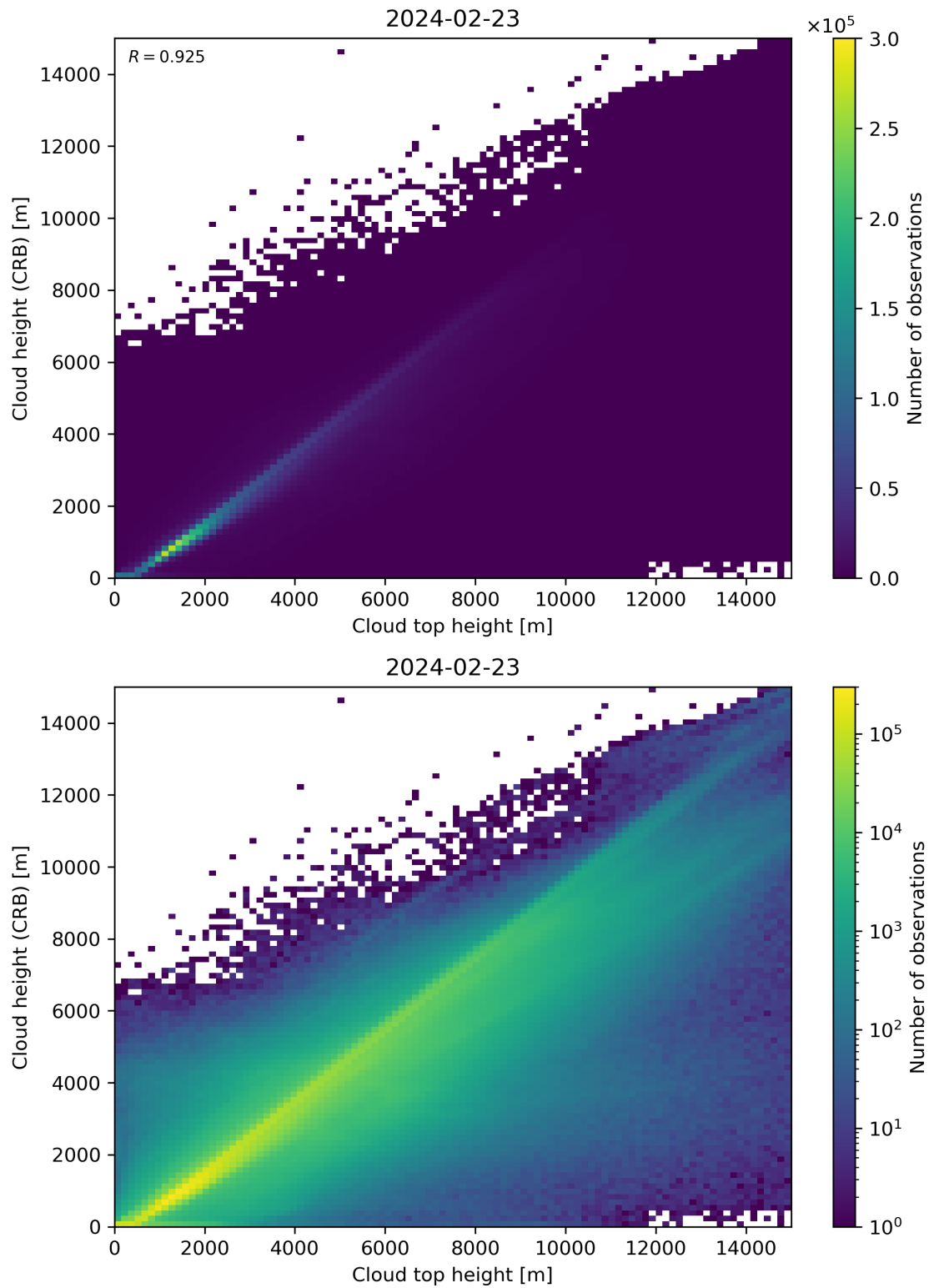
Figure 89: Scatter density plot of “Cloud top height” against “Cloud height (CRB)” for 2024-02-22 to 2024-02-24.
