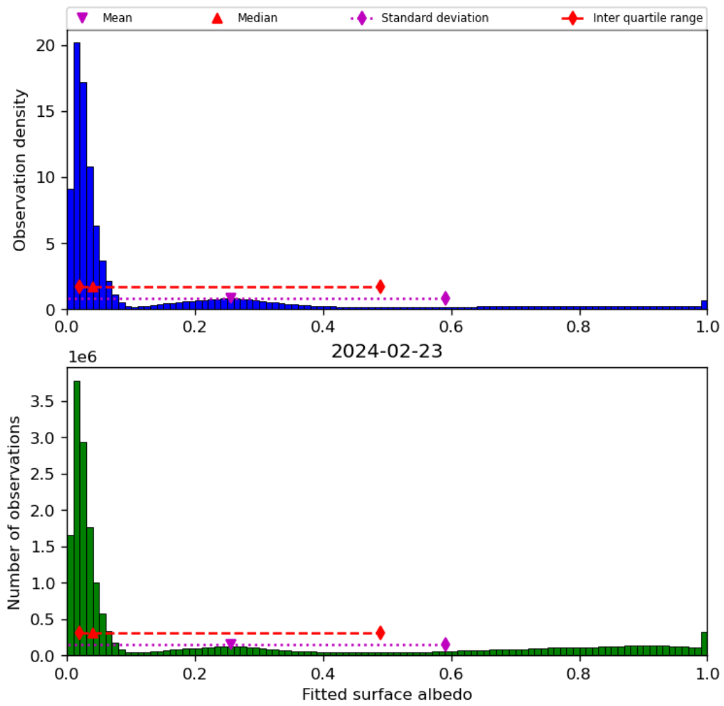
Figure 45: Histogram of “Fitted surface albedo” for 2024-02-22 to 2024-02-24
