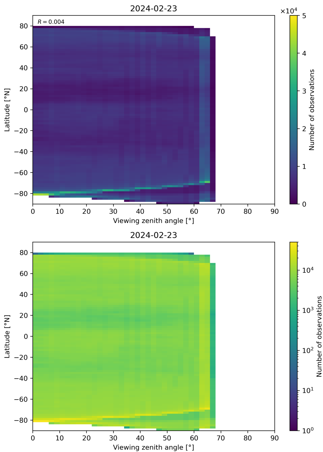
Figure 113: Scatter density plot of “Viewing zenith angle” against “Latitude” for 2024-02-22 to 2024-02-24.
