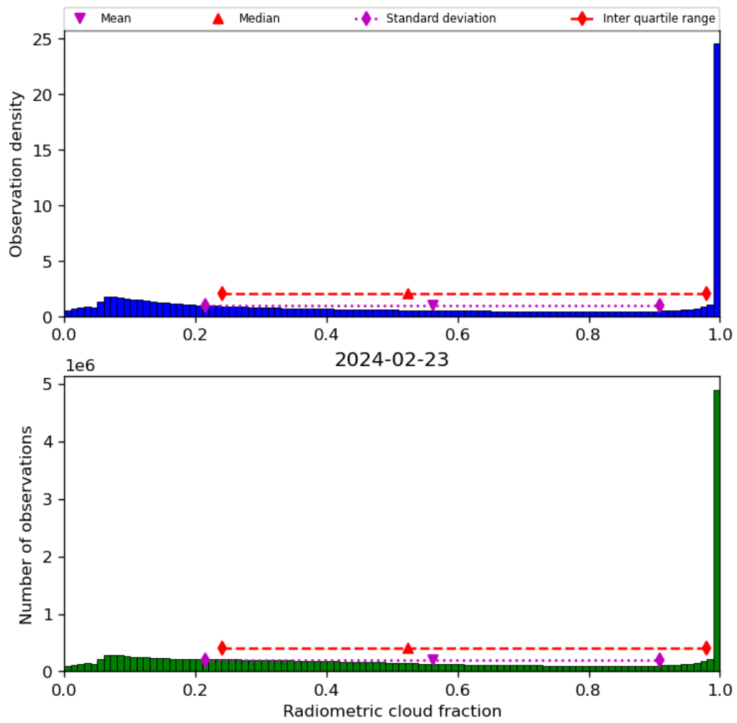
Figure 39: Histogram of “Radiometric cloud fraction” for 2024-02-22 to 2024-02-24
