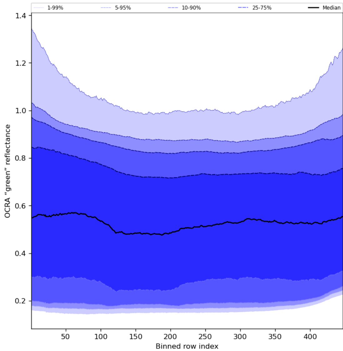
Figure 68: Along track statistics of “OCRA “green” reflectance” for 2024-02-22 to 2024-02-24
