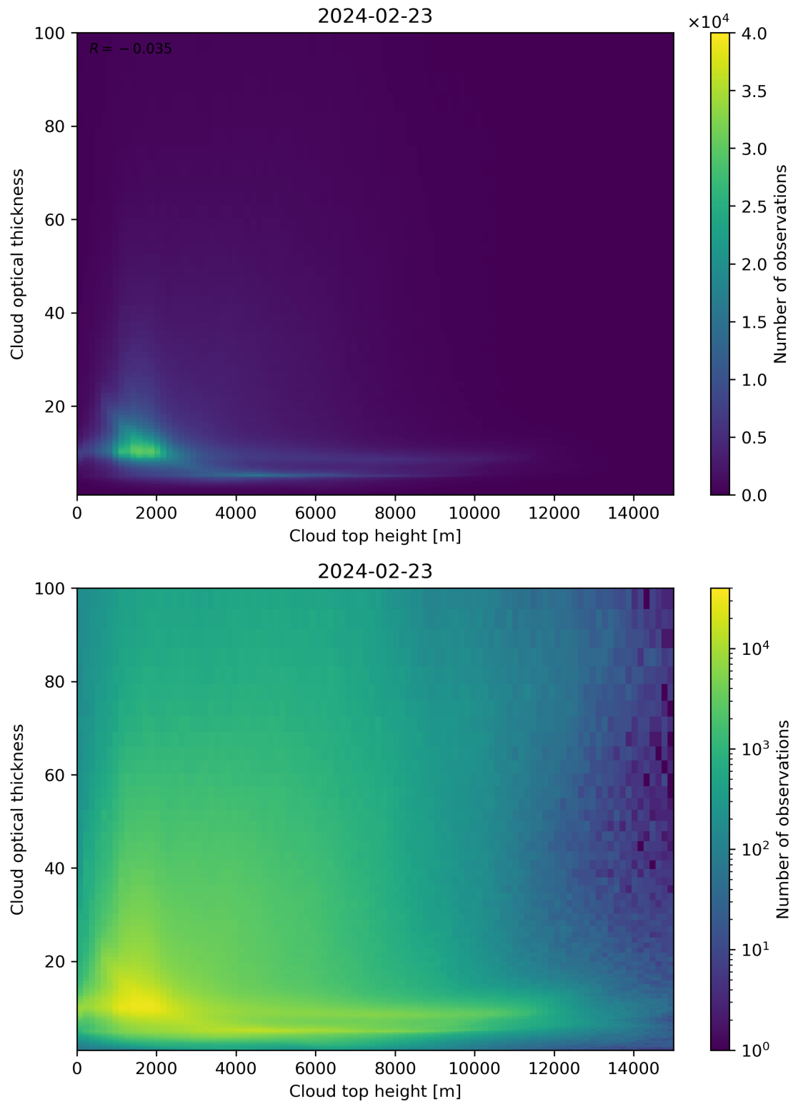
Figure 90: Scatter density plot of “Cloud top height” against “Cloud optical thickness” for 2024-02-22 to 2024-02-24.
