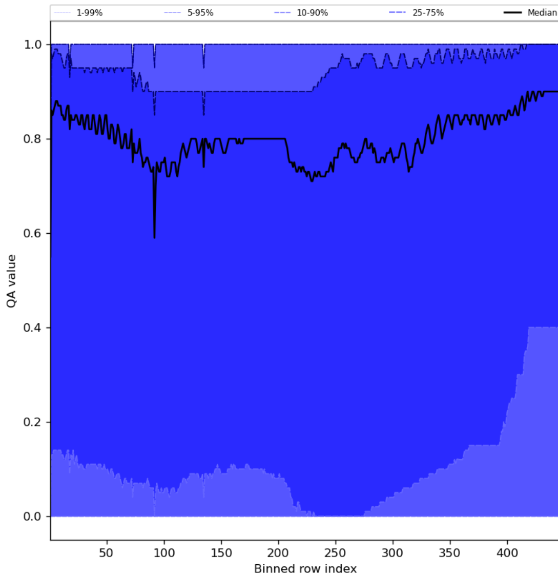
Figure 54: Along track statistics of "QA value" for 2024-02-22 to 2024-02-24
