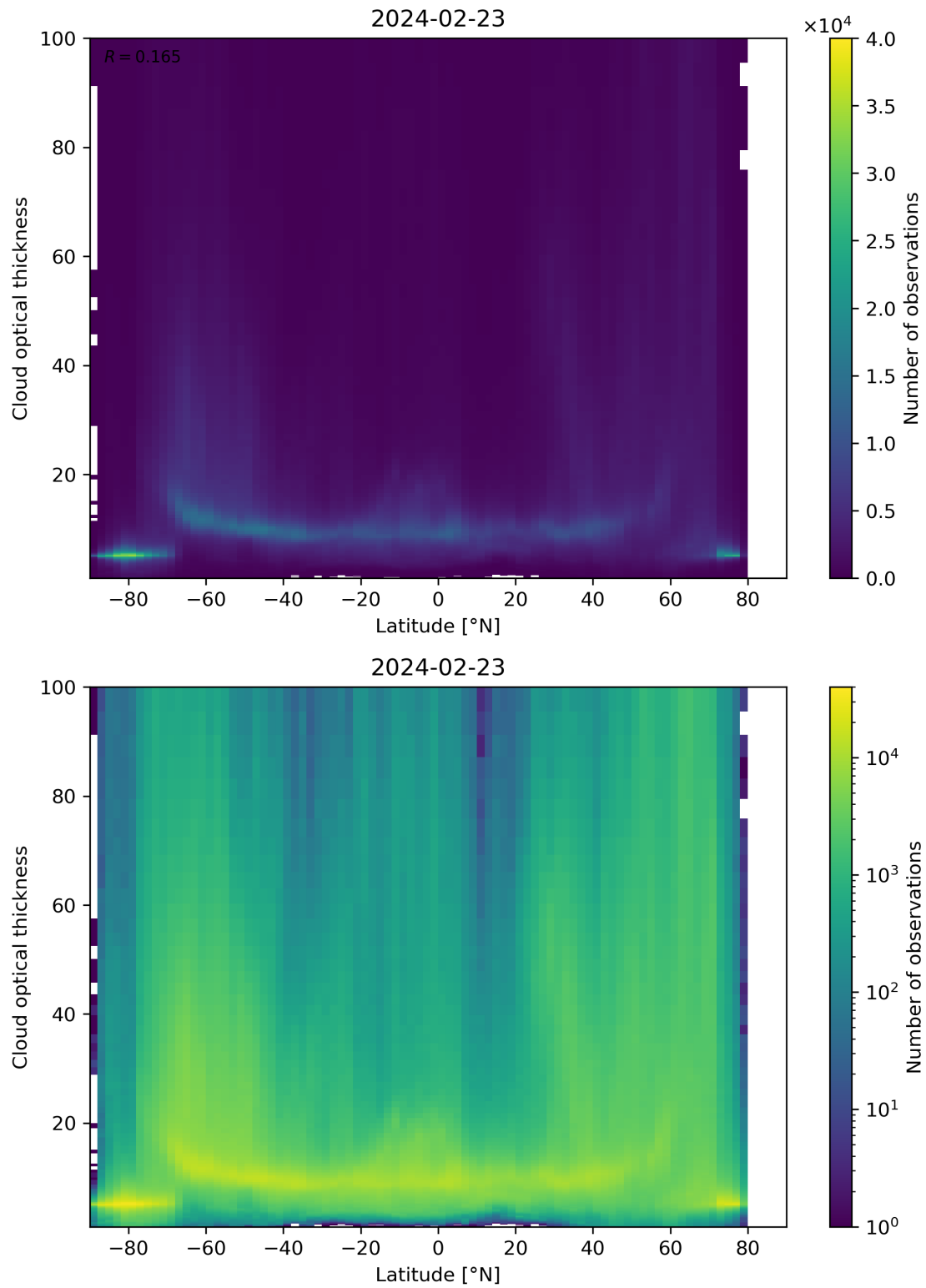
Figure 96: Scatter density plot of “Latitude” against “Cloud optical thickness” for 2024-02-22 to 2024-02-24.
