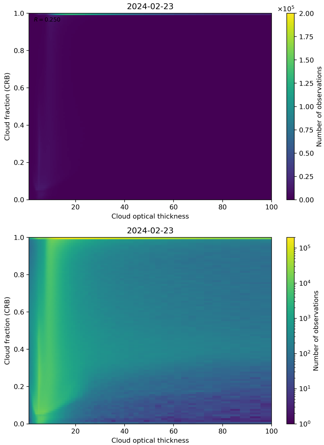
Figure 84: Scatter density plot of “Cloud optical thickness” against “Cloud fraction (CRB)” for 2024-02-22 to 2024-02-24.
