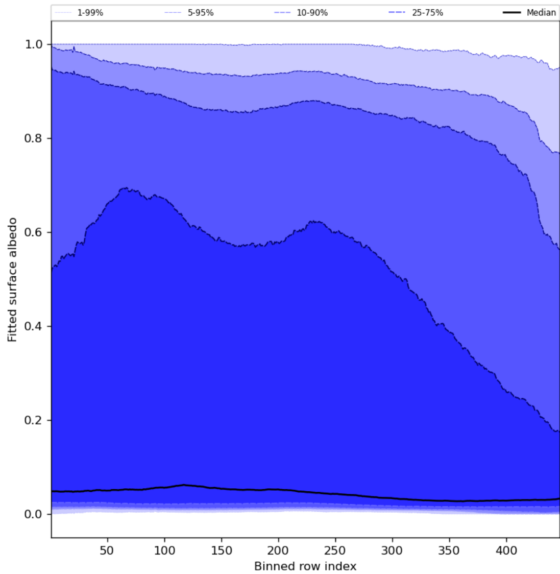
Figure 61: Along track statistics of “Fitted surface albedo” for 2024-02-22 to 2024-02-24
