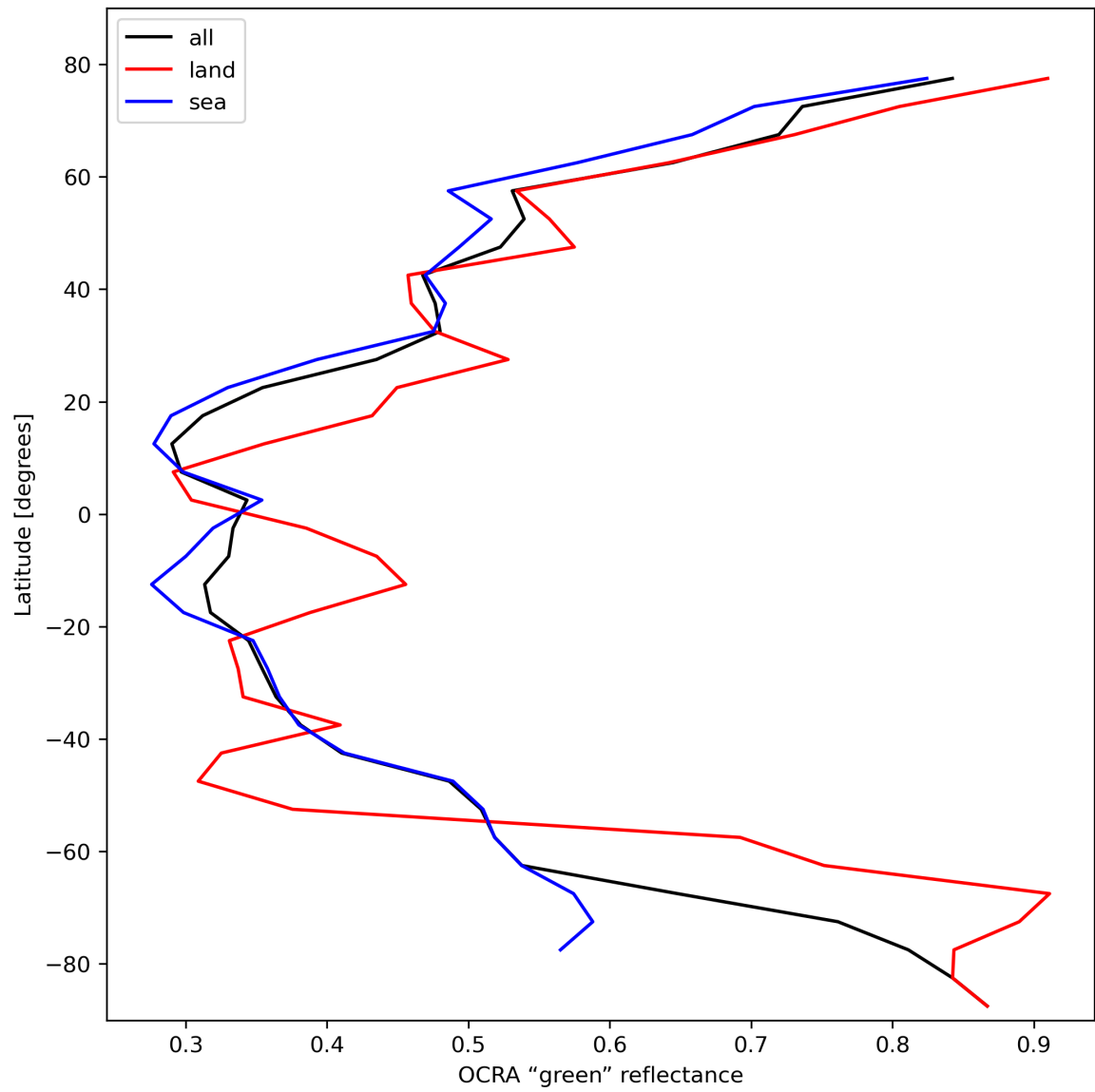
Figure 36: Zonal average of “OCRA “green” reflectance” for 2024-02-22 to 2024-02-24.
