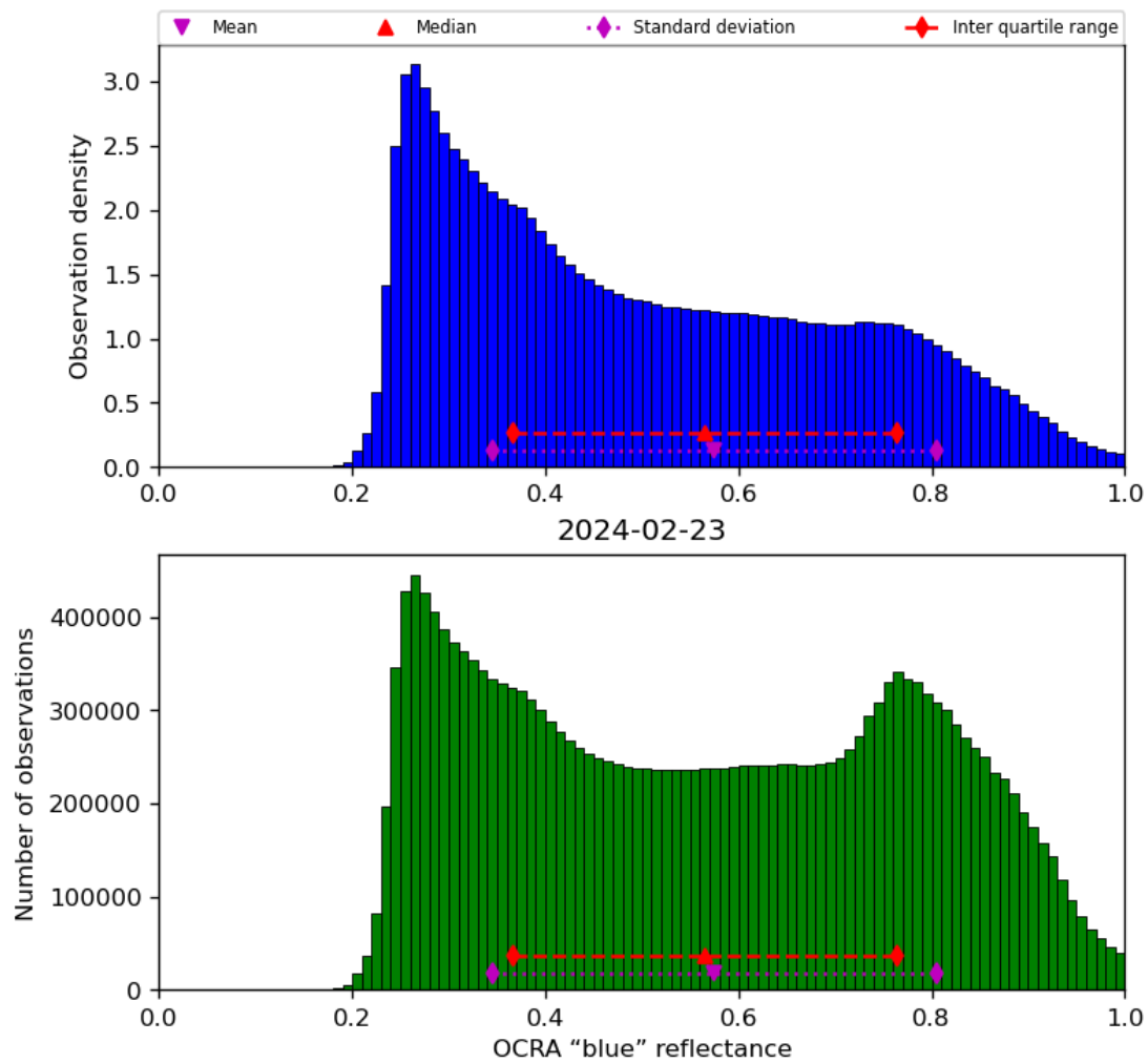
Figure 51: Histogram of “OCRA “blue” reflectance” for 2024-02-22 to 2024-02-24
