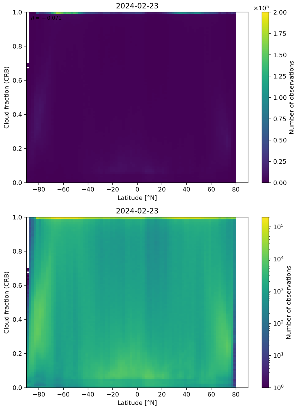
Figure 94: Scatter density plot of “Latitude” against “Cloud fraction (CRB)” for 2024-02-22 to 2024-02-24.
