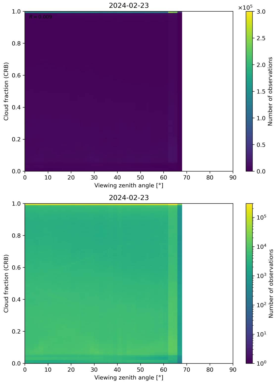
Figure 109: Scatter density plot of “Viewing zenith angle” against “Cloud fraction (CRB)” for 2024-02-22 to 2024-02-24.
