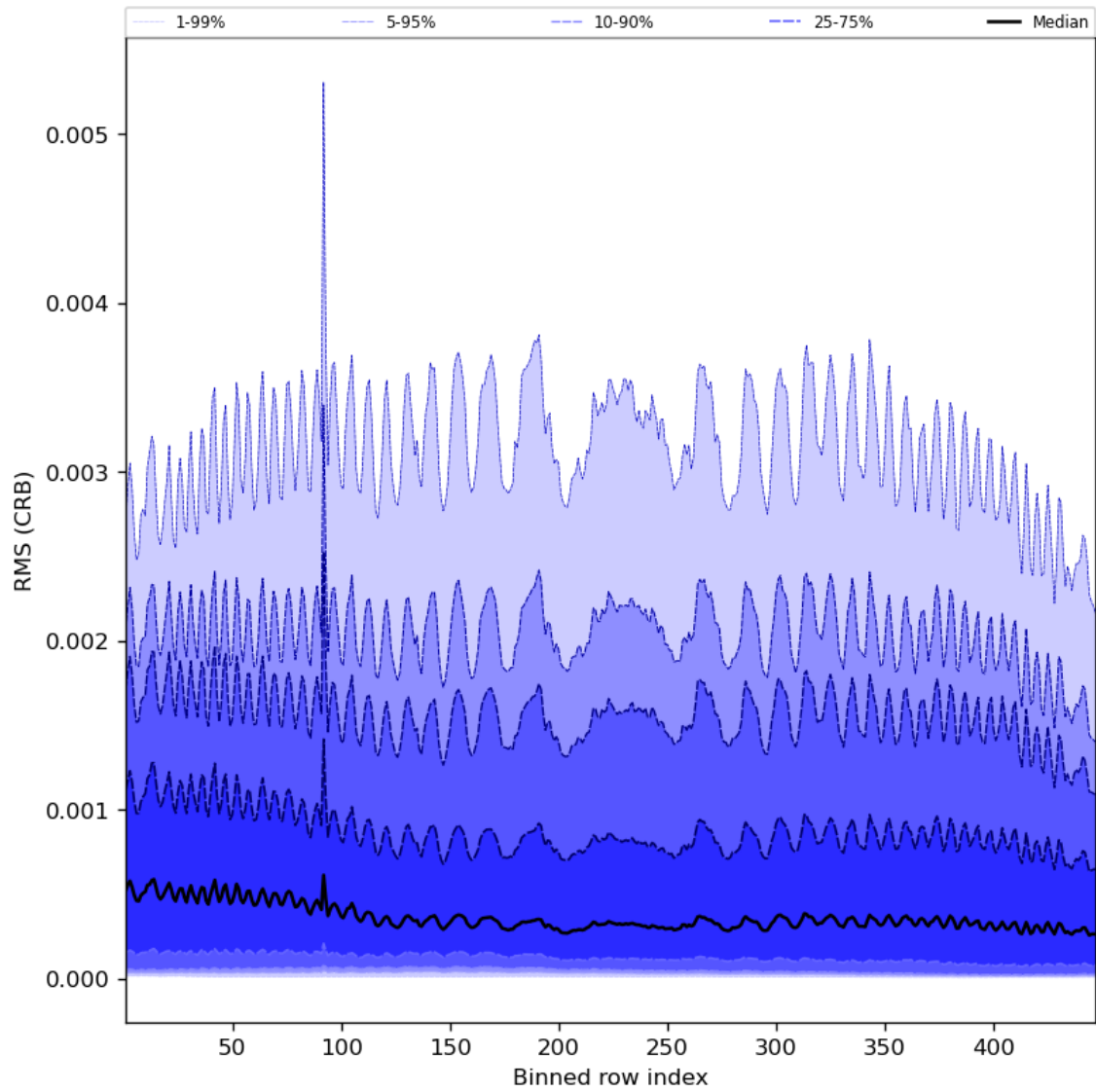
Figure 64: Along track statistics of “RMS (CRB)” for 2024-02-22 to 2024-02-24
