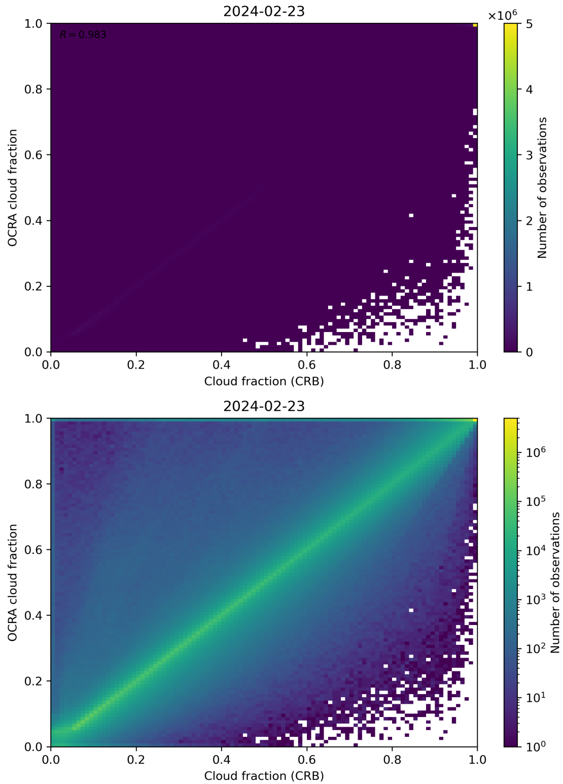
Figure 78: Scatter density plot of “Cloud fraction (CRB)” against “OCRA cloud fraction” for 2024-02-22 to 2024-02-24.
