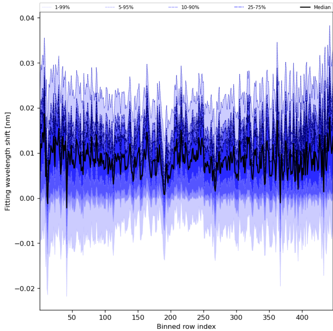
Figure 65: Along track statistics of “Fitting wavelength shift” for 2024-02-22 to 2024-02-24
