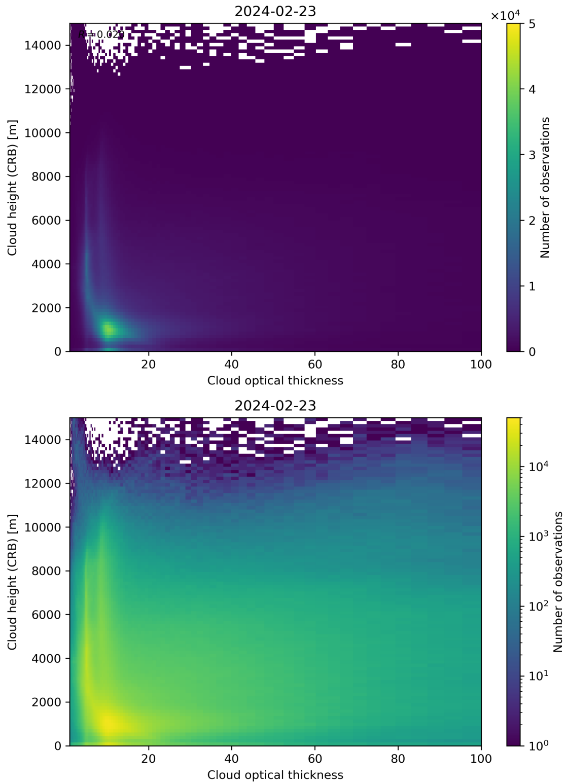
Figure 85: Scatter density plot of “Cloud optical thickness” against “Cloud height (CRB)” for 2024-02-22 to 2024-02-24.
