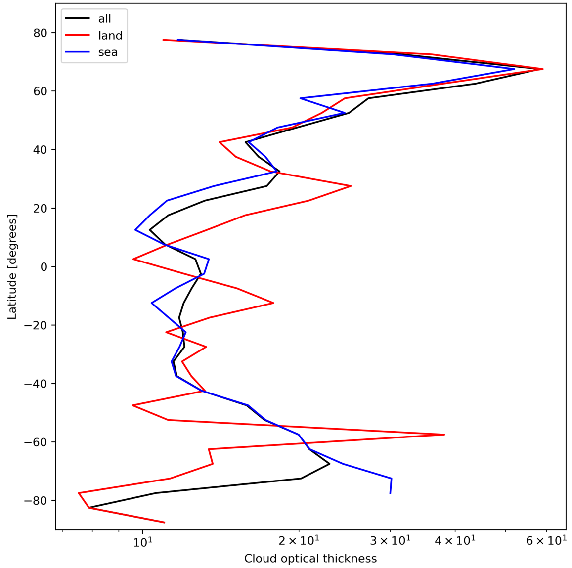
Figure 25: Zonal average of “Cloud optical thickness” for 2024-02-22 to 2024-02-24.
