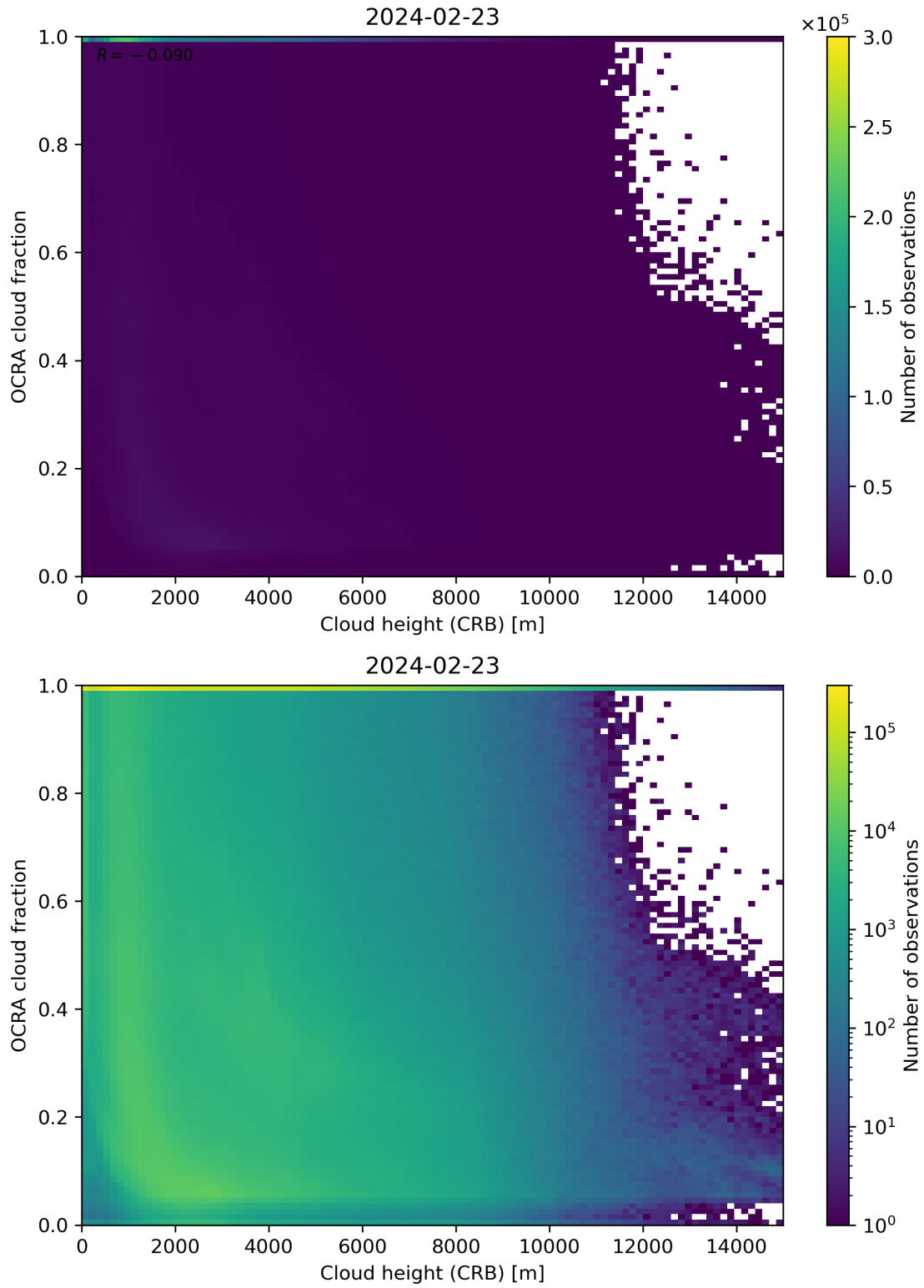
Figure 81: Scatter density plot of “Cloud height (CRB)” against “OCRA cloud fraction” for 2024-02-22 to 2024-02-24.
