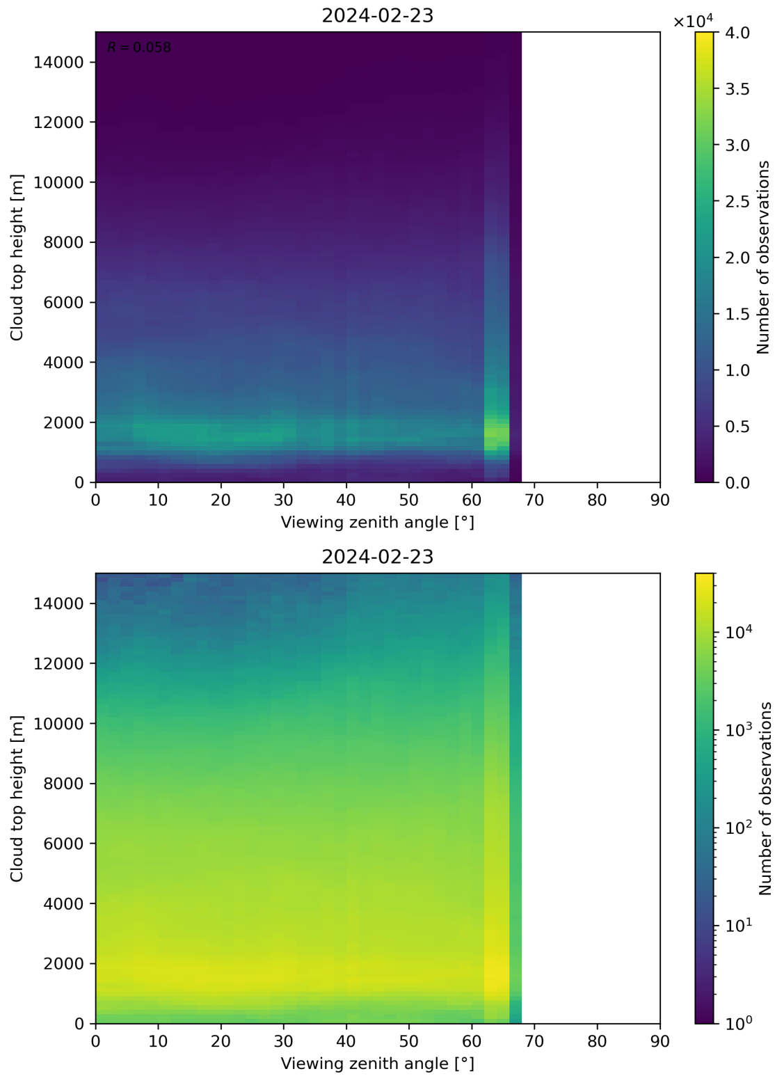
Figure 112: Scatter density plot of “Viewing zenith angle” against “Cloud top height” for 2024-02-22 to 2024-02-24.
