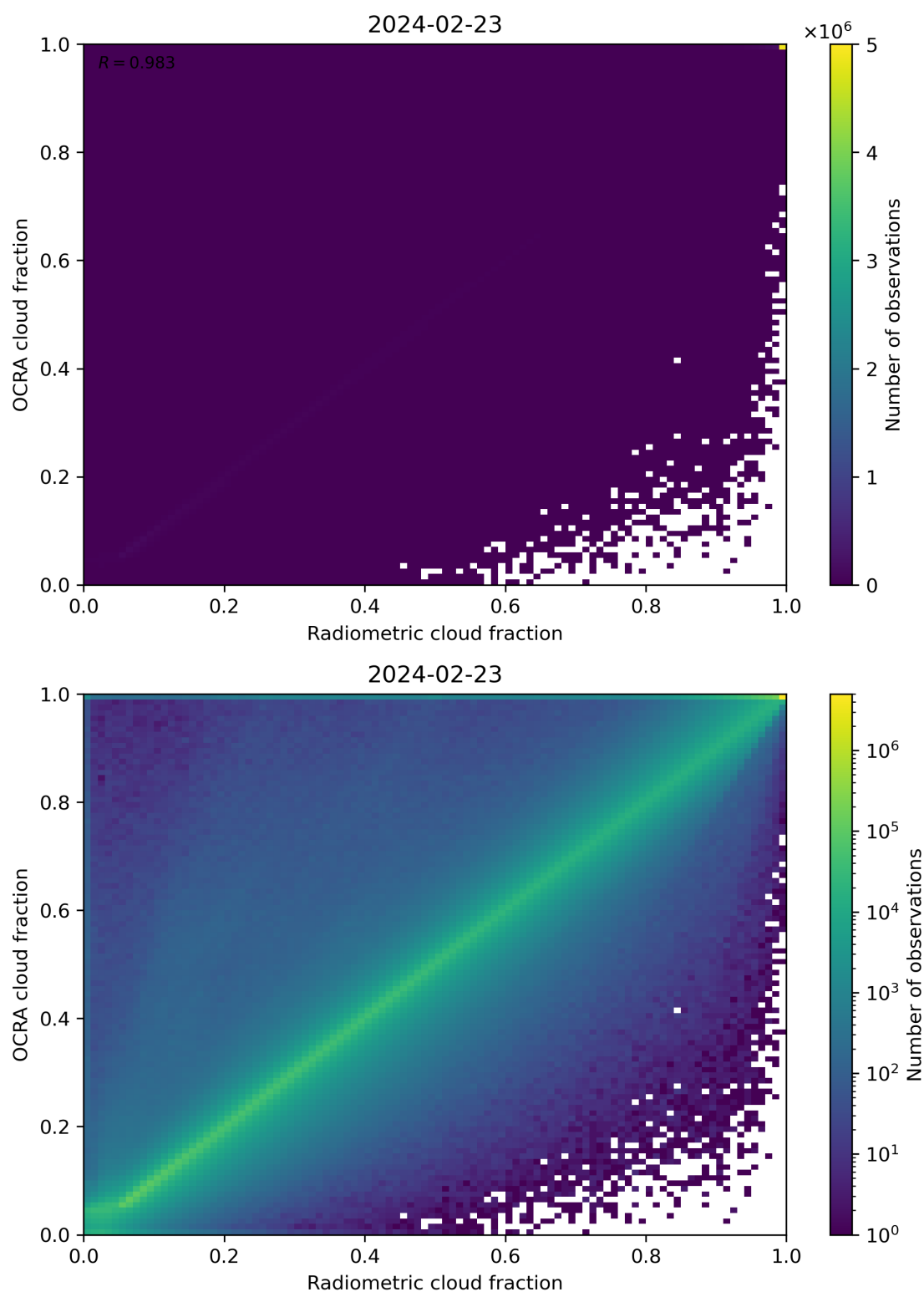
Figure 72: Scatter density plot of “Radiometric cloud fraction” against “OCRA cloud fraction” for 2024-02-22 to 2024-02-24.
