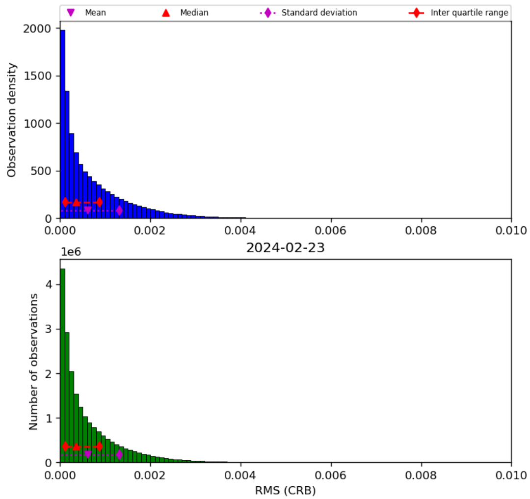
Figure 48: Histogram of “RMS (CRB)” for 2024-02-22 to 2024-02-24
