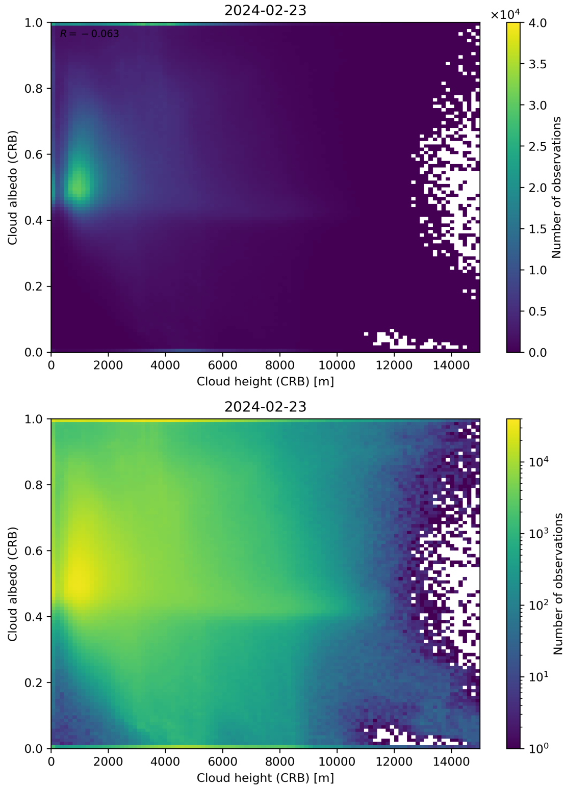
Figure 80: Scatter density plot of “Cloud height (CRB)” against “Cloud albedo (CRB)” for 2024-02-22 to 2024-02-24.
