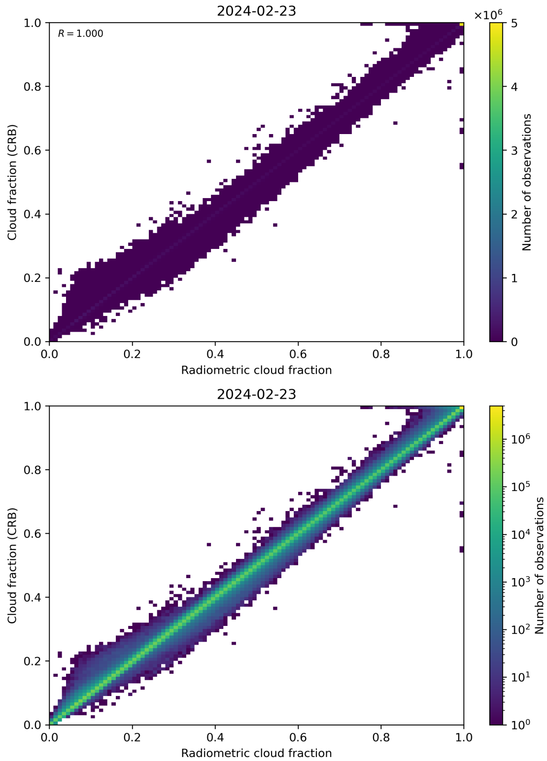
Figure 73: Scatter density plot of “Radiometric cloud fraction” against “Cloud fraction (CRB)” for 2024-02-22 to 2024-02-24.
