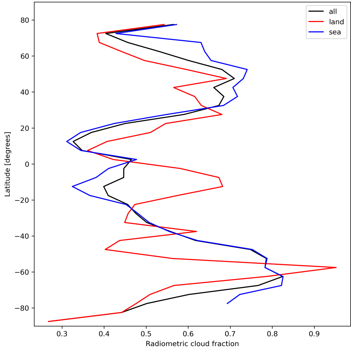
Figure 23: Zonal average of “Radiometric cloud fraction” for 2024-02-22 to 2024-02-24.
