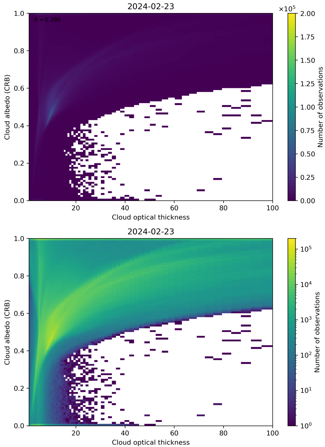
Figure 82: Scatter density plot of “Cloud optical thickness” against “Cloud albedo (CRB)” for 2024-02-22 to 2024-02-24.
