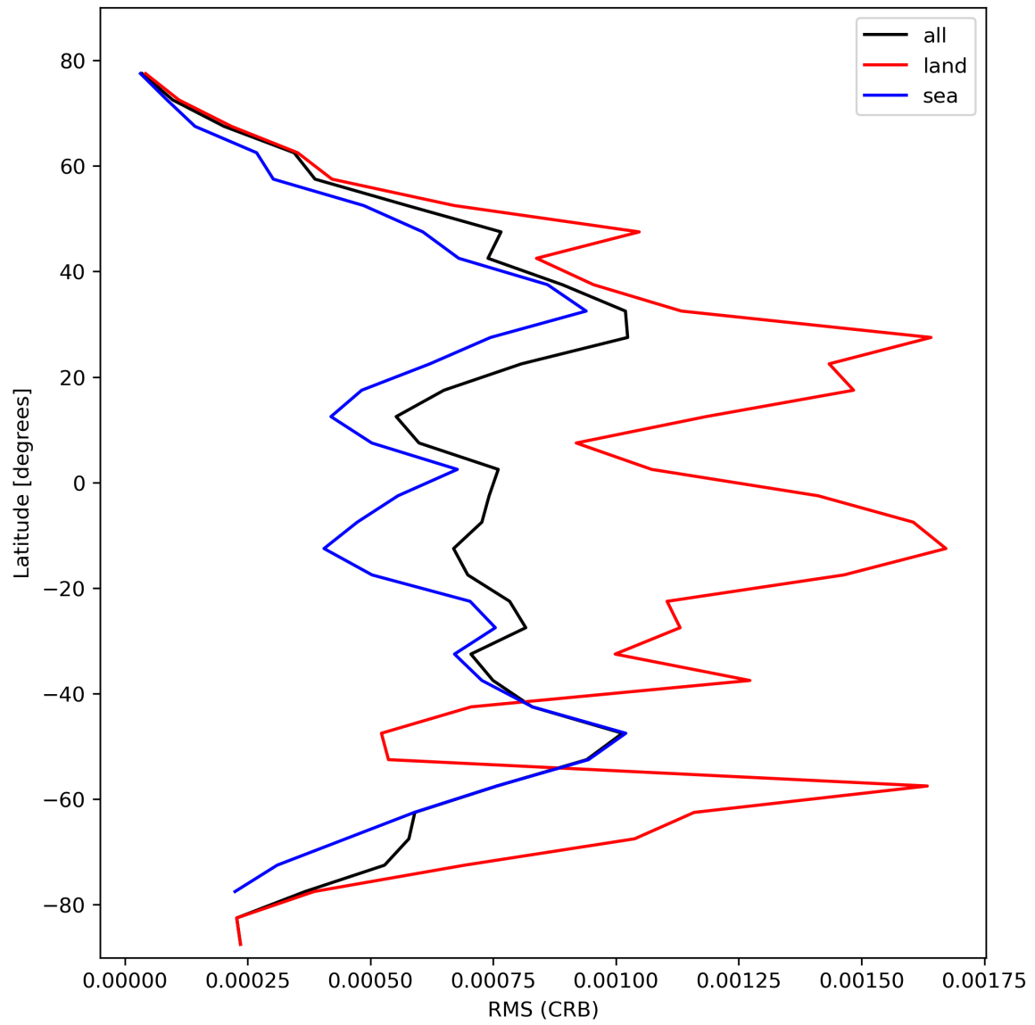
Figure 32: Zonal average of “RMS (CRB)” for 2024-02-22 to 2024-02-24.
