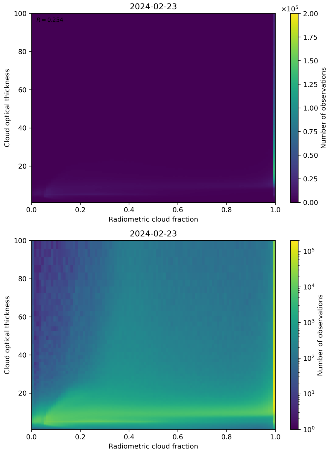
Figure 75: Scatter density plot of “Radiometric cloud fraction” against “Cloud optical thickness” for 2024-02-22 to 2024-02-24.
