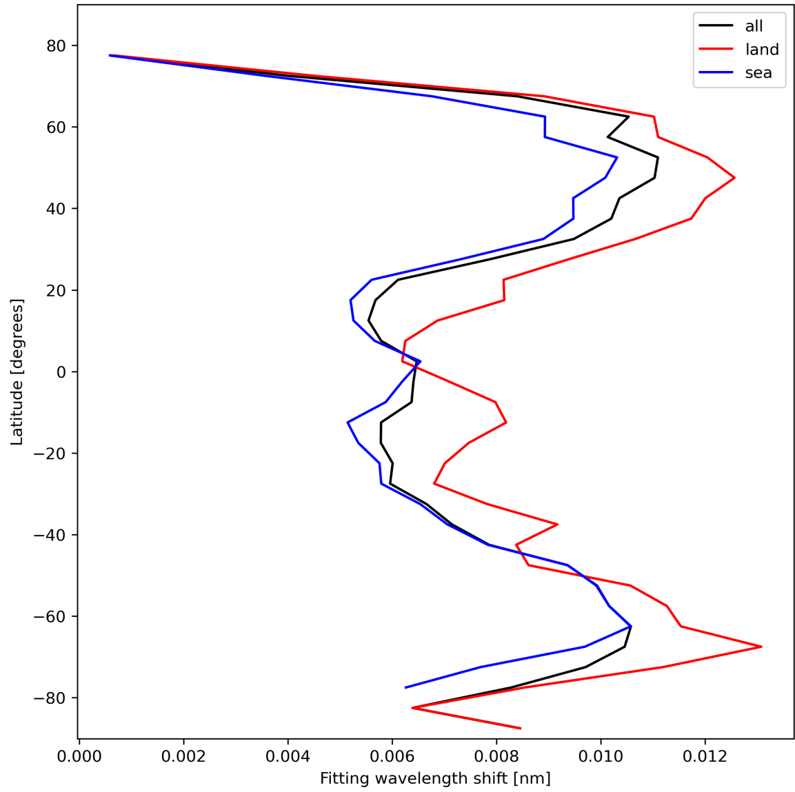
Figure 33: Zonal average of “Fitting wavelength shift” for 2024-02-22 to 2024-02-24.
