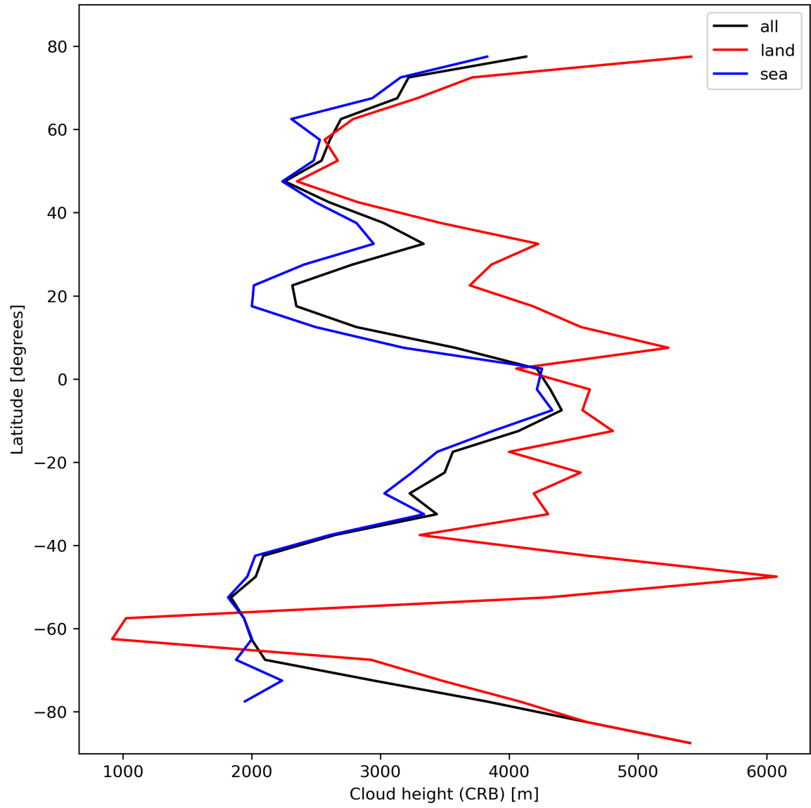
Figure 27: Zonal average of “Cloud height (CRB)” for 2024-02-22 to 2024-02-24.
