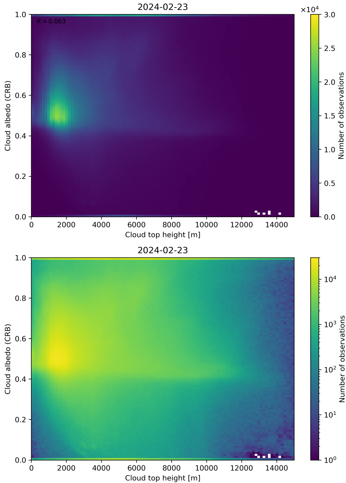
Figure 86: Scatter density plot of “Cloud top height” against “Cloud albedo (CRB)” for 2024-02-22 to 2024-02-24.
