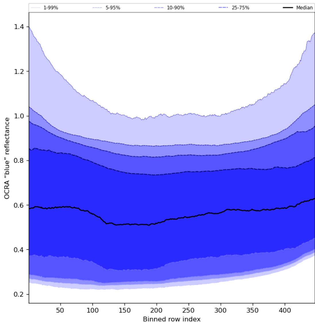
Figure 67: Along track statistics of “OCRA “blue” reflectance” for 2024-02-22 to 2024-02-24
