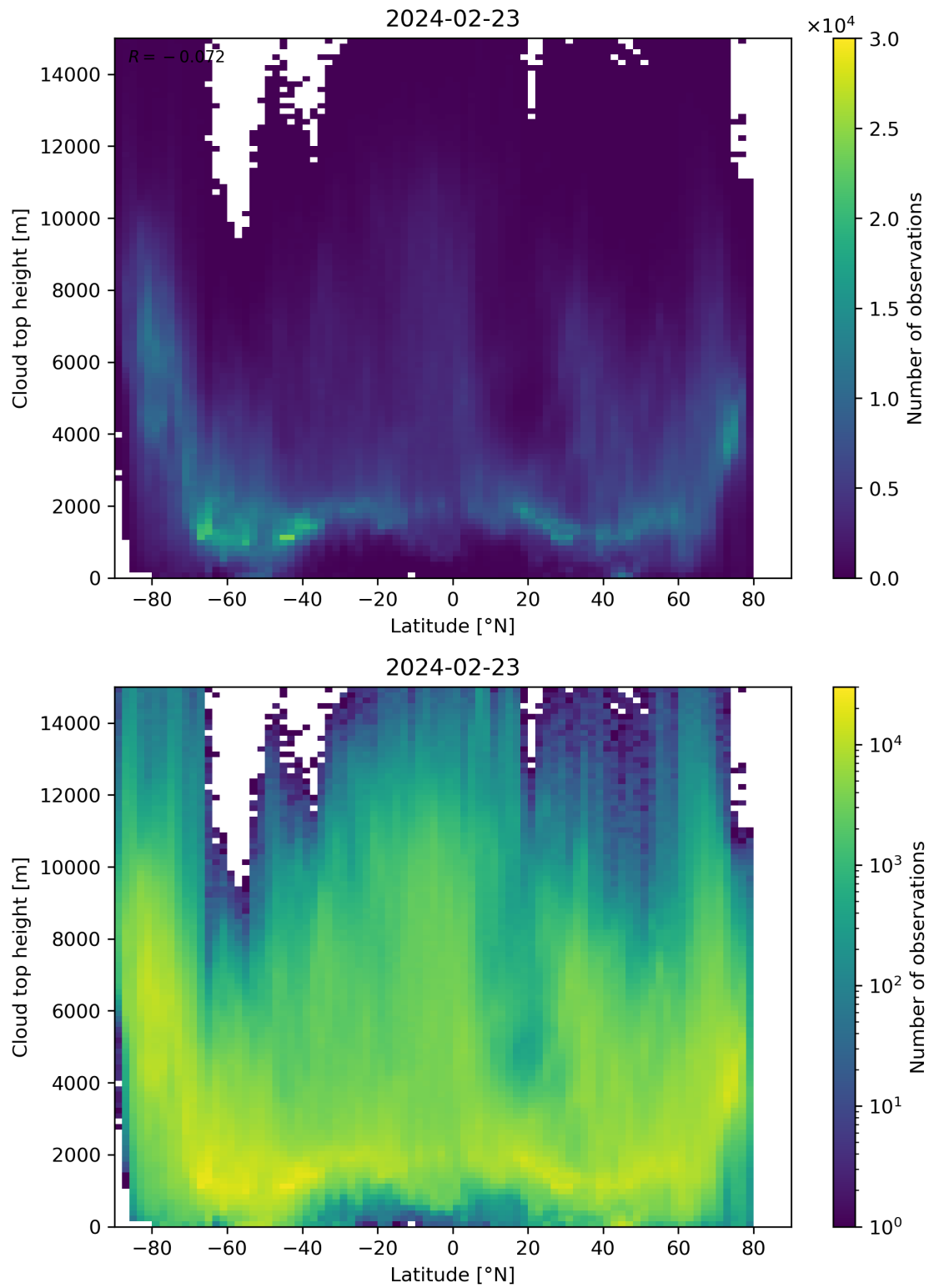
Figure 97: Scatter density plot of “Latitude” against “Cloud top height” for 2024-02-22 to 2024-02-24.
