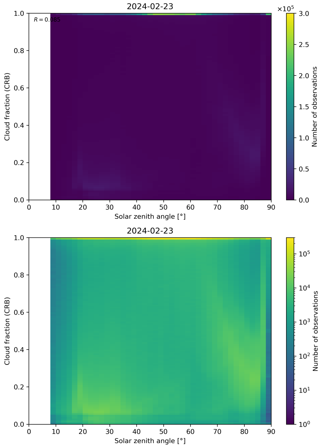
Figure 101: Scatter density plot of “Solar zenith angle” against “Cloud fraction (CRB)” for 2024-02-22 to 2024-02-24.
