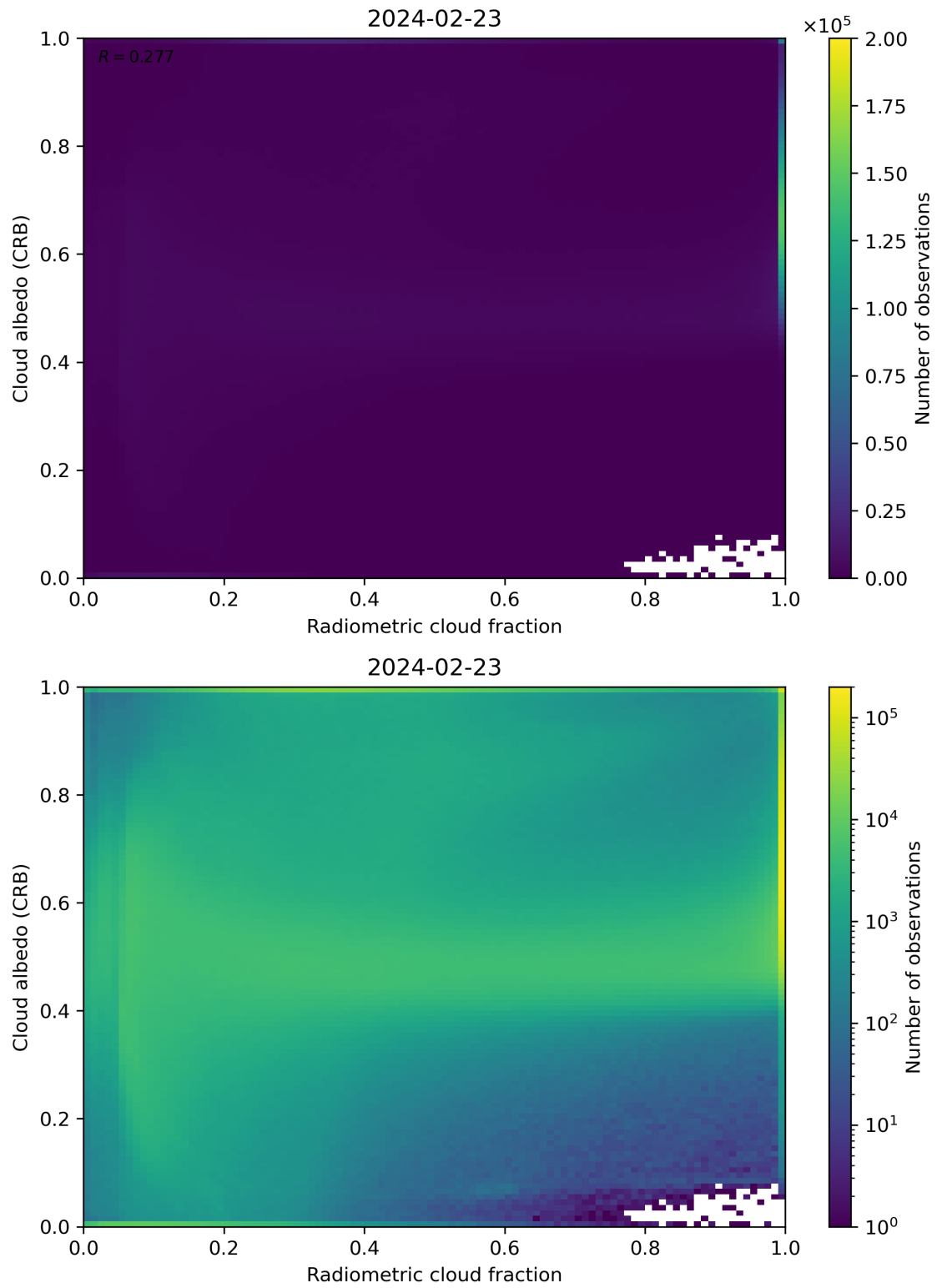
Figure 71: Scatter density plot of “Radiometric cloud fraction” against “Cloud albedo (CRB)” for 2024-02-22 to 2024-02-24.
