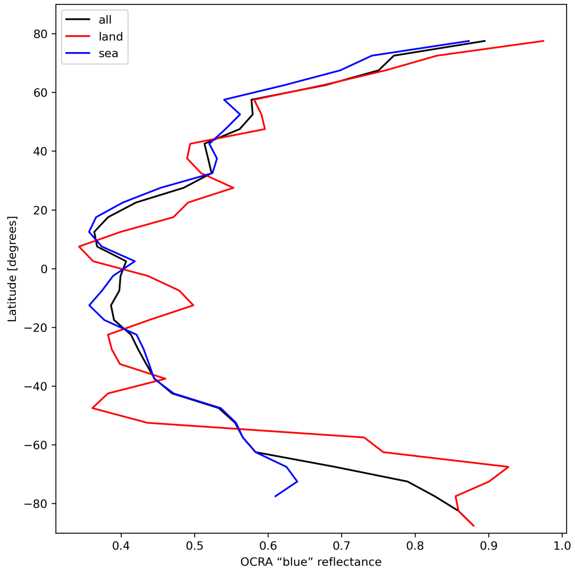
Figure 35: Zonal average of “OCRA “blue” reflectance” for 2024-02-22 to 2024-02-24.
