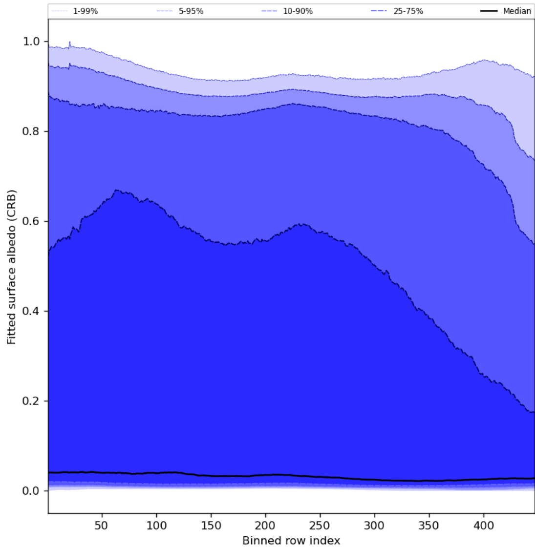
Figure 62: Along track statistics of “Fitted surface albedo (CRB)” for 2024-02-22 to 2024-02-24
