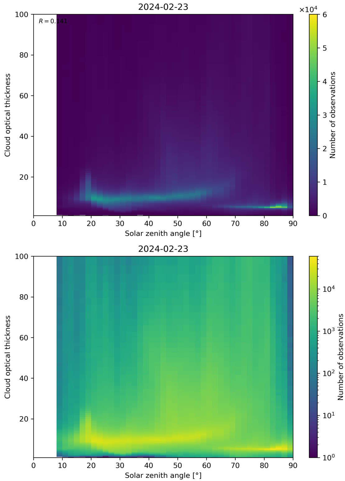
Figure 103: Scatter density plot of “Solar zenith angle” against “Cloud optical thickness” for 2024-02-22 to 2024-02-24.
