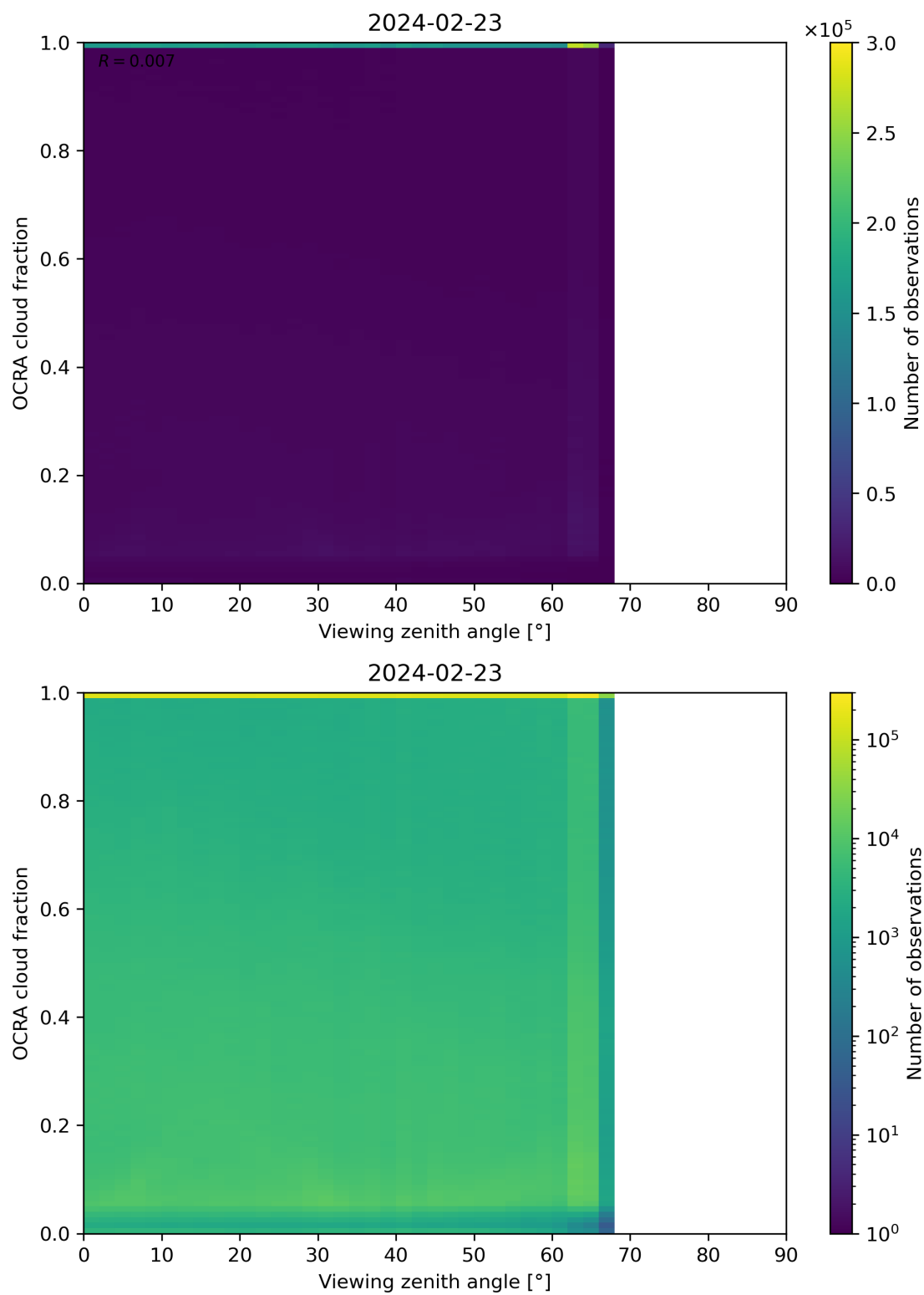
Figure 108: Scatter density plot of “Viewing zenith angle” against “OCRA cloud fraction” for 2024-02-22 to 2024-02-24.
