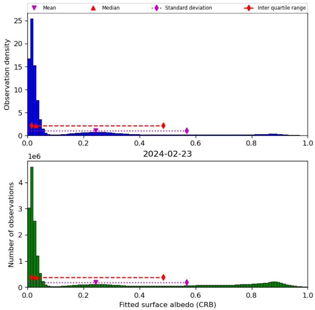
Figure 46: Histogram of “Fitted surface albedo (CRB)” for 2024-02-22 to 2024-02-24
