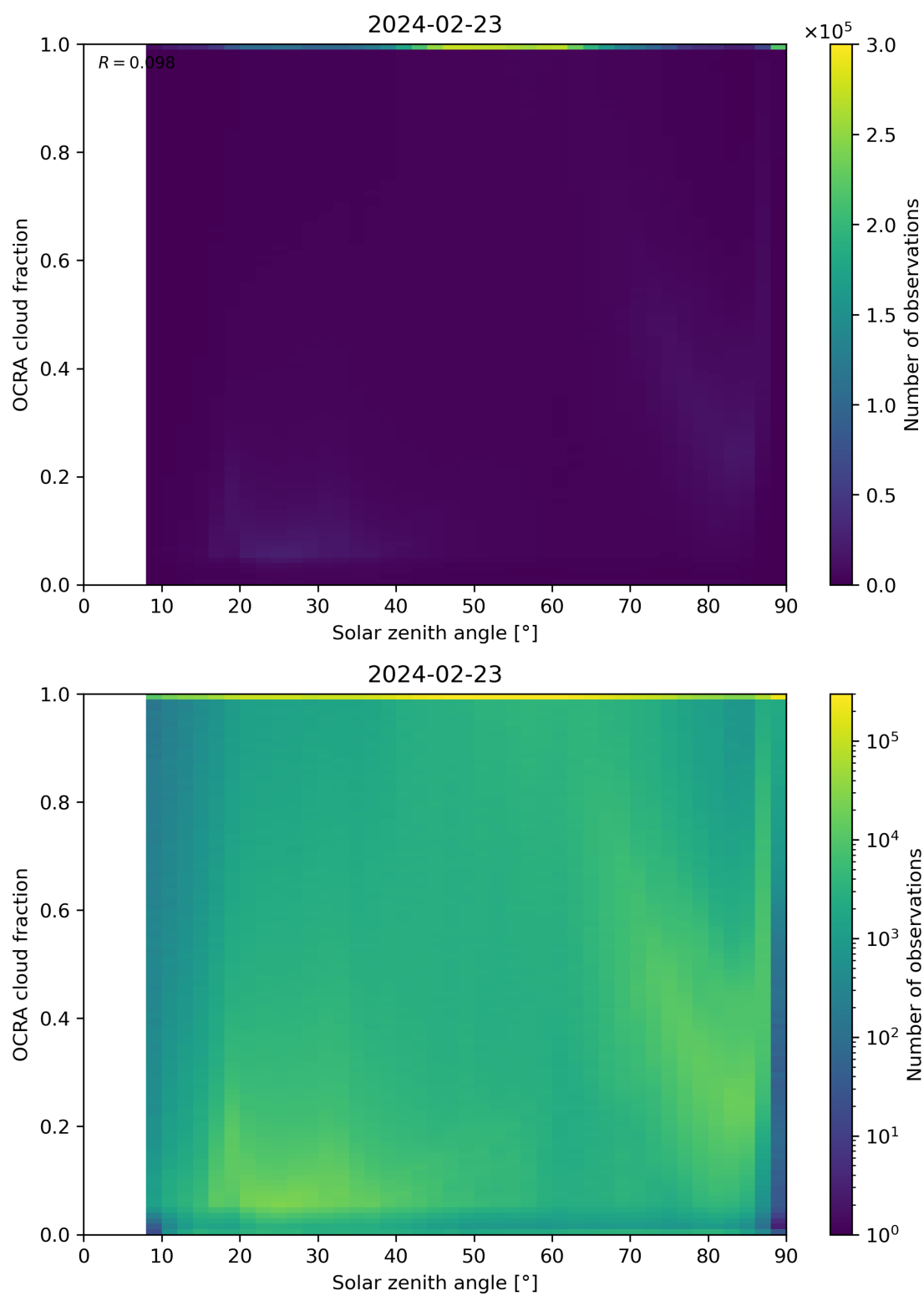
Figure 100: Scatter density plot of “Solar zenith angle” against “OCRA cloud fraction” for 2024-02-22 to 2024-02-24.
