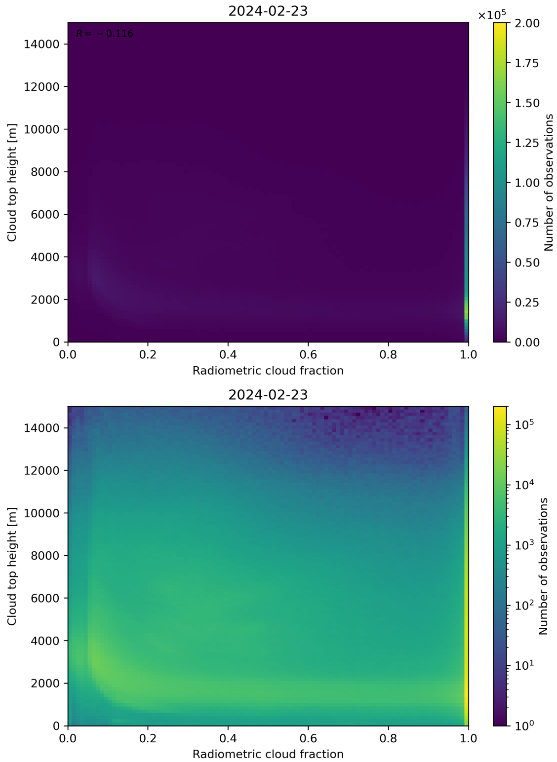
Figure 76: Scatter density plot of “Radiometric cloud fraction” against “Cloud top height” for 2024-02-22 to 2024-02-24.
