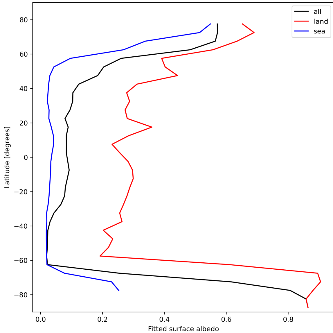
Figure 29: Zonal average of “Fitted surface albedo” for 2024-02-22 to 2024-02-24.
