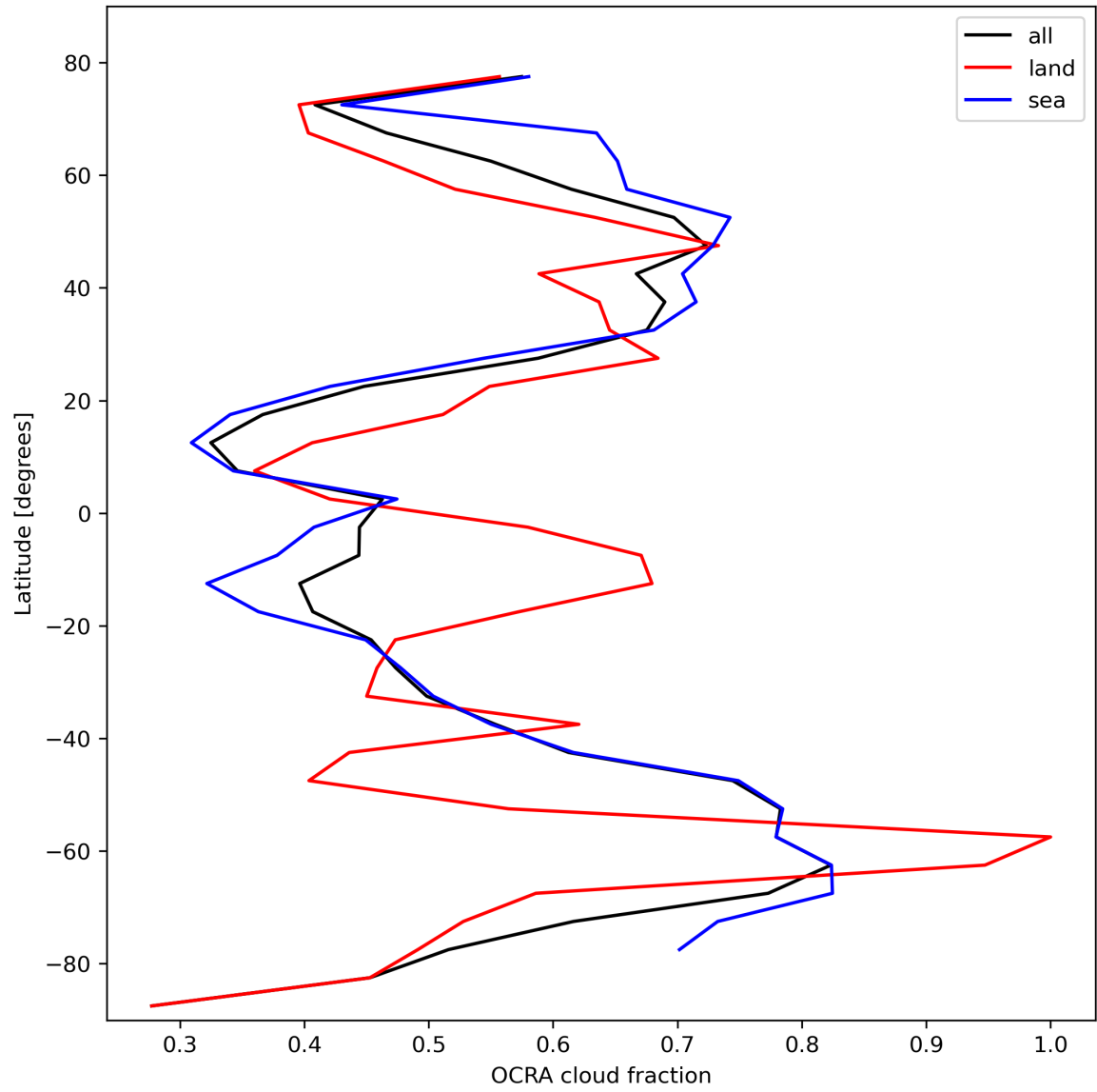
Figure 34: Zonal average of “OCRA cloud fraction” for 2024-02-22 to 2024-02-24.
