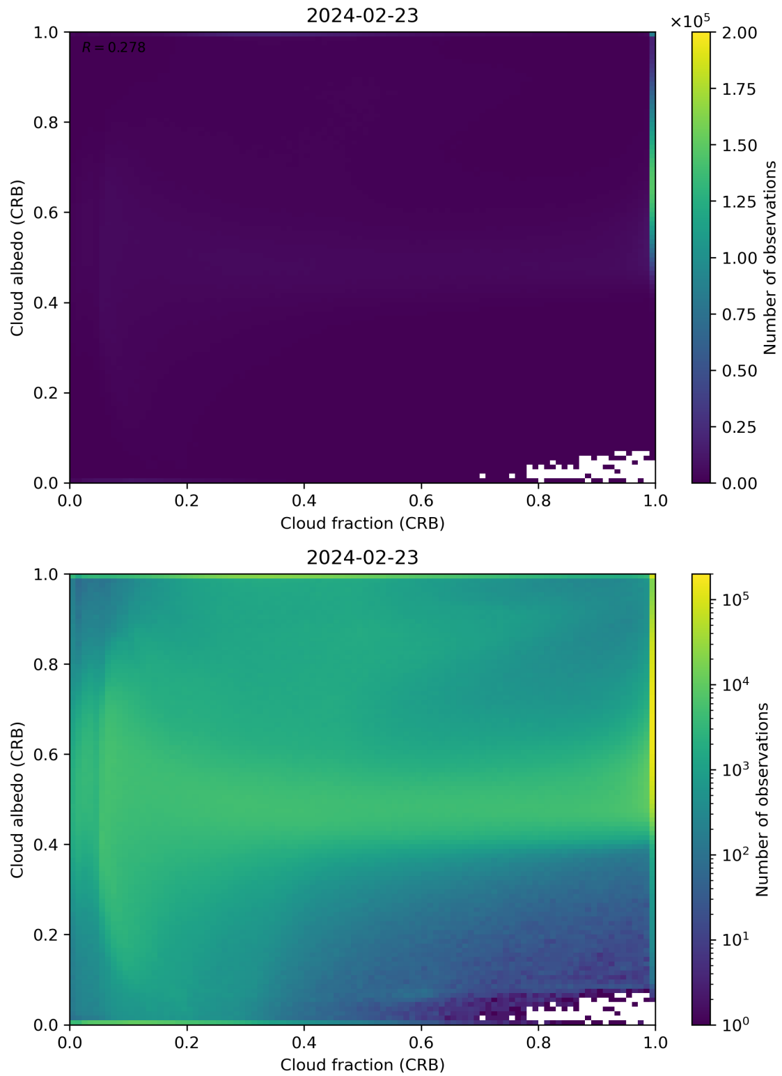
Figure 77: Scatter density plot of “Cloud fraction (CRB)” against “Cloud albedo (CRB)” for 2024-02-22 to 2024-02-24.
