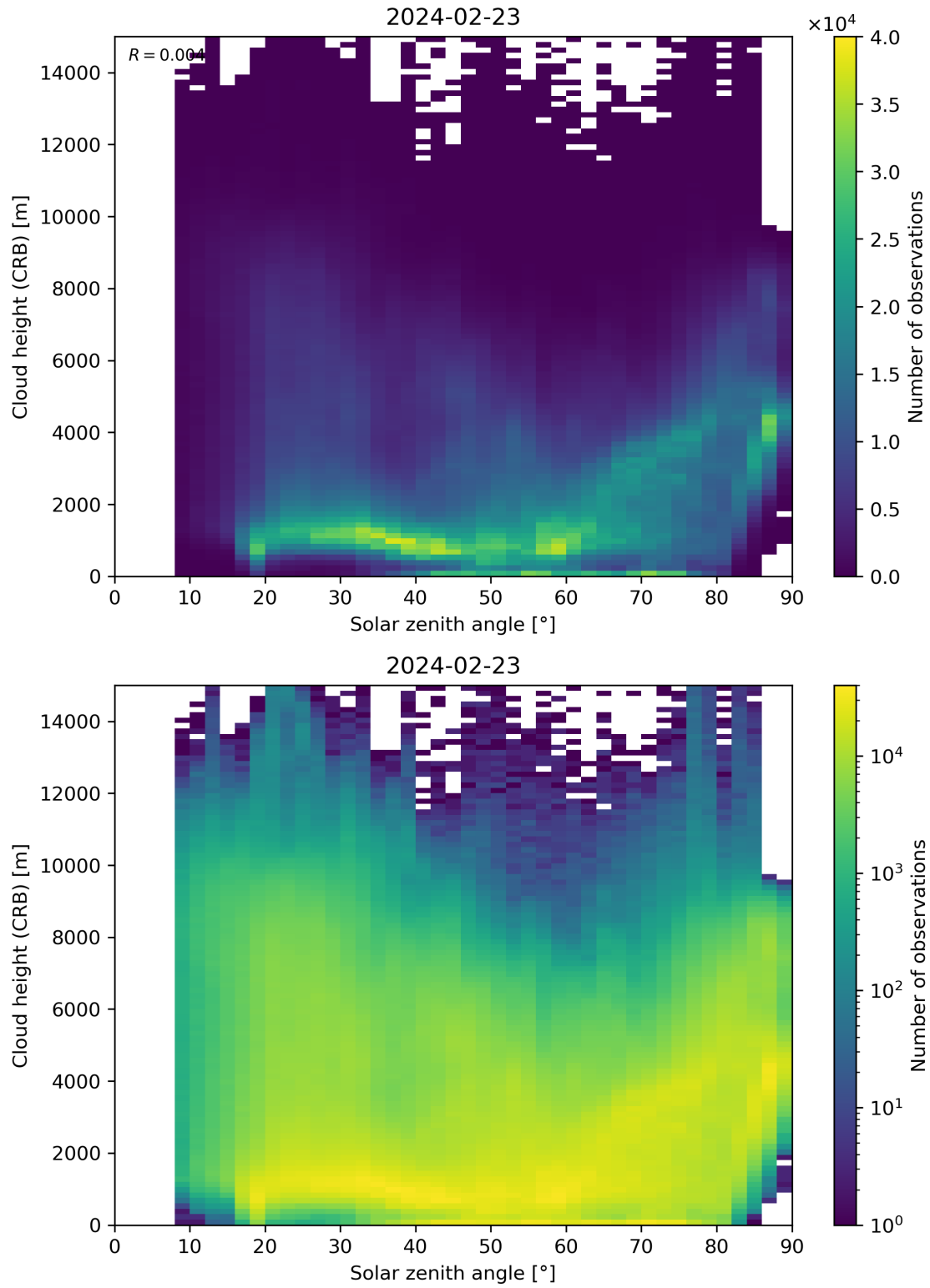
Figure 102: Scatter density plot of “Solar zenith angle” against “Cloud height (CRB)” for 2024-02-22 to 2024-02-24.
