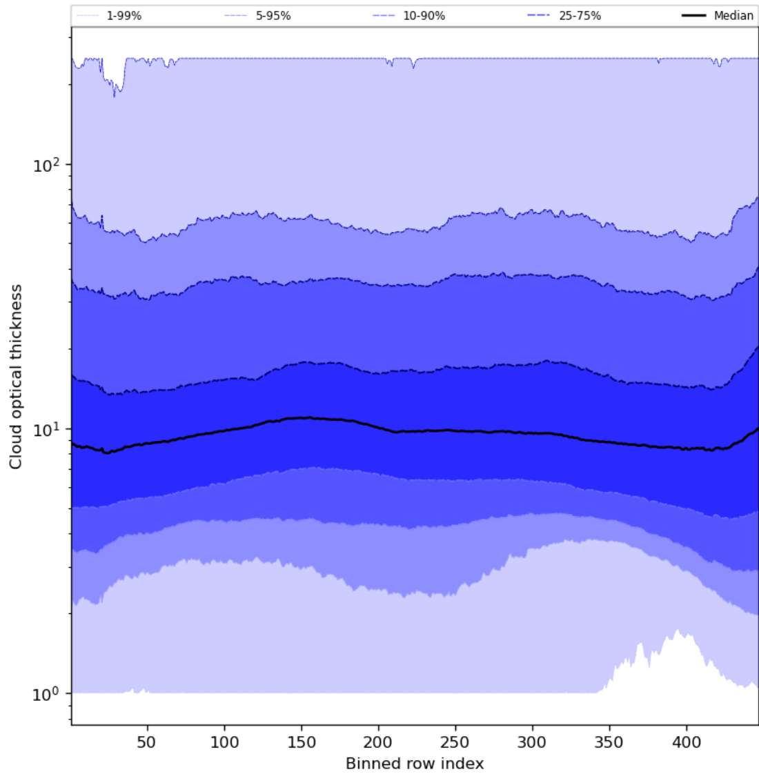
Figure 57: Along track statistics of “Cloud optical thickness” for 2024-02-22 to 2024-02-24
