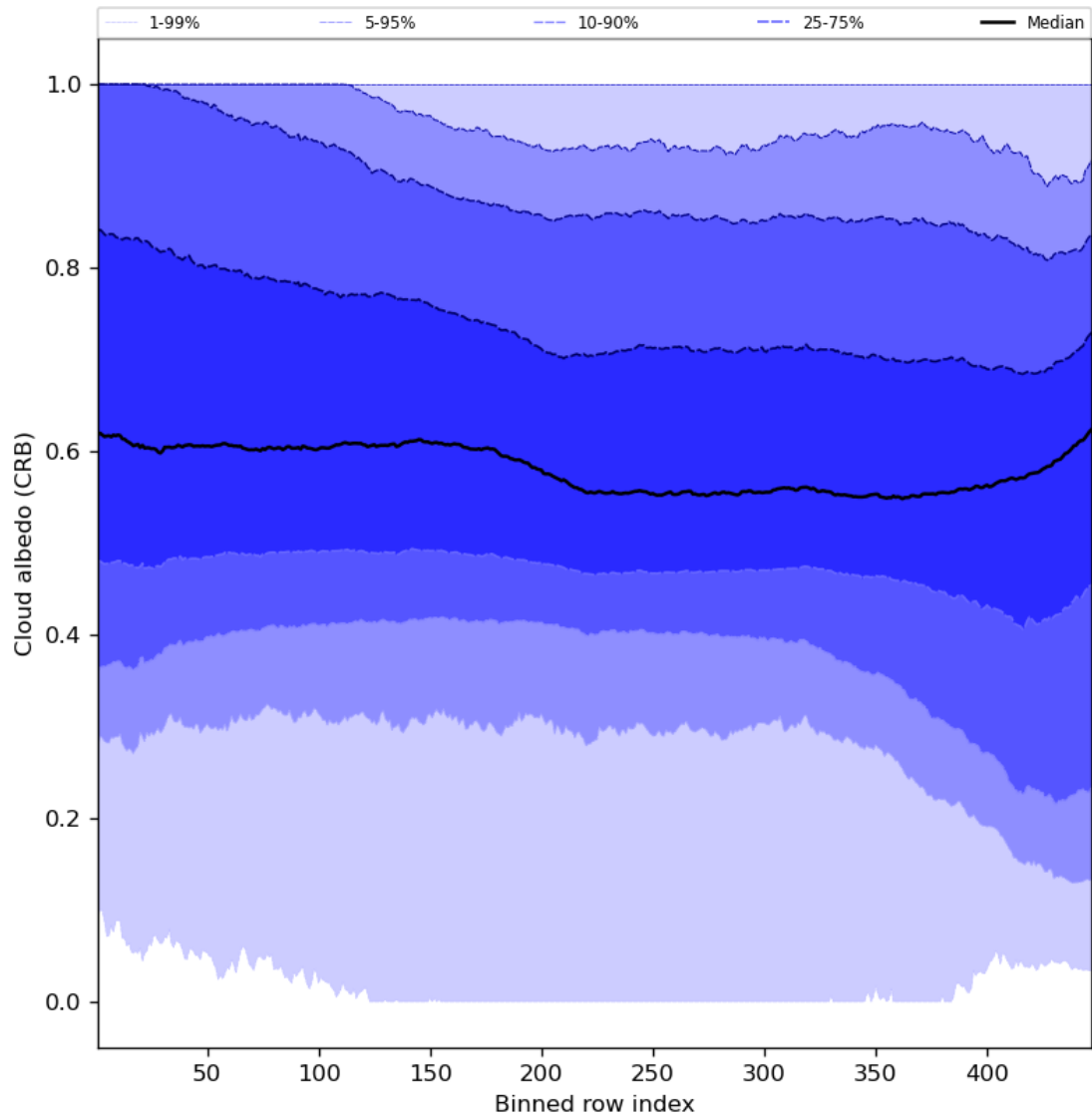
Figure 60: Along track statistics of “Cloud albedo (CRB)” for 2024-02-22 to 2024-02-24
