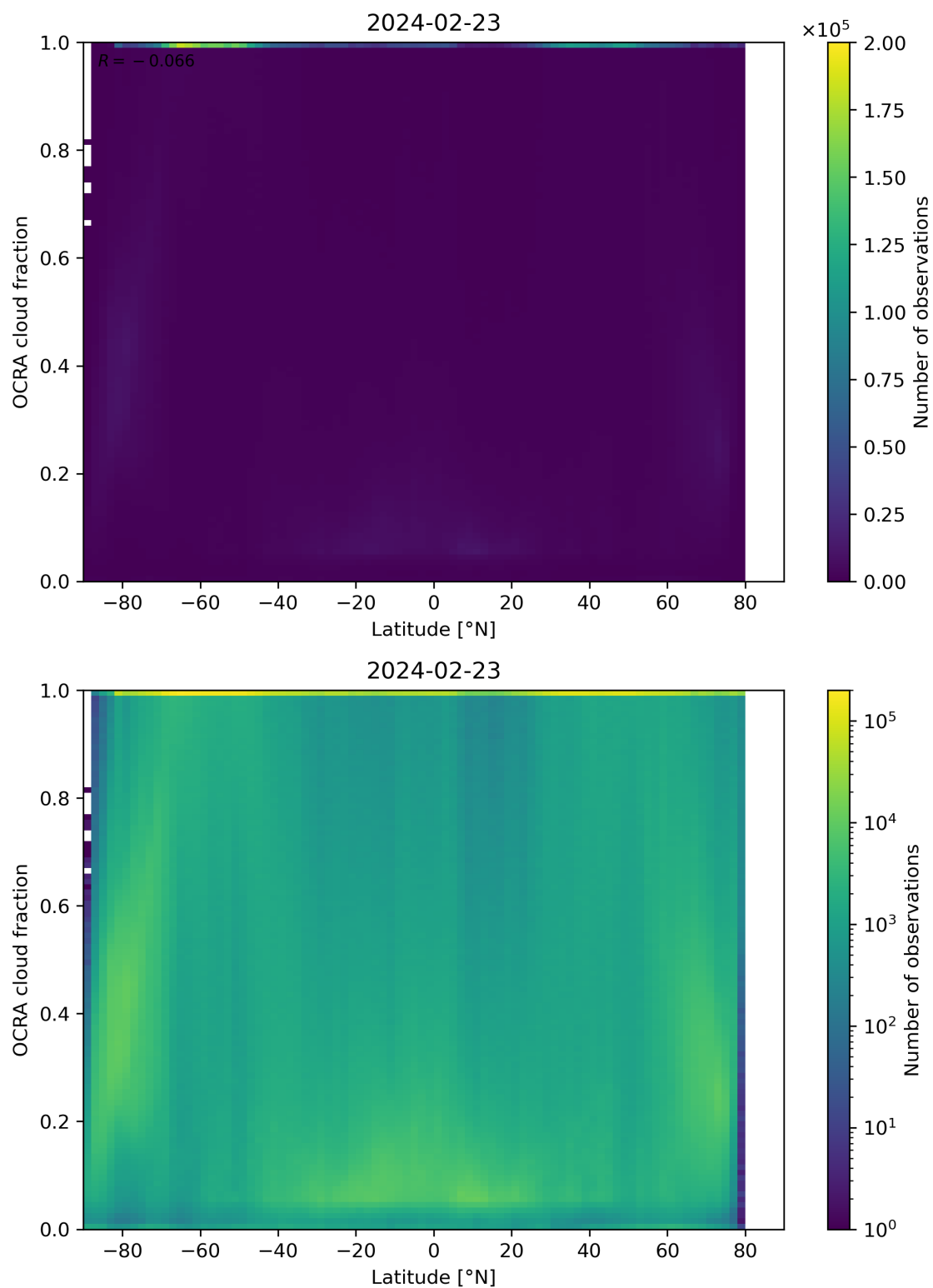
Figure 93: Scatter density plot of “Latitude” against “OCRA cloud fraction” for 2024-02-22 to 2024-02-24.
