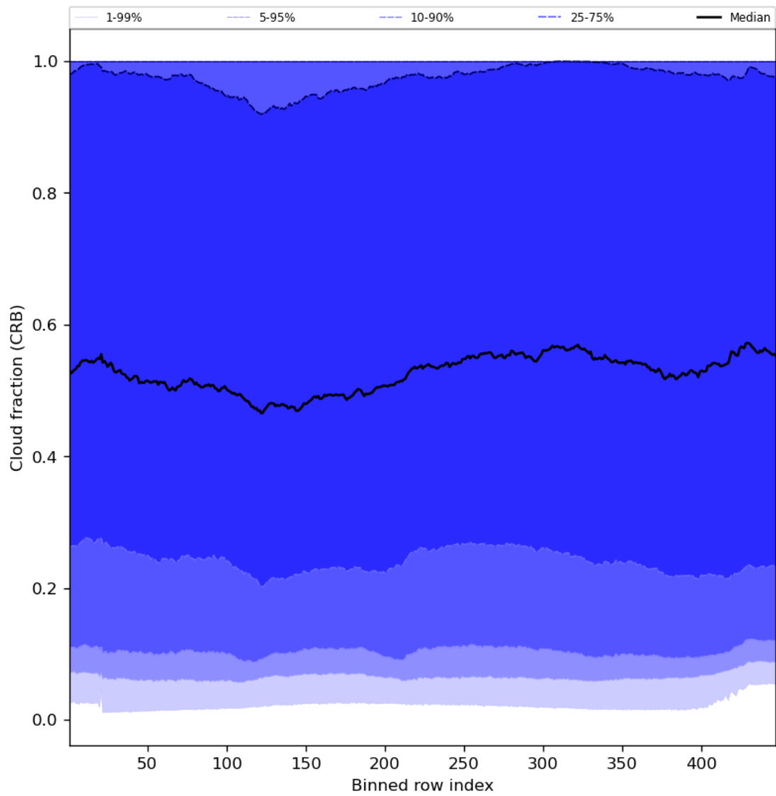
Figure 58: Along track statistics of “Cloud fraction (CRB)” for 2024-02-22 to 2024-02-24
