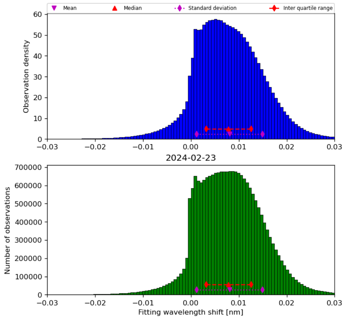
Figure 49: Histogram of “Fitting wavelength shift” for 2024-02-22 to 2024-02-24
