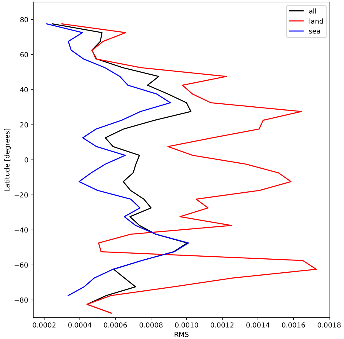
Figure 31: Zonal average of “RMS” for 2024-02-22 to 2024-02-24.
