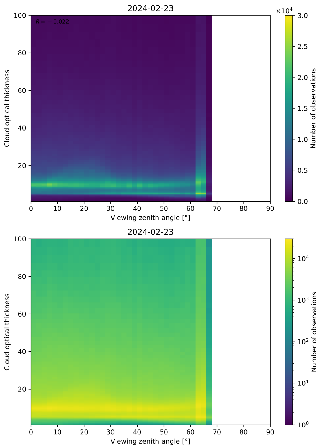
Figure 111: Scatter density plot of “Viewing zenith angle” against “Cloud optical thickness” for 2024-02-22 to 2024-02-24.
