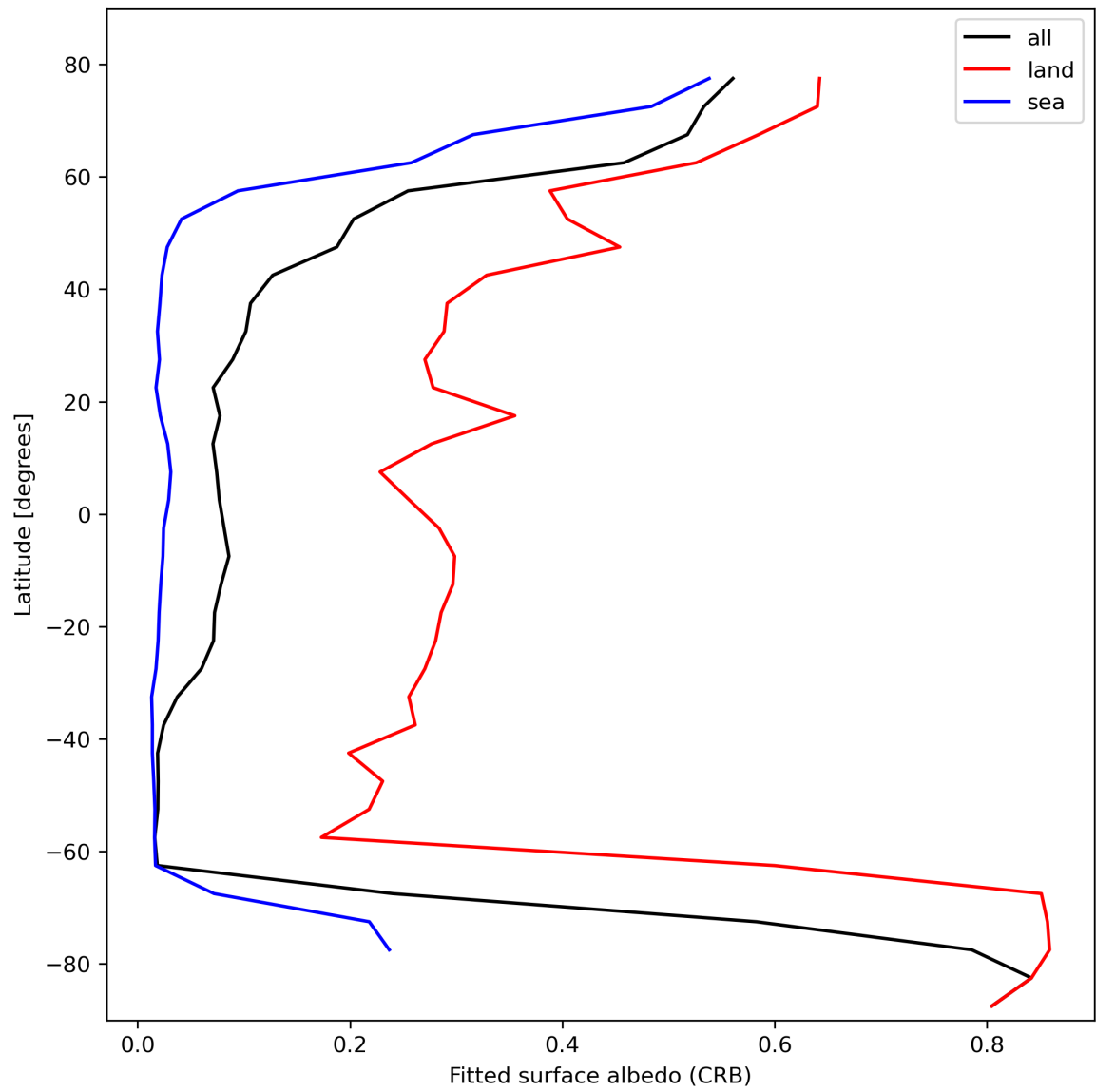
Figure 30: Zonal average of “Fitted surface albedo (CRB)” for 2024-02-22 to 2024-02-24.
