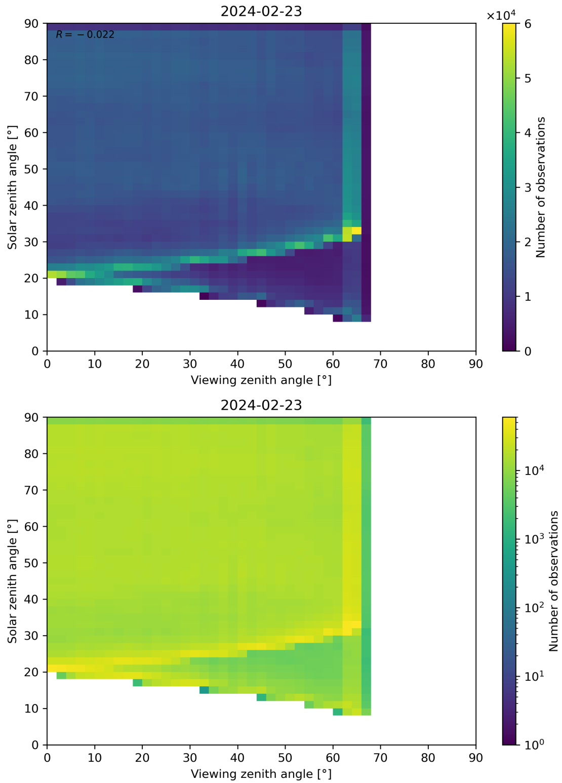
Figure 114: Scatter density plot of “Viewing zenith angle” against “Solar zenith angle” for 2024-02-22 to 2024-02-24.
