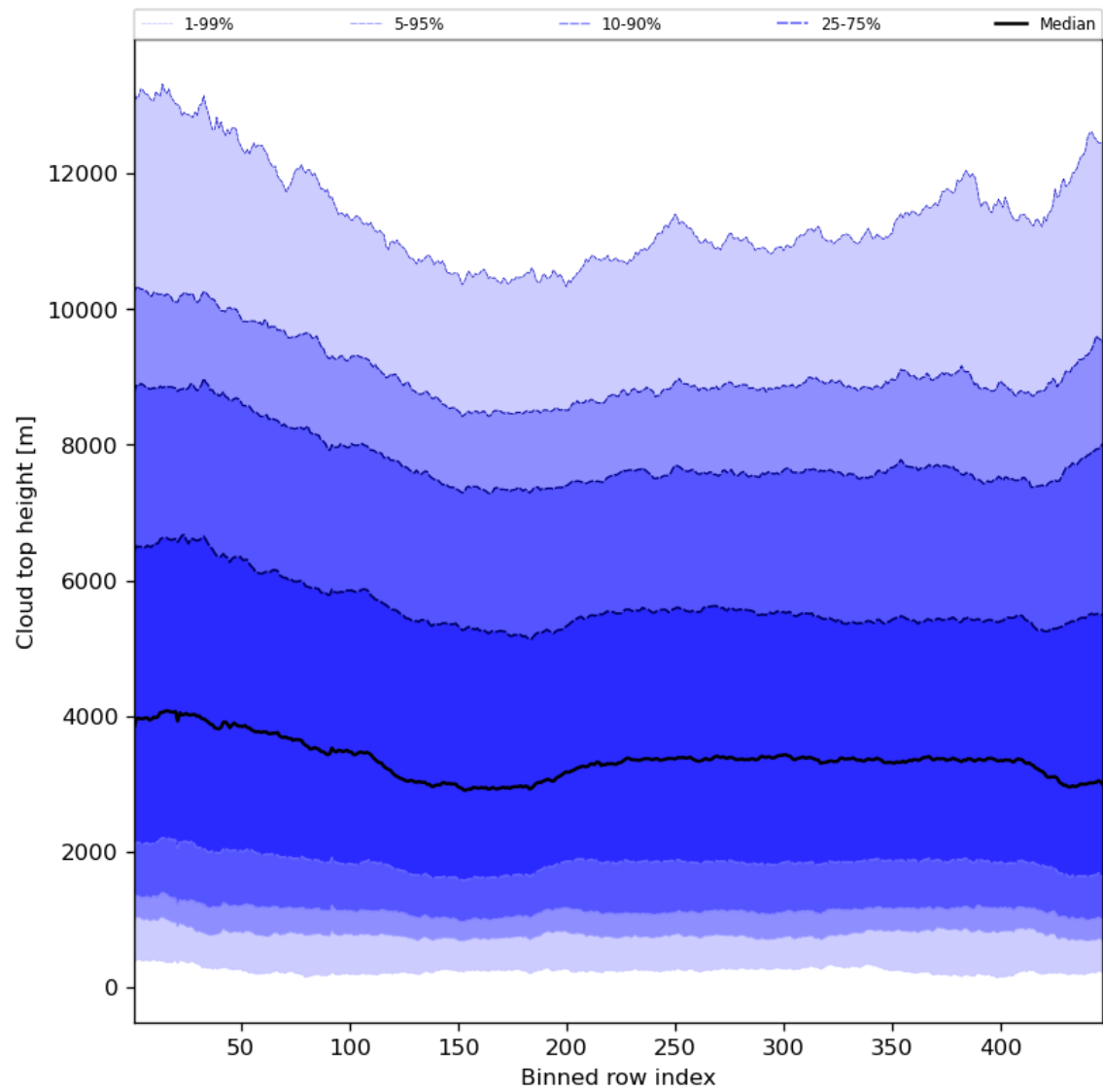
Figure 56: Along track statistics of “Cloud top height” for 2024-02-22 to 2024-02-24
