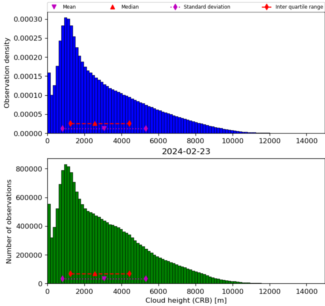
Figure 43: Histogram of “Cloud height (CRB)” for 2024-02-22 to 2024-02-24
