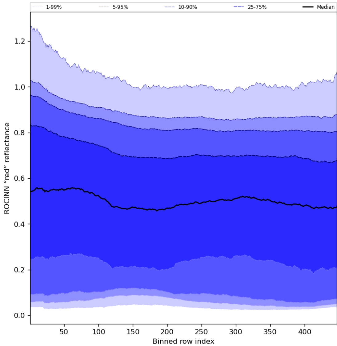
Figure 69: Along track statistics of “ROCINN “red” reflectance” for 2024-02-22 to 2024-02-24
