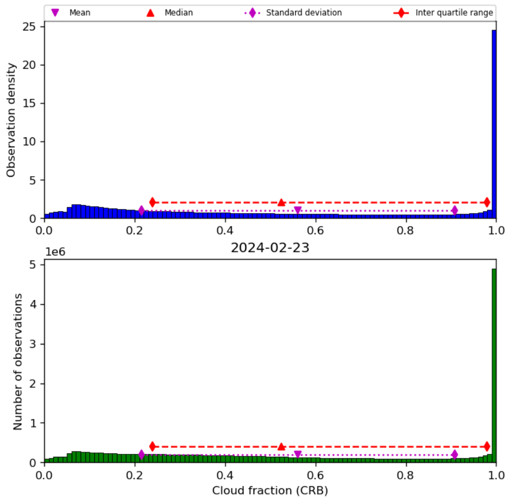
Figure 42: Histogram of “Cloud fraction (CRB)” for 2024-02-22 to 2024-02-24
