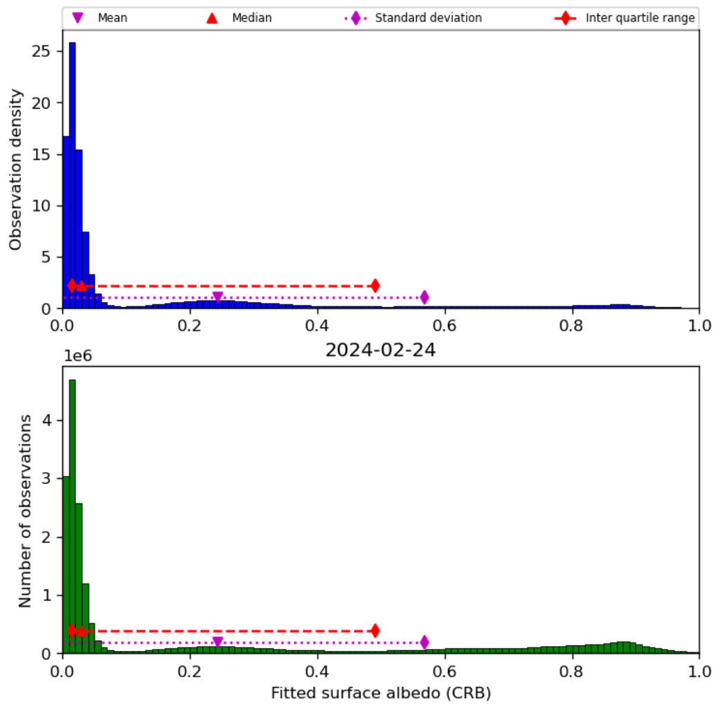
Figure 46: Histogram of “Fitted surface albedo (CRB)” for 2024-02-23 to 2024-02-25
