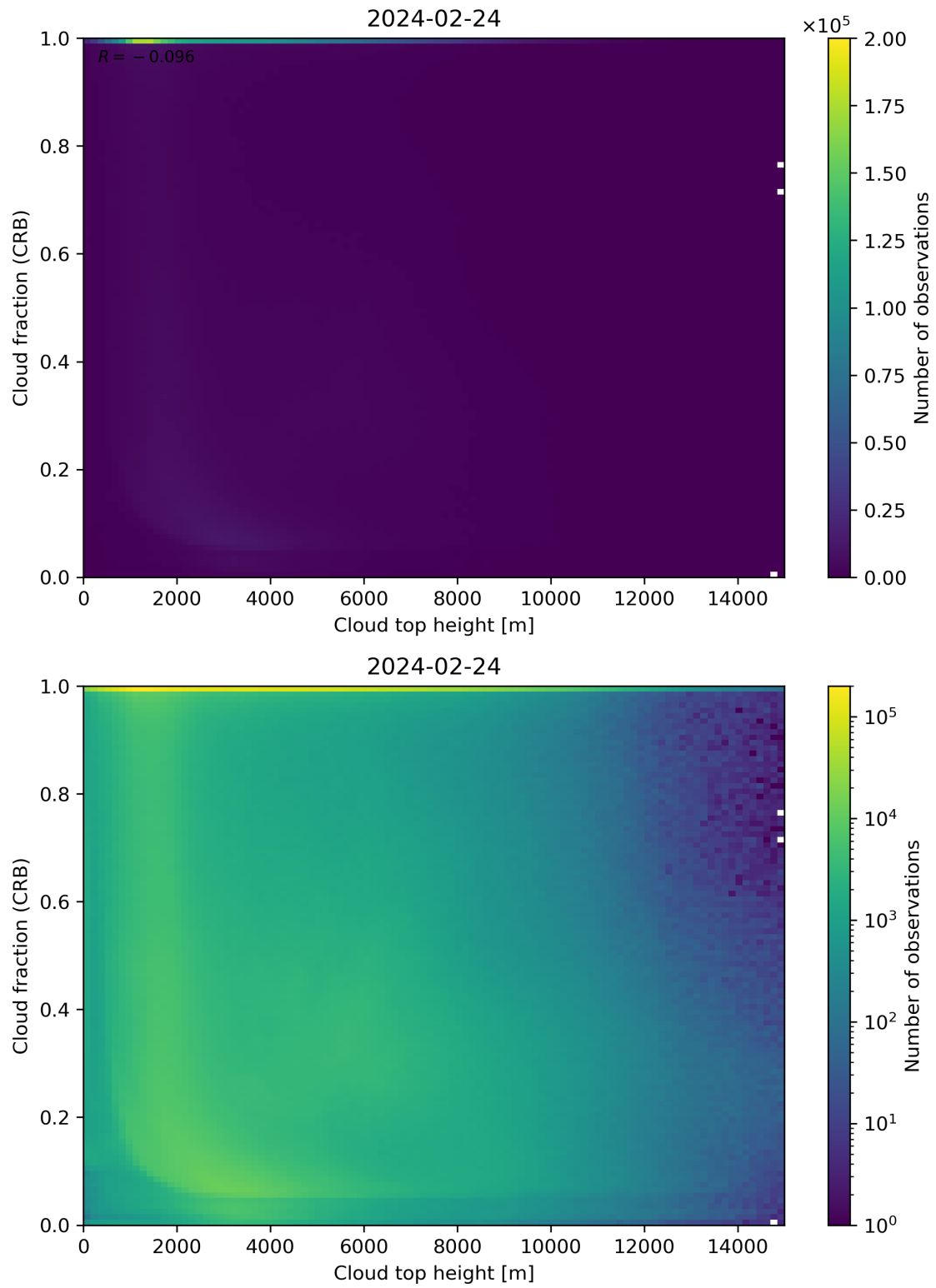
Figure 88: Scatter density plot of “Cloud top height” against “Cloud fraction (CRB)” for 2024-02-23 to 2024-02-25.
