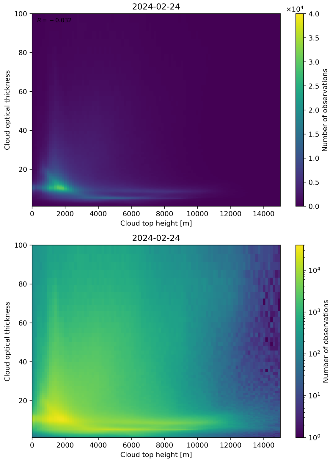
Figure 90: Scatter density plot of “Cloud top height” against “Cloud optical thickness” for 2024-02-23 to 2024-02-25.
