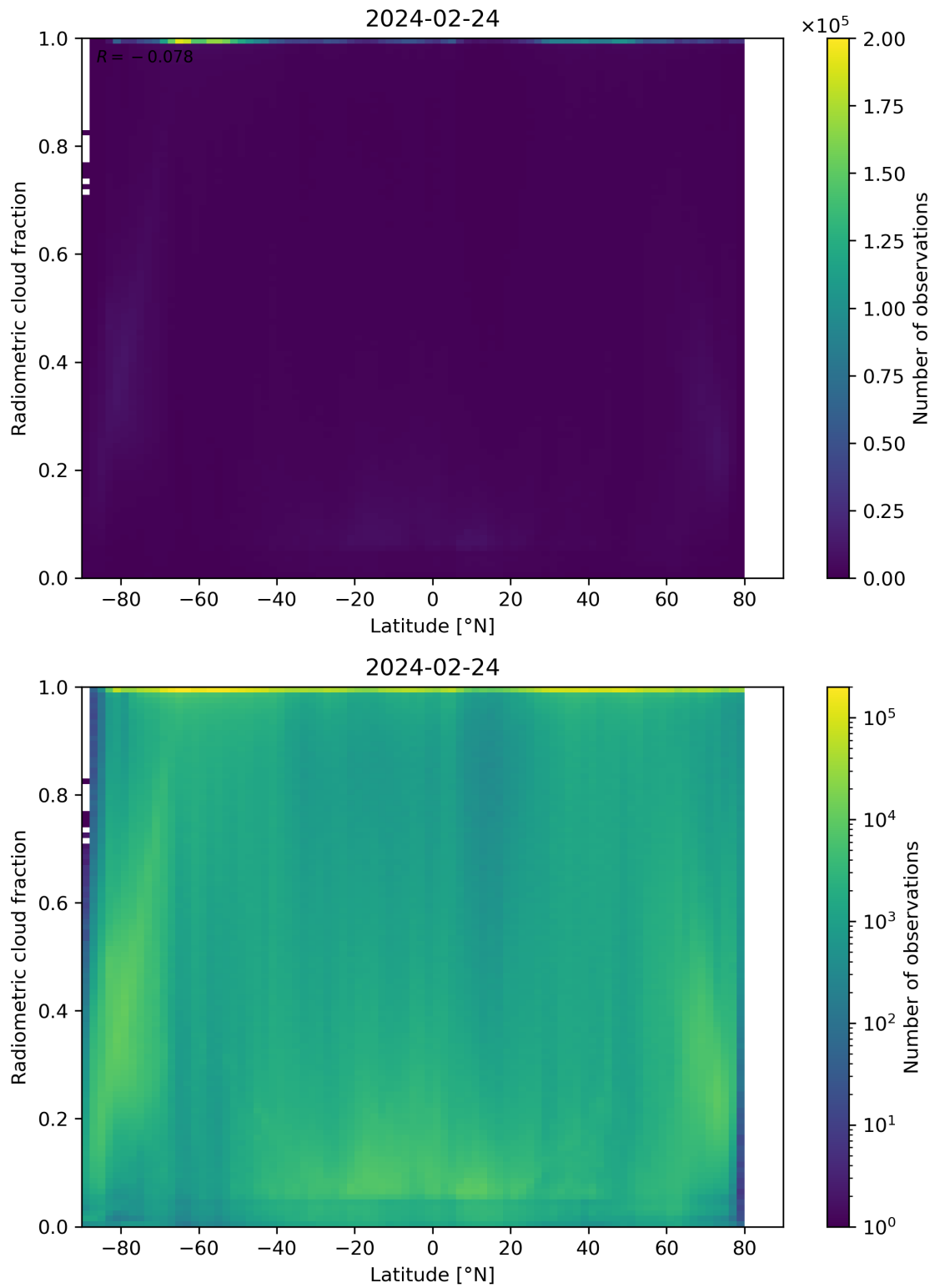
Figure 92: Scatter density plot of “Latitude” against “Radiometric cloud fraction” for 2024-02-23 to 2024-02-25.
