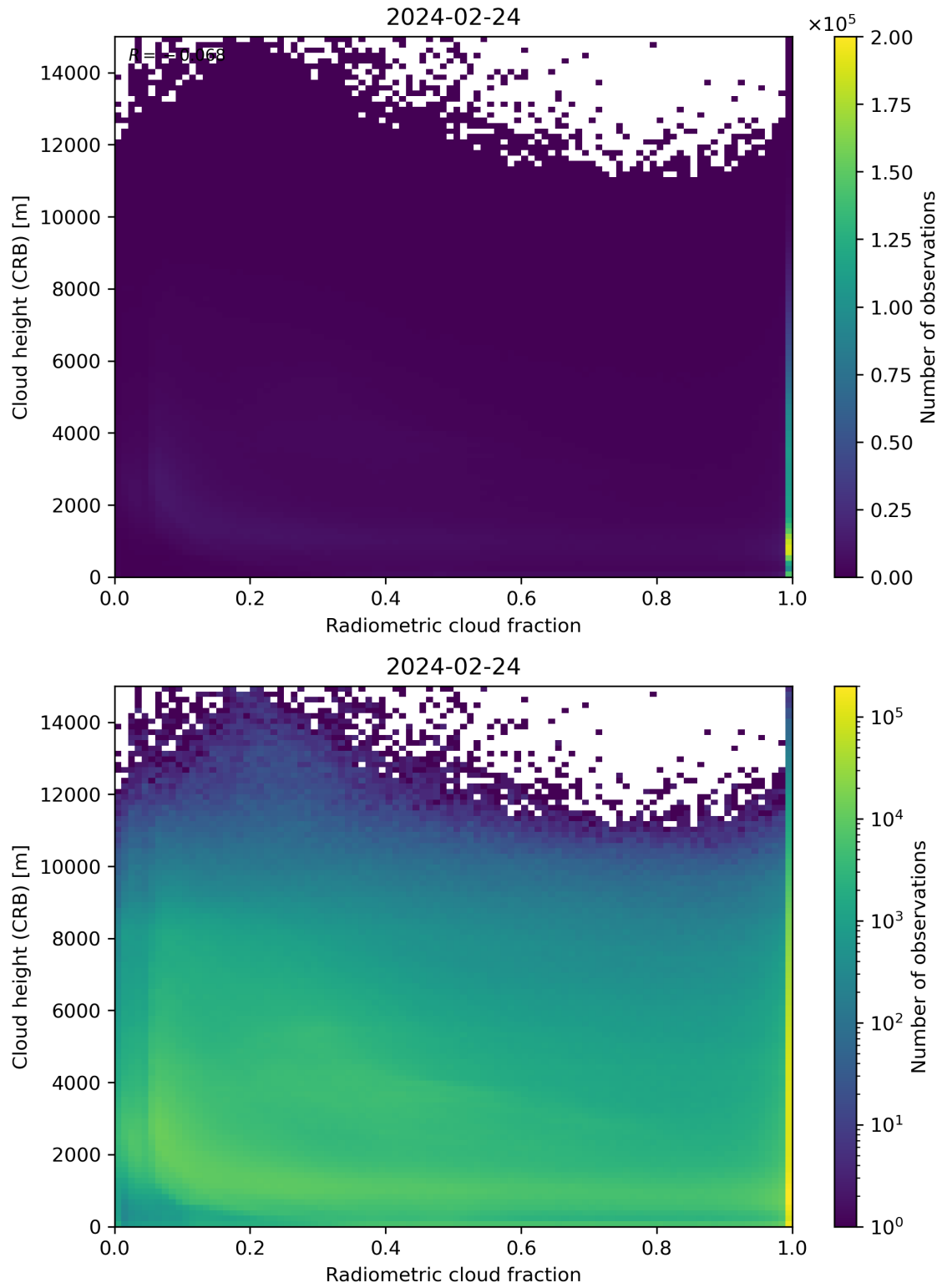
Figure 74: Scatter density plot of “Radiometric cloud fraction” against “Cloud height (CRB)” for 2024-02-23 to 2024-02-25.
