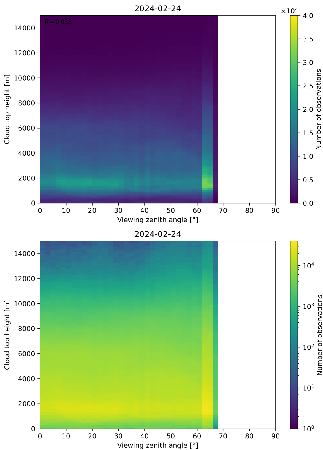
Figure 112: Scatter density plot of “Viewing zenith angle” against “Cloud top height” for 2024-02-23 to 2024-02-25.
