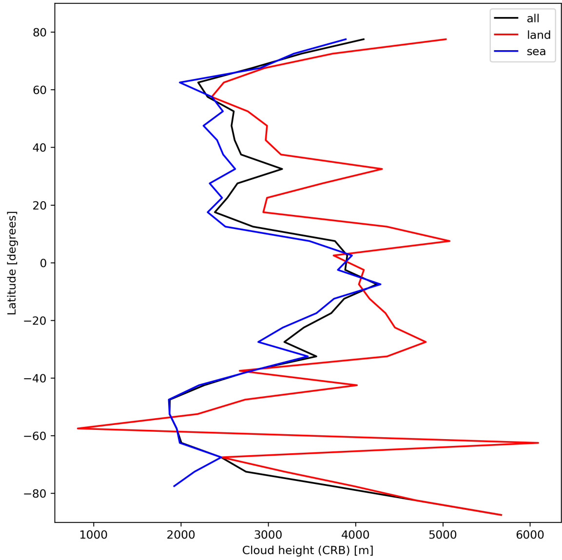
Figure 27: Zonal average of “Cloud height (CRB)” for 2024-02-23 to 2024-02-25.
