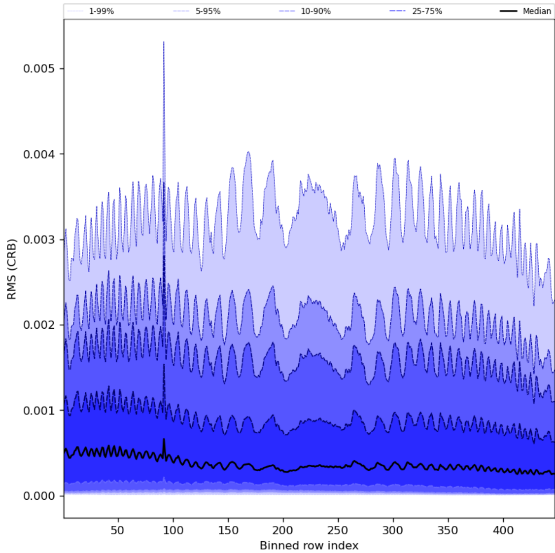
Figure 64: Along track statistics of “RMS (CRB)” for 2024-02-23 to 2024-02-25
