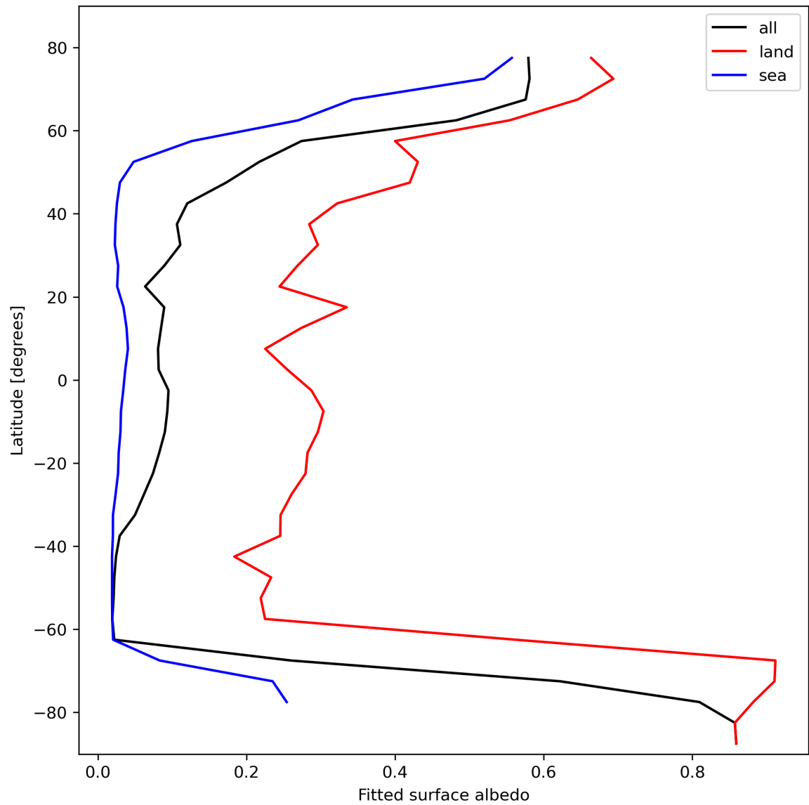
Figure 29: Zonal average of “Fitted surface albedo” for 2024-02-23 to 2024-02-25.
