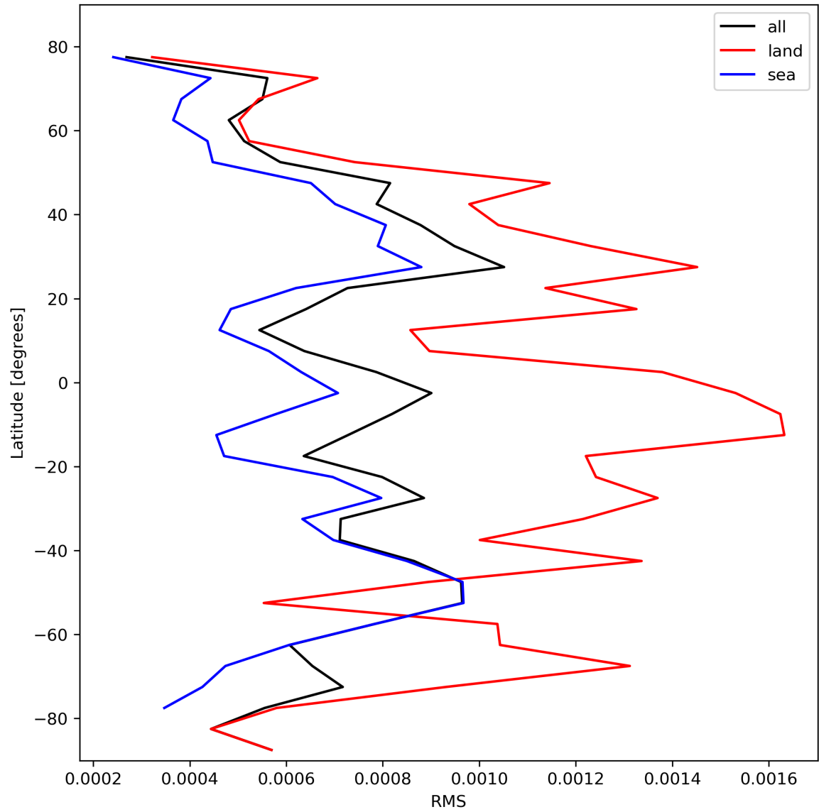
Figure 31: Zonal average of “RMS” for 2024-02-23 to 2024-02-25.
