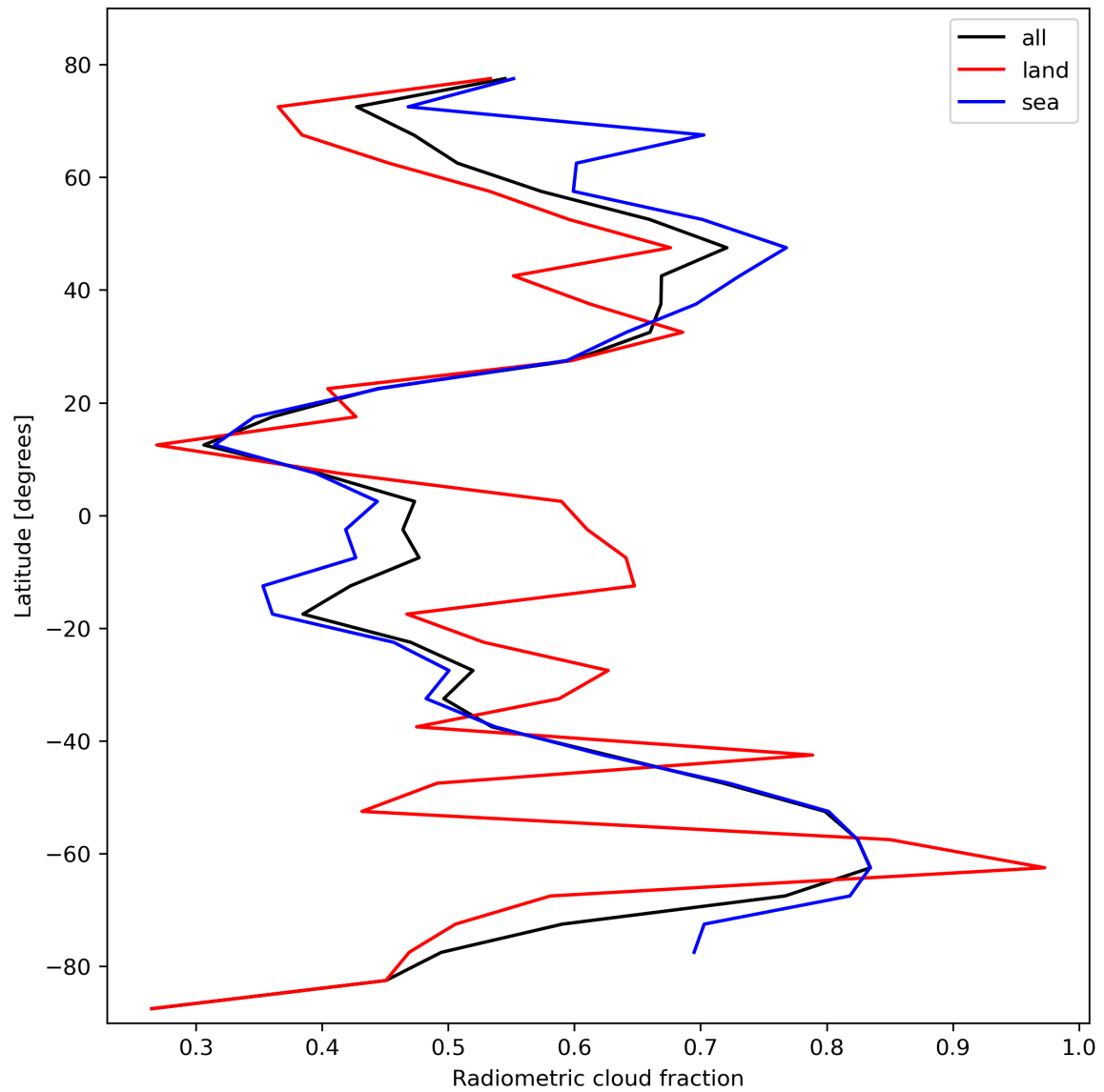
Figure 23: Zonal average of “Radiometric cloud fraction” for 2024-02-23 to 2024-02-25.
