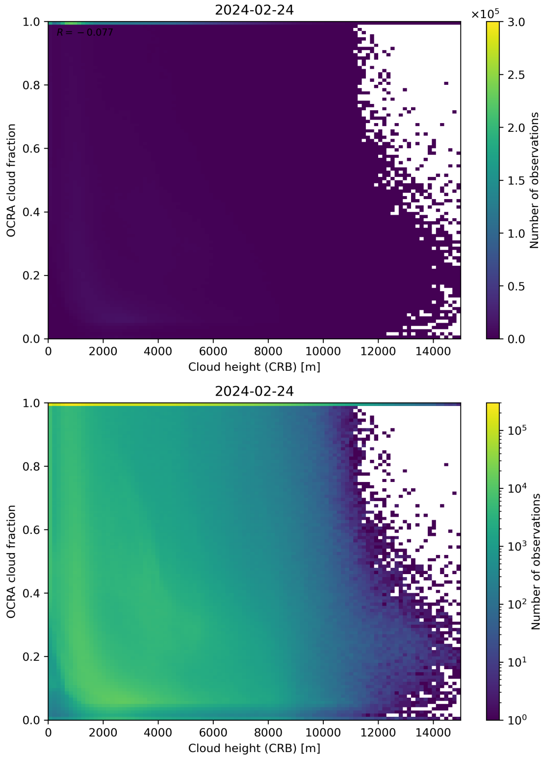
Figure 81: Scatter density plot of “Cloud height (CRB)” against “OCRA cloud fraction” for 2024-02-23 to 2024-02-25.
