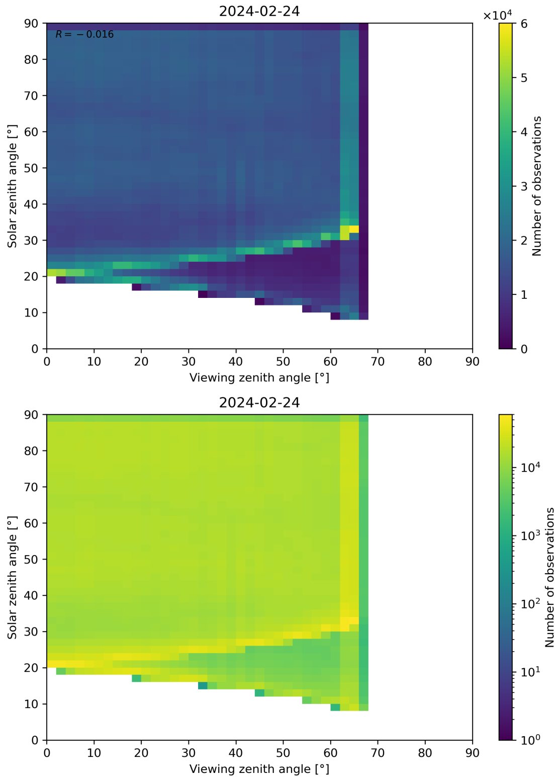
Figure 114: Scatter density plot of “Viewing zenith angle” against “Solar zenith angle” for 2024-02-23 to 2024-02-25.
