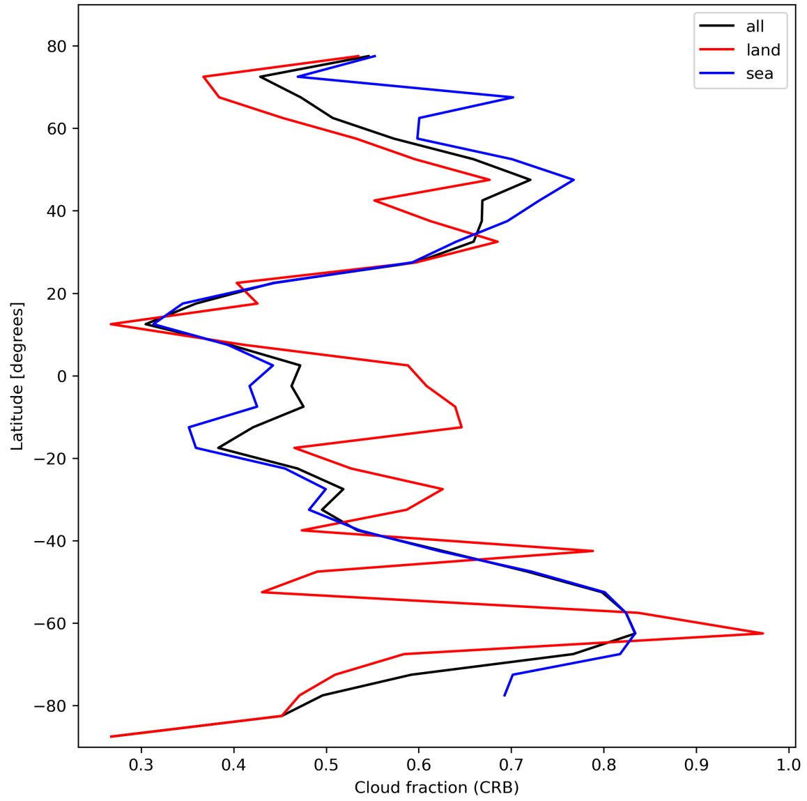
Figure 26: Zonal average of “Cloud fraction (CRB)” for 2024-02-23 to 2024-02-25.
