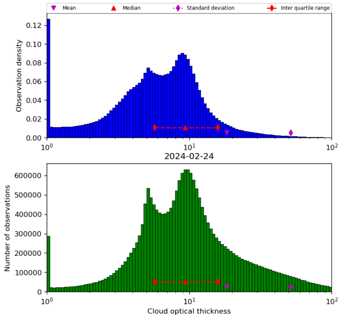
Figure 41: Histogram of “Cloud optical thickness” for 2024-02-23 to 2024-02-25
