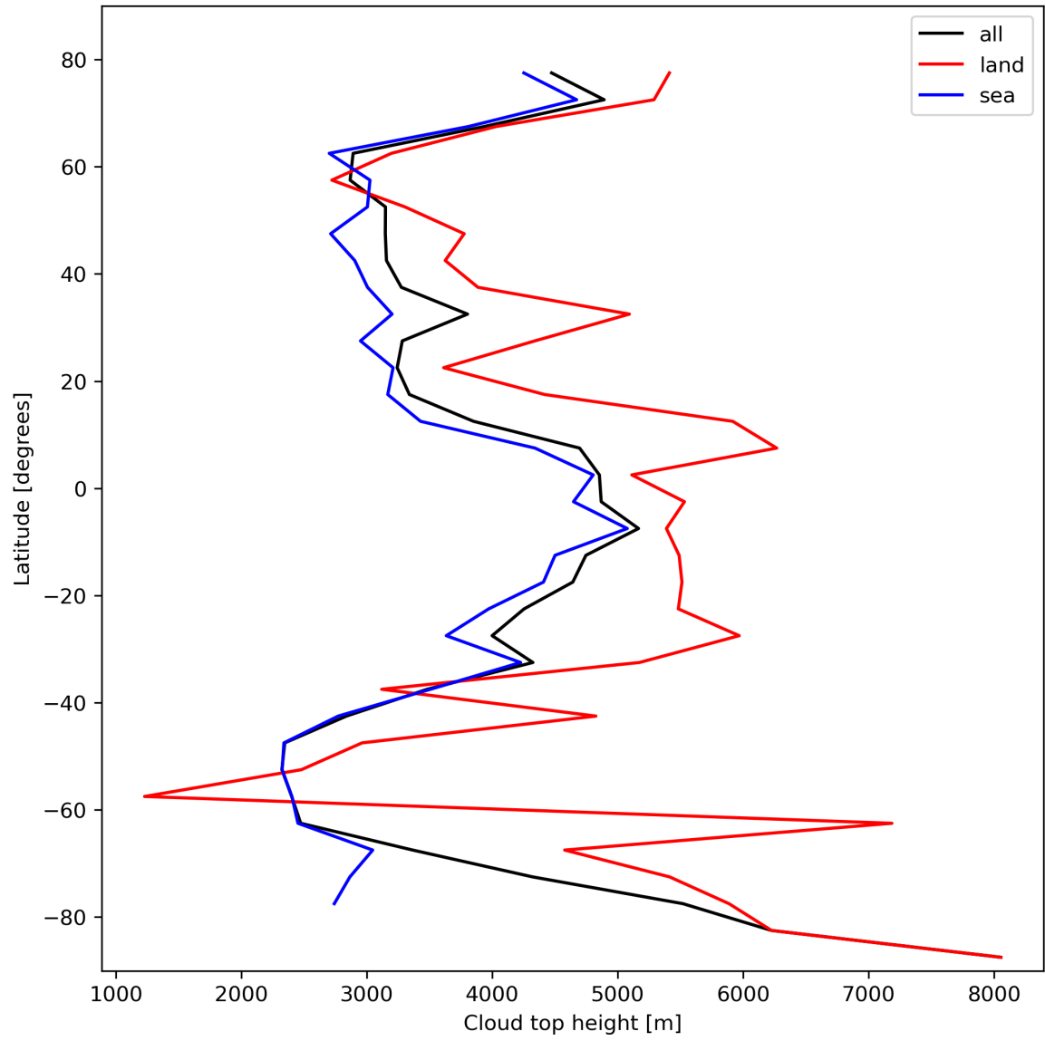
Figure 24: Zonal average of “Cloud top height” for 2024-02-23 to 2024-02-25.
