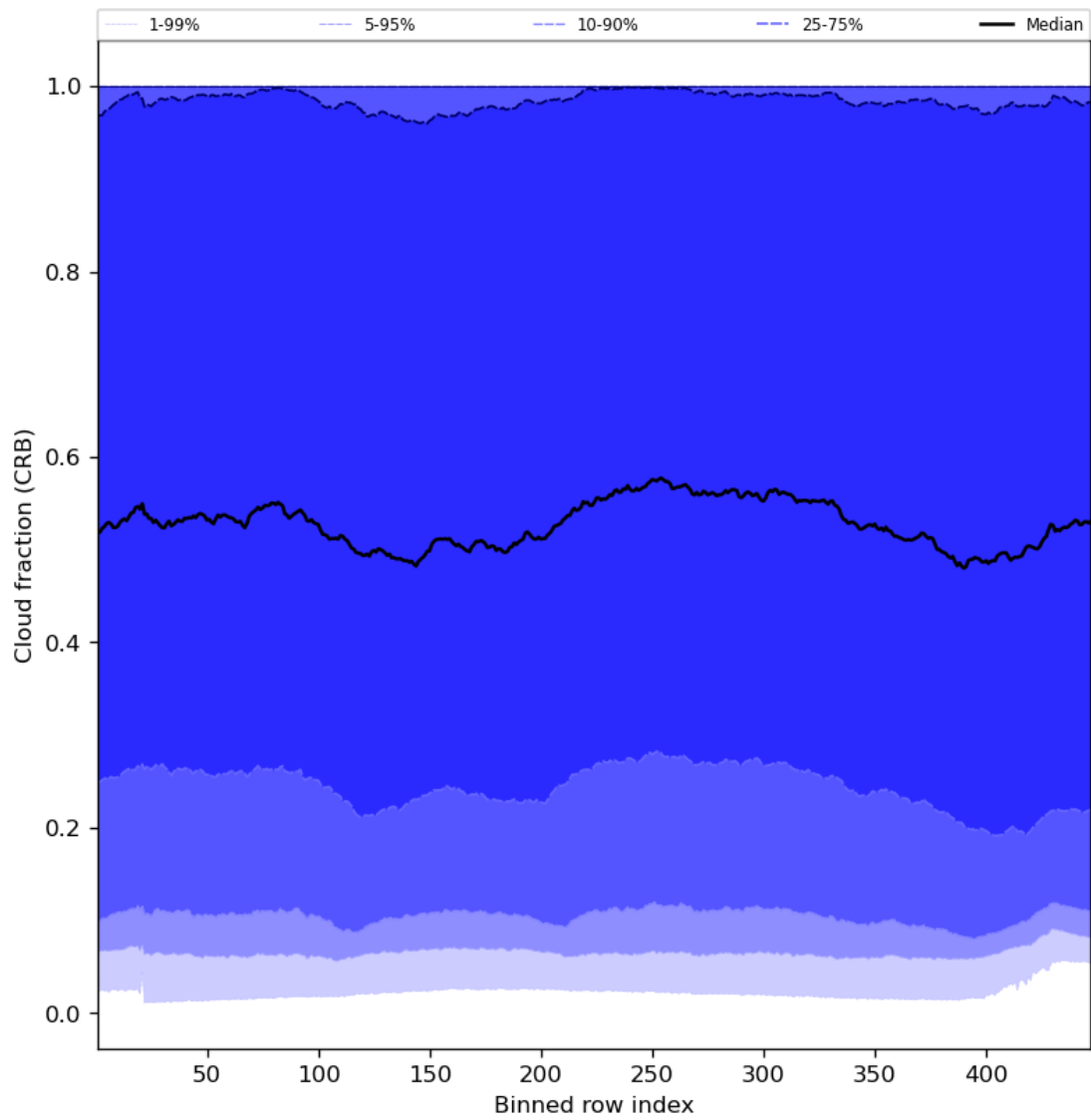
Figure 58: Along track statistics of “Cloud fraction (CRB)” for 2024-02-23 to 2024-02-25
