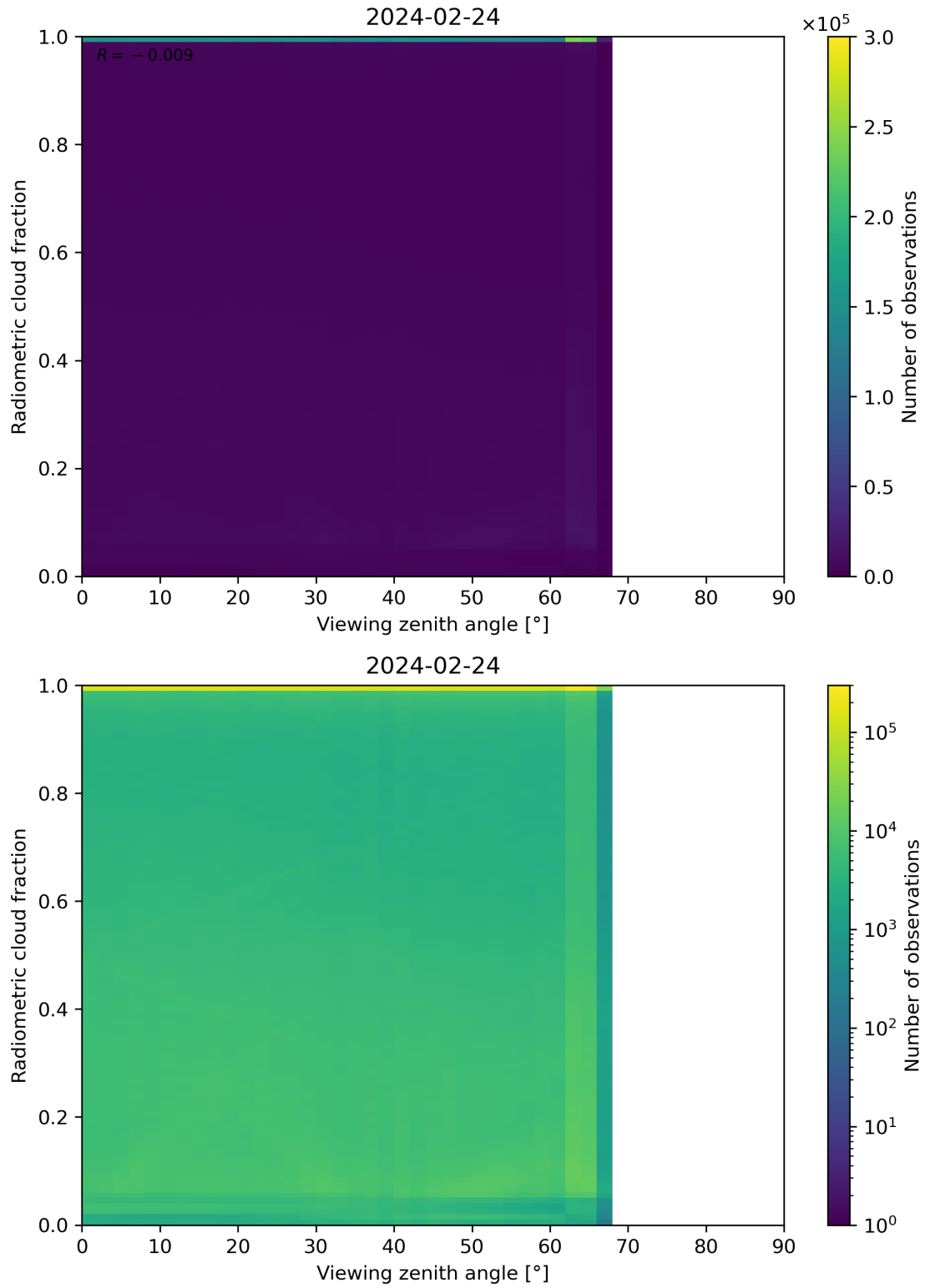
Figure 107: Scatter density plot of “Viewing zenith angle” against “Radiometric cloud fraction” for 2024-02-23 to 2024-02-25.
