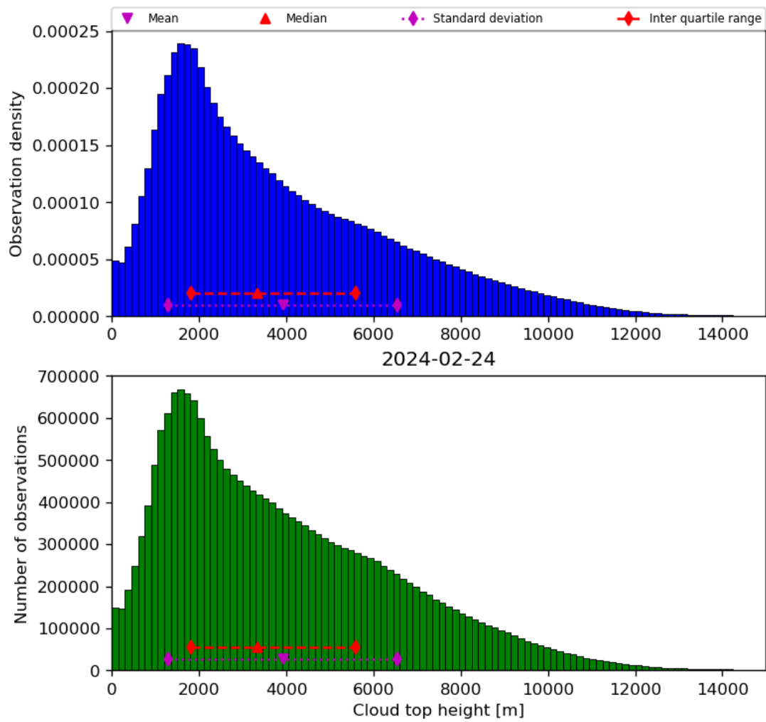
Figure 40: Histogram of “Cloud top height” for 2024-02-23 to 2024-02-25
