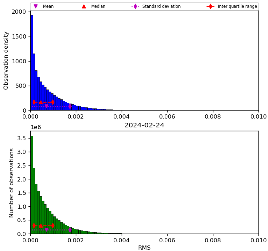
Figure 47: Histogram of “RMS” for 2024-02-23 to 2024-02-25
