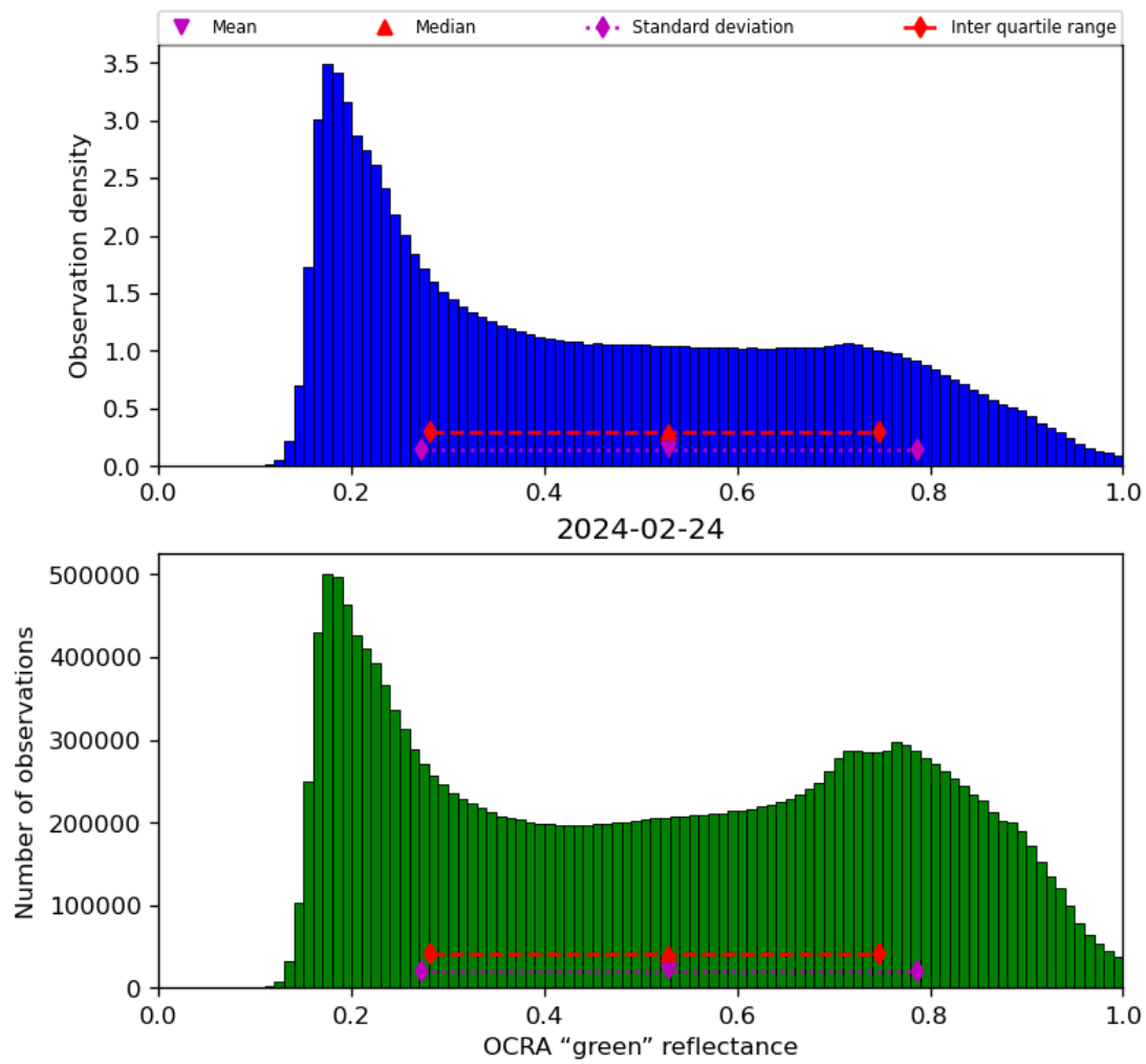
Figure 52: Histogram of “OCRA “green” reflectance” for 2024-02-23 to 2024-02-25
