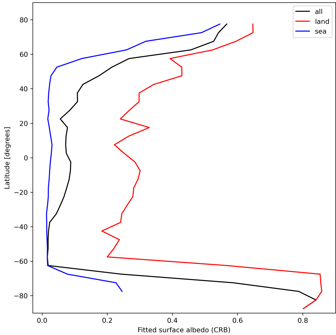
Figure 30: Zonal average of “Fitted surface albedo (CRB)” for 2024-02-23 to 2024-02-25.
