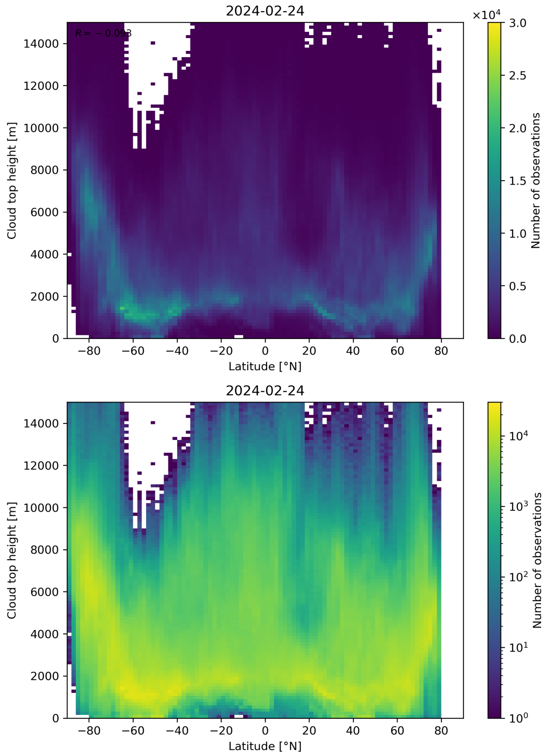
Figure 97: Scatter density plot of “Latitude” against “Cloud top height” for 2024-02-23 to 2024-02-25.
