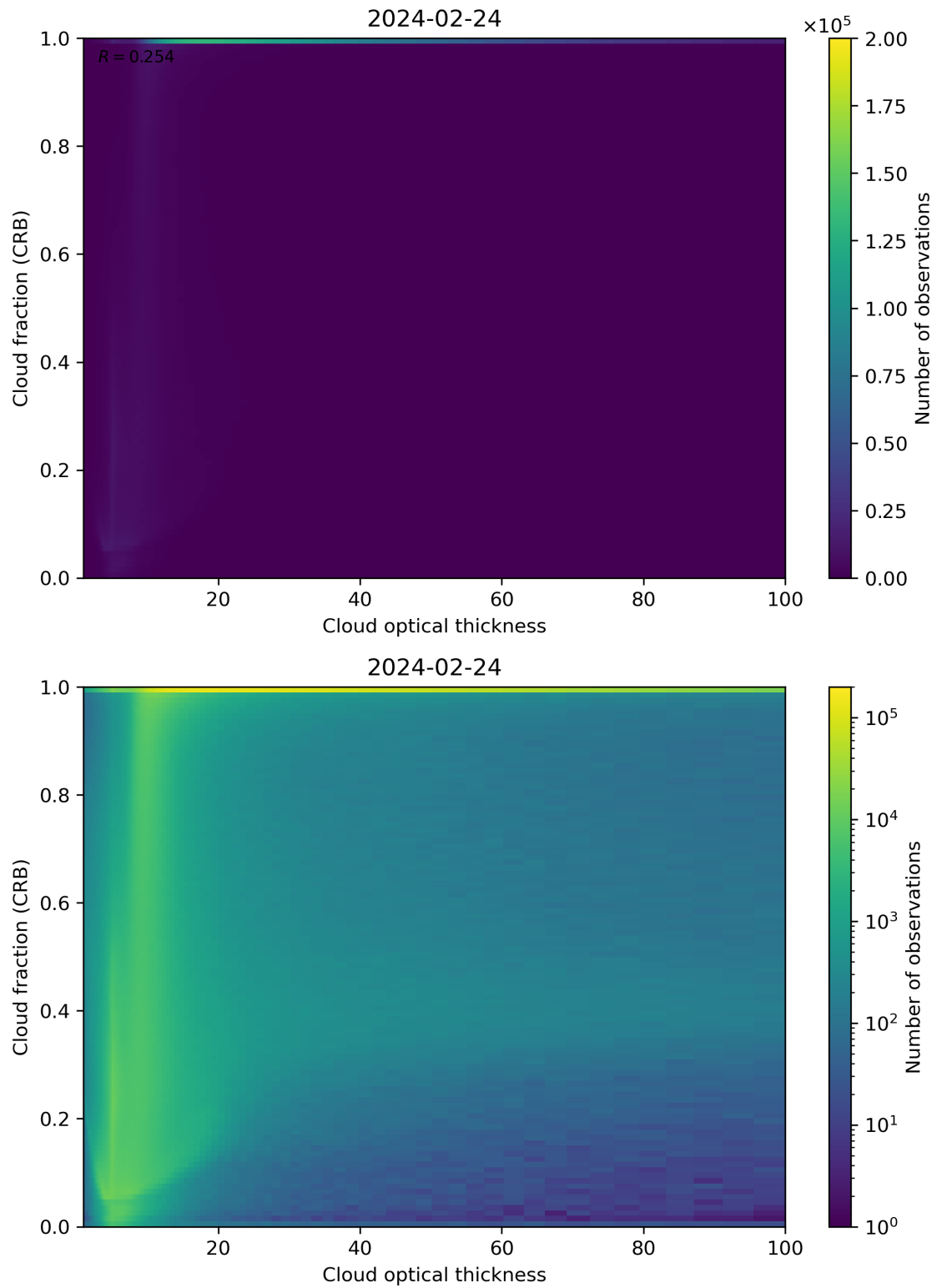
Figure 84: Scatter density plot of “Cloud optical thickness” against “Cloud fraction (CRB)” for 2024-02-23 to 2024-02-25.
