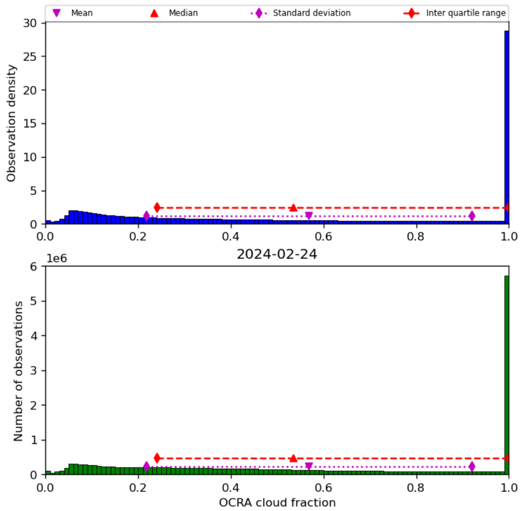
Figure 50: Histogram of “OCRA cloud fraction” for 2024-02-23 to 2024-02-25
