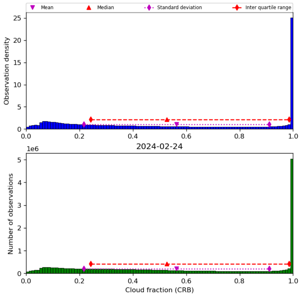
Figure 42: Histogram of “Cloud fraction (CRB)” for 2024-02-23 to 2024-02-25
