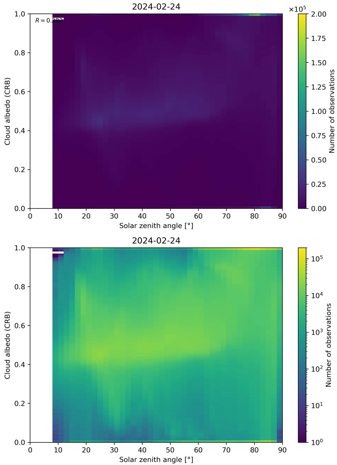
Figure 98: Scatter density plot of “Solar zenith angle” against “Cloud albedo (CRB)” for 2024-02-23 to 2024-02-25.
