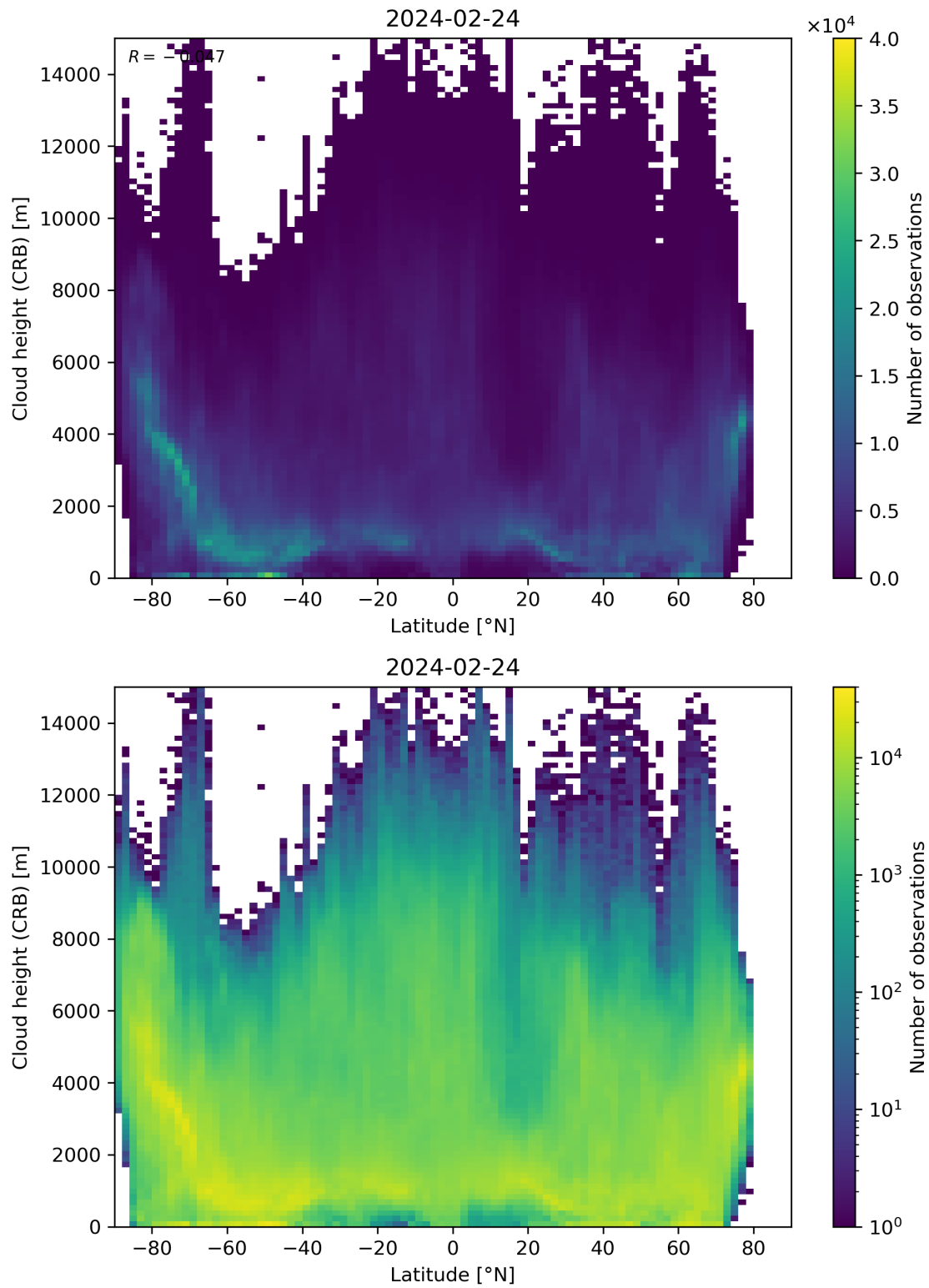
Figure 95: Scatter density plot of “Latitude” against “Cloud height (CRB)” for 2024-02-23 to 2024-02-25.
