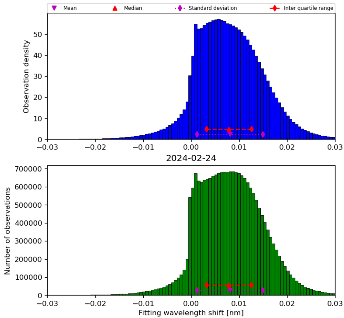
Figure 49: Histogram of “Fitting wavelength shift” for 2024-02-23 to 2024-02-25
