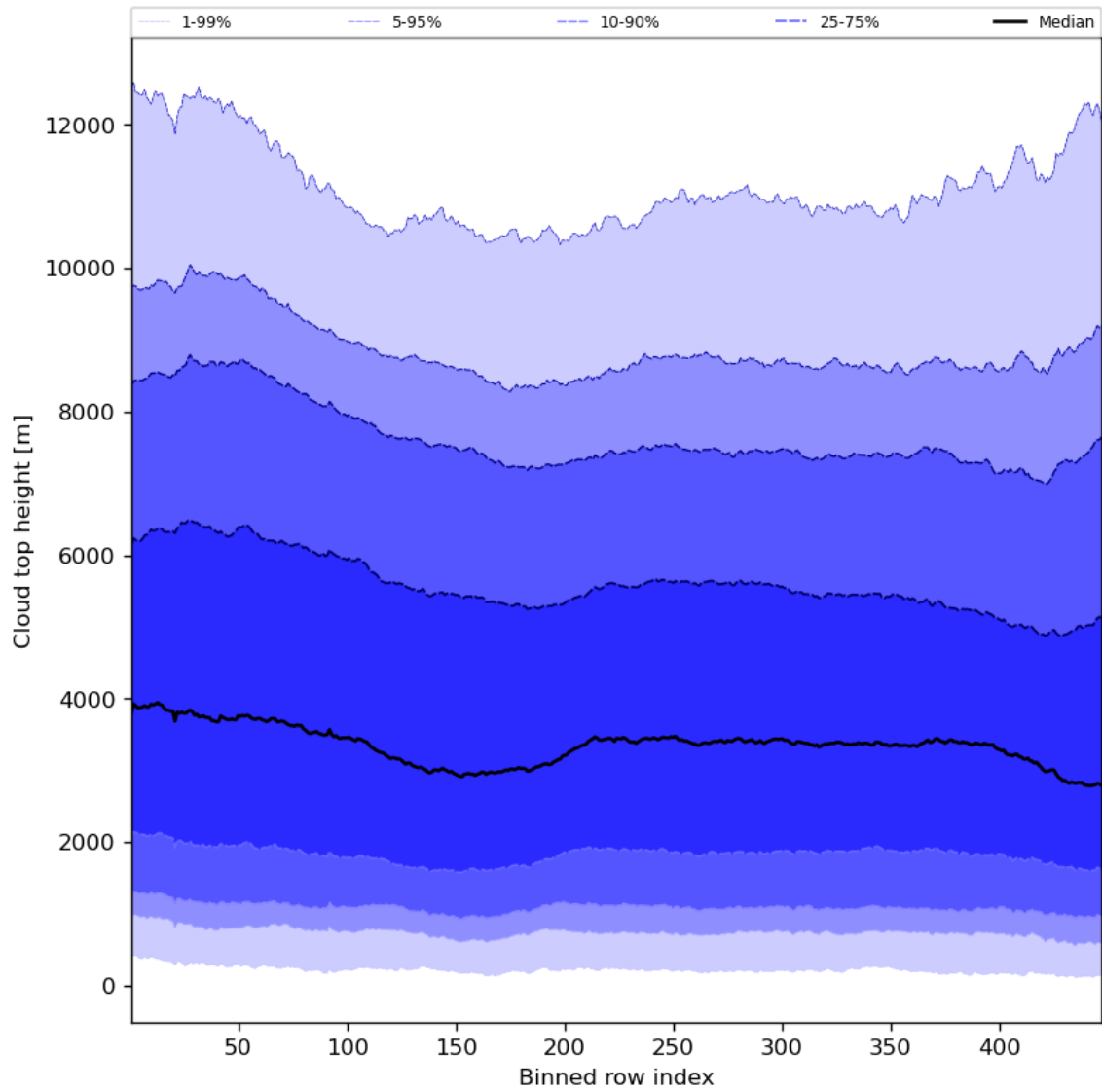
Figure 56: Along track statistics of “Cloud top height” for 2024-02-23 to 2024-02-25
