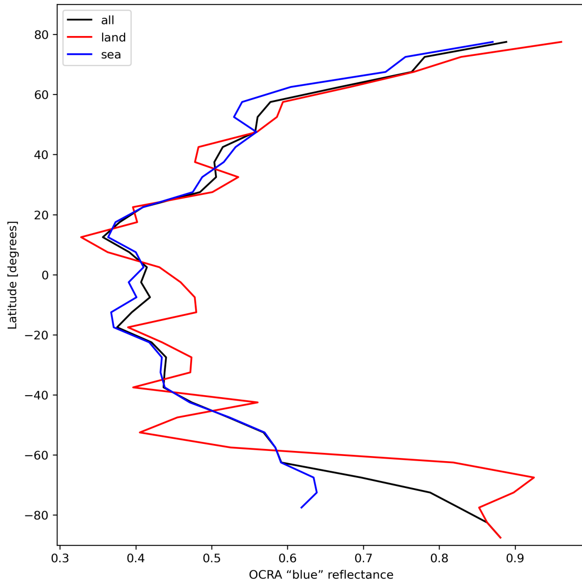
Figure 35: Zonal average of “OCRA “blue” reflectance” for 2024-02-23 to 2024-02-25.
