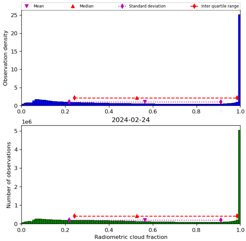
Figure 39: Histogram of “Radiometric cloud fraction” for 2024-02-23 to 2024-02-25
