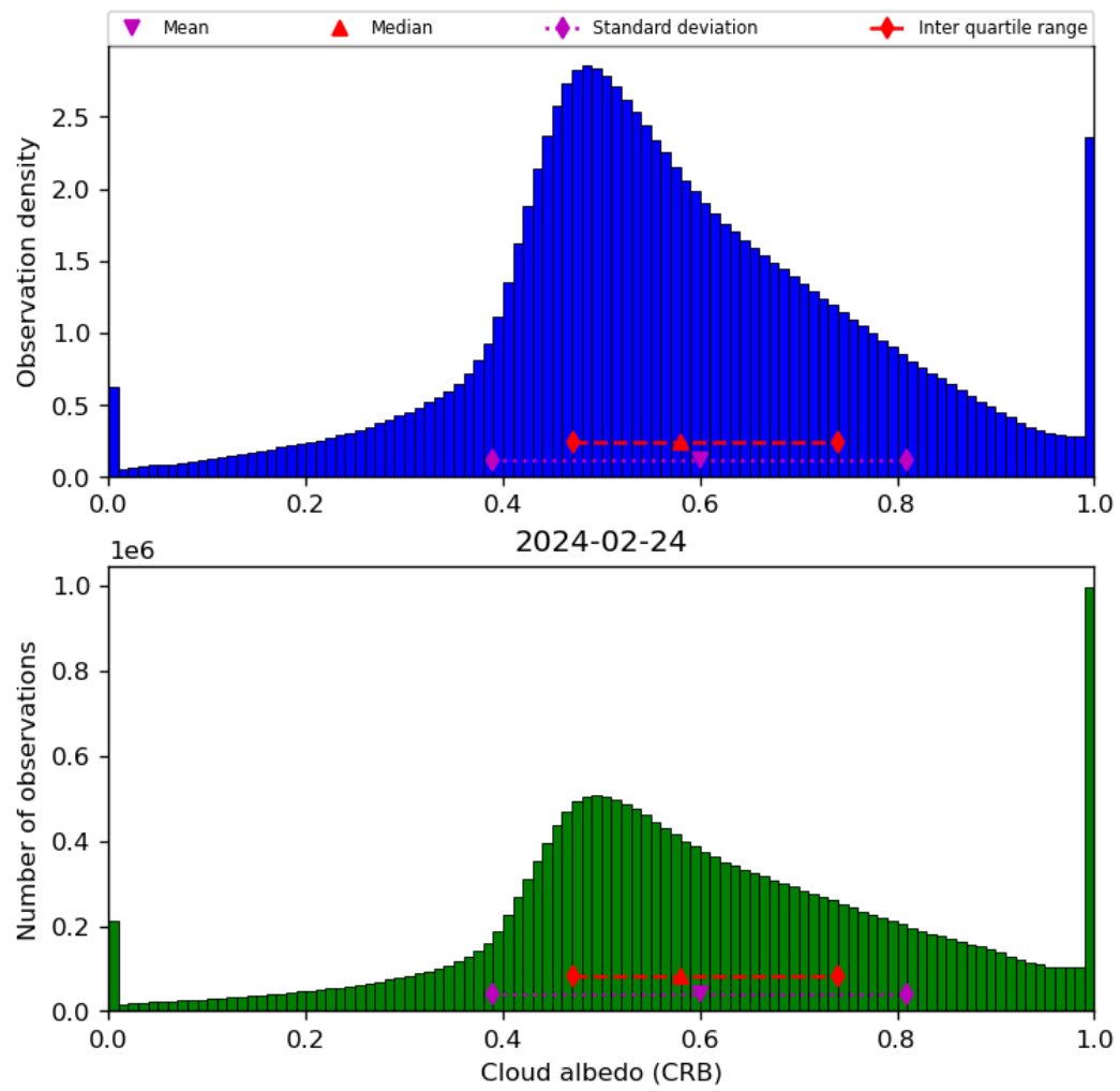
Figure 44: Histogram of “Cloud albedo (CRB)” for 2024-02-23 to 2024-02-25
