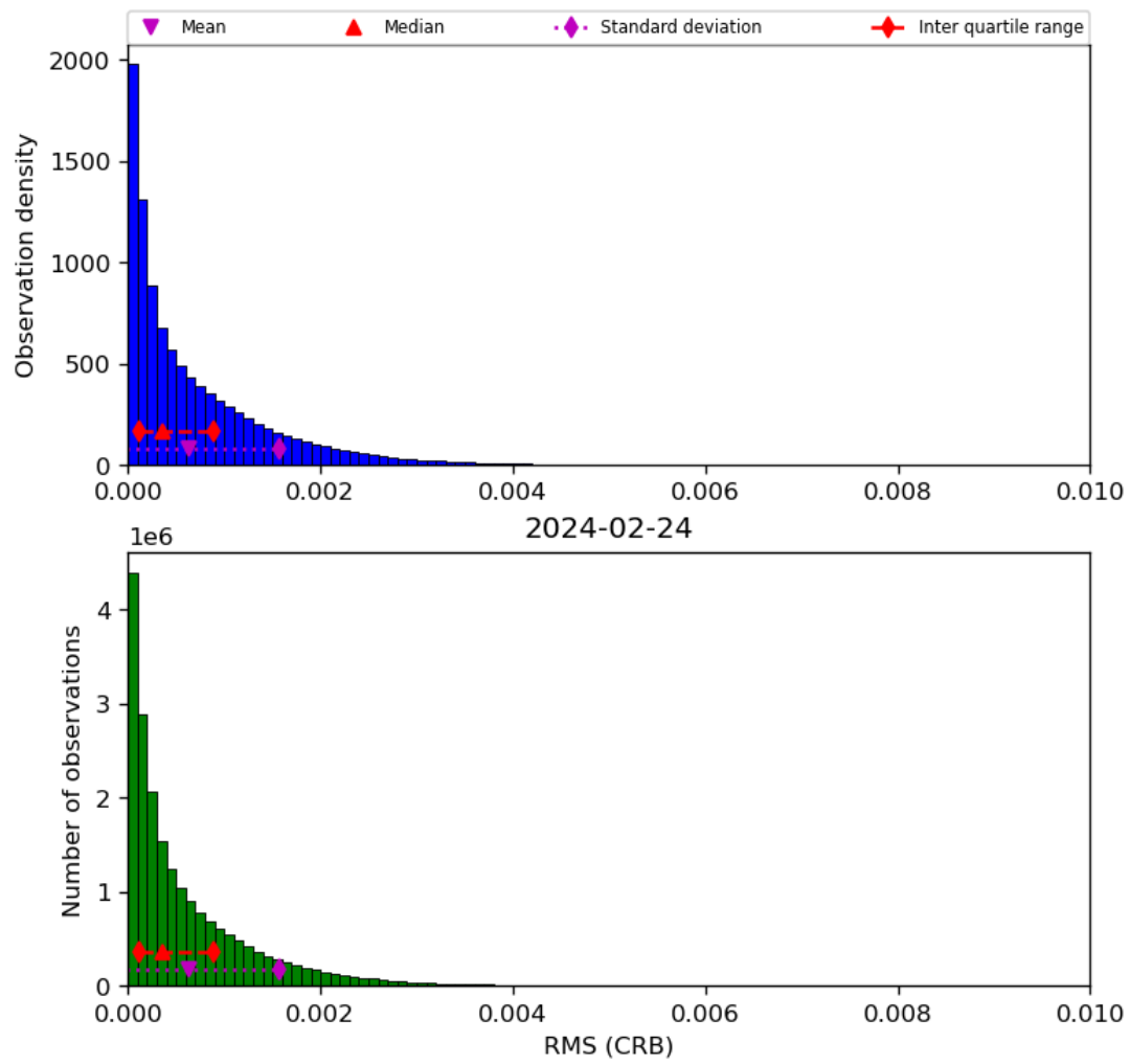
Figure 48: Histogram of “RMS (CRB)” for 2024-02-23 to 2024-02-25
