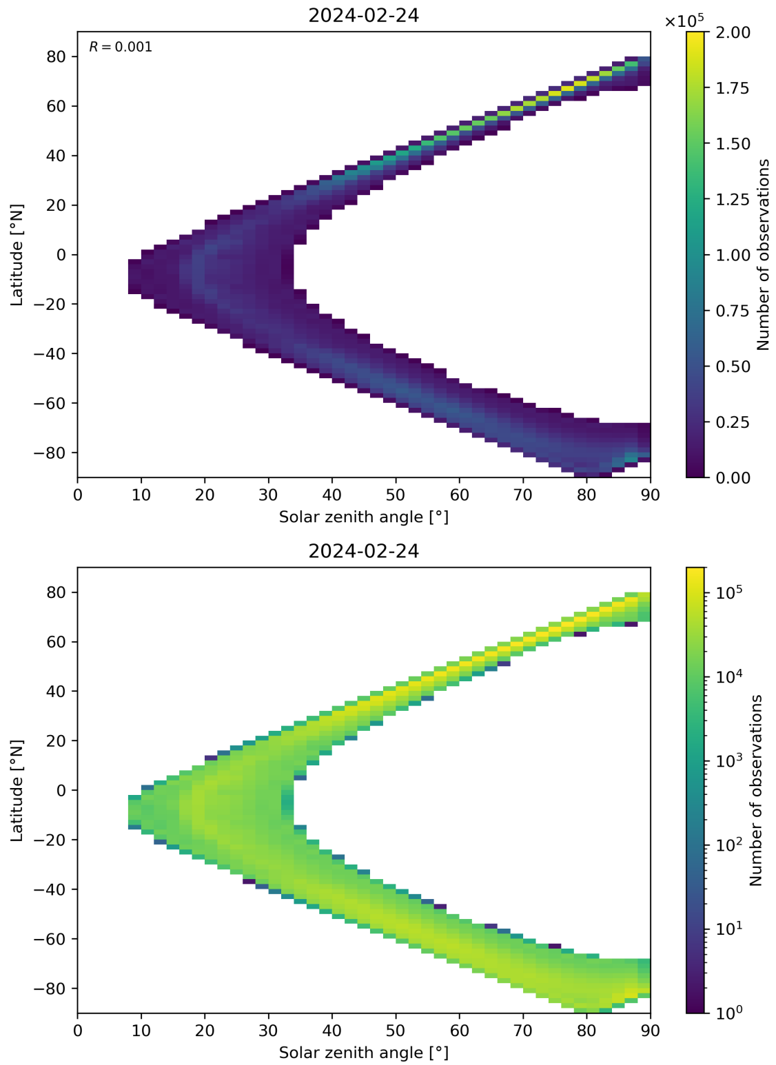
Figure 105: Scatter density plot of “Solar zenith angle” against “Latitude” for 2024-02-23 to 2024-02-25.
