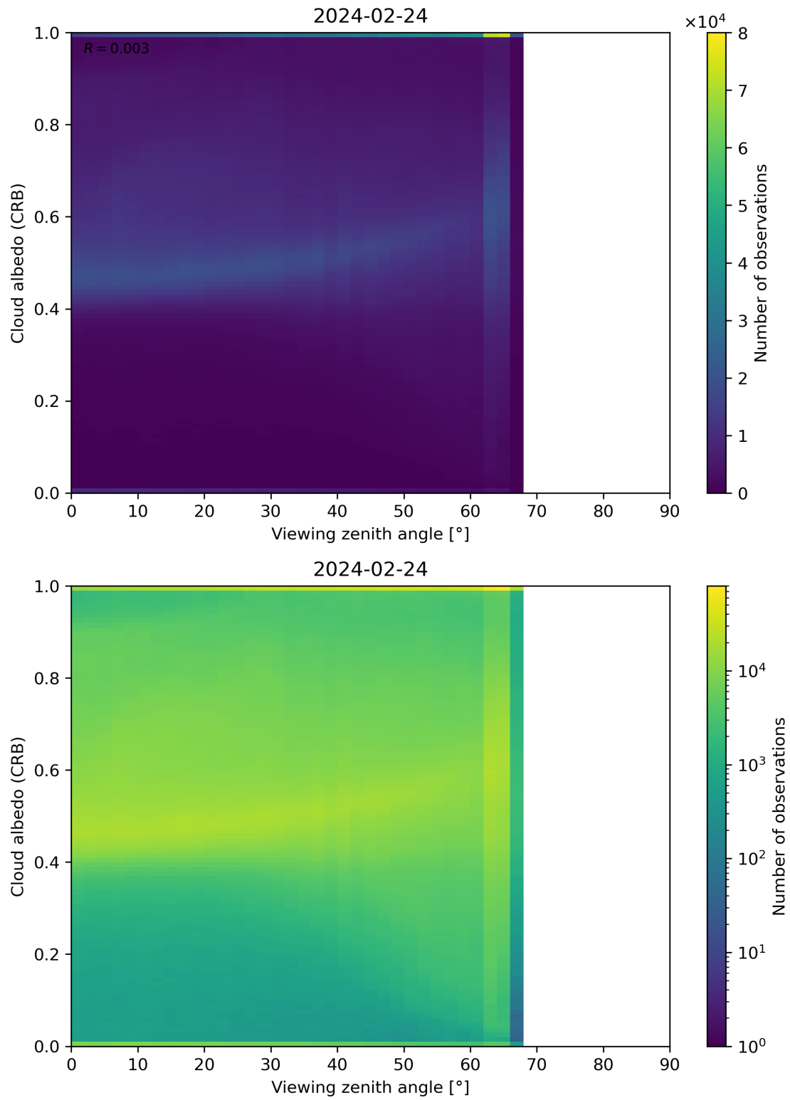
Figure 106: Scatter density plot of “Viewing zenith angle” against “Cloud albedo (CRB)” for 2024-02-23 to 2024-02-25.
