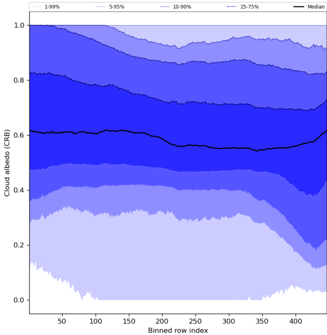
Figure 60: Along track statistics of “Cloud albedo (CRB)” for 2024-02-23 to 2024-02-25
