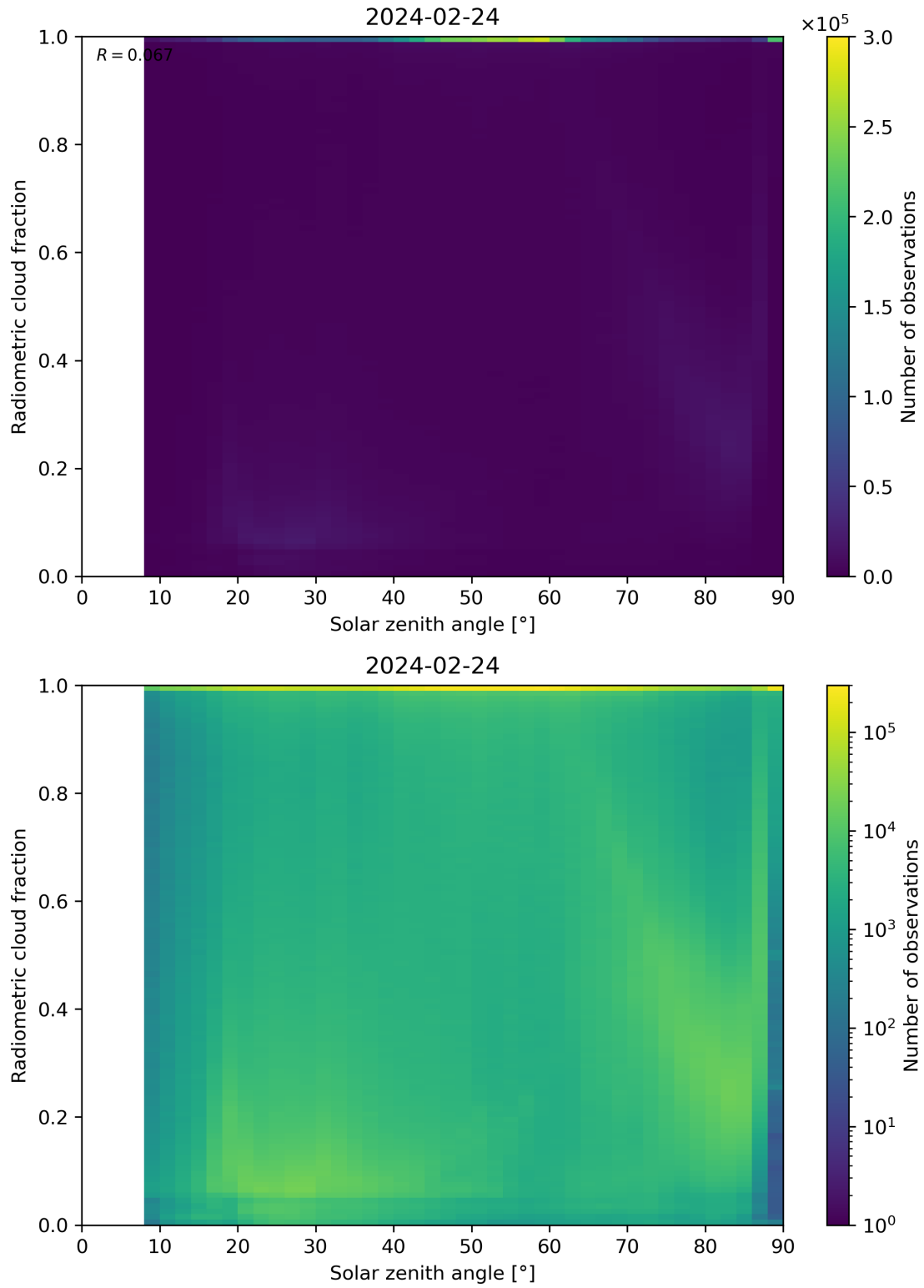
Figure 99: Scatter density plot of “Solar zenith angle” against “Radiometric cloud fraction” for 2024-02-23 to 2024-02-25.
