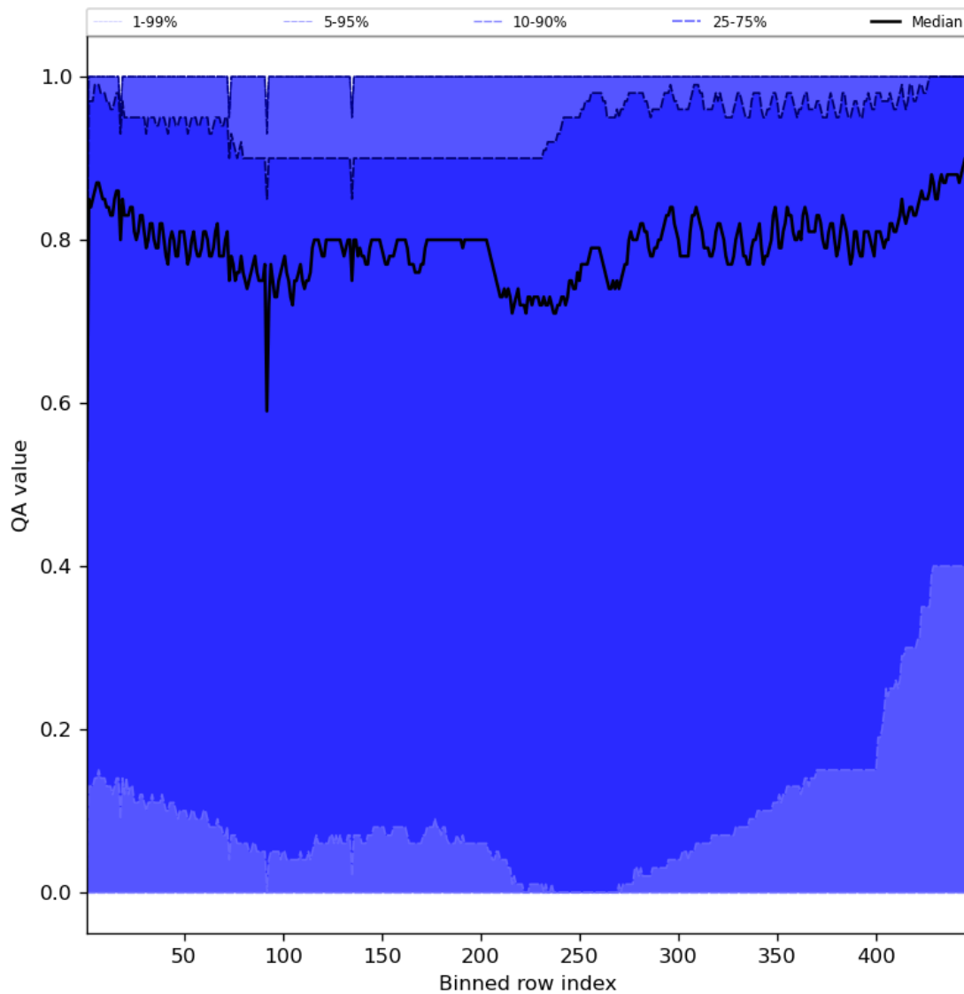
Figure 54: Along track statistics of “QA value” for 2024-02-23 to 2024-02-25
