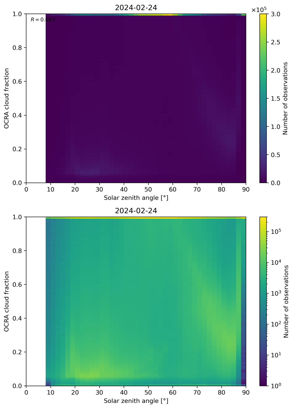
Figure 100: Scatter density plot of “Solar zenith angle” against “OCRA cloud fraction” for 2024-02-23 to 2024-02-25.
