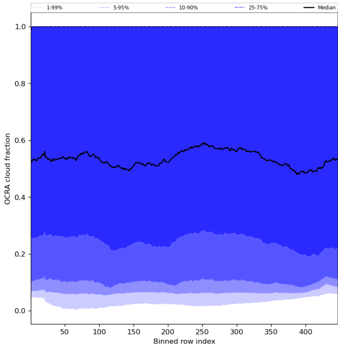
Figure 66: Along track statistics of “OCRA cloud fraction” for 2024-02-23 to 2024-02-25
