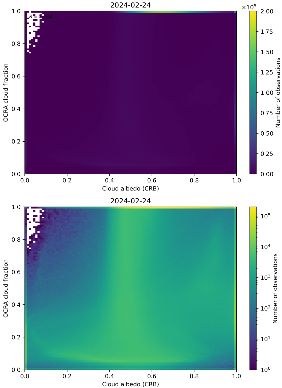
Figure 70: Scatter density plot of “Cloud albedo (CRB)” against “OCRA cloud fraction” for 2024-02-23 to 2024-02-25.
