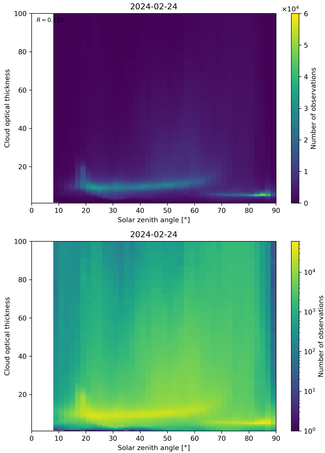
Figure 103: Scatter density plot of “Solar zenith angle” against “Cloud optical thickness” for 2024-02-23 to 2024-02-25.
