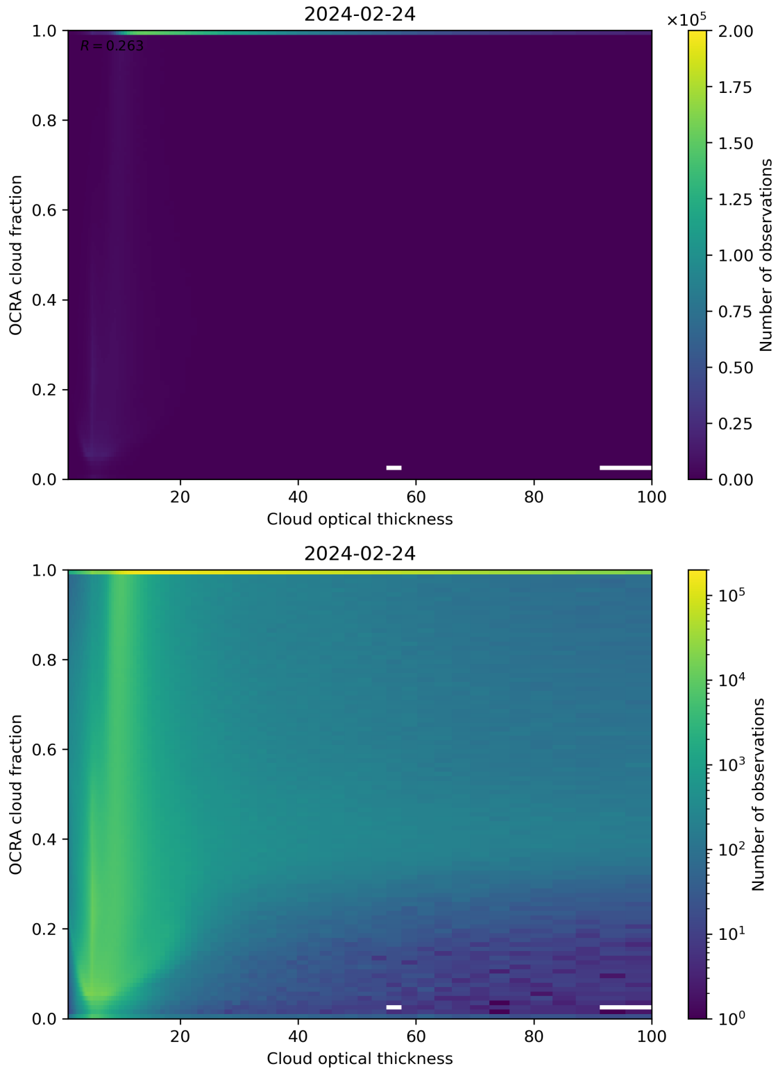
Figure 83: Scatter density plot of “Cloud optical thickness” against “OCRA cloud fraction” for 2024-02-23 to 2024-02-25.
