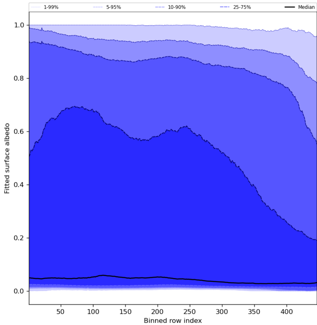
Figure 61: Along track statistics of “Fitted surface albedo” for 2024-02-23 to 2024-02-25
