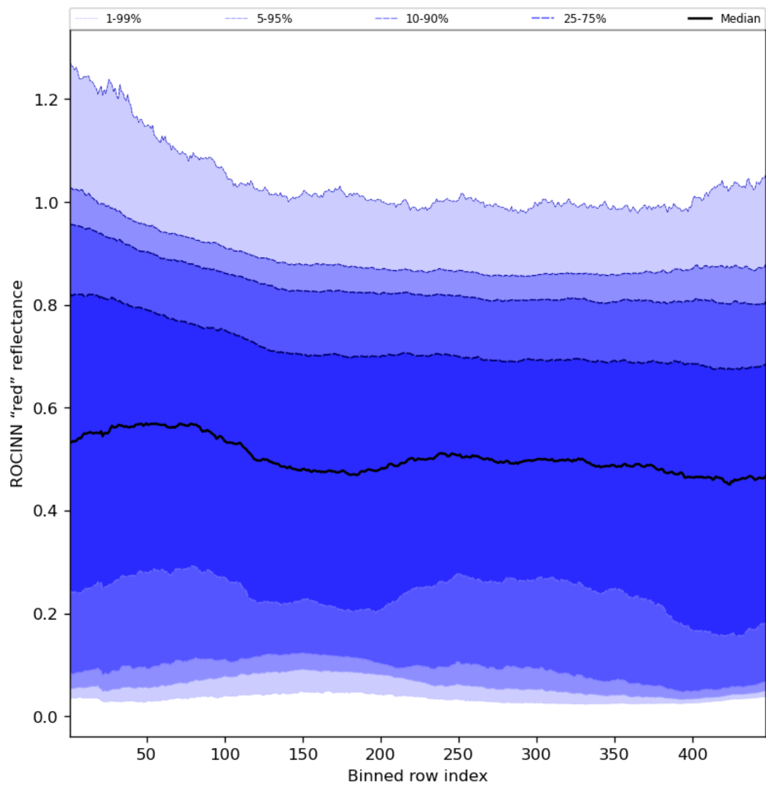
Figure 69: Along track statistics of “ROCINN “red” reflectance” for 2024-02-23 to 2024-02-25
