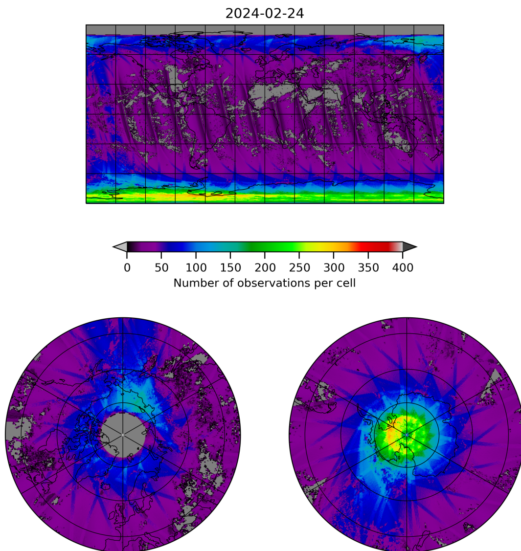
Figure 21: Map of the number of observations for 2024-02-23 to 2024-02-25
