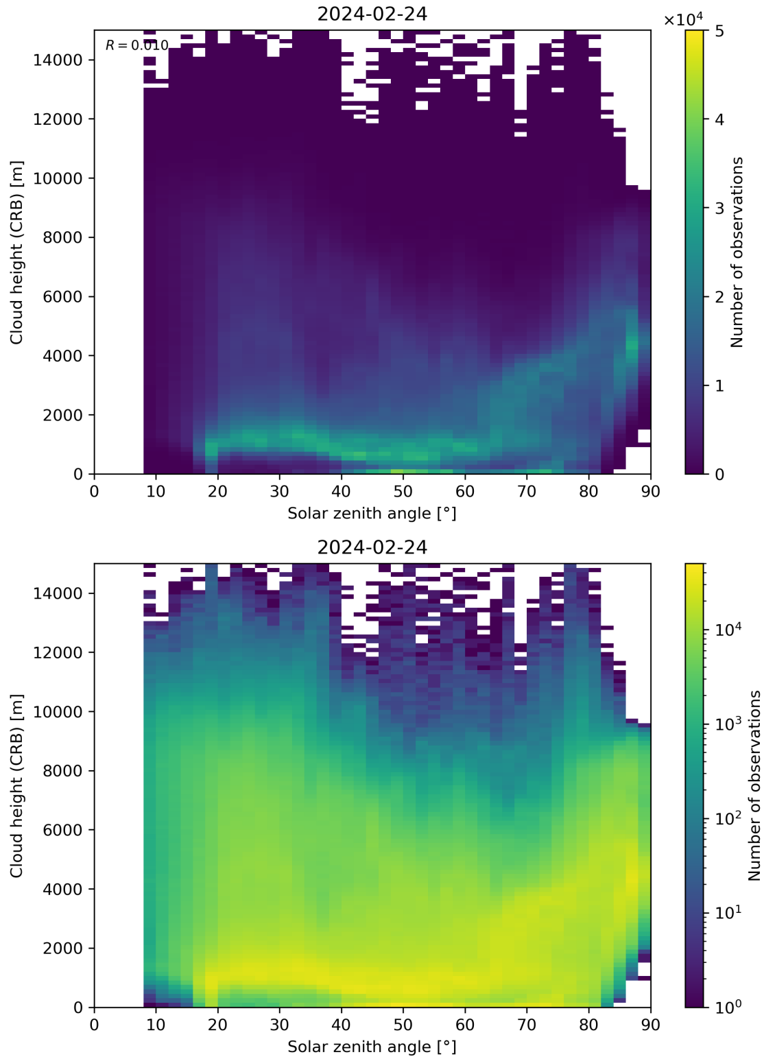
Figure 102: Scatter density plot of “Solar zenith angle” against “Cloud height (CRB)” for 2024-02-23 to 2024-02-25.
