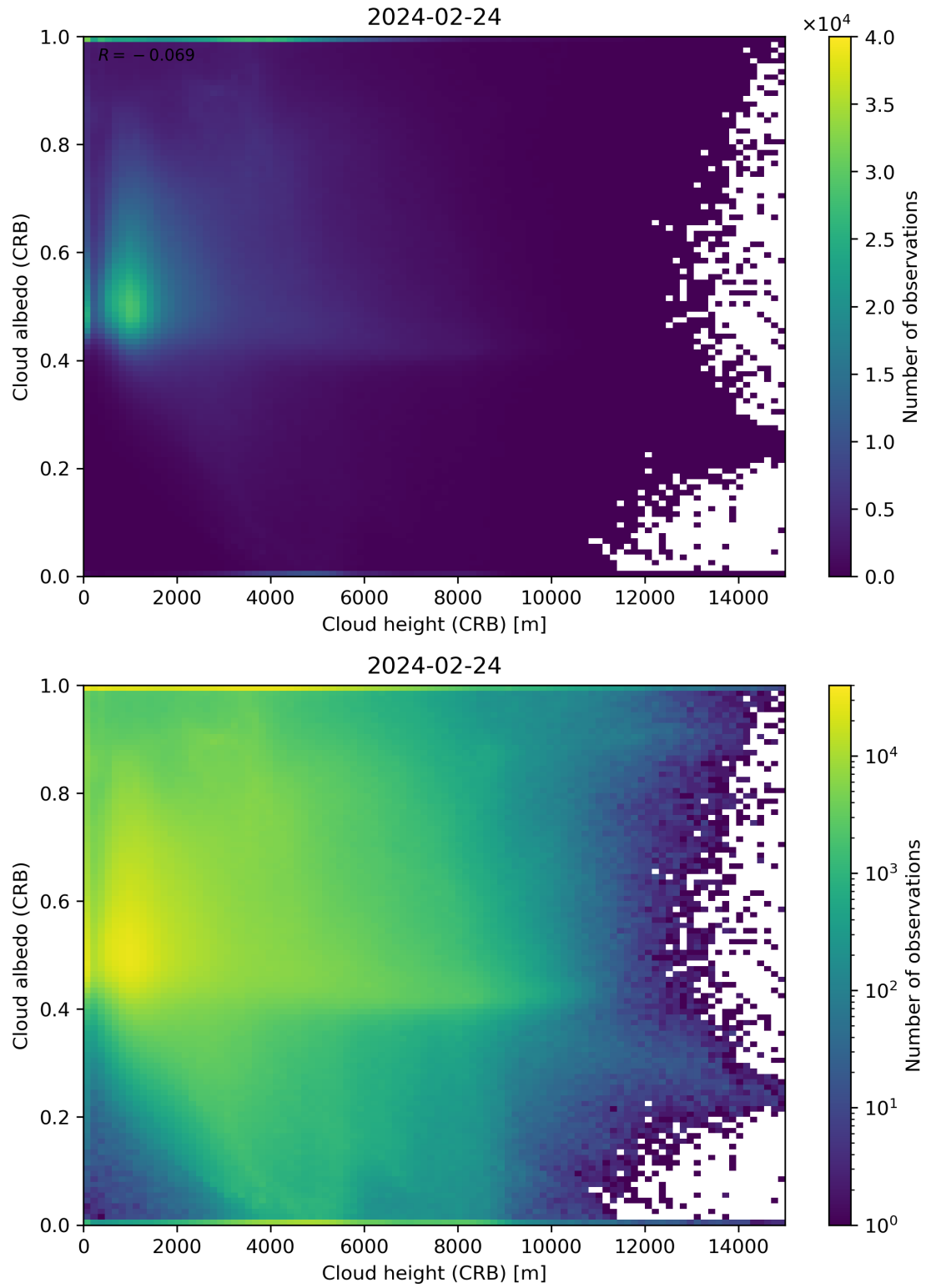
Figure 80: Scatter density plot of “Cloud height (CRB)” against “Cloud albedo (CRB)” for 2024-02-23 to 2024-02-25.
