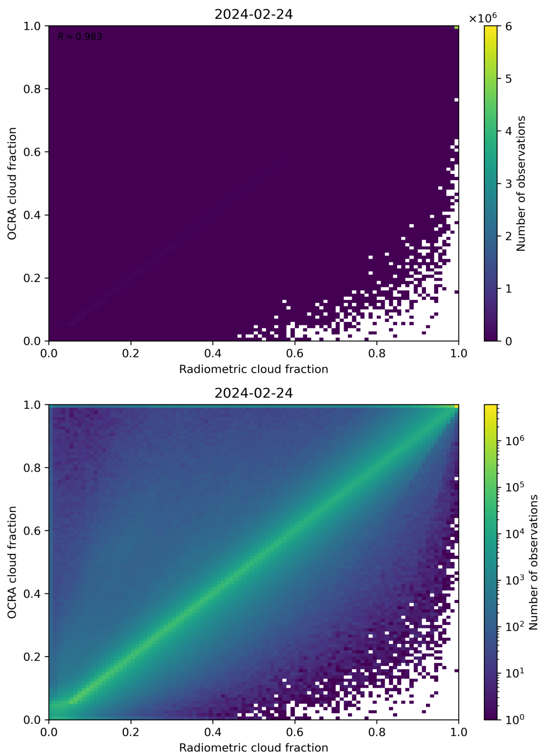
Figure 72: Scatter density plot of “Radiometric cloud fraction” against “OCRA cloud fraction” for 2024-02-23 to 2024-02-25.
