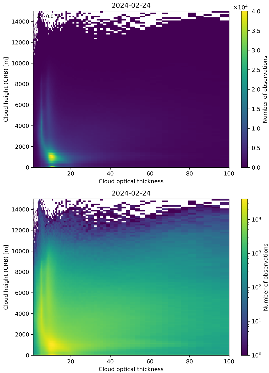
Figure 85: Scatter density plot of “Cloud optical thickness” against “Cloud height (CRB)” for 2024-02-23 to 2024-02-25.
