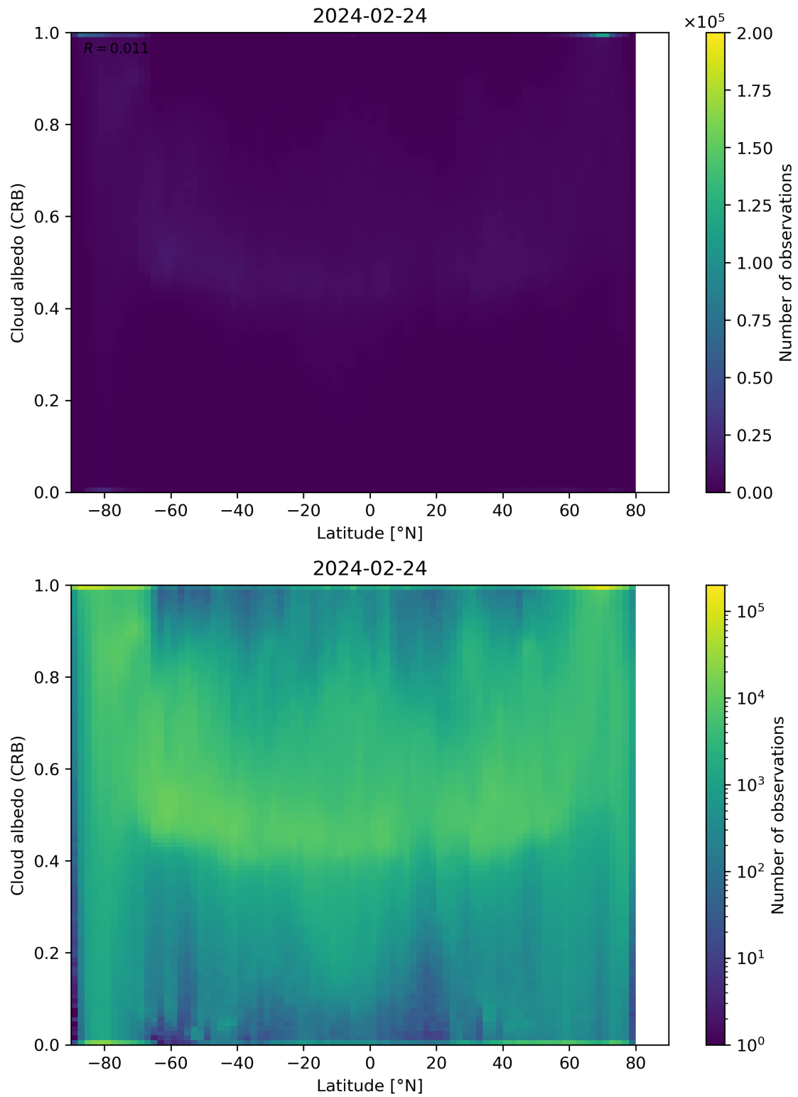
Figure 91: Scatter density plot of “Latitude” against “Cloud albedo (CRB)” for 2024-02-23 to 2024-02-25.
