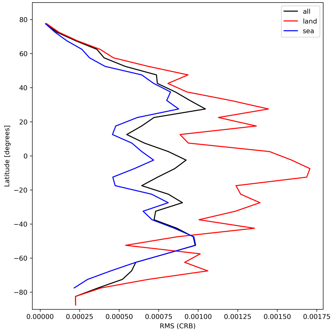
Figure 32: Zonal average of “RMS (CRB)” for 2024-02-23 to 2024-02-25.
