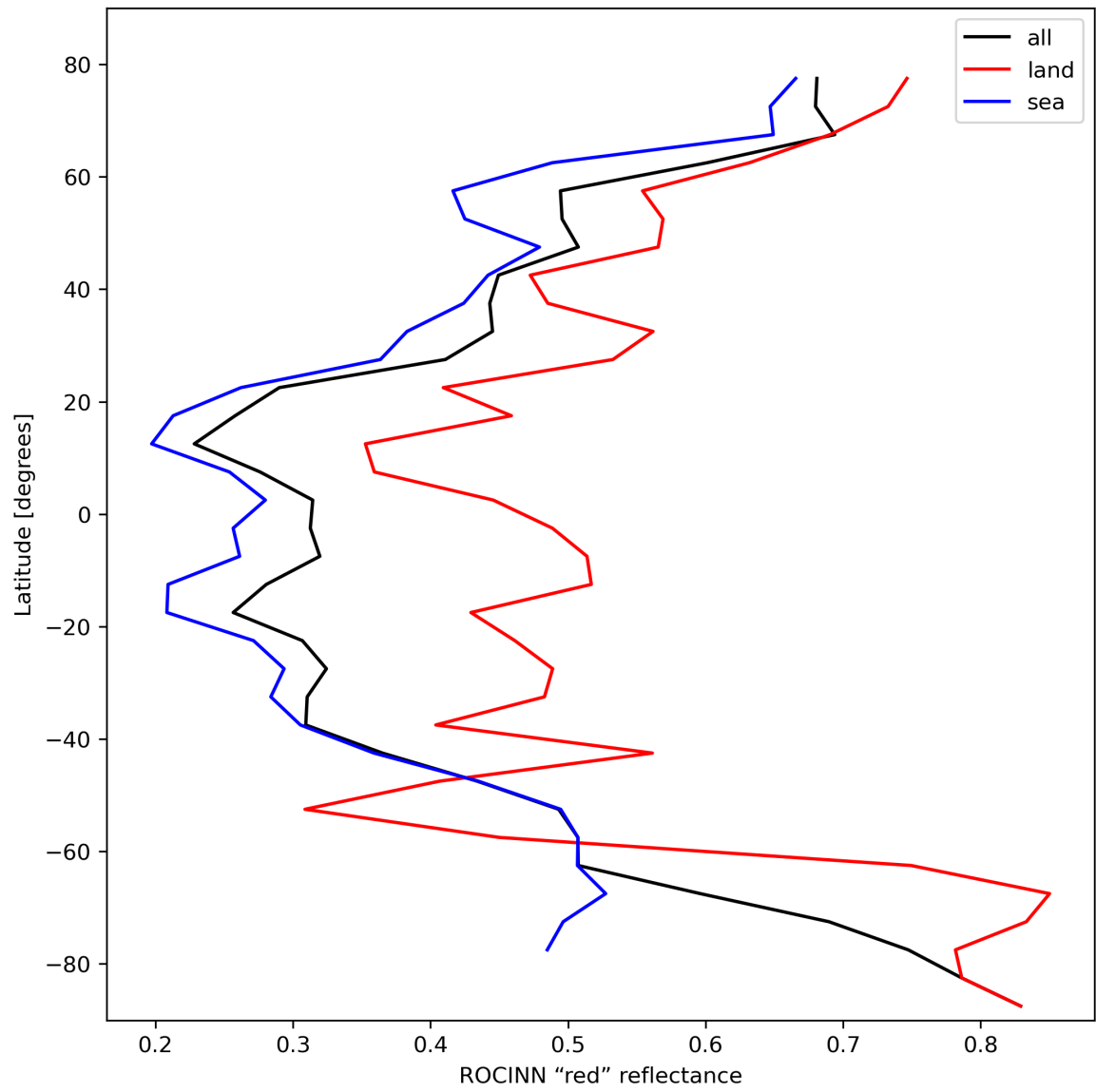
Figure 37: Zonal average of “ROCINN “red” reflectance” for 2024-02-23 to 2024-02-25.
