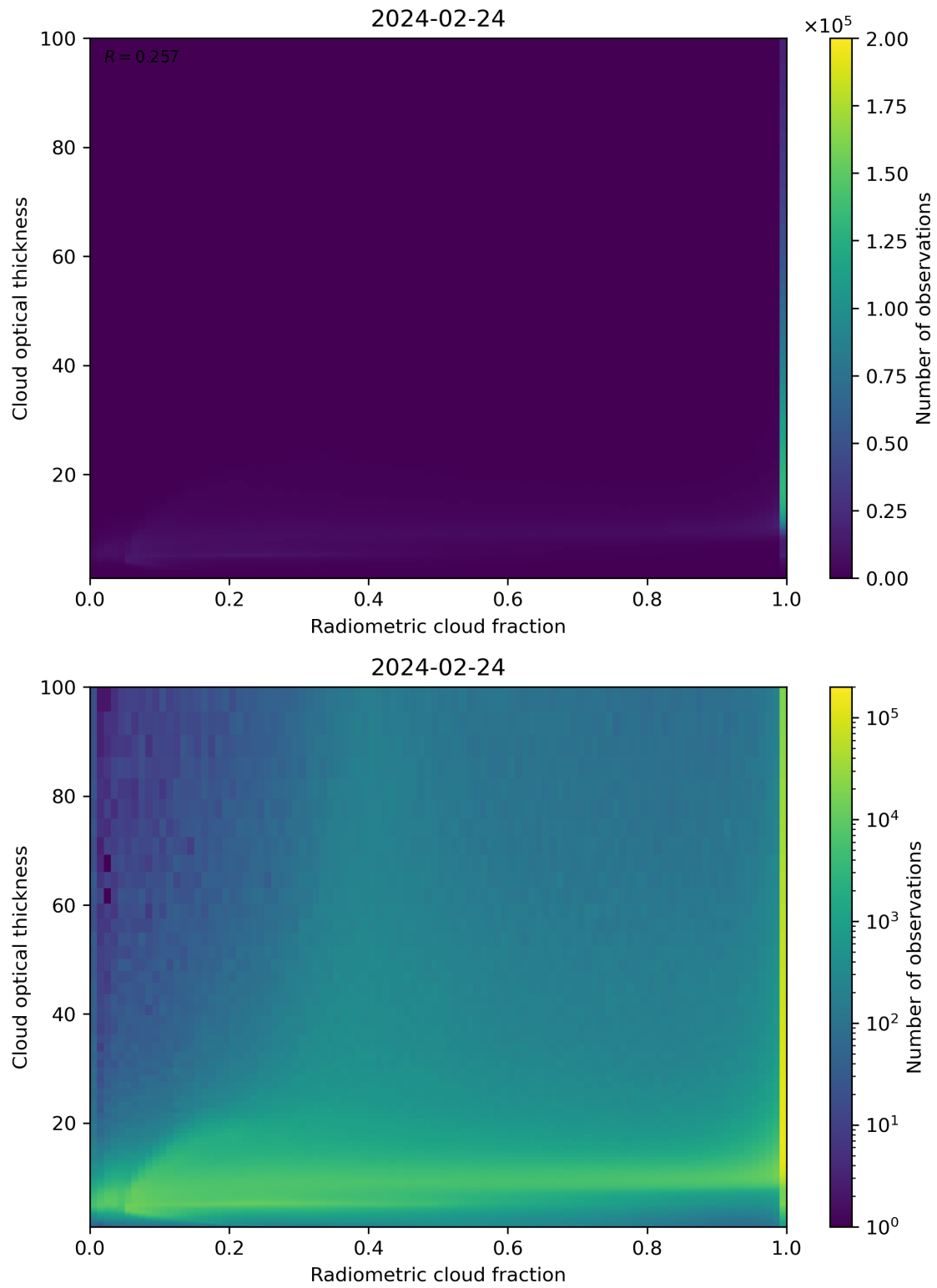
Figure 75: Scatter density plot of “Radiometric cloud fraction” against “Cloud optical thickness” for 2024-02-23 to 2024-02-25.
