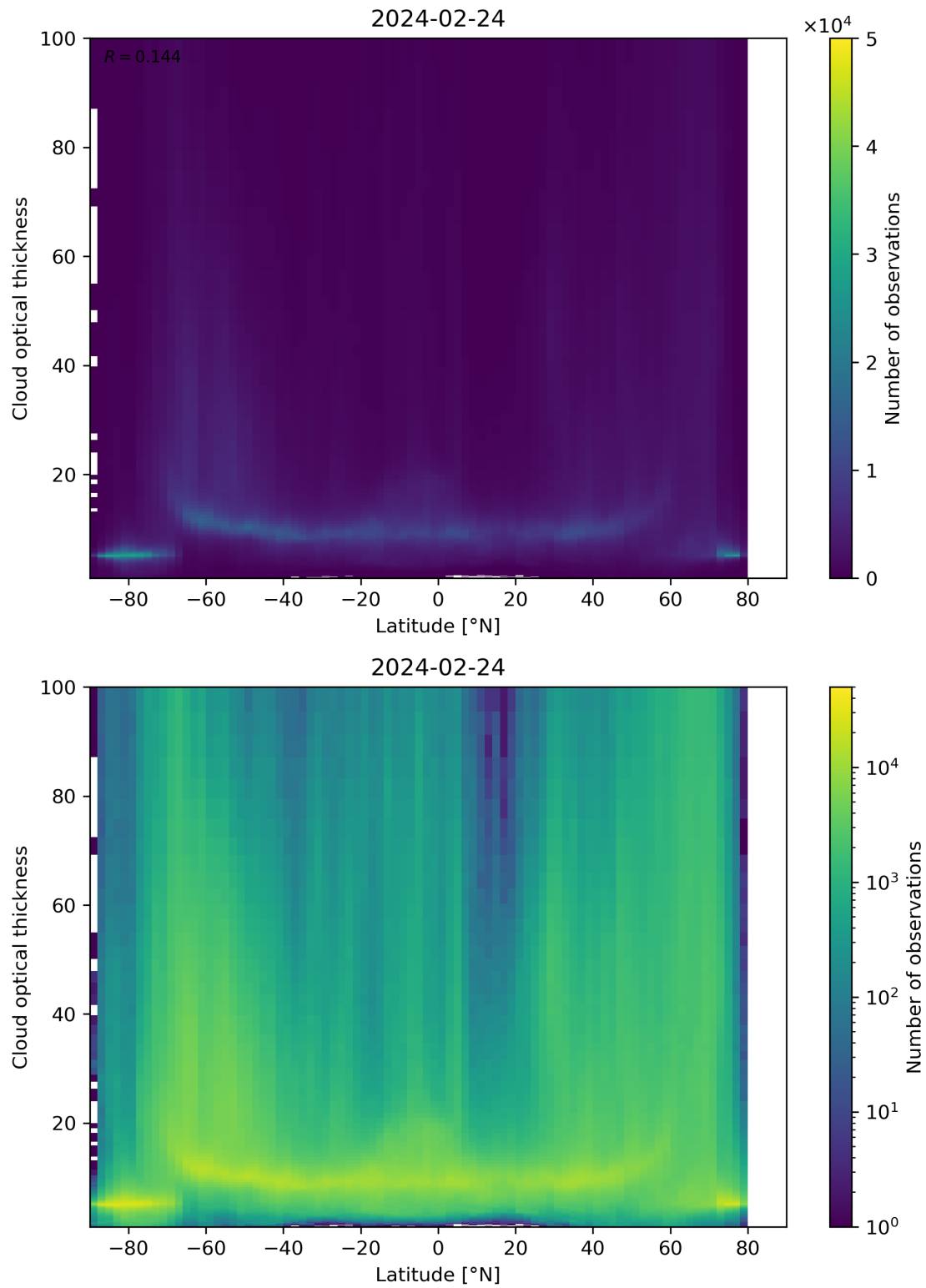
Figure 96: Scatter density plot of “Latitude” against “Cloud optical thickness” for 2024-02-23 to 2024-02-25.
