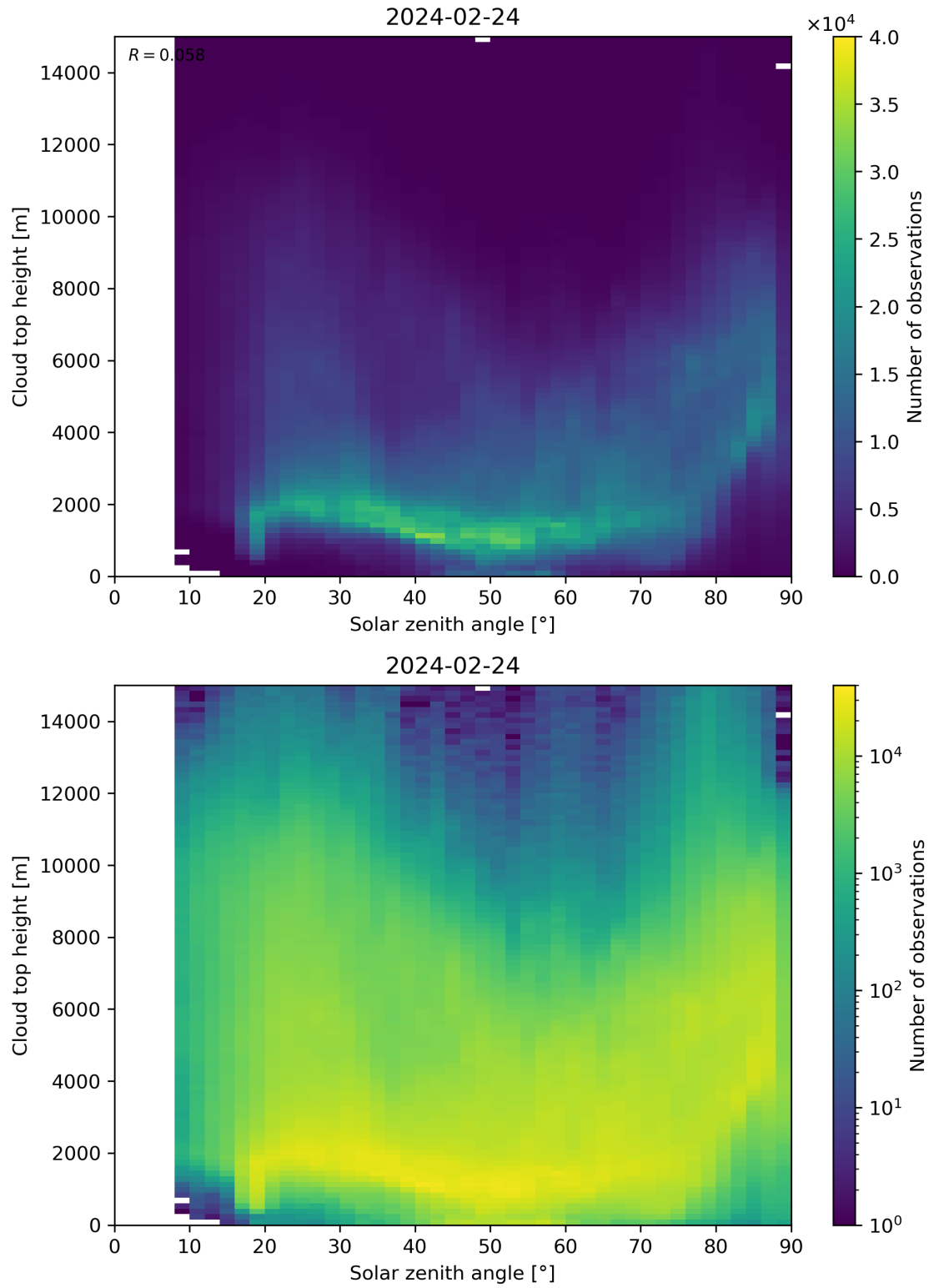
Figure 104: Scatter density plot of “Solar zenith angle” against “Cloud top height” for 2024-02-23 to 2024-02-25.
