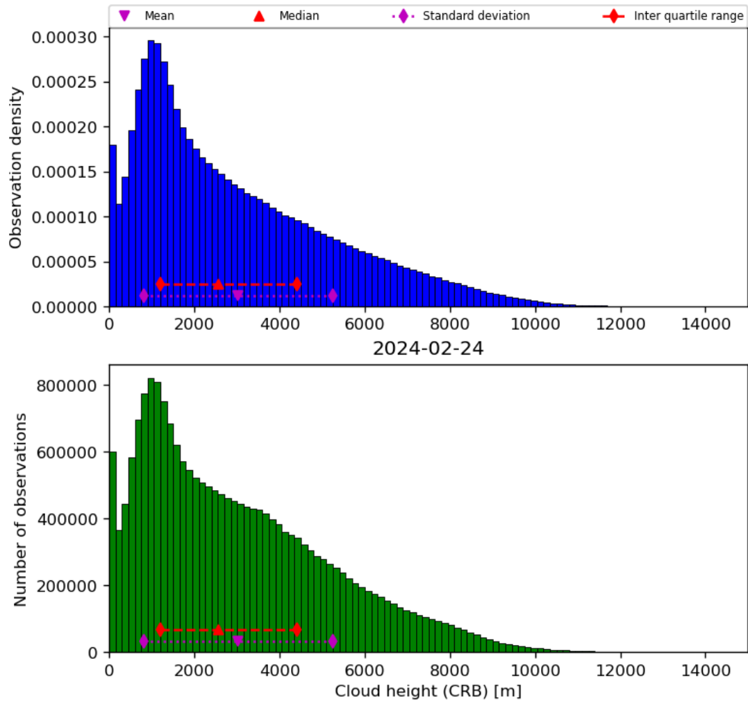
Figure 43: Histogram of “Cloud height (CRB)” for 2024-02-23 to 2024-02-25
