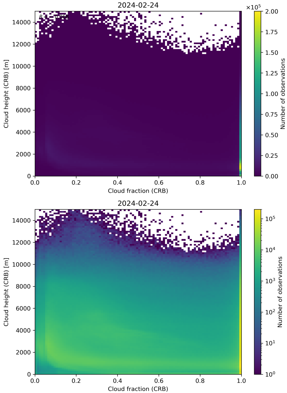
Figure 79: Scatter density plot of “Cloud fraction (CRB)” against “Cloud height (CRB)” for 2024-02-23 to 2024-02-25.
