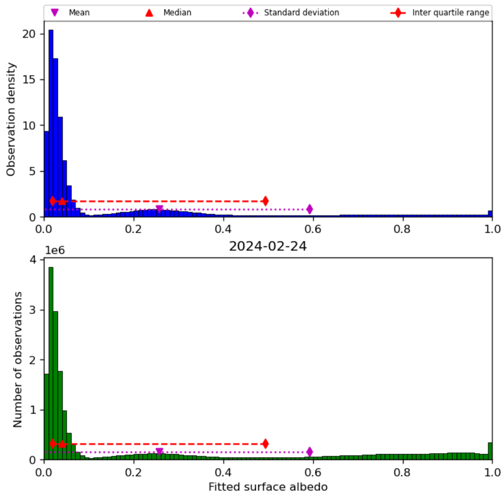
Figure 45: Histogram of “Fitted surface albedo” for 2024-02-23 to 2024-02-25
