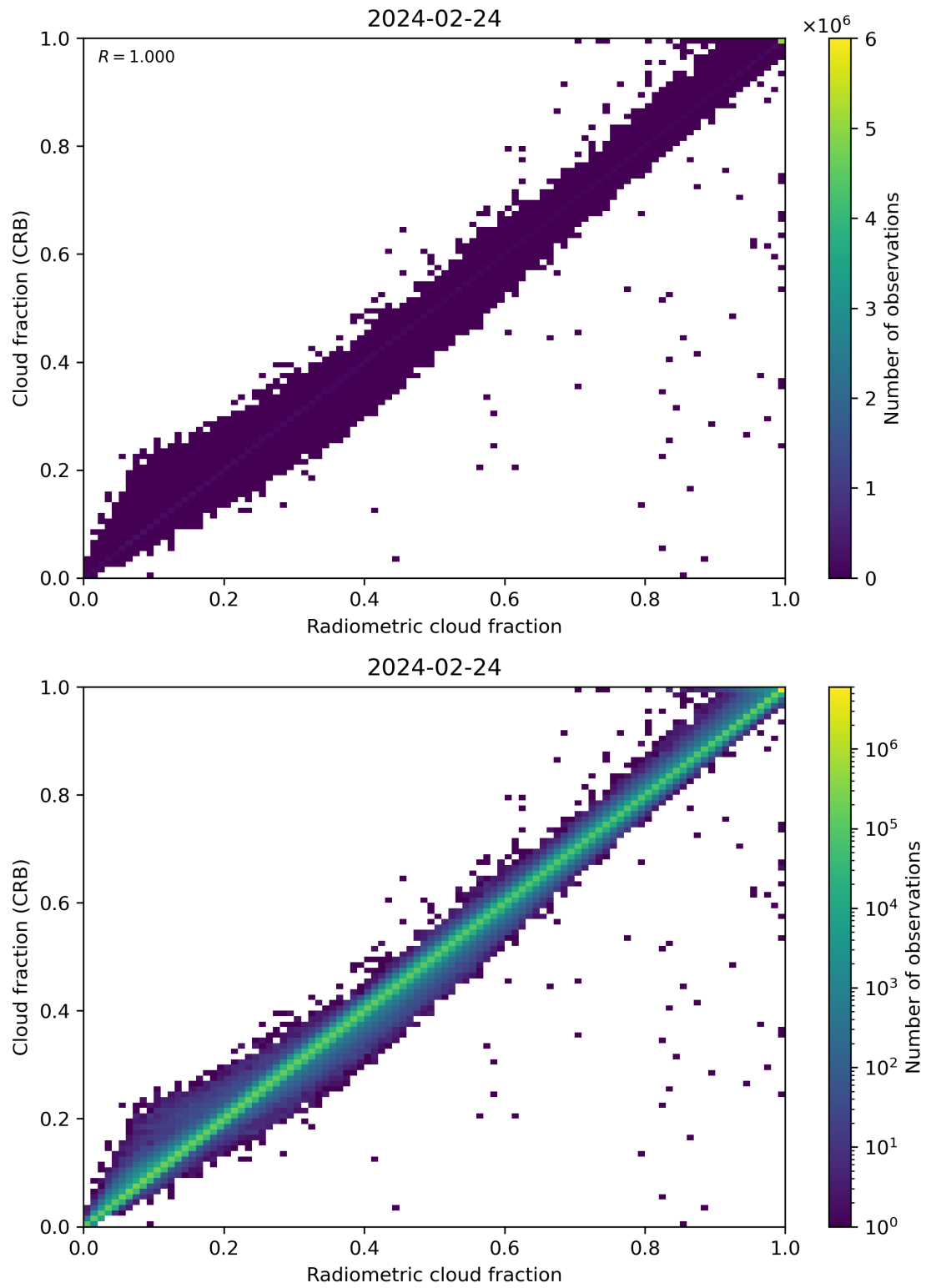
Figure 73: Scatter density plot of “Radiometric cloud fraction” against “Cloud fraction (CRB)” for 2024-02-23 to 2024-02-25.
