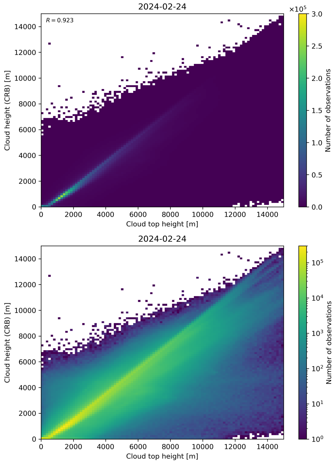
Figure 89: Scatter density plot of “Cloud top height” against “Cloud height (CRB)” for 2024-02-23 to 2024-02-25.
