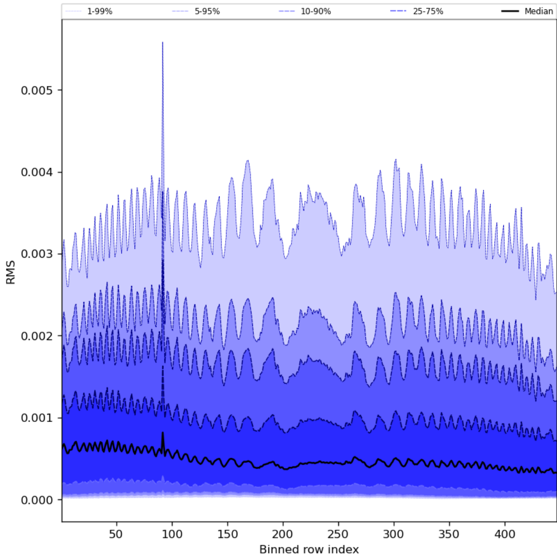
Figure 63: Along track statistics of “RMS” for 2024-02-23 to 2024-02-25
