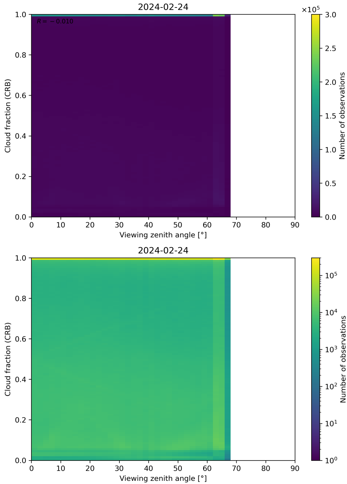
Figure 109: Scatter density plot of “Viewing zenith angle” against “Cloud fraction (CRB)” for 2024-02-23 to 2024-02-25.
