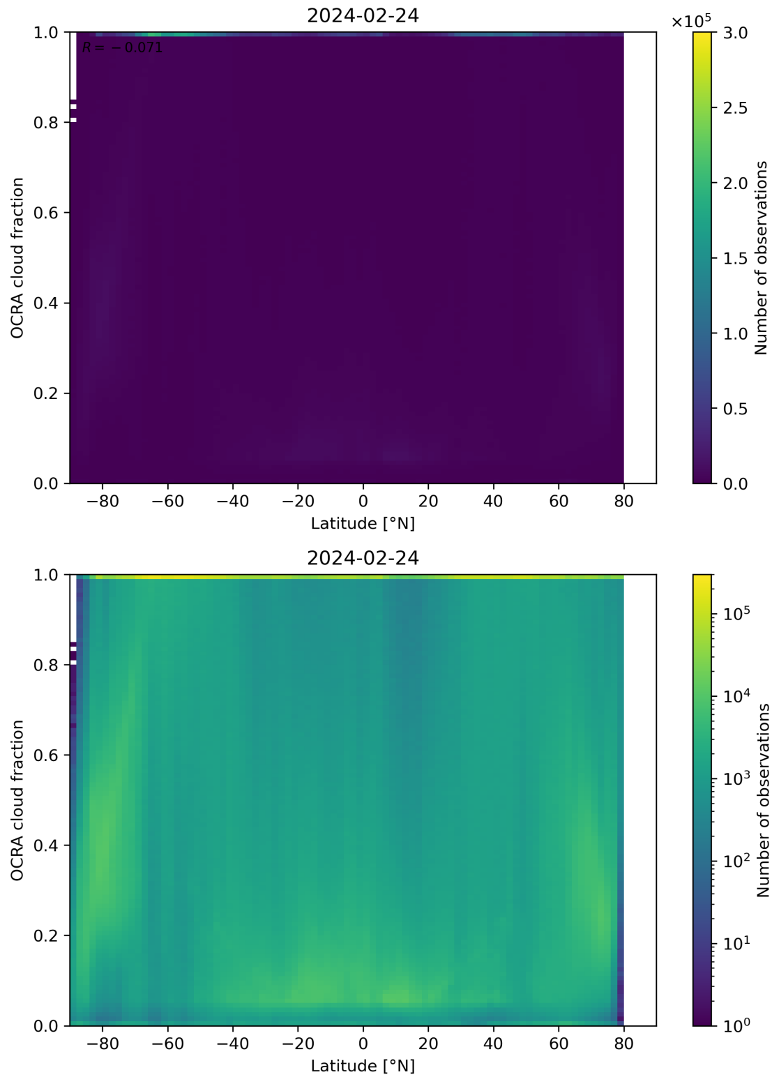
Figure 93: Scatter density plot of “Latitude” against “OCRA cloud fraction” for 2024-02-23 to 2024-02-25.
