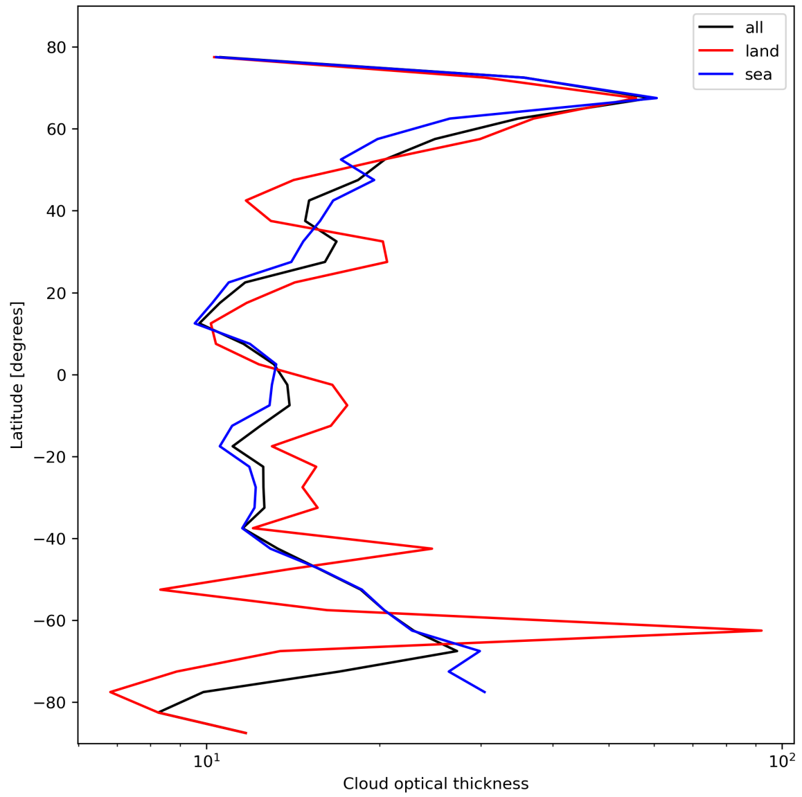
Figure 25: Zonal average of “Cloud optical thickness” for 2024-02-23 to 2024-02-25.
