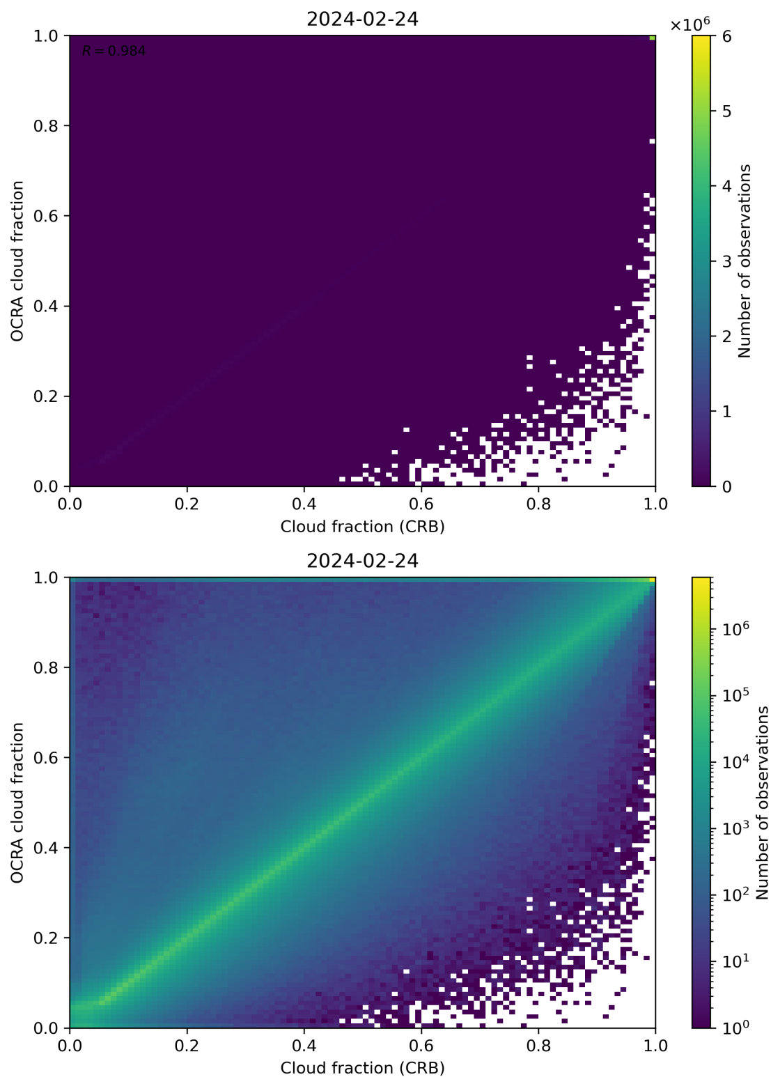
Figure 78: Scatter density plot of “Cloud fraction (CRB)” against “OCRA cloud fraction” for 2024-02-23 to 2024-02-25.
