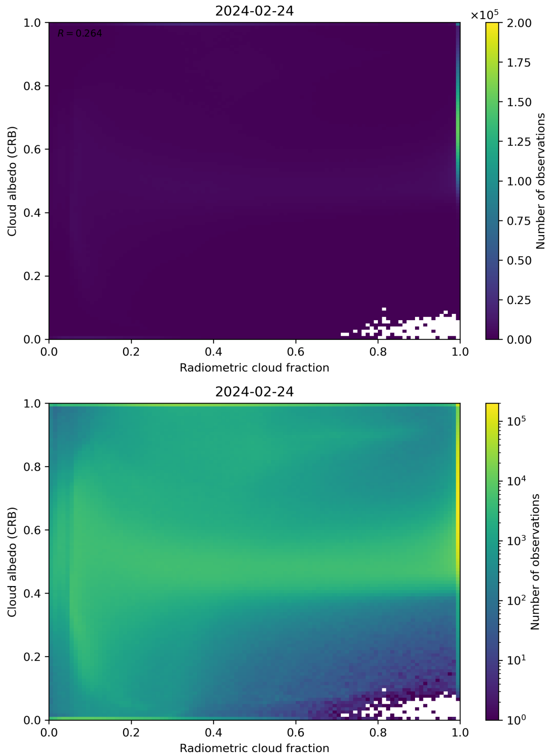
Figure 71: Scatter density plot of “Radiometric cloud fraction” against “Cloud albedo (CRB)” for 2024-02-23 to 2024-02-25.
