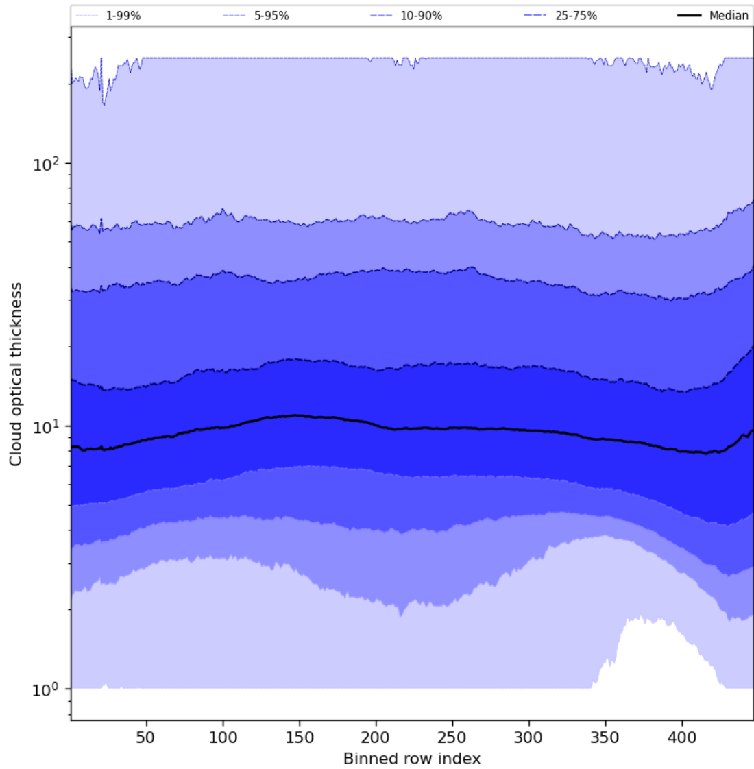
Figure 57: Along track statistics of “Cloud optical thickness” for 2024-02-23 to 2024-02-25
