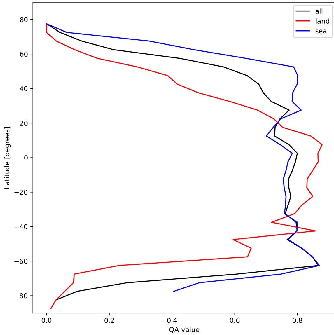
Figure 22: Zonal average of “QA value” for 2024-02-23 to 2024-02-25.
