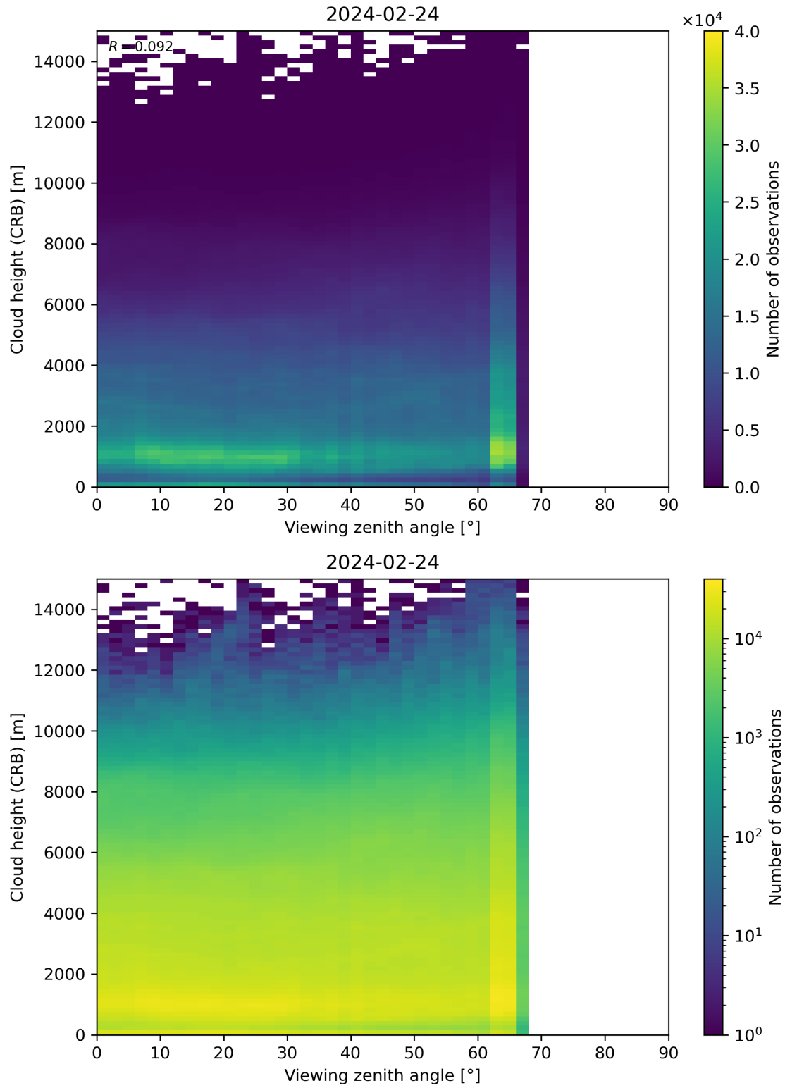
Figure 110: Scatter density plot of “Viewing zenith angle” against “Cloud height (CRB)” for 2024-02-23 to 2024-02-25.
