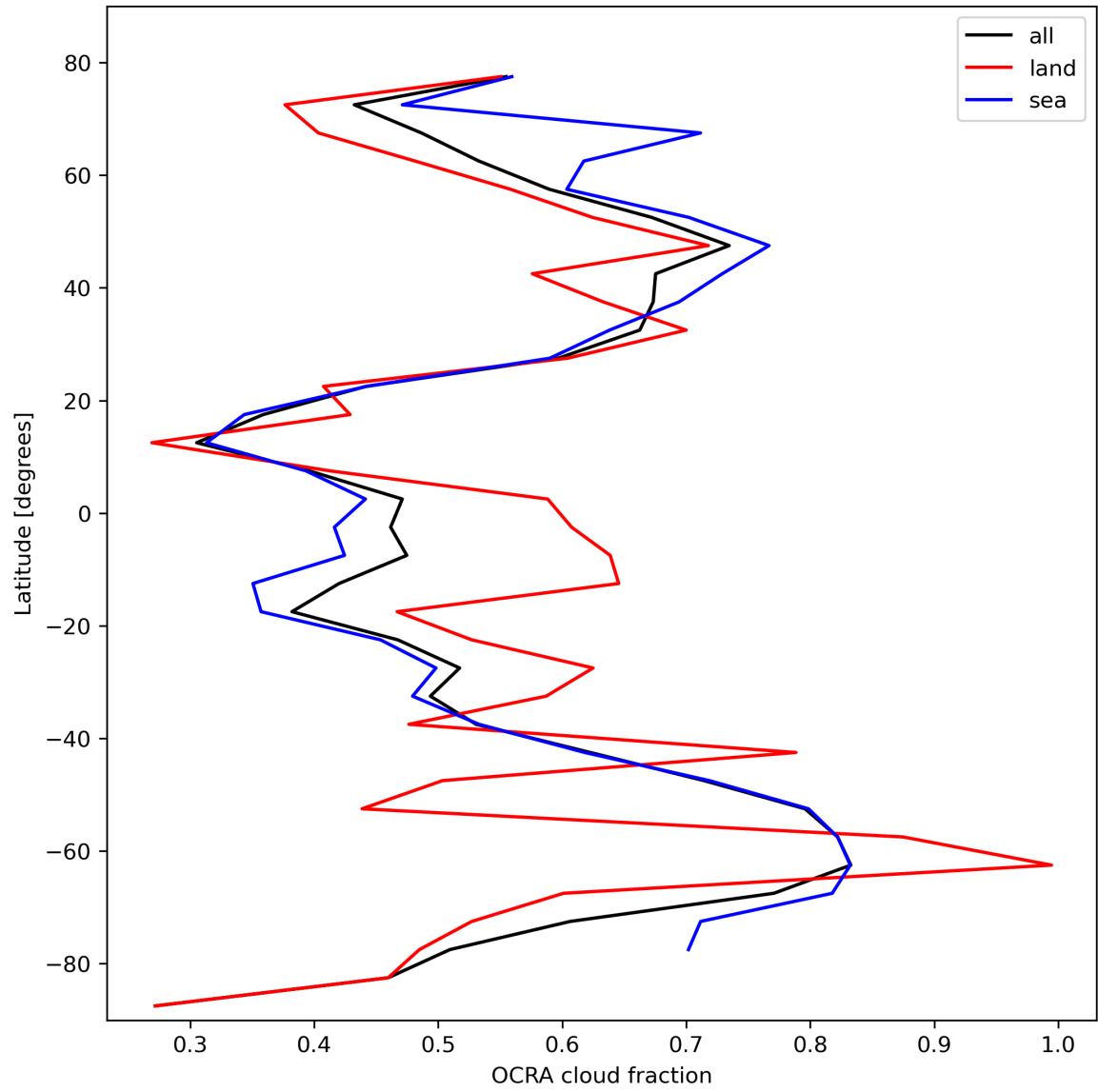
Figure 34: Zonal average of “OCRA cloud fraction” for 2024-02-23 to 2024-02-25.
