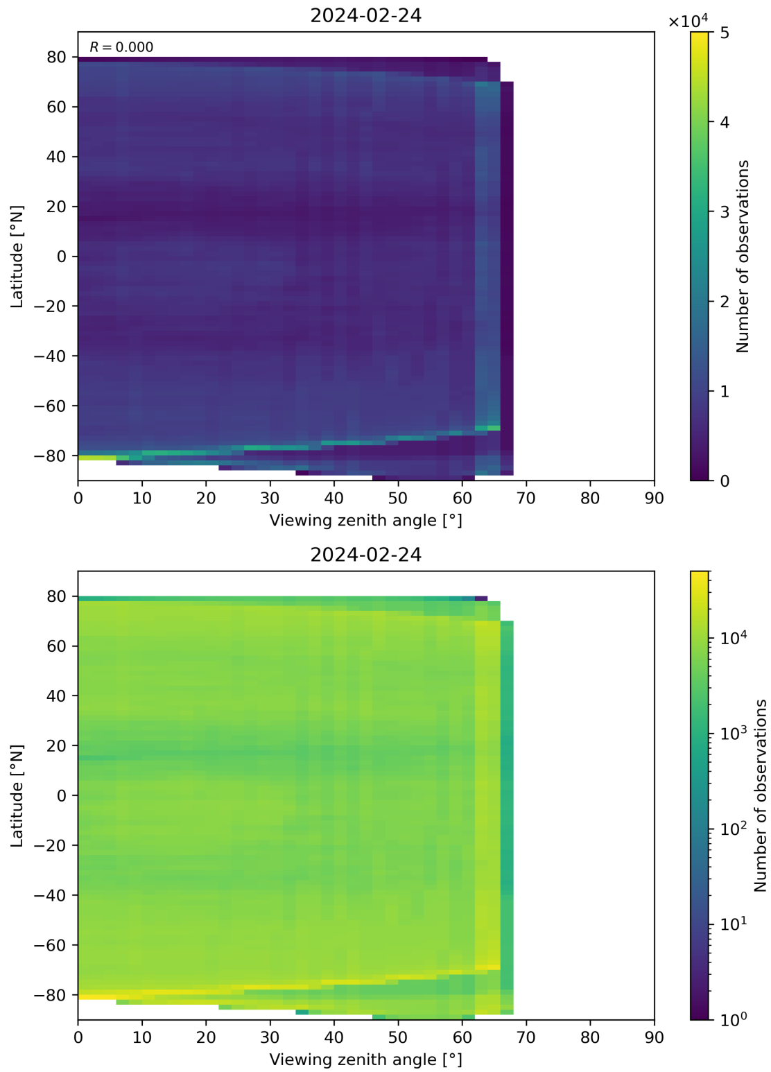
Figure 113: Scatter density plot of “Viewing zenith angle” against “Latitude” for 2024-02-23 to 2024-02-25.
