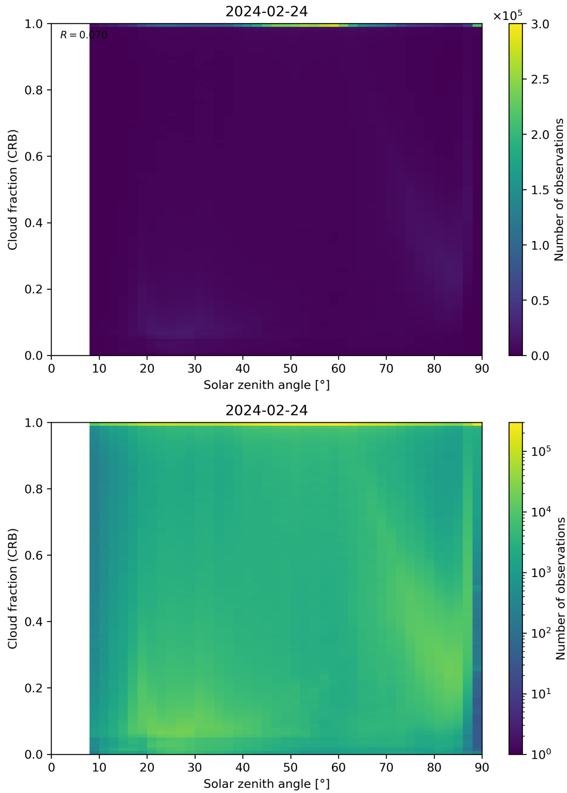
Figure 101: Scatter density plot of “Solar zenith angle” against “Cloud fraction (CRB)” for 2024-02-23 to 2024-02-25.
