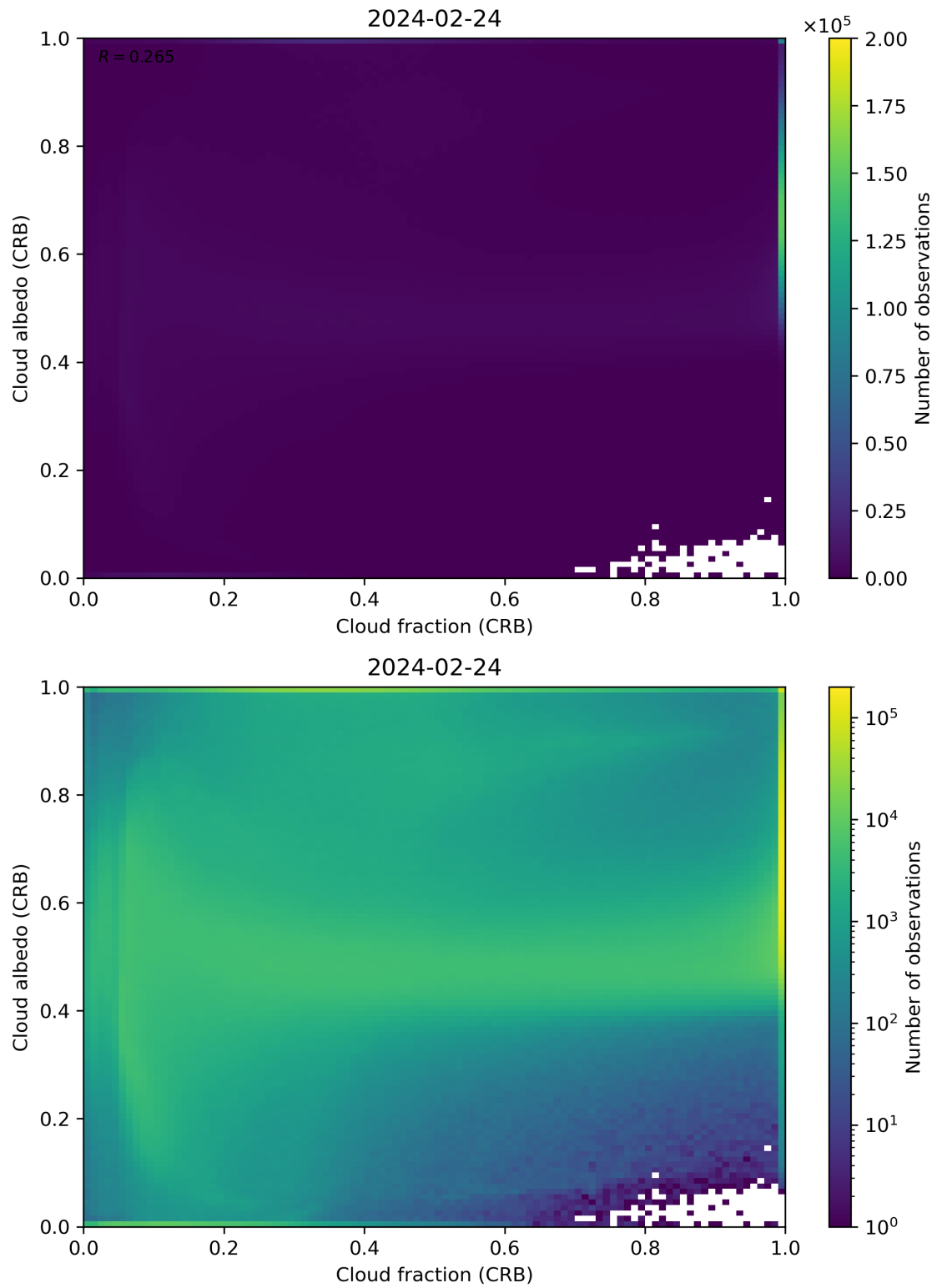
Figure 77: Scatter density plot of “Cloud fraction (CRB)” against “Cloud albedo (CRB)” for 2024-02-23 to 2024-02-25.
