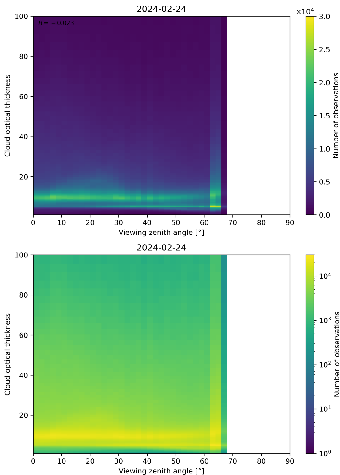
Figure 111: Scatter density plot of “Viewing zenith angle” against “Cloud optical thickness” for 2024-02-23 to 2024-02-25.
