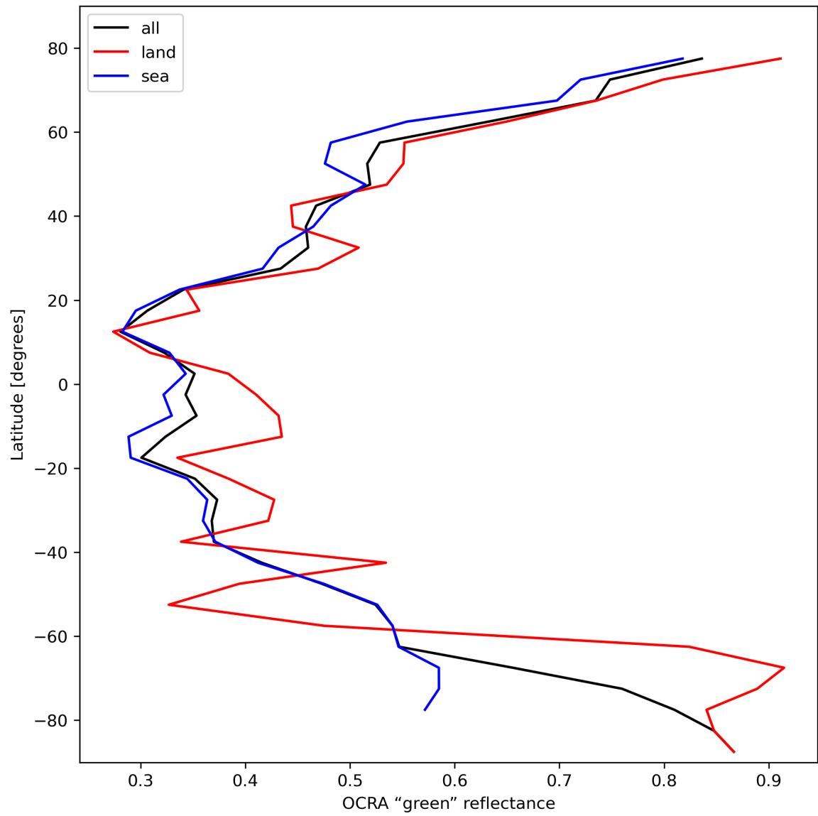
Figure 36: Zonal average of “OCRA “green” reflectance” for 2024-02-23 to 2024-02-25.
