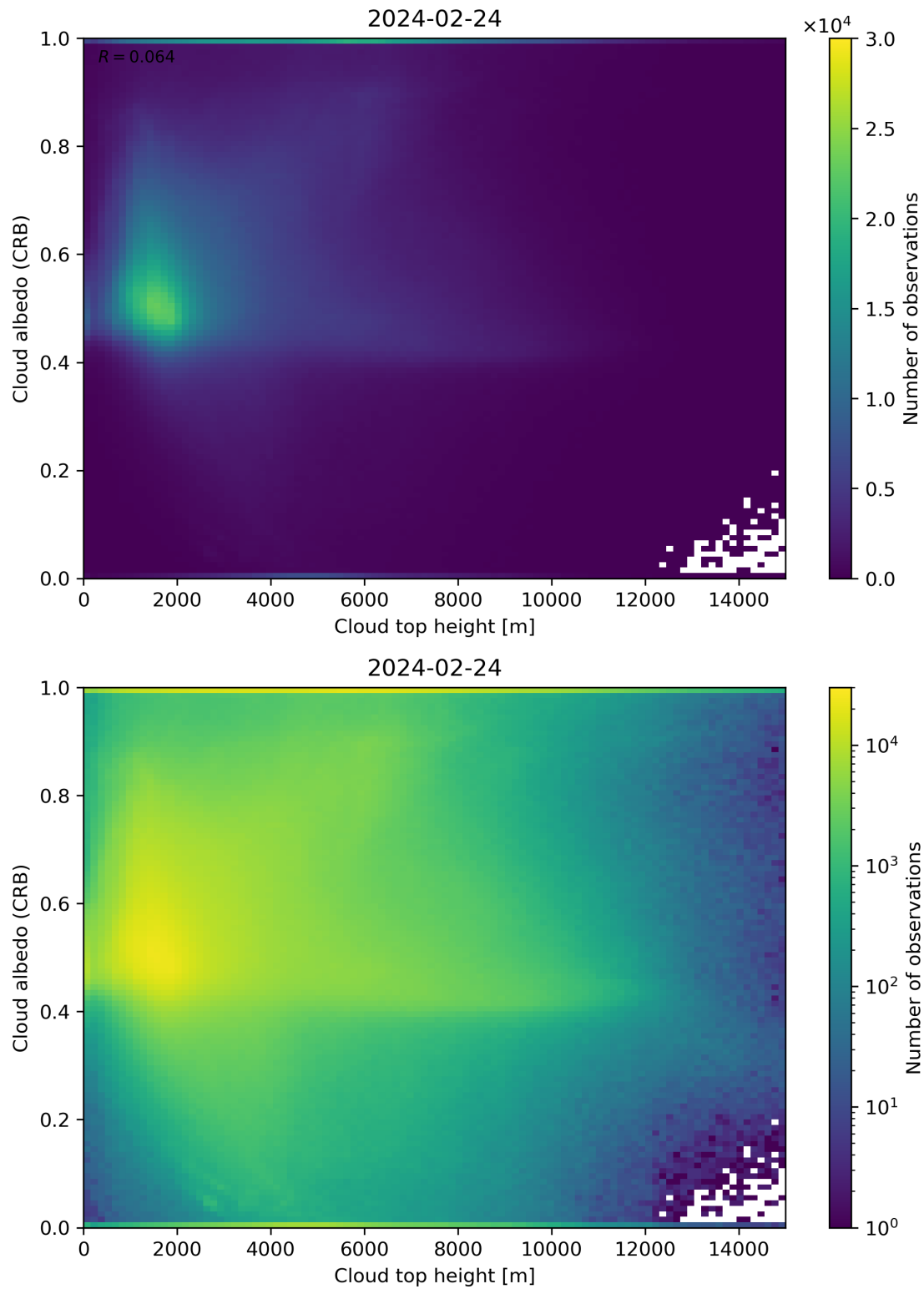
Figure 86: Scatter density plot of “Cloud top height” against “Cloud albedo (CRB)” for 2024-02-23 to 2024-02-25.
