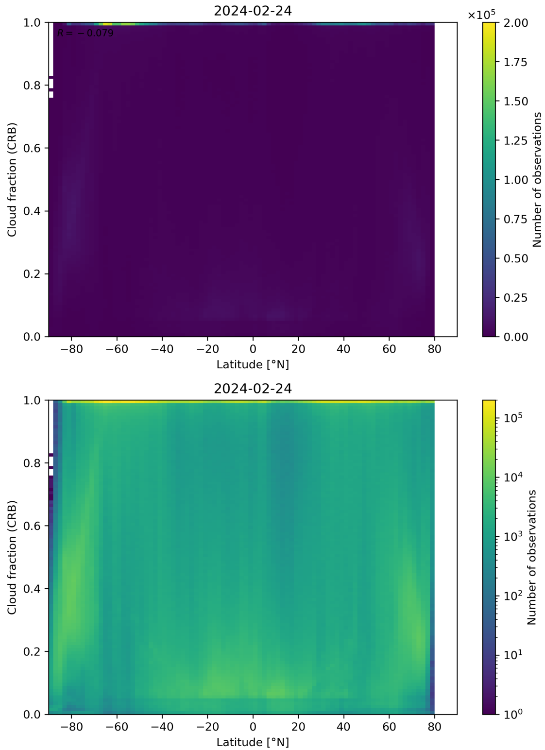
Figure 94: Scatter density plot of “Latitude” against “Cloud fraction (CRB)” for 2024-02-23 to 2024-02-25.
