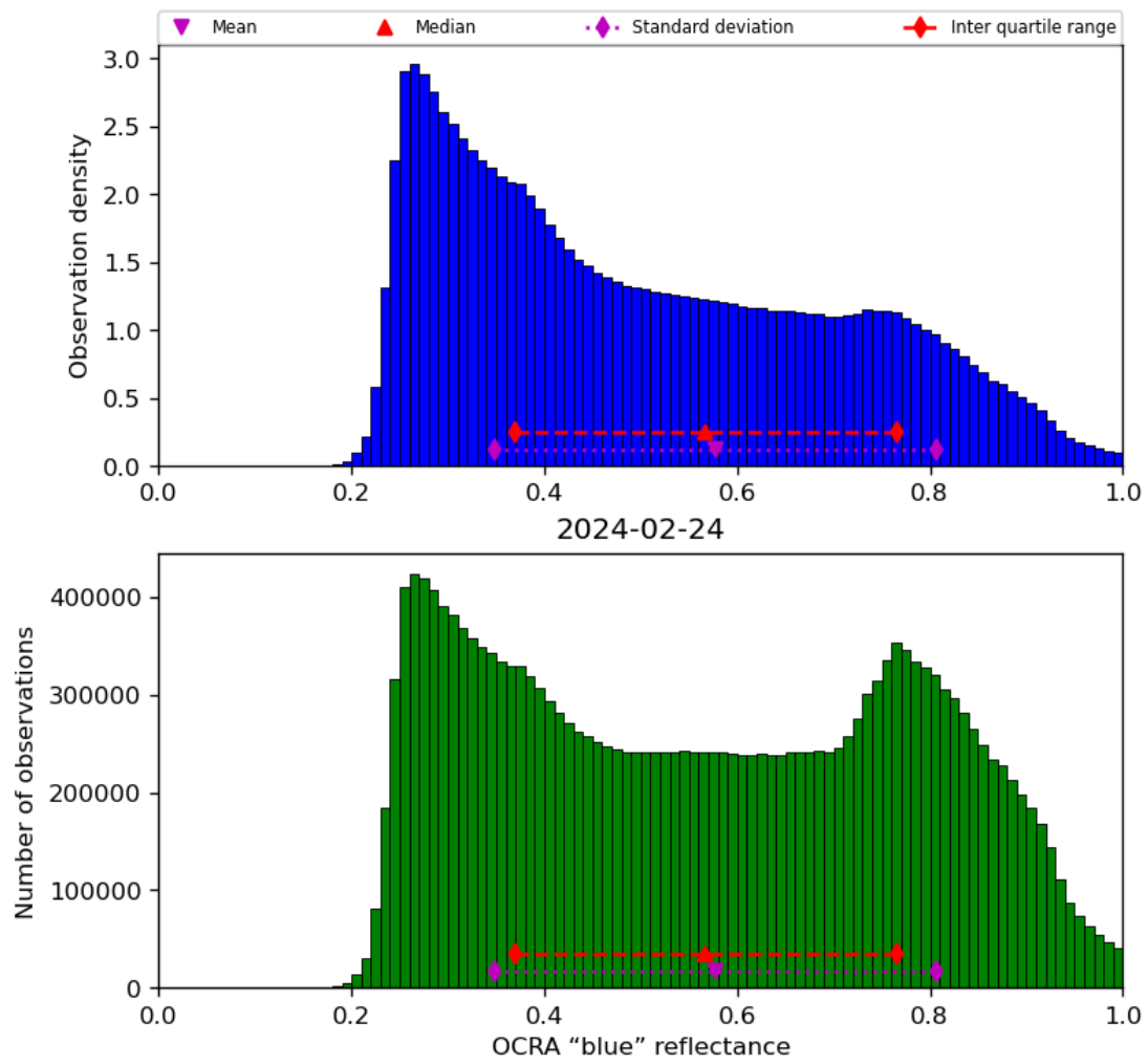
Figure 51: Histogram of “OCRA “blue” reflectance” for 2024-02-23 to 2024-02-25
