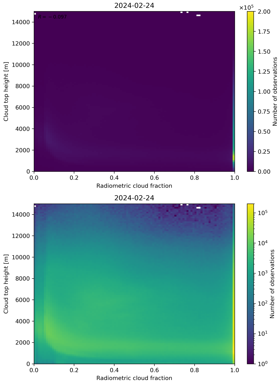
Figure 76: Scatter density plot of “Radiometric cloud fraction” against “Cloud top height” for 2024-02-23 to 2024-02-25.
