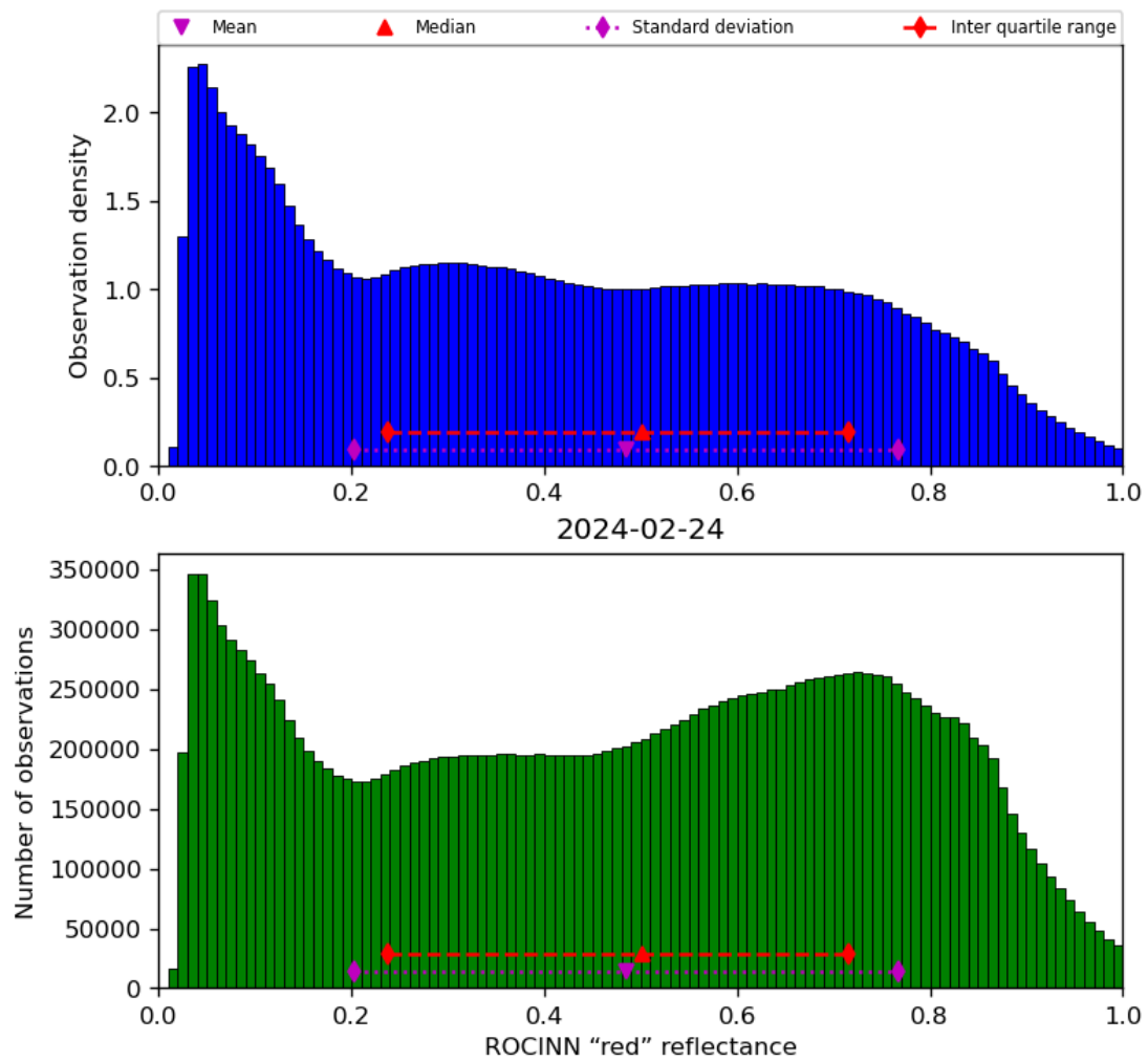
Figure 53: Histogram of “ROCINN “red” reflectance” for 2024-02-23 to 2024-02-25
