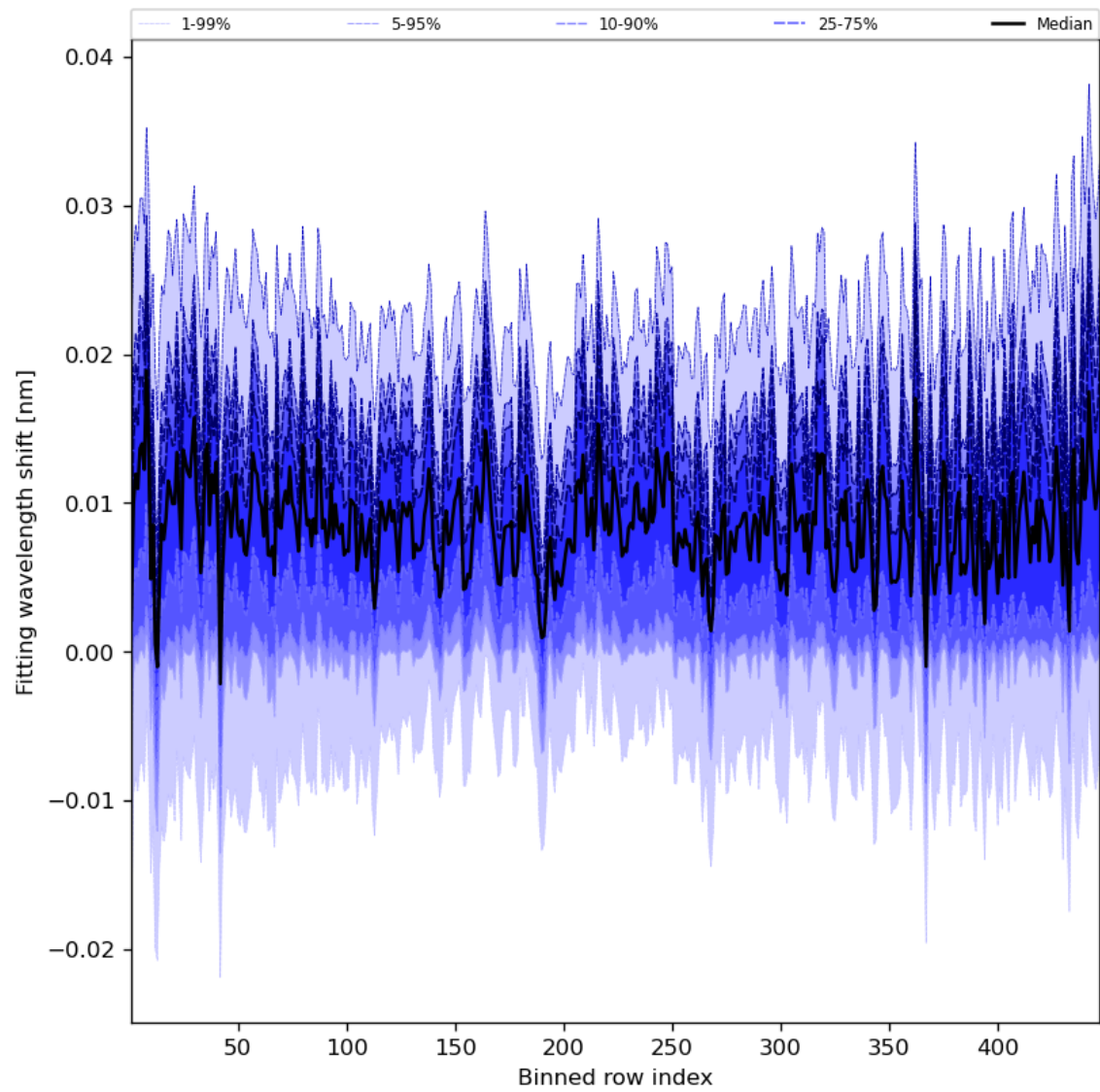
Figure 65: Along track statistics of “Fitting wavelength shift” for 2024-02-23 to 2024-02-25
