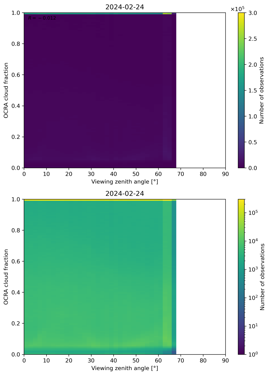
Figure 108: Scatter density plot of “Viewing zenith angle” against “OCRA cloud fraction” for 2024-02-23 to 2024-02-25.
