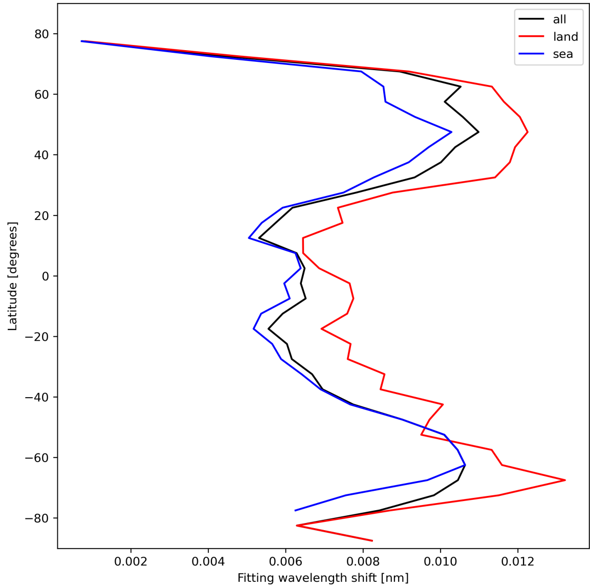
Figure 33: Zonal average of “Fitting wavelength shift” for 2024-02-23 to 2024-02-25.
