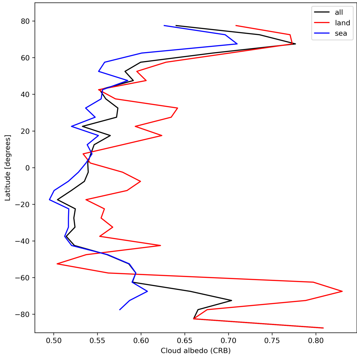
Figure 28: Zonal average of “Cloud albedo (CRB)” for 2024-02-23 to 2024-02-25.
