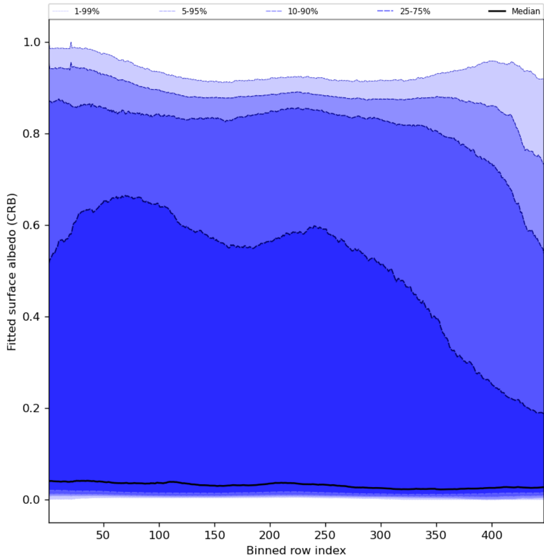
Figure 62: Along track statistics of “Fitted surface albedo (CRB)” for 2024-02-23 to 2024-02-25
