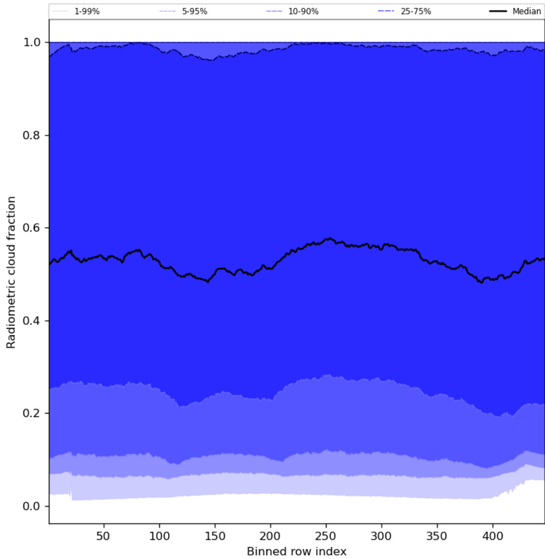
Figure 55: Along track statistics of “Radiometric cloud fraction” for 2024-02-23 to 2024-02-25
