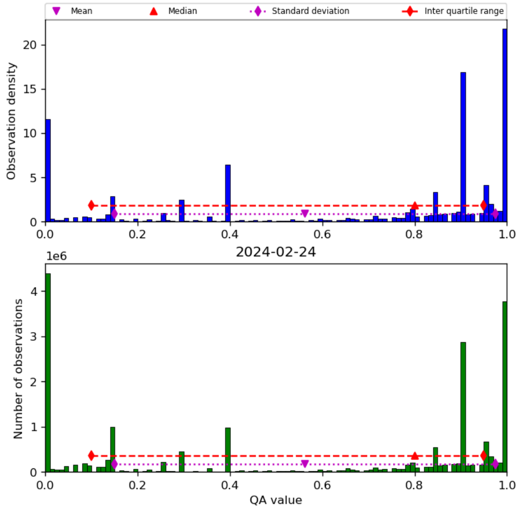
Figure 38: Histogram of “QA value” for 2024-02-23 to 2024-02-25
