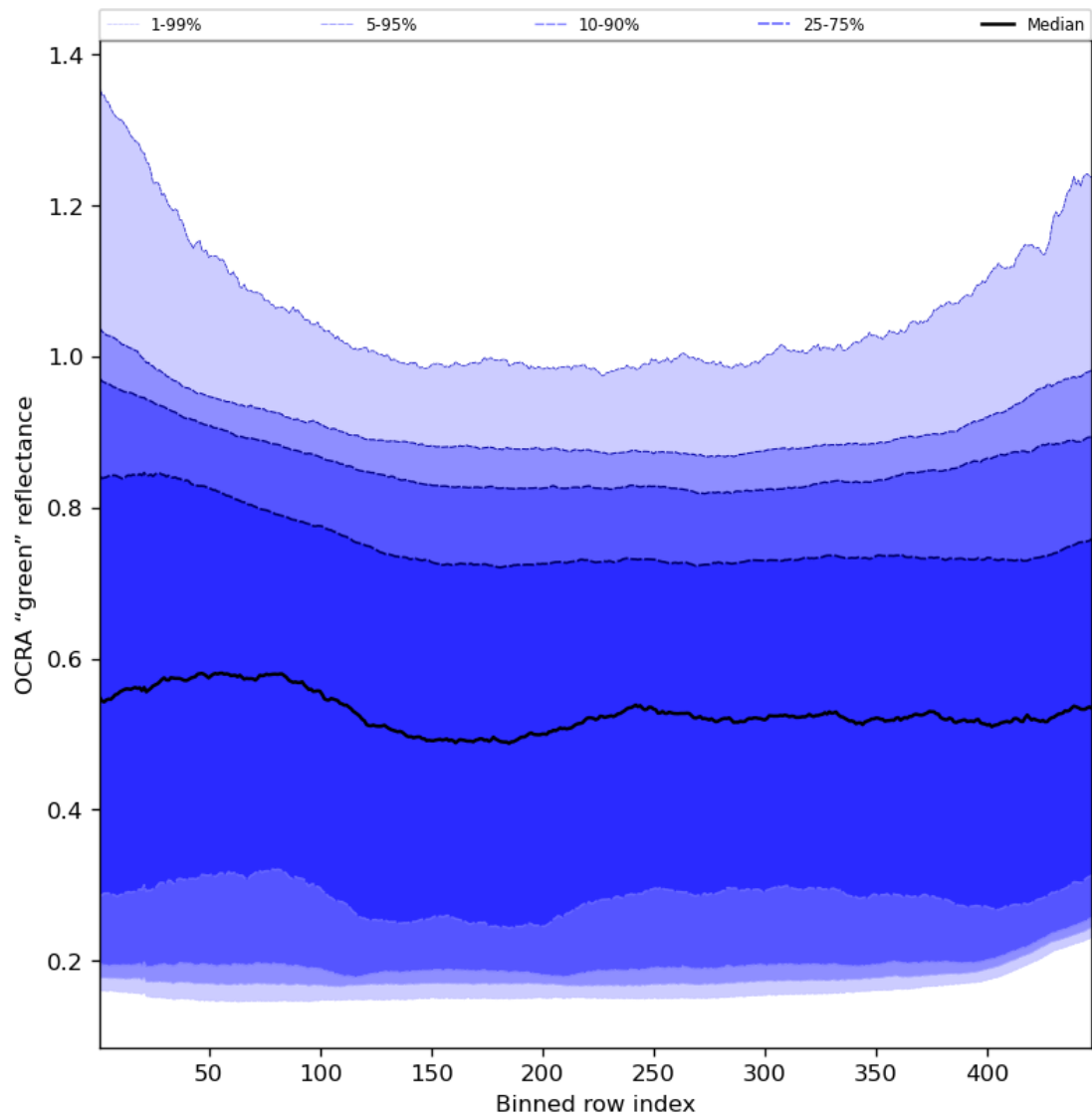
Figure 68: Along track statistics of “OCRA “green” reflectance” for 2024-02-23 to 2024-02-25
