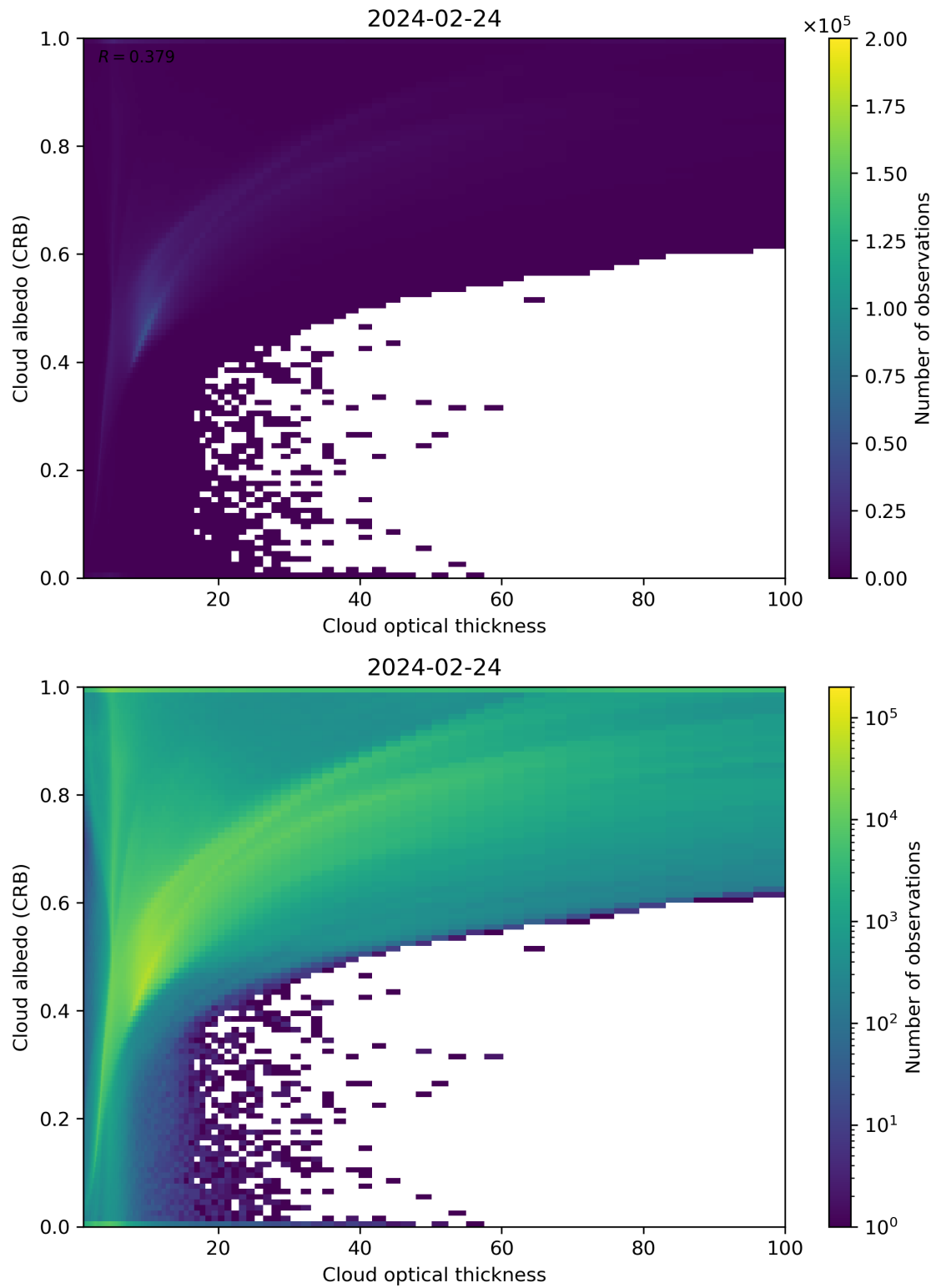
Figure 82: Scatter density plot of “Cloud optical thickness” against “Cloud albedo (CRB)” for 2024-02-23 to 2024-02-25.
