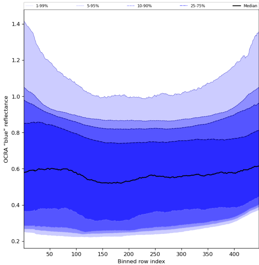
Figure 67: Along track statistics of “OCRA “blue” reflectance” for 2024-02-23 to 2024-02-25
