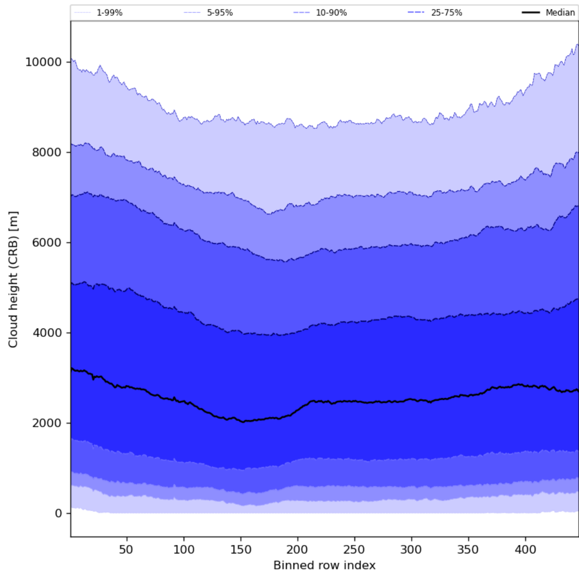
Figure 59: Along track statistics of “Cloud height (CRB)” for 2024-02-23 to 2024-02-25
