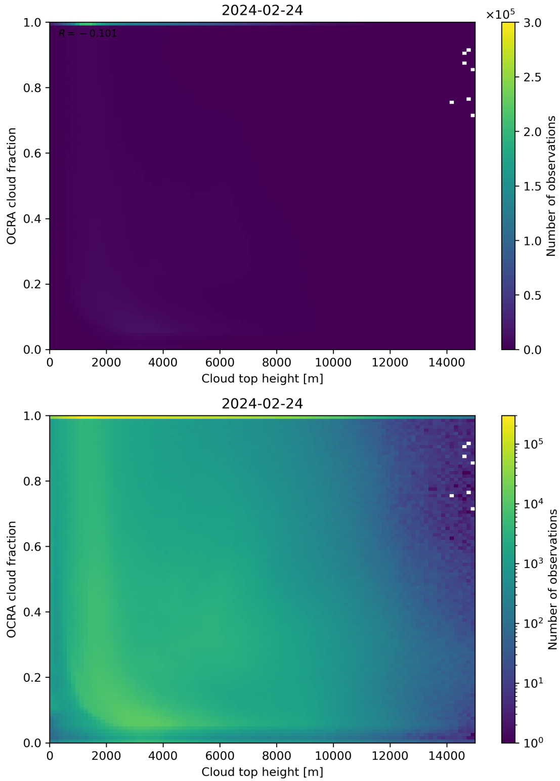
Figure 87: Scatter density plot of “Cloud top height” against “OCRA cloud fraction” for 2024-02-23 to 2024-02-25.
