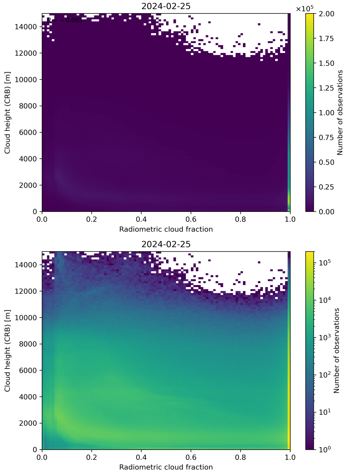
Figure 74: Scatter density plot of “Radiometric cloud fraction” against “Cloud height (CRB)” for 2024-02-24 to 2024-02-26.
