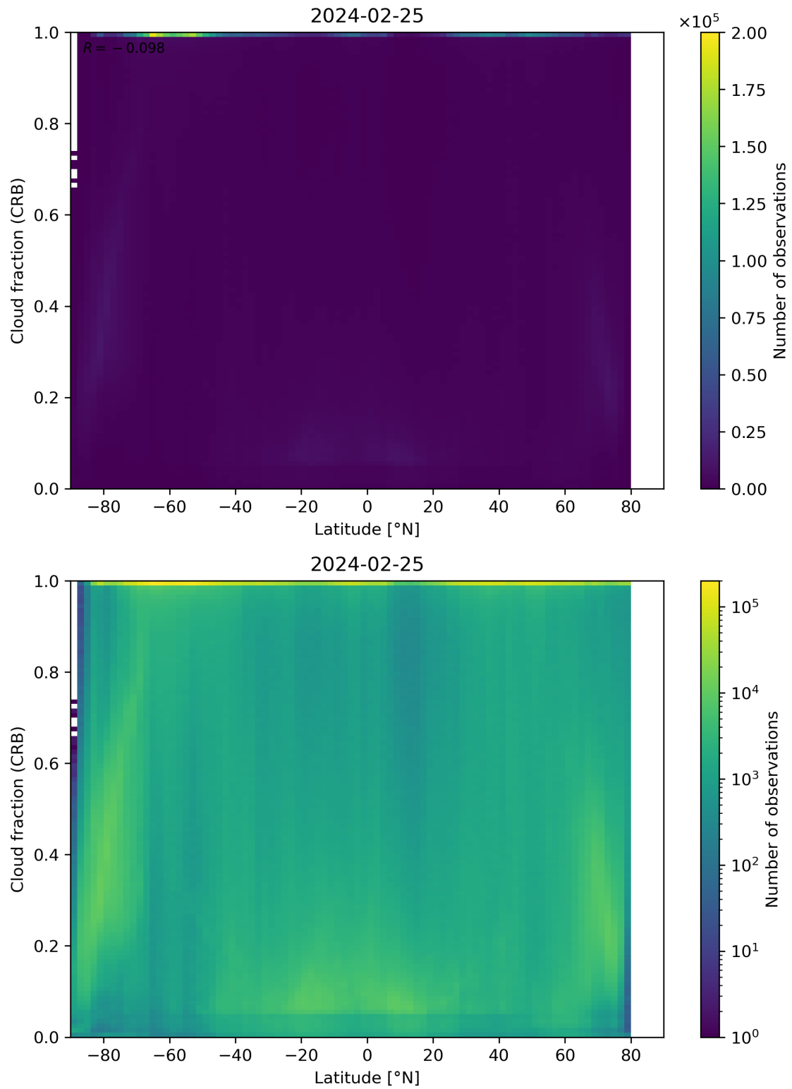
Figure 94: Scatter density plot of “Latitude” against “Cloud fraction (CRB)” for 2024-02-24 to 2024-02-26.
