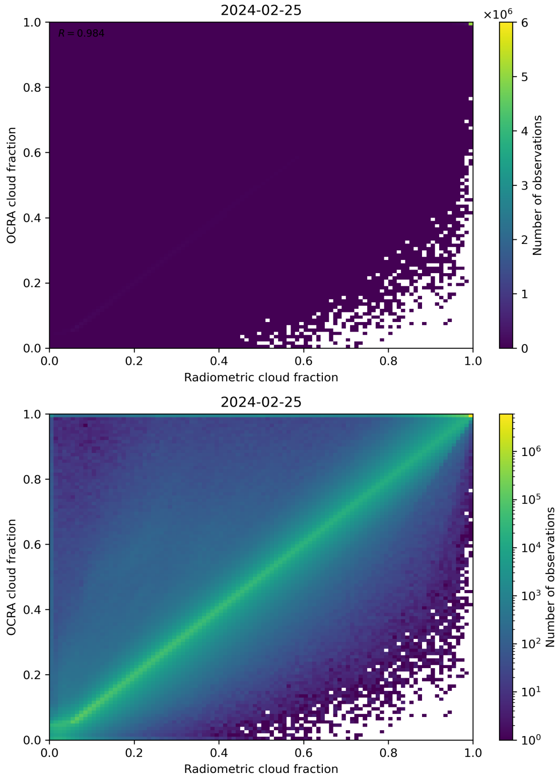
Figure 72: Scatter density plot of “Radiometric cloud fraction” against “OCRA cloud fraction” for 2024-02-24 to 2024-02-26.
