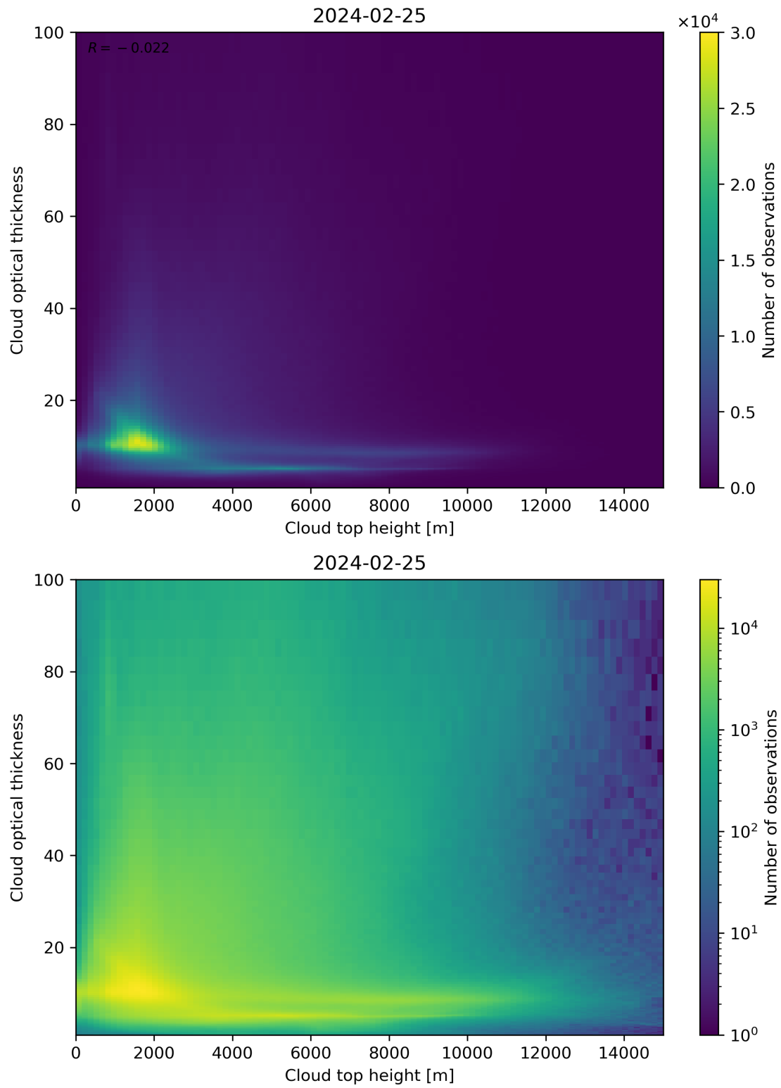
Figure 90: Scatter density plot of “Cloud top height” against “Cloud optical thickness” for 2024-02-24 to 2024-02-26.
