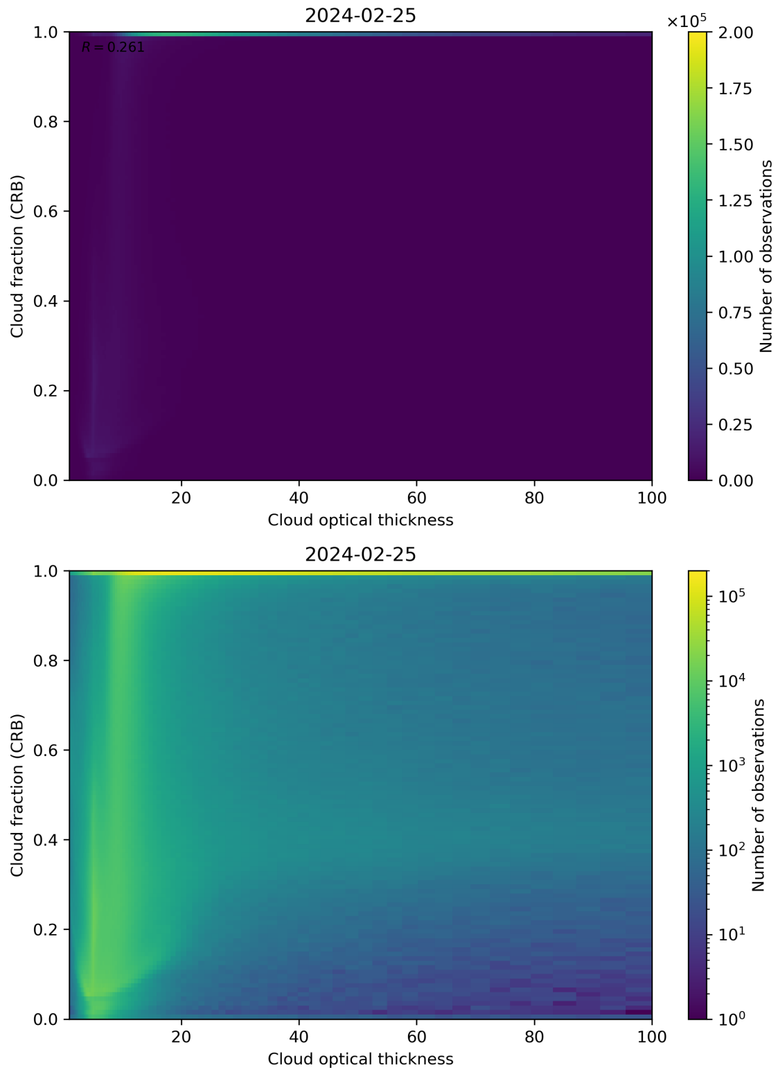
Figure 84: Scatter density plot of “Cloud optical thickness” against “Cloud fraction (CRB)” for 2024-02-24 to 2024-02-26.
