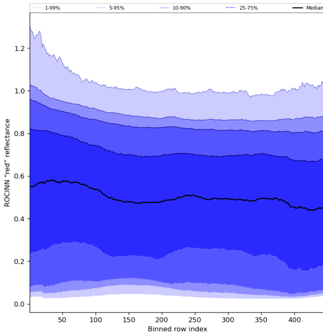
Figure 69: Along track statistics of “ROCINN “red” reflectance” for 2024-02-24 to 2024-02-26
