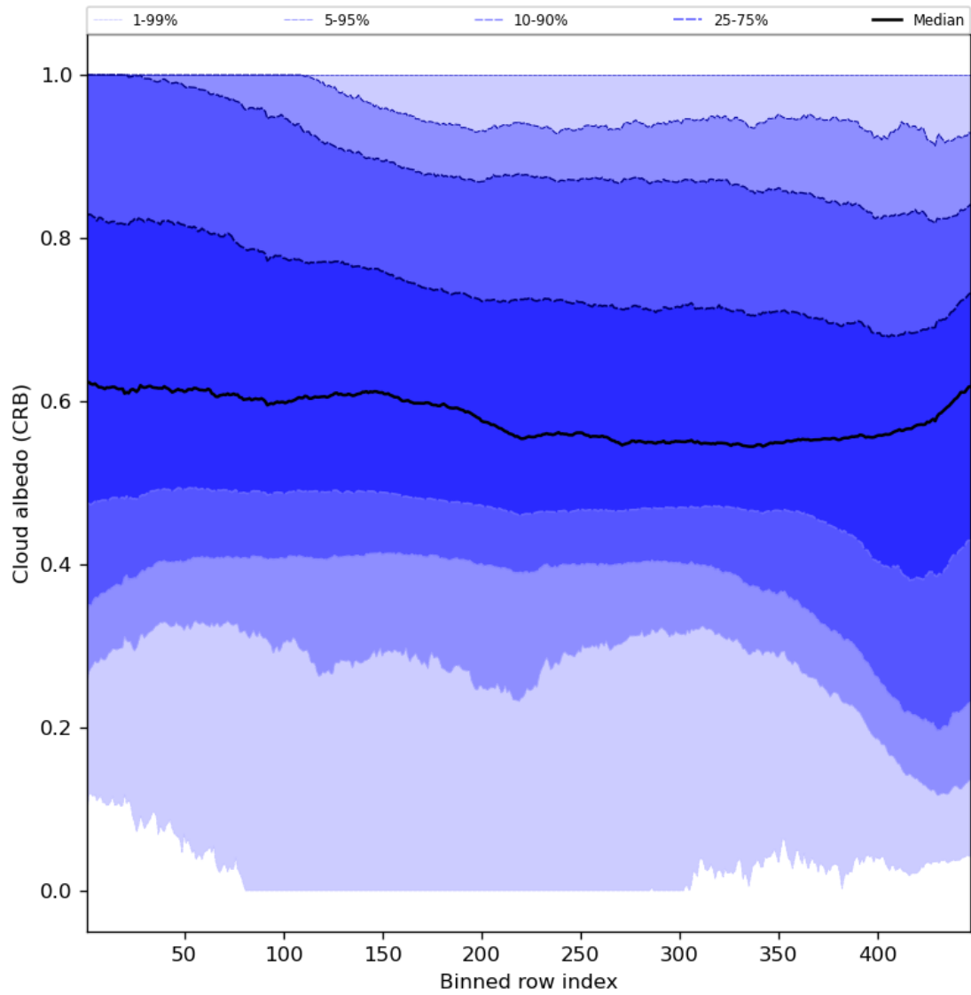
Figure 60: Along track statistics of “Cloud albedo (CRB)” for 2024-02-24 to 2024-02-26
