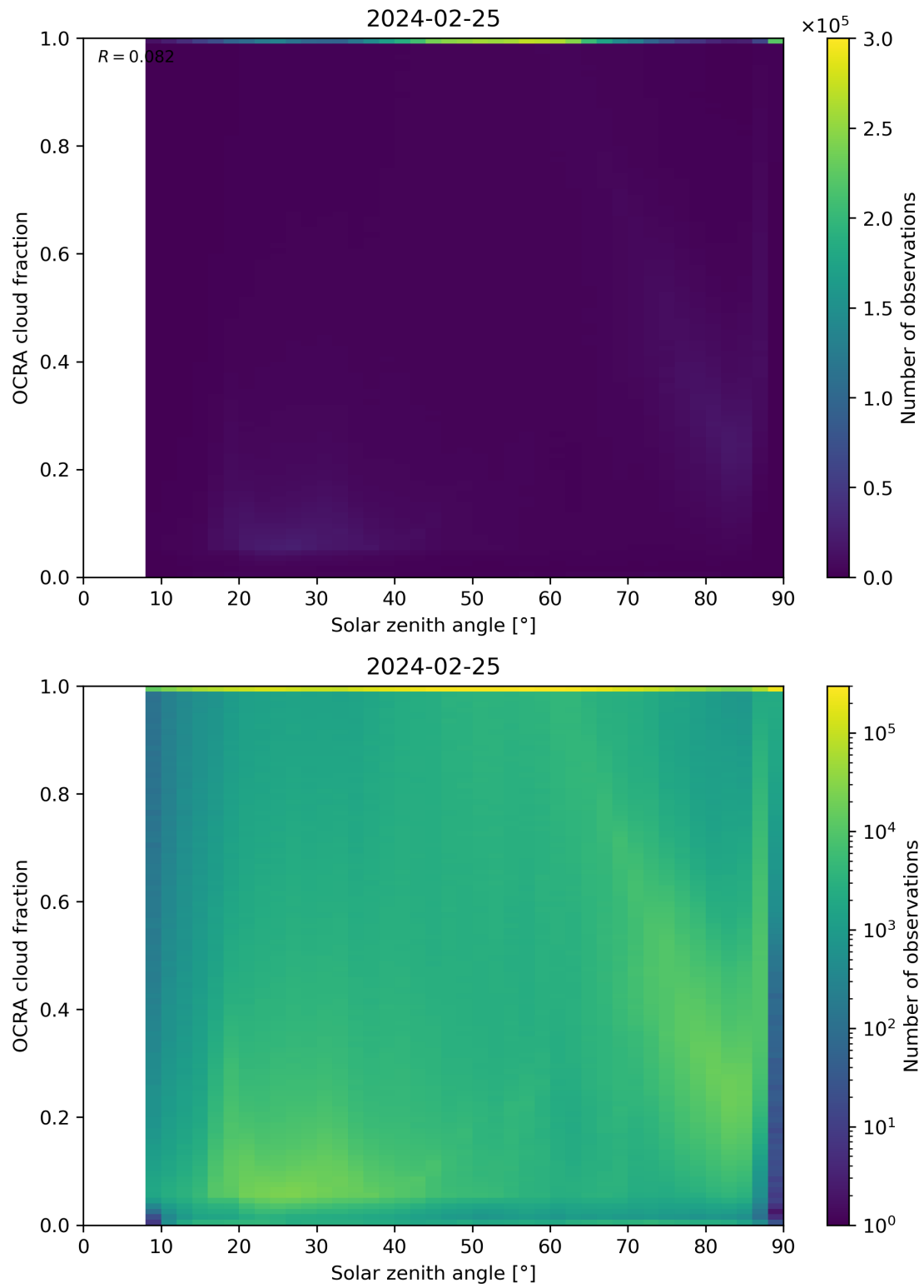
Figure 100: Scatter density plot of “Solar zenith angle” against “OCRA cloud fraction” for 2024-02-24 to 2024-02-26.
