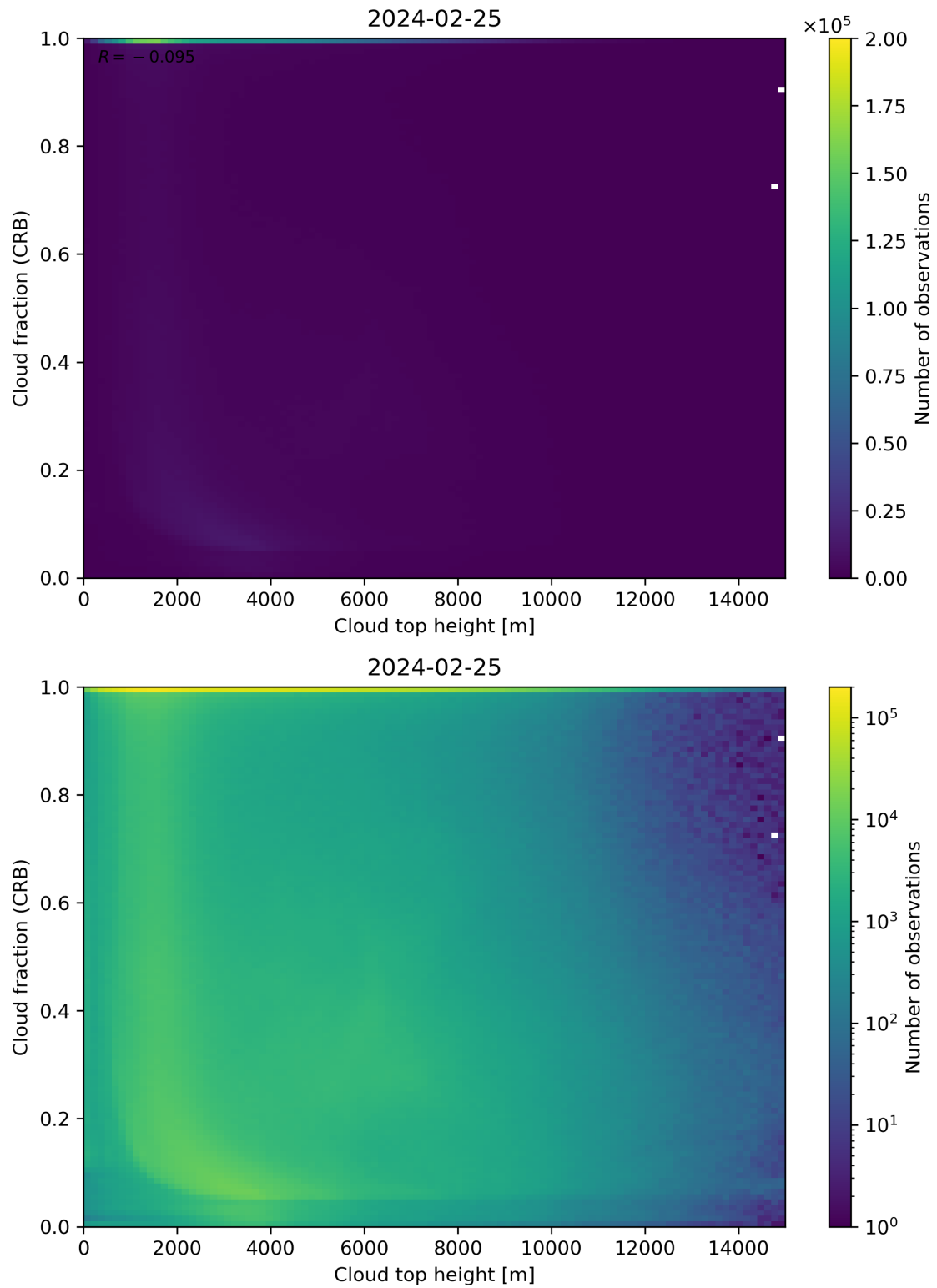
Figure 88: Scatter density plot of “Cloud top height” against “Cloud fraction (CRB)” for 2024-02-24 to 2024-02-26.
