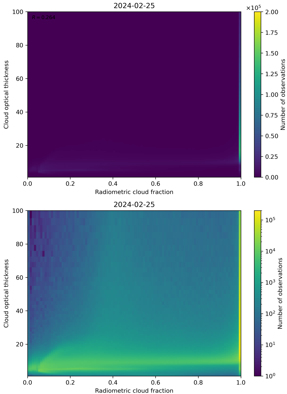
Figure 75: Scatter density plot of “Radiometric cloud fraction” against “Cloud optical thickness” for 2024-02-24 to 2024-02-26.
