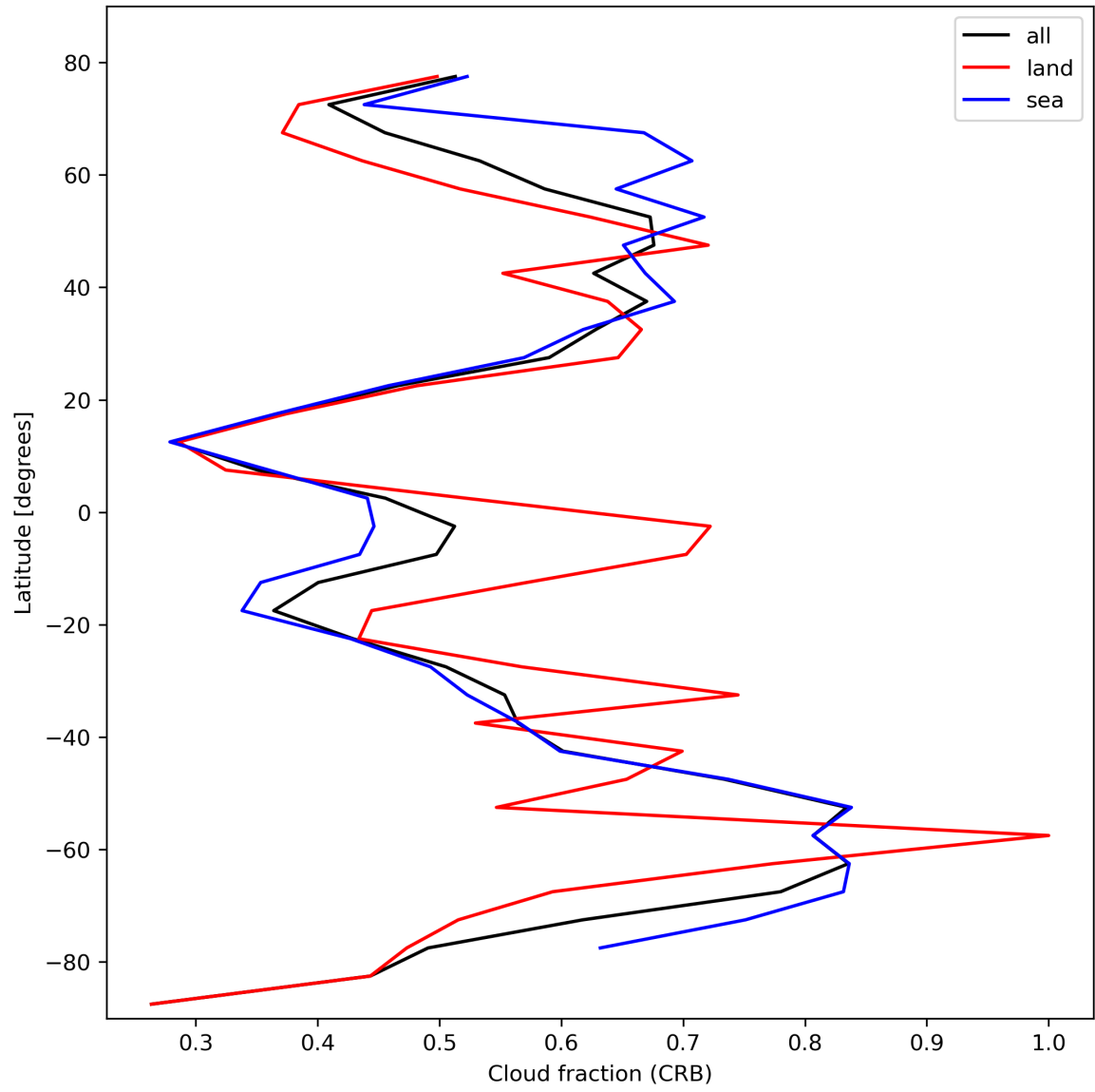
Figure 26: Zonal average of "Cloud fraction (CRB)" for 2024-02-24 to 2024-02-26.
