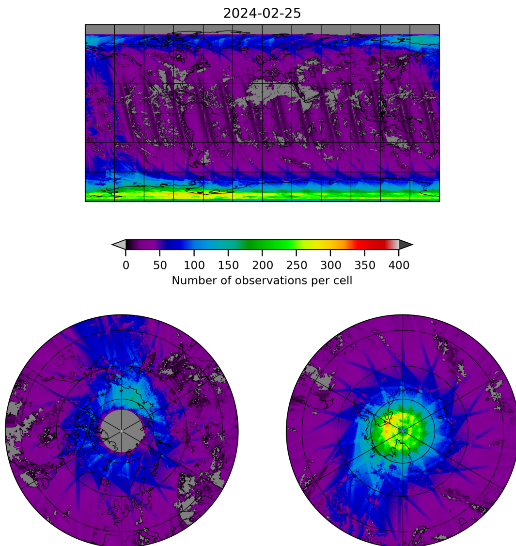
Figure 21: Map of the number of observations for 2024-02-24 to 2024-02-26
