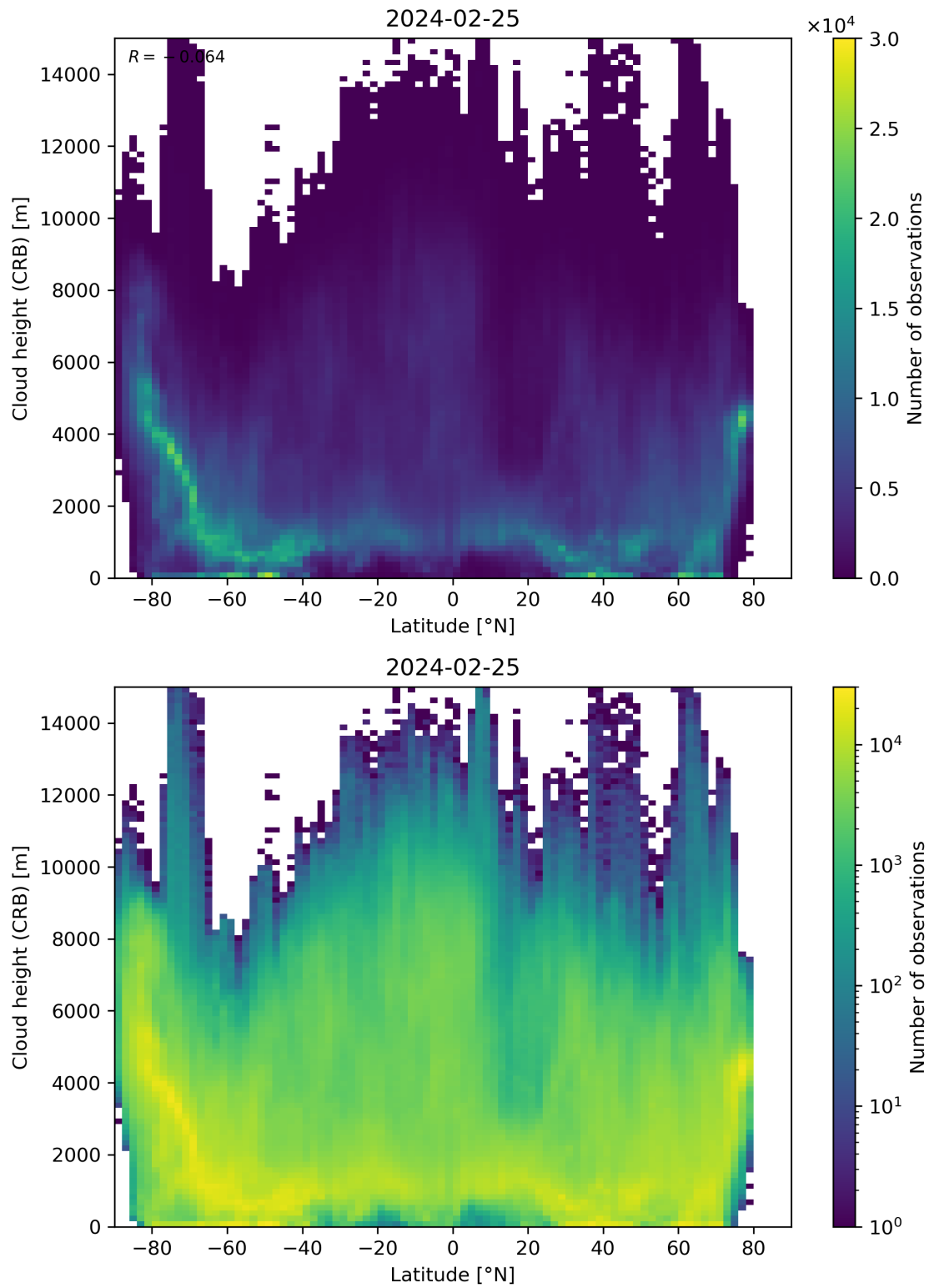
Figure 95: Scatter density plot of “Latitude” against “Cloud height (CRB)” for 2024-02-24 to 2024-02-26.
