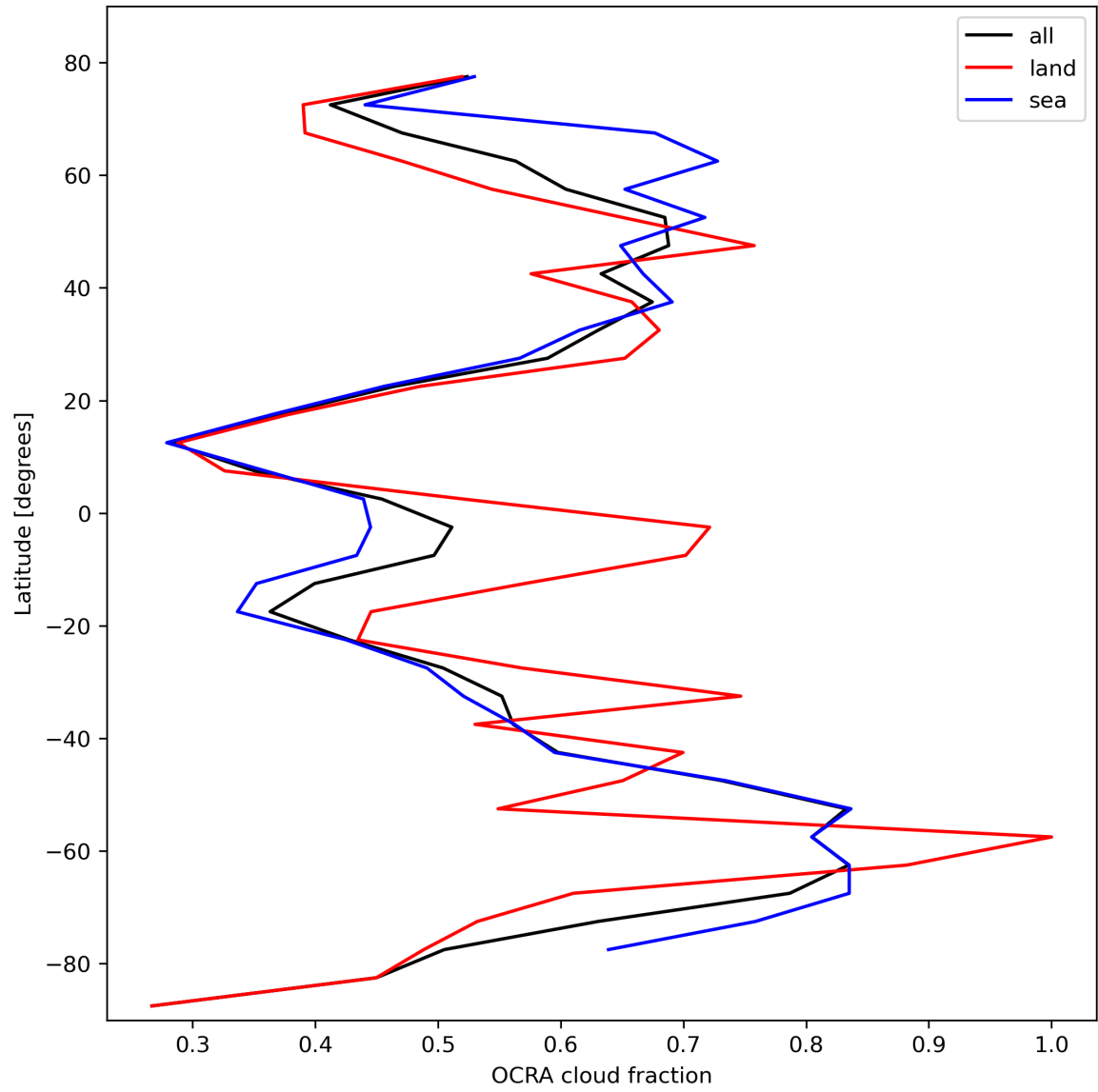
Figure 34: Zonal average of “OCRA cloud fraction” for 2024-02-24 to 2024-02-26.
