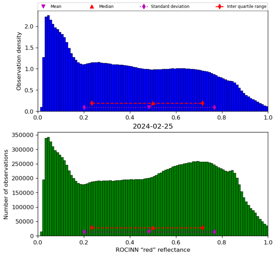
Figure 53: Histogram of “ROCINN “red” reflectance” for 2024-02-24 to 2024-02-26
