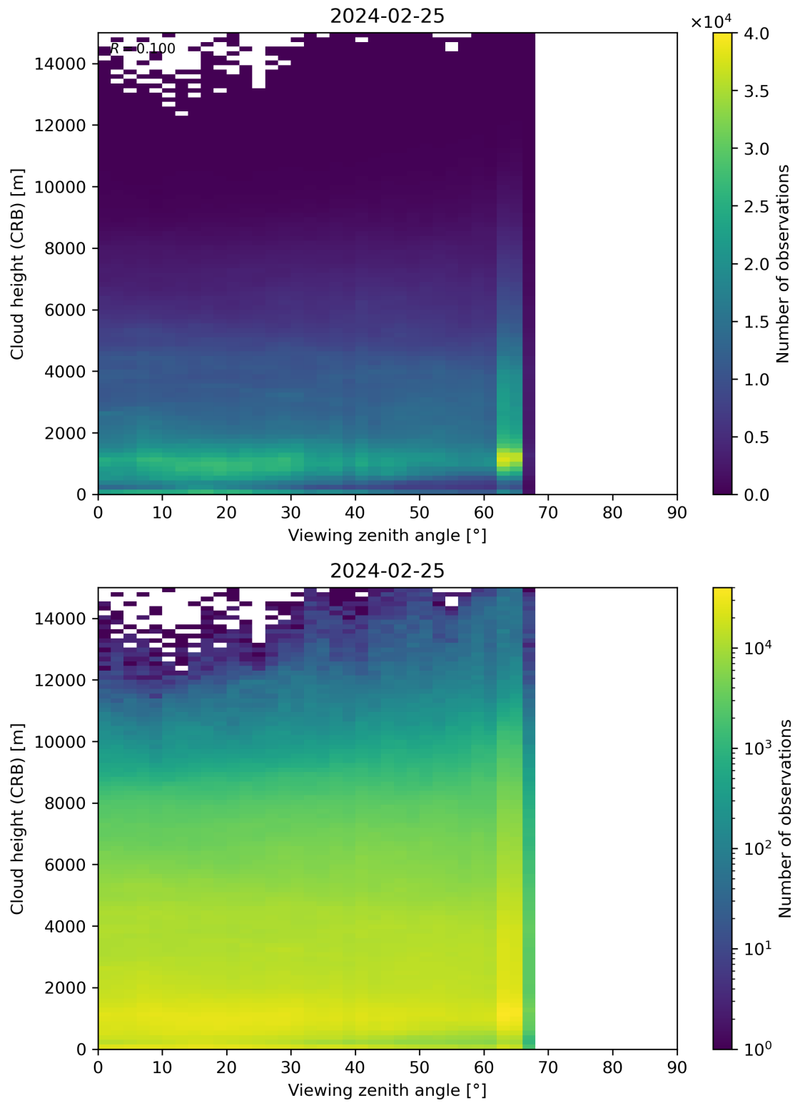
Figure 110: Scatter density plot of “Viewing zenith angle” against “Cloud height (CRB)” for 2024-02-24 to 2024-02-26.
