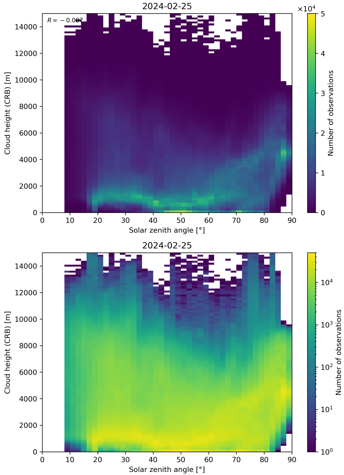
Figure 102: Scatter density plot of “Solar zenith angle” against “Cloud height (CRB)” for 2024-02-24 to 2024-02-26.
