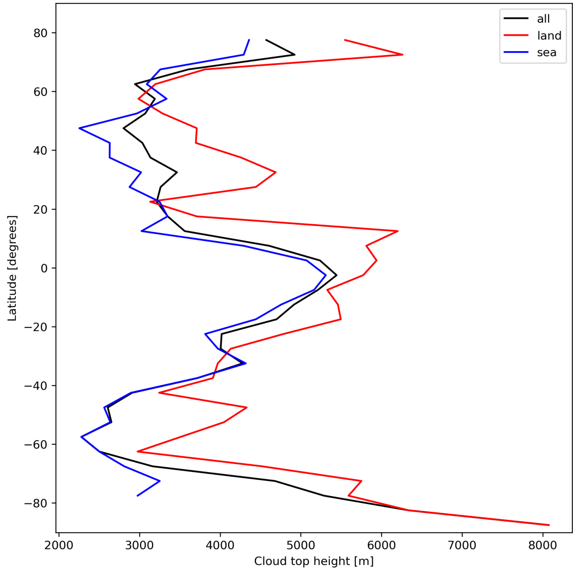
Figure 24: Zonal average of “Cloud top height” for 2024-02-24 to 2024-02-26.
