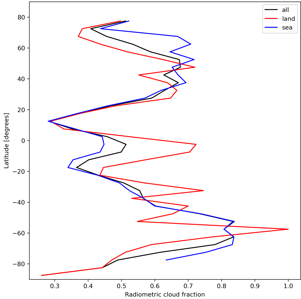
Figure 23: Zonal average of “Radiometric cloud fraction” for 2024-02-24 to 2024-02-26.
