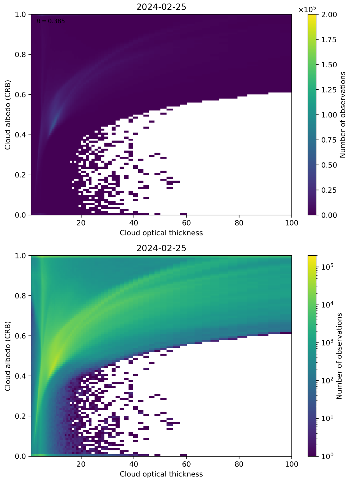
Figure 82: Scatter density plot of “Cloud optical thickness” against “Cloud albedo (CRB)” for 2024-02-24 to 2024-02-26.
