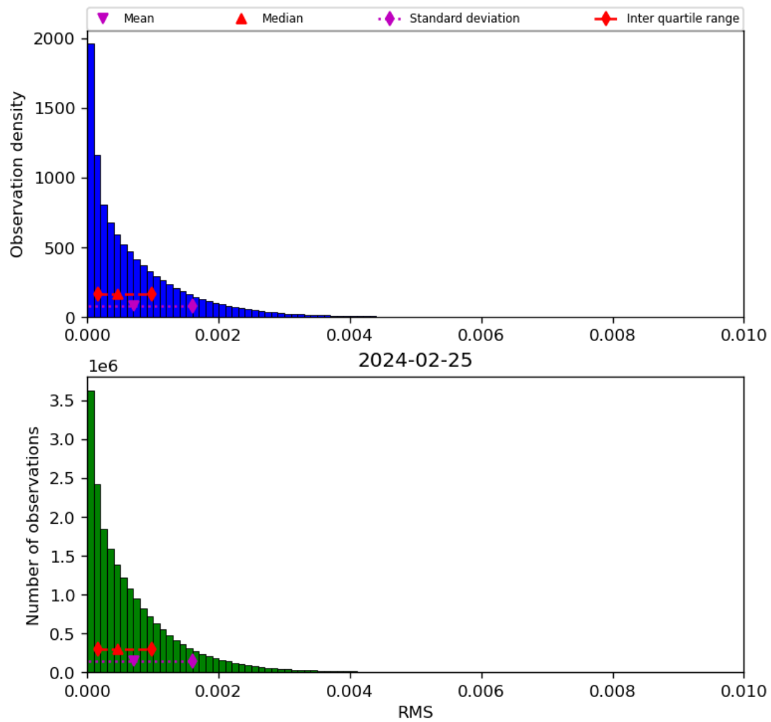
Figure 47: Histogram of “RMS” for 2024-02-24 to 2024-02-26
