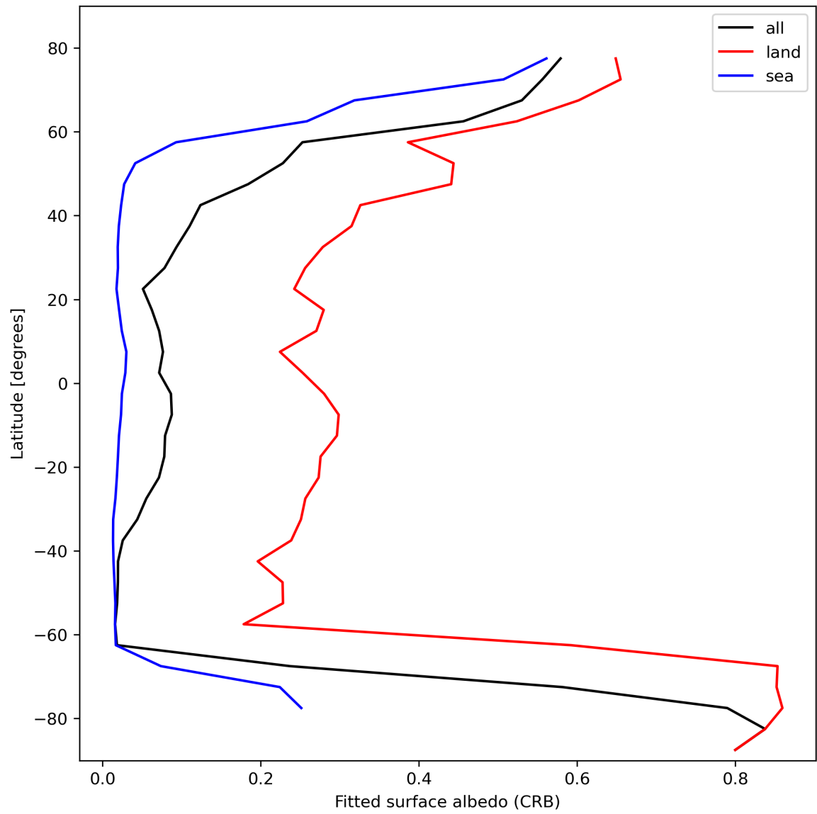
Figure 30: Zonal average of “Fitted surface albedo (CRB)” for 2024-02-24 to 2024-02-26.
