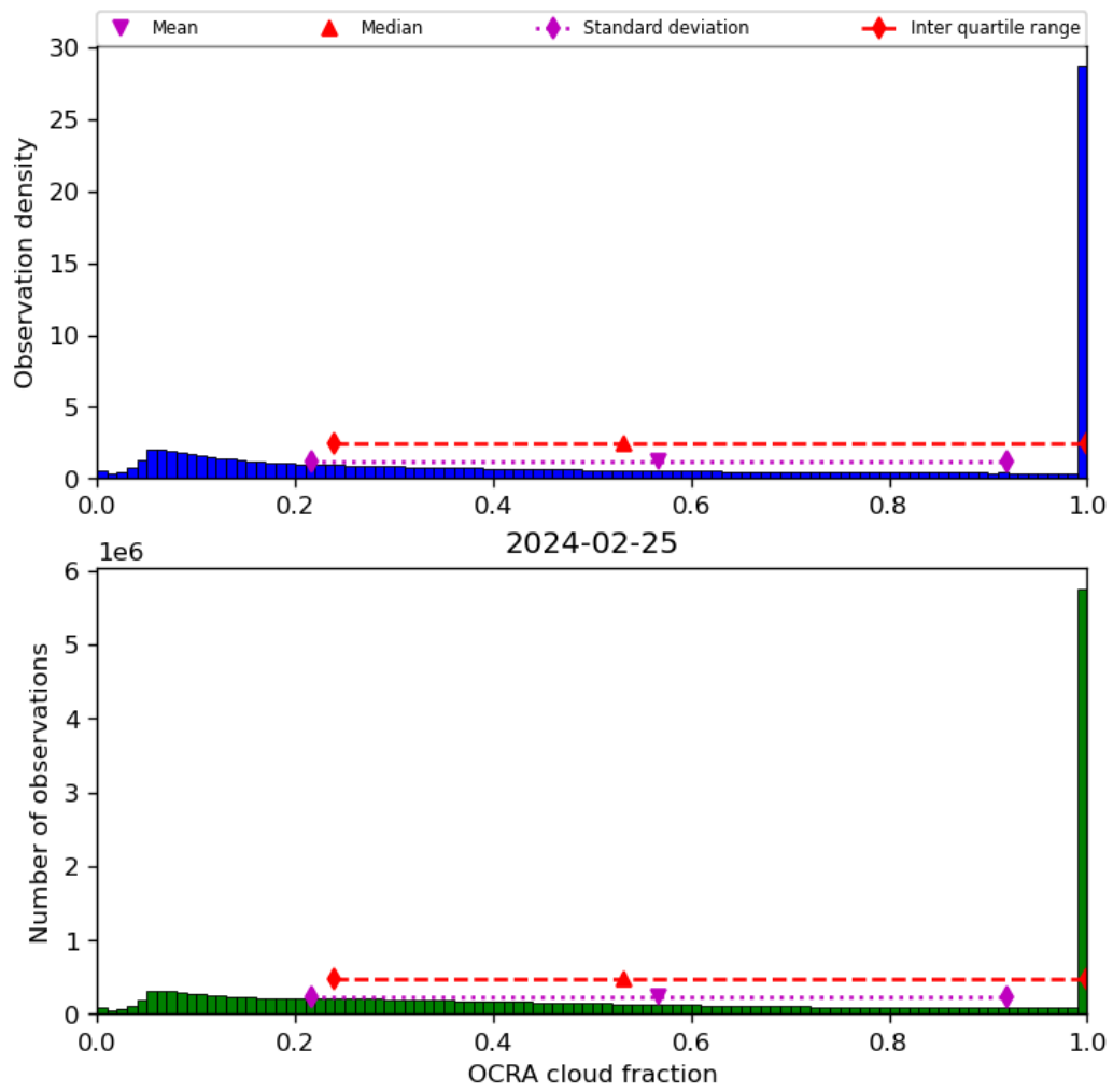
Figure 50: Histogram of “OCRA cloud fraction” for 2024-02-24 to 2024-02-26
