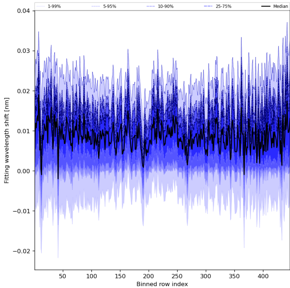
Figure 65: Along track statistics of “Fitting wavelength shift” for 2024-02-24 to 2024-02-26
