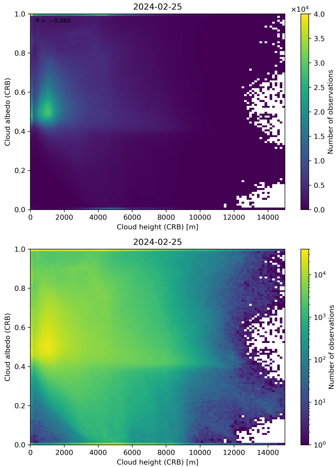
Figure 80: Scatter density plot of “Cloud height (CRB)” against “Cloud albedo (CRB)” for 2024-02-24 to 2024-02-26.
