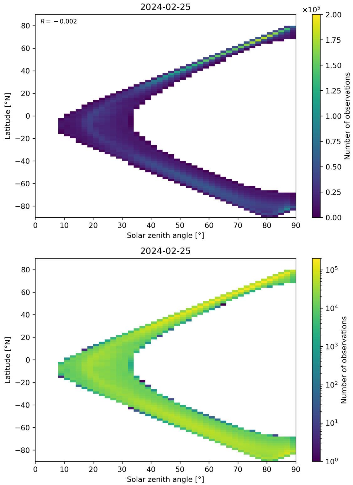
Figure 105: Scatter density plot of “Solar zenith angle” against “Latitude” for 2024-02-24 to 2024-02-26.
