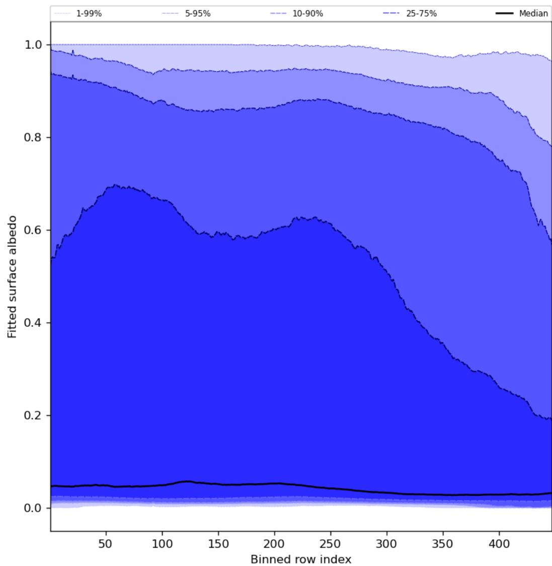
Figure 61: Along track statistics of “Fitted surface albedo” for 2024-02-24 to 2024-02-26
