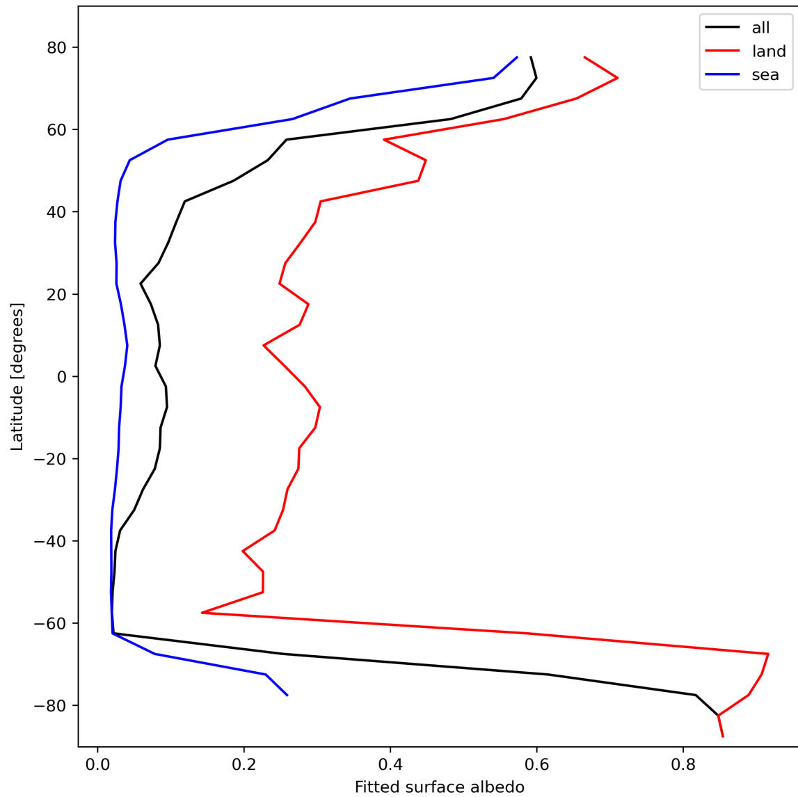
Figure 29: Zonal average of “Fitted surface albedo” for 2024-02-24 to 2024-02-26.
