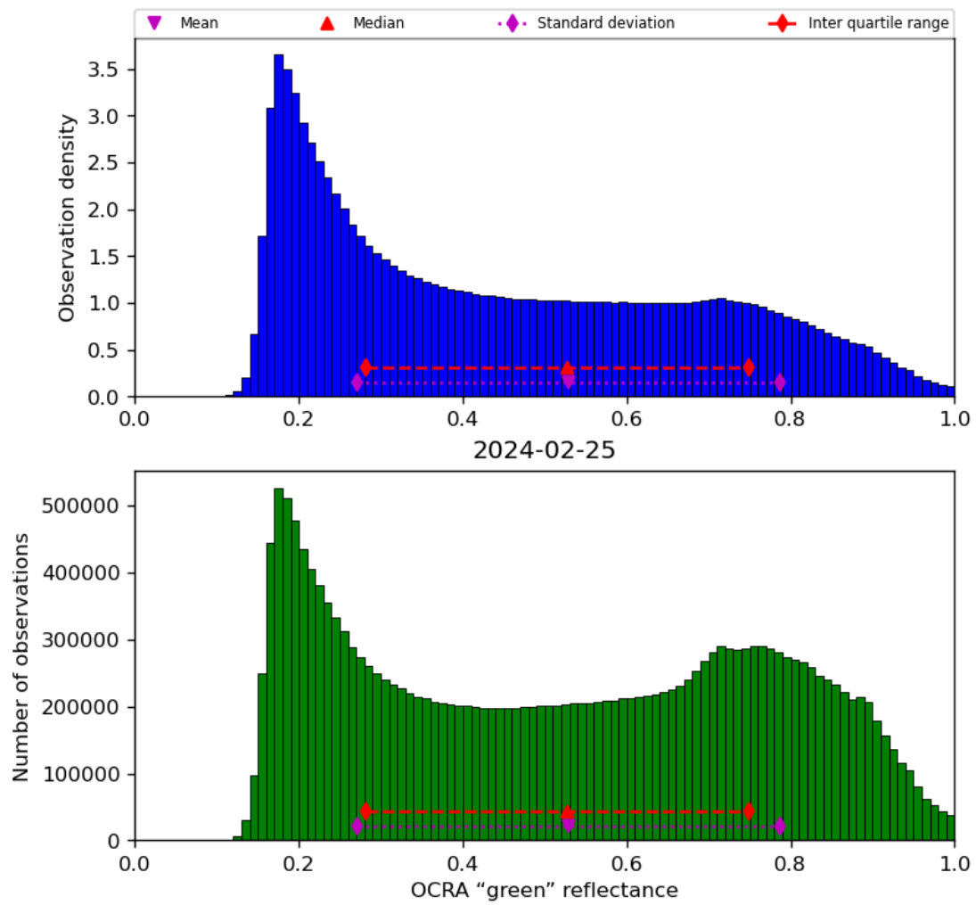
Figure 52: Histogram of “OCRA “green” reflectance” for 2024-02-24 to 2024-02-26
