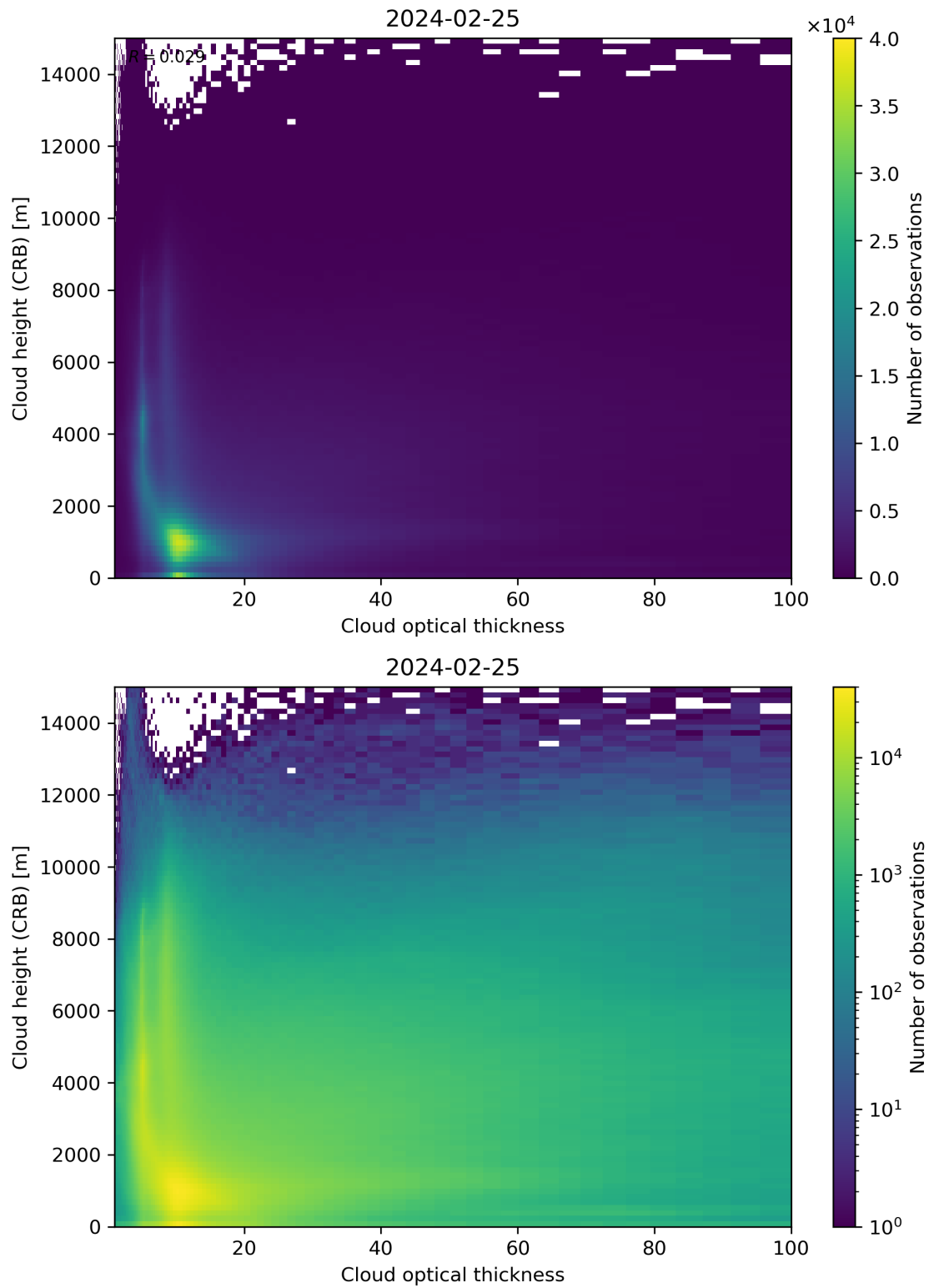
Figure 85: Scatter density plot of “Cloud optical thickness” against “Cloud height (CRB)” for 2024-02-24 to 2024-02-26.
