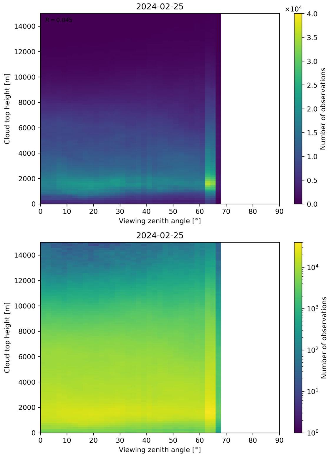
Figure 112: Scatter density plot of “Viewing zenith angle” against “Cloud top height” for 2024-02-24 to 2024-02-26.
