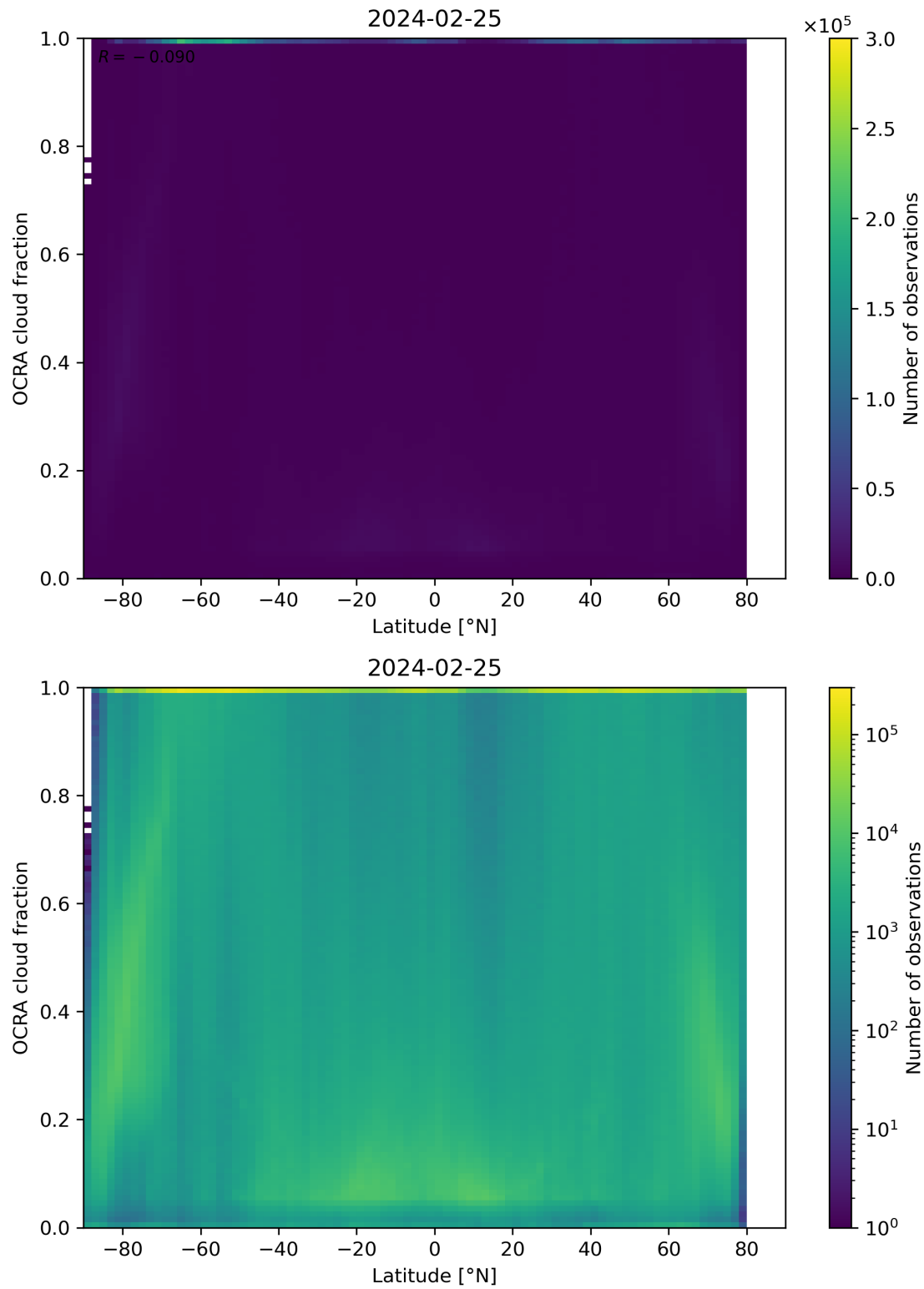
Figure 93: Scatter density plot of “Latitude” against “OCRA cloud fraction” for 2024-02-24 to 2024-02-26.
