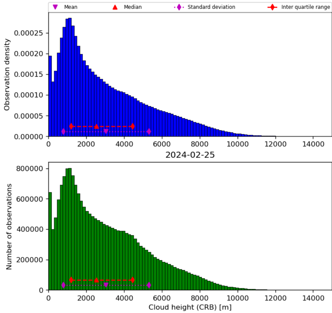
Figure 43: Histogram of “Cloud height (CRB)” for 2024-02-24 to 2024-02-26
