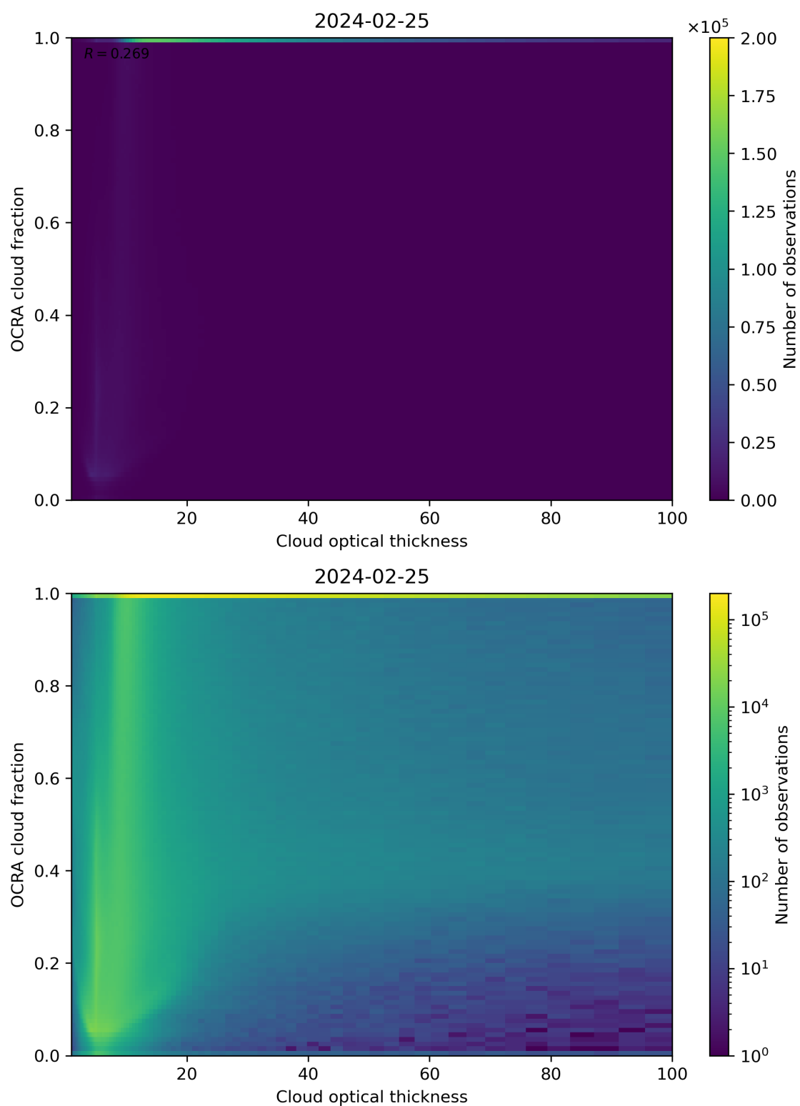
Figure 83: Scatter density plot of “Cloud optical thickness” against “OCRA cloud fraction” for 2024-02-24 to 2024-02-26.
