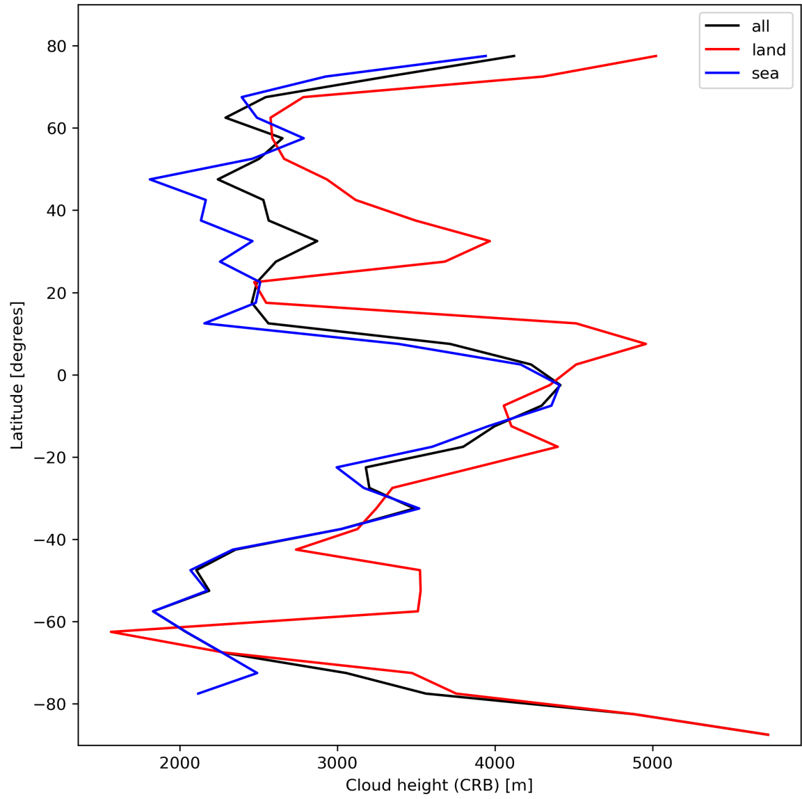
Figure 27: Zonal average of “Cloud height (CRB)” for 2024-02-24 to 2024-02-26.
