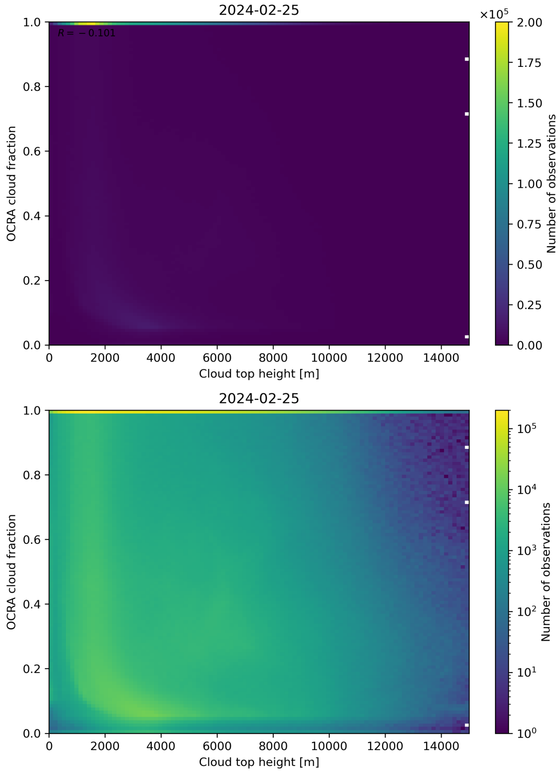
Figure 87: Scatter density plot of “Cloud top height” against “OCRA cloud fraction” for 2024-02-24 to 2024-02-26.
