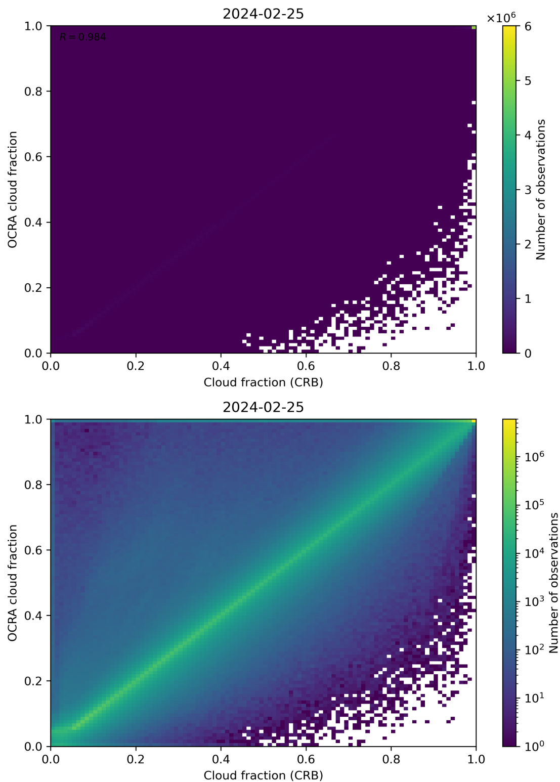
Figure 78: Scatter density plot of “Cloud fraction (CRB)” against “OCRA cloud fraction” for 2024-02-24 to 2024-02-26.
