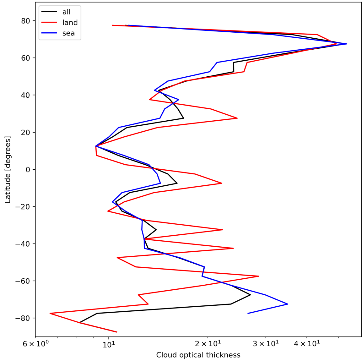
Figure 25: Zonal average of “Cloud optical thickness” for 2024-02-24 to 2024-02-26.
