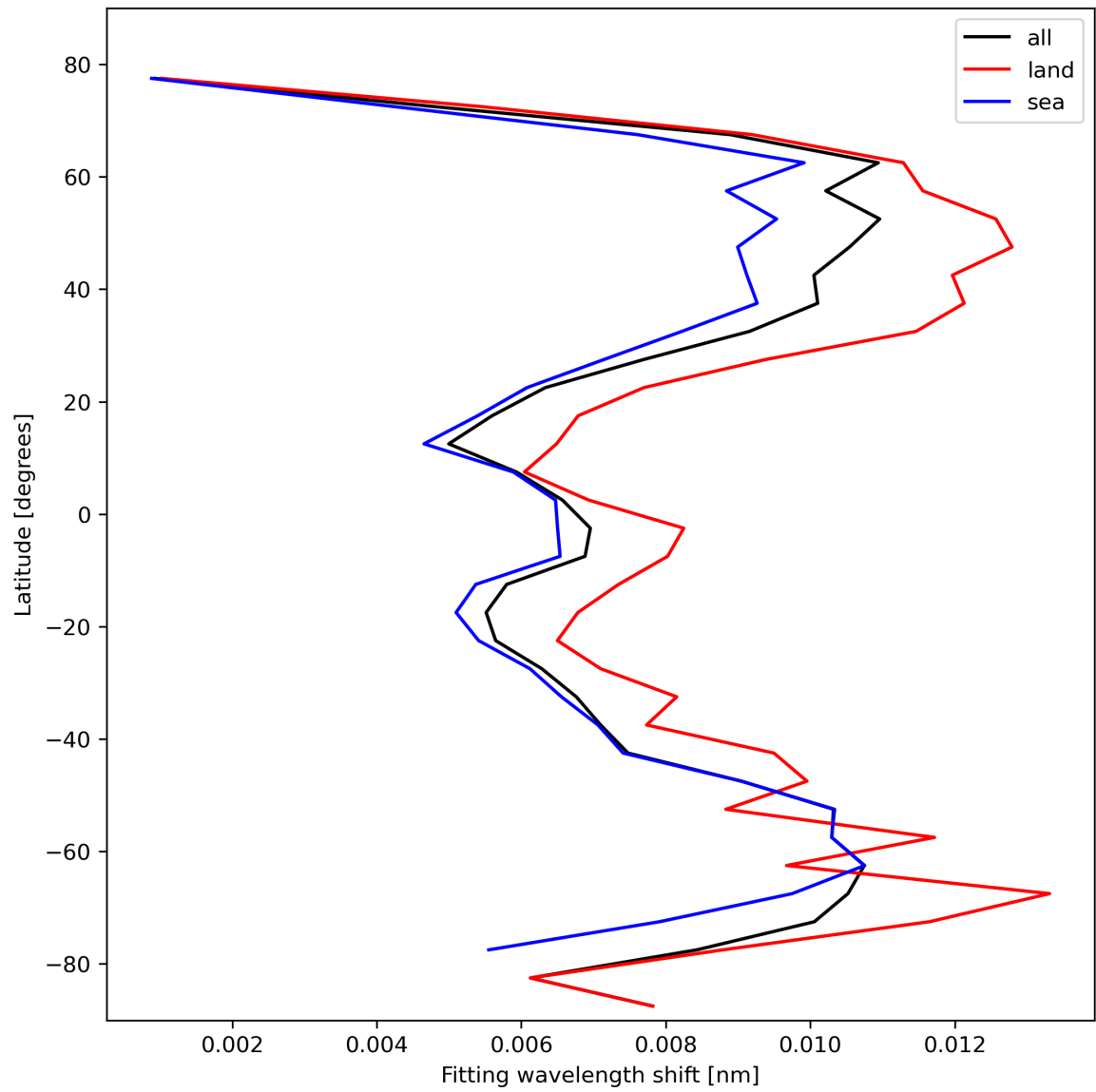
Figure 33: Zonal average of “Fitting wavelength shift” for 2024-02-24 to 2024-02-26.
