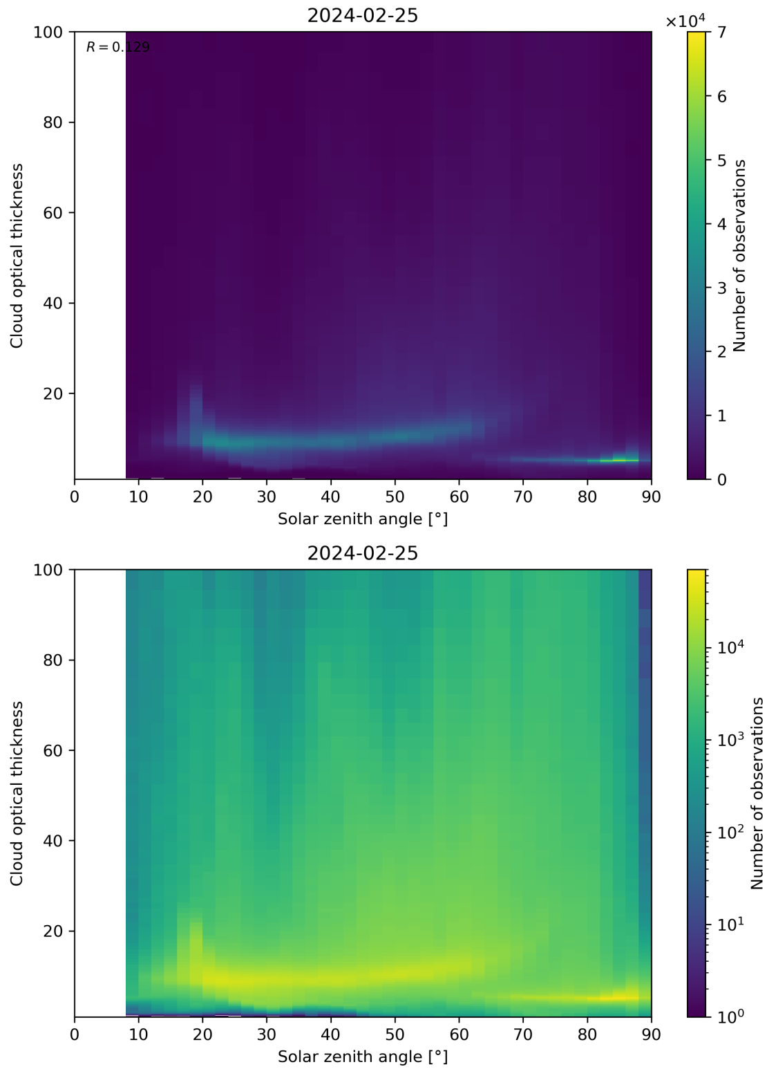
Figure 103: Scatter density plot of “Solar zenith angle” against “Cloud optical thickness” for 2024-02-24 to 2024-02-26.
