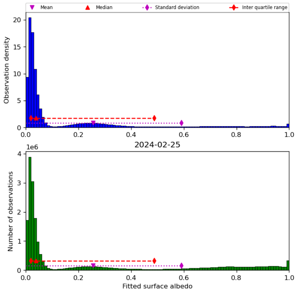
Figure 45: Histogram of “Fitted surface albedo” for 2024-02-24 to 2024-02-26
