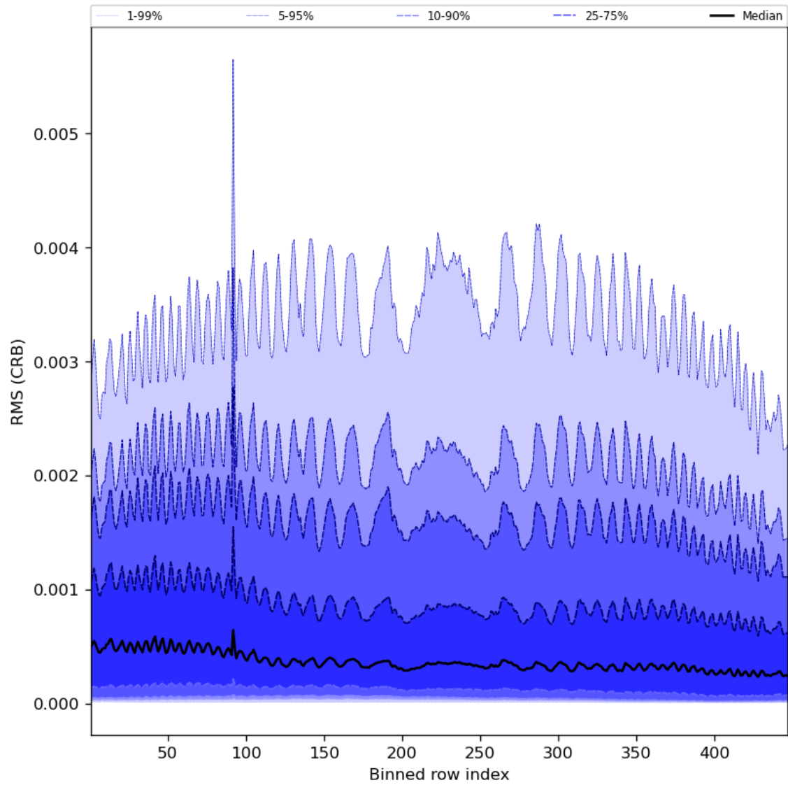
Figure 64: Along track statistics of “RMS (CRB)” for 2024-02-24 to 2024-02-26
