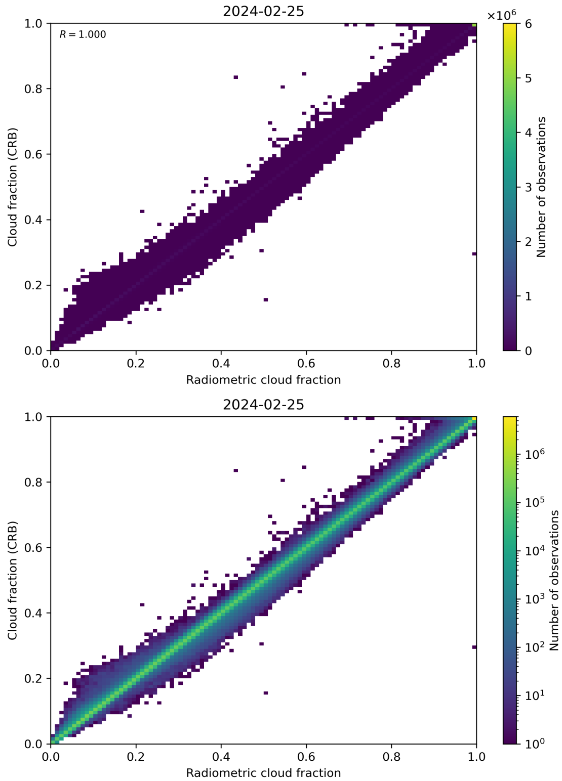
Figure 73: Scatter density plot of “Radiometric cloud fraction” against “Cloud fraction (CRB)” for 2024-02-24 to 2024-02-26.
