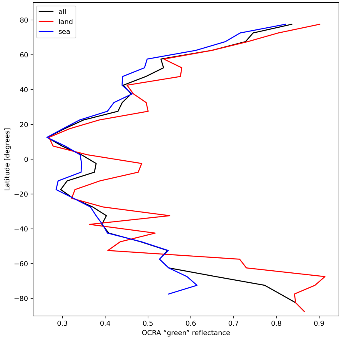
Figure 36: Zonal average of “OCRA “green” reflectance” for 2024-02-24 to 2024-02-26.
