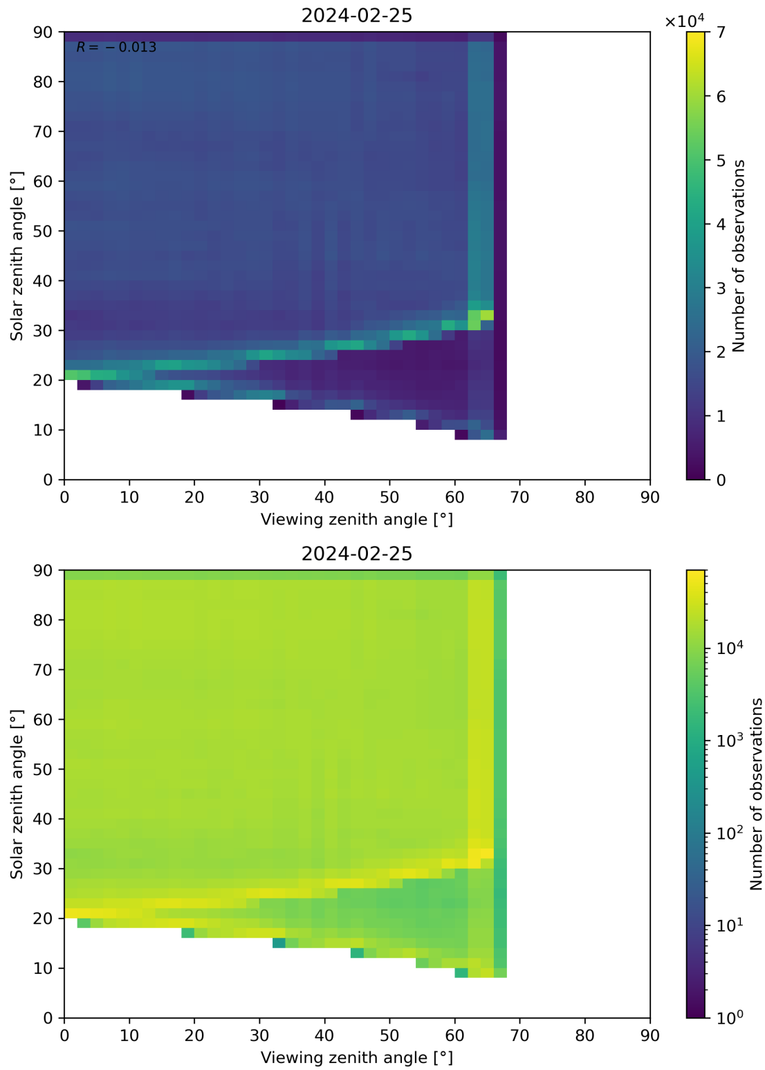
Figure 114: Scatter density plot of “Viewing zenith angle” against “Solar zenith angle” for 2024-02-24 to 2024-02-26.
