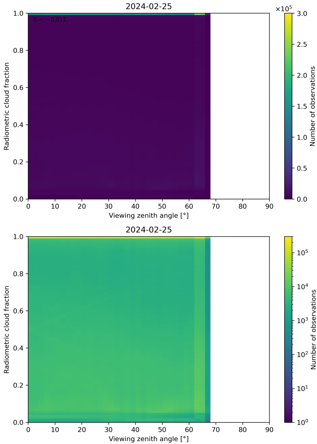
Figure 107: Scatter density plot of “Viewing zenith angle” against “Radiometric cloud fraction” for 2024-02-24 to 2024-02-26.
