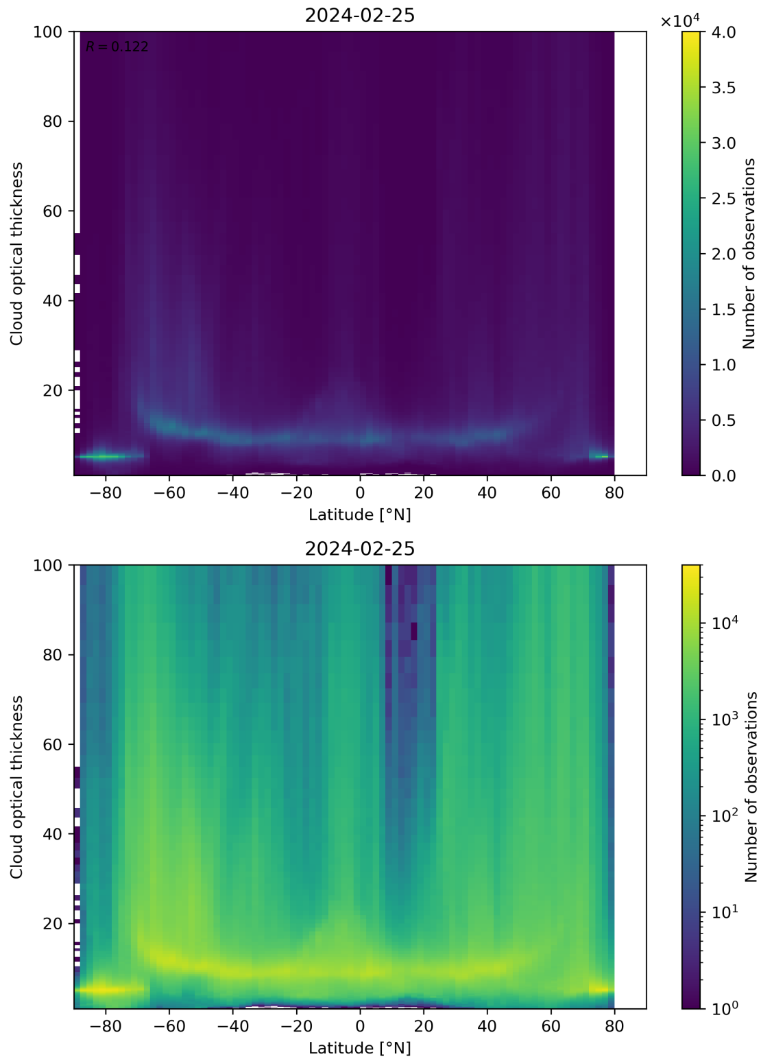
Figure 96: Scatter density plot of “Latitude” against “Cloud optical thickness” for 2024-02-24 to 2024-02-26.
