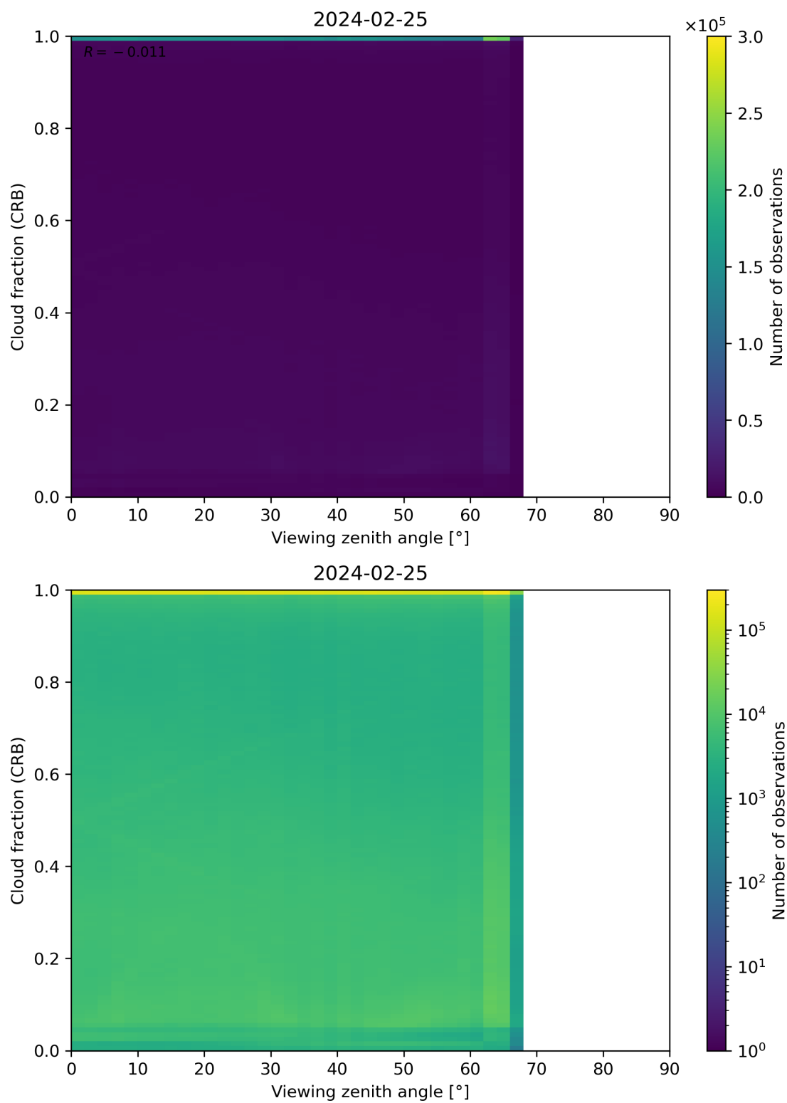
Figure 109: Scatter density plot of “Viewing zenith angle” against “Cloud fraction (CRB)” for 2024-02-24 to 2024-02-26.
