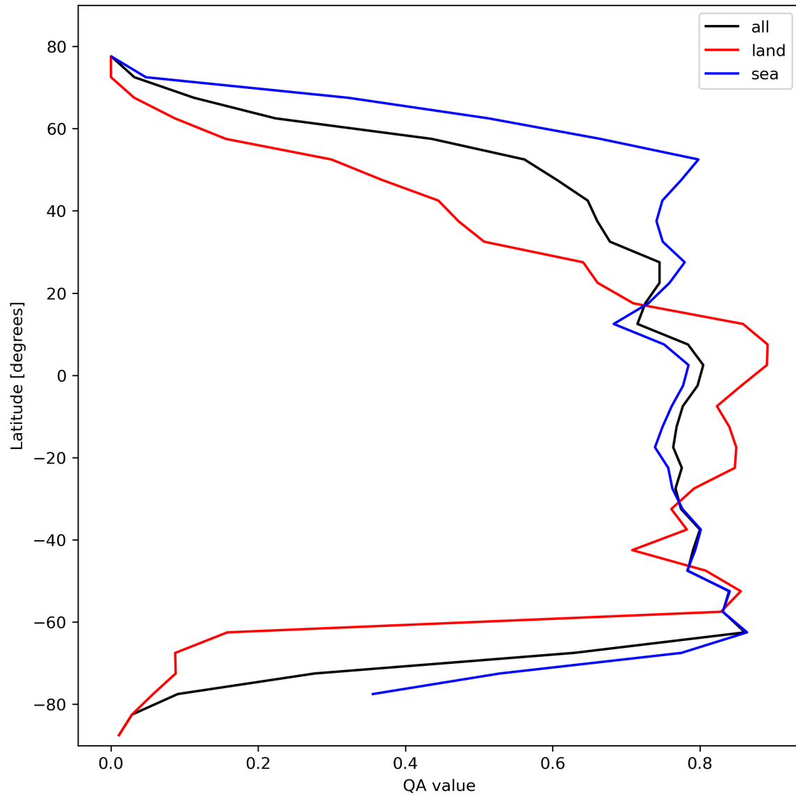
Figure 22: Zonal average of “QA value” for 2024-02-24 to 2024-02-26.
