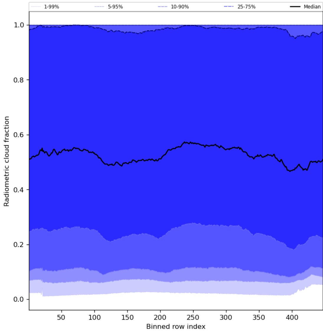
Figure 55: Along track statistics of “Radiometric cloud fraction” for 2024-02-24 to 2024-02-26
