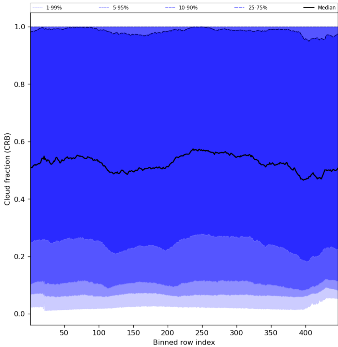
Figure 58: Along track statistics of “Cloud fraction (CRB)” for 2024-02-24 to 2024-02-26
