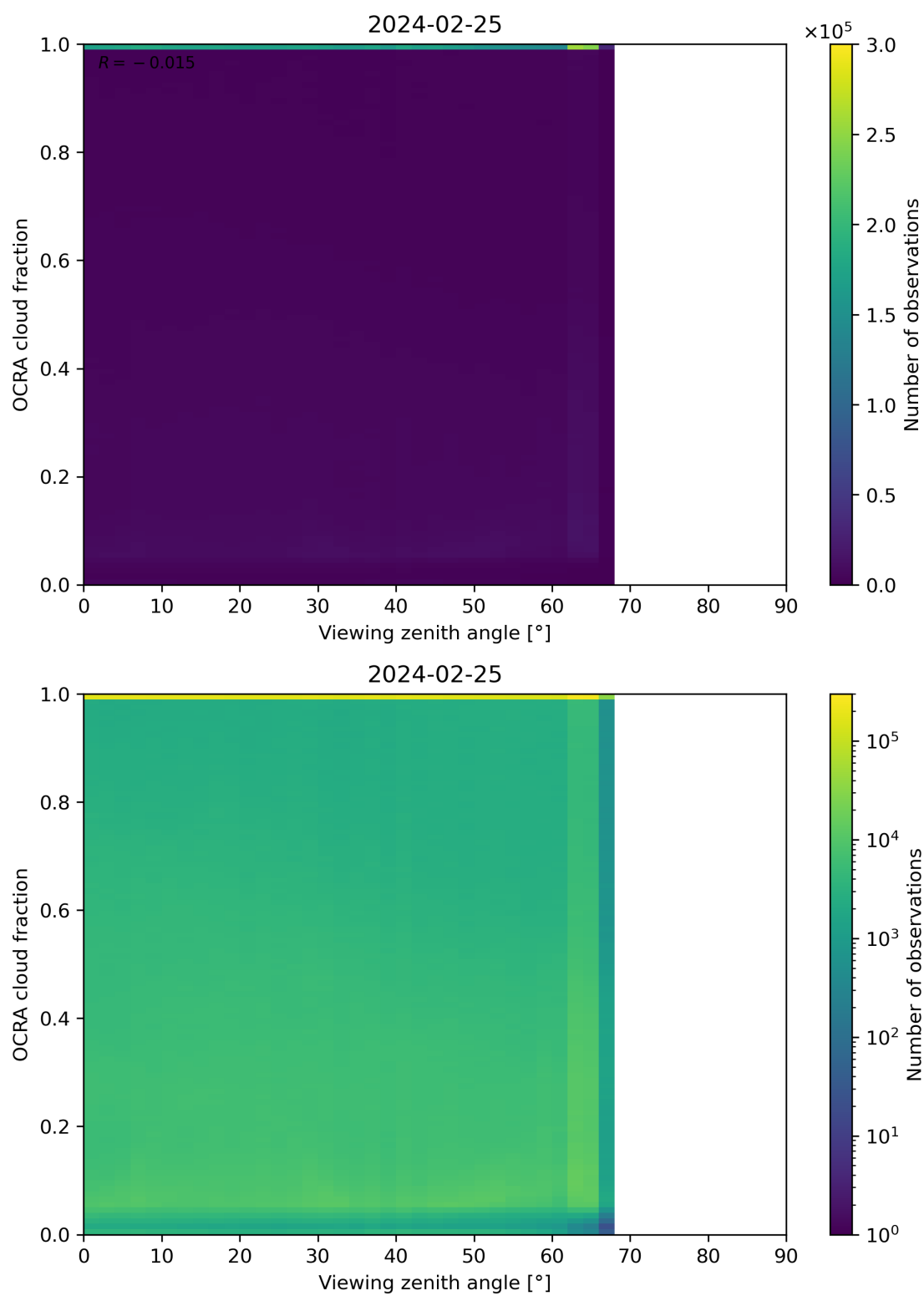
Figure 108: Scatter density plot of “Viewing zenith angle” against “OCRA cloud fraction” for 2024-02-24 to 2024-02-26.
