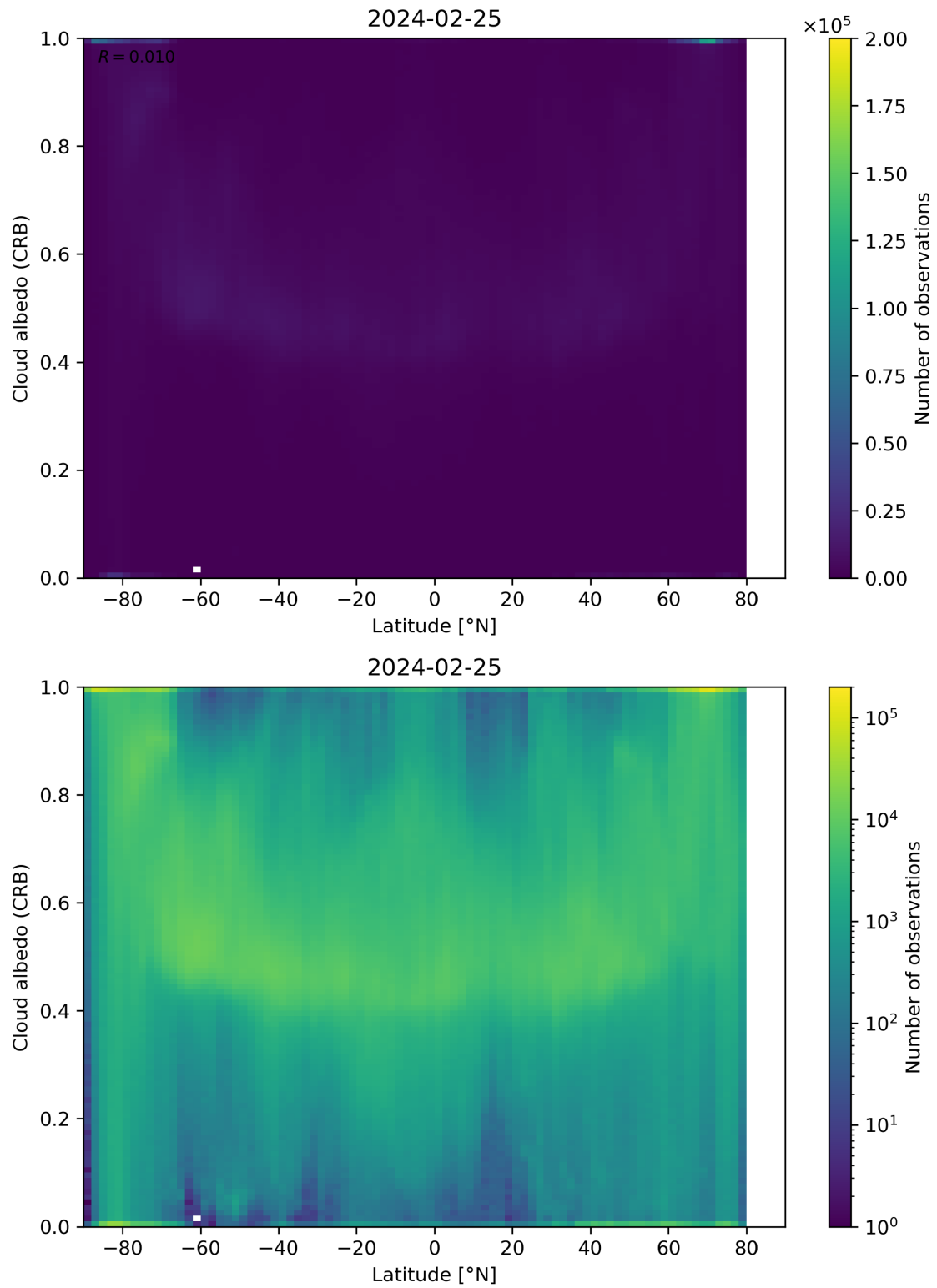
Figure 91: Scatter density plot of “Latitude” against “Cloud albedo (CRB)” for 2024-02-24 to 2024-02-26.
