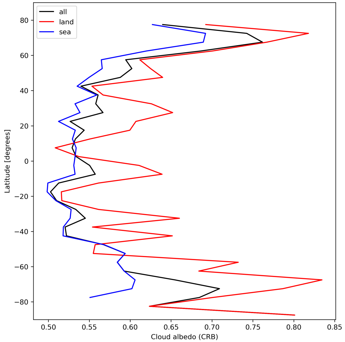
Figure 28: Zonal average of “Cloud albedo (CRB)” for 2024-02-24 to 2024-02-26.
