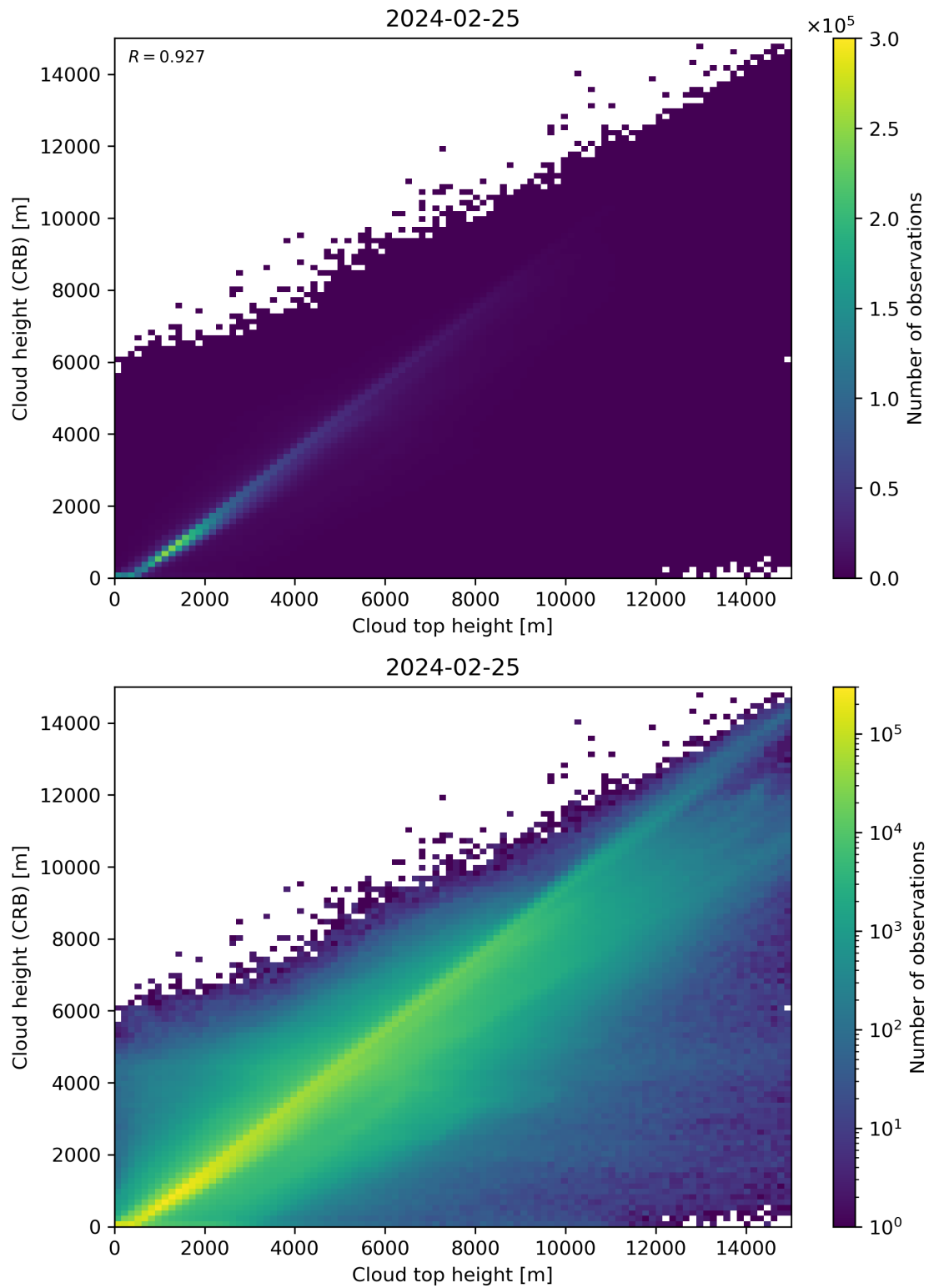
Figure 89: Scatter density plot of “Cloud top height” against “Cloud height (CRB)” for 2024-02-24 to 2024-02-26.
