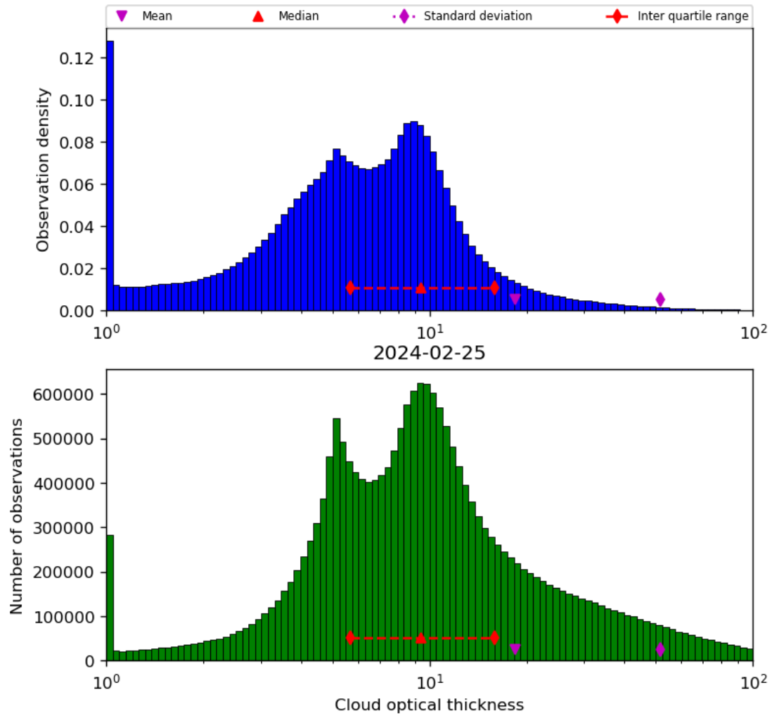
Figure 41: Histogram of “Cloud optical thickness” for 2024-02-24 to 2024-02-26
