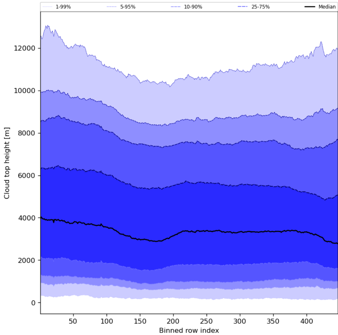
Figure 56: Along track statistics of “Cloud top height” for 2024-02-24 to 2024-02-26
