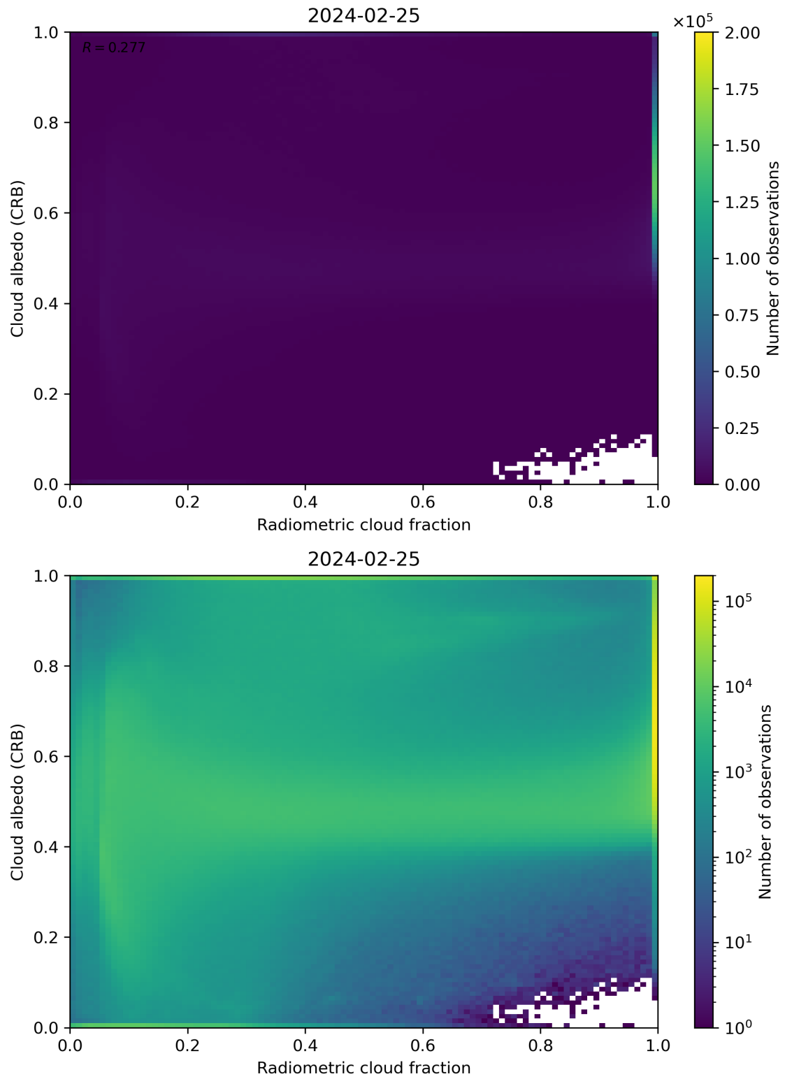
Figure 71: Scatter density plot of “Radiometric cloud fraction” against “Cloud albedo (CRB)” for 2024-02-24 to 2024-02-26.
