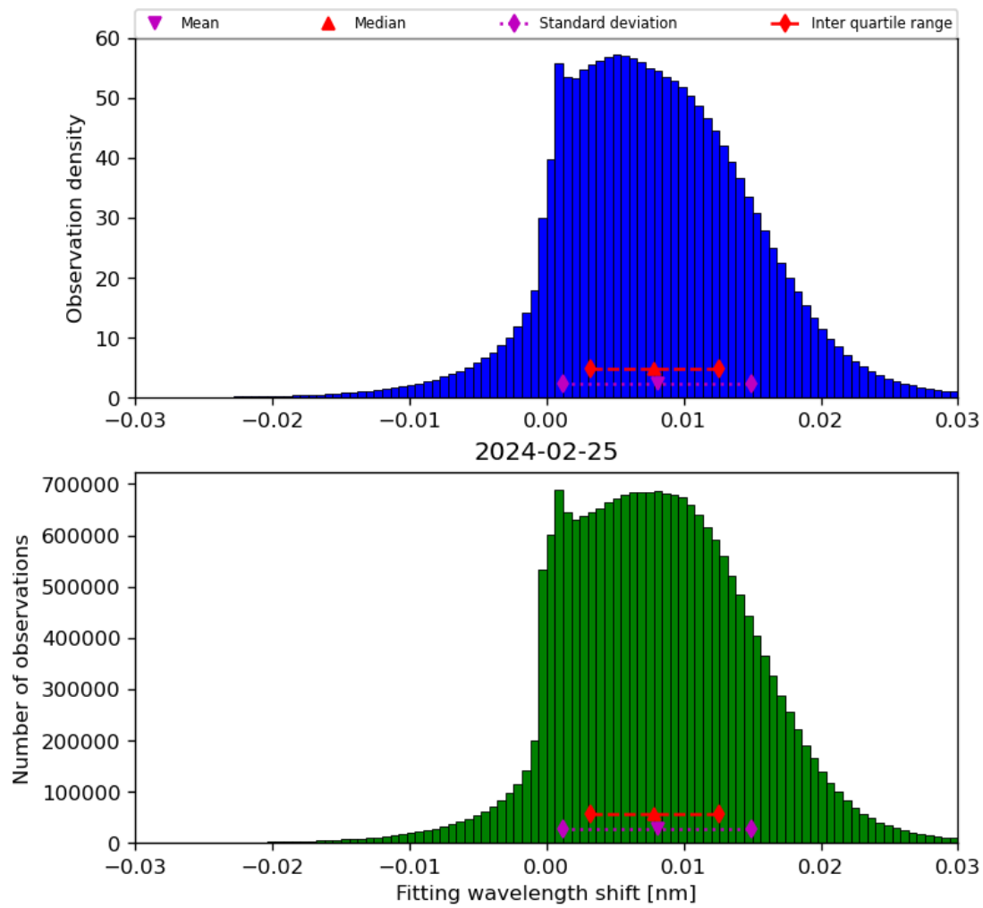
Figure 49: Histogram of “Fitting wavelength shift” for 2024-02-24 to 2024-02-26
