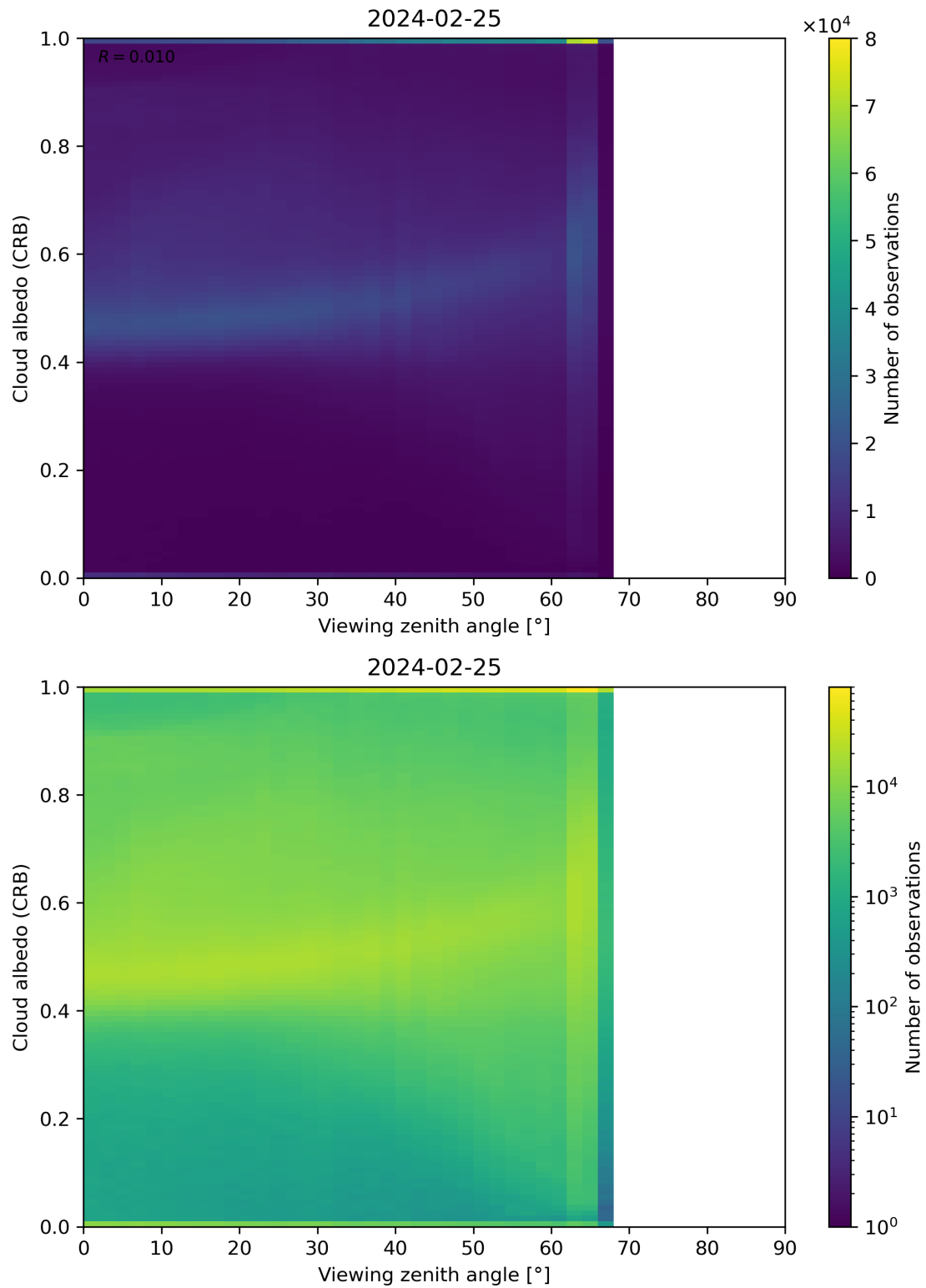
Figure 106: Scatter density plot of “Viewing zenith angle” against “Cloud albedo (CRB)” for 2024-02-24 to 2024-02-26.
