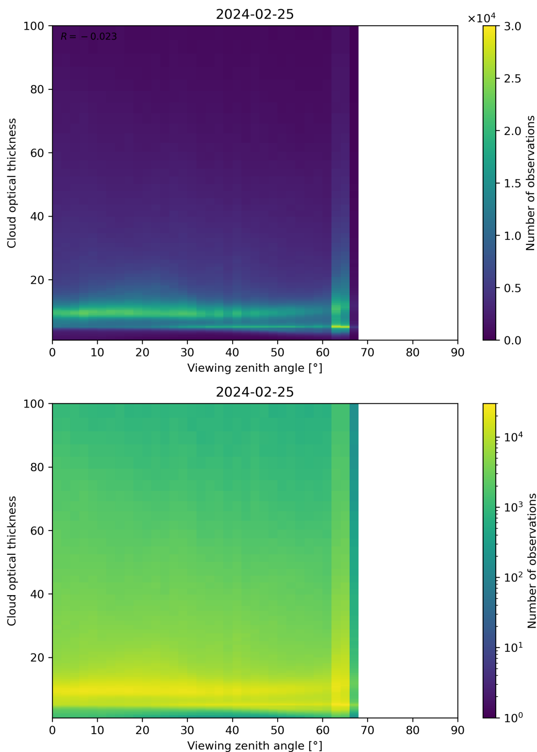
Figure 111: Scatter density plot of “Viewing zenith angle” against “Cloud optical thickness” for 2024-02-24 to 2024-02-26.
