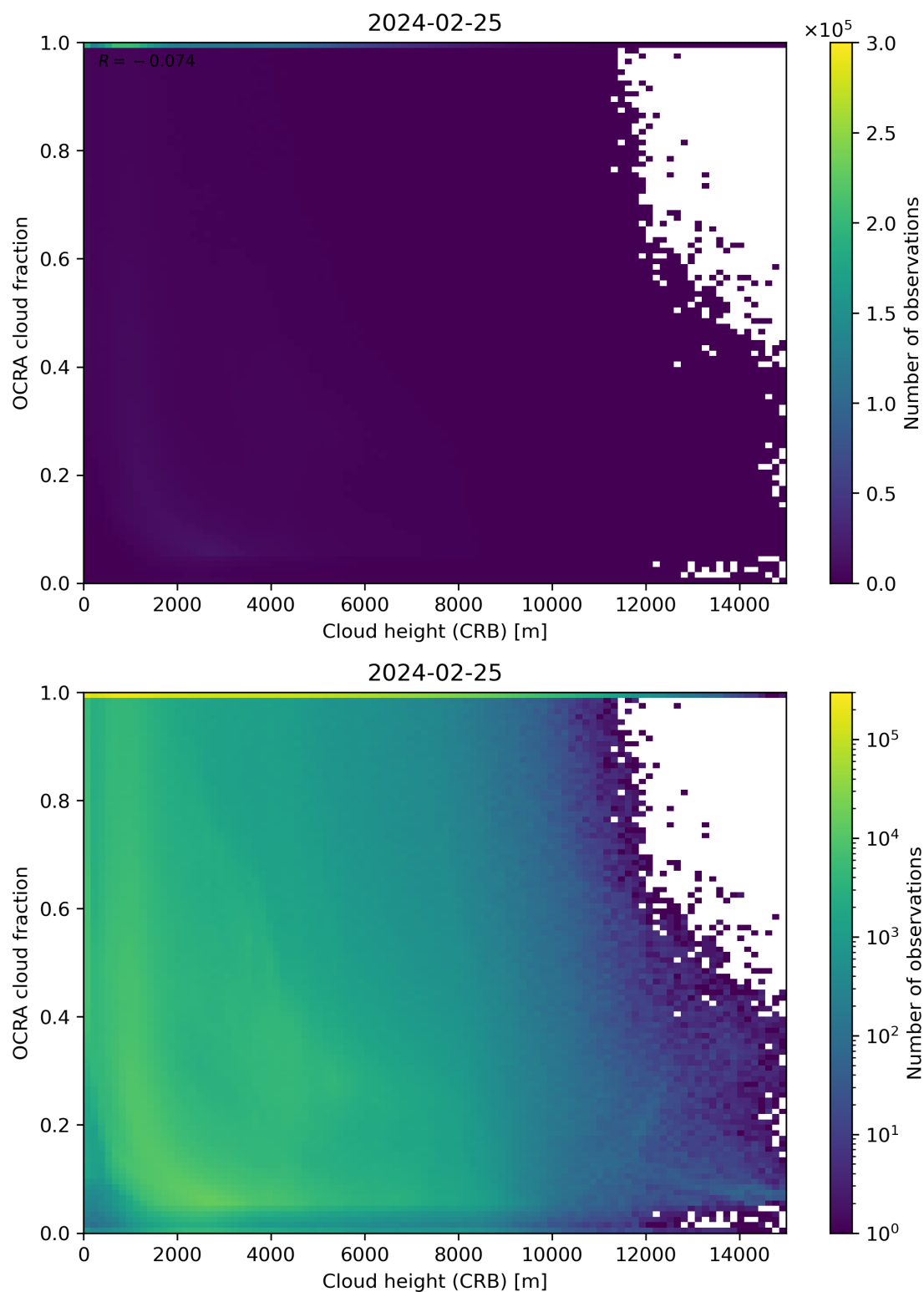
Figure 81: Scatter density plot of “Cloud height (CRB)” against “OCRA cloud fraction” for 2024-02-24 to 2024-02-26.
