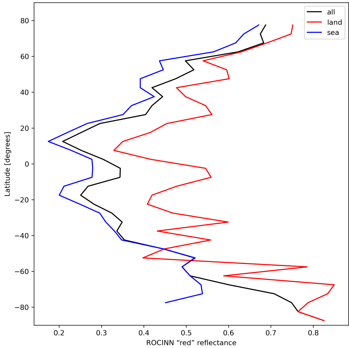
Figure 37: Zonal average of “ROCINN “red” reflectance” for 2024-02-24 to 2024-02-26.
