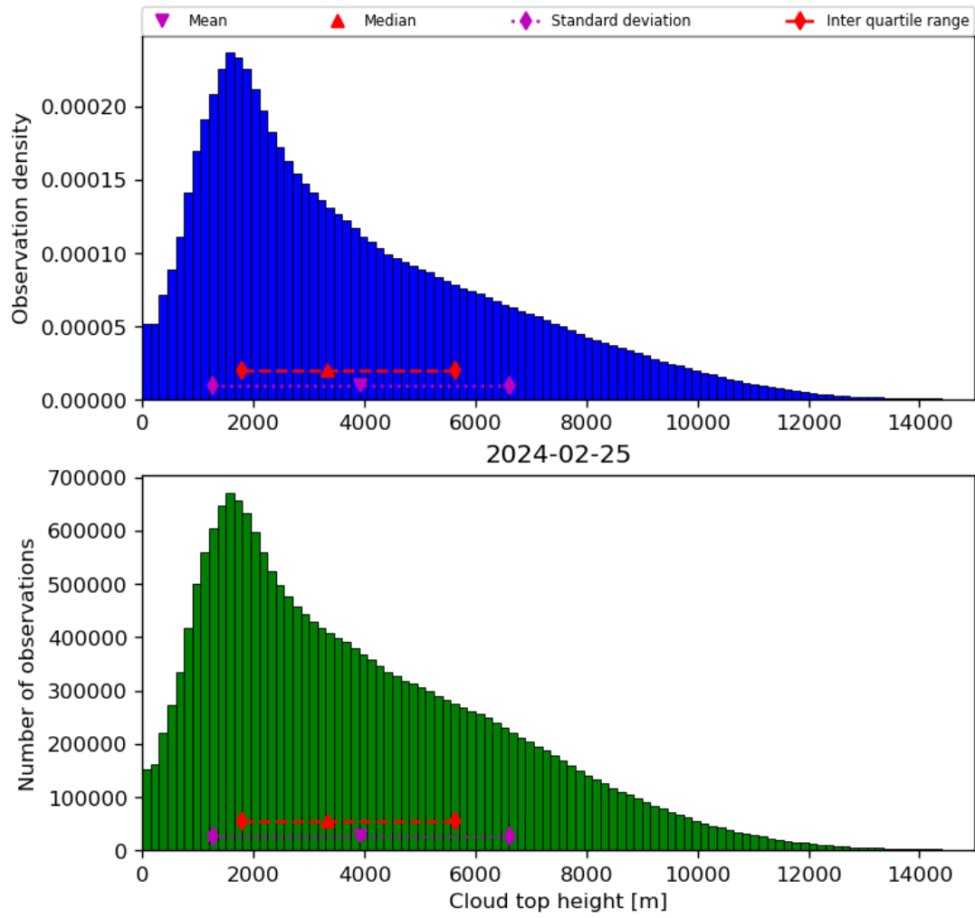
Figure 40: Histogram of “Cloud top height” for 2024-02-24 to 2024-02-26
