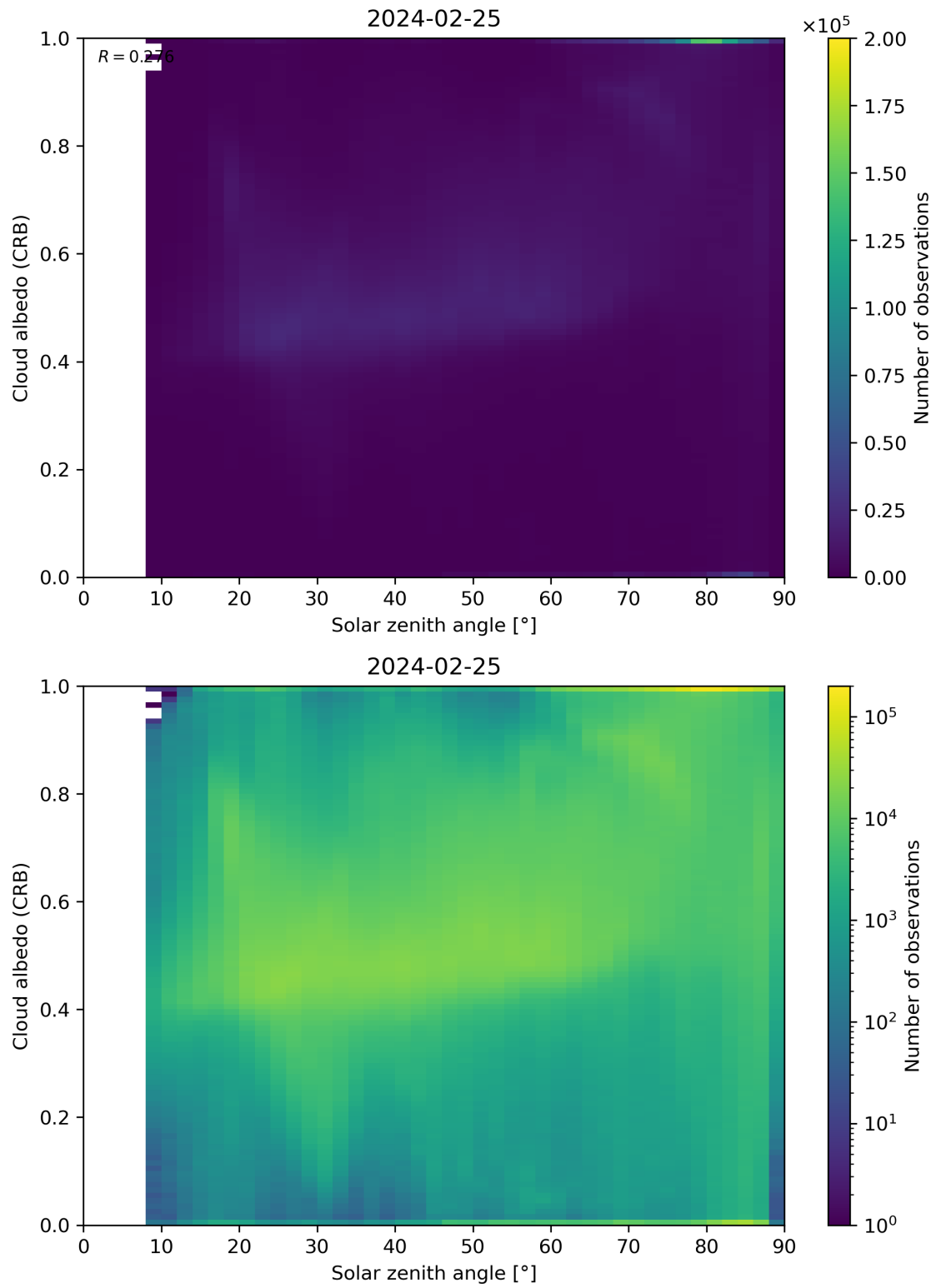
Figure 98: Scatter density plot of “Solar zenith angle” against “Cloud albedo (CRB)” for 2024-02-24 to 2024-02-26.
