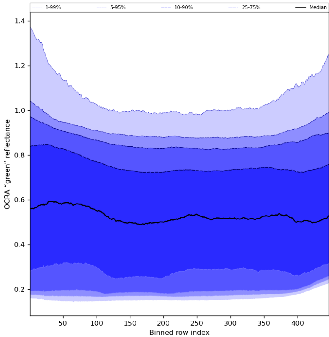
Figure 68: Along track statistics of "OCRA "green" reflectance" for 2024-02-24 to 2024-02-26
