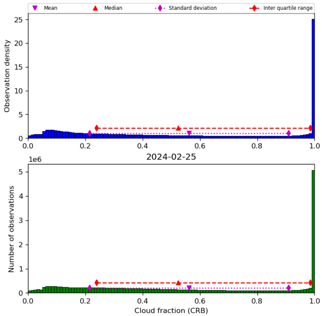
Figure 42: Histogram of “Cloud fraction (CRB)” for 2024-02-24 to 2024-02-26
