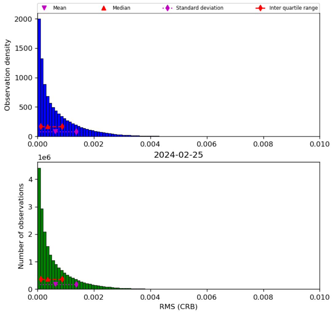
Figure 48: Histogram of “RMS (CRB)” for 2024-02-24 to 2024-02-26
