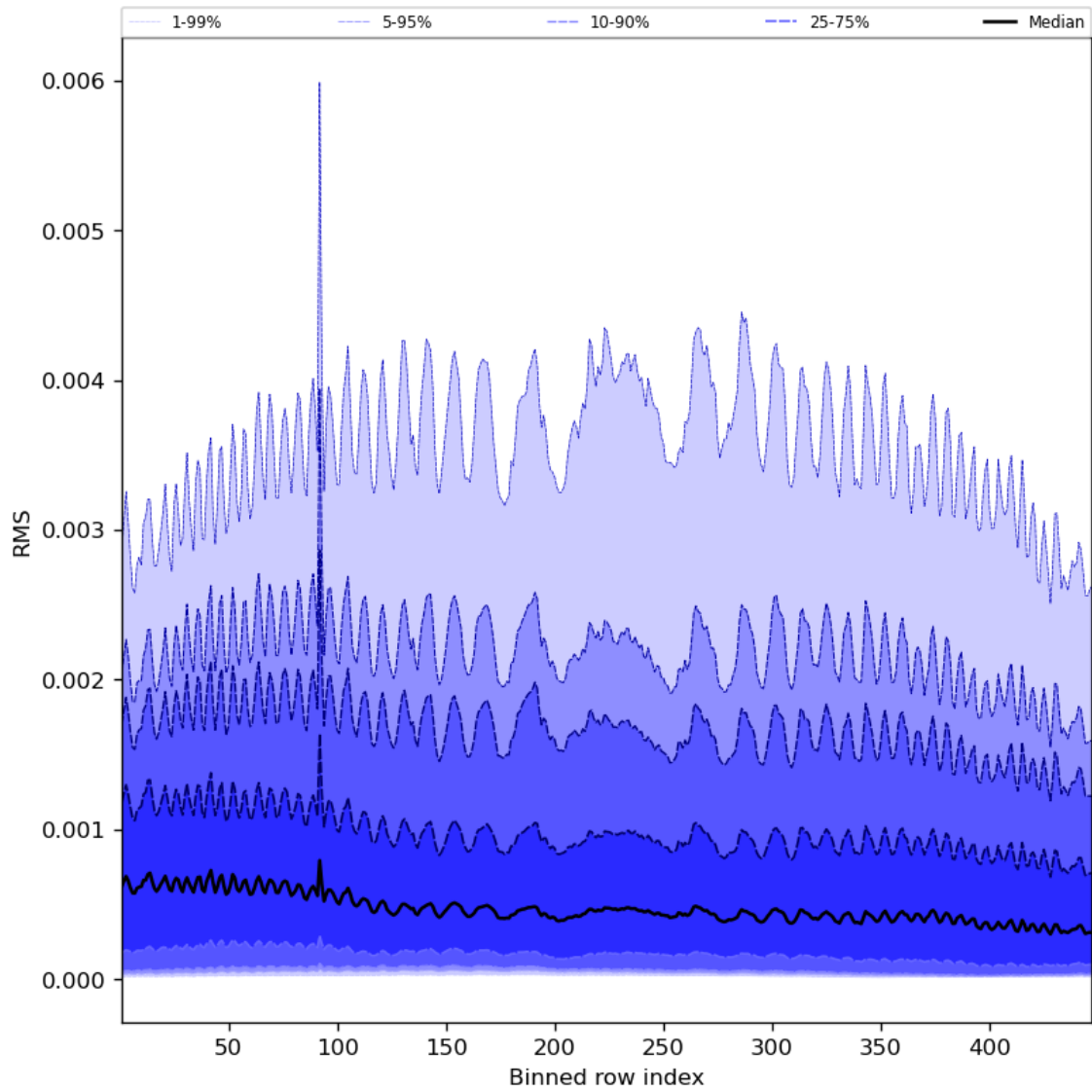
Figure 63: Along track statistics of “RMS” for 2024-02-24 to 2024-02-26
