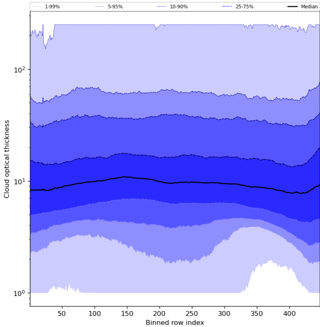
Figure 57: Along track statistics of “Cloud optical thickness” for 2024-02-24 to 2024-02-26
