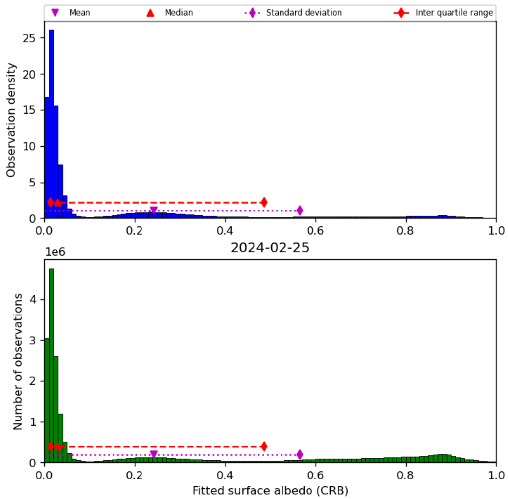
Figure 46: Histogram of “Fitted surface albedo (CRB)” for 2024-02-24 to 2024-02-26
