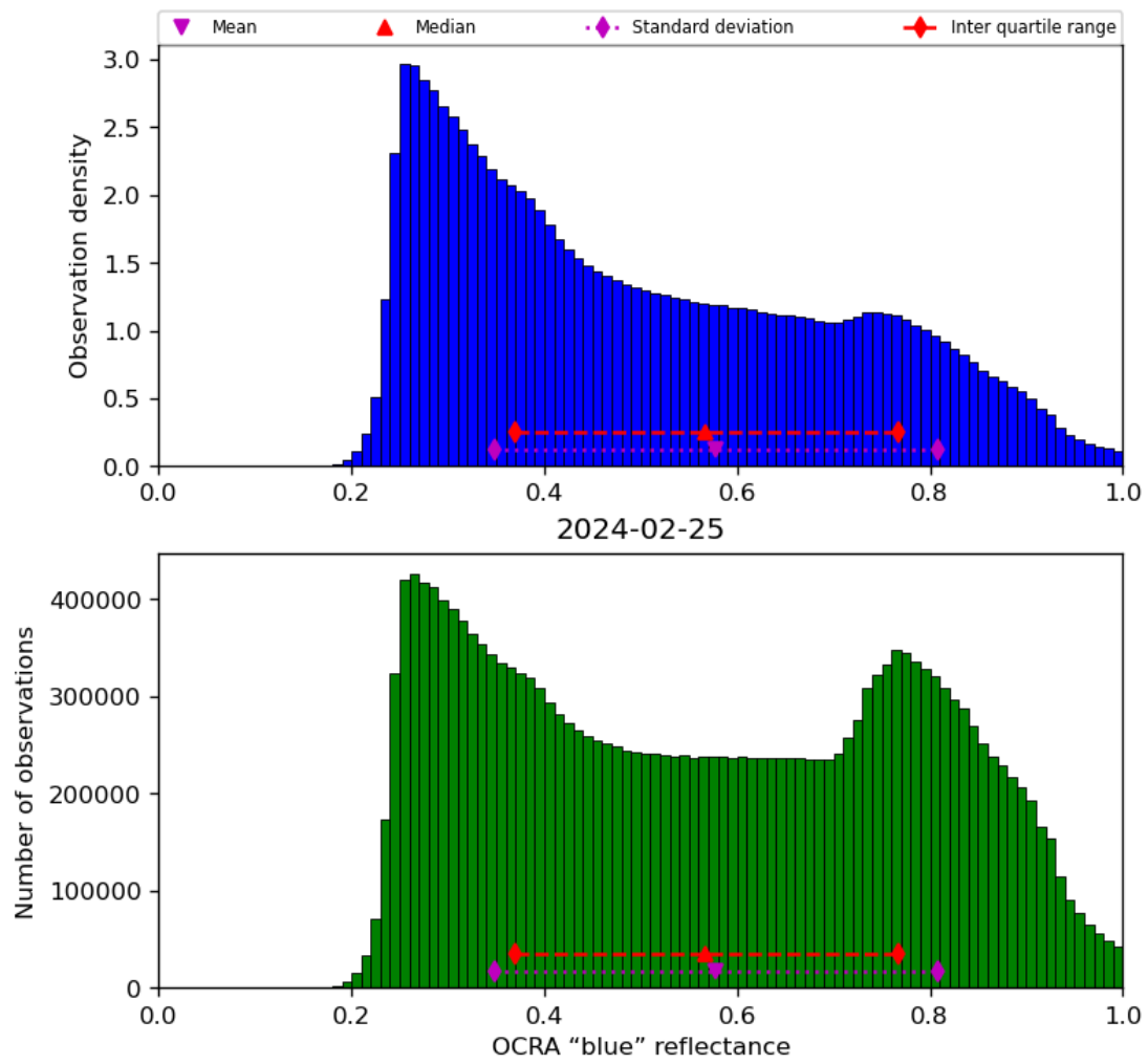
Figure 51: Histogram of “OCRA “blue” reflectance” for 2024-02-24 to 2024-02-26
