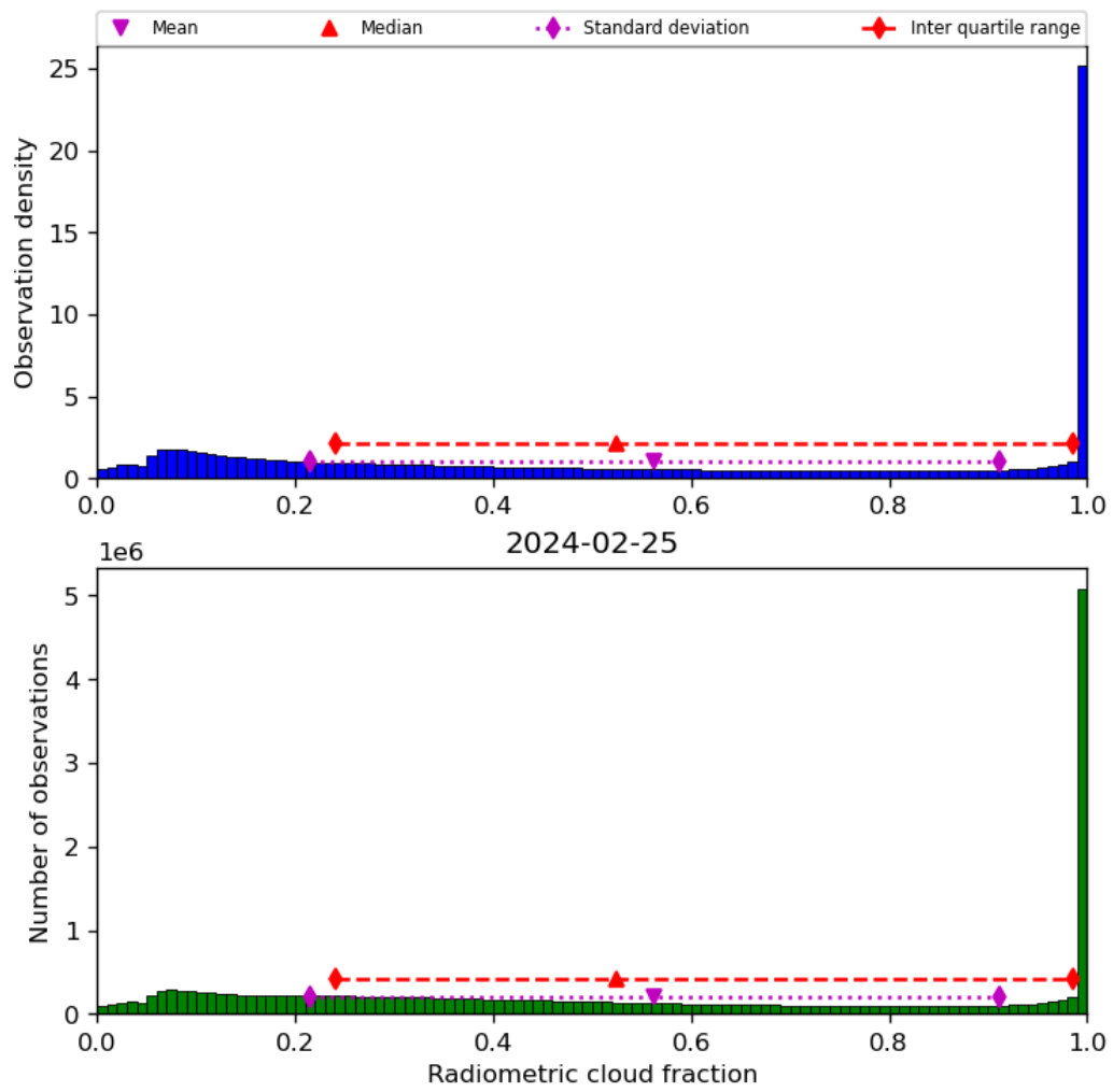
Figure 39: Histogram of “Radiometric cloud fraction” for 2024-02-24 to 2024-02-26
