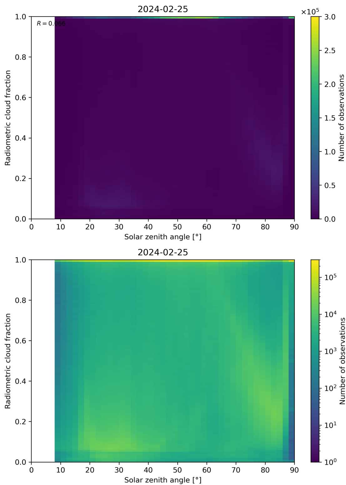
Figure 99: Scatter density plot of “Solar zenith angle” against “Radiometric cloud fraction” for 2024-02-24 to 2024-02-26.
