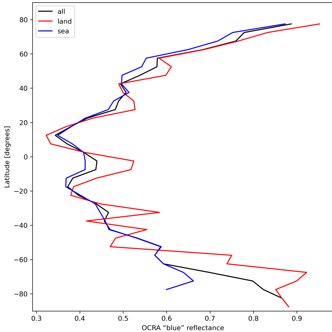
Figure 35: Zonal average of “OCRA “blue” reflectance” for 2024-02-24 to 2024-02-26.
