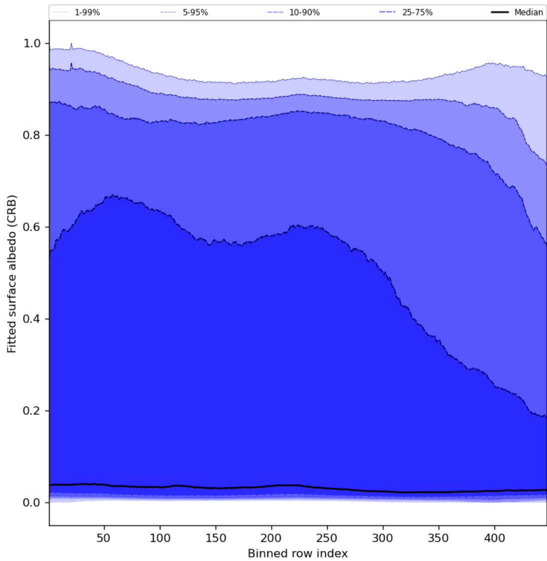
Figure 62: Along track statistics of “Fitted surface albedo (CRB)” for 2024-02-24 to 2024-02-26
