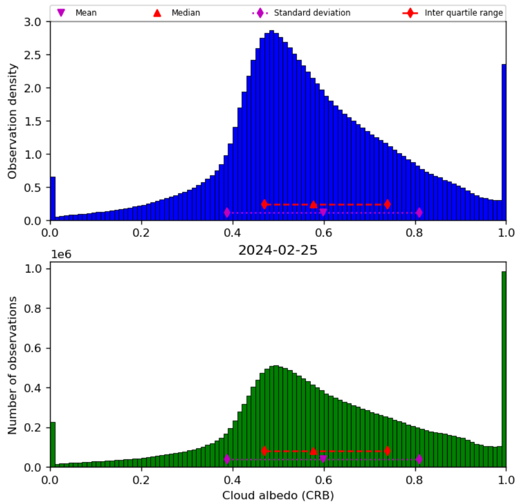
Figure 44: Histogram of “Cloud albedo (CRB)” for 2024-02-24 to 2024-02-26
