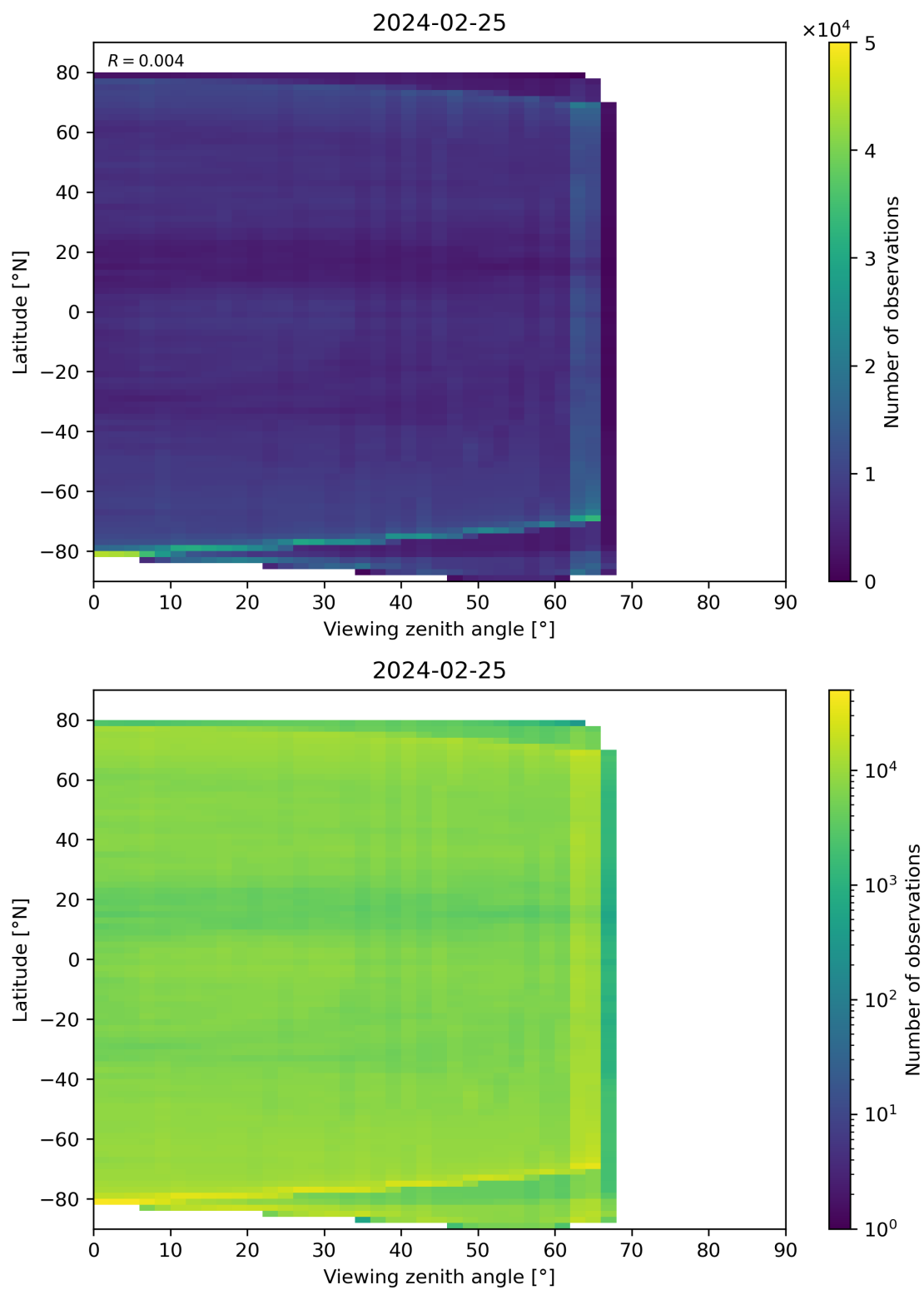
Figure 113: Scatter density plot of “Viewing zenith angle” against “Latitude” for 2024-02-24 to 2024-02-26.
