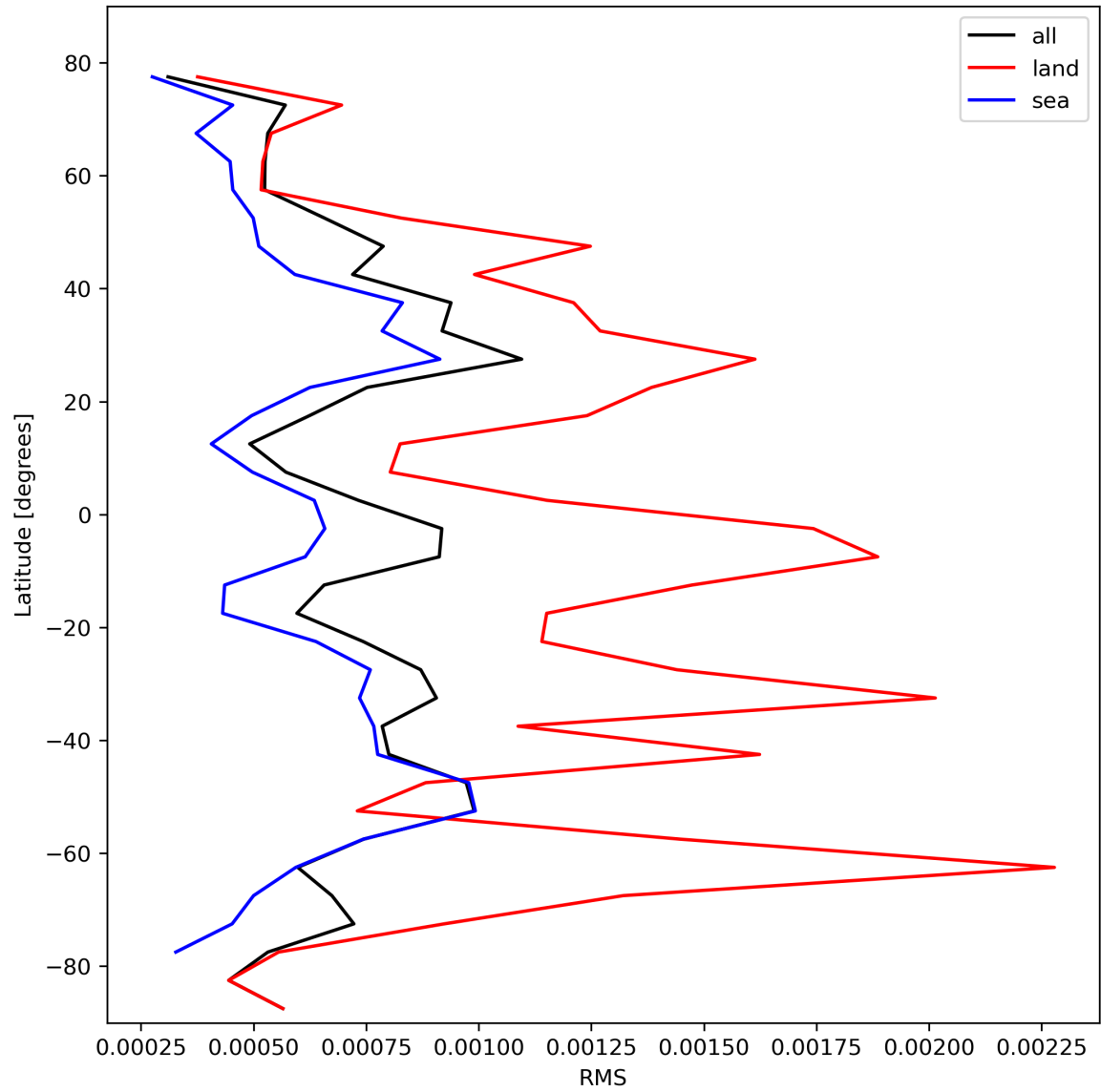
Figure 31: Zonal average of “RMS” for 2024-02-24 to 2024-02-26.
