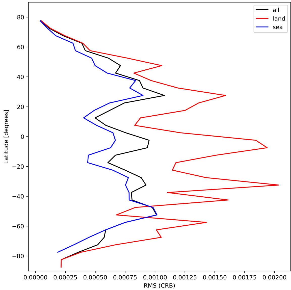
Figure 32: Zonal average of “RMS (CRB)” for 2024-02-24 to 2024-02-26.
