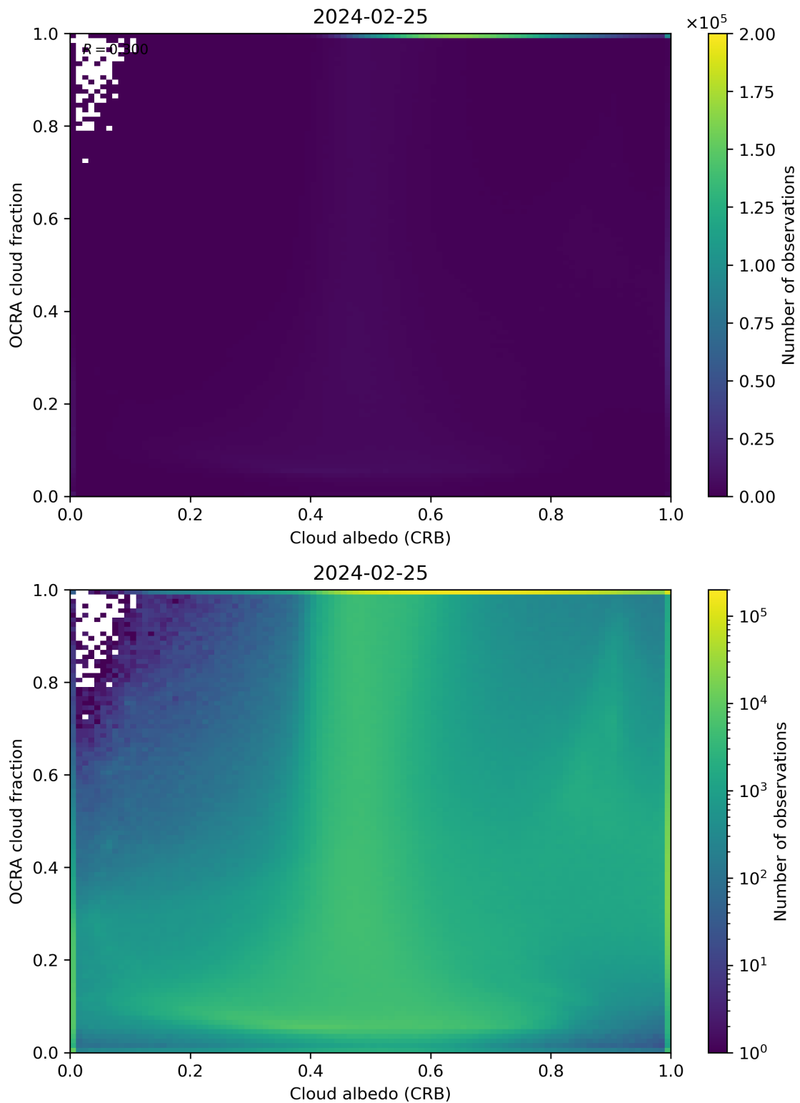
Figure 70: Scatter density plot of “Cloud albedo (CRB)” against “OCRA cloud fraction” for 2024-02-24 to 2024-02-26.
