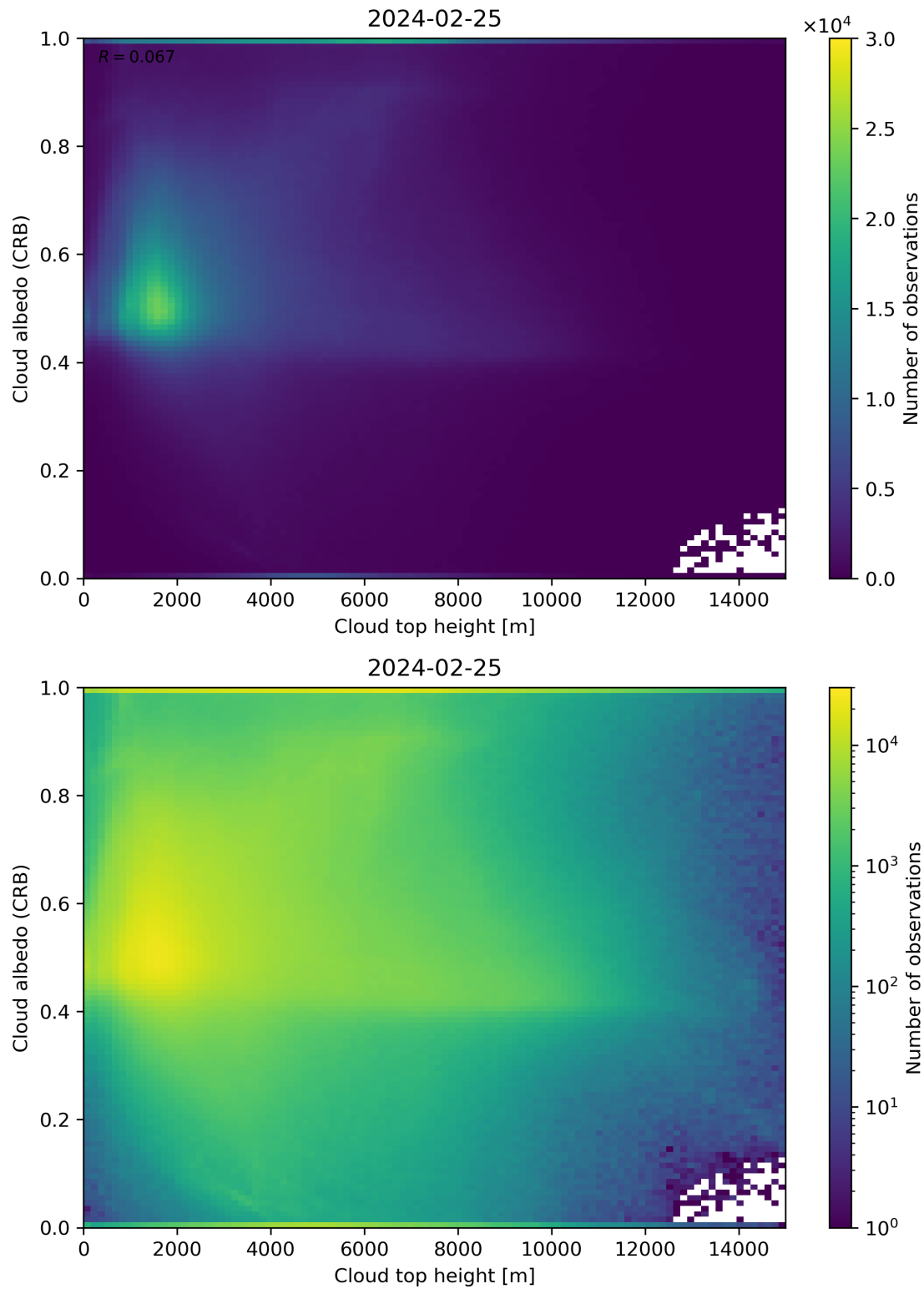
Figure 86: Scatter density plot of “Cloud top height” against “Cloud albedo (CRB)” for 2024-02-24 to 2024-02-26.
