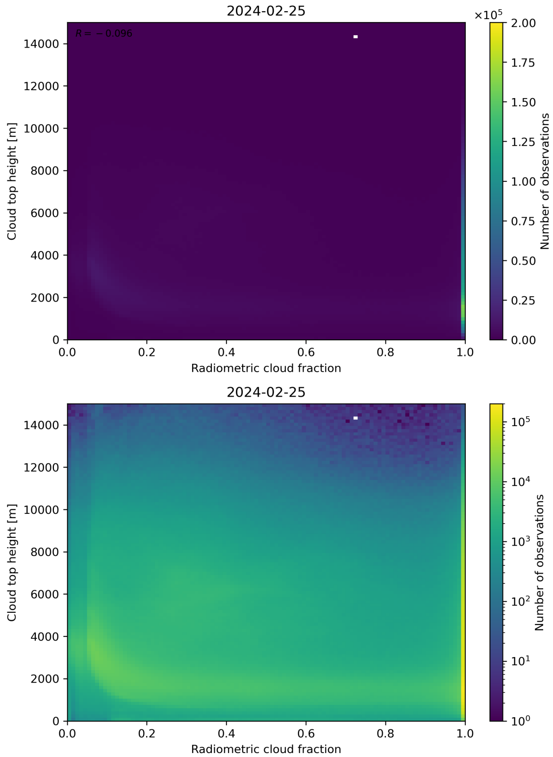
Figure 76: Scatter density plot of “Radiometric cloud fraction” against “Cloud top height” for 2024-02-24 to 2024-02-26.
