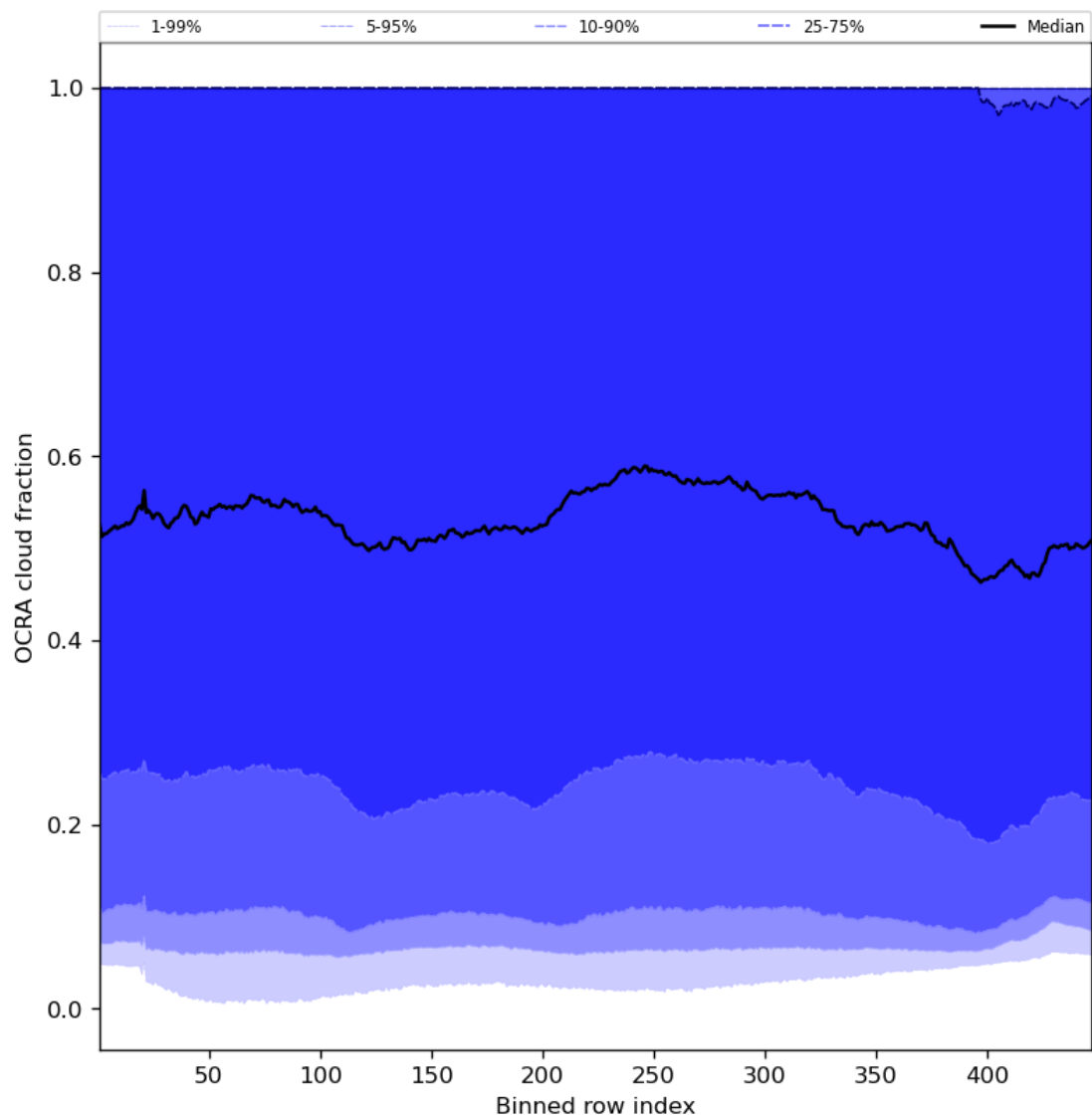
Figure 66: Along track statistics of “OCRA cloud fraction” for 2024-02-24 to 2024-02-26
