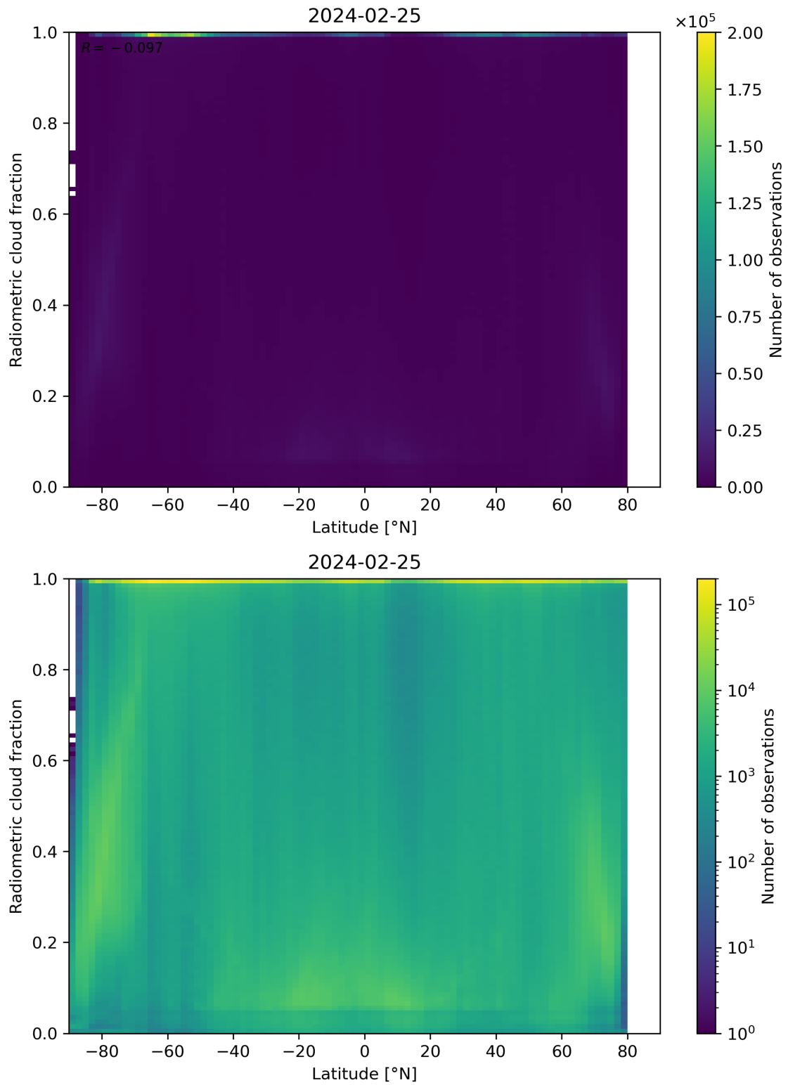
Figure 92: Scatter density plot of “Latitude” against “Radiometric cloud fraction” for 2024-02-24 to 2024-02-26.
