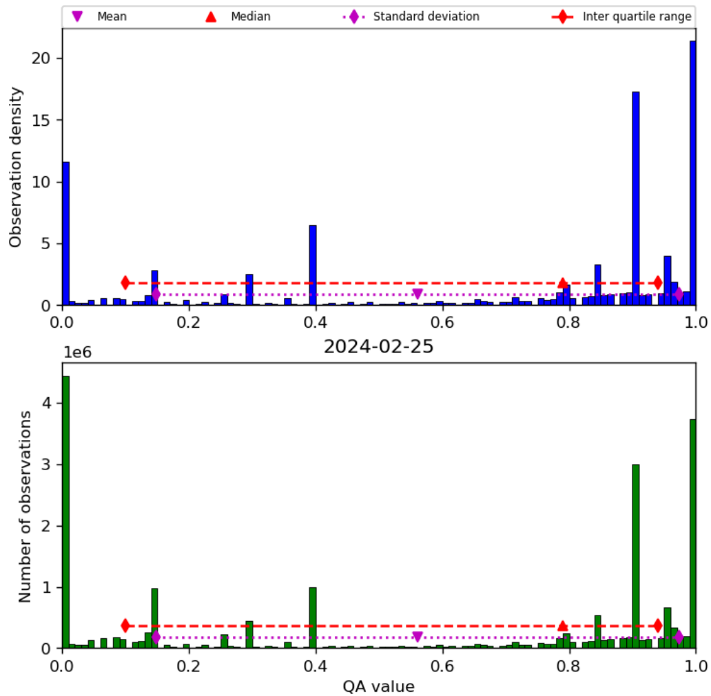
Figure 38: Histogram of “QA value” for 2024-02-24 to 2024-02-26
