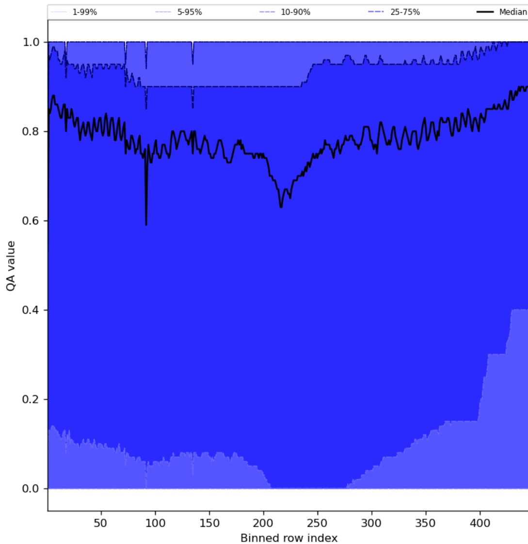
Figure 54: Along track statistics of “QA value” for 2024-02-24 to 2024-02-26
