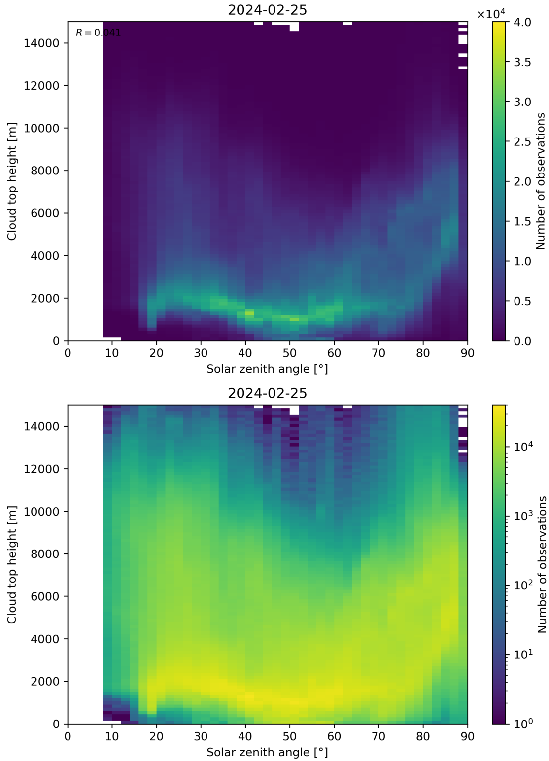
Figure 104: Scatter density plot of “Solar zenith angle” against “Cloud top height” for 2024-02-24 to 2024-02-26.
