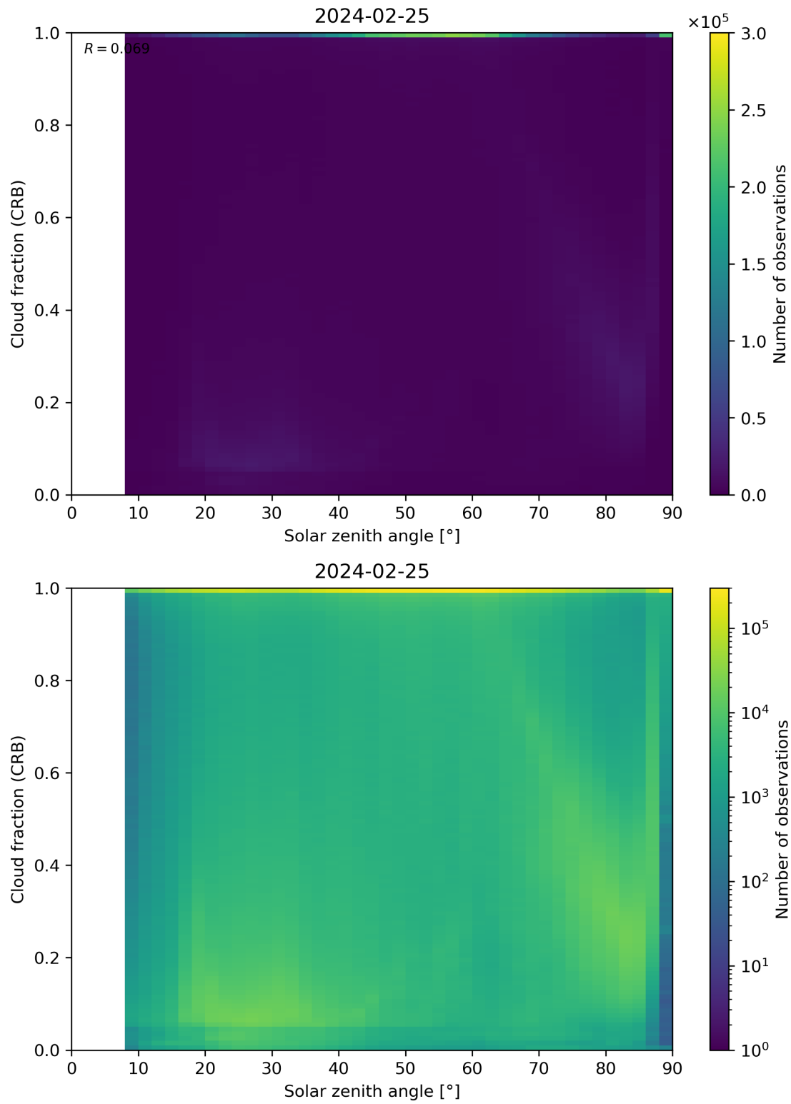
Figure 101: Scatter density plot of “Solar zenith angle” against “Cloud fraction (CRB)” for 2024-02-24 to 2024-02-26.
