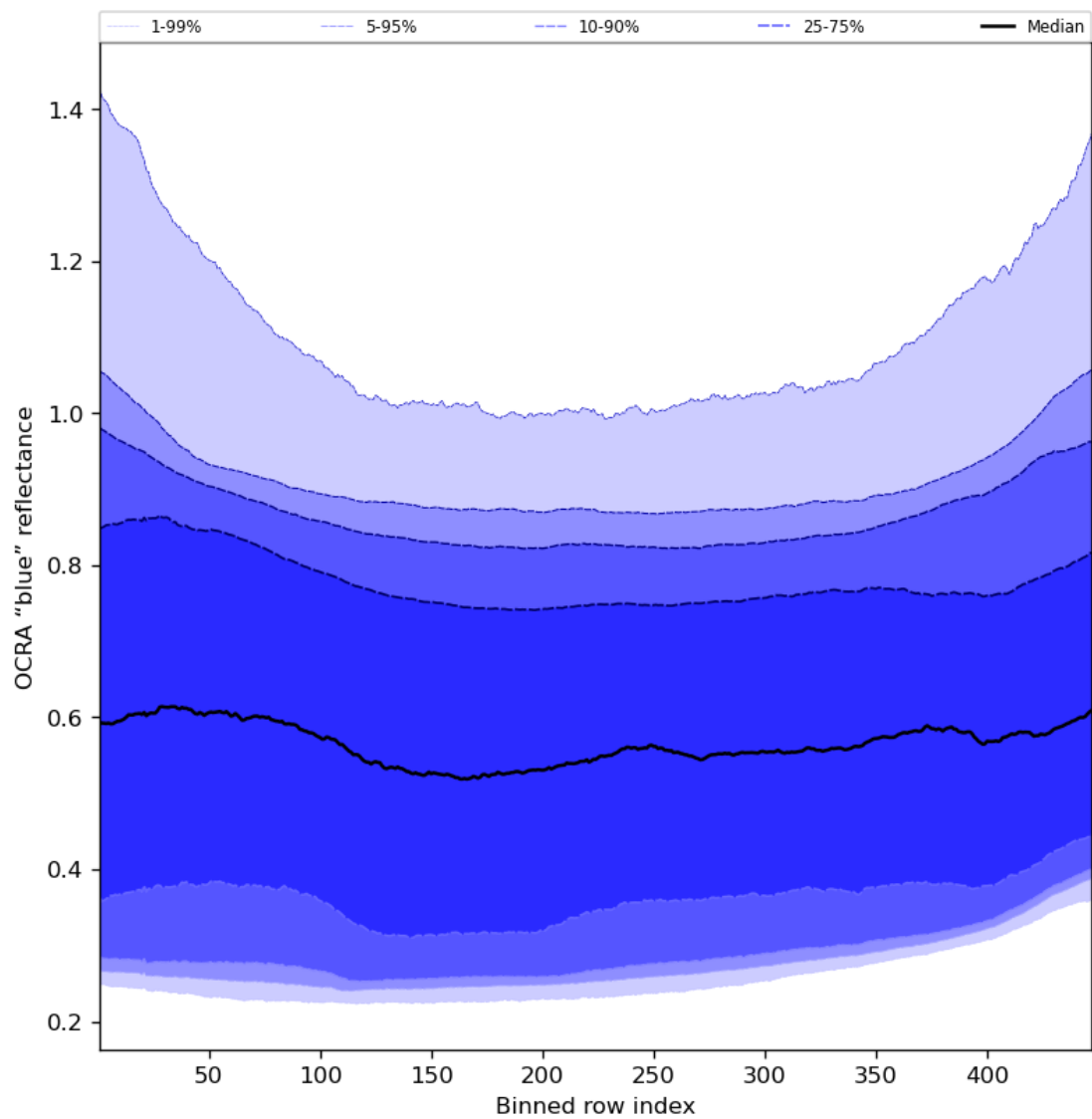
Figure 67: Along track statistics of “OCRA “blue” reflectance” for 2024-02-24 to 2024-02-26
