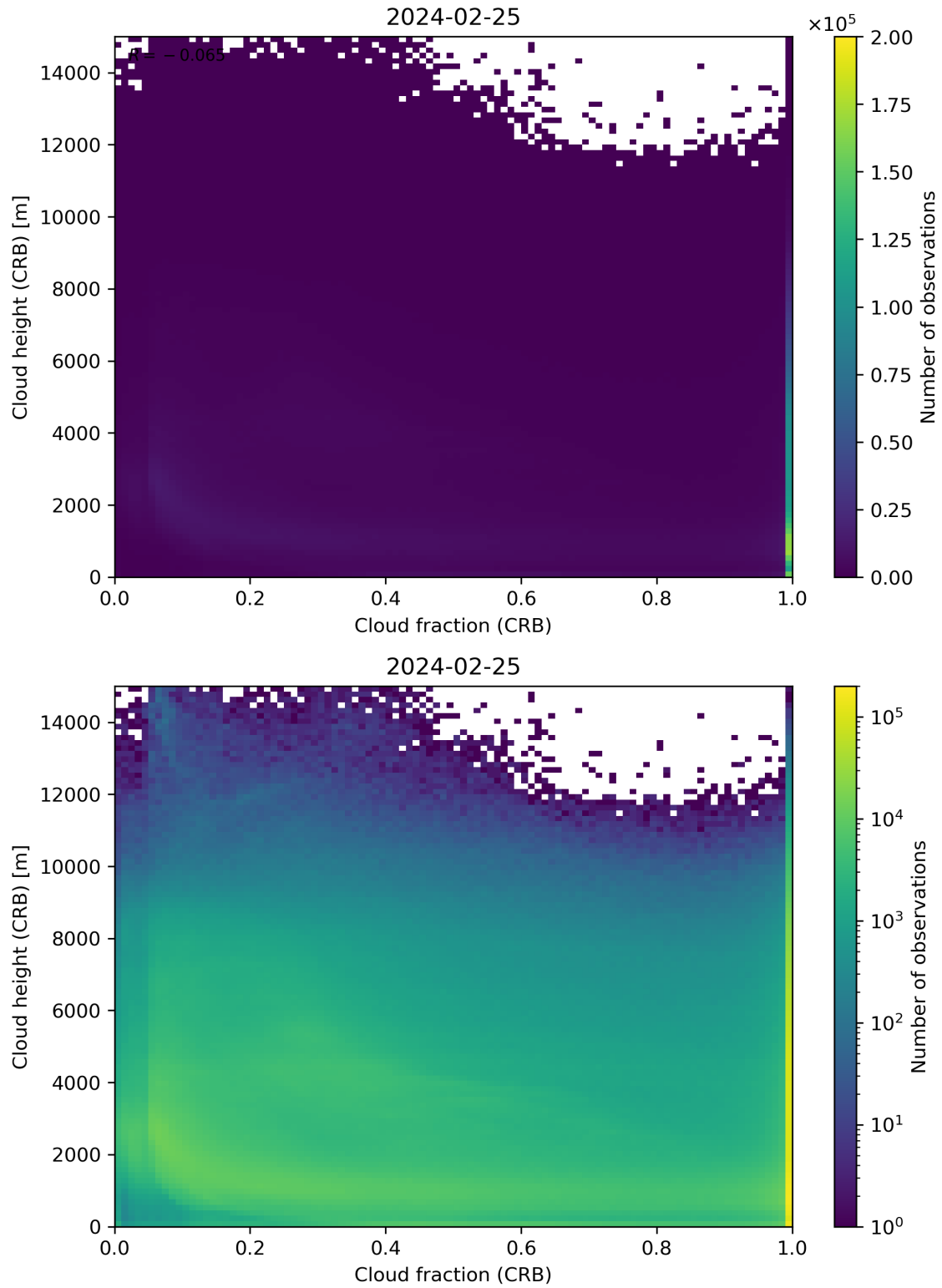
Figure 79: Scatter density plot of “Cloud fraction (CRB)” against “Cloud height (CRB)” for 2024-02-24 to 2024-02-26.
