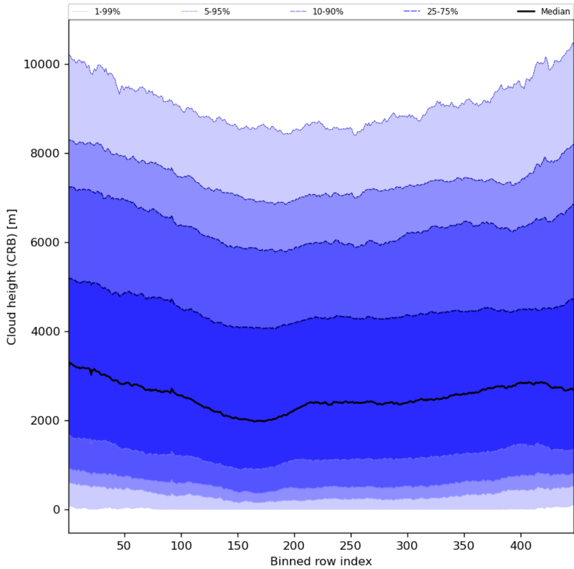
Figure 59: Along track statistics of “Cloud height (CRB)” for 2024-02-24 to 2024-02-26
