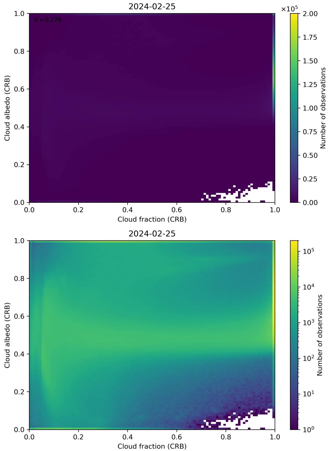
Figure 77: Scatter density plot of “Cloud fraction (CRB)” against “Cloud albedo (CRB)” for 2024-02-24 to 2024-02-26.
