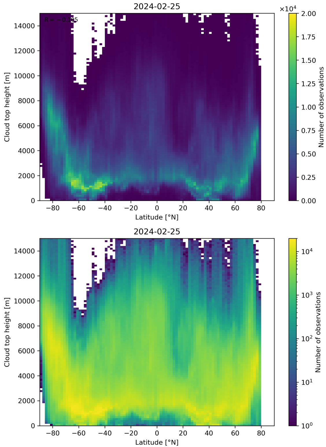
Figure 97: Scatter density plot of “Latitude” against “Cloud top height” for 2024-02-24 to 2024-02-26.
