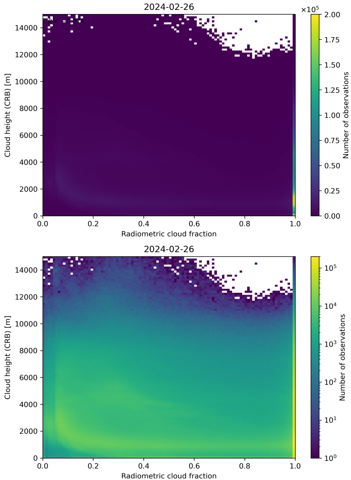
Figure 74: Scatter density plot of “Radiometric cloud fraction” against “Cloud height (CRB)” for 2024-02-25 to 2024-02-27.
