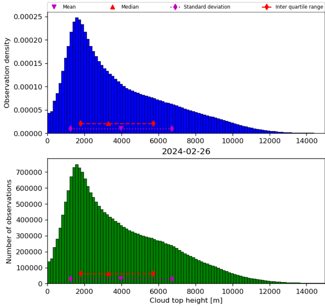
Figure 40: Histogram of “Cloud top height” for 2024-02-25 to 2024-02-27
