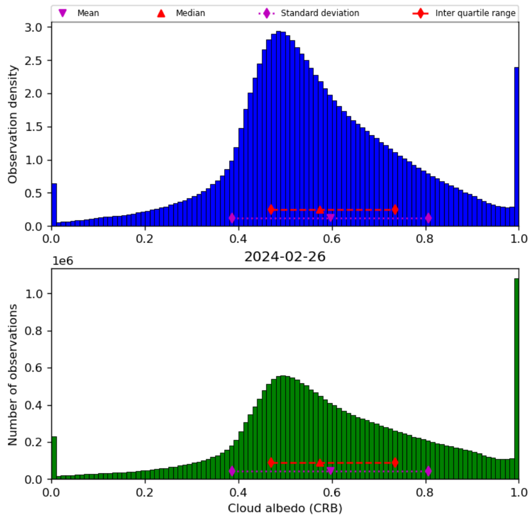
Figure 44: Histogram of “Cloud albedo (CRB)” for 2024-02-25 to 2024-02-27
