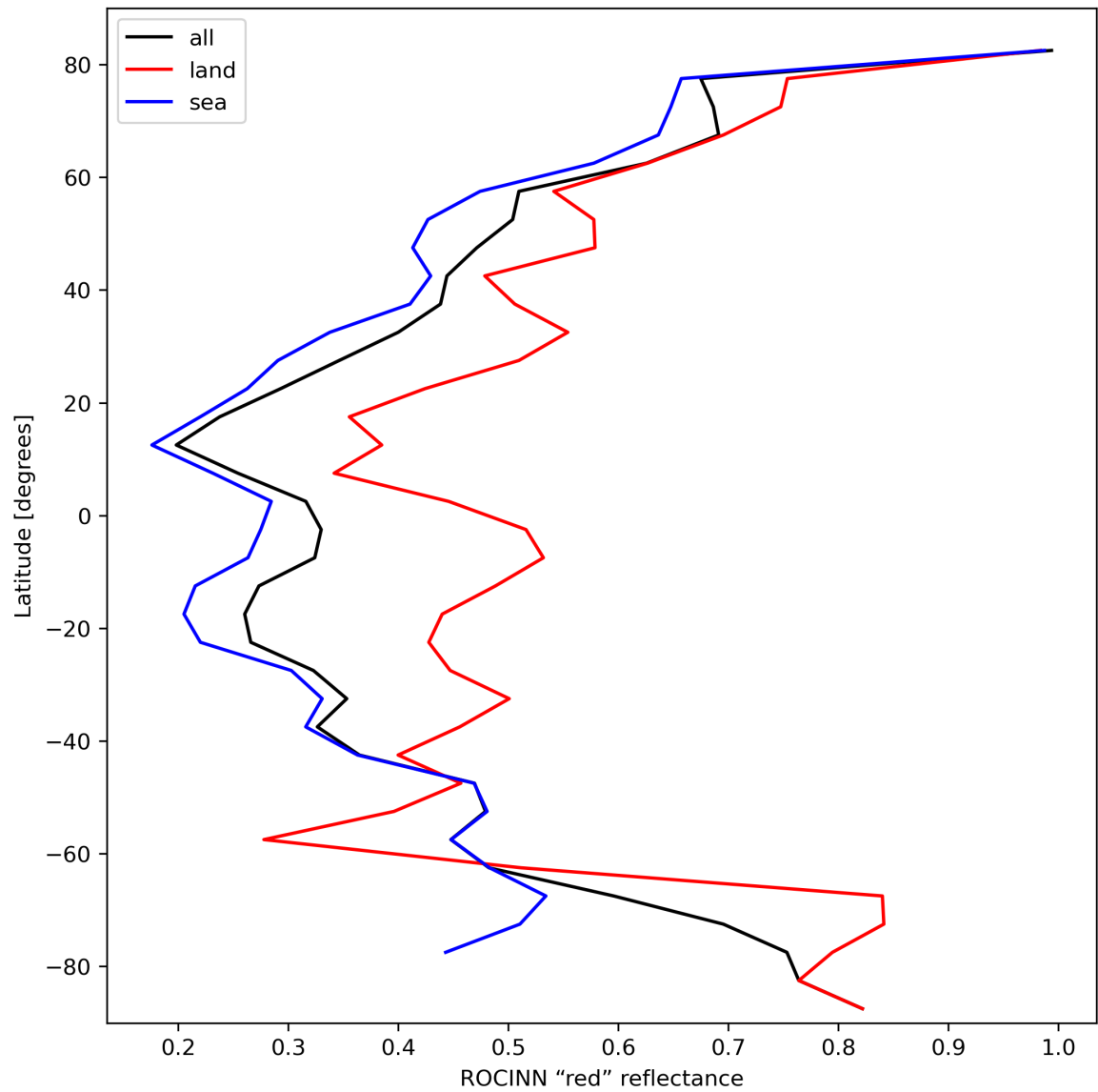
Figure 37: Zonal average of “ROCINN “red” reflectance” for 2024-02-25 to 2024-02-27.
