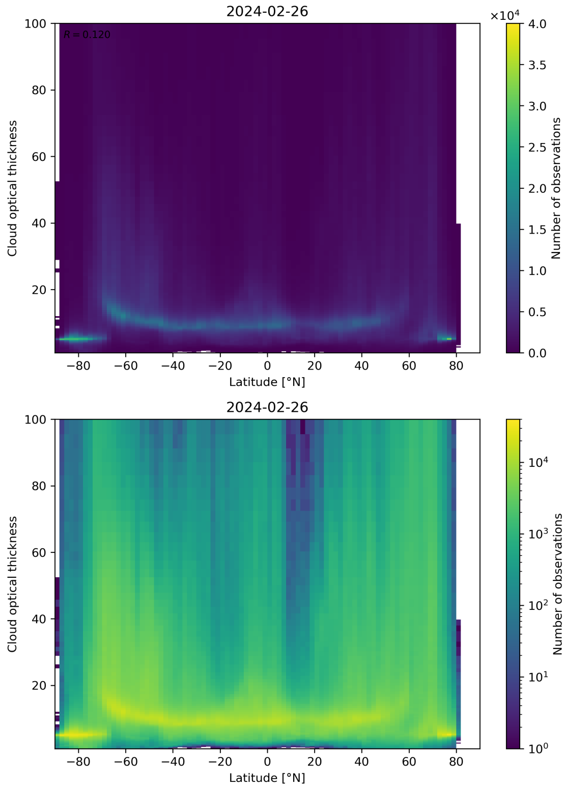
Figure 96: Scatter density plot of “Latitude” against “Cloud optical thickness” for 2024-02-25 to 2024-02-27.
