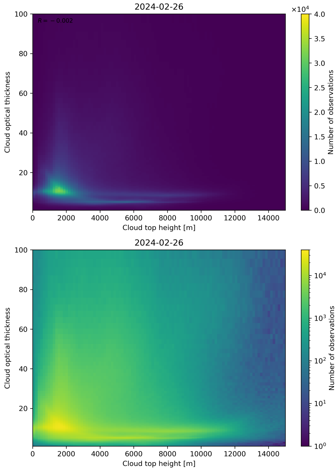
Figure 90: Scatter density plot of “Cloud top height” against “Cloud optical thickness” for 2024-02-25 to 2024-02-27.
