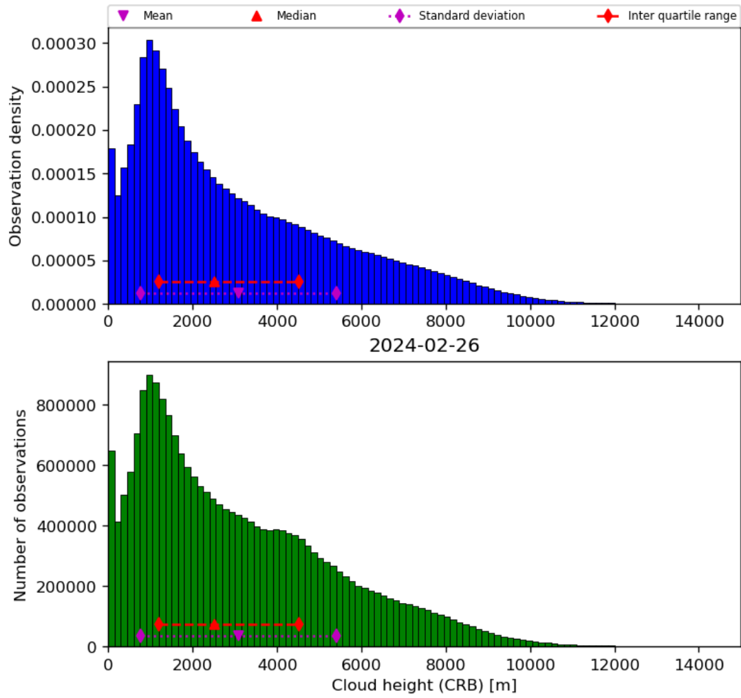
Figure 43: Histogram of “Cloud height (CRB)” for 2024-02-25 to 2024-02-27
