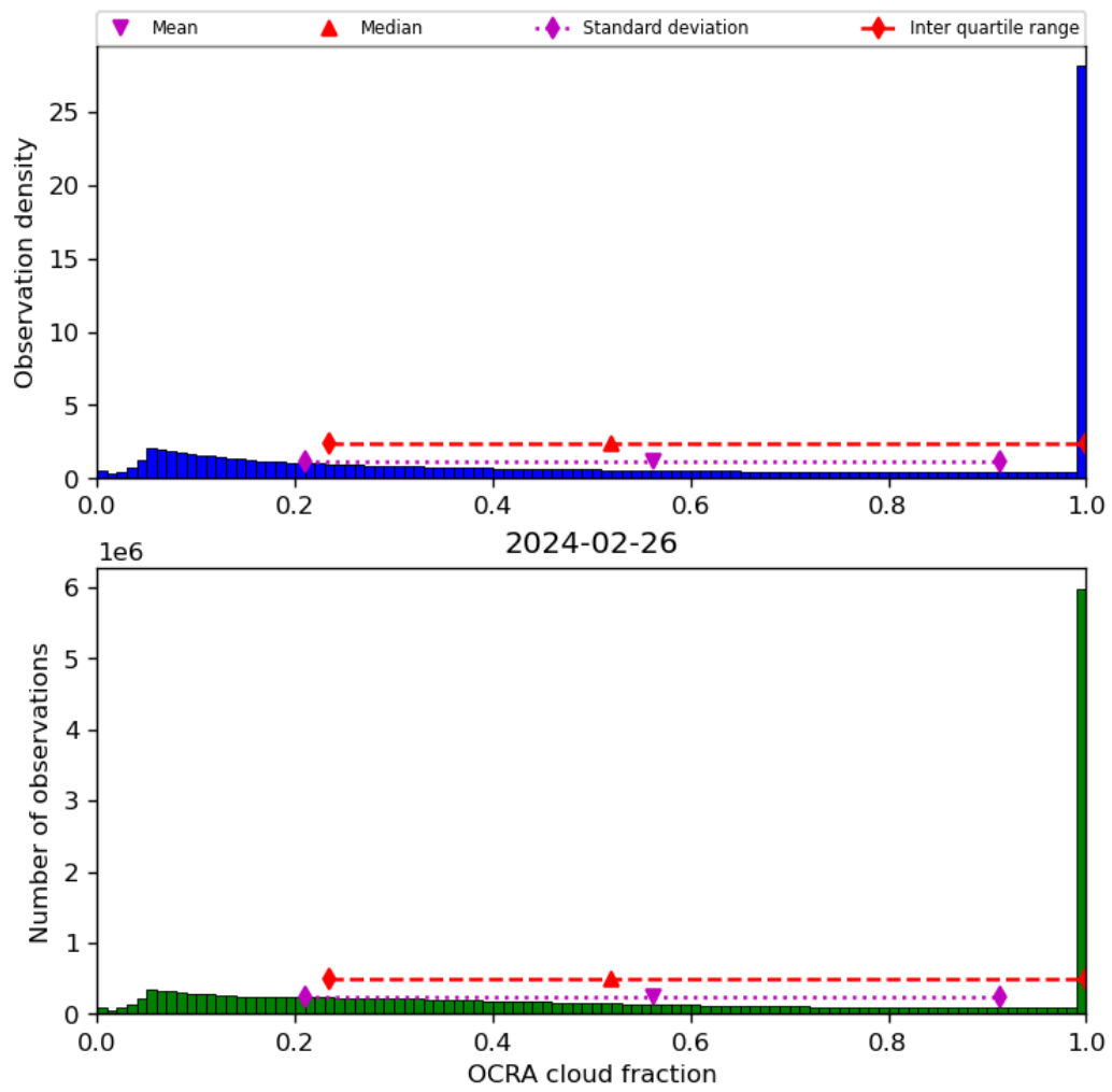
Figure 50: Histogram of “OCRA cloud fraction” for 2024-02-25 to 2024-02-27
