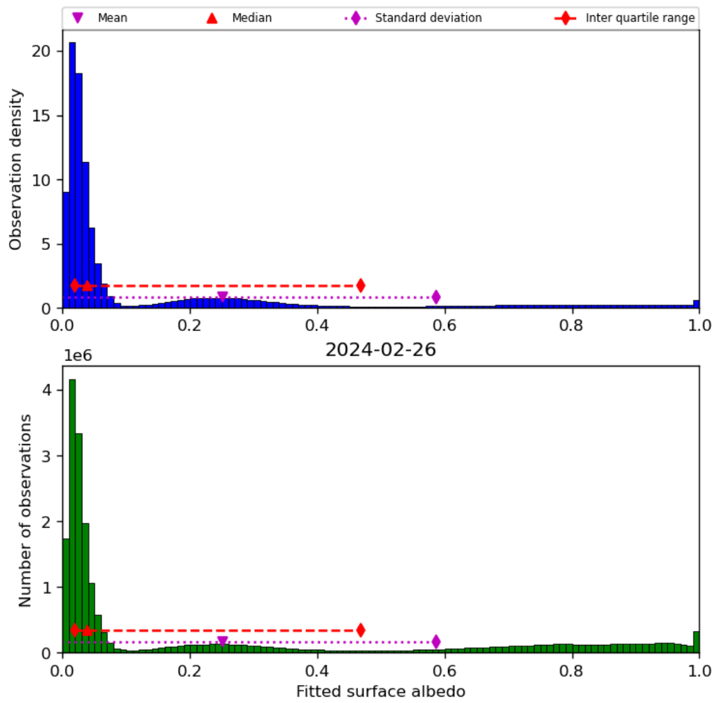
Figure 45: Histogram of “Fitted surface albedo” for 2024-02-25 to 2024-02-27
