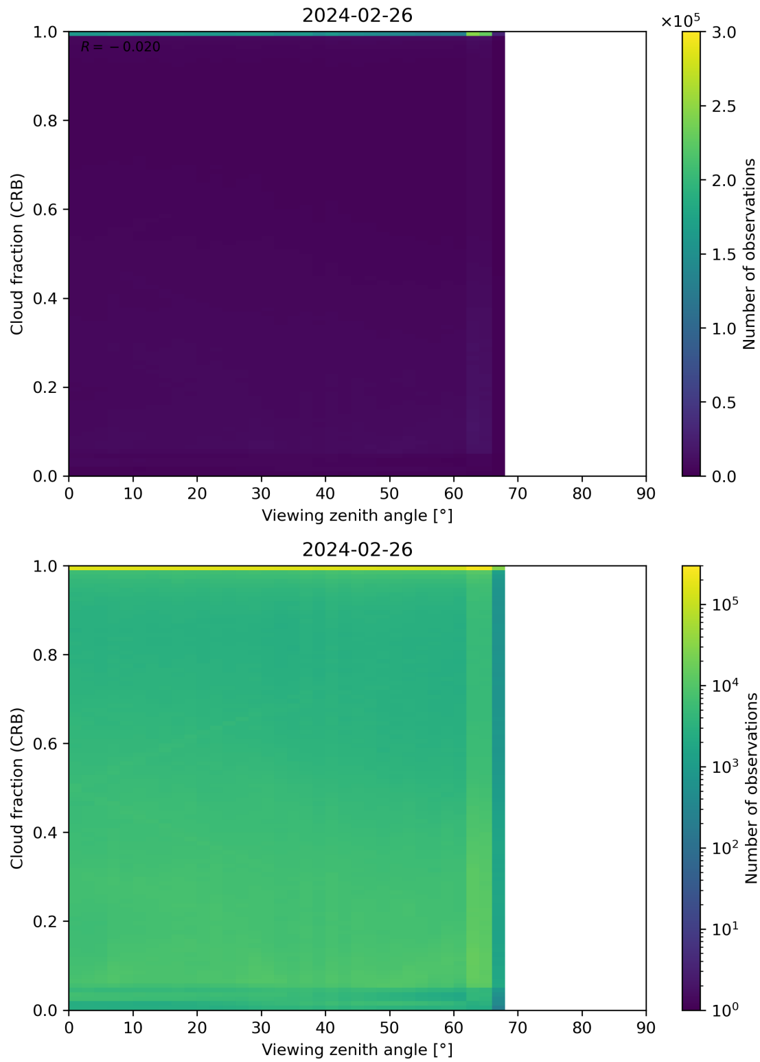
Figure 109: Scatter density plot of “Viewing zenith angle” against “Cloud fraction (CRB)” for 2024-02-25 to 2024-02-27.
