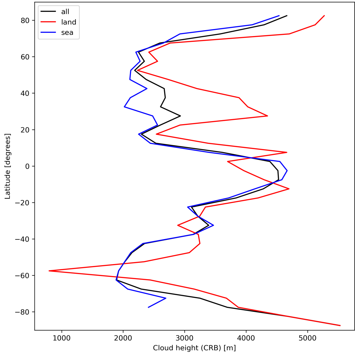
Figure 27: Zonal average of “Cloud height (CRB)” for 2024-02-25 to 2024-02-27.
