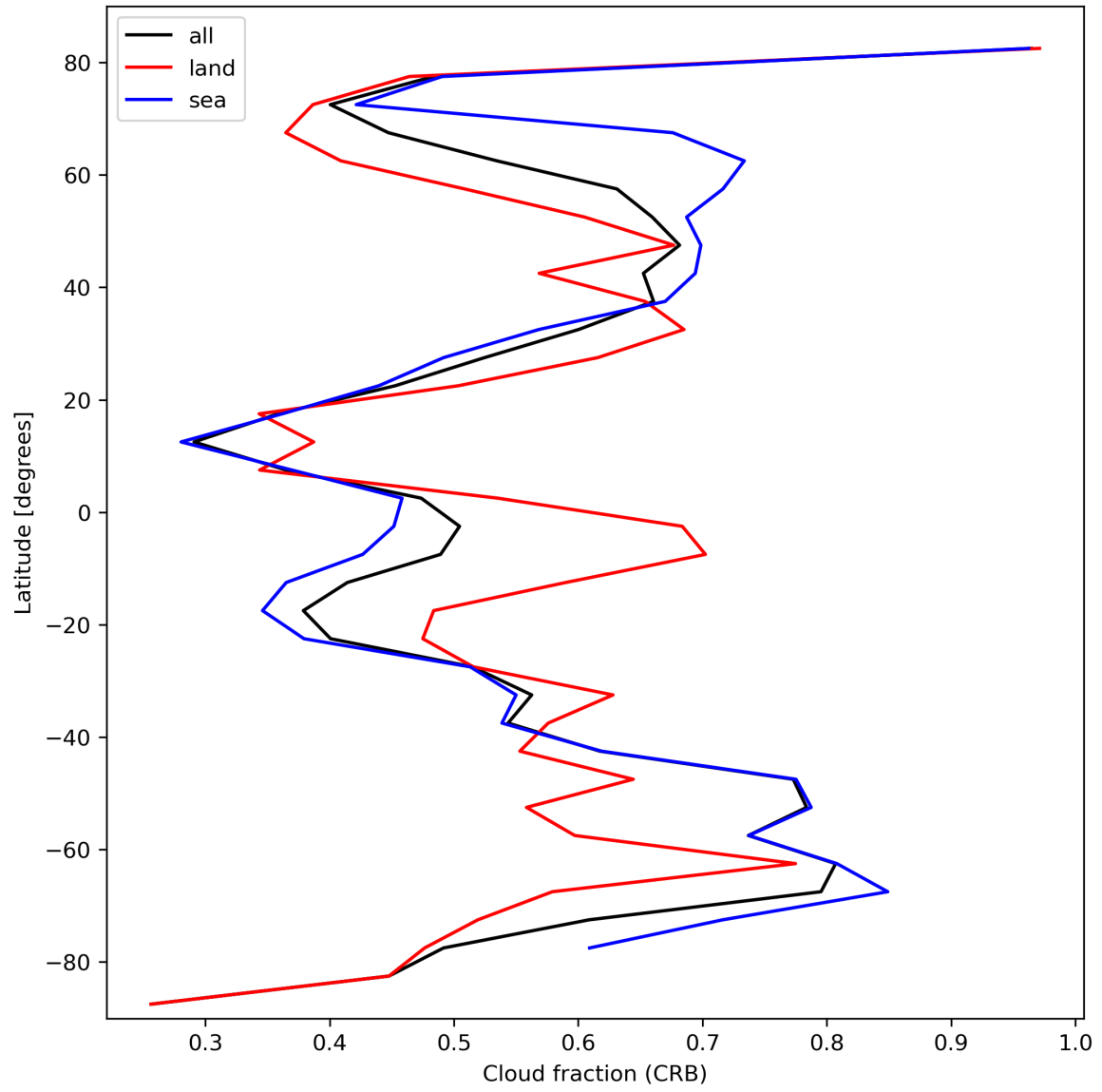
Figure 26: Zonal average of “Cloud fraction (CRB)” for 2024-02-25 to 2024-02-27.
