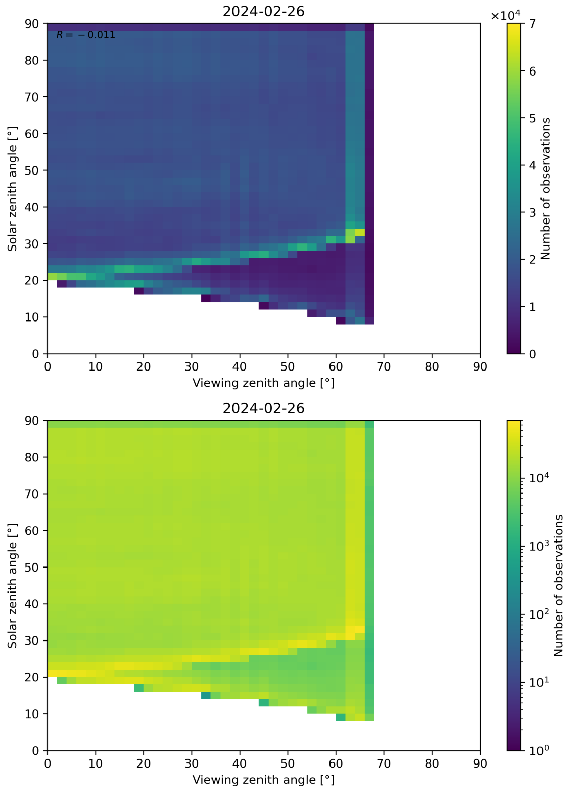
Figure 114: Scatter density plot of “Viewing zenith angle” against “Solar zenith angle” for 2024-02-25 to 2024-02-27.
