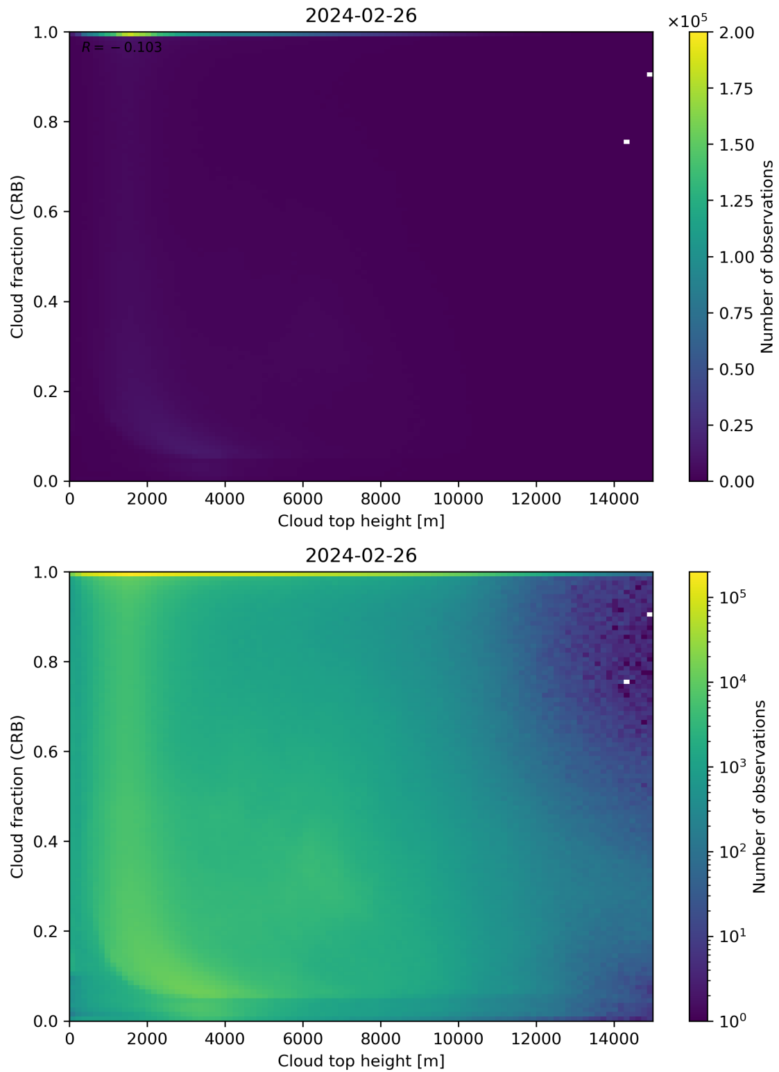
Figure 88: Scatter density plot of “Cloud top height” against “Cloud fraction (CRB)” for 2024-02-25 to 2024-02-27.
