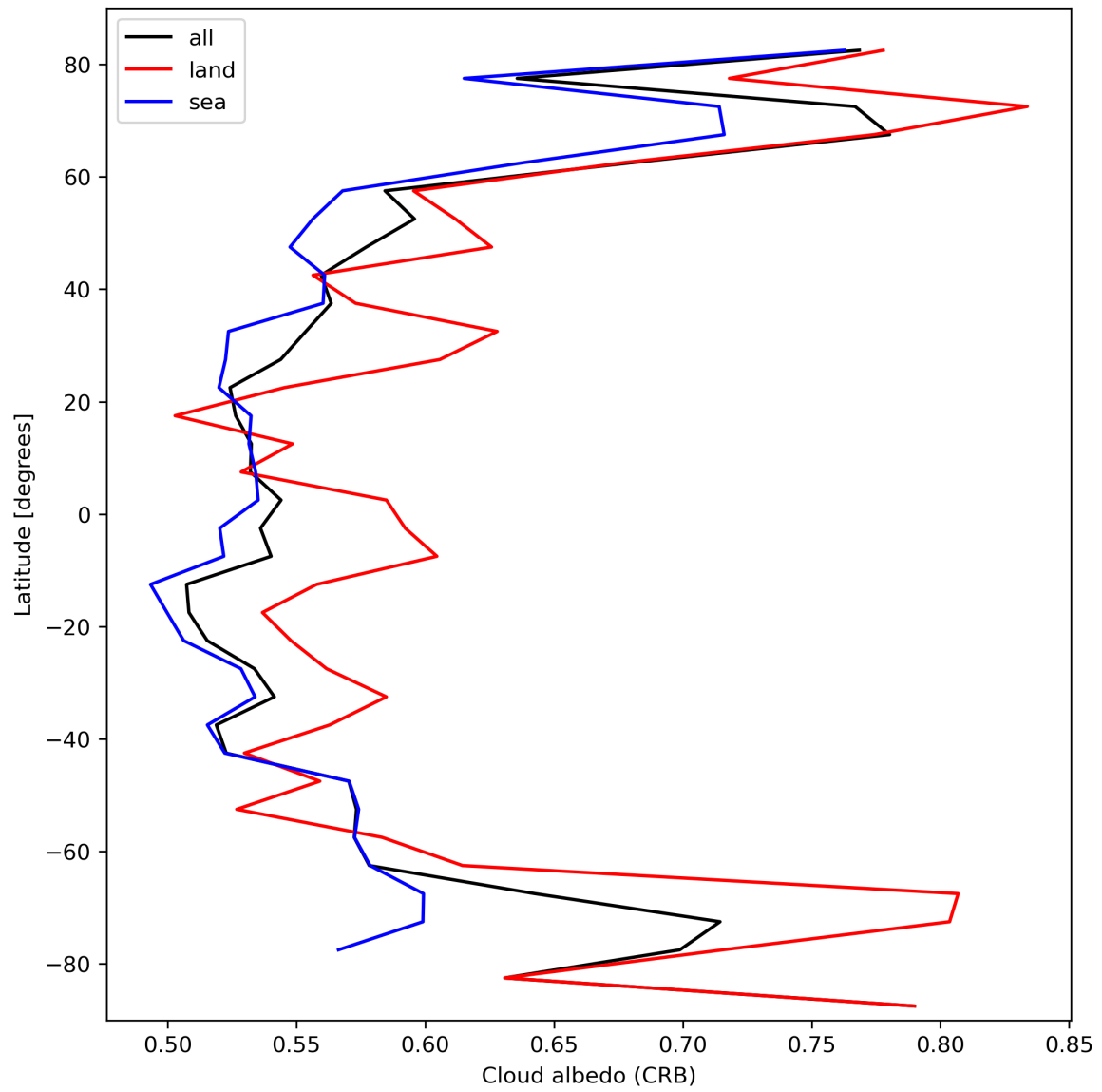
Figure 28: Zonal average of “Cloud albedo (CRB)” for 2024-02-25 to 2024-02-27.
