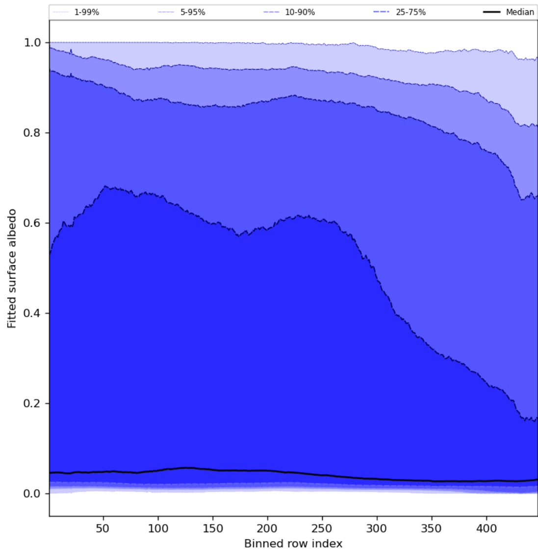
Figure 61: Along track statistics of “Fitted surface albedo” for 2024-02-25 to 2024-02-27
