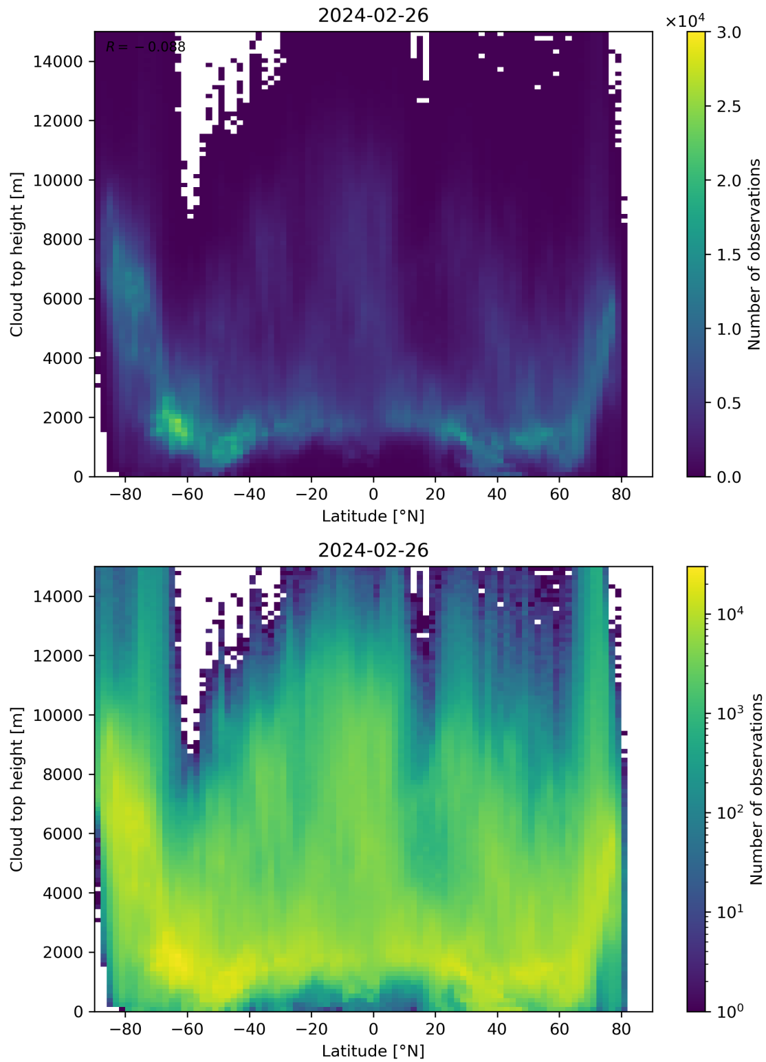
Figure 97: Scatter density plot of “Latitude” against “Cloud top height” for 2024-02-25 to 2024-02-27.
