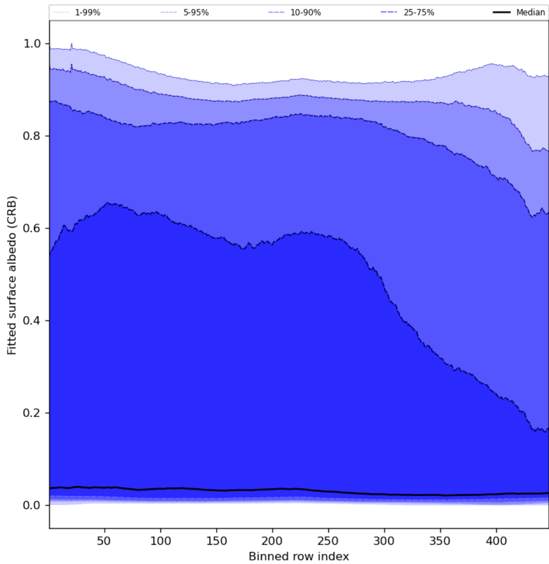
Figure 62: Along track statistics of “Fitted surface albedo (CRB)” for 2024-02-25 to 2024-02-27
