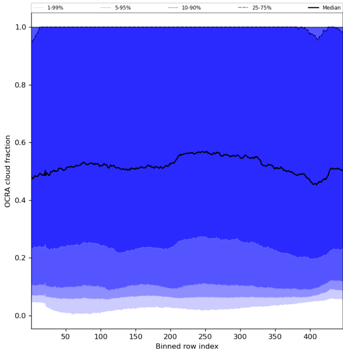
Figure 66: Along track statistics of “OCRA cloud fraction” for 2024-02-25 to 2024-02-27
