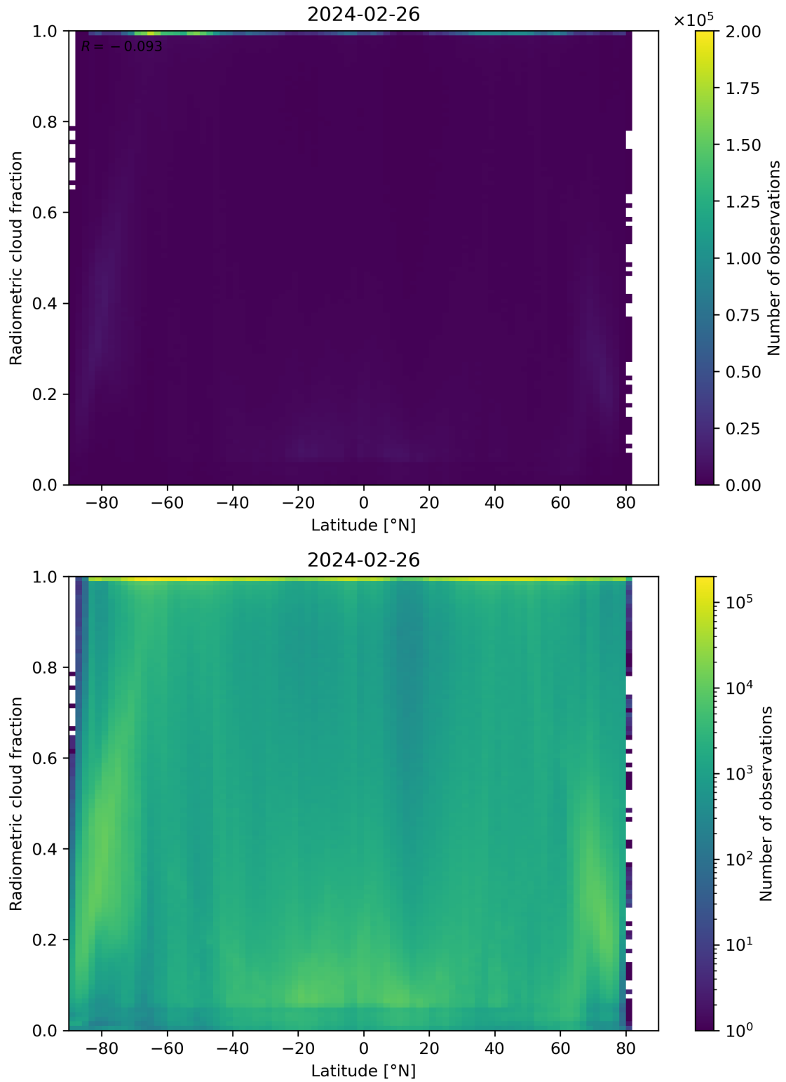
Figure 92: Scatter density plot of “Latitude” against “Radiometric cloud fraction” for 2024-02-25 to 2024-02-27.
