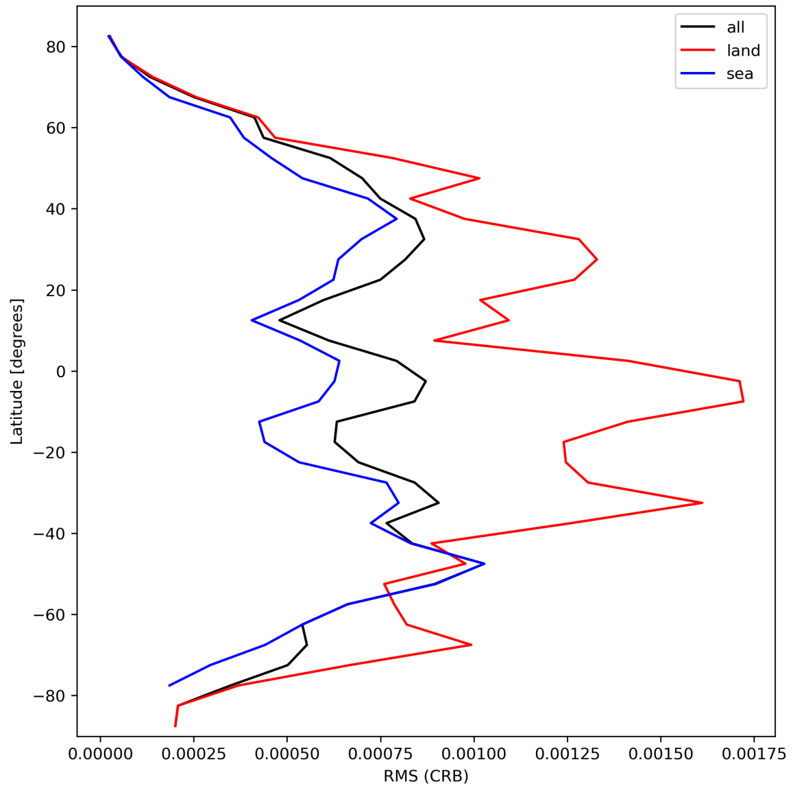
Figure 32: Zonal average of “RMS (CRB)” for 2024-02-25 to 2024-02-27.
