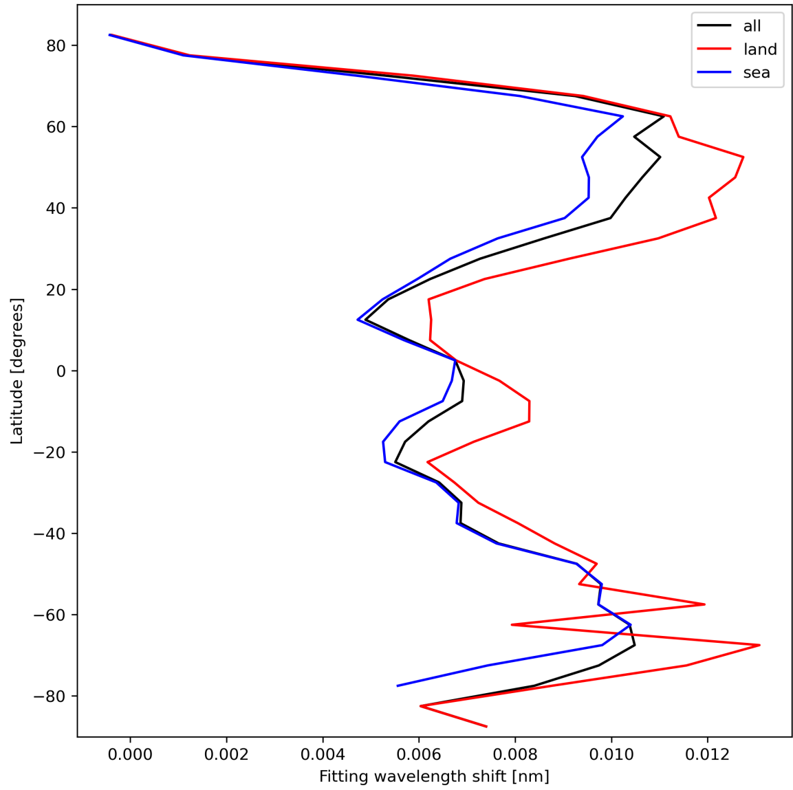
Figure 33: Zonal average of “Fitting wavelength shift” for 2024-02-25 to 2024-02-27.
