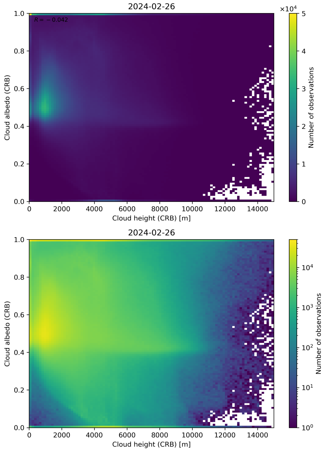
Figure 80: Scatter density plot of “Cloud height (CRB)” against “Cloud albedo (CRB)” for 2024-02-25 to 2024-02-27.
