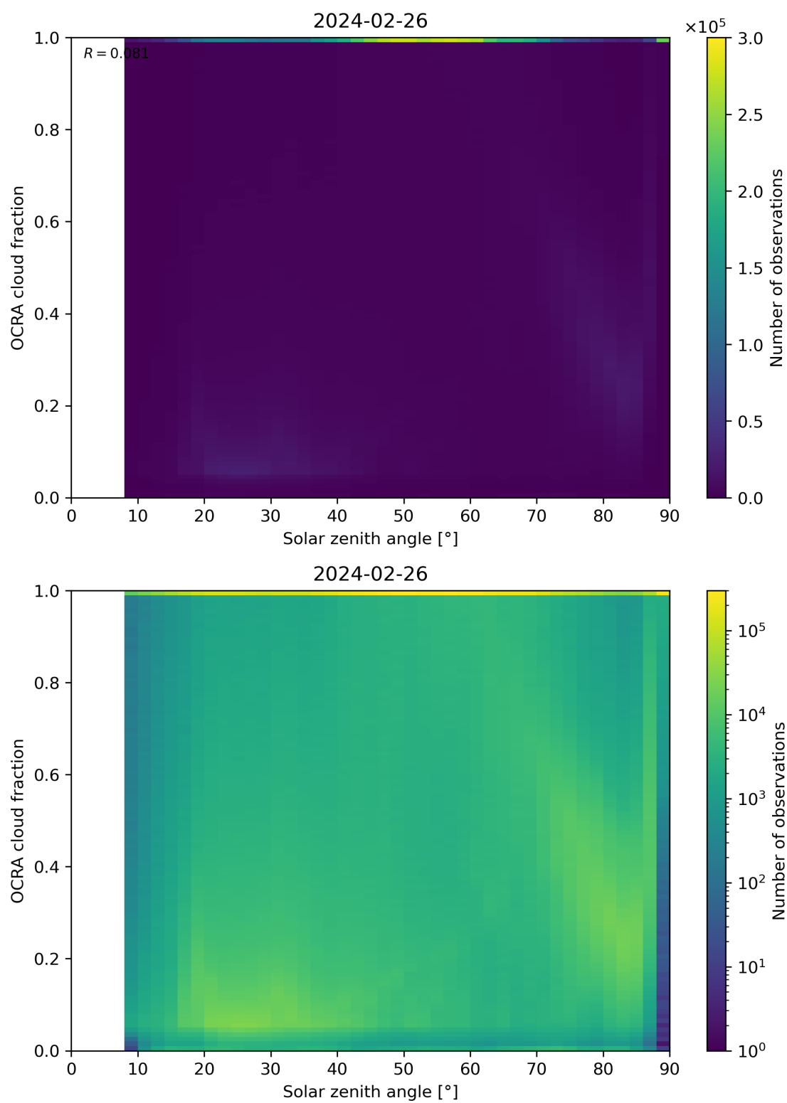
Figure 100: Scatter density plot of “Solar zenith angle” against “OCRA cloud fraction” for 2024-02-25 to 2024-02-27.
