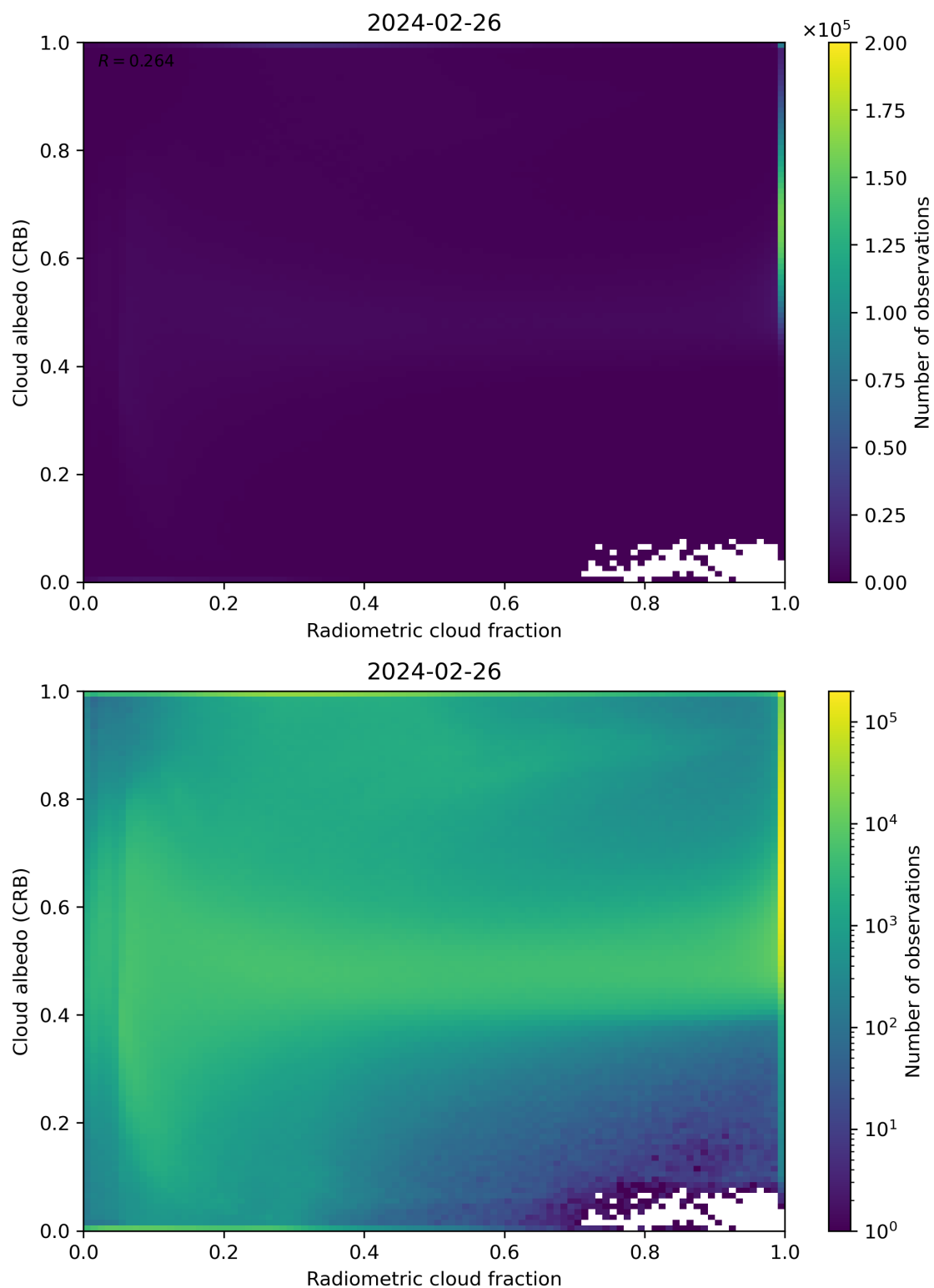
Figure 71: Scatter density plot of “Radiometric cloud fraction” against “Cloud albedo (CRB)” for 2024-02-25 to 2024-02-27.
