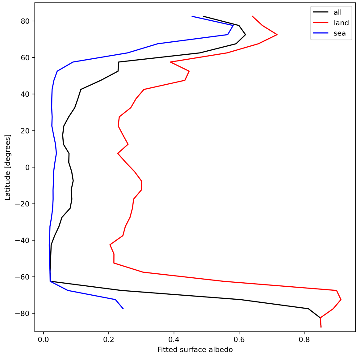
Figure 29: Zonal average of “Fitted surface albedo” for 2024-02-25 to 2024-02-27.
