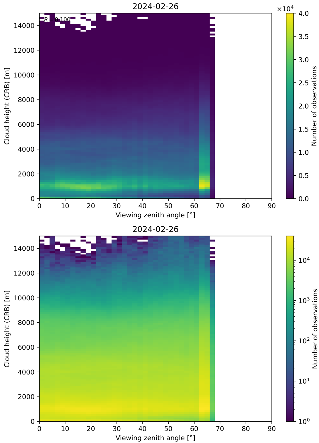
Figure 110: Scatter density plot of “Viewing zenith angle” against “Cloud height (CRB)” for 2024-02-25 to 2024-02-27.
