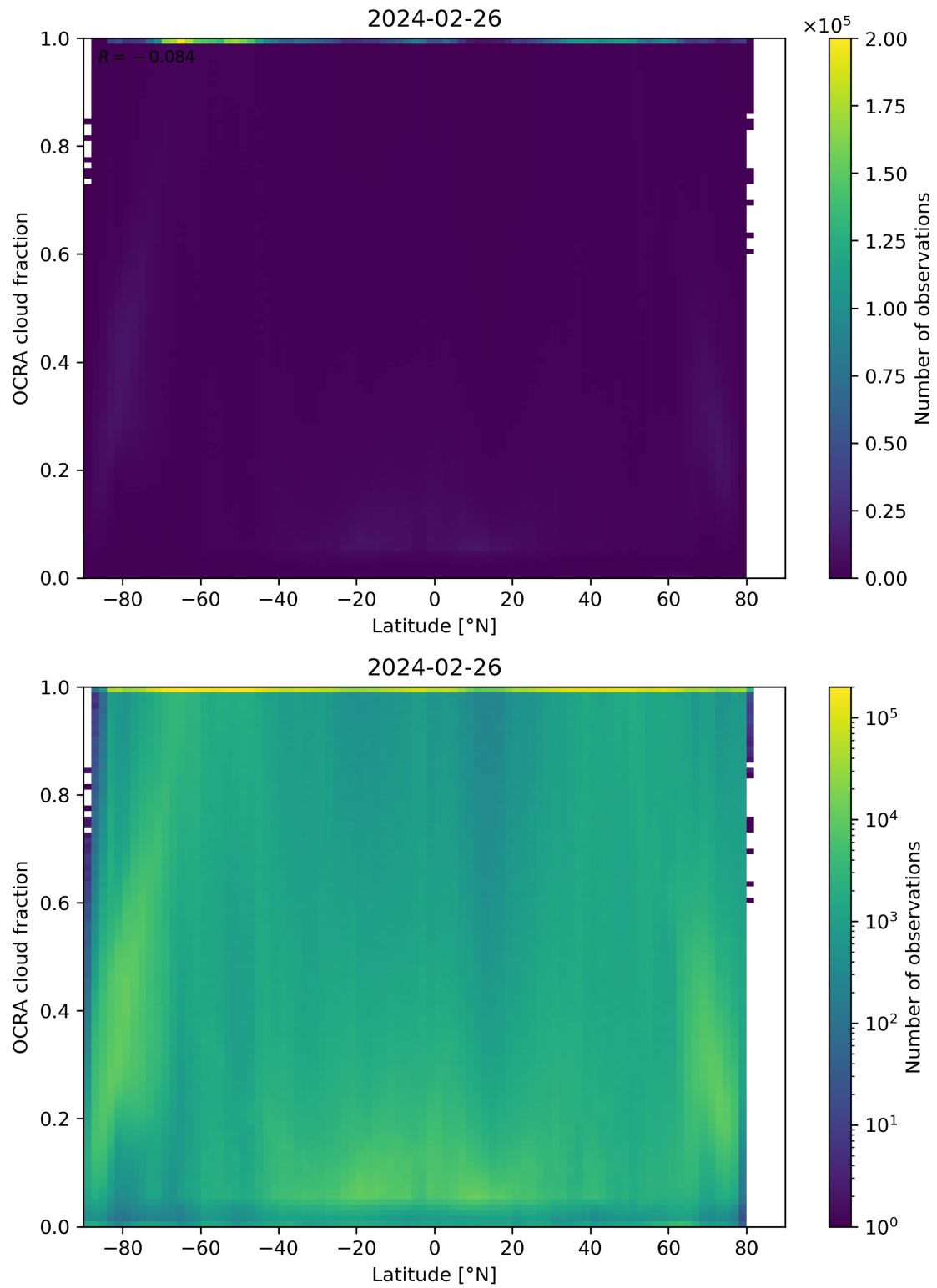
Figure 93: Scatter density plot of “Latitude” against “OCRA cloud fraction” for 2024-02-25 to 2024-02-27.
