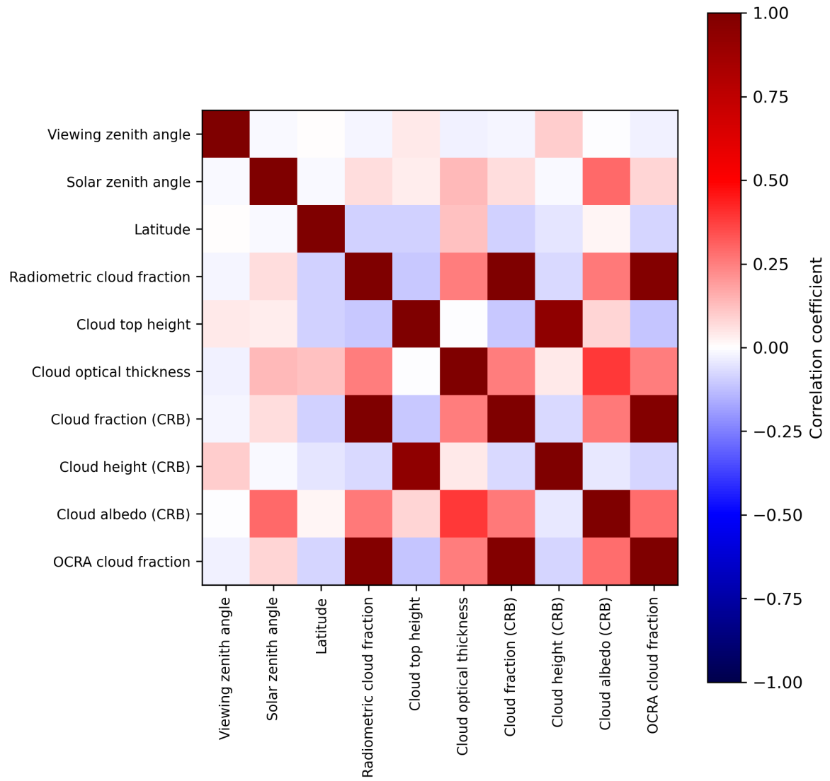
Figure 2: Map of correlation matrix for 2024-02-25 to 2024-02-27.
