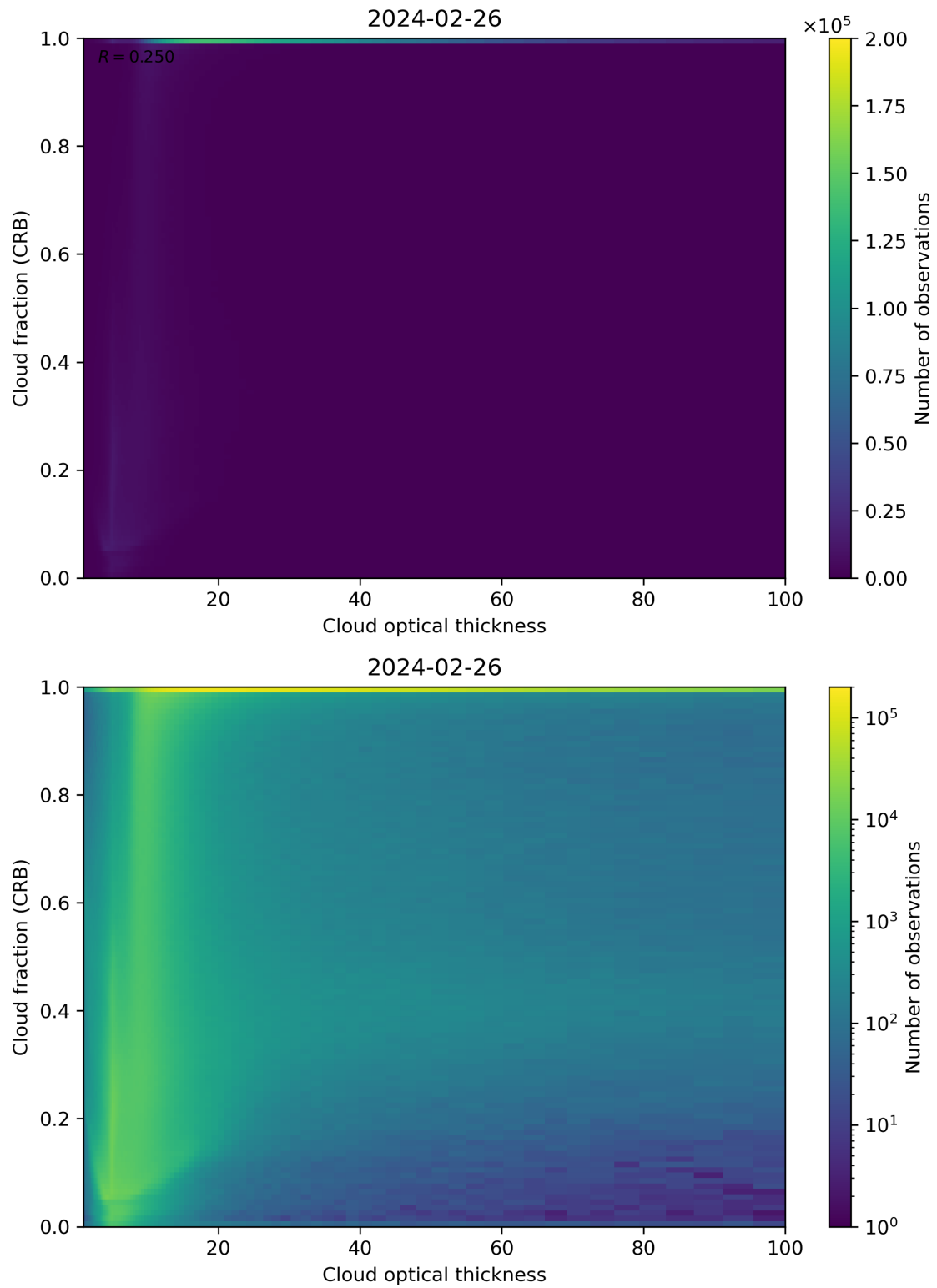
Figure 84: Scatter density plot of “Cloud optical thickness” against “Cloud fraction (CRB)” for 2024-02-25 to 2024-02-27.
