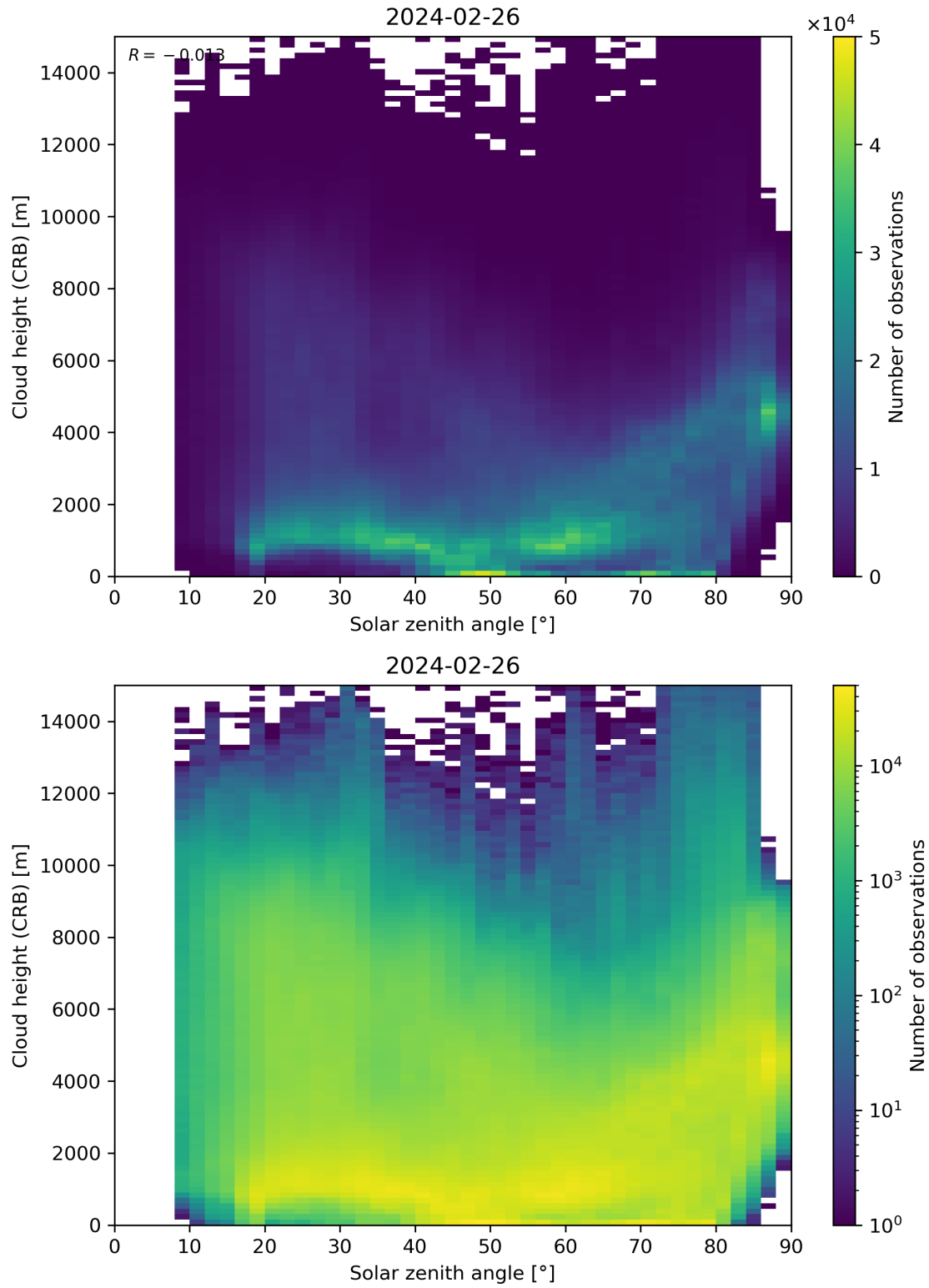
Figure 102: Scatter density plot of “Solar zenith angle” against “Cloud height (CRB)” for 2024-02-25 to 2024-02-27.
