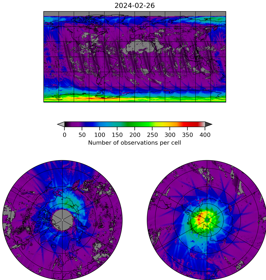
Figure 21: Map of the number of observations for 2024-02-25 to 2024-02-27
