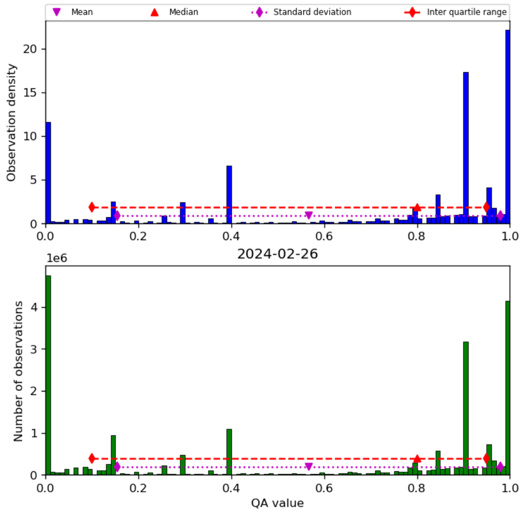
Figure 38: Histogram of “QA value” for 2024-02-25 to 2024-02-27
