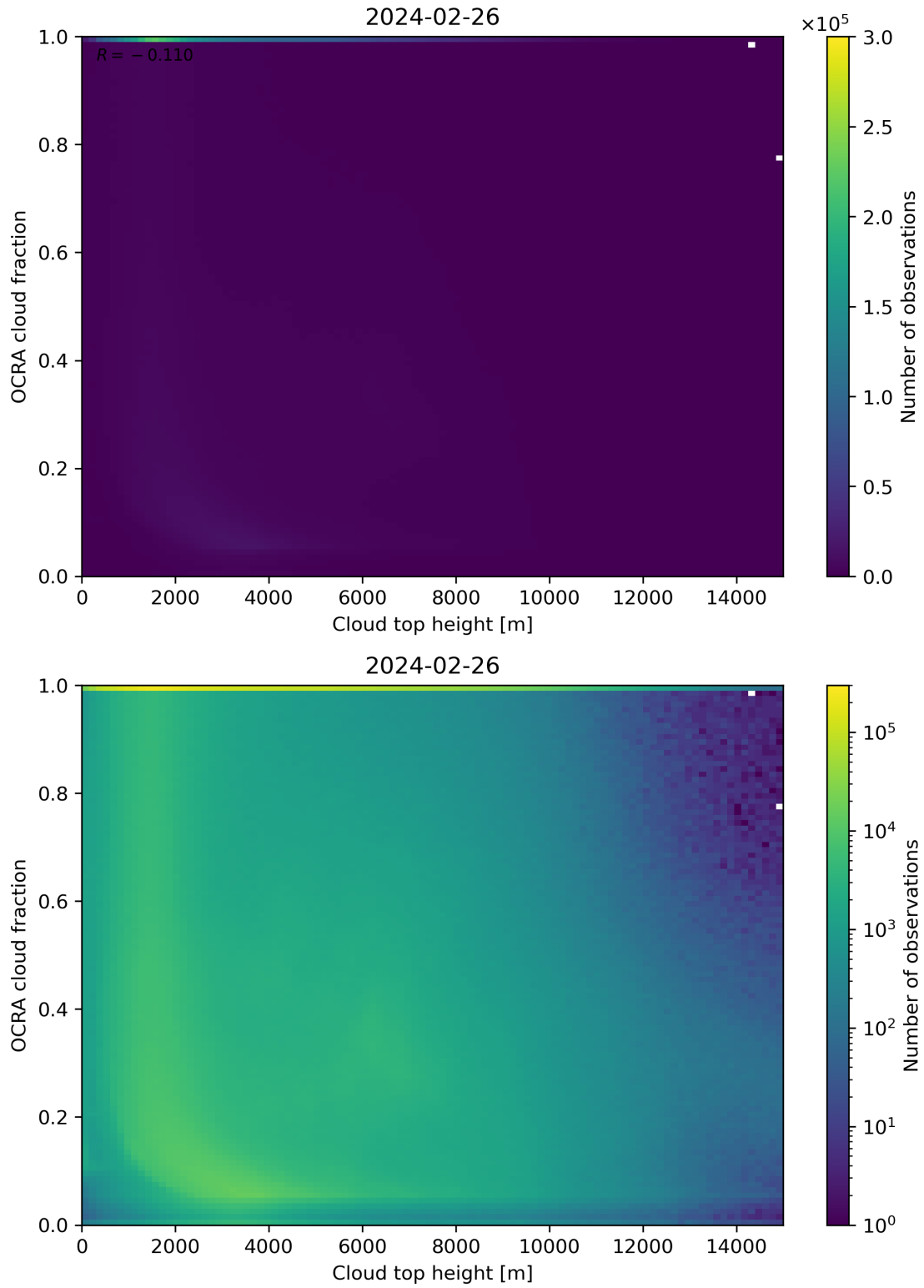
Figure 87: Scatter density plot of “Cloud top height” against “OCRA cloud fraction” for 2024-02-25 to 2024-02-27.
