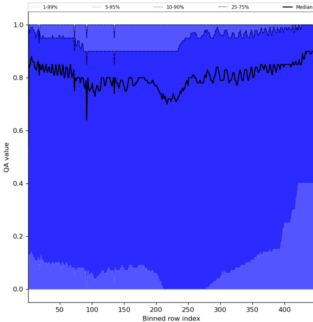
Figure 54: Along track statistics of “QA value” for 2024-02-25 to 2024-02-27
