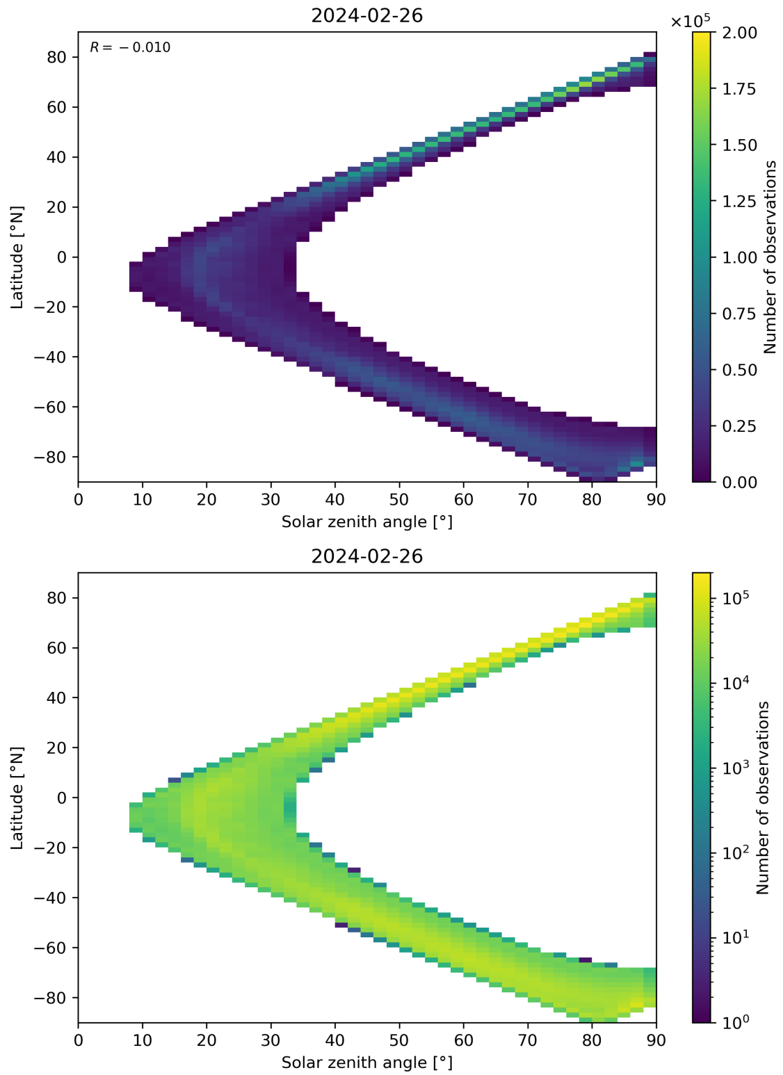
Figure 105: Scatter density plot of “Solar zenith angle” against “Latitude” for 2024-02-25 to 2024-02-27.
