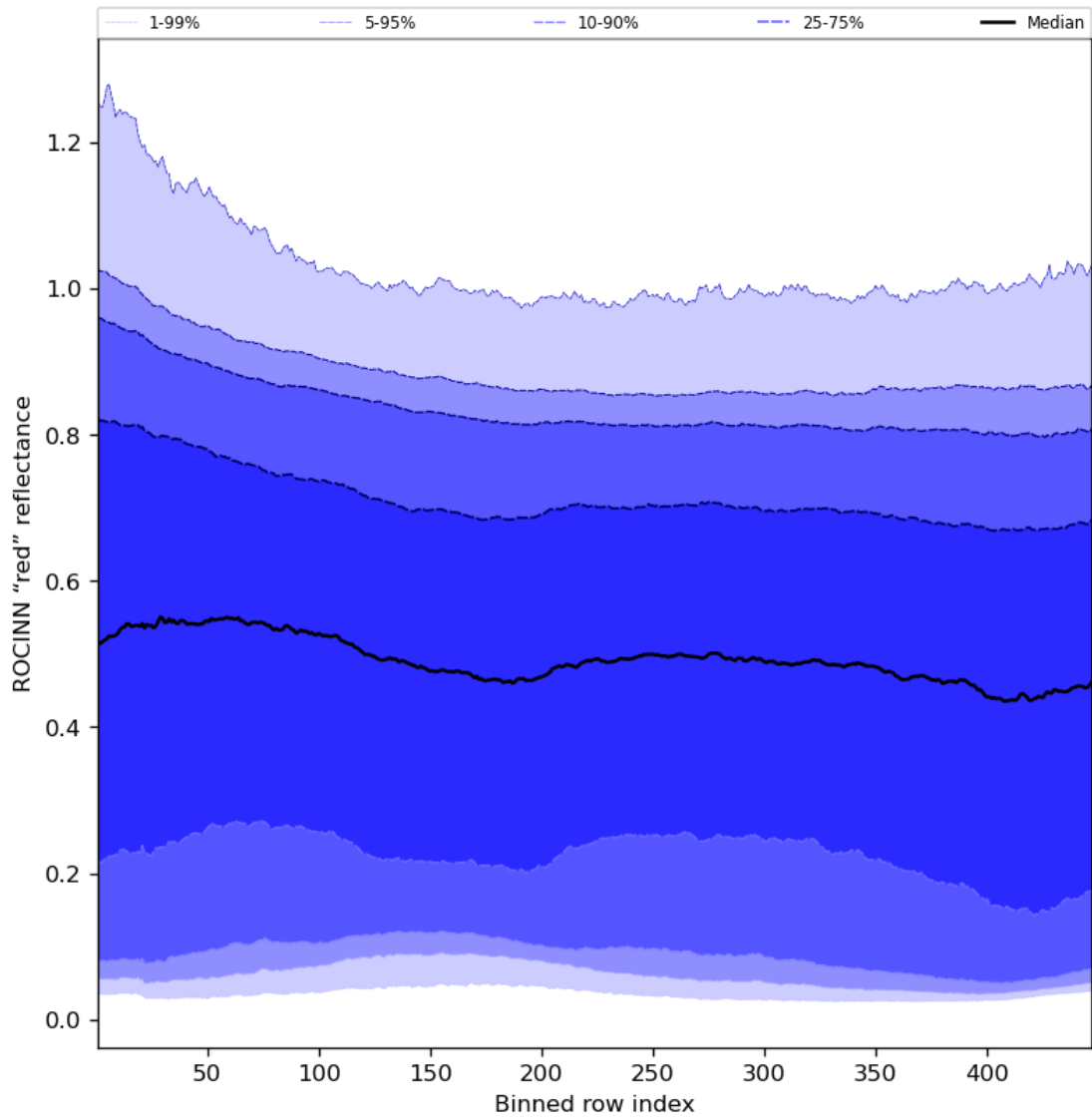
Figure 69: Along track statistics of “ROCINN “red” reflectance” for 2024-02-25 to 2024-02-27
