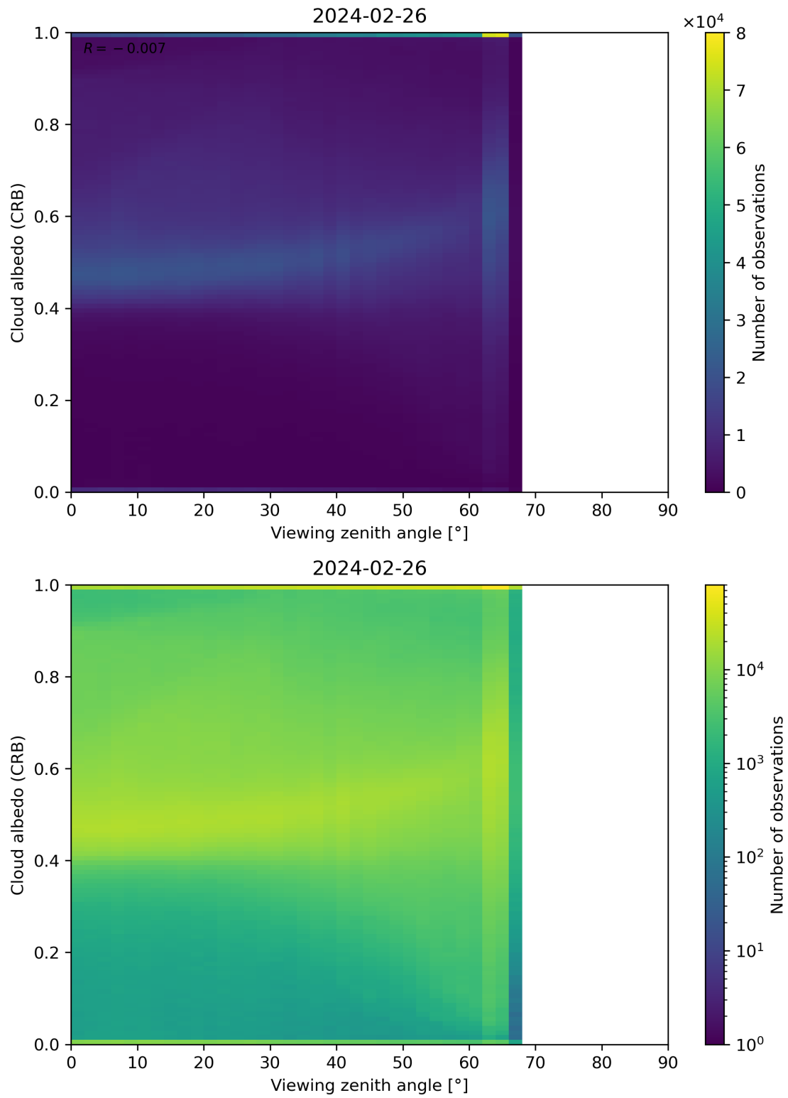
Figure 106: Scatter density plot of “Viewing zenith angle” against “Cloud albedo (CRB)” for 2024-02-25 to 2024-02-27.
