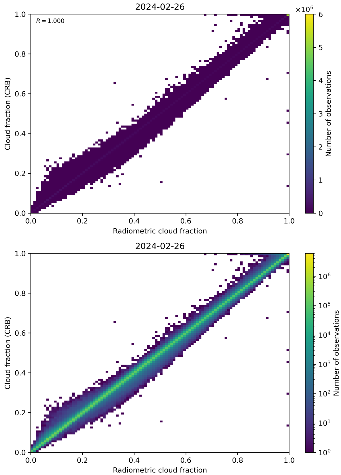
Figure 73: Scatter density plot of “Radiometric cloud fraction” against “Cloud fraction (CRB)” for 2024-02-25 to 2024-02-27.
