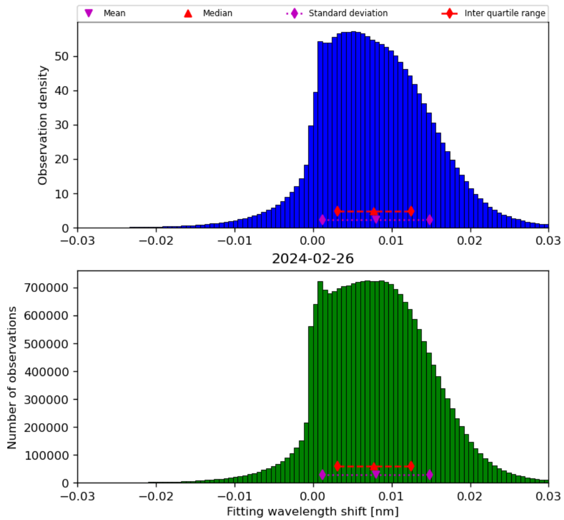
Figure 49: Histogram of “Fitting wavelength shift” for 2024-02-25 to 2024-02-27
