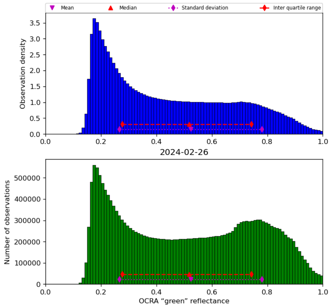
Figure 52: Histogram of “OCRA “green” reflectance” for 2024-02-25 to 2024-02-27
