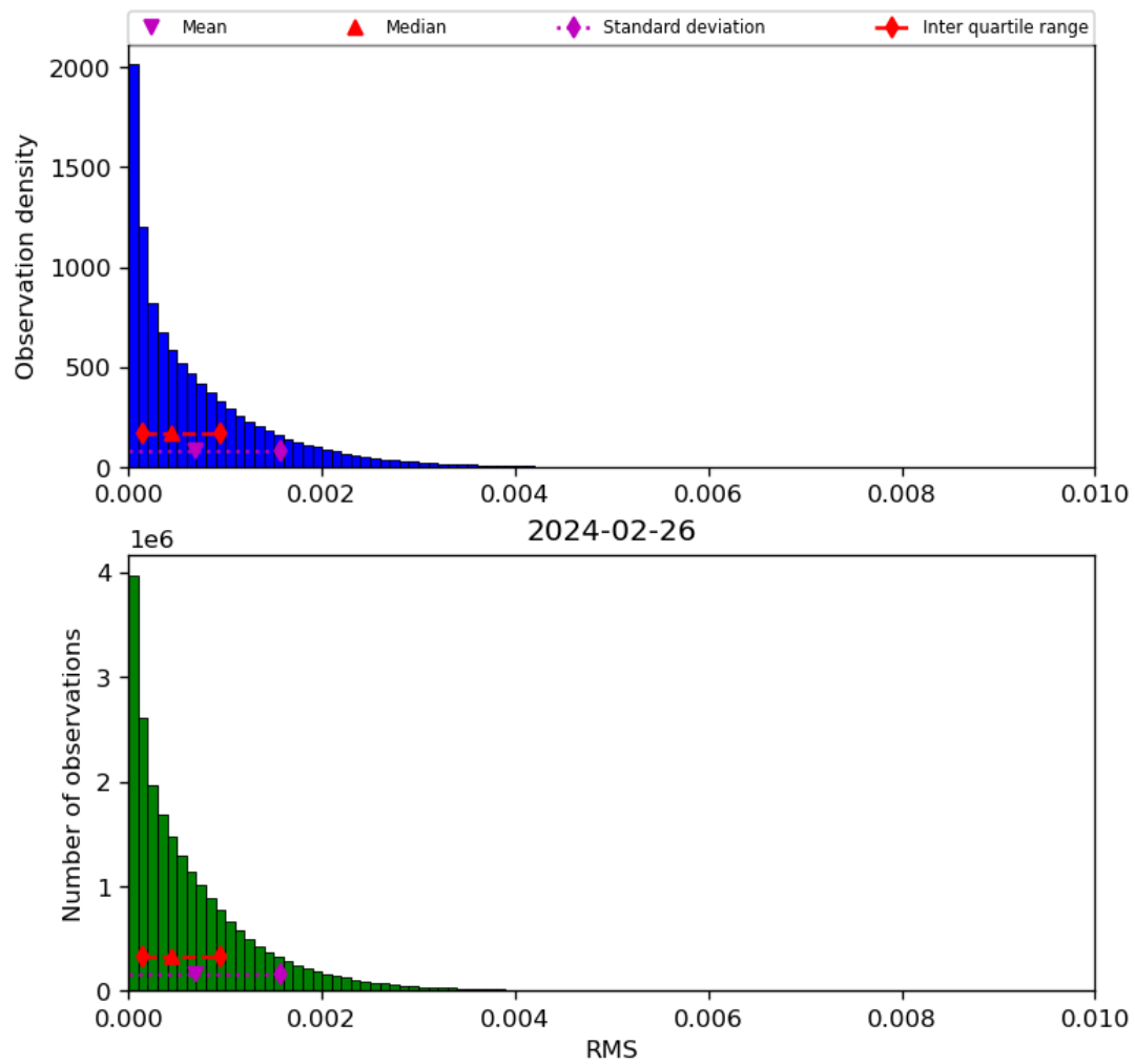
Figure 47: Histogram of “RMS” for 2024-02-25 to 2024-02-27
