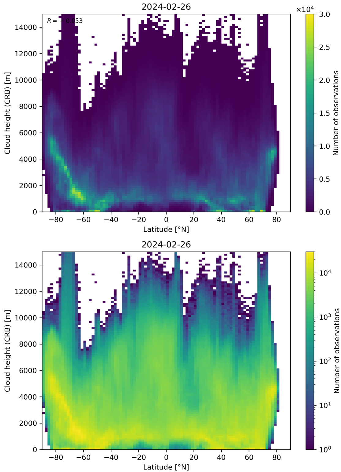
Figure 95: Scatter density plot of “Latitude” against “Cloud height (CRB)” for 2024-02-25 to 2024-02-27.
