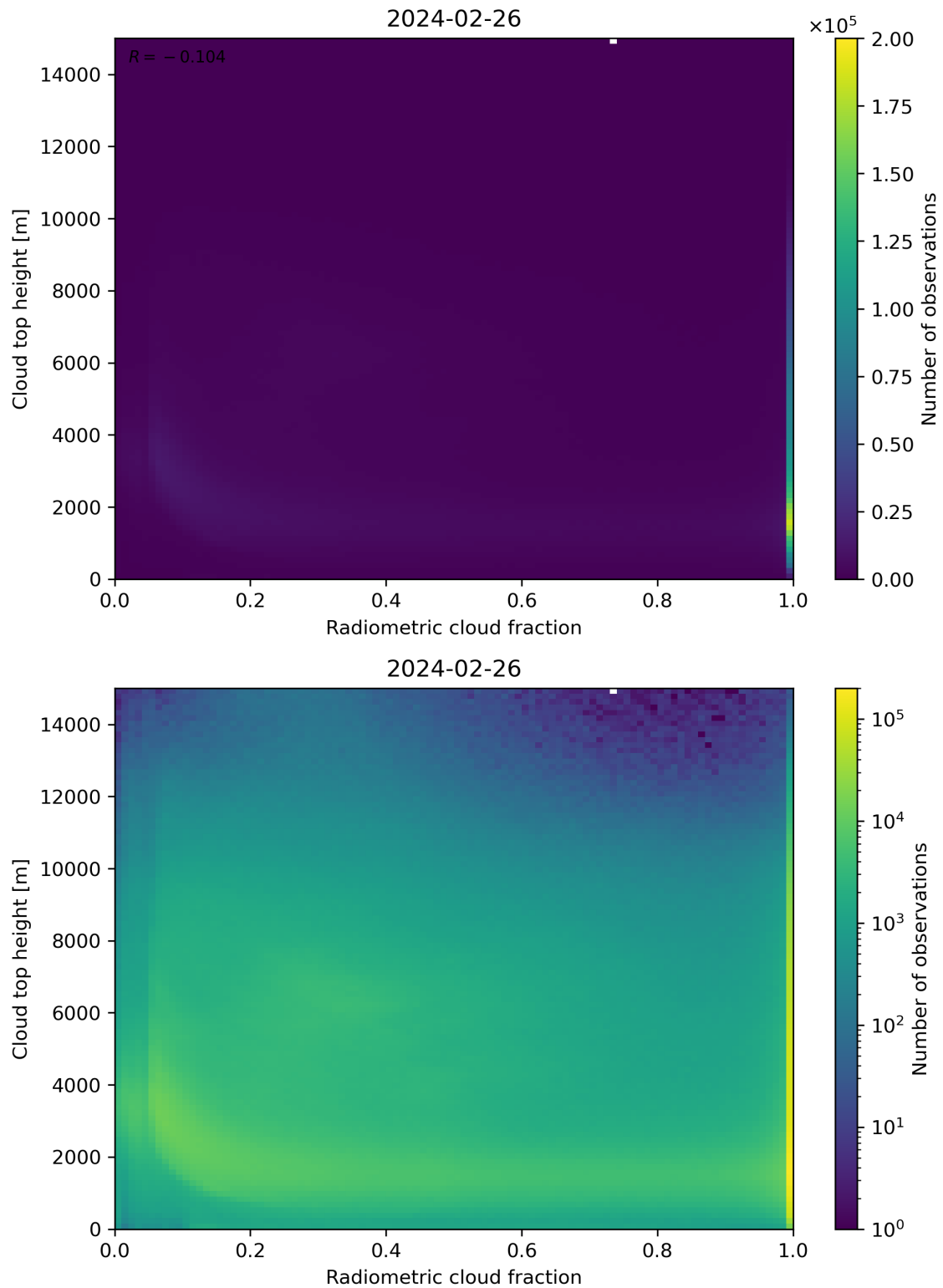
Figure 76: Scatter density plot of “Radiometric cloud fraction” against “Cloud top height” for 2024-02-25 to 2024-02-27.
