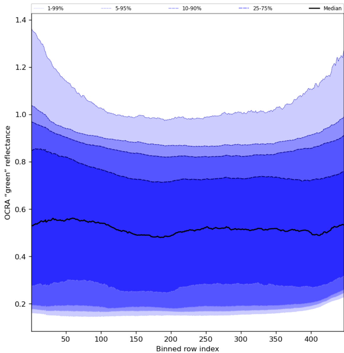
Figure 68: Along track statistics of “OCRA “green” reflectance” for 2024-02-25 to 2024-02-27
