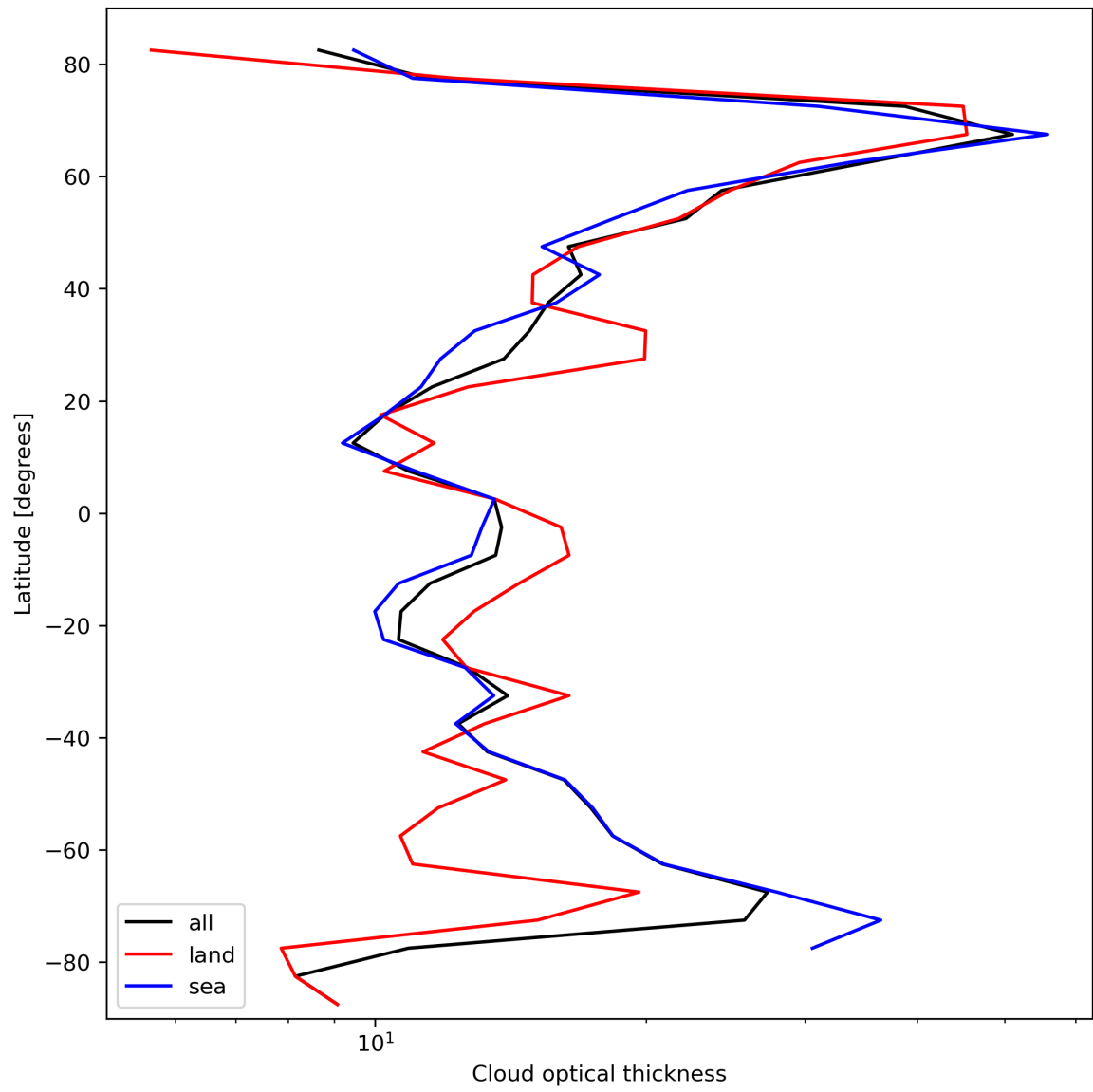
Figure 25: Zonal average of “Cloud optical thickness” for 2024-02-25 to 2024-02-27.
