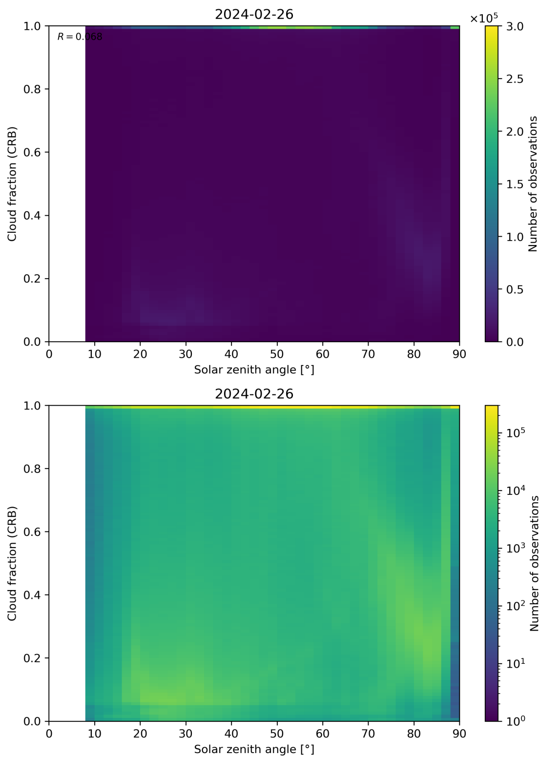
Figure 101: Scatter density plot of “Solar zenith angle” against “Cloud fraction (CRB)” for 2024-02-25 to 2024-02-27.
