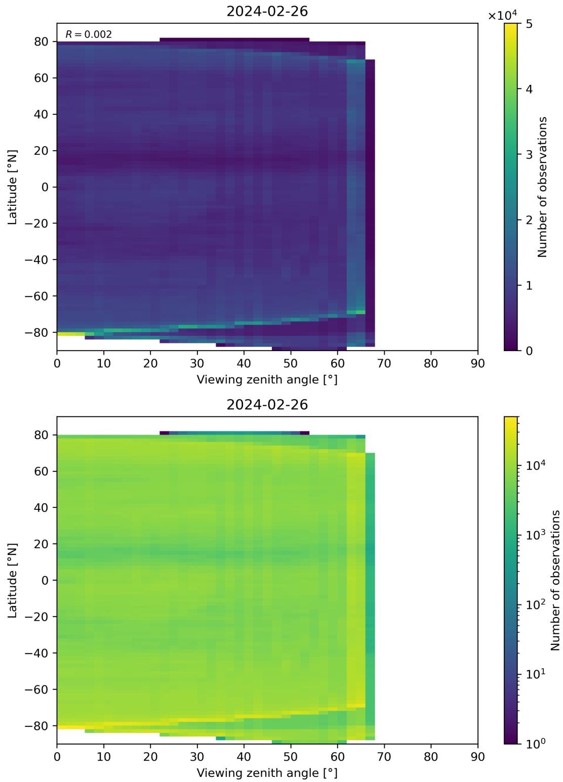
Figure 113: Scatter density plot of “Viewing zenith angle” against “Latitude” for 2024-02-25 to 2024-02-27.
