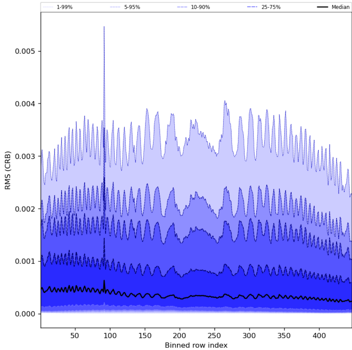
Figure 64: Along track statistics of “RMS (CRB)” for 2024-02-25 to 2024-02-27
