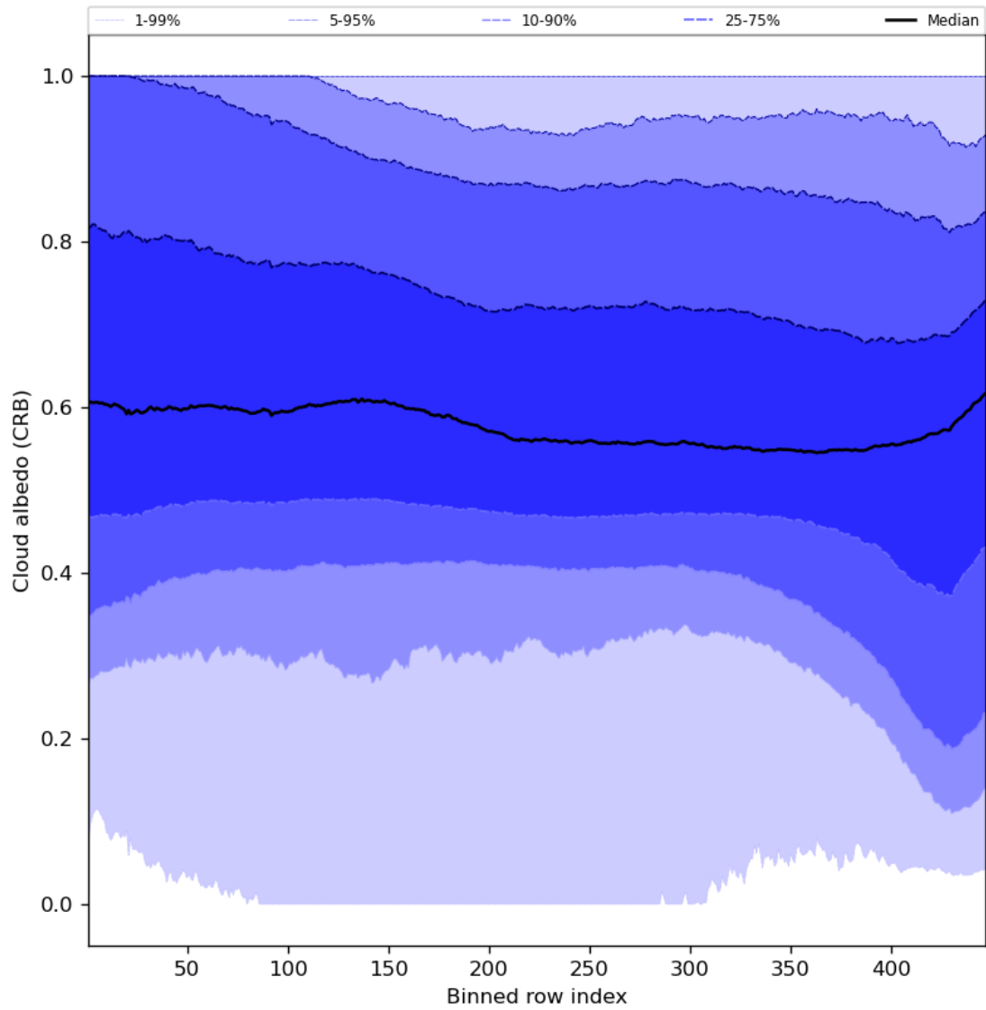
Figure 60: Along track statistics of “Cloud albedo (CRB)” for 2024-02-25 to 2024-02-27
