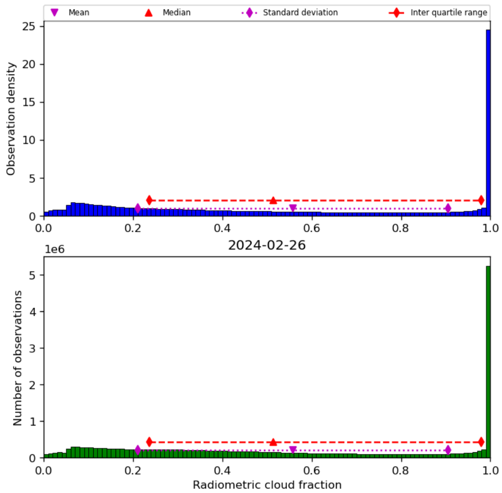
Figure 39: Histogram of “Radiometric cloud fraction” for 2024-02-25 to 2024-02-27
