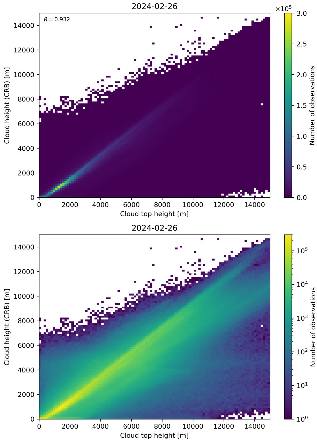
Figure 89: Scatter density plot of “Cloud top height” against “Cloud height (CRB)” for 2024-02-25 to 2024-02-27.
