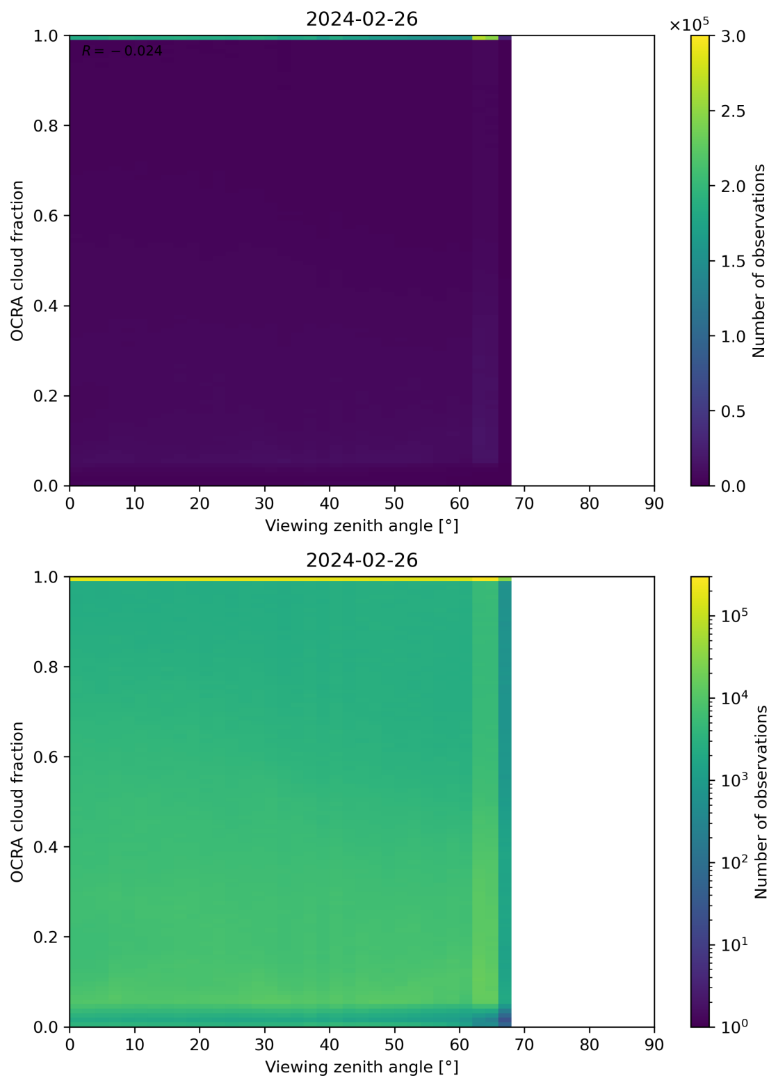
Figure 108: Scatter density plot of “Viewing zenith angle” against “OCRA cloud fraction” for 2024-02-25 to 2024-02-27.
