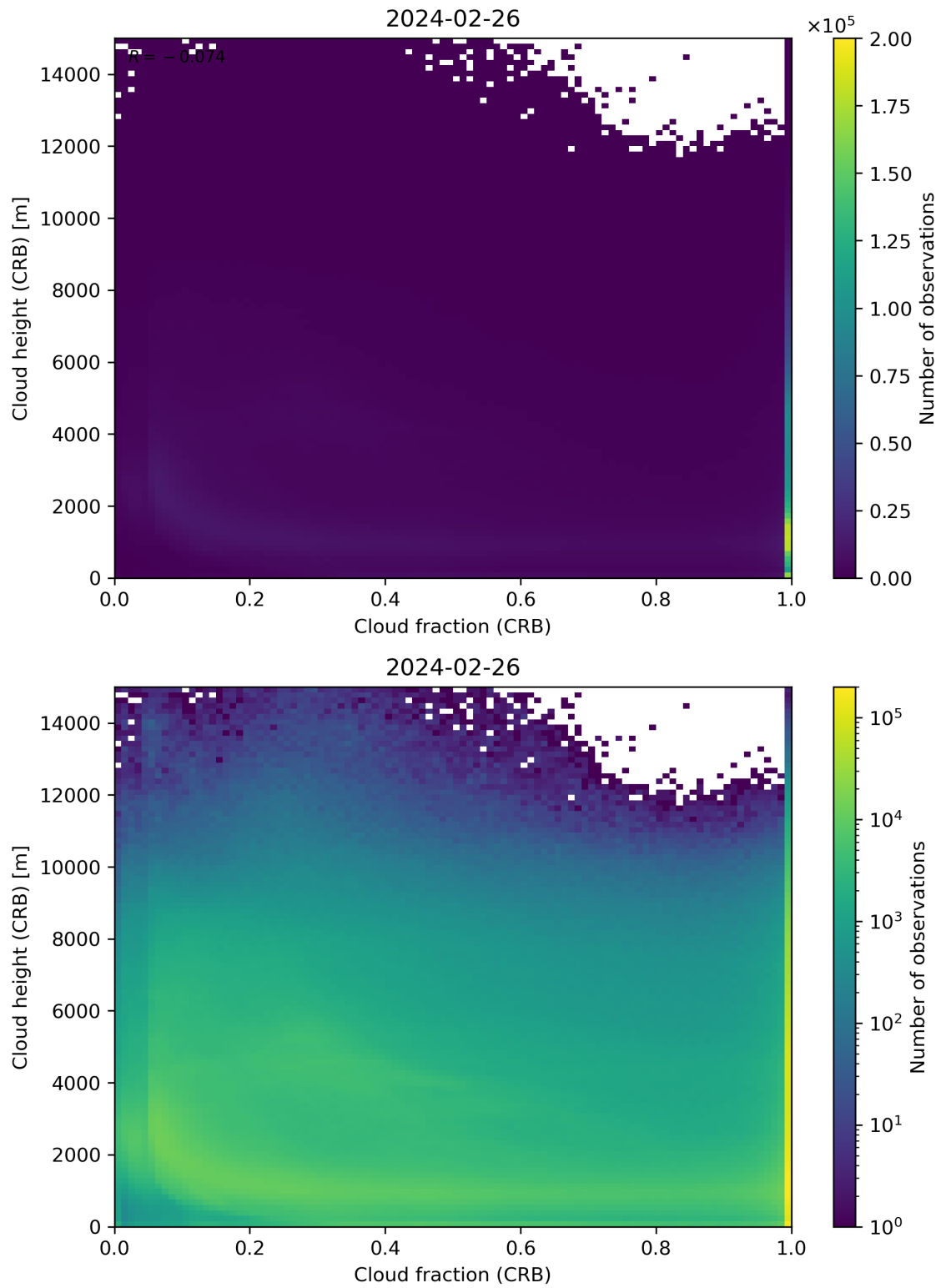
Figure 79: Scatter density plot of “Cloud fraction (CRB)” against “Cloud height (CRB)” for 2024-02-25 to 2024-02-27.
