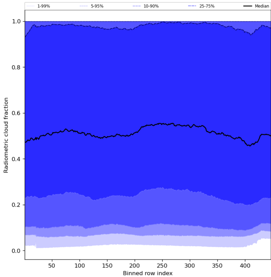
Figure 55: Along track statistics of “Radiometric cloud fraction” for 2024-02-25 to 2024-02-27
