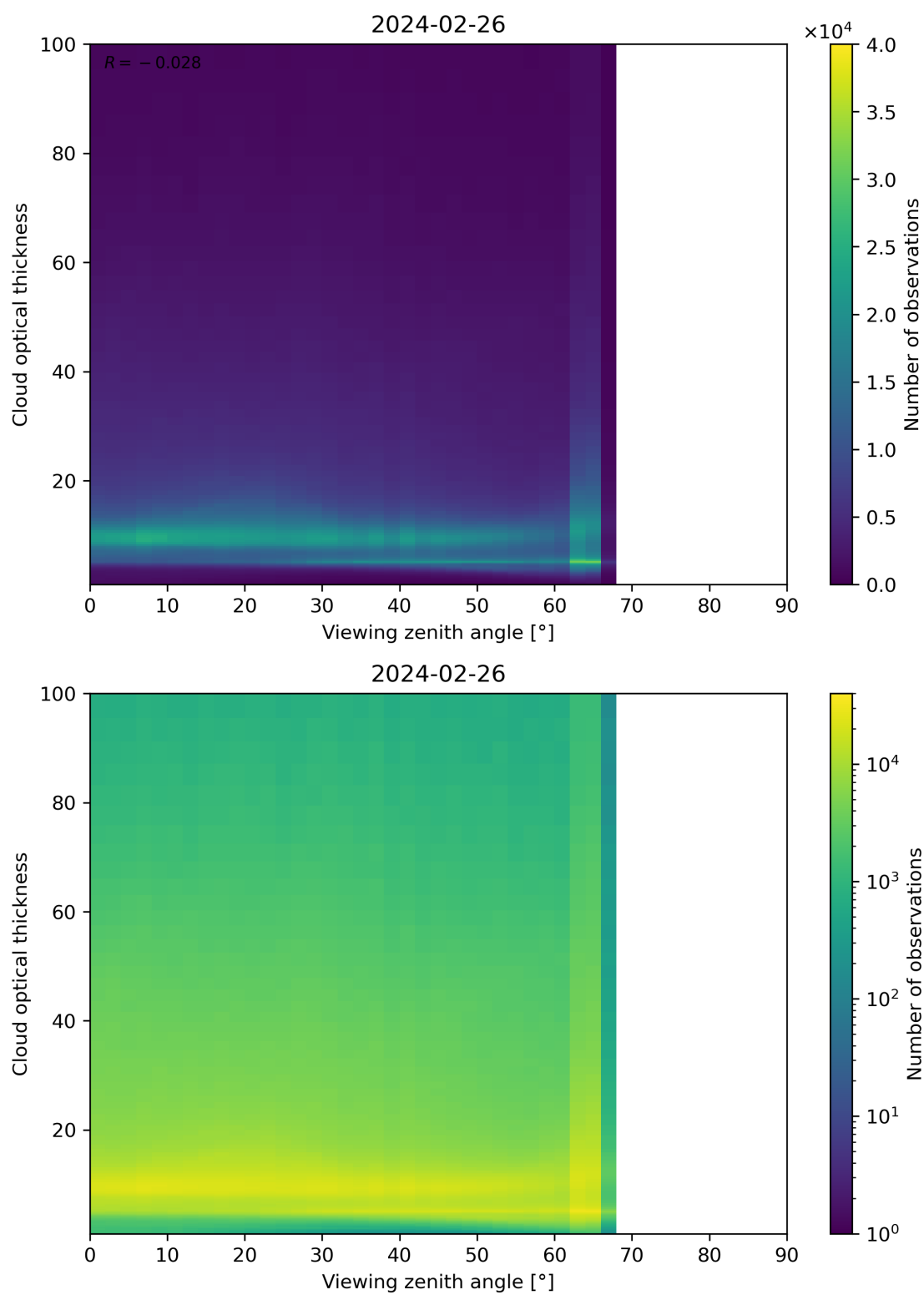
Figure 111: Scatter density plot of “Viewing zenith angle” against “Cloud optical thickness” for 2024-02-25 to 2024-02-27.
