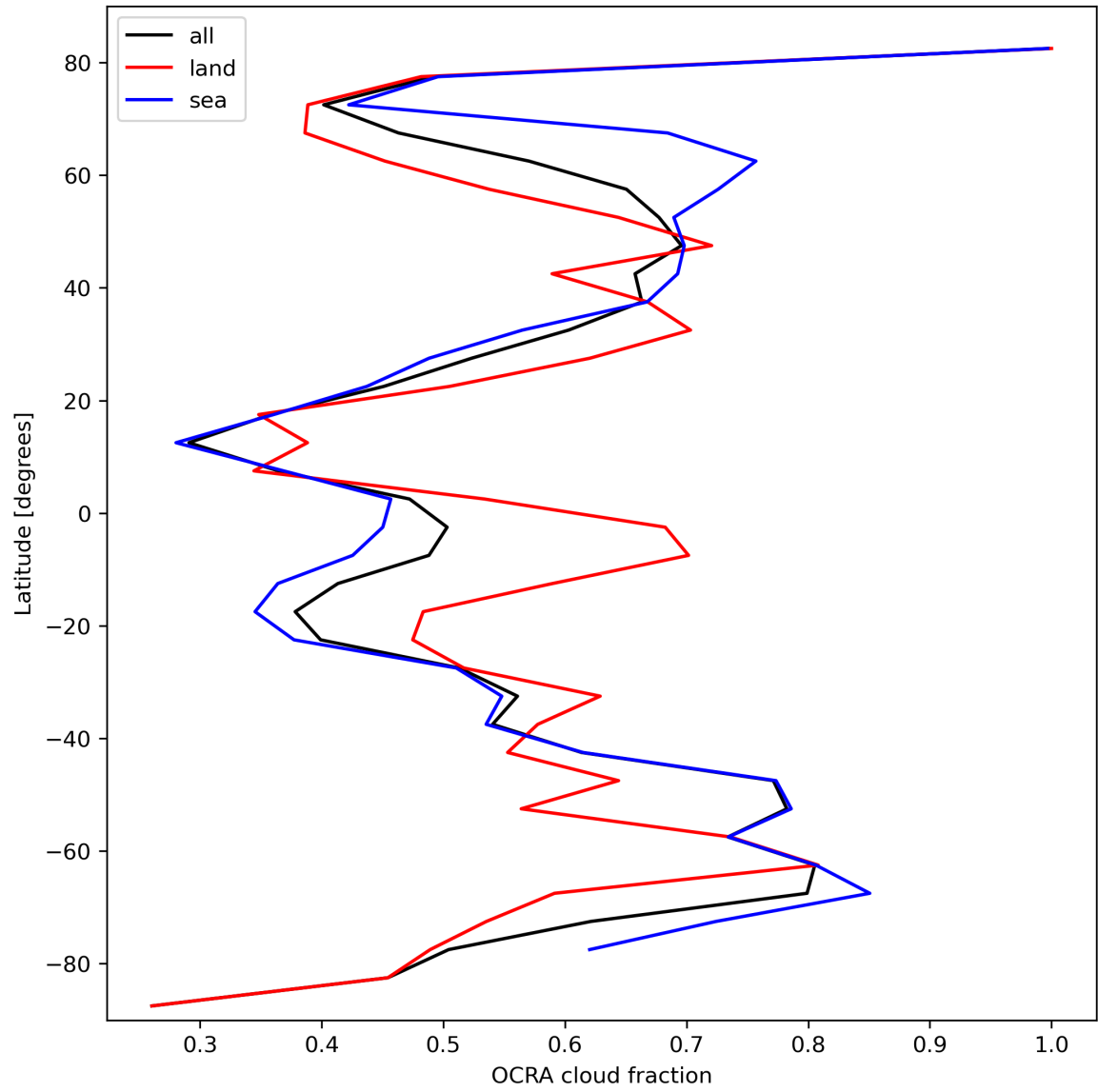
Figure 34: Zonal average of “OCRA cloud fraction” for 2024-02-25 to 2024-02-27.
