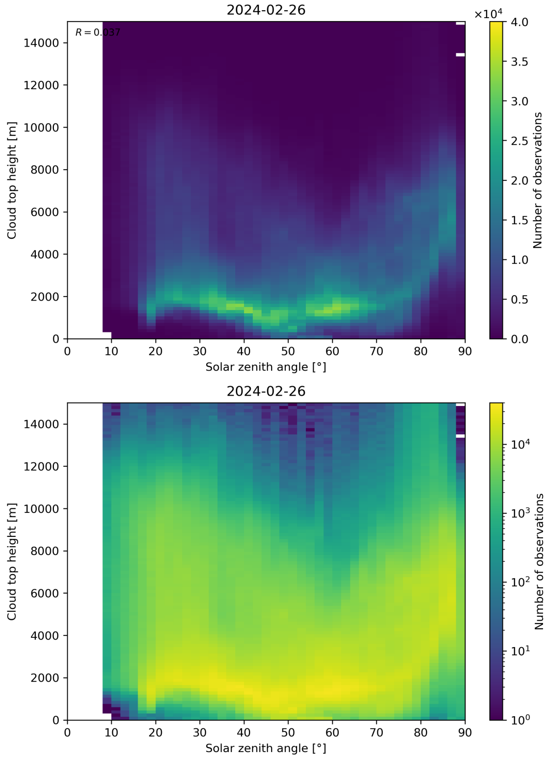
Figure 104: Scatter density plot of “Solar zenith angle” against “Cloud top height” for 2024-02-25 to 2024-02-27.
