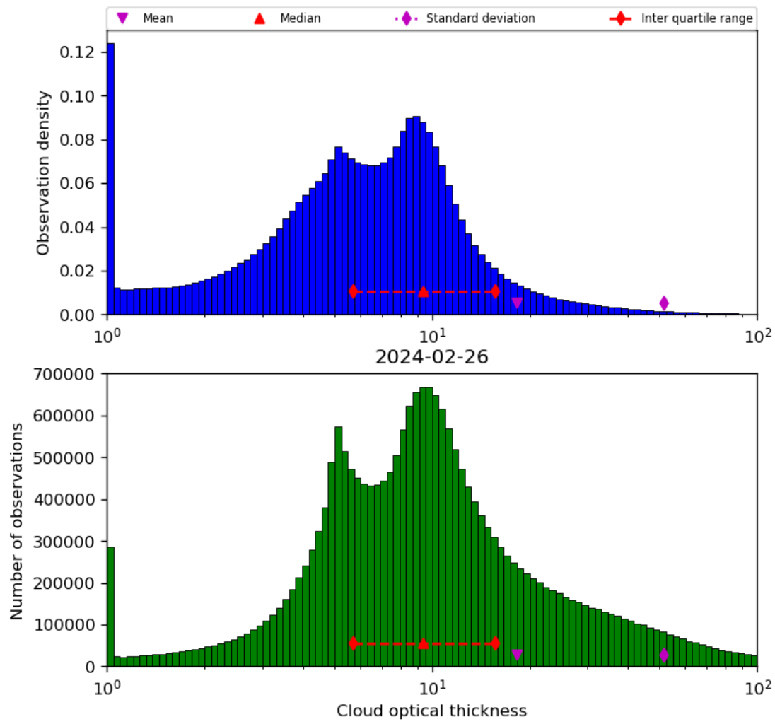
Figure 41: Histogram of “Cloud optical thickness” for 2024-02-25 to 2024-02-27
