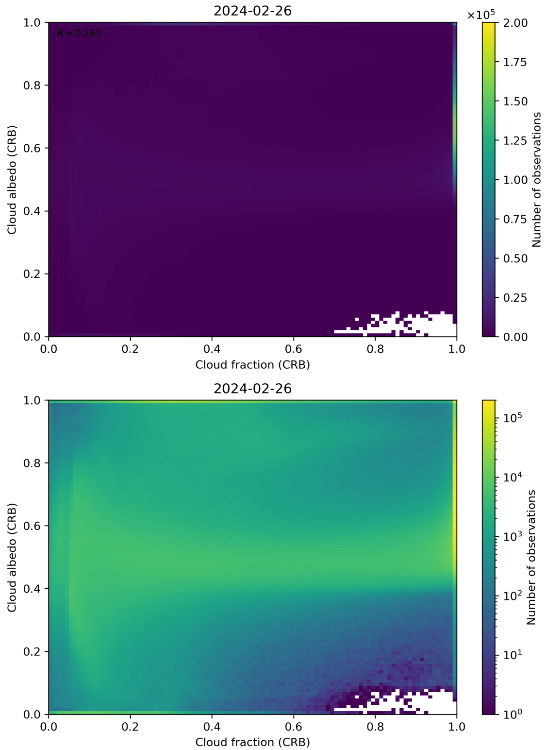
Figure 77: Scatter density plot of “Cloud fraction (CRB)” against “Cloud albedo (CRB)” for 2024-02-25 to 2024-02-27.
