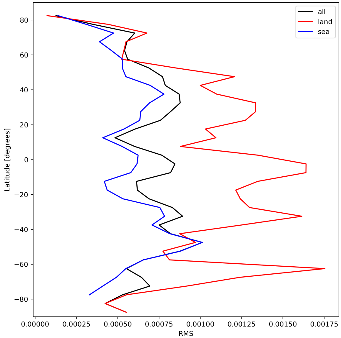
Figure 31: Zonal average of “RMS” for 2024-02-25 to 2024-02-27.
