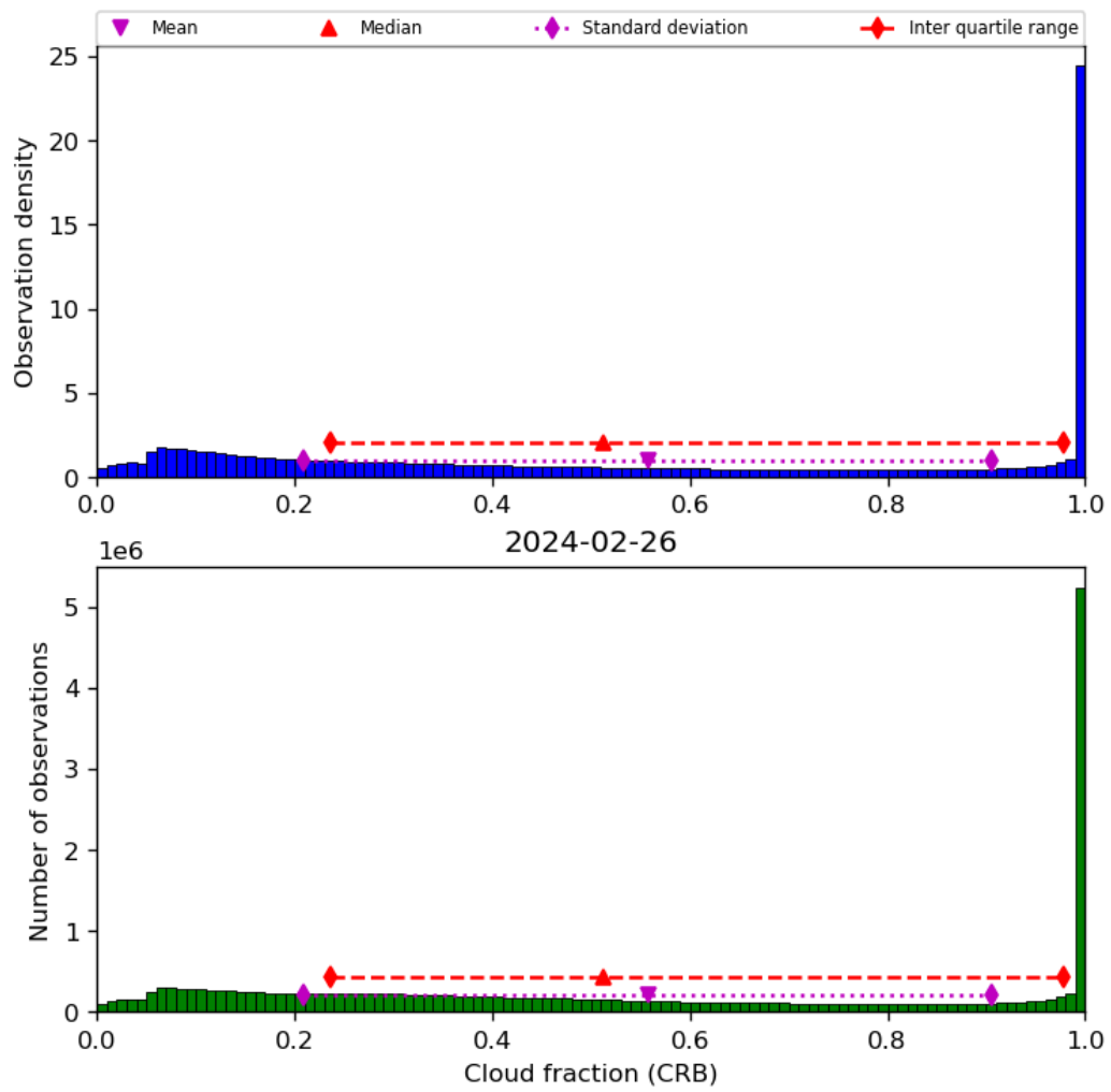
Figure 42: Histogram of “Cloud fraction (CRB)” for 2024-02-25 to 2024-02-27
