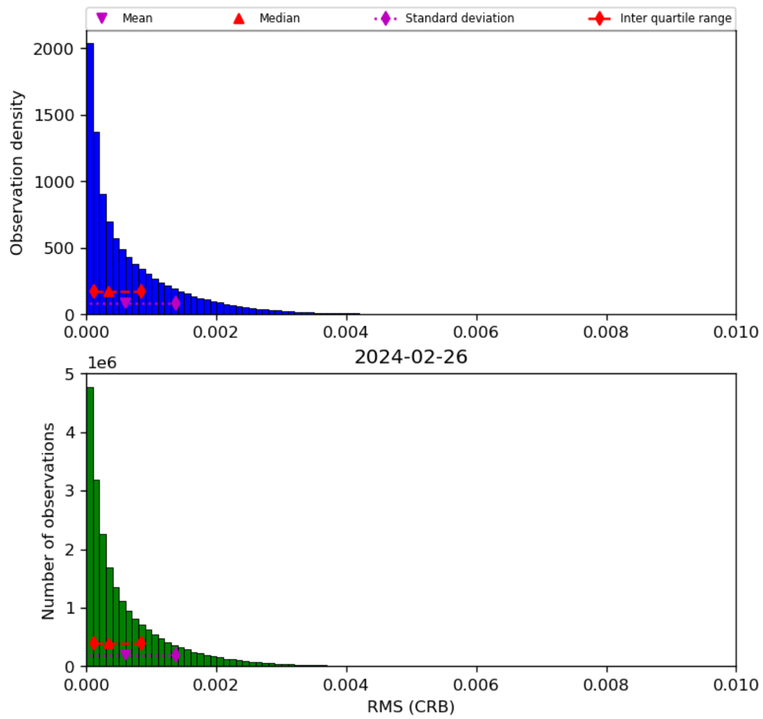
Figure 48: Histogram of “RMS (CRB)” for 2024-02-25 to 2024-02-27
