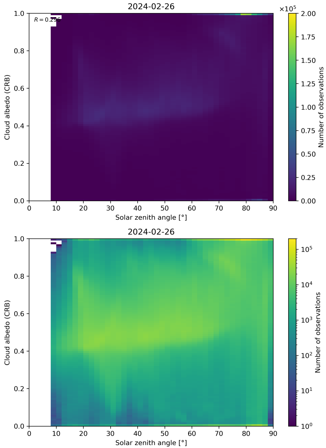
Figure 98: Scatter density plot of “Solar zenith angle” against “Cloud albedo (CRB)” for 2024-02-25 to 2024-02-27.
