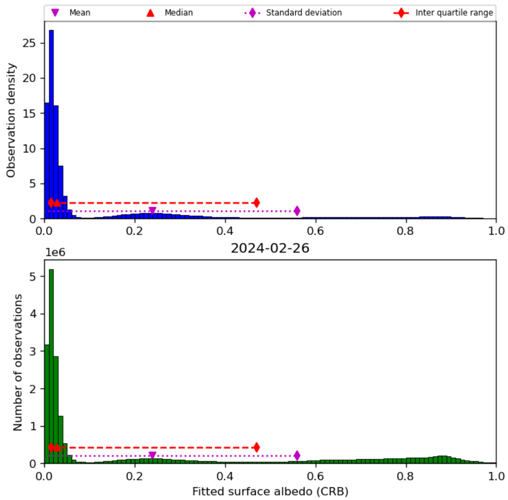
Figure 46: Histogram of “Fitted surface albedo (CRB)” for 2024-02-25 to 2024-02-27
