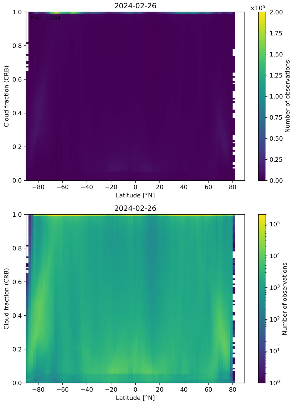
Figure 94: Scatter density plot of “Latitude” against “Cloud fraction (CRB)” for 2024-02-25 to 2024-02-27.
