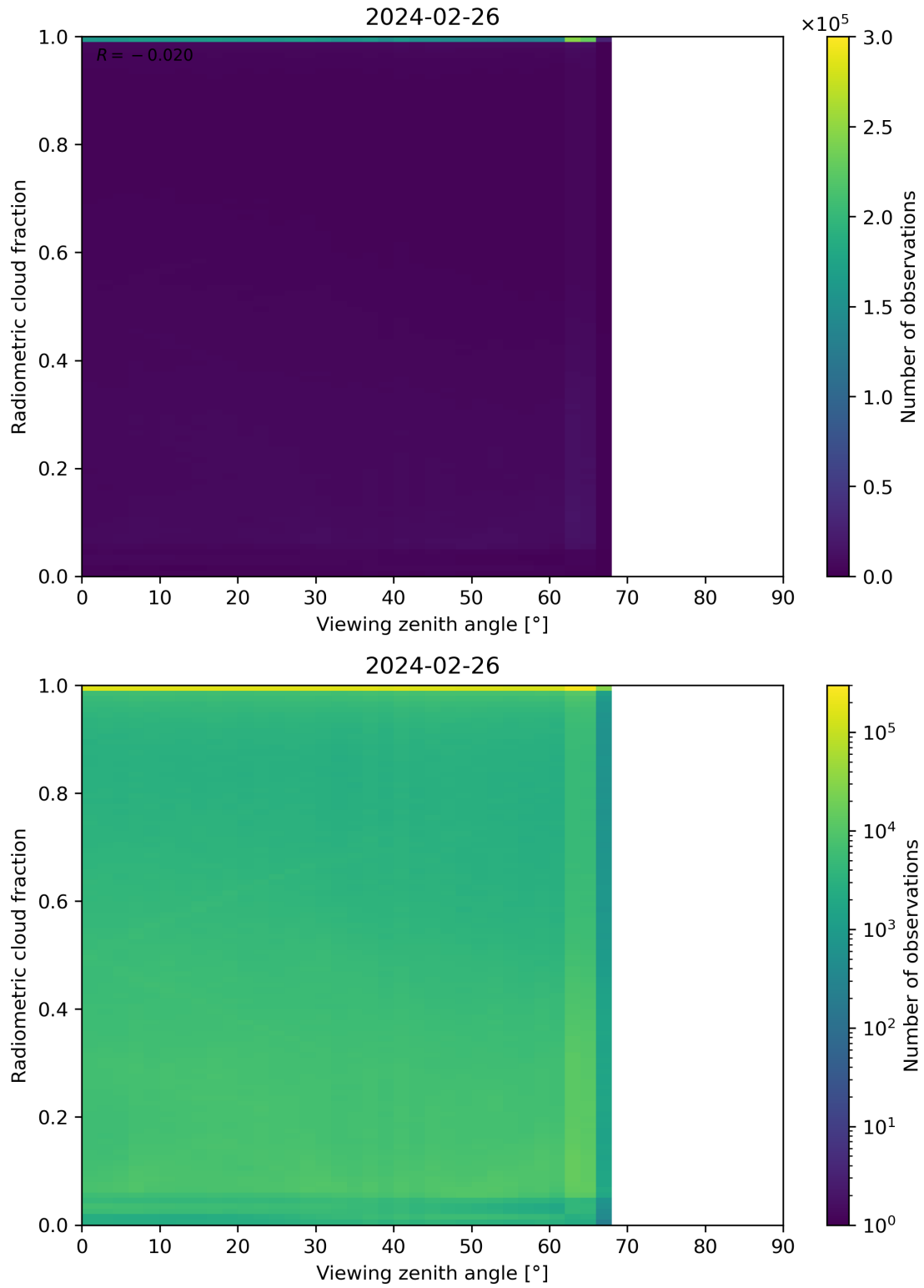
Figure 107: Scatter density plot of “Viewing zenith angle” against “Radiometric cloud fraction” for 2024-02-25 to 2024-02-27.
