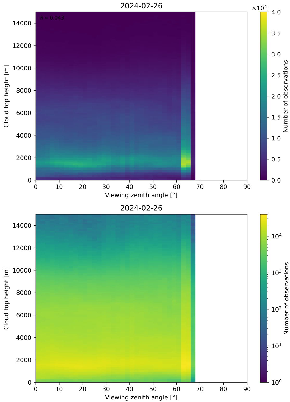
Figure 112: Scatter density plot of “Viewing zenith angle” against “Cloud top height” for 2024-02-25 to 2024-02-27.
