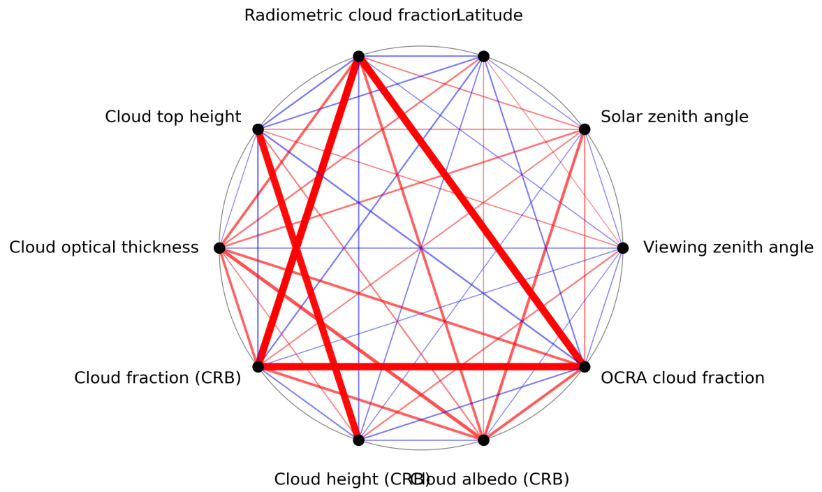
Figure 1: Map of correlation graph for 2024-02-25 to 2024-02-27.
