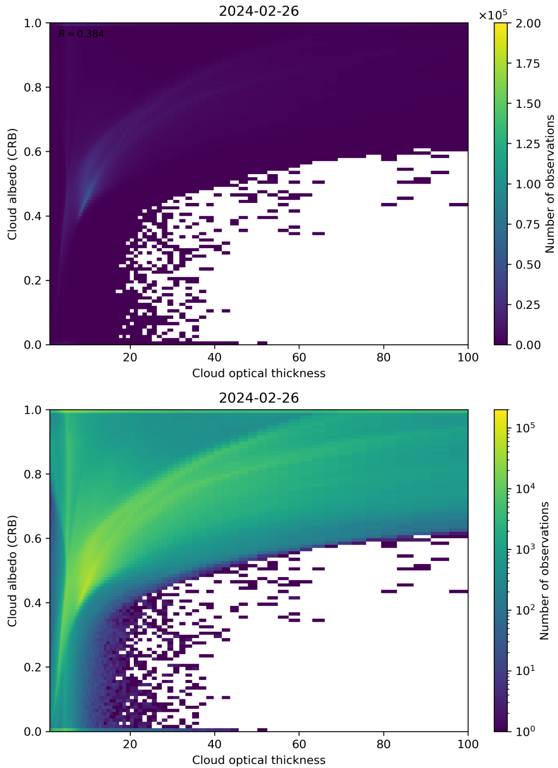
Figure 82: Scatter density plot of “Cloud optical thickness” against “Cloud albedo (CRB)” for 2024-02-25 to 2024-02-27.
