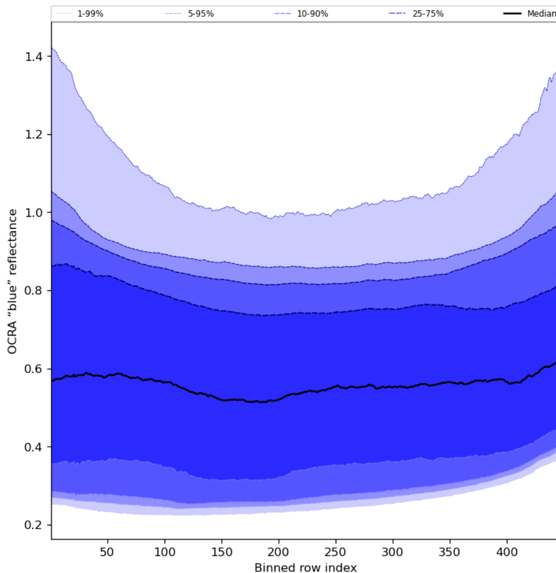
Figure 67: Along track statistics of "OCRA "blue" reflectance" for 2024-02-25 to 2024-02-27
