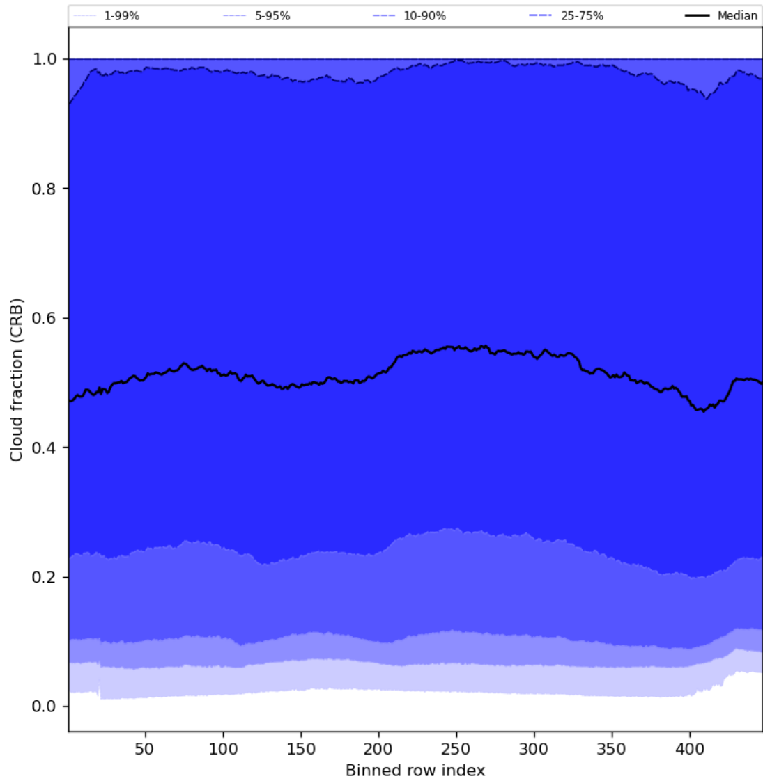
Figure 58: Along track statistics of “Cloud fraction (CRB)” for 2024-02-25 to 2024-02-27
