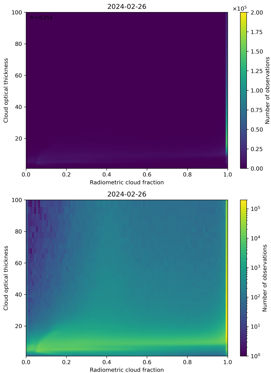
Figure 75: Scatter density plot of “Radiometric cloud fraction” against “Cloud optical thickness” for 2024-02-25 to 2024-02-27.
