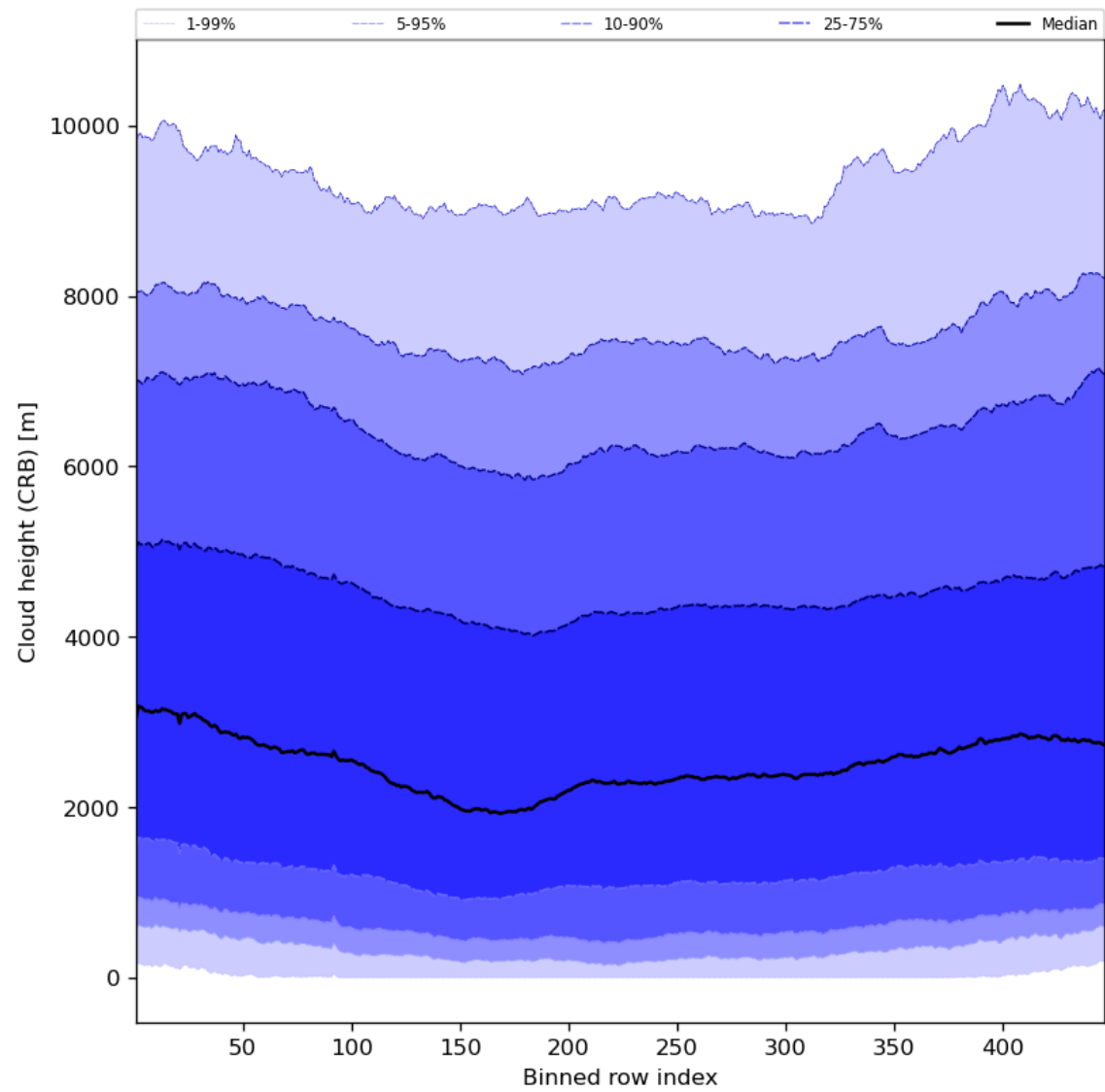
Figure 59: Along track statistics of “Cloud height (CRB)” for 2024-02-25 to 2024-02-27
