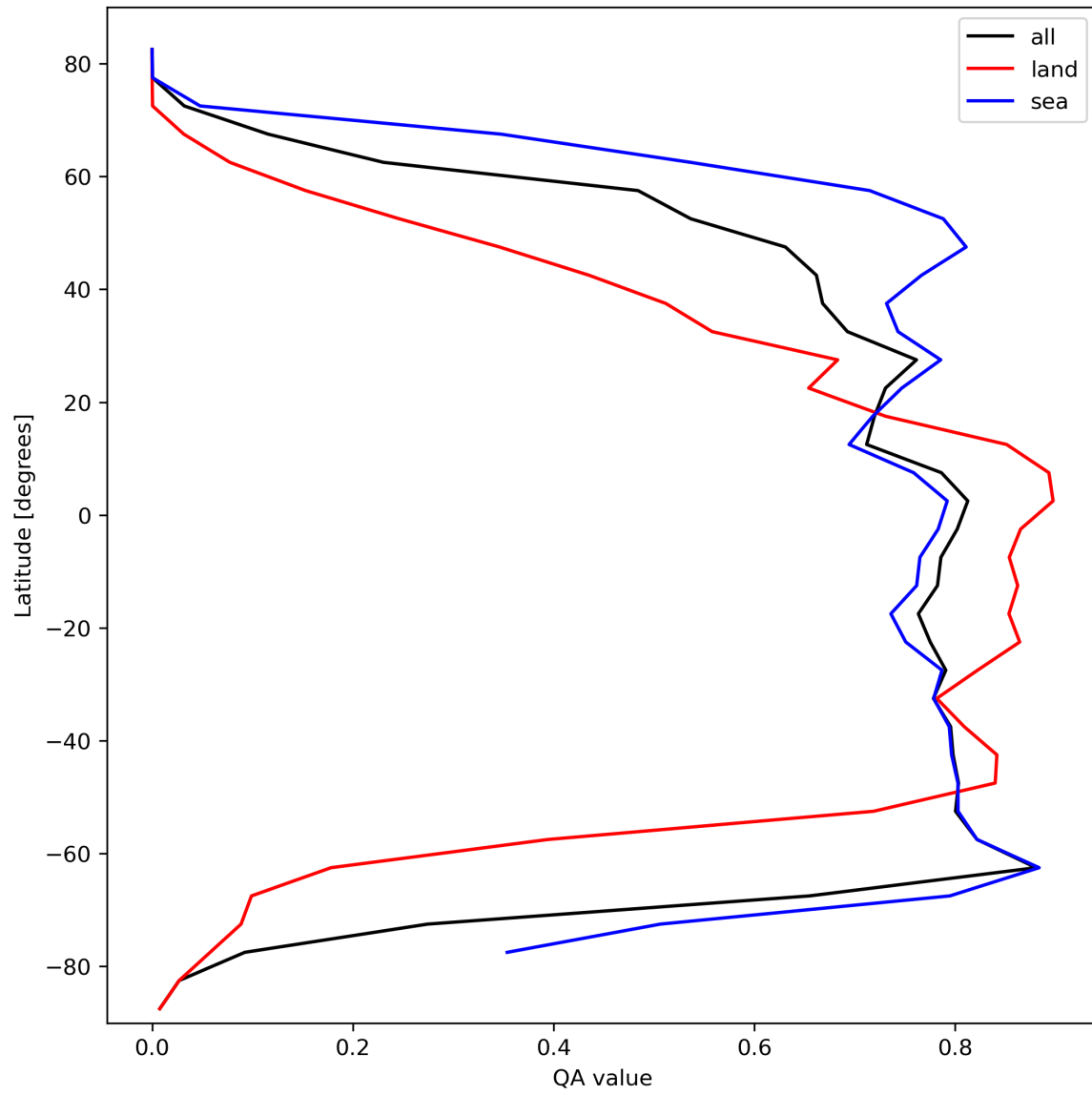
Figure 22: Zonal average of “QA value” for 2024-02-25 to 2024-02-27.
