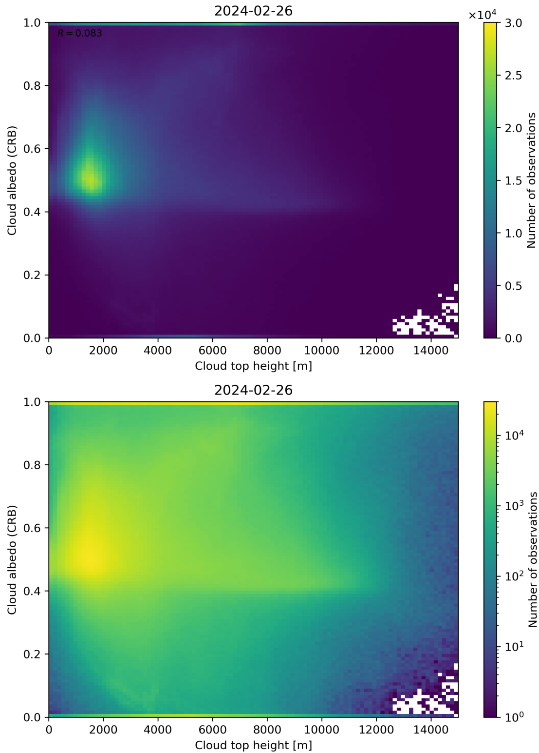
Figure 86: Scatter density plot of “Cloud top height” against “Cloud albedo (CRB)” for 2024-02-25 to 2024-02-27.
