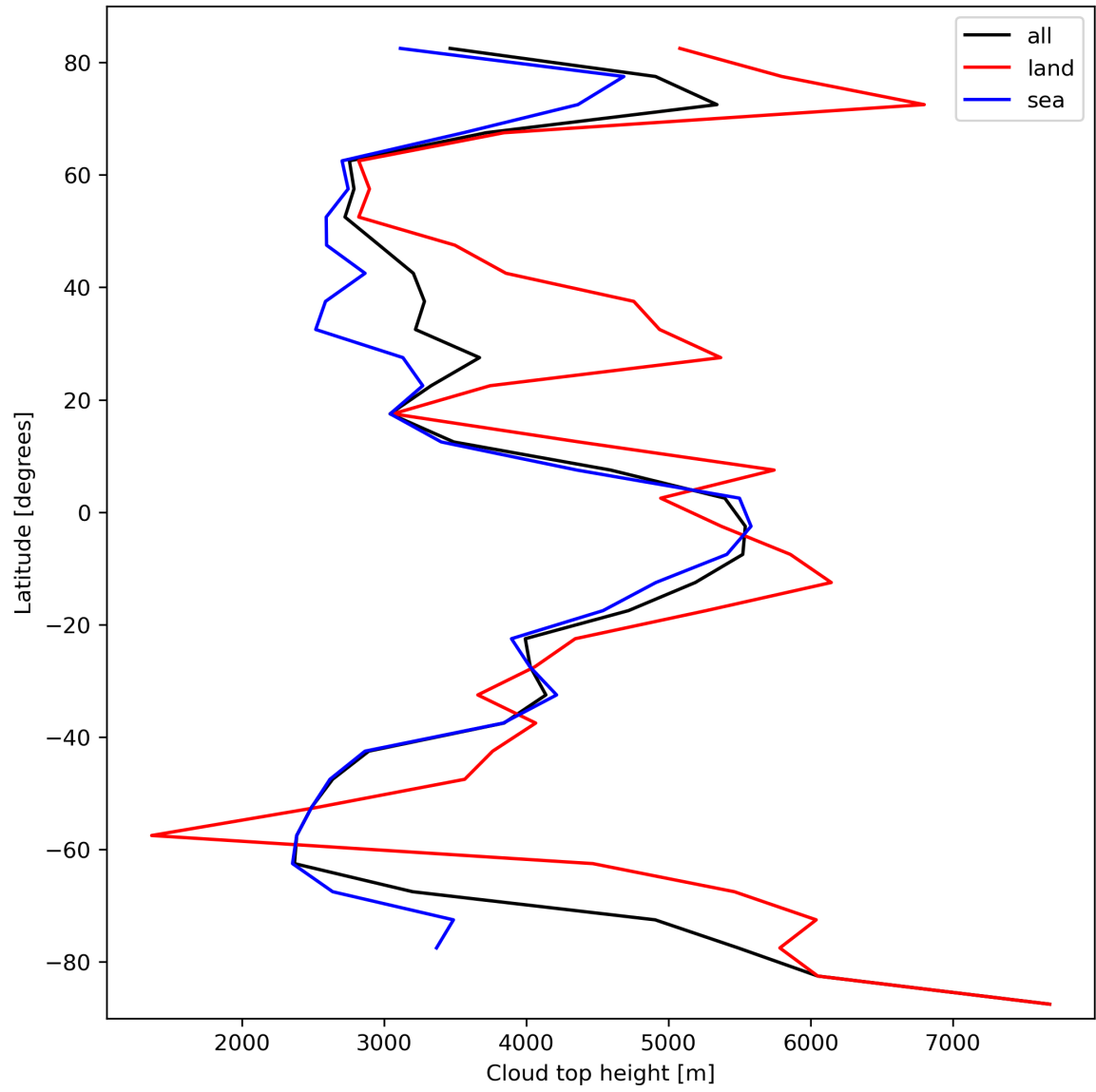
Figure 24: Zonal average of “Cloud top height” for 2024-02-25 to 2024-02-27.
