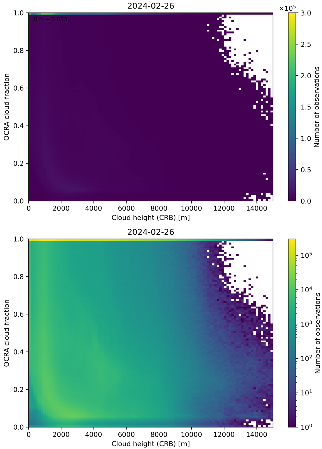
Figure 81: Scatter density plot of “Cloud height (CRB)” against “OCRA cloud fraction” for 2024-02-25 to 2024-02-27.
