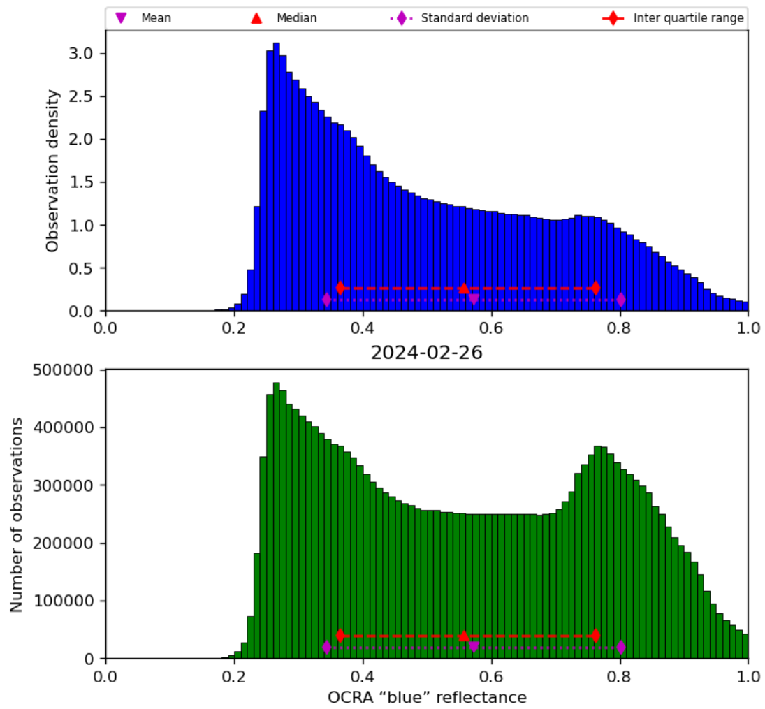
Figure 51: Histogram of “OCRA “blue” reflectance” for 2024-02-25 to 2024-02-27
