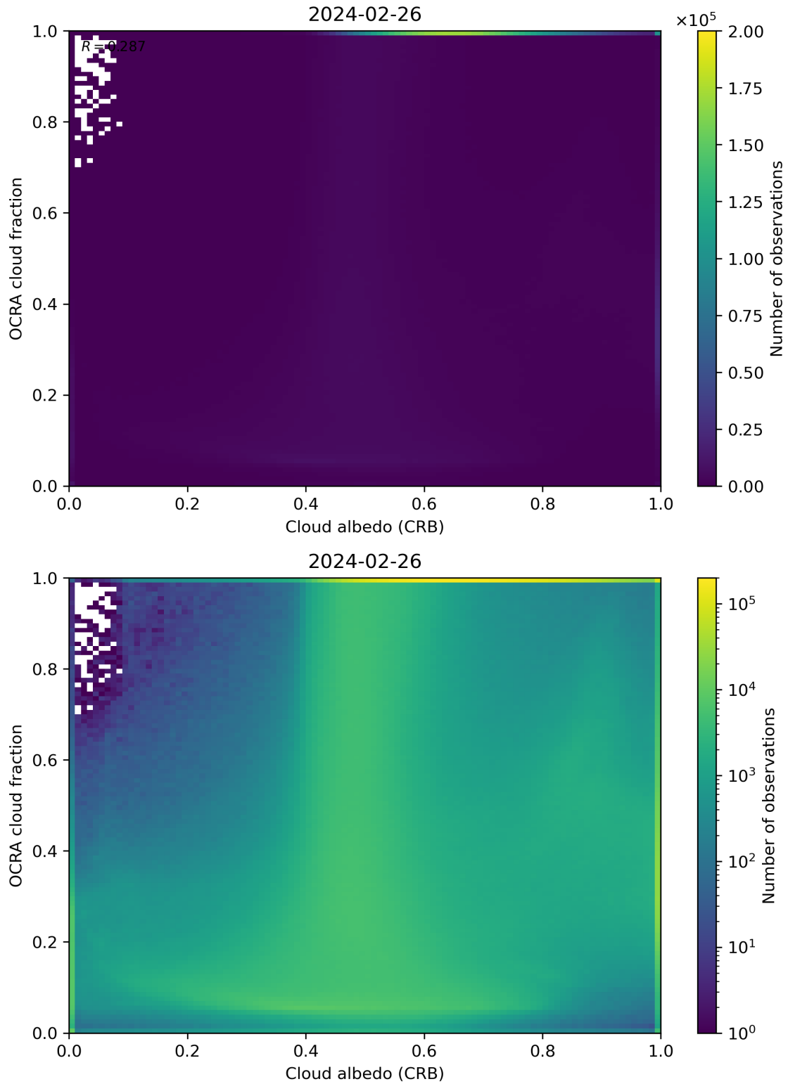
Figure 70: Scatter density plot of “Cloud albedo (CRB)” against “OCRA cloud fraction” for 2024-02-25 to 2024-02-27.
