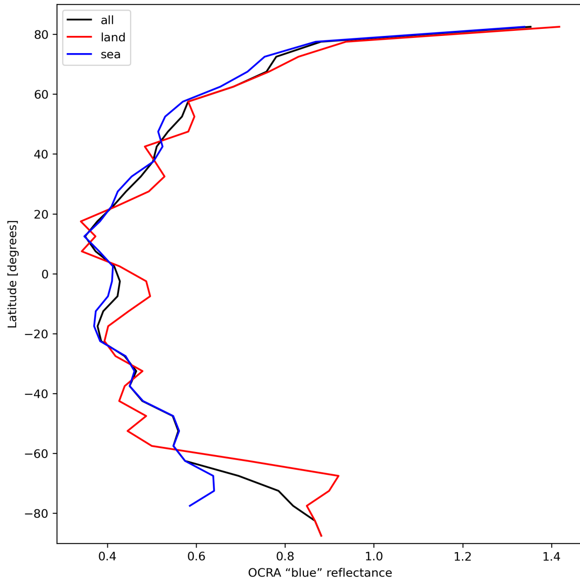
Figure 35: Zonal average of “OCRA “blue” reflectance” for 2024-02-25 to 2024-02-27.
