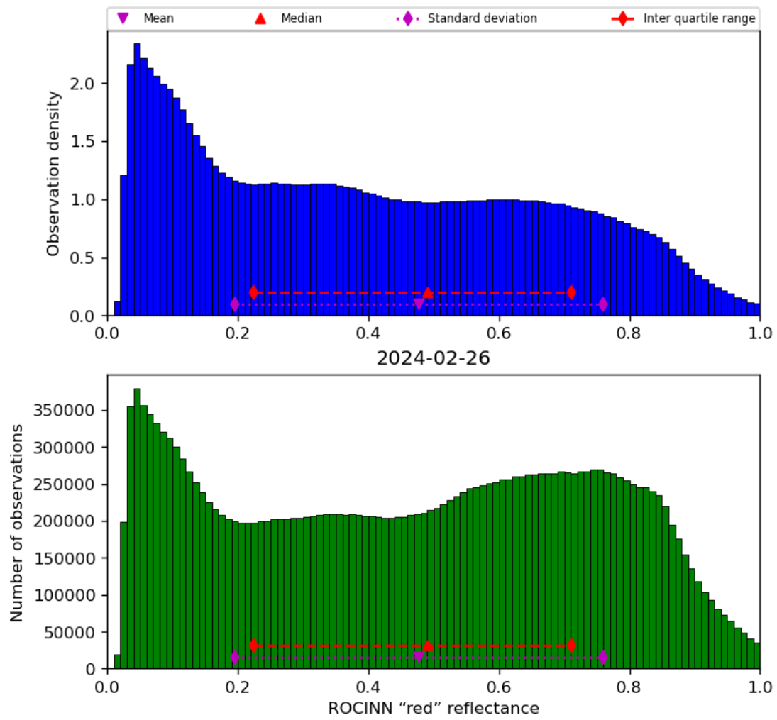
Figure 53: Histogram of “ROCINN “red” reflectance” for 2024-02-25 to 2024-02-27
