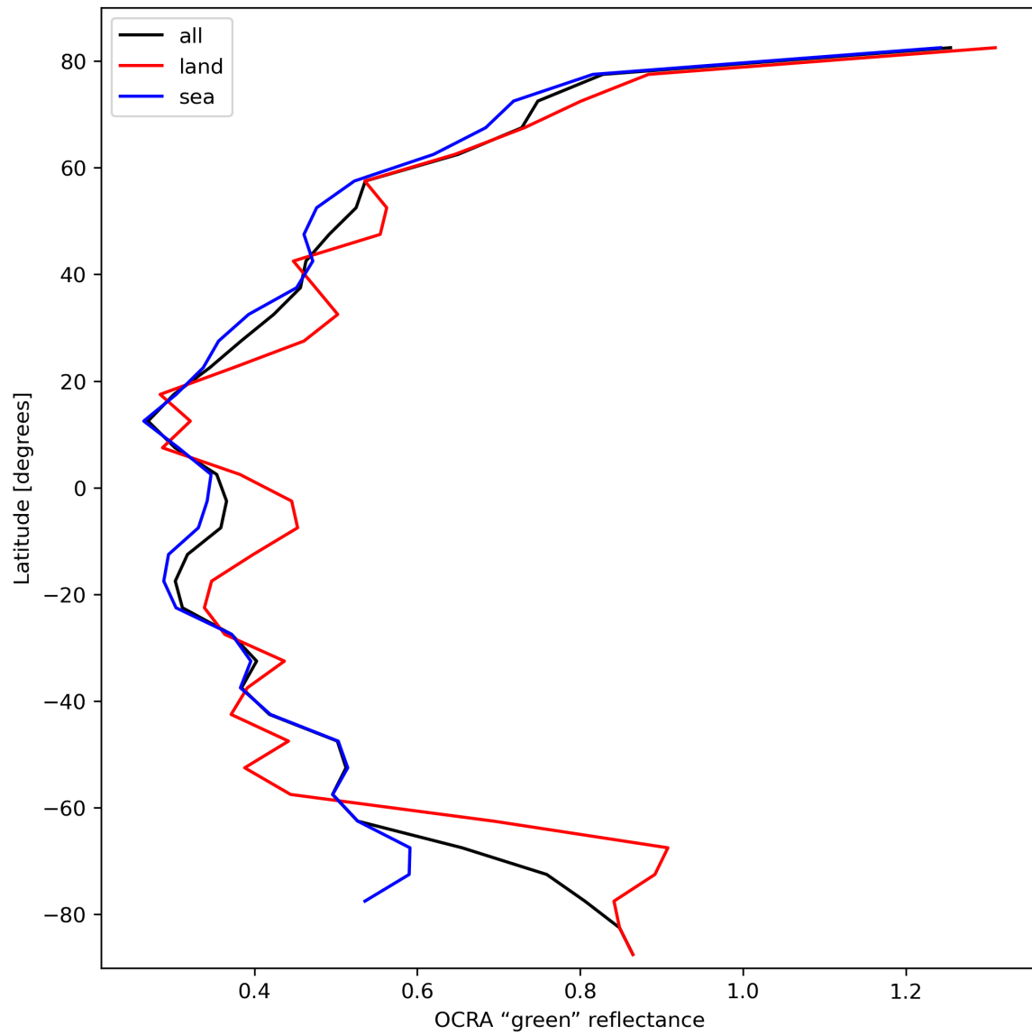
Figure 36: Zonal average of “OCRA “green” reflectance” for 2024-02-25 to 2024-02-27.
