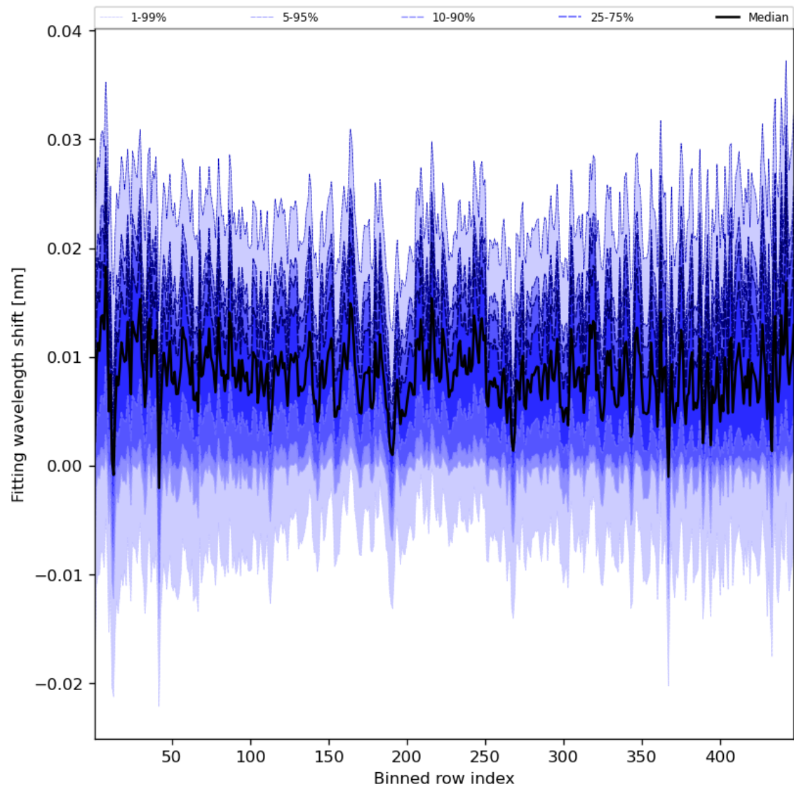
Figure 65: Along track statistics of “Fitting wavelength shift” for 2024-02-25 to 2024-02-27
