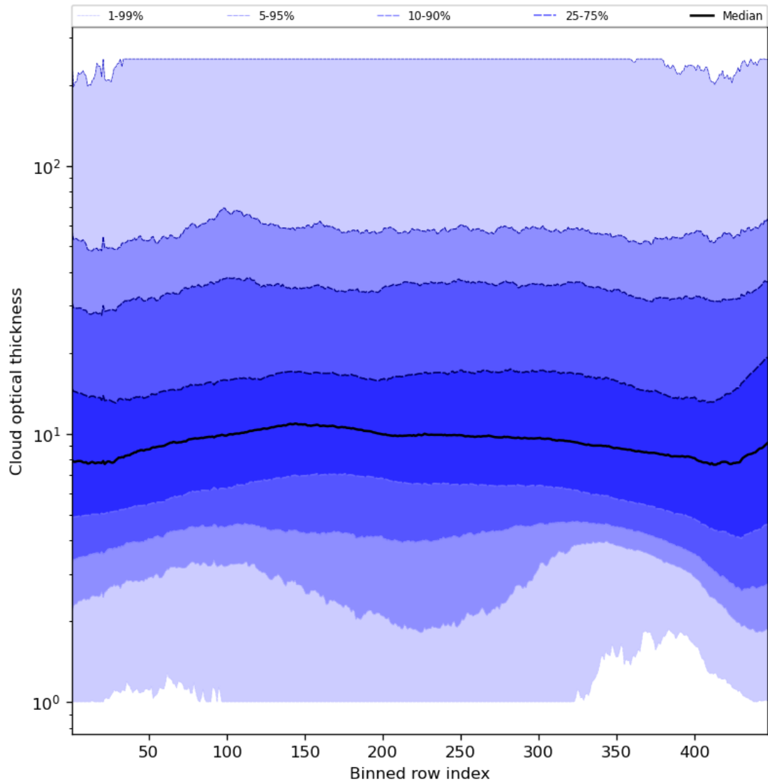
Figure 57: Along track statistics of “Cloud optical thickness” for 2024-02-25 to 2024-02-27
