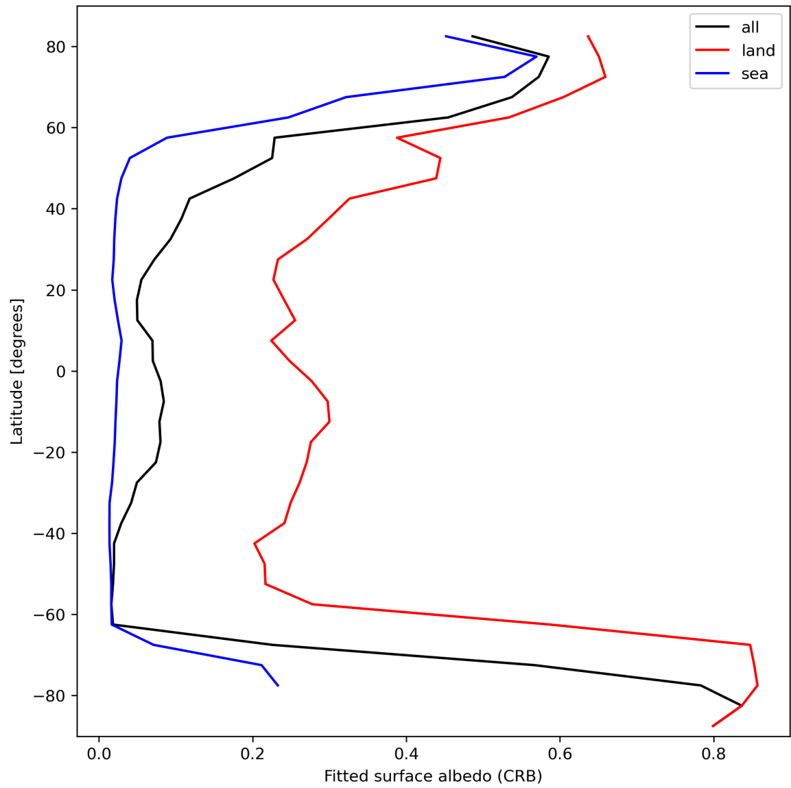
Figure 30: Zonal average of “Fitted surface albedo (CRB)” for 2024-02-25 to 2024-02-27.
