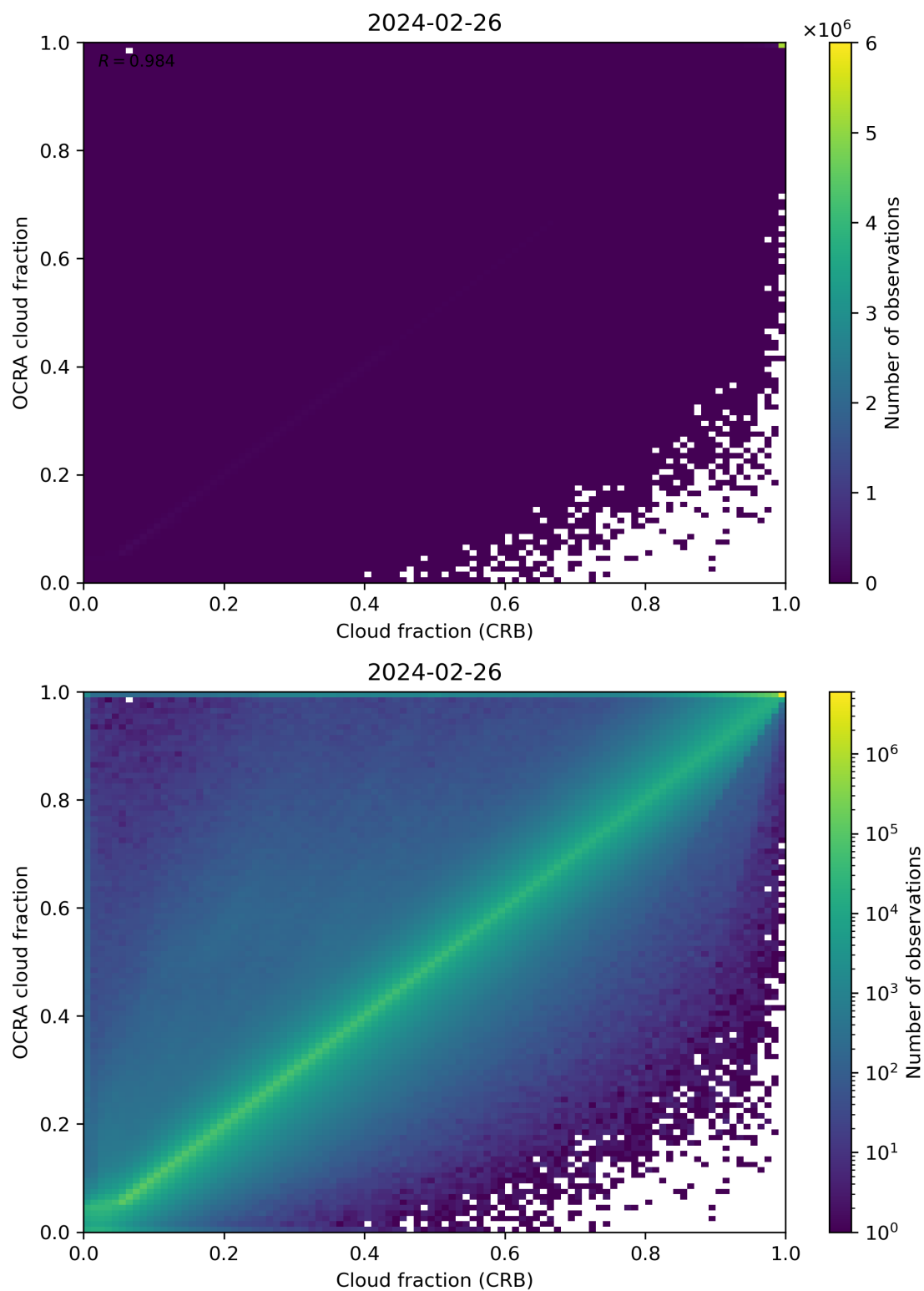
Figure 78: Scatter density plot of “Cloud fraction (CRB)” against “OCRA cloud fraction” for 2024-02-25 to 2024-02-27.
