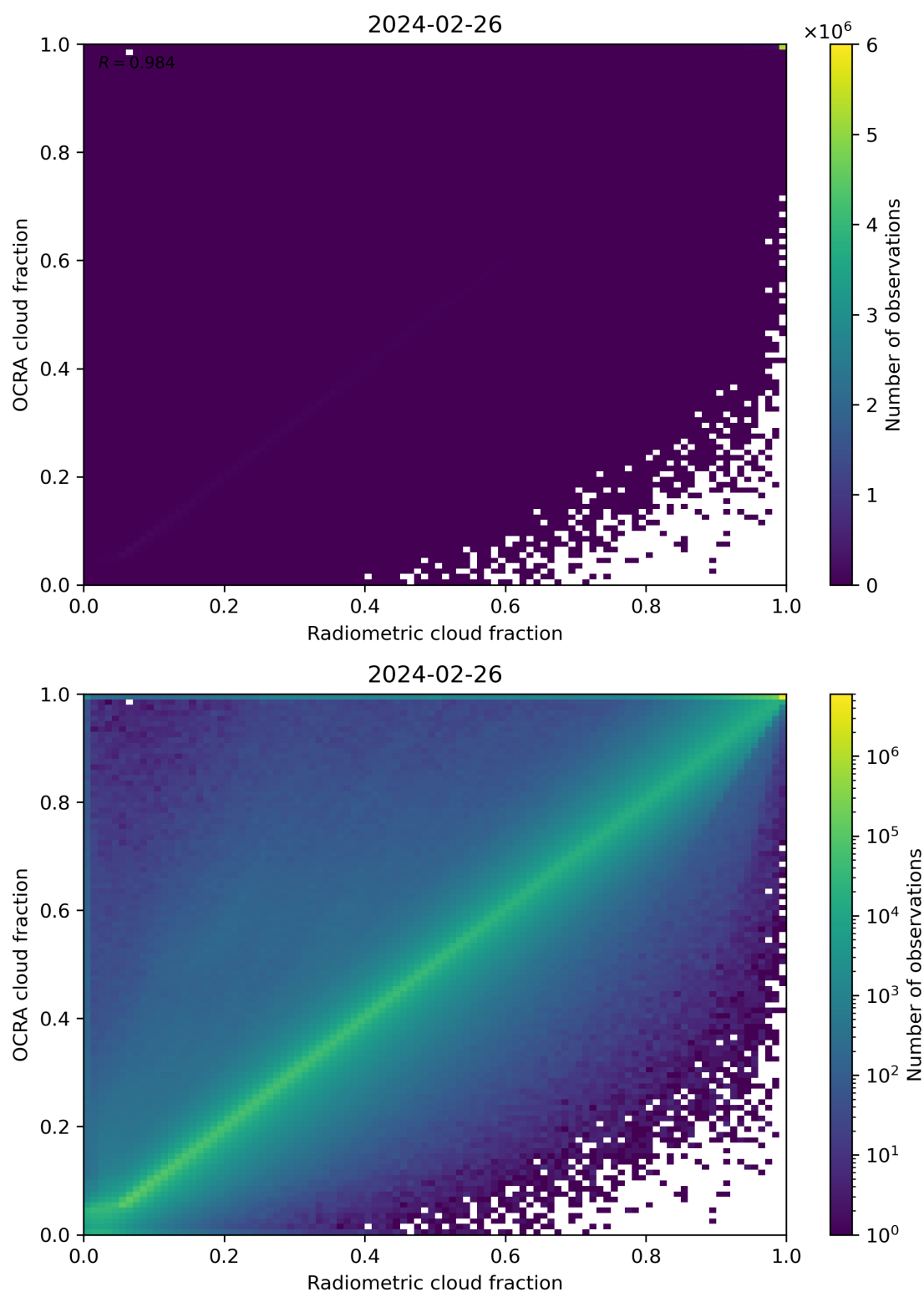
Figure 72: Scatter density plot of “Radiometric cloud fraction” against “OCRA cloud fraction” for 2024-02-25 to 2024-02-27.
