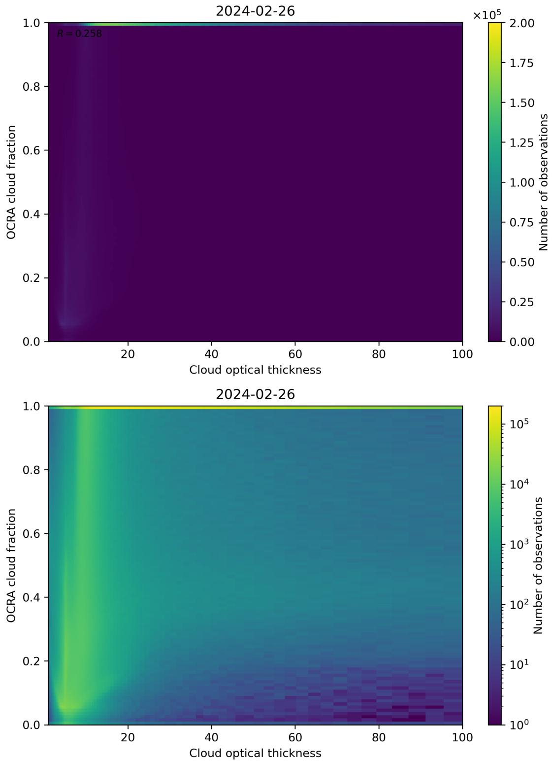
Figure 83: Scatter density plot of “Cloud optical thickness” against “OCRA cloud fraction” for 2024-02-25 to 2024-02-27.
