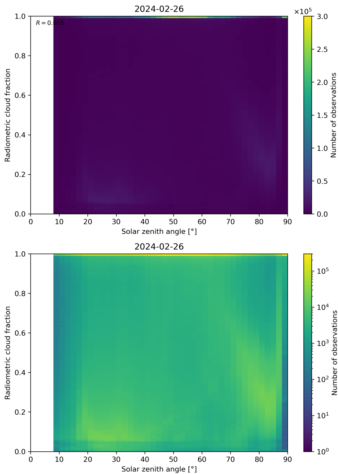
Figure 99: Scatter density plot of “Solar zenith angle” against “Radiometric cloud fraction” for 2024-02-25 to 2024-02-27.
