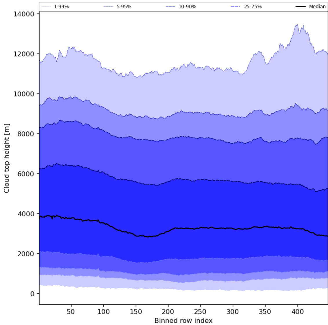
Figure 56: Along track statistics of “Cloud top height” for 2024-02-25 to 2024-02-27
