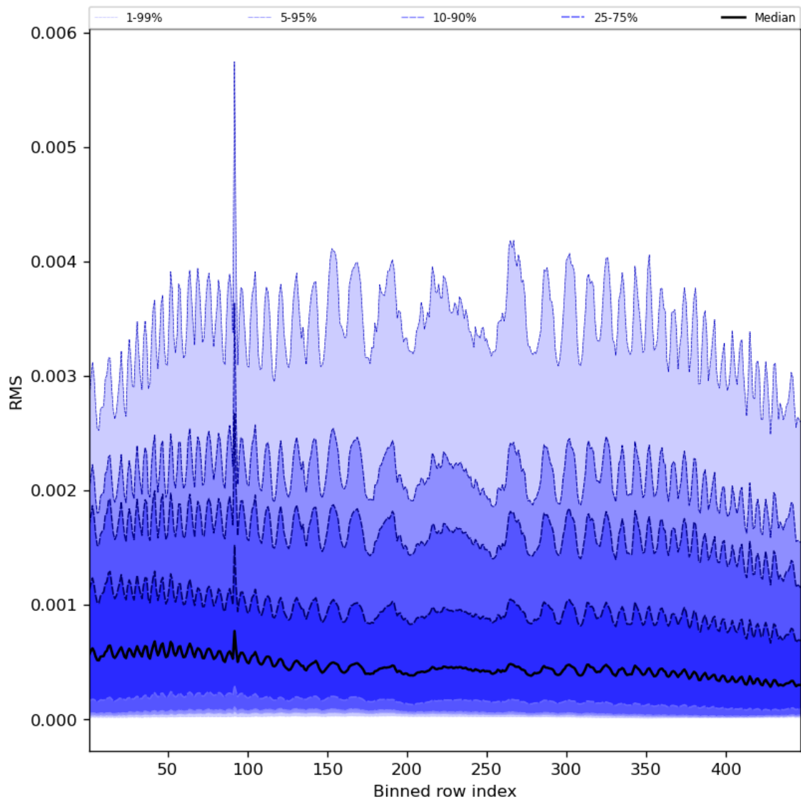
Figure 63: Along track statistics of “RMS” for 2024-02-25 to 2024-02-27
