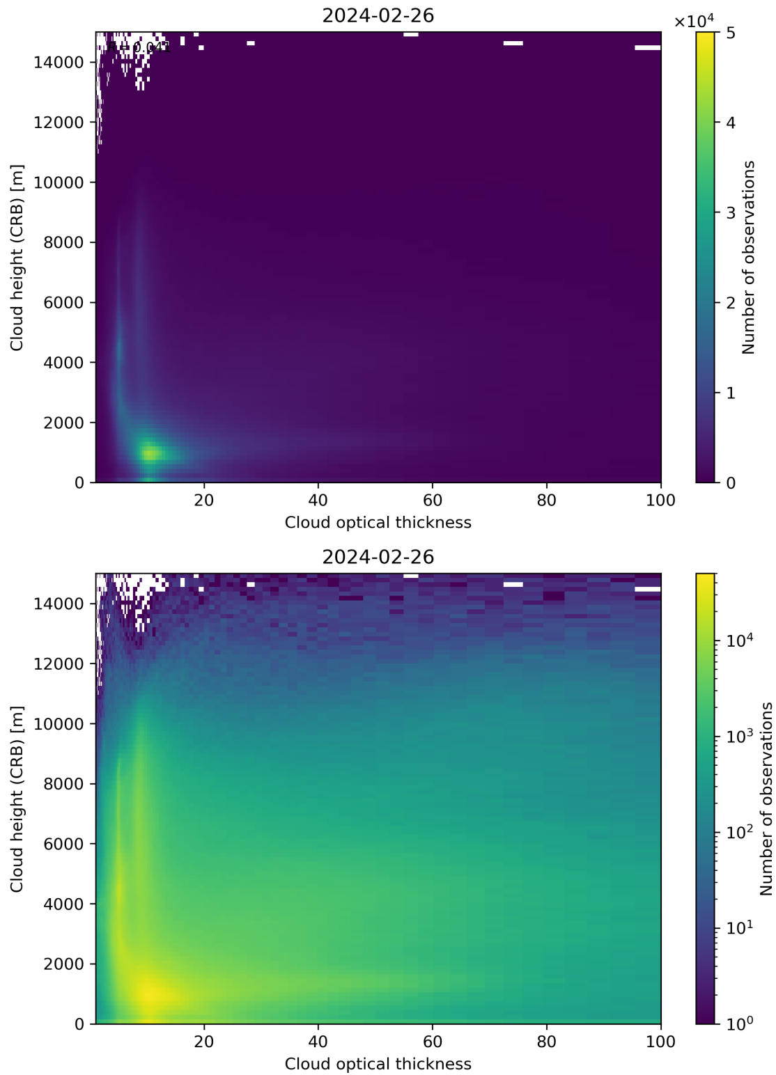
Figure 85: Scatter density plot of “Cloud optical thickness” against “Cloud height (CRB)” for 2024-02-25 to 2024-02-27.
