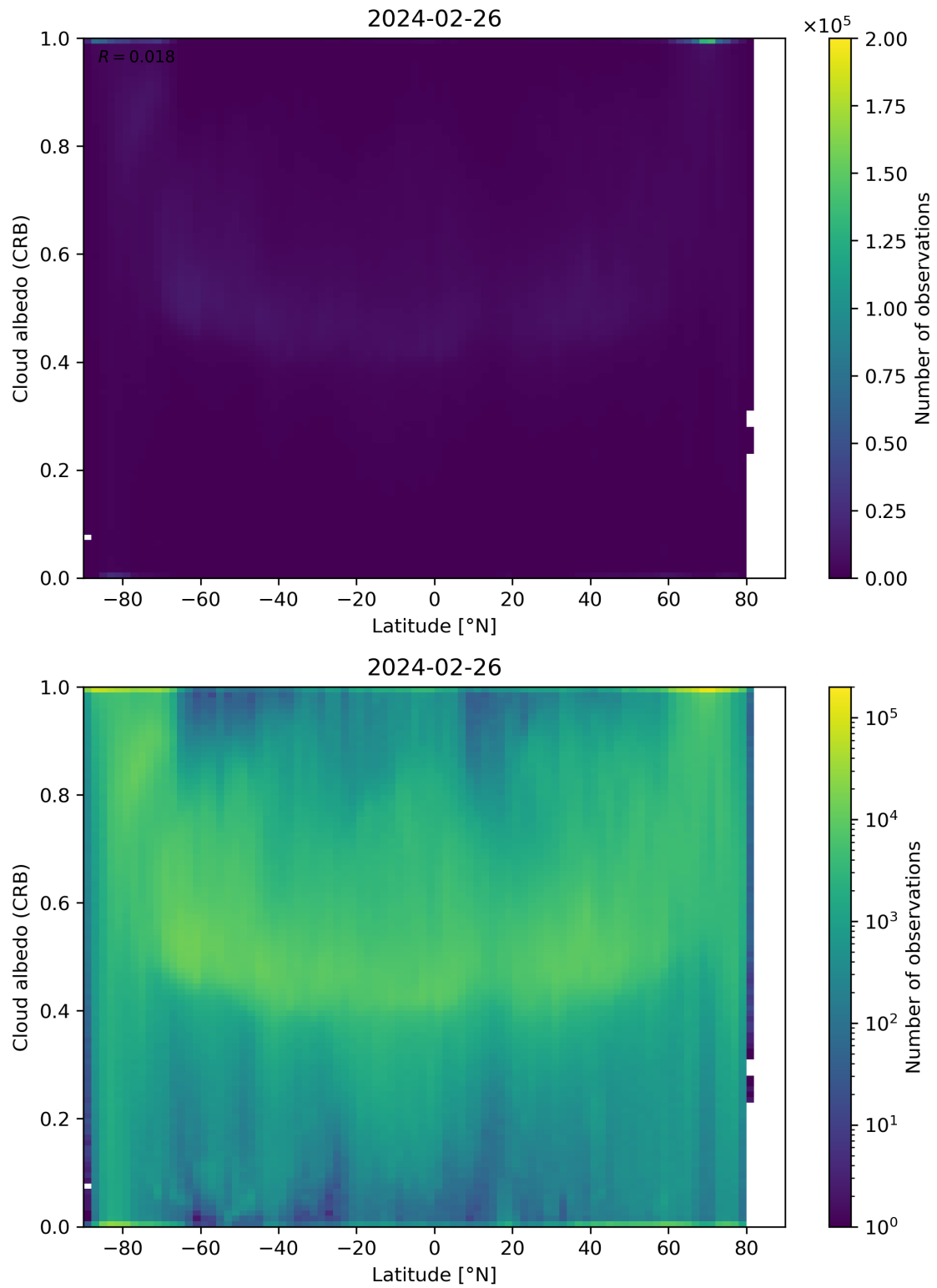
Figure 91: Scatter density plot of “Latitude” against “Cloud albedo (CRB)” for 2024-02-25 to 2024-02-27.
