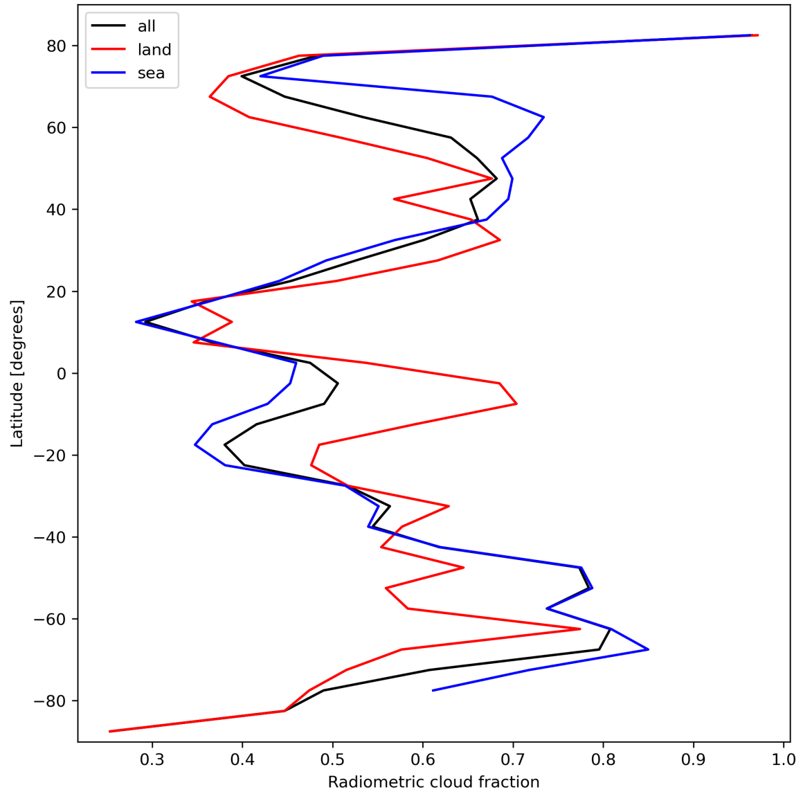
Figure 23: Zonal average of “Radiometric cloud fraction” for 2024-02-25 to 2024-02-27.
