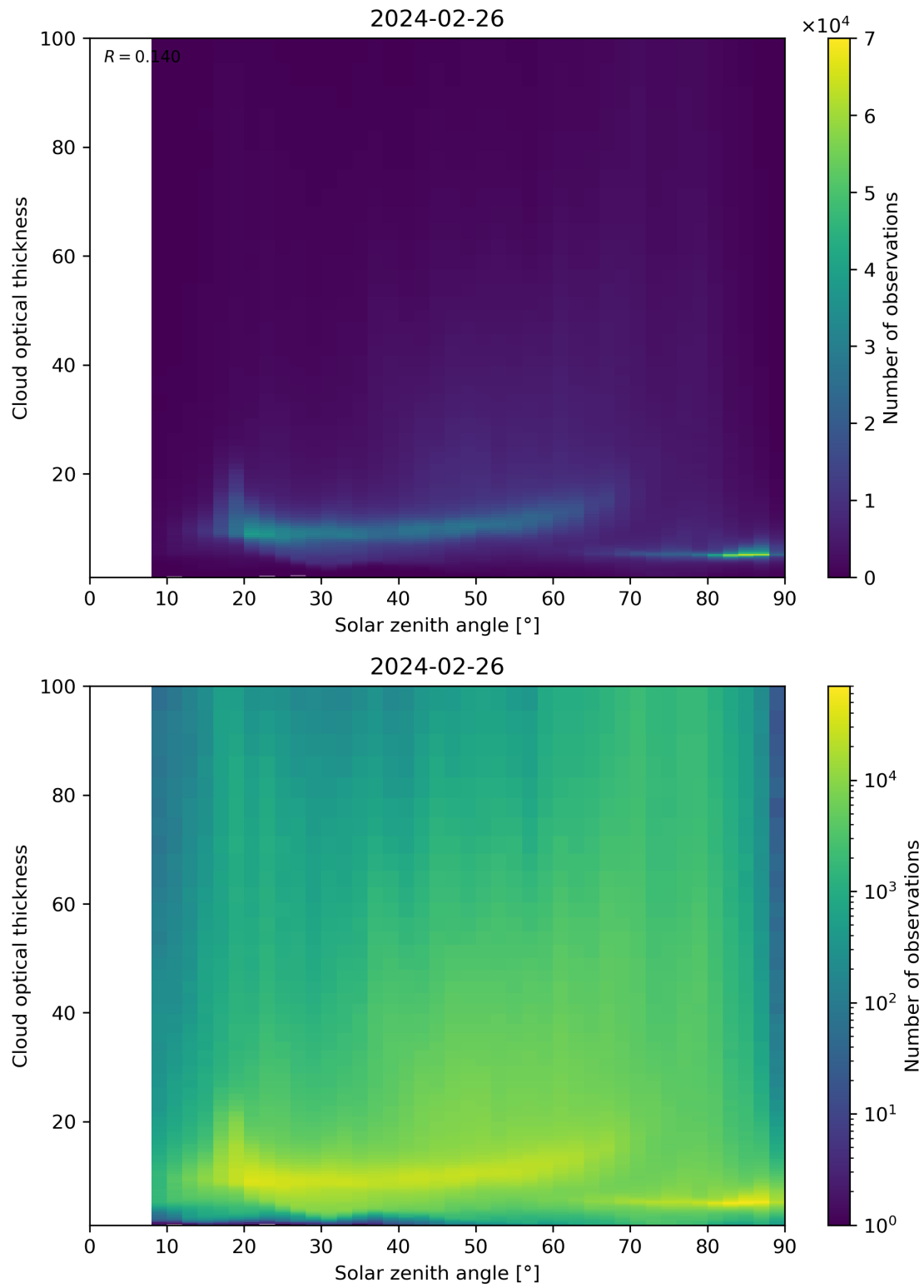
Figure 103: Scatter density plot of “Solar zenith angle” against “Cloud optical thickness” for 2024-02-25 to 2024-02-27.
