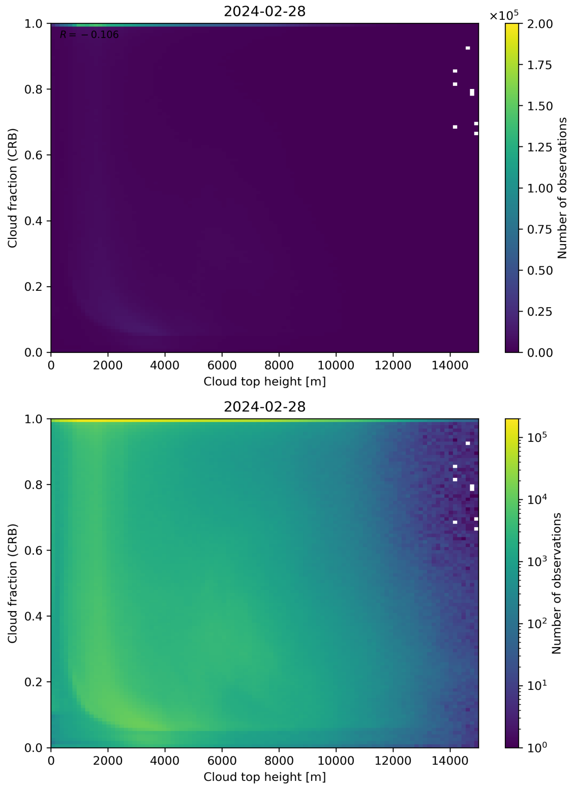
Figure 88: Scatter density plot of “Cloud top height” against “Cloud fraction (CRB)” for 2024-02-27 to 2024-02-29.
