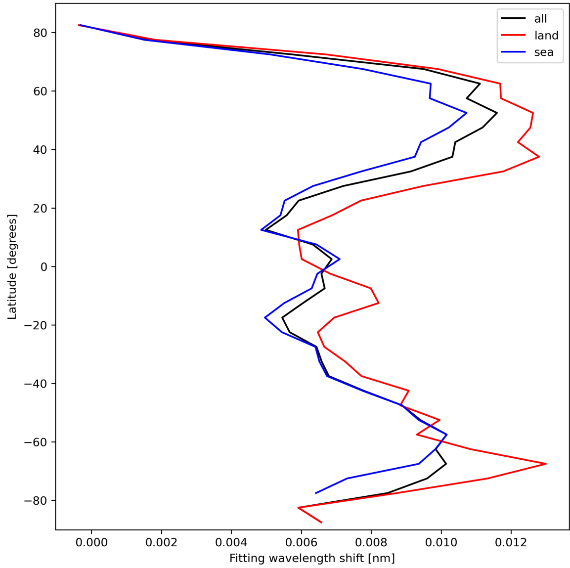
Figure 33: Zonal average of “Fitting wavelength shift” for 2024-02-27 to 2024-02-29.
