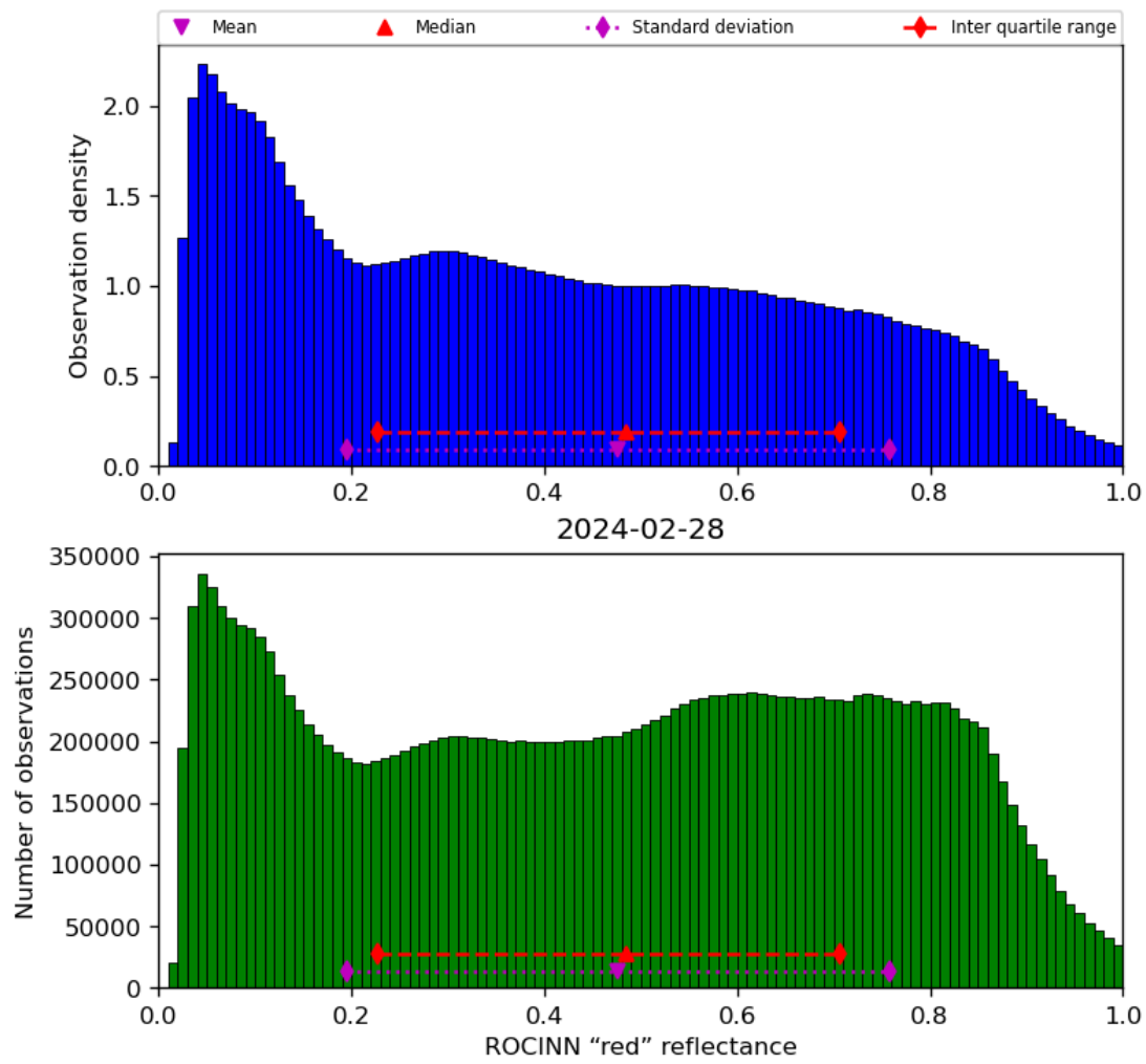
Figure 53: Histogram of “ROCINN “red” reflectance” for 2024-02-27 to 2024-02-29
