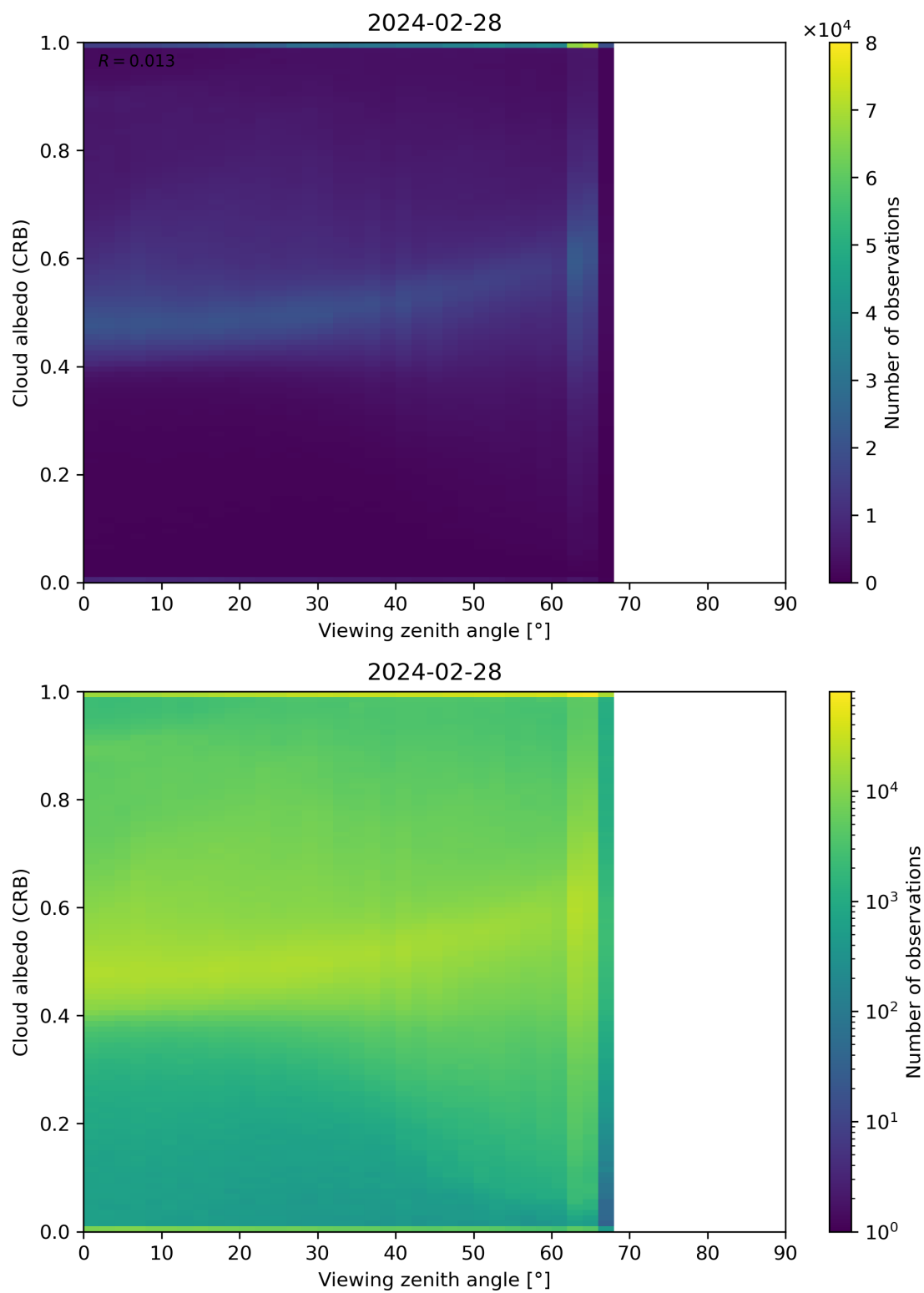
Figure 106: Scatter density plot of “Viewing zenith angle” against “Cloud albedo (CRB)” for 2024-02-27 to 2024-02-29.
