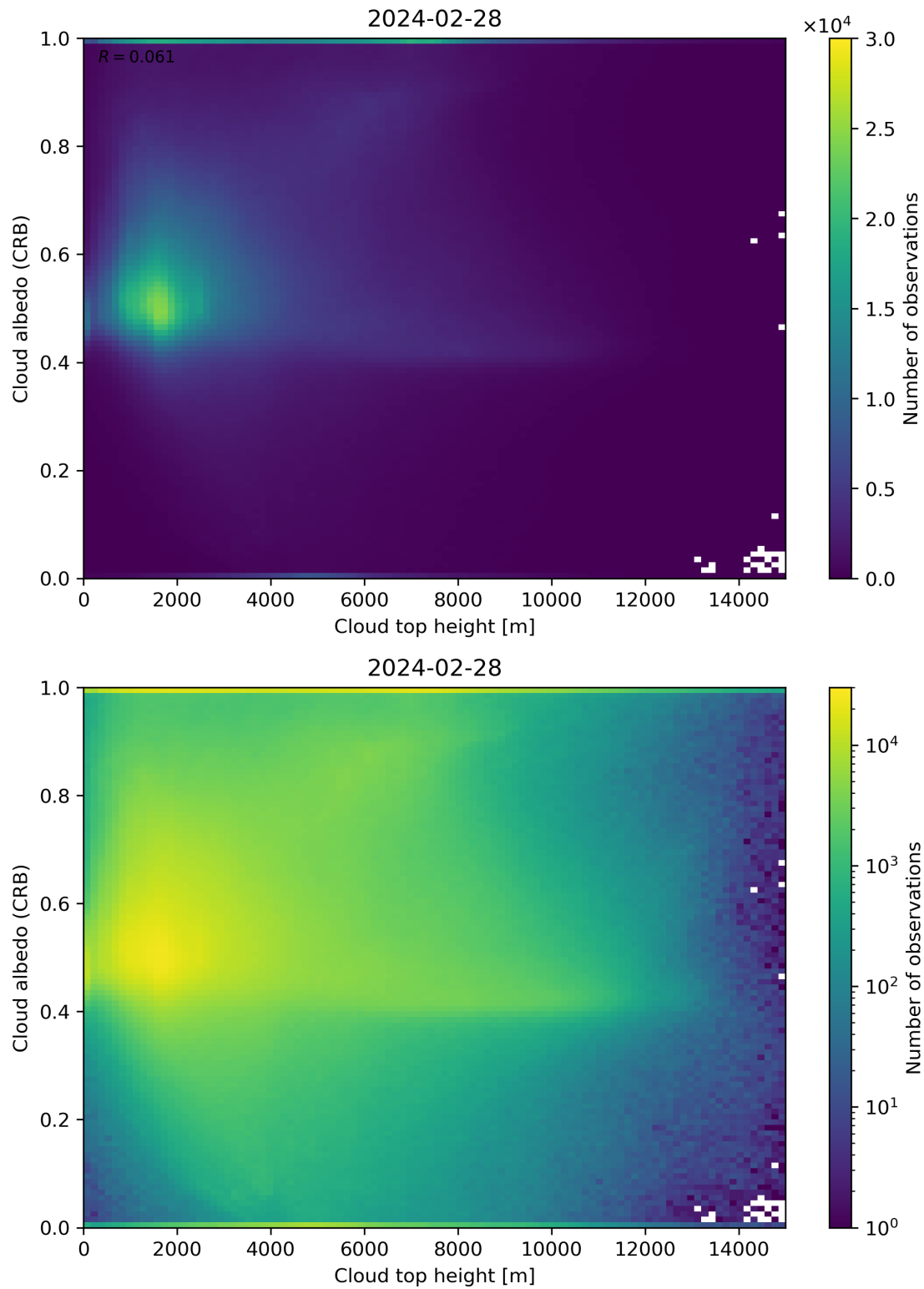
Figure 86: Scatter density plot of “Cloud top height” against “Cloud albedo (CRB)” for 2024-02-27 to 2024-02-29.
