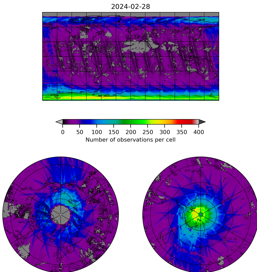
Figure 21: Map of the number of observations for 2024-02-27 to 2024-02-29
