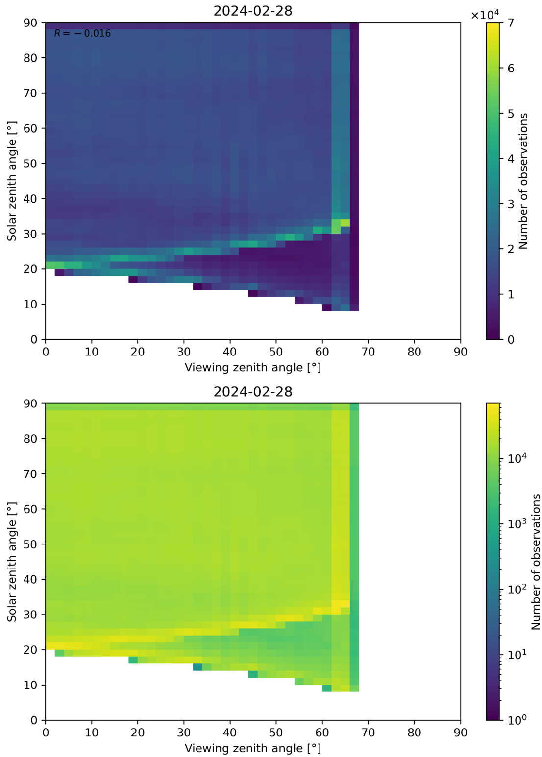
Figure 114: Scatter density plot of “Viewing zenith angle” against “Solar zenith angle” for 2024-02-27 to 2024-02-29.
