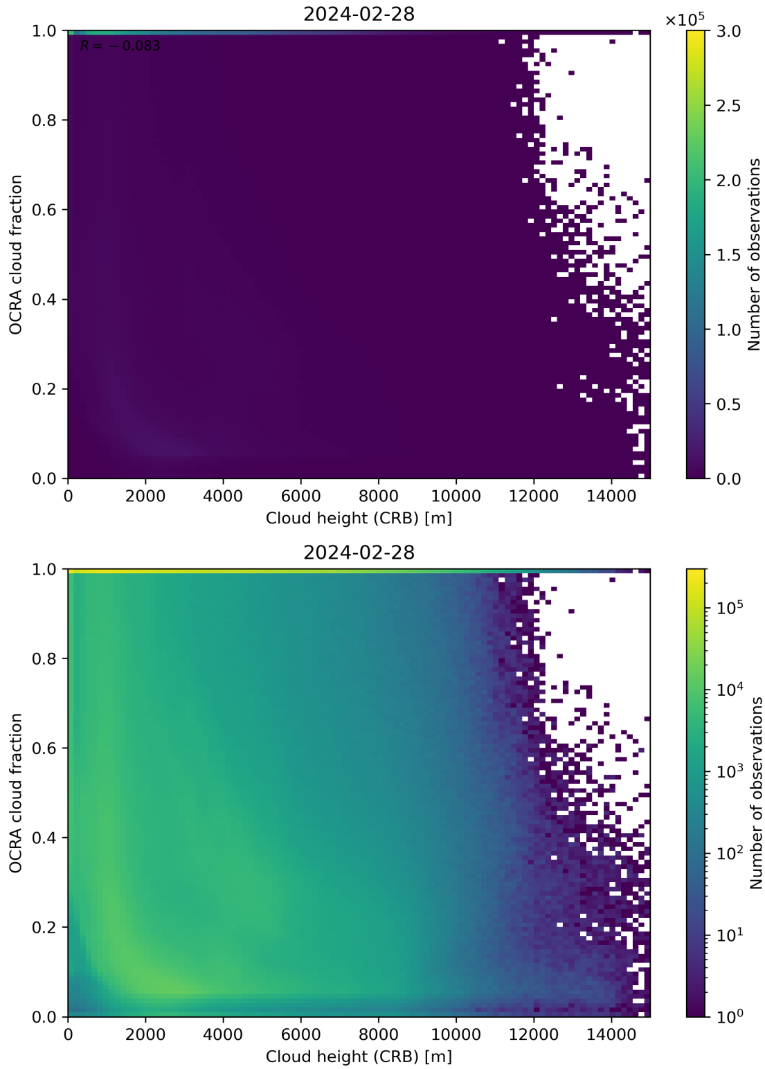
Figure 81: Scatter density plot of “Cloud height (CRB)” against “OCRA cloud fraction” for 2024-02-27 to 2024-02-29.
