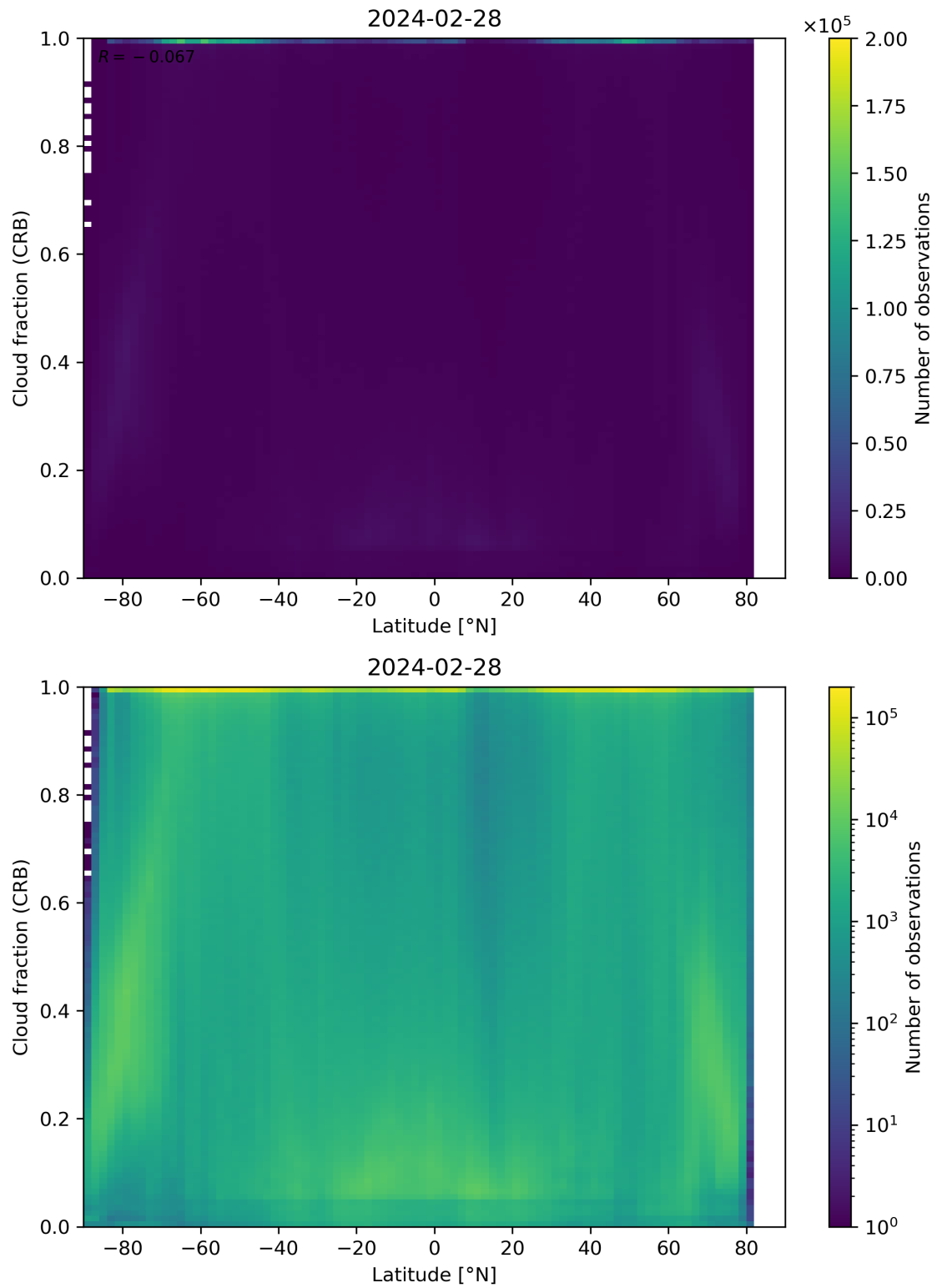
Figure 94: Scatter density plot of “Latitude” against “Cloud fraction (CRB)” for 2024-02-27 to 2024-02-29.
