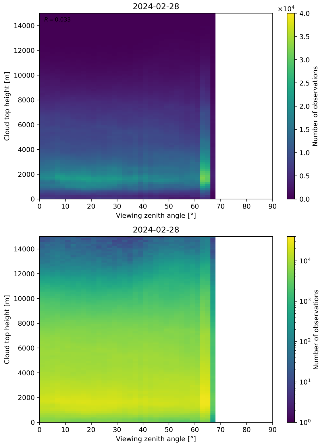
Figure 112: Scatter density plot of “Viewing zenith angle” against “Cloud top height” for 2024-02-27 to 2024-02-29.
