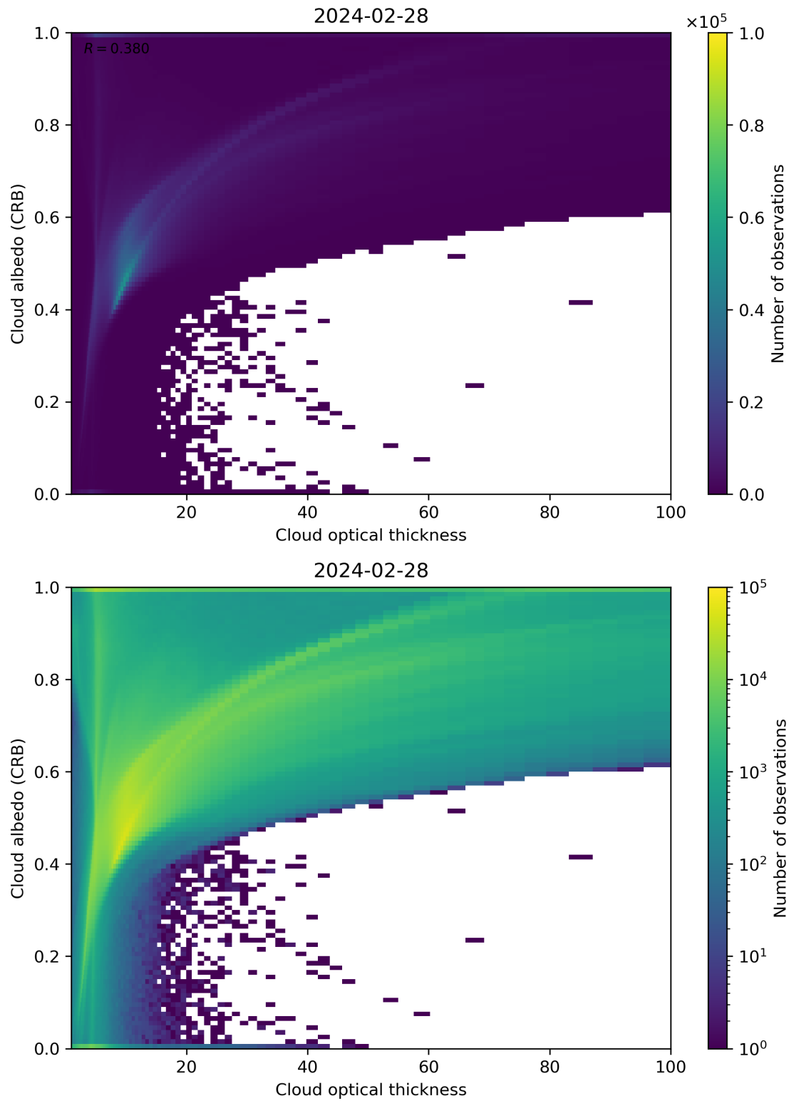
Figure 82: Scatter density plot of “Cloud optical thickness” against “Cloud albedo (CRB)” for 2024-02-27 to 2024-02-29.
