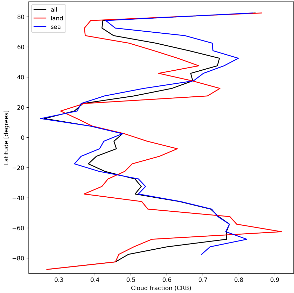
Figure 26: Zonal average of “Cloud fraction (CRB)” for 2024-02-27 to 2024-02-29.
