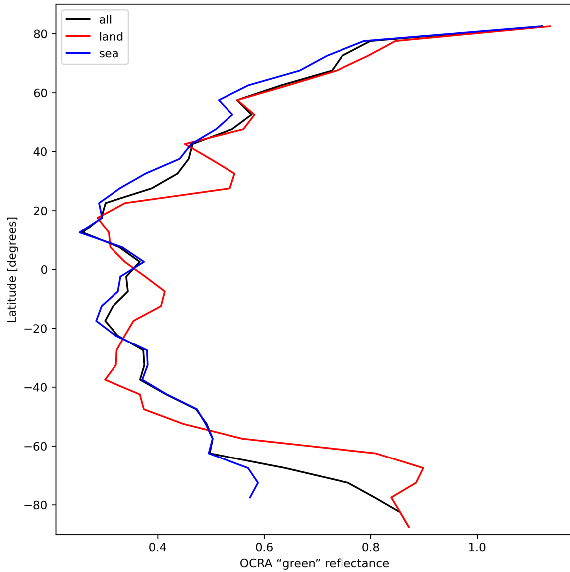
Figure 36: Zonal average of “OCRA “green” reflectance” for 2024-02-27 to 2024-02-29.
