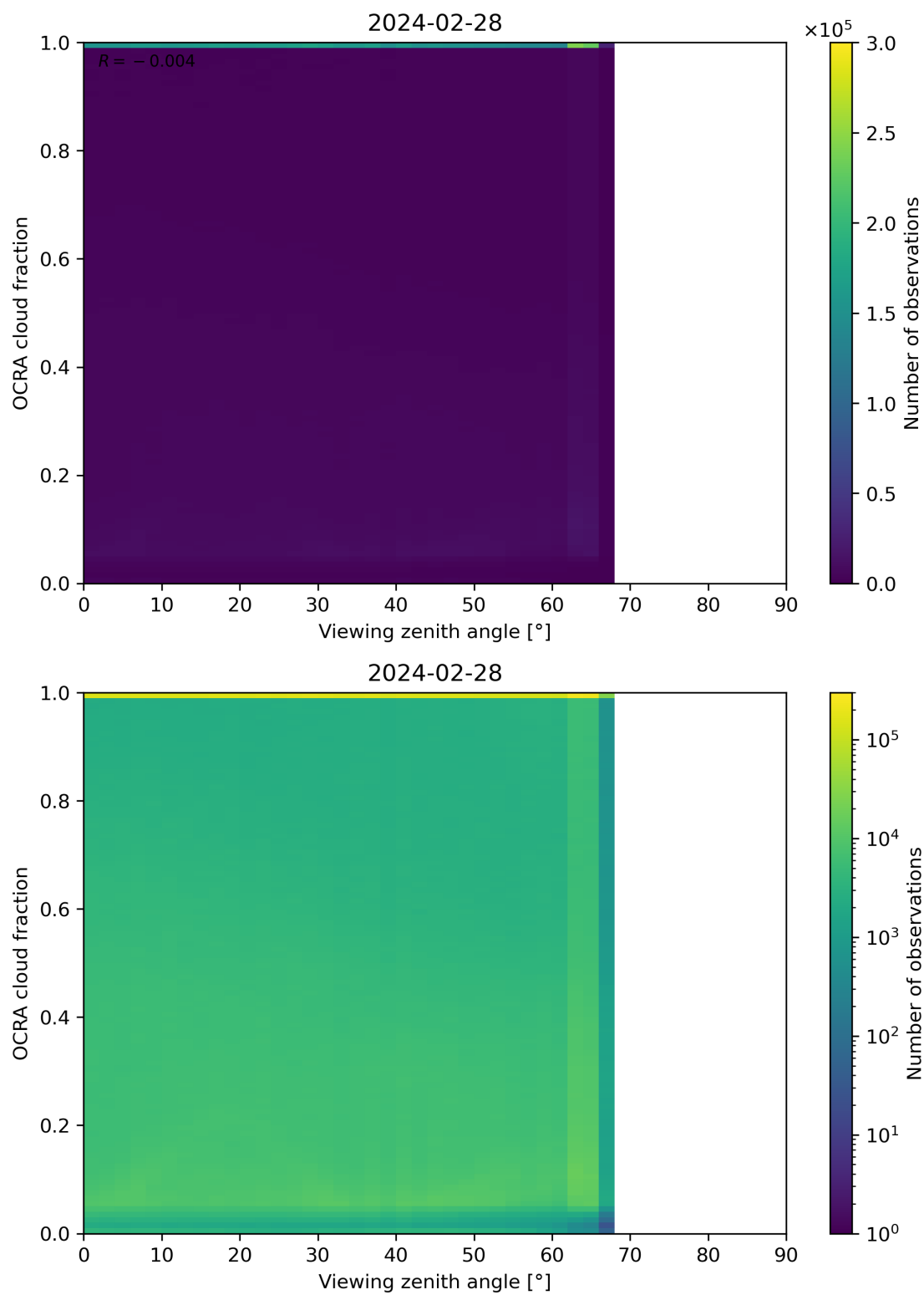
Figure 108: Scatter density plot of “Viewing zenith angle” against “OCRA cloud fraction” for 2024-02-27 to 2024-02-29.
