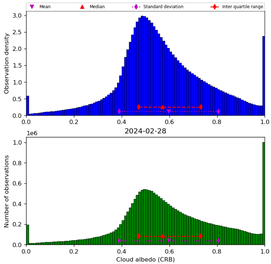
Figure 44: Histogram of “Cloud albedo (CRB)” for 2024-02-27 to 2024-02-29
