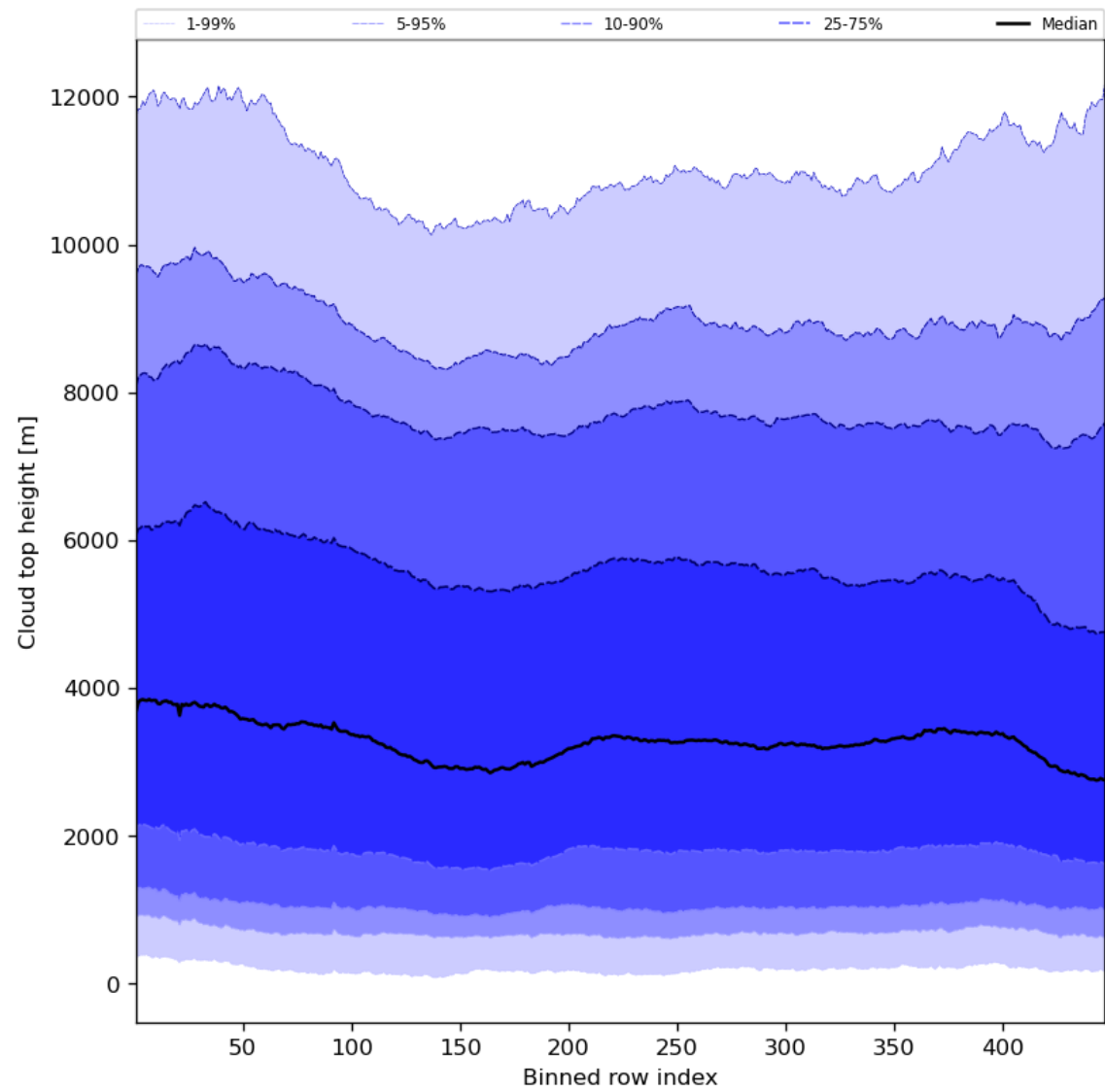
Figure 56: Along track statistics of “Cloud top height” for 2024-02-27 to 2024-02-29
