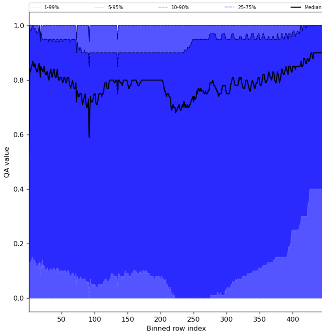
Figure 54: Along track statistics of “QA value” for 2024-02-27 to 2024-02-29
