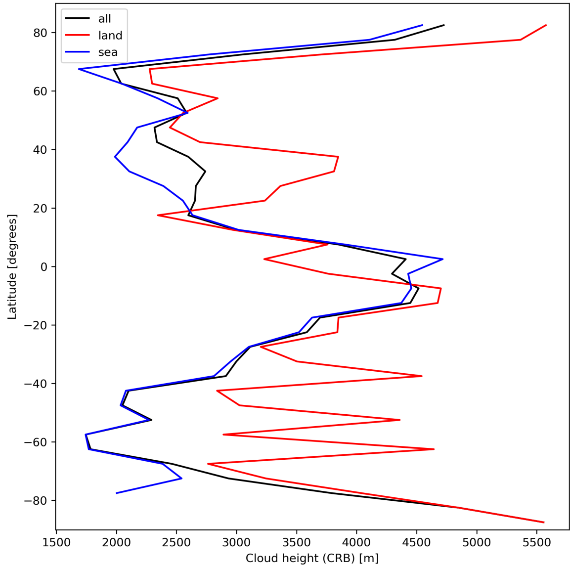
Figure 27: Zonal average of “Cloud height (CRB)” for 2024-02-27 to 2024-02-29.
