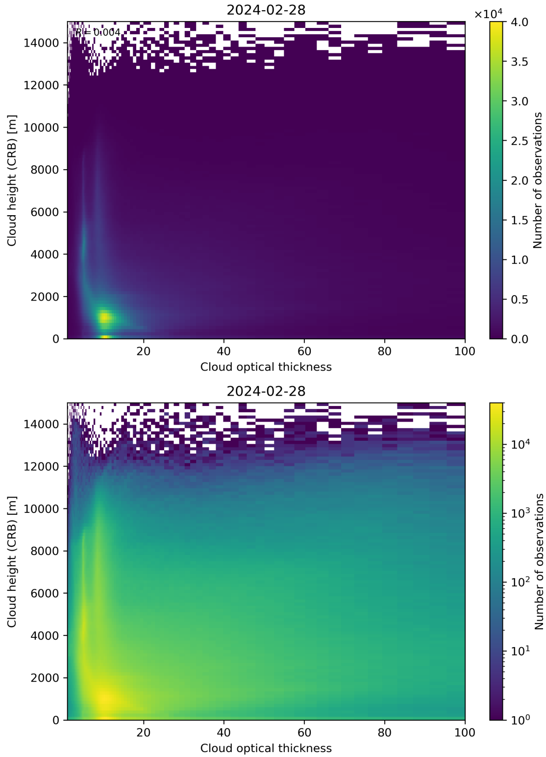
Figure 85: Scatter density plot of “Cloud optical thickness” against “Cloud height (CRB)” for 2024-02-27 to 2024-02-29.
