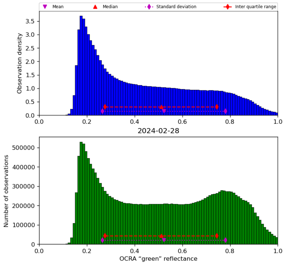
Figure 52: Histogram of “OCRA “green” reflectance” for 2024-02-27 to 2024-02-29
