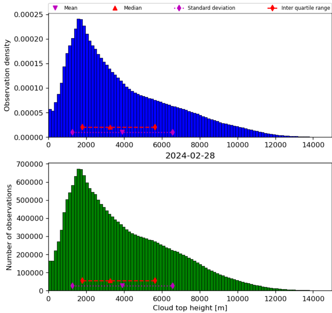
Figure 40: Histogram of “Cloud top height” for 2024-02-27 to 2024-02-29
