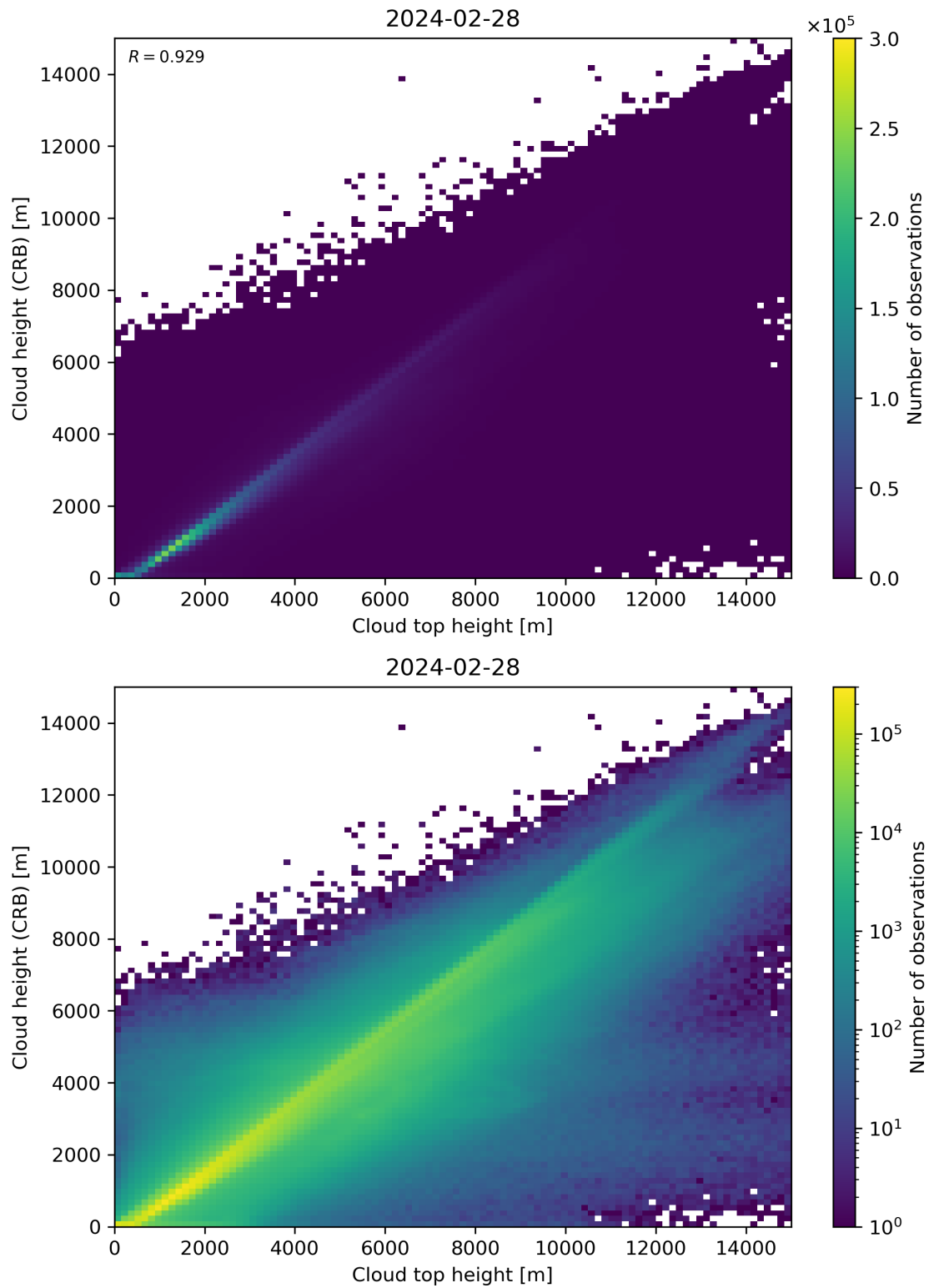
Figure 89: Scatter density plot of “Cloud top height” against “Cloud height (CRB)” for 2024-02-27 to 2024-02-29.
