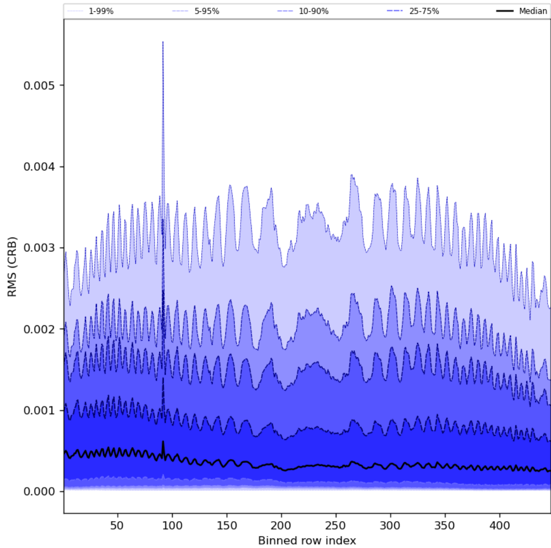
Figure 64: Along track statistics of “RMS (CRB)” for 2024-02-27 to 2024-02-29
