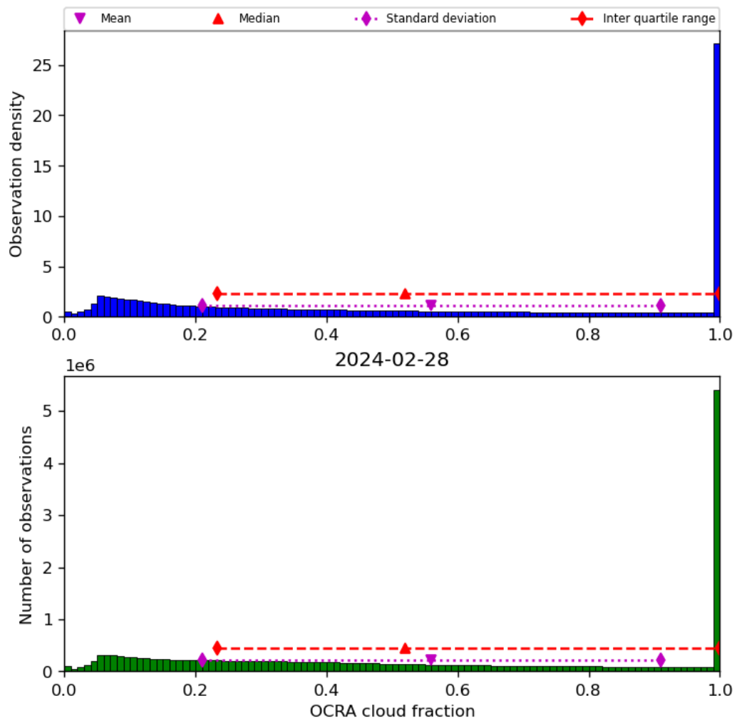
Figure 50: Histogram of “OCRA cloud fraction” for 2024-02-27 to 2024-02-29
