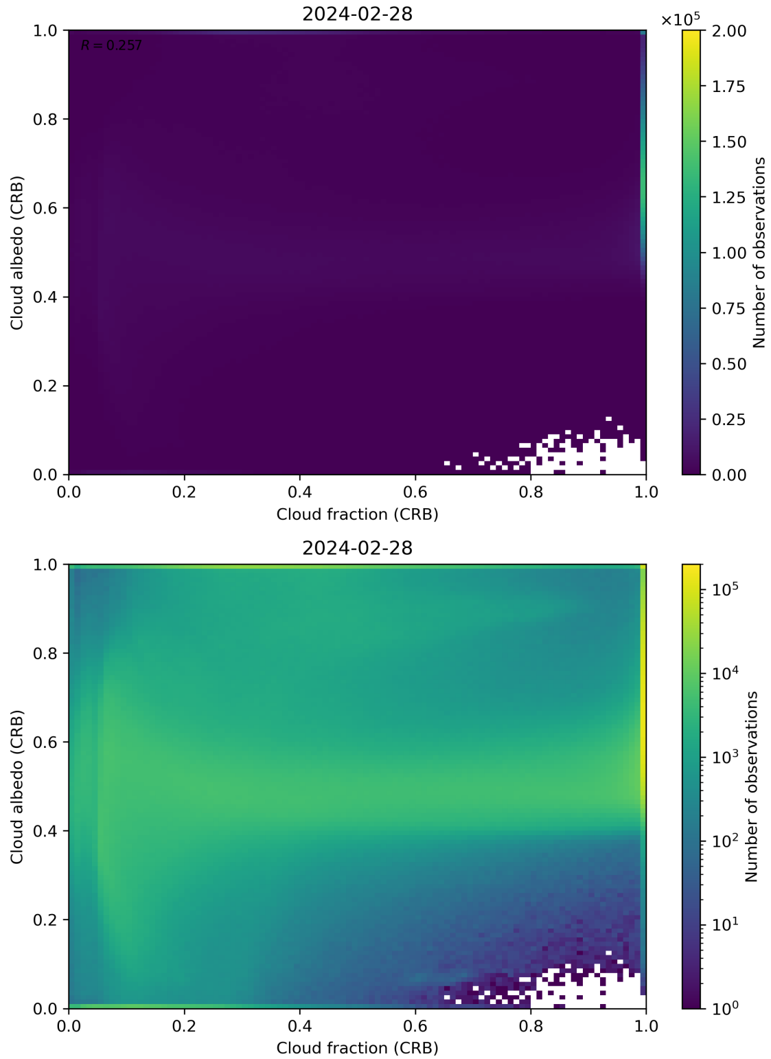
Figure 77: Scatter density plot of “Cloud fraction (CRB)” against “Cloud albedo (CRB)” for 2024-02-27 to 2024-02-29.
