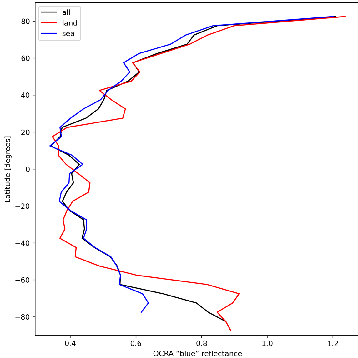
Figure 35: Zonal average of “OCRA “blue” reflectance” for 2024-02-27 to 2024-02-29.
