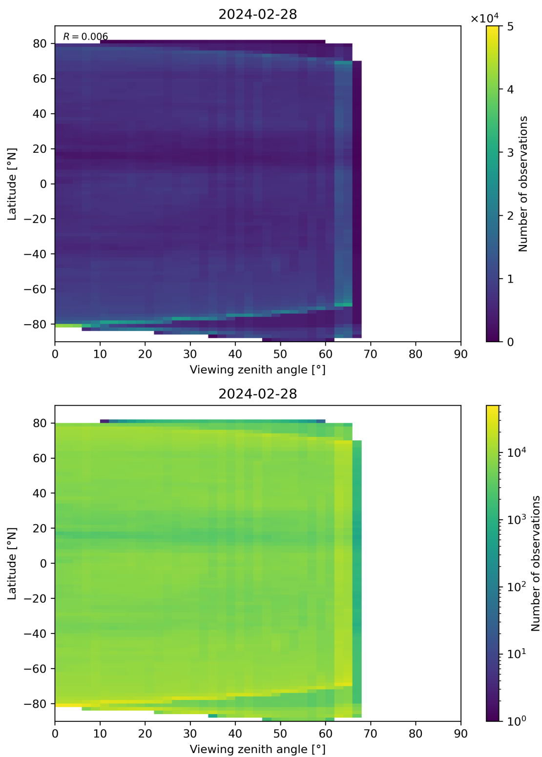
Figure 113: Scatter density plot of “Viewing zenith angle” against “Latitude” for 2024-02-27 to 2024-02-29.
