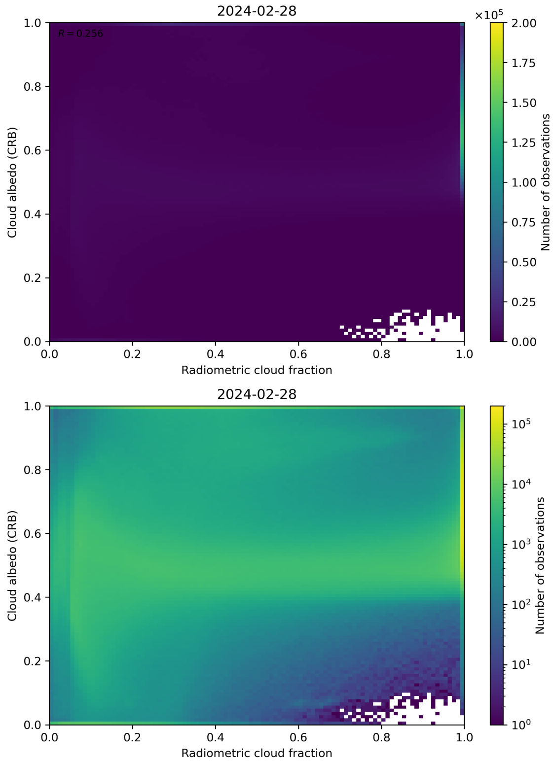
Figure 71: Scatter density plot of “Radiometric cloud fraction” against “Cloud albedo (CRB)” for 2024-02-27 to 2024-02-29.
