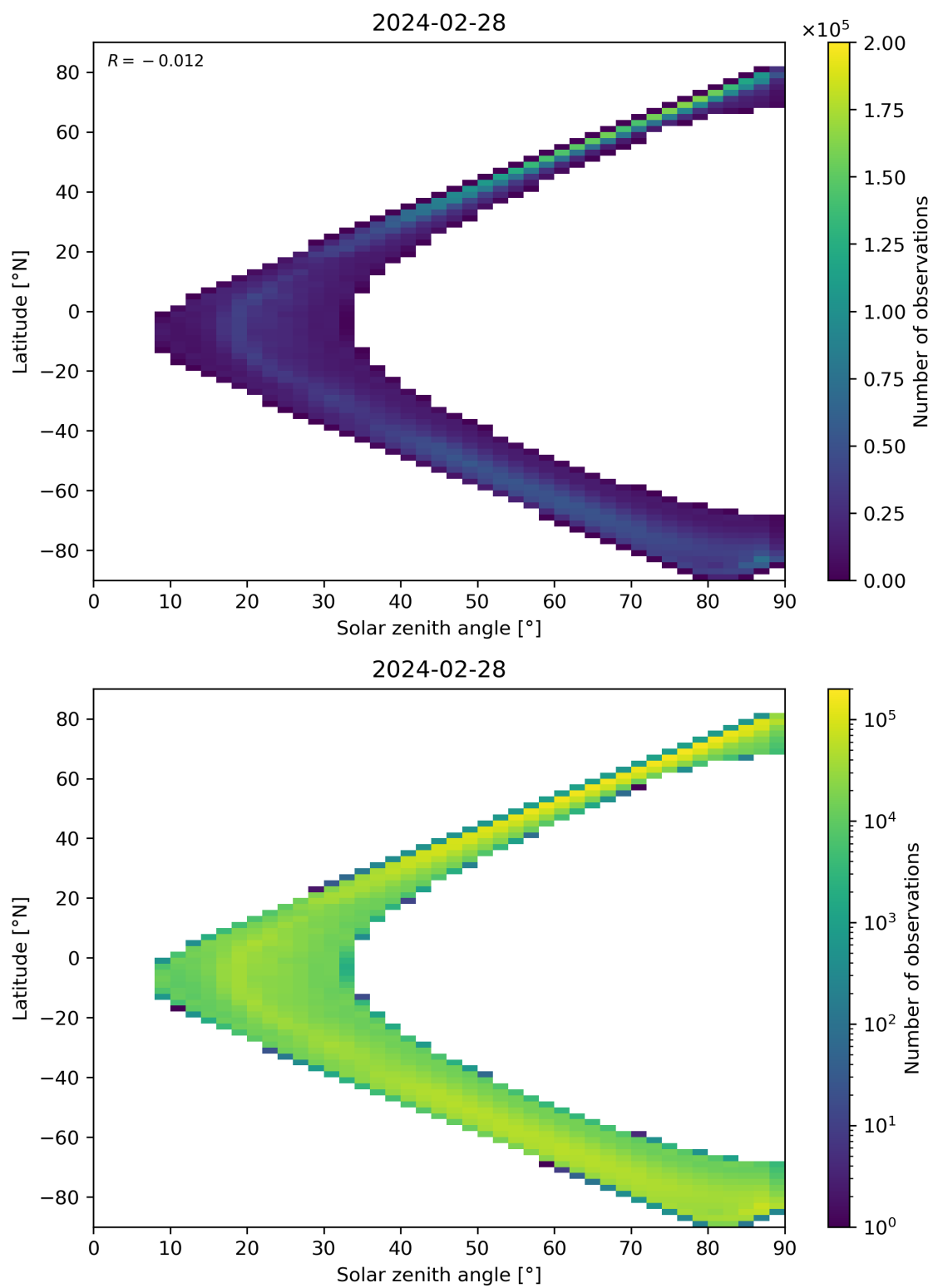
Figure 105: Scatter density plot of “Solar zenith angle” against “Latitude” for 2024-02-27 to 2024-02-29.
