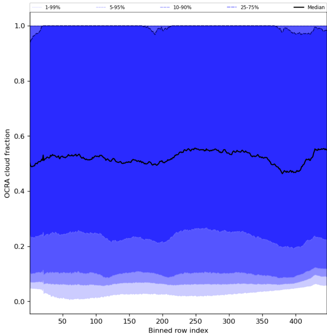
Figure 66: Along track statistics of “OCRA cloud fraction” for 2024-02-27 to 2024-02-29
