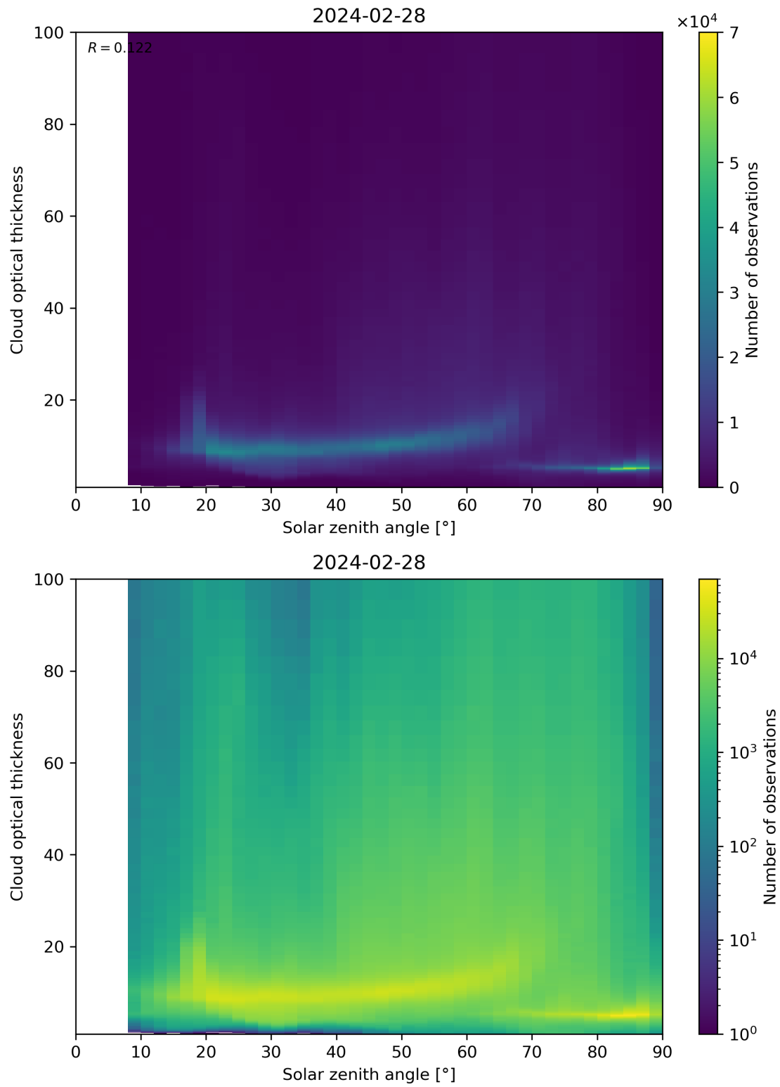
Figure 103: Scatter density plot of “Solar zenith angle” against “Cloud optical thickness” for 2024-02-27 to 2024-02-29.
