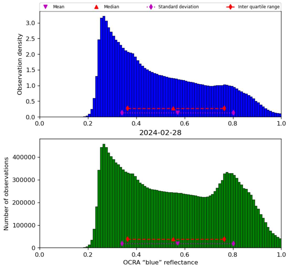
Figure 51: Histogram of “OCRA “blue” reflectance” for 2024-02-27 to 2024-02-29
