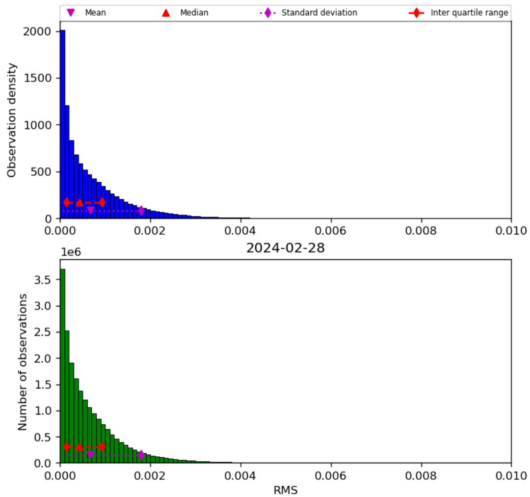
Figure 47: Histogram of “RMS” for 2024-02-27 to 2024-02-29
