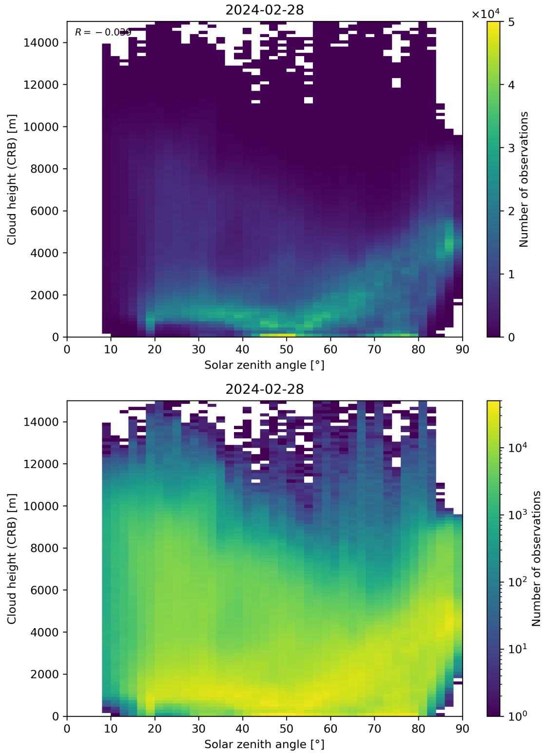
Figure 102: Scatter density plot of “Solar zenith angle” against “Cloud height (CRB)” for 2024-02-27 to 2024-02-29.
