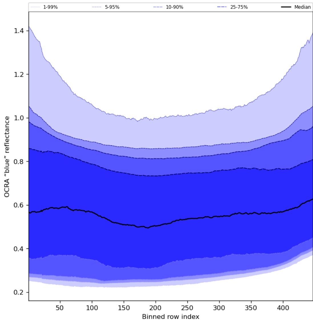
Figure 67: Along track statistics of "OCRA "blue" reflectance" for 2024-02-27 to 2024-02-29
