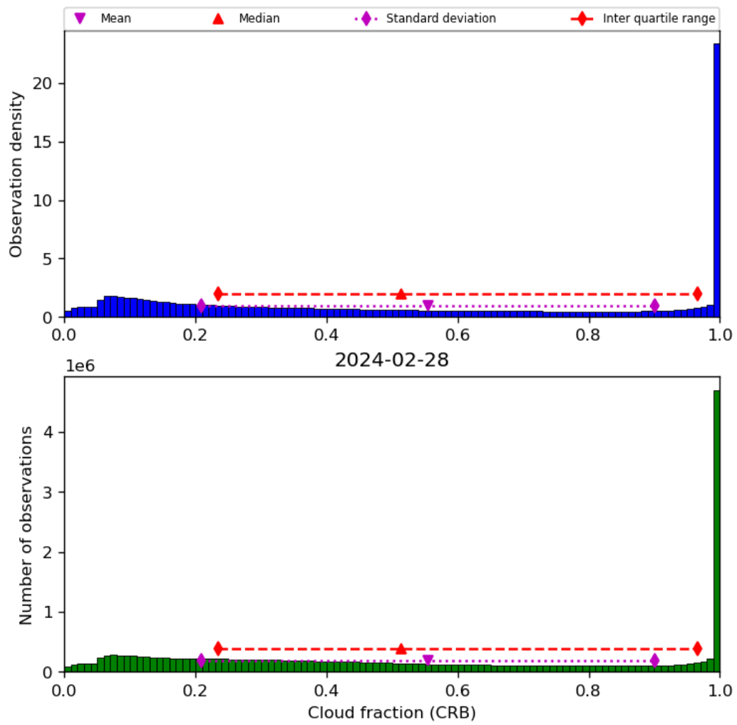
Figure 42: Histogram of “Cloud fraction (CRB)” for 2024-02-27 to 2024-02-29
