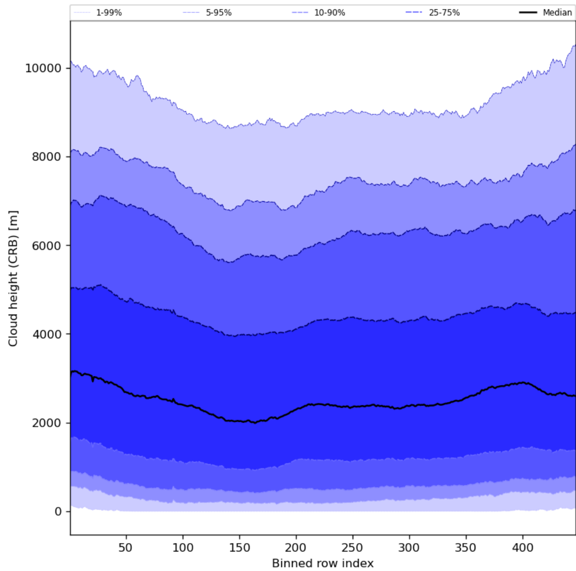
Figure 59: Along track statistics of “Cloud height (CRB)” for 2024-02-27 to 2024-02-29
