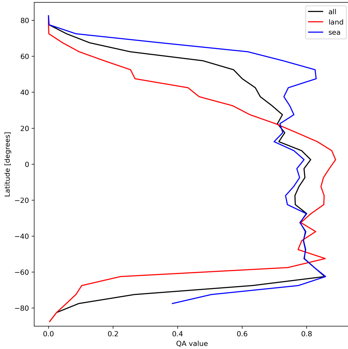
Figure 22: Zonal average of “QA value” for 2024-02-27 to 2024-02-29.
