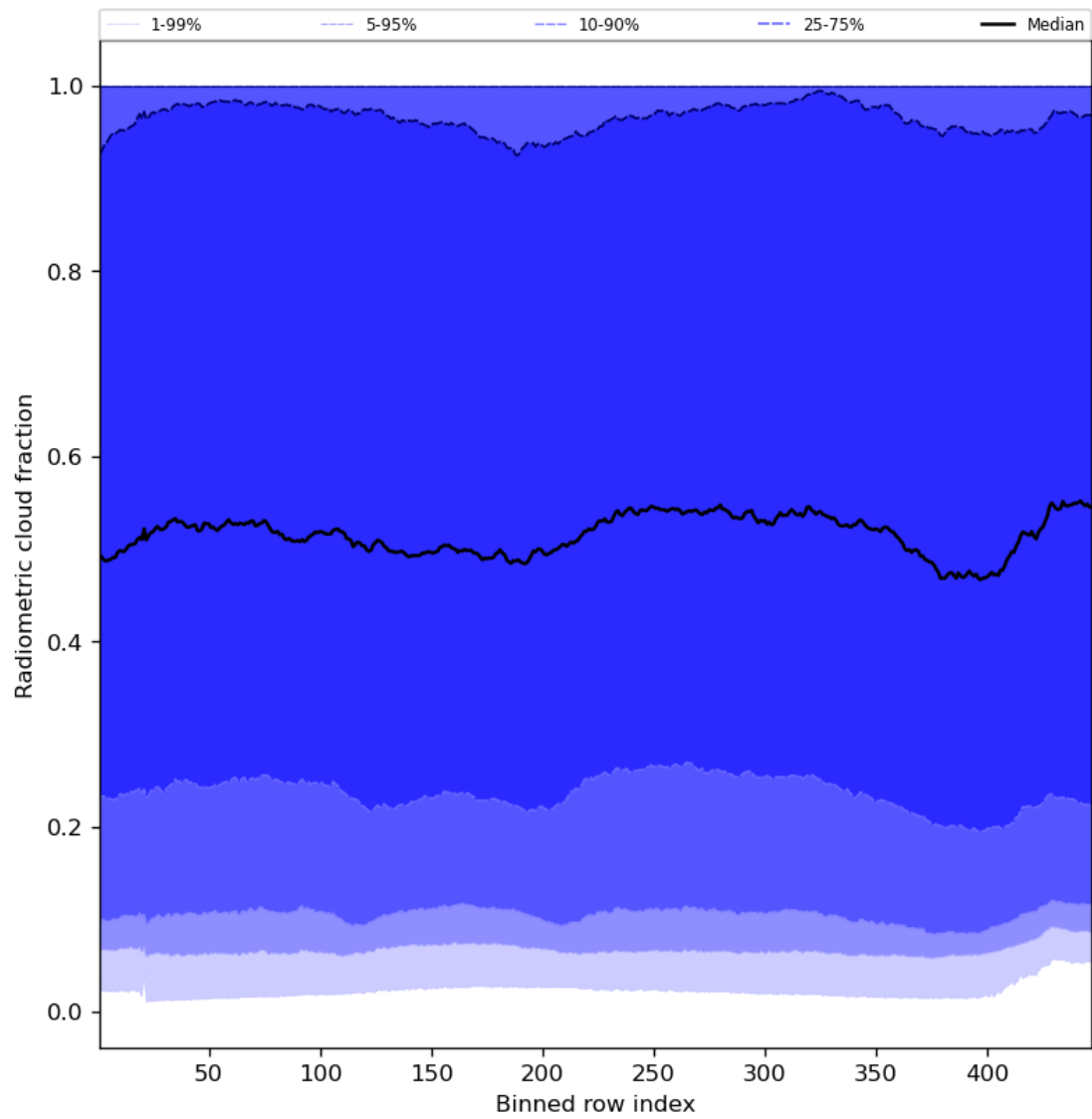
Figure 55: Along track statistics of “Radiometric cloud fraction” for 2024-02-27 to 2024-02-29
