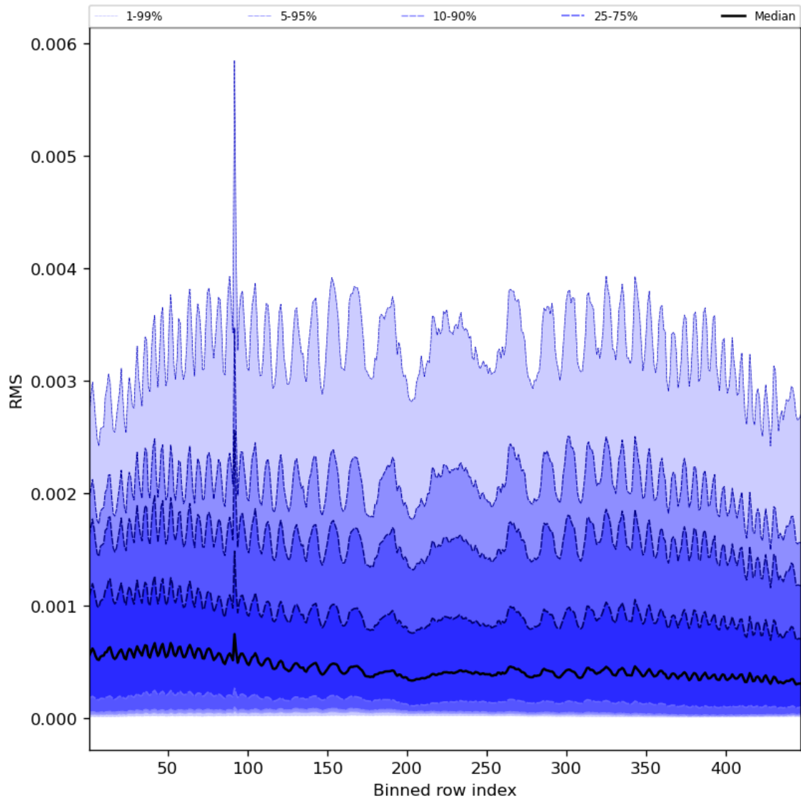
Figure 63: Along track statistics of “RMS” for 2024-02-27 to 2024-02-29
