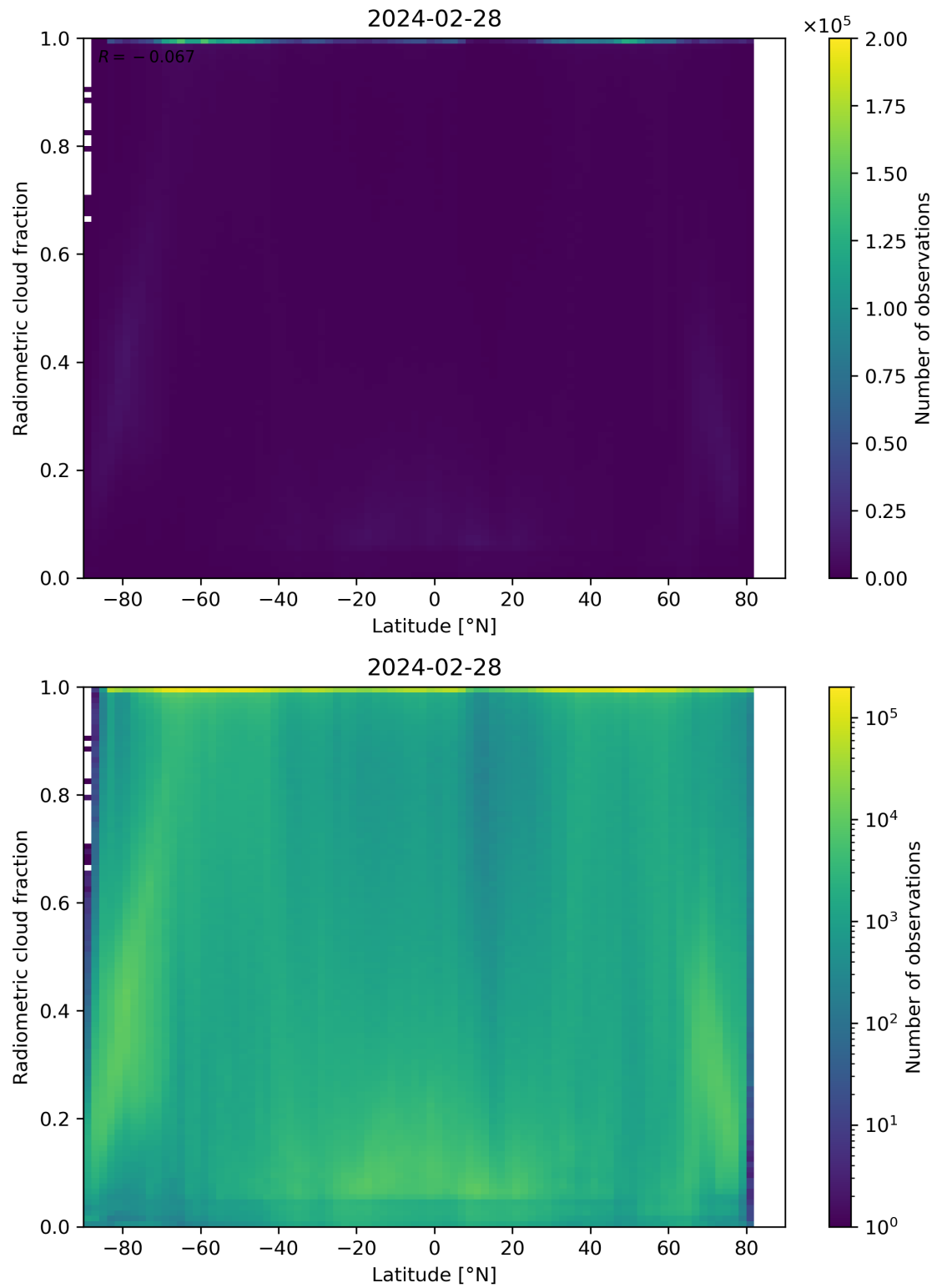
Figure 92: Scatter density plot of “Latitude” against “Radiometric cloud fraction” for 2024-02-27 to 2024-02-29.
