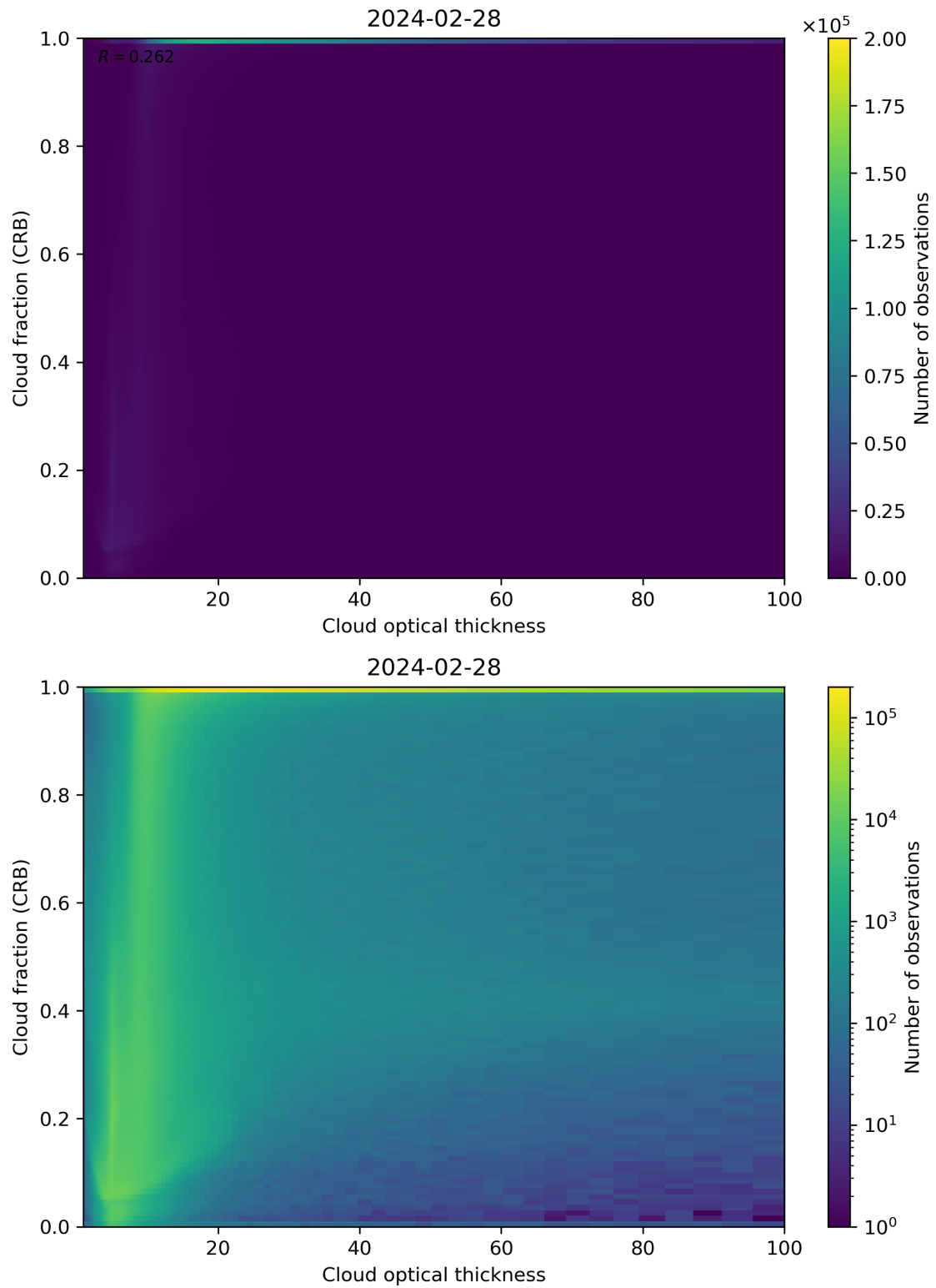
Figure 84: Scatter density plot of “Cloud optical thickness” against “Cloud fraction (CRB)” for 2024-02-27 to 2024-02-29.
