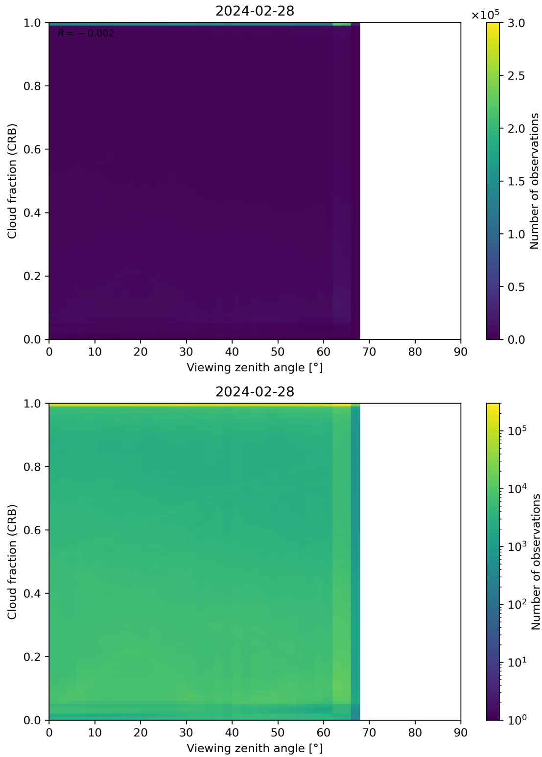
Figure 109: Scatter density plot of “Viewing zenith angle” against “Cloud fraction (CRB)” for 2024-02-27 to 2024-02-29.
