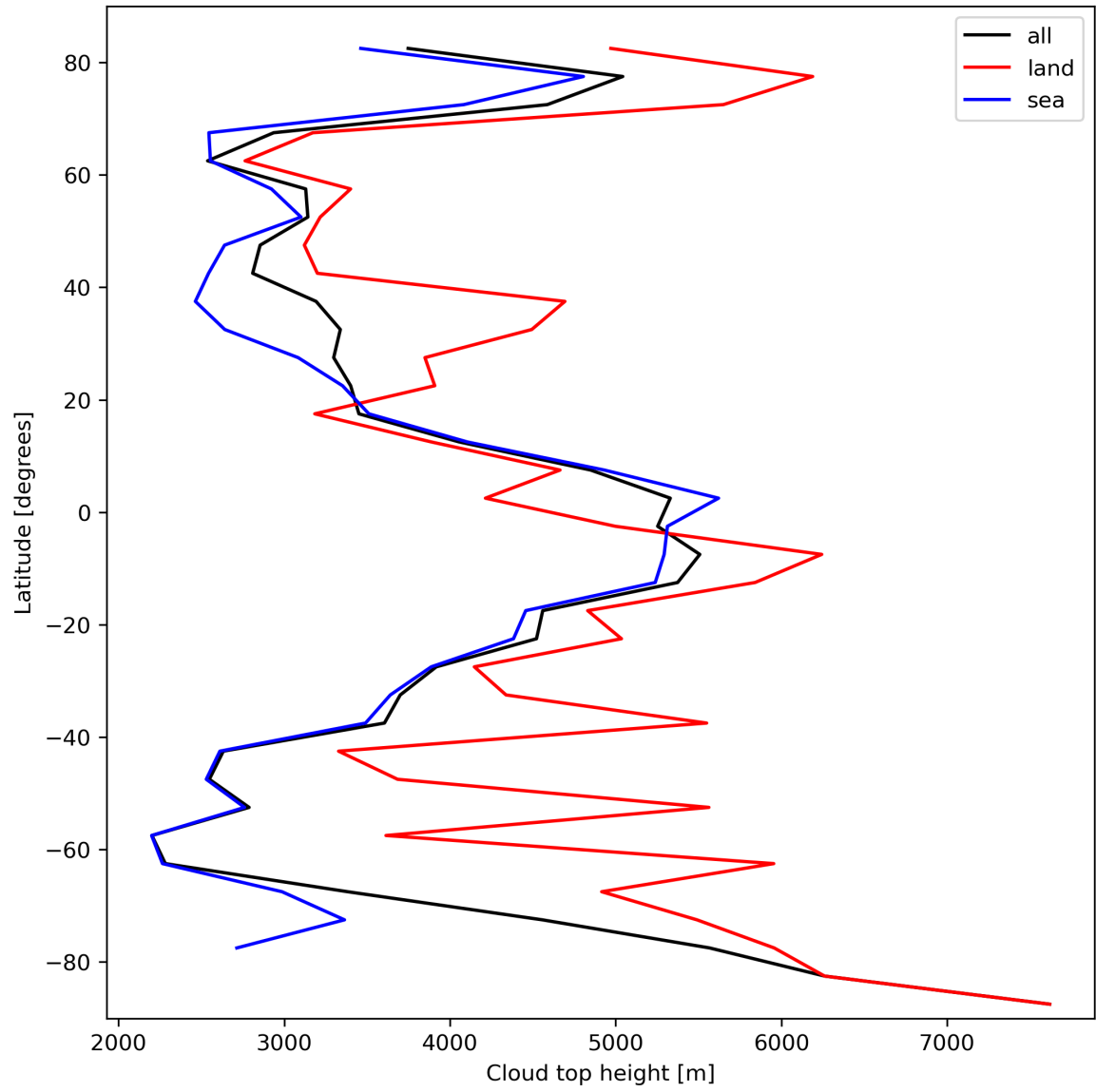
Figure 24: Zonal average of “Cloud top height” for 2024-02-27 to 2024-02-29.
