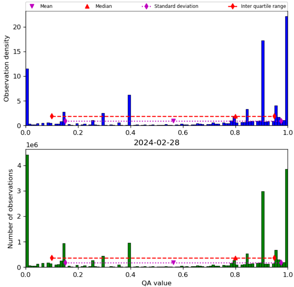
Figure 38: Histogram of “QA value” for 2024-02-27 to 2024-02-29
