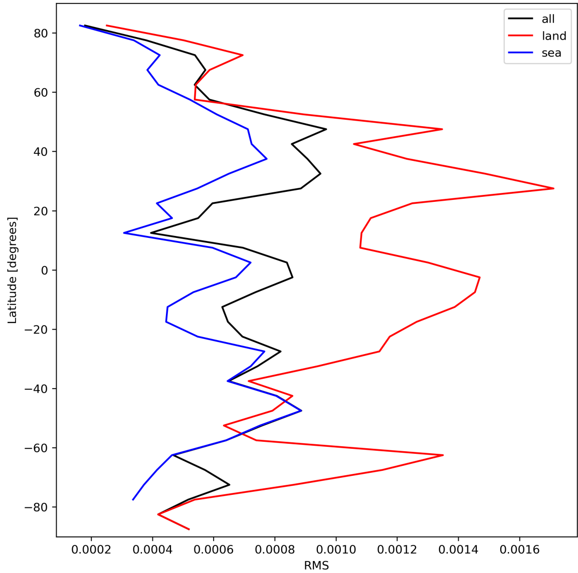
Figure 31: Zonal average of “RMS” for 2024-02-27 to 2024-02-29.
