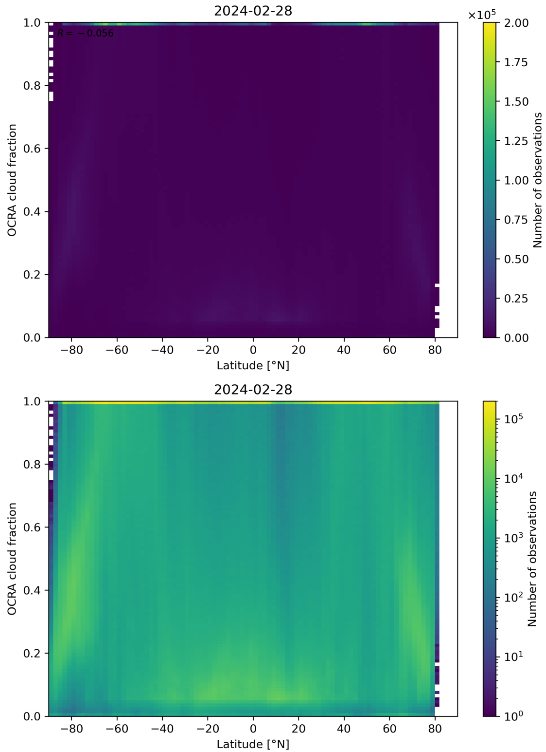
Figure 93: Scatter density plot of “Latitude” against “OCRA cloud fraction” for 2024-02-27 to 2024-02-29.
