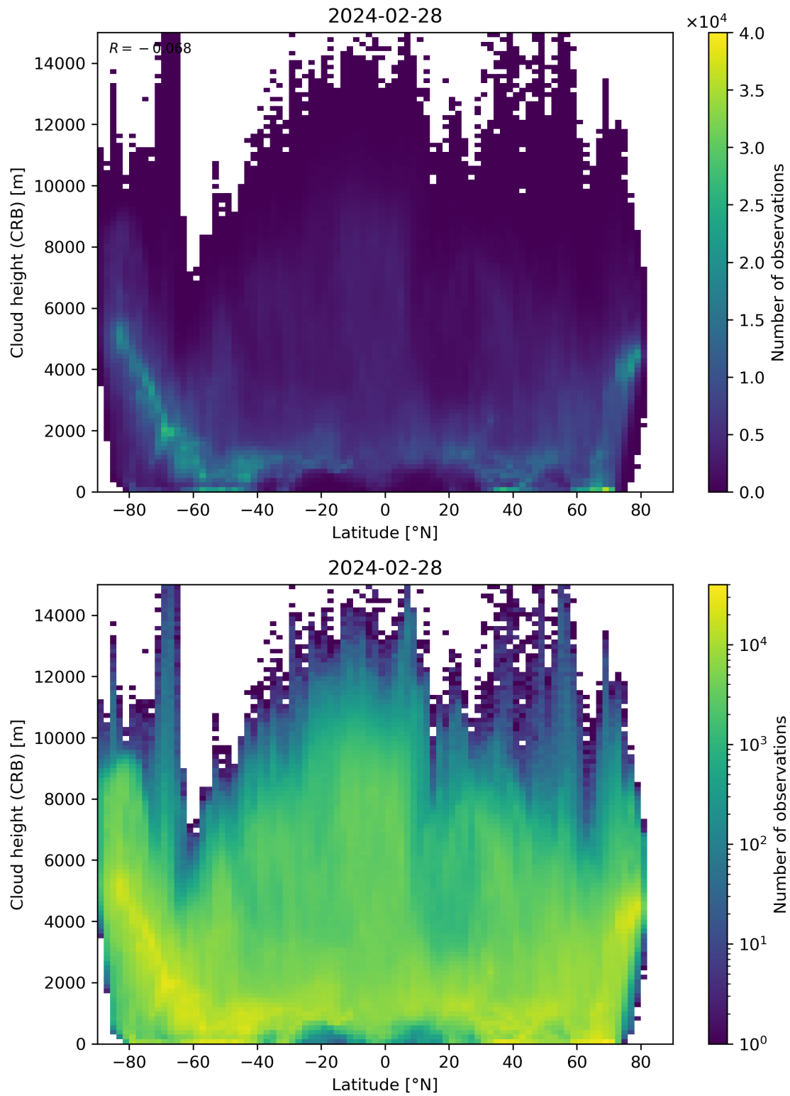
Figure 95: Scatter density plot of “Latitude” against “Cloud height (CRB)” for 2024-02-27 to 2024-02-29.
