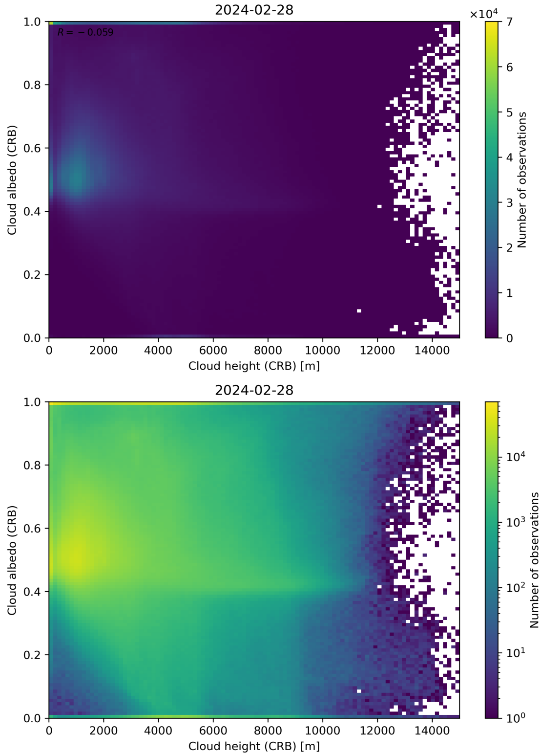
Figure 80: Scatter density plot of “Cloud height (CRB)” against “Cloud albedo (CRB)” for 2024-02-27 to 2024-02-29.
