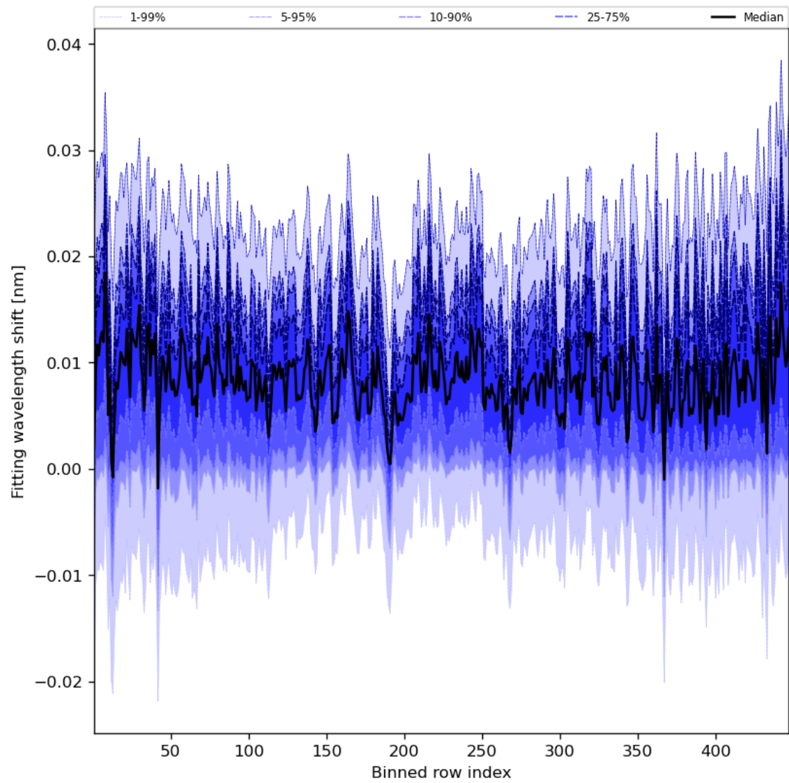
Figure 65: Along track statistics of “Fitting wavelength shift” for 2024-02-27 to 2024-02-29
