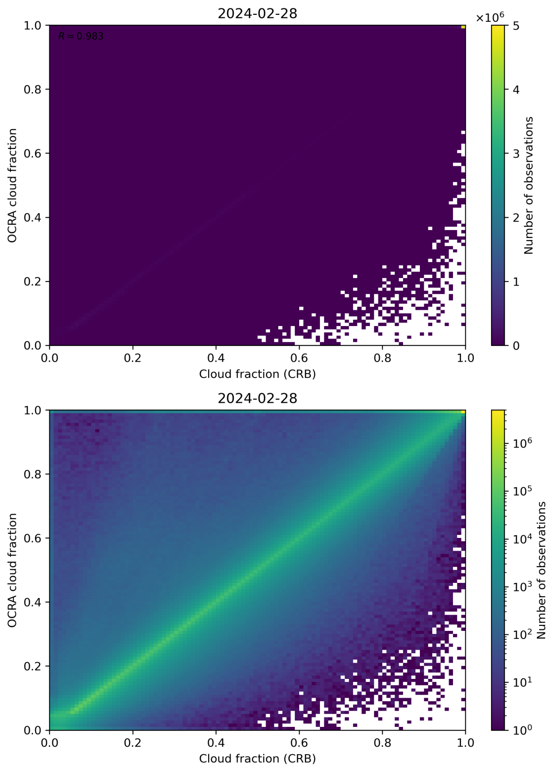
Figure 78: Scatter density plot of “Cloud fraction (CRB)” against “OCRA cloud fraction” for 2024-02-27 to 2024-02-29.
