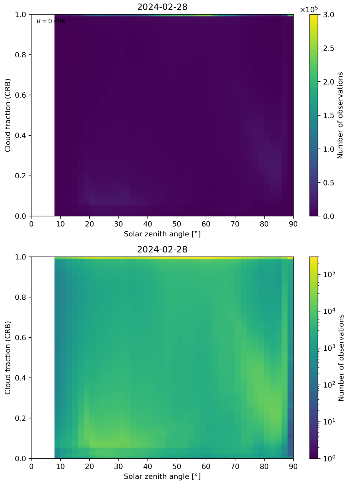
Figure 101: Scatter density plot of “Solar zenith angle” against “Cloud fraction (CRB)” for 2024-02-27 to 2024-02-29.
