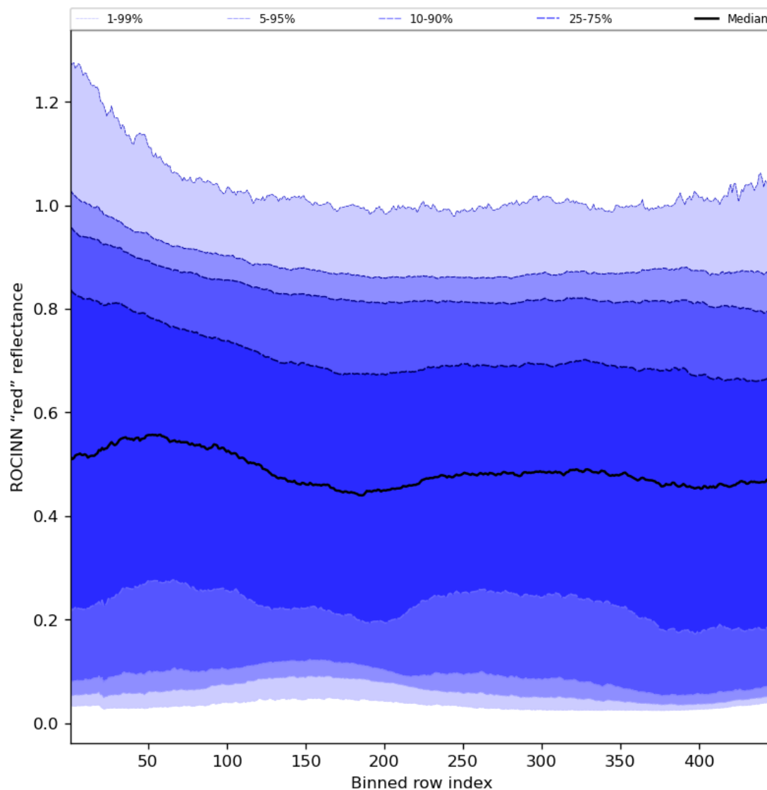
Figure 69: Along track statistics of “ROCINN “red” reflectance” for 2024-02-27 to 2024-02-29
