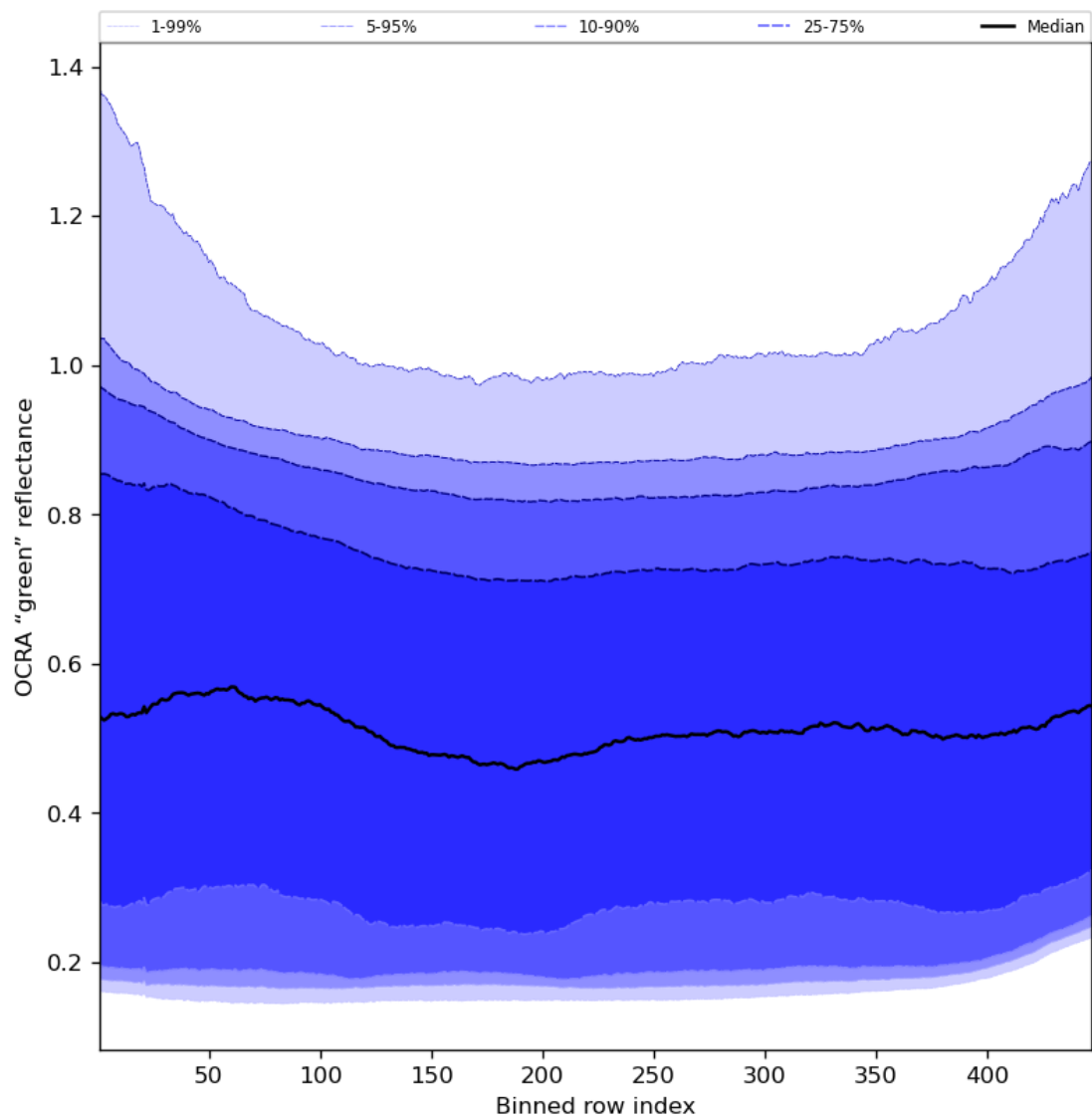
Figure 68: Along track statistics of "OCRA "green" reflectance" for 2024-02-27 to 2024-02-29
