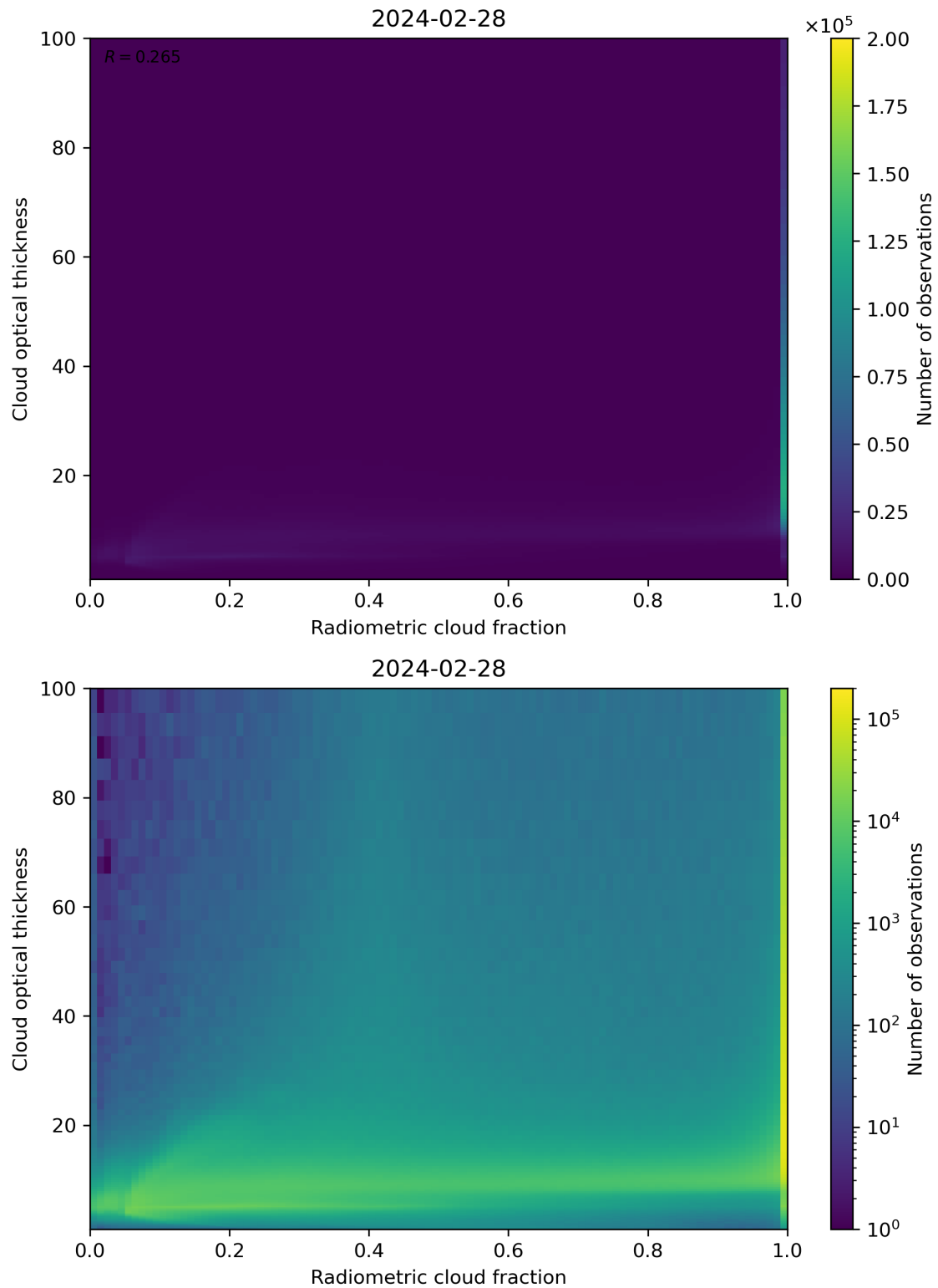
Figure 75: Scatter density plot of “Radiometric cloud fraction” against “Cloud optical thickness” for 2024-02-27 to 2024-02-29.
