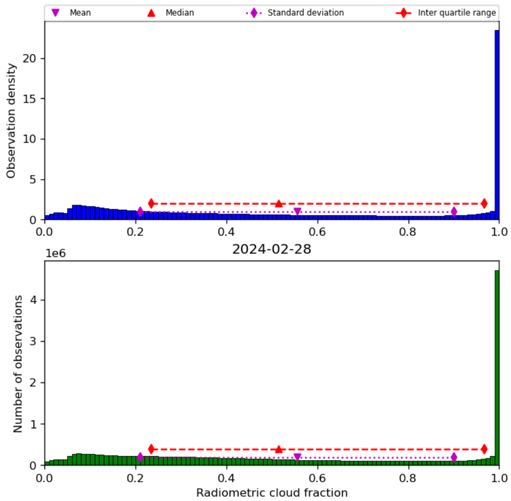
Figure 39: Histogram of “Radiometric cloud fraction” for 2024-02-27 to 2024-02-29
