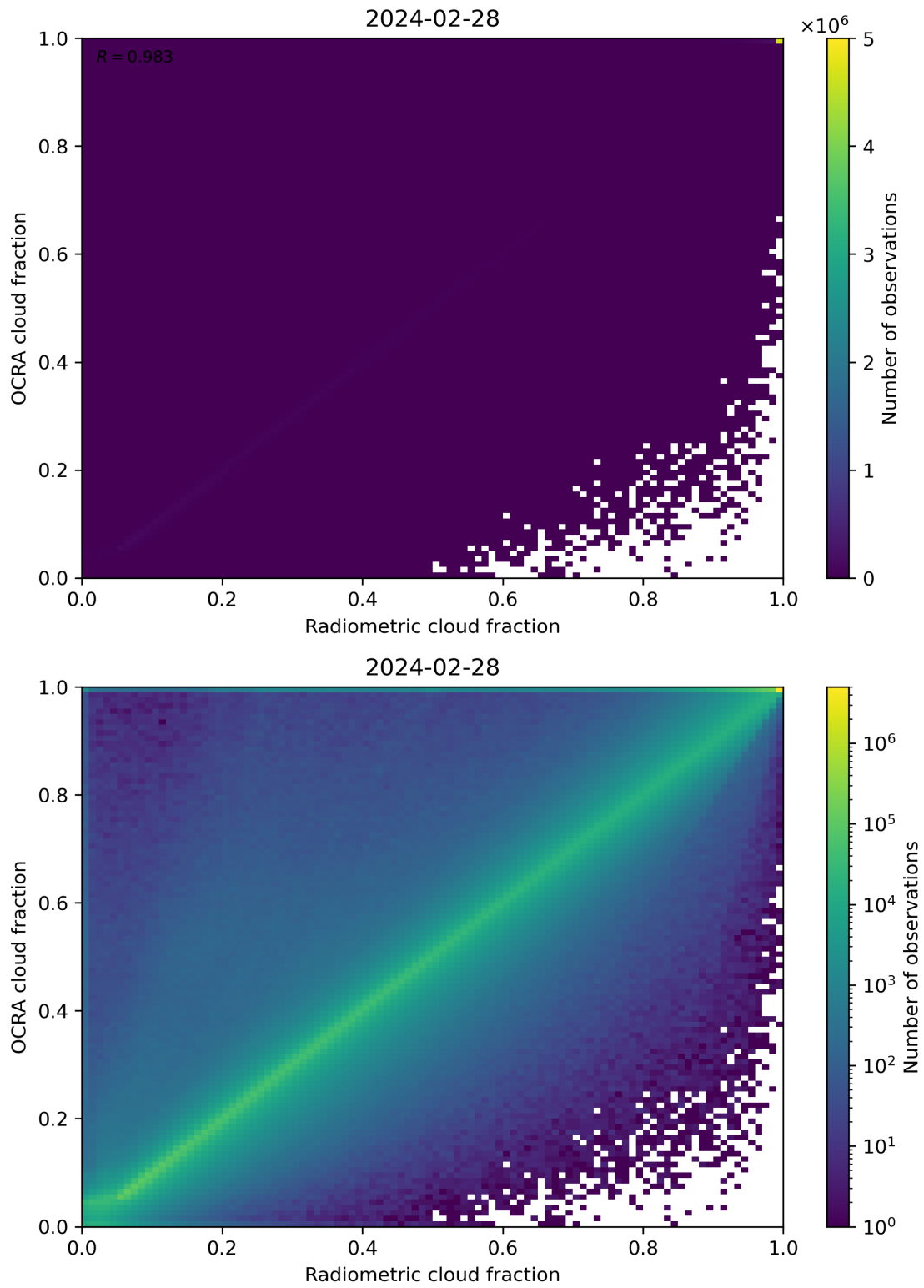
Figure 72: Scatter density plot of “Radiometric cloud fraction” against “OCRA cloud fraction” for 2024-02-27 to 2024-02-29.
