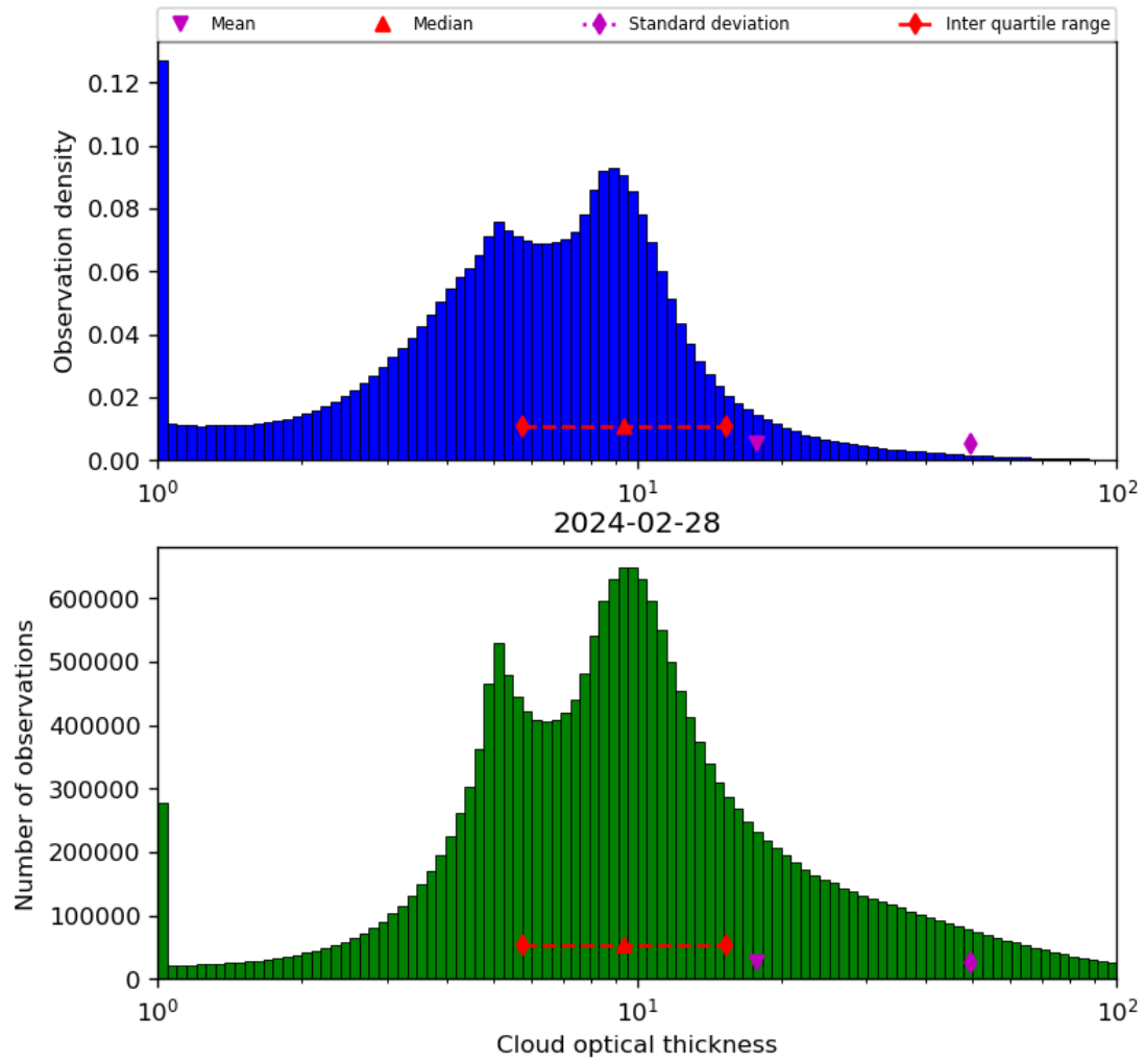
Figure 41: Histogram of “Cloud optical thickness” for 2024-02-27 to 2024-02-29
