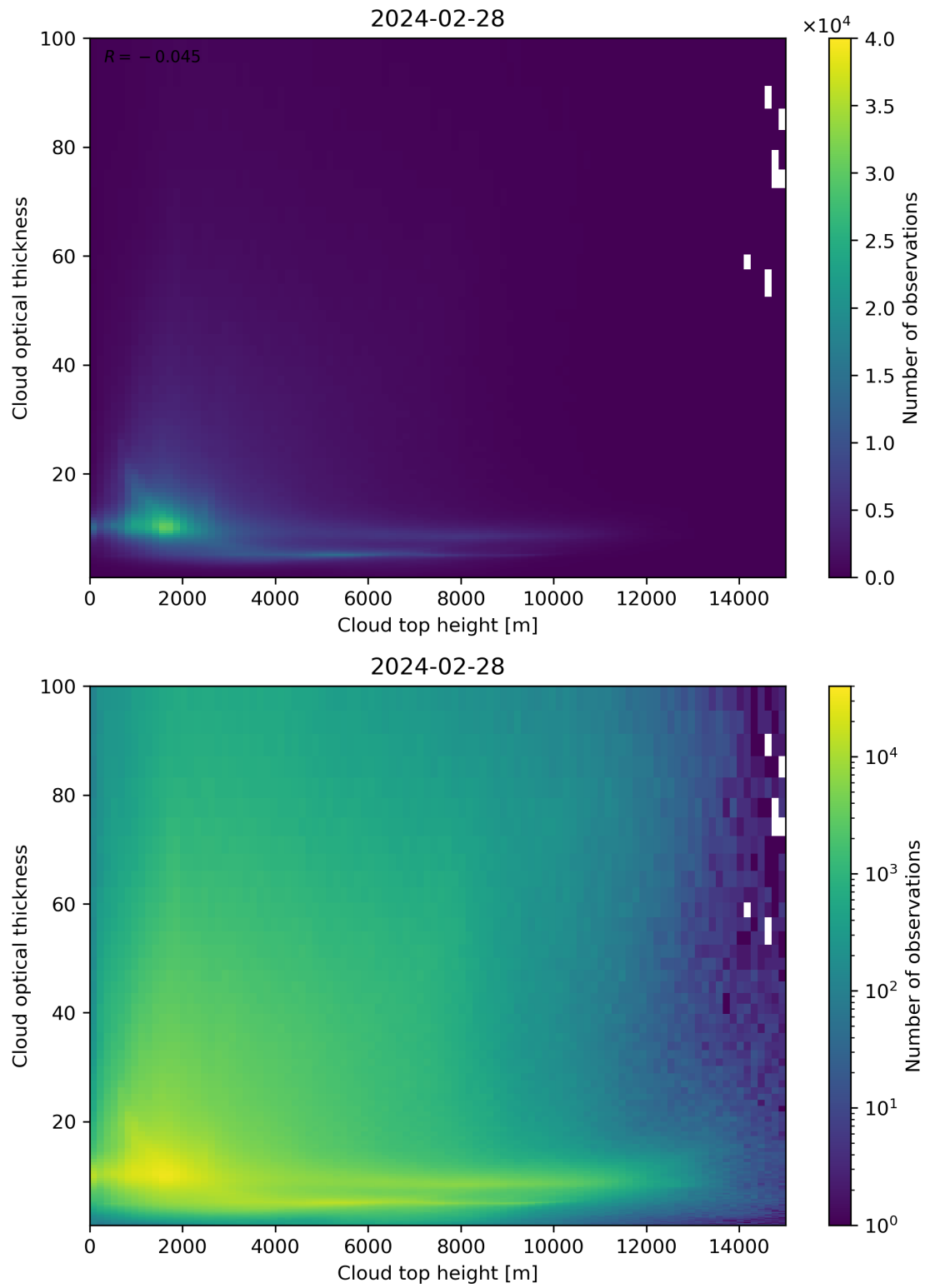
Figure 90: Scatter density plot of “Cloud top height” against “Cloud optical thickness” for 2024-02-27 to 2024-02-29.
