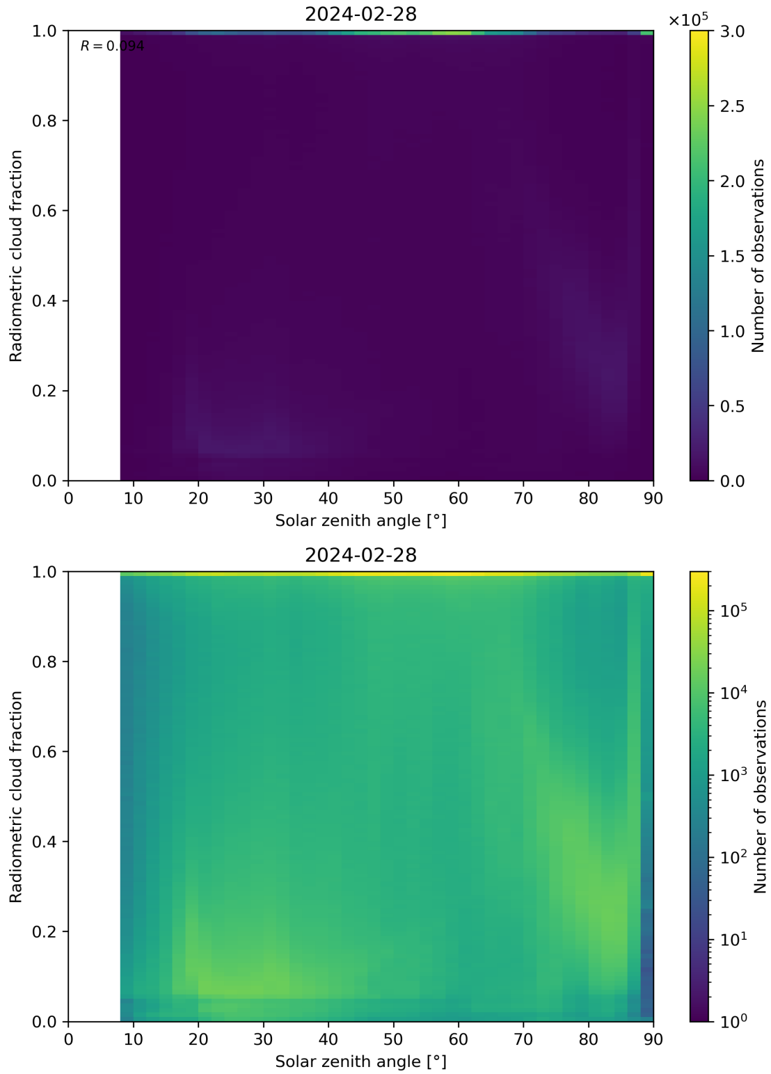
Figure 99: Scatter density plot of “Solar zenith angle” against “Radiometric cloud fraction” for 2024-02-27 to 2024-02-29.
