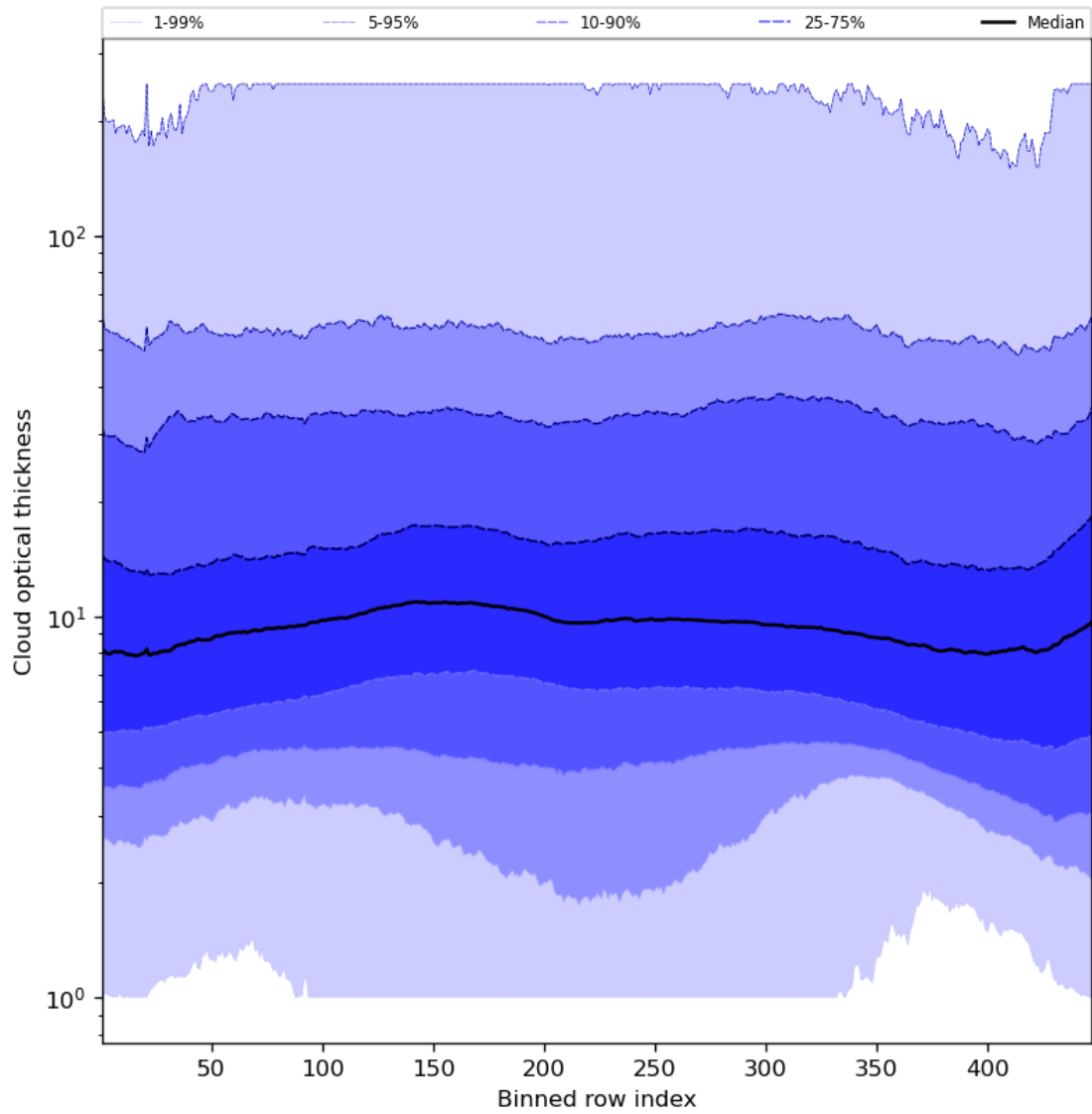
Figure 57: Along track statistics of “Cloud optical thickness” for 2024-02-27 to 2024-02-29
