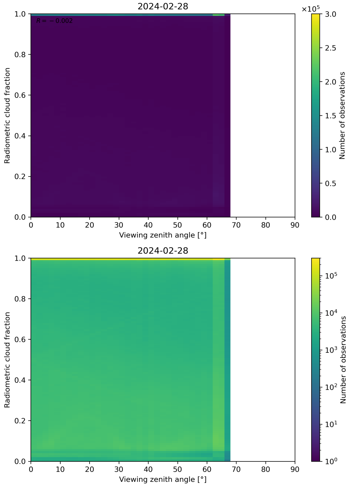
Figure 107: Scatter density plot of “Viewing zenith angle” against “Radiometric cloud fraction” for 2024-02-27 to 2024-02-29.
