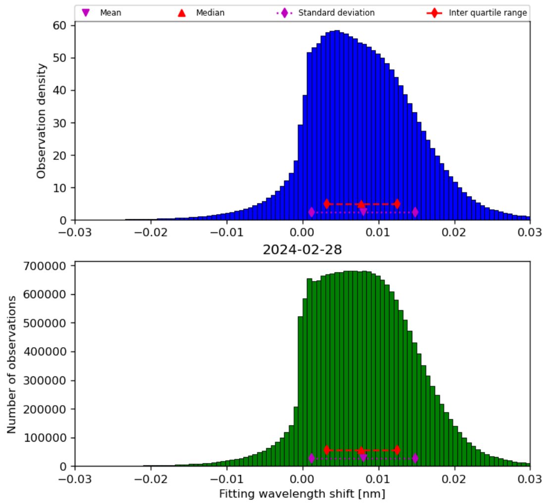
Figure 49: Histogram of “Fitting wavelength shift” for 2024-02-27 to 2024-02-29
