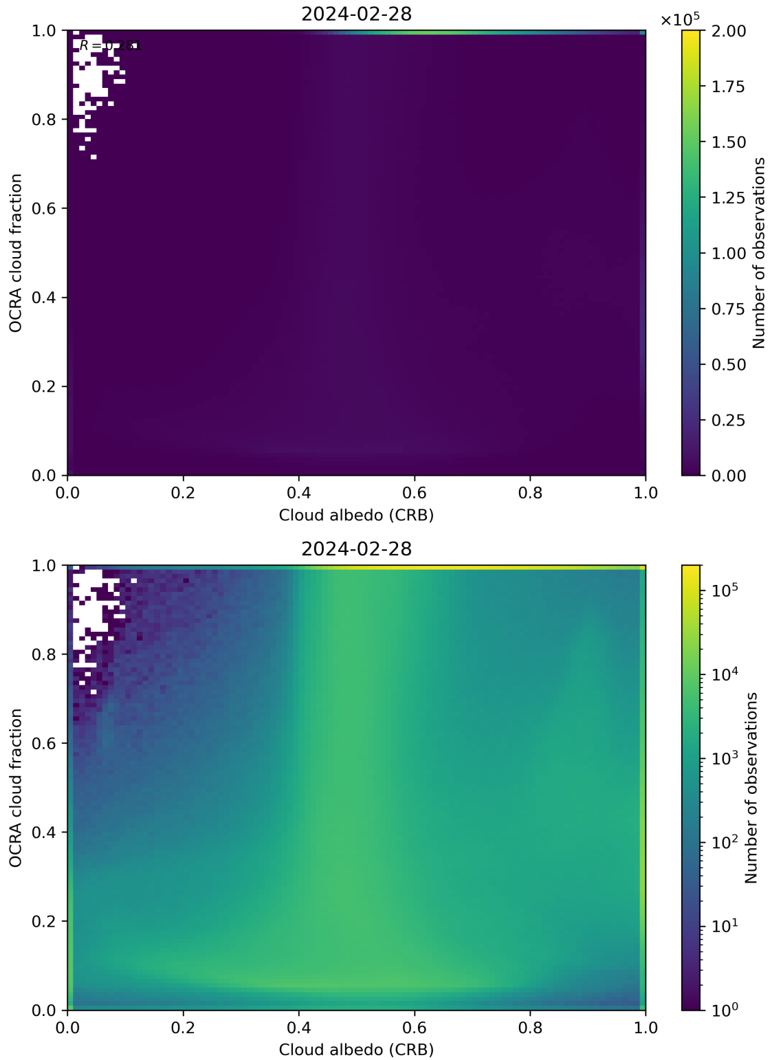
Figure 70: Scatter density plot of “Cloud albedo (CRB)” against “OCRA cloud fraction” for 2024-02-27 to 2024-02-29.
