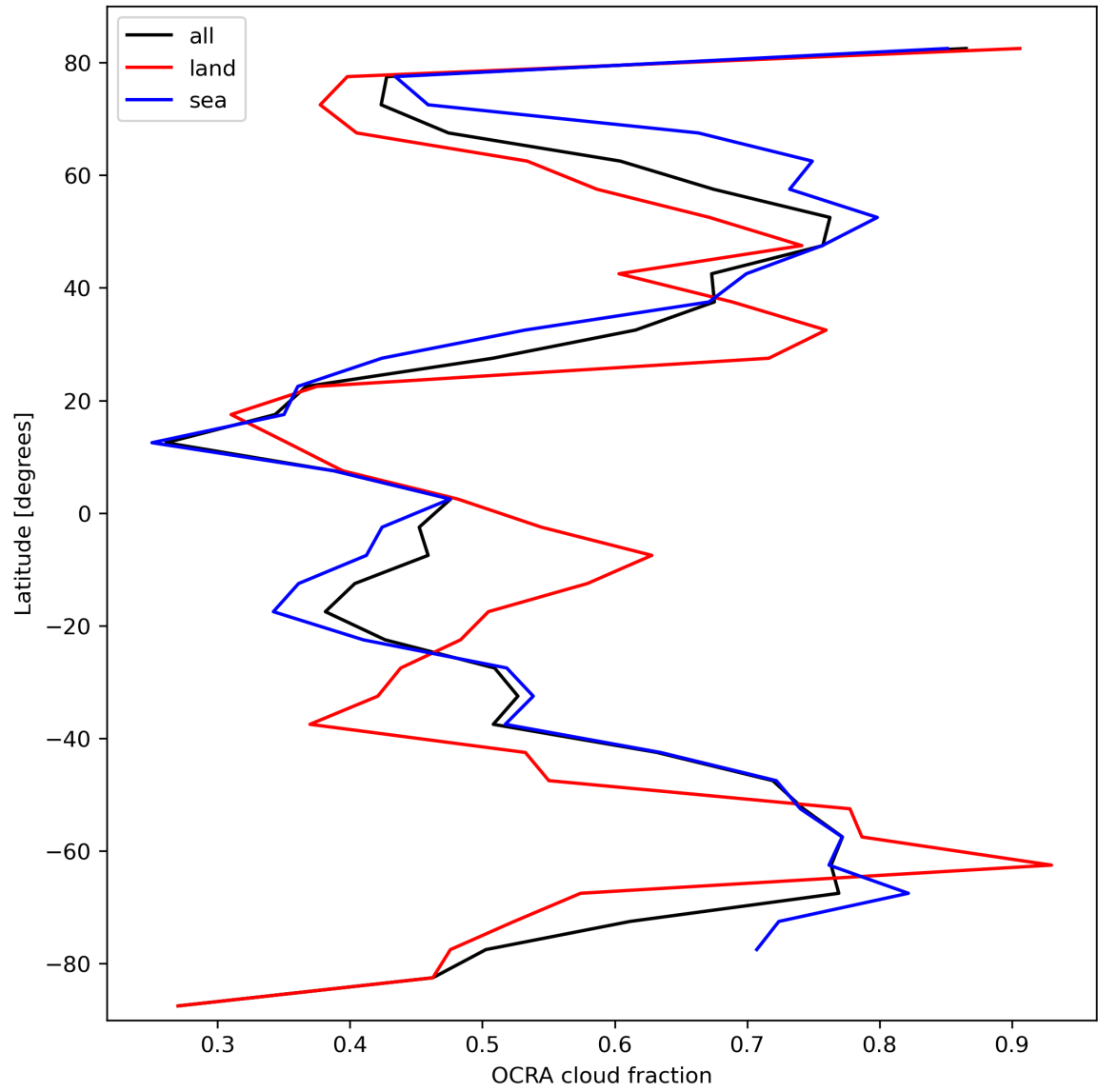
Figure 34: Zonal average of “OCRA cloud fraction” for 2024-02-27 to 2024-02-29.
