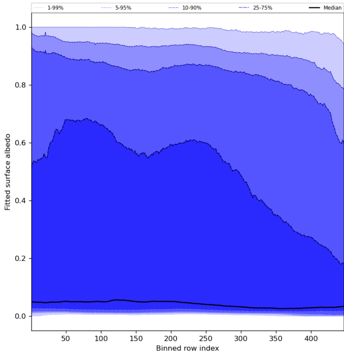
Figure 61: Along track statistics of “Fitted surface albedo” for 2024-02-27 to 2024-02-29
