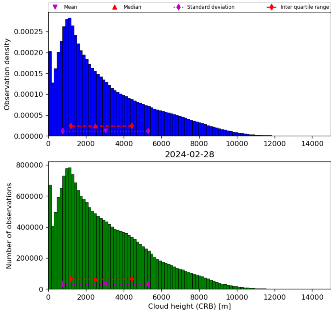
Figure 43: Histogram of “Cloud height (CRB)” for 2024-02-27 to 2024-02-29
