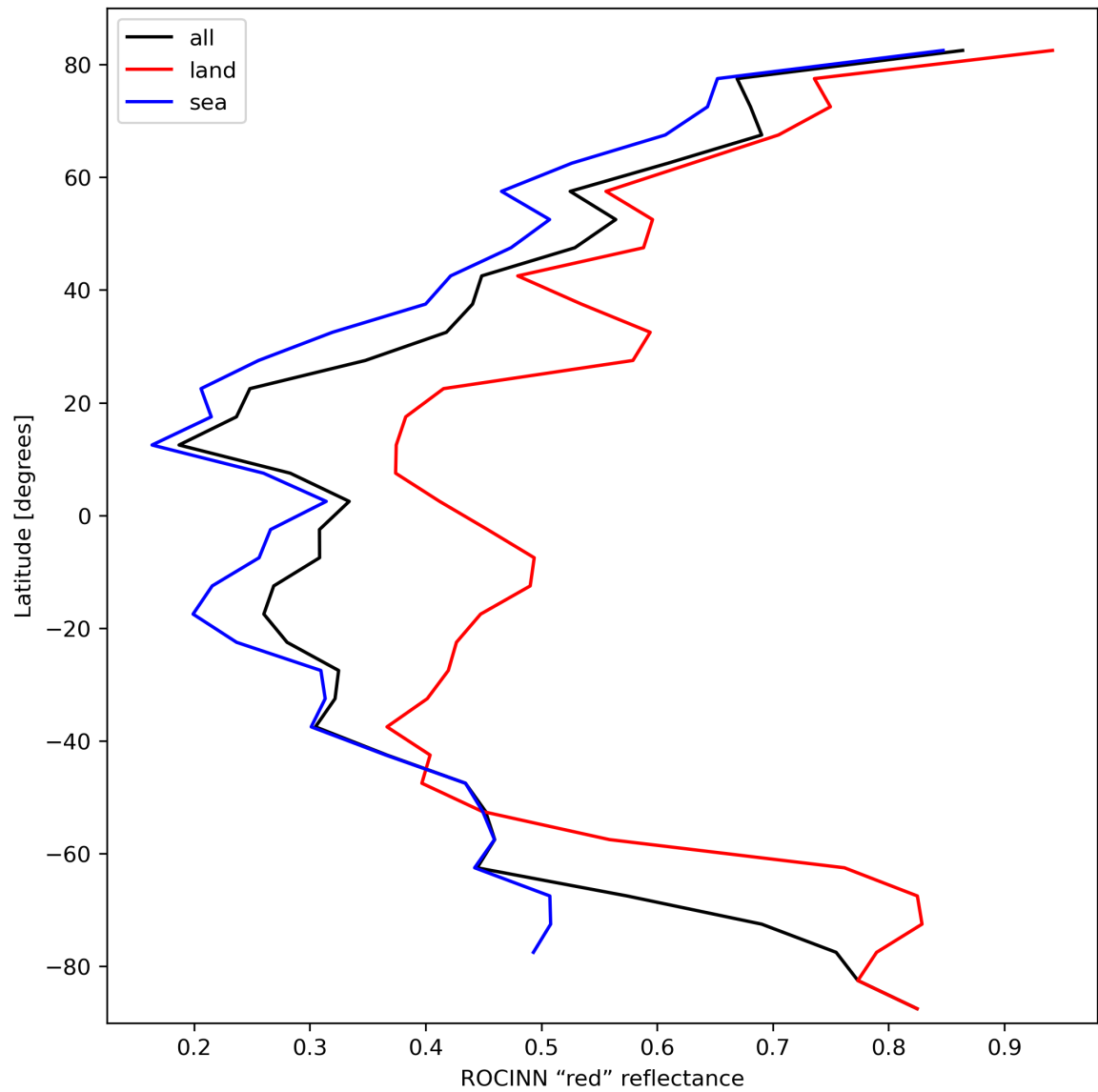
Figure 37: Zonal average of “ROCINN “red” reflectance” for 2024-02-27 to 2024-02-29.
