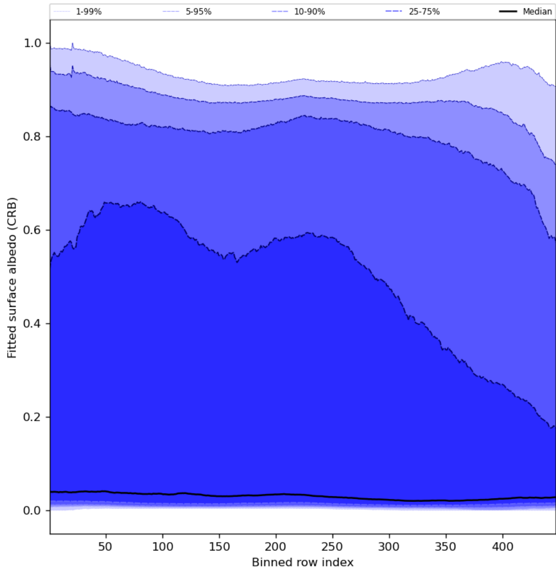
Figure 62: Along track statistics of “Fitted surface albedo (CRB)” for 2024-02-27 to 2024-02-29
