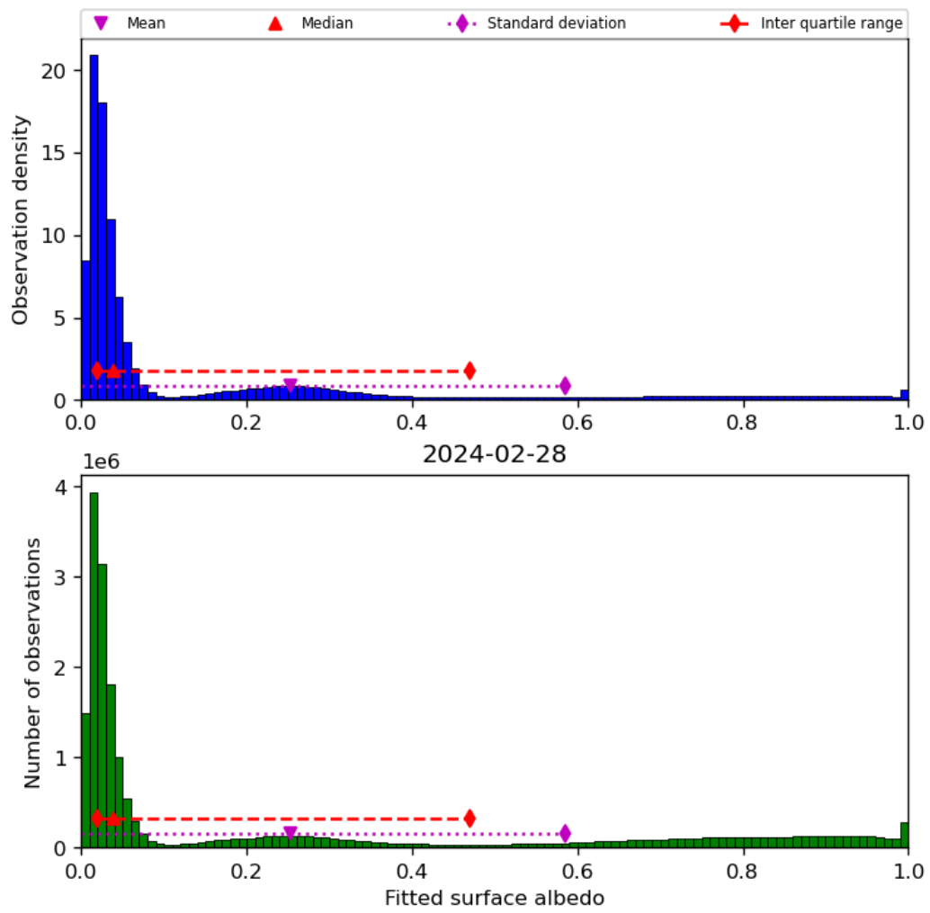
Figure 45: Histogram of “Fitted surface albedo” for 2024-02-27 to 2024-02-29
