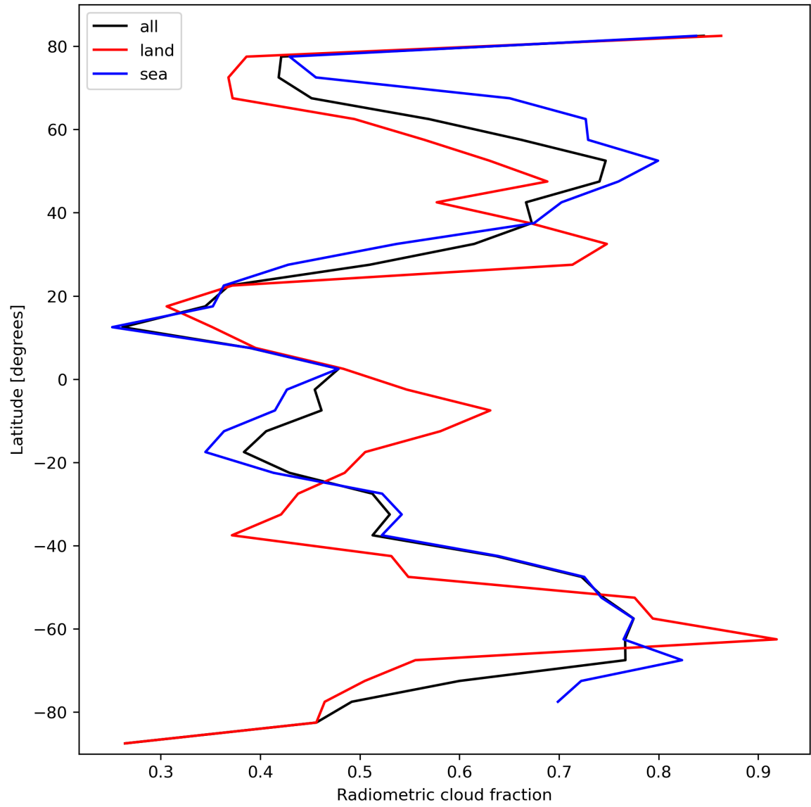
Figure 23: Zonal average of “Radiometric cloud fraction” for 2024-02-27 to 2024-02-29.
