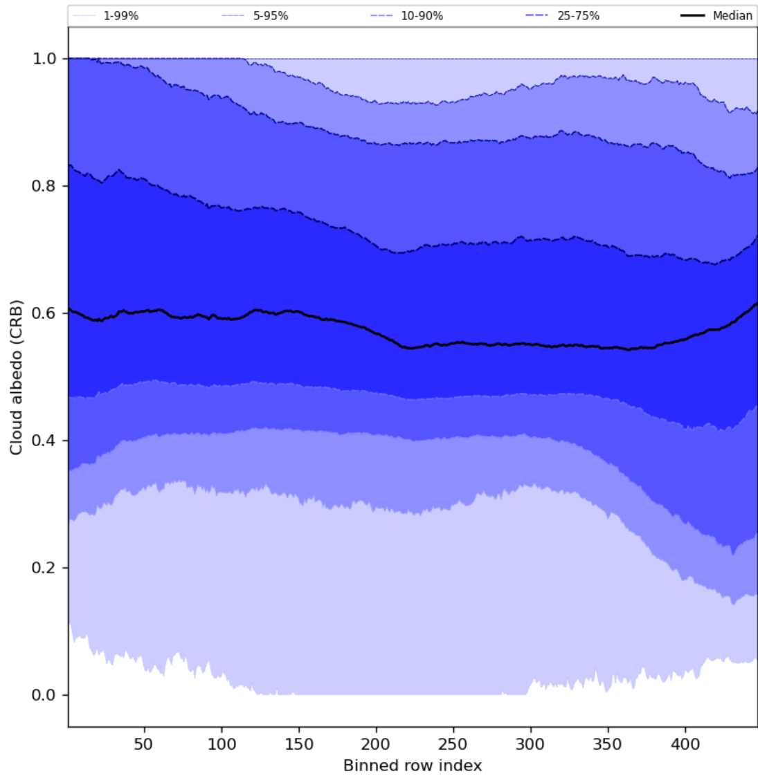
Figure 60: Along track statistics of “Cloud albedo (CRB)” for 2024-02-27 to 2024-02-29
