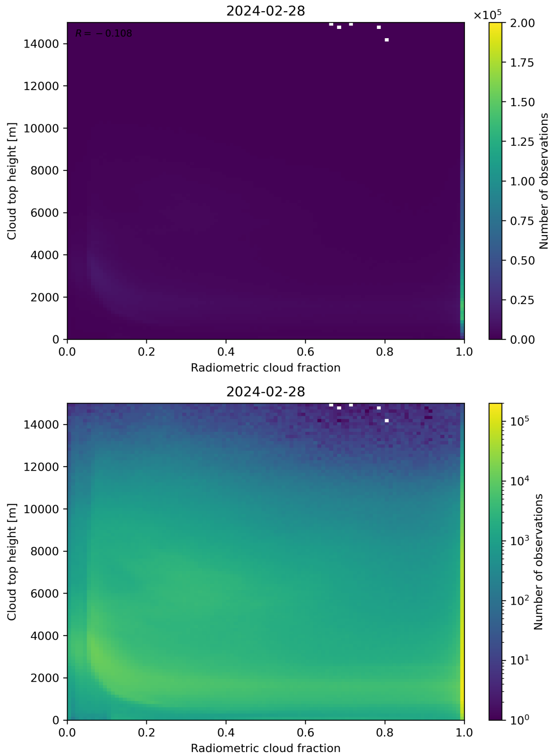
Figure 76: Scatter density plot of “Radiometric cloud fraction” against “Cloud top height” for 2024-02-27 to 2024-02-29.
