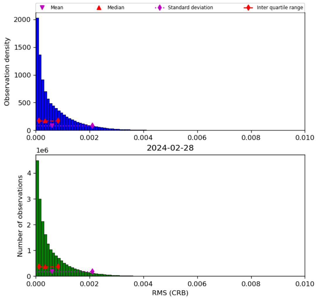
Figure 48: Histogram of “RMS (CRB)” for 2024-02-27 to 2024-02-29
