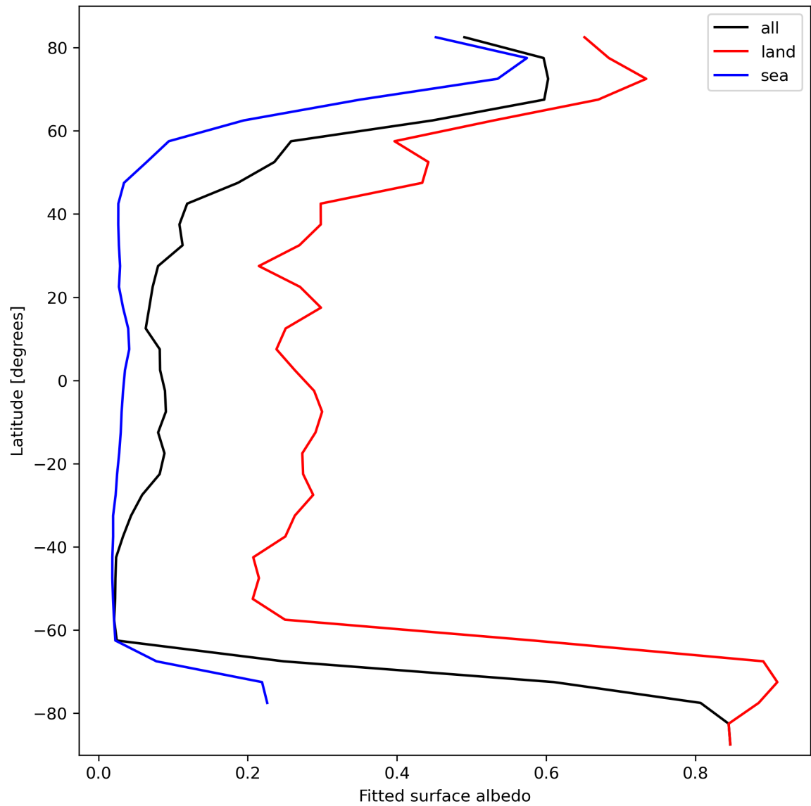
Figure 29: Zonal average of “Fitted surface albedo” for 2024-02-27 to 2024-02-29.
