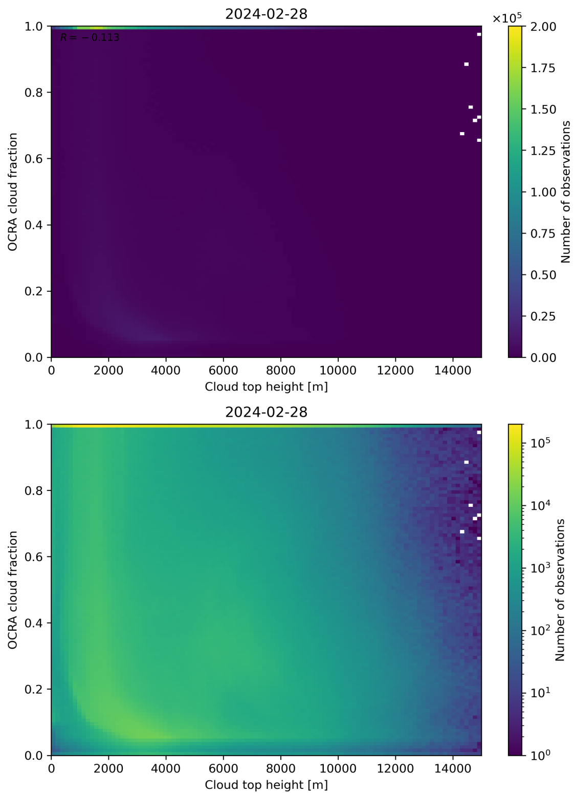
Figure 87: Scatter density plot of “Cloud top height” against “OCRA cloud fraction” for 2024-02-27 to 2024-02-29.
