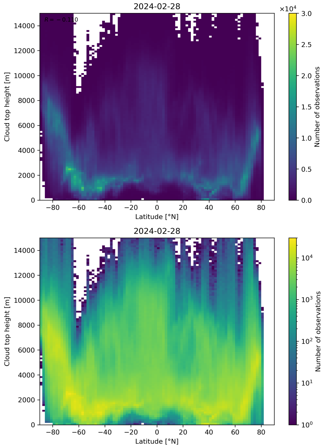
Figure 97: Scatter density plot of “Latitude” against “Cloud top height” for 2024-02-27 to 2024-02-29.
