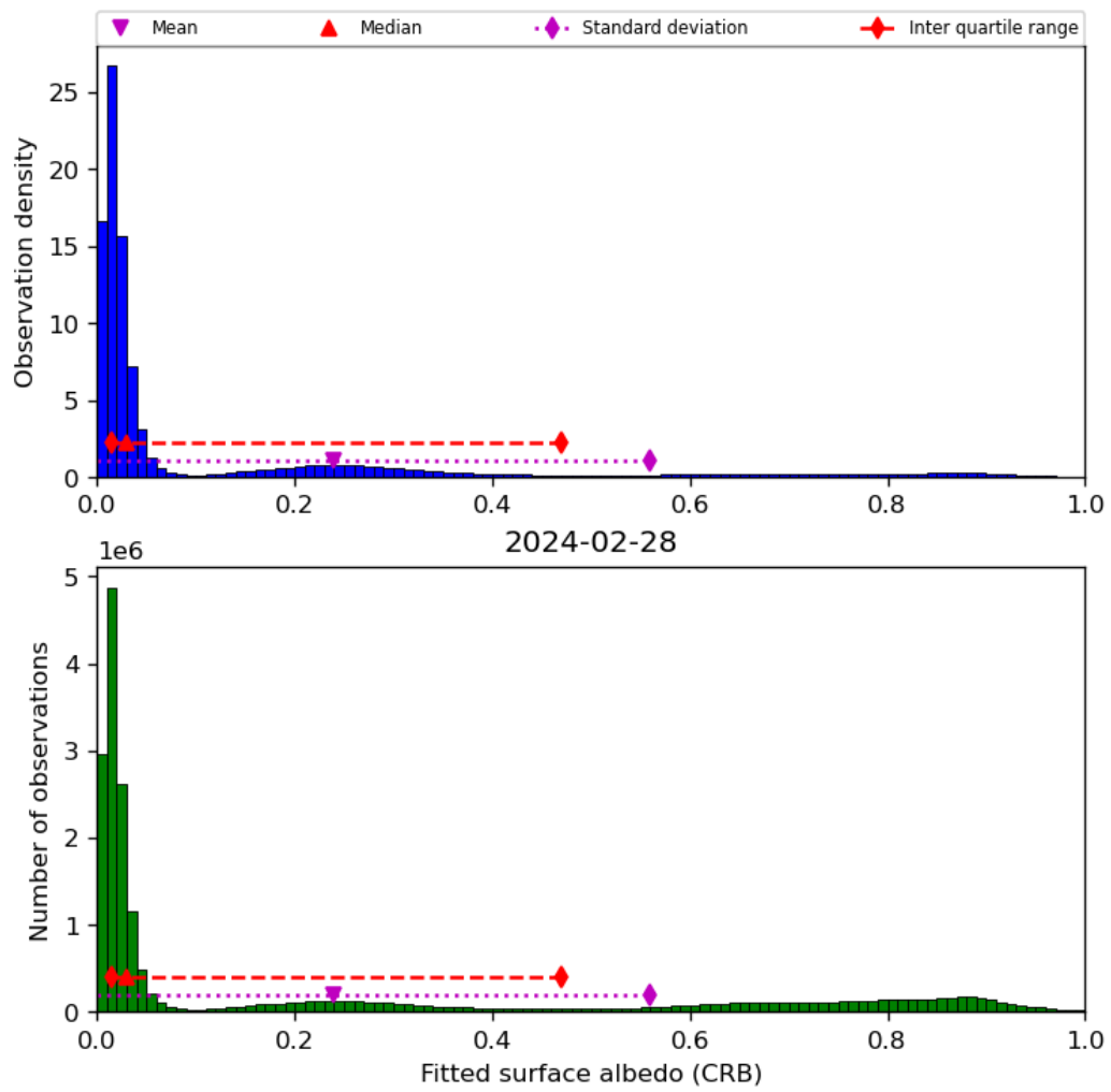
Figure 46: Histogram of “Fitted surface albedo (CRB)” for 2024-02-27 to 2024-02-29
