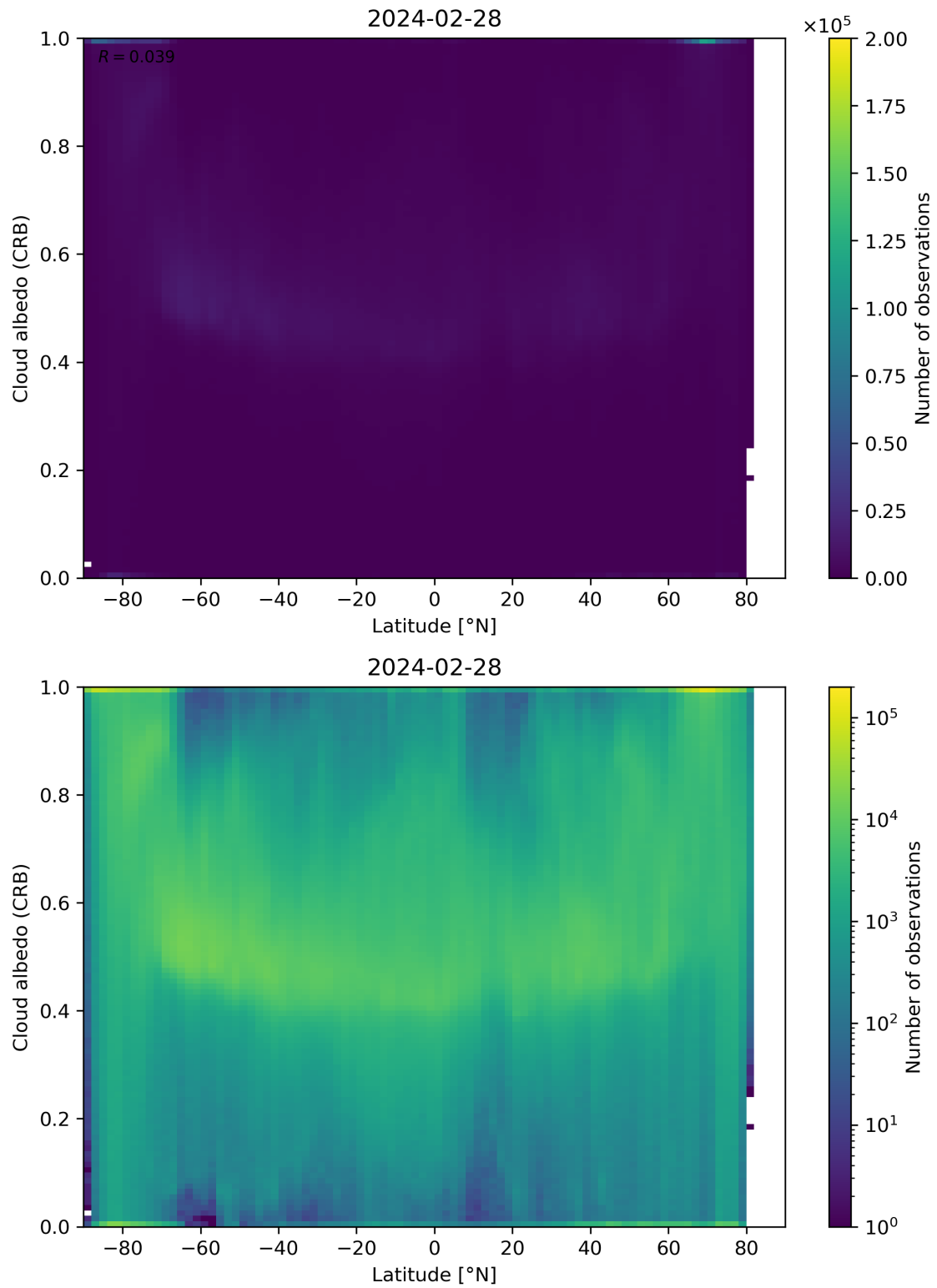
Figure 91: Scatter density plot of “Latitude” against “Cloud albedo (CRB)” for 2024-02-27 to 2024-02-29.
