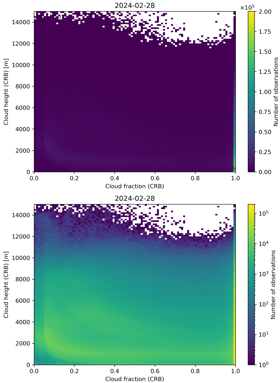
Figure 79: Scatter density plot of “Cloud fraction (CRB)” against “Cloud height (CRB)” for 2024-02-27 to 2024-02-29.
