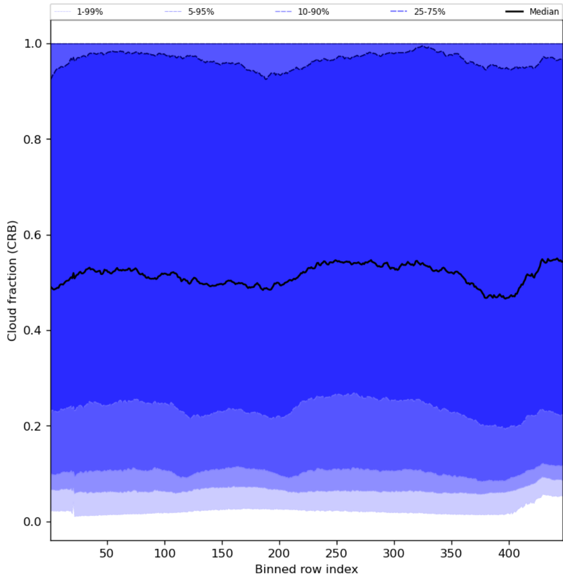
Figure 58: Along track statistics of “Cloud fraction (CRB)” for 2024-02-27 to 2024-02-29
