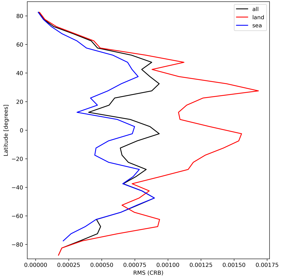
Figure 32: Zonal average of “RMS (CRB)” for 2024-02-27 to 2024-02-29.
