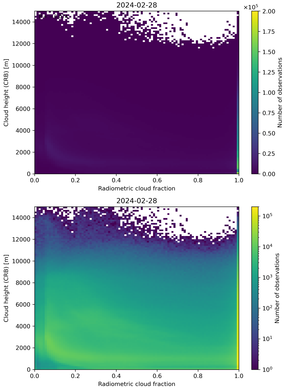
Figure 74: Scatter density plot of “Radiometric cloud fraction” against “Cloud height (CRB)” for 2024-02-27 to 2024-02-29.
