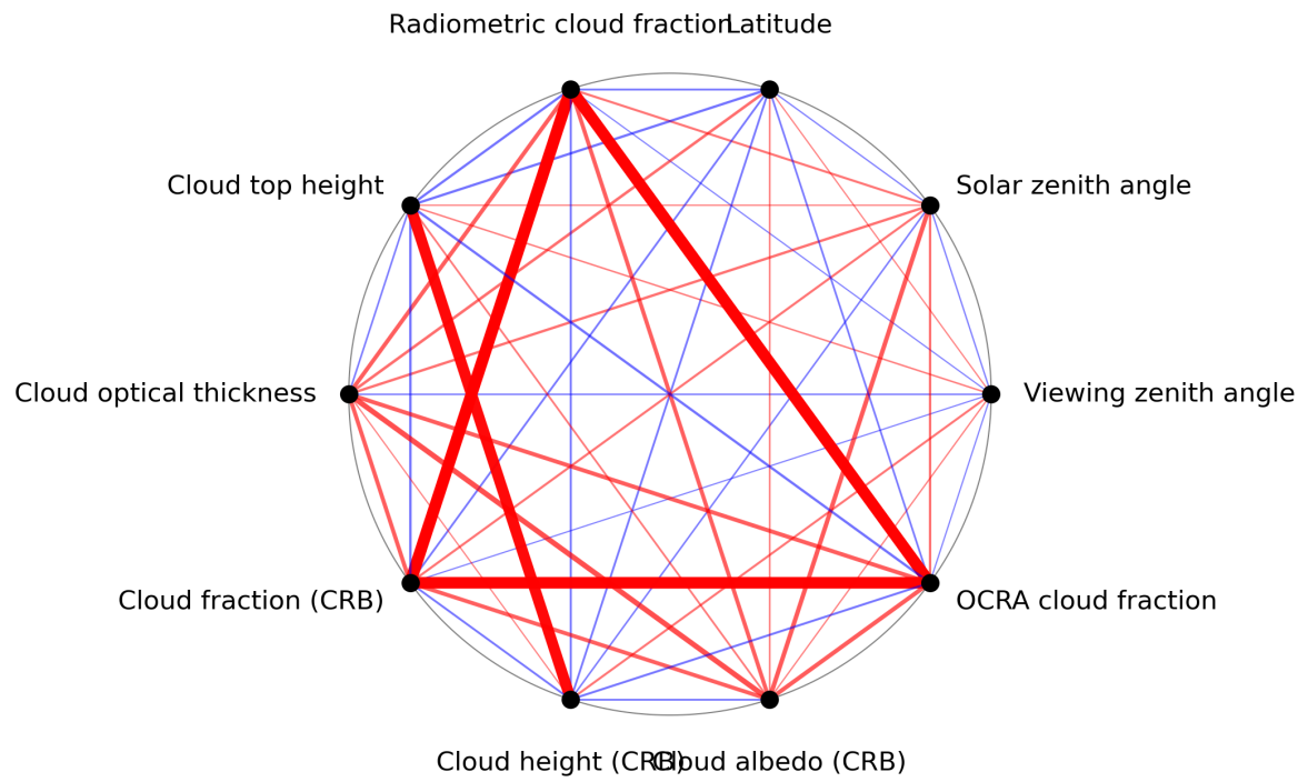
Figure 1: Map of correlation graph for 2024-02-27 to 2024-02-29.
