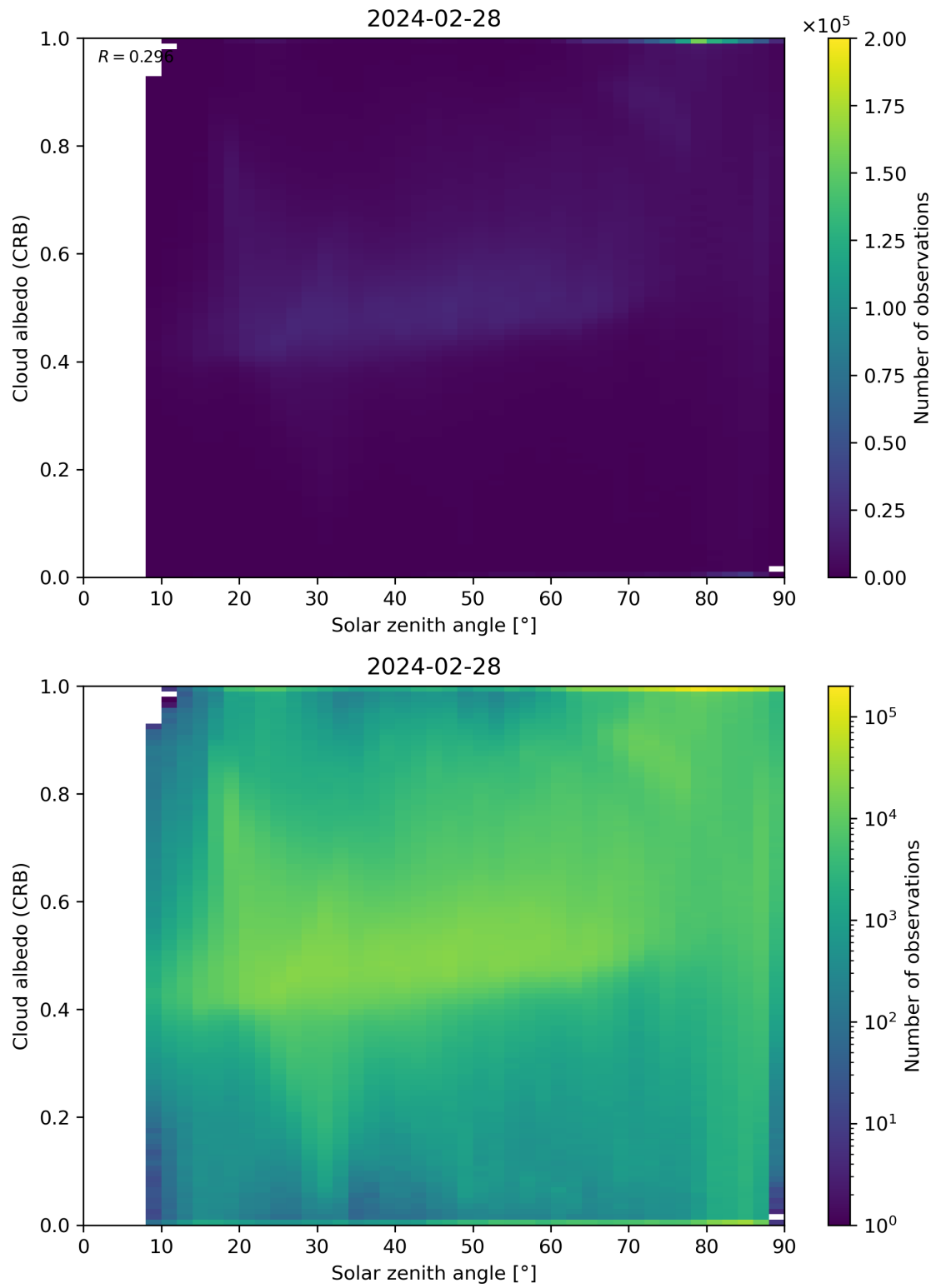
Figure 98: Scatter density plot of “Solar zenith angle” against “Cloud albedo (CRB)” for 2024-02-27 to 2024-02-29.
