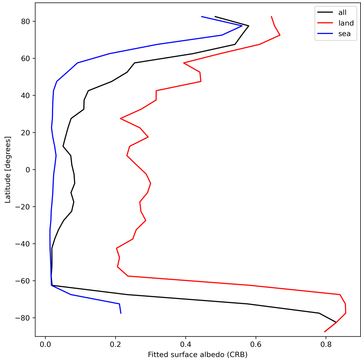
Figure 30: Zonal average of “Fitted surface albedo (CRB)” for 2024-02-27 to 2024-02-29.
