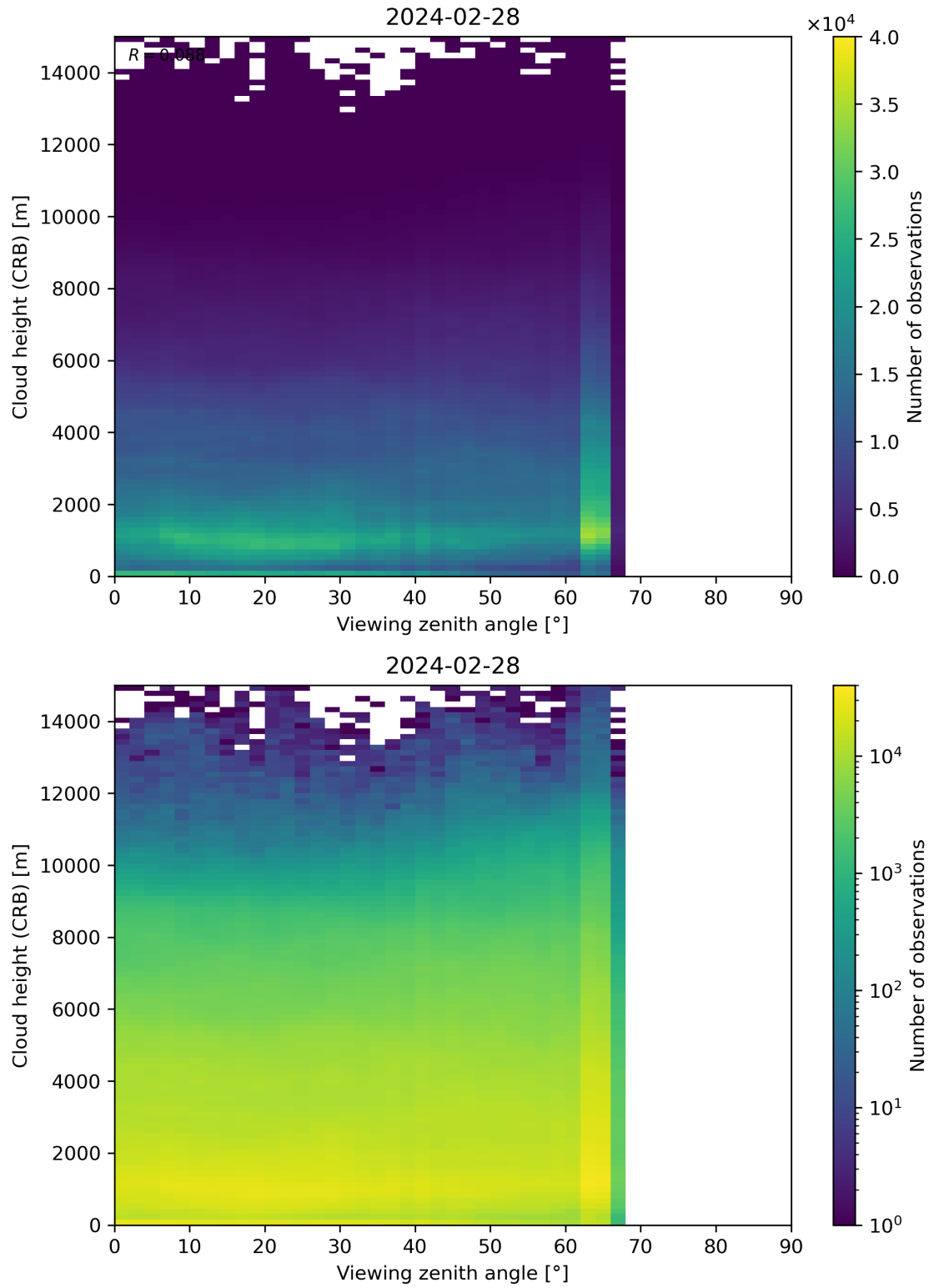
Figure 110: Scatter density plot of “Viewing zenith angle” against “Cloud height (CRB)” for 2024-02-27 to 2024-02-29.
