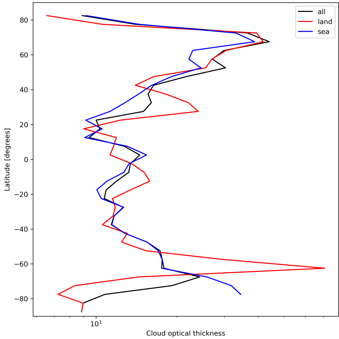
Figure 25: Zonal average of “Cloud optical thickness” for 2024-02-27 to 2024-02-29.
