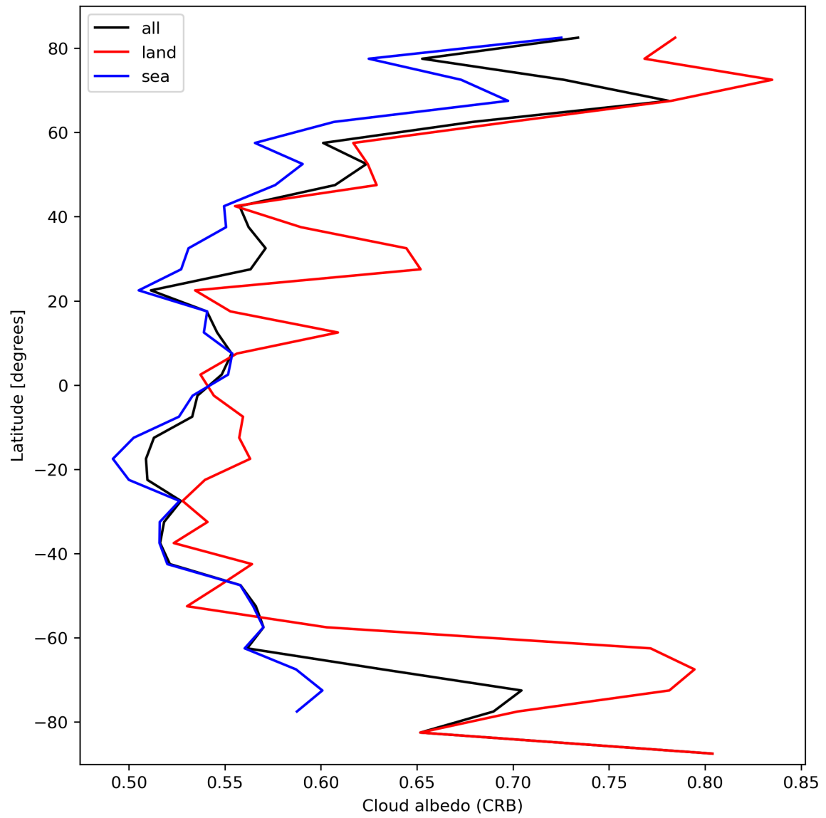
Figure 28: Zonal average of “Cloud albedo (CRB)” for 2024-02-27 to 2024-02-29.
