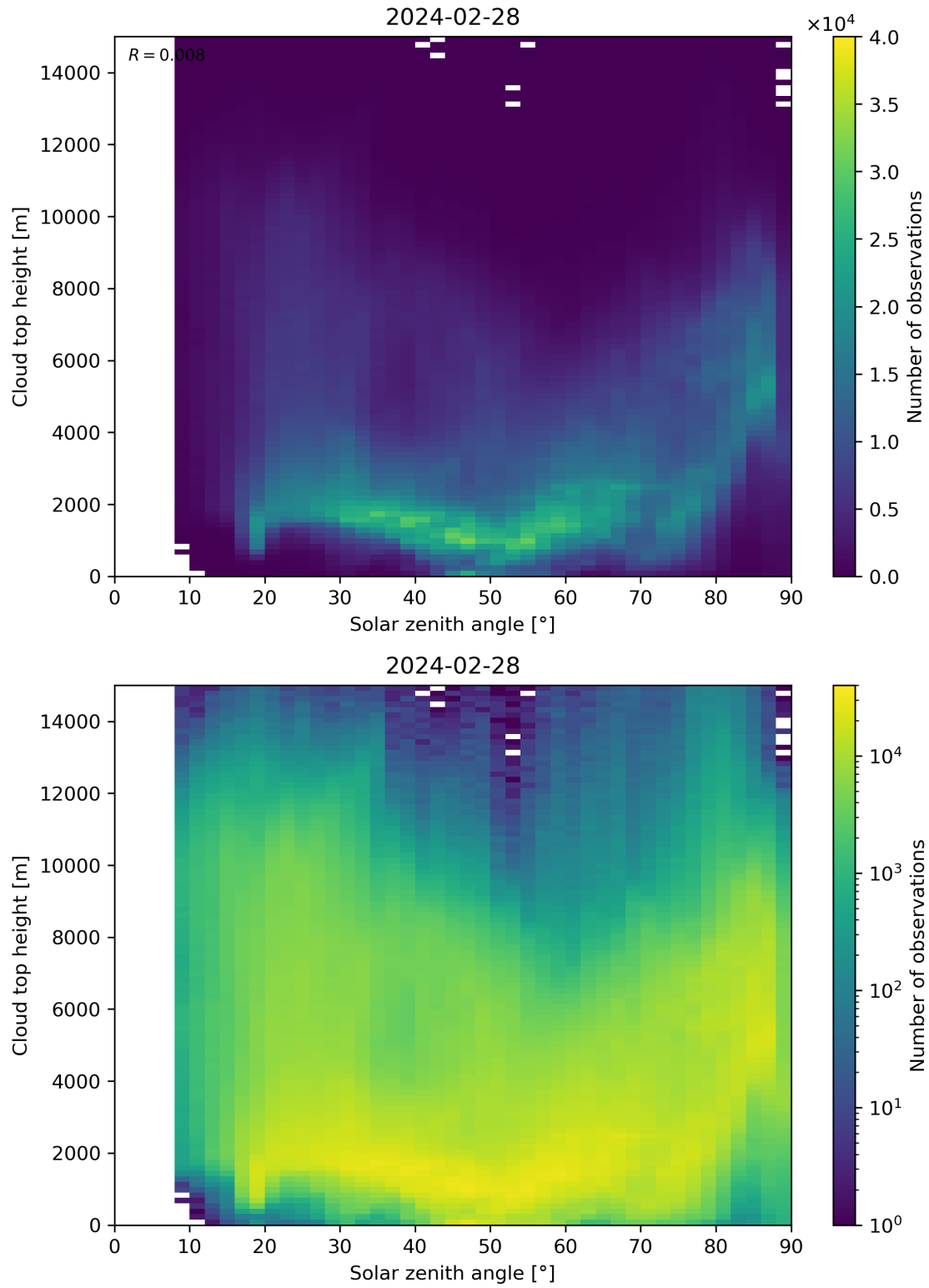
Figure 104: Scatter density plot of “Solar zenith angle” against “Cloud top height” for 2024-02-27 to 2024-02-29.
