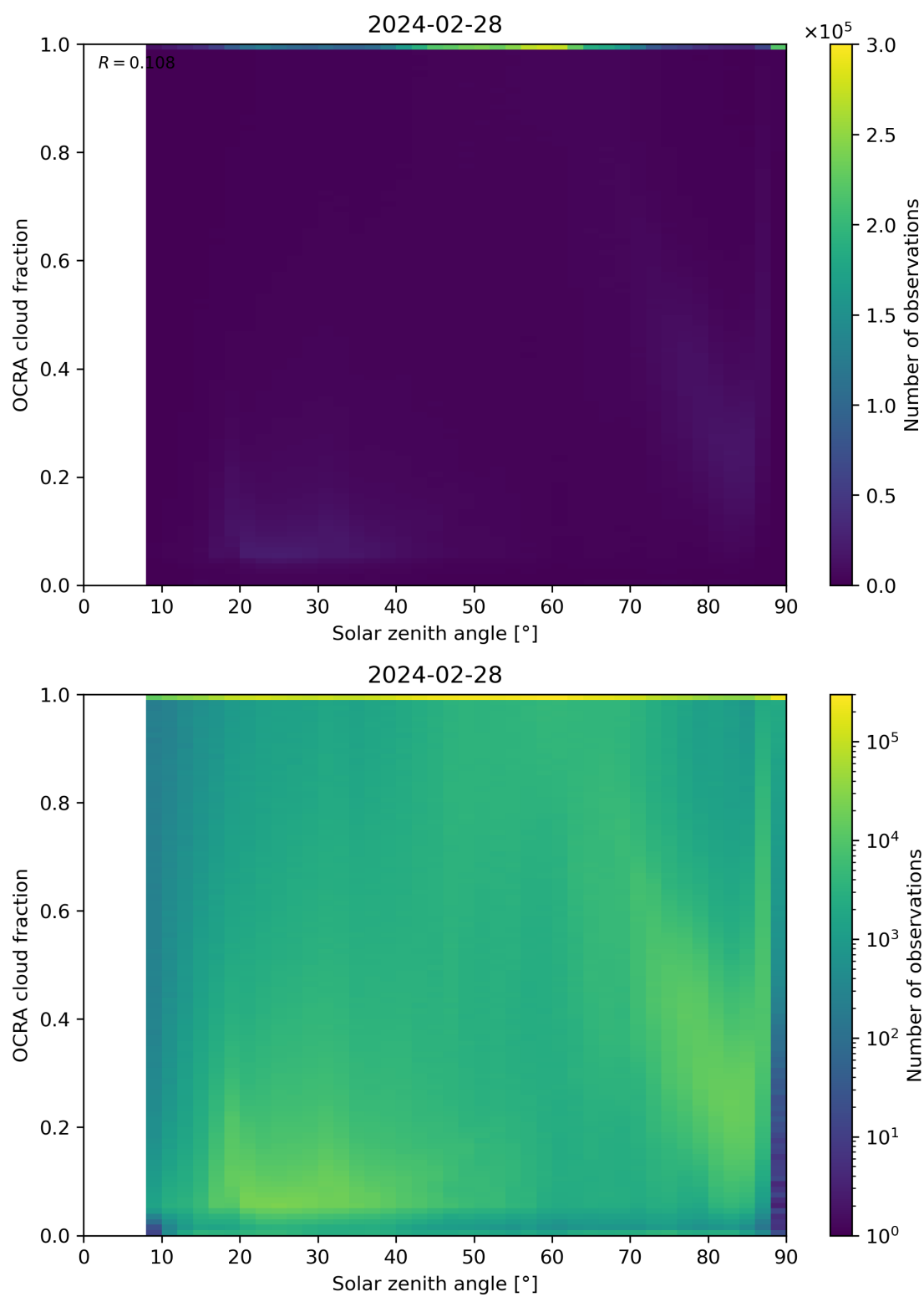
Figure 100: Scatter density plot of “Solar zenith angle” against “OCRA cloud fraction” for 2024-02-27 to 2024-02-29.
