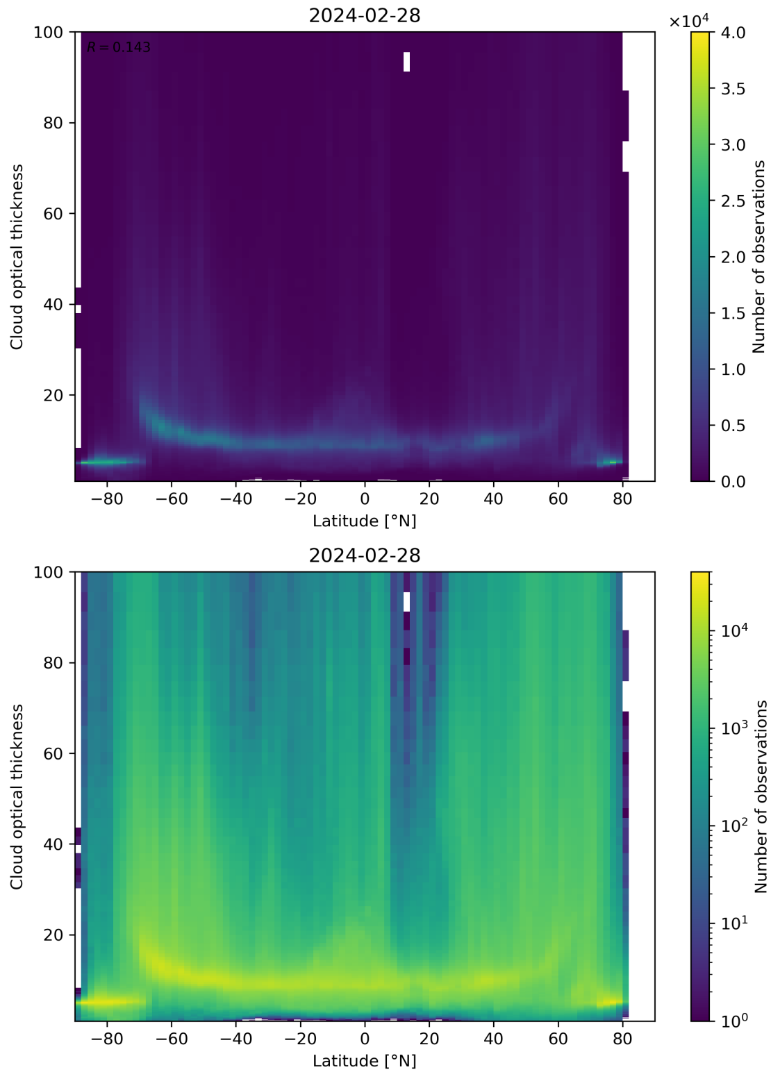
Figure 96: Scatter density plot of “Latitude” against “Cloud optical thickness” for 2024-02-27 to 2024-02-29.
