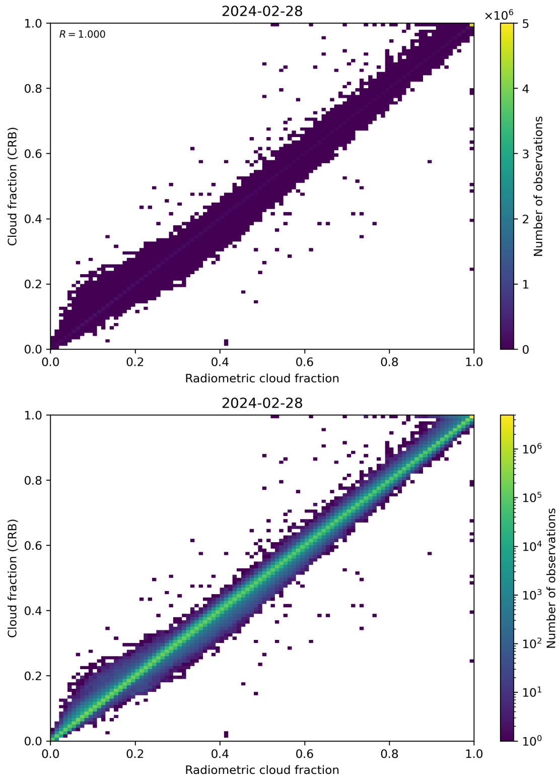
Figure 73: Scatter density plot of “Radiometric cloud fraction” against “Cloud fraction (CRB)” for 2024-02-27 to 2024-02-29.
