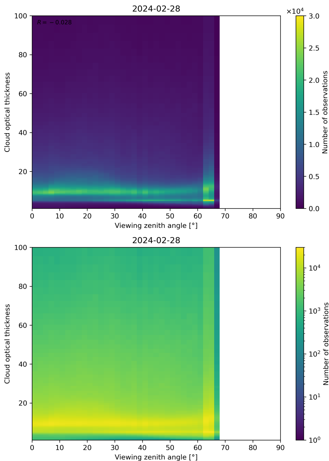
Figure 111: Scatter density plot of “Viewing zenith angle” against “Cloud optical thickness” for 2024-02-27 to 2024-02-29.
