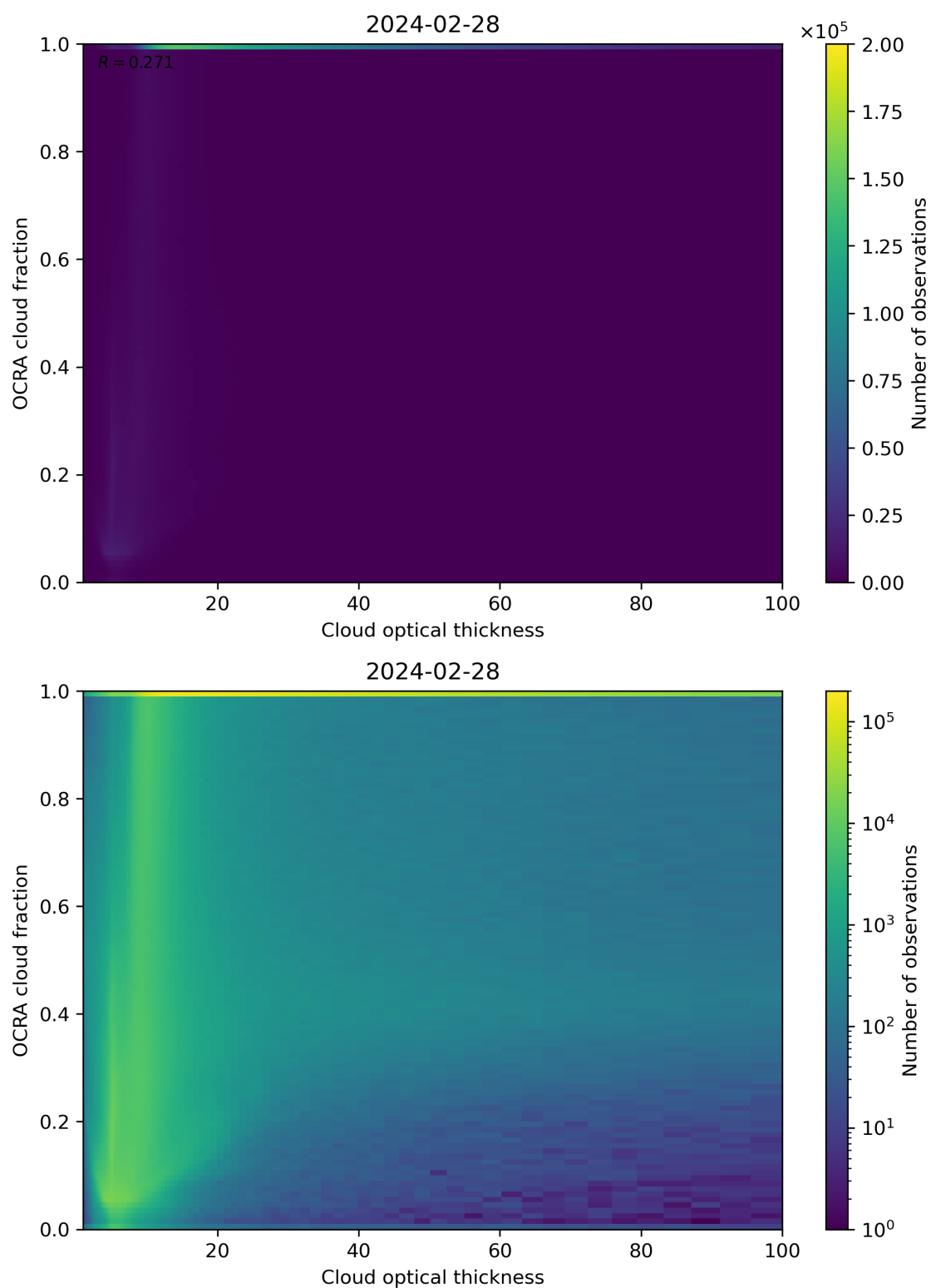
Figure 83: Scatter density plot of “Cloud optical thickness” against “OCRA cloud fraction” for 2024-02-27 to 2024-02-29.
