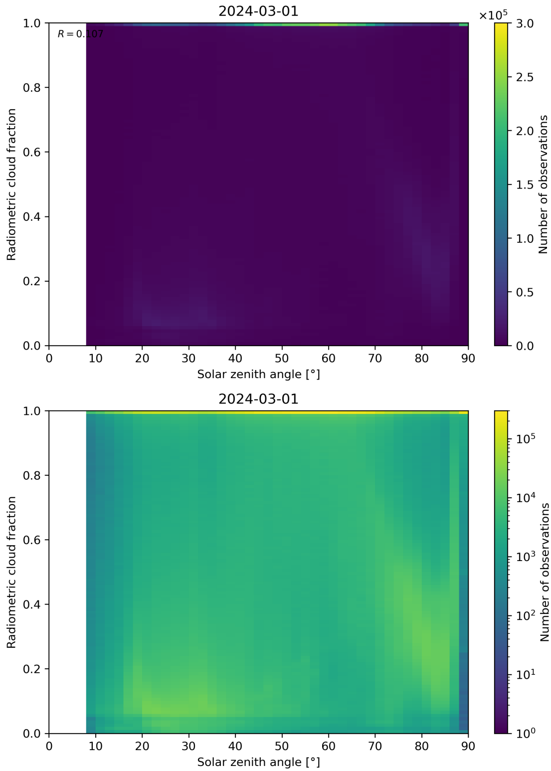
Figure 99: Scatter density plot of “Solar zenith angle” against “Radiometric cloud fraction” for 2024-02-29 to 2024-03-02.
