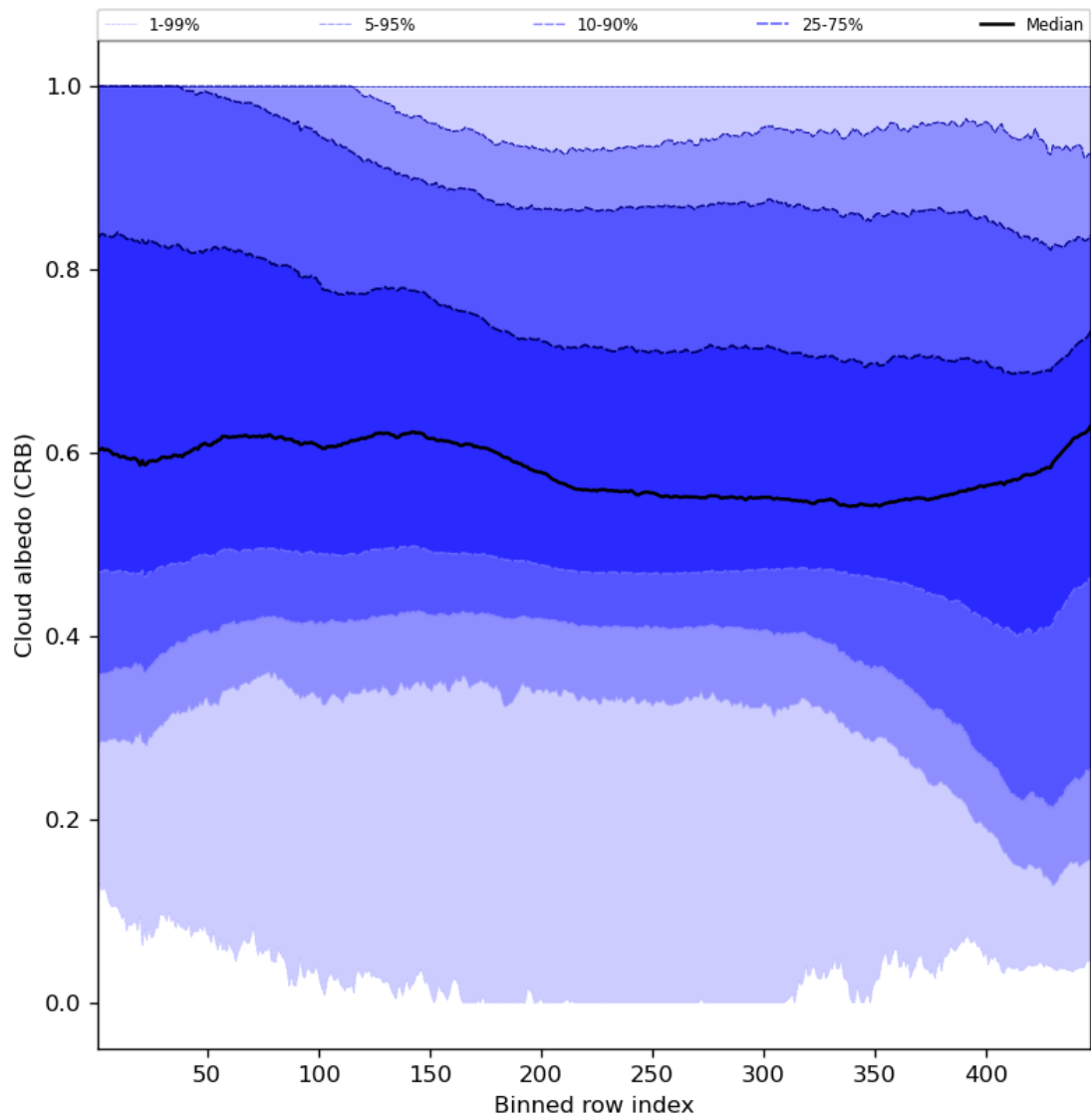
Figure 60: Along track statistics of “Cloud albedo (CRB)” for 2024-02-29 to 2024-03-02
