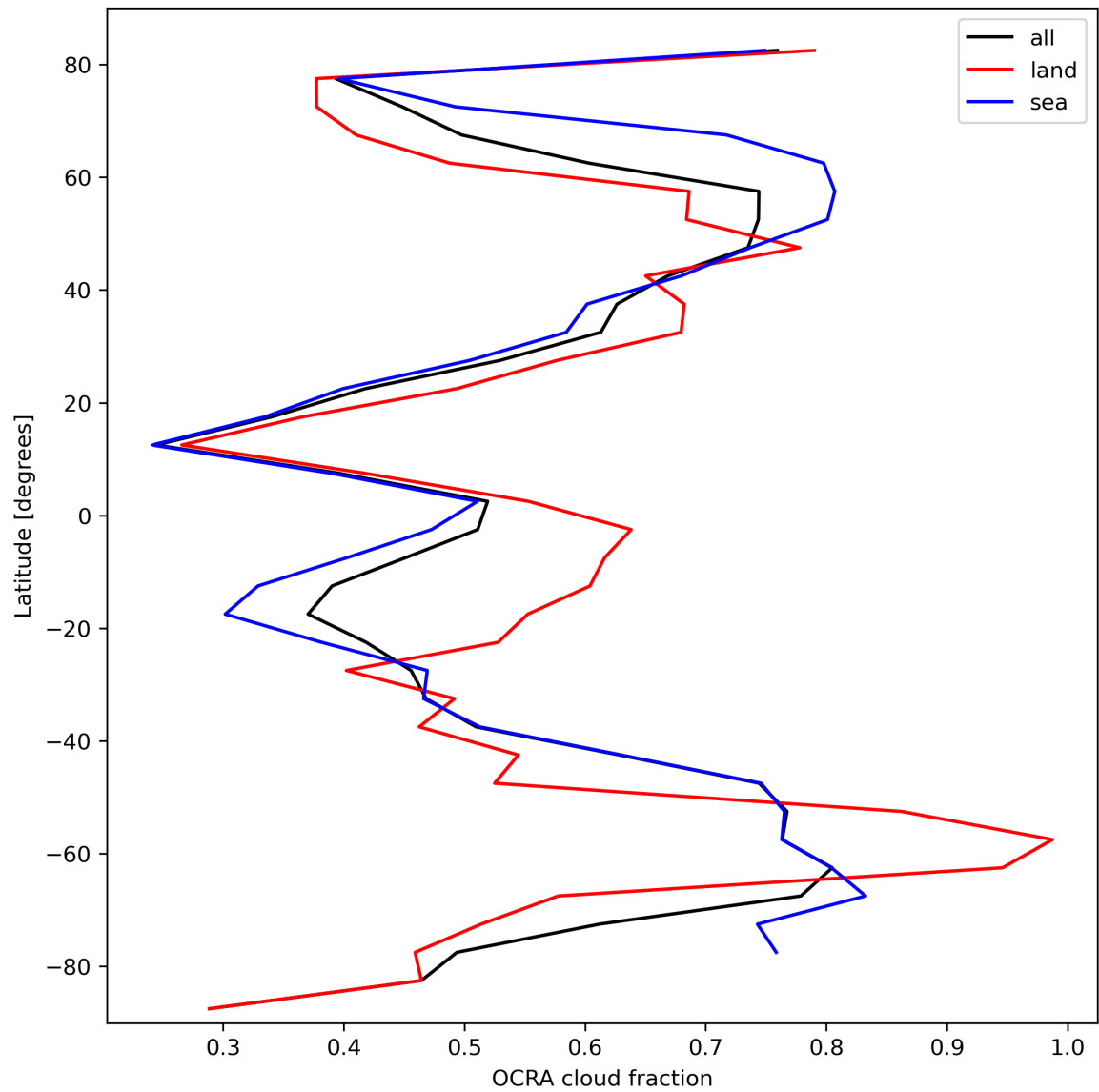
Figure 34: Zonal average of “OCRA cloud fraction” for 2024-02-29 to 2024-03-02.
