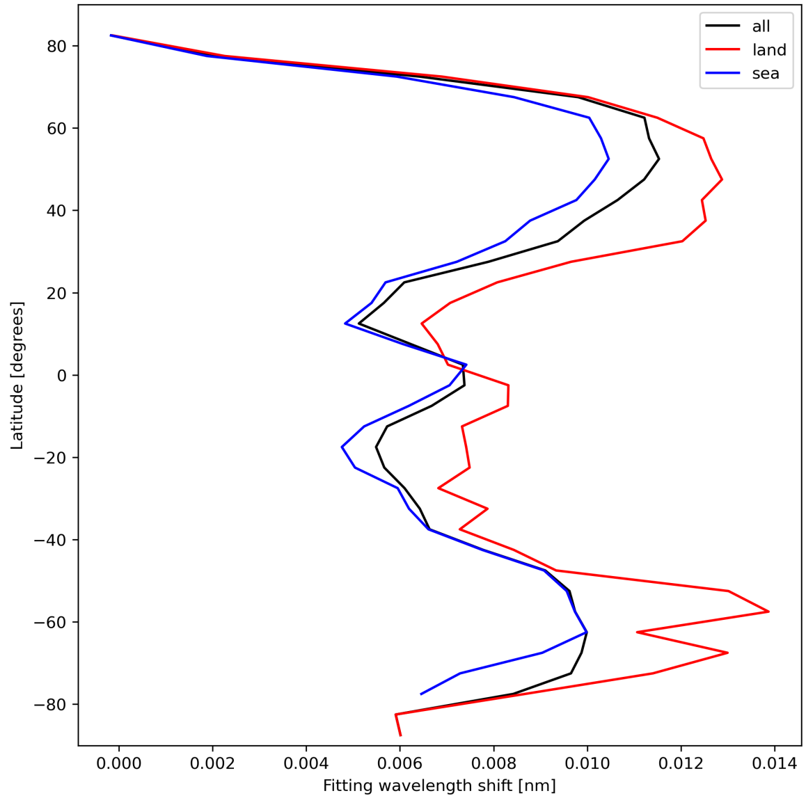
Figure 33: Zonal average of “Fitting wavelength shift” for 2024-02-29 to 2024-03-02.
