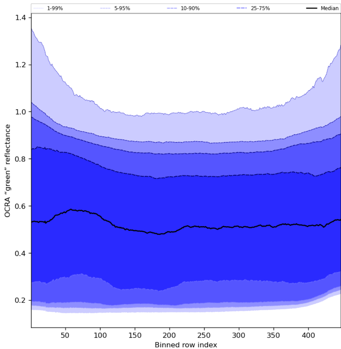
Figure 68: Along track statistics of "OCRA "green" reflectance" for 2024-02-29 to 2024-03-02
