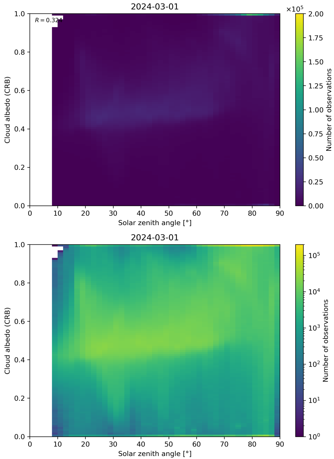
Figure 98: Scatter density plot of “Solar zenith angle” against “Cloud albedo (CRB)” for 2024-02-29 to 2024-03-02.
