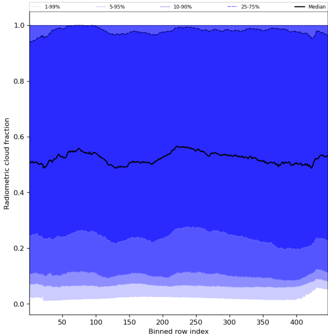
Figure 55: Along track statistics of “Radiometric cloud fraction” for 2024-02-29 to 2024-03-02
