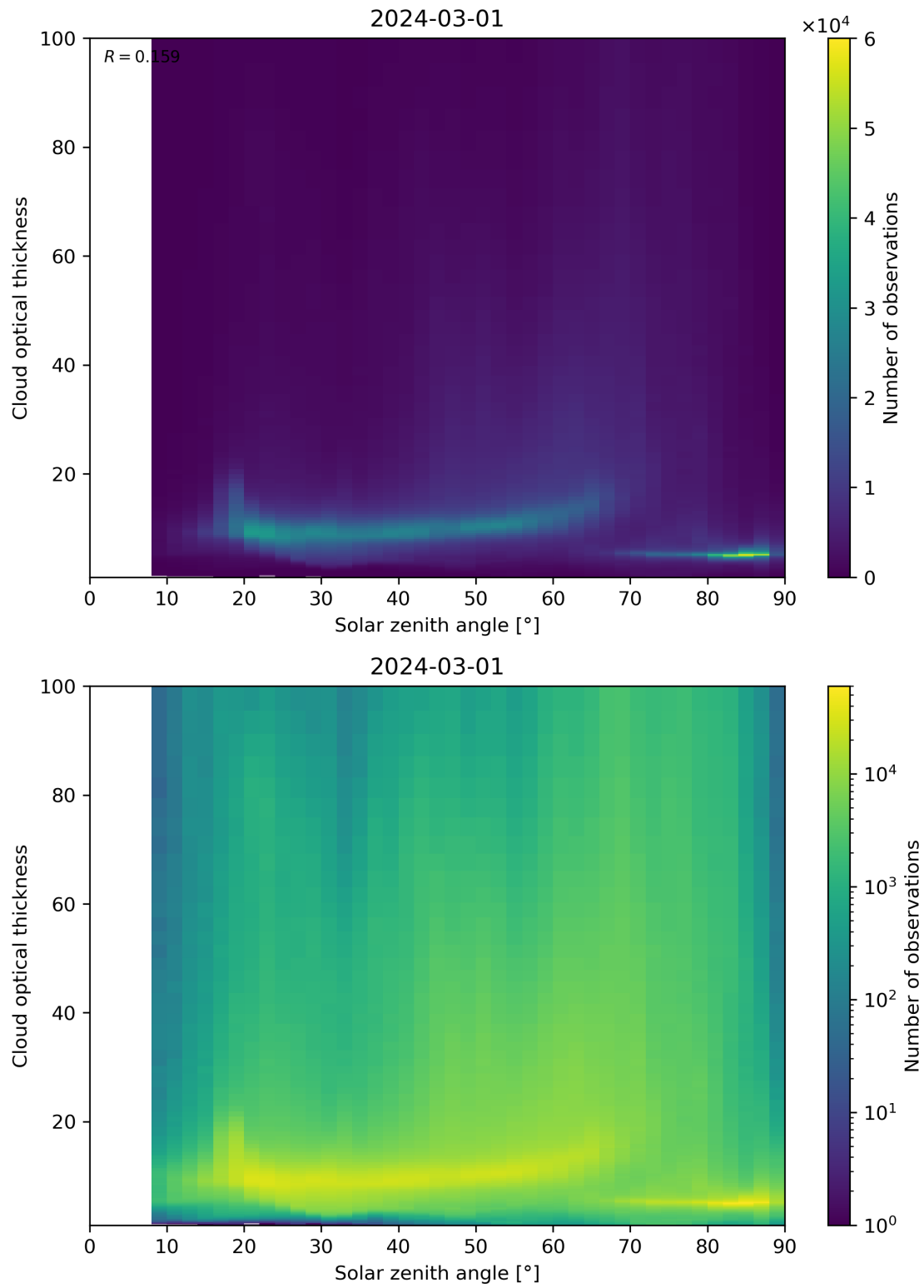
Figure 103: Scatter density plot of “Solar zenith angle” against “Cloud optical thickness” for 2024-02-29 to 2024-03-02.
