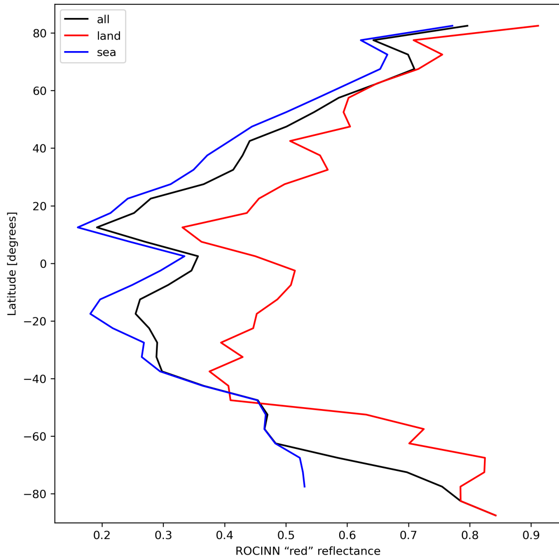
Figure 37: Zonal average of “ROCINN “red” reflectance” for 2024-02-29 to 2024-03-02.
