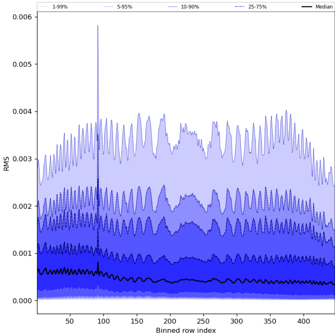
Figure 63: Along track statistics of “RMS” for 2024-02-29 to 2024-03-02
