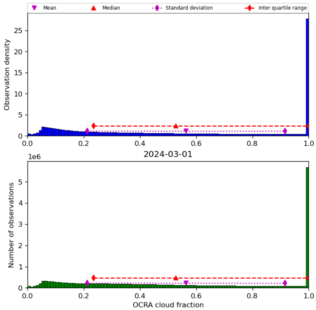
Figure 50: Histogram of “OCRA cloud fraction” for 2024-02-29 to 2024-03-02
