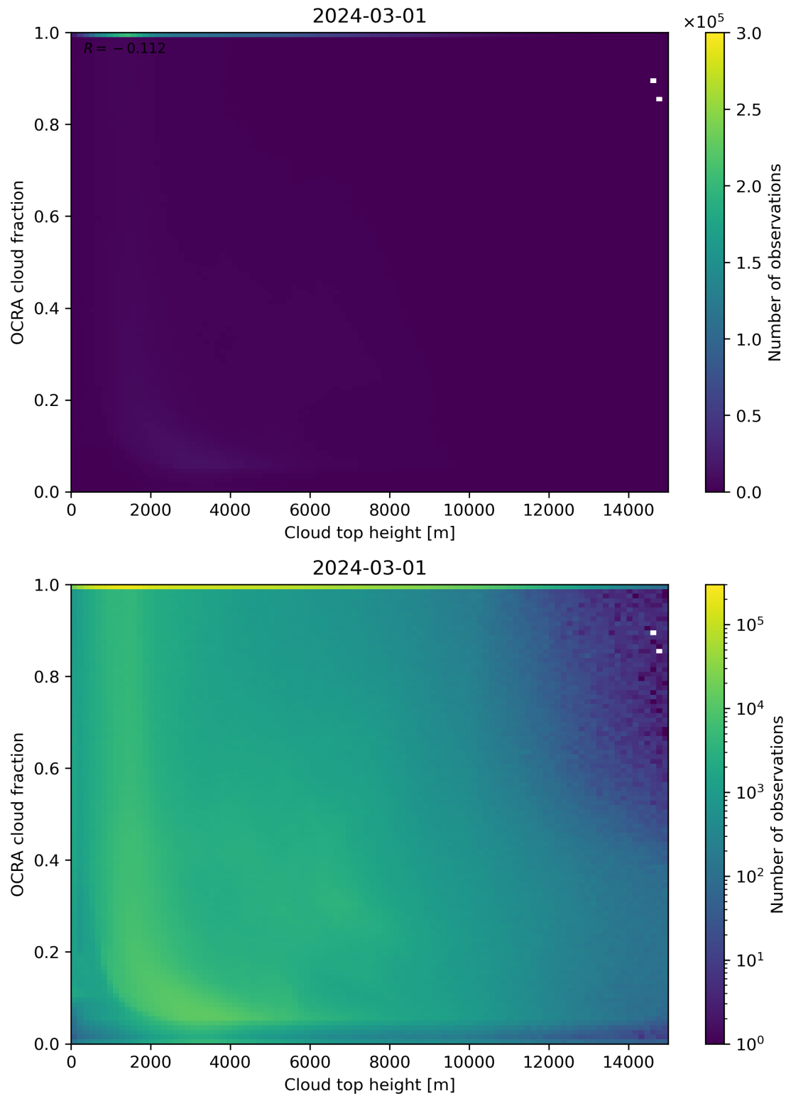
Figure 87: Scatter density plot of “Cloud top height” against “OCRA cloud fraction” for 2024-02-29 to 2024-03-02.
