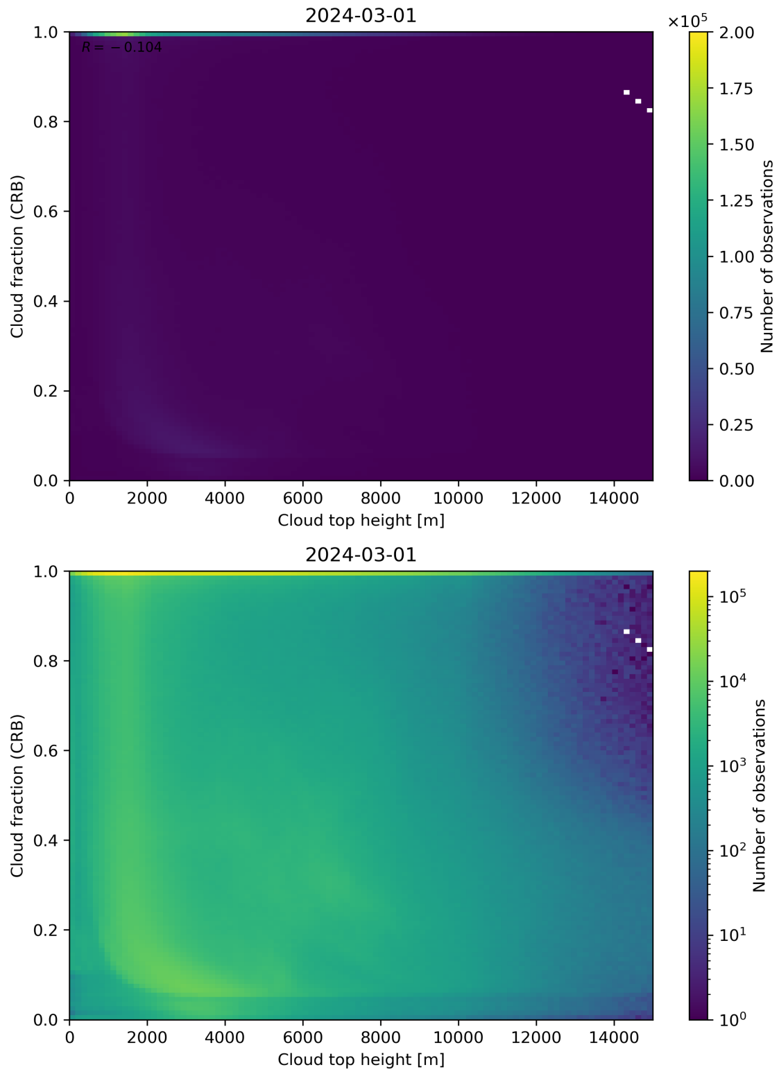
Figure 88: Scatter density plot of “Cloud top height” against “Cloud fraction (CRB)” for 2024-02-29 to 2024-03-02.
