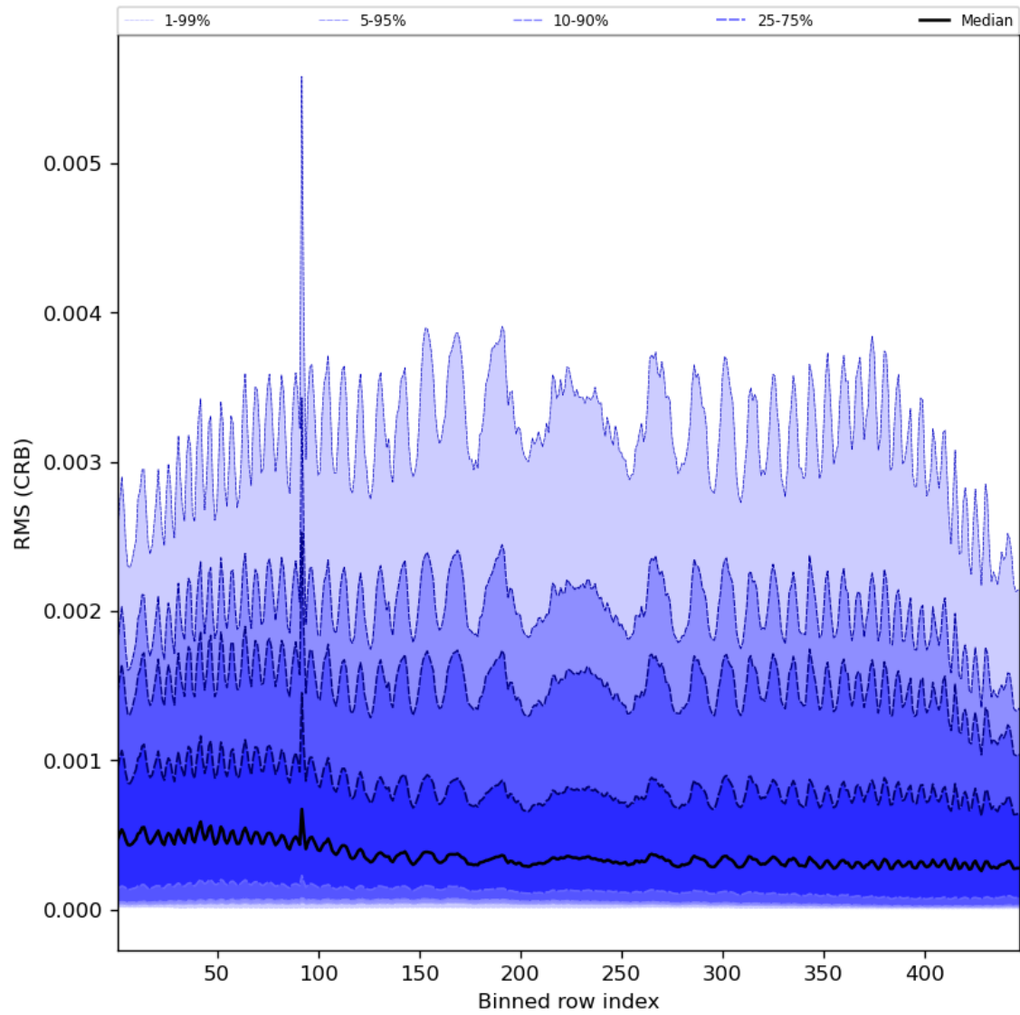
Figure 64: Along track statistics of “RMS (CRB)” for 2024-02-29 to 2024-03-02
