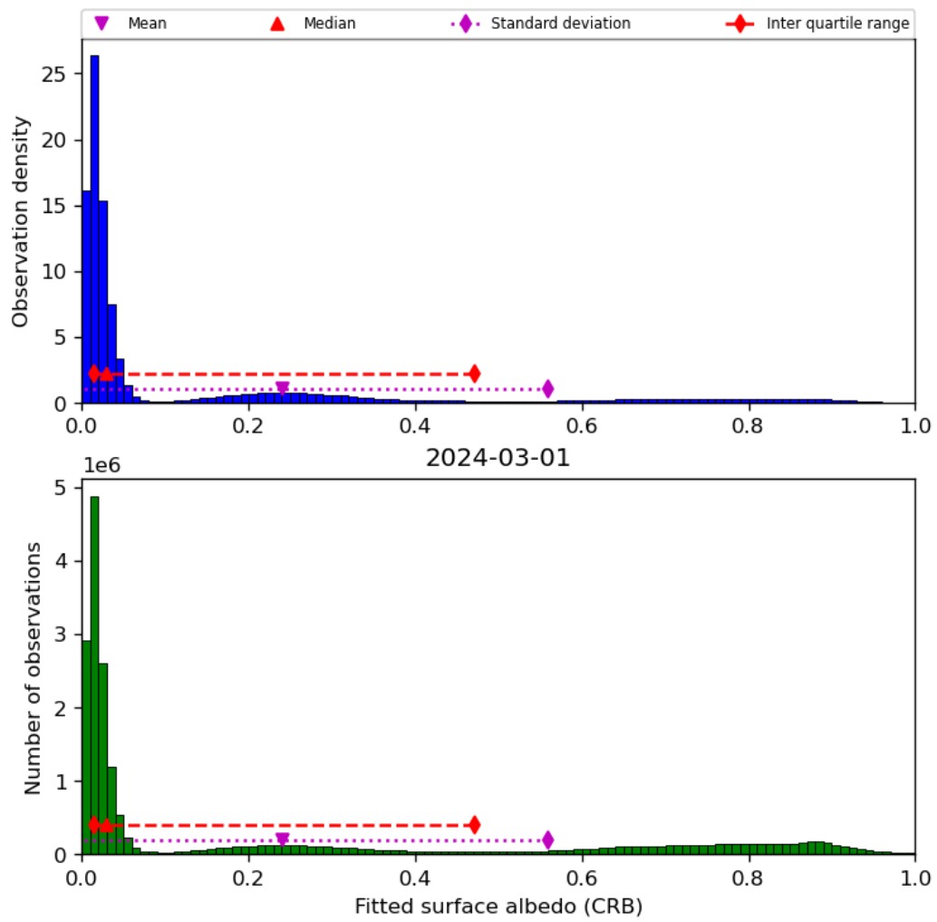
Figure 46: Histogram of “Fitted surface albedo (CRB)” for 2024-02-29 to 2024-03-02
