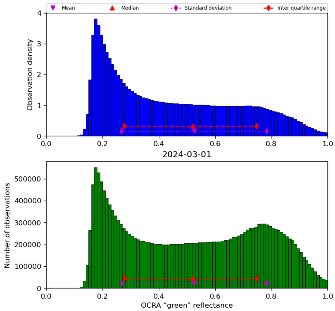
Figure 52: Histogram of “OCRA “green” reflectance” for 2024-02-29 to 2024-03-02
