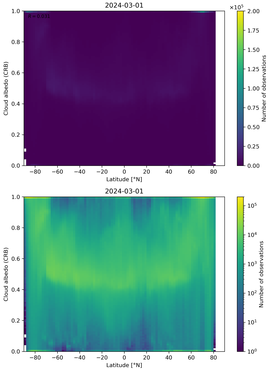
Figure 91: Scatter density plot of “Latitude” against “Cloud albedo (CRB)” for 2024-02-29 to 2024-03-02.
