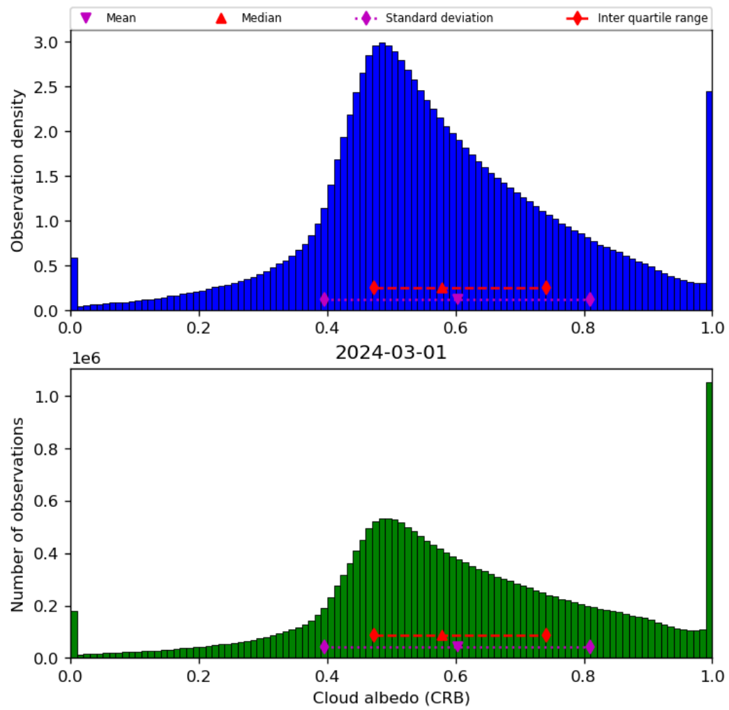
Figure 44: Histogram of “Cloud albedo (CRB)” for 2024-02-29 to 2024-03-02
