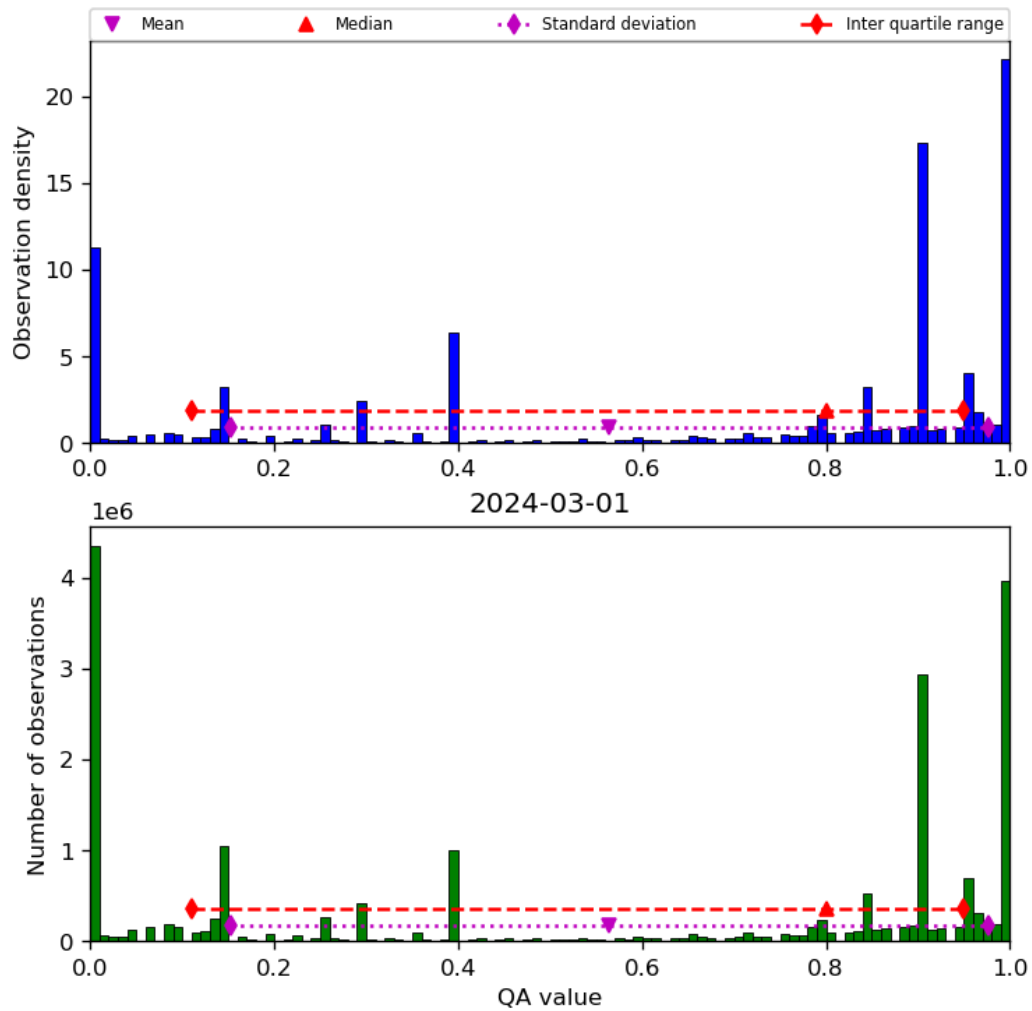
Figure 38: Histogram of “QA value” for 2024-02-29 to 2024-03-02
