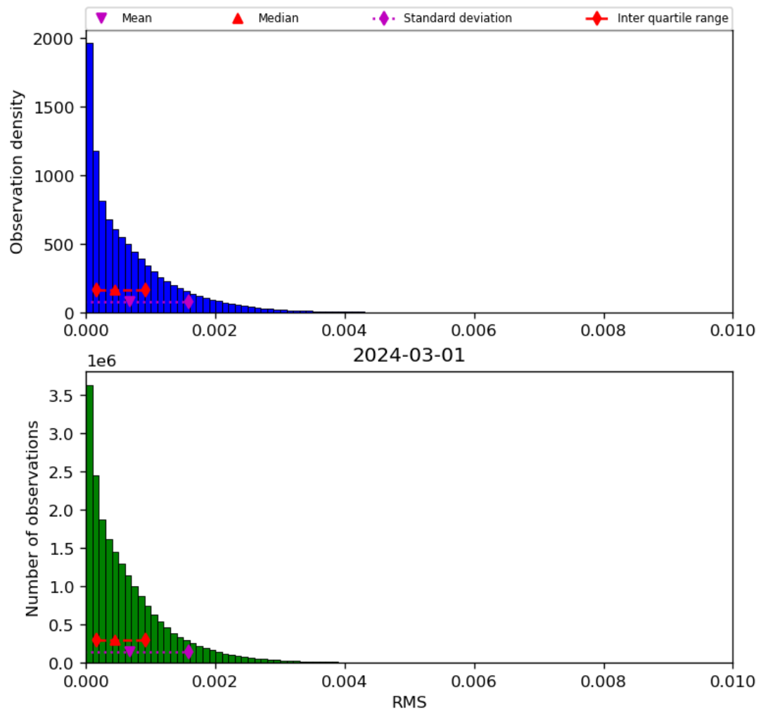
Figure 47: Histogram of “RMS” for 2024-02-29 to 2024-03-02
