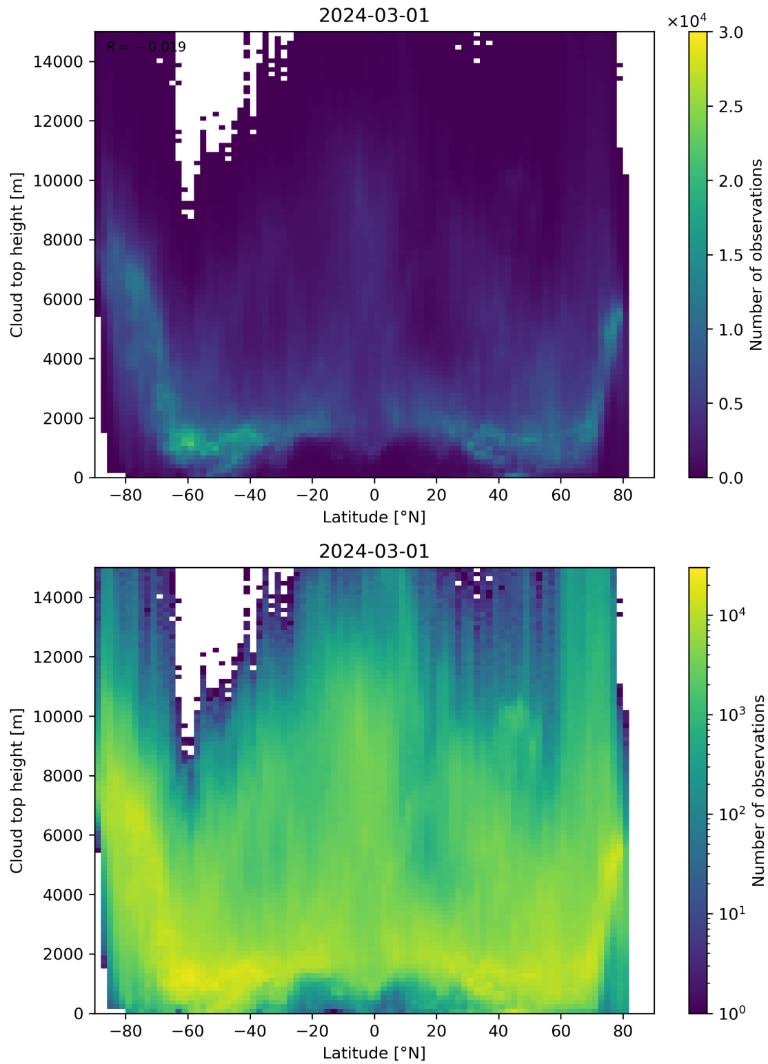
Figure 97: Scatter density plot of “Latitude” against “Cloud top height” for 2024-02-29 to 2024-03-02.
