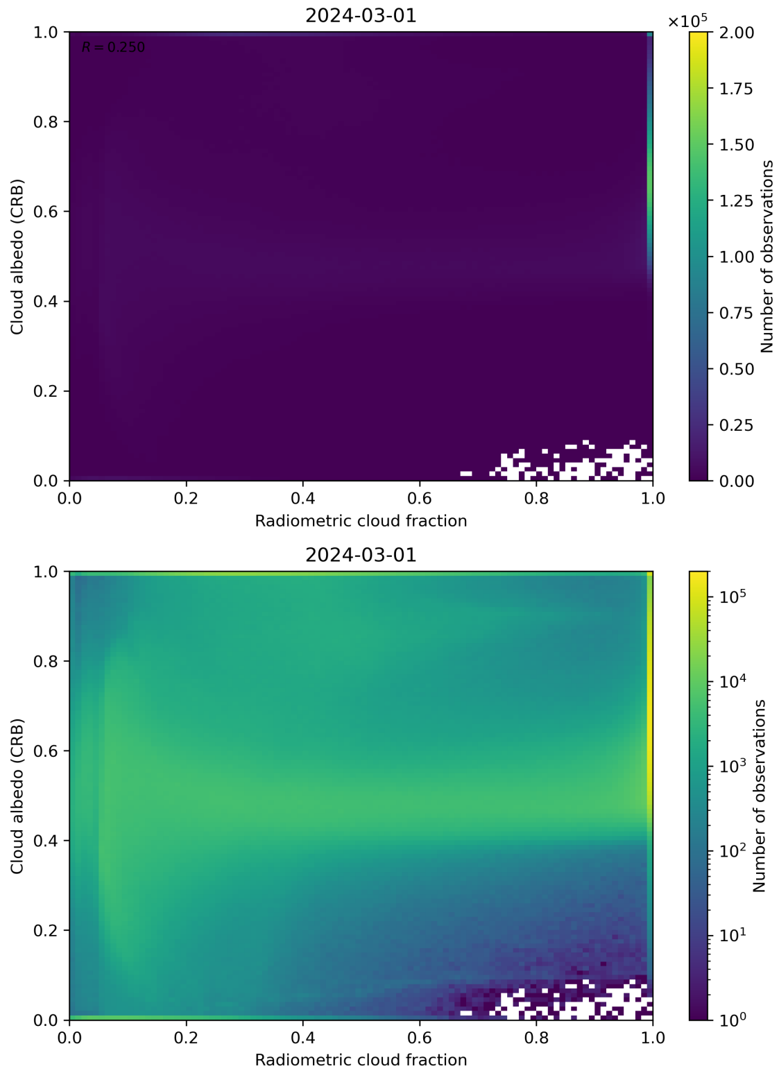
Figure 71: Scatter density plot of “Radiometric cloud fraction” against “Cloud albedo (CRB)” for 2024-02-29 to 2024-03-02.
