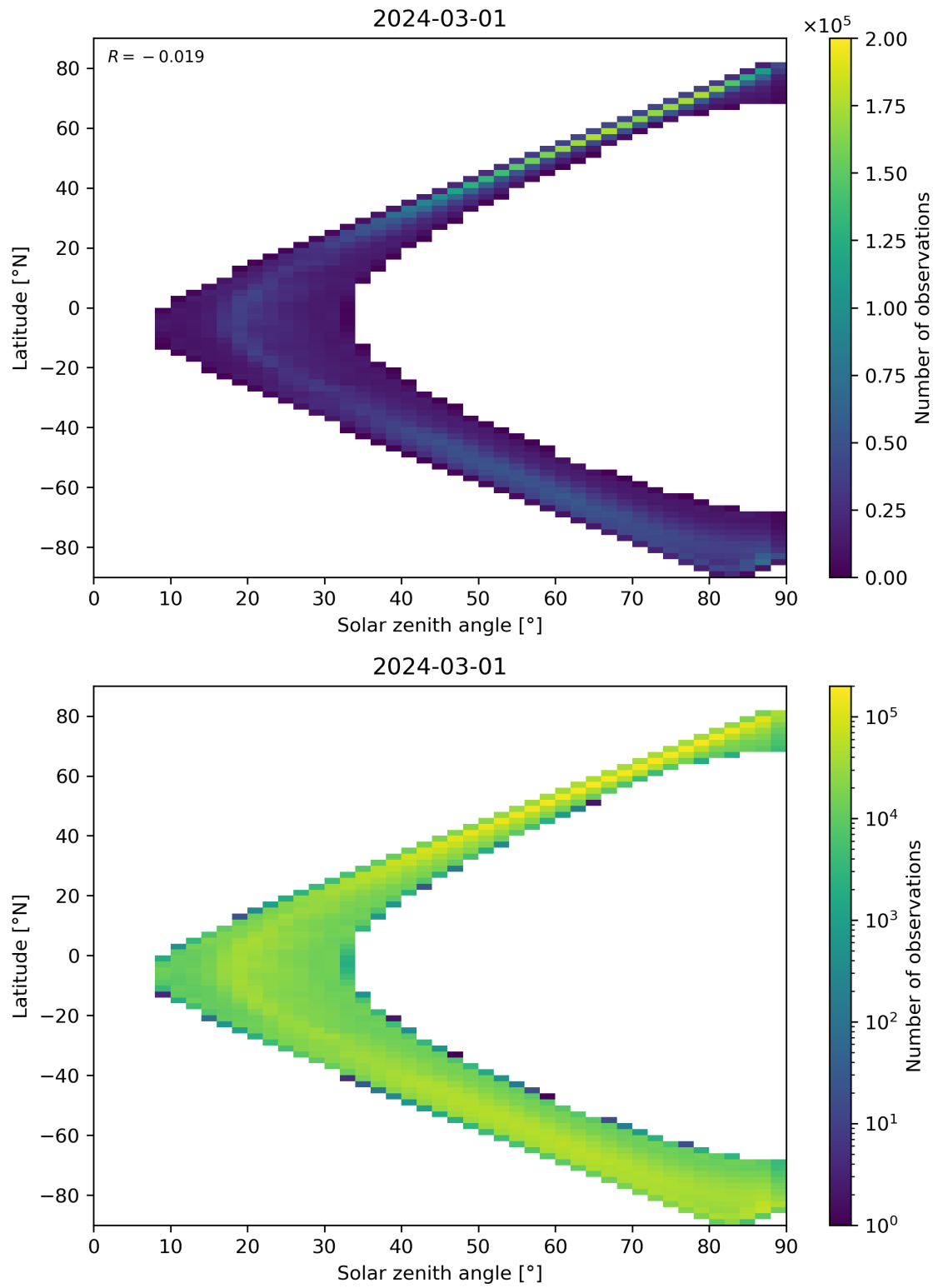
Figure 105: Scatter density plot of “Solar zenith angle” against “Latitude” for 2024-02-29 to 2024-03-02.
