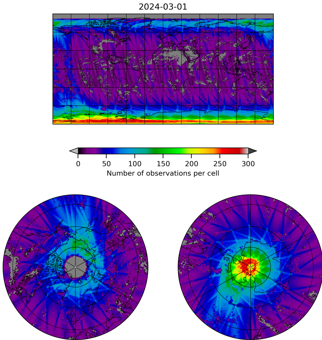
Figure 21: Map of the number of observations for 2024-02-29 to 2024-03-02
