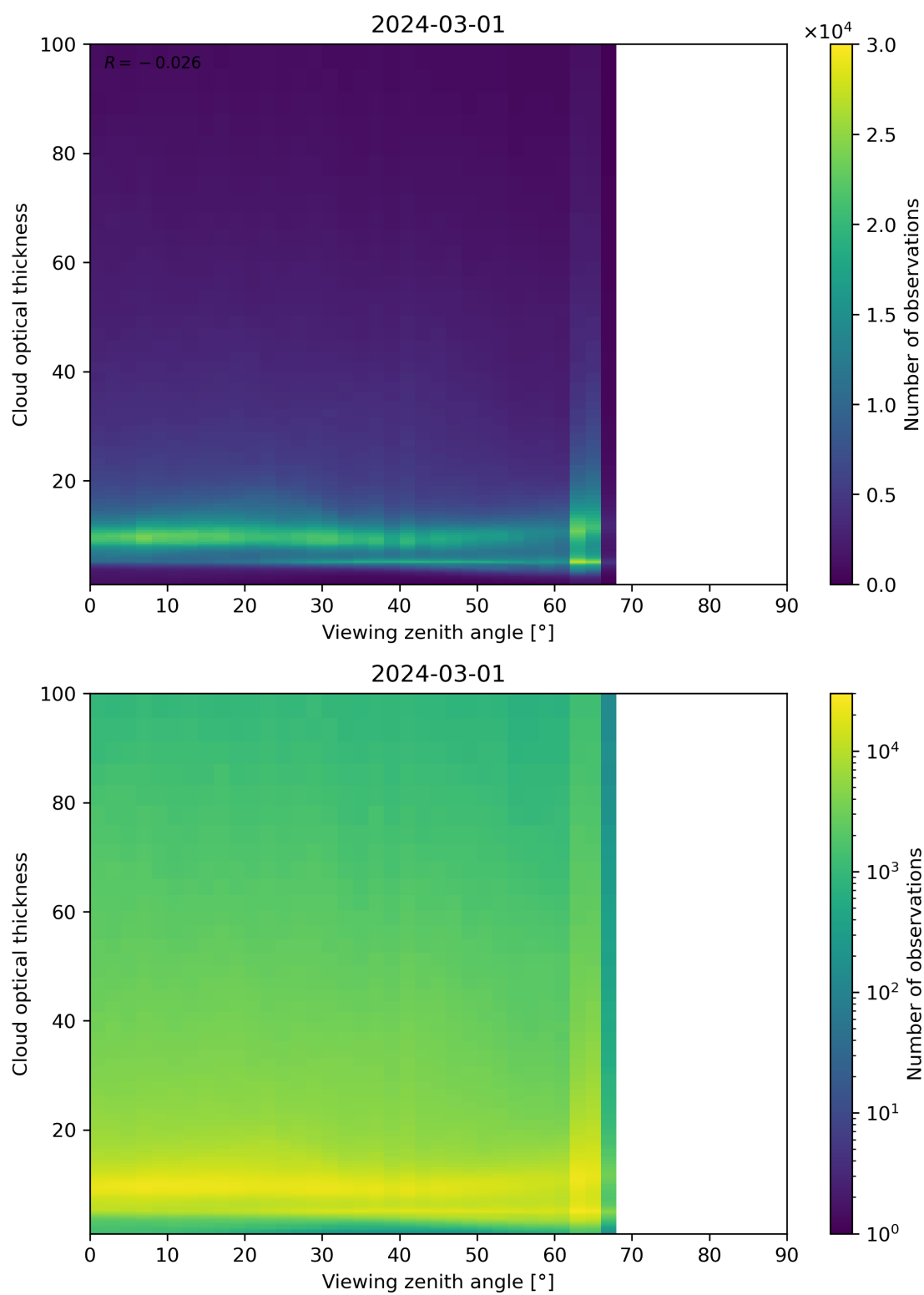
Figure 111: Scatter density plot of “Viewing zenith angle” against “Cloud optical thickness” for 2024-02-29 to 2024-03-02.
