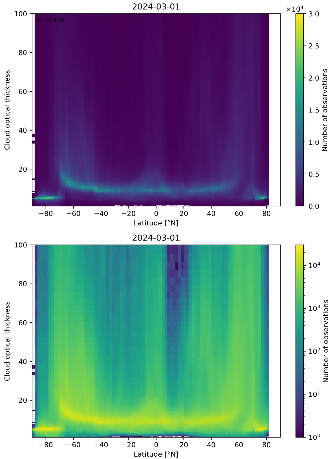
Figure 96: Scatter density plot of “Latitude” against “Cloud optical thickness” for 2024-02-29 to 2024-03-02.
