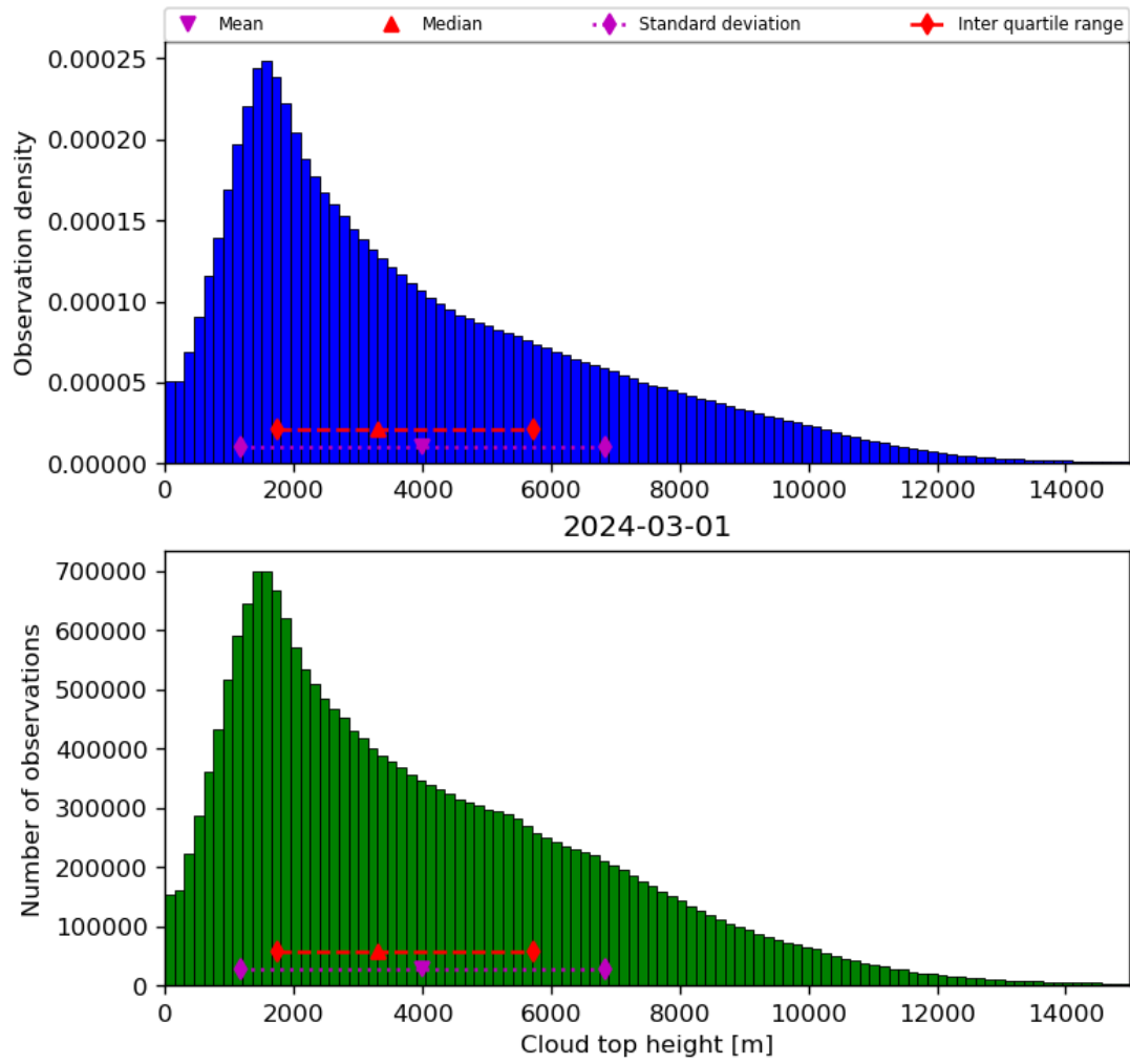
Figure 40: Histogram of “Cloud top height” for 2024-02-29 to 2024-03-02
