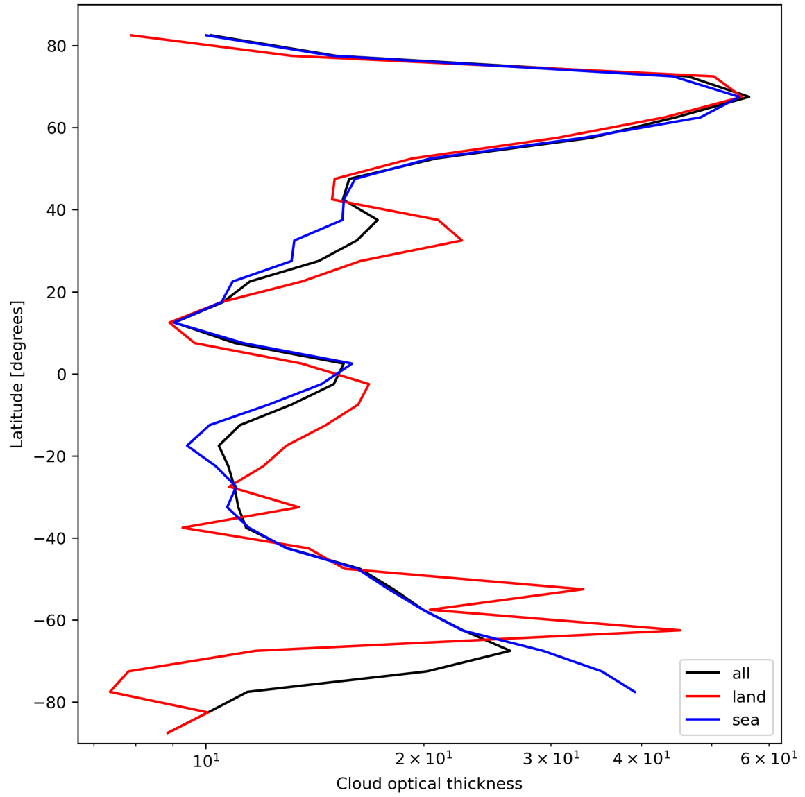
Figure 25: Zonal average of “Cloud optical thickness” for 2024-02-29 to 2024-03-02.
