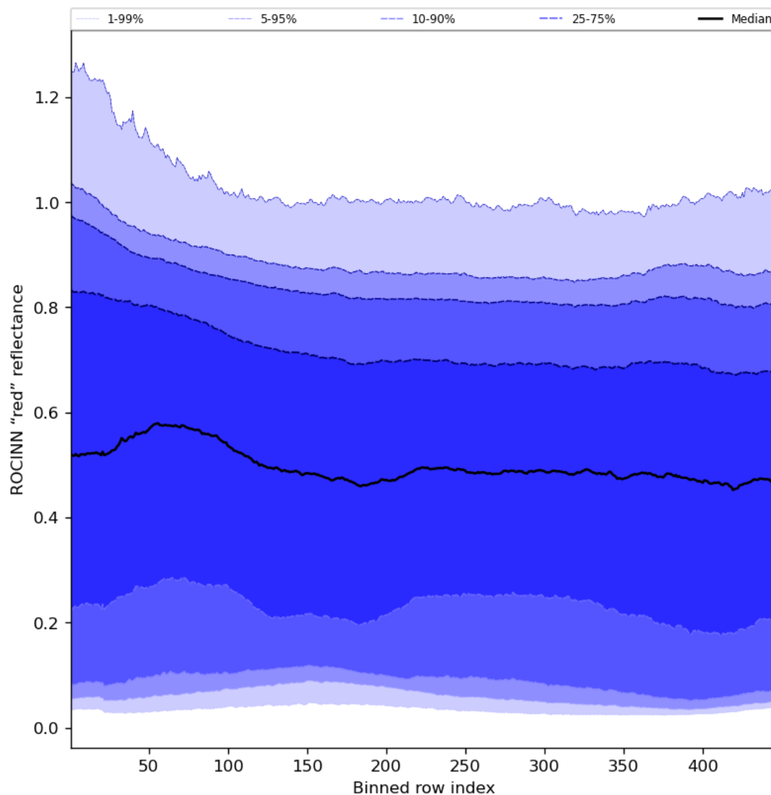
Figure 69: Along track statistics of “ROCINN “red” reflectance” for 2024-02-29 to 2024-03-02
