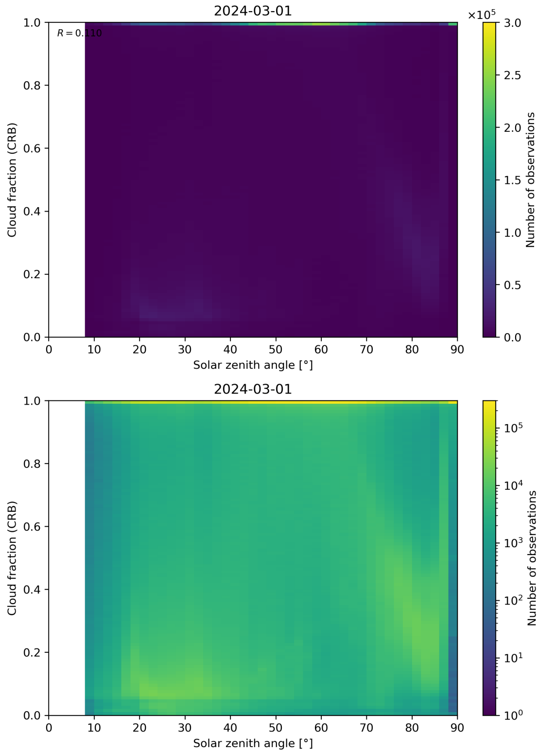
Figure 101: Scatter density plot of “Solar zenith angle” against “Cloud fraction (CRB)” for 2024-02-29 to 2024-03-02.
