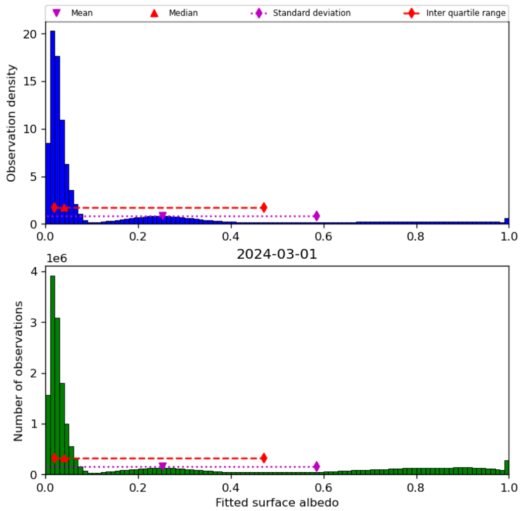
Figure 45: Histogram of “Fitted surface albedo” for 2024-02-29 to 2024-03-02
