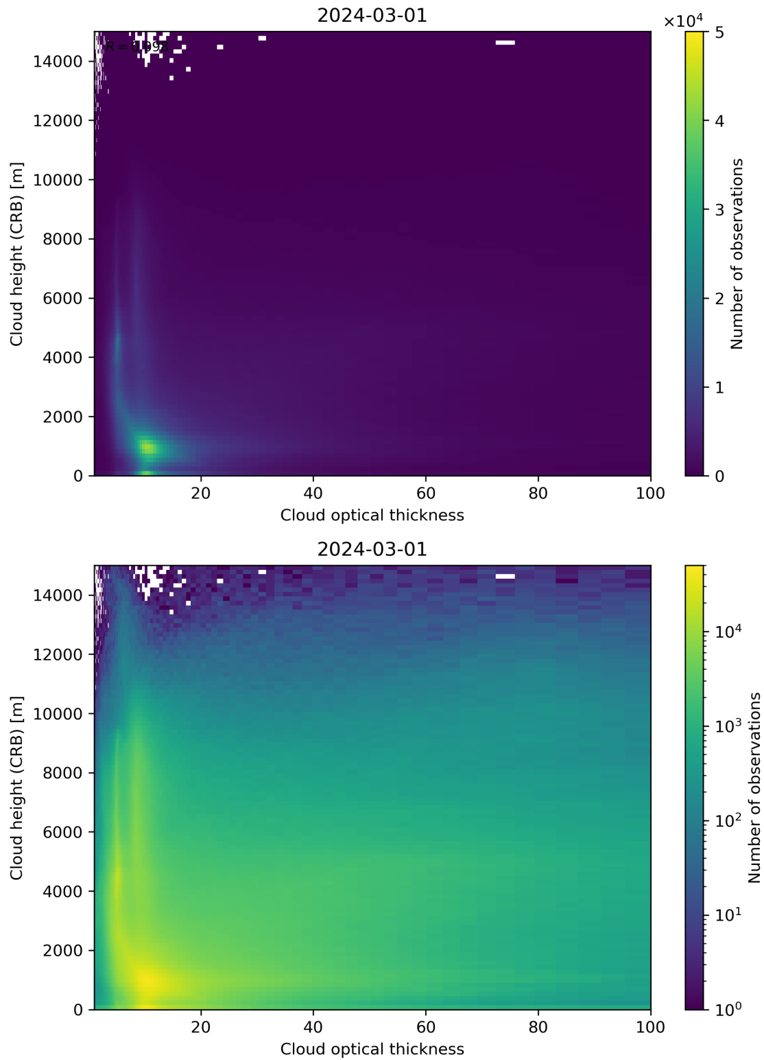
Figure 85: Scatter density plot of “Cloud optical thickness” against “Cloud height (CRB)” for 2024-02-29 to 2024-03-02.
