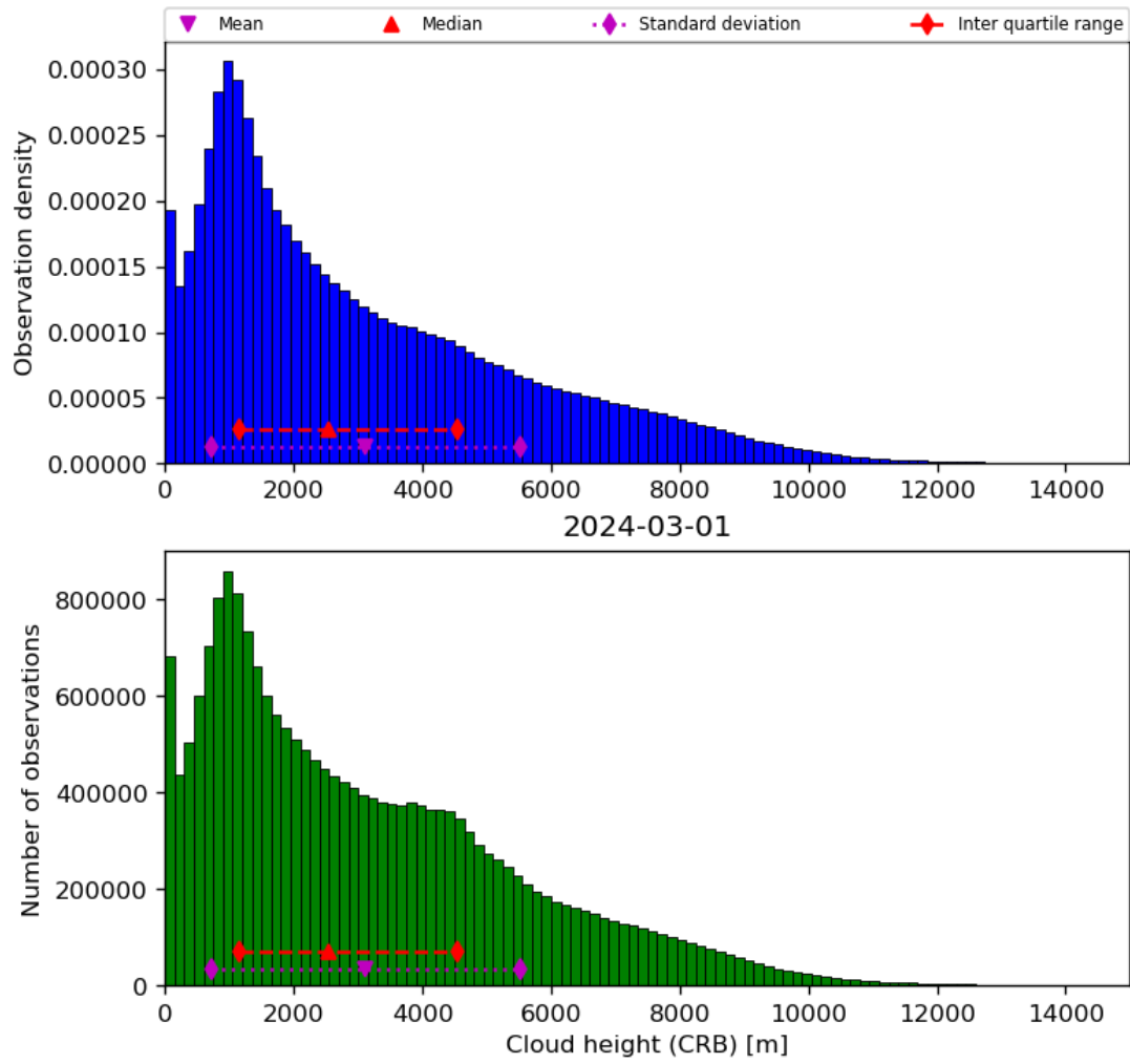
Figure 43: Histogram of “Cloud height (CRB)” for 2024-02-29 to 2024-03-02
