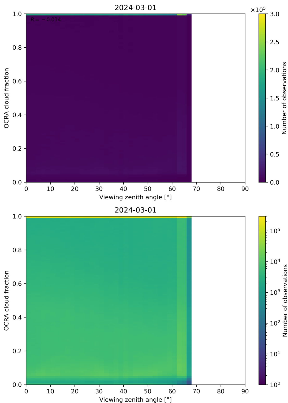
Figure 108: Scatter density plot of “Viewing zenith angle” against “OCRA cloud fraction” for 2024-02-29 to 2024-03-02.
