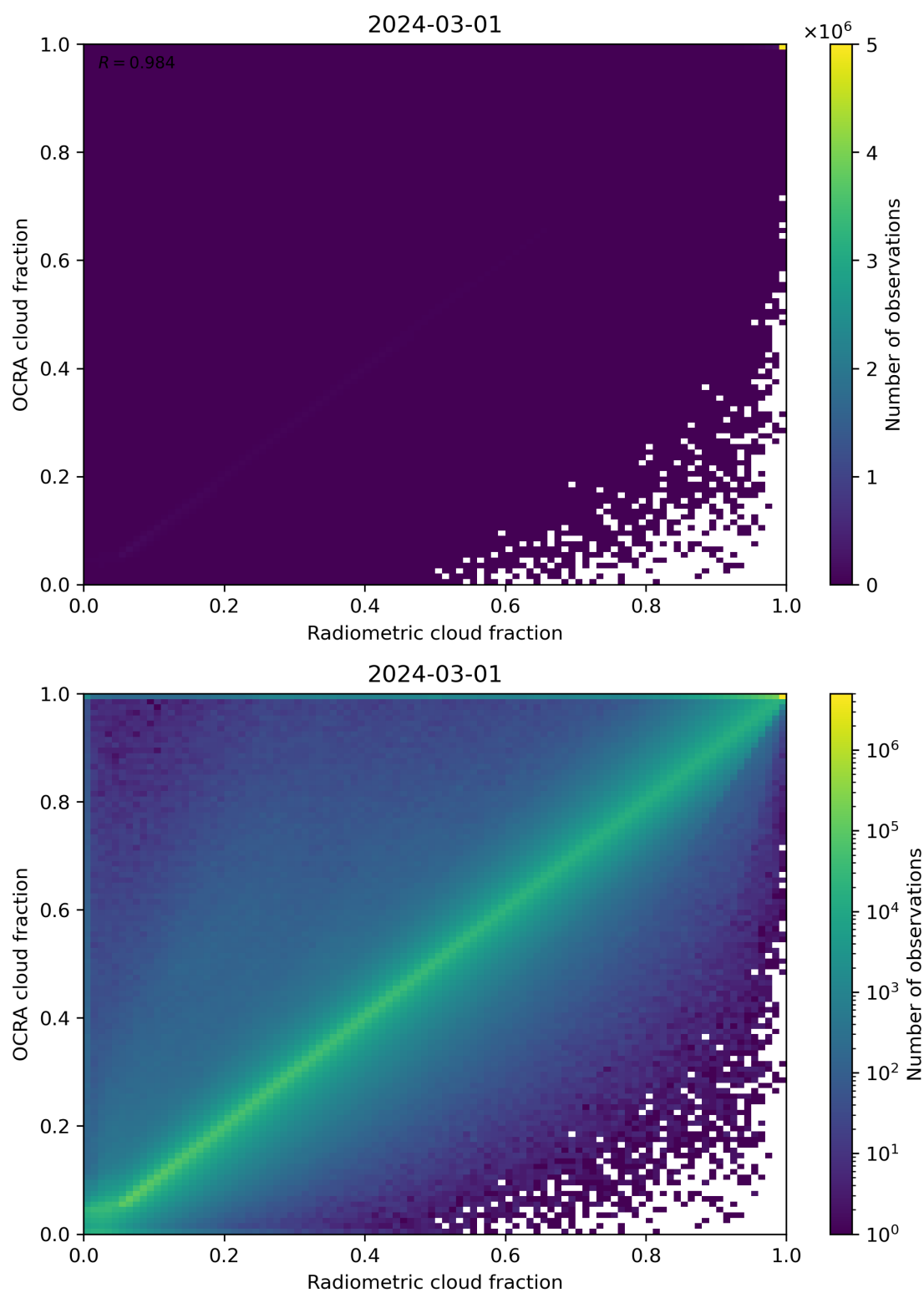
Figure 72: Scatter density plot of “Radiometric cloud fraction” against “OCRA cloud fraction” for 2024-02-29 to 2024-03-02.
