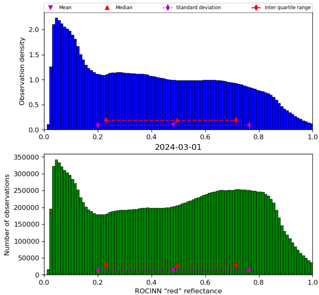
Figure 53: Histogram of “ROCINN “red” reflectance” for 2024-02-29 to 2024-03-02
