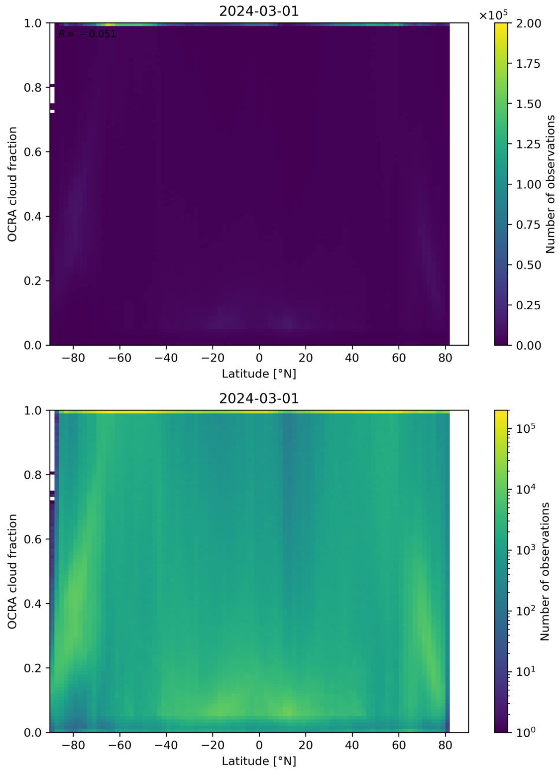
Figure 93: Scatter density plot of “Latitude” against “OCRA cloud fraction” for 2024-02-29 to 2024-03-02.
