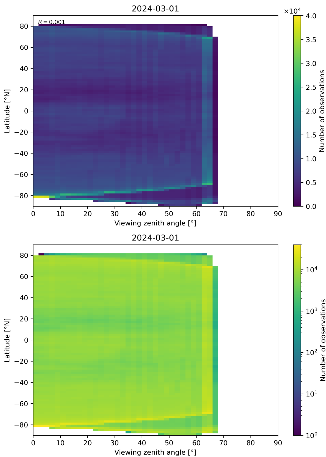
Figure 113: Scatter density plot of “Viewing zenith angle” against “Latitude” for 2024-02-29 to 2024-03-02.
