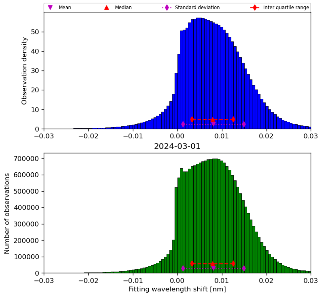
Figure 49: Histogram of “Fitting wavelength shift” for 2024-02-29 to 2024-03-02
