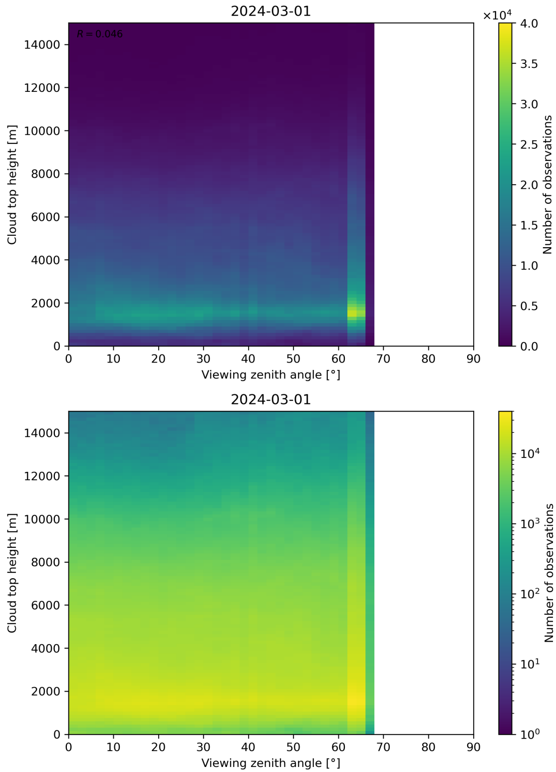
Figure 112: Scatter density plot of “Viewing zenith angle” against “Cloud top height” for 2024-02-29 to 2024-03-02.
