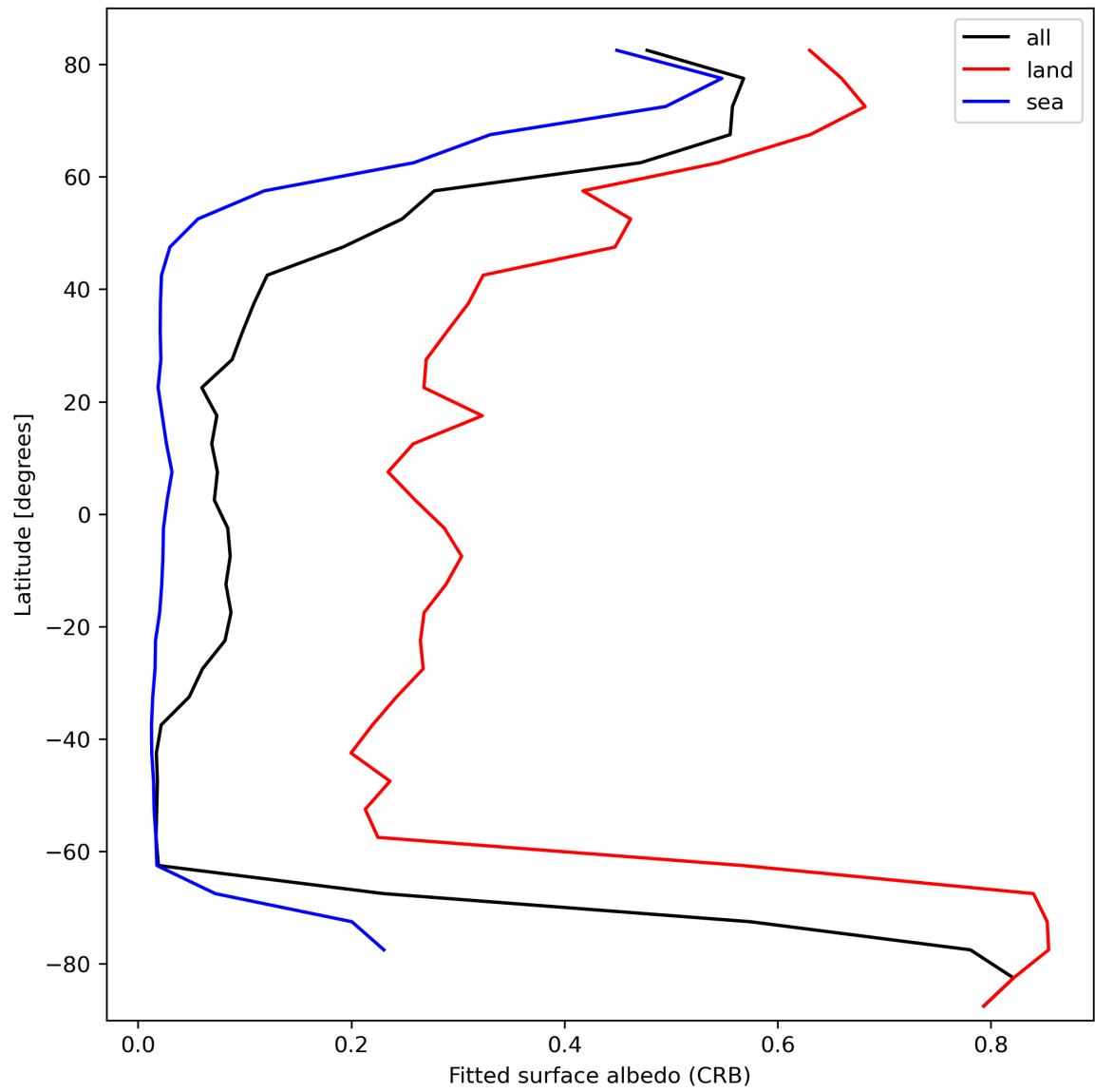
Figure 30: Zonal average of “Fitted surface albedo (CRB)” for 2024-02-29 to 2024-03-02.
