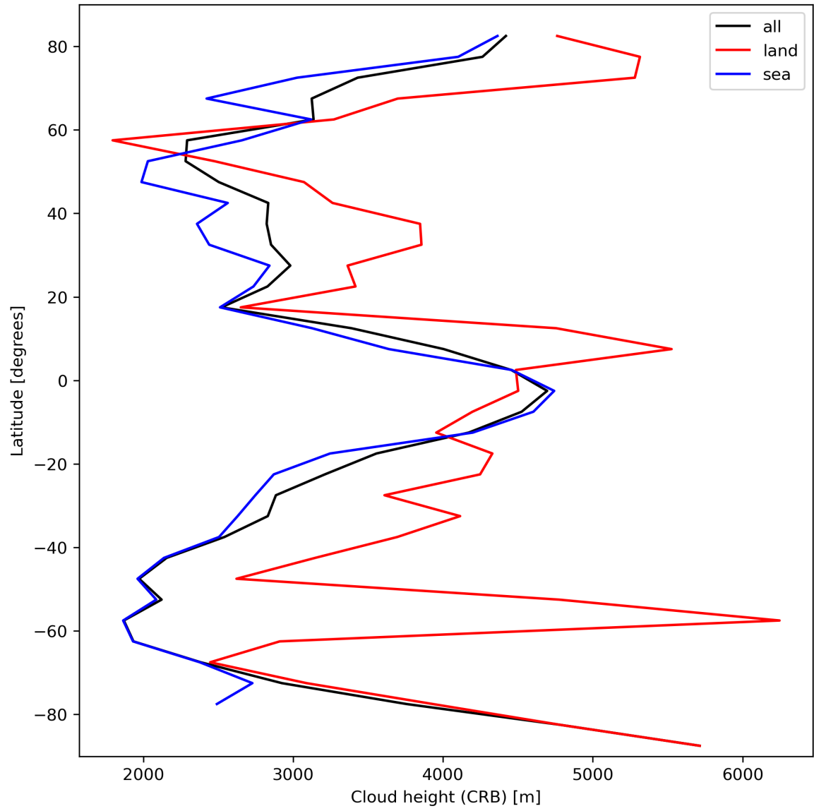
Figure 27: Zonal average of “Cloud height (CRB)” for 2024-02-29 to 2024-03-02.
