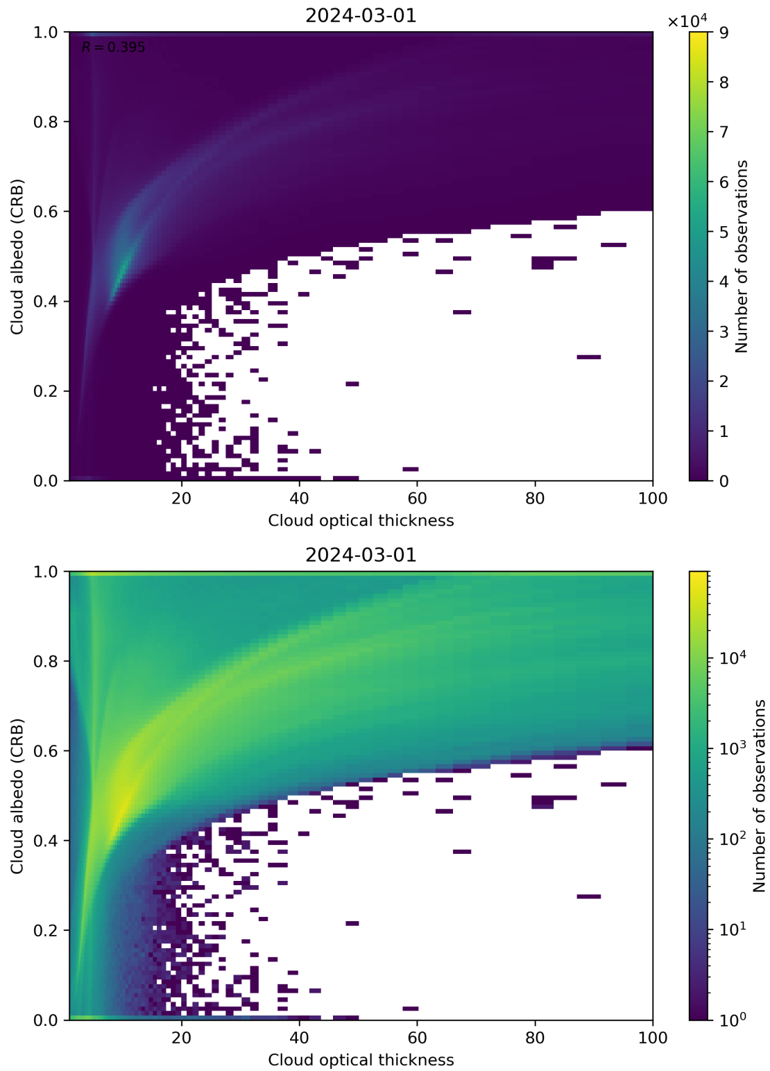
Figure 82: Scatter density plot of “Cloud optical thickness” against “Cloud albedo (CRB)” for 2024-02-29 to 2024-03-02.
