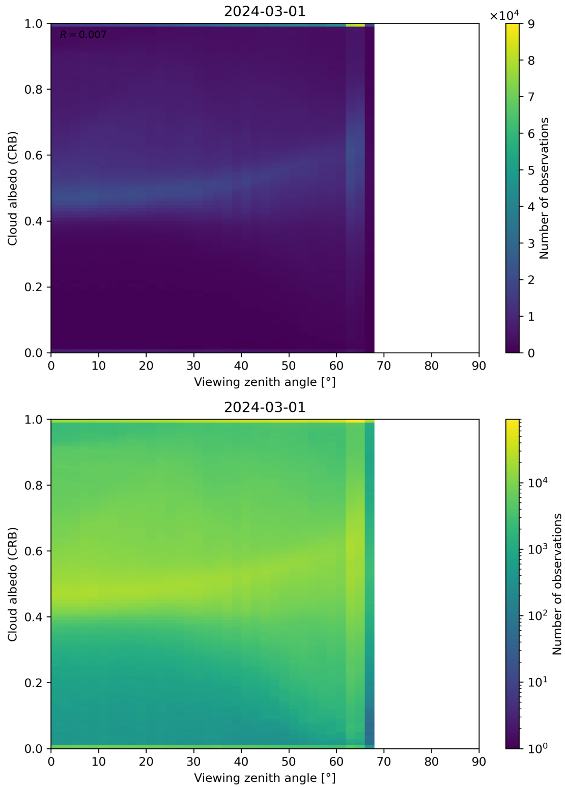
Figure 106: Scatter density plot of “Viewing zenith angle” against “Cloud albedo (CRB)” for 2024-02-29 to 2024-03-02.
