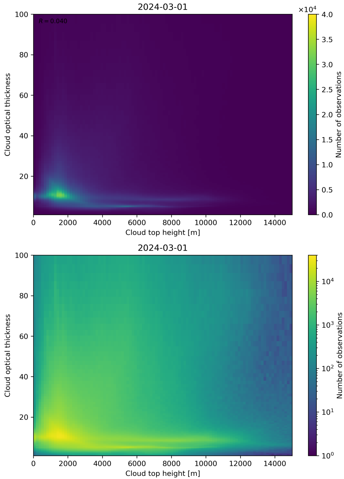
Figure 90: Scatter density plot of “Cloud top height” against “Cloud optical thickness” for 2024-02-29 to 2024-03-02.
