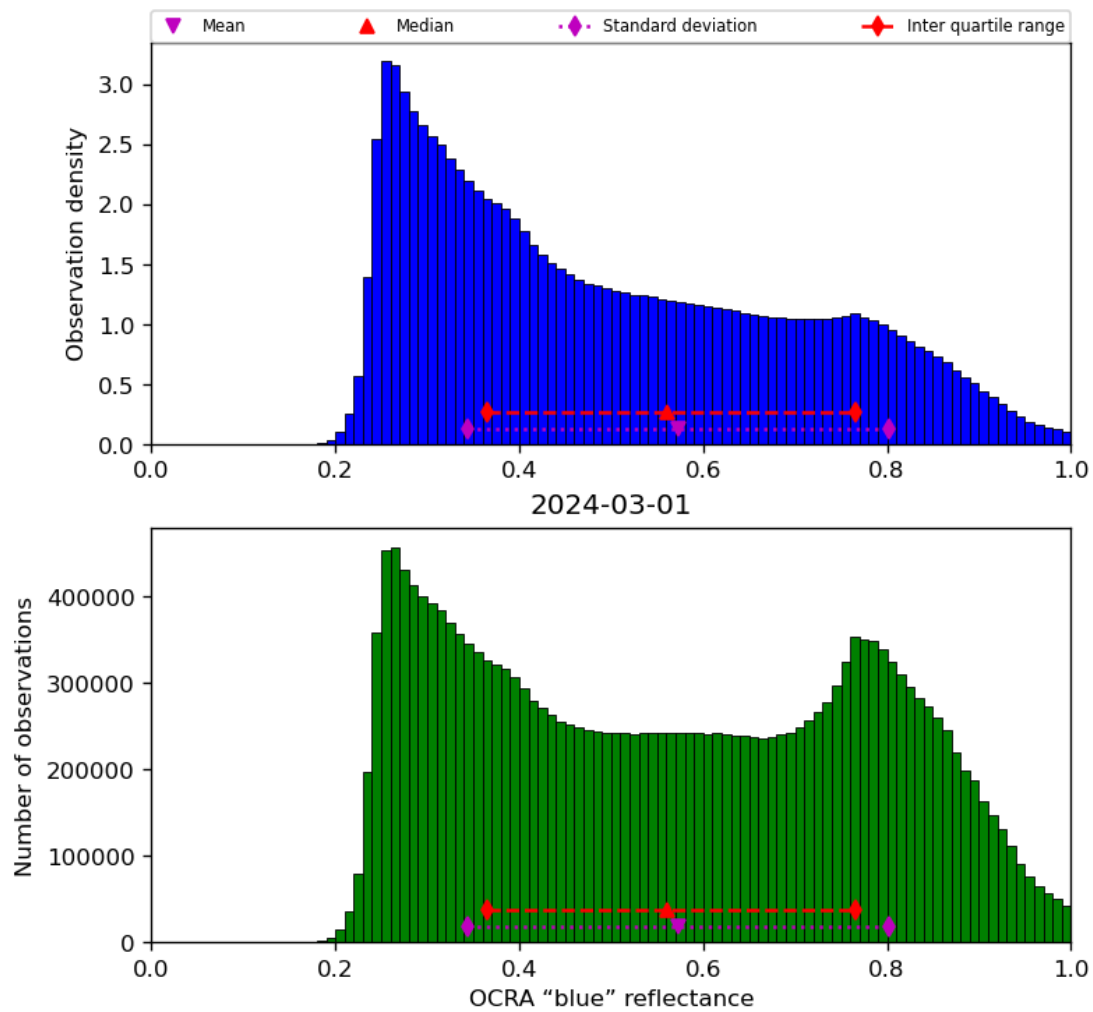
Figure 51: Histogram of “OCRA “blue” reflectance” for 2024-02-29 to 2024-03-02
