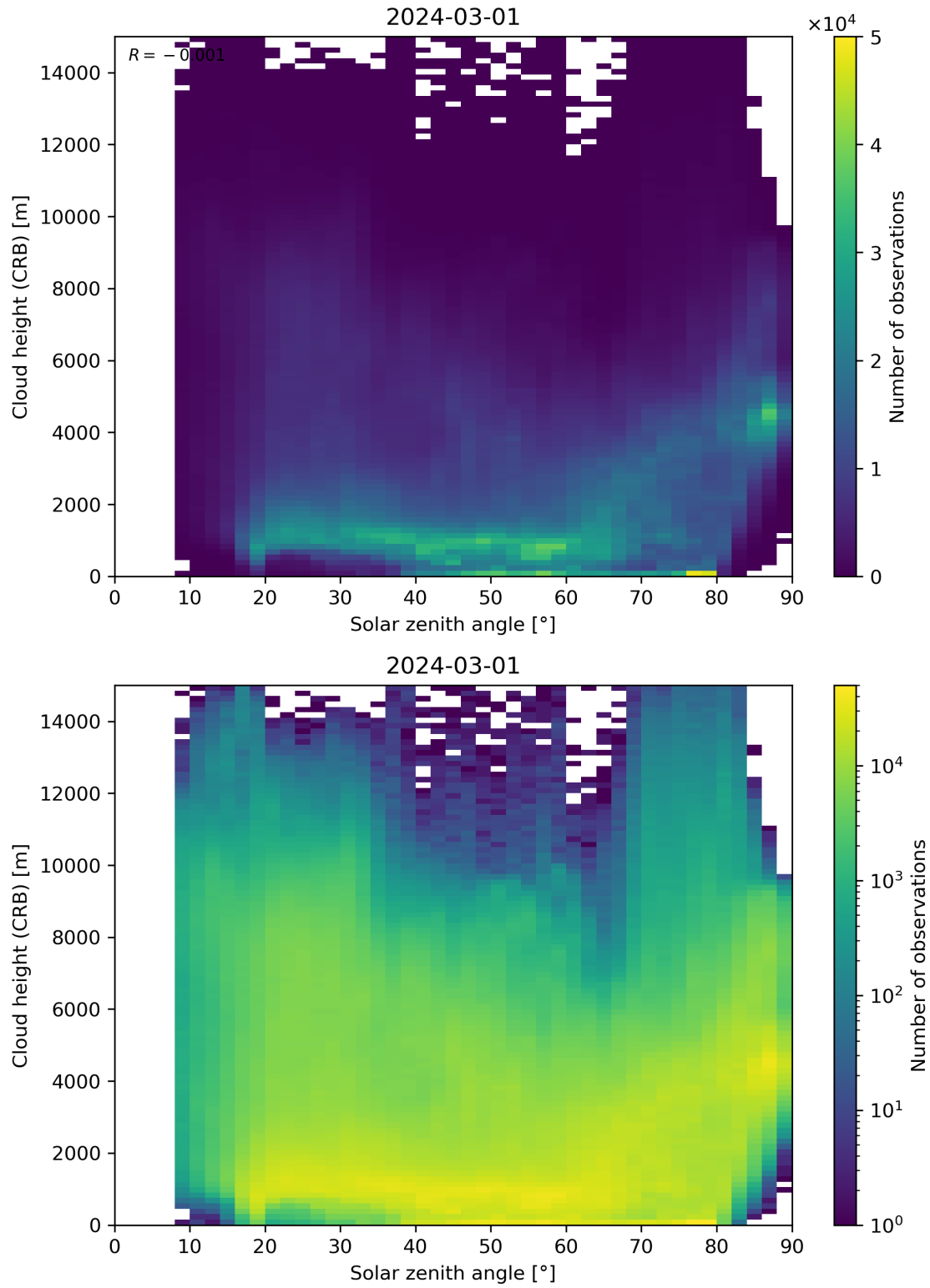
Figure 102: Scatter density plot of “Solar zenith angle” against “Cloud height (CRB)” for 2024-02-29 to 2024-03-02.
