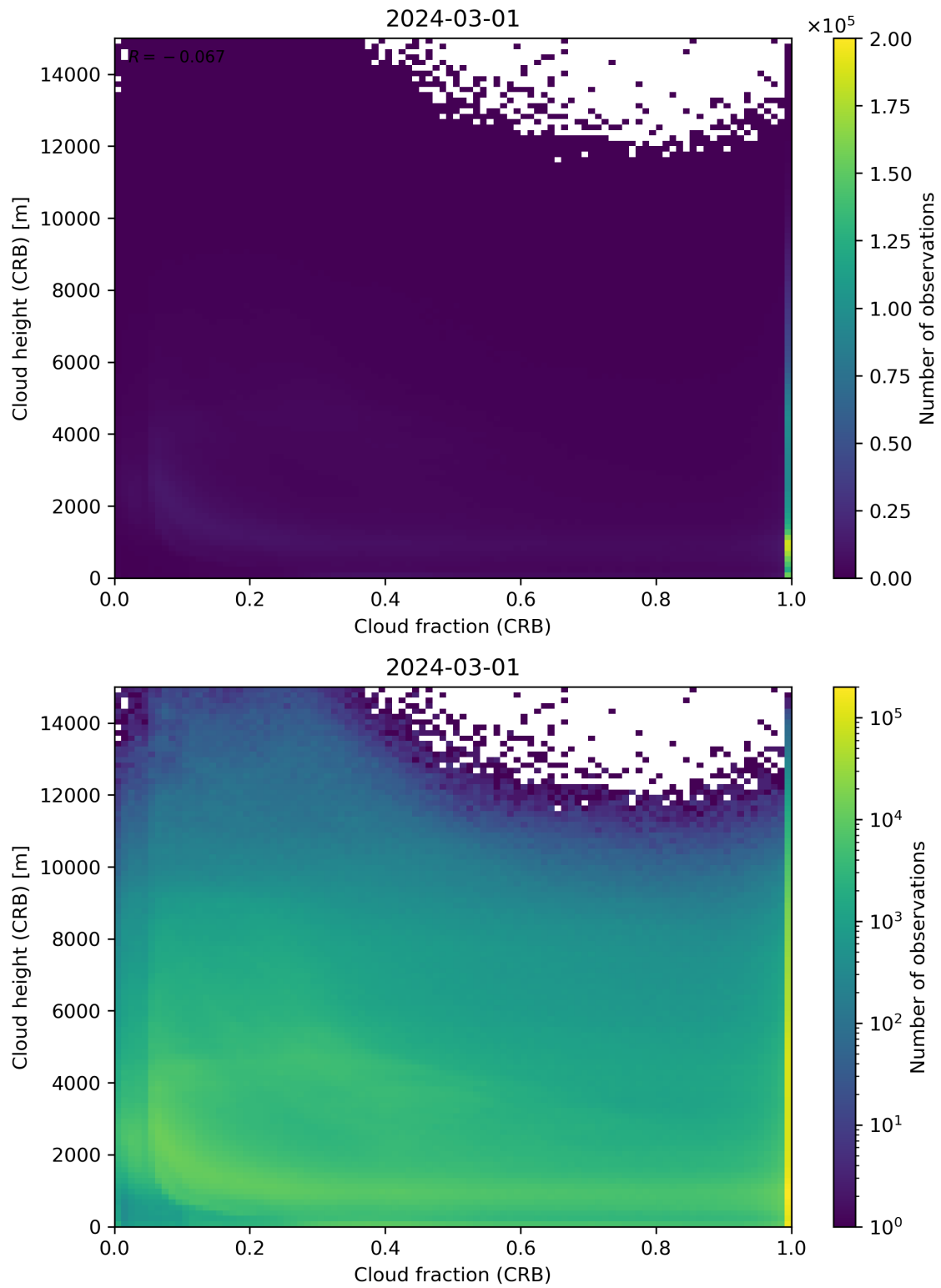
Figure 79: Scatter density plot of “Cloud fraction (CRB)” against “Cloud height (CRB)” for 2024-02-29 to 2024-03-02.
