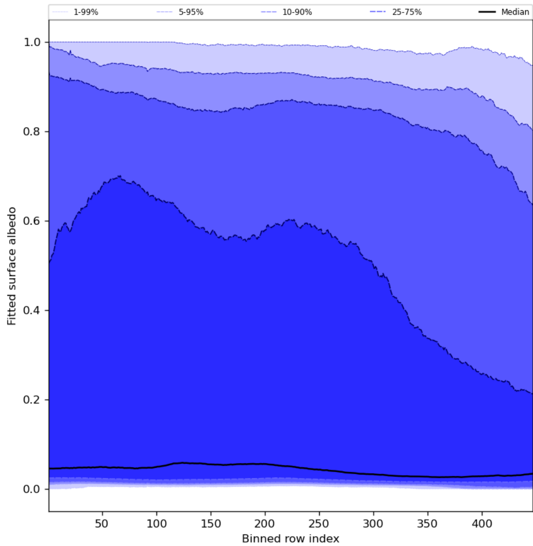
Figure 61: Along track statistics of “Fitted surface albedo” for 2024-02-29 to 2024-03-02
