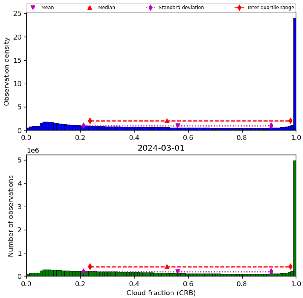
Figure 42: Histogram of “Cloud fraction (CRB)” for 2024-02-29 to 2024-03-02
