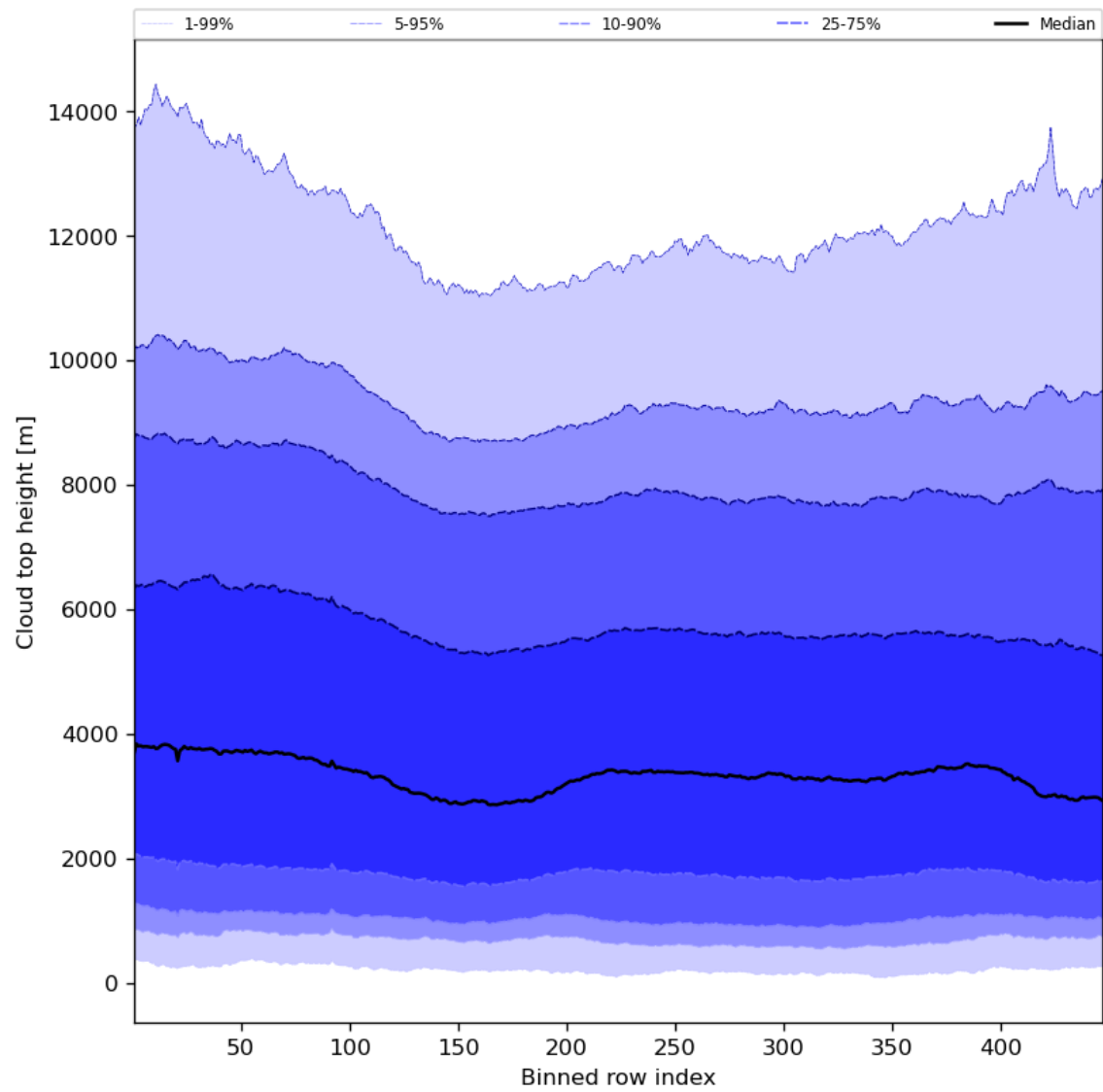
Figure 56: Along track statistics of “Cloud top height” for 2024-02-29 to 2024-03-02
