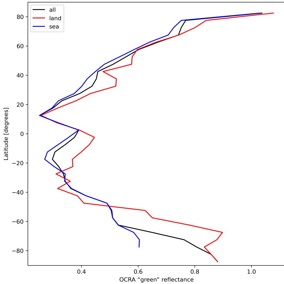
Figure 36: Zonal average of “OCRA “green” reflectance” for 2024-02-29 to 2024-03-02.
