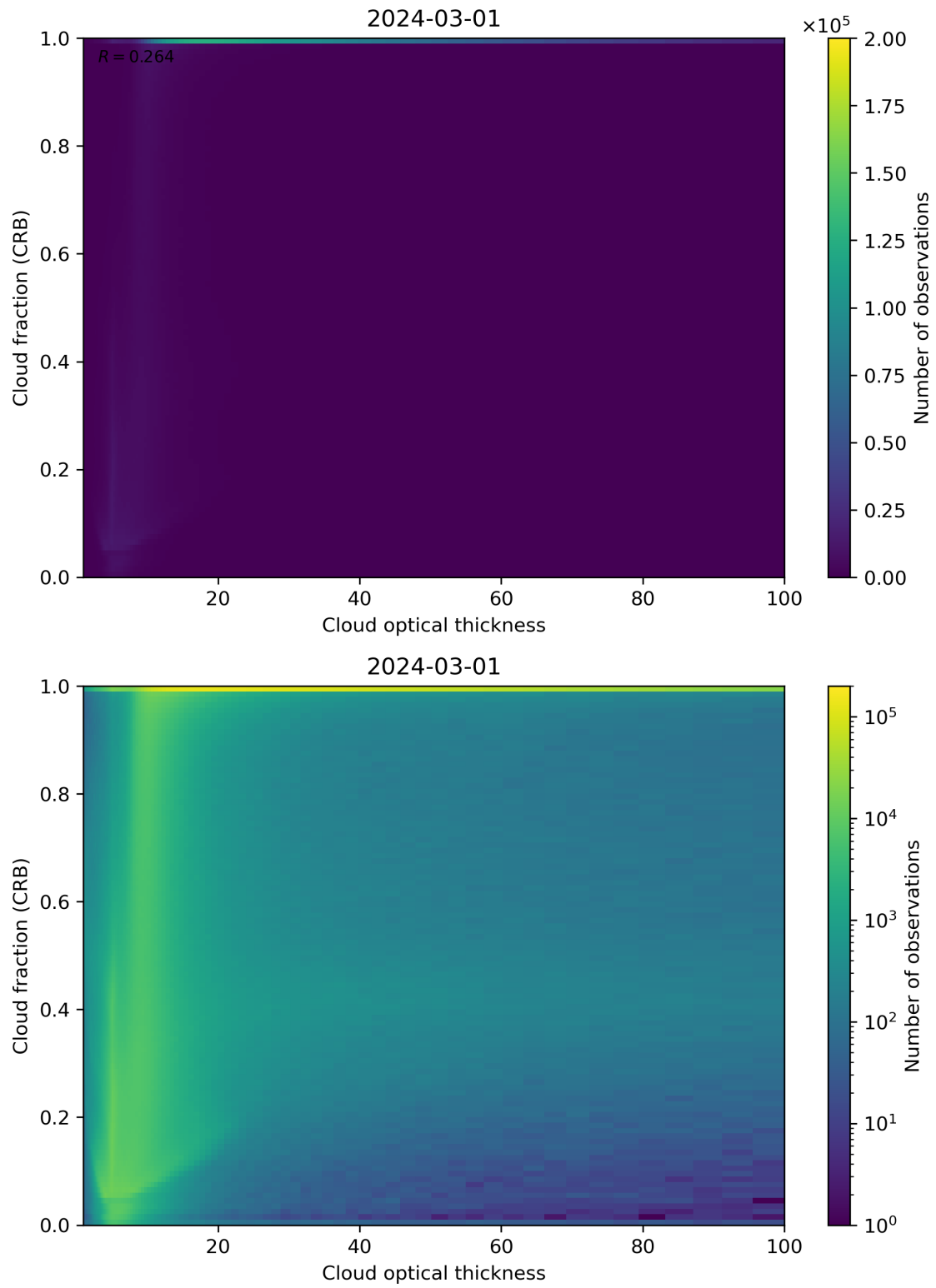
Figure 84: Scatter density plot of “Cloud optical thickness” against “Cloud fraction (CRB)” for 2024-02-29 to 2024-03-02.
