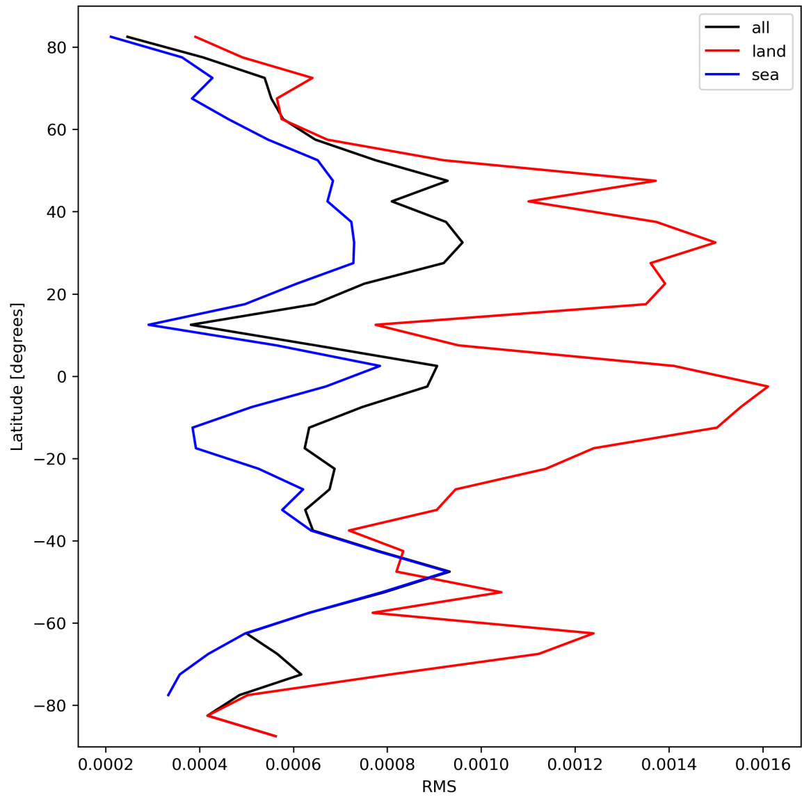
Figure 31: Zonal average of “RMS” for 2024-02-29 to 2024-03-02.
