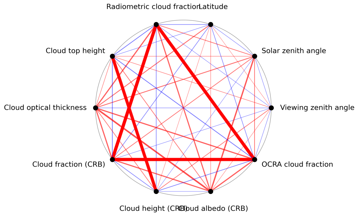
Figure 1: Map of correlation graph for 2024-02-29 to 2024-03-02.
