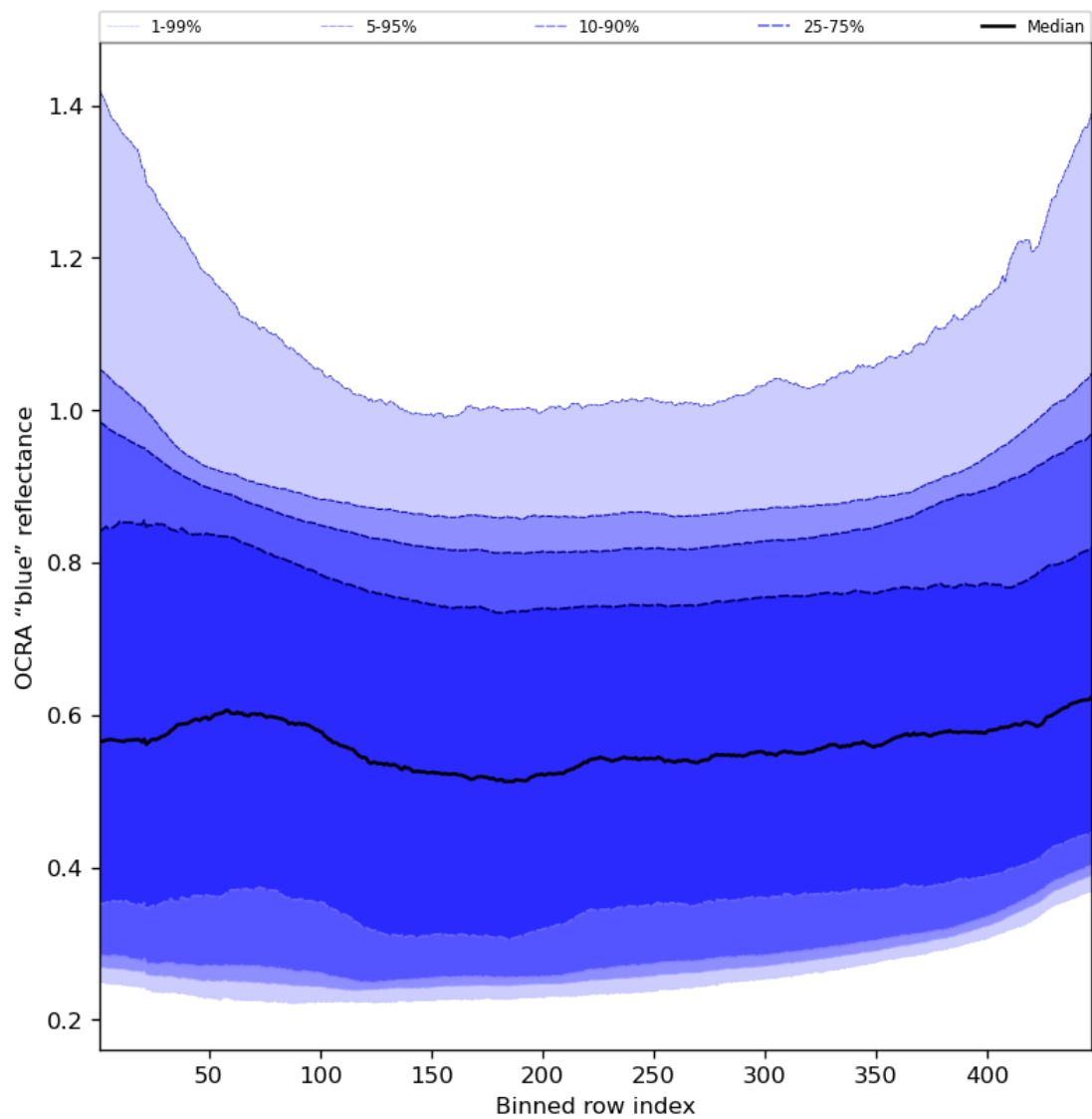
Figure 67: Along track statistics of "OCRA "blue" reflectance" for 2024-02-29 to 2024-03-02
