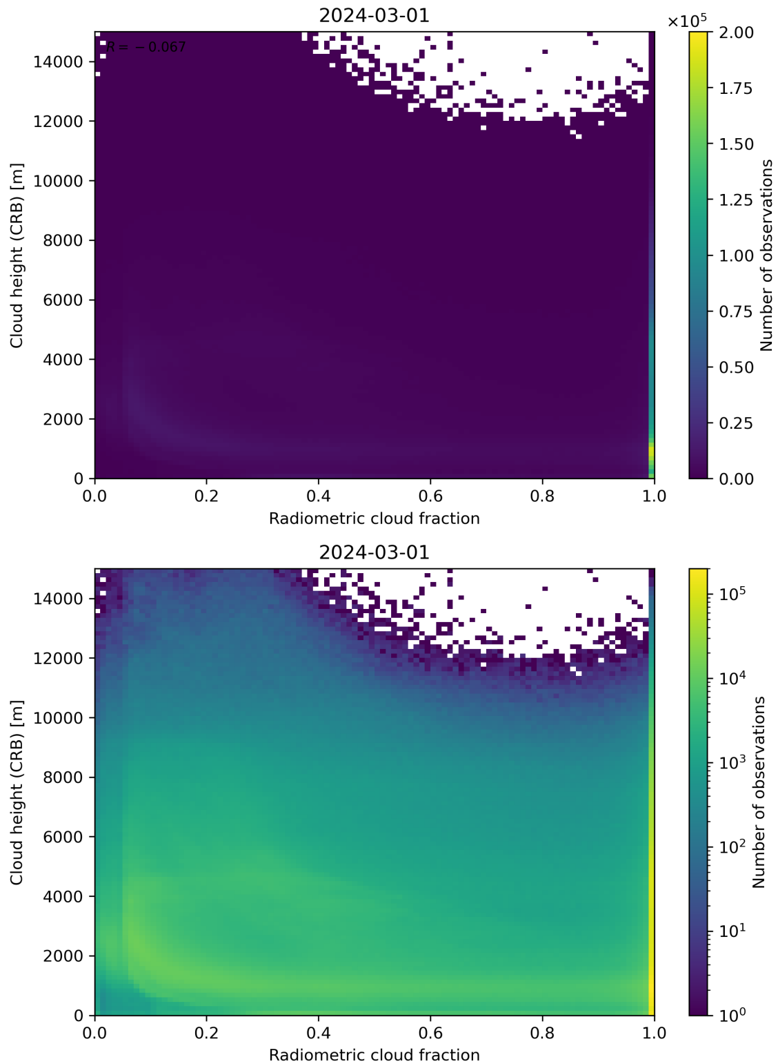
Figure 74: Scatter density plot of “Radiometric cloud fraction” against “Cloud height (CRB)” for 2024-02-29 to 2024-03-02.
