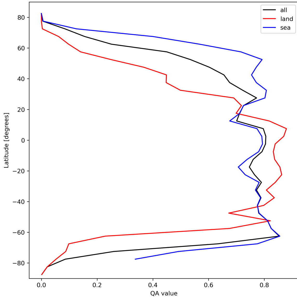
Figure 22: Zonal average of “QA value” for 2024-02-29 to 2024-03-02.
