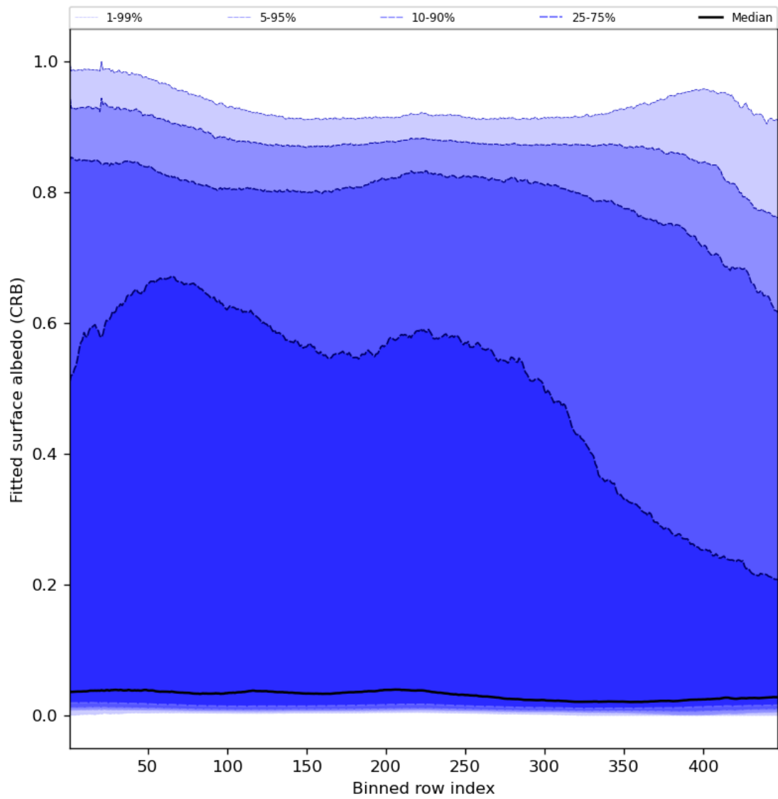
Figure 62: Along track statistics of “Fitted surface albedo (CRB)” for 2024-02-29 to 2024-03-02
