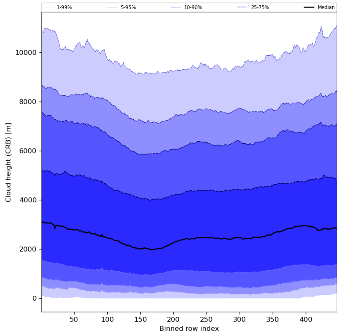
Figure 59: Along track statistics of “Cloud height (CRB)” for 2024-02-29 to 2024-03-02
