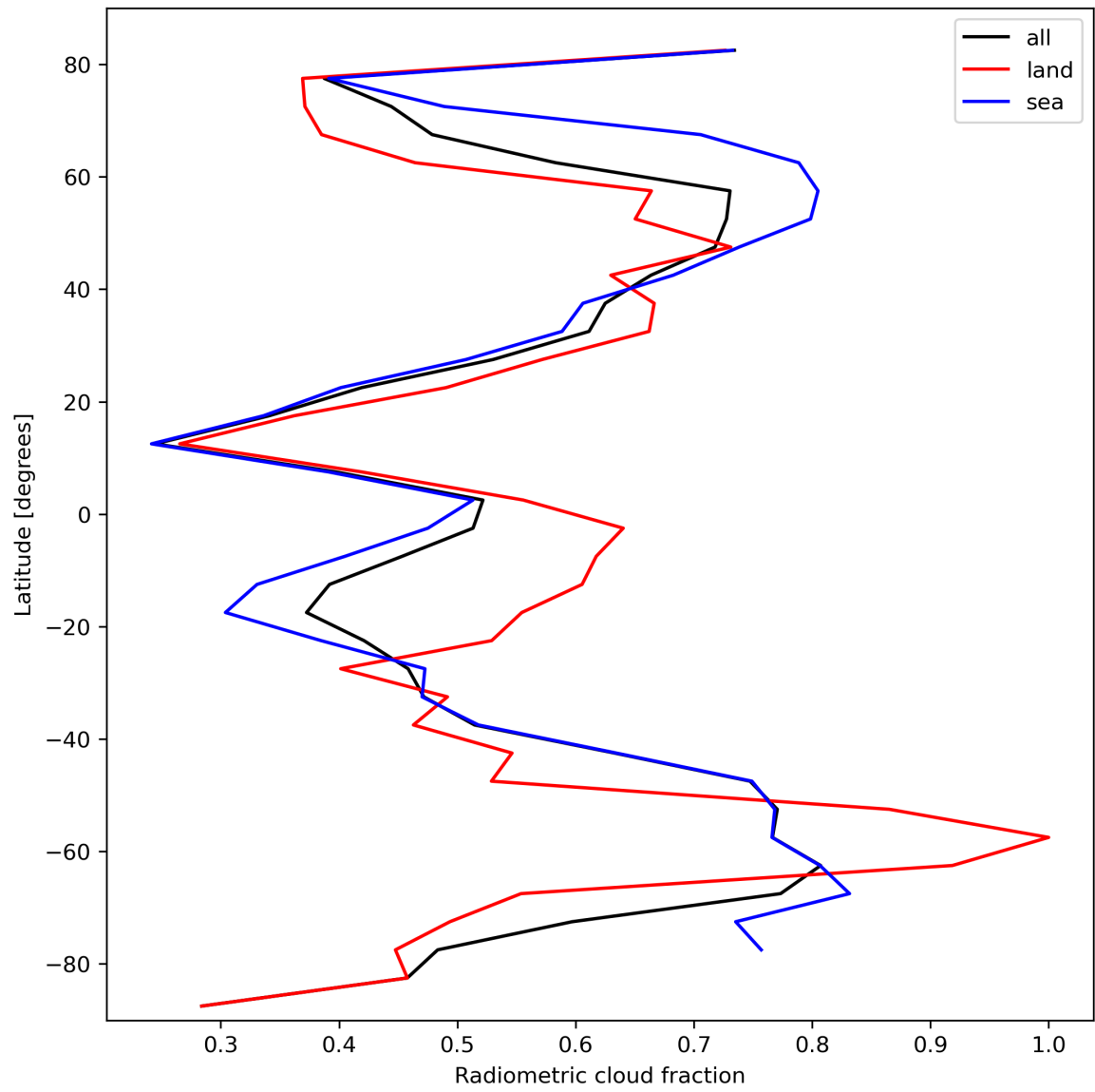
Figure 23: Zonal average of “Radiometric cloud fraction” for 2024-02-29 to 2024-03-02.
