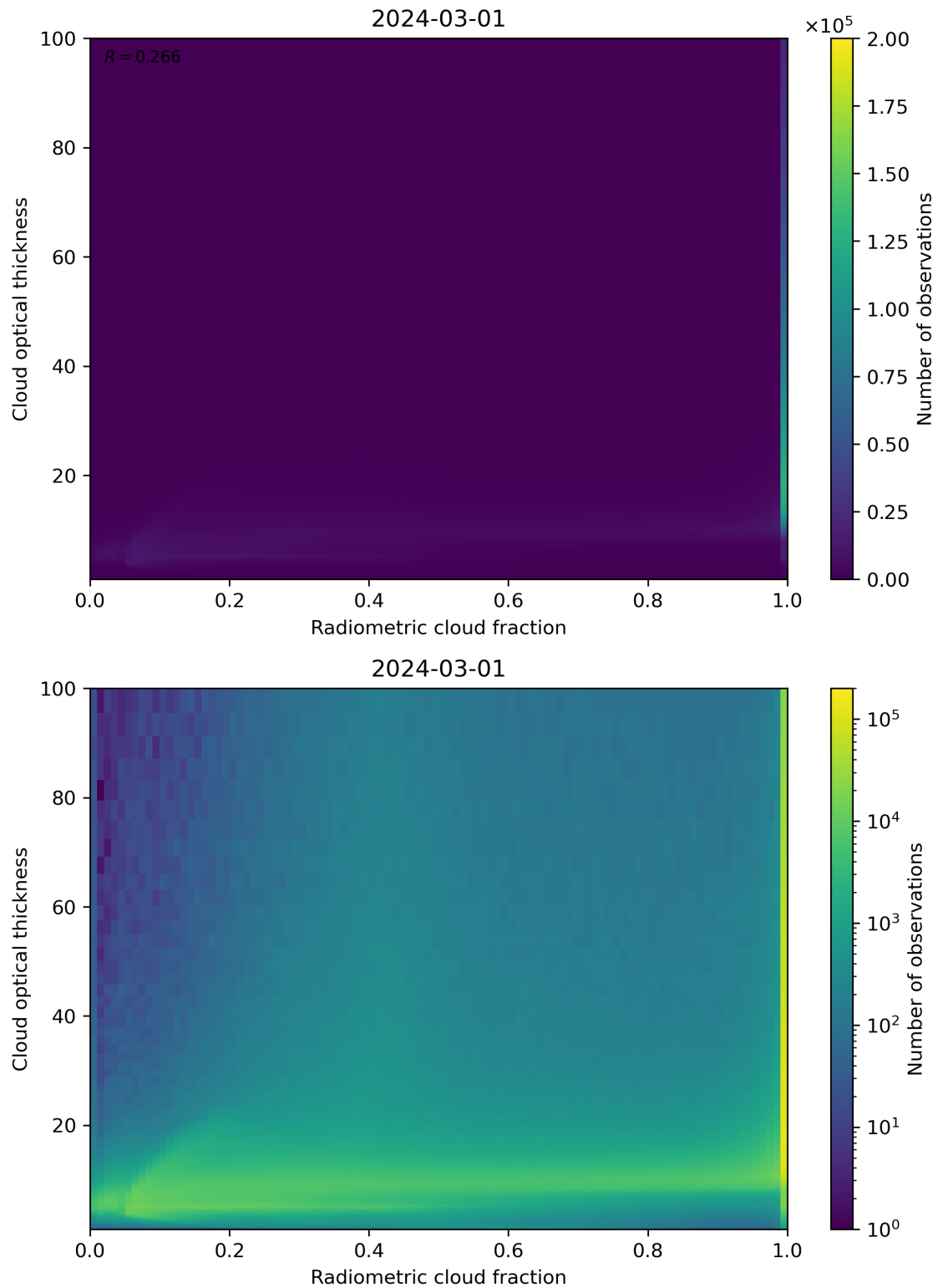
Figure 75: Scatter density plot of “Radiometric cloud fraction” against “Cloud optical thickness” for 2024-02-29 to 2024-03-02.
