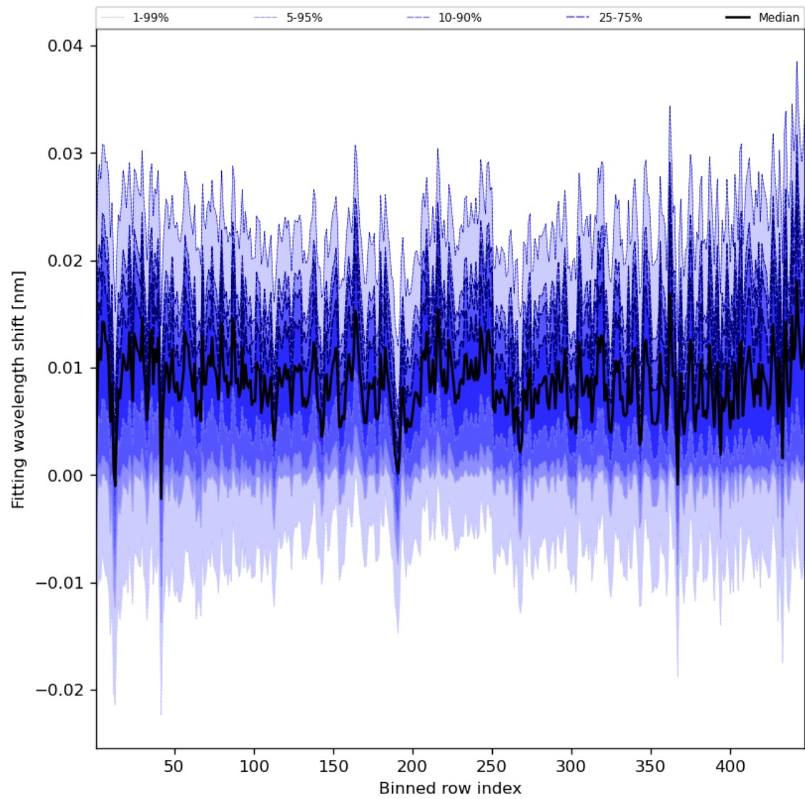
Figure 65: Along track statistics of “Fitting wavelength shift” for 2024-02-29 to 2024-03-02
