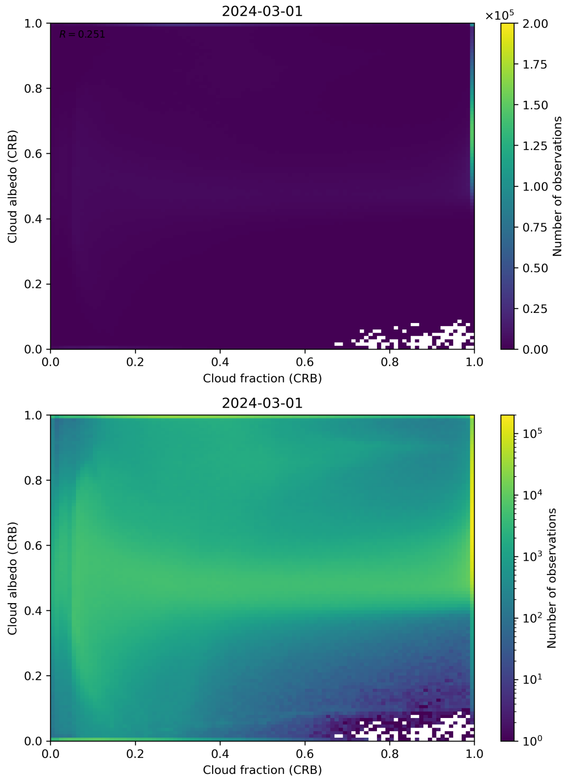
Figure 77: Scatter density plot of “Cloud fraction (CRB)” against “Cloud albedo (CRB)” for 2024-02-29 to 2024-03-02.
