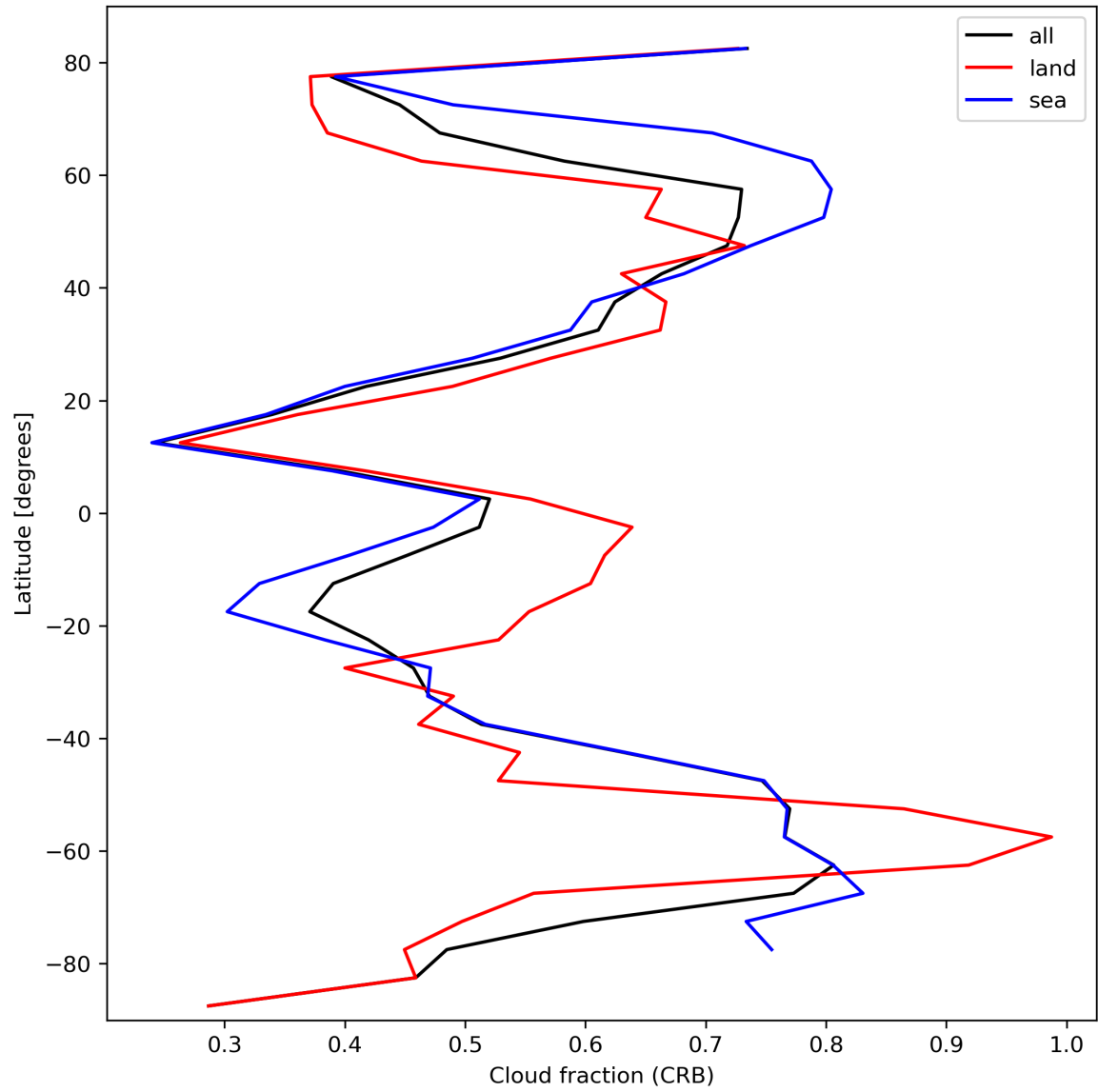
Figure 26: Zonal average of “Cloud fraction (CRB)” for 2024-02-29 to 2024-03-02.
