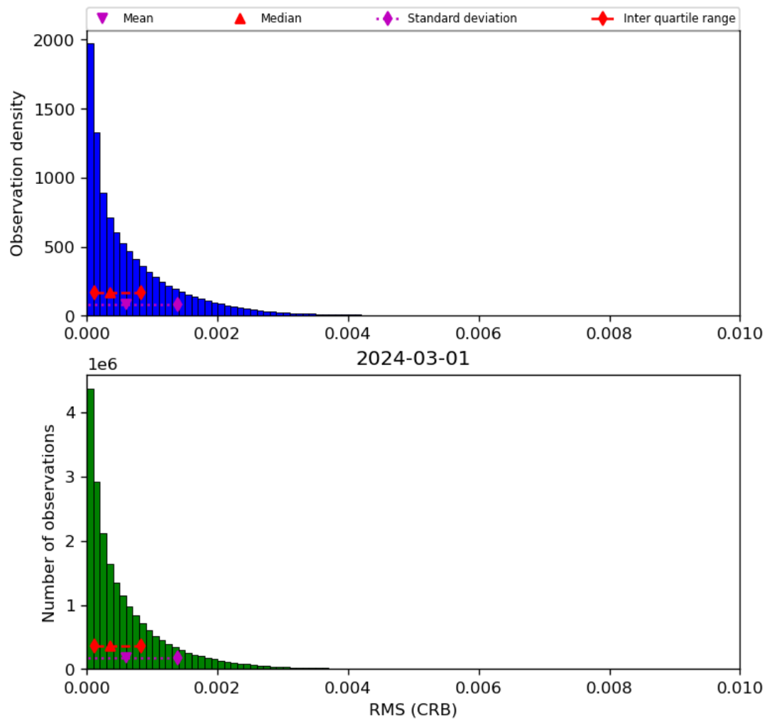
Figure 48: Histogram of “RMS (CRB)” for 2024-02-29 to 2024-03-02
