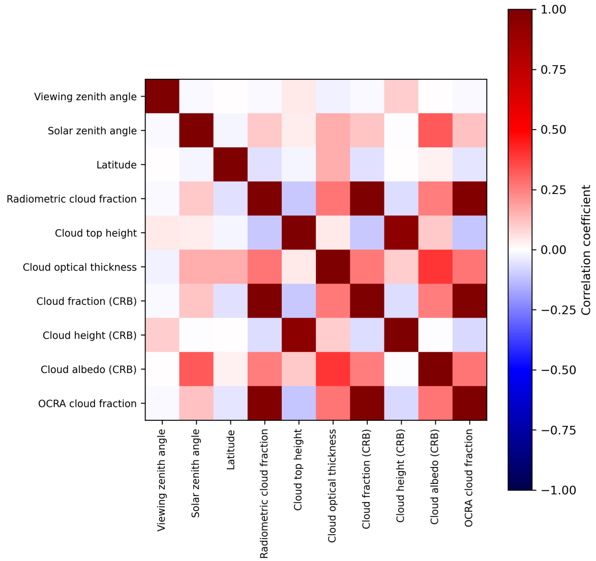
Figure 2: Map of correlation matrix for 2024-02-29 to 2024-03-02.
