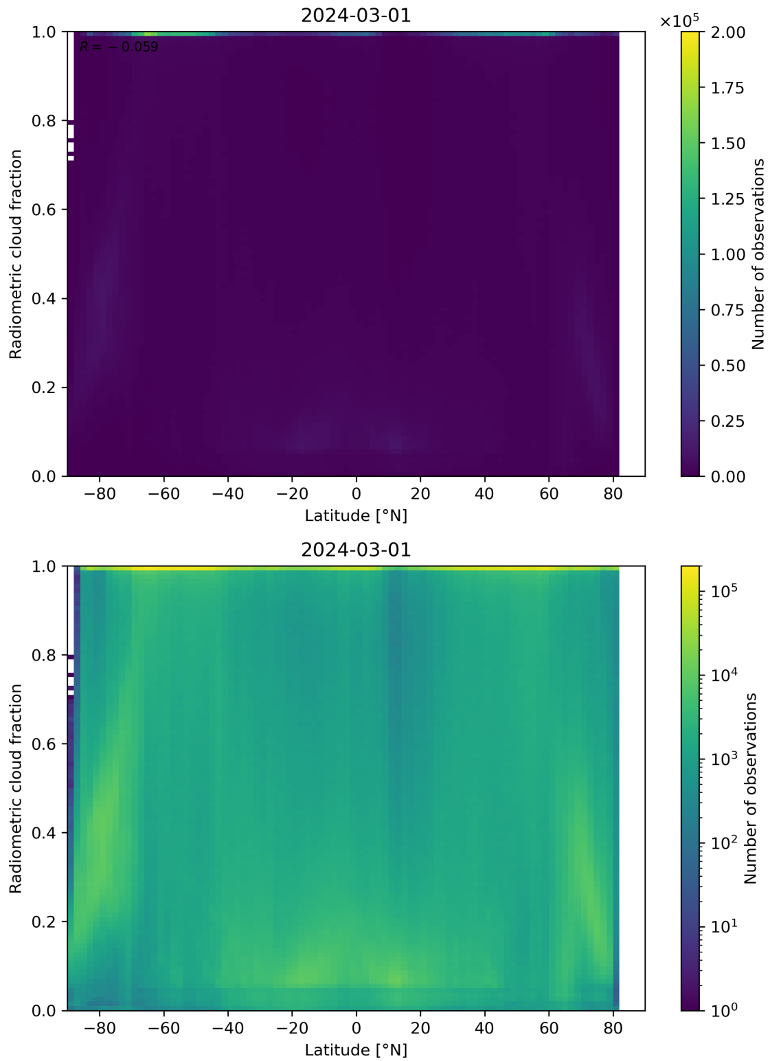
Figure 92: Scatter density plot of “Latitude” against “Radiometric cloud fraction” for 2024-02-29 to 2024-03-02.
