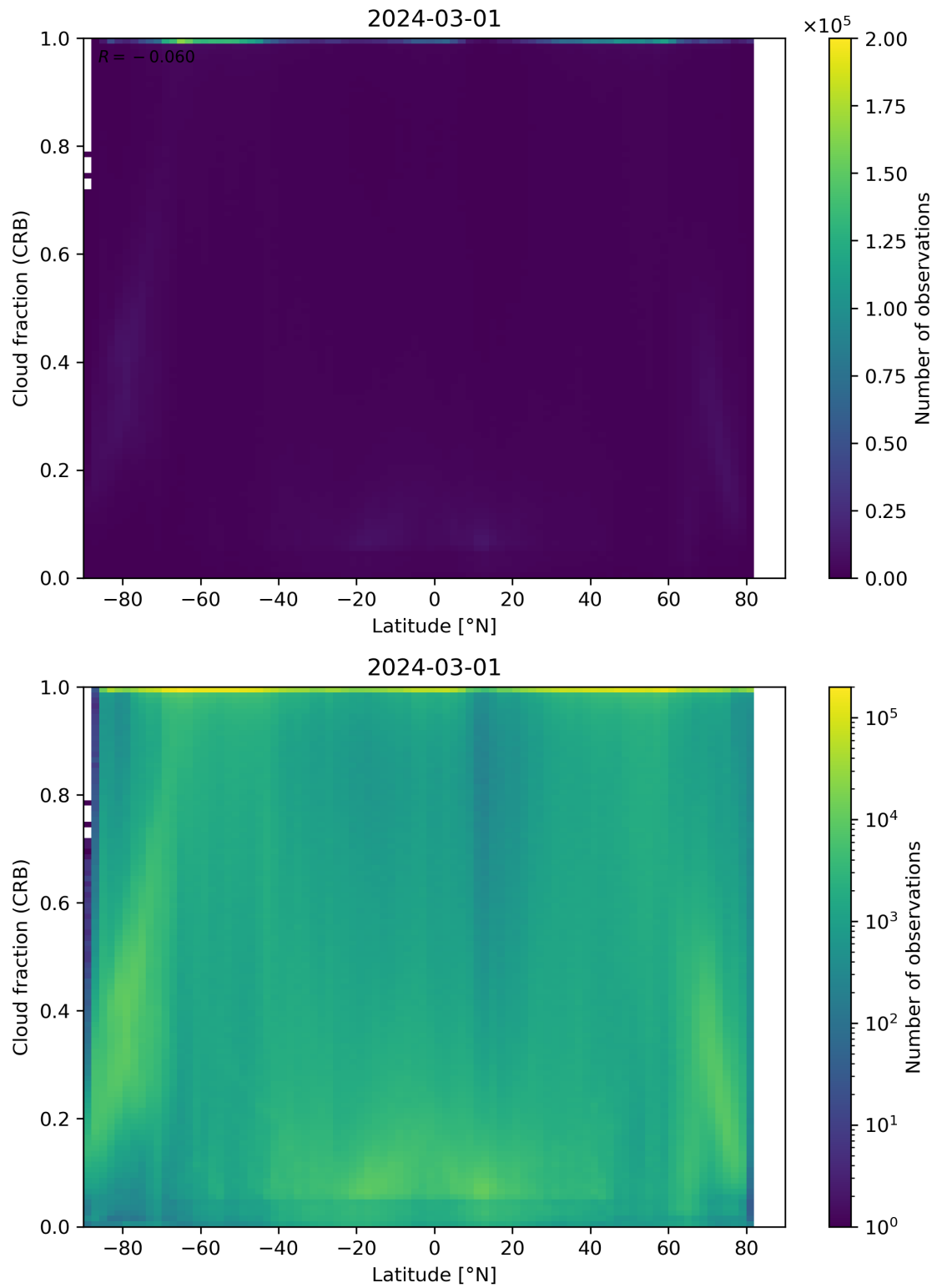
Figure 94: Scatter density plot of “Latitude” against “Cloud fraction (CRB)” for 2024-02-29 to 2024-03-02.
