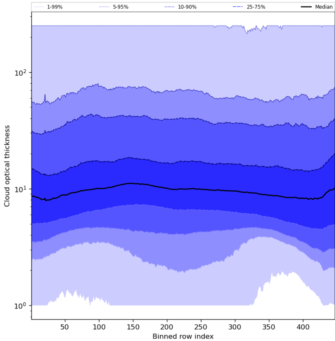
Figure 57: Along track statistics of “Cloud optical thickness” for 2024-02-29 to 2024-03-02
