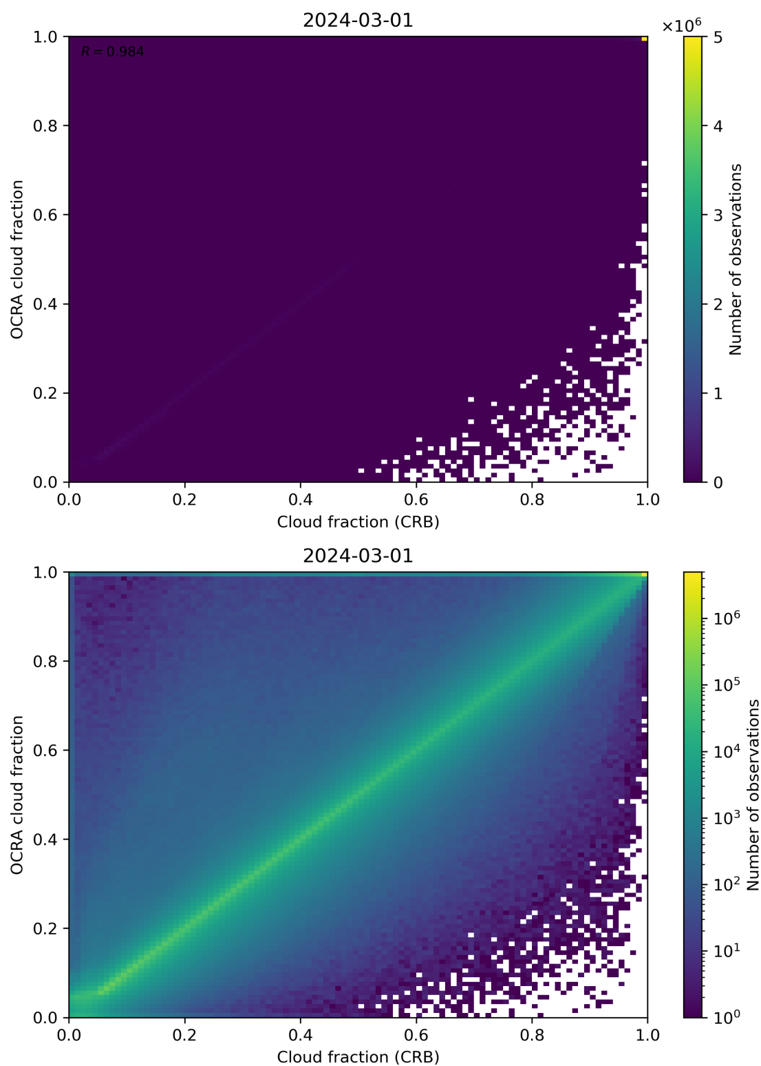
Figure 78: Scatter density plot of “Cloud fraction (CRB)” against “OCRA cloud fraction” for 2024-02-29 to 2024-03-02.
