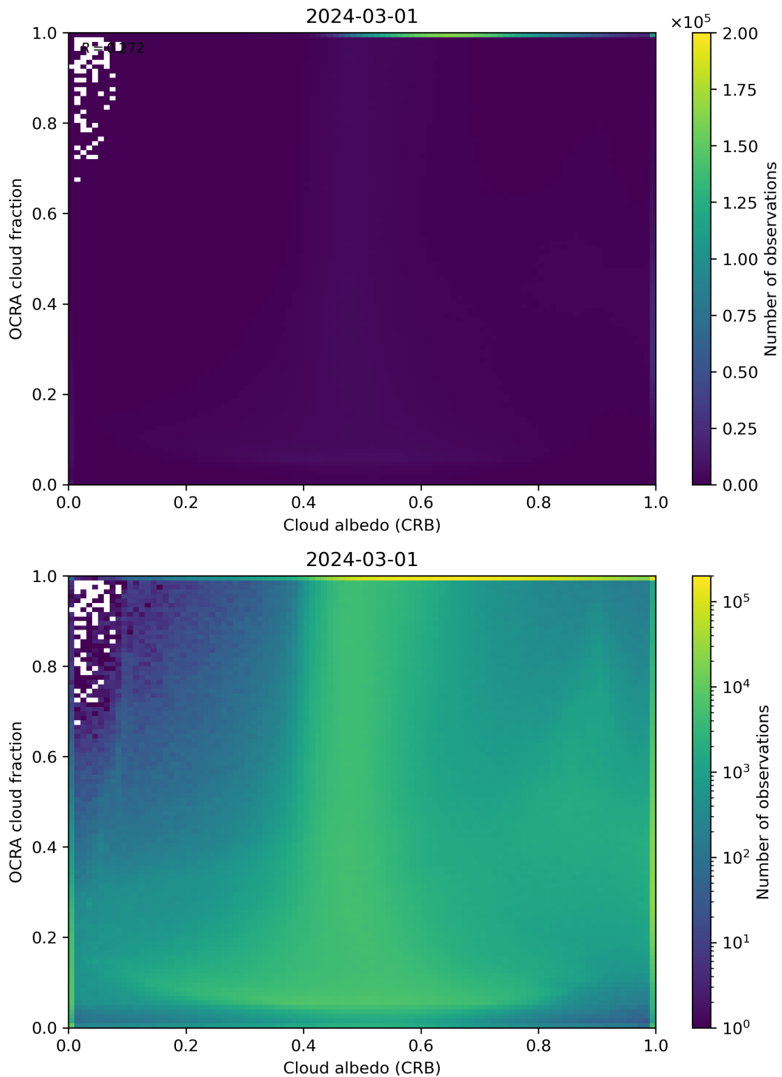
Figure 70: Scatter density plot of “Cloud albedo (CRB)” against “OCRA cloud fraction” for 2024-02-29 to 2024-03-02.
