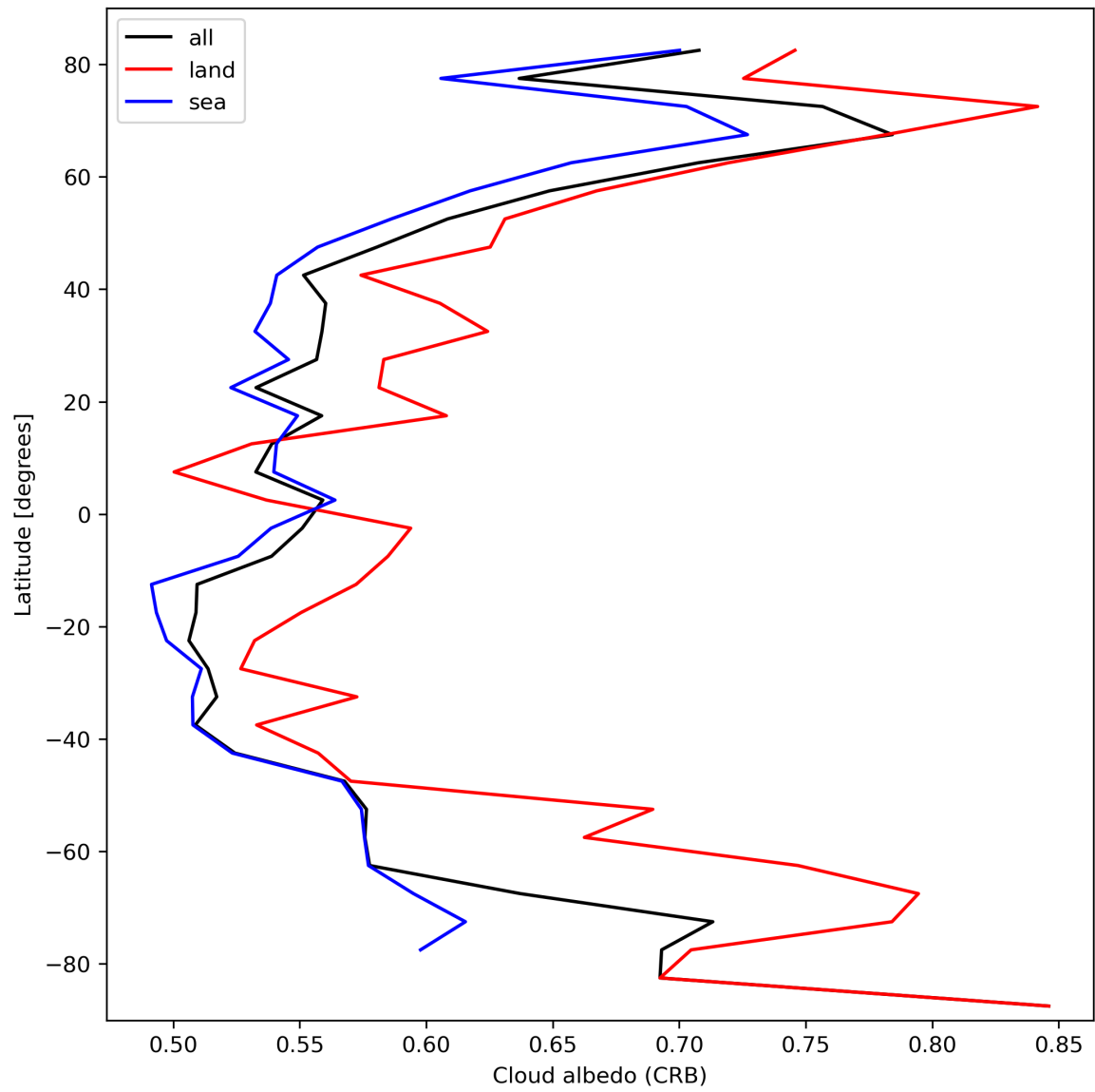
Figure 28: Zonal average of “Cloud albedo (CRB)” for 2024-02-29 to 2024-03-02.
