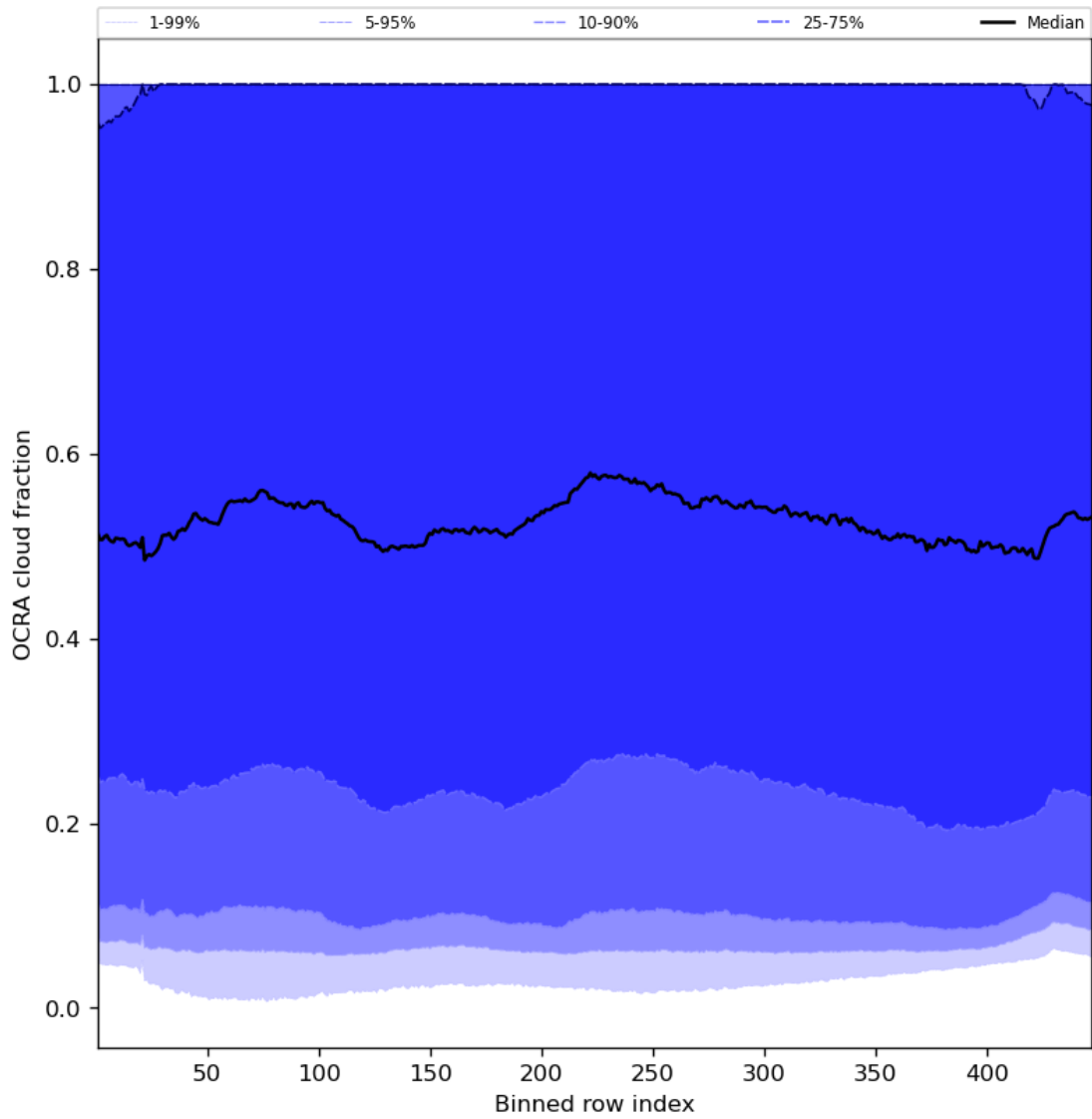
Figure 66: Along track statistics of “OCRA cloud fraction” for 2024-02-29 to 2024-03-02
