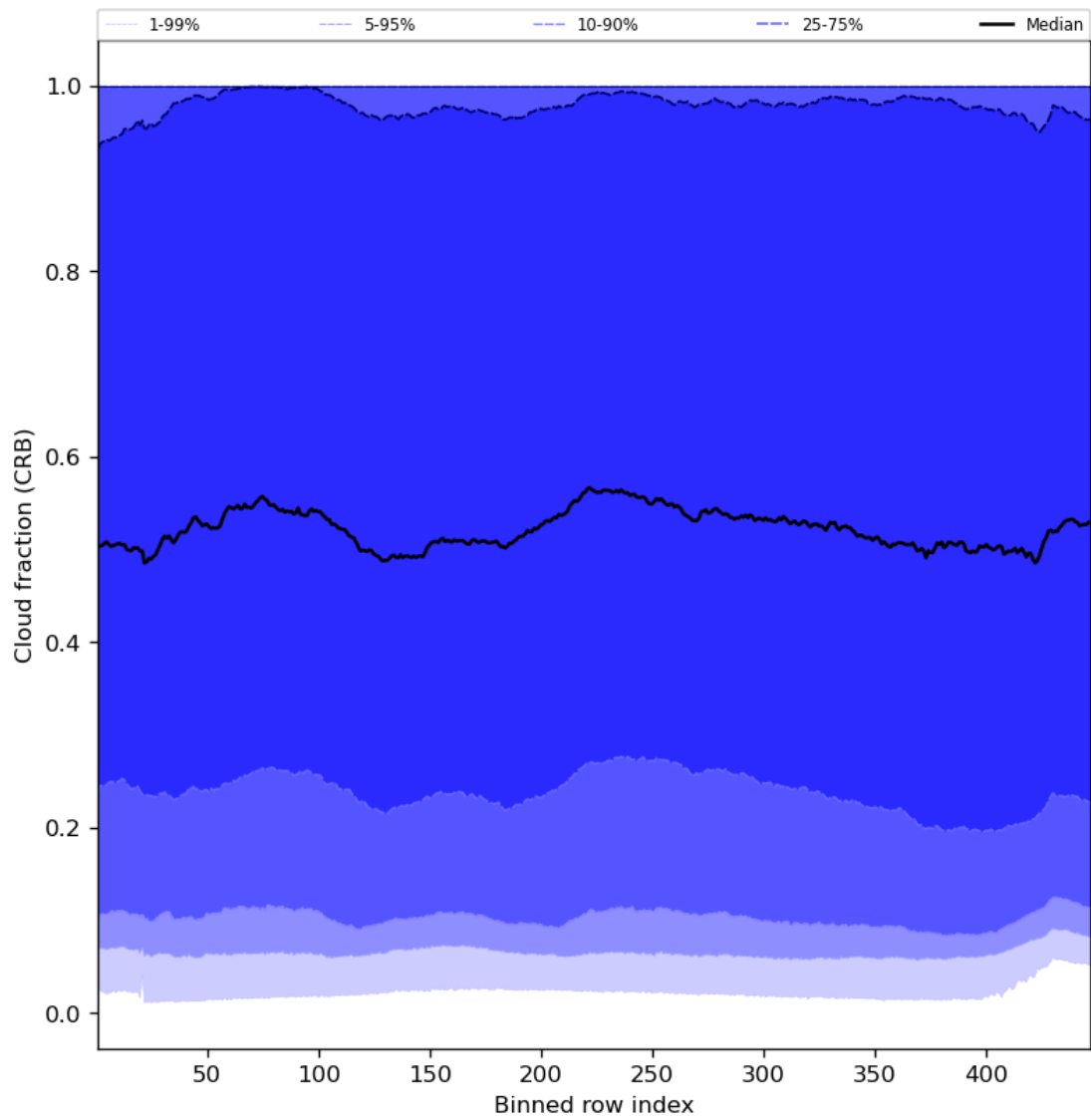
Figure 58: Along track statistics of “Cloud fraction (CRB)” for 2024-02-29 to 2024-03-02
