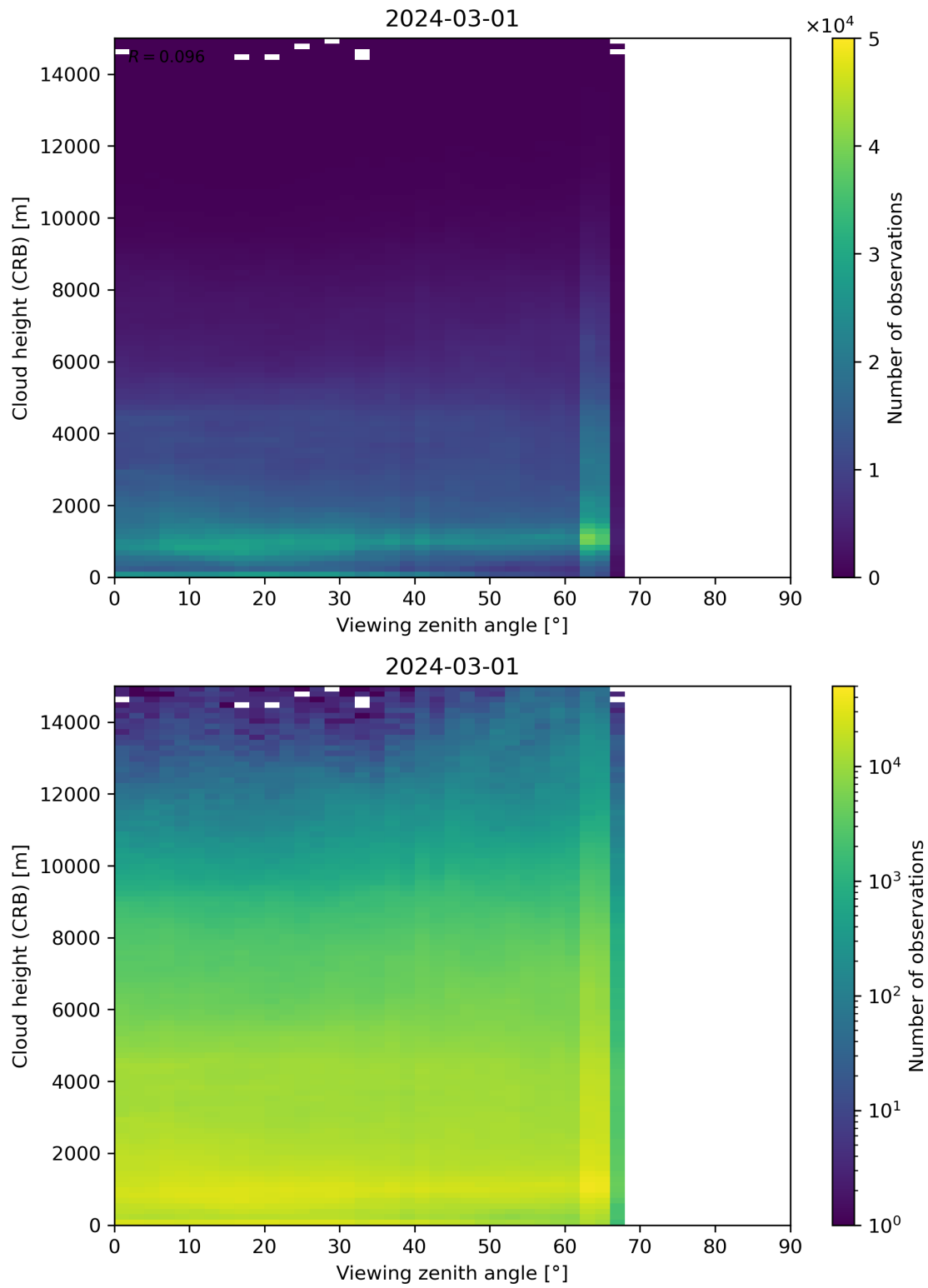
Figure 110: Scatter density plot of “Viewing zenith angle” against “Cloud height (CRB)” for 2024-02-29 to 2024-03-02.
