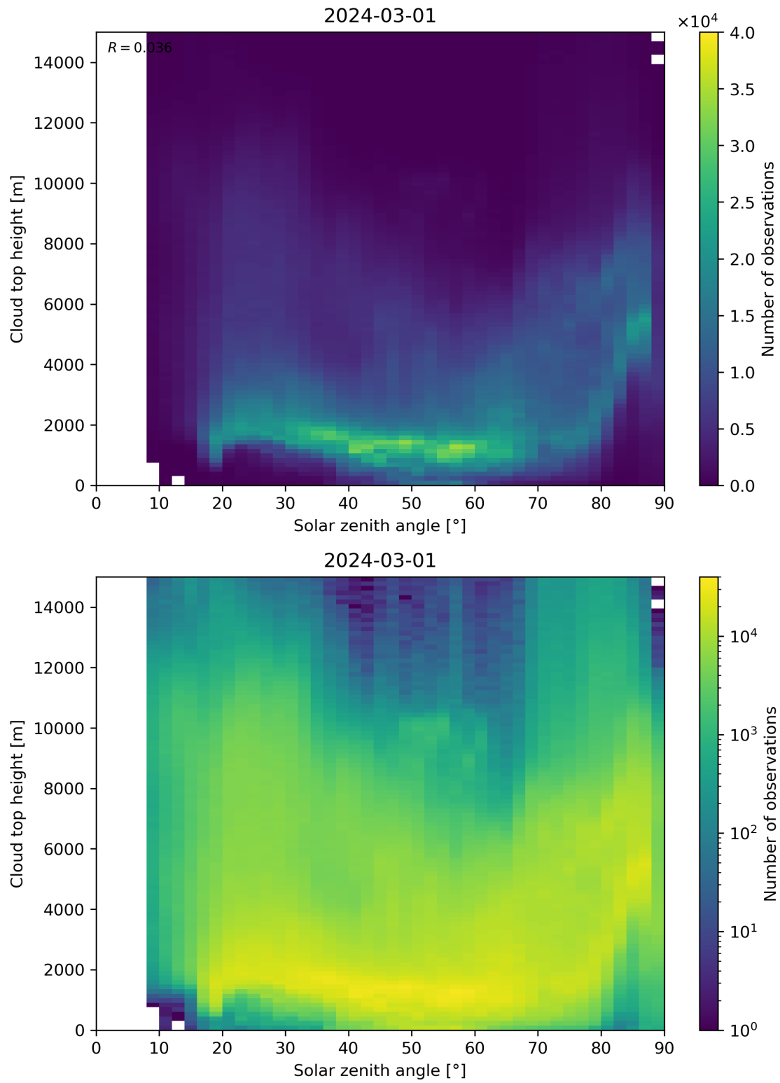
Figure 104: Scatter density plot of “Solar zenith angle” against “Cloud top height” for 2024-02-29 to 2024-03-02.
