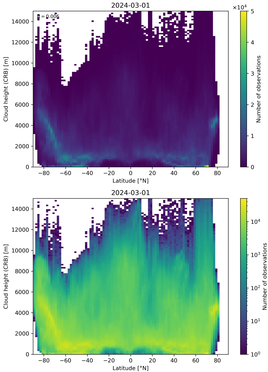
Figure 95: Scatter density plot of “Latitude” against “Cloud height (CRB)” for 2024-02-29 to 2024-03-02.
