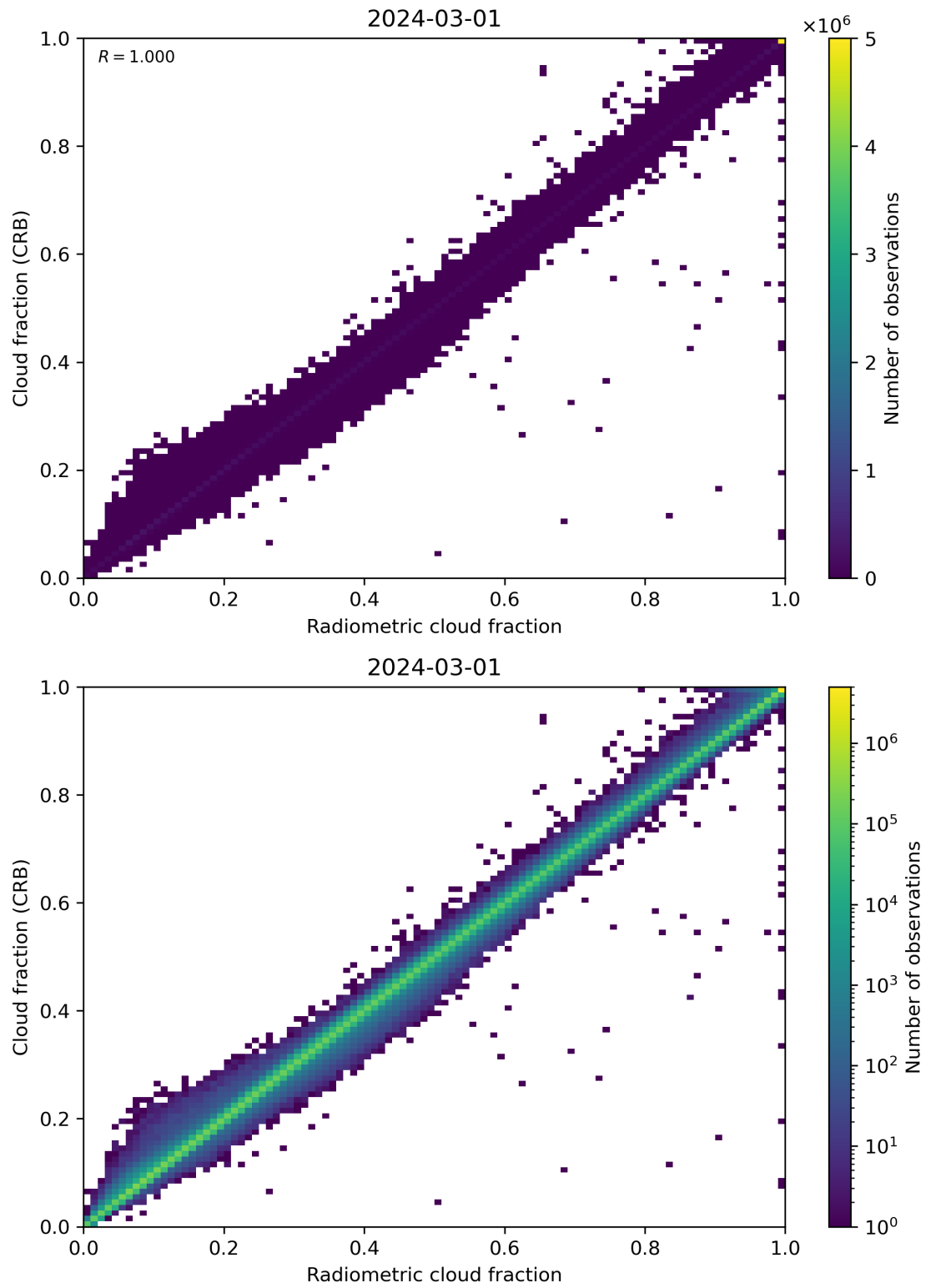
Figure 73: Scatter density plot of “Radiometric cloud fraction” against “Cloud fraction (CRB)” for 2024-02-29 to 2024-03-02.
