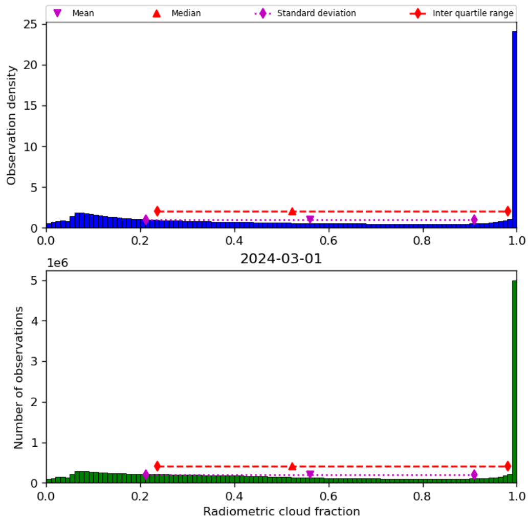
Figure 39: Histogram of “Radiometric cloud fraction” for 2024-02-29 to 2024-03-02
