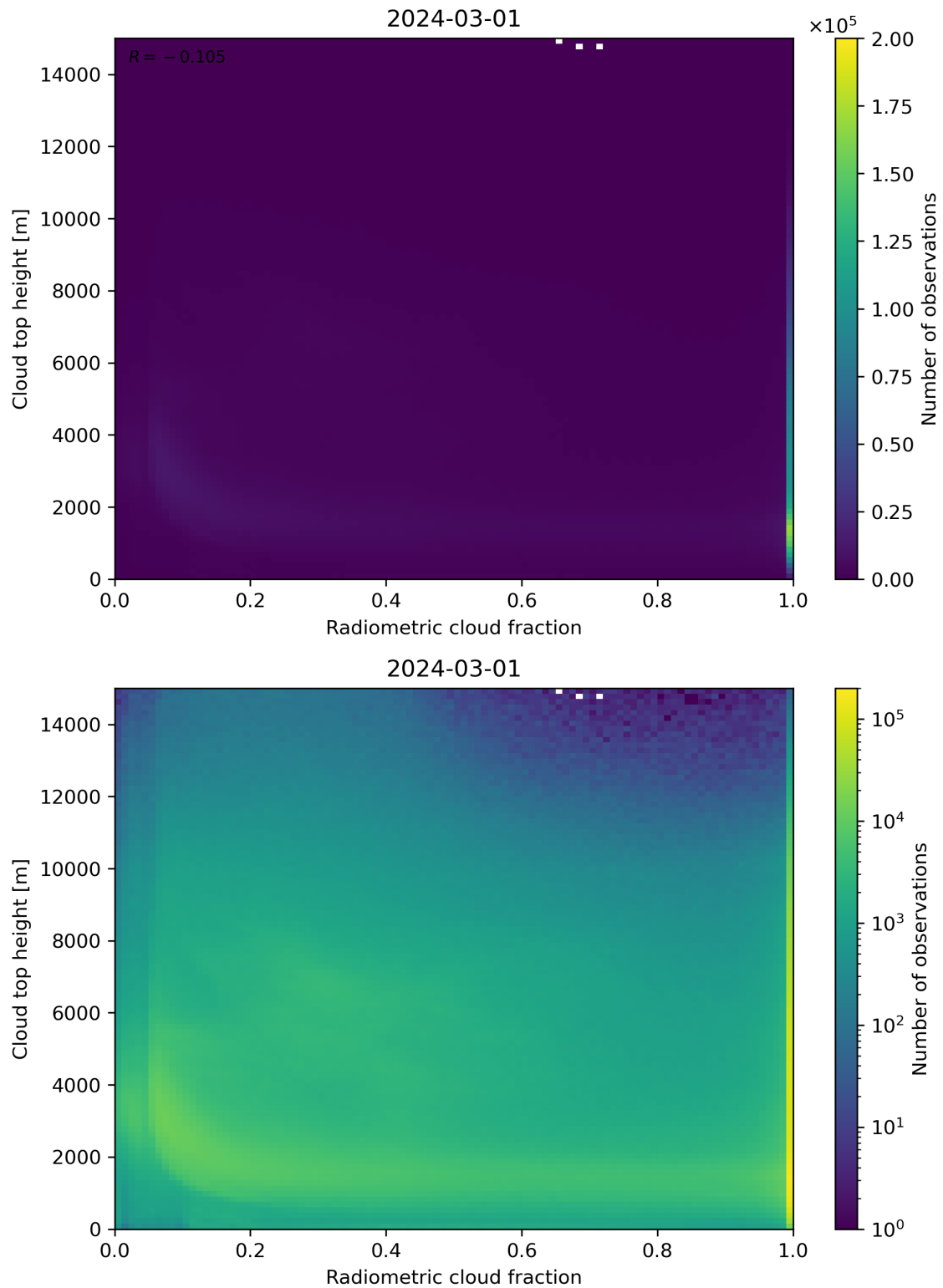
Figure 76: Scatter density plot of “Radiometric cloud fraction” against “Cloud top height” for 2024-02-29 to 2024-03-02.
