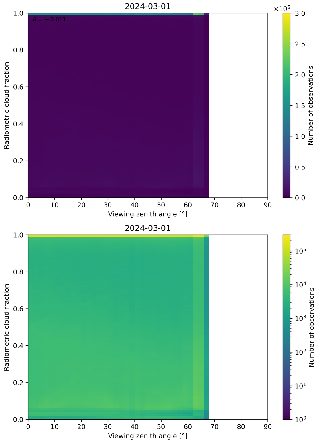
Figure 107: Scatter density plot of “Viewing zenith angle” against “Radiometric cloud fraction” for 2024-02-29 to 2024-03-02.
