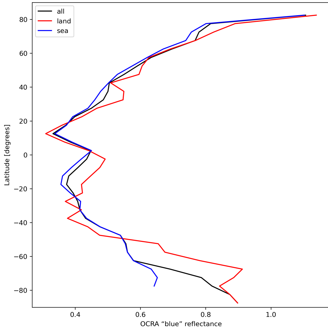
Figure 35: Zonal average of “OCRA “blue” reflectance” for 2024-02-29 to 2024-03-02.
