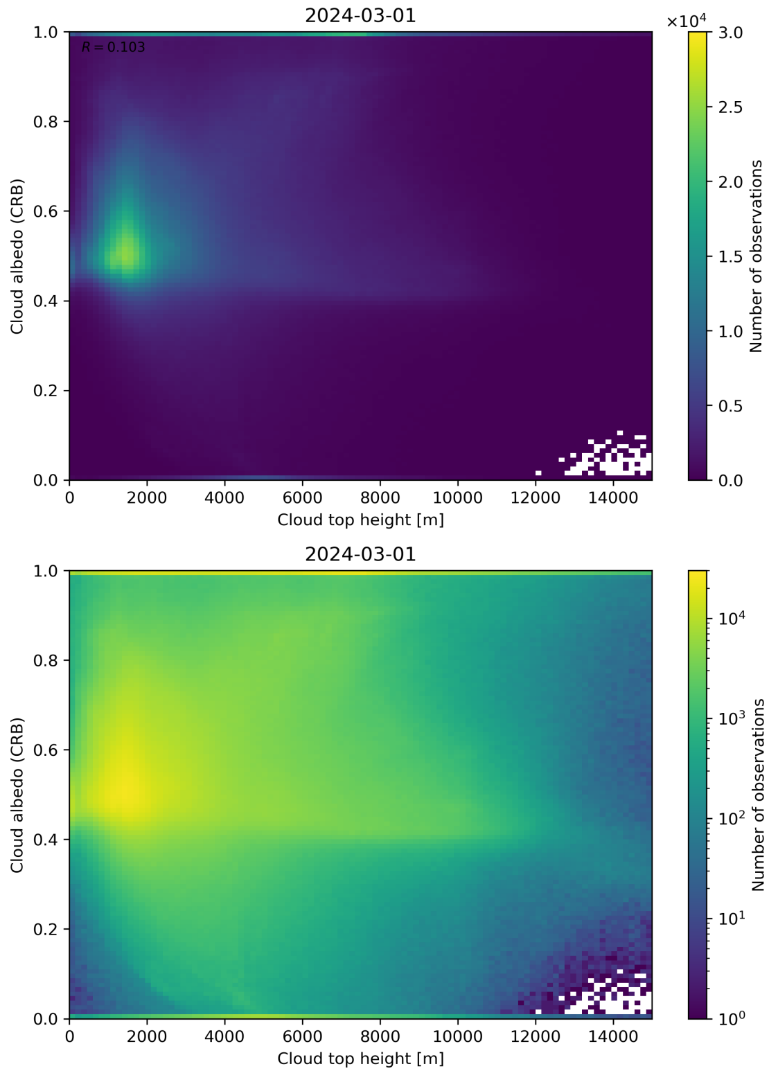
Figure 86: Scatter density plot of “Cloud top height” against “Cloud albedo (CRB)” for 2024-02-29 to 2024-03-02.
