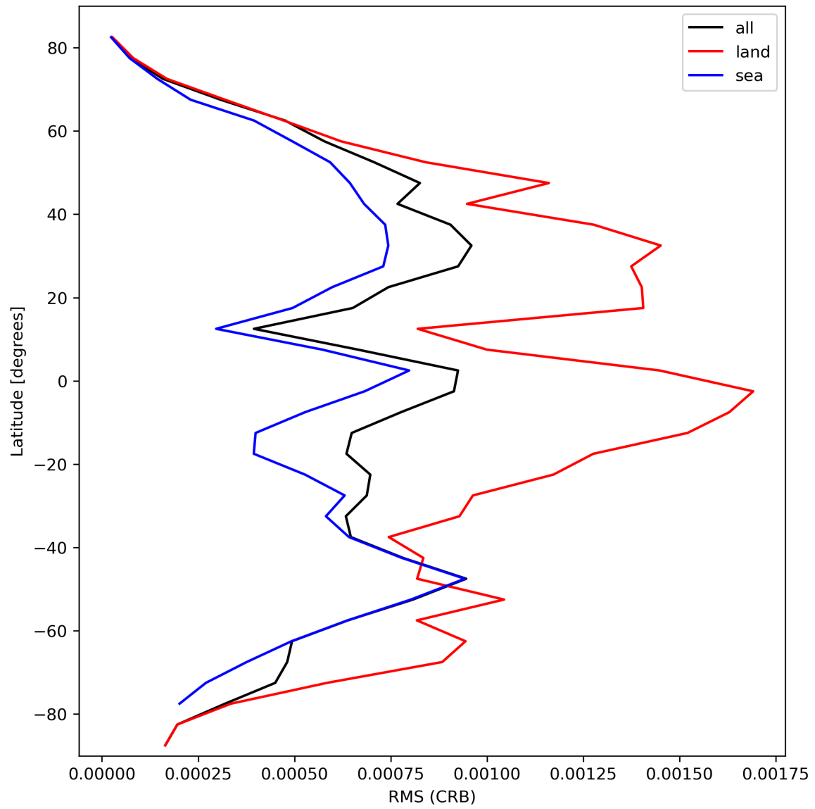
Figure 32: Zonal average of “RMS (CRB)” for 2024-02-29 to 2024-03-02.
