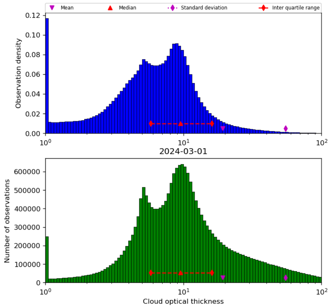
Figure 41: Histogram of “Cloud optical thickness” for 2024-02-29 to 2024-03-02
