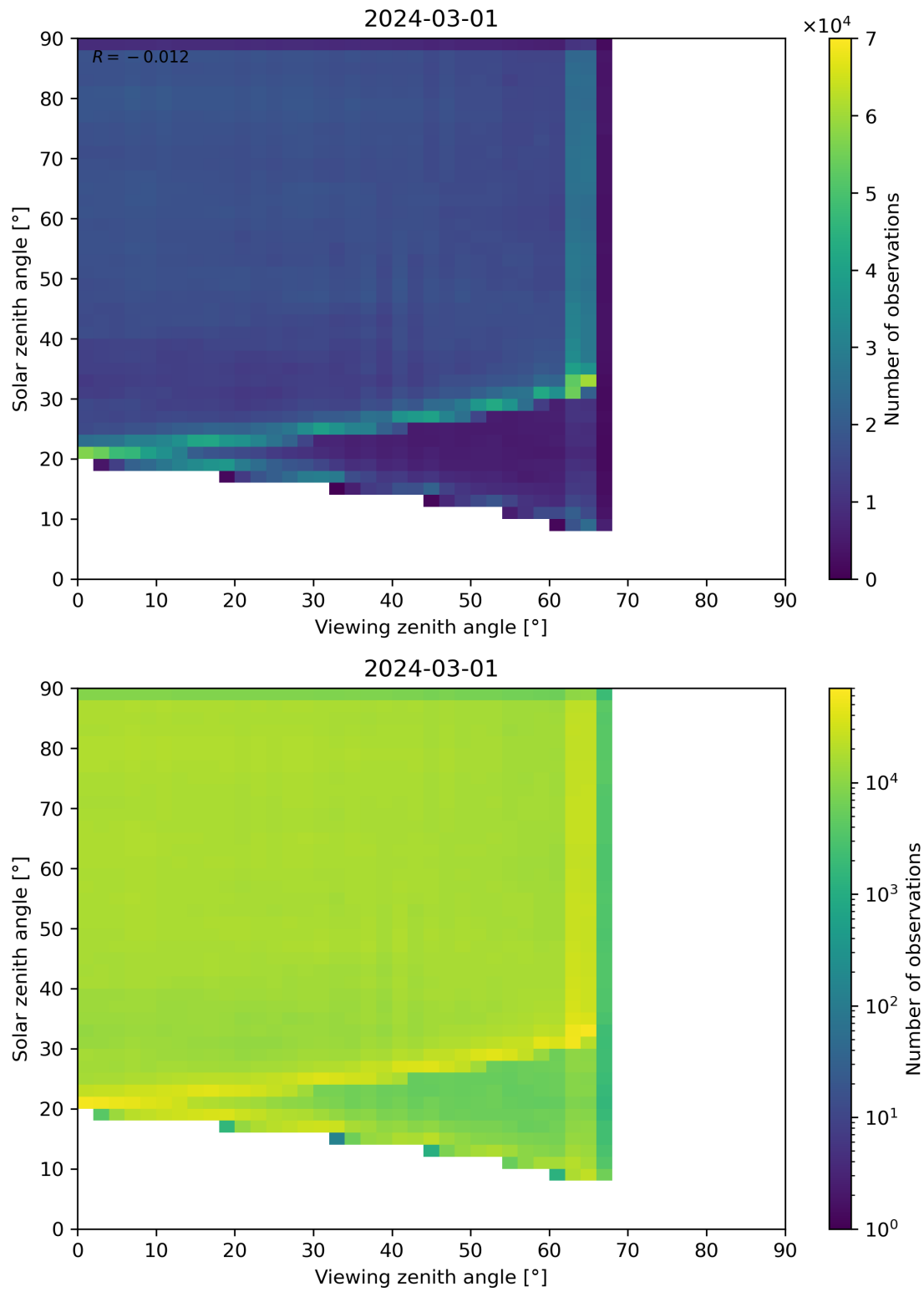
Figure 114: Scatter density plot of “Viewing zenith angle” against “Solar zenith angle” for 2024-02-29 to 2024-03-02.
