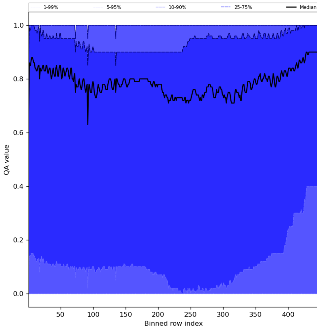
Figure 54: Along track statistics of “QA value” for 2024-02-29 to 2024-03-02
