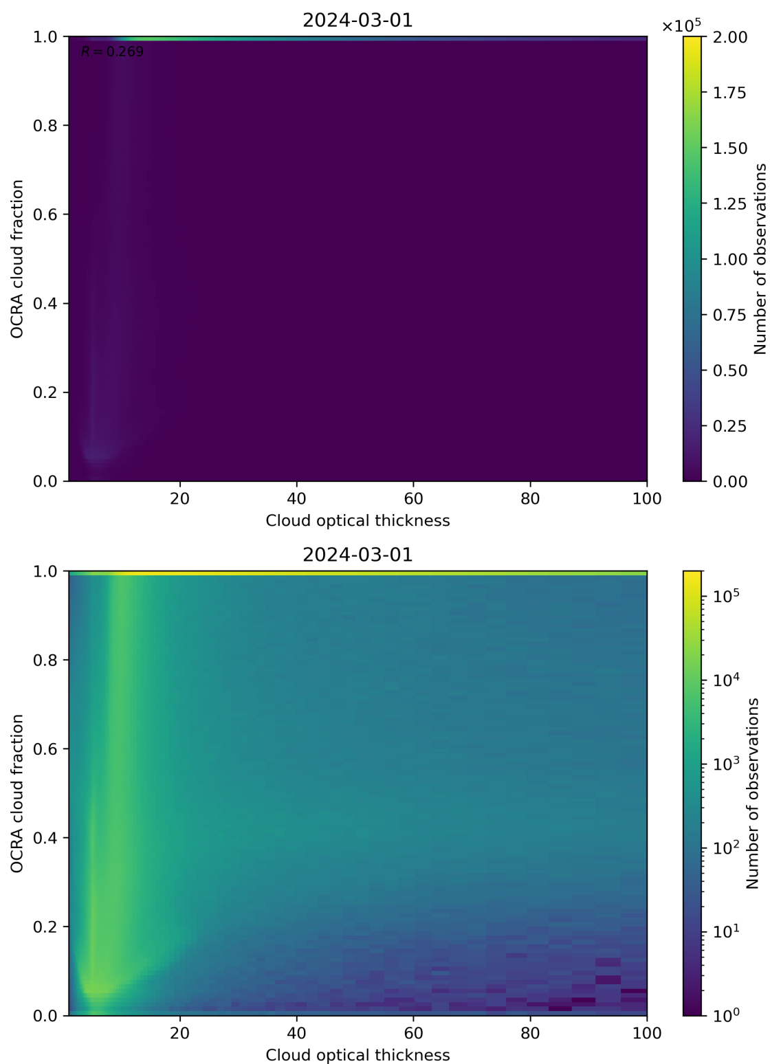
Figure 83: Scatter density plot of “Cloud optical thickness” against “OCRA cloud fraction” for 2024-02-29 to 2024-03-02.
