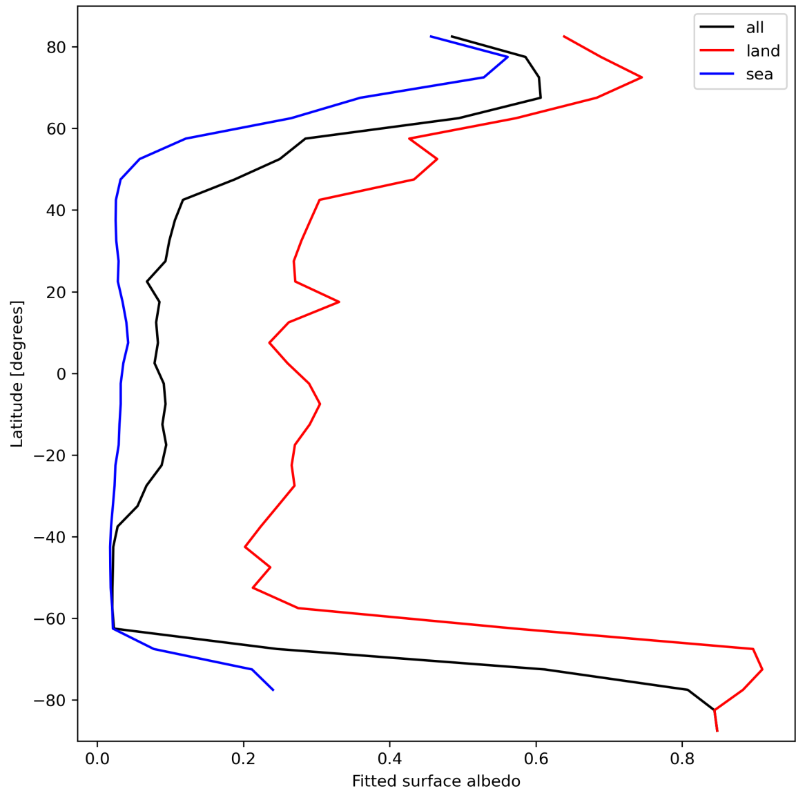
Figure 29: Zonal average of “Fitted surface albedo” for 2024-02-29 to 2024-03-02.
