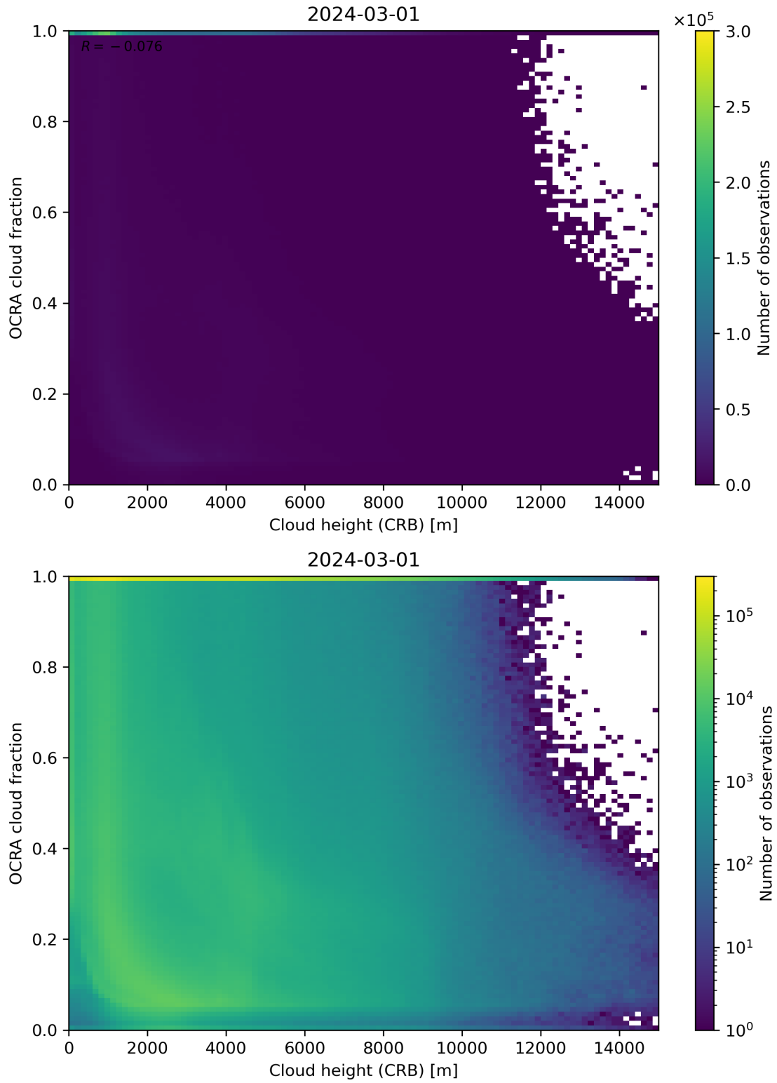
Figure 81: Scatter density plot of “Cloud height (CRB)” against “OCRA cloud fraction” for 2024-02-29 to 2024-03-02.
