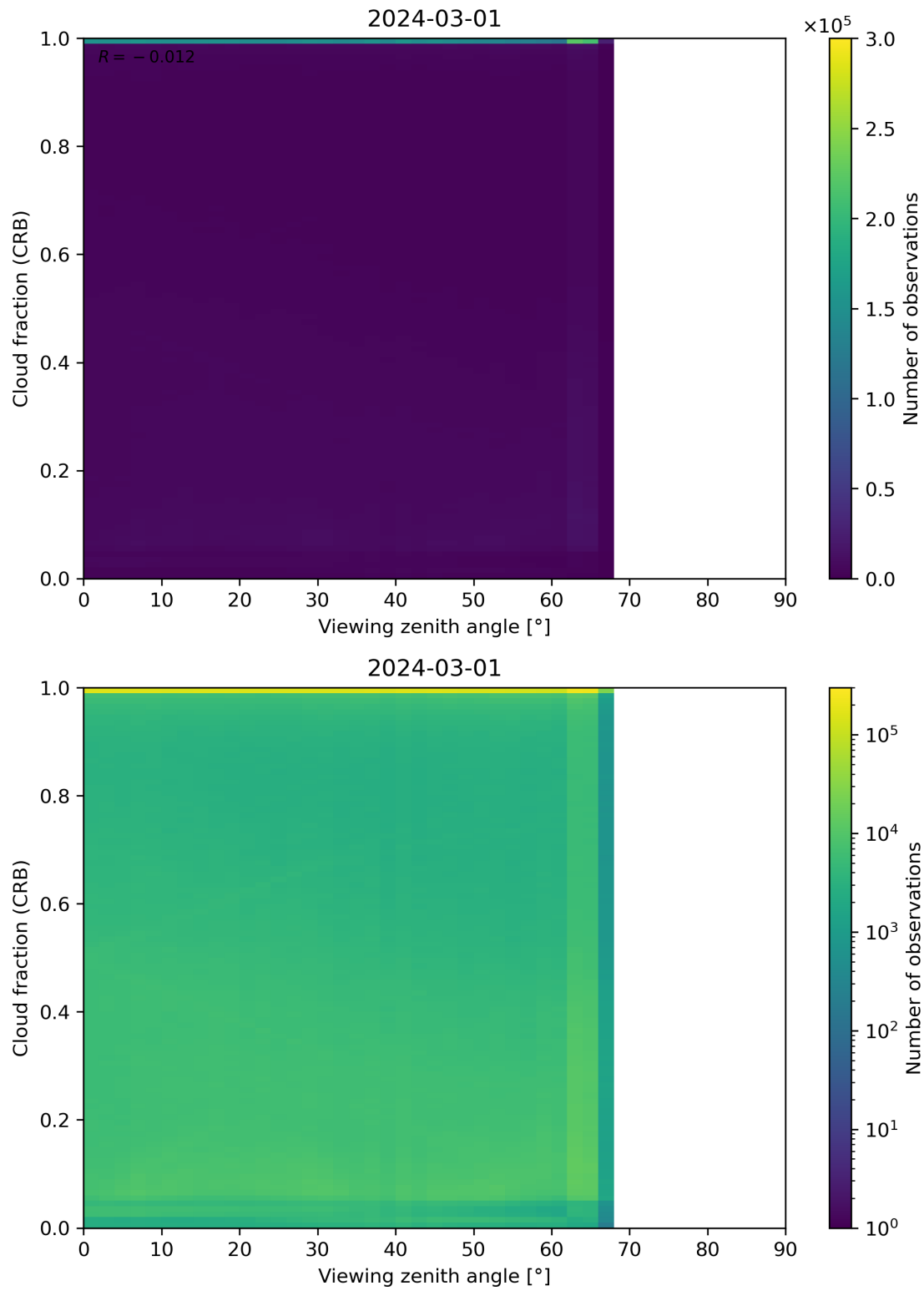
Figure 109: Scatter density plot of “Viewing zenith angle” against “Cloud fraction (CRB)” for 2024-02-29 to 2024-03-02.
