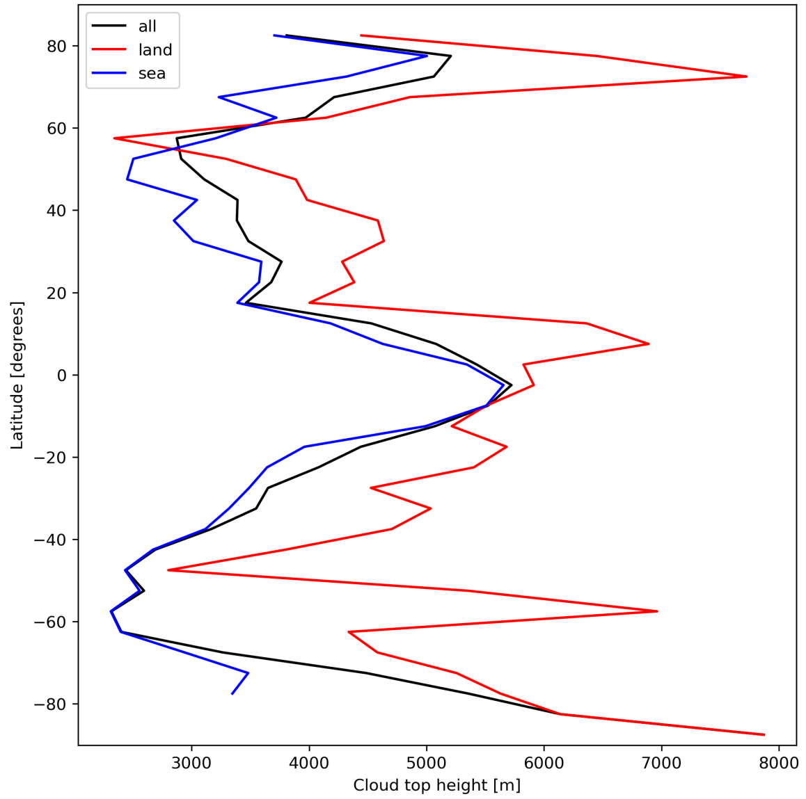
Figure 24: Zonal average of “Cloud top height” for 2024-02-29 to 2024-03-02.
