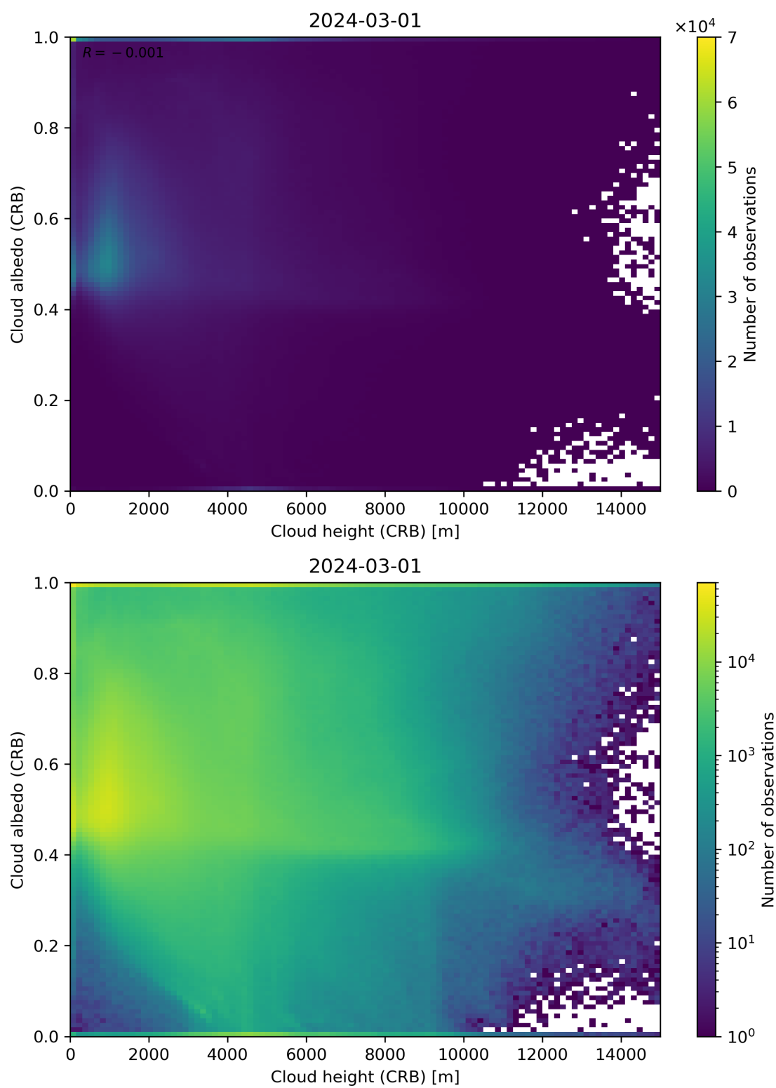
Figure 80: Scatter density plot of “Cloud height (CRB)” against “Cloud albedo (CRB)” for 2024-02-29 to 2024-03-02.
