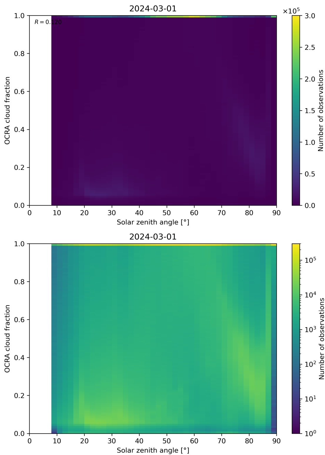
Figure 100: Scatter density plot of “Solar zenith angle” against “OCRA cloud fraction” for 2024-02-29 to 2024-03-02.
