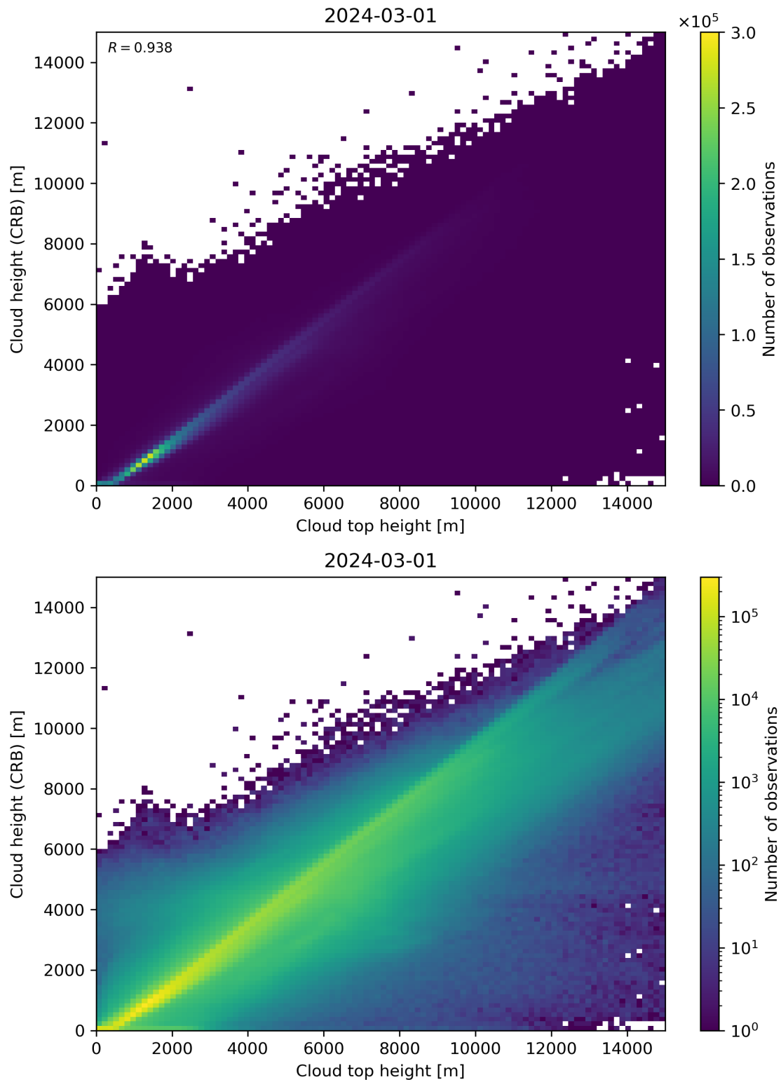
Figure 89: Scatter density plot of “Cloud top height” against “Cloud height (CRB)” for 2024-02-29 to 2024-03-02.
