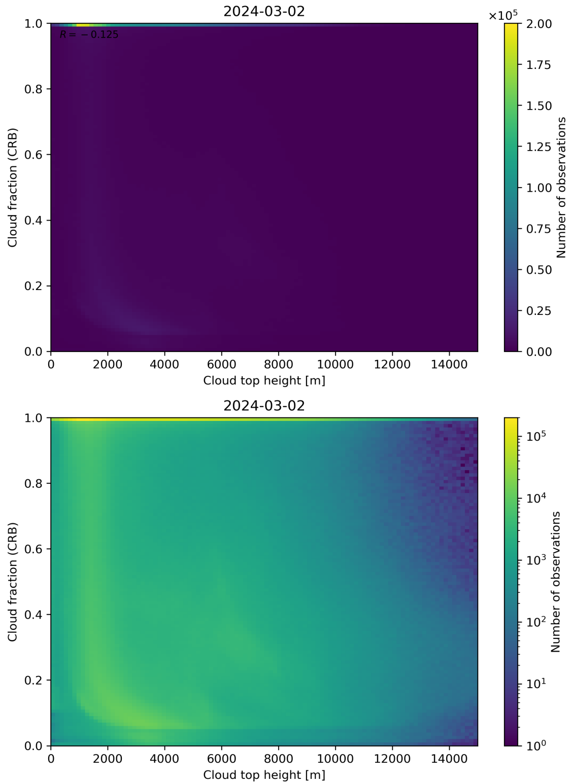
Figure 88: Scatter density plot of “Cloud top height” against “Cloud fraction (CRB)” for 2024-03-01 to 2024-03-03.
