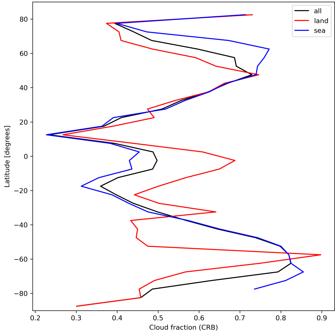
Figure 26: Zonal average of “Cloud fraction (CRB)” for 2024-03-01 to 2024-03-03.
