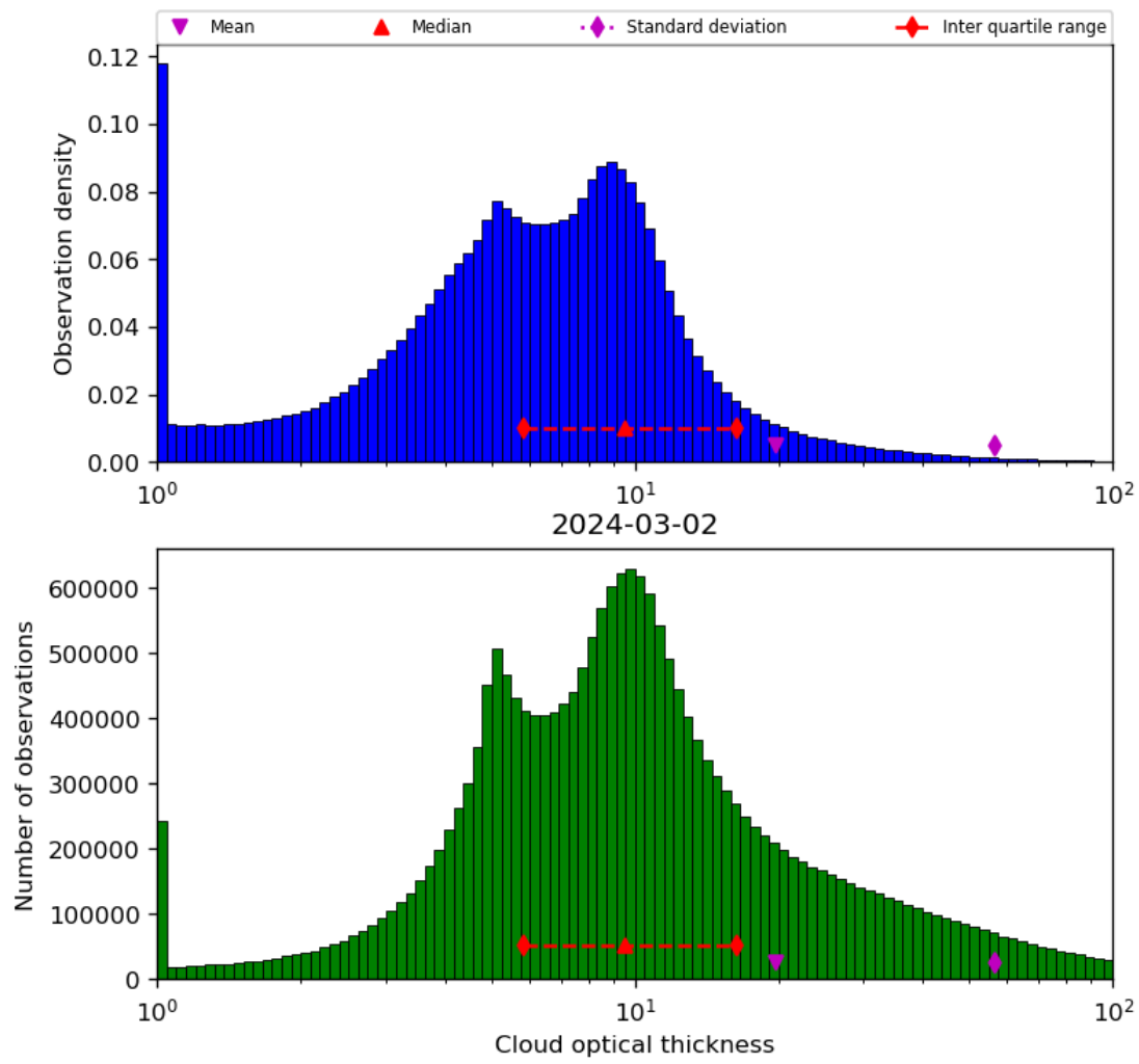
Figure 41: Histogram of “Cloud optical thickness” for 2024-03-01 to 2024-03-03
