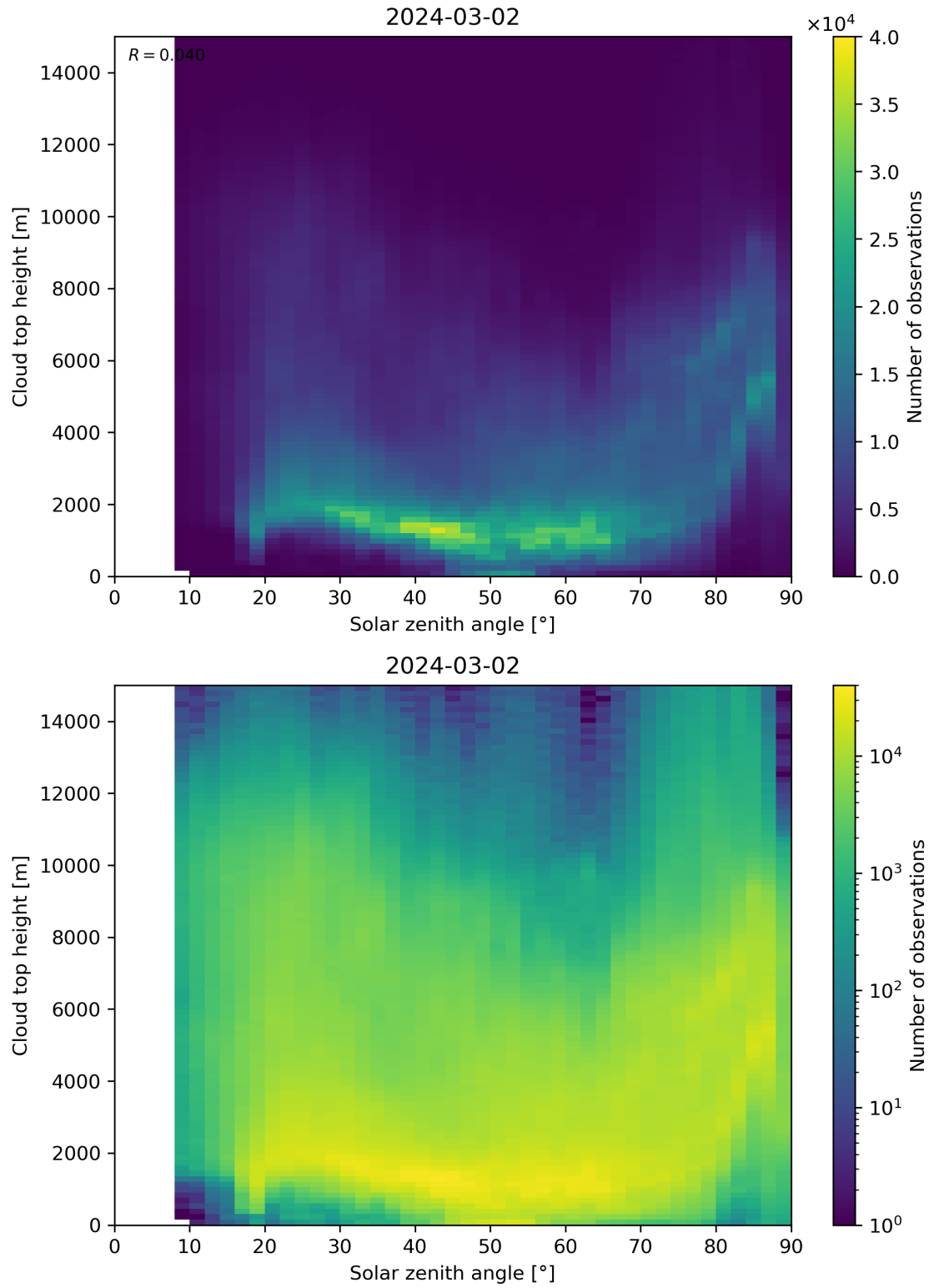
Figure 104: Scatter density plot of “Solar zenith angle” against “Cloud top height” for 2024-03-01 to 2024-03-03.
