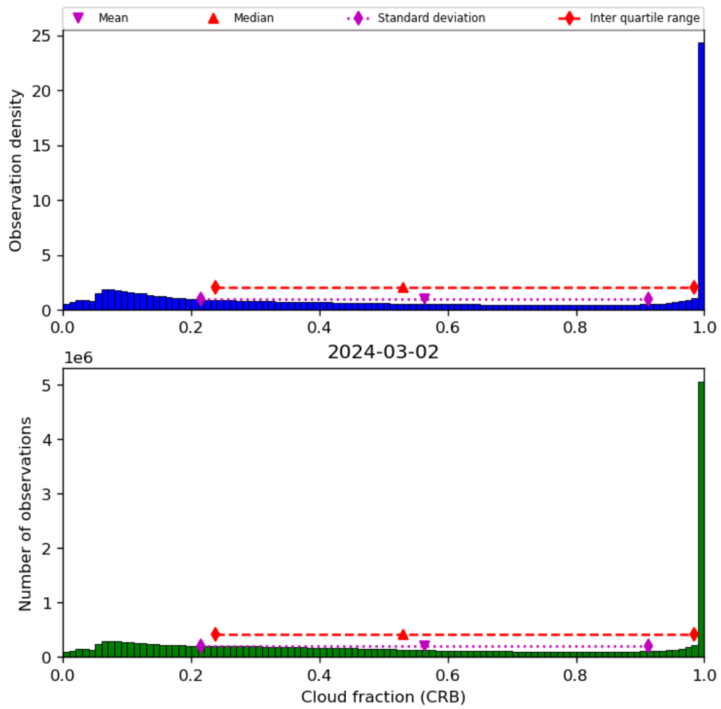
Figure 42: Histogram of “Cloud fraction (CRB)” for 2024-03-01 to 2024-03-03
