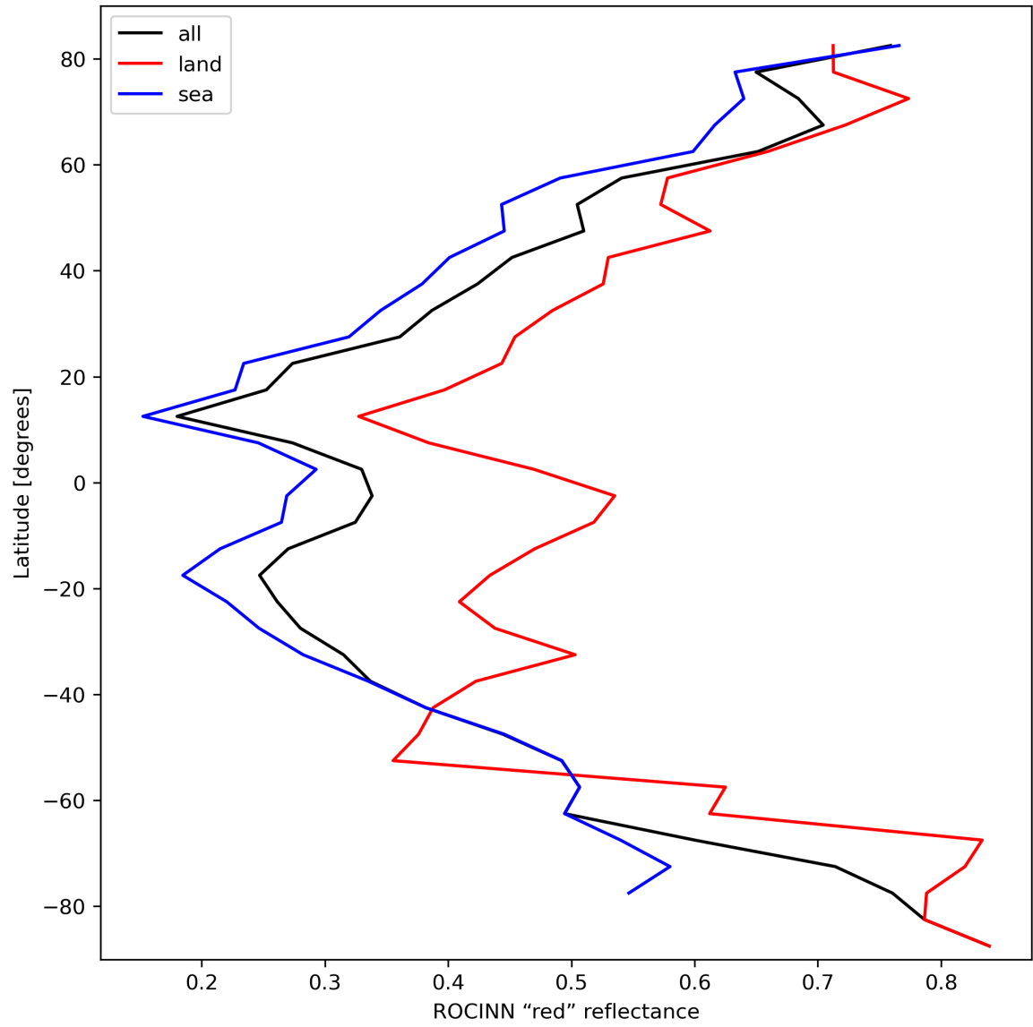
Figure 37: Zonal average of “ROCINN “red” reflectance” for 2024-03-01 to 2024-03-03.
