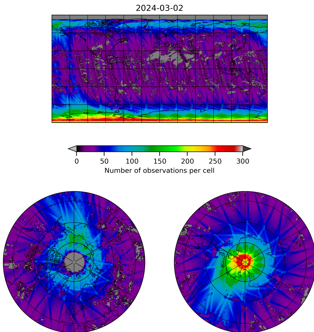
Figure 21: Map of the number of observations for 2024-03-01 to 2024-03-03
