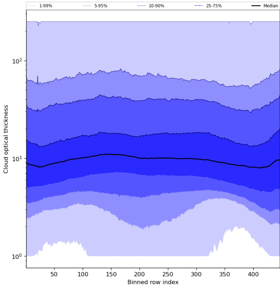
Figure 57: Along track statistics of “Cloud optical thickness” for 2024-03-01 to 2024-03-03
