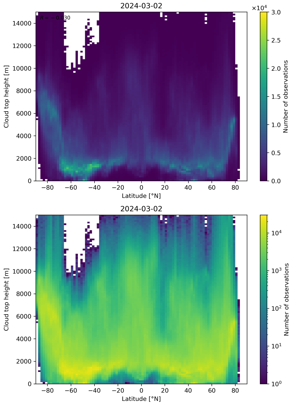
Figure 97: Scatter density plot of “Latitude” against “Cloud top height” for 2024-03-01 to 2024-03-03.
