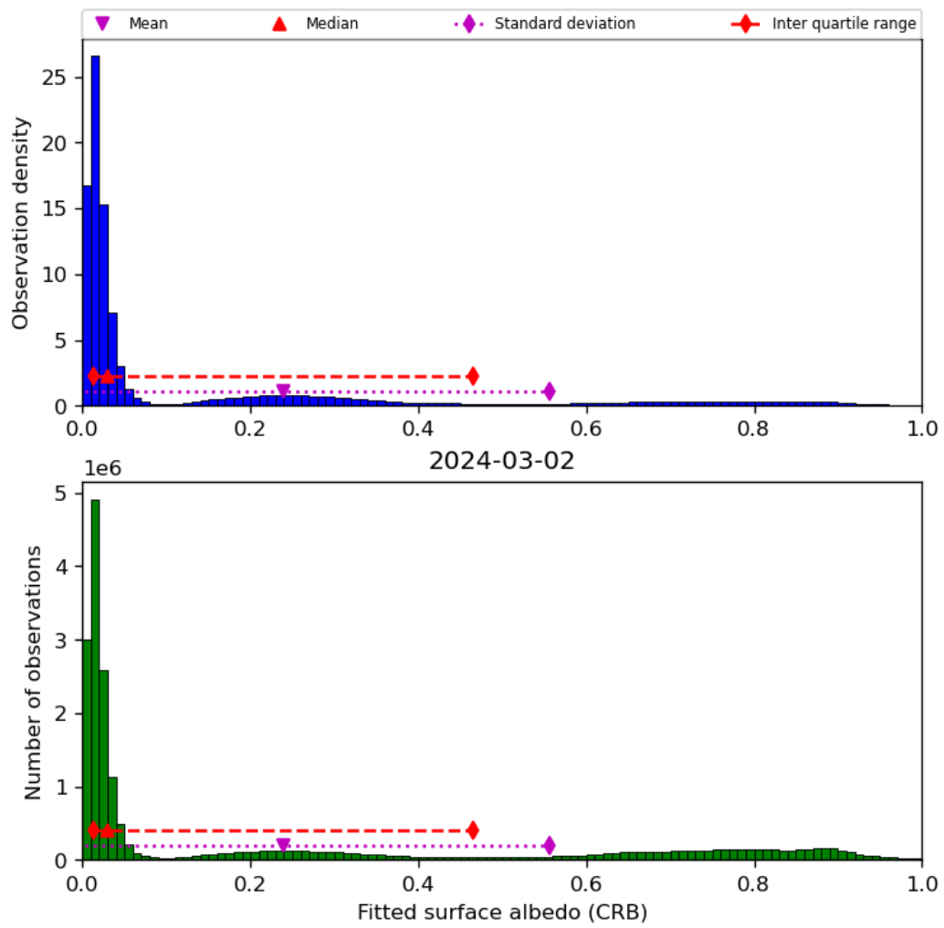
Figure 46: Histogram of “Fitted surface albedo (CRB)” for 2024-03-01 to 2024-03-03
