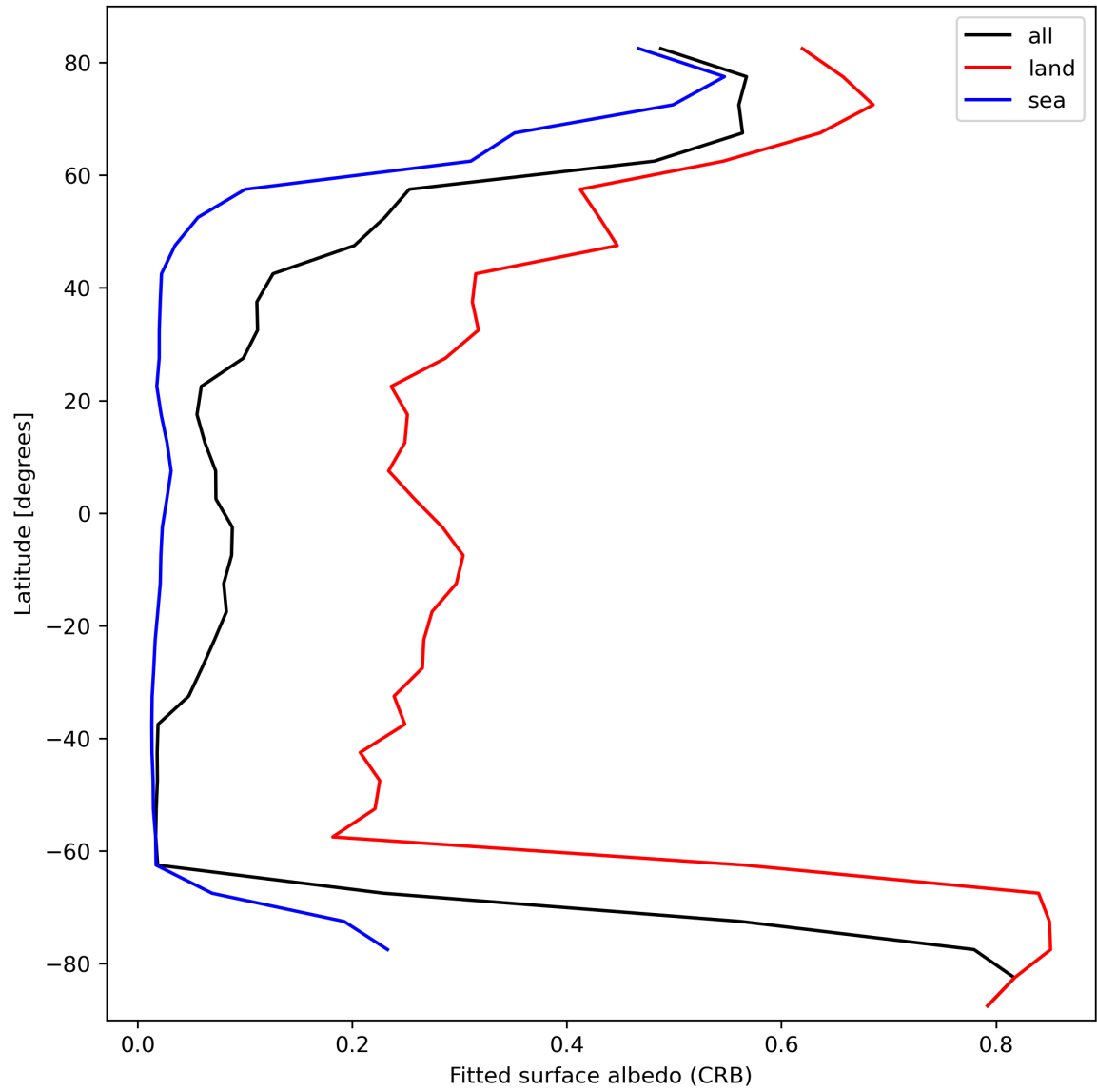
Figure 30: Zonal average of “Fitted surface albedo (CRB)” for 2024-03-01 to 2024-03-03.
