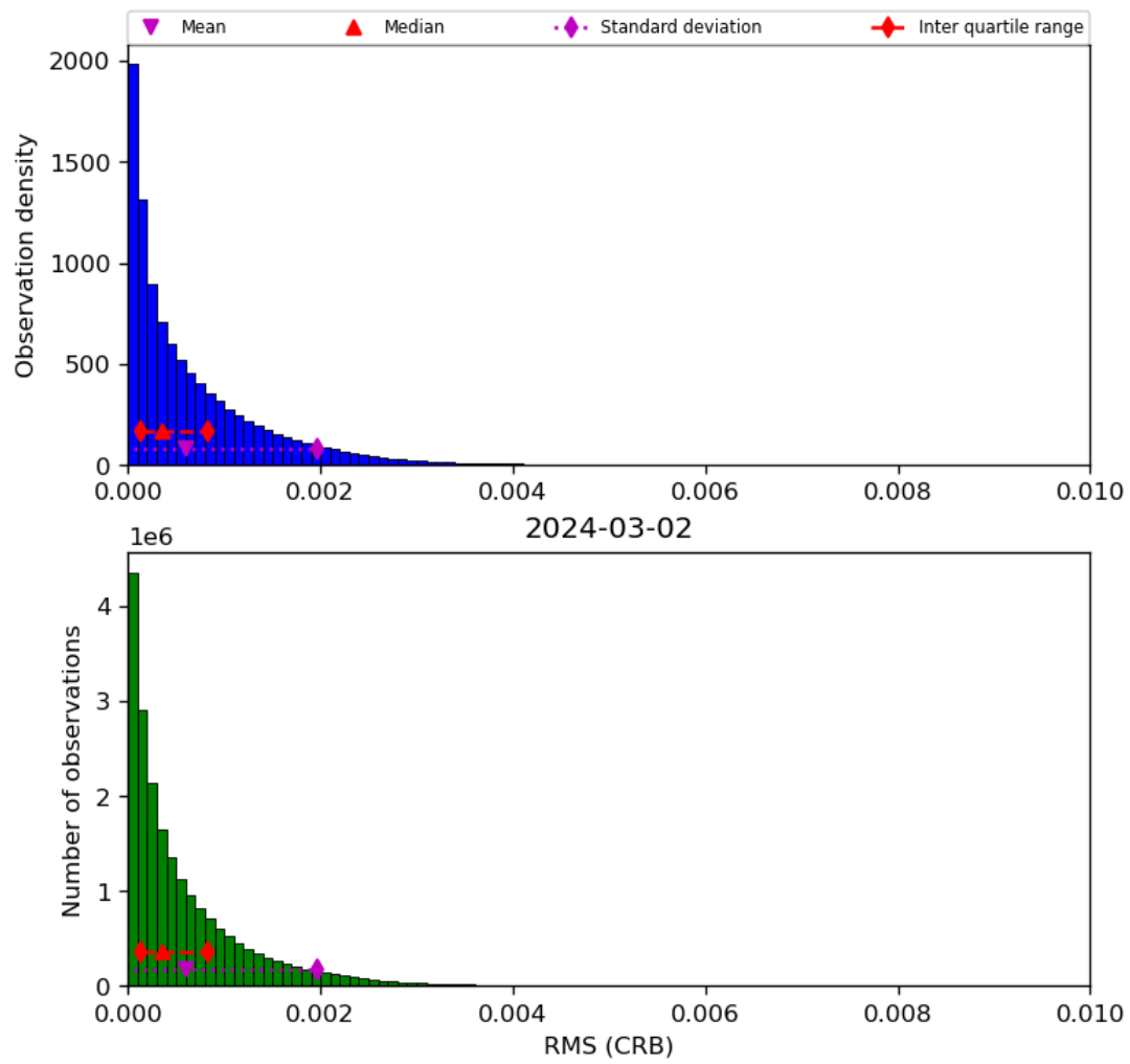
Figure 48: Histogram of “RMS (CRB)” for 2024-03-01 to 2024-03-03
