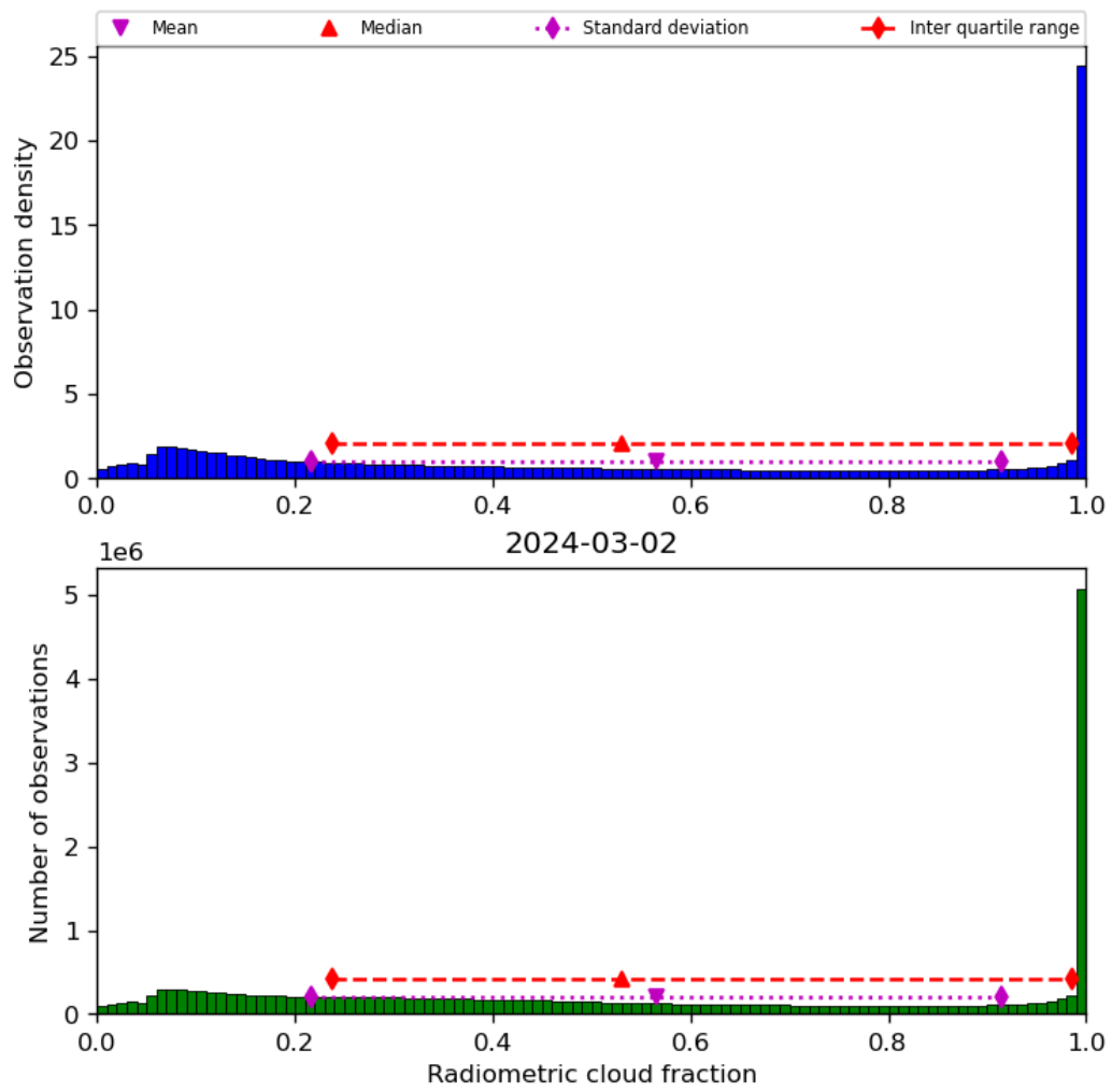
Figure 39: Histogram of “Radiometric cloud fraction” for 2024-03-01 to 2024-03-03
