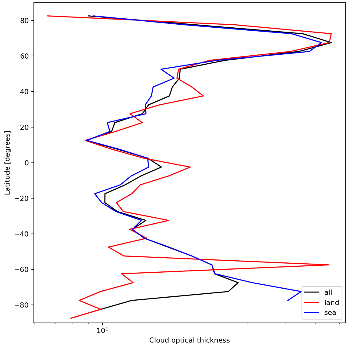
Figure 25: Zonal average of “Cloud optical thickness” for 2024-03-01 to 2024-03-03.
