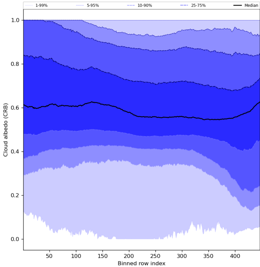
Figure 60: Along track statistics of “Cloud albedo (CRB)” for 2024-03-01 to 2024-03-03
