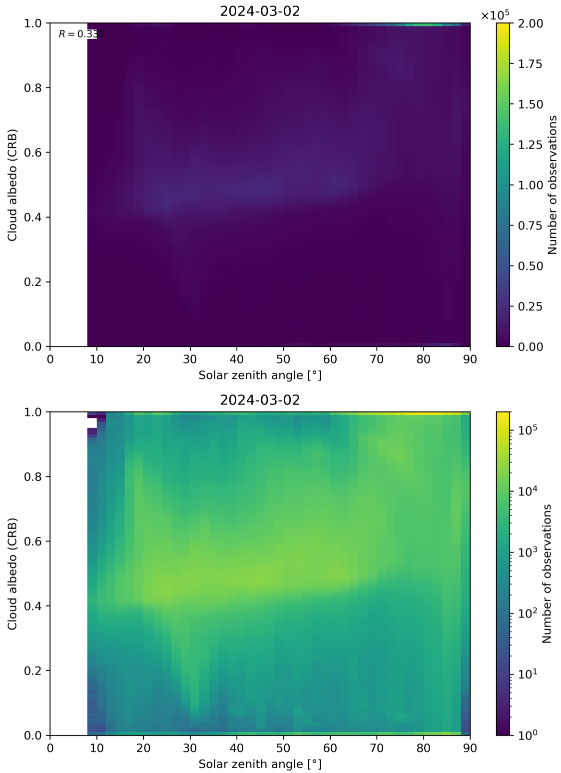
Figure 98: Scatter density plot of “Solar zenith angle” against “Cloud albedo (CRB)” for 2024-03-01 to 2024-03-03.
