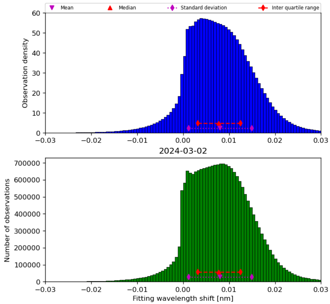
Figure 49: Histogram of “Fitting wavelength shift” for 2024-03-01 to 2024-03-03
