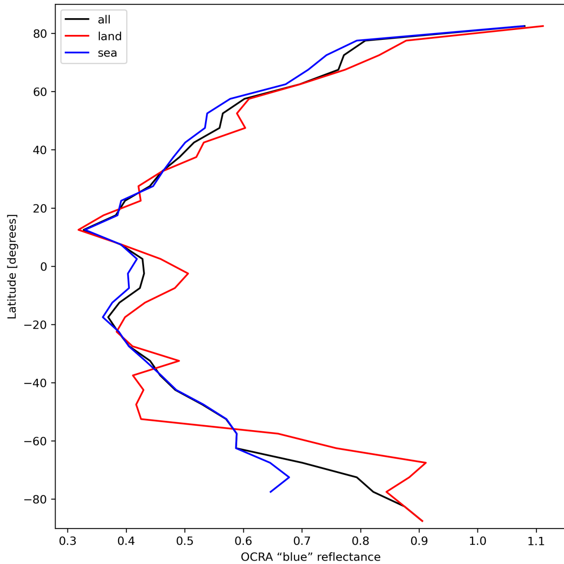
Figure 35: Zonal average of “OCRA “blue” reflectance” for 2024-03-01 to 2024-03-03.
