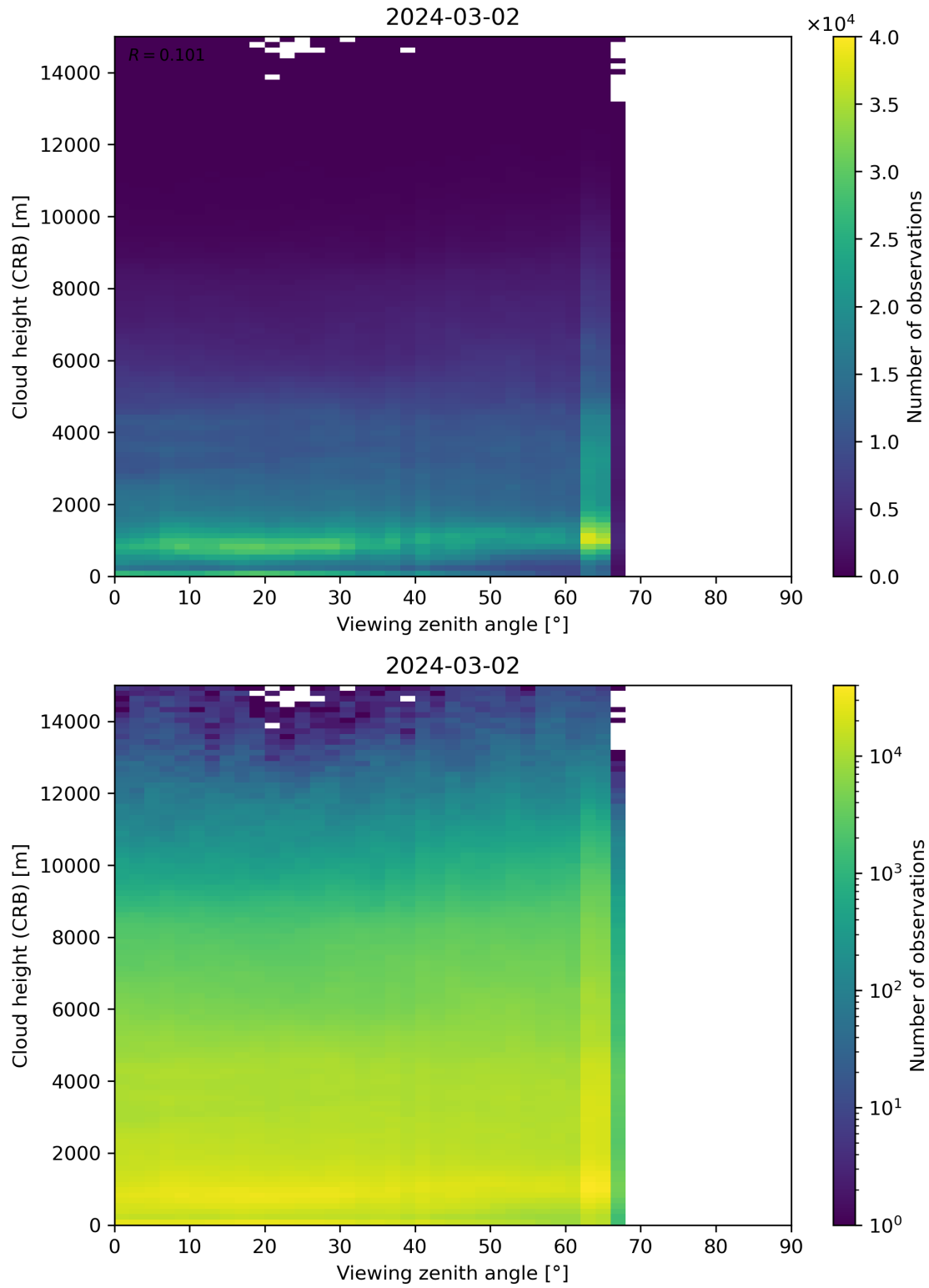
Figure 110: Scatter density plot of “Viewing zenith angle” against “Cloud height (CRB)” for 2024-03-01 to 2024-03-03.
