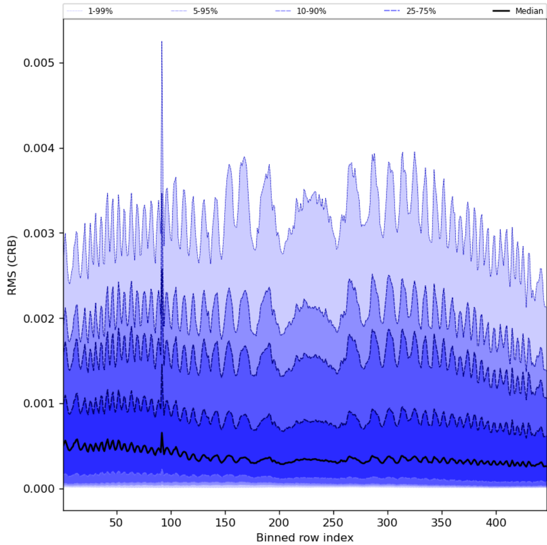
Figure 64: Along track statistics of “RMS (CRB)” for 2024-03-01 to 2024-03-03
