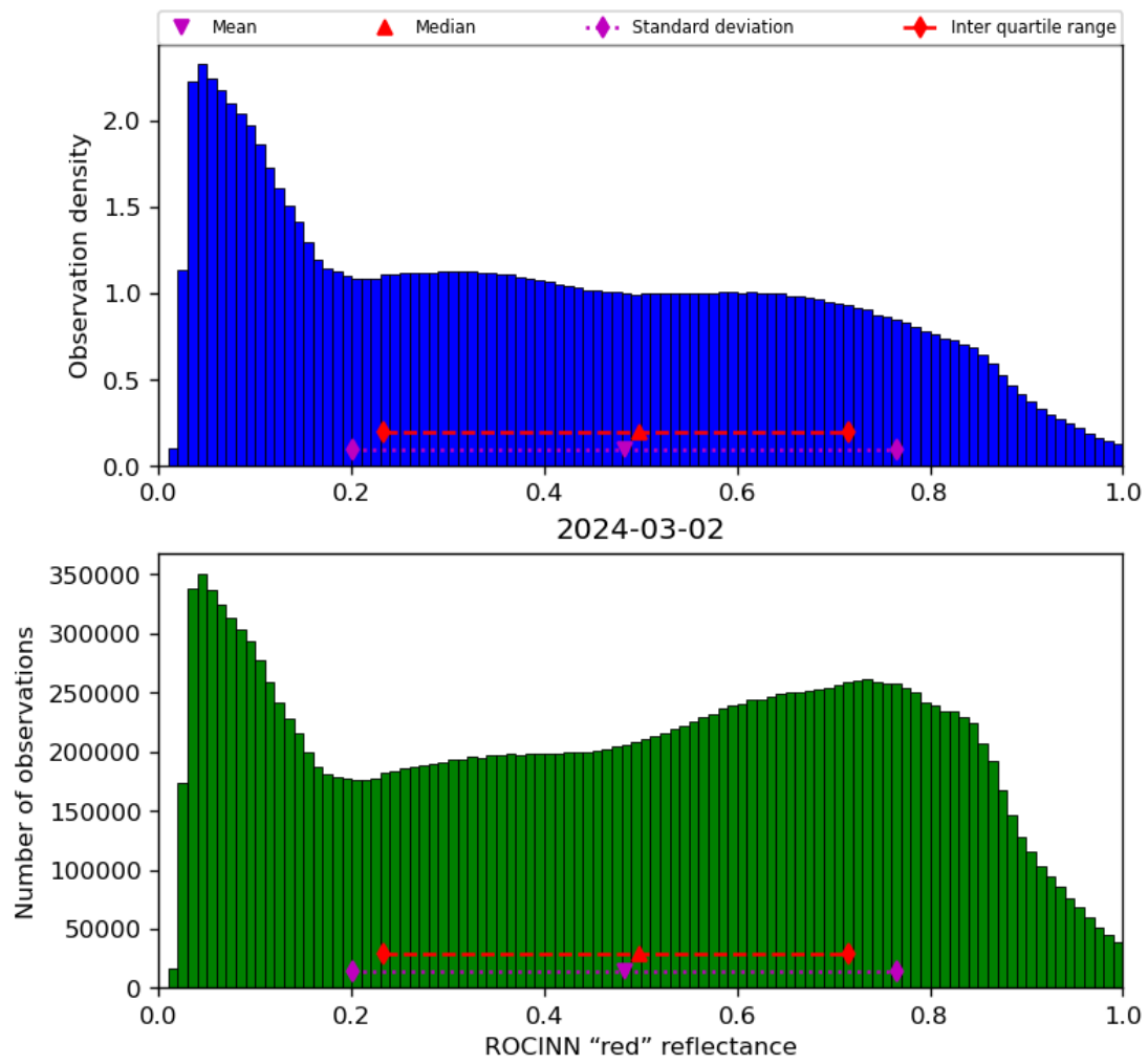
Figure 53: Histogram of “ROCINN “red” reflectance” for 2024-03-01 to 2024-03-03
