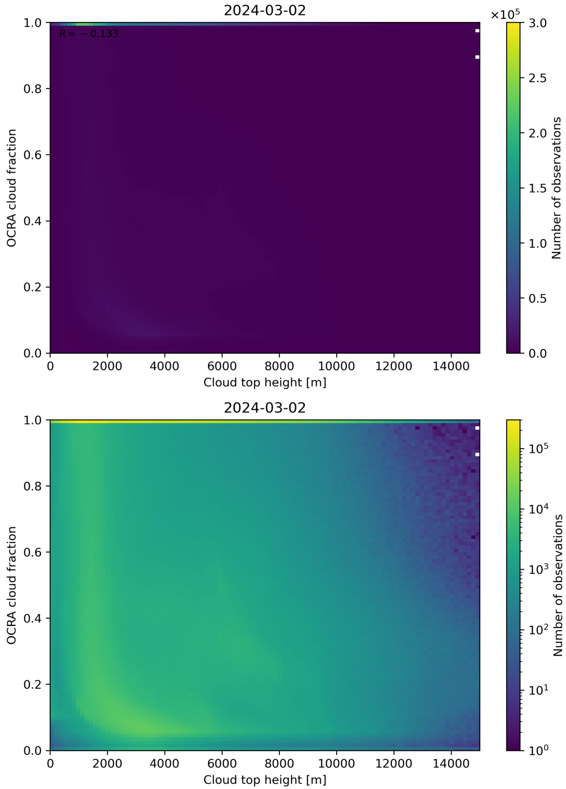
Figure 87: Scatter density plot of “Cloud top height” against “OCRA cloud fraction” for 2024-03-01 to 2024-03-03.
