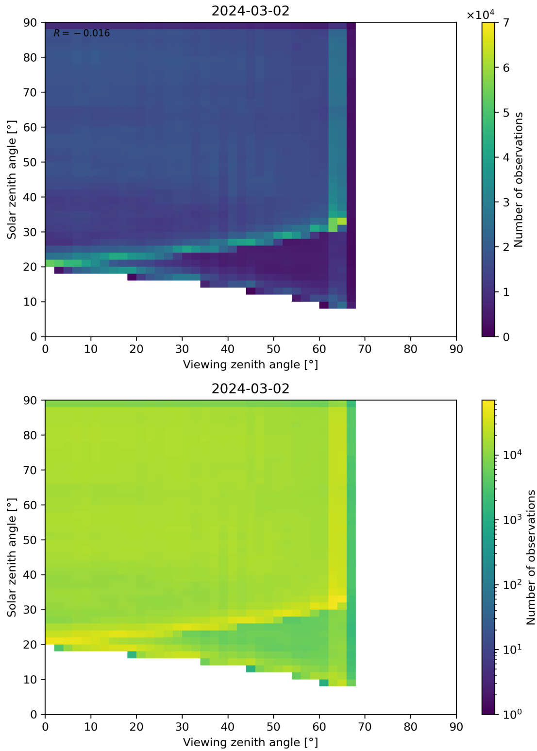
Figure 114: Scatter density plot of “Viewing zenith angle” against “Solar zenith angle” for 2024-03-01 to 2024-03-03.
