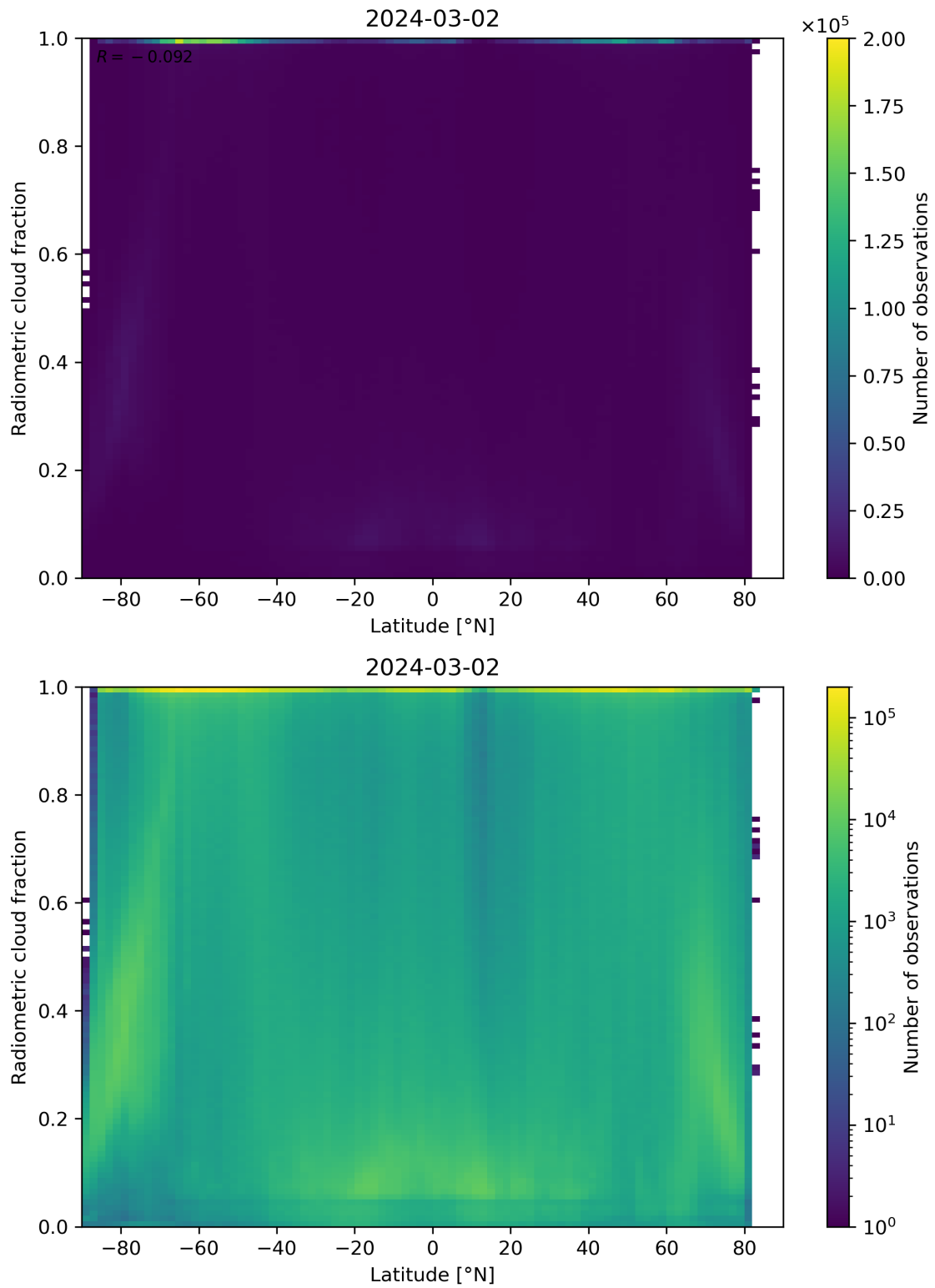
Figure 92: Scatter density plot of “Latitude” against “Radiometric cloud fraction” for 2024-03-01 to 2024-03-03.
