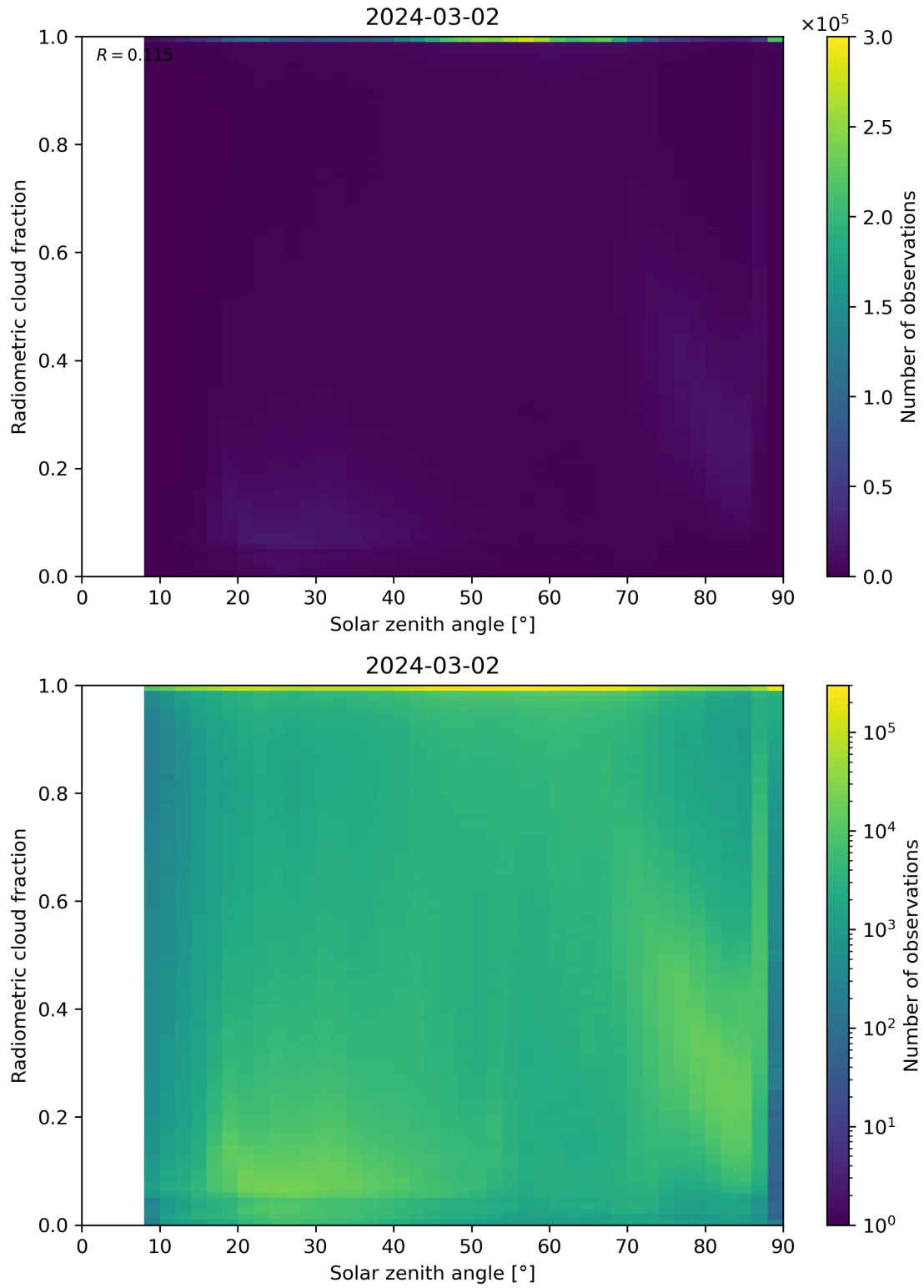
Figure 99: Scatter density plot of “Solar zenith angle” against “Radiometric cloud fraction” for 2024-03-01 to 2024-03-03.
