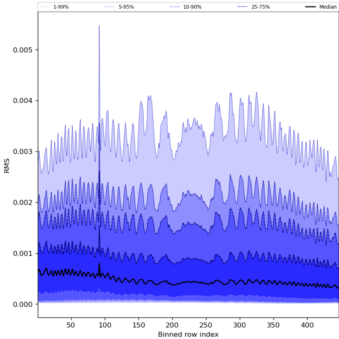
Figure 63: Along track statistics of “RMS” for 2024-03-01 to 2024-03-03
