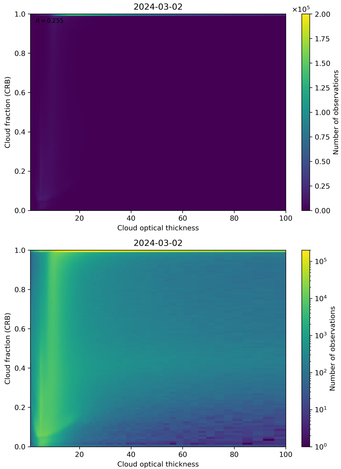
Figure 84: Scatter density plot of “Cloud optical thickness” against “Cloud fraction (CRB)” for 2024-03-01 to 2024-03-03.
