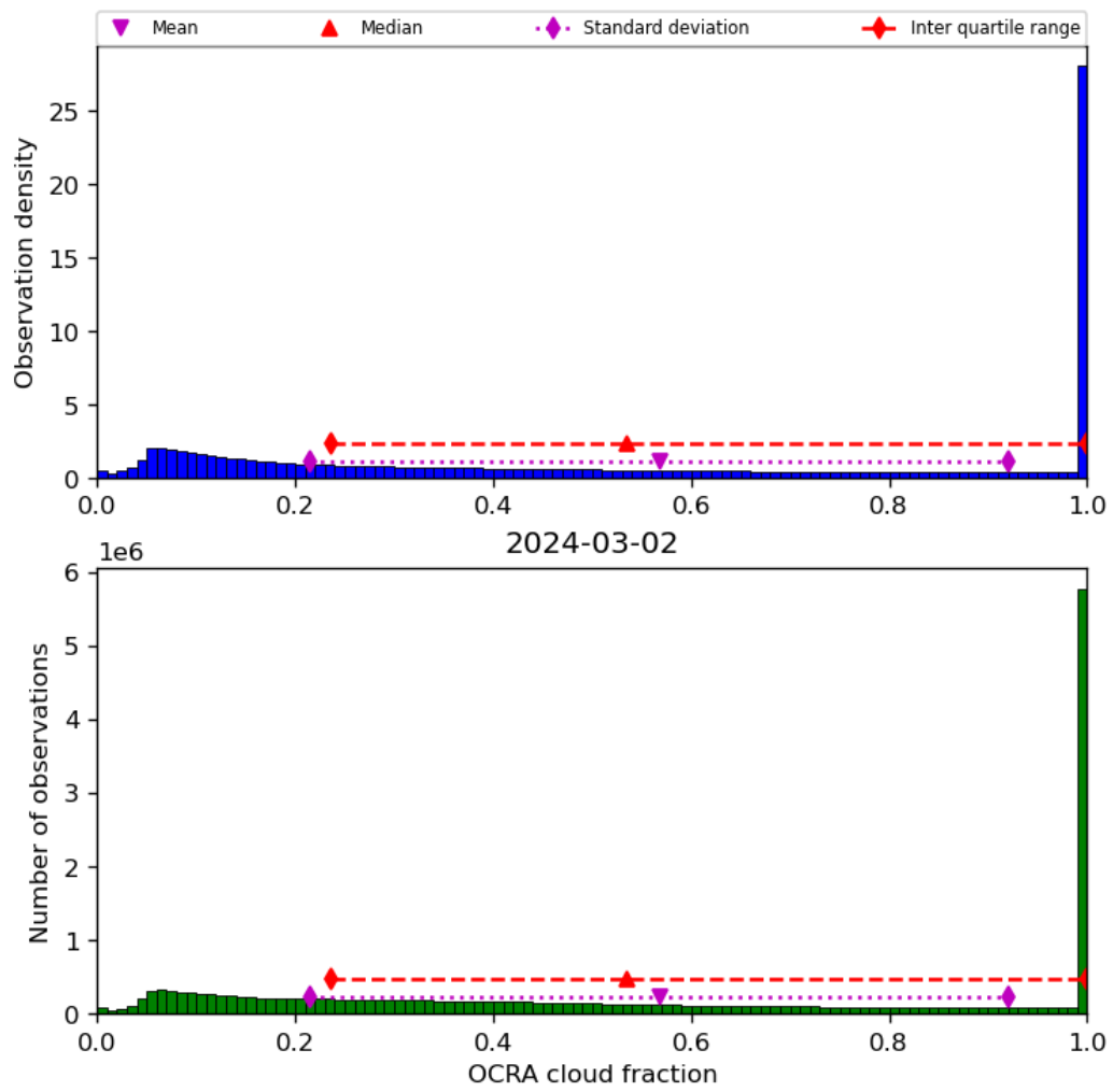
Figure 50: Histogram of “OCRA cloud fraction” for 2024-03-01 to 2024-03-03
