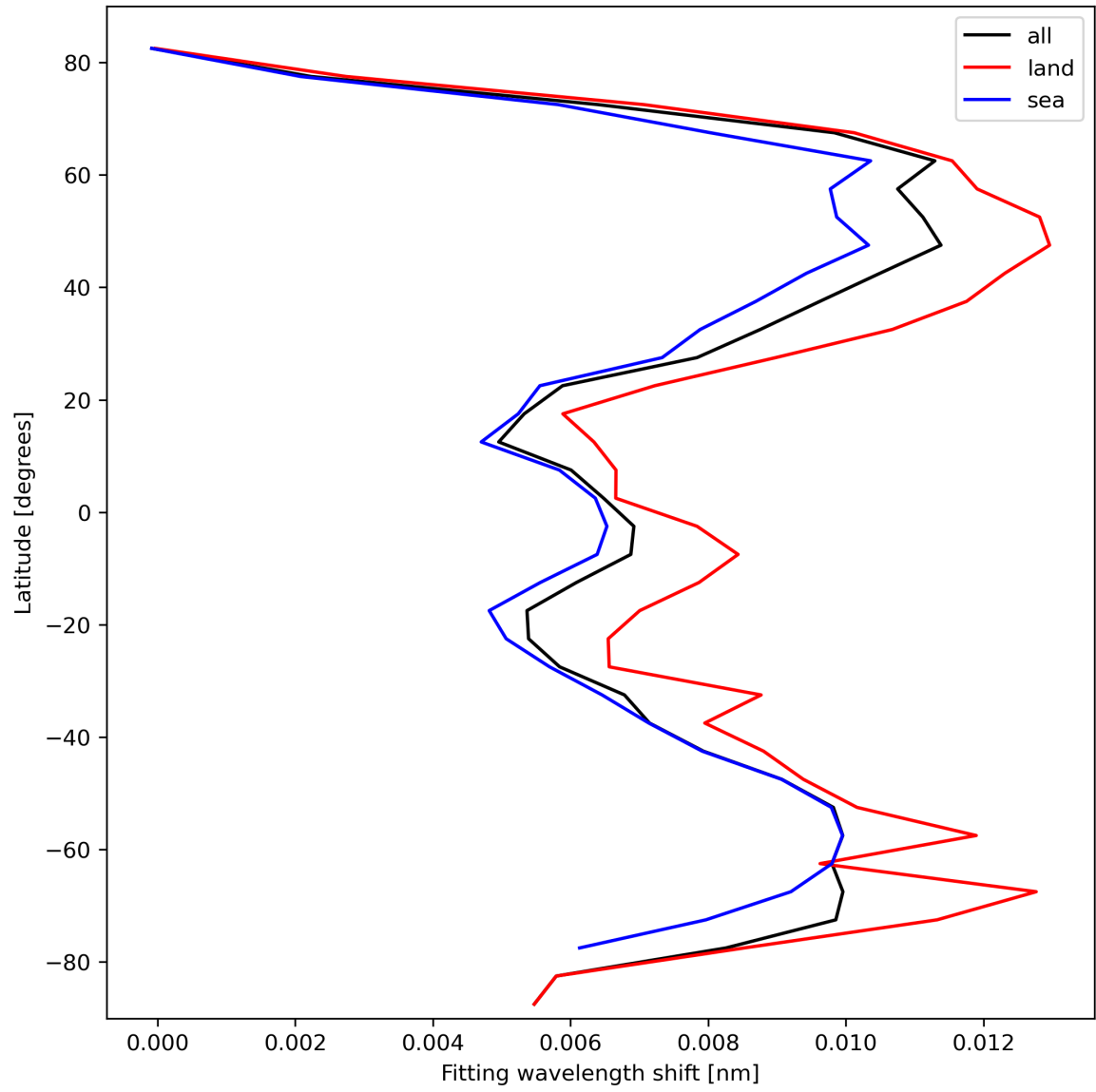
Figure 33: Zonal average of “Fitting wavelength shift” for 2024-03-01 to 2024-03-03.
