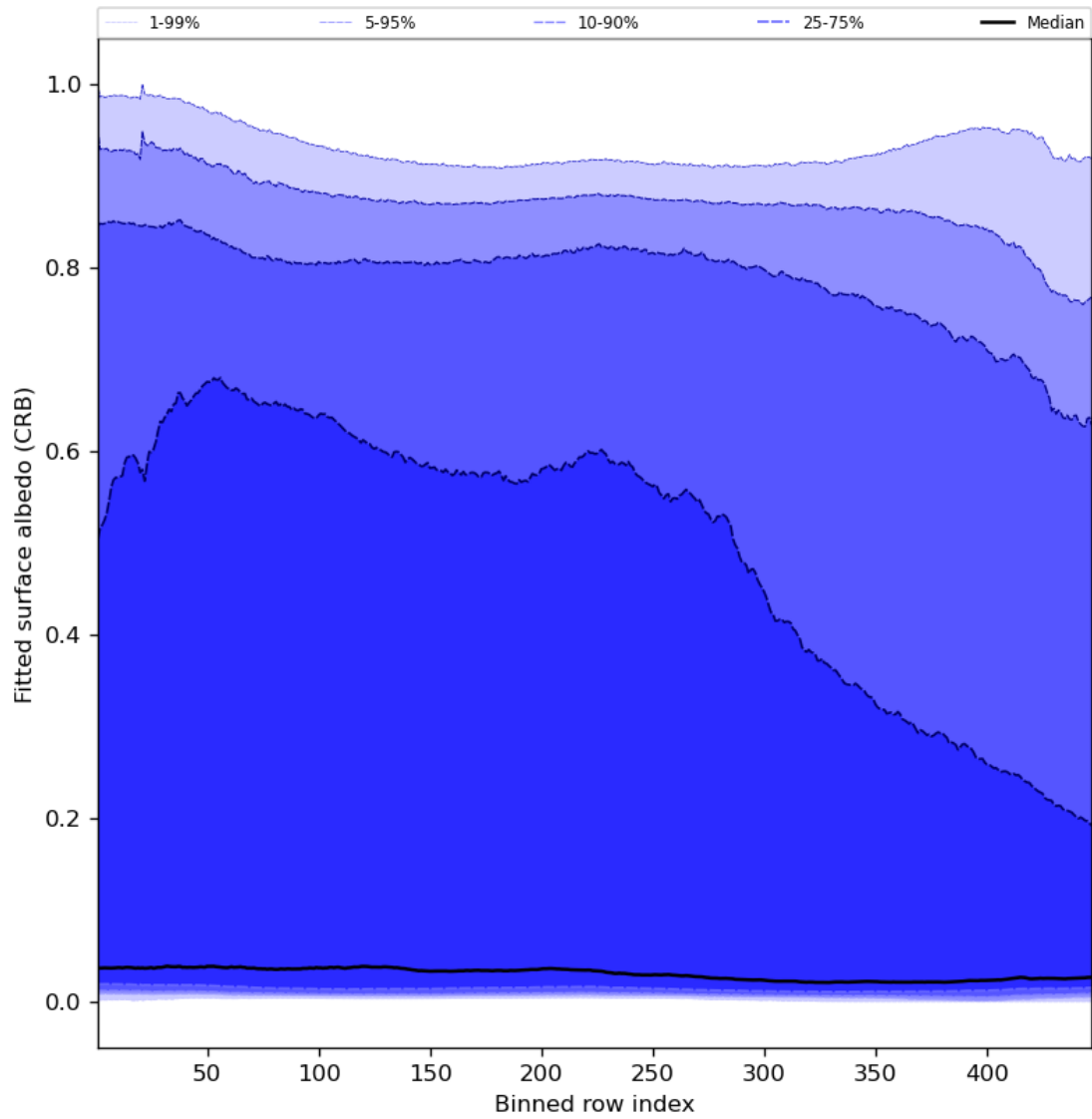
Figure 62: Along track statistics of “Fitted surface albedo (CRB)” for 2024-03-01 to 2024-03-03
