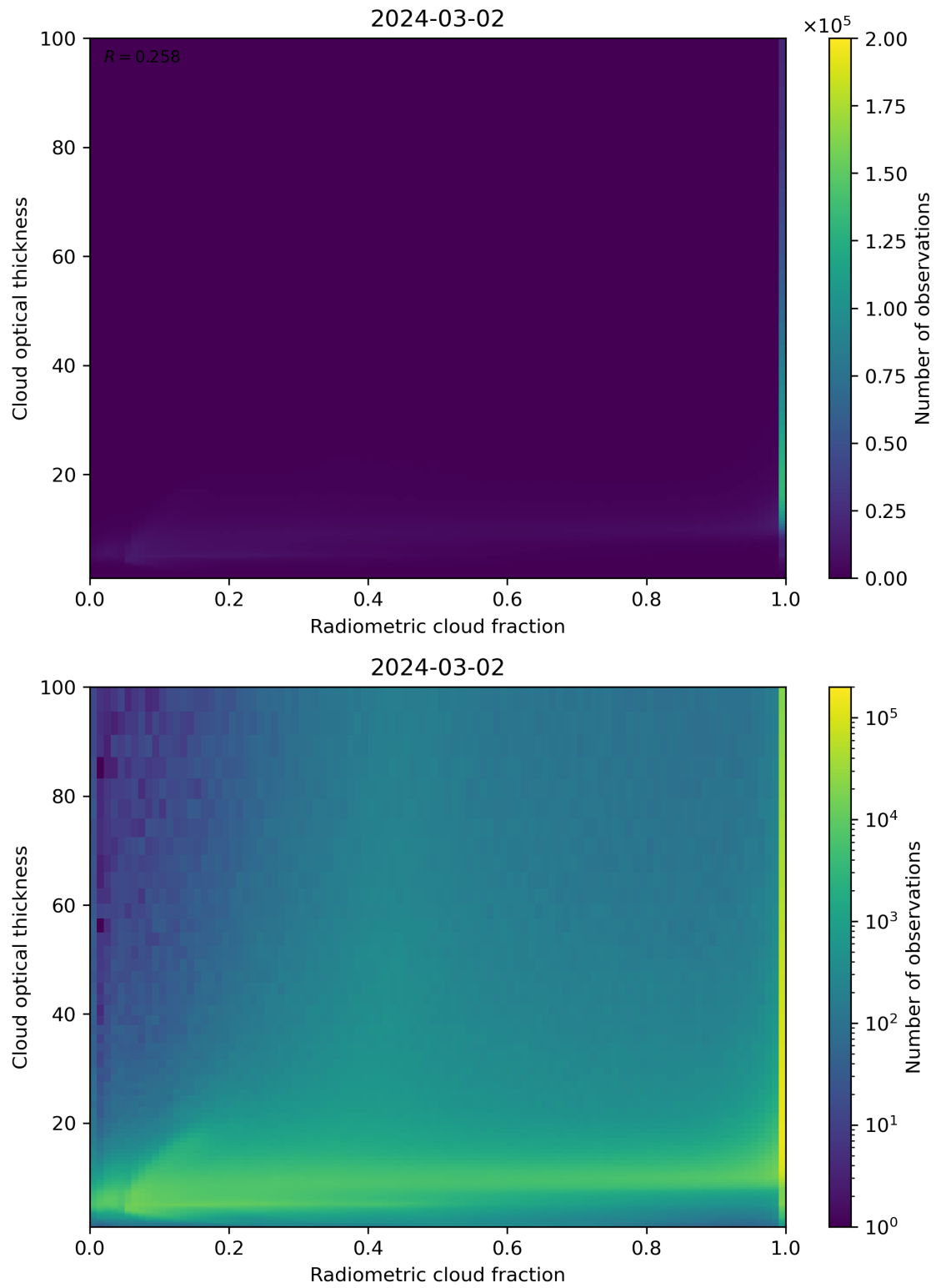
Figure 75: Scatter density plot of “Radiometric cloud fraction” against “Cloud optical thickness” for 2024-03-01 to 2024-03-03.
