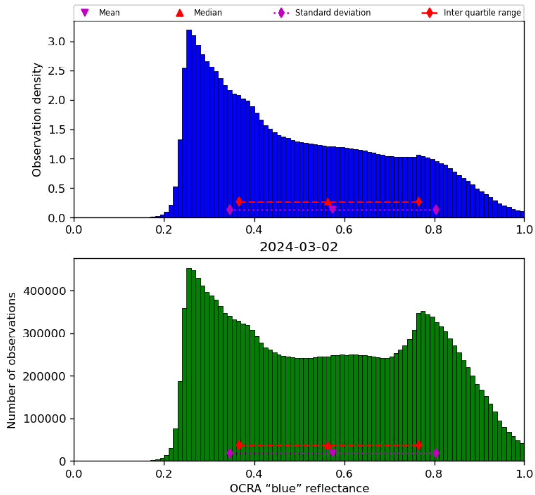
Figure 51: Histogram of “OCRA “blue” reflectance” for 2024-03-01 to 2024-03-03
