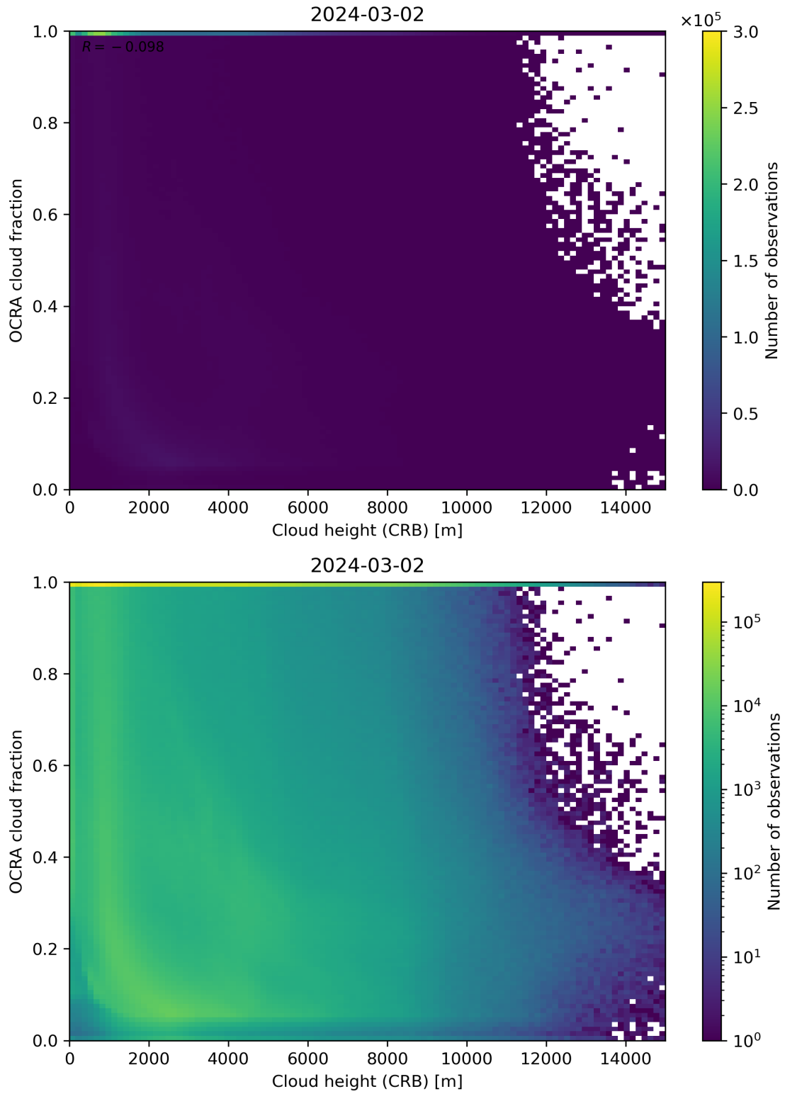
Figure 81: Scatter density plot of “Cloud height (CRB)” against “OCRA cloud fraction” for 2024-03-01 to 2024-03-03.
