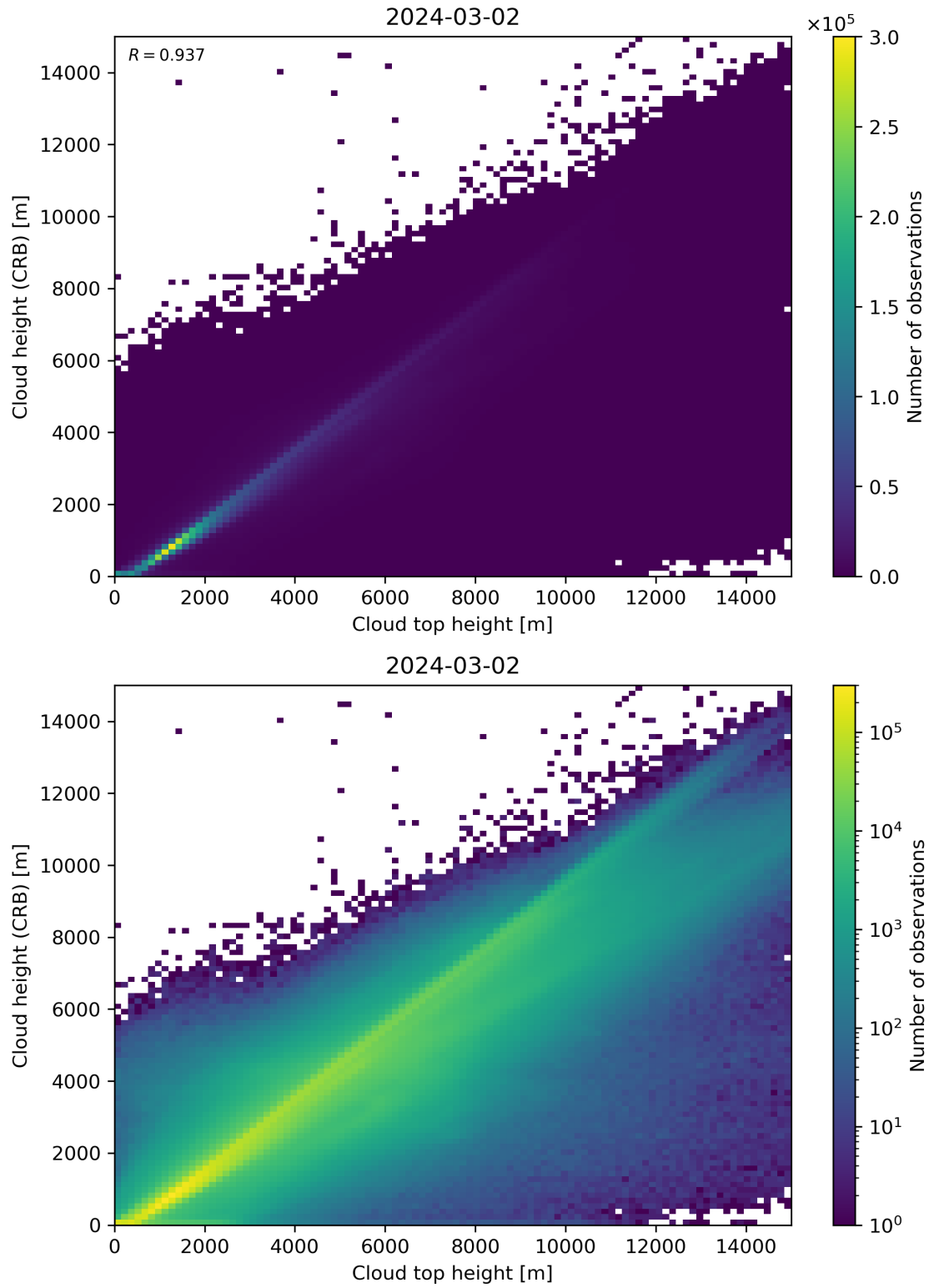
Figure 89: Scatter density plot of “Cloud top height” against “Cloud height (CRB)” for 2024-03-01 to 2024-03-03.
