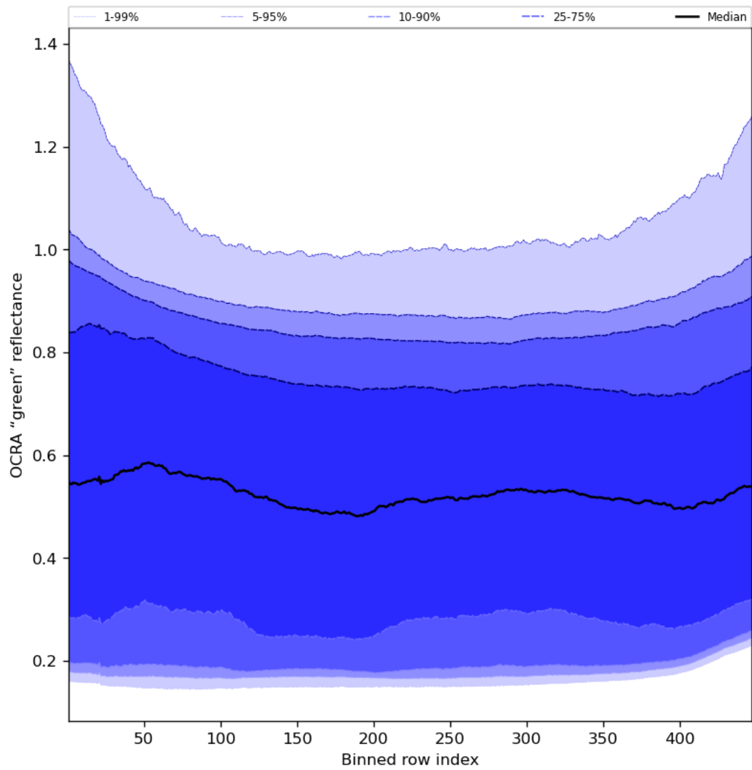
Figure 68: Along track statistics of “OCRA “green” reflectance” for 2024-03-01 to 2024-03-03
