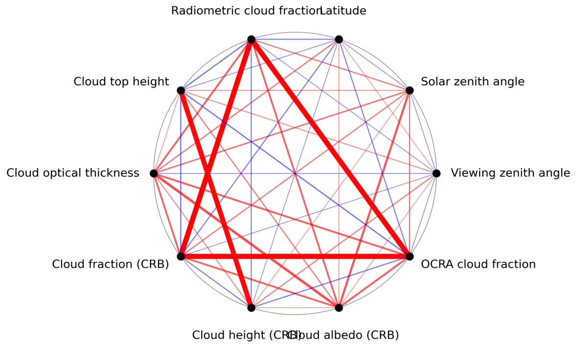
Figure 1: Map of correlation graph for 2024-03-01 to 2024-03-03.
