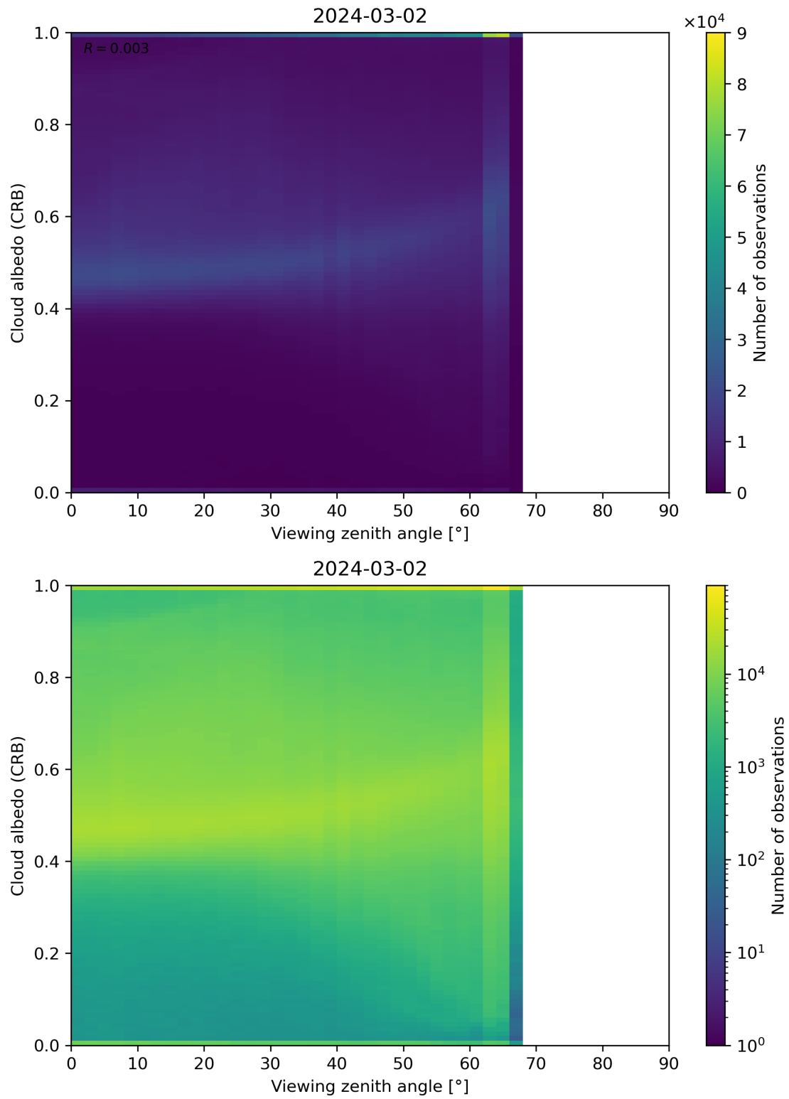
Figure 106: Scatter density plot of “Viewing zenith angle” against “Cloud albedo (CRB)” for 2024-03-01 to 2024-03-03.
