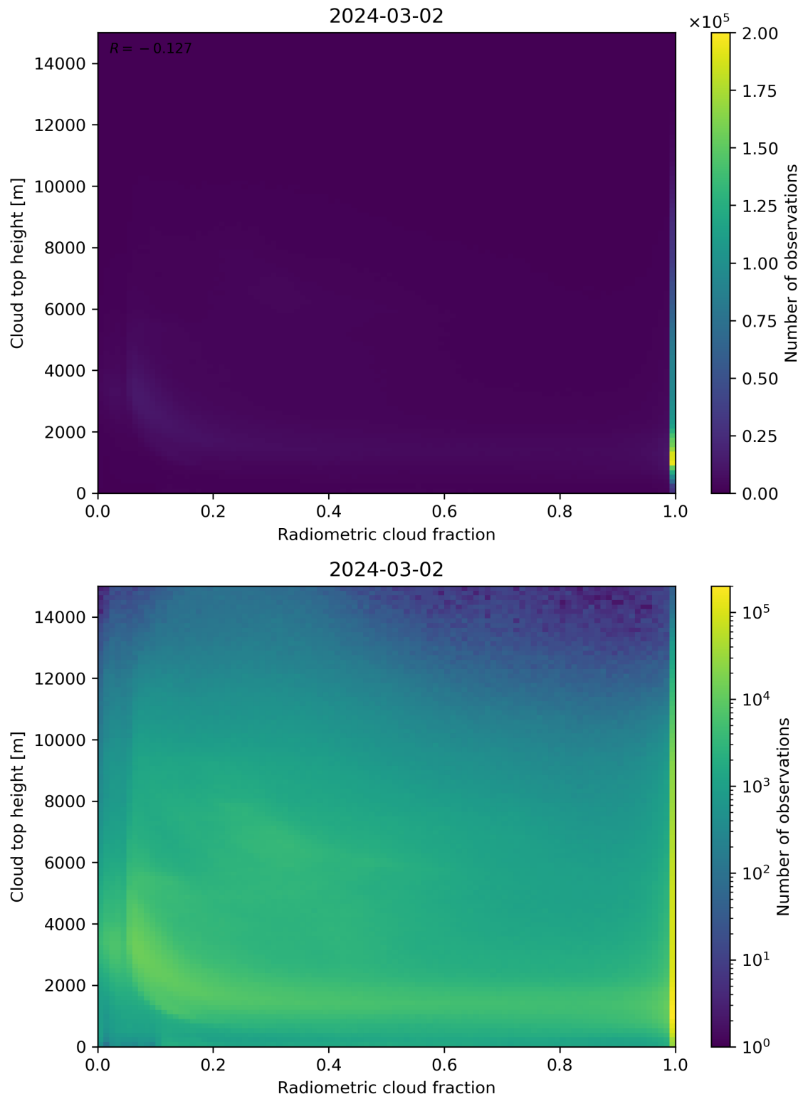
Figure 76: Scatter density plot of “Radiometric cloud fraction” against “Cloud top height” for 2024-03-01 to 2024-03-03.
