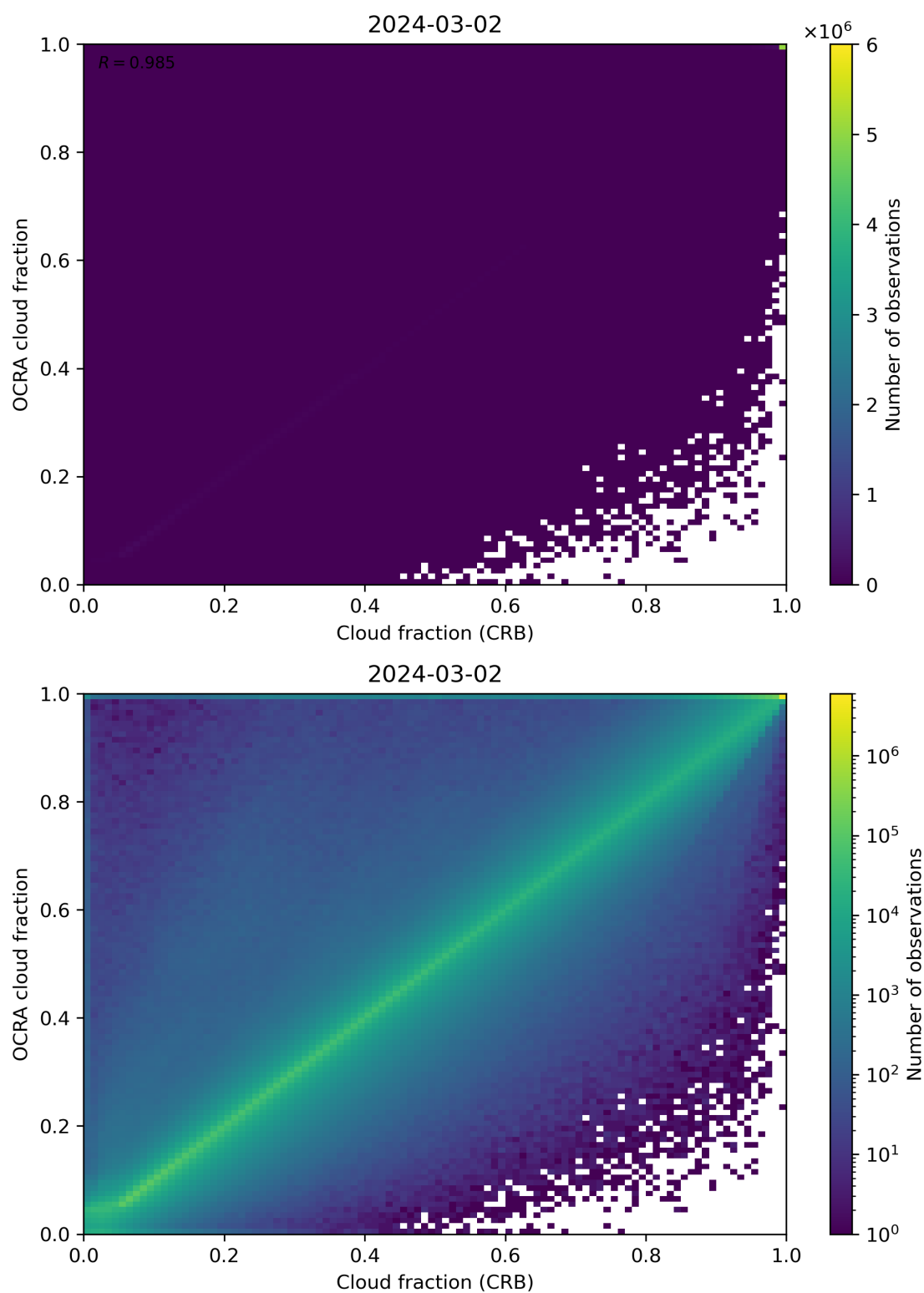
Figure 78: Scatter density plot of “Cloud fraction (CRB)” against “OCRA cloud fraction” for 2024-03-01 to 2024-03-03.
