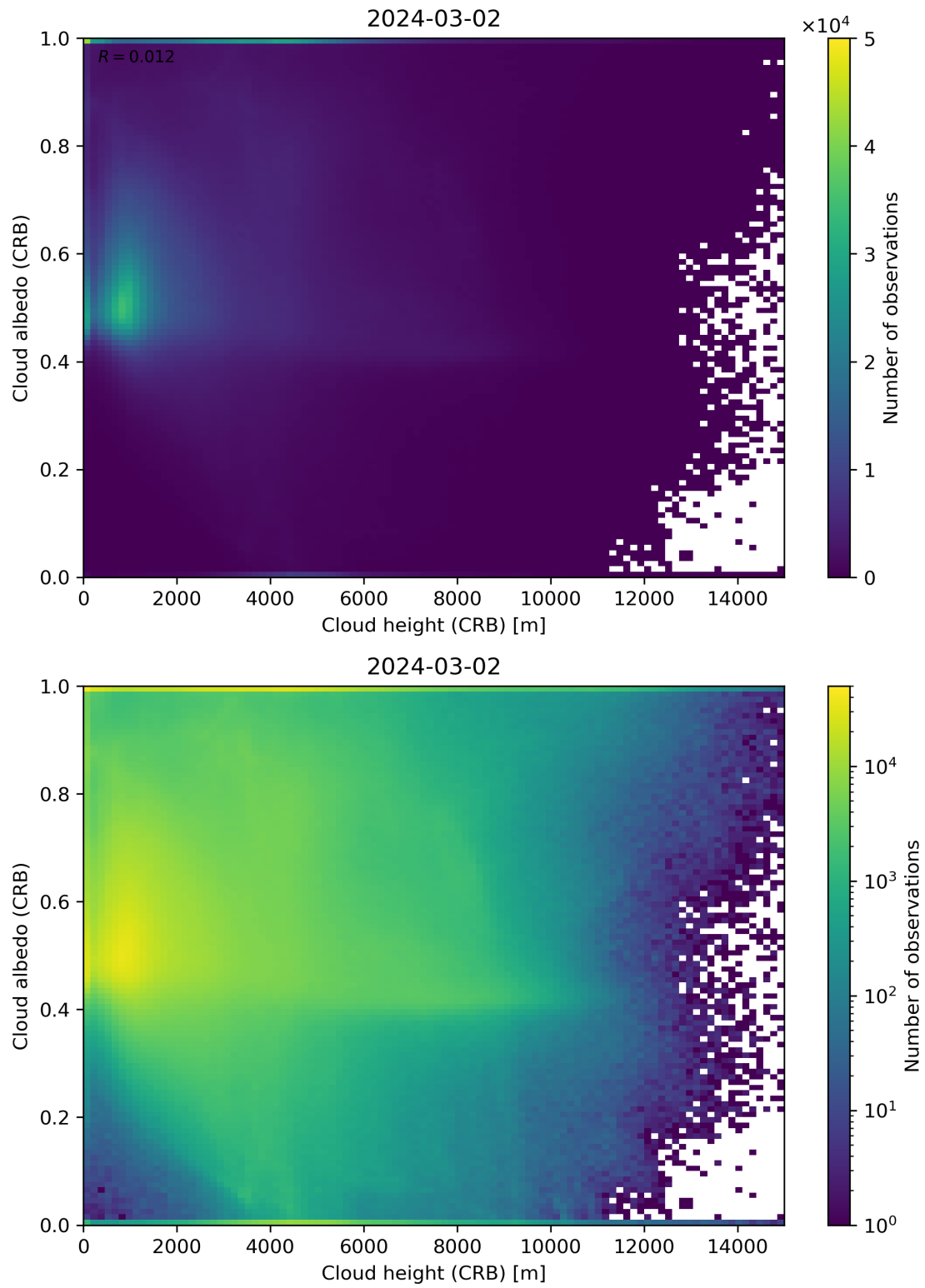
Figure 80: Scatter density plot of “Cloud height (CRB)” against “Cloud albedo (CRB)” for 2024-03-01 to 2024-03-03.
