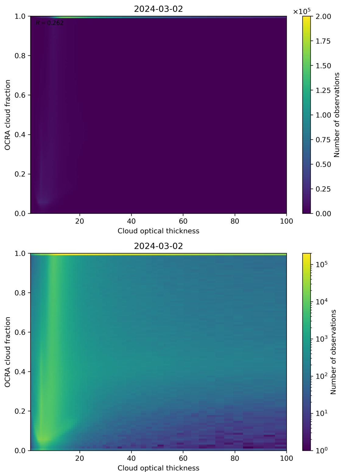
Figure 83: Scatter density plot of “Cloud optical thickness” against “OCRA cloud fraction” for 2024-03-01 to 2024-03-03.
