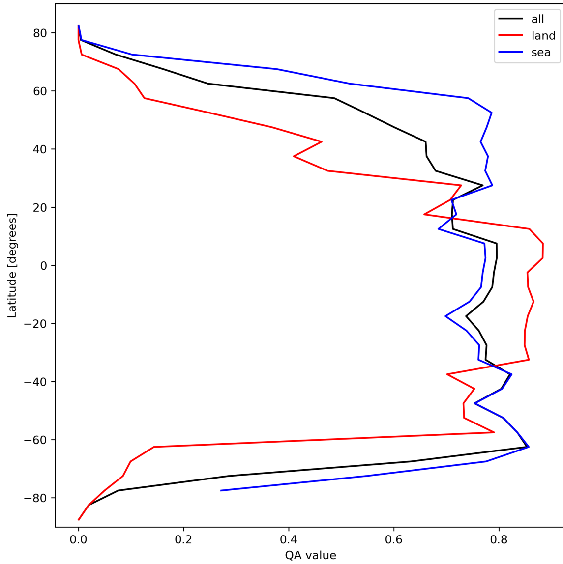
Figure 22: Zonal average of “QA value” for 2024-03-01 to 2024-03-03.
