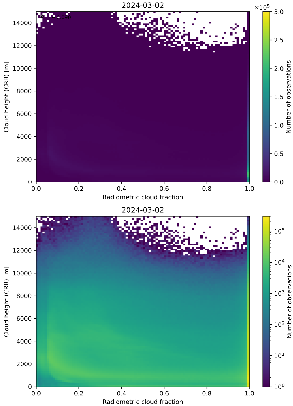
Figure 74: Scatter density plot of “Radiometric cloud fraction” against “Cloud height (CRB)” for 2024-03-01 to 2024-03-03.
