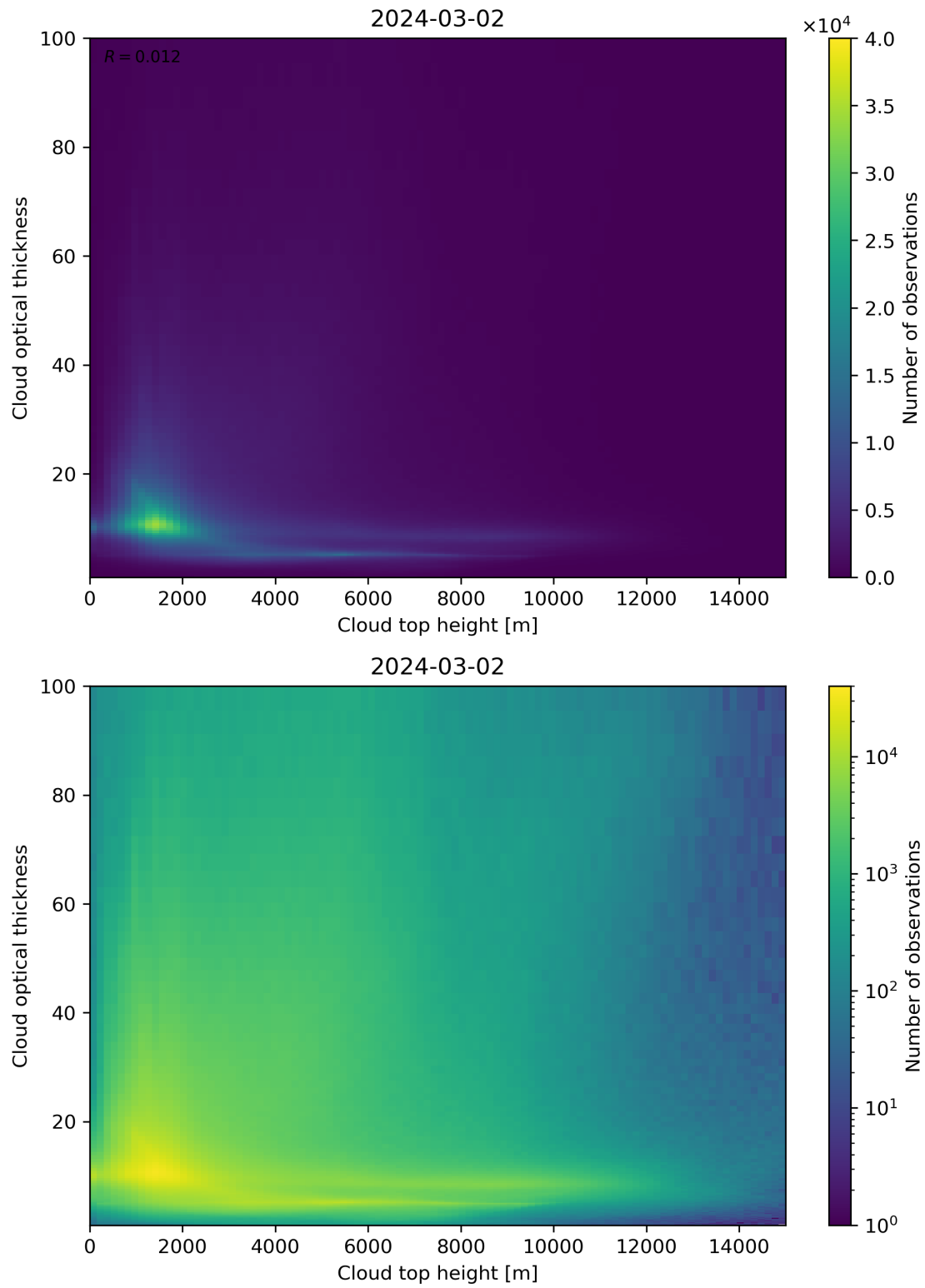
Figure 90: Scatter density plot of “Cloud top height” against “Cloud optical thickness” for 2024-03-01 to 2024-03-03.
