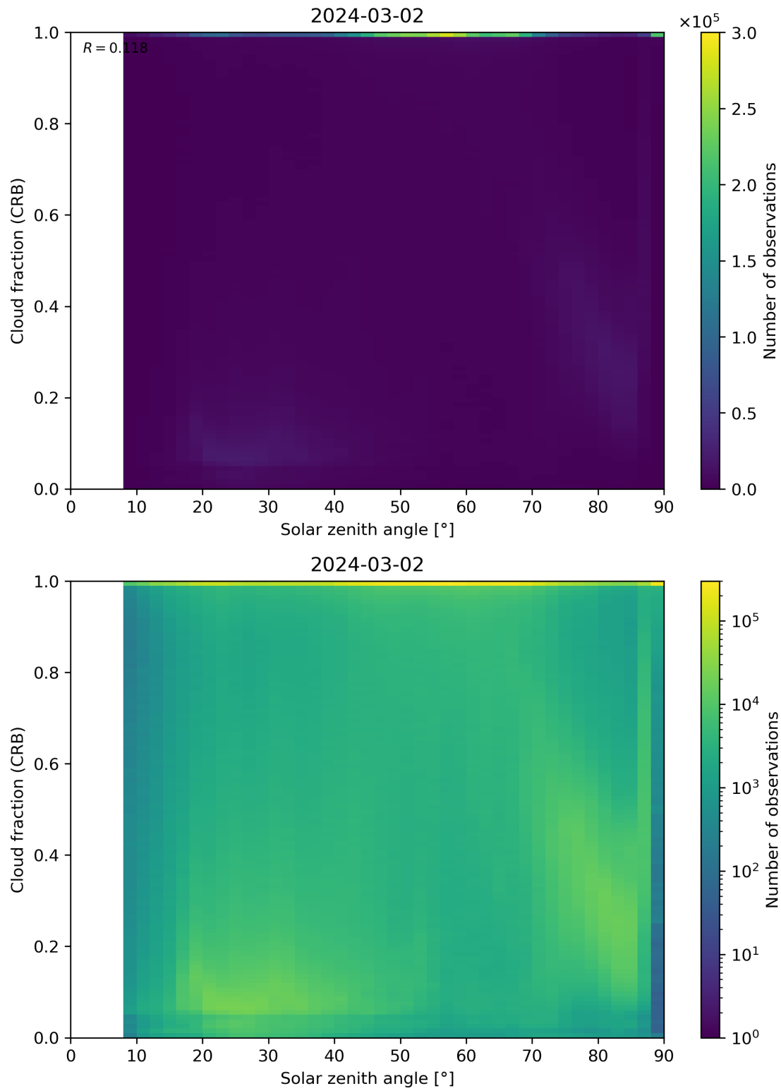
Figure 101: Scatter density plot of “Solar zenith angle” against “Cloud fraction (CRB)” for 2024-03-01 to 2024-03-03.
