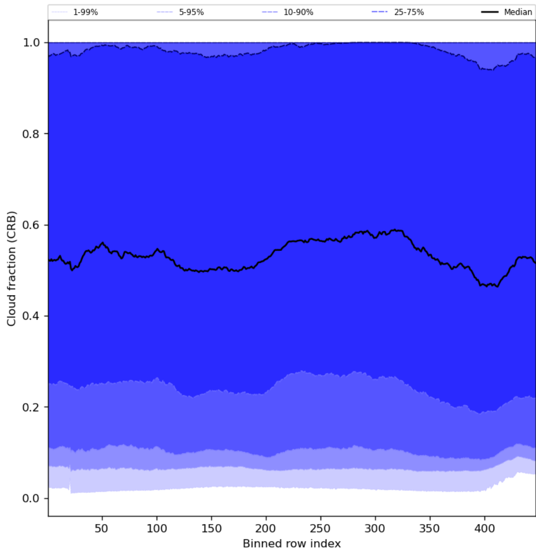
Figure 58: Along track statistics of “Cloud fraction (CRB)” for 2024-03-01 to 2024-03-03
