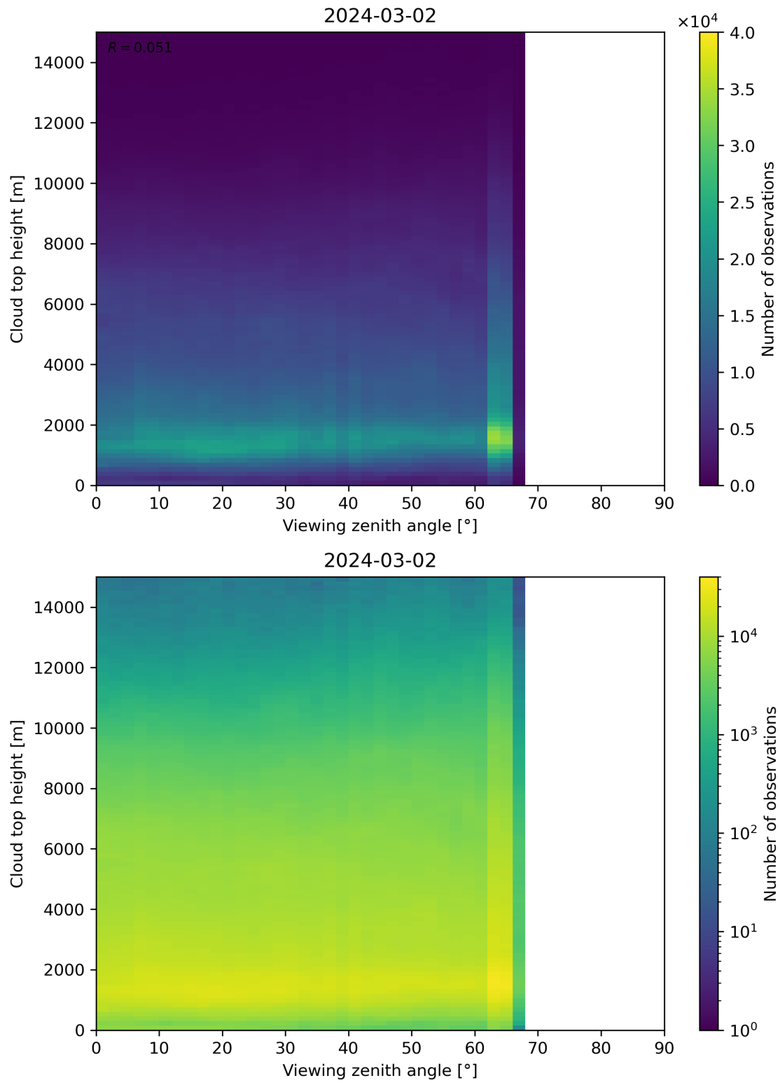
Figure 112: Scatter density plot of “Viewing zenith angle” against “Cloud top height” for 2024-03-01 to 2024-03-03.
