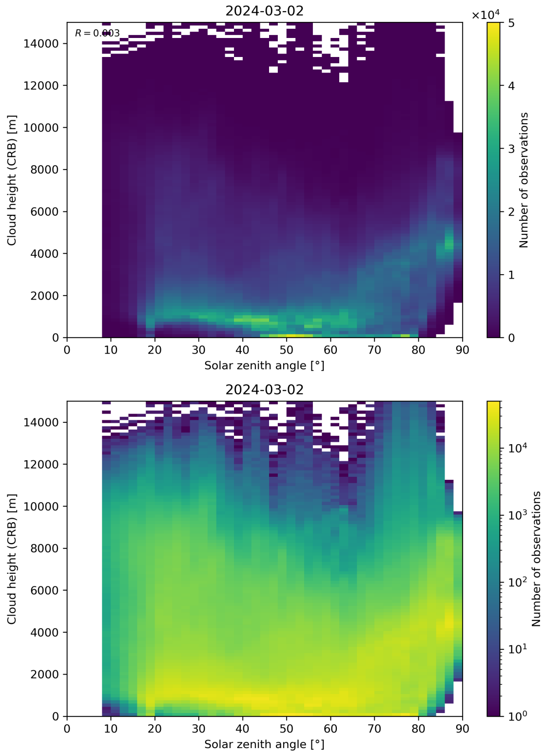
Figure 102: Scatter density plot of “Solar zenith angle” against “Cloud height (CRB)” for 2024-03-01 to 2024-03-03.
