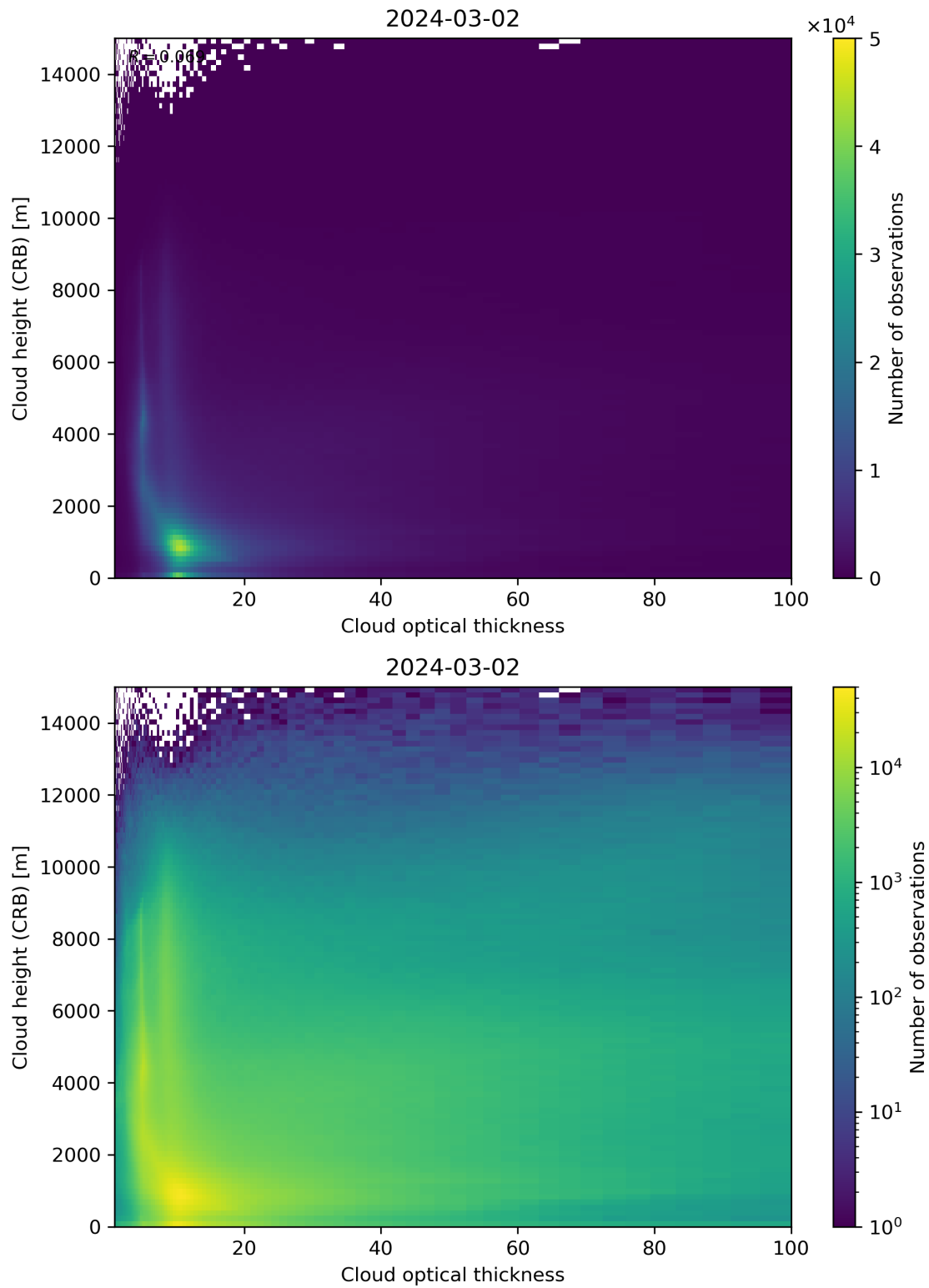
Figure 85: Scatter density plot of “Cloud optical thickness” against “Cloud height (CRB)” for 2024-03-01 to 2024-03-03.
