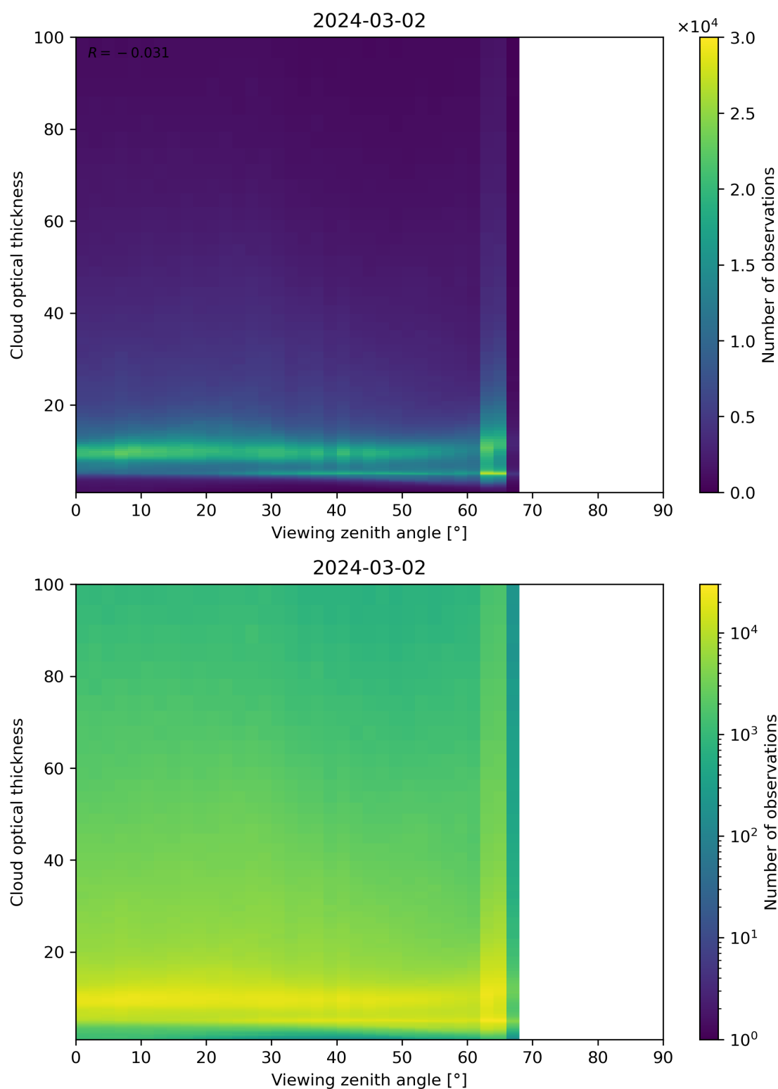
Figure 111: Scatter density plot of “Viewing zenith angle” against “Cloud optical thickness” for 2024-03-01 to 2024-03-03.
