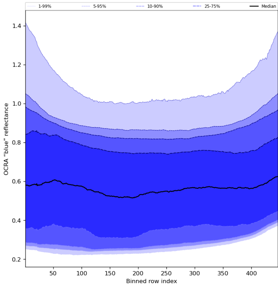
Figure 67: Along track statistics of “OCRA “blue” reflectance” for 2024-03-01 to 2024-03-03
