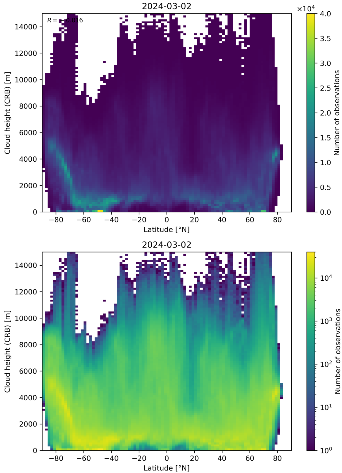
Figure 95: Scatter density plot of “Latitude” against “Cloud height (CRB)” for 2024-03-01 to 2024-03-03.
