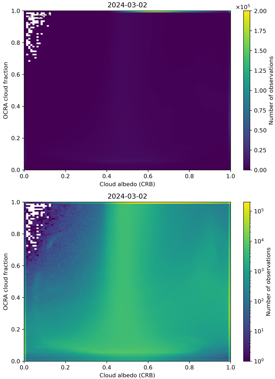
Figure 70: Scatter density plot of “Cloud albedo (CRB)” against “OCRA cloud fraction” for 2024-03-01 to 2024-03-03.
