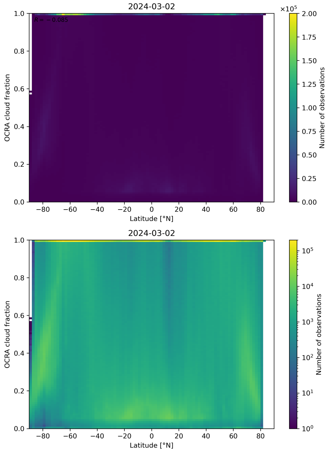
Figure 93: Scatter density plot of “Latitude” against “OCRA cloud fraction” for 2024-03-01 to 2024-03-03.
