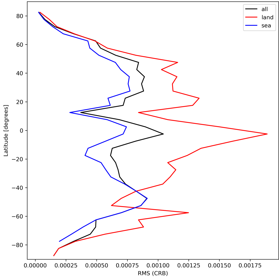
Figure 32: Zonal average of “RMS (CRB)” for 2024-03-01 to 2024-03-03.
