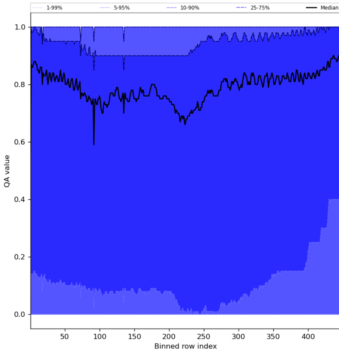
Figure 54: Along track statistics of “QA value” for 2024-03-01 to 2024-03-03
