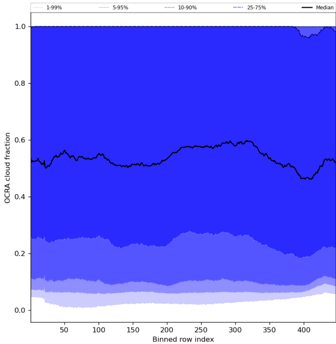
Figure 66: Along track statistics of “OCRA cloud fraction” for 2024-03-01 to 2024-03-03
