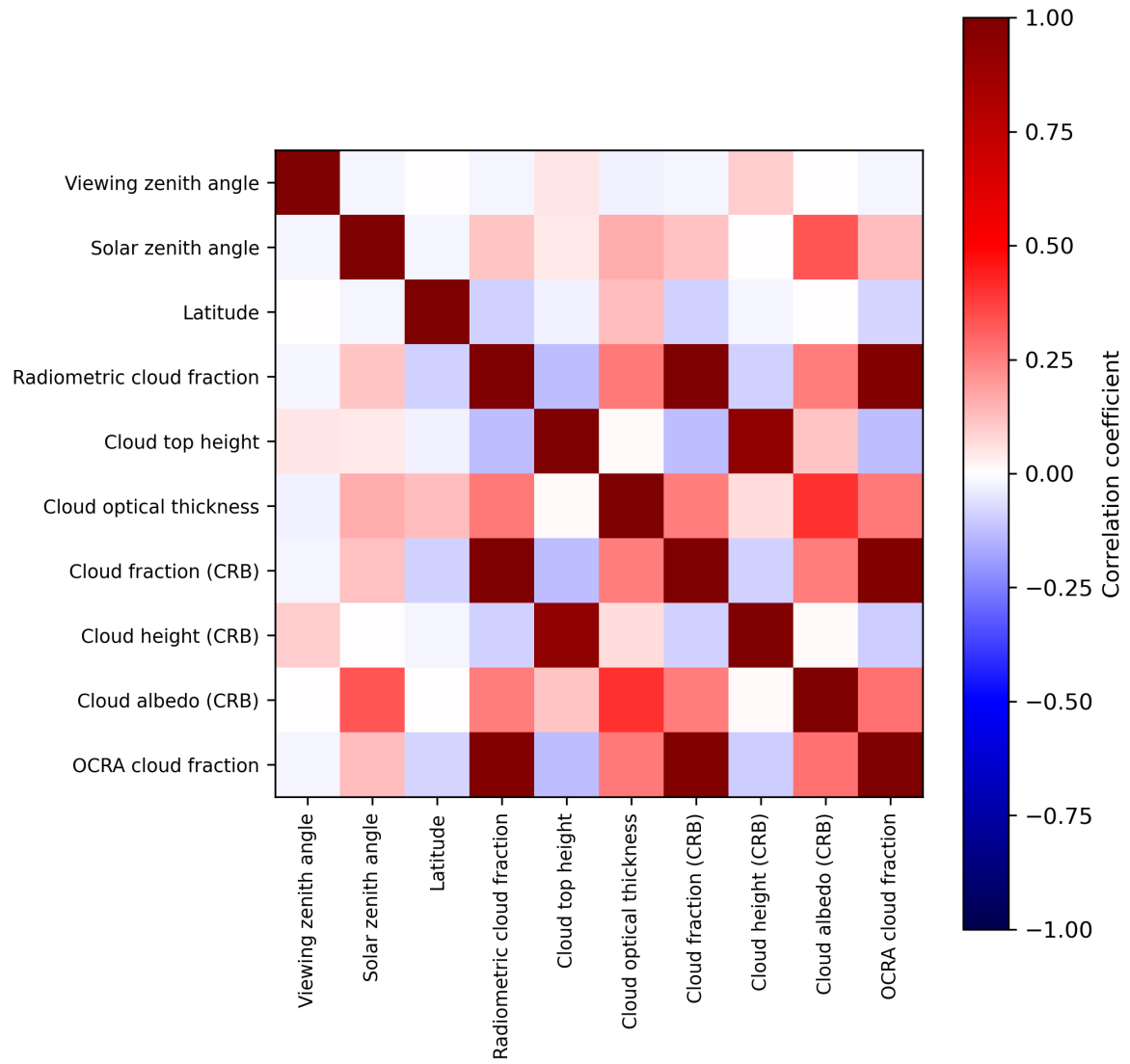
Figure 2: Map of correlation matrix for 2024-03-01 to 2024-03-03.
