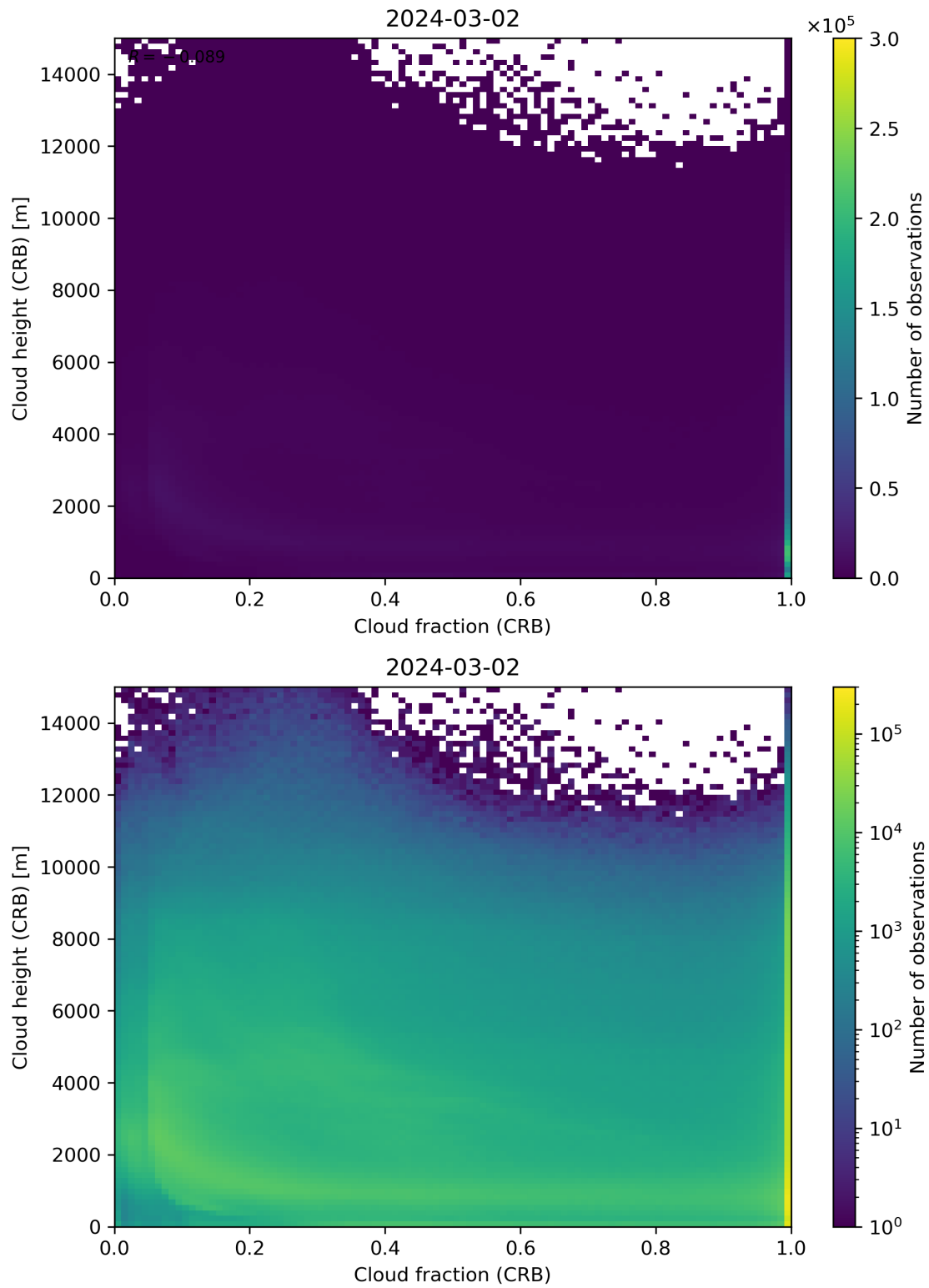
Figure 79: Scatter density plot of “Cloud fraction (CRB)” against “Cloud height (CRB)” for 2024-03-01 to 2024-03-03.
