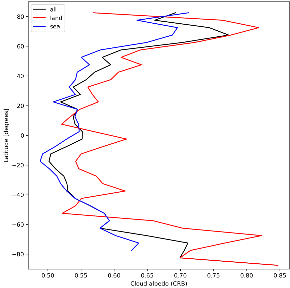
Figure 28: Zonal average of “Cloud albedo (CRB)” for 2024-03-01 to 2024-03-03.
