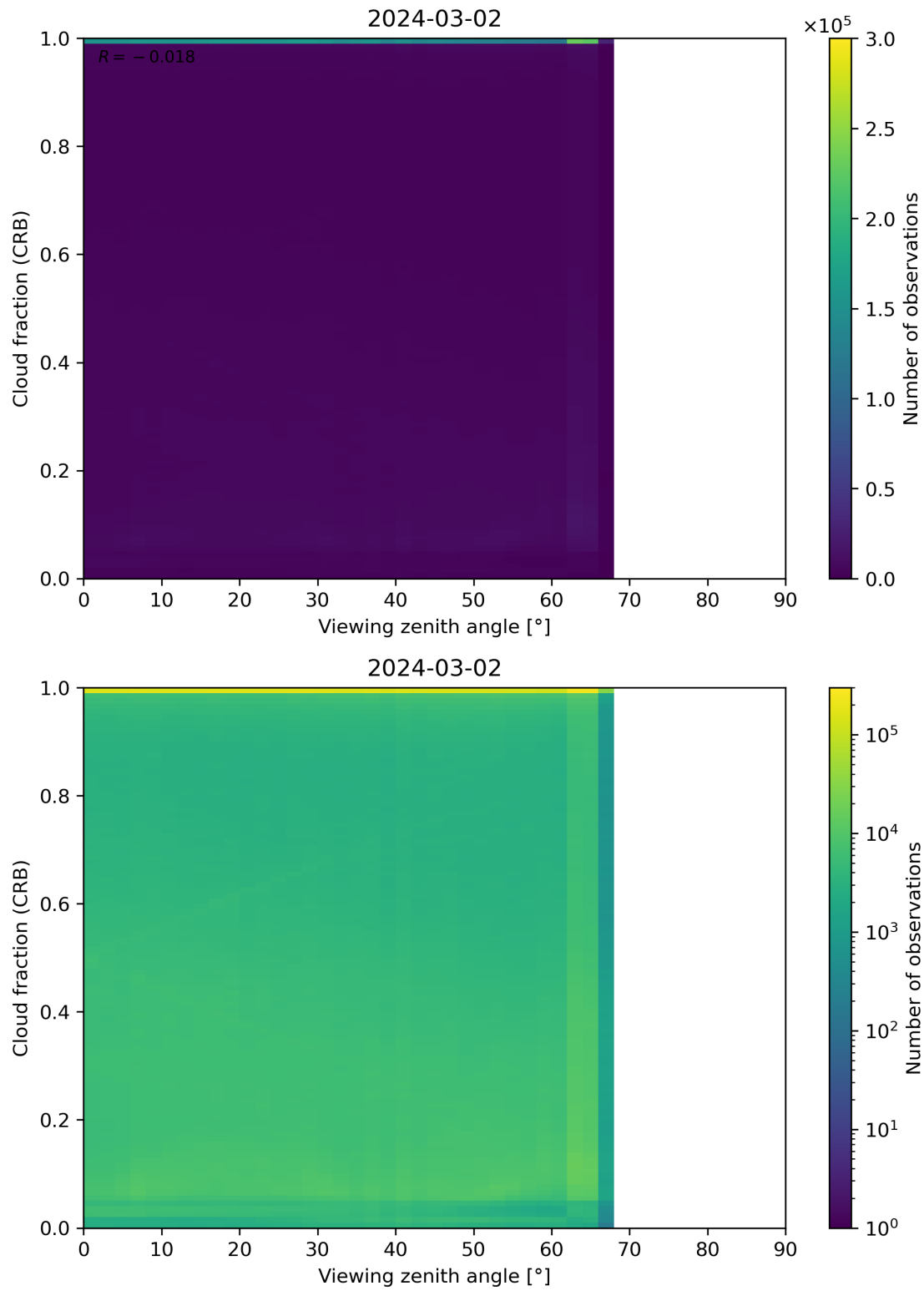
Figure 109: Scatter density plot of “Viewing zenith angle” against “Cloud fraction (CRB)” for 2024-03-01 to 2024-03-03.
