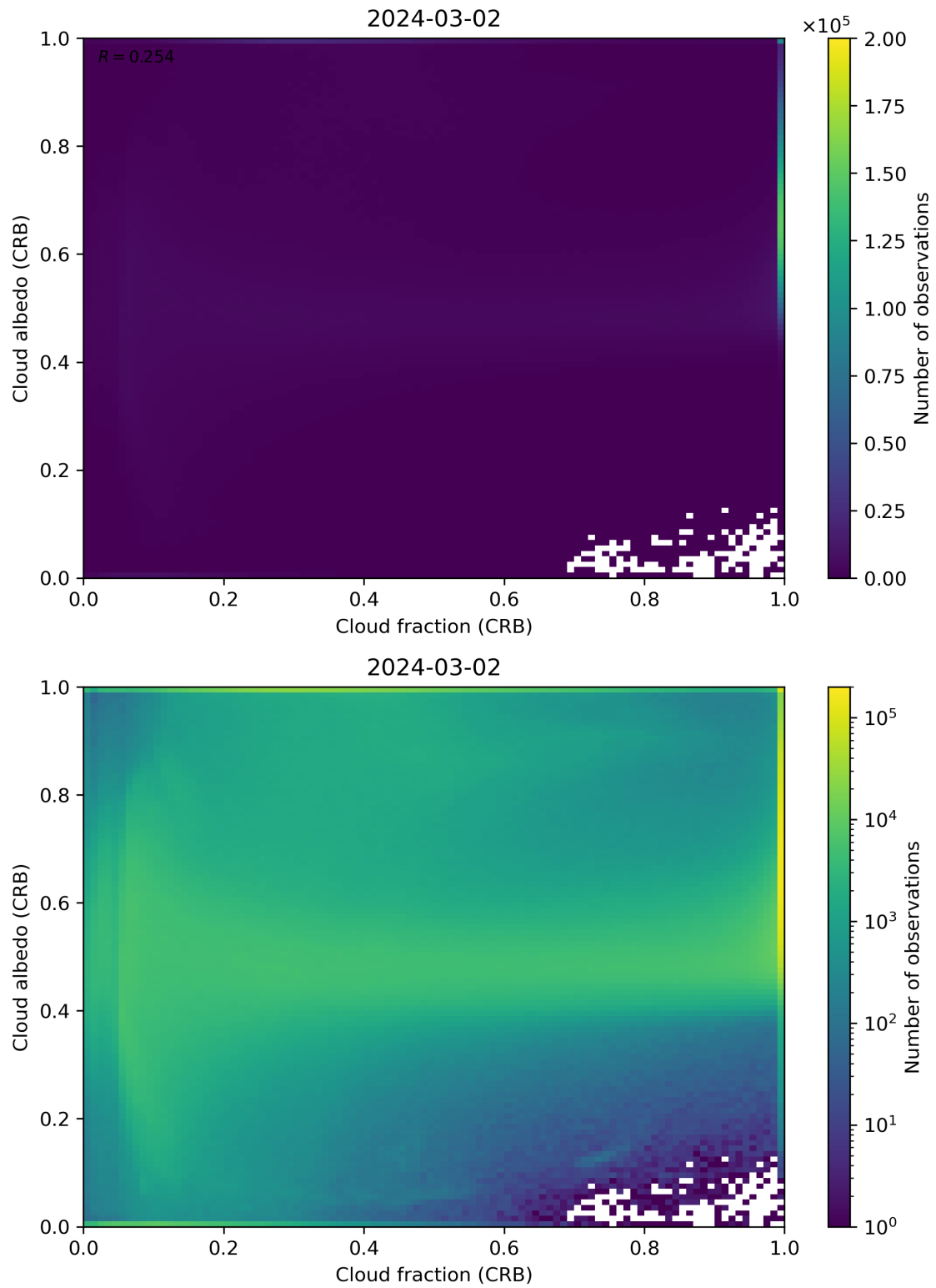
Figure 77: Scatter density plot of “Cloud fraction (CRB)” against “Cloud albedo (CRB)” for 2024-03-01 to 2024-03-03.
