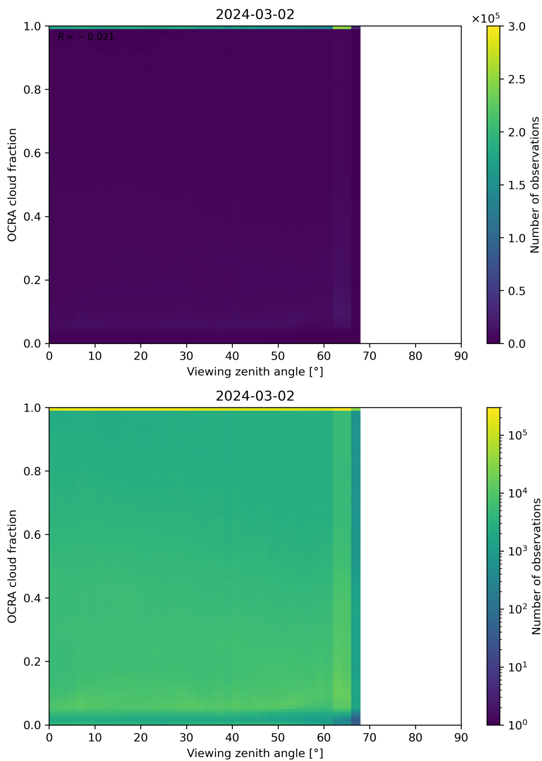
Figure 108: Scatter density plot of “Viewing zenith angle” against “OCRA cloud fraction” for 2024-03-01 to 2024-03-03.
