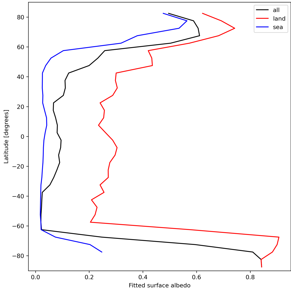
Figure 29: Zonal average of “Fitted surface albedo” for 2024-03-01 to 2024-03-03.
