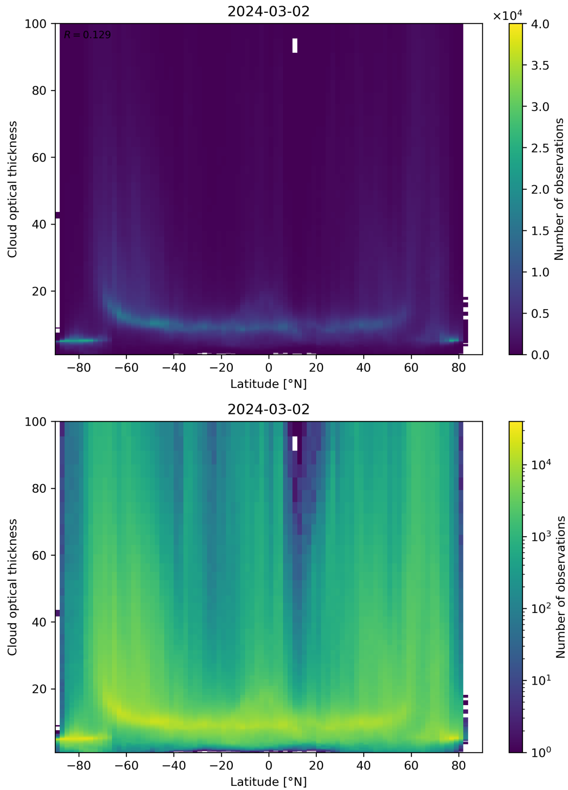
Figure 96: Scatter density plot of “Latitude” against “Cloud optical thickness” for 2024-03-01 to 2024-03-03.
