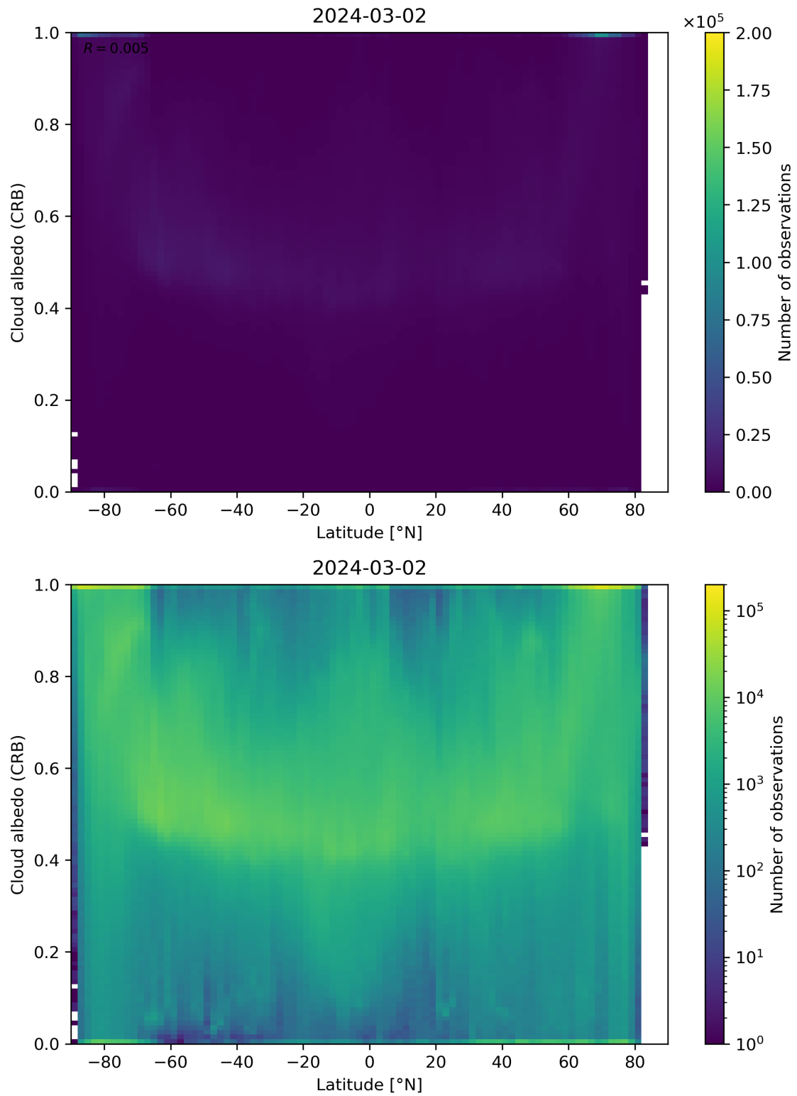
Figure 91: Scatter density plot of “Latitude” against “Cloud albedo (CRB)” for 2024-03-01 to 2024-03-03.
