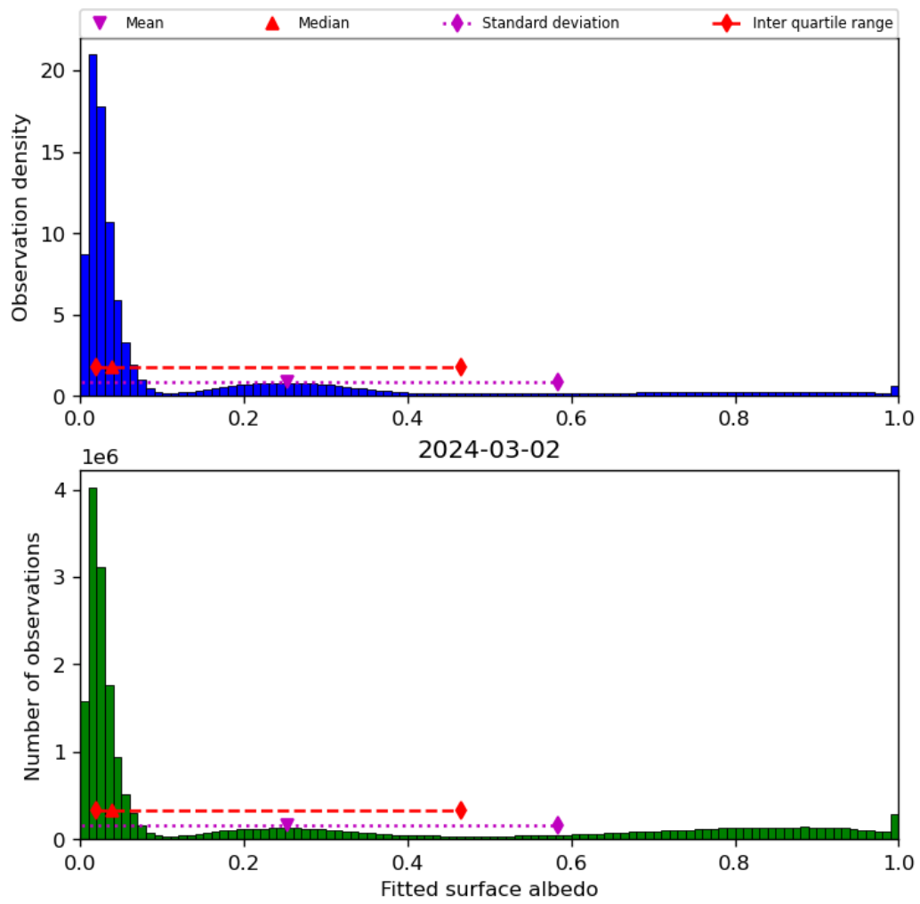
Figure 45: Histogram of “Fitted surface albedo” for 2024-03-01 to 2024-03-03
