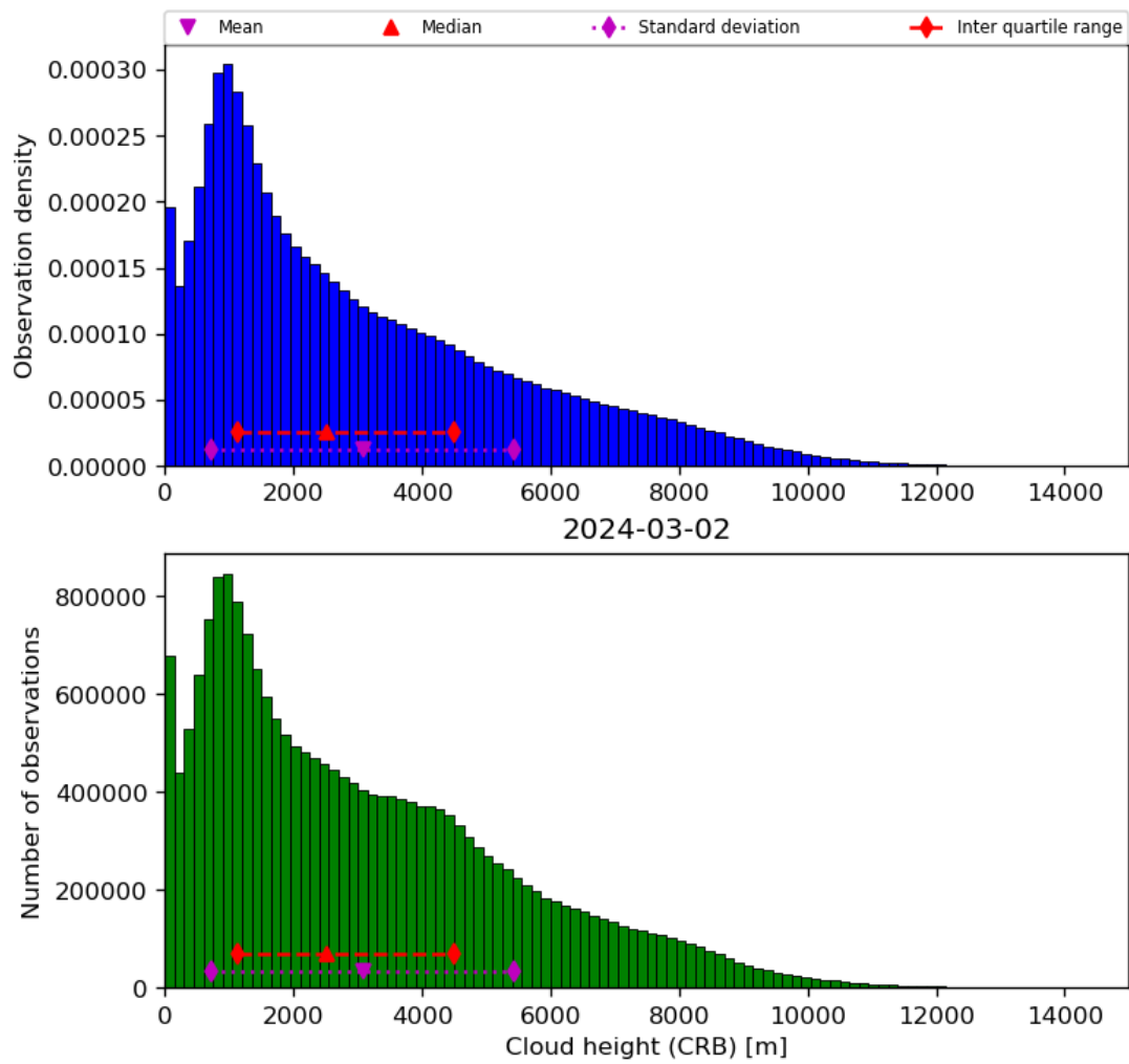
Figure 43: Histogram of “Cloud height (CRB)” for 2024-03-01 to 2024-03-03
