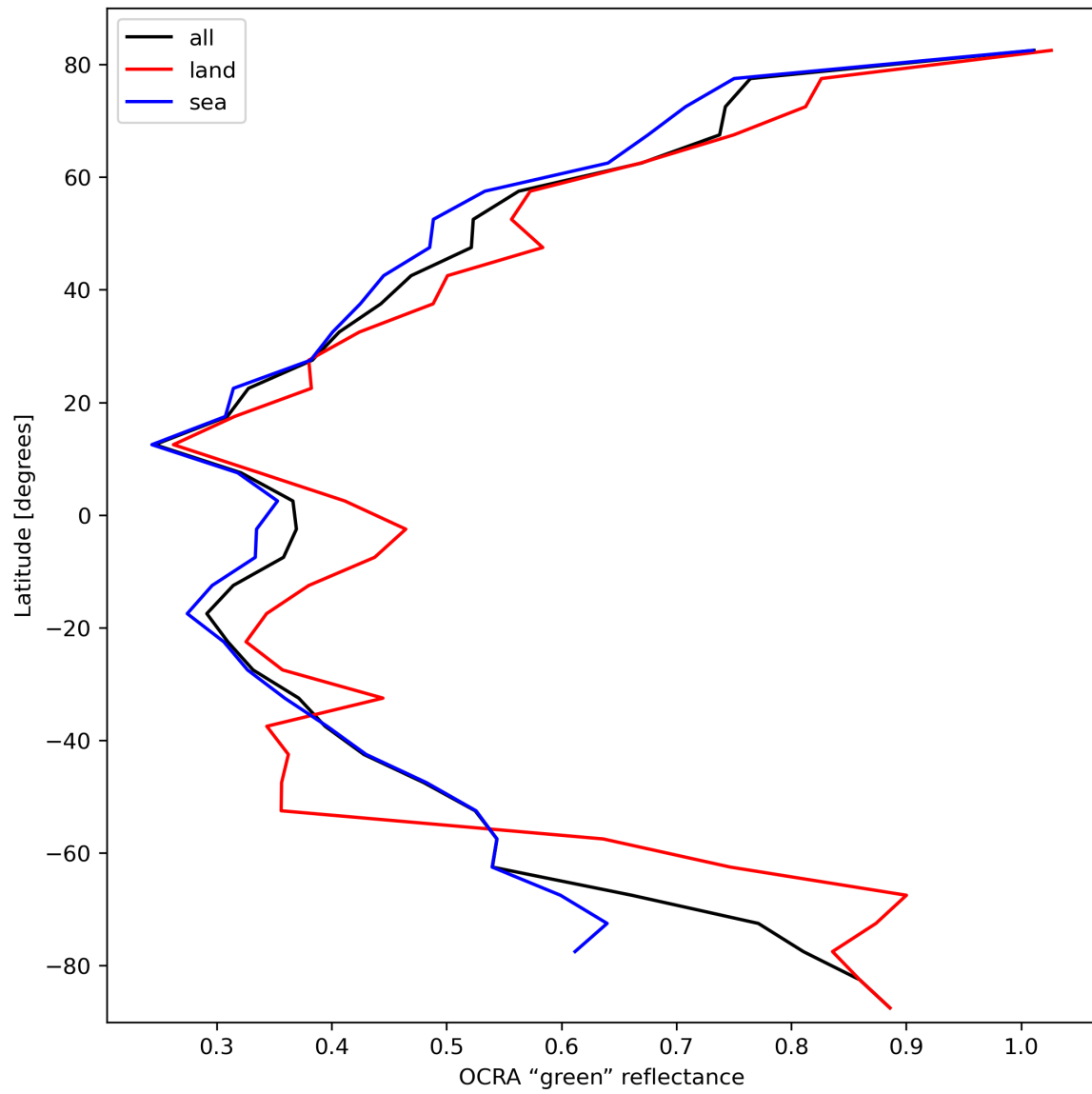
Figure 36: Zonal average of “OCRA “green” reflectance” for 2024-03-01 to 2024-03-03.
