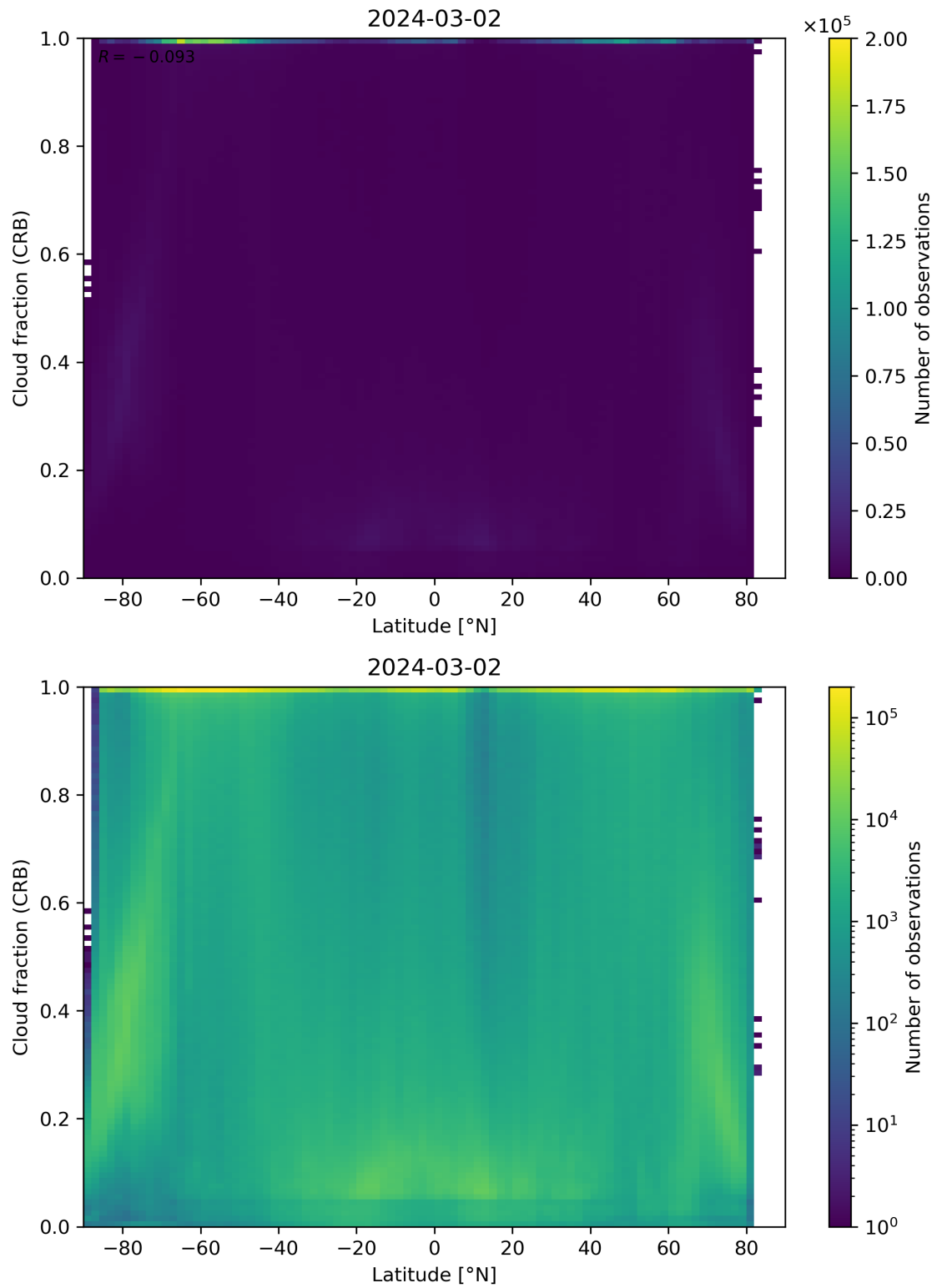
Figure 94: Scatter density plot of “Latitude” against “Cloud fraction (CRB)” for 2024-03-01 to 2024-03-03.
