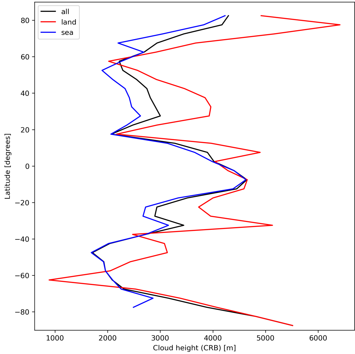
Figure 27: Zonal average of “Cloud height (CRB)” for 2024-03-01 to 2024-03-03.
