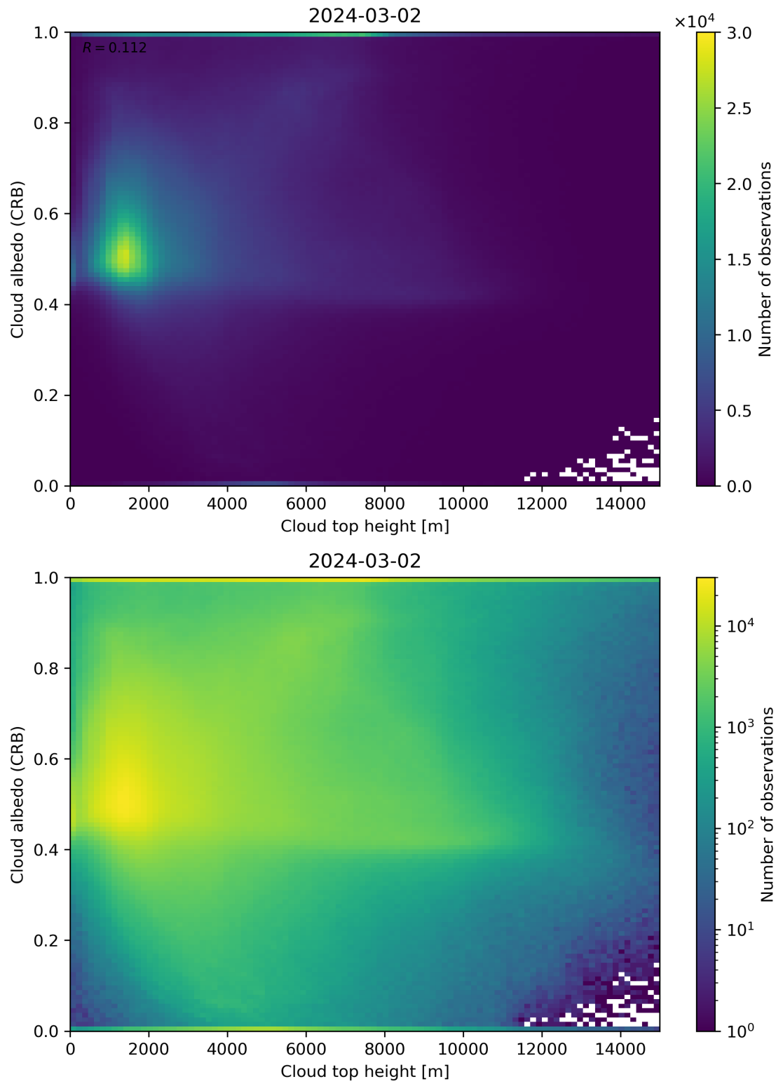
Figure 86: Scatter density plot of “Cloud top height” against “Cloud albedo (CRB)” for 2024-03-01 to 2024-03-03.
