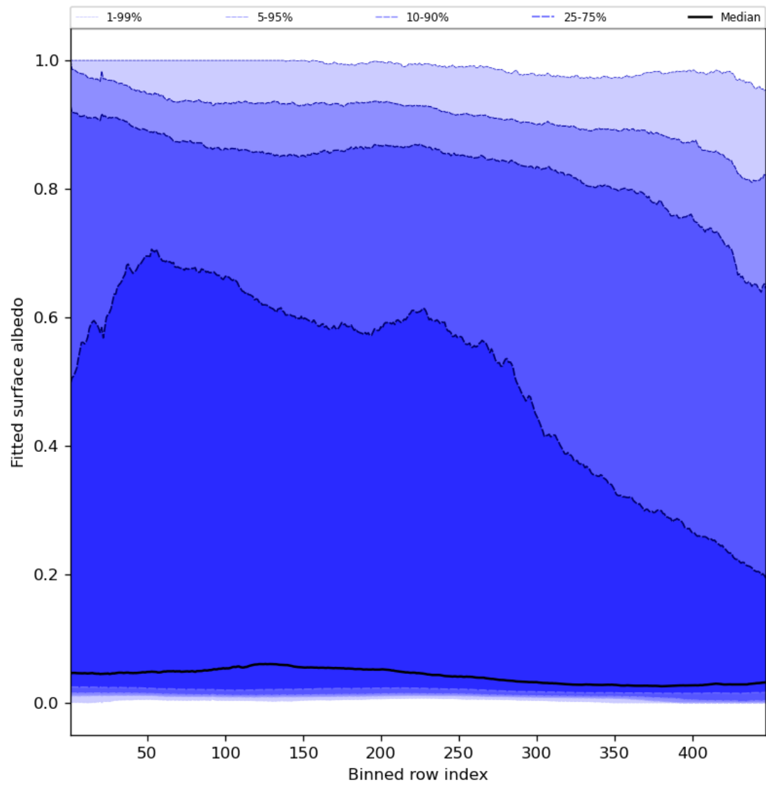
Figure 61: Along track statistics of “Fitted surface albedo” for 2024-03-01 to 2024-03-03
