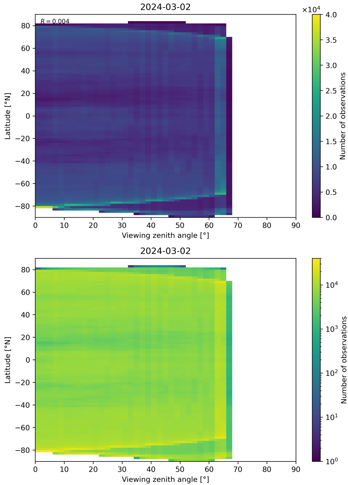
Figure 113: Scatter density plot of “Viewing zenith angle” against “Latitude” for 2024-03-01 to 2024-03-03.
