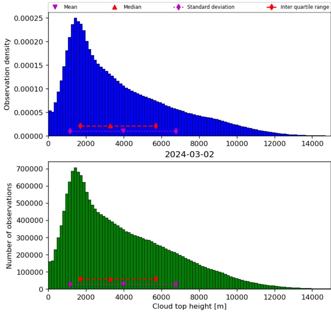
Figure 40: Histogram of “Cloud top height” for 2024-03-01 to 2024-03-03
