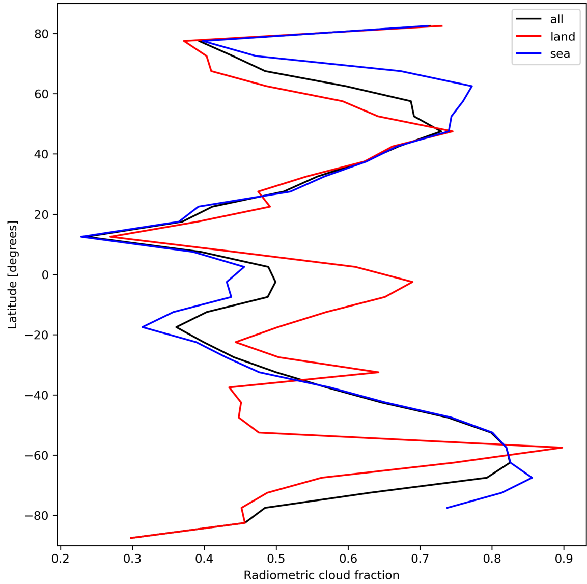
Figure 23: Zonal average of “Radiometric cloud fraction” for 2024-03-01 to 2024-03-03.
