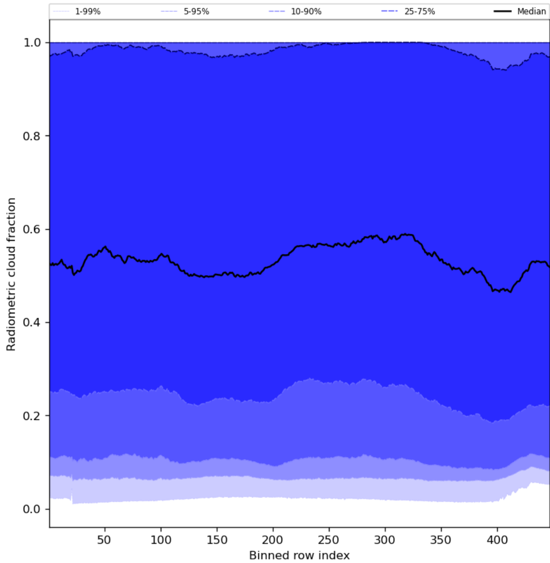
Figure 55: Along track statistics of “Radiometric cloud fraction” for 2024-03-01 to 2024-03-03
