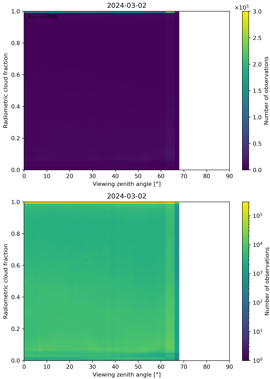
Figure 107: Scatter density plot of “Viewing zenith angle” against “Radiometric cloud fraction” for 2024-03-01 to 2024-03-03.
