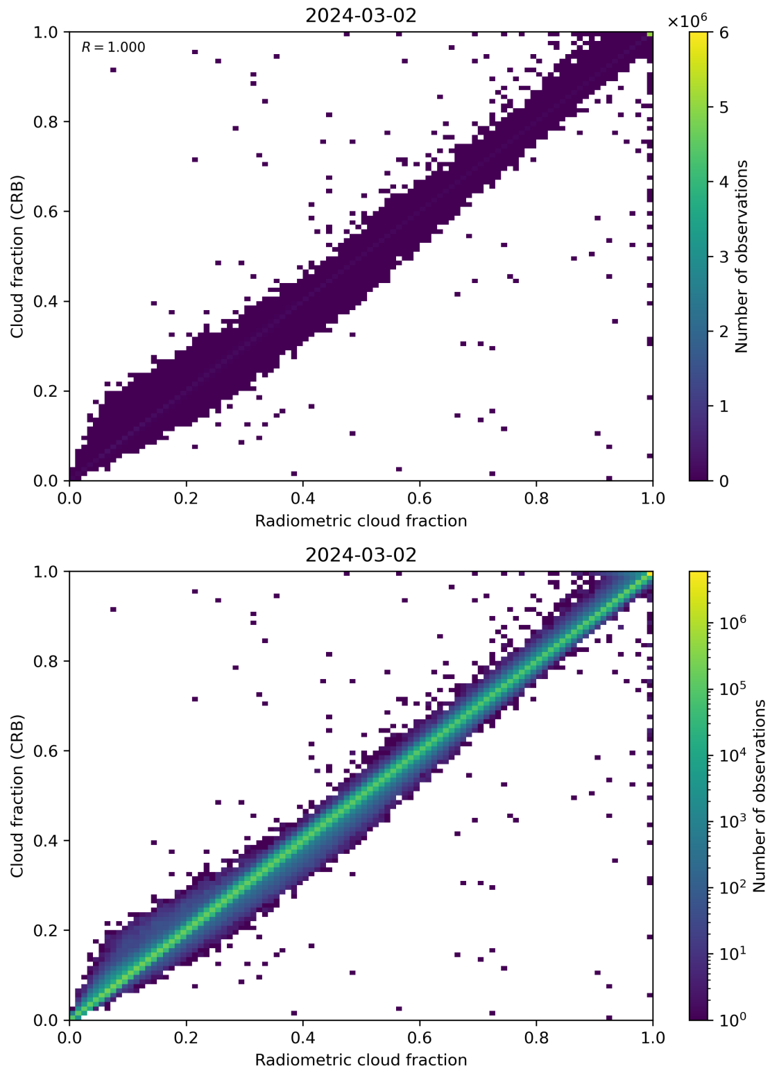
Figure 73: Scatter density plot of “Radiometric cloud fraction” against “Cloud fraction (CRB)” for 2024-03-01 to 2024-03-03.
