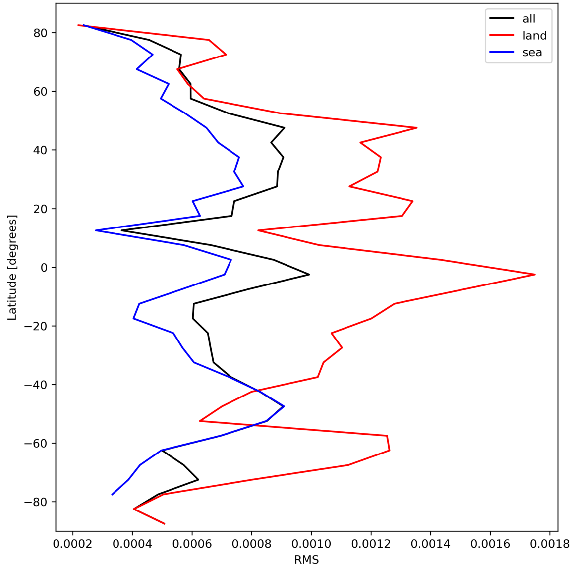
Figure 31: Zonal average of “RMS” for 2024-03-01 to 2024-03-03.
