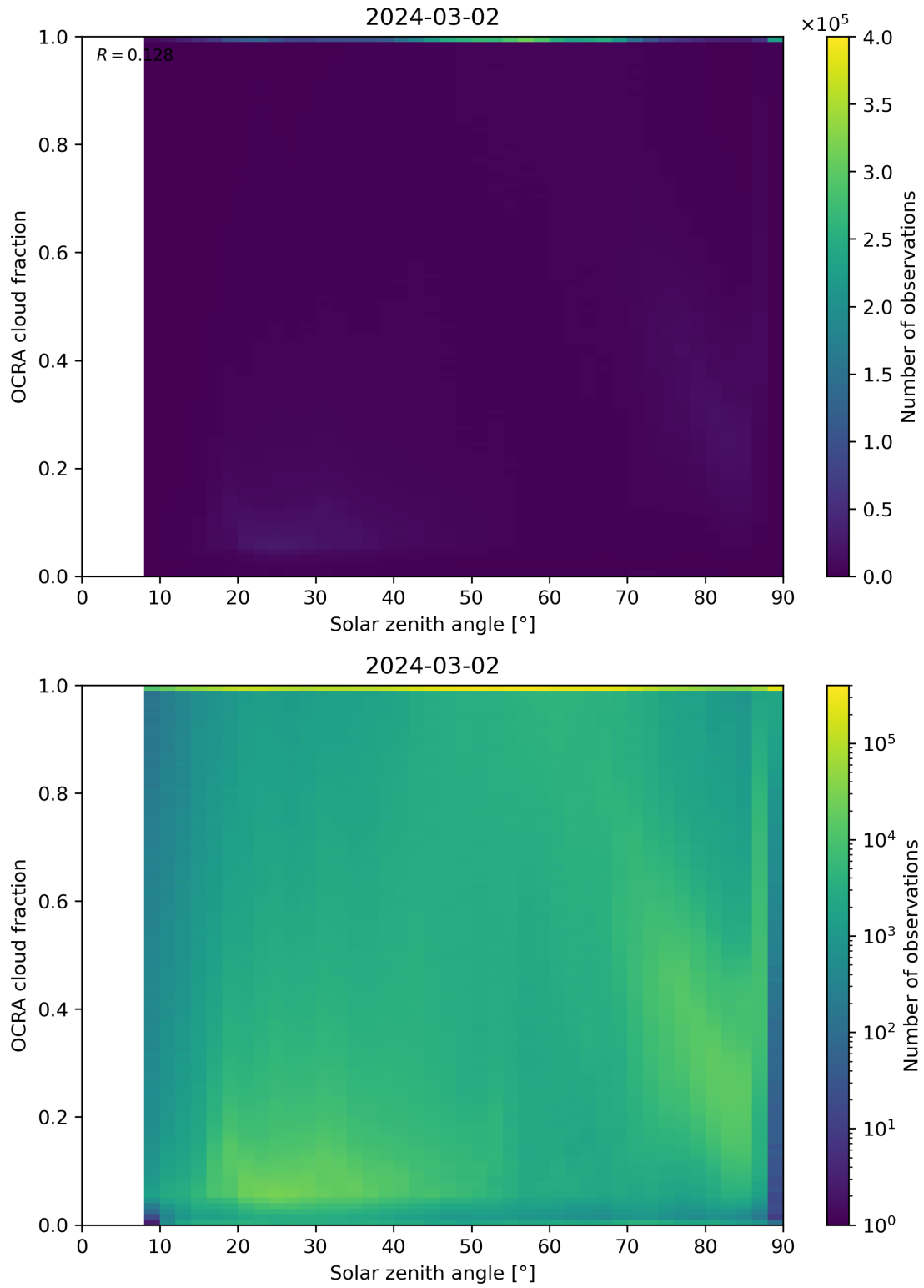
Figure 100: Scatter density plot of “Solar zenith angle” against “OCRA cloud fraction” for 2024-03-01 to 2024-03-03.
