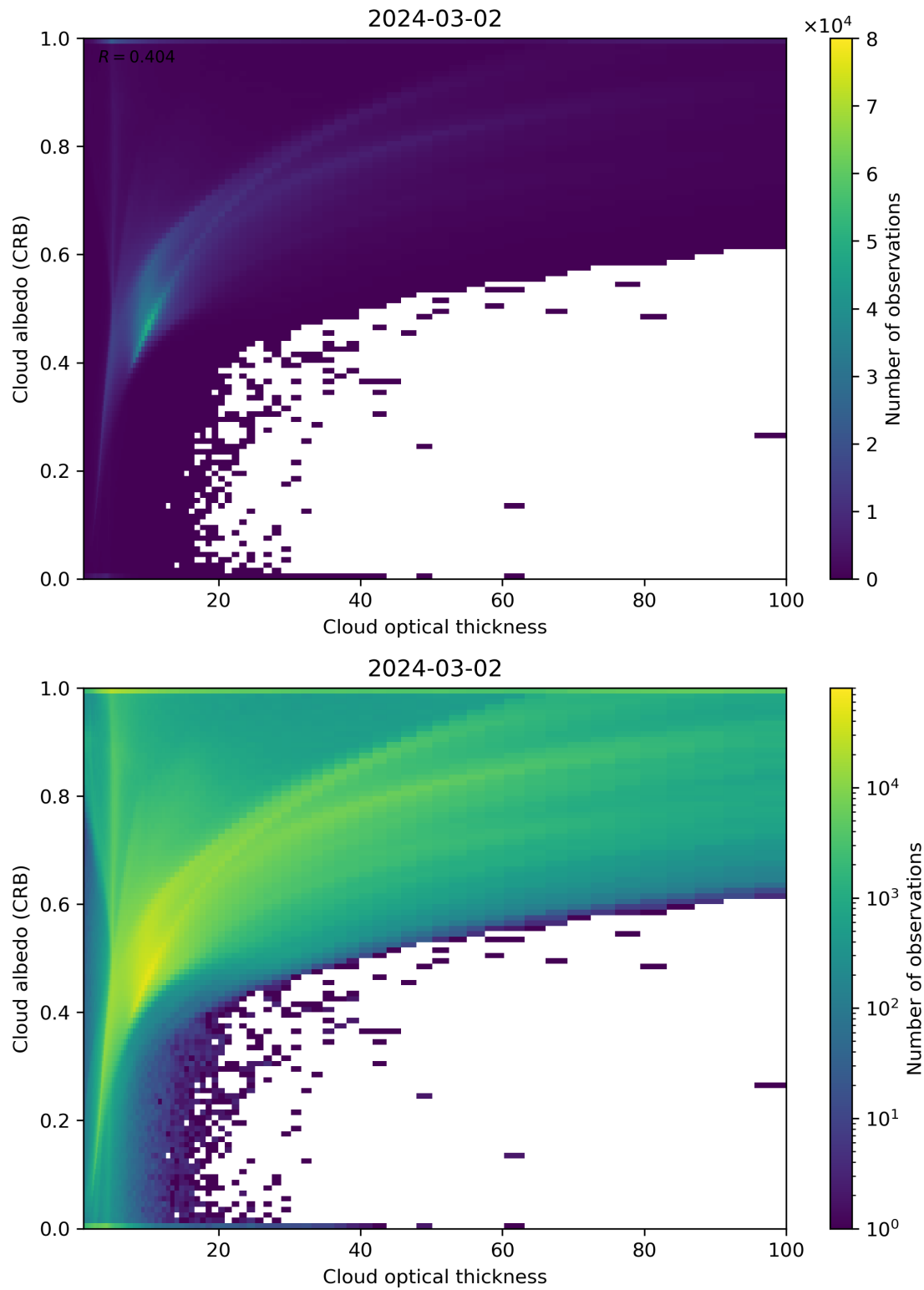
Figure 82: Scatter density plot of “Cloud optical thickness” against “Cloud albedo (CRB)” for 2024-03-01 to 2024-03-03.
