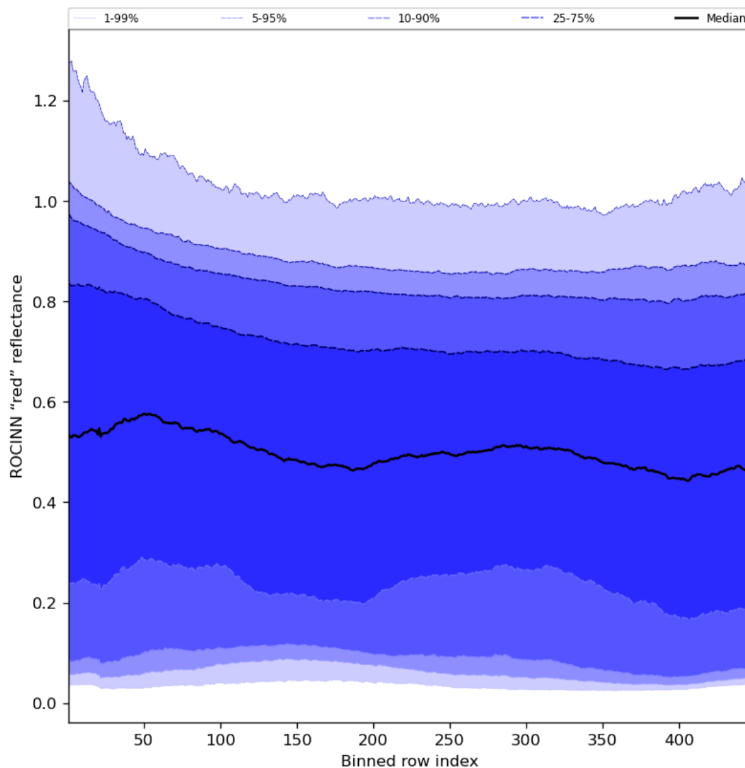
Figure 69: Along track statistics of “ROCINN “red” reflectance” for 2024-03-01 to 2024-03-03
