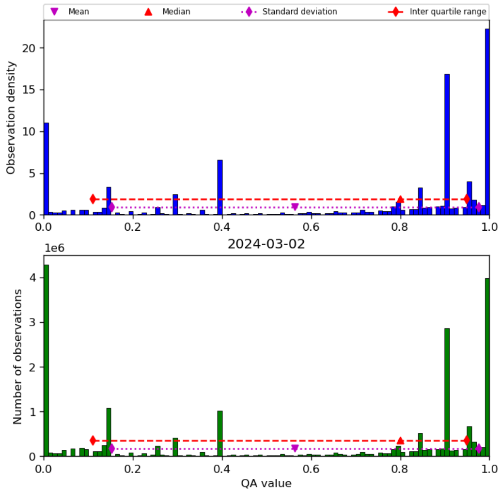
Figure 38: Histogram of “QA value” for 2024-03-01 to 2024-03-03
