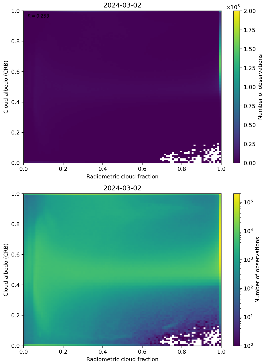
Figure 71: Scatter density plot of “Radiometric cloud fraction” against “Cloud albedo (CRB)” for 2024-03-01 to 2024-03-03.
