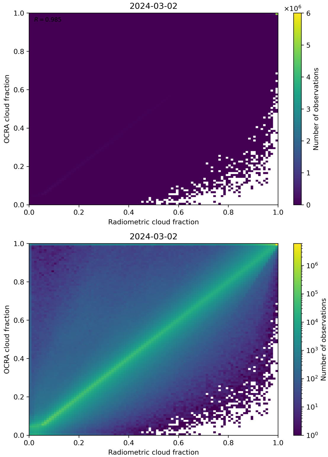
Figure 72: Scatter density plot of “Radiometric cloud fraction” against “OCRA cloud fraction” for 2024-03-01 to 2024-03-03.
