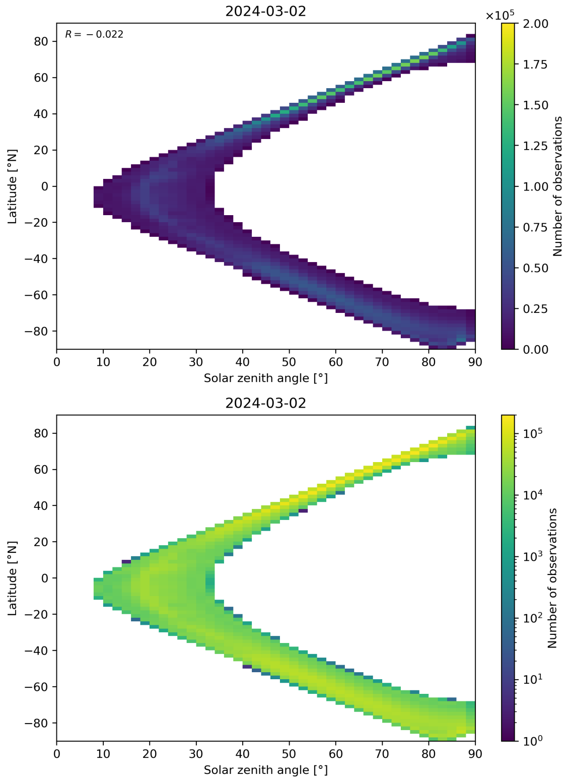
Figure 105: Scatter density plot of “Solar zenith angle” against “Latitude” for 2024-03-01 to 2024-03-03.
