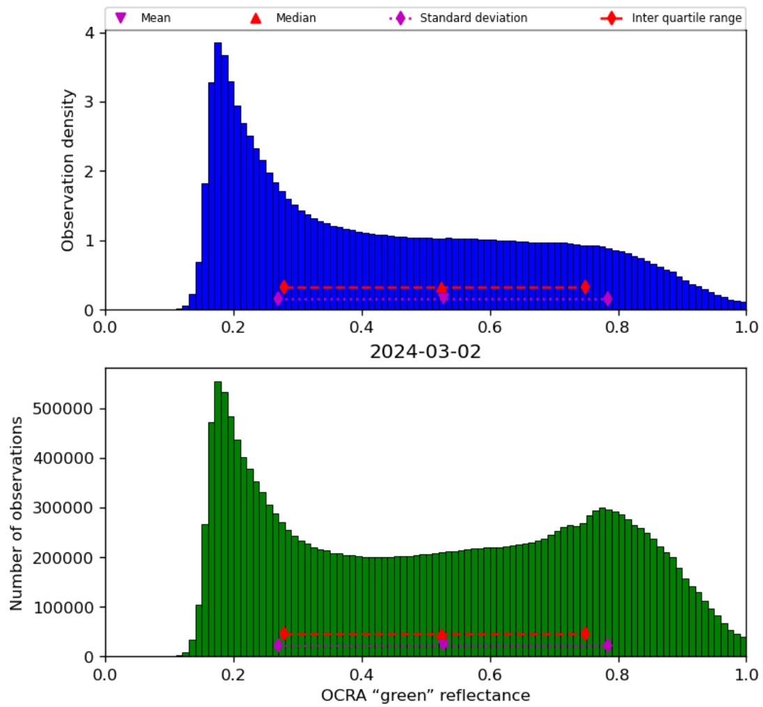
Figure 52: Histogram of “OCRA “green” reflectance” for 2024-03-01 to 2024-03-03
