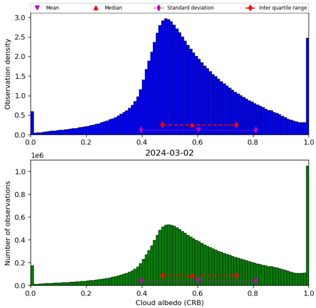
Figure 44: Histogram of “Cloud albedo (CRB)” for 2024-03-01 to 2024-03-03
