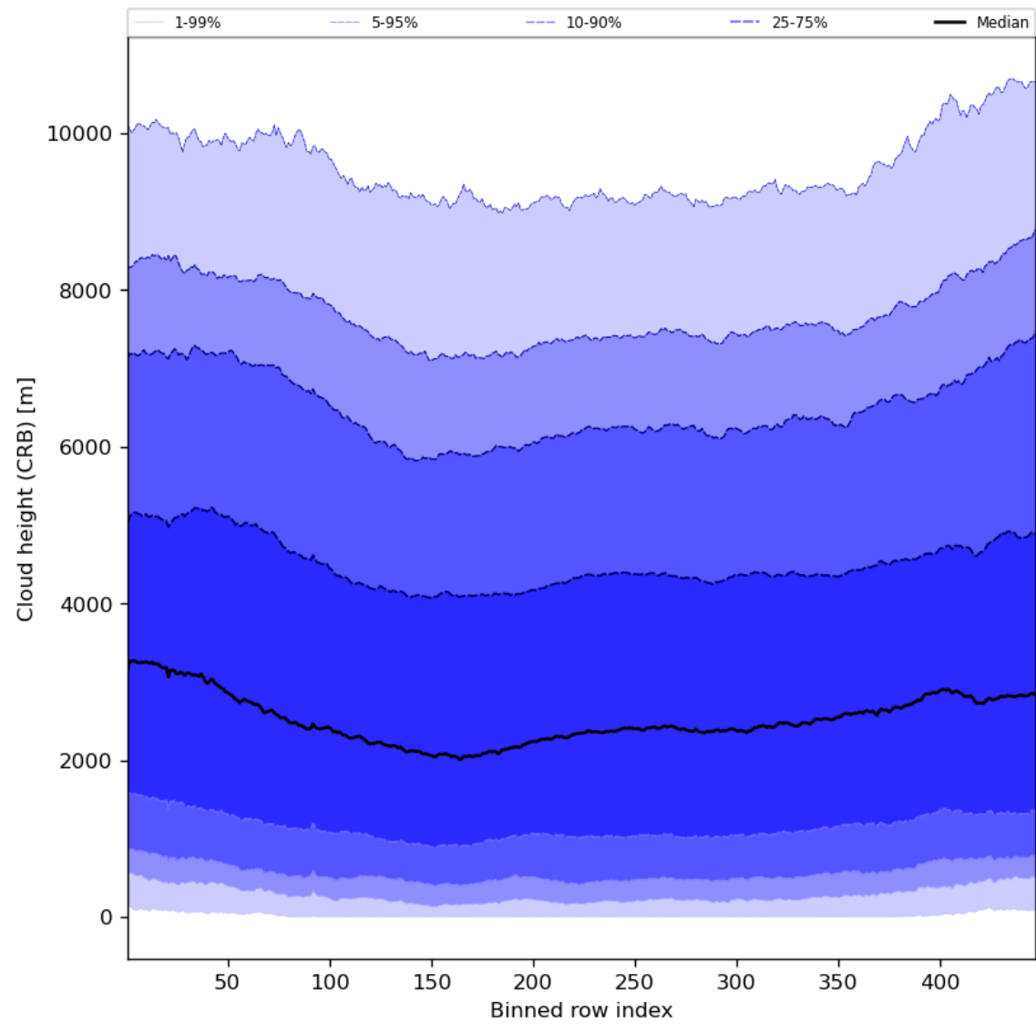
Figure 59: Along track statistics of “Cloud height (CRB)” for 2024-03-01 to 2024-03-03
