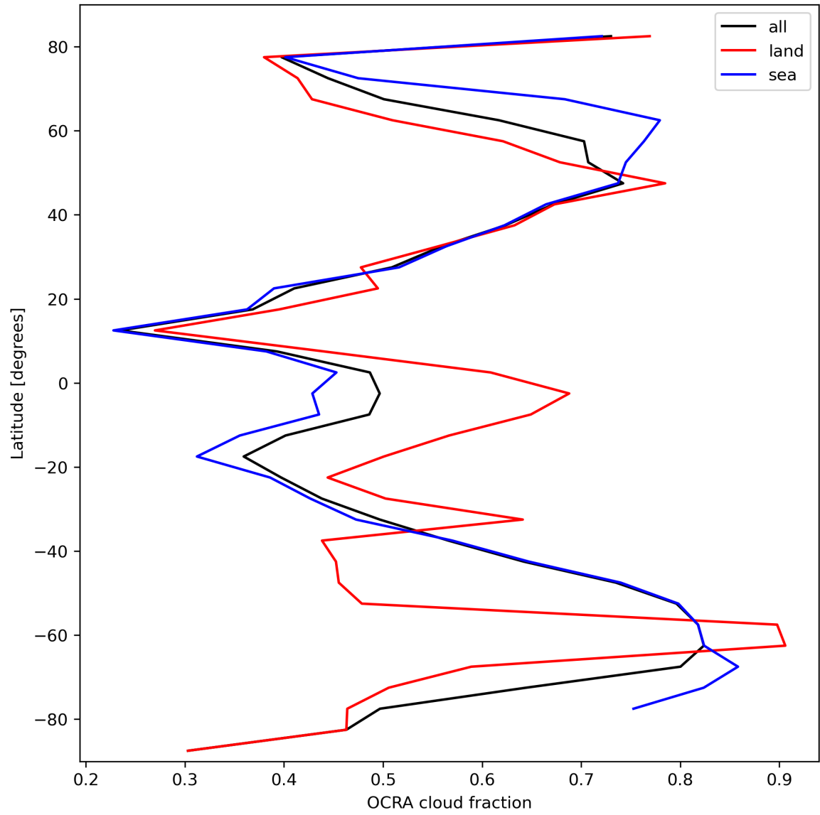
Figure 34: Zonal average of “OCRA cloud fraction” for 2024-03-01 to 2024-03-03.
