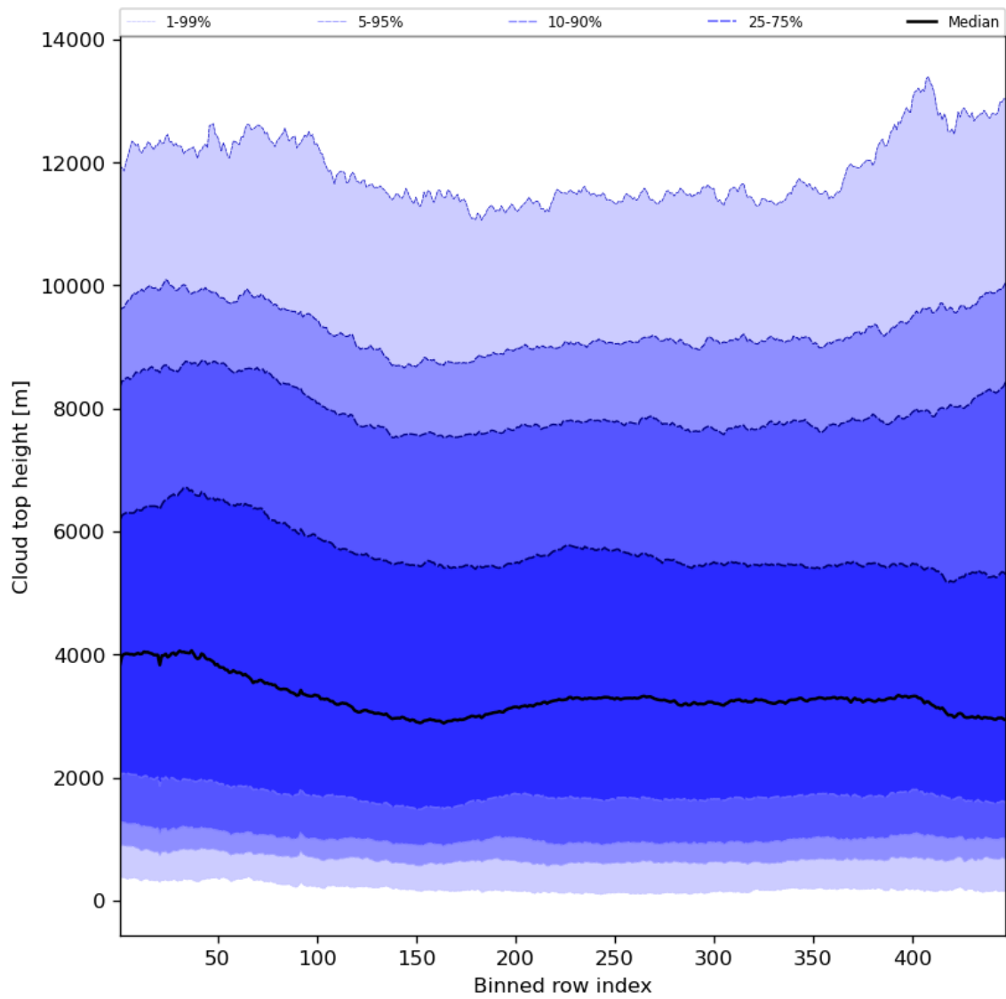
Figure 56: Along track statistics of “Cloud top height” for 2024-03-01 to 2024-03-03
