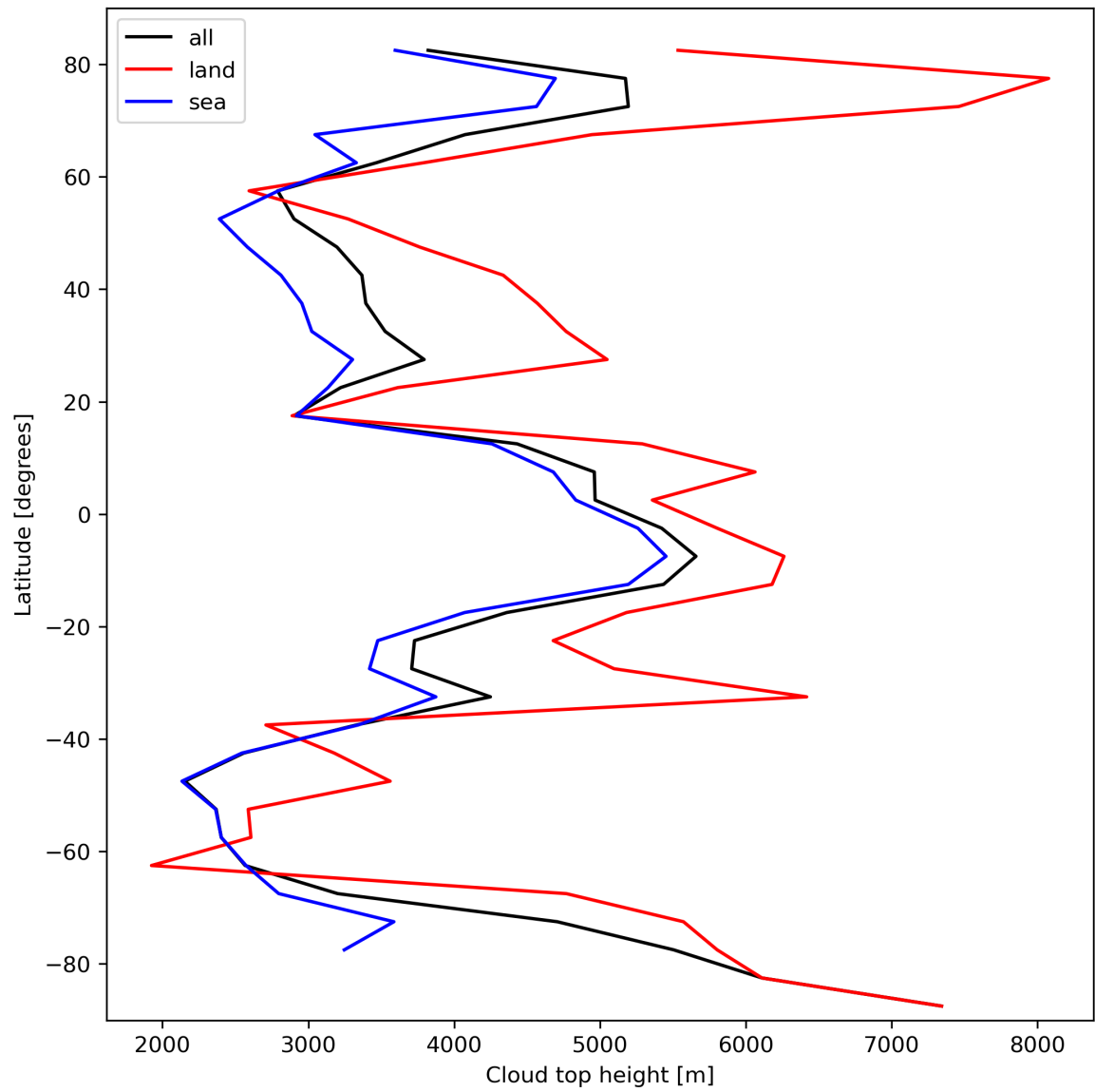
Figure 24: Zonal average of “Cloud top height” for 2024-03-01 to 2024-03-03.
