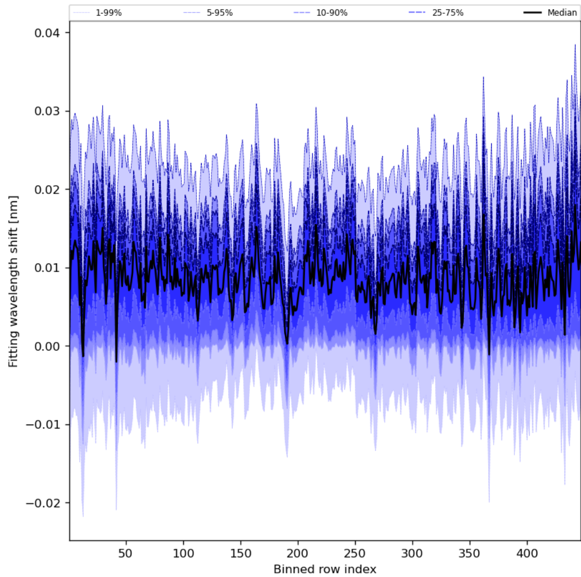
Figure 65: Along track statistics of “Fitting wavelength shift” for 2024-03-01 to 2024-03-03
