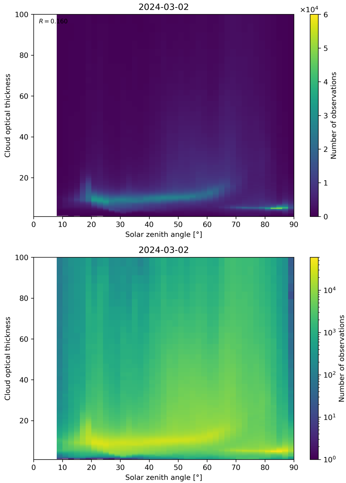
Figure 103: Scatter density plot of “Solar zenith angle” against “Cloud optical thickness” for 2024-03-01 to 2024-03-03.
