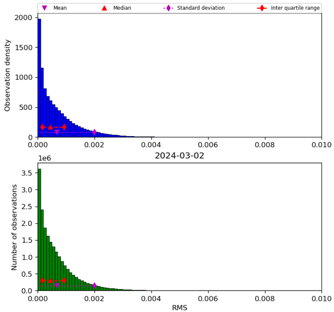
Figure 47: Histogram of “RMS” for 2024-03-01 to 2024-03-03
