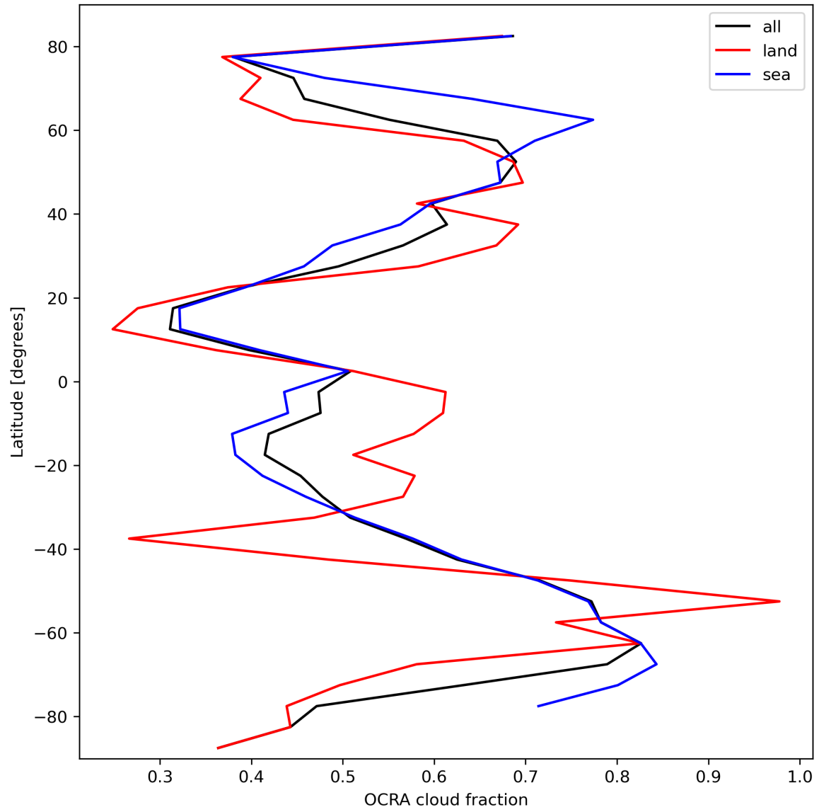
Figure 34: Zonal average of “OCRA cloud fraction” for 2024-03-04 to 2024-03-06.
