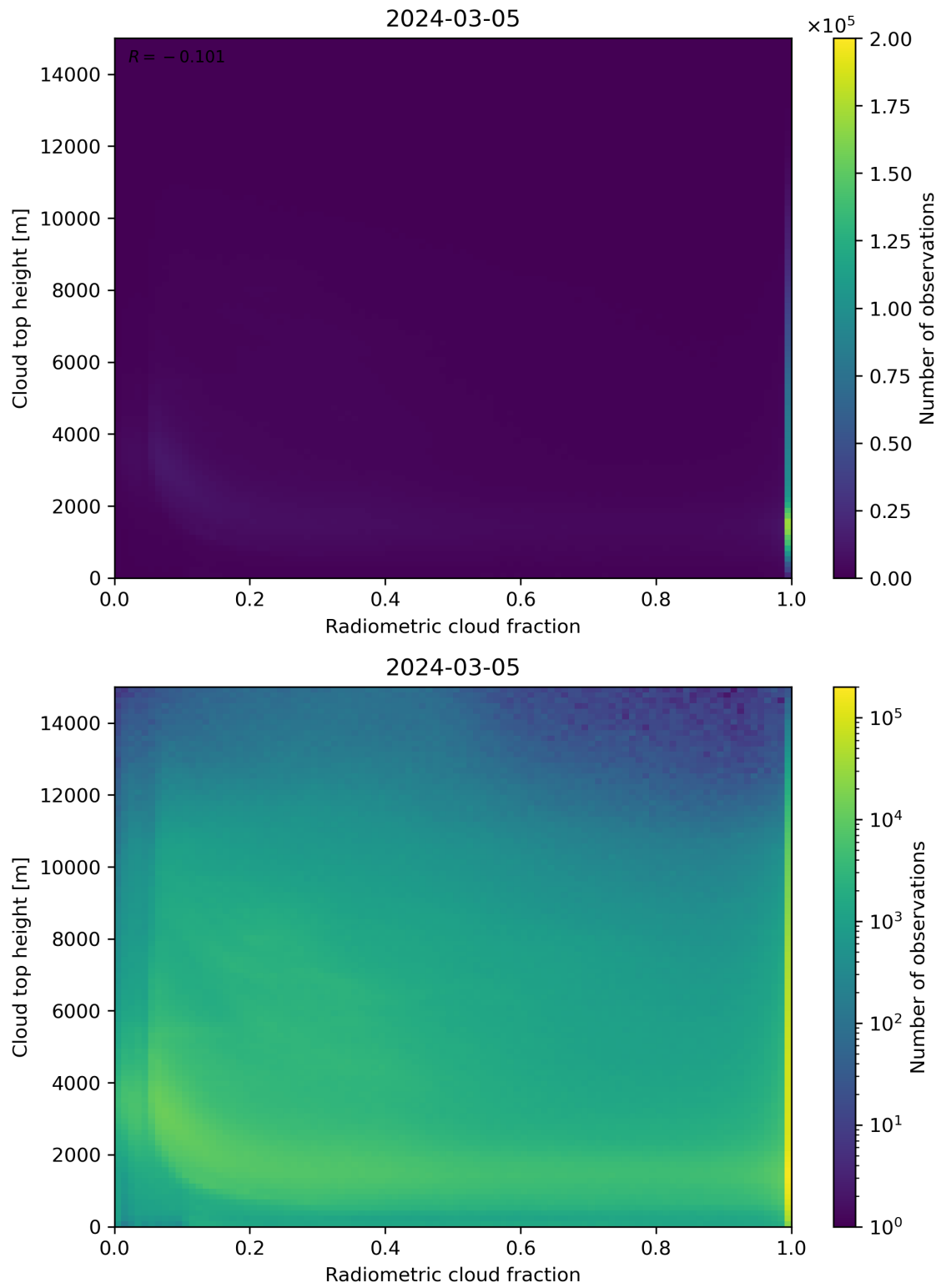
Figure 76: Scatter density plot of “Radiometric cloud fraction” against “Cloud top height” for 2024-03-04 to 2024-03-06.
