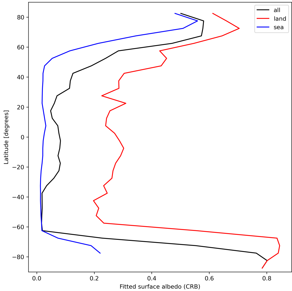
Figure 30: Zonal average of “Fitted surface albedo (CRB)” for 2024-03-04 to 2024-03-06.
