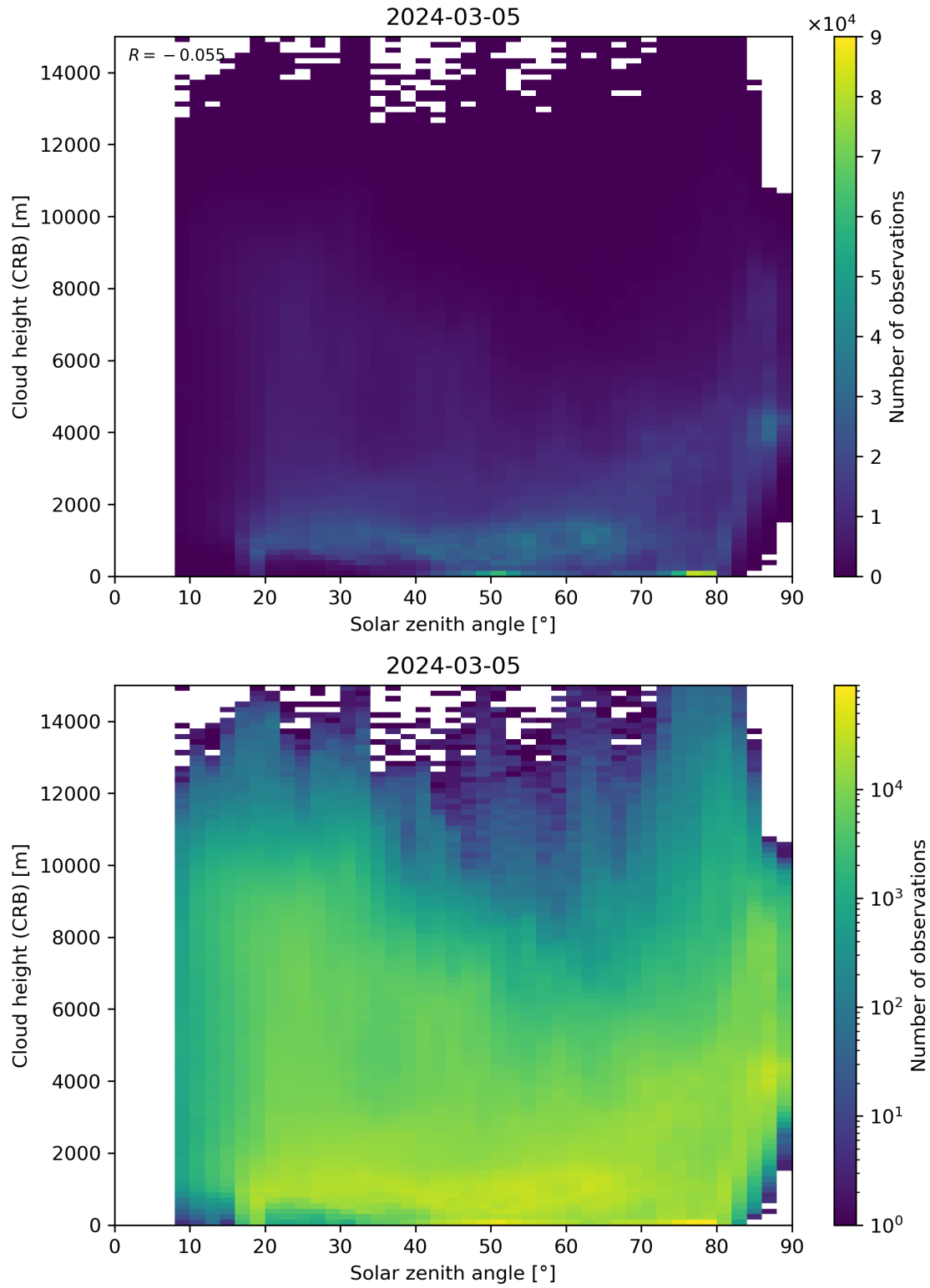
Figure 102: Scatter density plot of “Solar zenith angle” against “Cloud height (CRB)” for 2024-03-04 to 2024-03-06.
