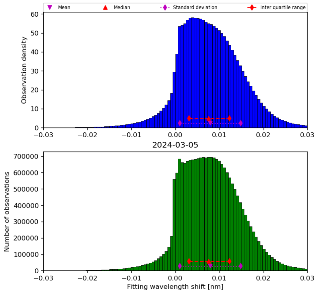
Figure 49: Histogram of “Fitting wavelength shift” for 2024-03-04 to 2024-03-06
