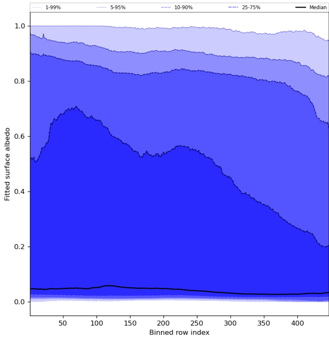
Figure 61: Along track statistics of “Fitted surface albedo” for 2024-03-04 to 2024-03-06
