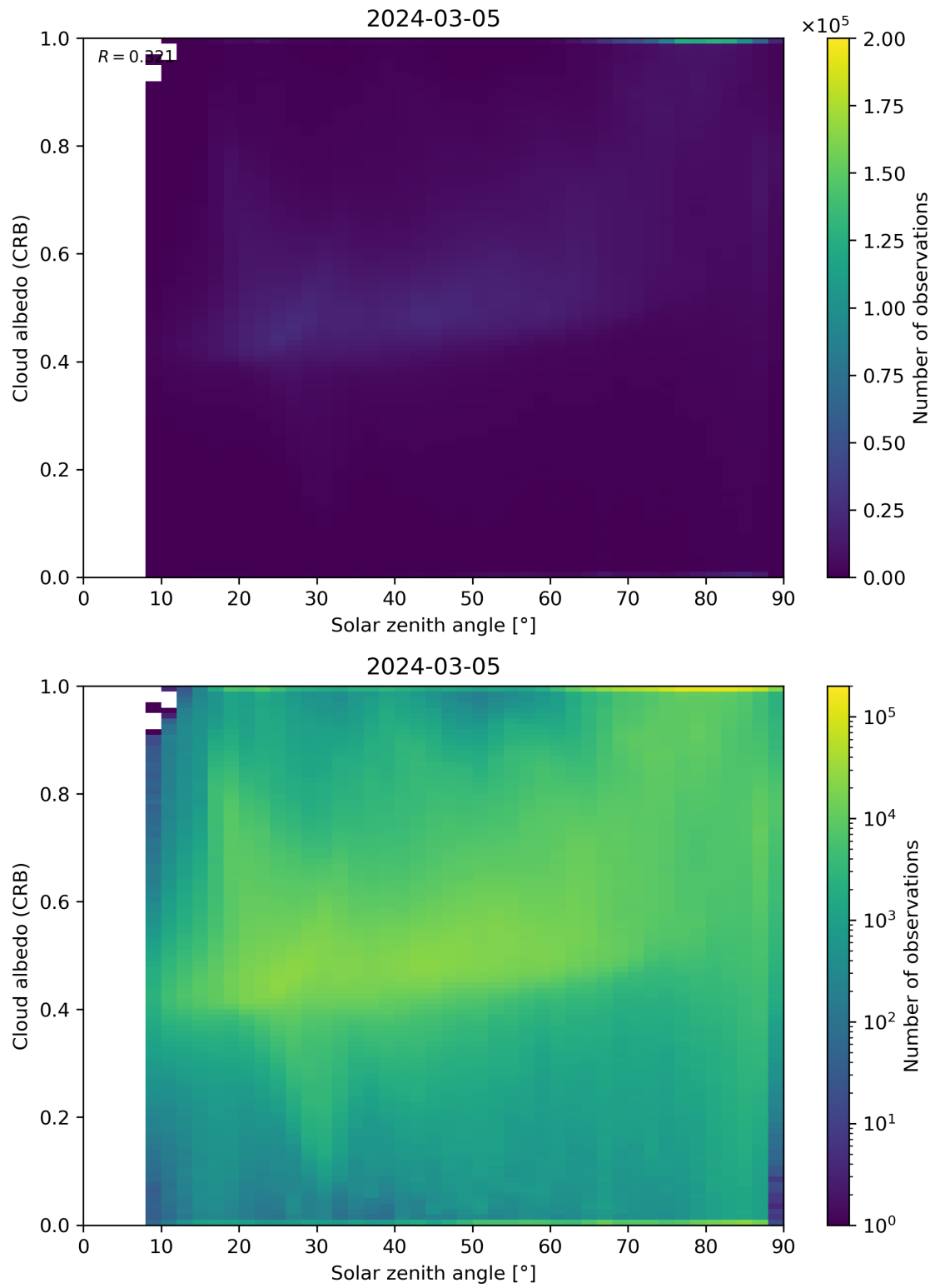
Figure 98: Scatter density plot of “Solar zenith angle” against “Cloud albedo (CRB)” for 2024-03-04 to 2024-03-06.
