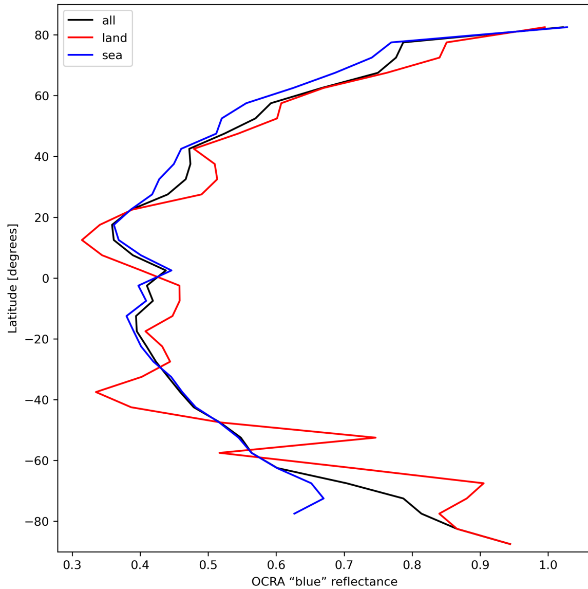
Figure 35: Zonal average of “OCRA “blue” reflectance” for 2024-03-04 to 2024-03-06.
