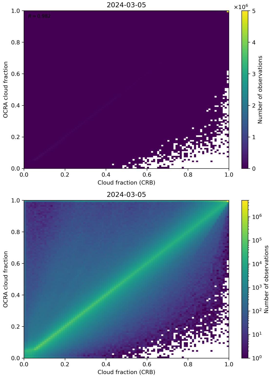
Figure 78: Scatter density plot of “Cloud fraction (CRB)” against “OCRA cloud fraction” for 2024-03-04 to 2024-03-06.
