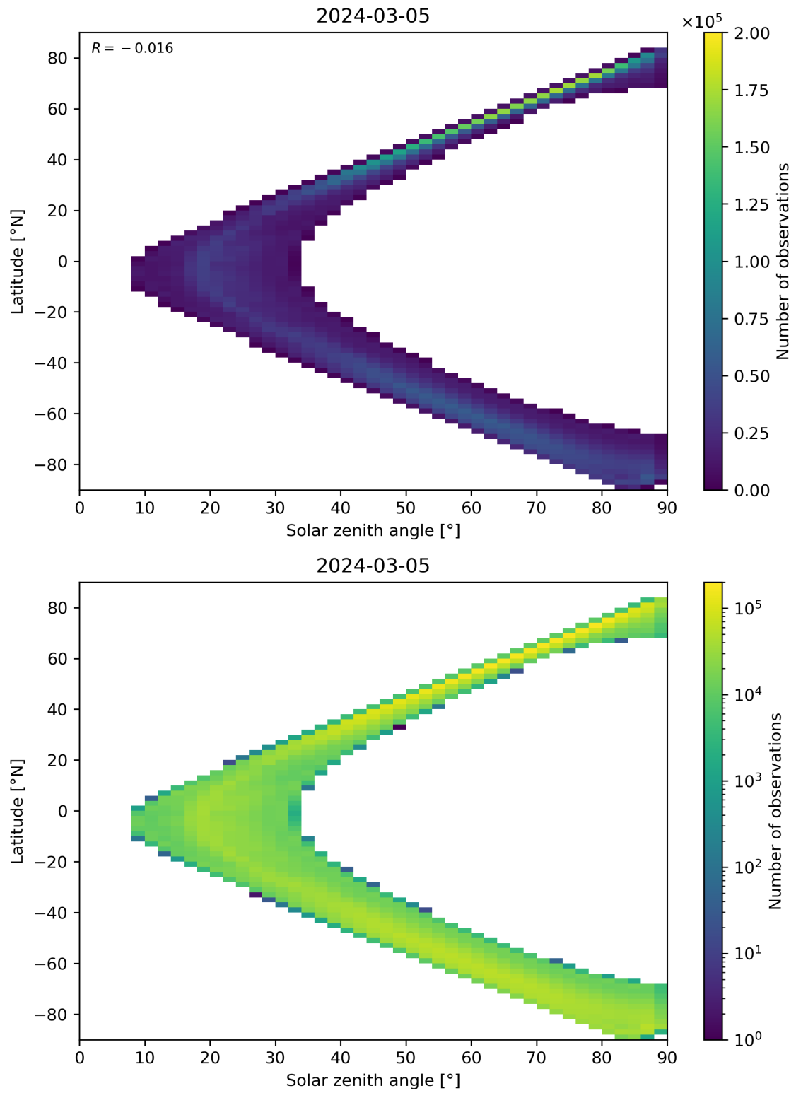
Figure 105: Scatter density plot of “Solar zenith angle” against “Latitude” for 2024-03-04 to 2024-03-06.
