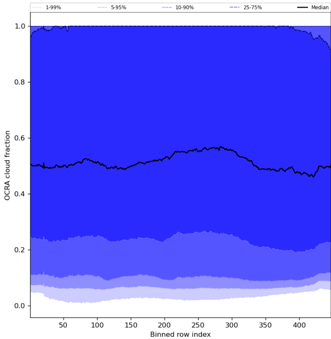
Figure 66: Along track statistics of “OCRA cloud fraction” for 2024-03-04 to 2024-03-06
