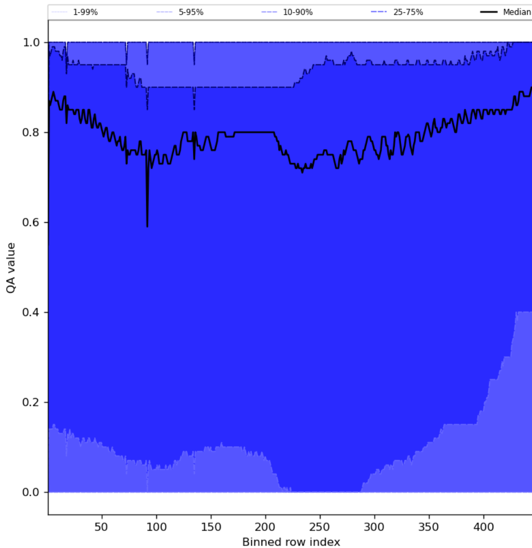
Figure 54: Along track statistics of “QA value” for 2024-03-04 to 2024-03-06
