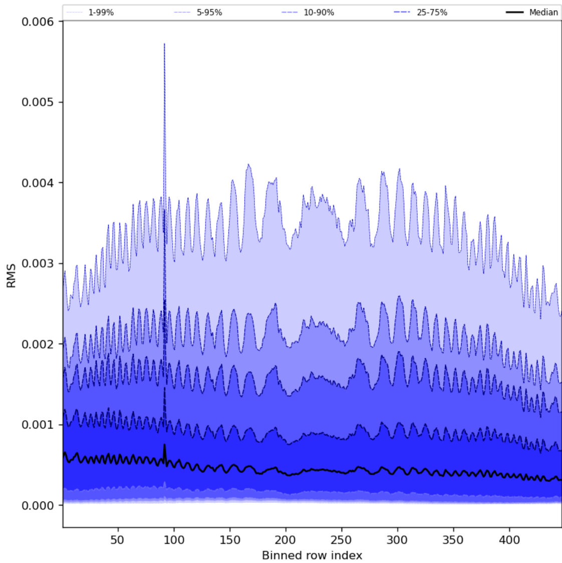
Figure 63: Along track statistics of “RMS” for 2024-03-04 to 2024-03-06
