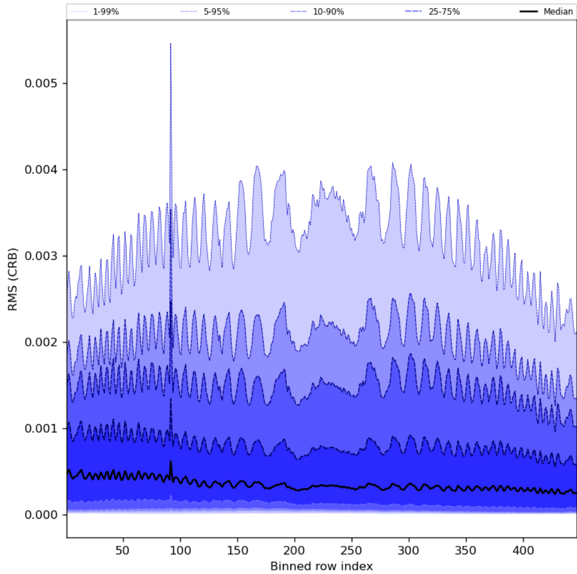
Figure 64: Along track statistics of “RMS (CRB)” for 2024-03-04 to 2024-03-06
