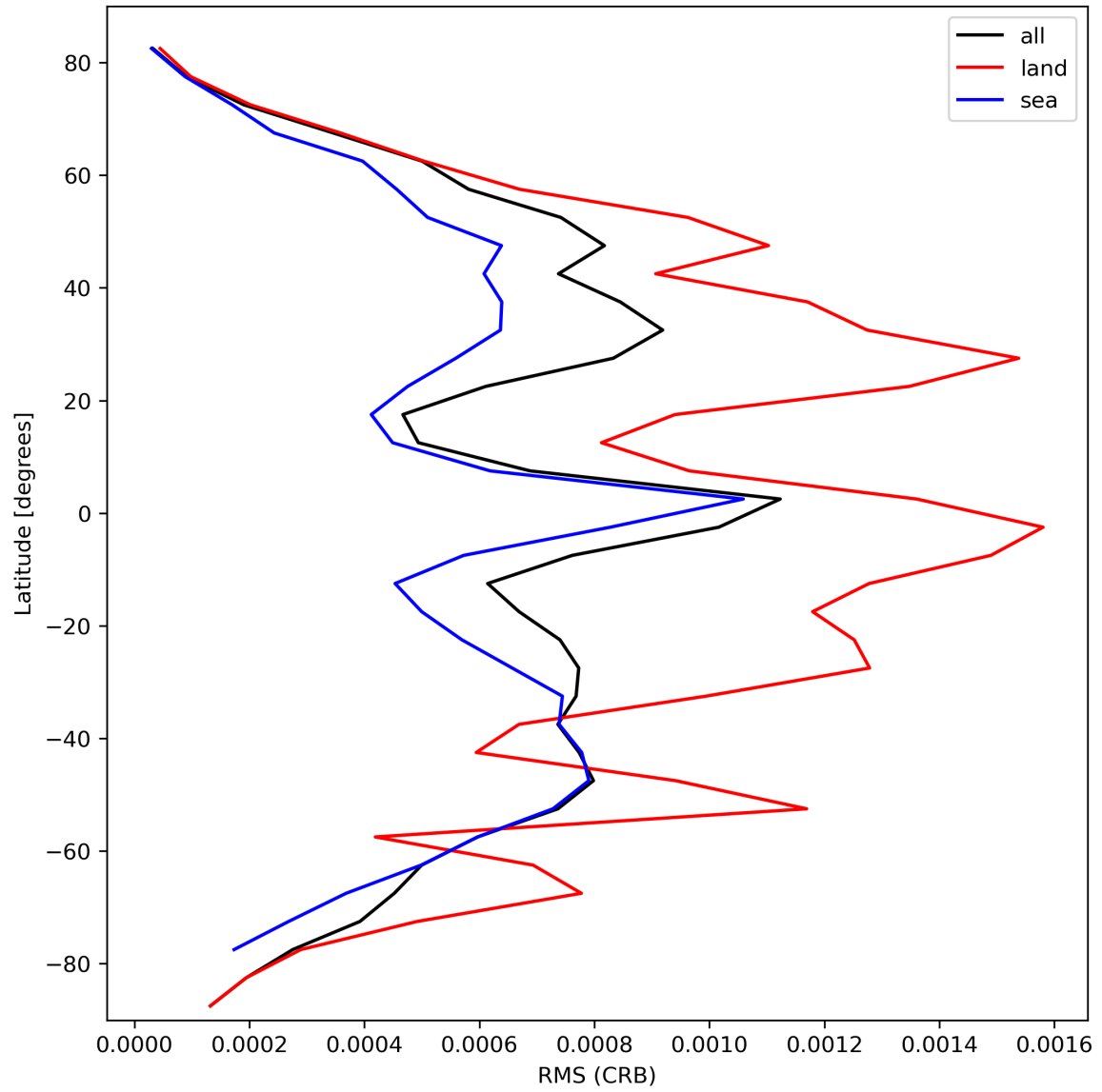
Figure 32: Zonal average of “RMS (CRB)” for 2024-03-04 to 2024-03-06.
