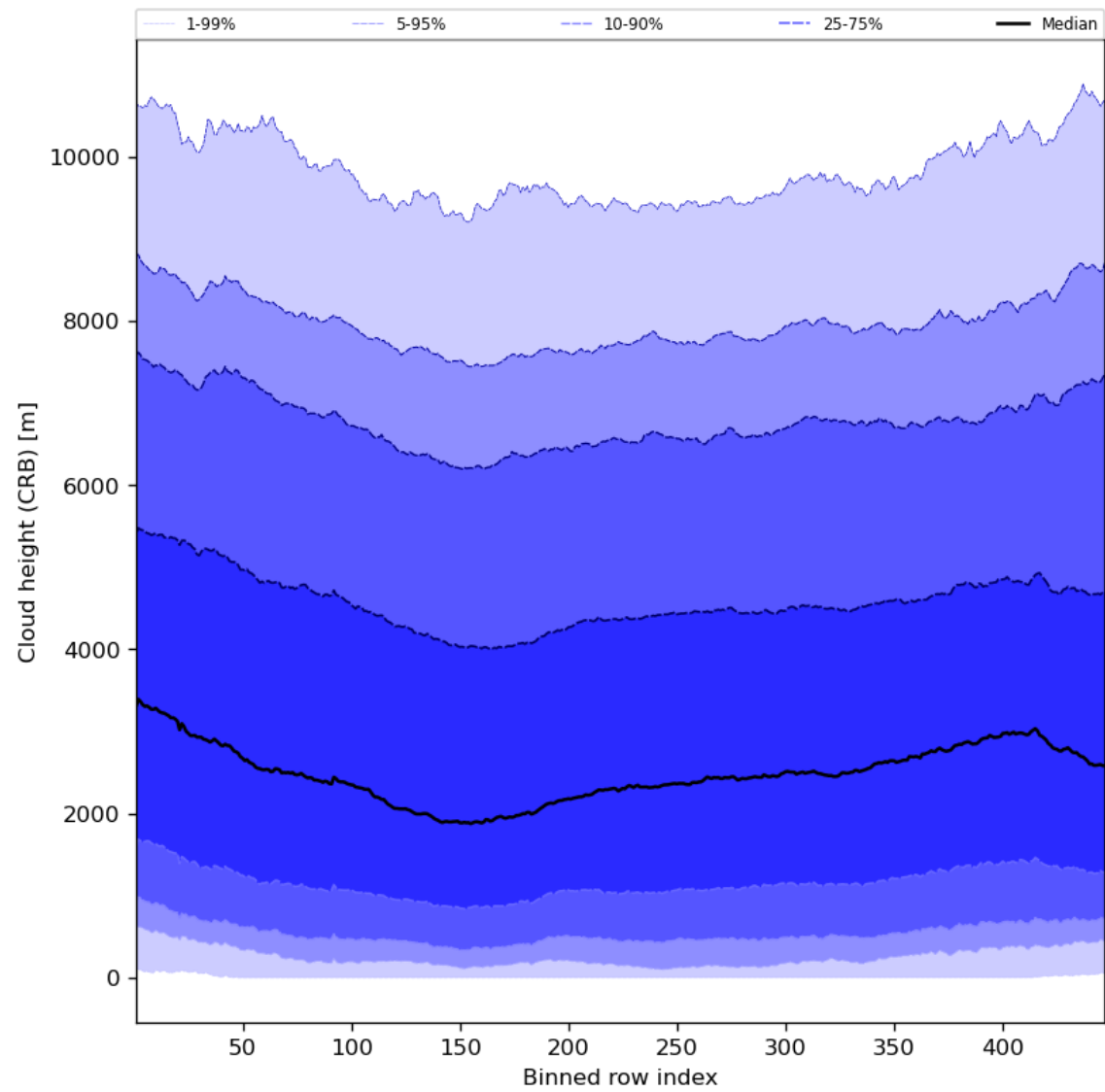
Figure 59: Along track statistics of “Cloud height (CRB)” for 2024-03-04 to 2024-03-06
