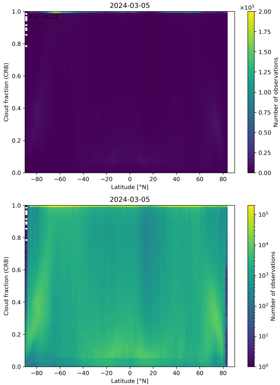
Figure 94: Scatter density plot of “Latitude” against “Cloud fraction (CRB)” for 2024-03-04 to 2024-03-06.
