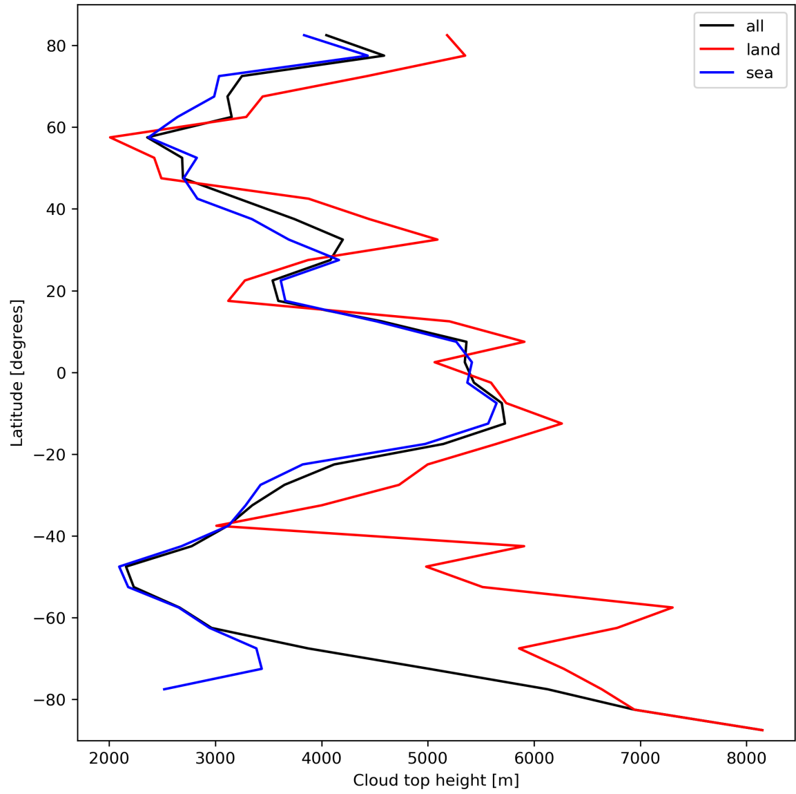
Figure 24: Zonal average of “Cloud top height” for 2024-03-04 to 2024-03-06.
