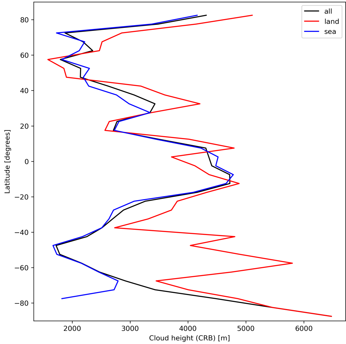
Figure 27: Zonal average of “Cloud height (CRB)” for 2024-03-04 to 2024-03-06.
