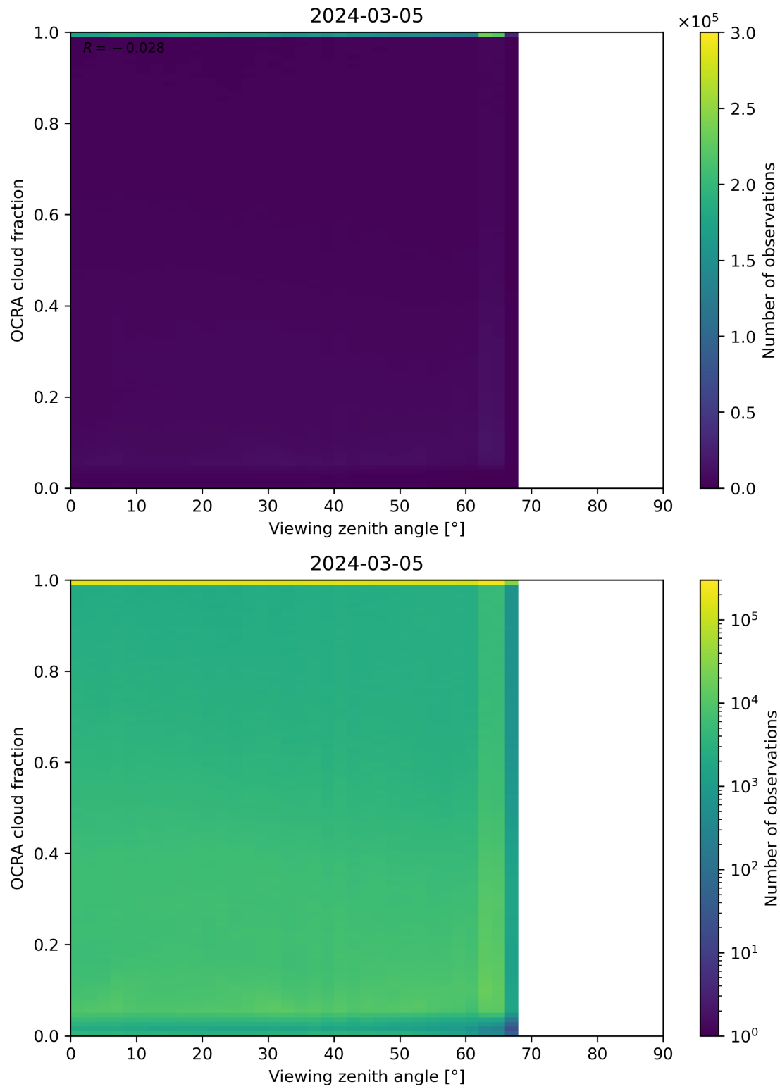
Figure 108: Scatter density plot of “Viewing zenith angle” against “OCRA cloud fraction” for 2024-03-04 to 2024-03-06.
