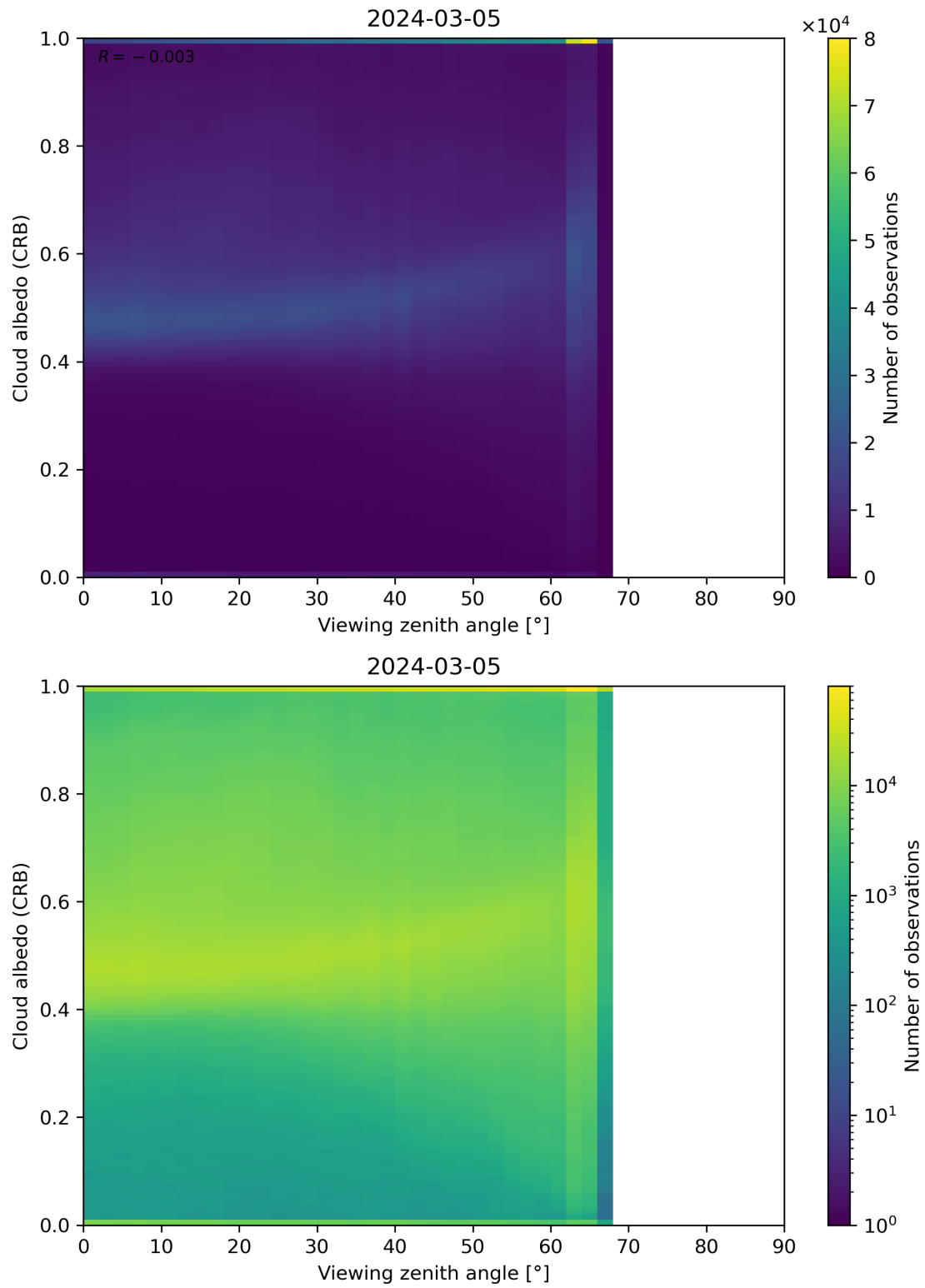
Figure 106: Scatter density plot of “Viewing zenith angle” against “Cloud albedo (CRB)” for 2024-03-04 to 2024-03-06.
