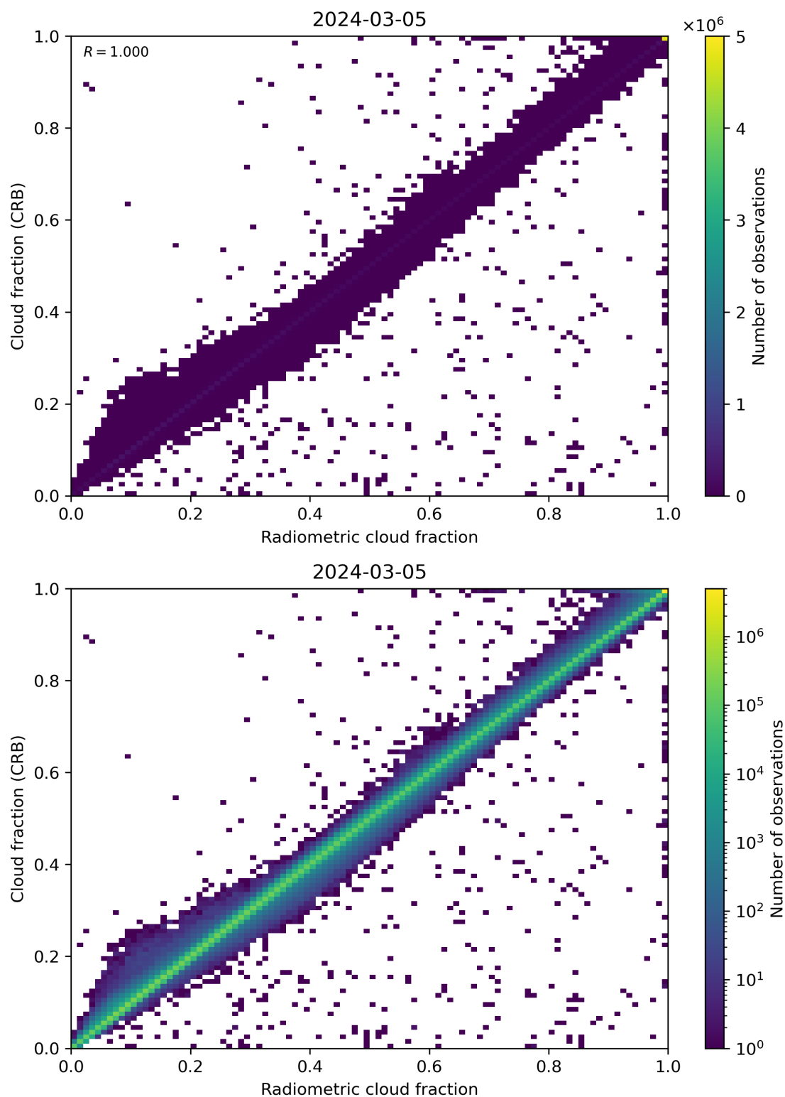
Figure 73: Scatter density plot of “Radiometric cloud fraction” against “Cloud fraction (CRB)” for 2024-03-04 to 2024-03-06.
