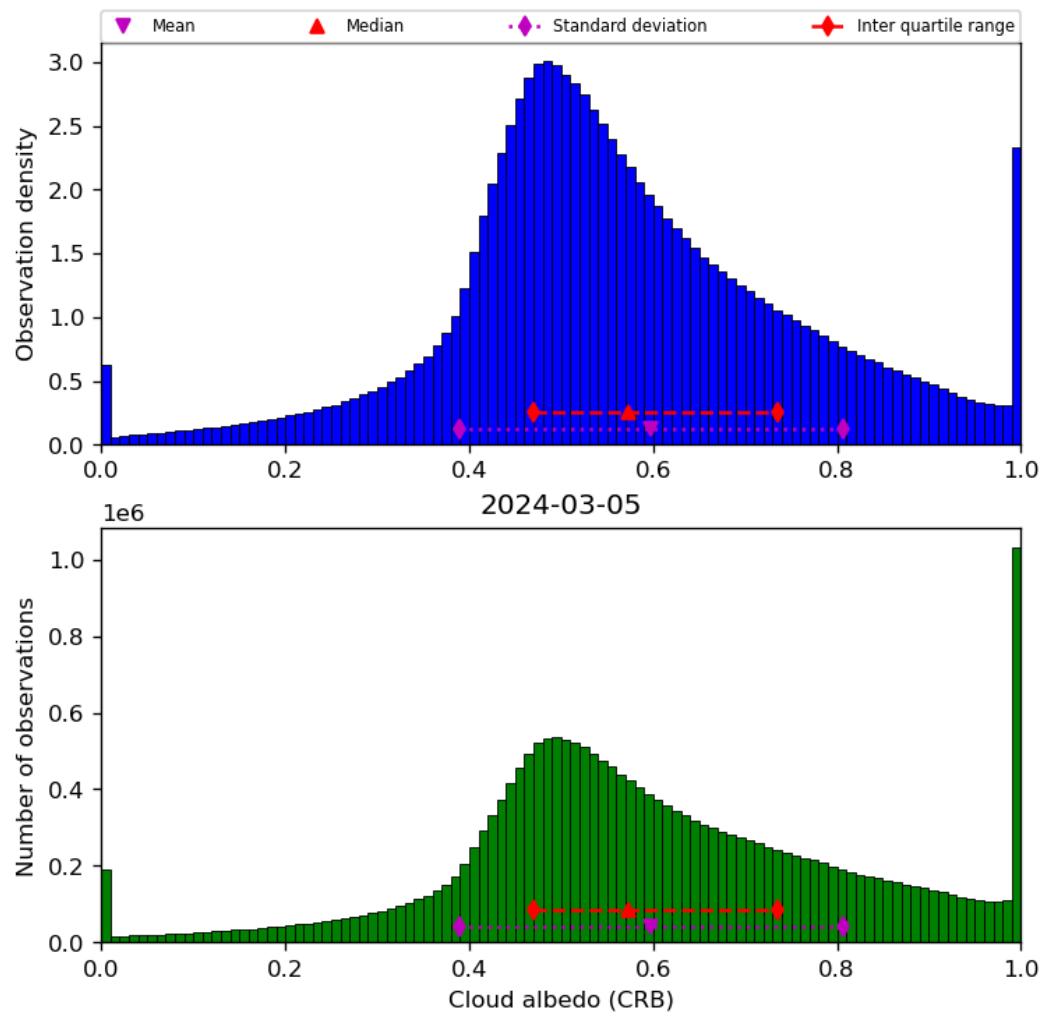
Figure 44: Histogram of “Cloud albedo (CRB)” for 2024-03-04 to 2024-03-06
