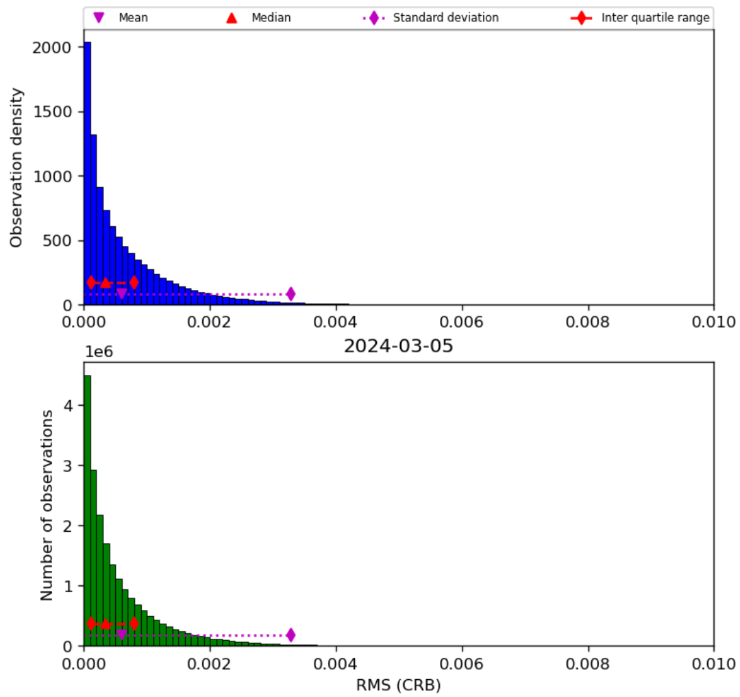
Figure 48: Histogram of “RMS (CRB)” for 2024-03-04 to 2024-03-06
