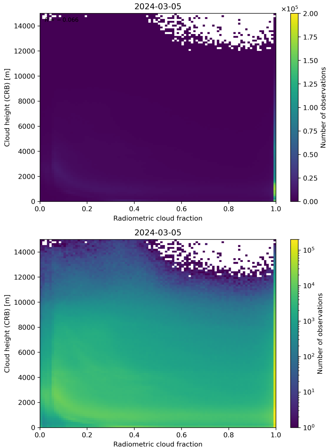
Figure 74: Scatter density plot of “Radiometric cloud fraction” against “Cloud height (CRB)” for 2024-03-04 to 2024-03-06.
