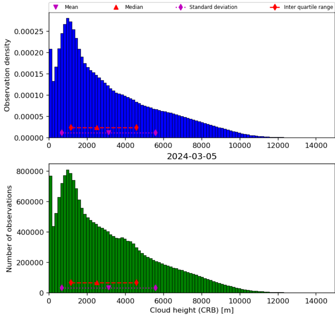
Figure 43: Histogram of “Cloud height (CRB)” for 2024-03-04 to 2024-03-06
