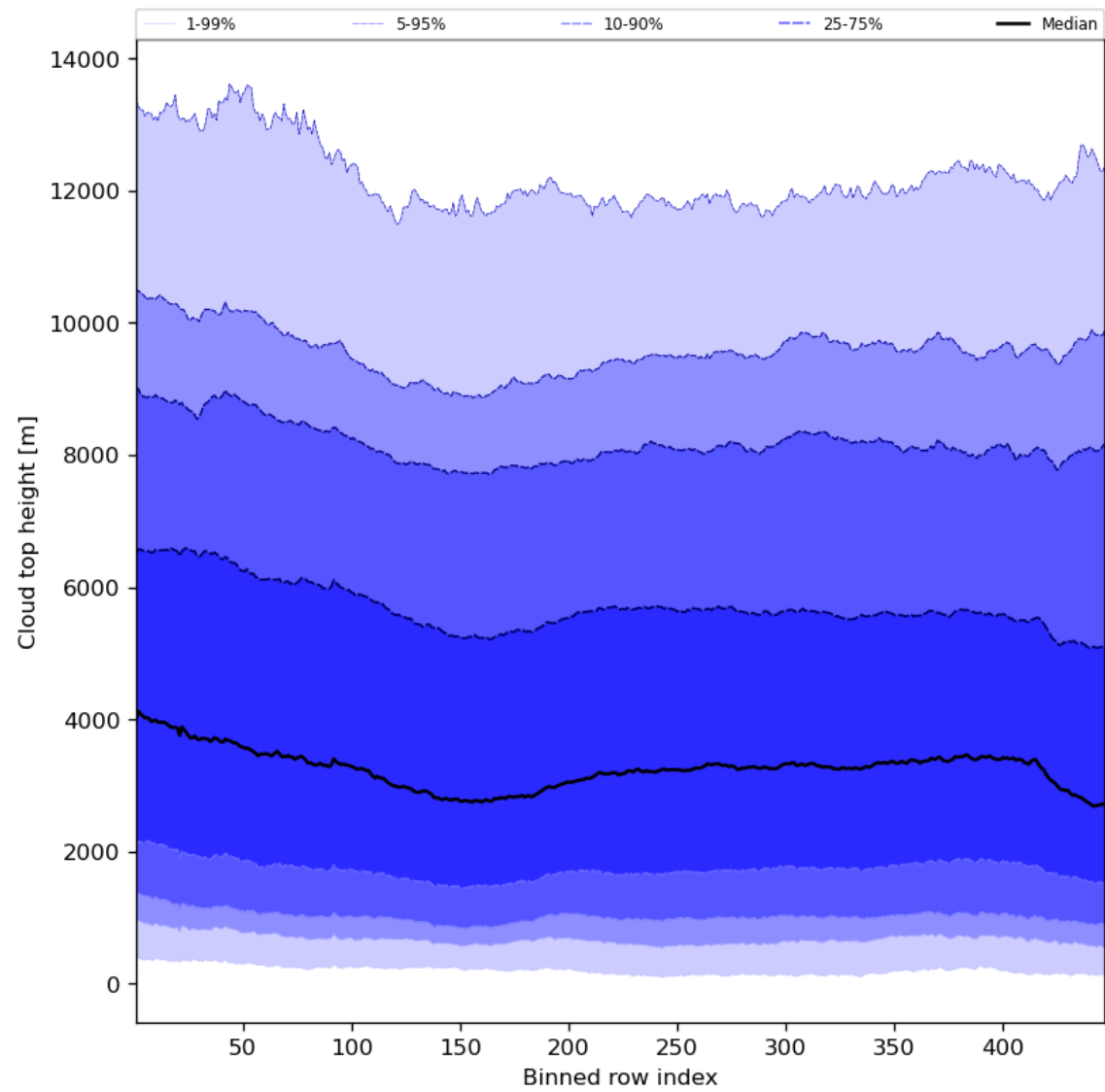
Figure 56: Along track statistics of “Cloud top height” for 2024-03-04 to 2024-03-06
