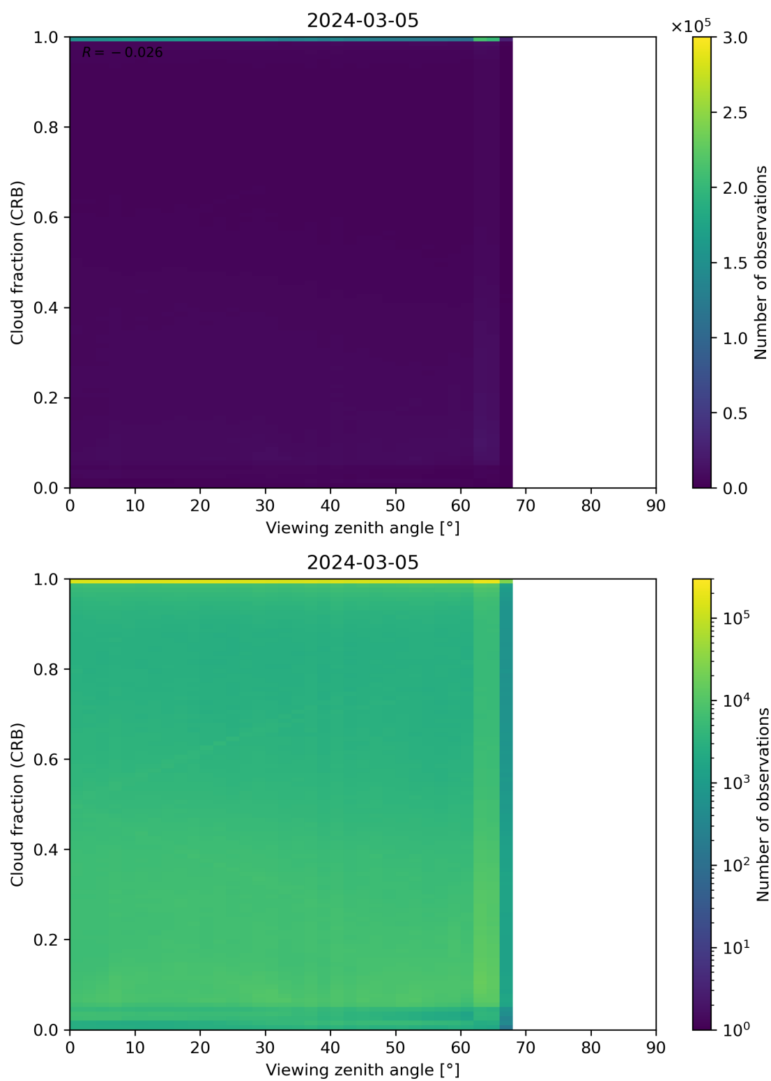
Figure 109: Scatter density plot of “Viewing zenith angle” against “Cloud fraction (CRB)” for 2024-03-04 to 2024-03-06.
