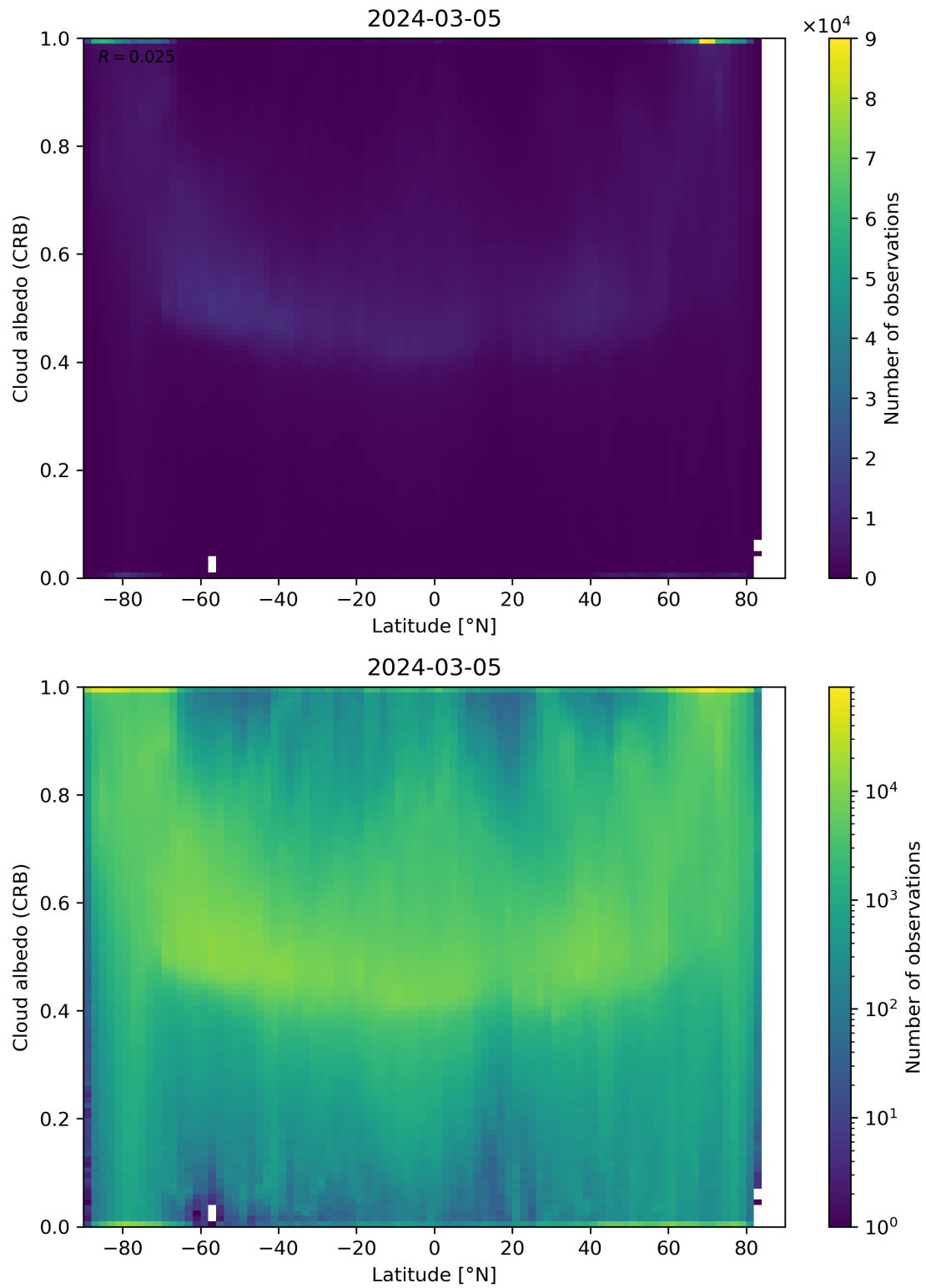
Figure 91: Scatter density plot of “Latitude” against “Cloud albedo (CRB)” for 2024-03-04 to 2024-03-06.
