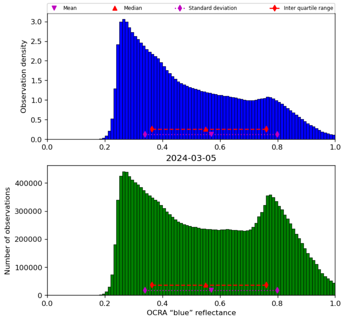
Figure 51: Histogram of “OCRA “blue” reflectance” for 2024-03-04 to 2024-03-06
