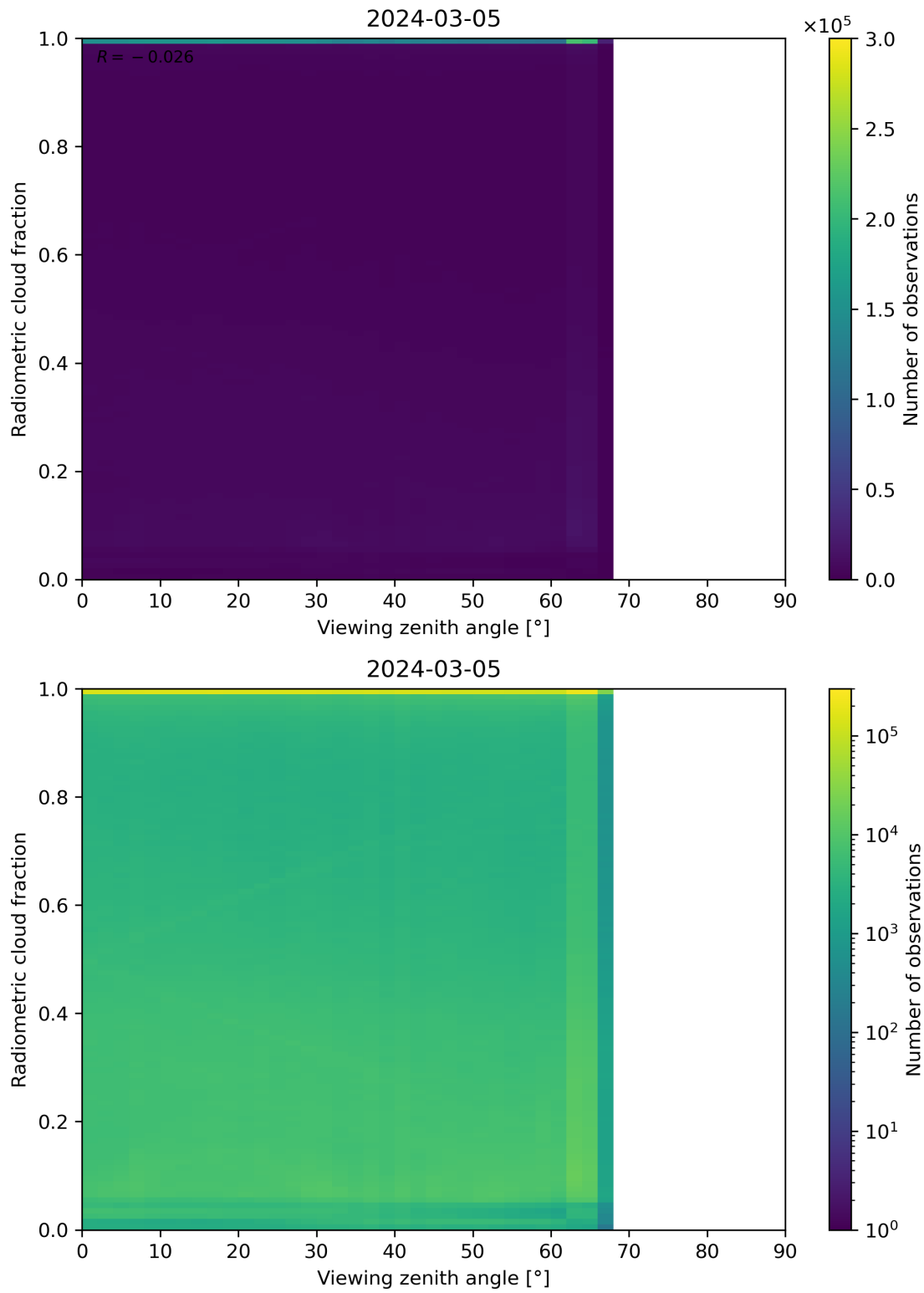
Figure 107: Scatter density plot of “Viewing zenith angle” against “Radiometric cloud fraction” for 2024-03-04 to 2024-03-06.
