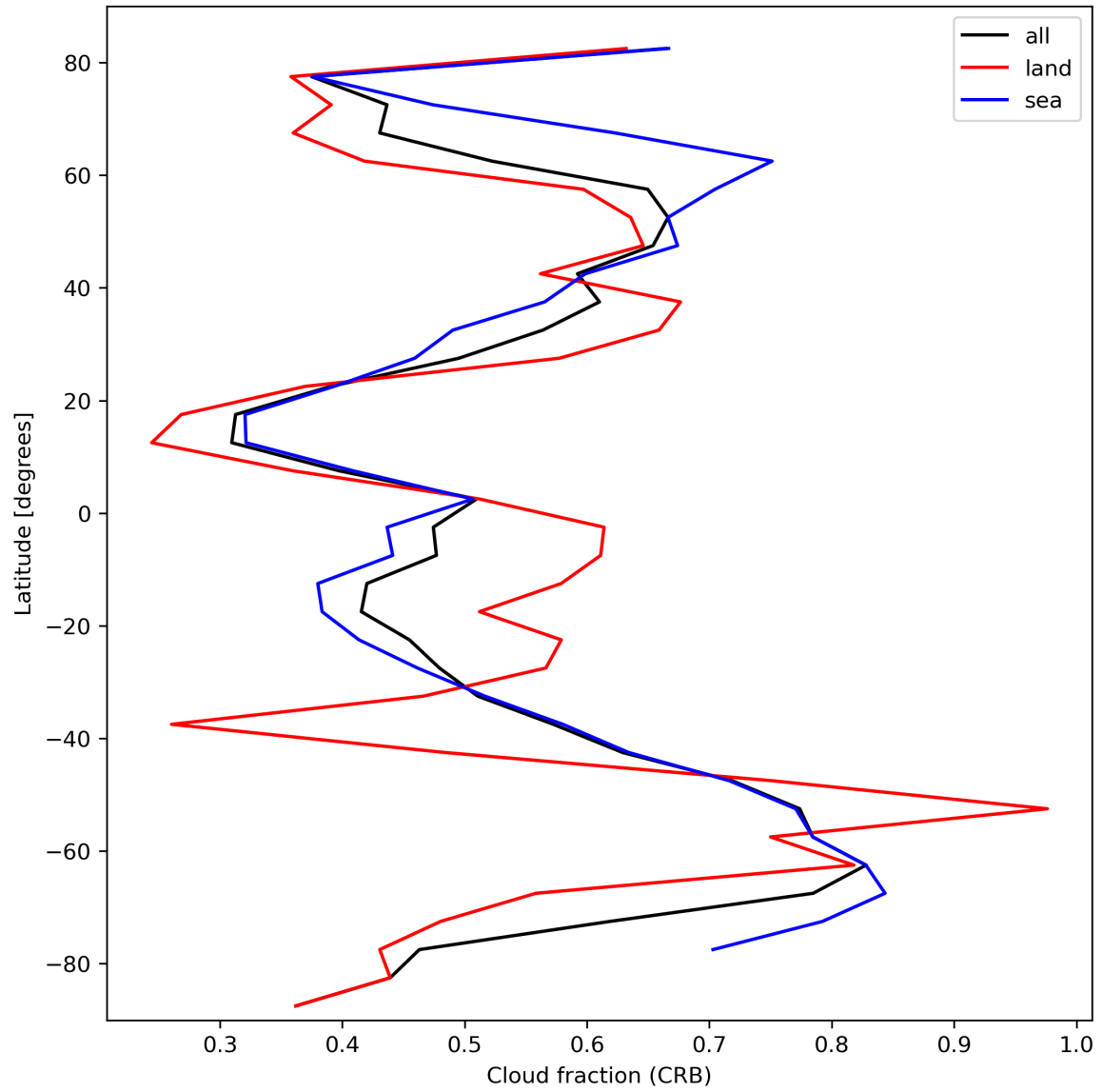
Figure 26: Zonal average of “Cloud fraction (CRB)” for 2024-03-04 to 2024-03-06.
