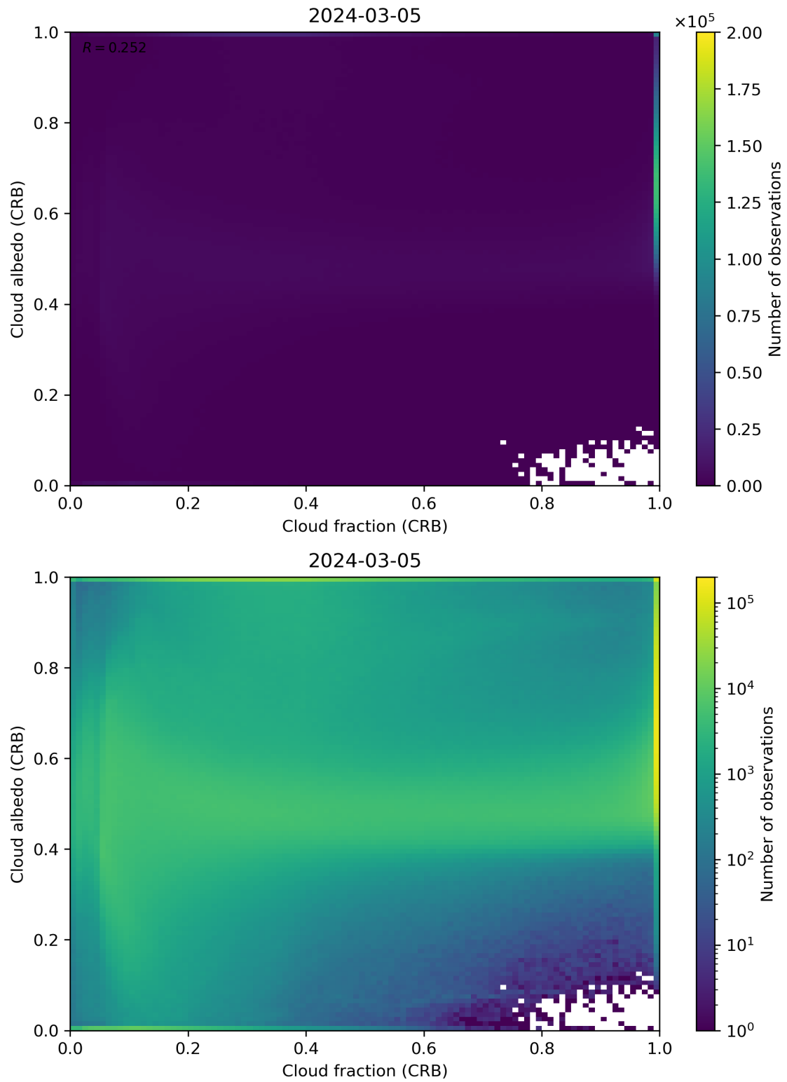
Figure 77: Scatter density plot of “Cloud fraction (CRB)” against “Cloud albedo (CRB)” for 2024-03-04 to 2024-03-06.
