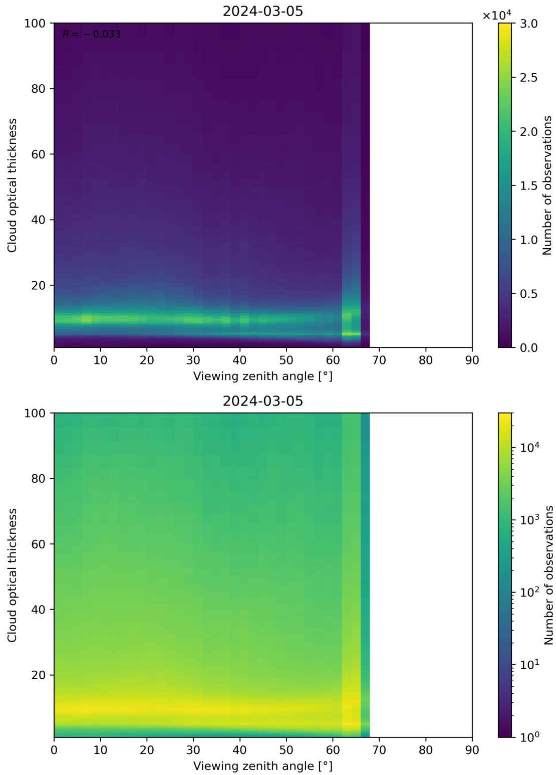
Figure 111: Scatter density plot of “Viewing zenith angle” against “Cloud optical thickness” for 2024-03-04 to 2024-03-06.
