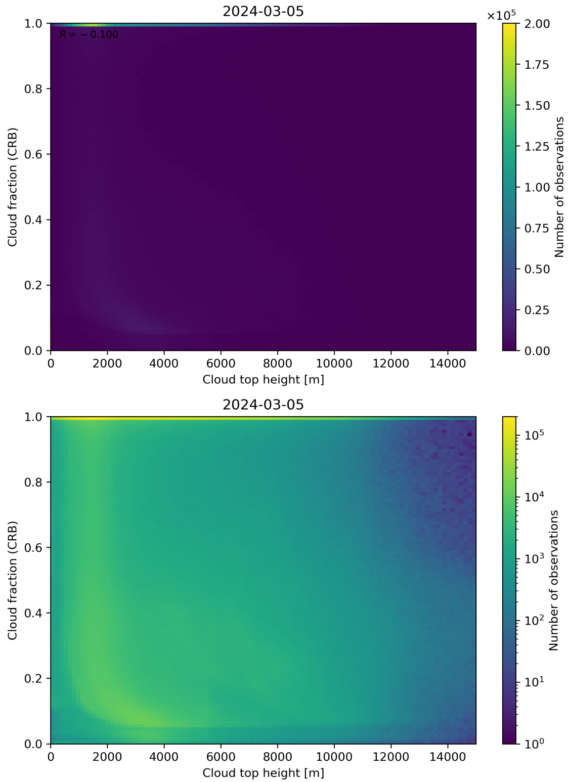
Figure 88: Scatter density plot of “Cloud top height” against “Cloud fraction (CRB)” for 2024-03-04 to 2024-03-06.
