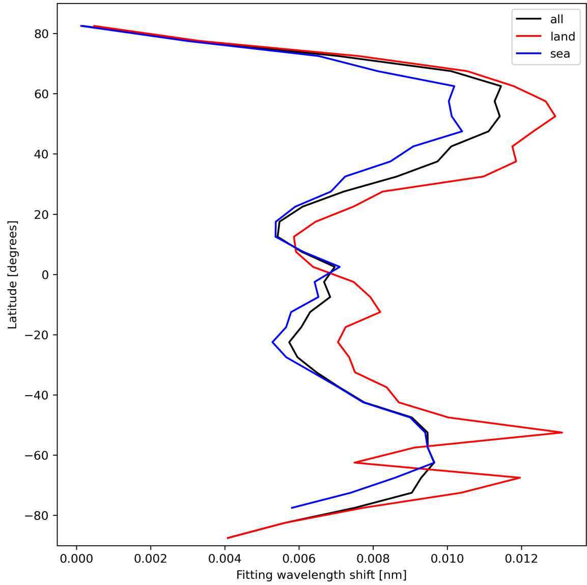
Figure 33: Zonal average of “Fitting wavelength shift” for 2024-03-04 to 2024-03-06.
