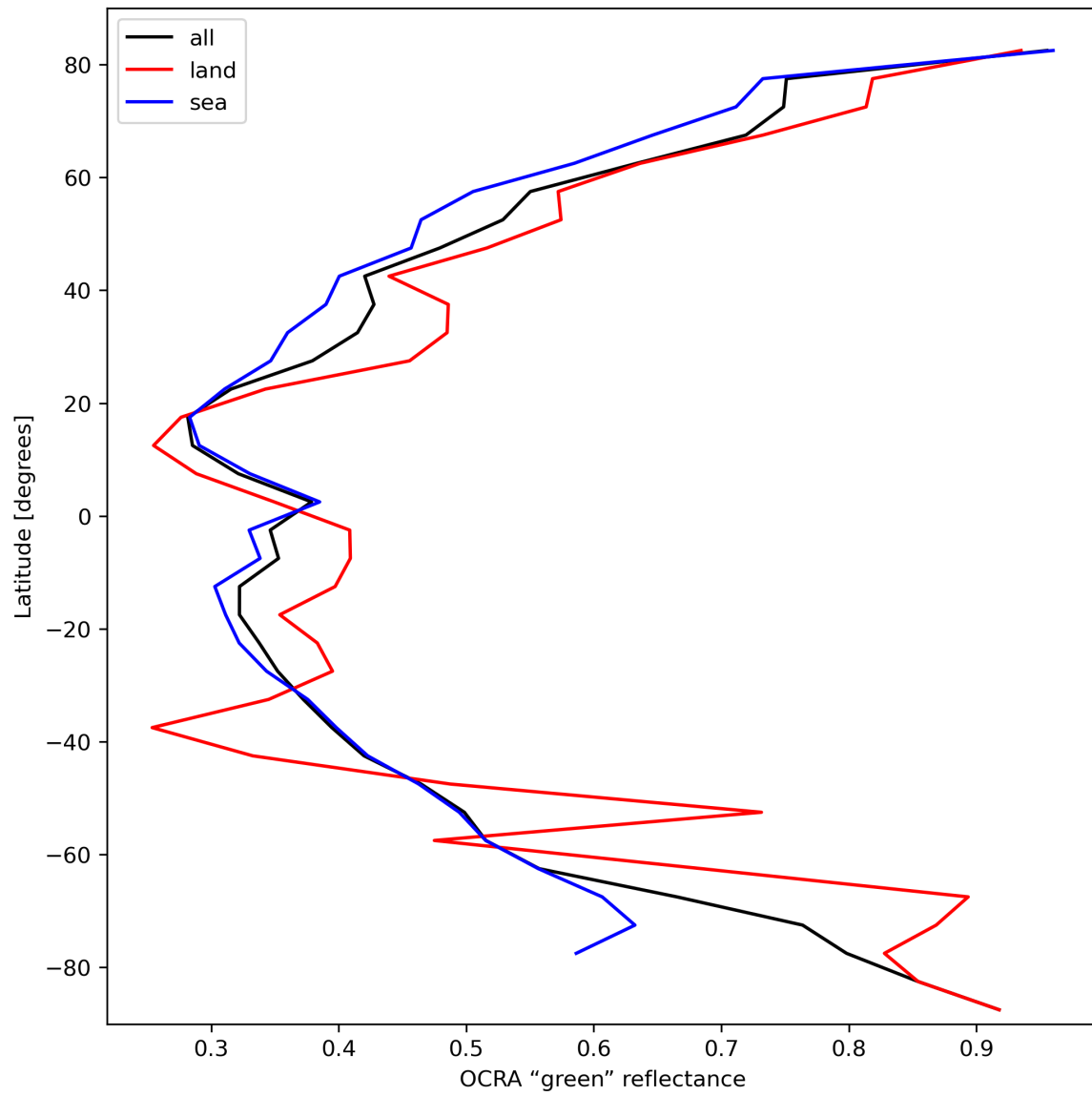
Figure 36: Zonal average of “OCRA “green” reflectance” for 2024-03-04 to 2024-03-06.
