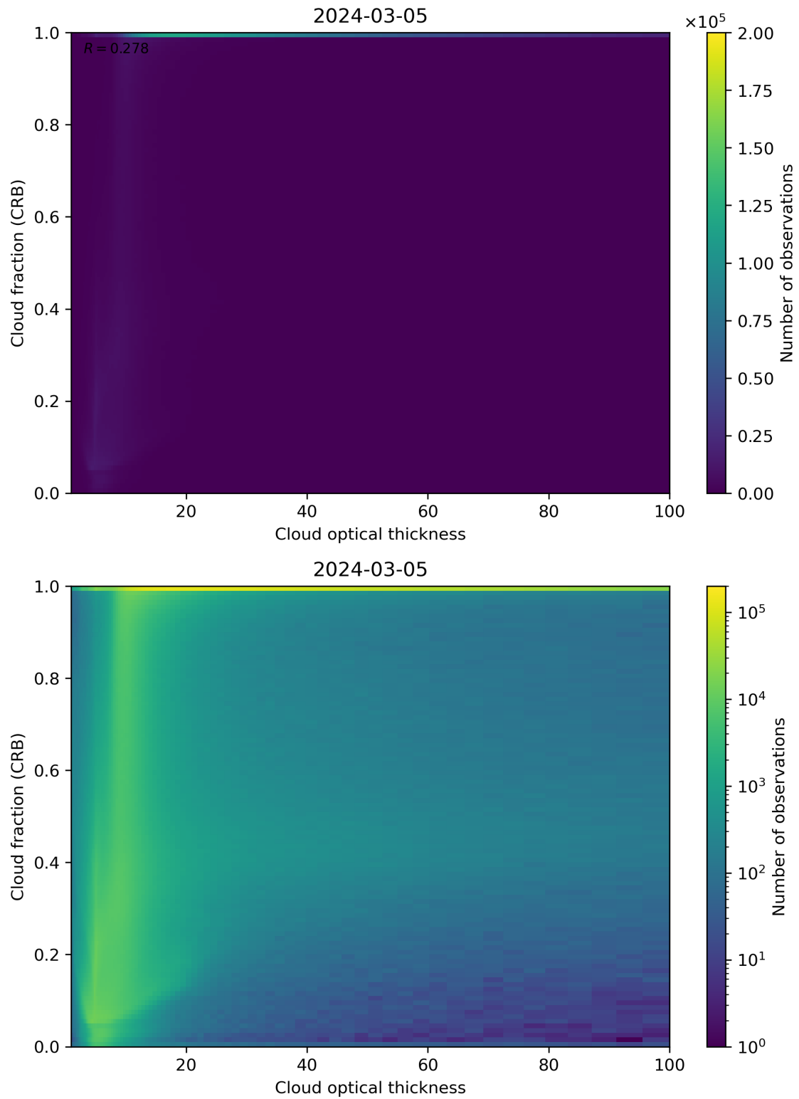
Figure 84: Scatter density plot of “Cloud optical thickness” against “Cloud fraction (CRB)” for 2024-03-04 to 2024-03-06.
