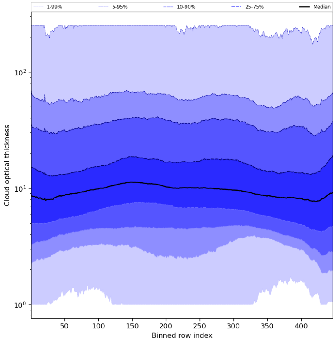
Figure 57: Along track statistics of “Cloud optical thickness” for 2024-03-04 to 2024-03-06
