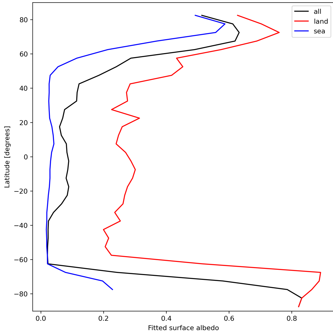
Figure 29: Zonal average of “Fitted surface albedo” for 2024-03-04 to 2024-03-06.
