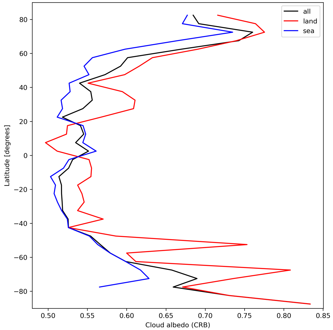
Figure 28: Zonal average of “Cloud albedo (CRB)” for 2024-03-04 to 2024-03-06.
