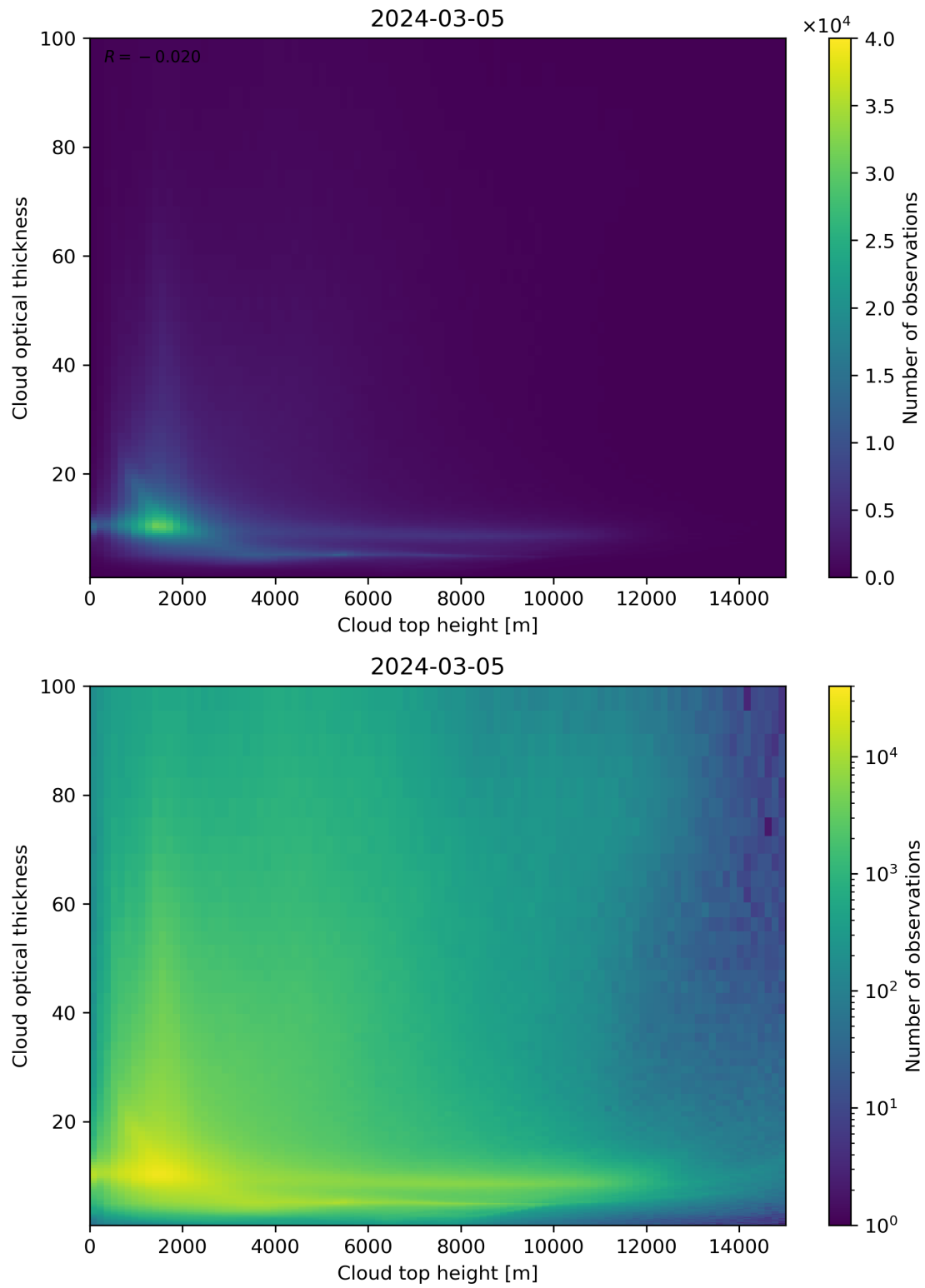
Figure 90: Scatter density plot of “Cloud top height” against “Cloud optical thickness” for 2024-03-04 to 2024-03-06.
