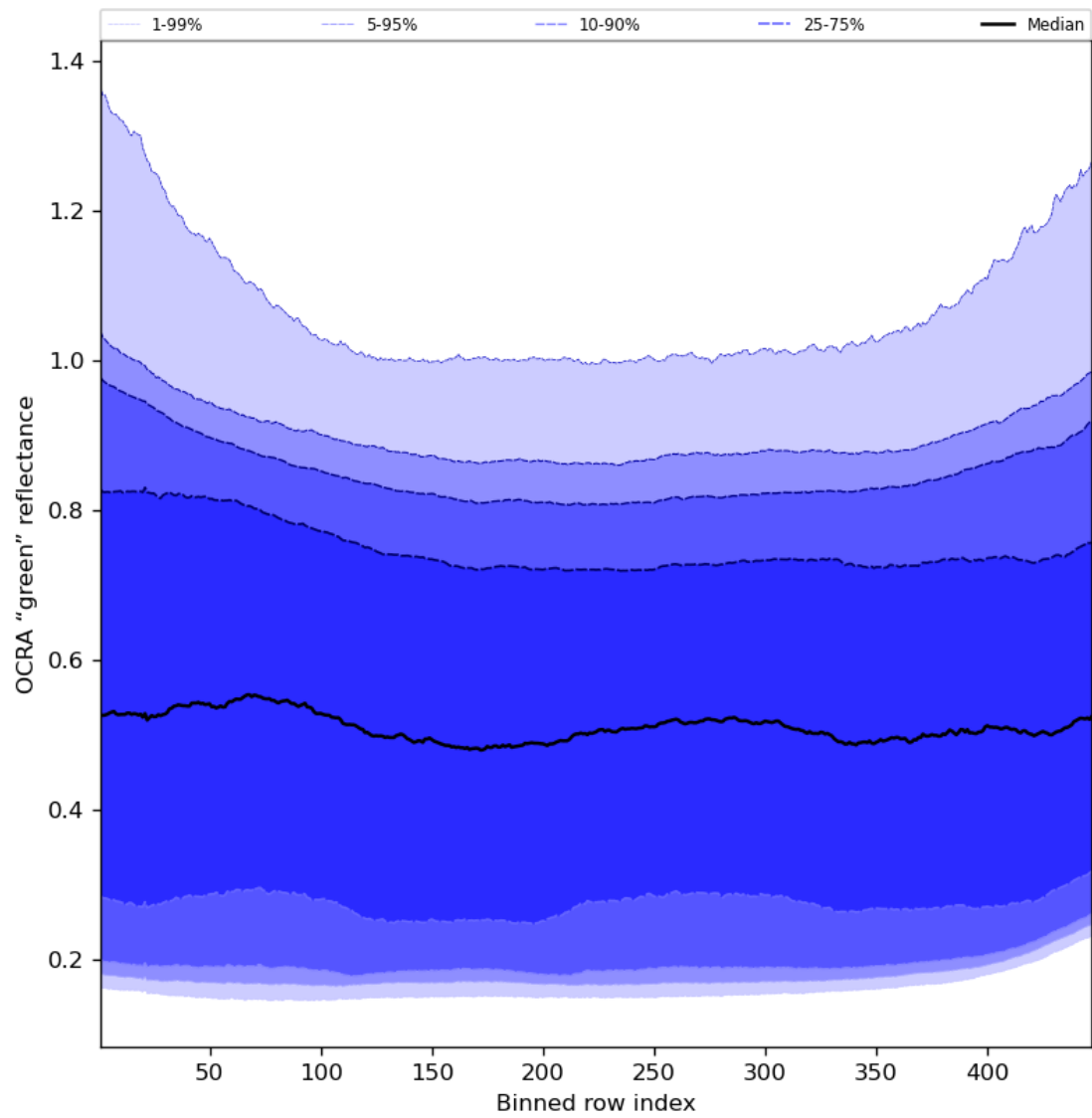
Figure 68: Along track statistics of "OCRA "green" reflectance" for 2024-03-04 to 2024-03-06
