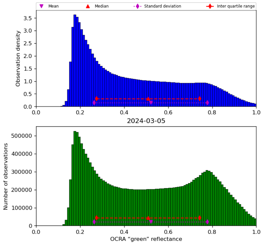
Figure 52: Histogram of “OCRA “green” reflectance” for 2024-03-04 to 2024-03-06
