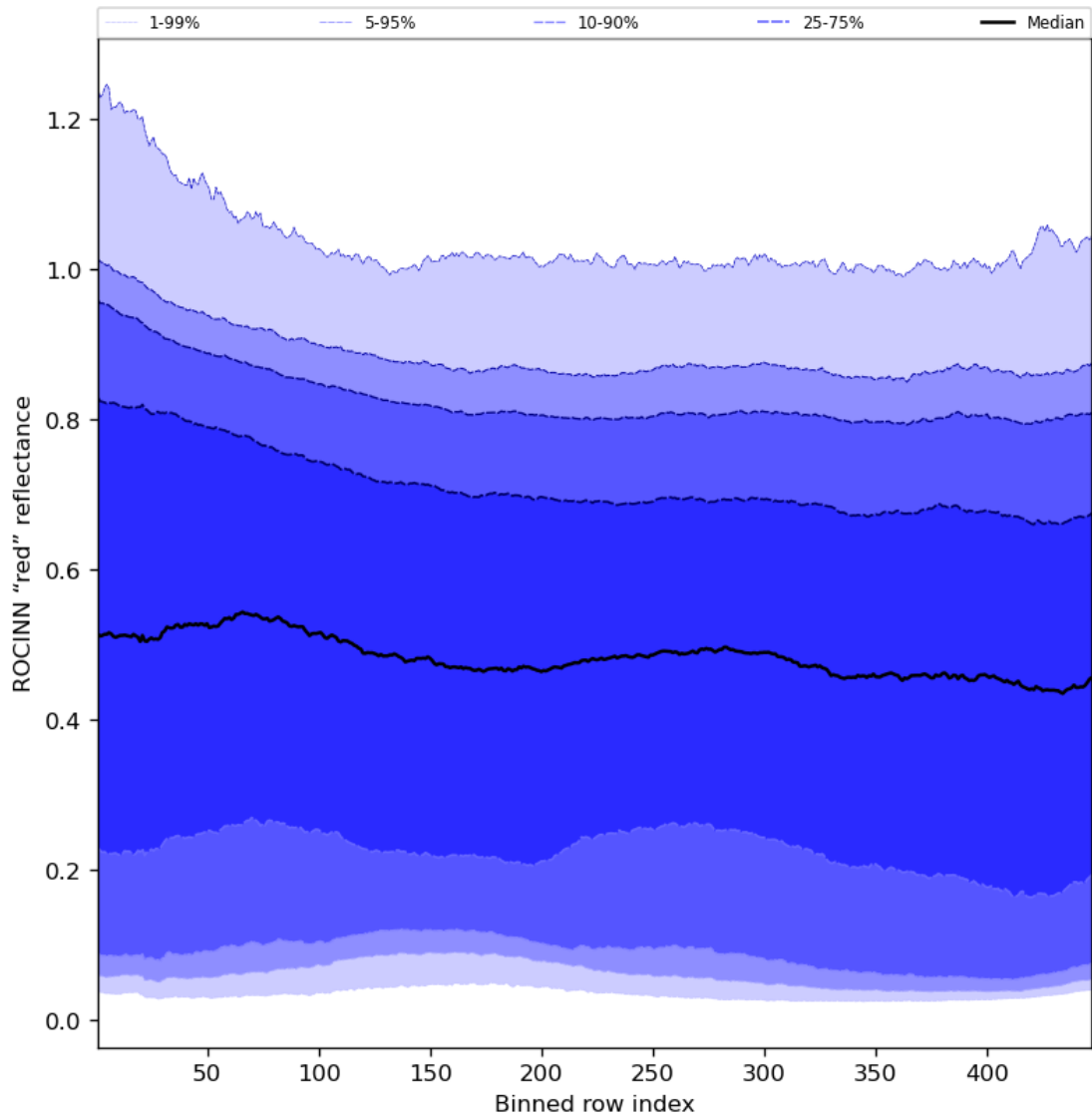
Figure 69: Along track statistics of “ROCINN “red” reflectance” for 2024-03-04 to 2024-03-06
