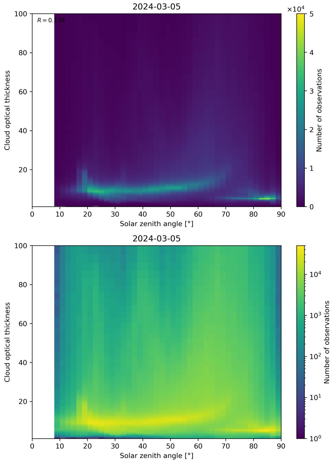
Figure 103: Scatter density plot of “Solar zenith angle” against “Cloud optical thickness” for 2024-03-04 to 2024-03-06.
