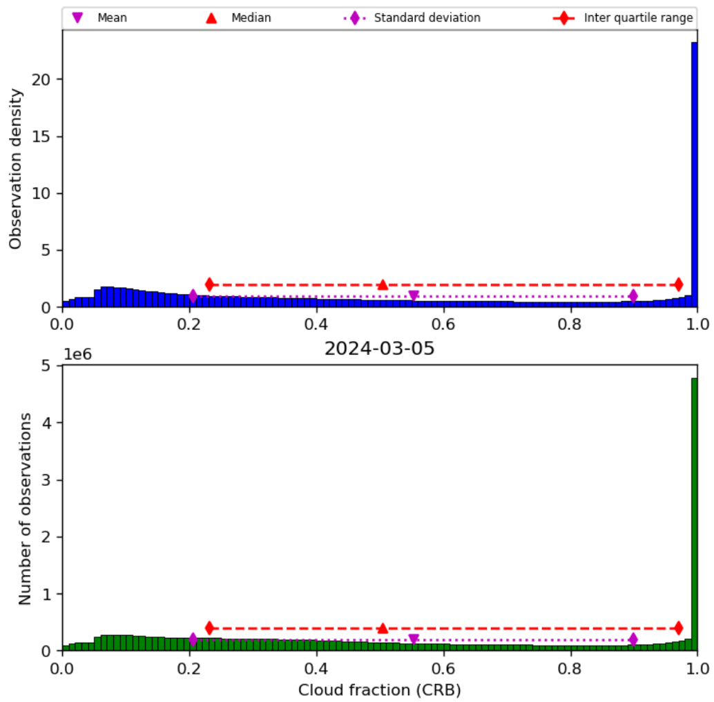
Figure 42: Histogram of “Cloud fraction (CRB)” for 2024-03-04 to 2024-03-06
