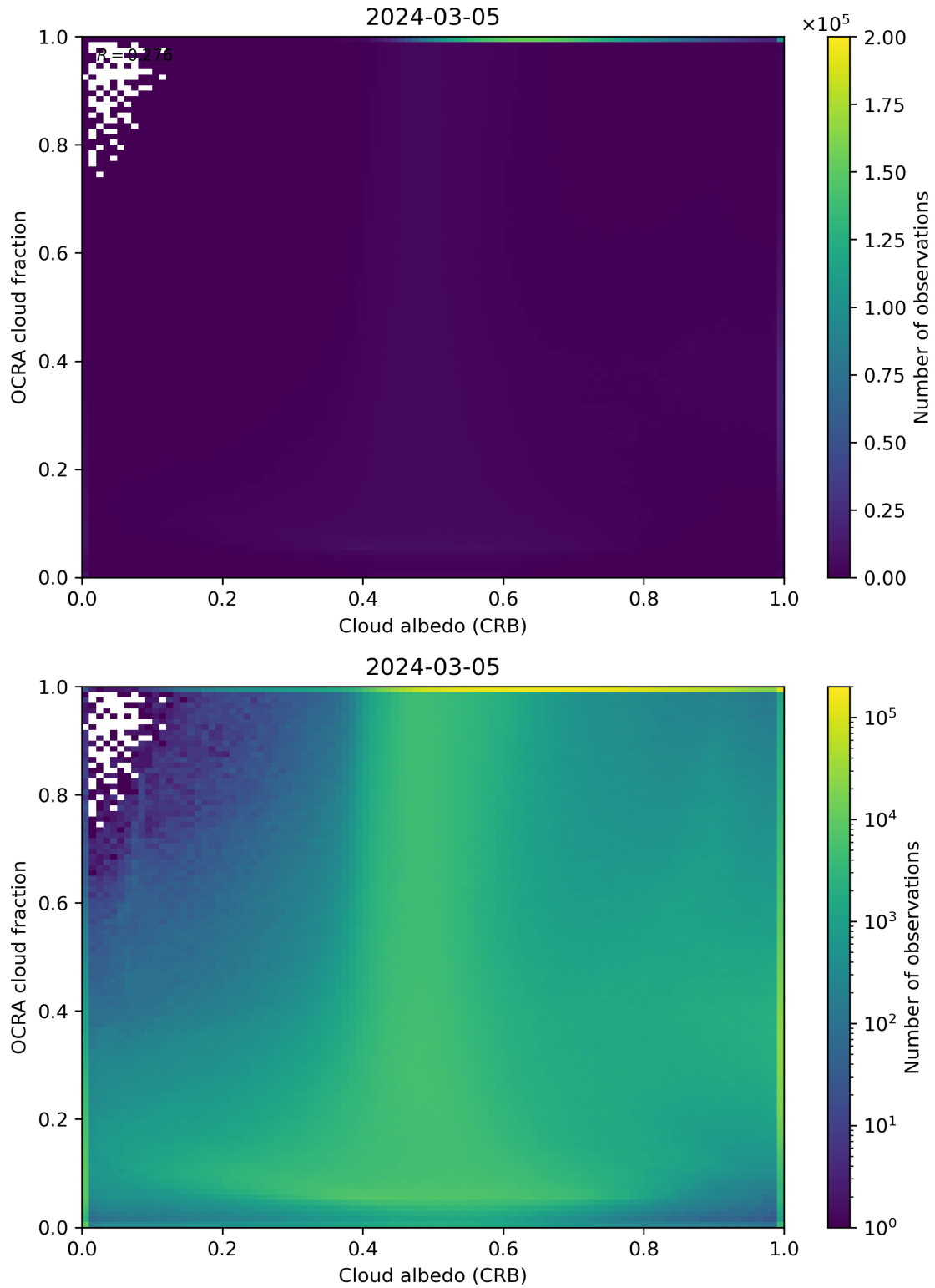
Figure 70: Scatter density plot of “Cloud albedo (CRB)” against “OCRA cloud fraction” for 2024-03-04 to 2024-03-06.
