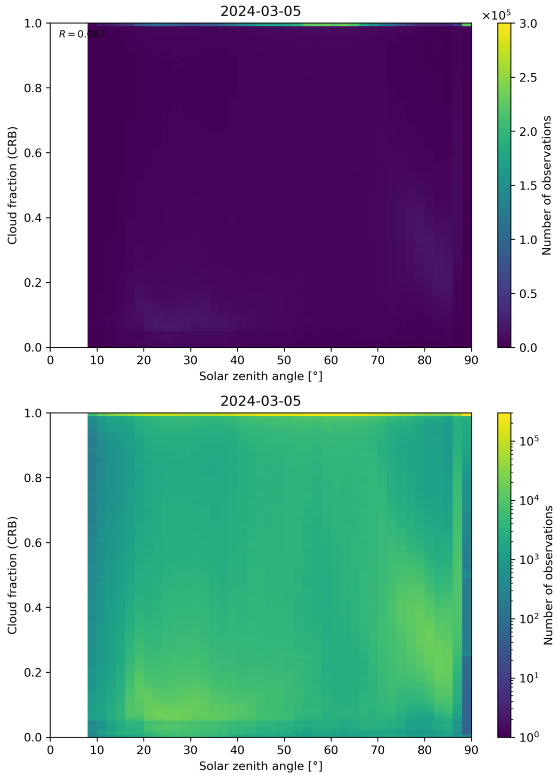
Figure 101: Scatter density plot of “Solar zenith angle” against “Cloud fraction (CRB)” for 2024-03-04 to 2024-03-06.
