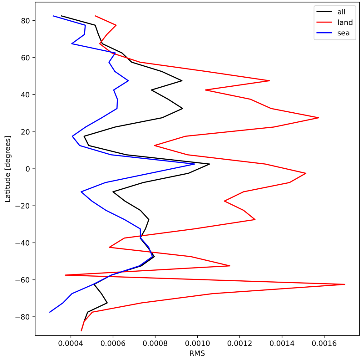
Figure 31: Zonal average of “RMS” for 2024-03-04 to 2024-03-06.
