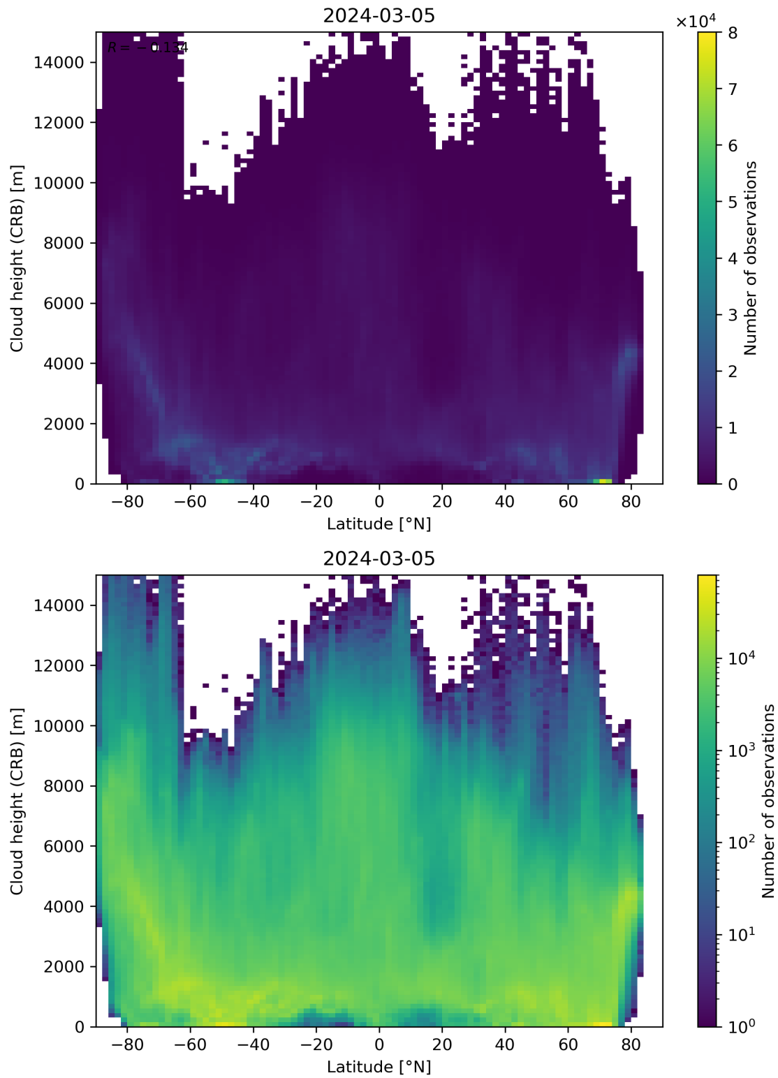
Figure 95: Scatter density plot of “Latitude” against “Cloud height (CRB)” for 2024-03-04 to 2024-03-06.
