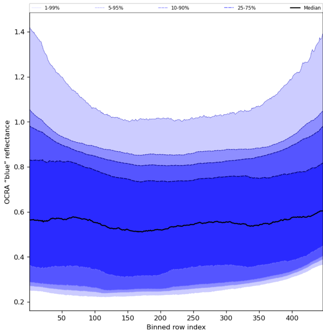
Figure 67: Along track statistics of “OCRA “blue” reflectance” for 2024-03-04 to 2024-03-06
