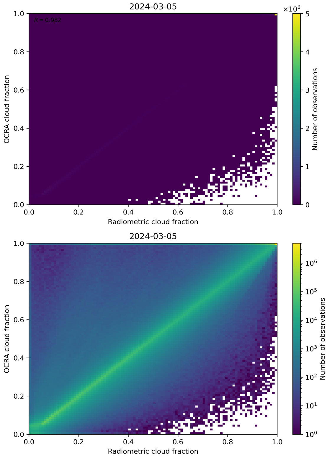
Figure 72: Scatter density plot of “Radiometric cloud fraction” against “OCRA cloud fraction” for 2024-03-04 to 2024-03-06.
