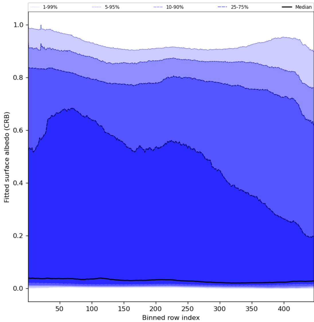
Figure 62: Along track statistics of “Fitted surface albedo (CRB)” for 2024-03-04 to 2024-03-06
