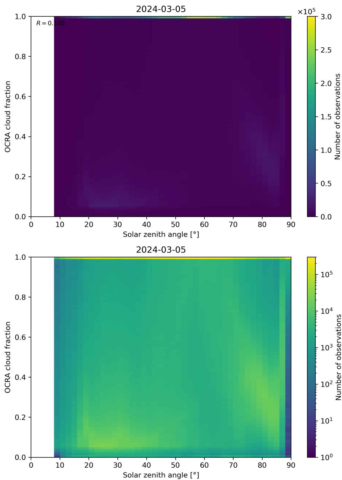
Figure 100: Scatter density plot of “Solar zenith angle” against “OCRA cloud fraction” for 2024-03-04 to 2024-03-06.
