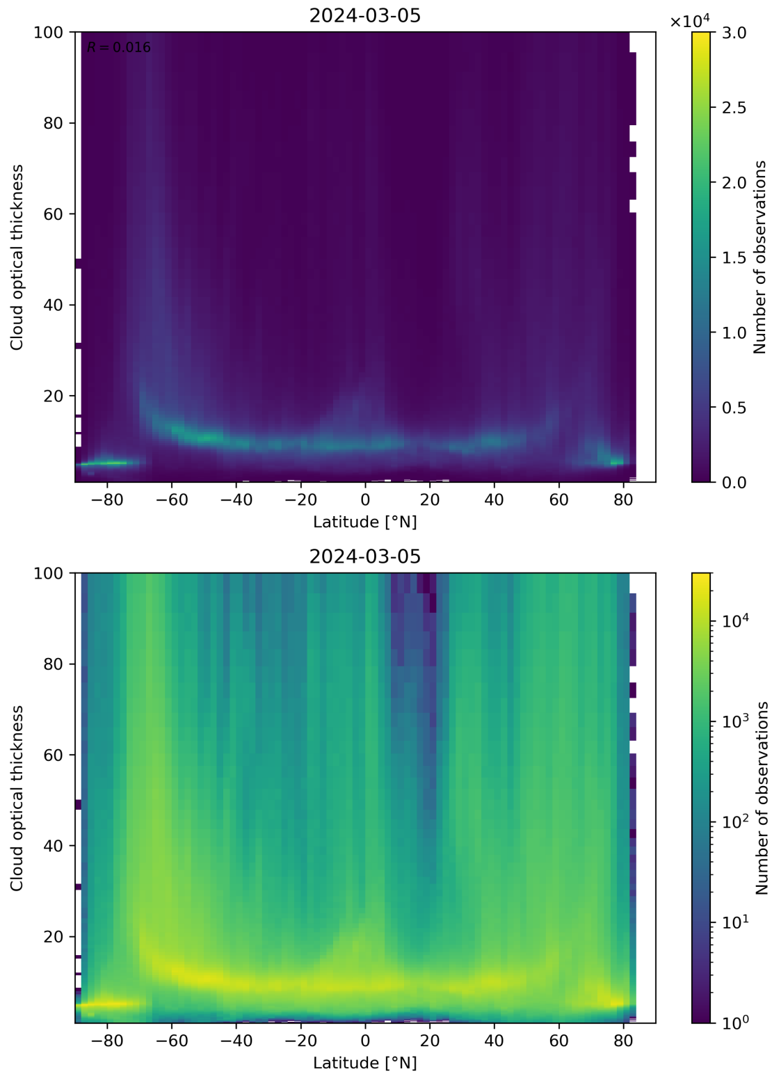
Figure 96: Scatter density plot of “Latitude” against “Cloud optical thickness” for 2024-03-04 to 2024-03-06.
