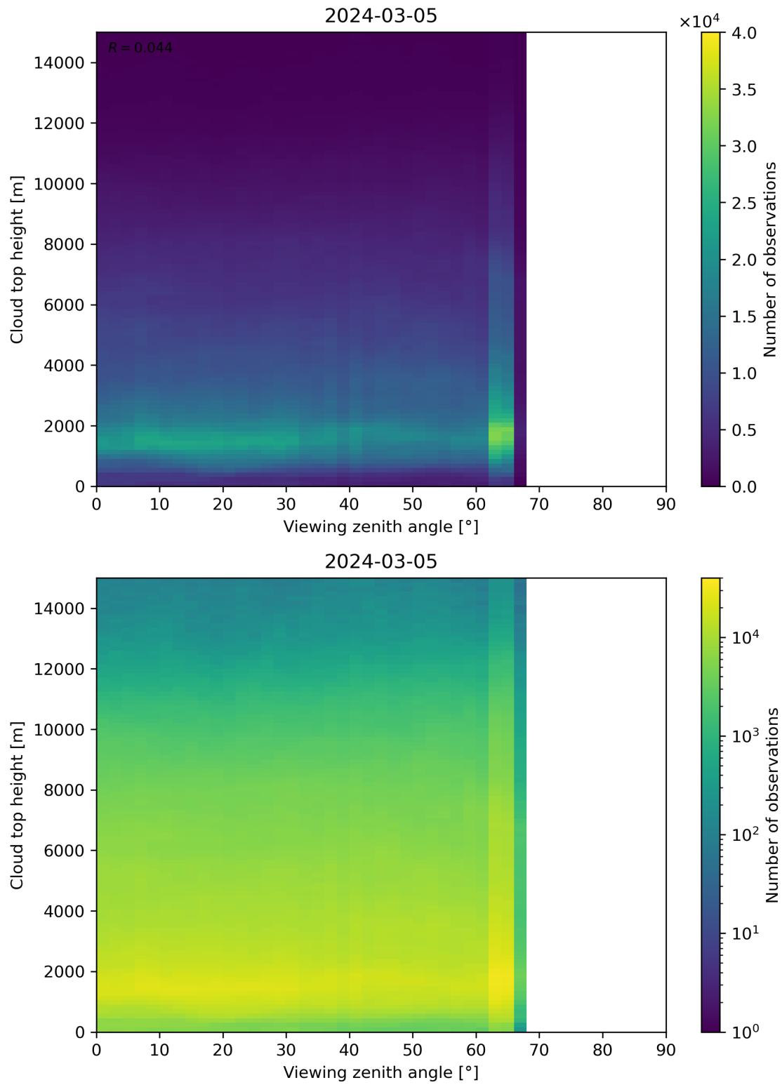
Figure 112: Scatter density plot of “Viewing zenith angle” against “Cloud top height” for 2024-03-04 to 2024-03-06.
