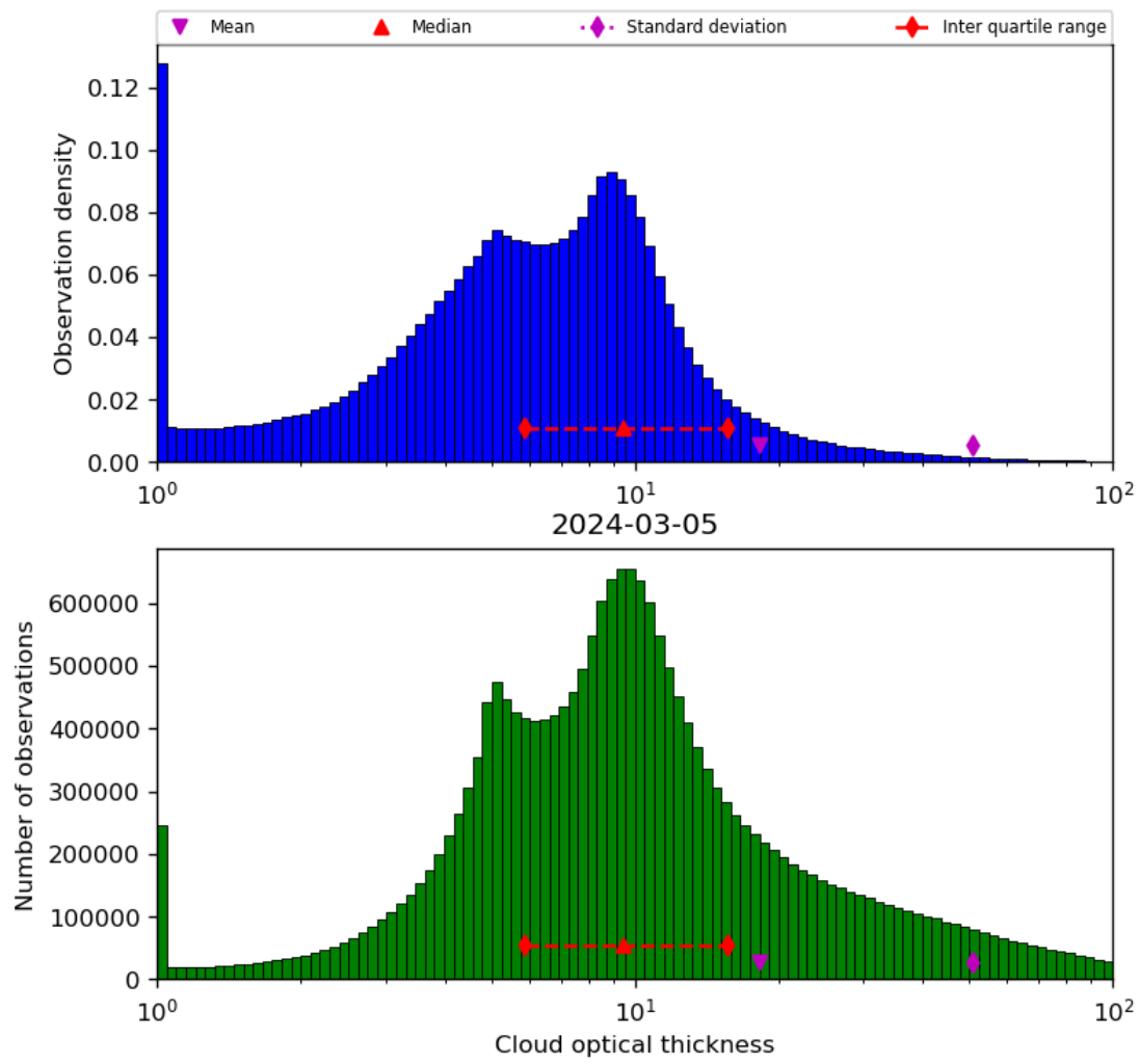
Figure 41: Histogram of “Cloud optical thickness” for 2024-03-04 to 2024-03-06
