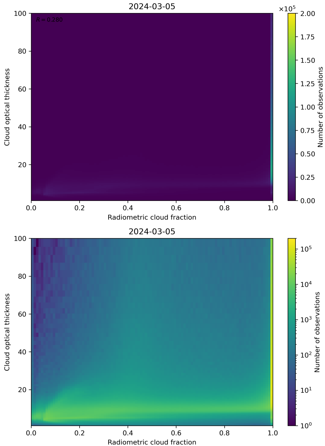
Figure 75: Scatter density plot of “Radiometric cloud fraction” against “Cloud optical thickness” for 2024-03-04 to 2024-03-06.
