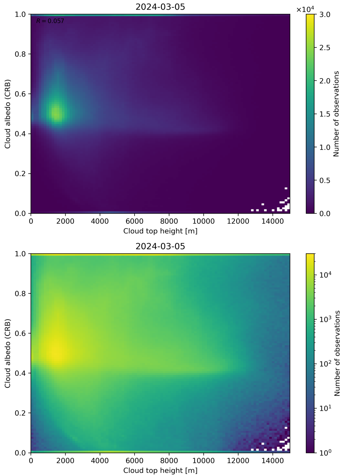
Figure 86: Scatter density plot of “Cloud top height” against “Cloud albedo (CRB)” for 2024-03-04 to 2024-03-06.
