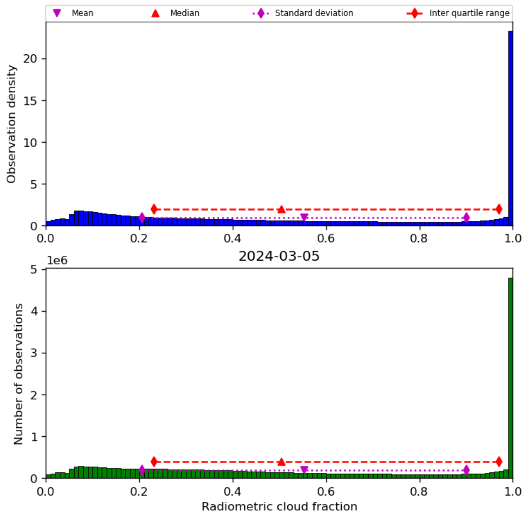
Figure 39: Histogram of “Radiometric cloud fraction” for 2024-03-04 to 2024-03-06
