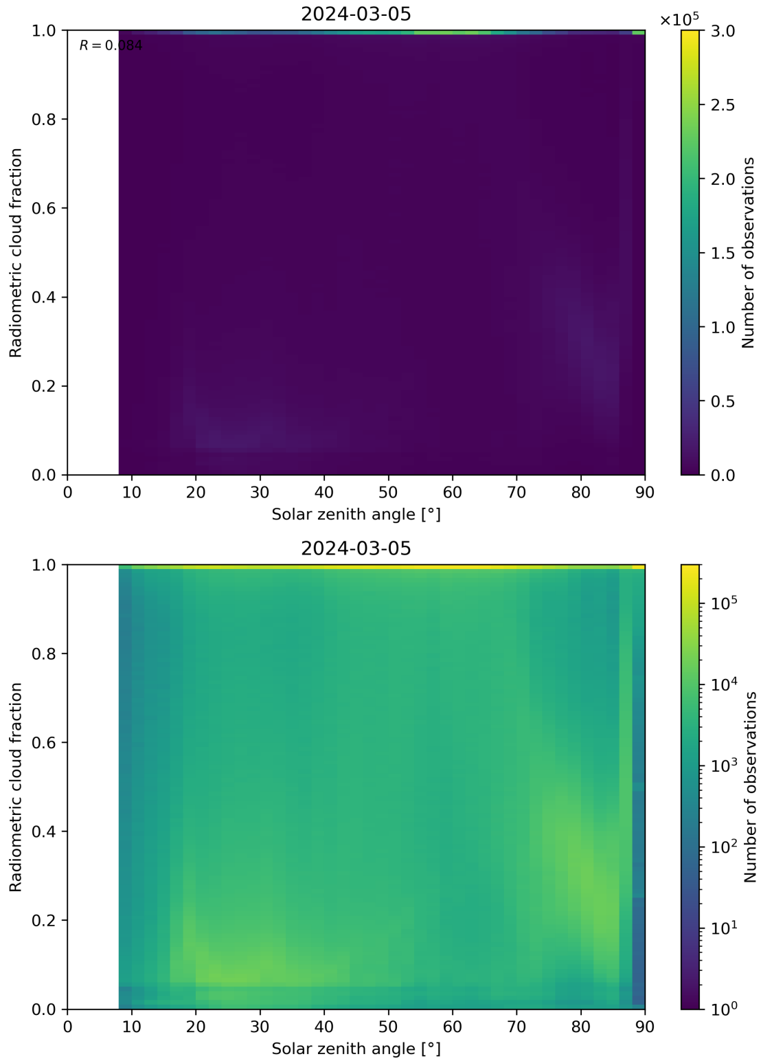
Figure 99: Scatter density plot of “Solar zenith angle” against “Radiometric cloud fraction” for 2024-03-04 to 2024-03-06.
