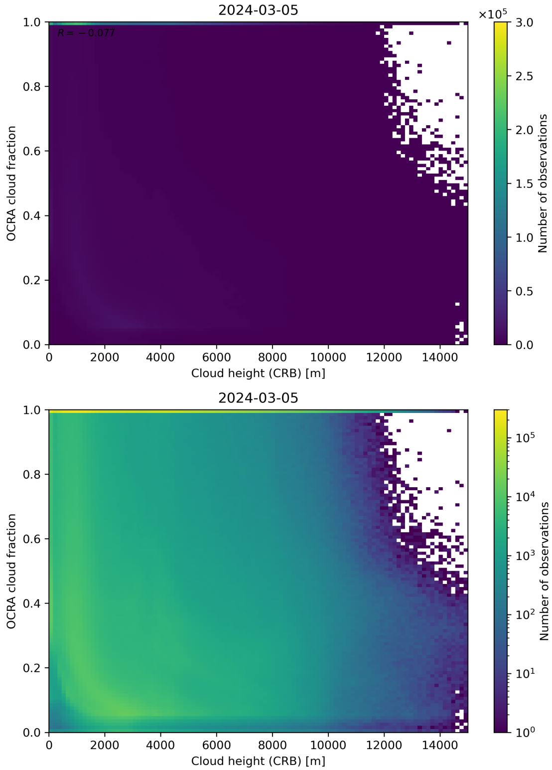
Figure 81: Scatter density plot of “Cloud height (CRB)” against “OCRA cloud fraction” for 2024-03-04 to 2024-03-06.
