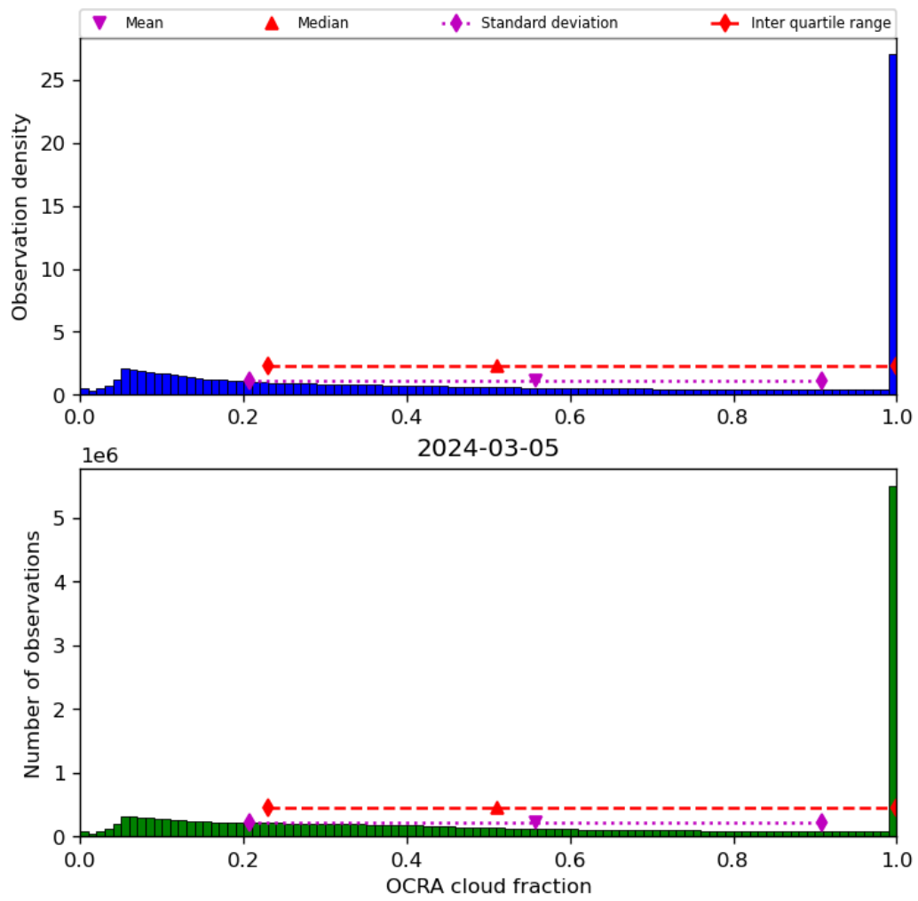
Figure 50: Histogram of “OCRA cloud fraction” for 2024-03-04 to 2024-03-06
