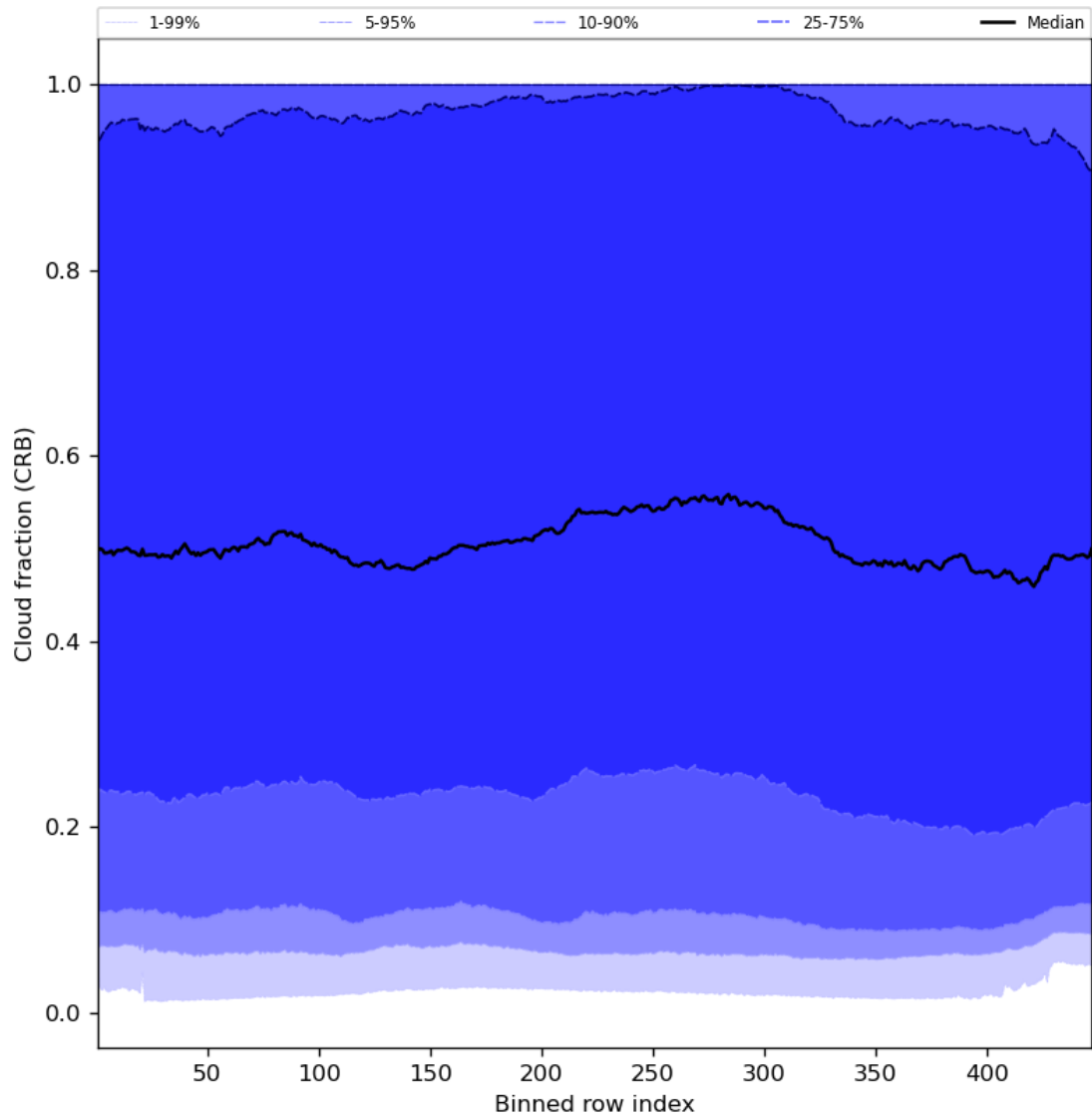
Figure 58: Along track statistics of “Cloud fraction (CRB)” for 2024-03-04 to 2024-03-06
