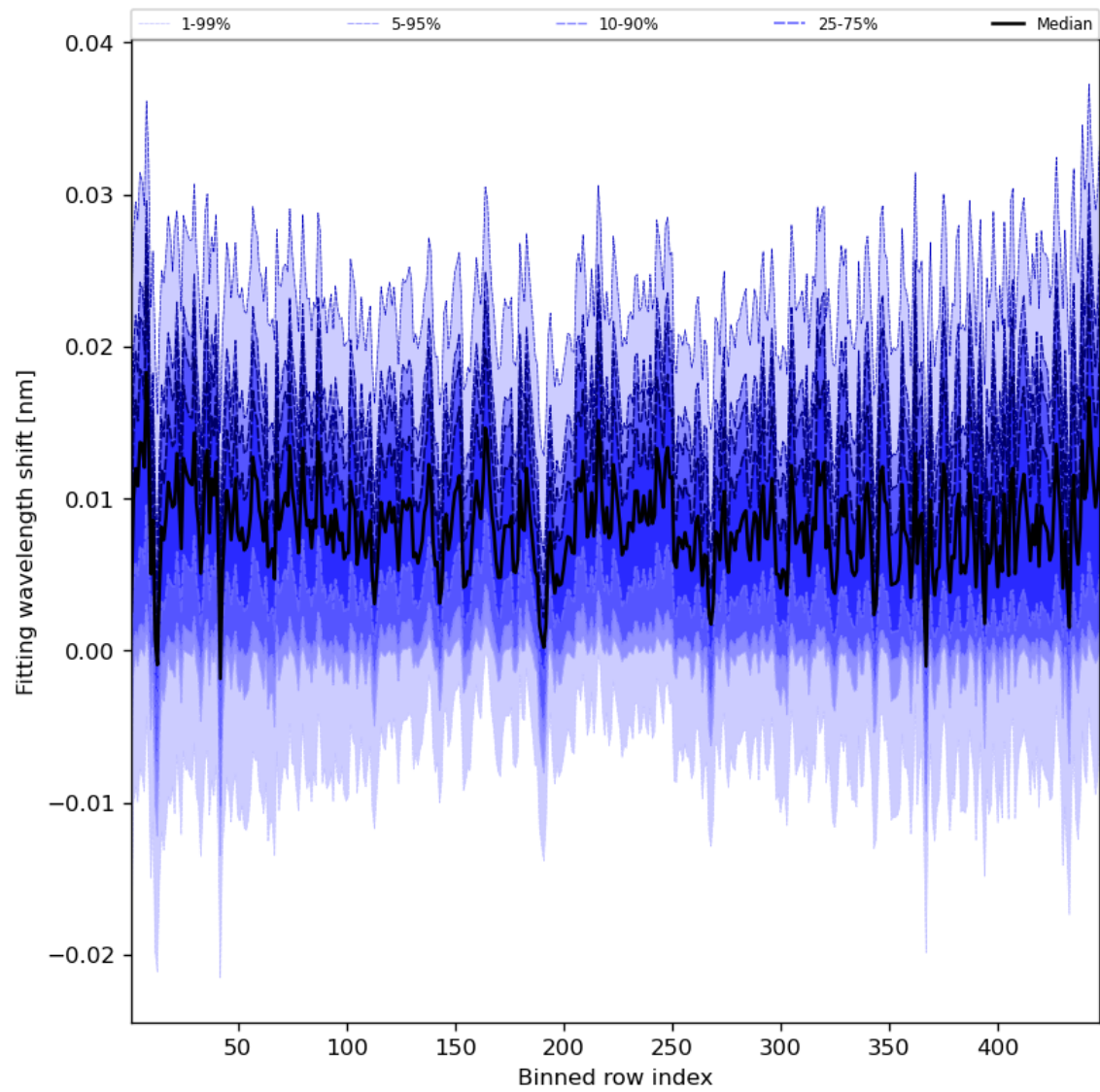
Figure 65: Along track statistics of “Fitting wavelength shift” for 2024-03-04 to 2024-03-06
