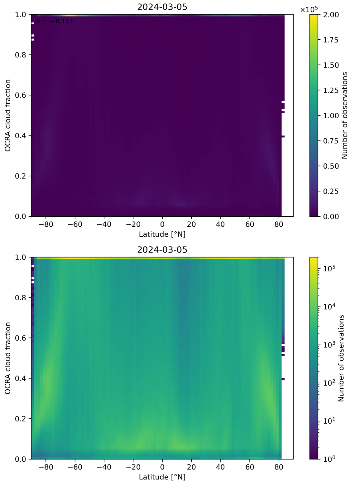
Figure 93: Scatter density plot of “Latitude” against “OCRA cloud fraction” for 2024-03-04 to 2024-03-06.
