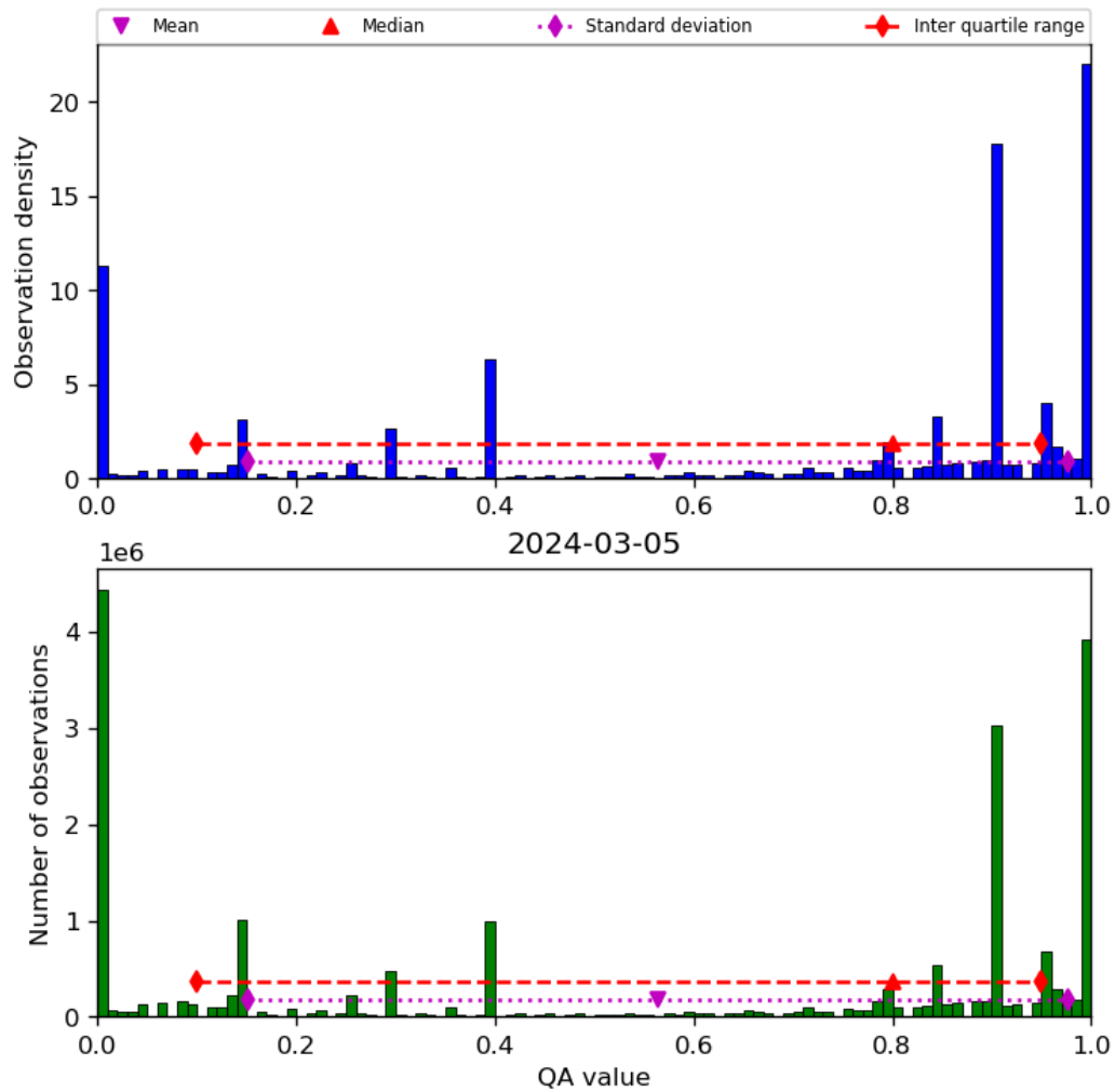
Figure 38: Histogram of “QA value” for 2024-03-04 to 2024-03-06
