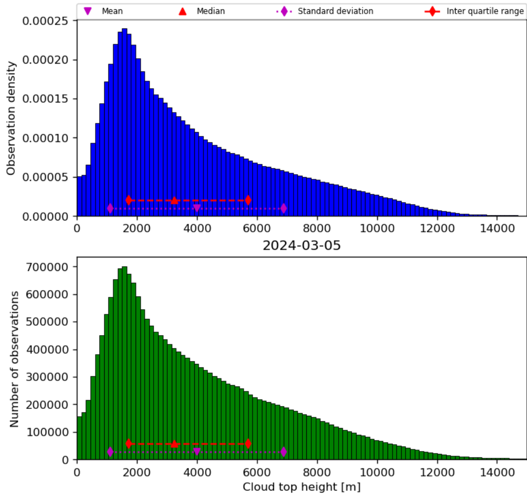
Figure 40: Histogram of “Cloud top height” for 2024-03-04 to 2024-03-06
