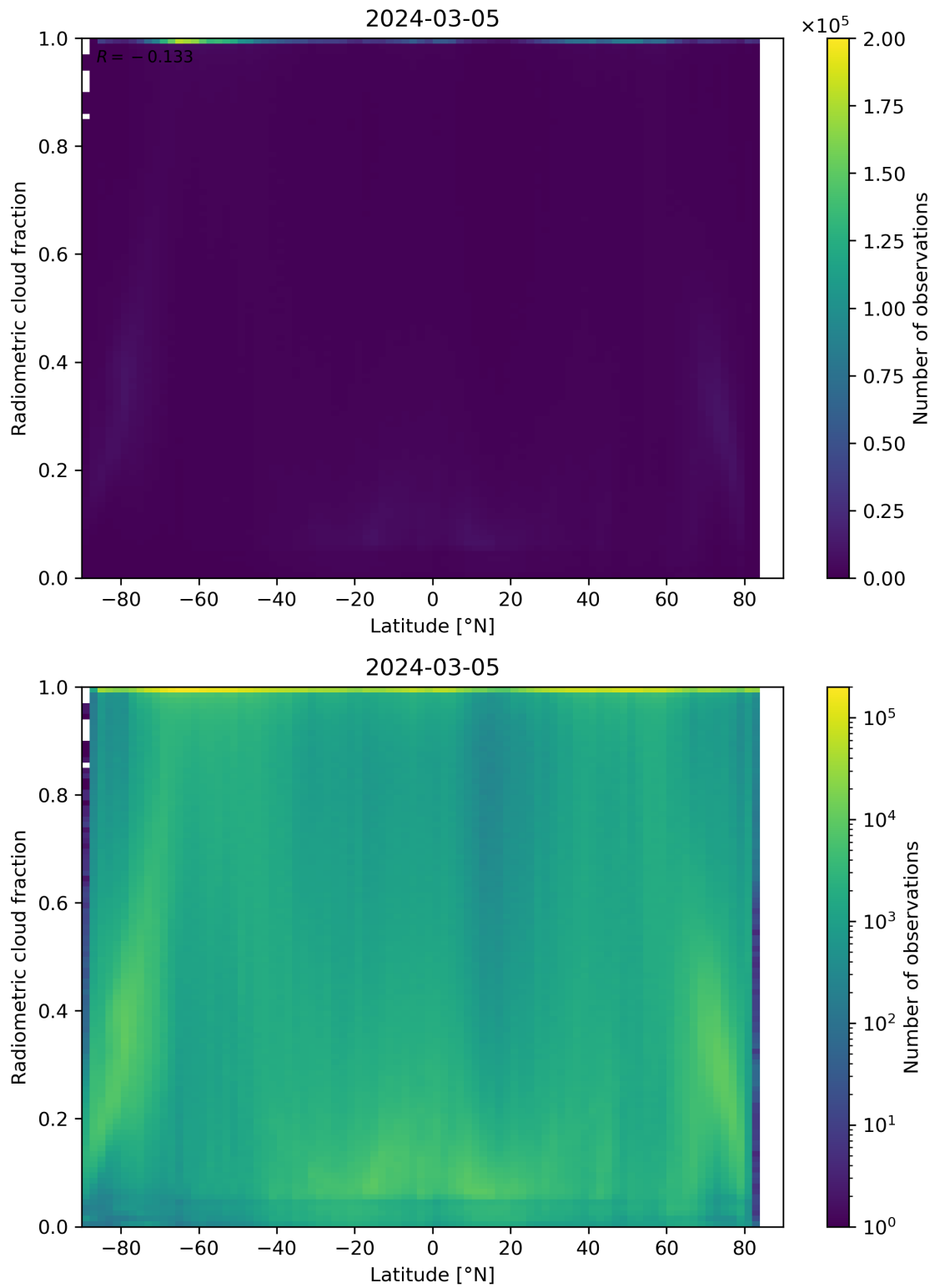
Figure 92: Scatter density plot of “Latitude” against “Radiometric cloud fraction” for 2024-03-04 to 2024-03-06.
