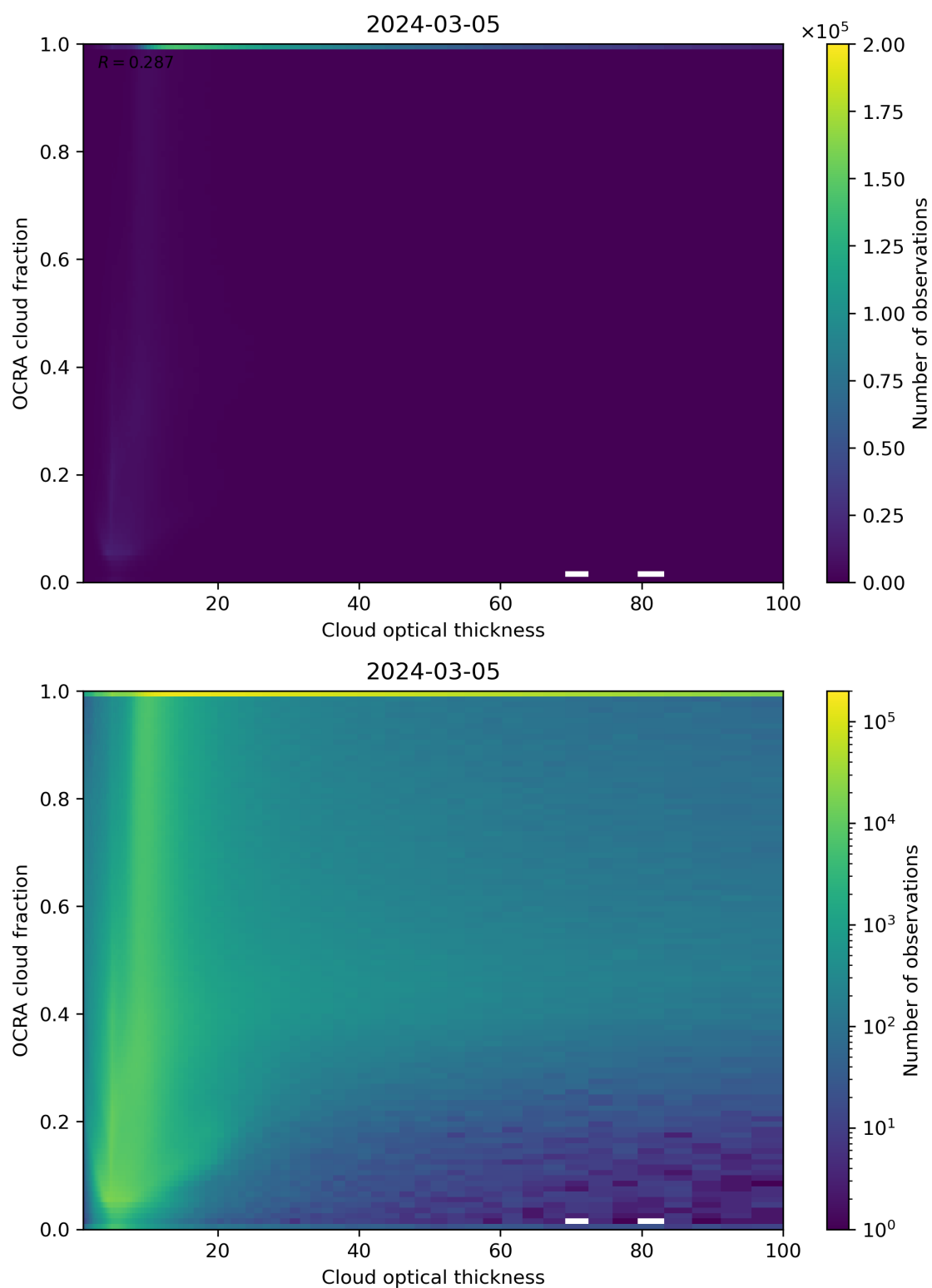
Figure 83: Scatter density plot of “Cloud optical thickness” against “OCRA cloud fraction” for 2024-03-04 to 2024-03-06.
