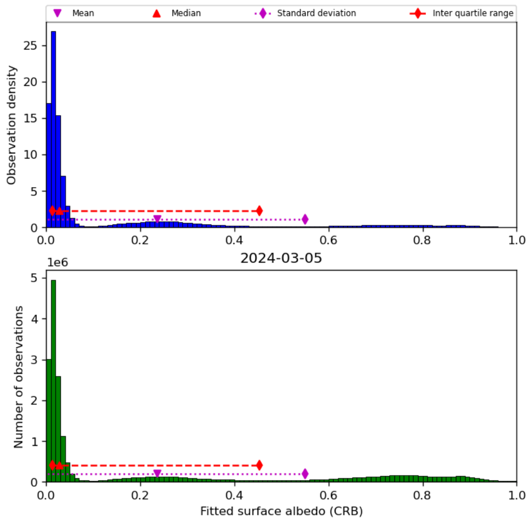
Figure 46: Histogram of “Fitted surface albedo (CRB)” for 2024-03-04 to 2024-03-06
