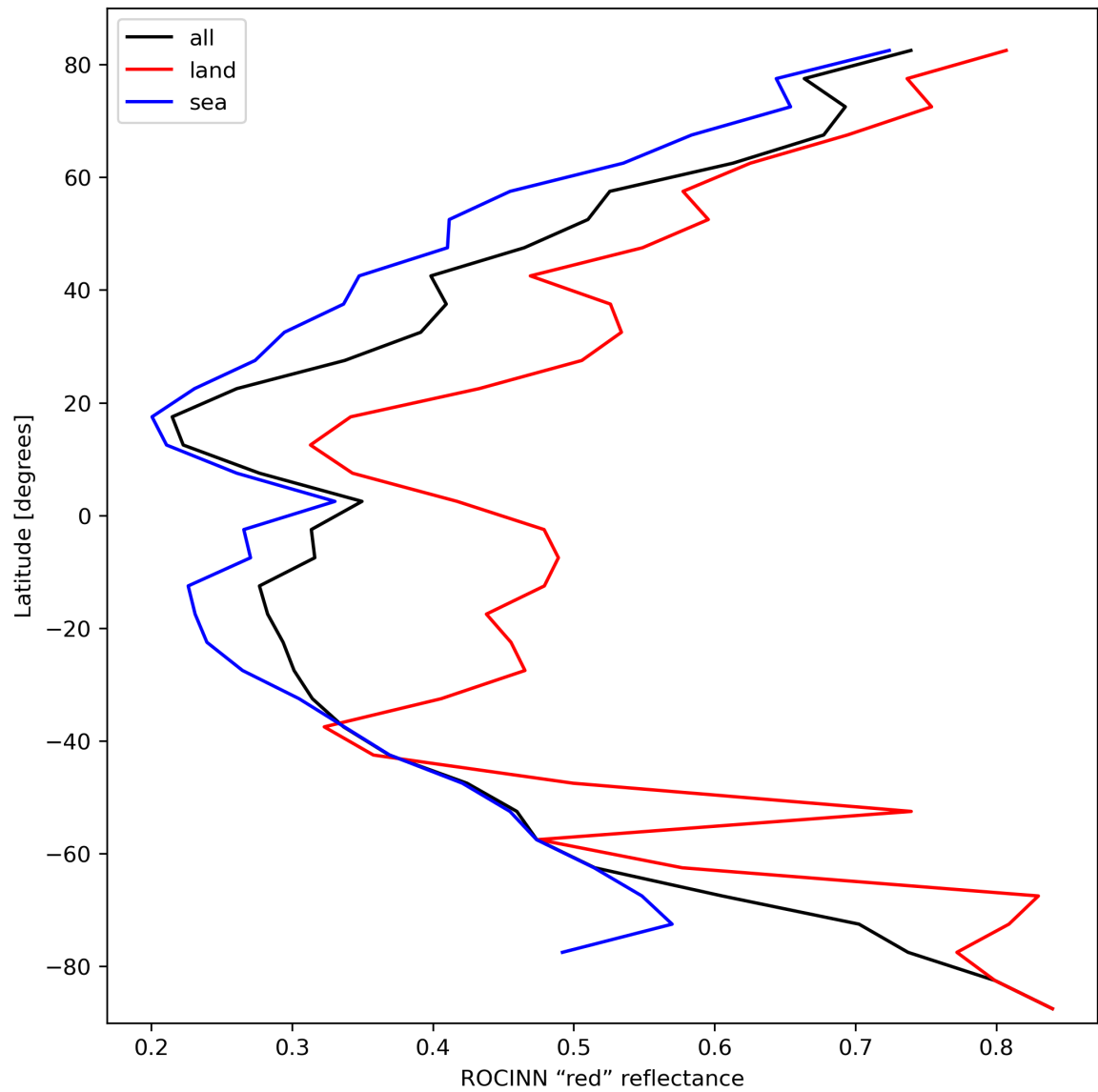
Figure 37: Zonal average of “ROCINN “red” reflectance” for 2024-03-04 to 2024-03-06.
