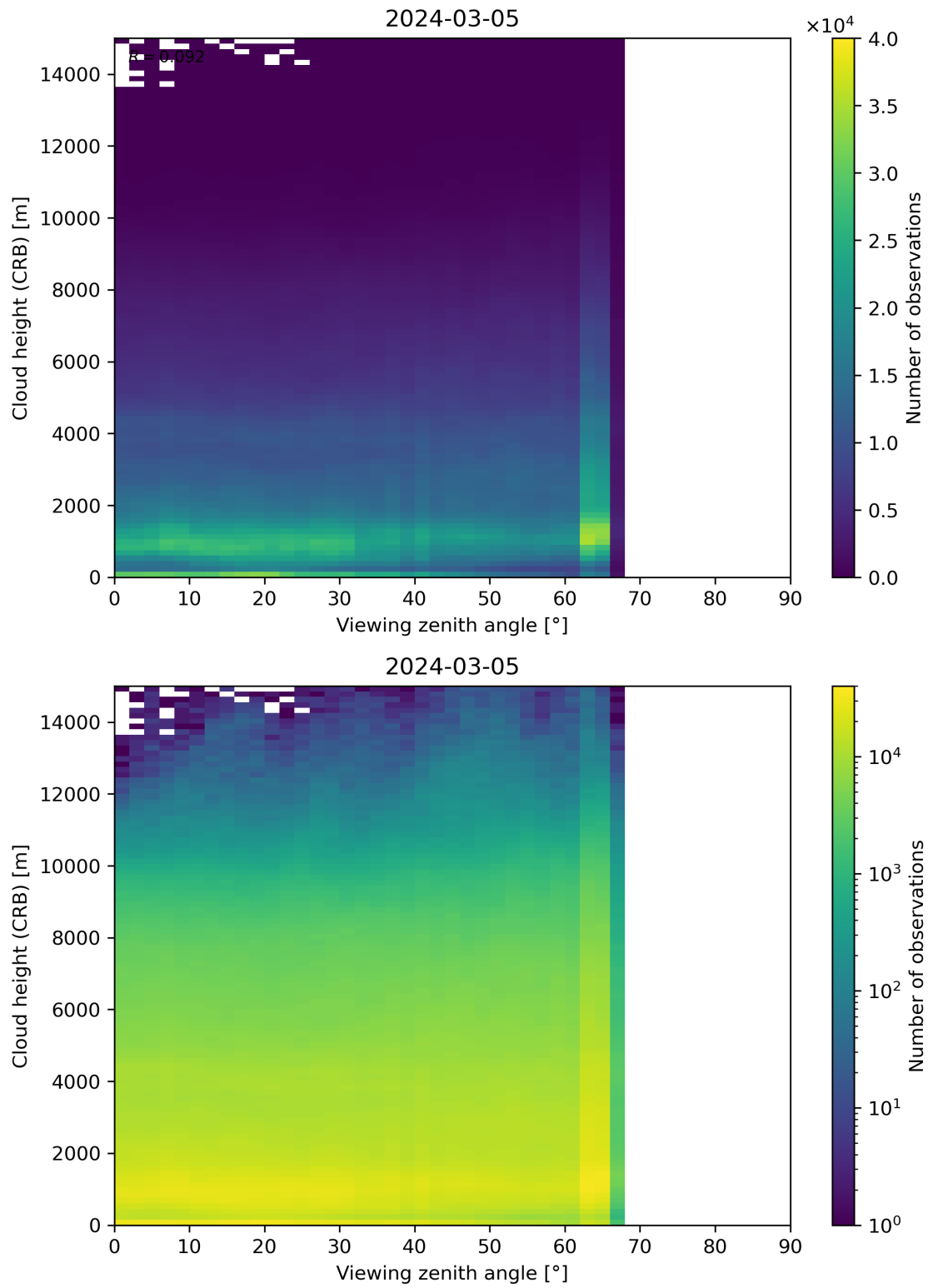
Figure 110: Scatter density plot of “Viewing zenith angle” against “Cloud height (CRB)” for 2024-03-04 to 2024-03-06.
