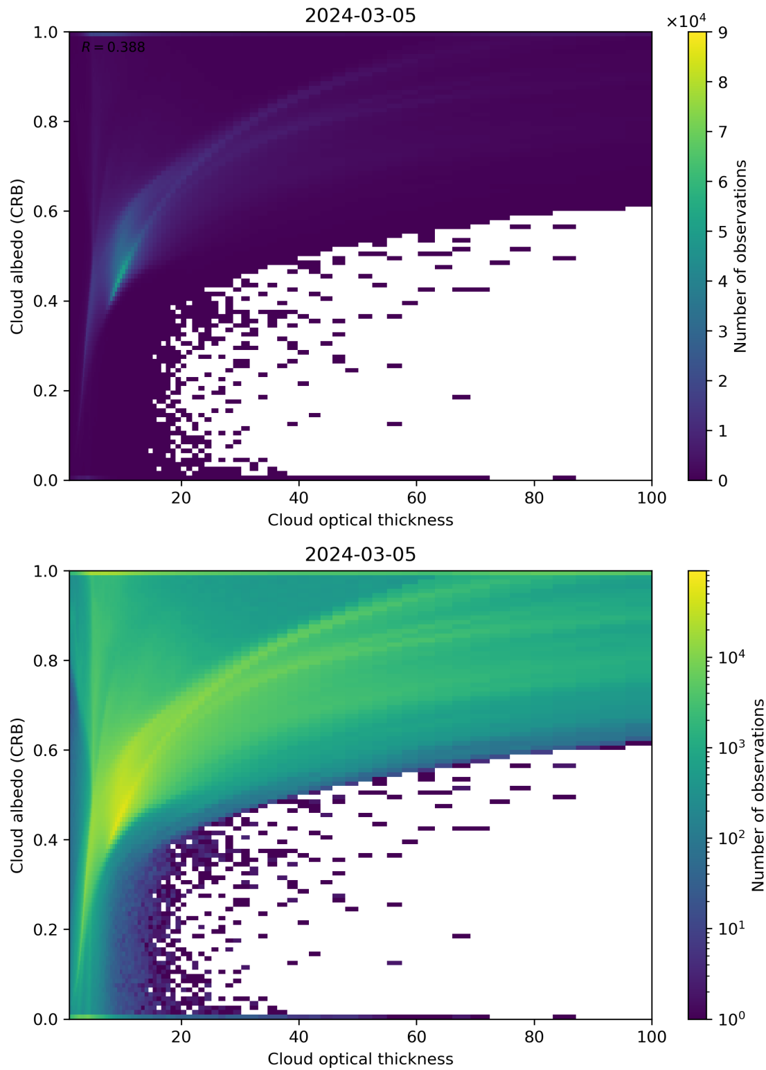
Figure 82: Scatter density plot of “Cloud optical thickness” against “Cloud albedo (CRB)” for 2024-03-04 to 2024-03-06.
