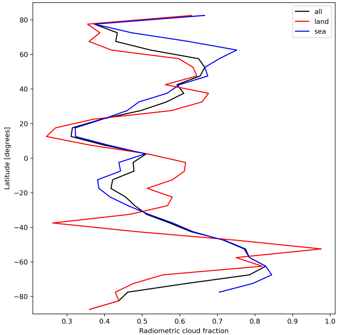
Figure 23: Zonal average of “Radiometric cloud fraction” for 2024-03-04 to 2024-03-06.
