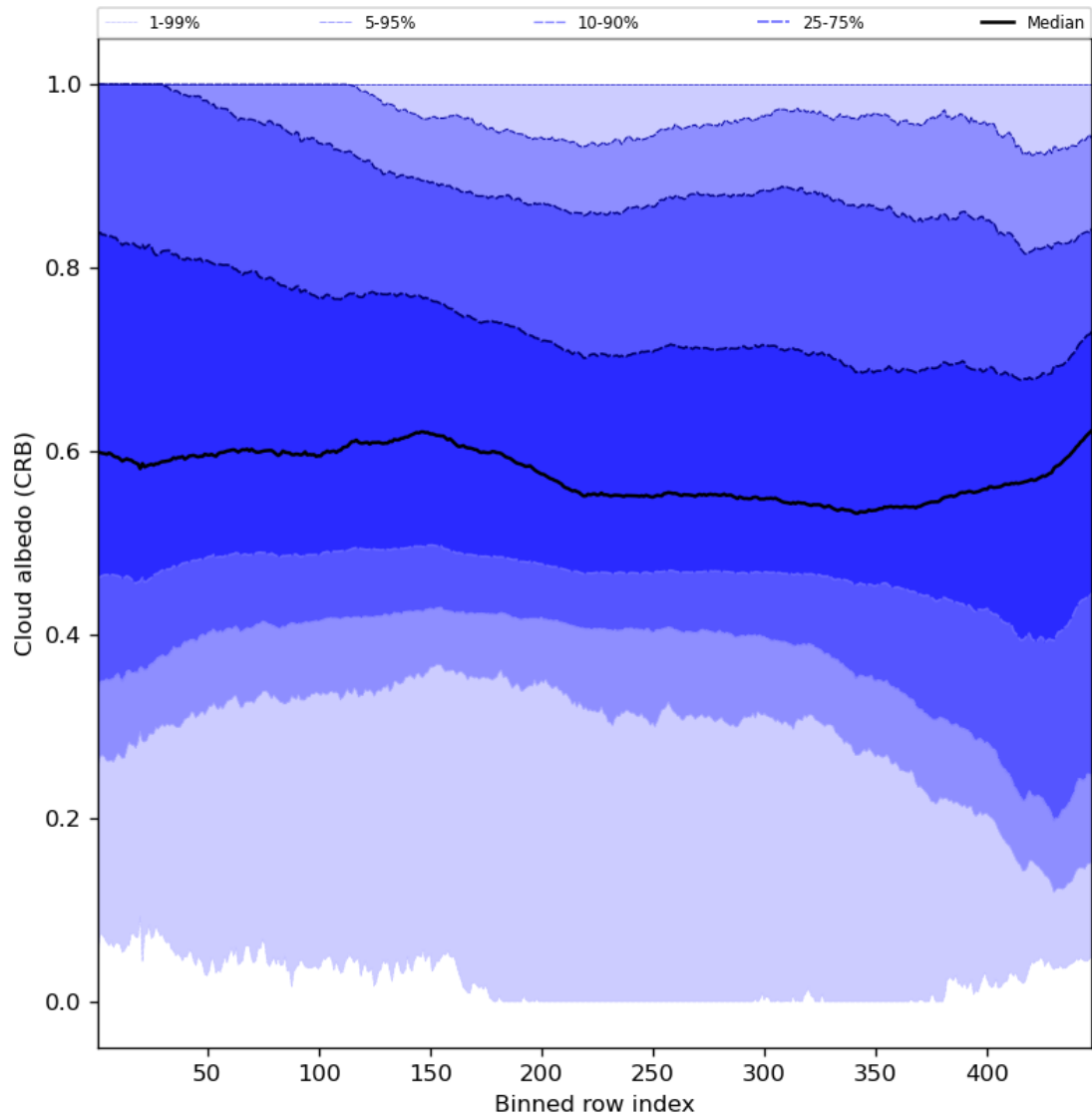
Figure 60: Along track statistics of “Cloud albedo (CRB)” for 2024-03-04 to 2024-03-06
