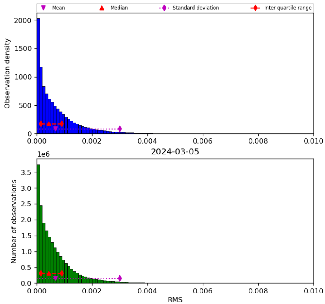
Figure 47: Histogram of “RMS” for 2024-03-04 to 2024-03-06
