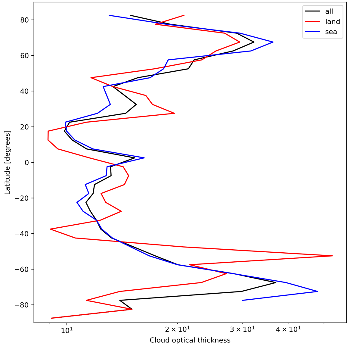
Figure 25: Zonal average of “Cloud optical thickness” for 2024-03-04 to 2024-03-06.
