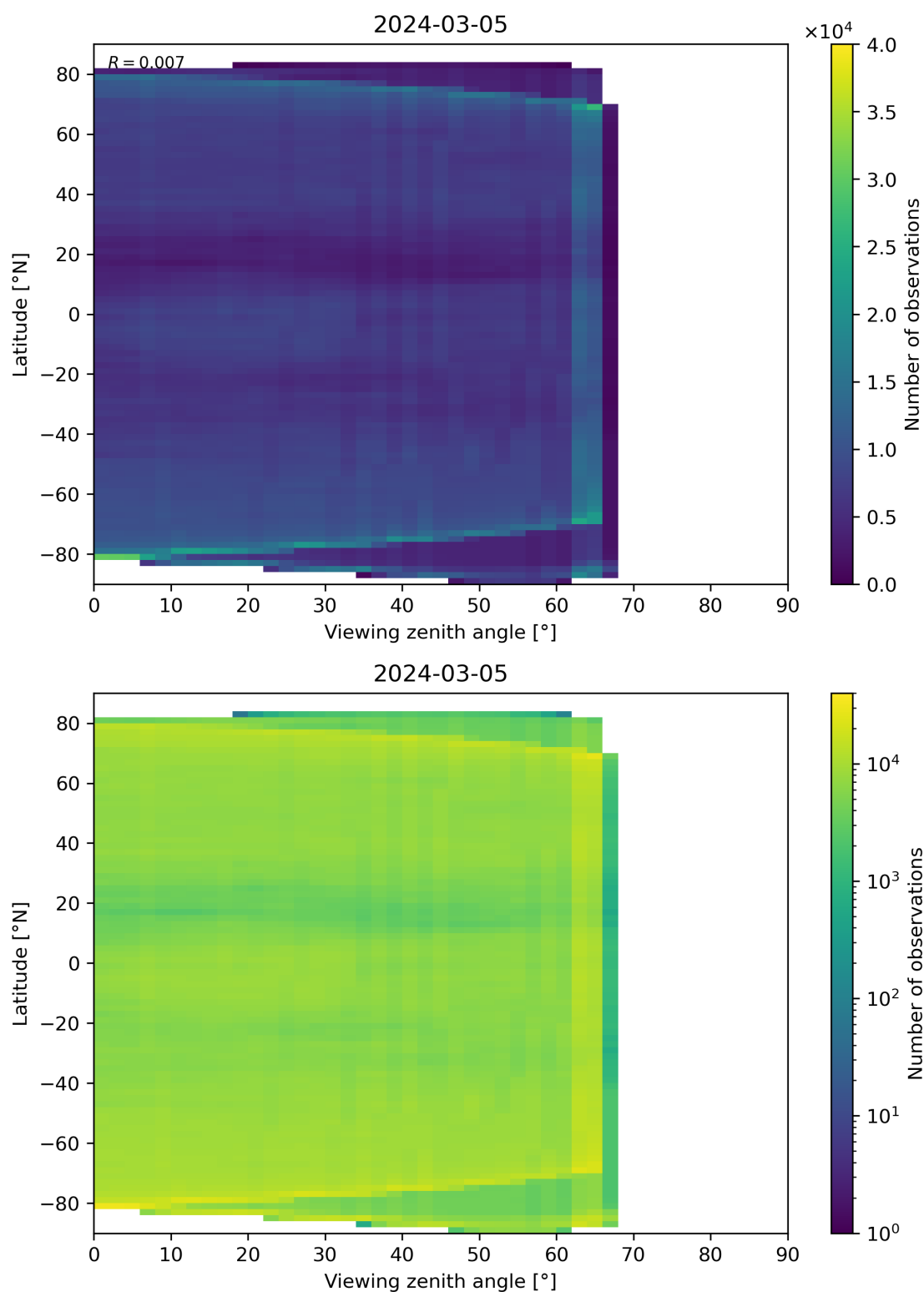
Figure 113: Scatter density plot of “Viewing zenith angle” against “Latitude” for 2024-03-04 to 2024-03-06.
