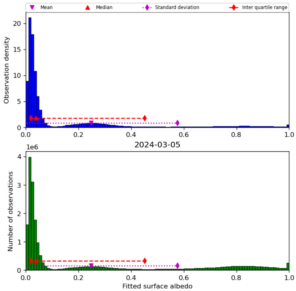
Figure 45: Histogram of “Fitted surface albedo” for 2024-03-04 to 2024-03-06
