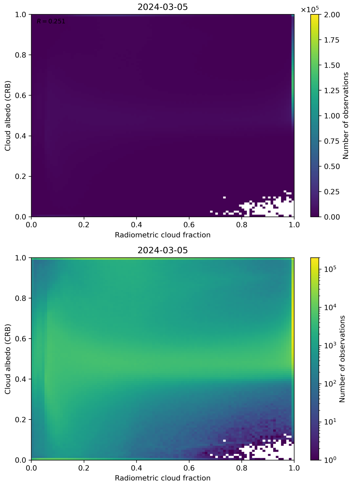
Figure 71: Scatter density plot of “Radiometric cloud fraction” against “Cloud albedo (CRB)” for 2024-03-04 to 2024-03-06.
