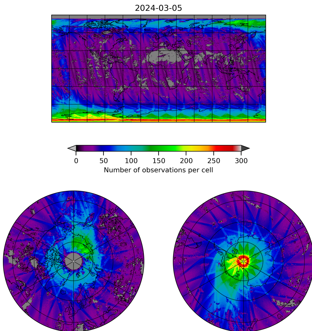
Figure 21: Map of the number of observations for 2024-03-04 to 2024-03-06
