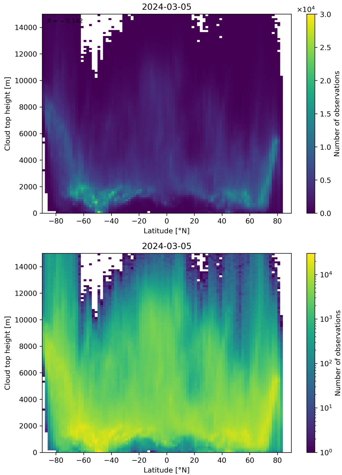
Figure 97: Scatter density plot of “Latitude” against “Cloud top height” for 2024-03-04 to 2024-03-06.
