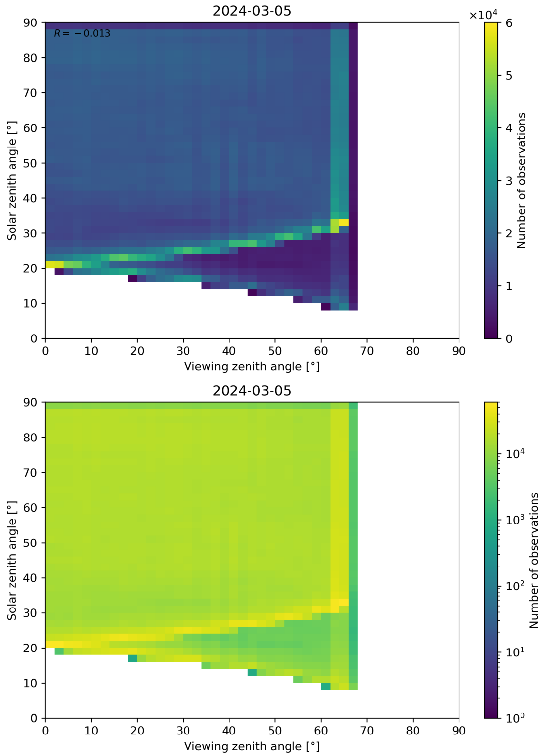
Figure 114: Scatter density plot of “Viewing zenith angle” against “Solar zenith angle” for 2024-03-04 to 2024-03-06.
