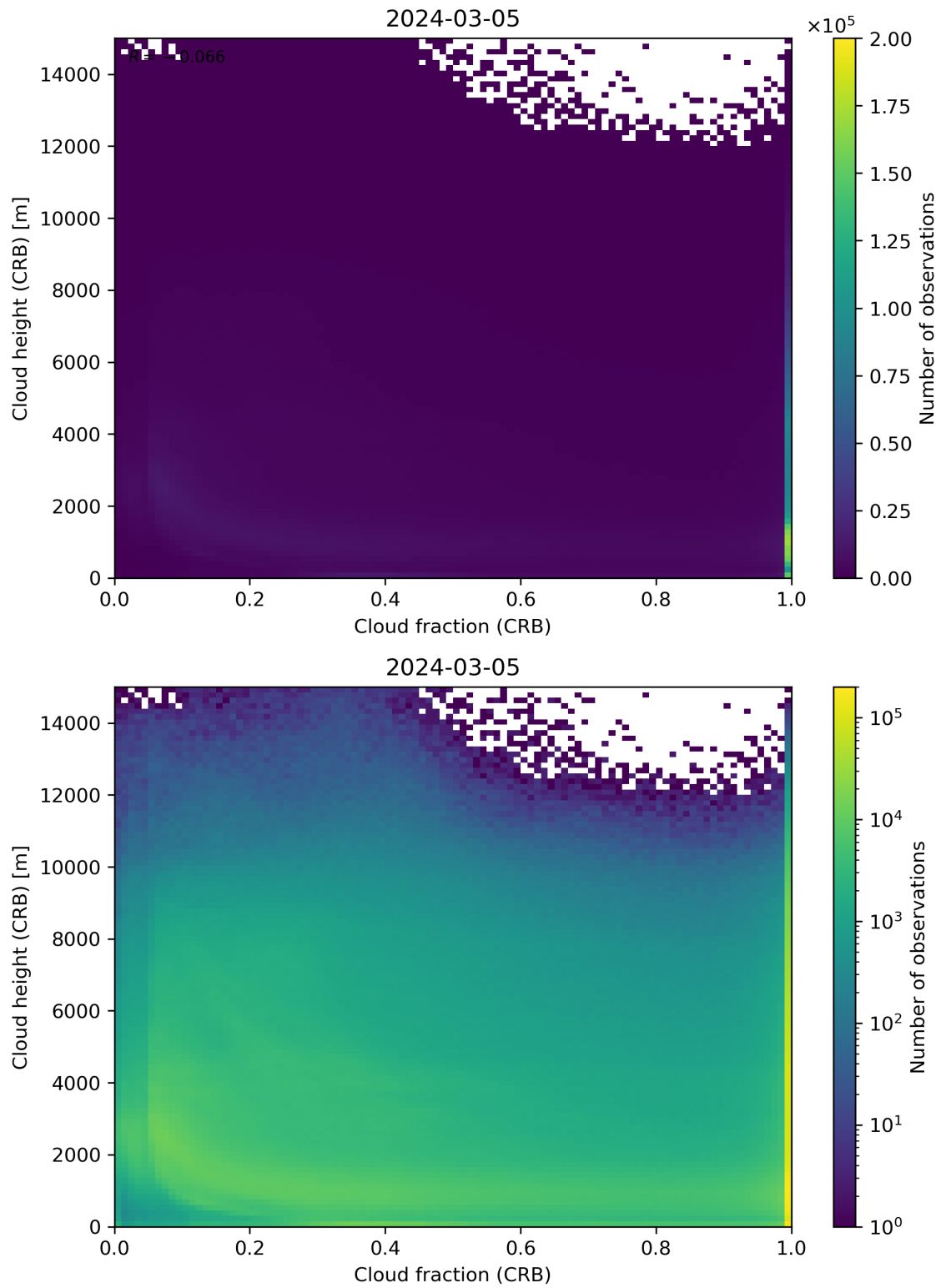
Figure 79: Scatter density plot of “Cloud fraction (CRB)” against “Cloud height (CRB)” for 2024-03-04 to 2024-03-06.
