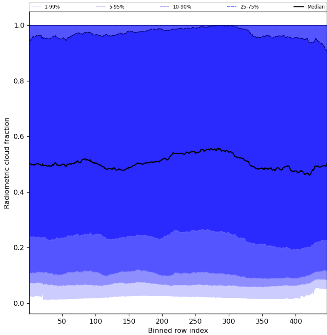
Figure 55: Along track statistics of “Radiometric cloud fraction” for 2024-03-04 to 2024-03-06
