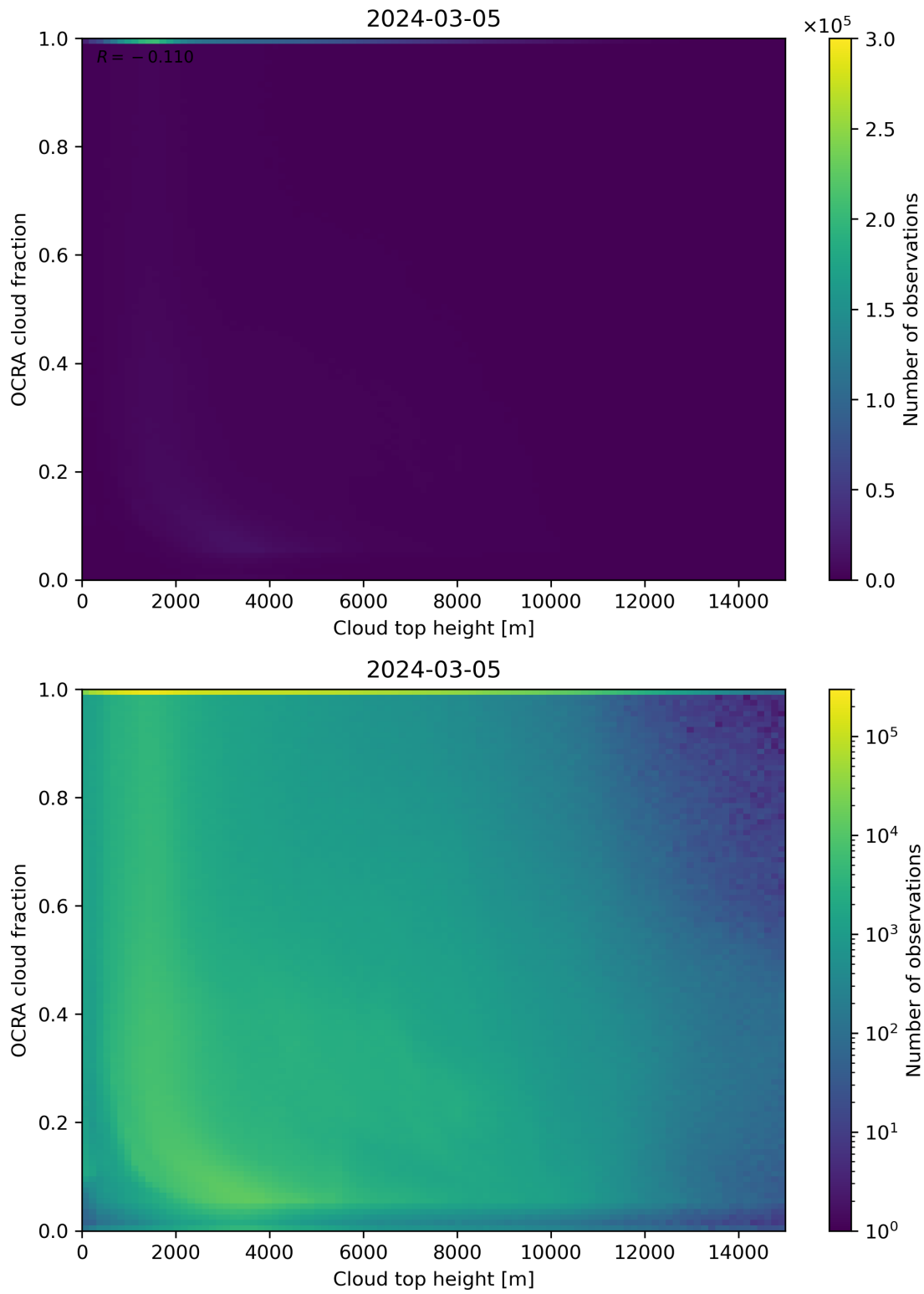
Figure 87: Scatter density plot of “Cloud top height” against “OCRA cloud fraction” for 2024-03-04 to 2024-03-06.
