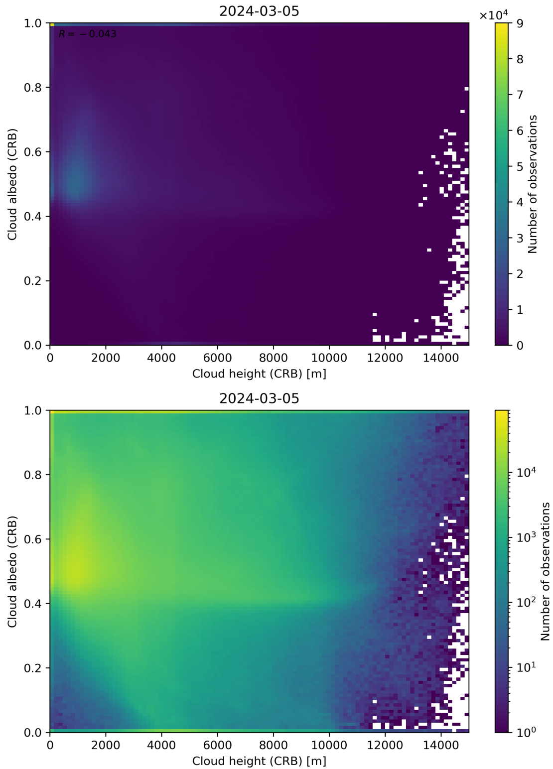
Figure 80: Scatter density plot of “Cloud height (CRB)” against “Cloud albedo (CRB)” for 2024-03-04 to 2024-03-06.
