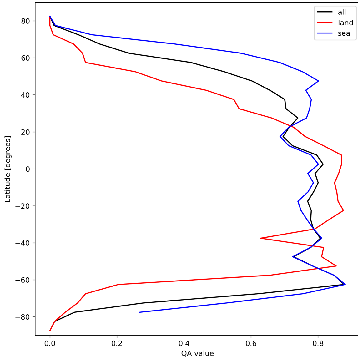
Figure 22: Zonal average of “QA value” for 2024-03-04 to 2024-03-06.
