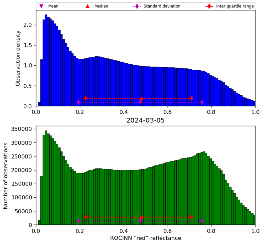
Figure 53: Histogram of “ROCINN “red” reflectance” for 2024-03-04 to 2024-03-06
