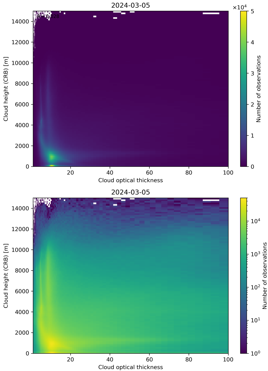
Figure 85: Scatter density plot of “Cloud optical thickness” against “Cloud height (CRB)” for 2024-03-04 to 2024-03-06.
