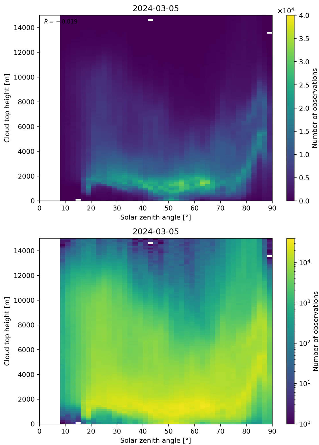
Figure 104: Scatter density plot of “Solar zenith angle” against “Cloud top height” for 2024-03-04 to 2024-03-06.
