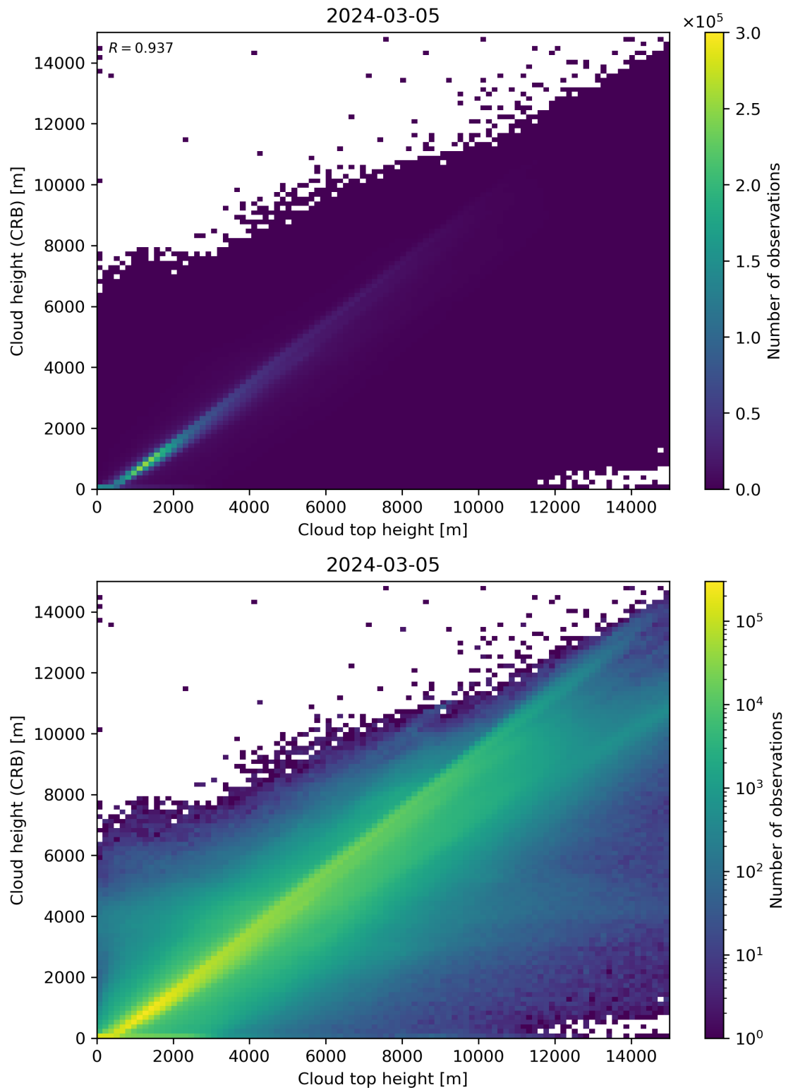
Figure 89: Scatter density plot of “Cloud top height” against “Cloud height (CRB)” for 2024-03-04 to 2024-03-06.
