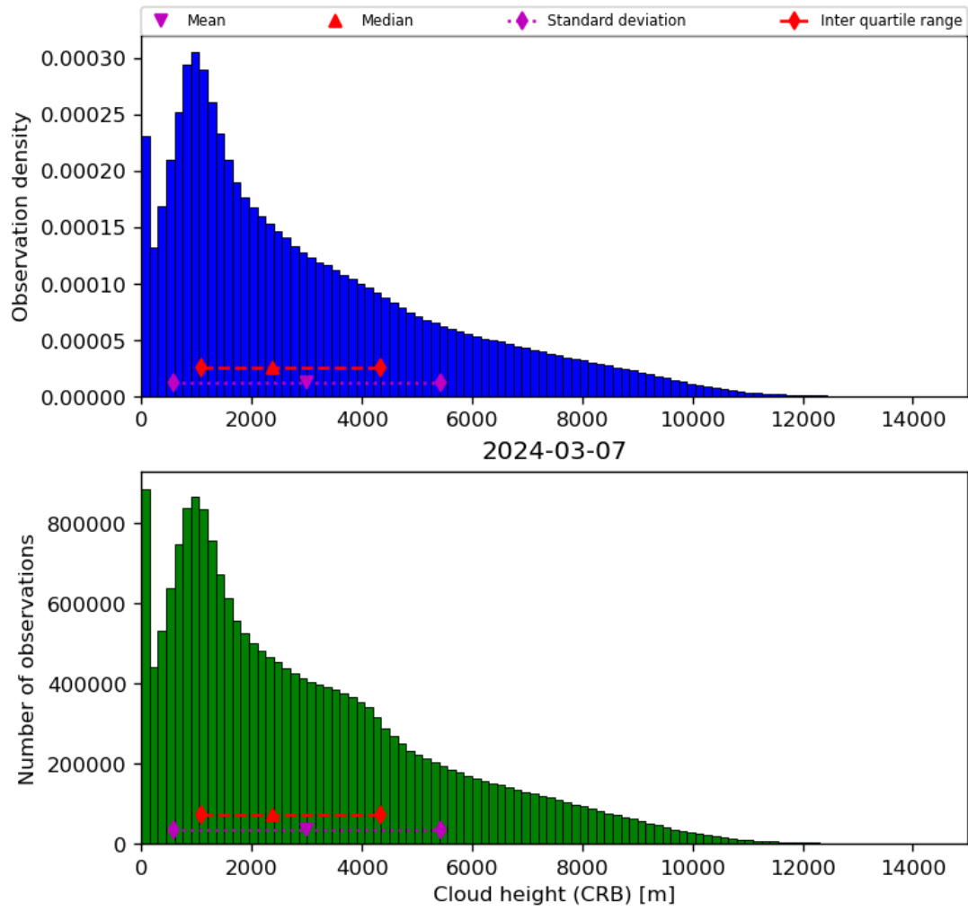
Figure 43: Histogram of “Cloud height (CRB)” for 2024-03-06 to 2024-03-08
