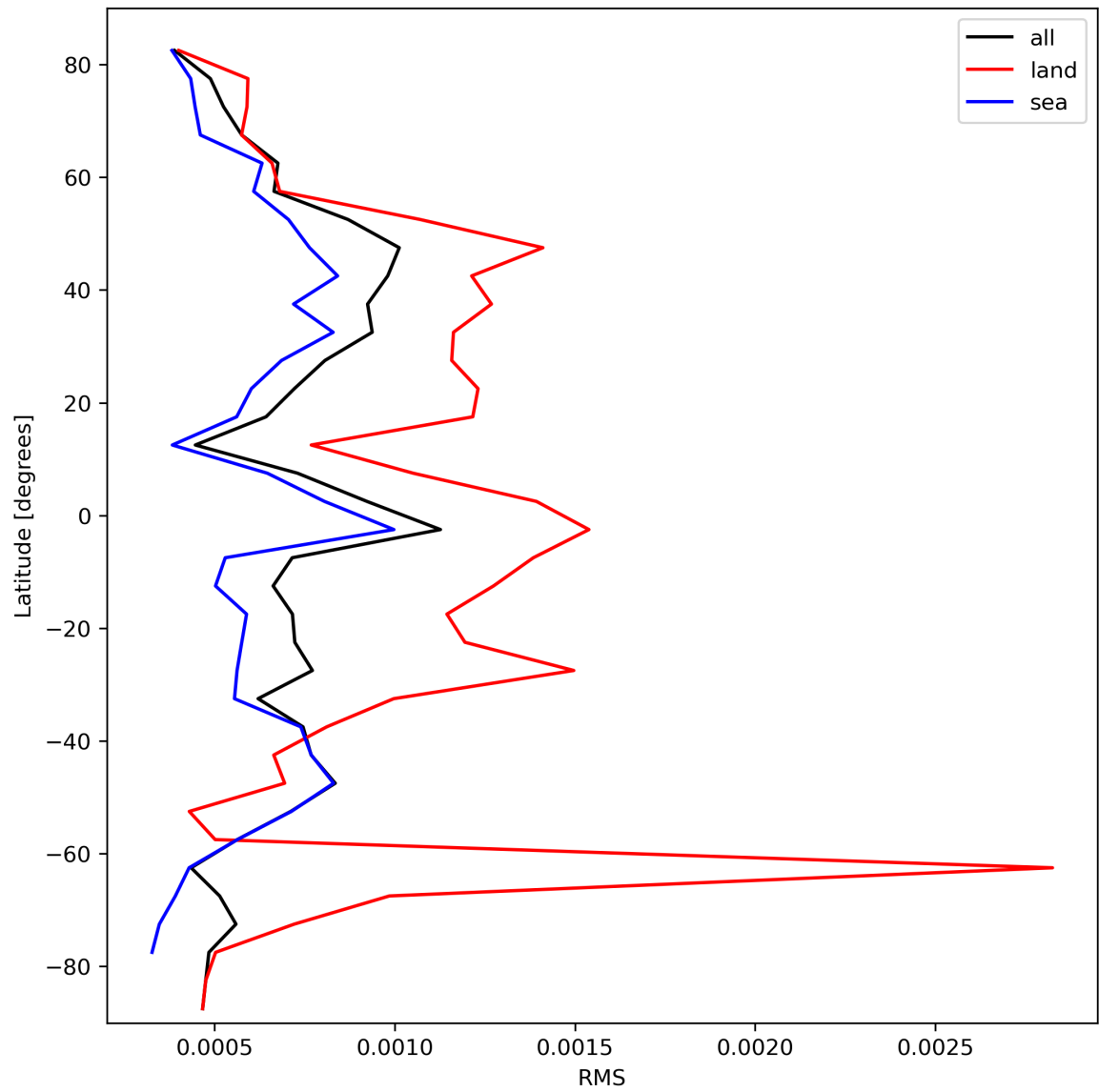
Figure 31: Zonal average of “RMS” for 2024-03-06 to 2024-03-08.
