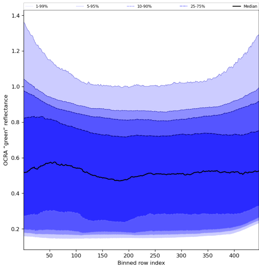
Figure 68: Along track statistics of "OCRA "green" reflectance" for 2024-03-06 to 2024-03-08
