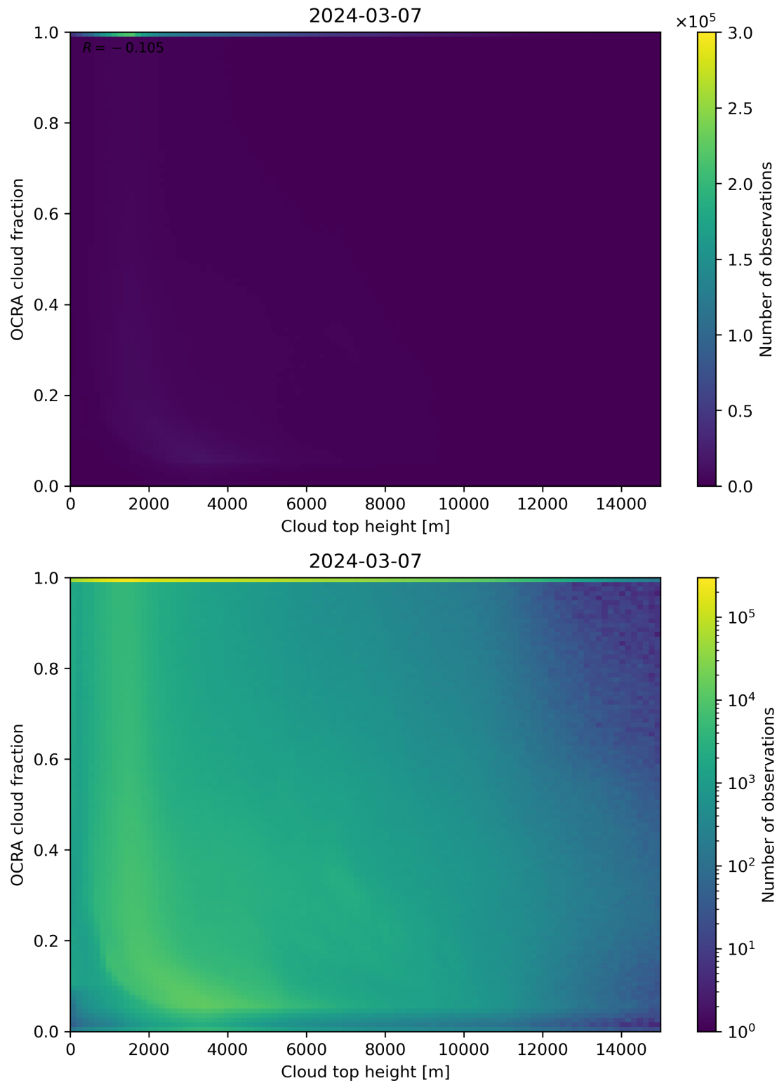
Figure 87: Scatter density plot of “Cloud top height” against “OCRA cloud fraction” for 2024-03-06 to 2024-03-08.
