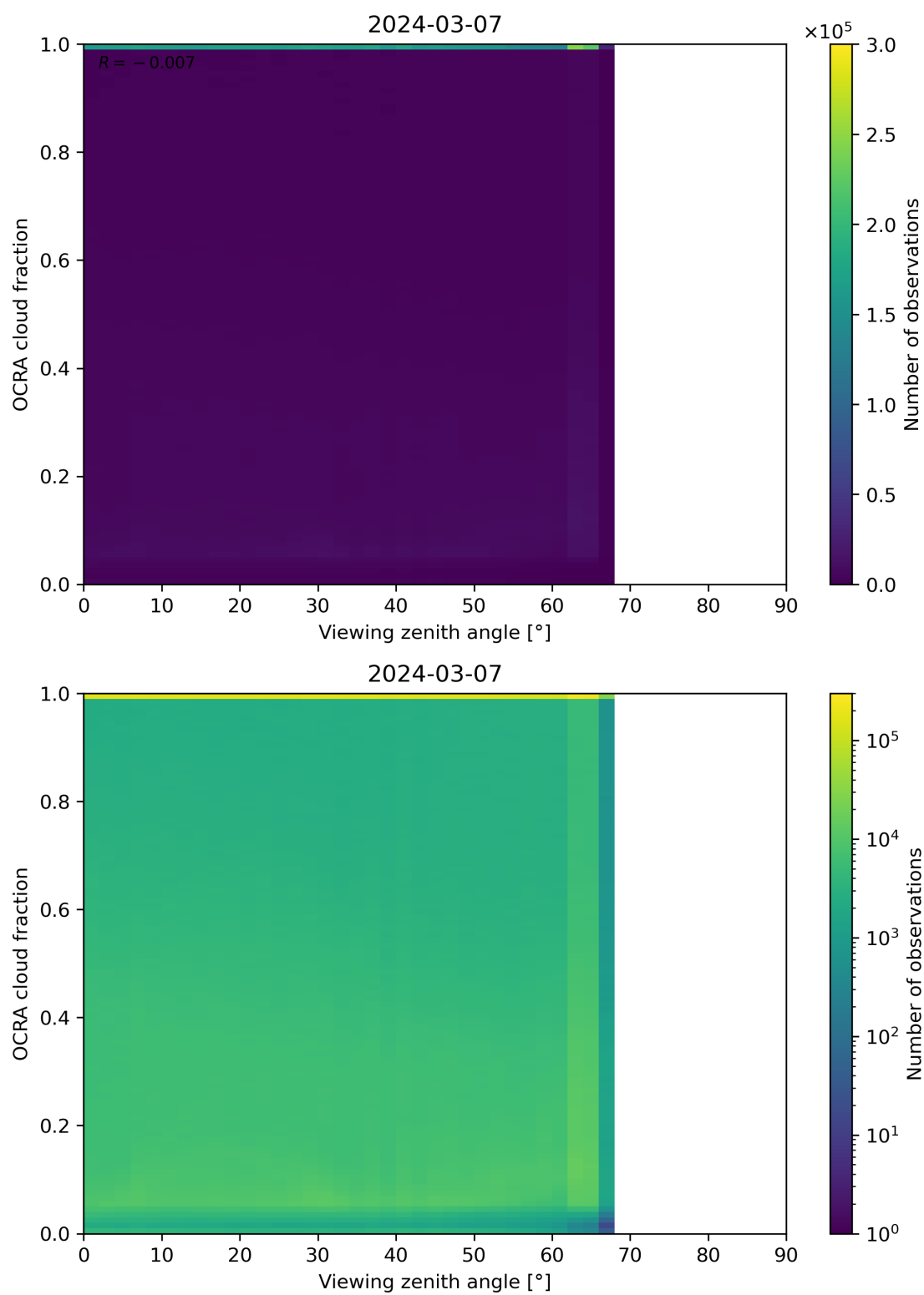
Figure 108: Scatter density plot of “Viewing zenith angle” against “OCRA cloud fraction” for 2024-03-06 to 2024-03-08.
