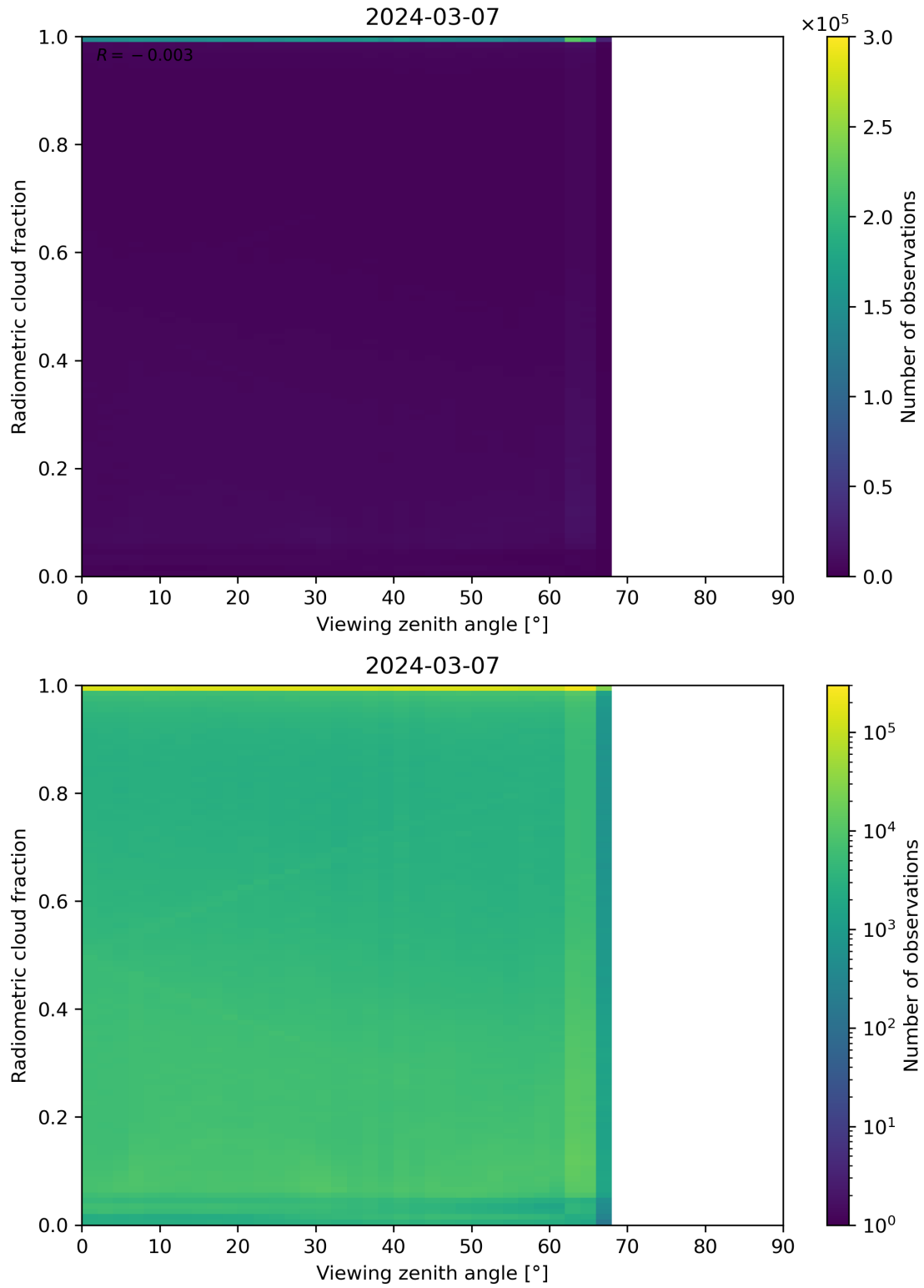
Figure 107: Scatter density plot of “Viewing zenith angle” against “Radiometric cloud fraction” for 2024-03-06 to 2024-03-08.
