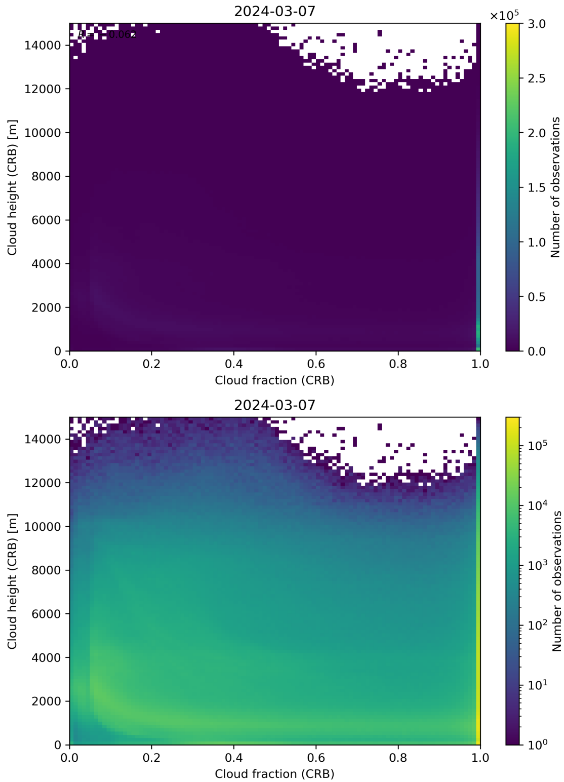
Figure 79: Scatter density plot of “Cloud fraction (CRB)” against “Cloud height (CRB)” for 2024-03-06 to 2024-03-08.
