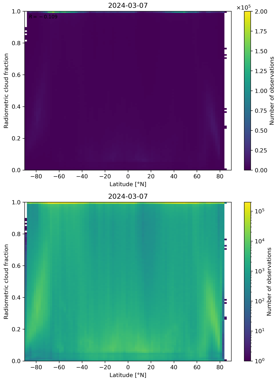
Figure 92: Scatter density plot of “Latitude” against “Radiometric cloud fraction” for 2024-03-06 to 2024-03-08.
