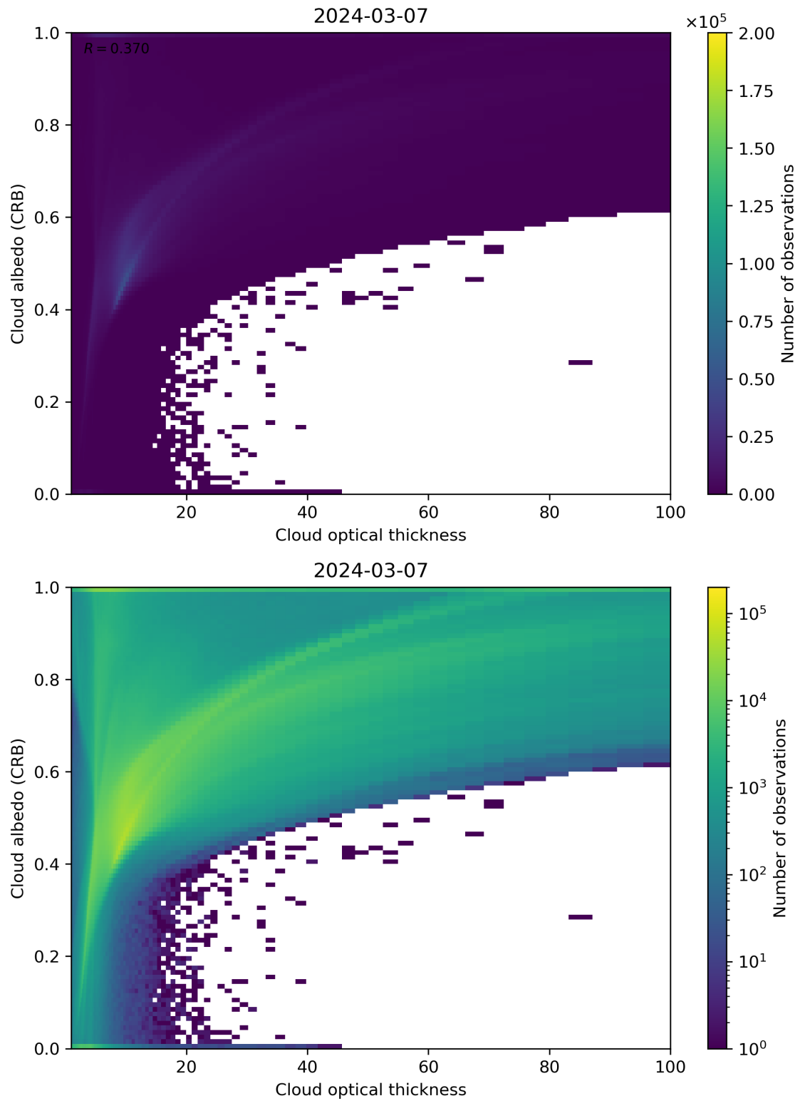
Figure 82: Scatter density plot of “Cloud optical thickness” against “Cloud albedo (CRB)” for 2024-03-06 to 2024-03-08.
