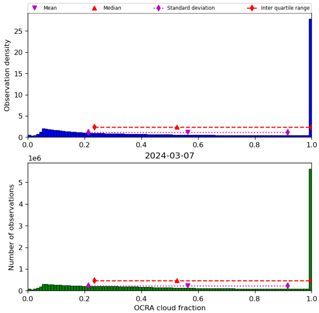
Figure 50: Histogram of “OCRA cloud fraction” for 2024-03-06 to 2024-03-08
