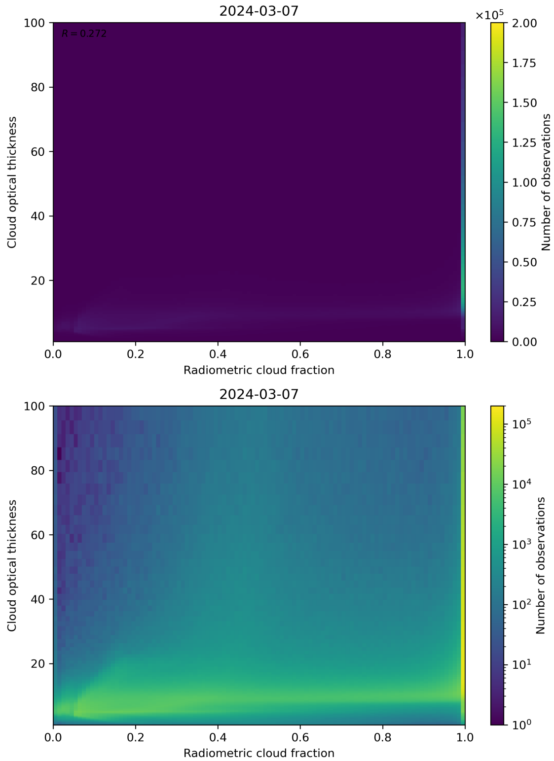
Figure 75: Scatter density plot of “Radiometric cloud fraction” against “Cloud optical thickness” for 2024-03-06 to 2024-03-08.
