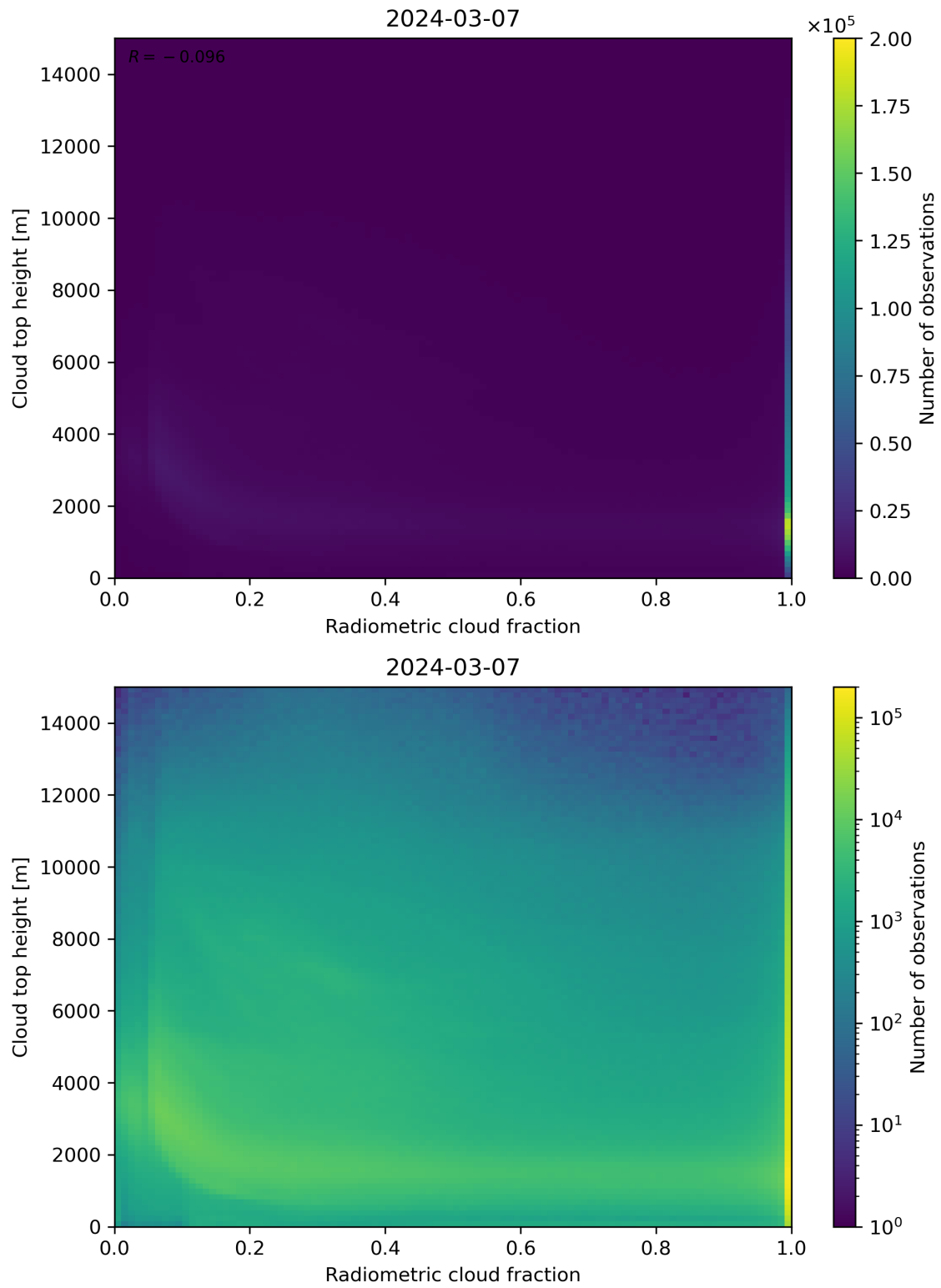
Figure 76: Scatter density plot of “Radiometric cloud fraction” against “Cloud top height” for 2024-03-06 to 2024-03-08.
