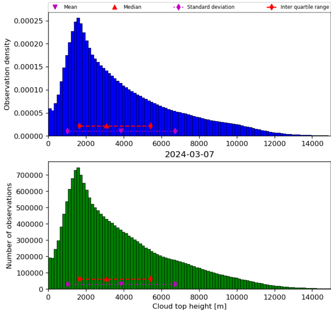
Figure 40: Histogram of “Cloud top height” for 2024-03-06 to 2024-03-08
