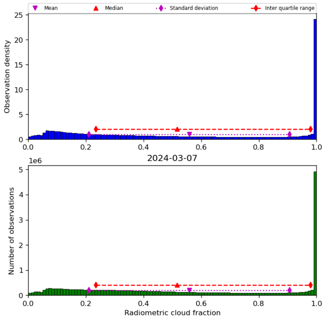
Figure 39: Histogram of “Radiometric cloud fraction” for 2024-03-06 to 2024-03-08
