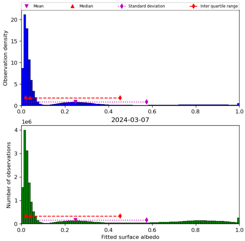
Figure 45: Histogram of “Fitted surface albedo” for 2024-03-06 to 2024-03-08
