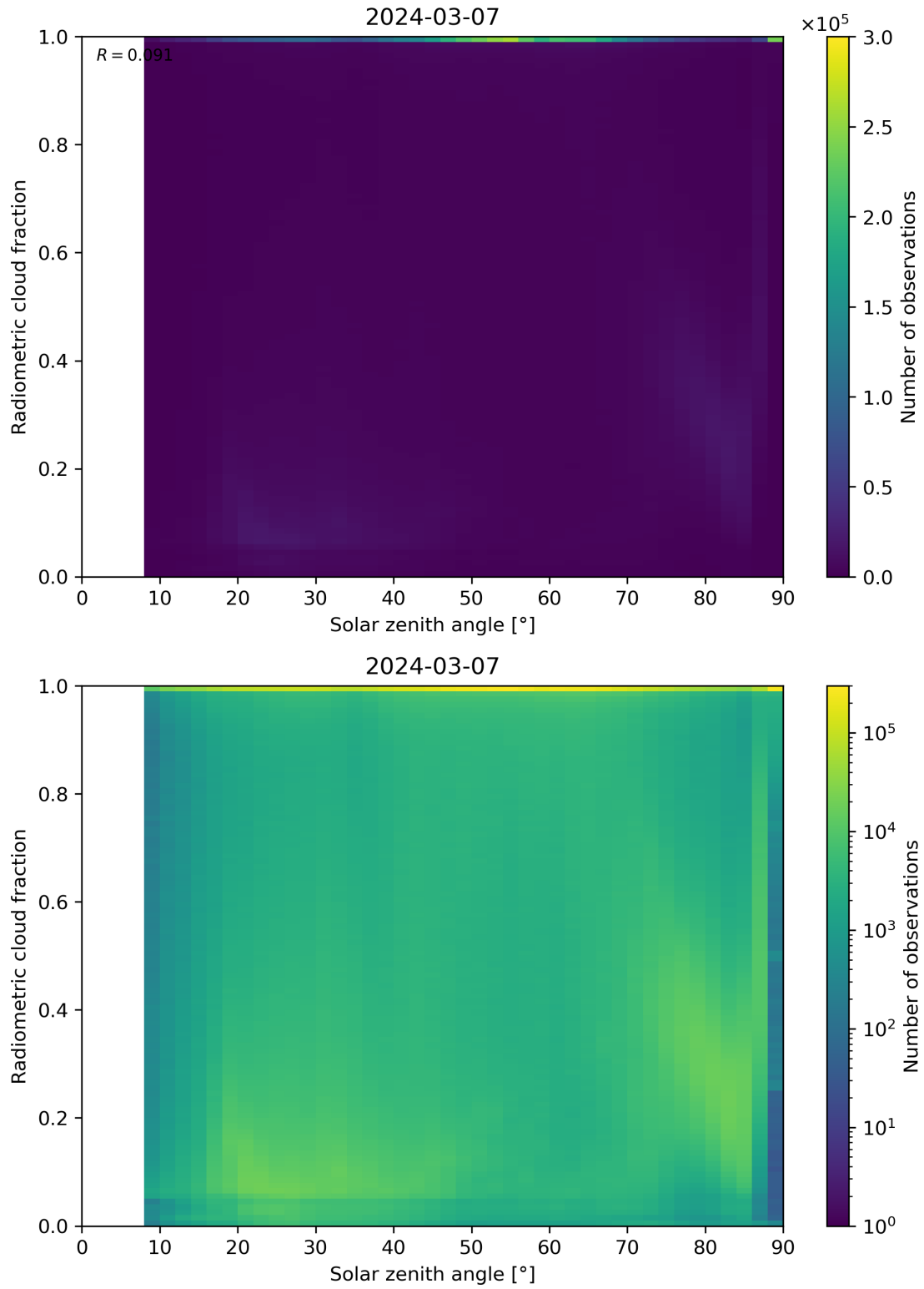
Figure 99: Scatter density plot of “Solar zenith angle” against “Radiometric cloud fraction” for 2024-03-06 to 2024-03-08.
