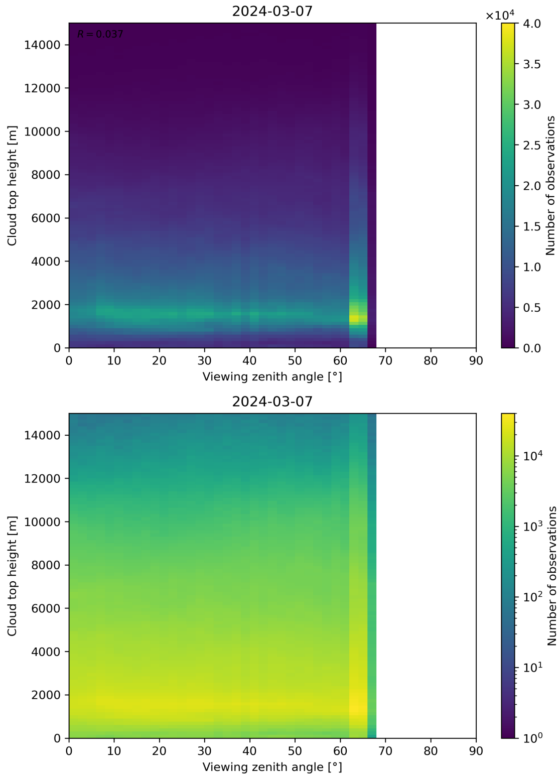
Figure 112: Scatter density plot of “Viewing zenith angle” against “Cloud top height” for 2024-03-06 to 2024-03-08.
