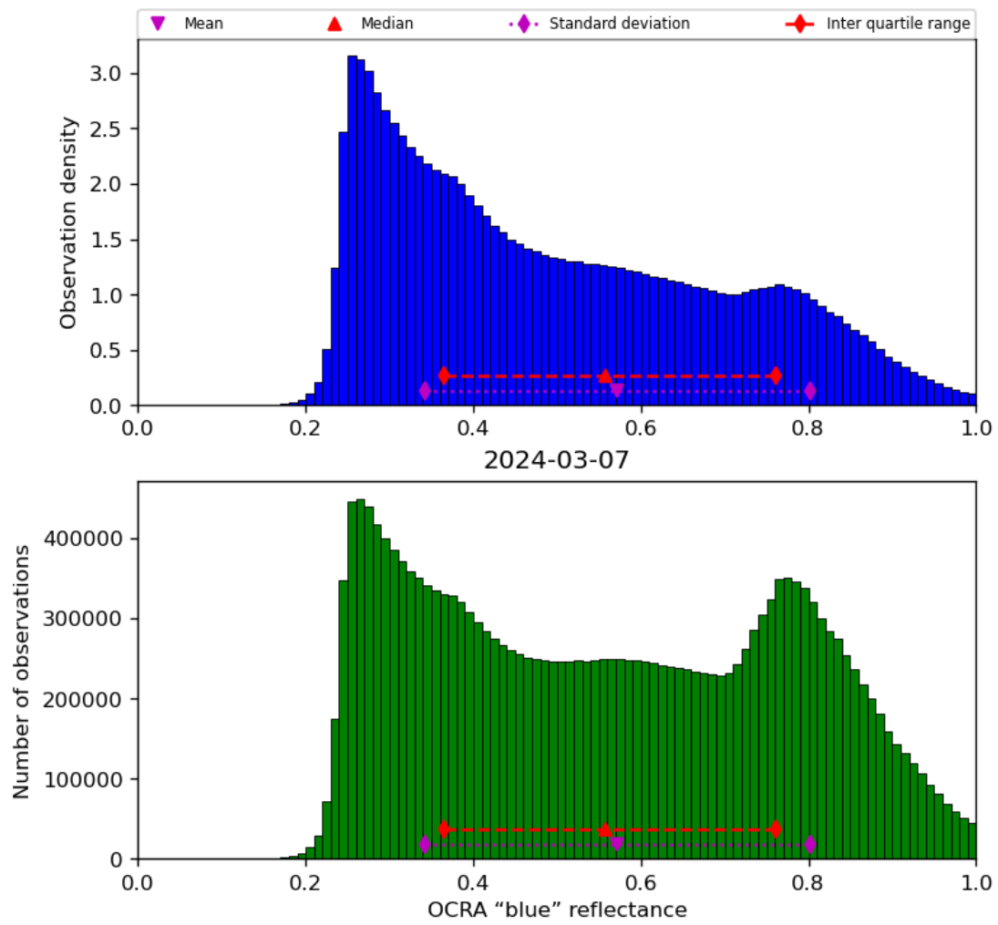
Figure 51: Histogram of “OCRA “blue” reflectance” for 2024-03-06 to 2024-03-08
