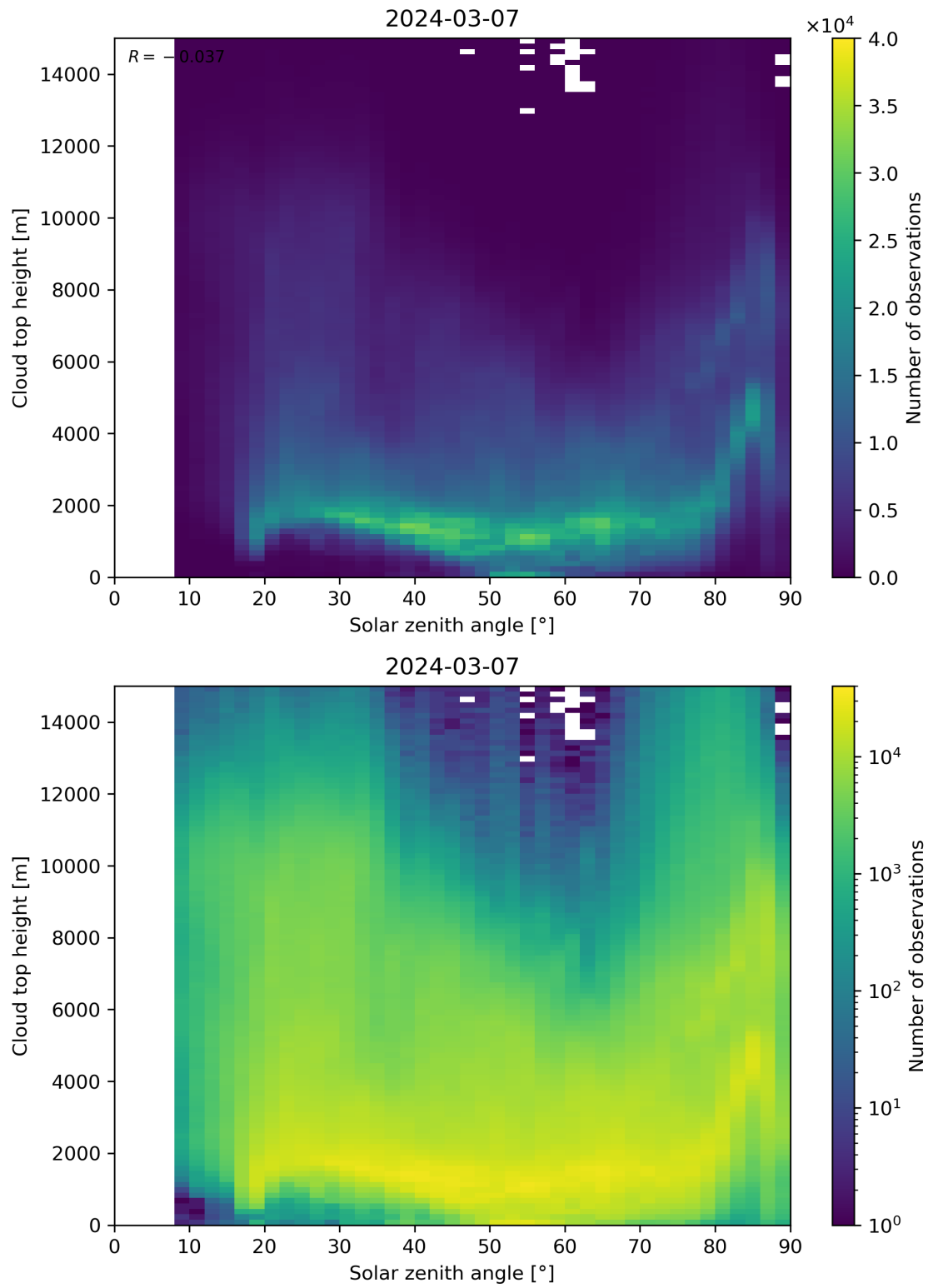
Figure 104: Scatter density plot of “Solar zenith angle” against “Cloud top height” for 2024-03-06 to 2024-03-08.
