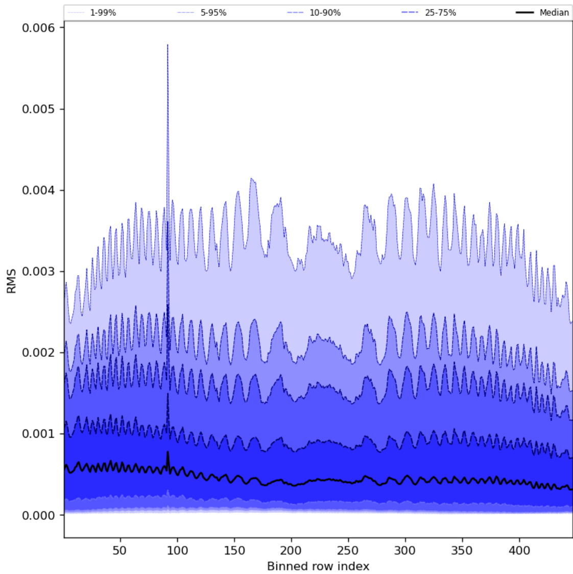
Figure 63: Along track statistics of “RMS” for 2024-03-06 to 2024-03-08
