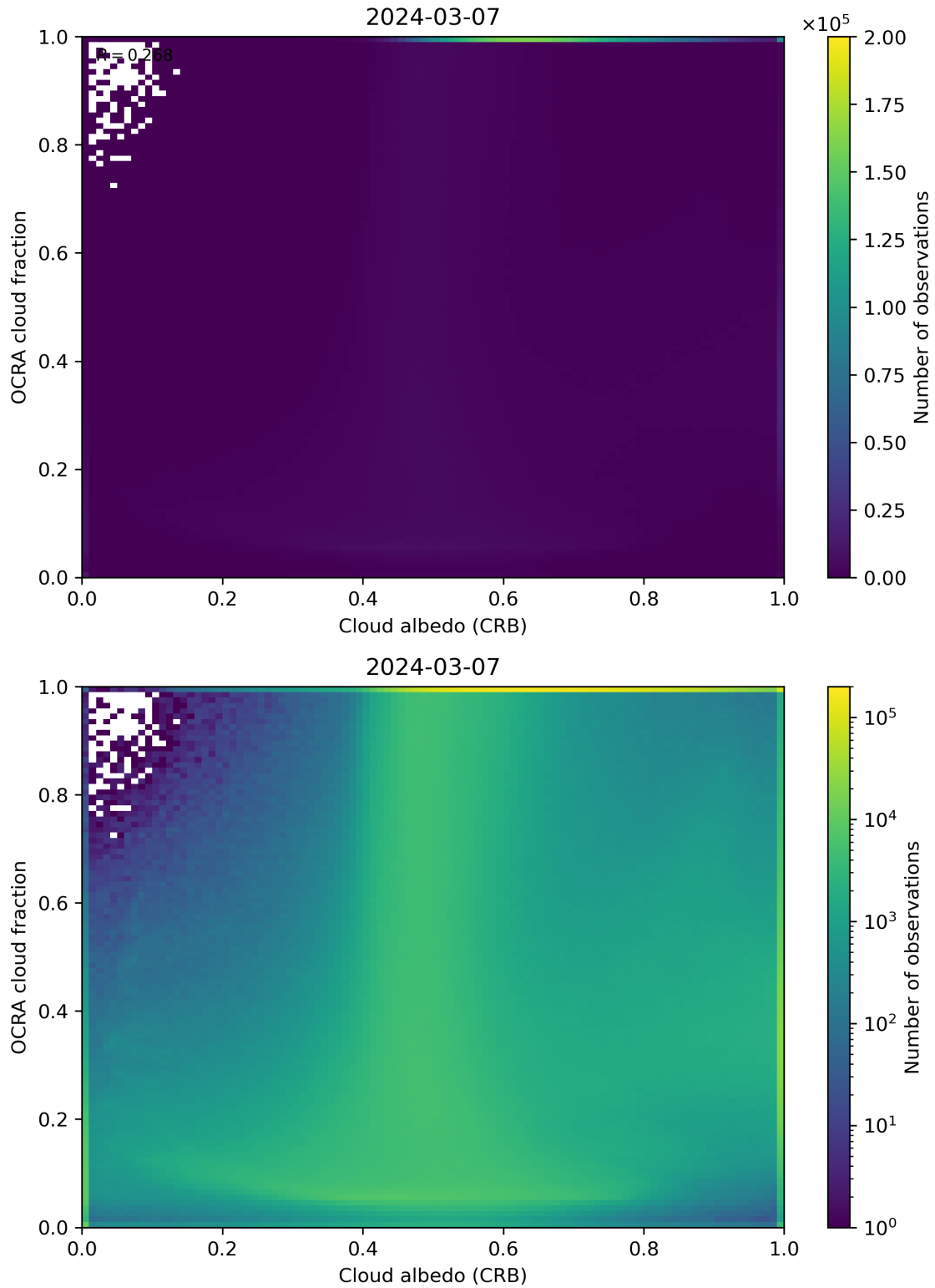
Figure 70: Scatter density plot of “Cloud albedo (CRB)” against “OCRA cloud fraction” for 2024-03-06 to 2024-03-08.
