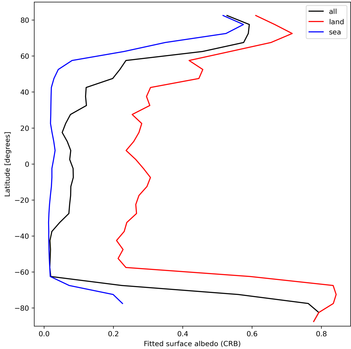
Figure 30: Zonal average of “Fitted surface albedo (CRB)” for 2024-03-06 to 2024-03-08.
