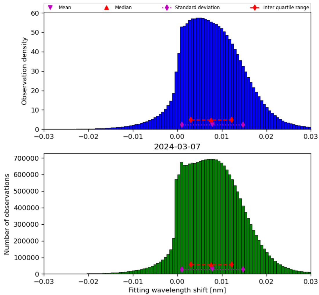
Figure 49: Histogram of “Fitting wavelength shift” for 2024-03-06 to 2024-03-08
