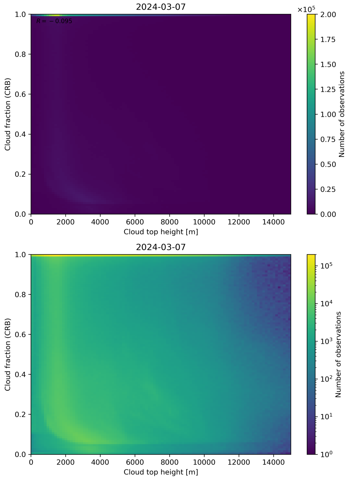
Figure 88: Scatter density plot of “Cloud top height” against “Cloud fraction (CRB)” for 2024-03-06 to 2024-03-08.
