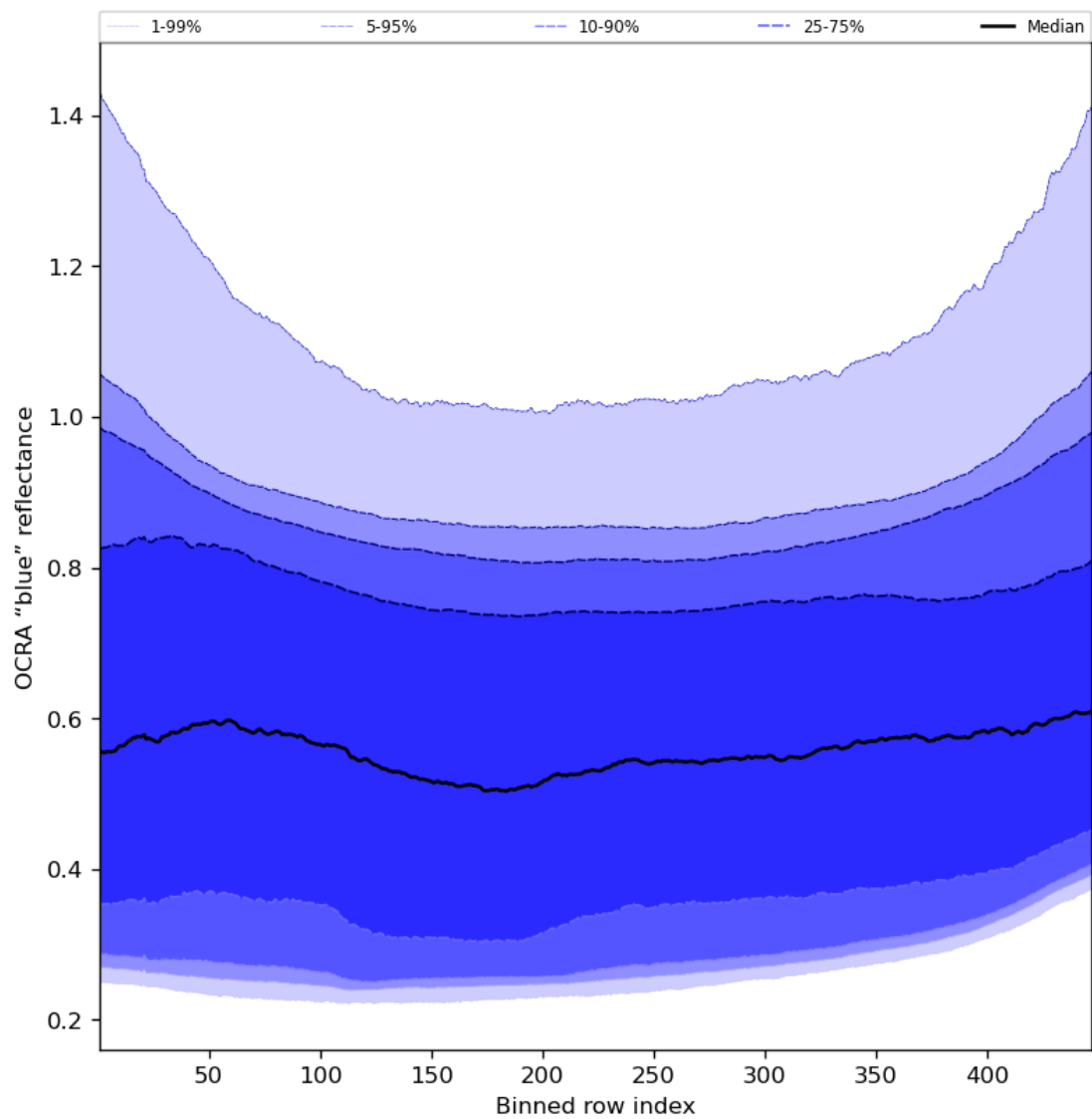
Figure 67: Along track statistics of “OCRA “blue” reflectance” for 2024-03-06 to 2024-03-08
