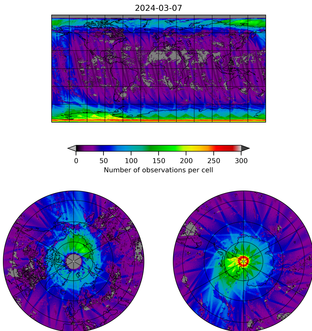
Figure 21: Map of the number of observations for 2024-03-06 to 2024-03-08
