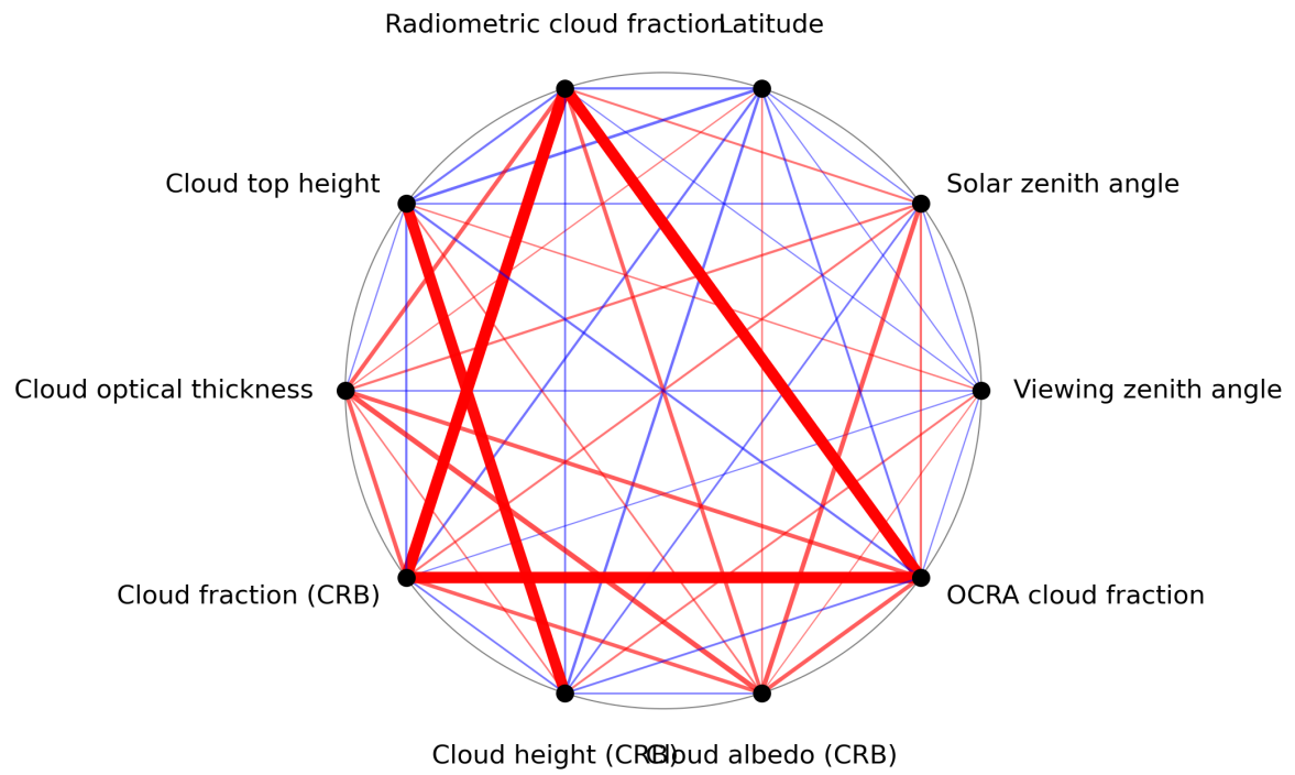
Figure 1: Map of correlation graph for 2024-03-06 to 2024-03-08.
