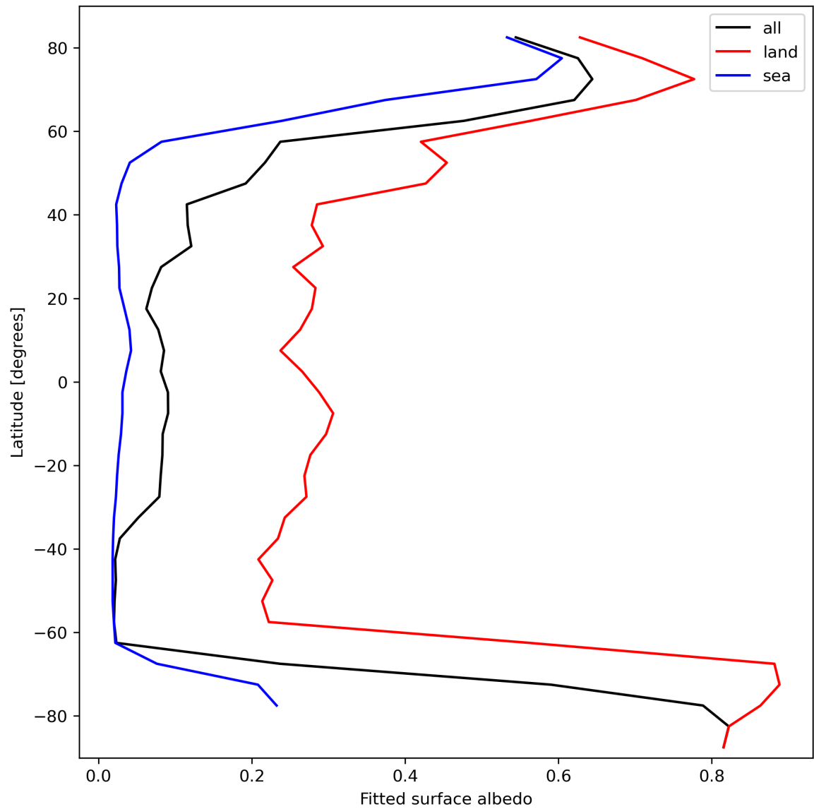
Figure 29: Zonal average of “Fitted surface albedo” for 2024-03-06 to 2024-03-08.
