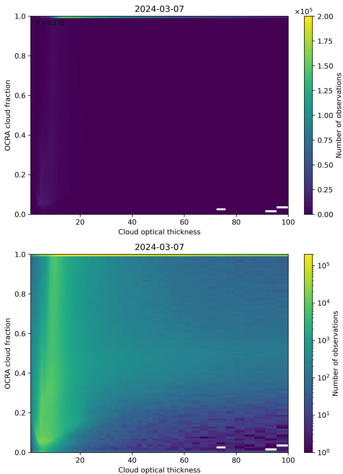
Figure 83: Scatter density plot of “Cloud optical thickness” against “OCRA cloud fraction” for 2024-03-06 to 2024-03-08.
