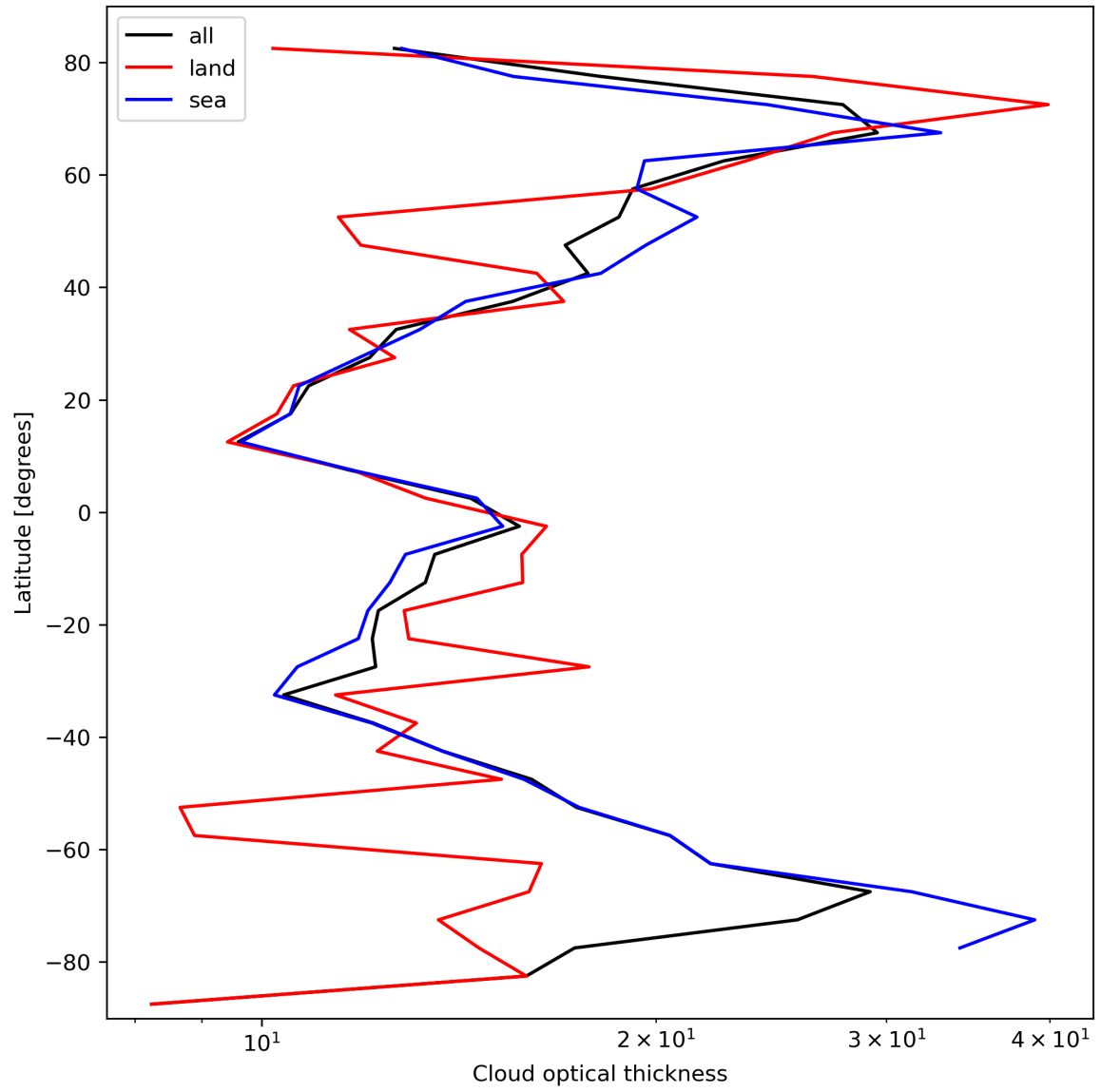
Figure 25: Zonal average of “Cloud optical thickness” for 2024-03-06 to 2024-03-08.
