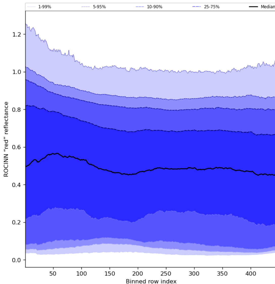
Figure 69: Along track statistics of “ROCINN “red” reflectance” for 2024-03-06 to 2024-03-08
