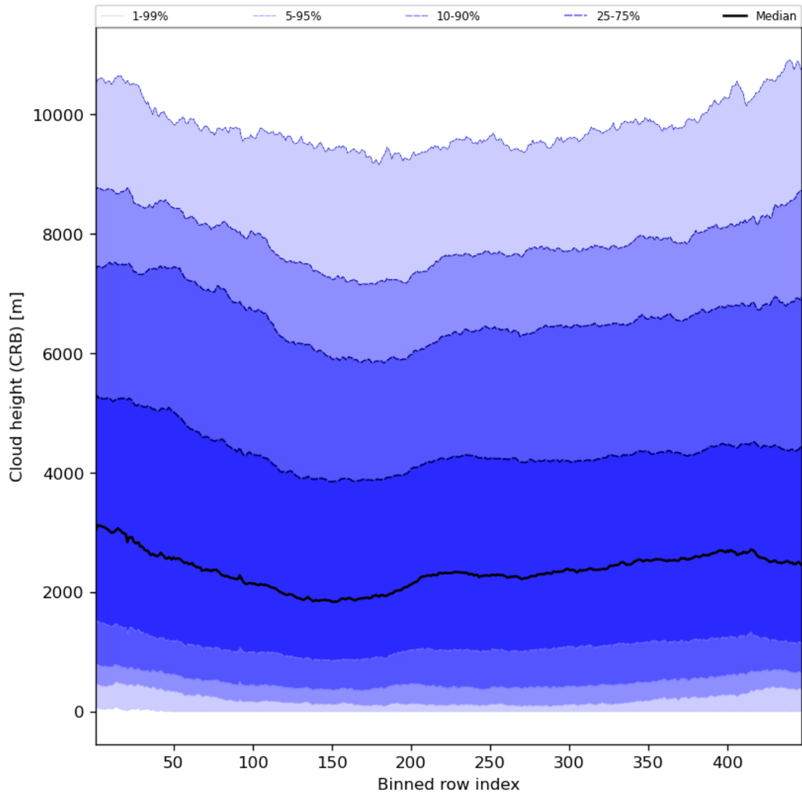
Figure 59: Along track statistics of “Cloud height (CRB)” for 2024-03-06 to 2024-03-08
