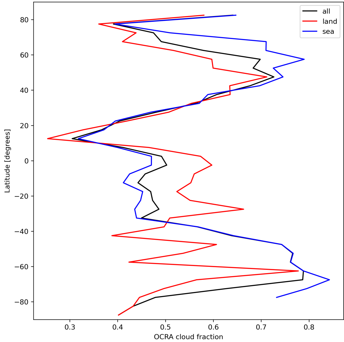
Figure 34: Zonal average of “OCRA cloud fraction” for 2024-03-06 to 2024-03-08.
