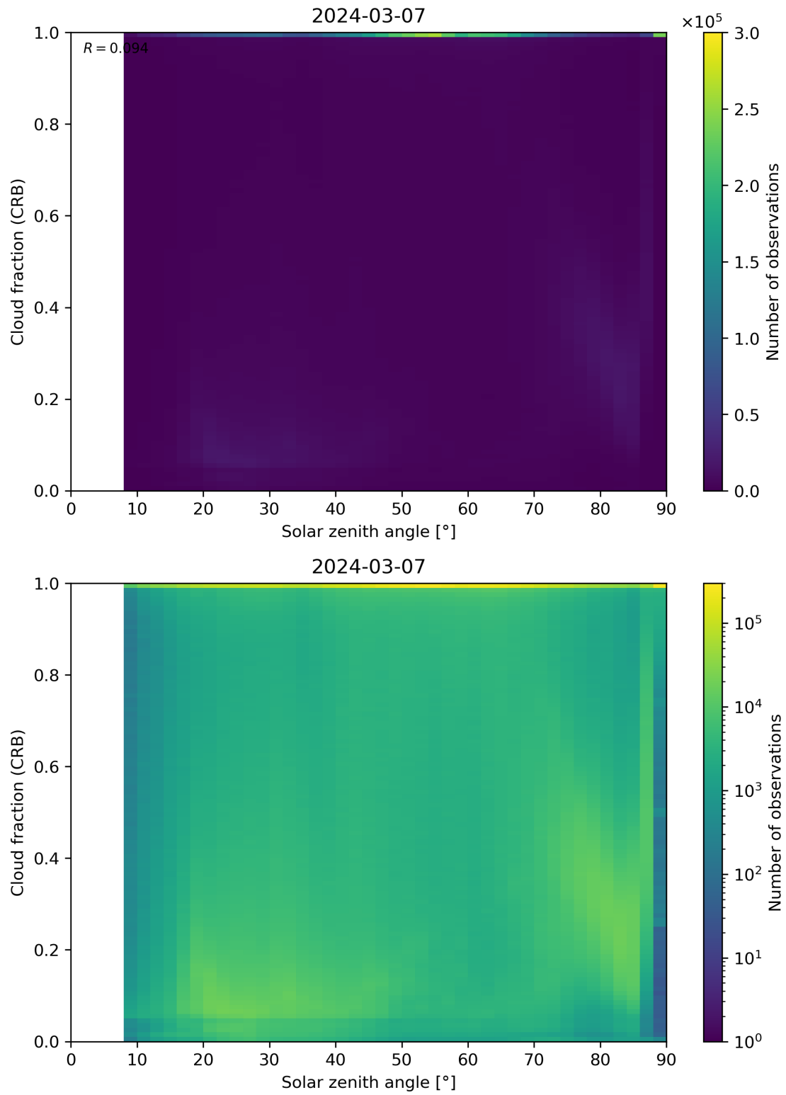
Figure 101: Scatter density plot of “Solar zenith angle” against “Cloud fraction (CRB)” for 2024-03-06 to 2024-03-08.
