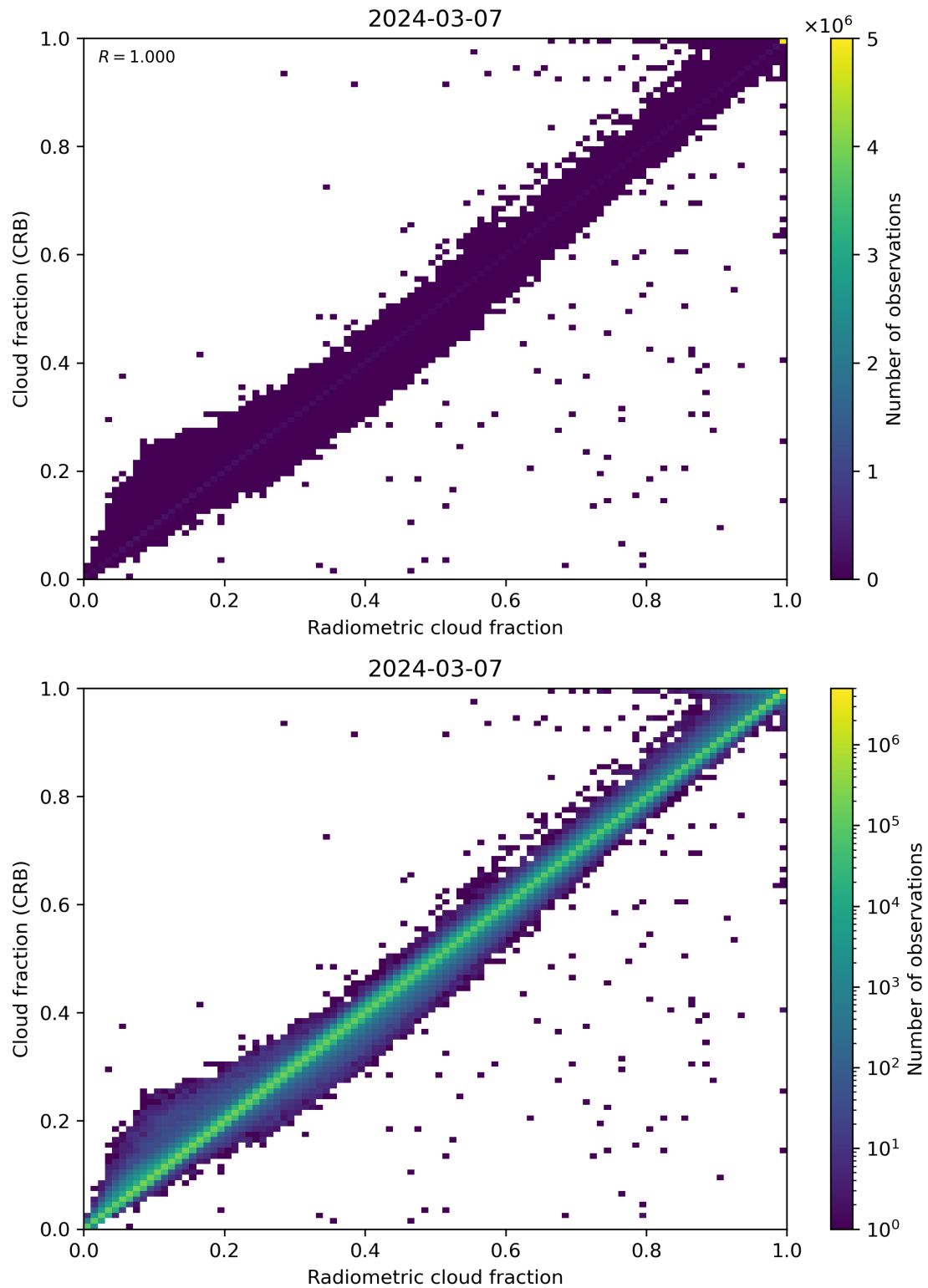
Figure 73: Scatter density plot of “Radiometric cloud fraction” against “Cloud fraction (CRB)” for 2024-03-06 to 2024-03-08.
