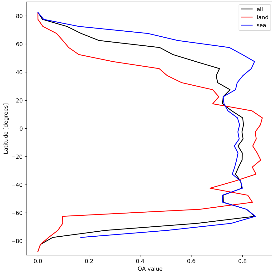
Figure 22: Zonal average of “QA value” for 2024-03-06 to 2024-03-08.
