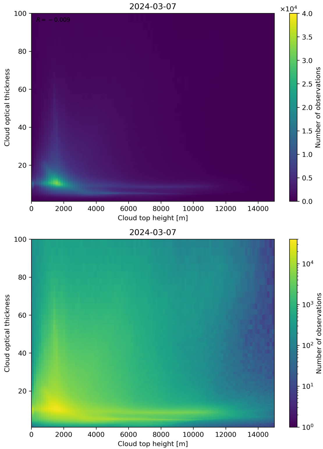
Figure 90: Scatter density plot of “Cloud top height” against “Cloud optical thickness” for 2024-03-06 to 2024-03-08.
