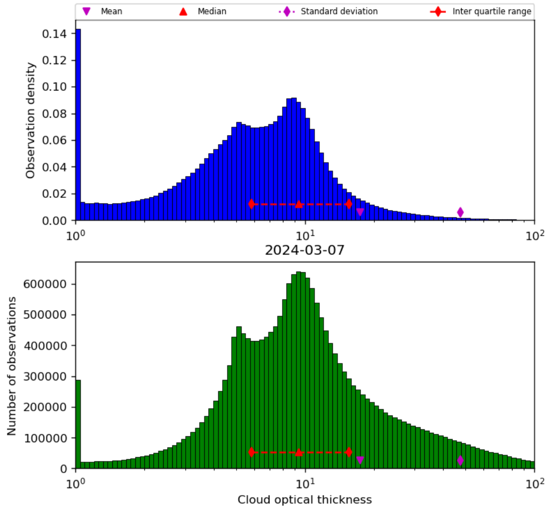
Figure 41: Histogram of “Cloud optical thickness” for 2024-03-06 to 2024-03-08
