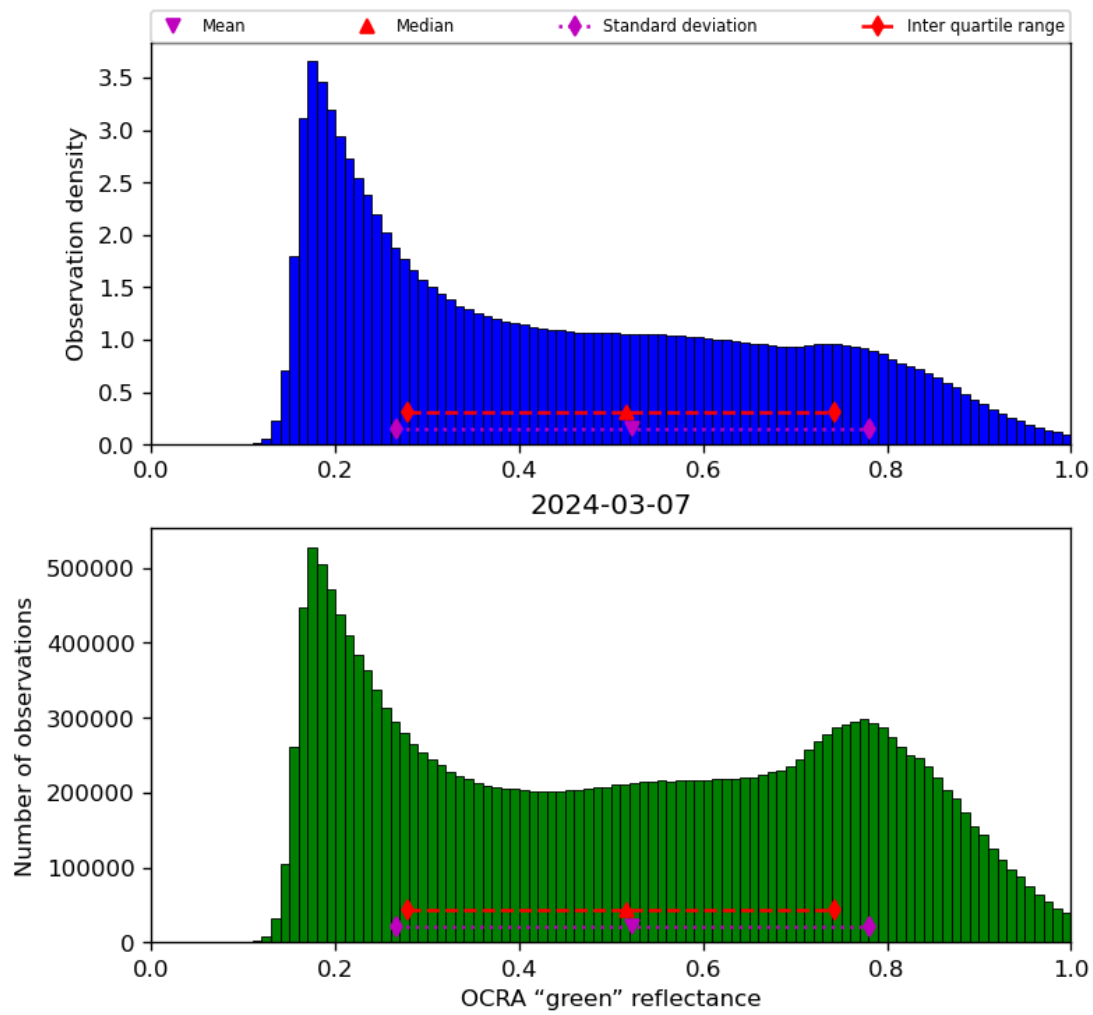
Figure 52: Histogram of “OCRA “green” reflectance” for 2024-03-06 to 2024-03-08
