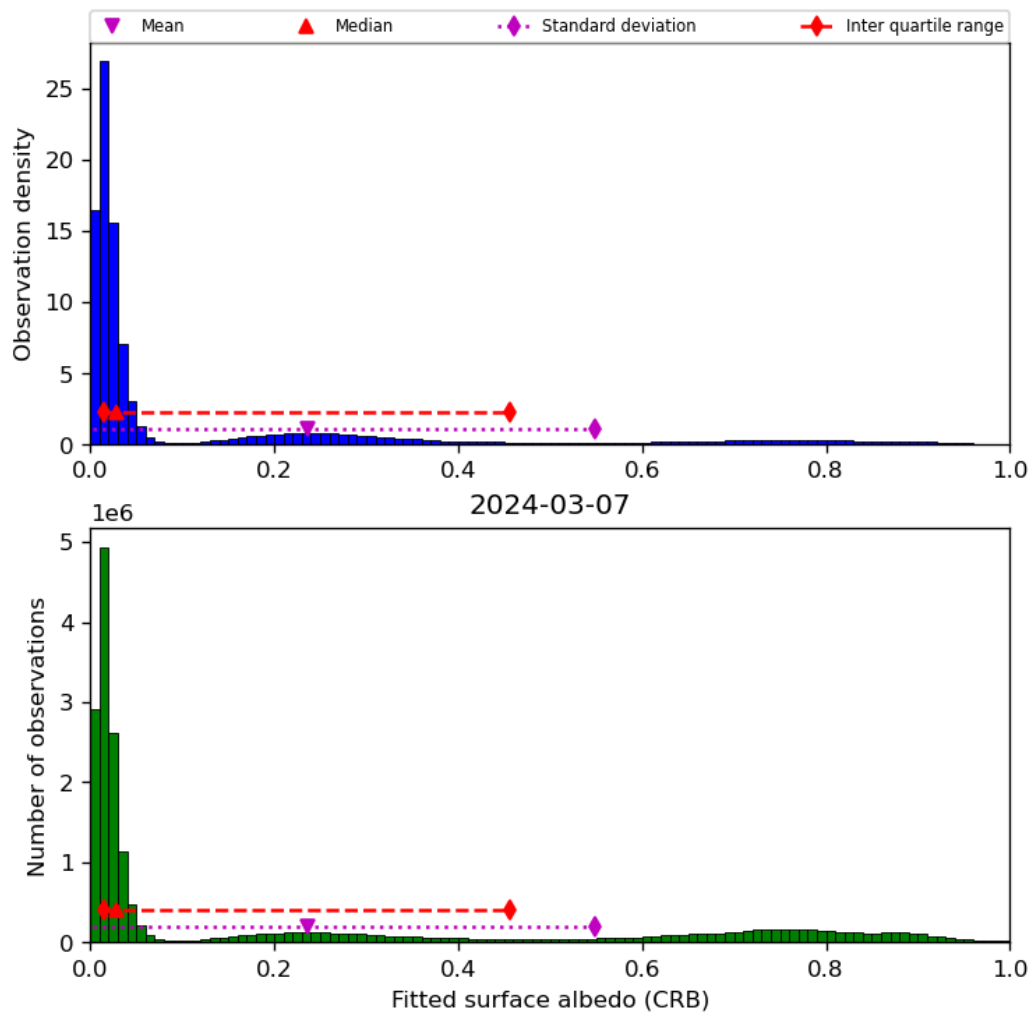
Figure 46: Histogram of “Fitted surface albedo (CRB)” for 2024-03-06 to 2024-03-08
