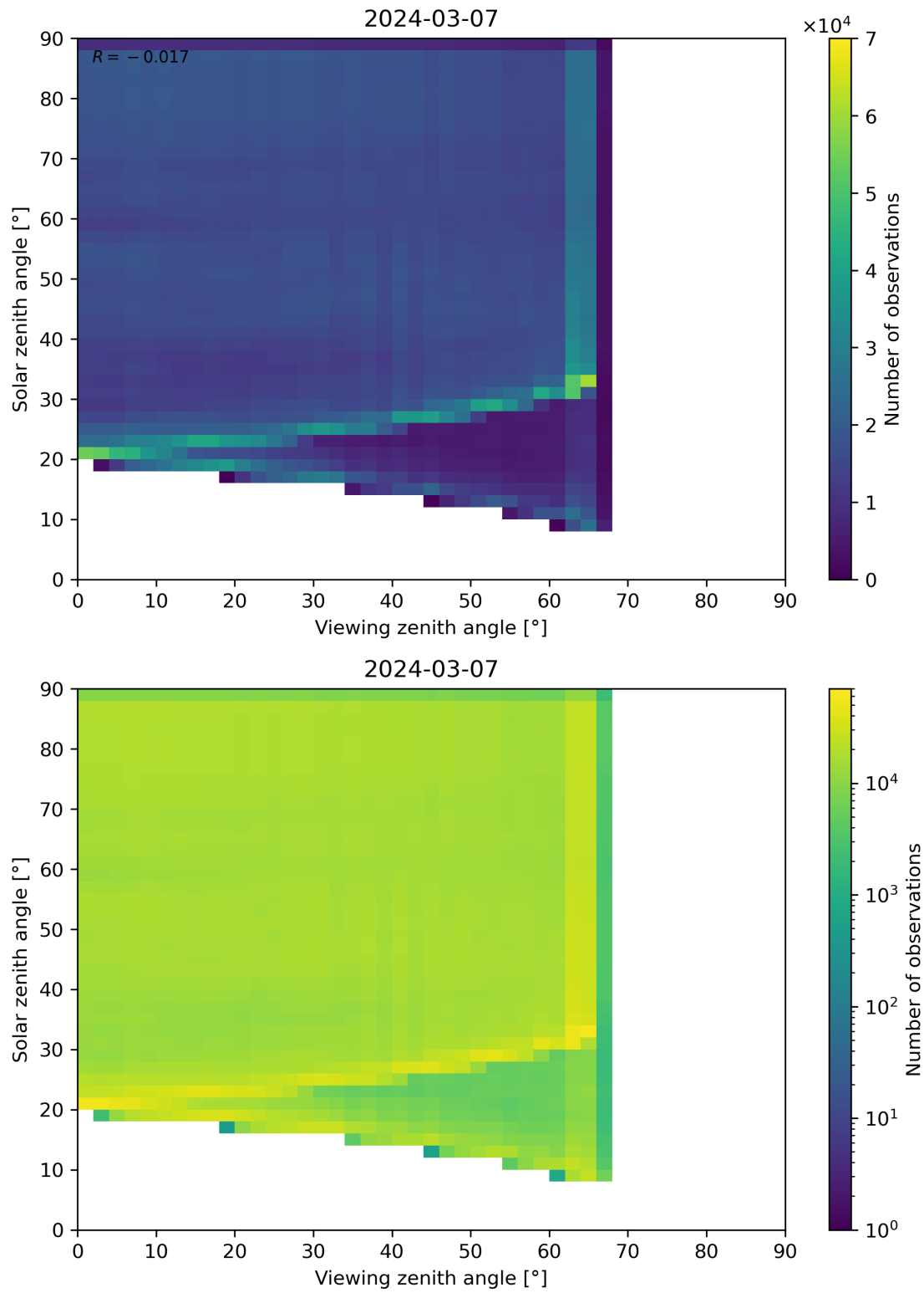
Figure 114: Scatter density plot of “Viewing zenith angle” against “Solar zenith angle” for 2024-03-06 to 2024-03-08.
