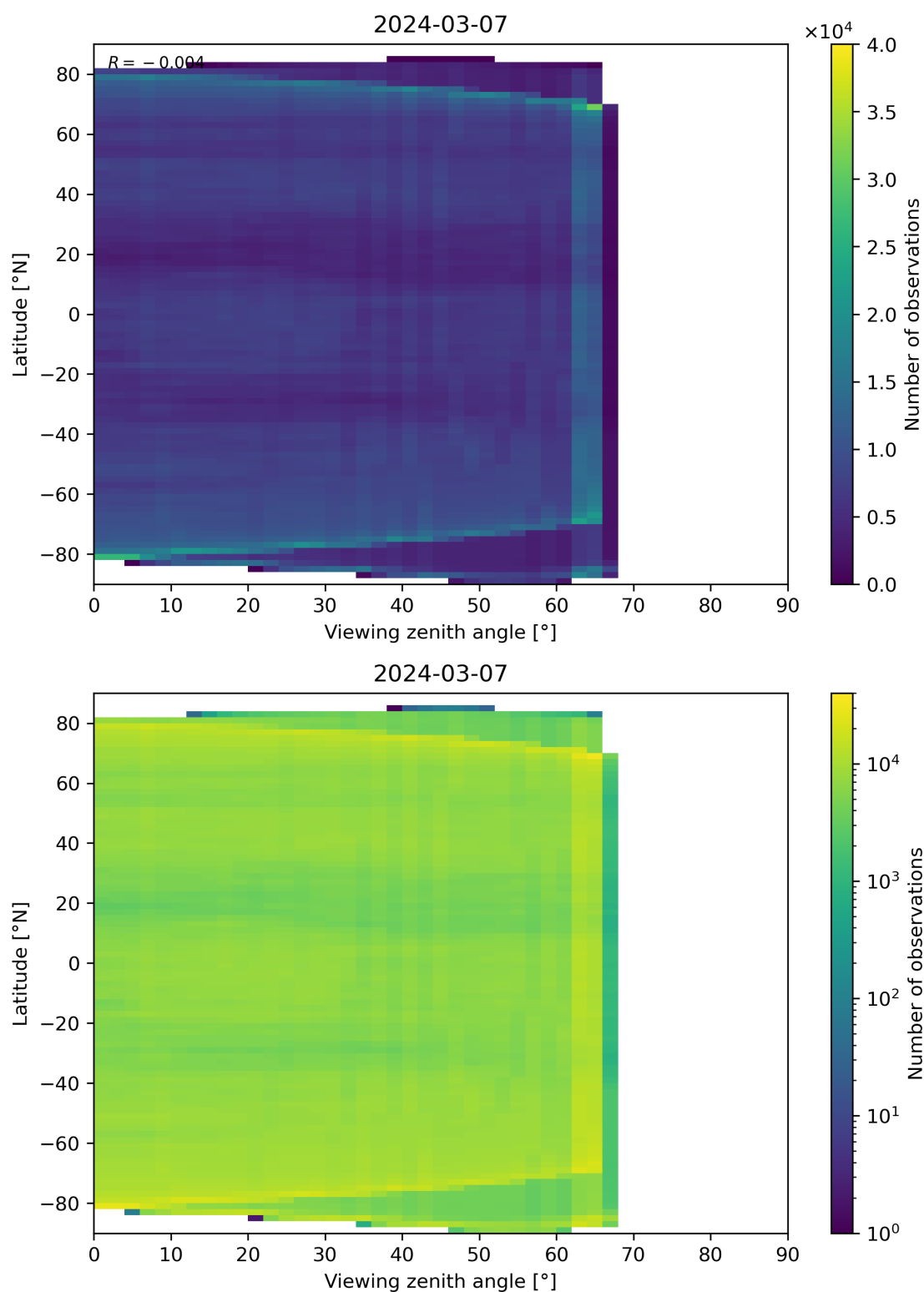
Figure 113: Scatter density plot of “Viewing zenith angle” against “Latitude” for 2024-03-06 to 2024-03-08.
