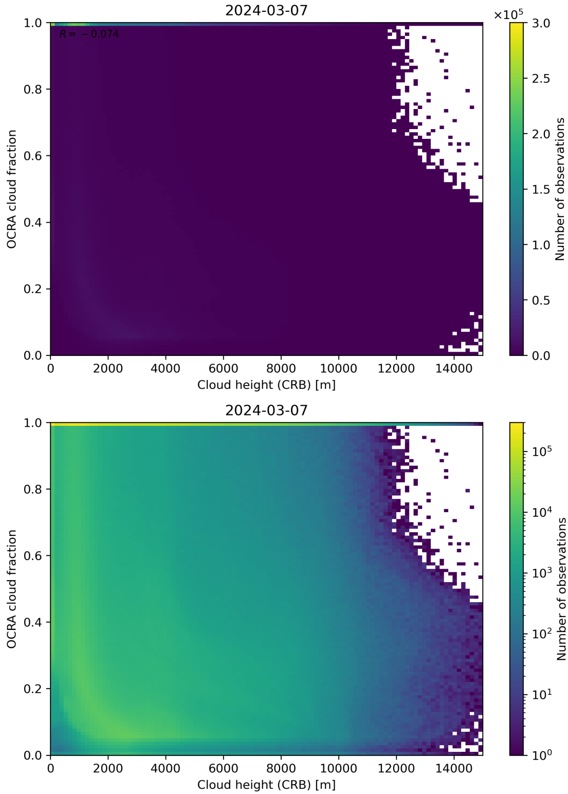
Figure 81: Scatter density plot of “Cloud height (CRB)” against “OCRA cloud fraction” for 2024-03-06 to 2024-03-08.
