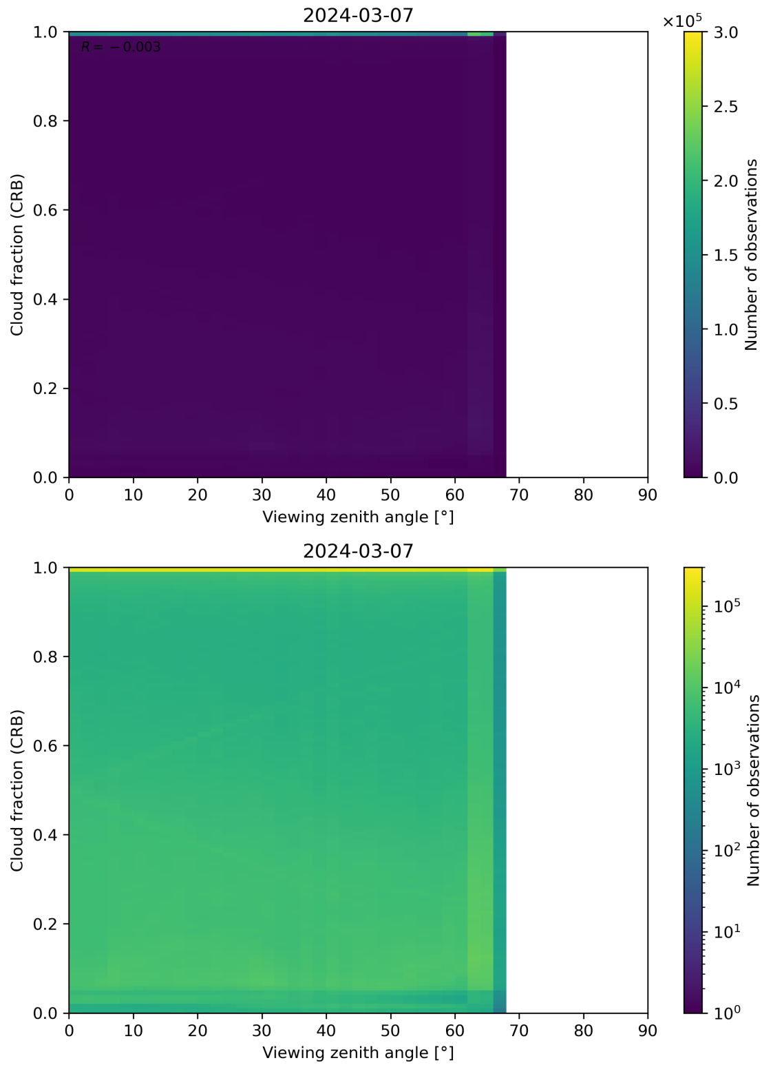
Figure 109: Scatter density plot of “Viewing zenith angle” against “Cloud fraction (CRB)” for 2024-03-06 to 2024-03-08.
