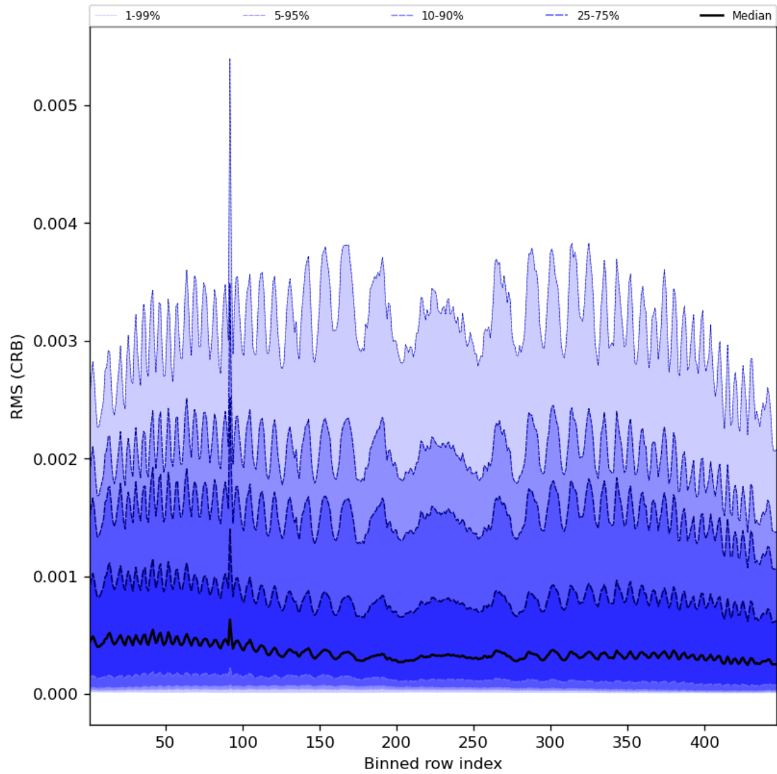
Figure 64: Along track statistics of “RMS (CRB)” for 2024-03-06 to 2024-03-08
