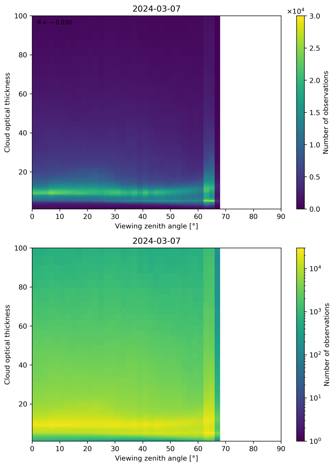
Figure 111: Scatter density plot of “Viewing zenith angle” against “Cloud optical thickness” for 2024-03-06 to 2024-03-08.
