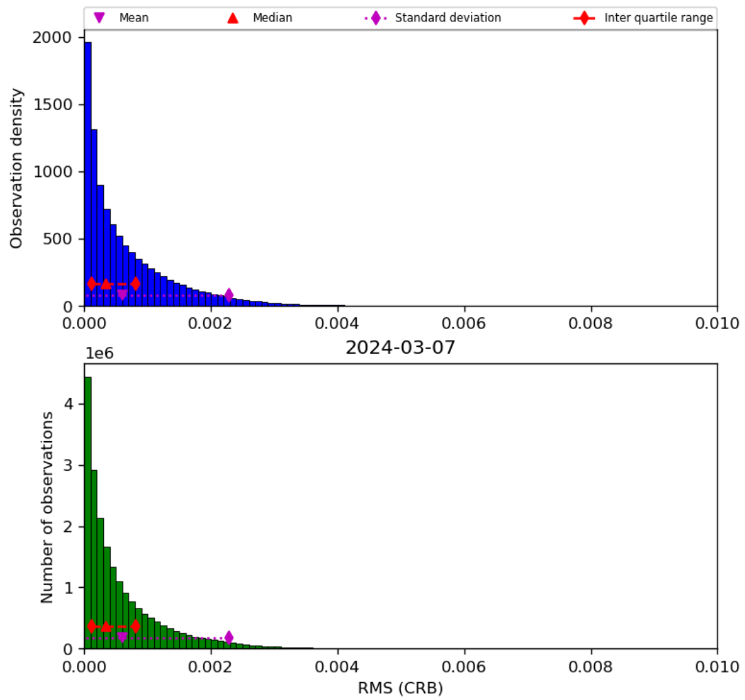
Figure 48: Histogram of “RMS (CRB)” for 2024-03-06 to 2024-03-08
