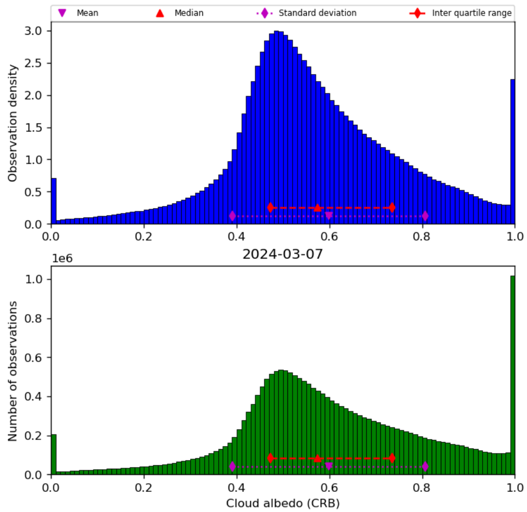
Figure 44: Histogram of “Cloud albedo (CRB)” for 2024-03-06 to 2024-03-08
