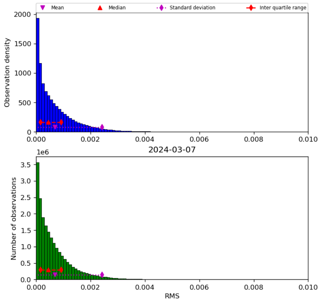
Figure 47: Histogram of “RMS” for 2024-03-06 to 2024-03-08
