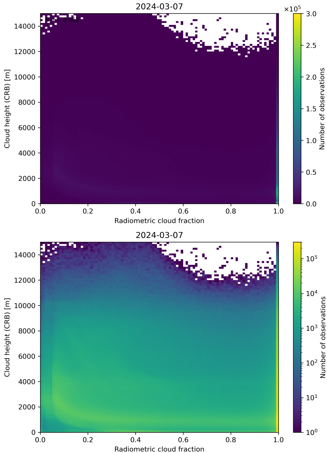
Figure 74: Scatter density plot of “Radiometric cloud fraction” against “Cloud height (CRB)” for 2024-03-06 to 2024-03-08.
