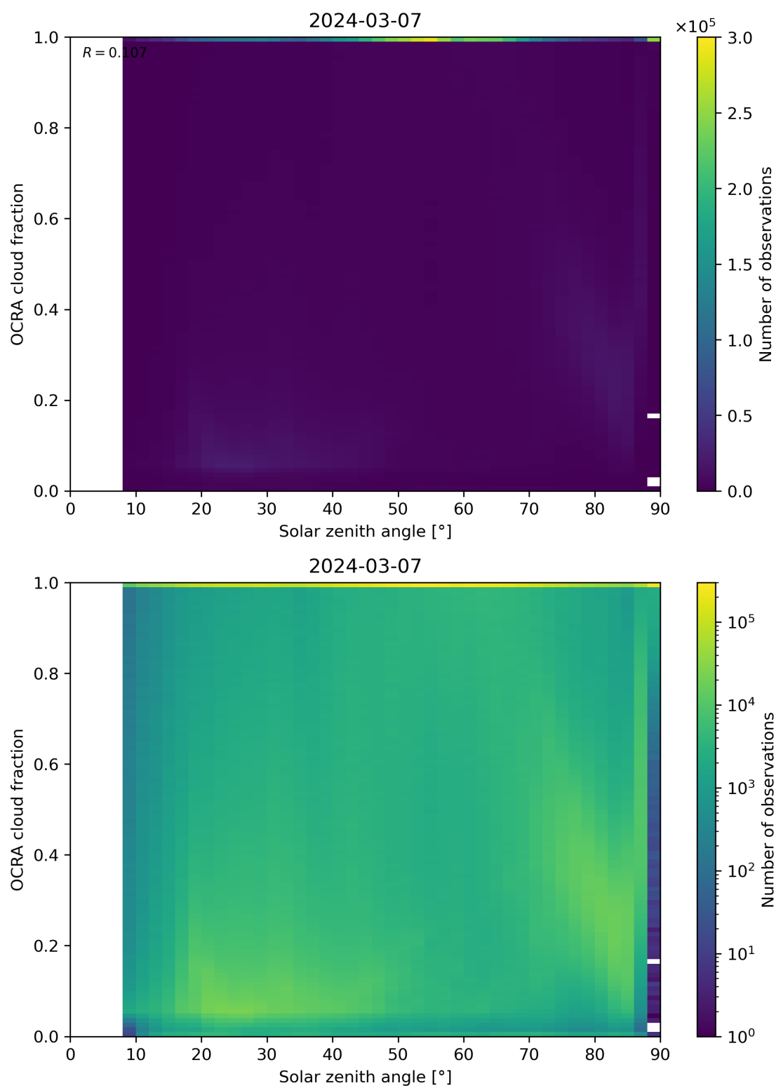
Figure 100: Scatter density plot of “Solar zenith angle” against “OCRA cloud fraction” for 2024-03-06 to 2024-03-08.
