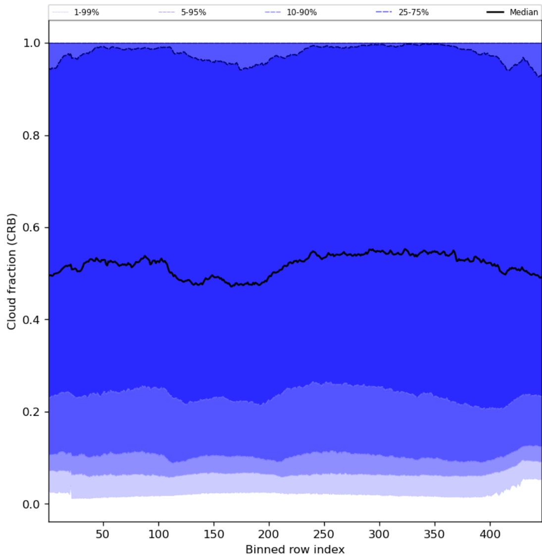
Figure 58: Along track statistics of “Cloud fraction (CRB)” for 2024-03-06 to 2024-03-08
