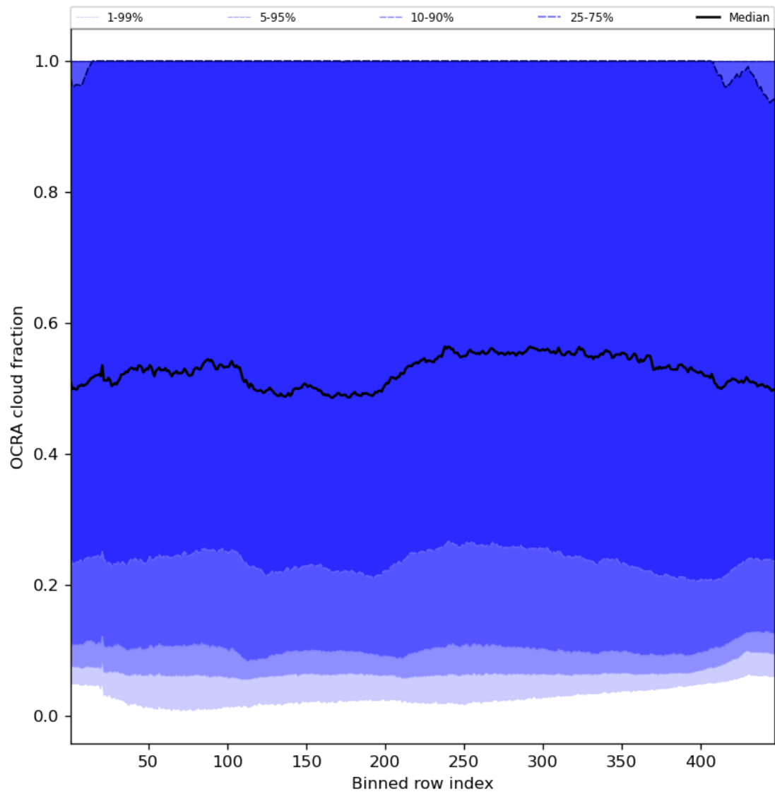
Figure 66: Along track statistics of “OCRA cloud fraction” for 2024-03-06 to 2024-03-08
