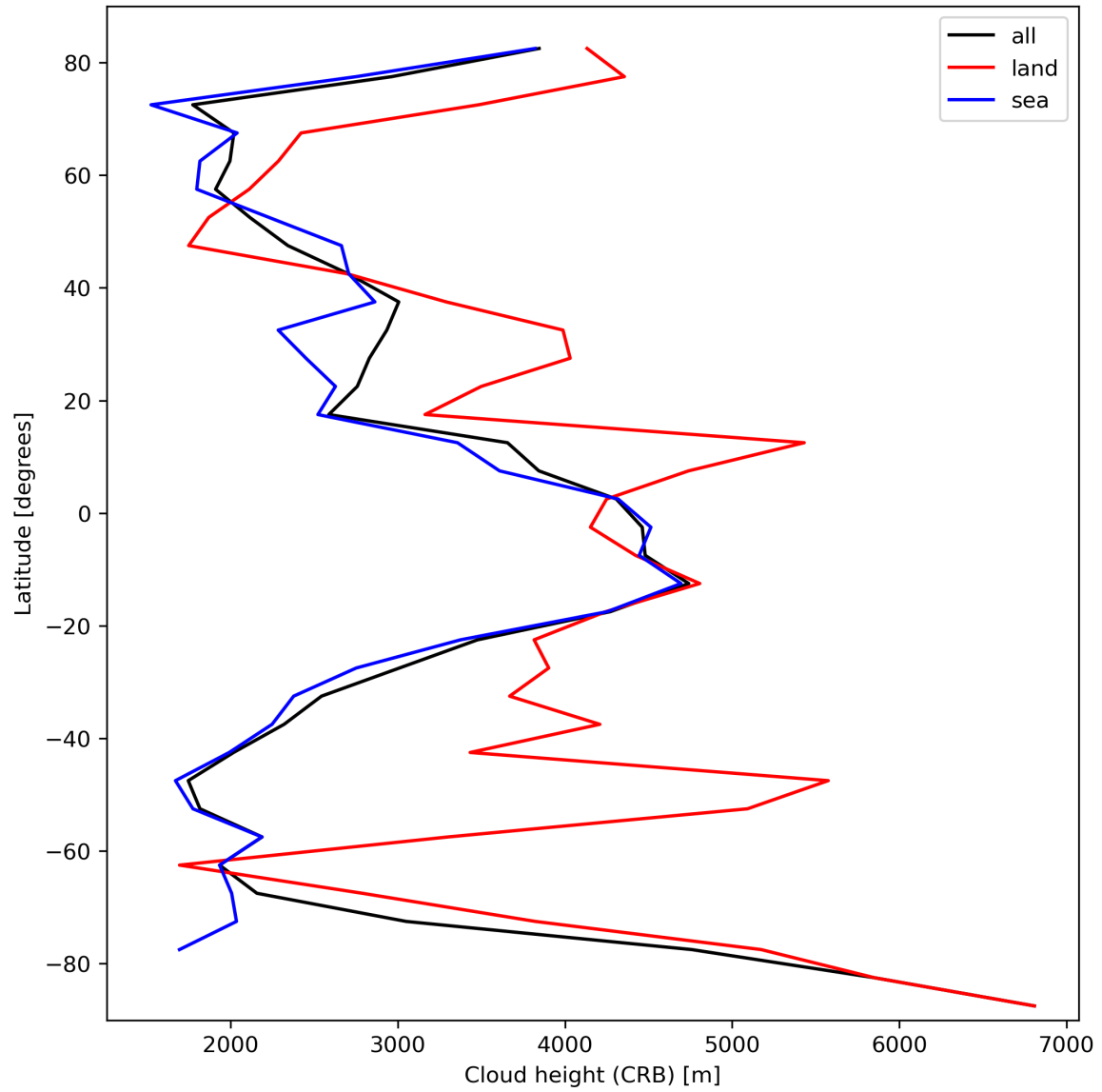
Figure 27: Zonal average of “Cloud height (CRB)” for 2024-03-06 to 2024-03-08.
