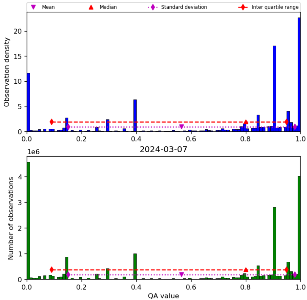
Figure 38: Histogram of “QA value” for 2024-03-06 to 2024-03-08
