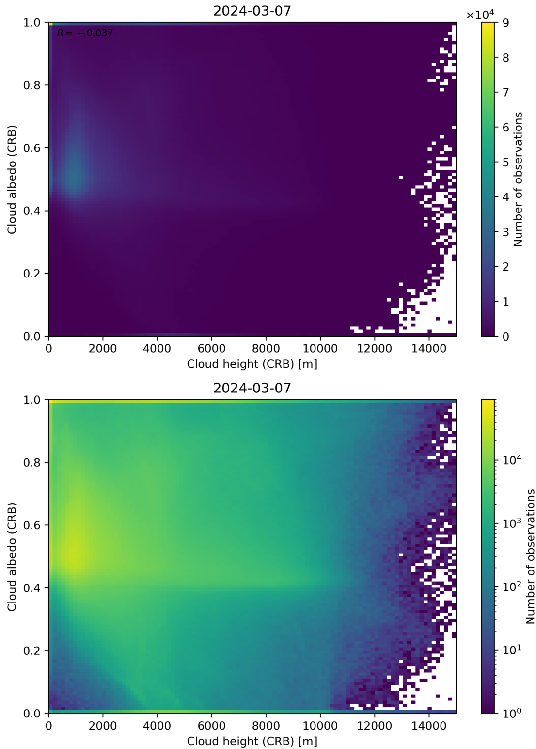
Figure 80: Scatter density plot of “Cloud height (CRB)” against “Cloud albedo (CRB)” for 2024-03-06 to 2024-03-08.
