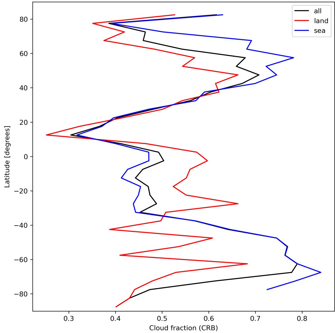
Figure 26: Zonal average of “Cloud fraction (CRB)” for 2024-03-06 to 2024-03-08.
