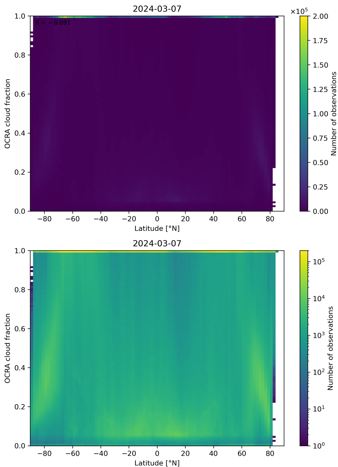
Figure 93: Scatter density plot of “Latitude” against “OCRA cloud fraction” for 2024-03-06 to 2024-03-08.
