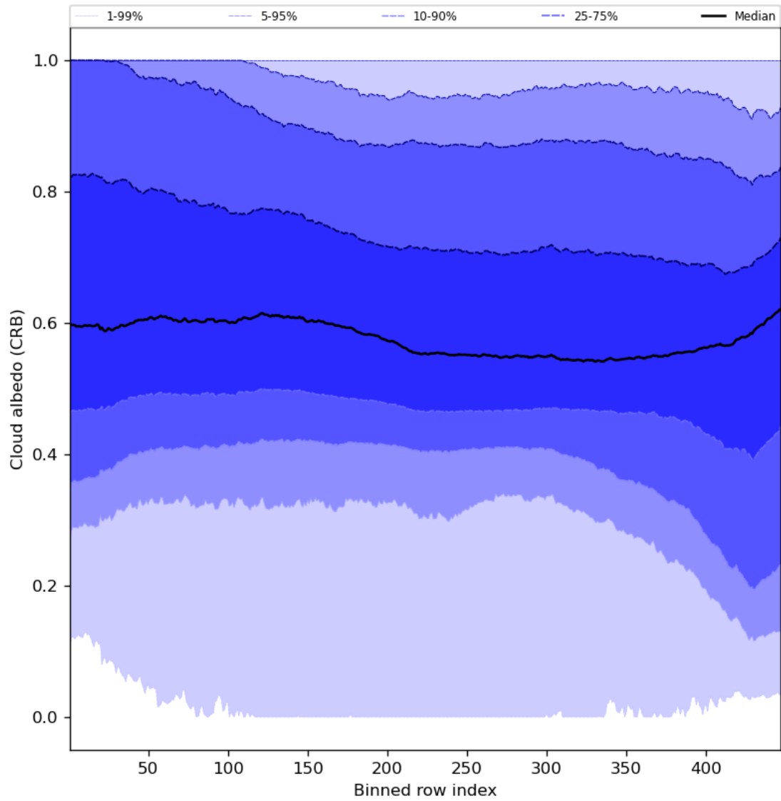
Figure 60: Along track statistics of “Cloud albedo (CRB)” for 2024-03-06 to 2024-03-08
