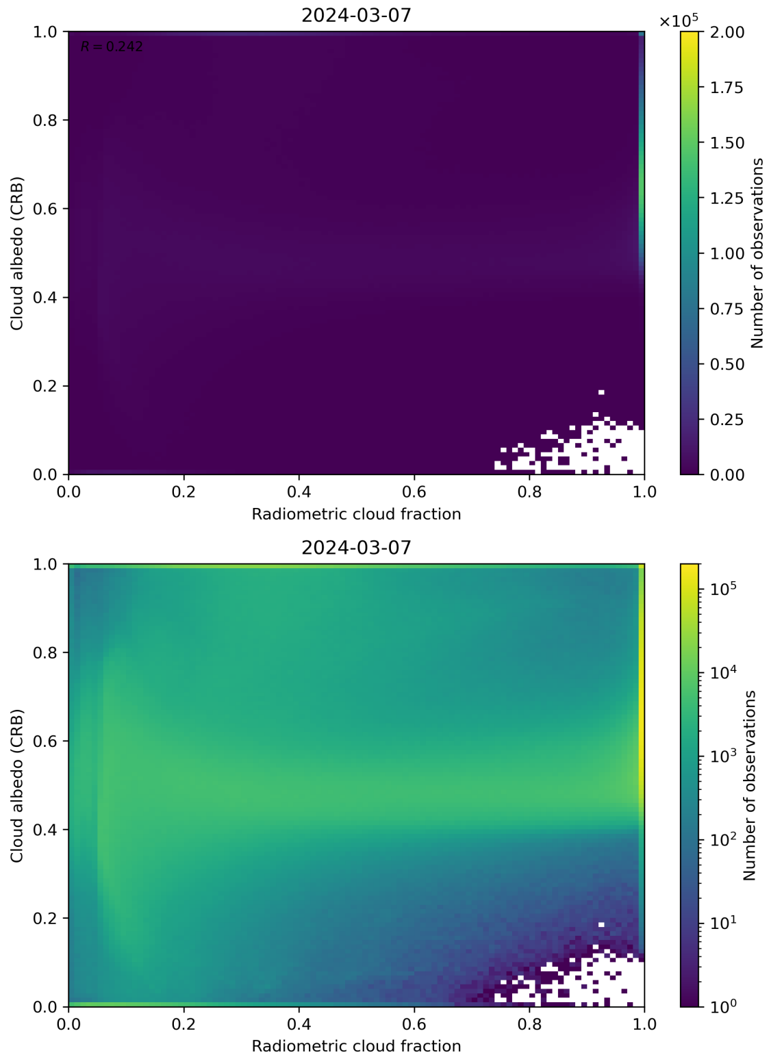
Figure 71: Scatter density plot of “Radiometric cloud fraction” against “Cloud albedo (CRB)” for 2024-03-06 to 2024-03-08.
