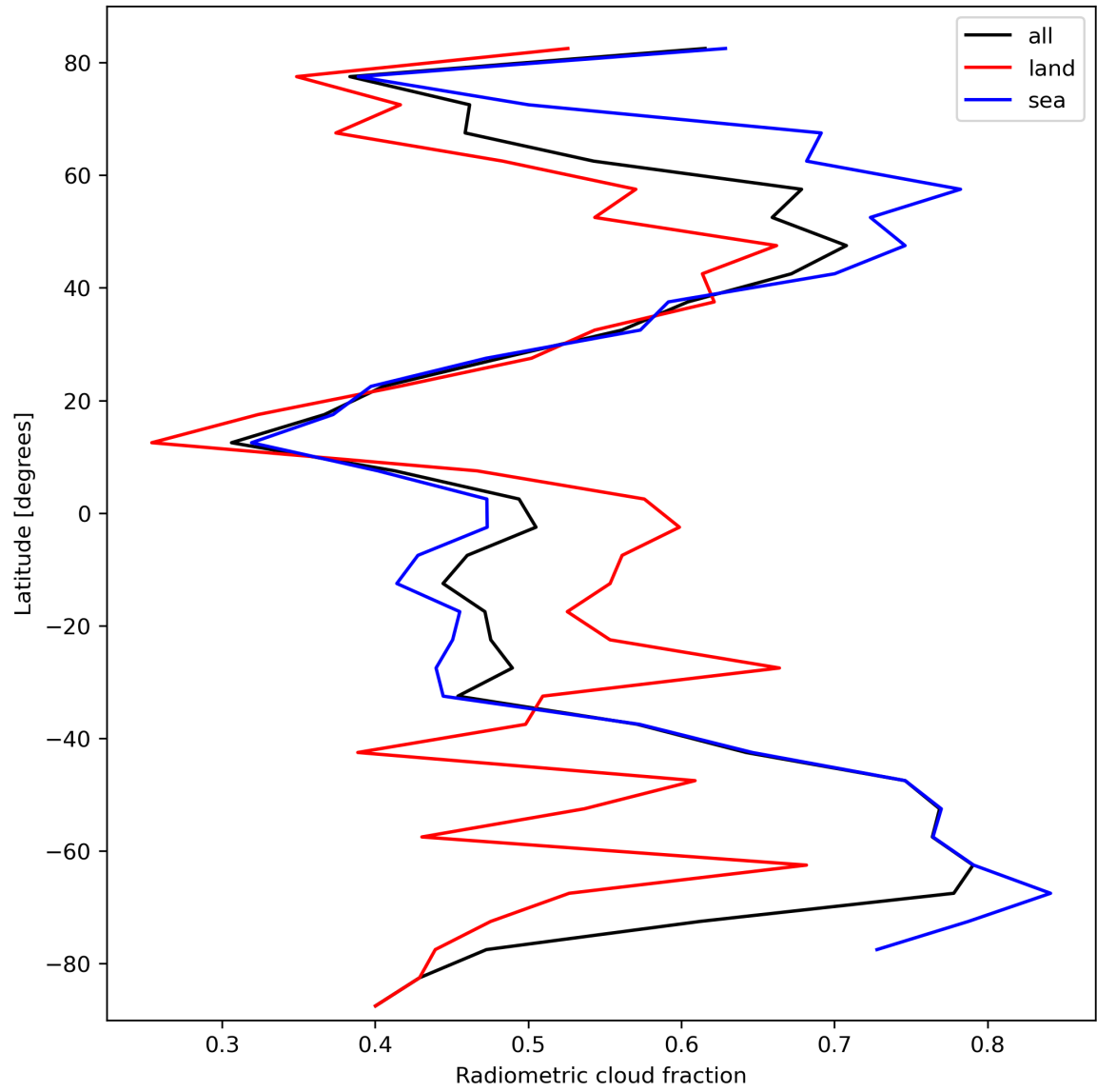
Figure 23: Zonal average of “Radiometric cloud fraction” for 2024-03-06 to 2024-03-08.
