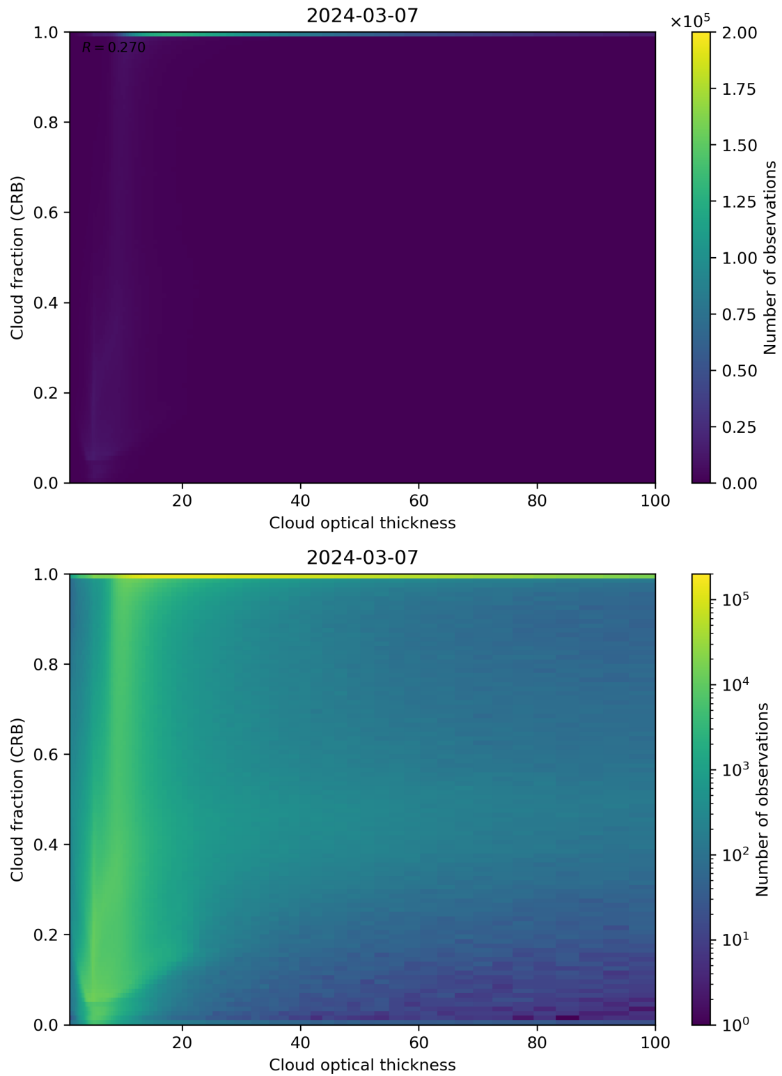
Figure 84: Scatter density plot of “Cloud optical thickness” against “Cloud fraction (CRB)” for 2024-03-06 to 2024-03-08.
