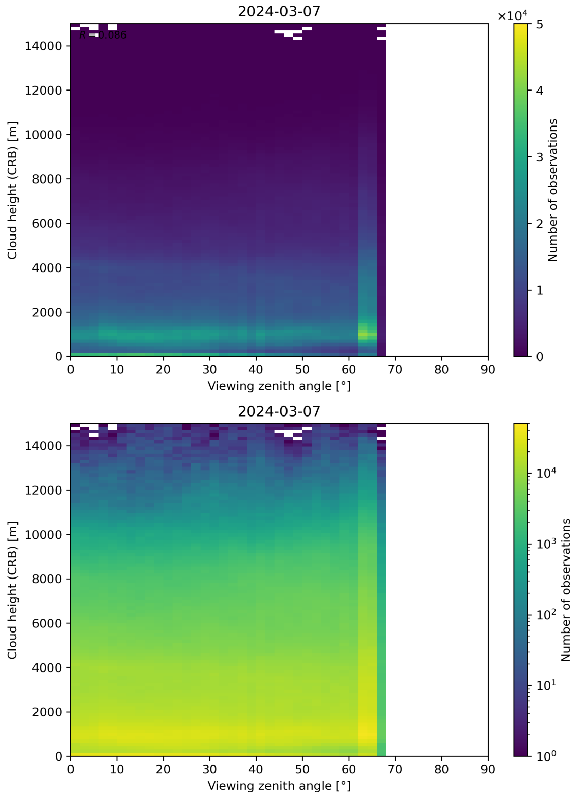
Figure 110: Scatter density plot of “Viewing zenith angle” against “Cloud height (CRB)” for 2024-03-06 to 2024-03-08.
