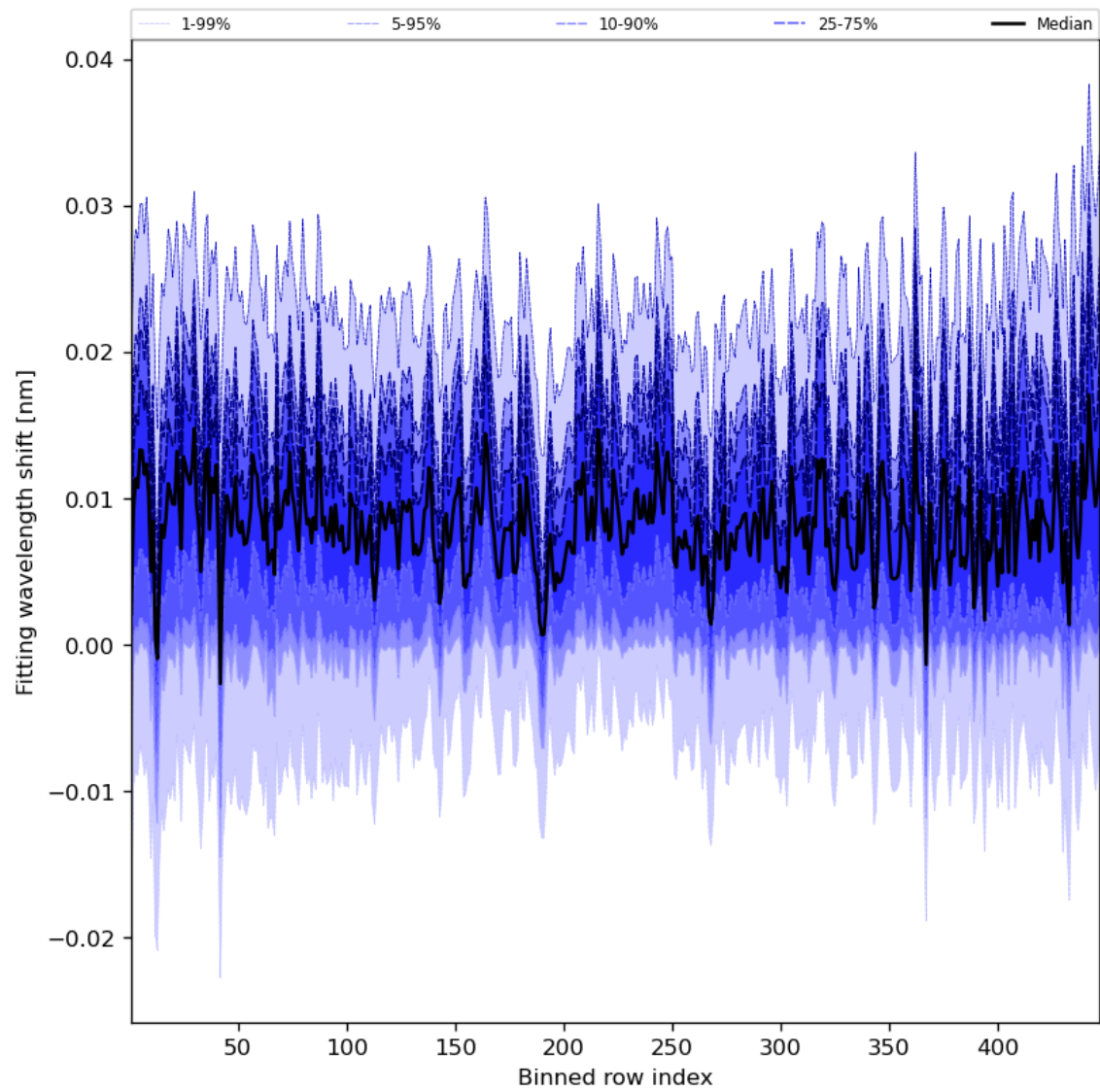
Figure 65: Along track statistics of “Fitting wavelength shift” for 2024-03-06 to 2024-03-08
