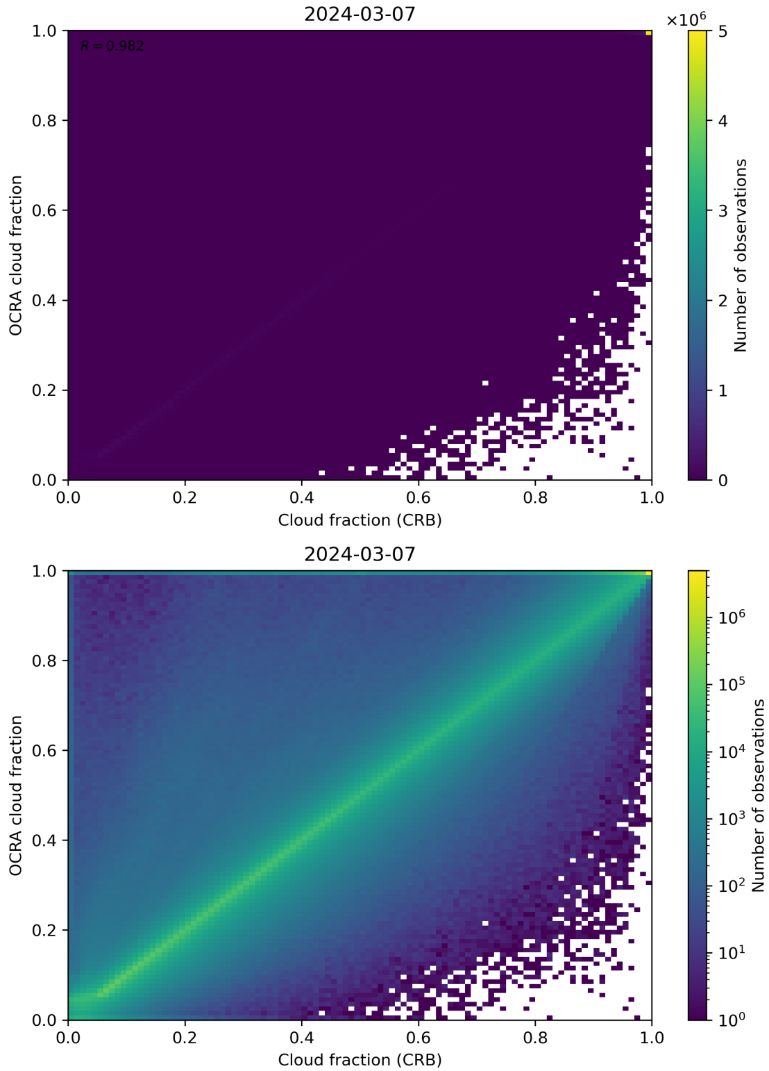
Figure 78: Scatter density plot of “Cloud fraction (CRB)” against “OCRA cloud fraction” for 2024-03-06 to 2024-03-08.
