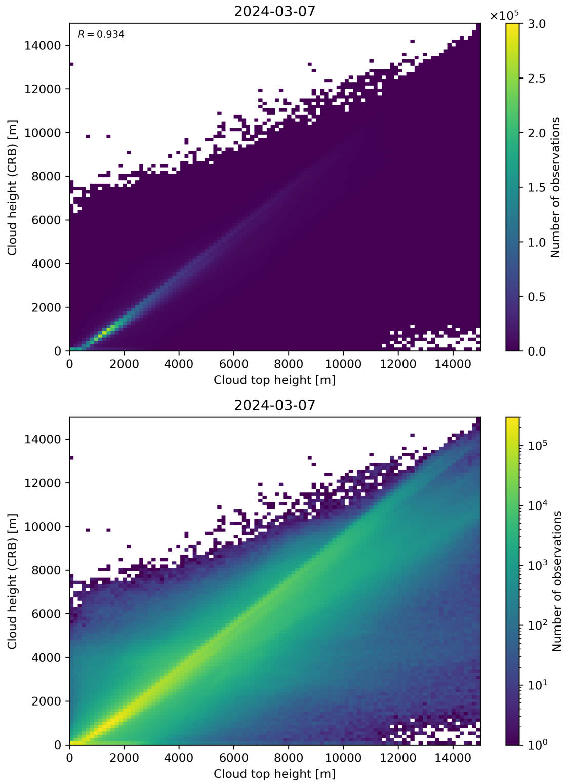
Figure 89: Scatter density plot of “Cloud top height” against “Cloud height (CRB)” for 2024-03-06 to 2024-03-08.
