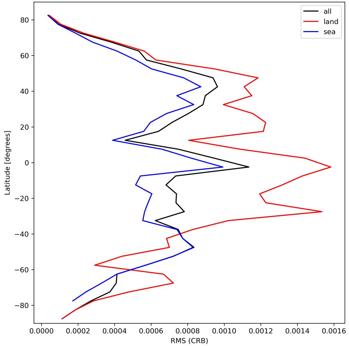
Figure 32: Zonal average of “RMS (CRB)” for 2024-03-06 to 2024-03-08.
