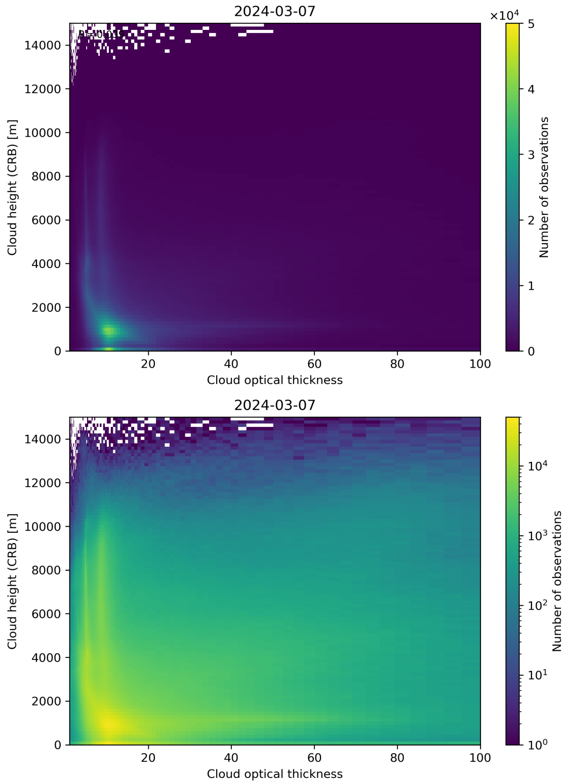
Figure 85: Scatter density plot of “Cloud optical thickness” against “Cloud height (CRB)” for 2024-03-06 to 2024-03-08.
