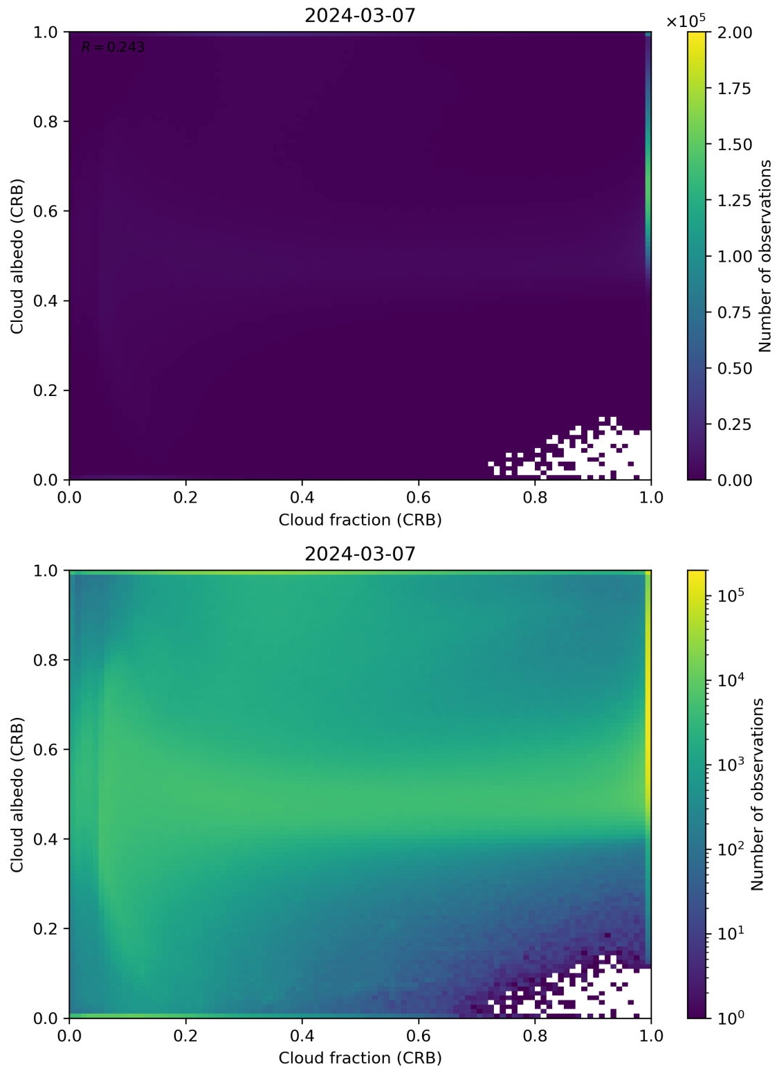
Figure 77: Scatter density plot of “Cloud fraction (CRB)” against “Cloud albedo (CRB)” for 2024-03-06 to 2024-03-08.
