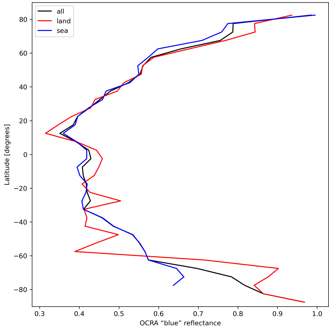
Figure 35: Zonal average of "OCRA "blue" reflectance" for 2024-03-06 to 2024-03-08.
