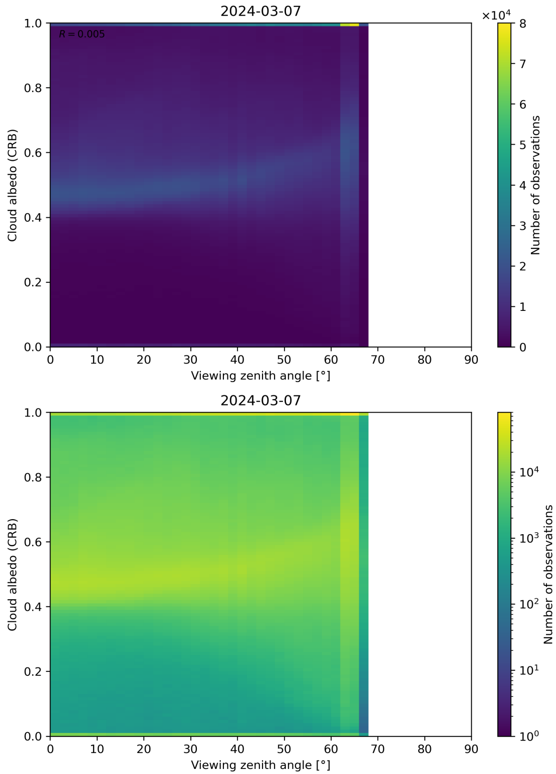
Figure 106: Scatter density plot of “Viewing zenith angle” against “Cloud albedo (CRB)” for 2024-03-06 to 2024-03-08.
