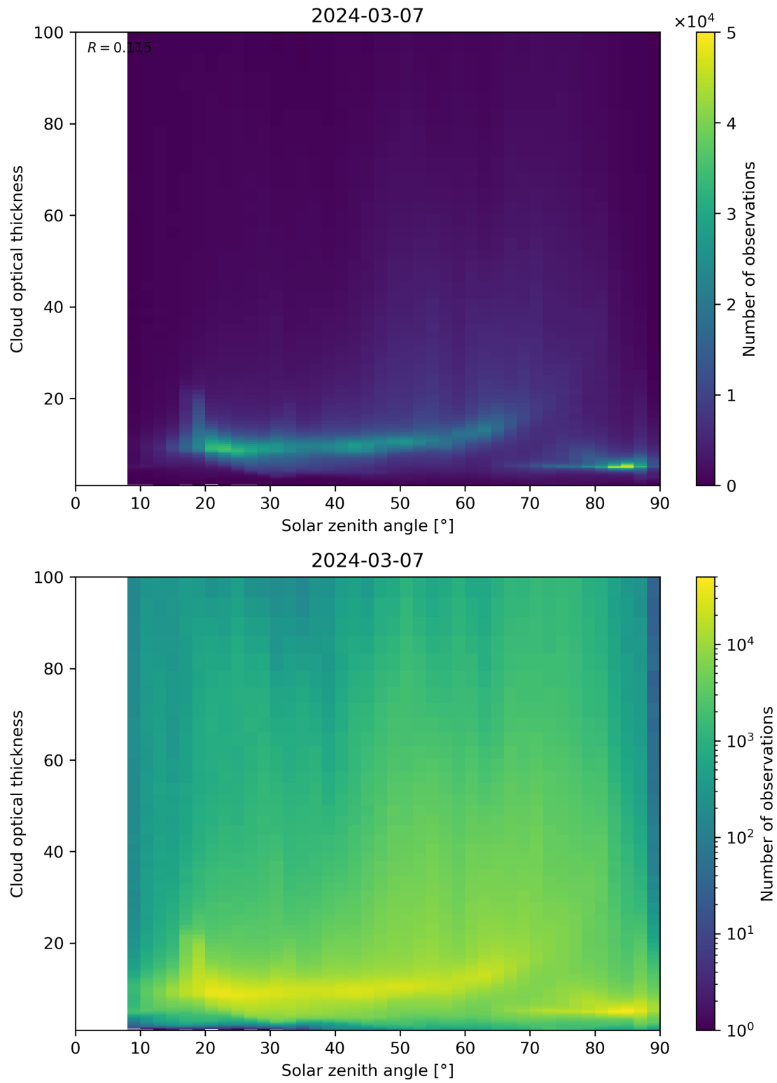
Figure 103: Scatter density plot of “Solar zenith angle” against “Cloud optical thickness” for 2024-03-06 to 2024-03-08.
