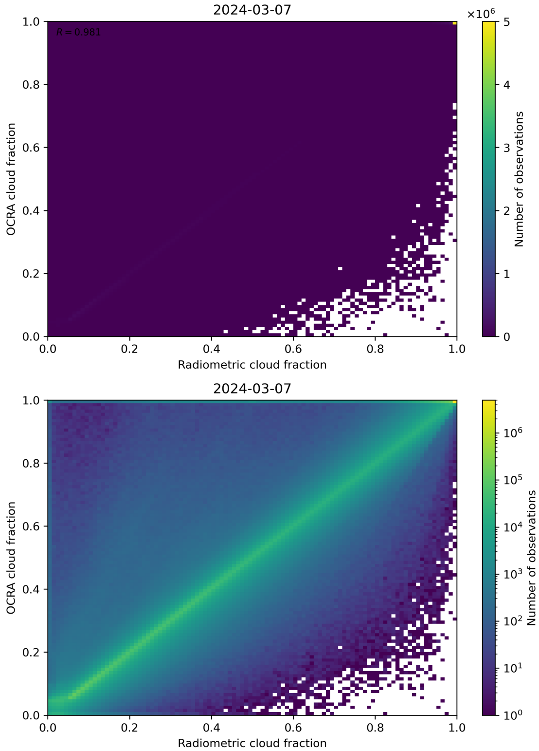
Figure 72: Scatter density plot of “Radiometric cloud fraction” against “OCRA cloud fraction” for 2024-03-06 to 2024-03-08.
