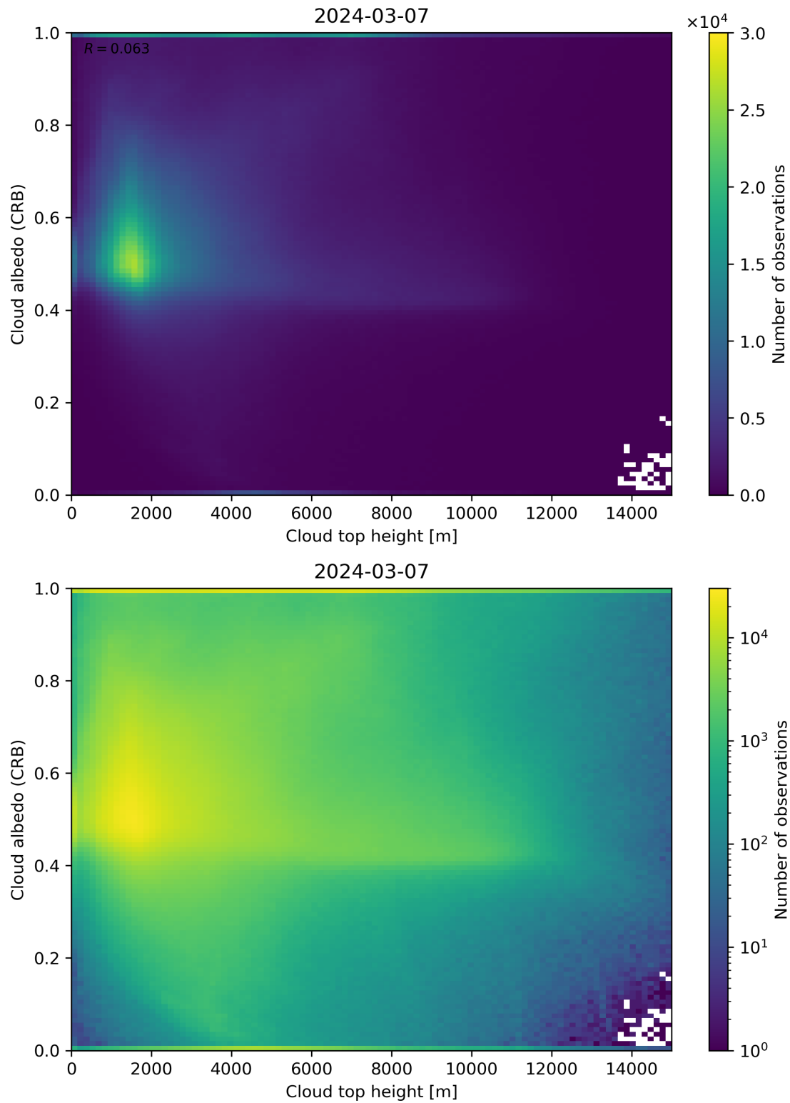
Figure 86: Scatter density plot of “Cloud top height” against “Cloud albedo (CRB)” for 2024-03-06 to 2024-03-08.
