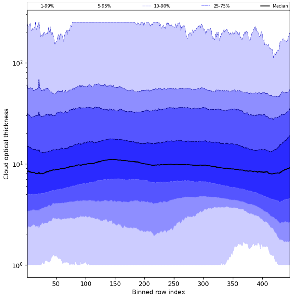
Figure 57: Along track statistics of “Cloud optical thickness” for 2024-03-06 to 2024-03-08
