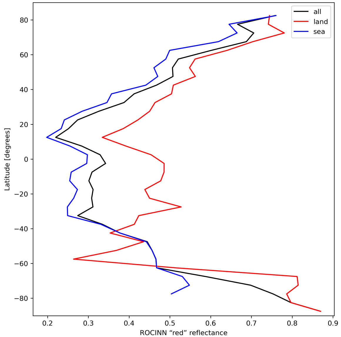
Figure 37: Zonal average of “ROCINN “red” reflectance” for 2024-03-06 to 2024-03-08.
