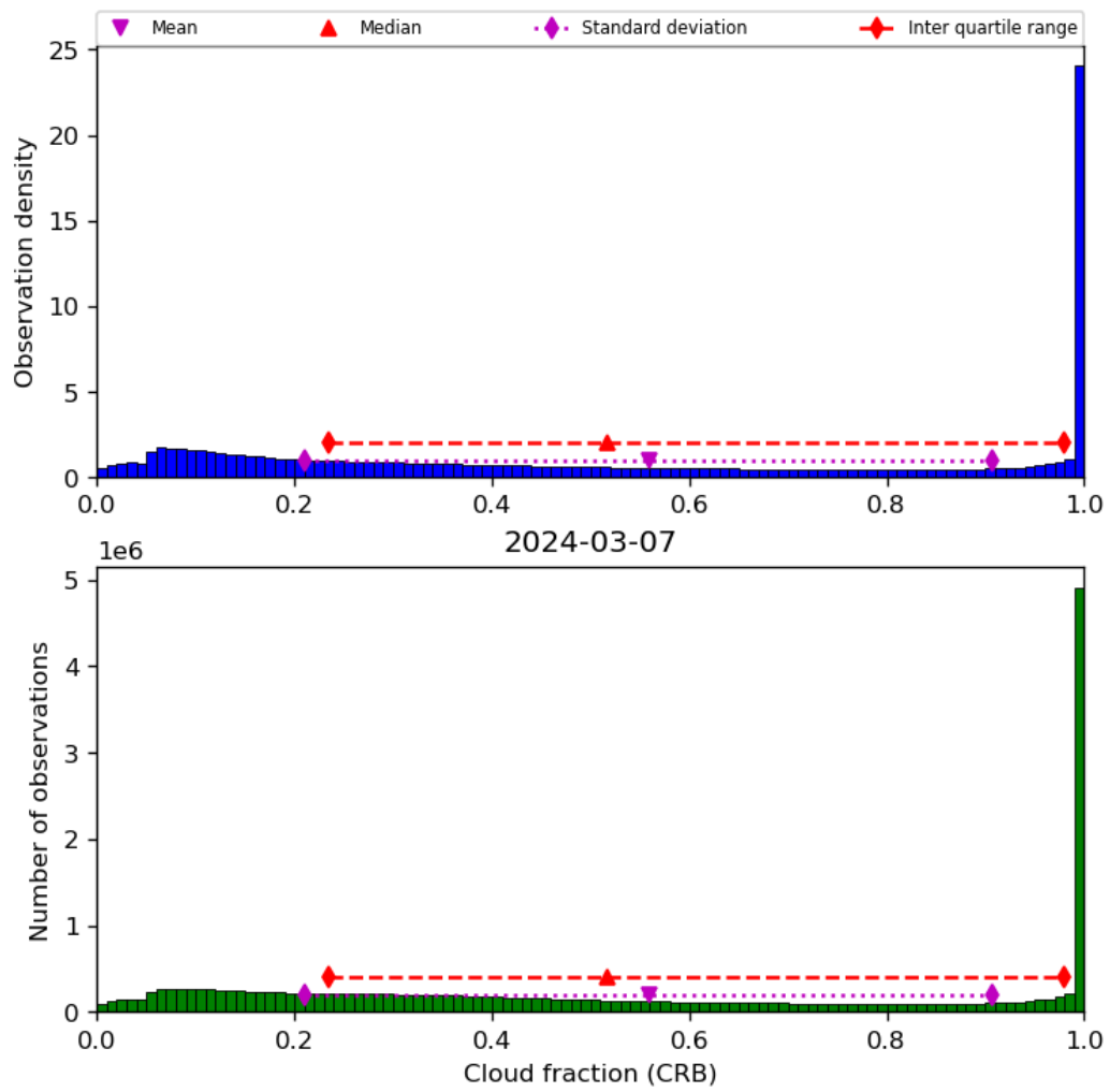
Figure 42: Histogram of “Cloud fraction (CRB)” for 2024-03-06 to 2024-03-08
