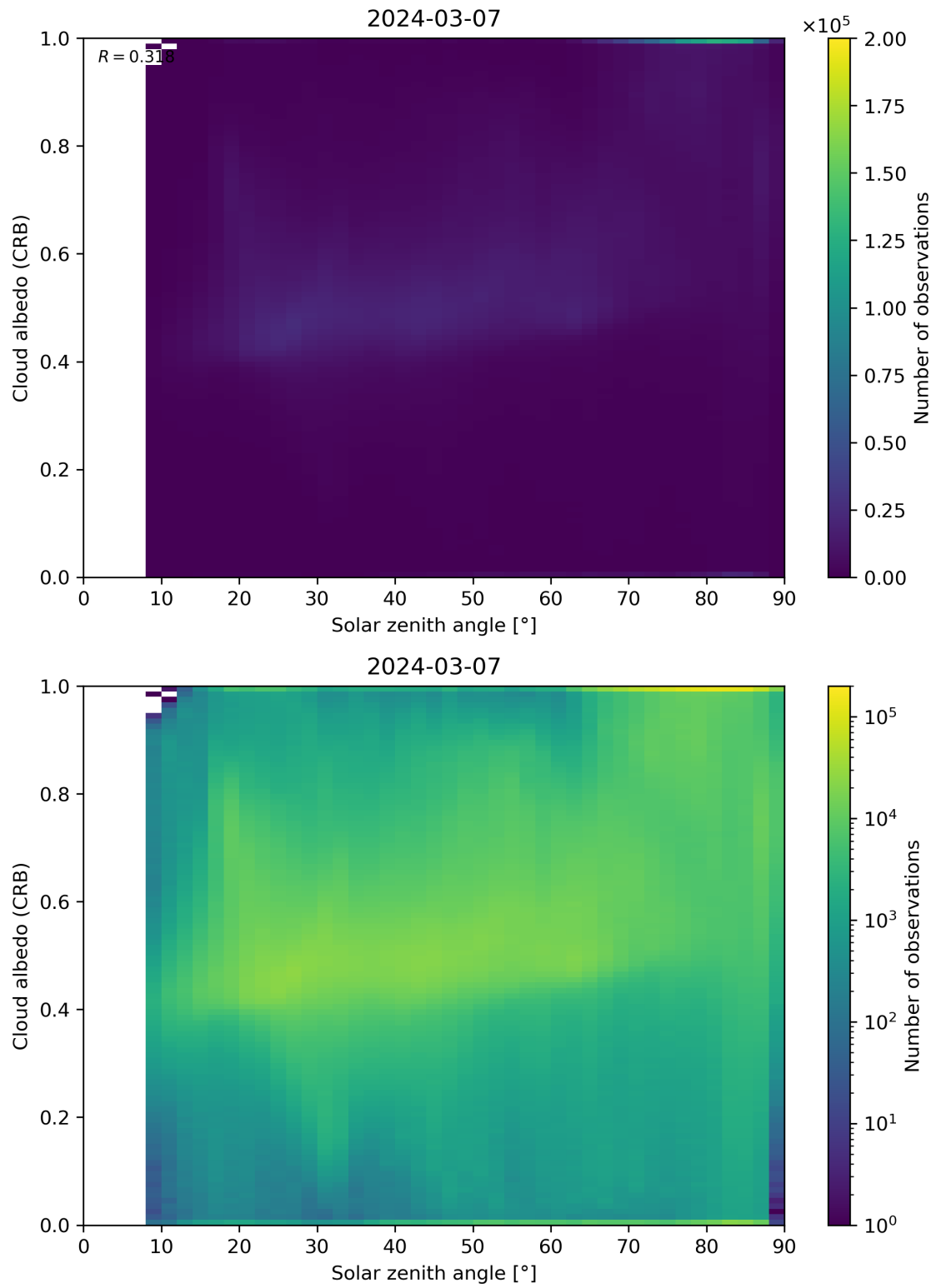
Figure 98: Scatter density plot of “Solar zenith angle” against “Cloud albedo (CRB)” for 2024-03-06 to 2024-03-08.
