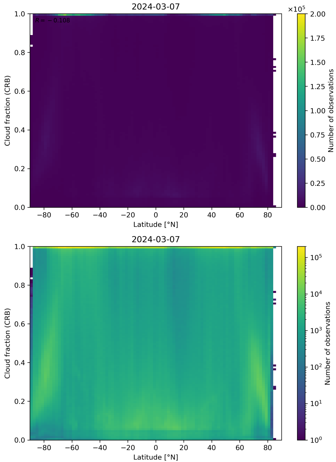
Figure 94: Scatter density plot of “Latitude” against “Cloud fraction (CRB)” for 2024-03-06 to 2024-03-08.
