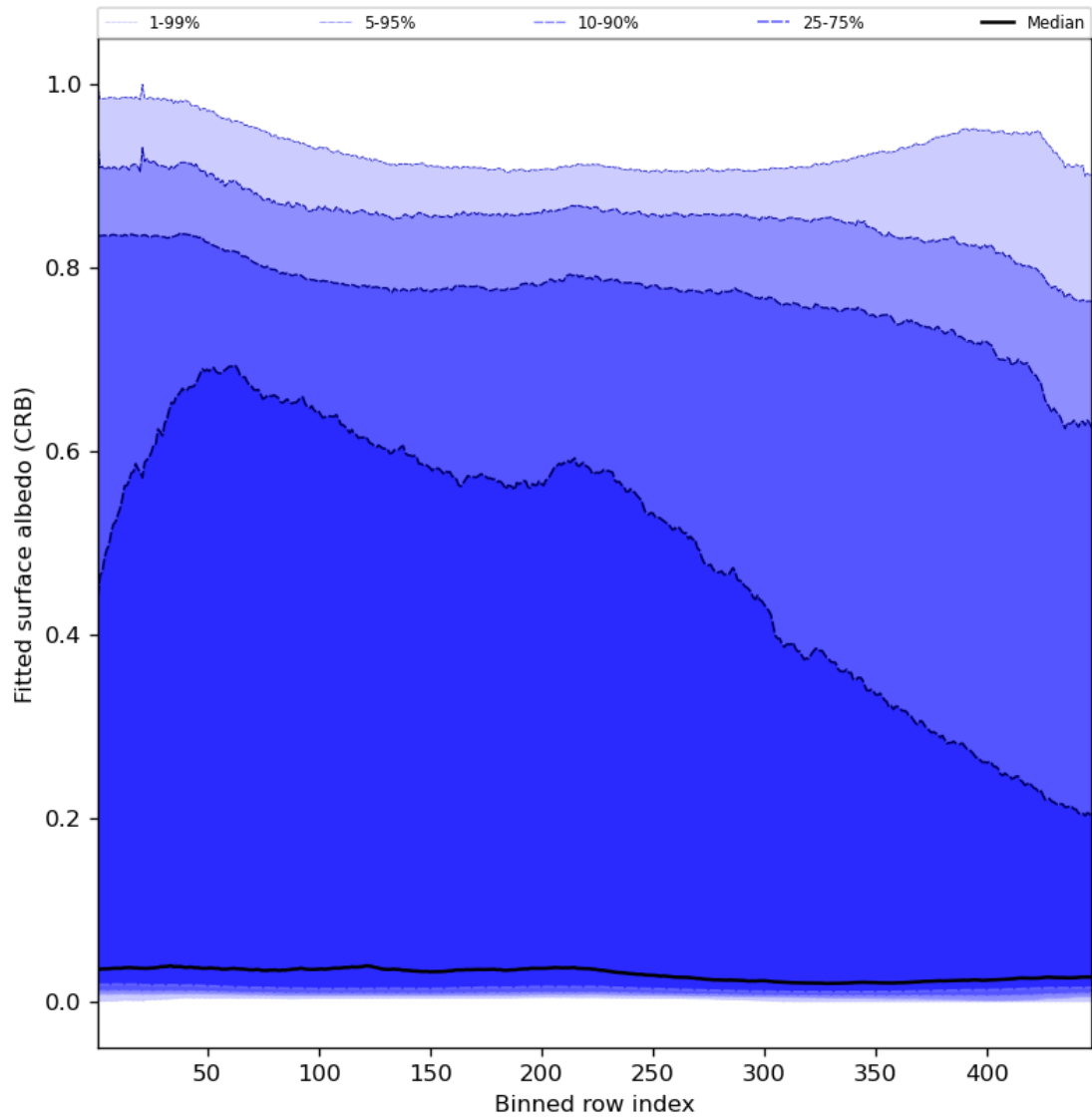
Figure 62: Along track statistics of “Fitted surface albedo (CRB)” for 2024-03-06 to 2024-03-08
