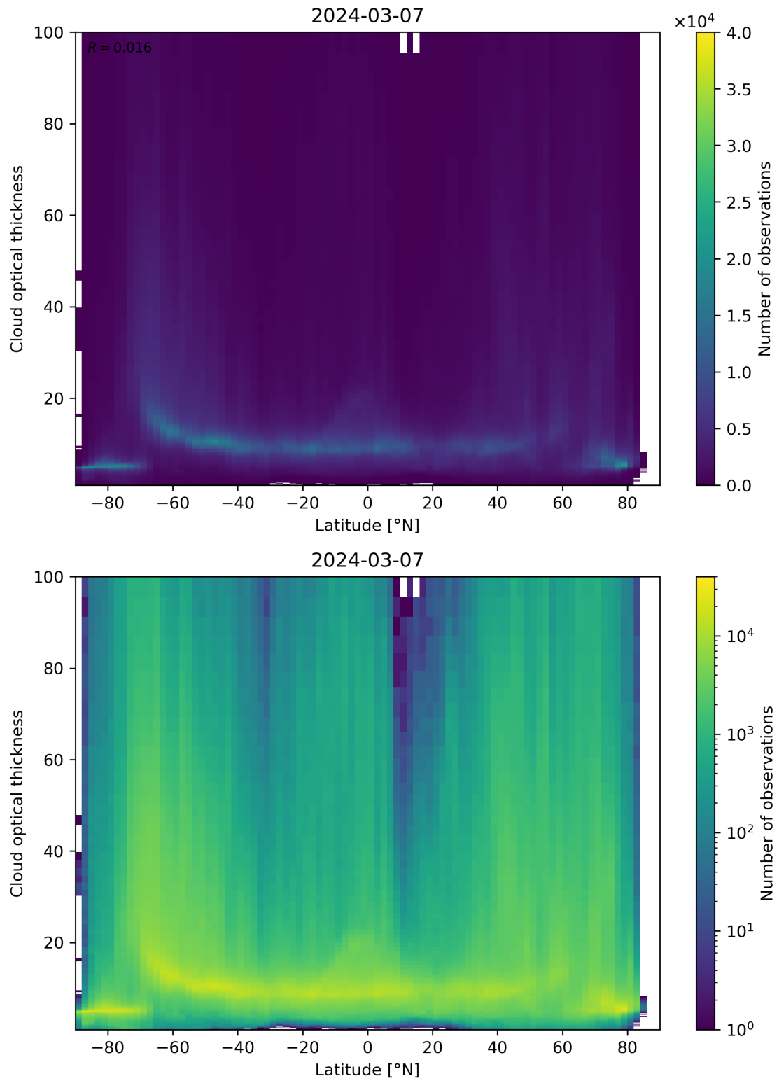
Figure 96: Scatter density plot of “Latitude” against “Cloud optical thickness” for 2024-03-06 to 2024-03-08.
