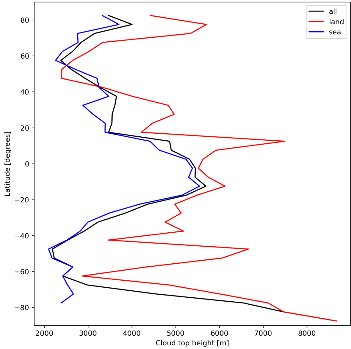
Figure 24: Zonal average of “Cloud top height” for 2024-03-06 to 2024-03-08.
