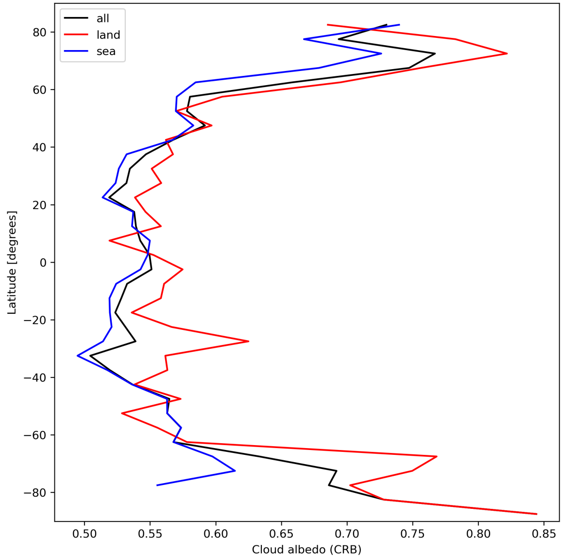
Figure 28: Zonal average of “Cloud albedo (CRB)” for 2024-03-06 to 2024-03-08.
