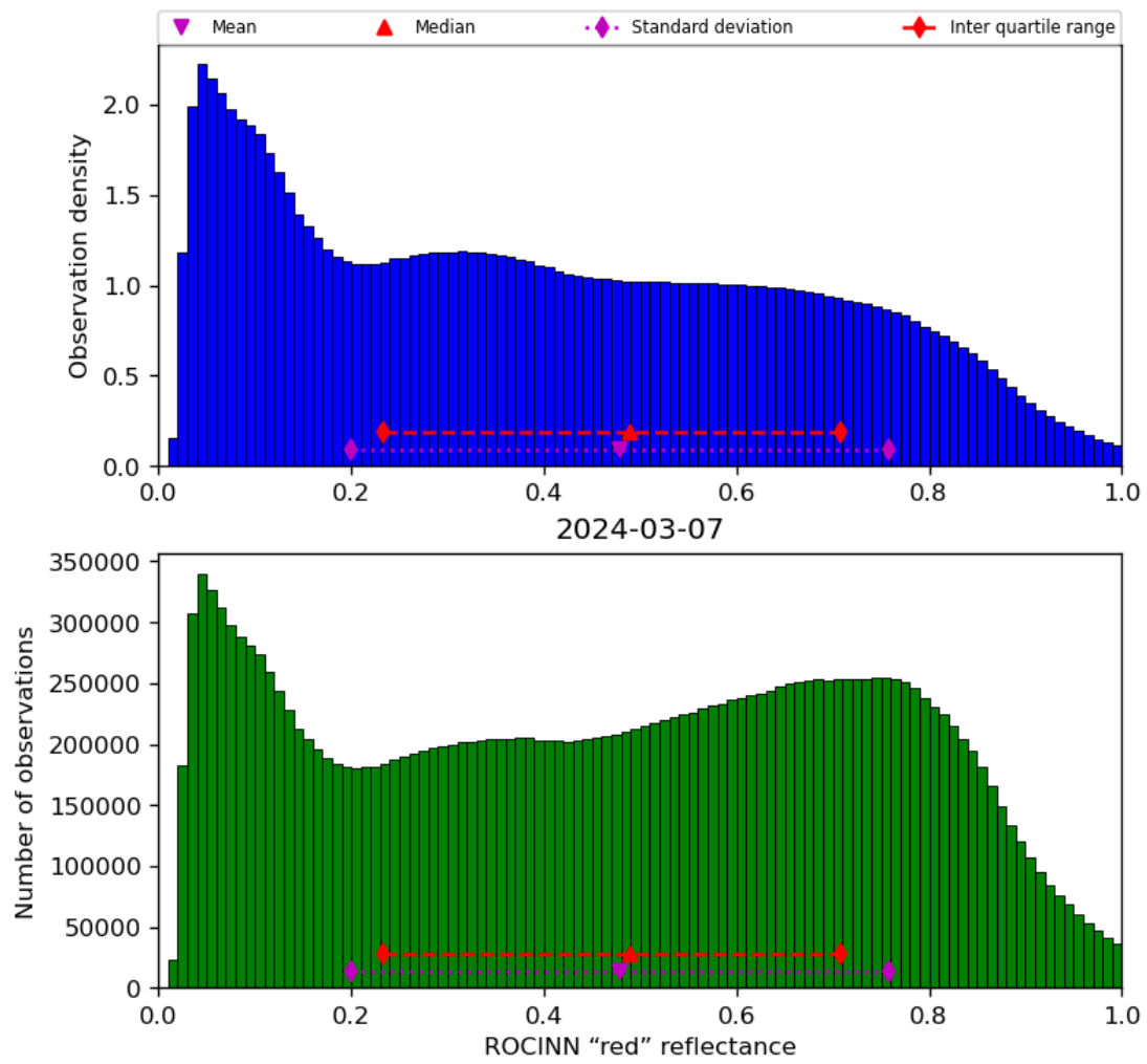
Figure 53: Histogram of “ROCINN “red” reflectance” for 2024-03-06 to 2024-03-08
