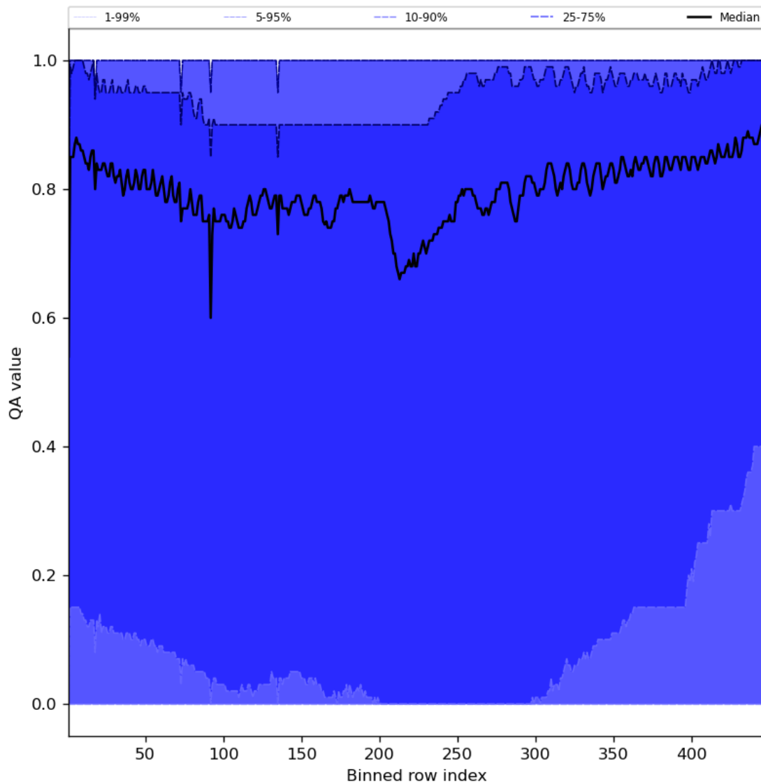
Figure 54: Along track statistics of “QA value” for 2024-03-06 to 2024-03-08
