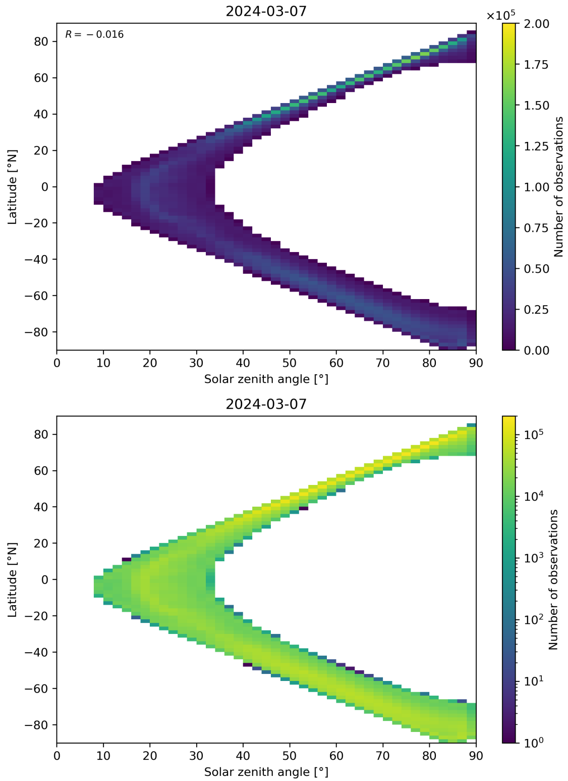
Figure 105: Scatter density plot of “Solar zenith angle” against “Latitude” for 2024-03-06 to 2024-03-08.
