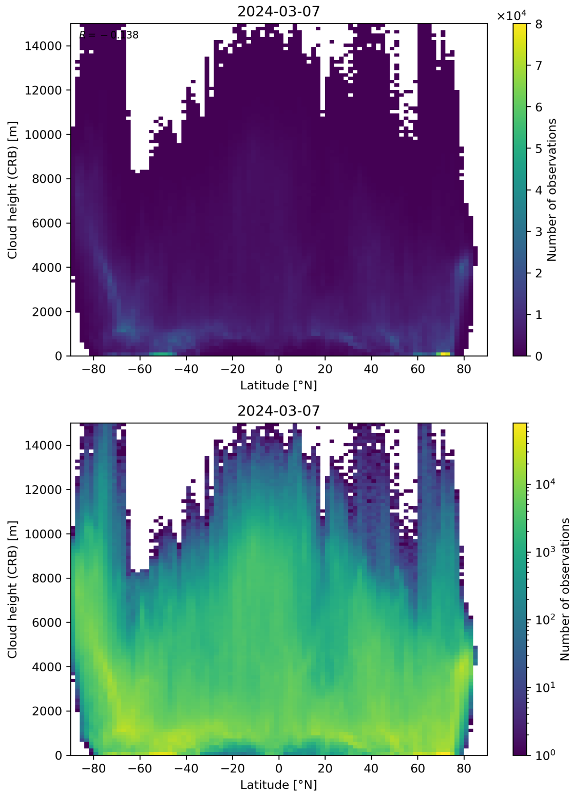
Figure 95: Scatter density plot of “Latitude” against “Cloud height (CRB)” for 2024-03-06 to 2024-03-08.
