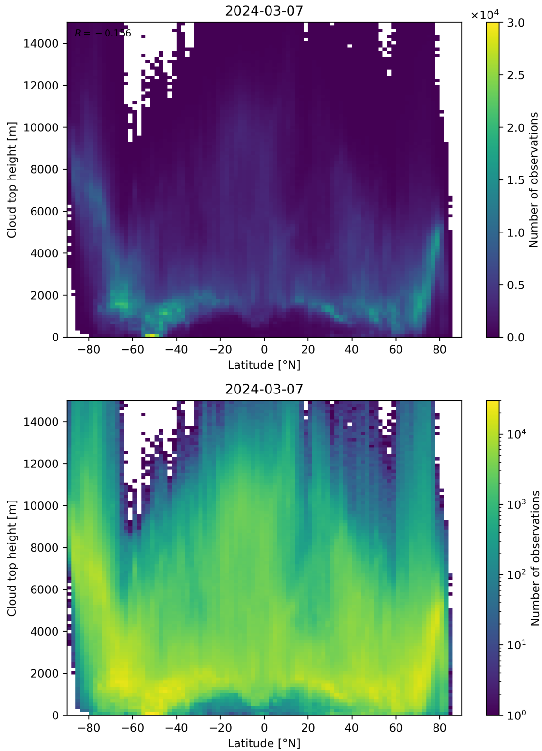
Figure 97: Scatter density plot of “Latitude” against “Cloud top height” for 2024-03-06 to 2024-03-08.
