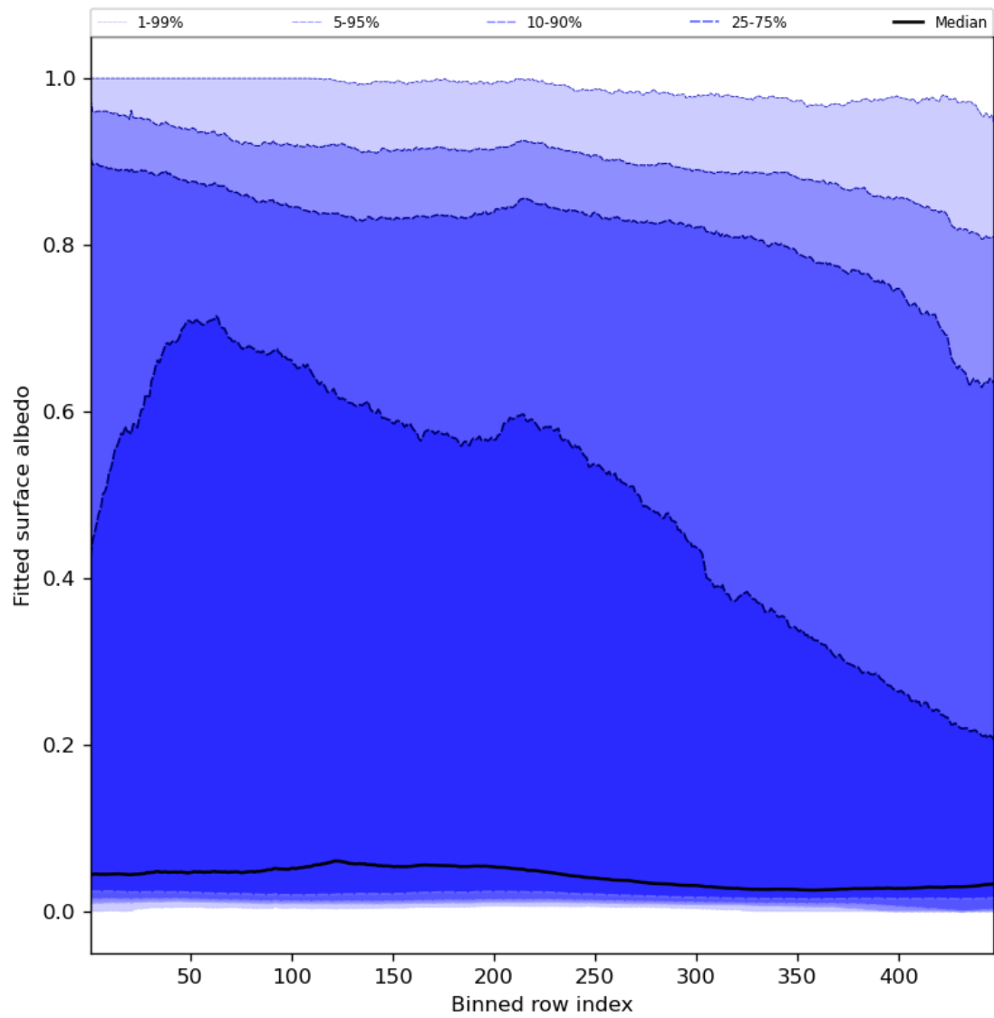
Figure 61: Along track statistics of “Fitted surface albedo” for 2024-03-06 to 2024-03-08
