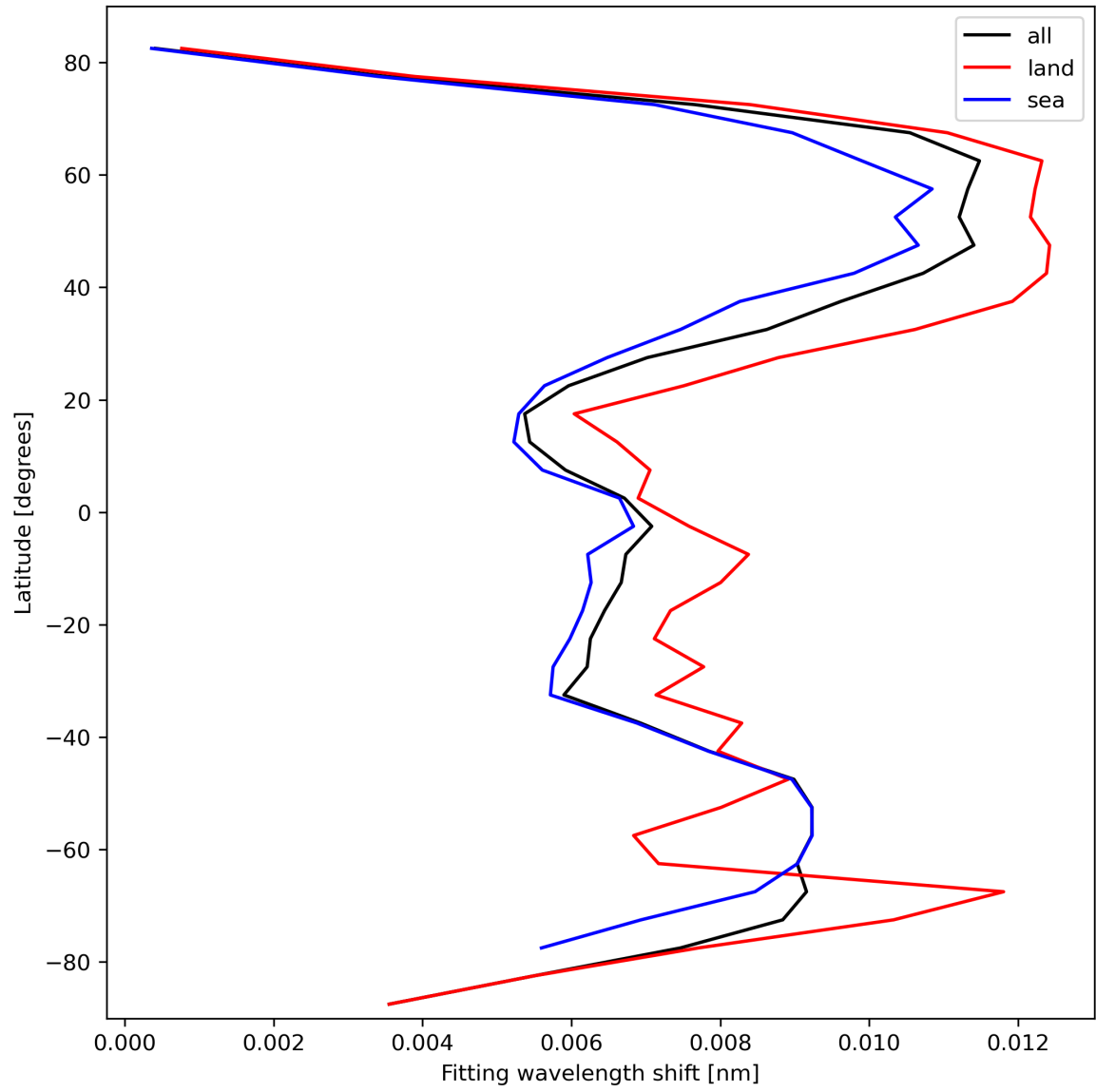
Figure 33: Zonal average of “Fitting wavelength shift” for 2024-03-06 to 2024-03-08.
