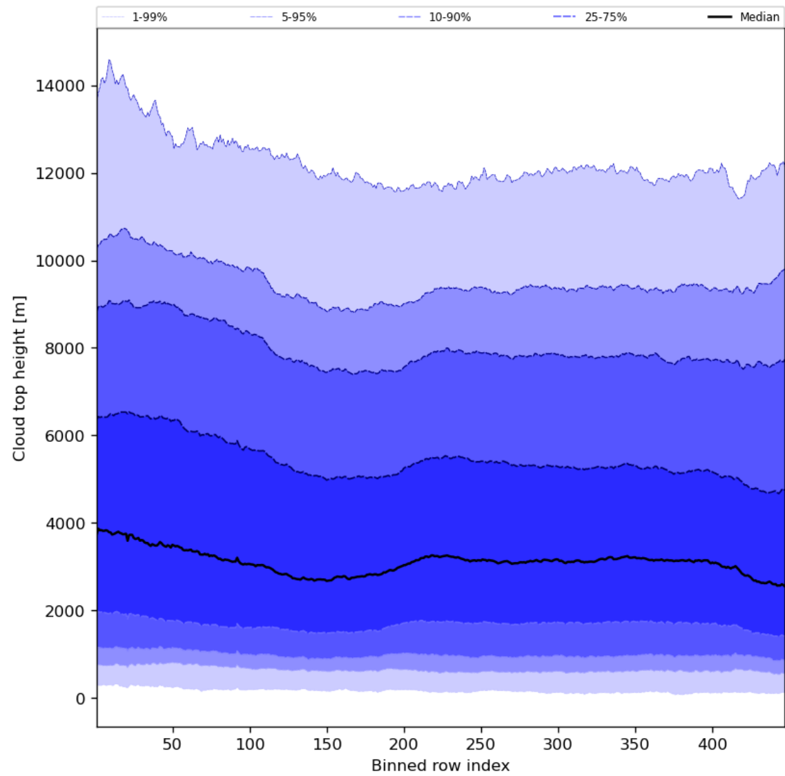
Figure 56: Along track statistics of “Cloud top height” for 2024-03-06 to 2024-03-08
