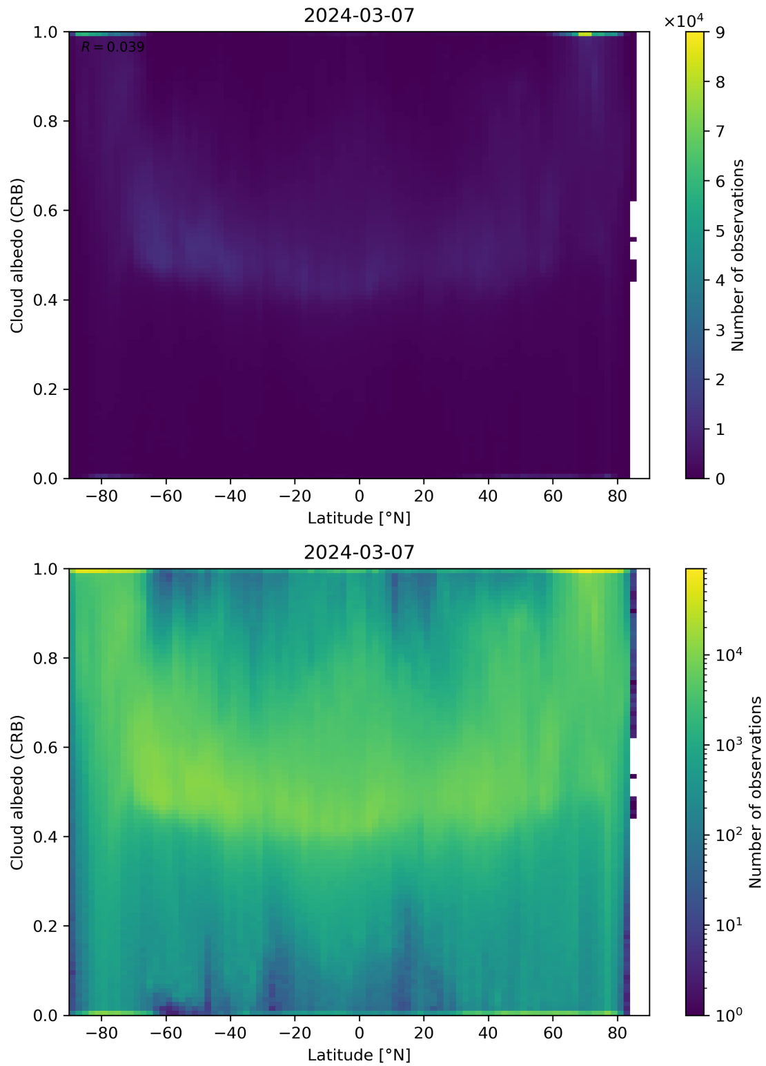
Figure 91: Scatter density plot of “Latitude” against “Cloud albedo (CRB)” for 2024-03-06 to 2024-03-08.
