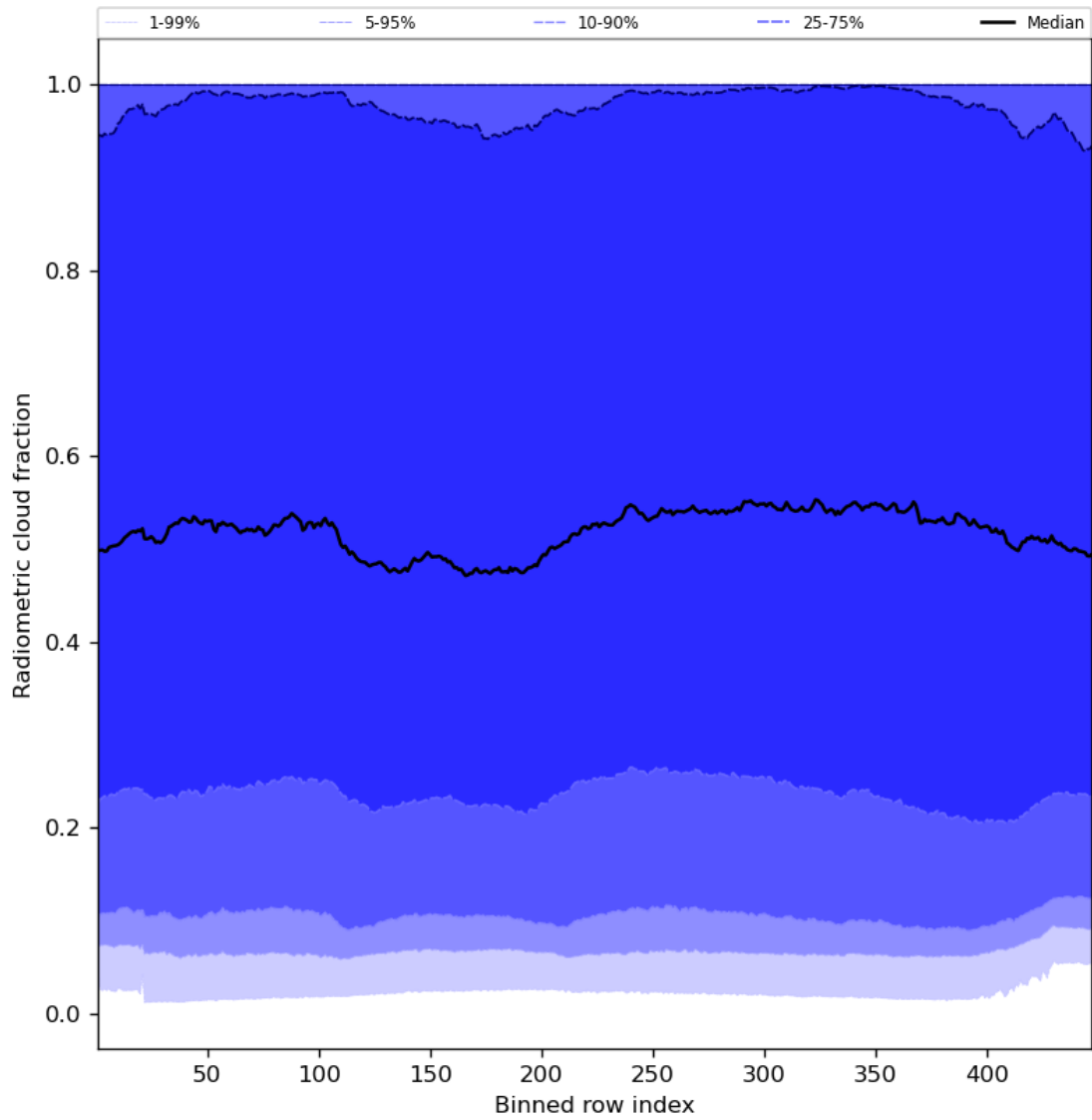
Figure 55: Along track statistics of “Radiometric cloud fraction” for 2024-03-06 to 2024-03-08
