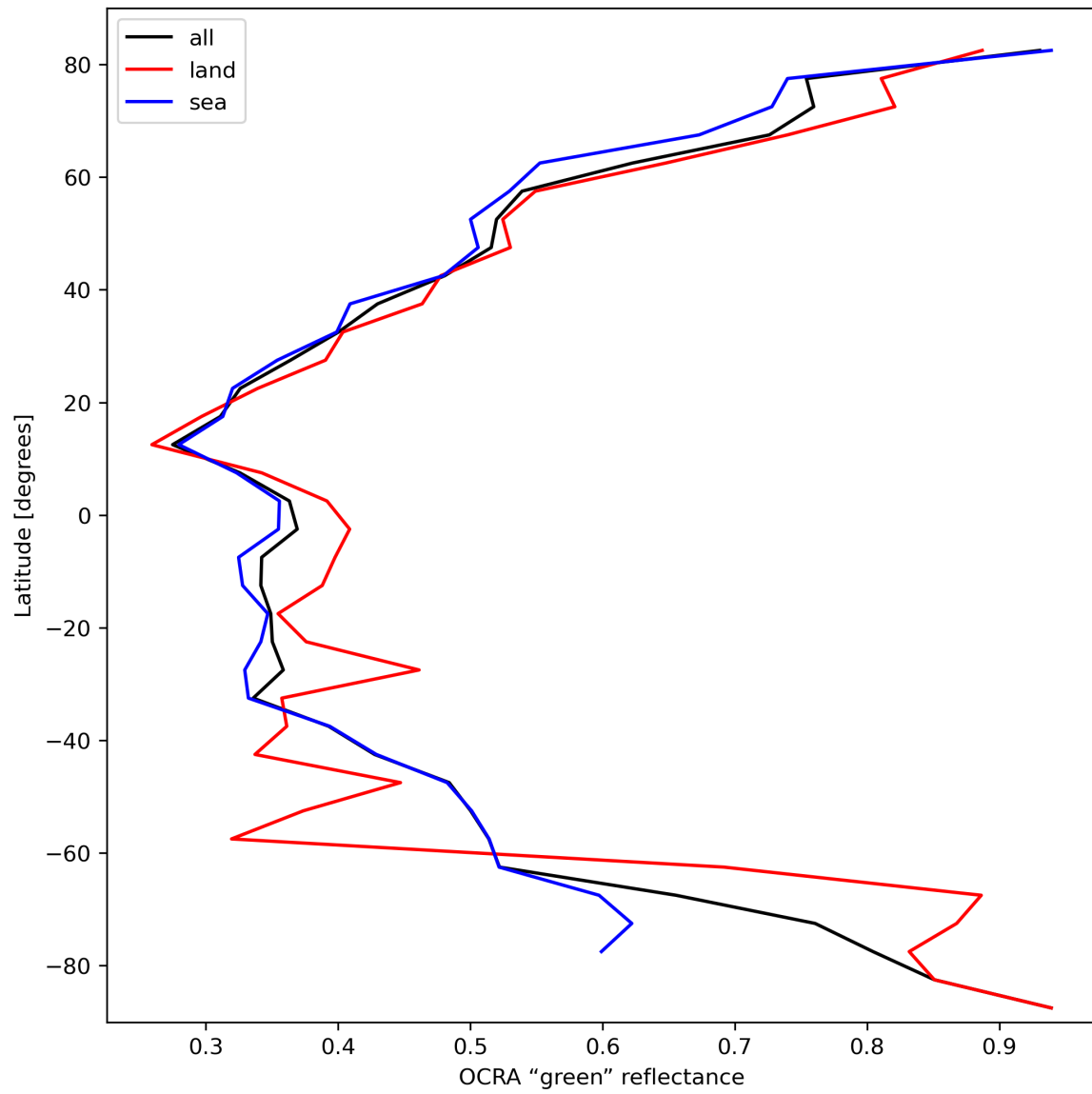
Figure 36: Zonal average of “OCRA “green” reflectance” for 2024-03-06 to 2024-03-08.
