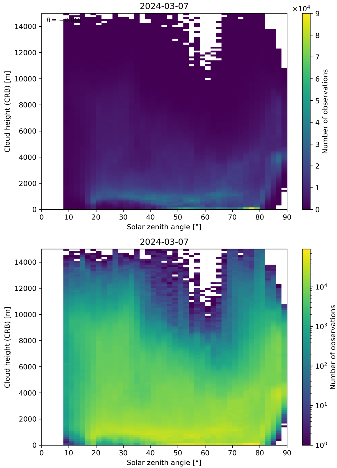
Figure 102: Scatter density plot of “Solar zenith angle” against “Cloud height (CRB)” for 2024-03-06 to 2024-03-08.
