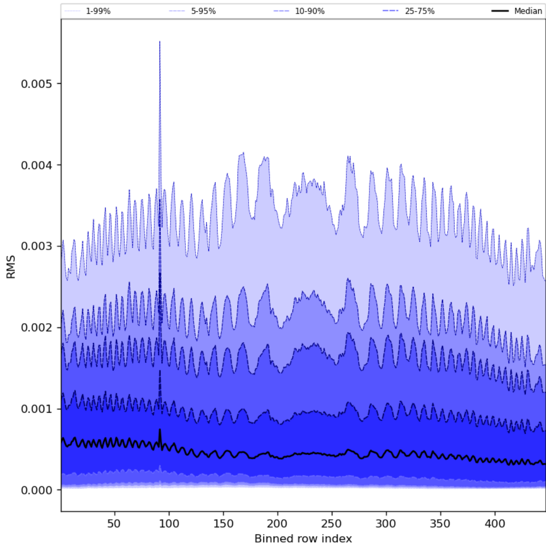
Figure 63: Along track statistics of “RMS” for 2024-03-07 to 2024-03-09
