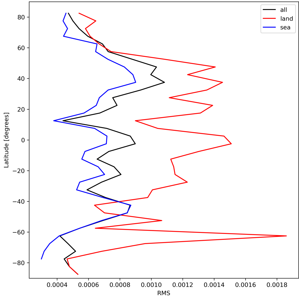
Figure 31: Zonal average of “RMS” for 2024-03-07 to 2024-03-09.
