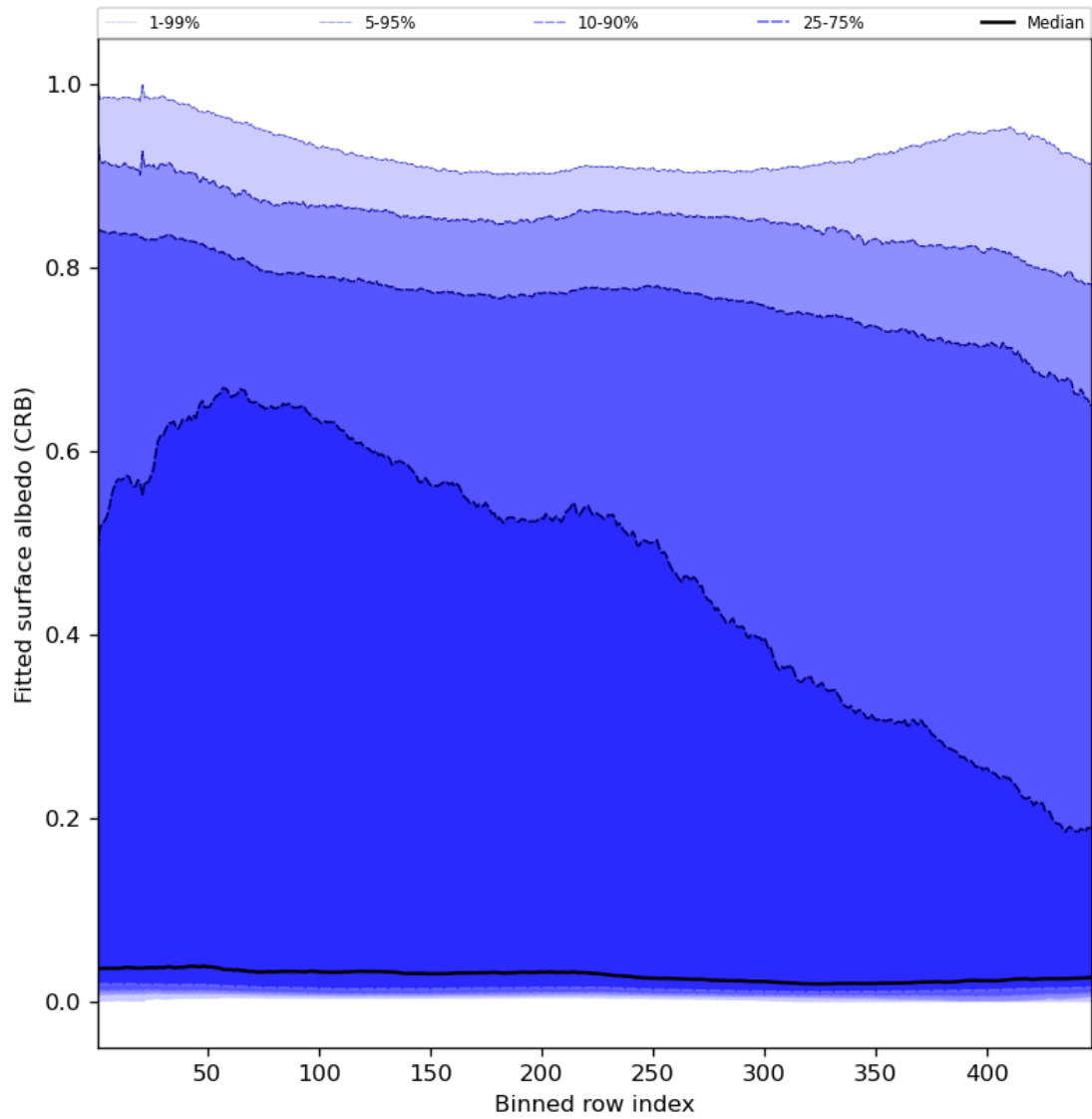
Figure 62: Along track statistics of “Fitted surface albedo (CRB)” for 2024-03-07 to 2024-03-09
