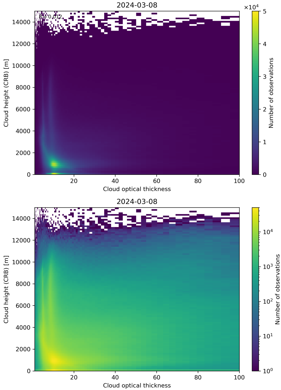
Figure 85: Scatter density plot of “Cloud optical thickness” against “Cloud height (CRB)” for 2024-03-07 to 2024-03-09.
