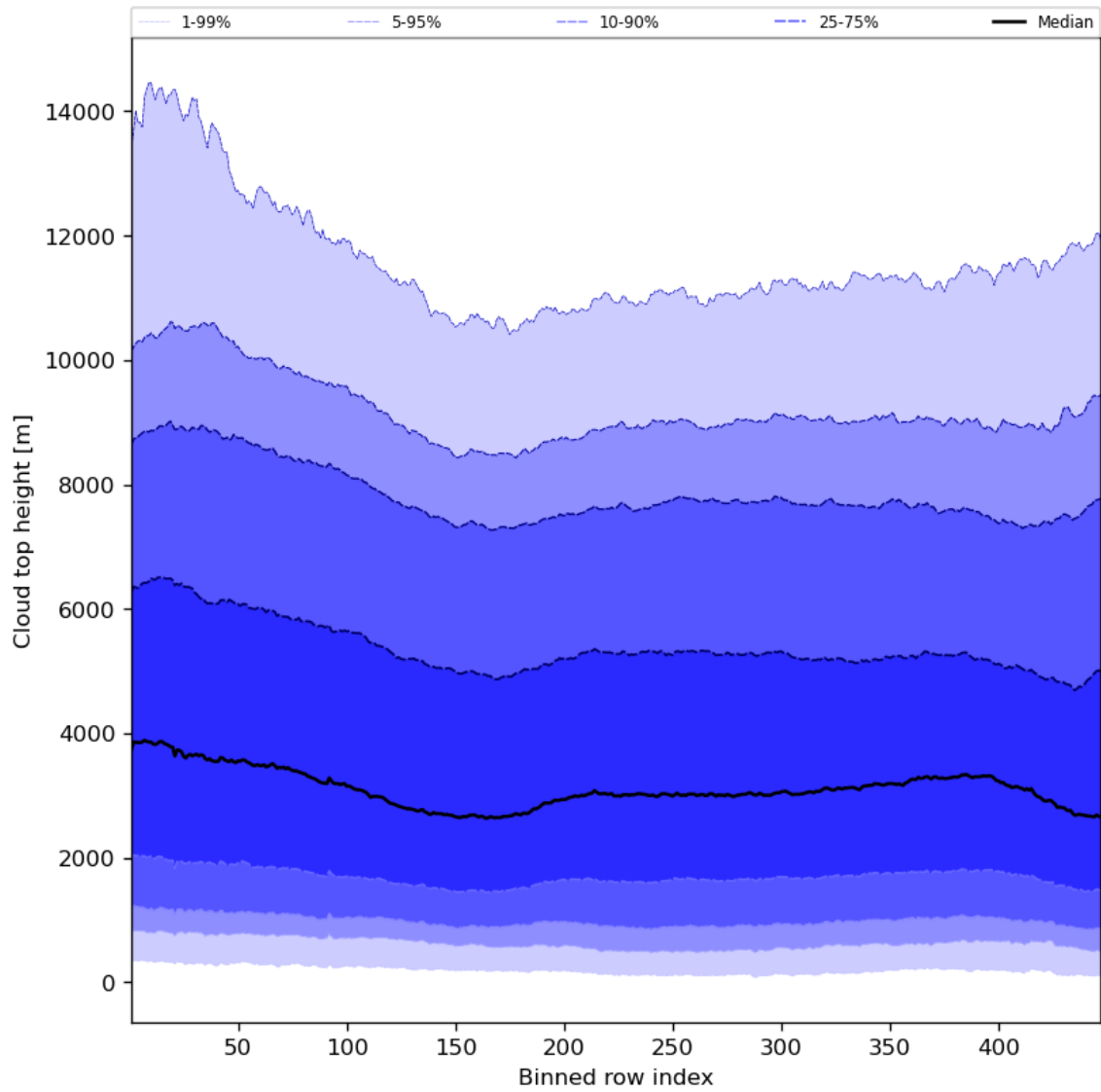
Figure 56: Along track statistics of “Cloud top height” for 2024-03-07 to 2024-03-09
