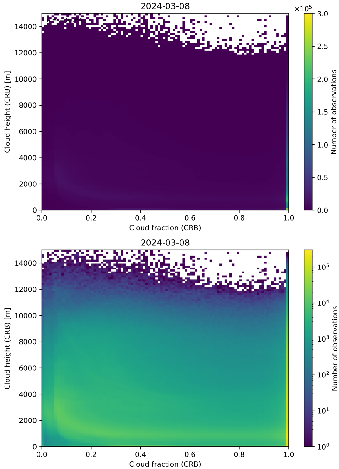
Figure 79: Scatter density plot of “Cloud fraction (CRB)” against “Cloud height (CRB)” for 2024-03-07 to 2024-03-09.
