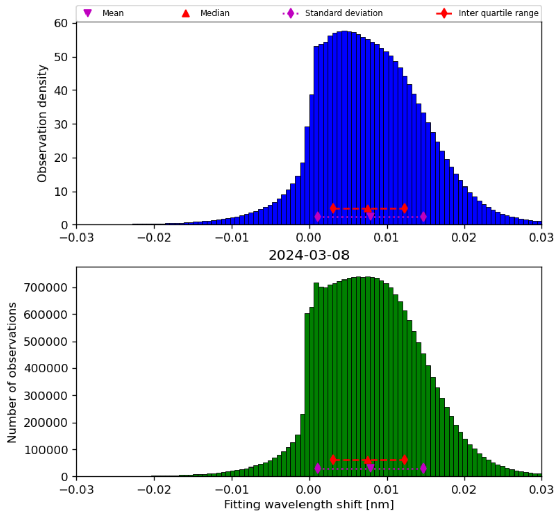
Figure 49: Histogram of “Fitting wavelength shift” for 2024-03-07 to 2024-03-09
