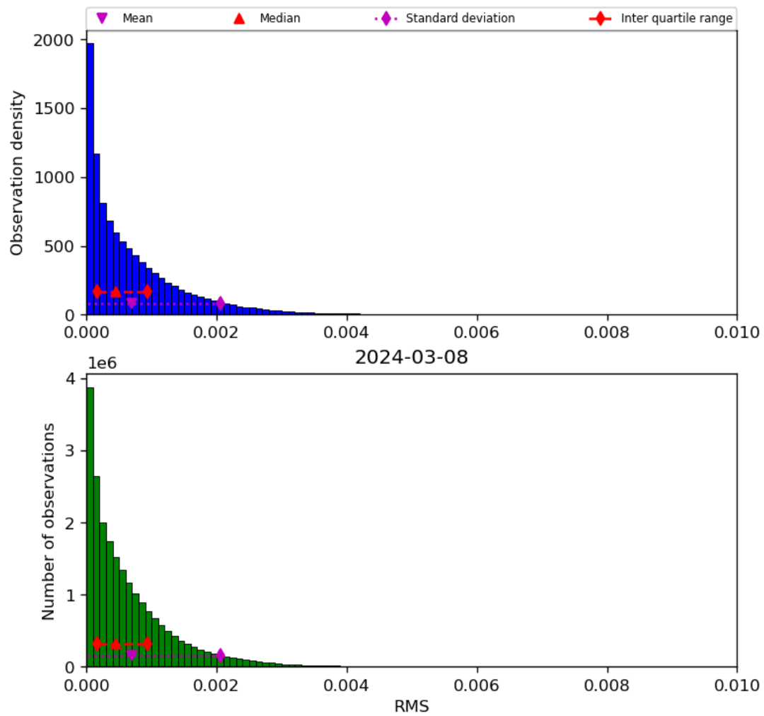
Figure 47: Histogram of “RMS” for 2024-03-07 to 2024-03-09
