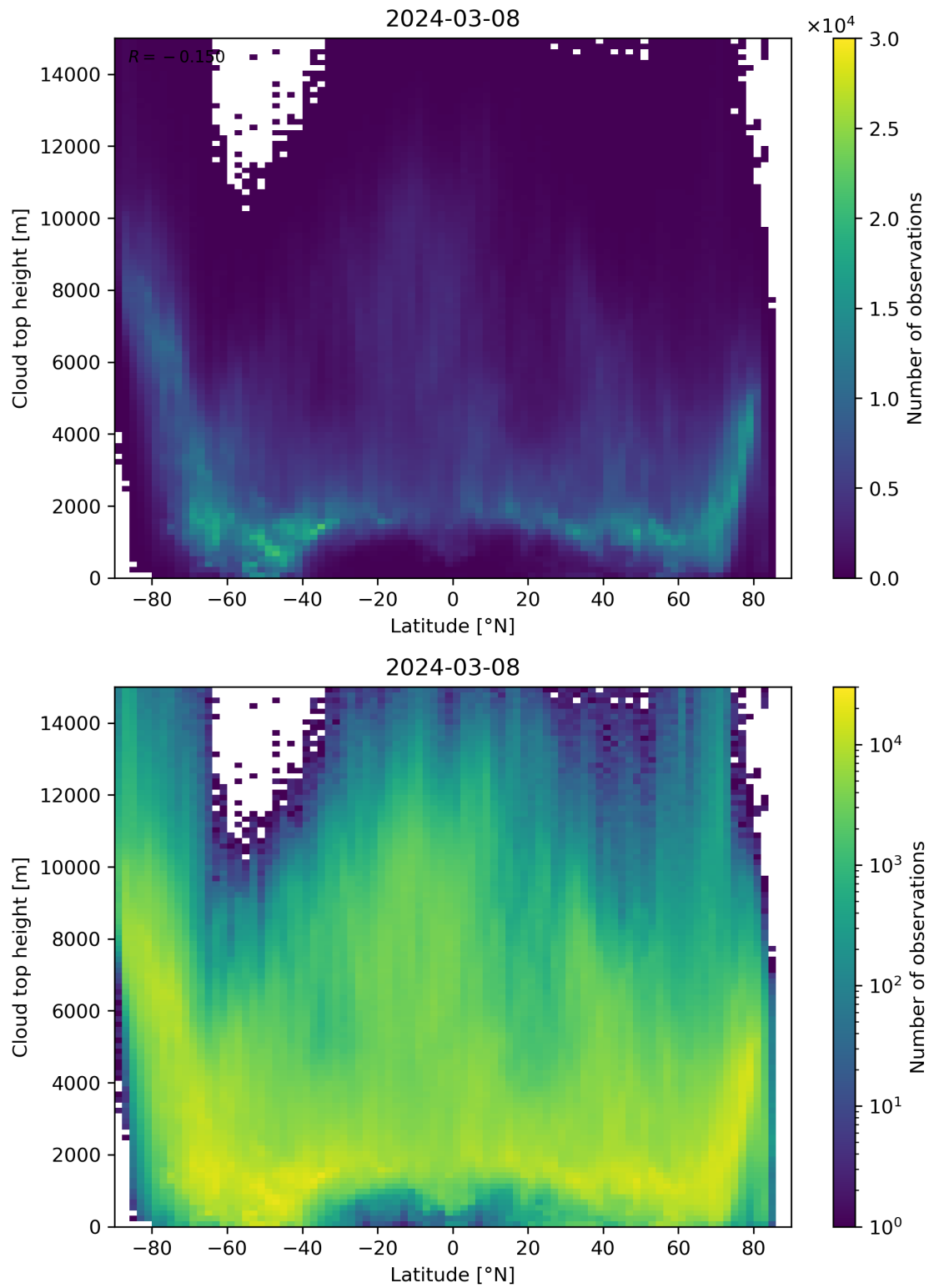
Figure 97: Scatter density plot of “Latitude” against “Cloud top height” for 2024-03-07 to 2024-03-09.
