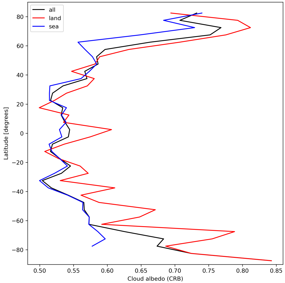
Figure 28: Zonal average of “Cloud albedo (CRB)” for 2024-03-07 to 2024-03-09.
