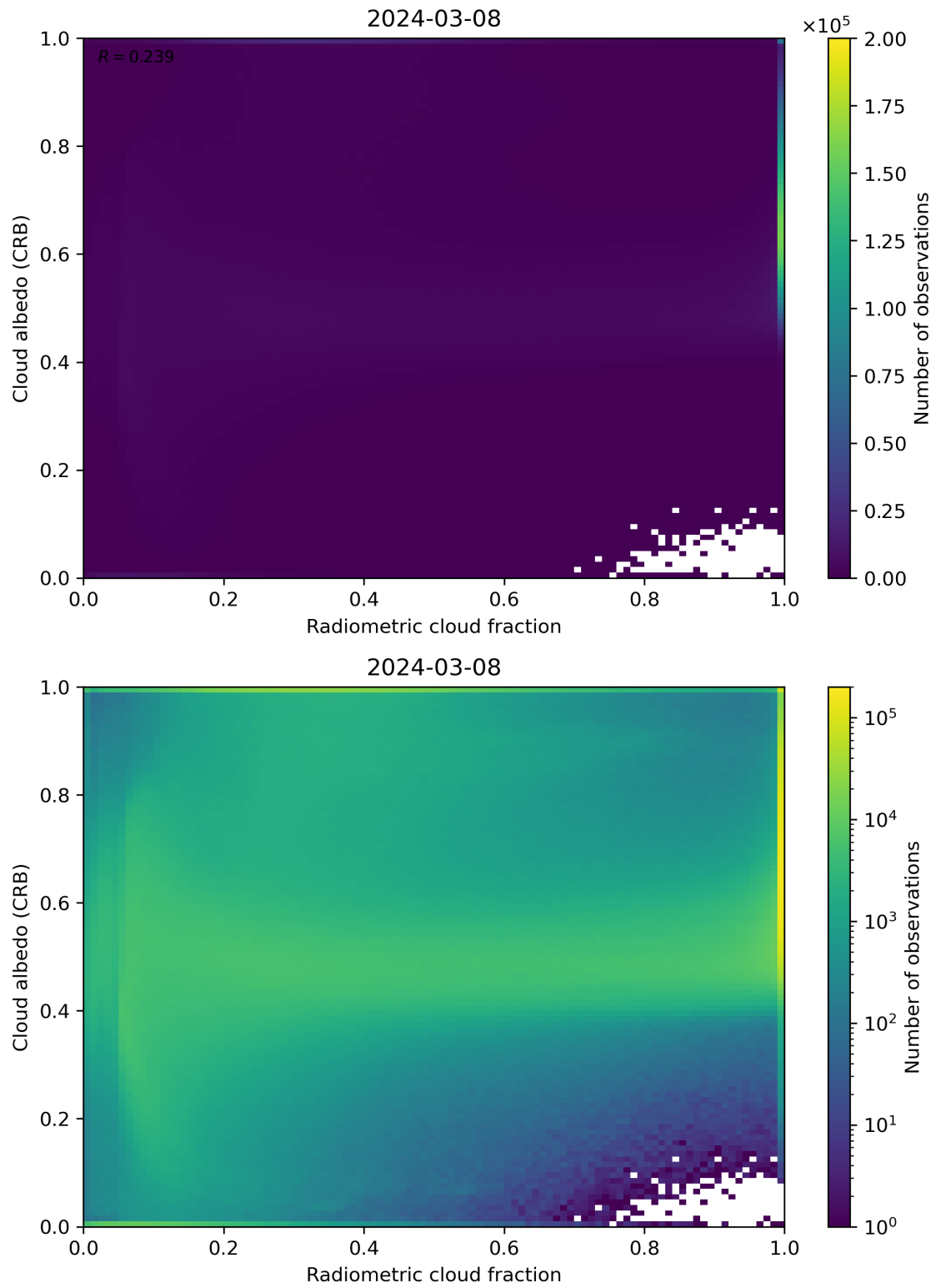
Figure 71: Scatter density plot of “Radiometric cloud fraction” against “Cloud albedo (CRB)” for 2024-03-07 to 2024-03-09.
