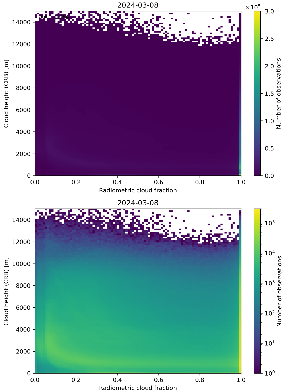
Figure 74: Scatter density plot of “Radiometric cloud fraction” against “Cloud height (CRB)” for 2024-03-07 to 2024-03-09.
