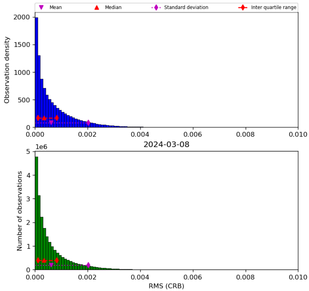
Figure 48: Histogram of “RMS (CRB)” for 2024-03-07 to 2024-03-09
