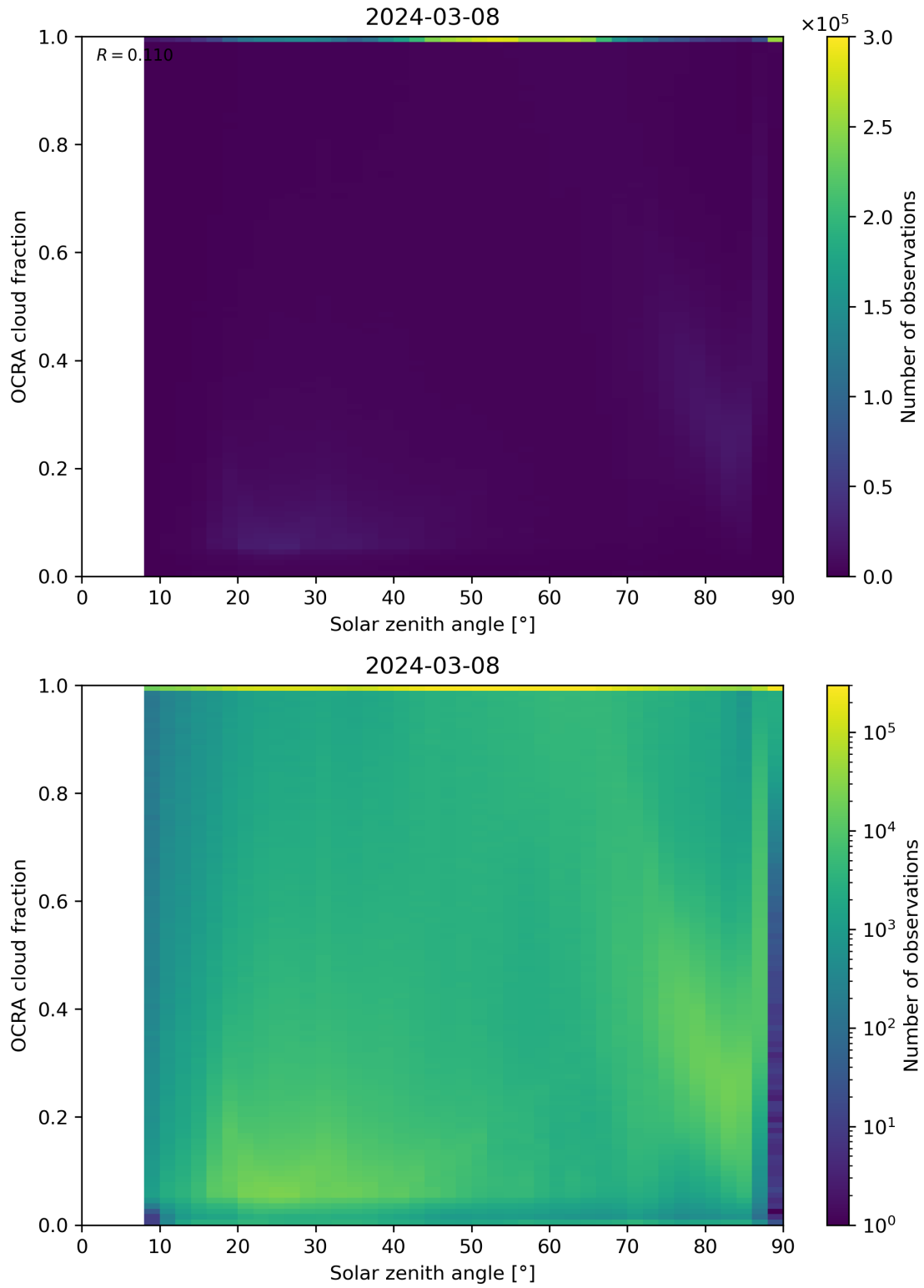
Figure 100: Scatter density plot of “Solar zenith angle” against “OCRA cloud fraction” for 2024-03-07 to 2024-03-09.
