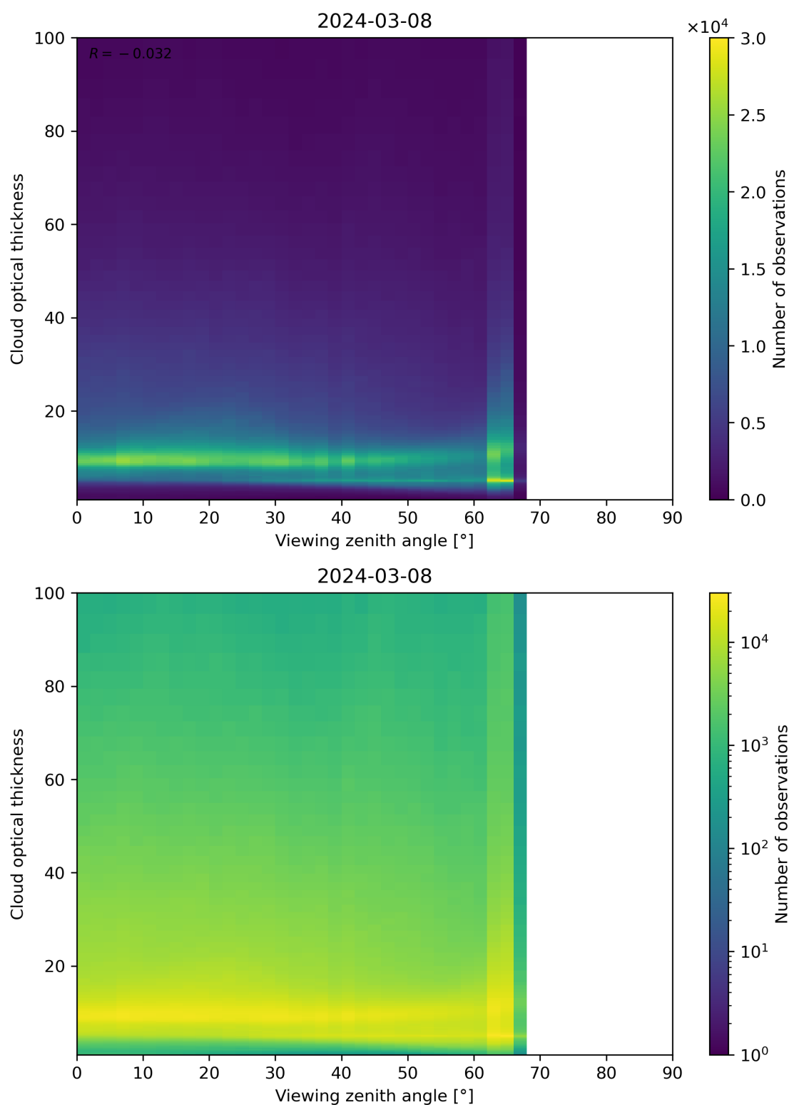
Figure 111: Scatter density plot of “Viewing zenith angle” against “Cloud optical thickness” for 2024-03-07 to 2024-03-09.
