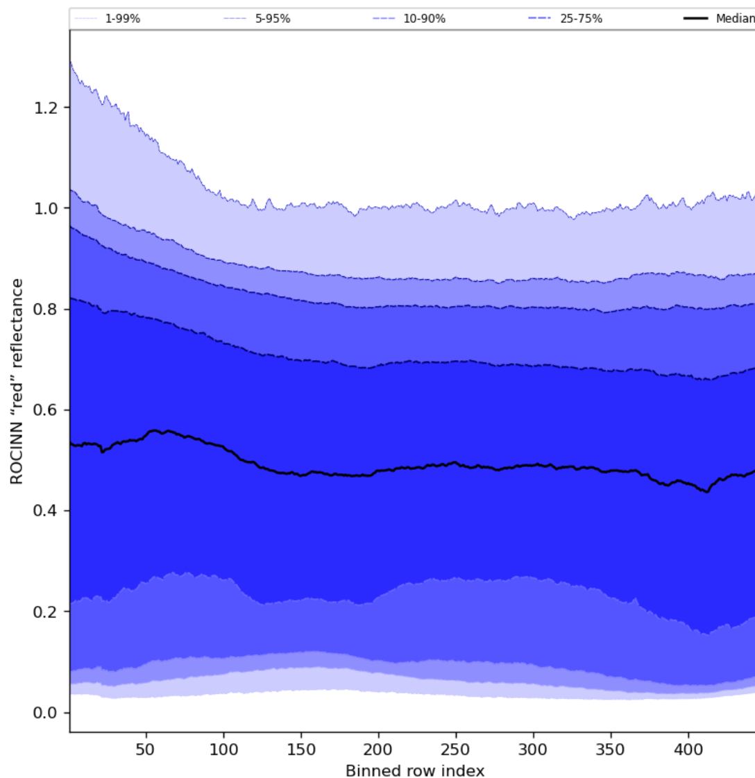
Figure 69: Along track statistics of “ROCINN “red” reflectance” for 2024-03-07 to 2024-03-09
