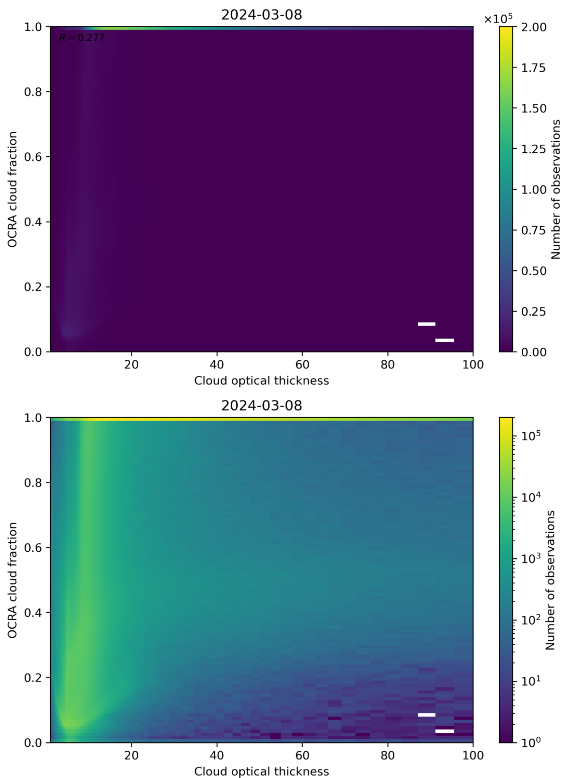
Figure 83: Scatter density plot of “Cloud optical thickness” against “OCRA cloud fraction” for 2024-03-07 to 2024-03-09.
