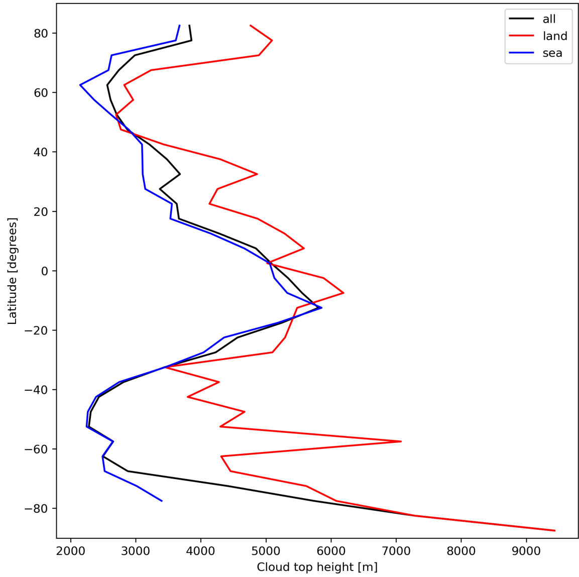
Figure 24: Zonal average of “Cloud top height” for 2024-03-07 to 2024-03-09.
