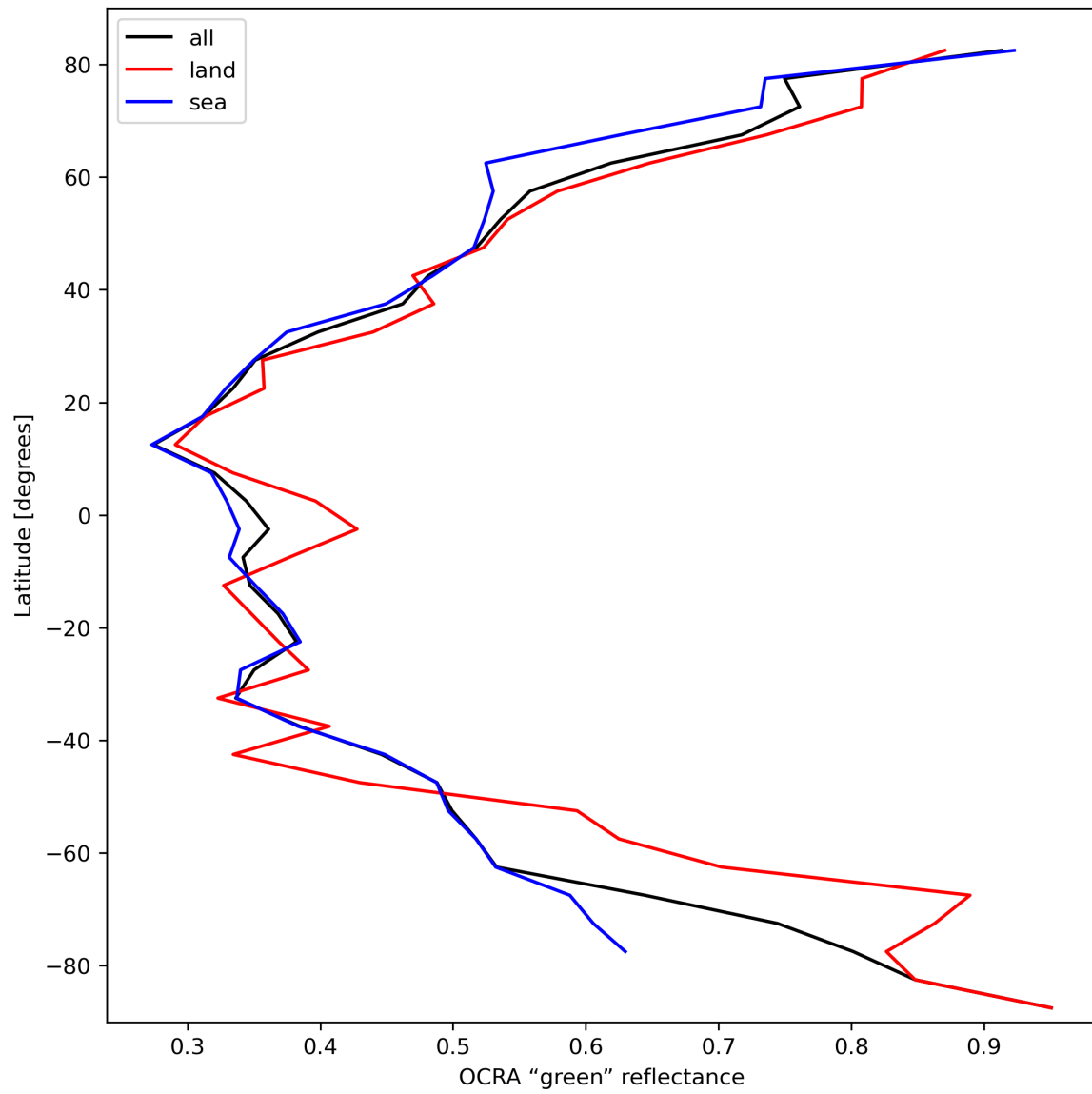
Figure 36: Zonal average of “OCRA “green” reflectance” for 2024-03-07 to 2024-03-09.
