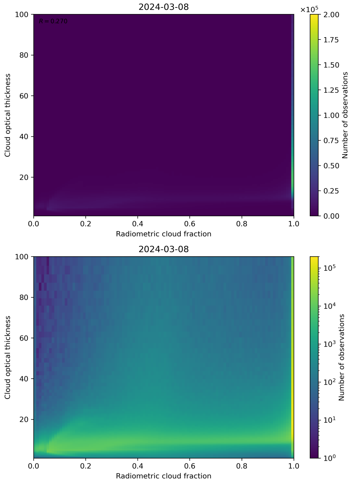
Figure 75: Scatter density plot of “Radiometric cloud fraction” against “Cloud optical thickness” for 2024-03-07 to 2024-03-09.
