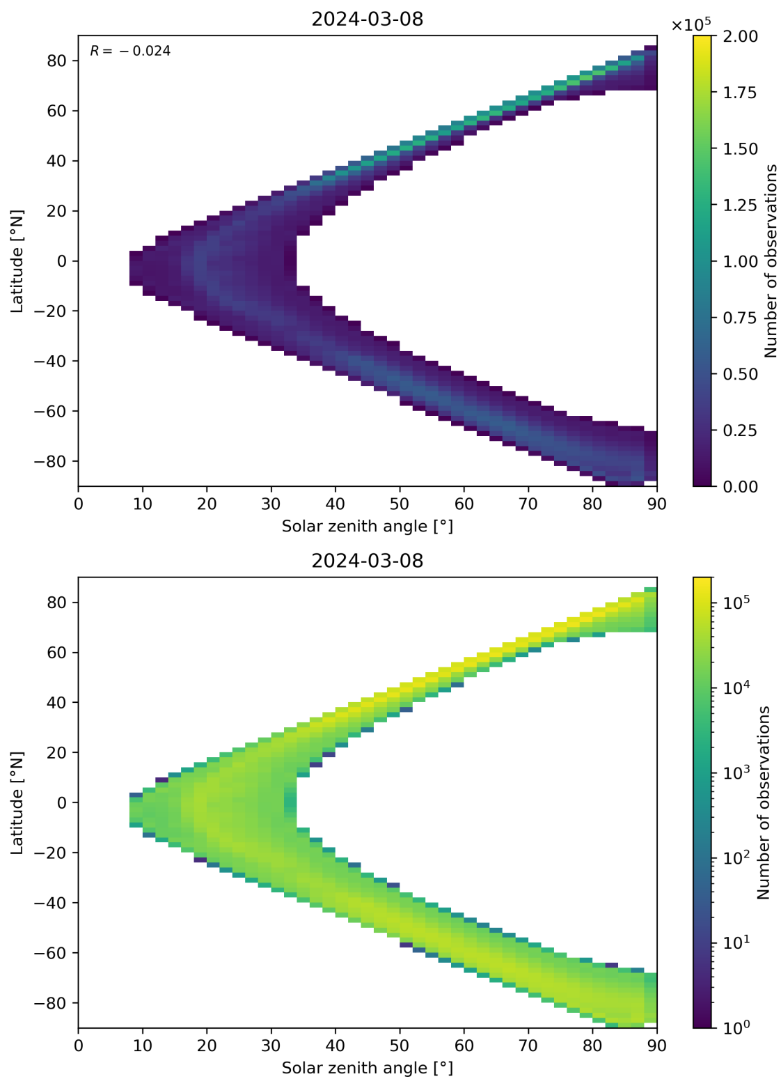
Figure 105: Scatter density plot of “Solar zenith angle” against “Latitude” for 2024-03-07 to 2024-03-09.
