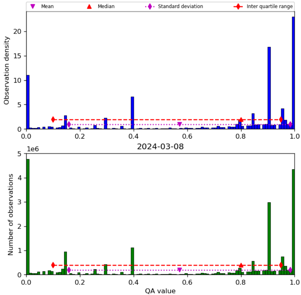
Figure 38: Histogram of “QA value” for 2024-03-07 to 2024-03-09
