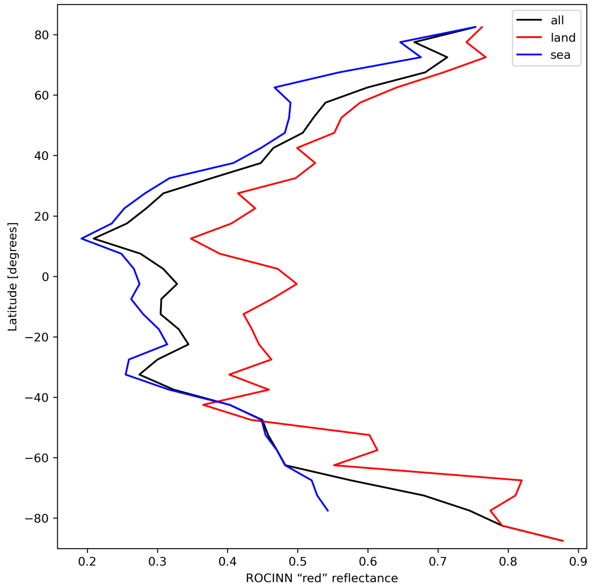
Figure 37: Zonal average of “ROCINN “red” reflectance” for 2024-03-07 to 2024-03-09.
