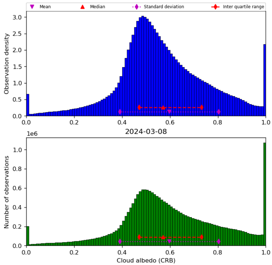
Figure 44: Histogram of “Cloud albedo (CRB)” for 2024-03-07 to 2024-03-09
