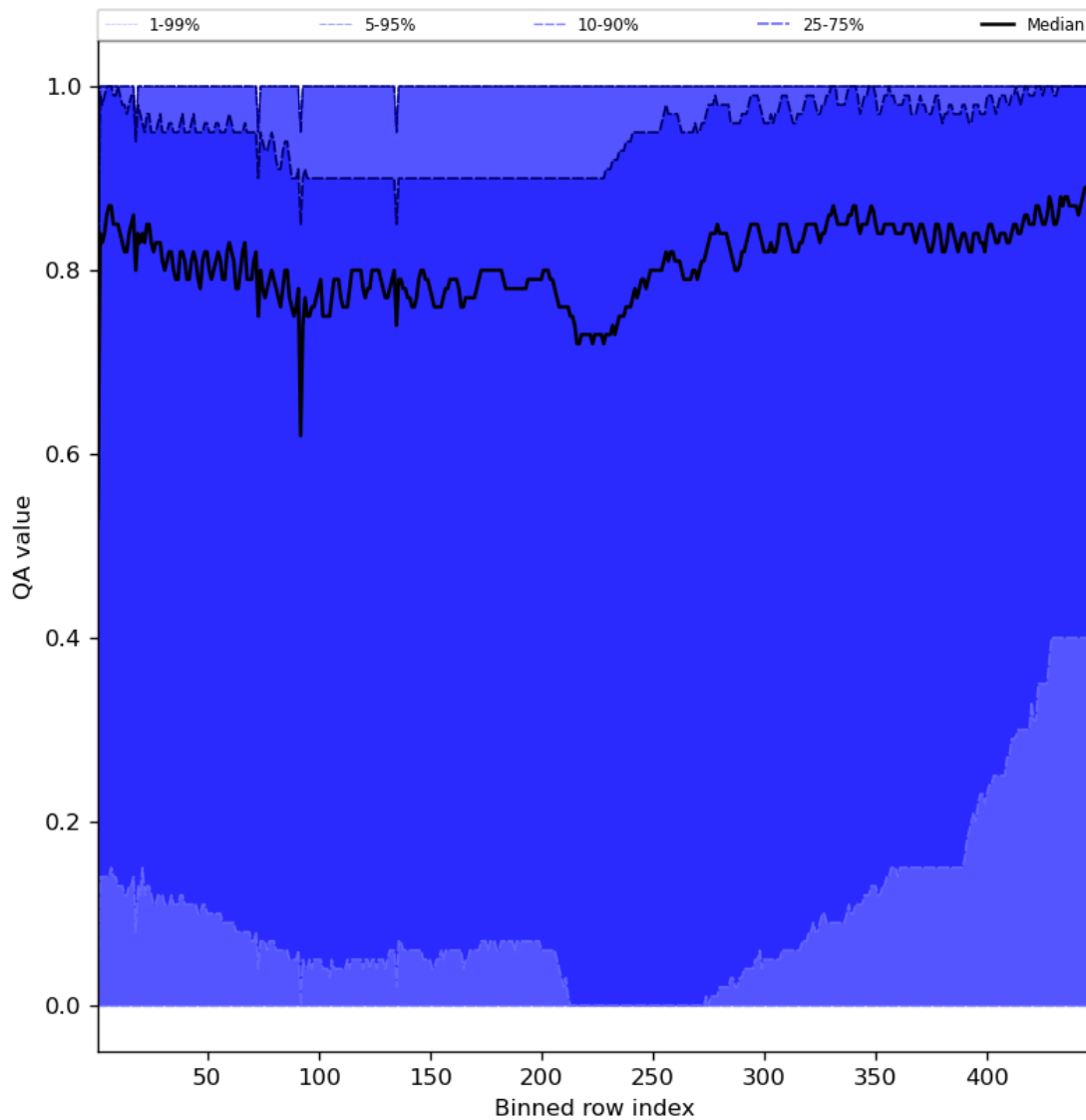
Figure 54: Along track statistics of “QA value” for 2024-03-07 to 2024-03-09
