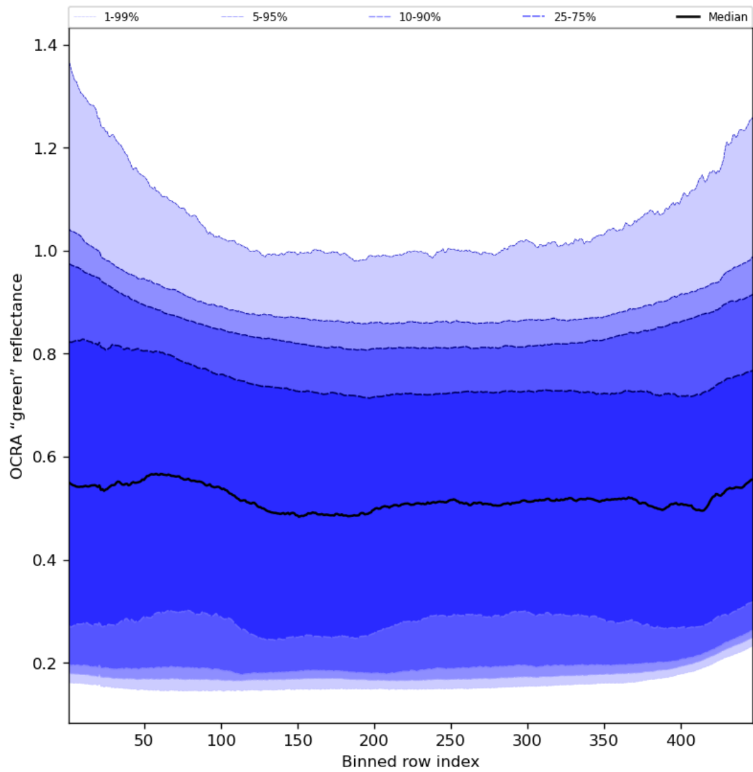
Figure 68: Along track statistics of “OCRA “green” reflectance” for 2024-03-07 to 2024-03-09
