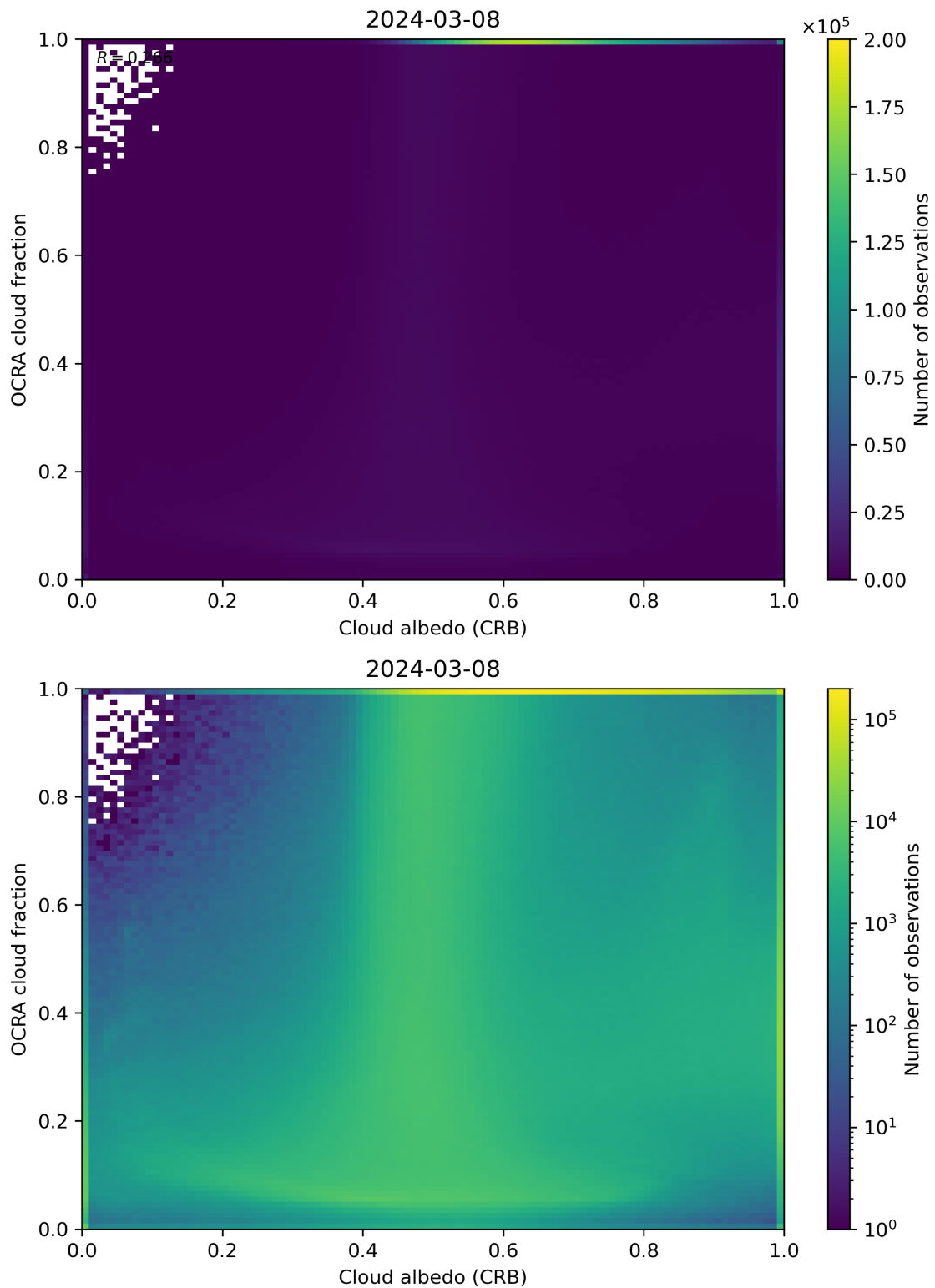
Figure 70: Scatter density plot of “Cloud albedo (CRB)” against “OCRA cloud fraction” for 2024-03-07 to 2024-03-09.
