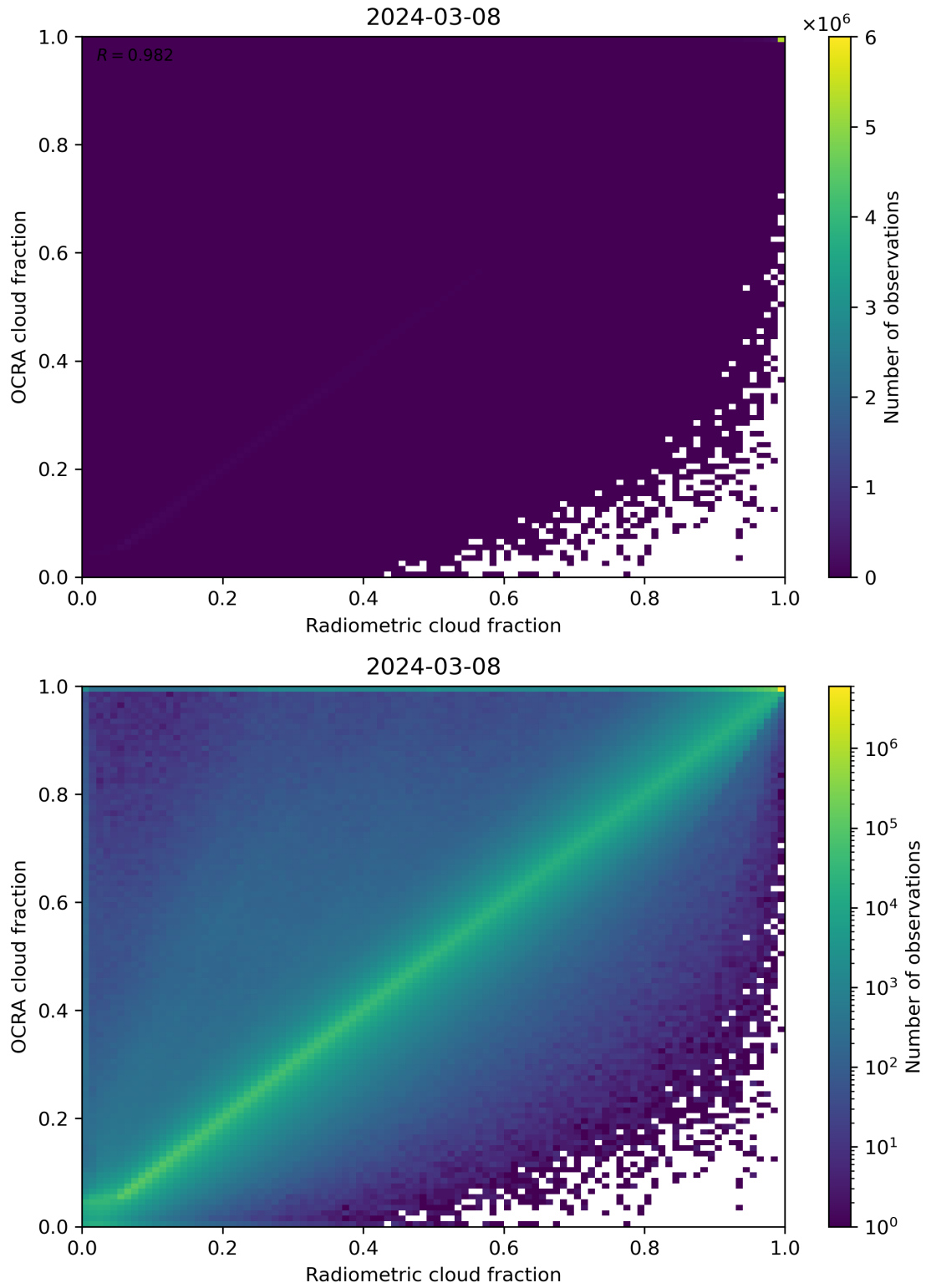
Figure 72: Scatter density plot of “Radiometric cloud fraction” against “OCRA cloud fraction” for 2024-03-07 to 2024-03-09.
