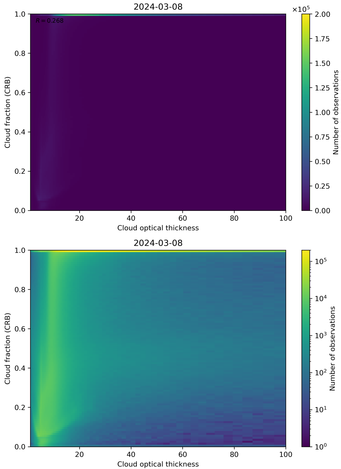
Figure 84: Scatter density plot of “Cloud optical thickness” against “Cloud fraction (CRB)” for 2024-03-07 to 2024-03-09.
