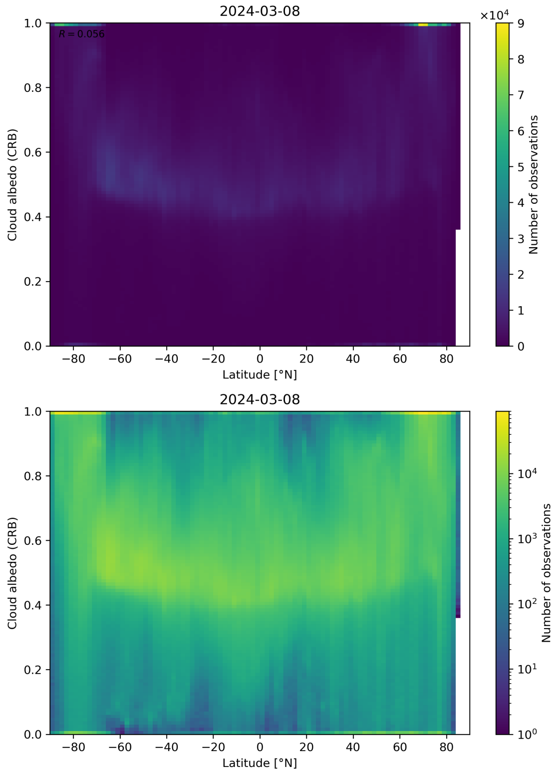
Figure 91: Scatter density plot of “Latitude” against “Cloud albedo (CRB)” for 2024-03-07 to 2024-03-09.
