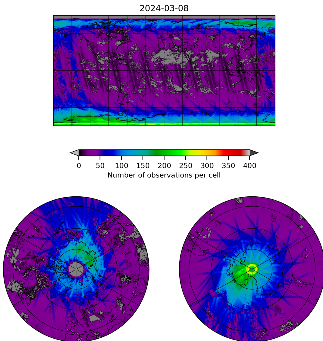
Figure 21: Map of the number of observations for 2024-03-07 to 2024-03-09
