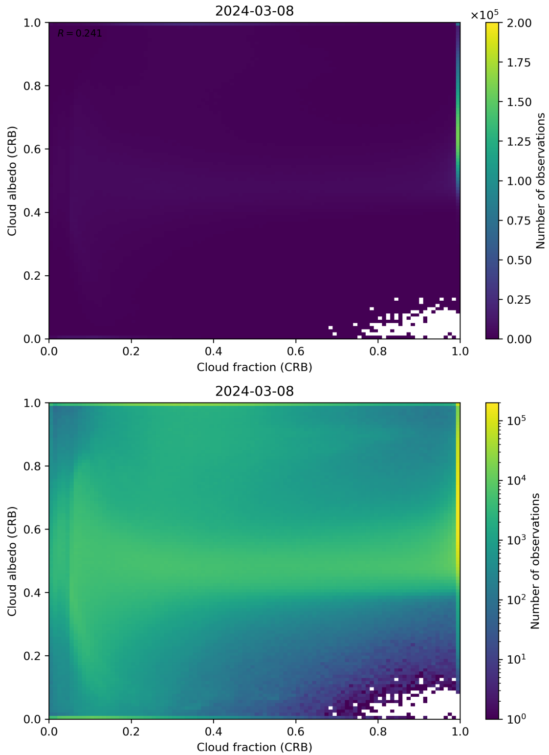
Figure 77: Scatter density plot of “Cloud fraction (CRB)” against “Cloud albedo (CRB)” for 2024-03-07 to 2024-03-09.
