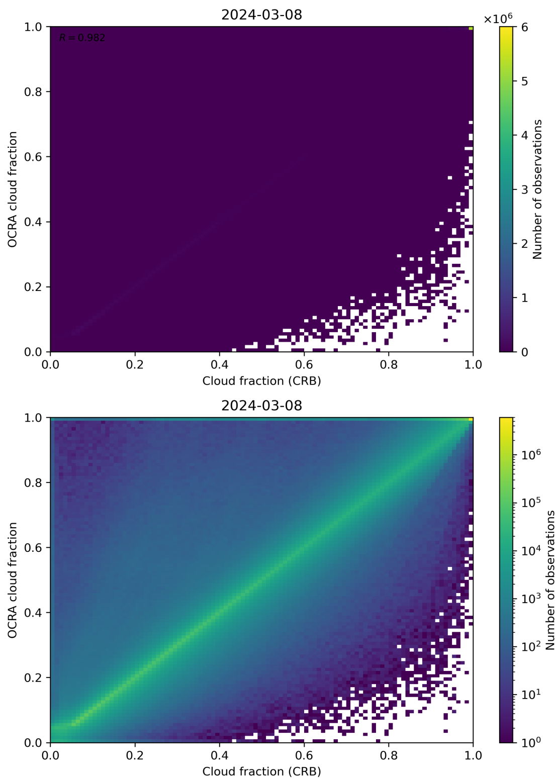
Figure 78: Scatter density plot of “Cloud fraction (CRB)” against “OCRA cloud fraction” for 2024-03-07 to 2024-03-09.
