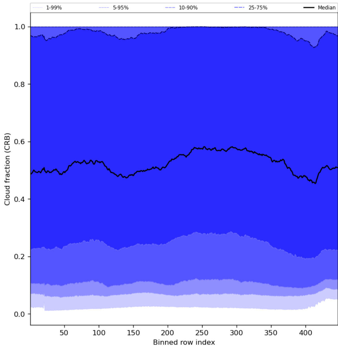
Figure 58: Along track statistics of “Cloud fraction (CRB)” for 2024-03-07 to 2024-03-09
