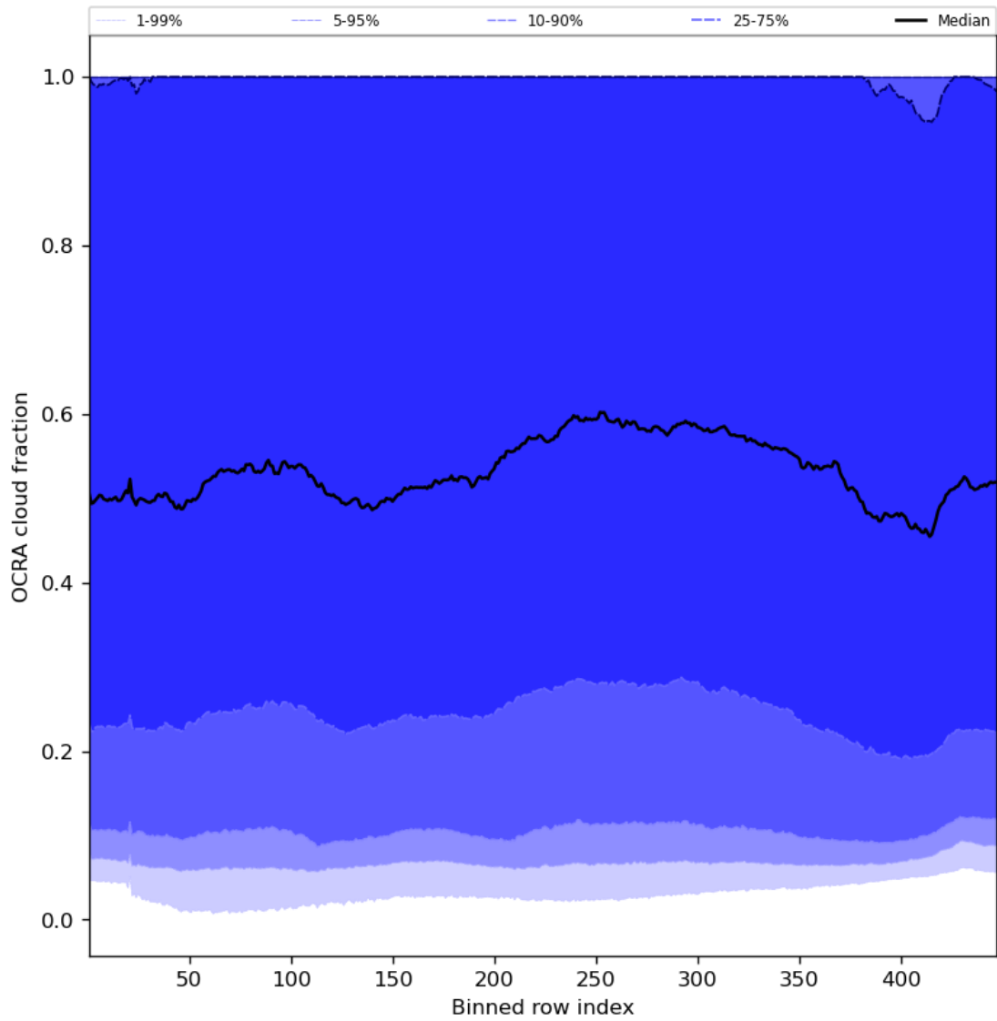
Figure 66: Along track statistics of “OCRA cloud fraction” for 2024-03-07 to 2024-03-09
