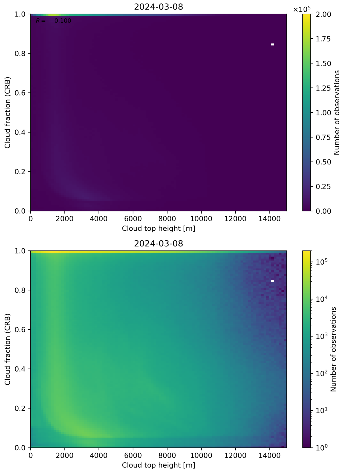
Figure 88: Scatter density plot of “Cloud top height” against “Cloud fraction (CRB)” for 2024-03-07 to 2024-03-09.
