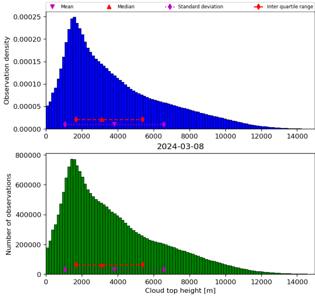
Figure 40: Histogram of “Cloud top height” for 2024-03-07 to 2024-03-09
