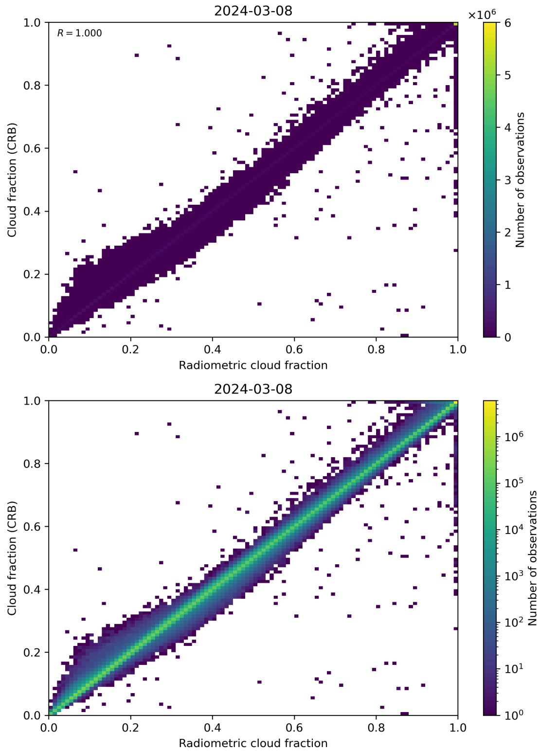
Figure 73: Scatter density plot of “Radiometric cloud fraction” against “Cloud fraction (CRB)” for 2024-03-07 to 2024-03-09.
