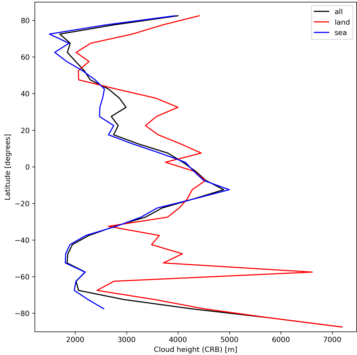
Figure 27: Zonal average of “Cloud height (CRB)” for 2024-03-07 to 2024-03-09.
