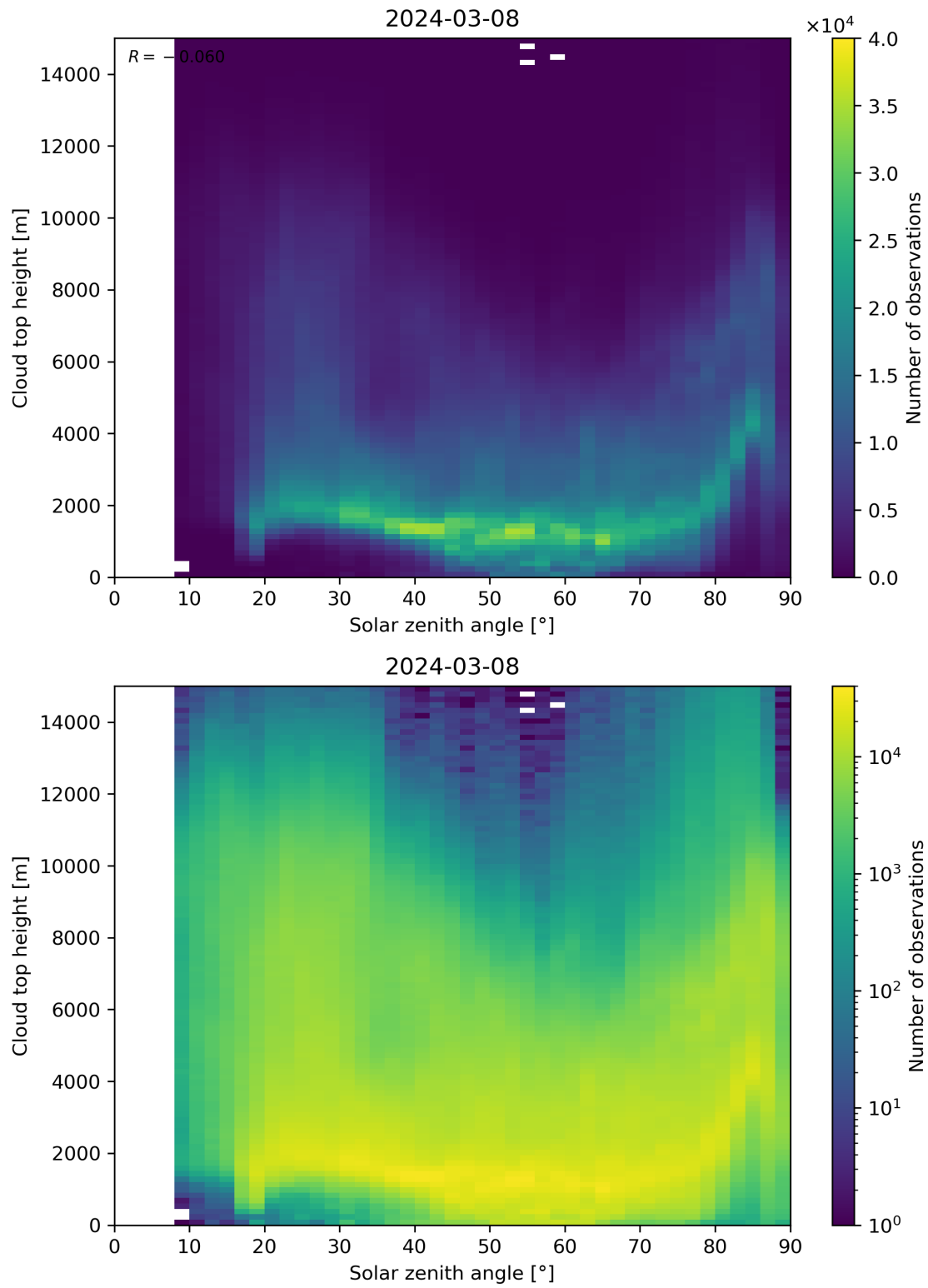
Figure 104: Scatter density plot of “Solar zenith angle” against “Cloud top height” for 2024-03-07 to 2024-03-09.
