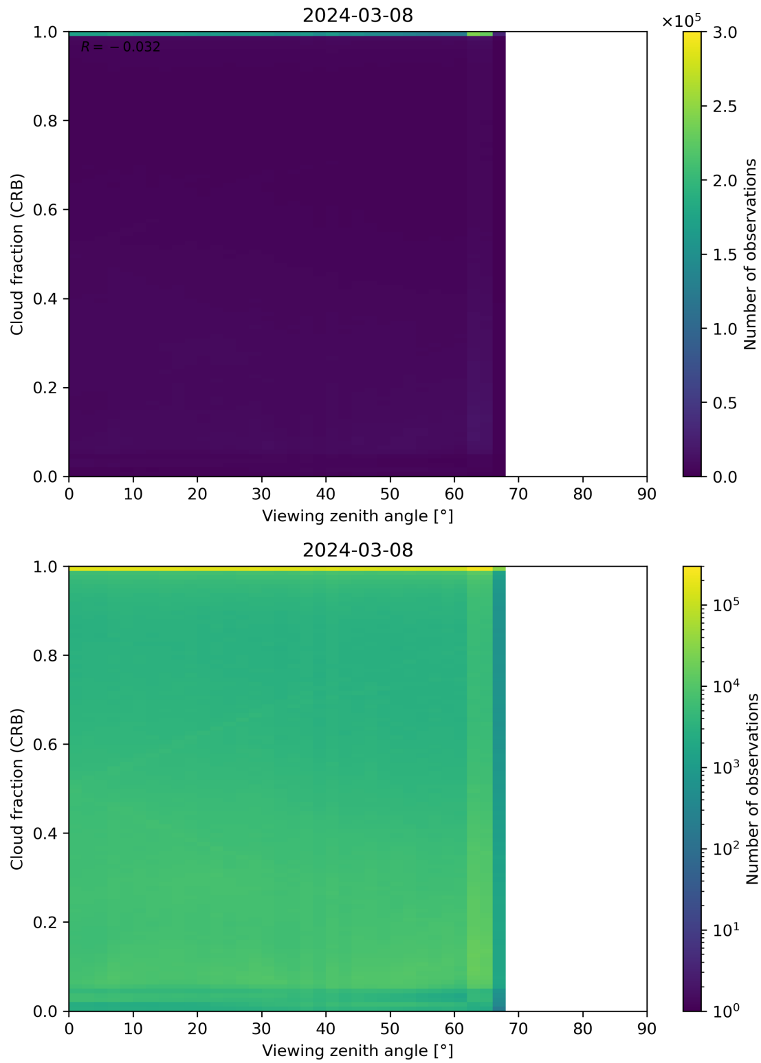
Figure 109: Scatter density plot of “Viewing zenith angle” against “Cloud fraction (CRB)” for 2024-03-07 to 2024-03-09.
