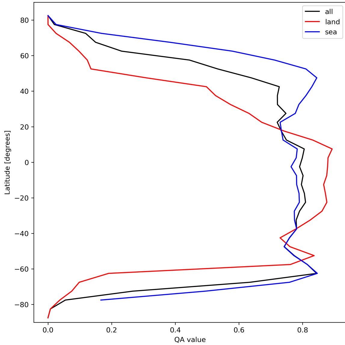
Figure 22: Zonal average of “QA value” for 2024-03-07 to 2024-03-09.
