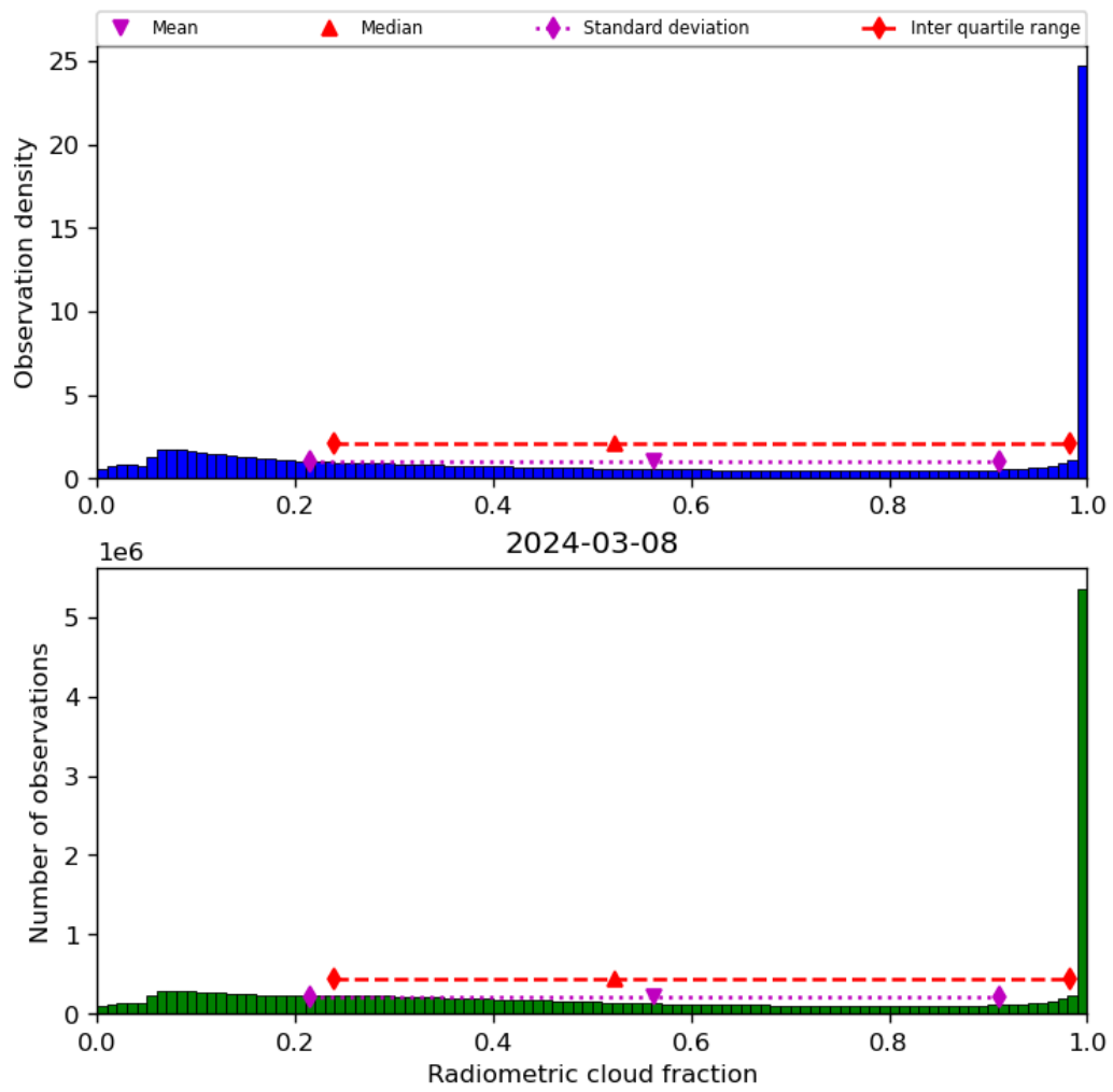
Figure 39: Histogram of “Radiometric cloud fraction” for 2024-03-07 to 2024-03-09
