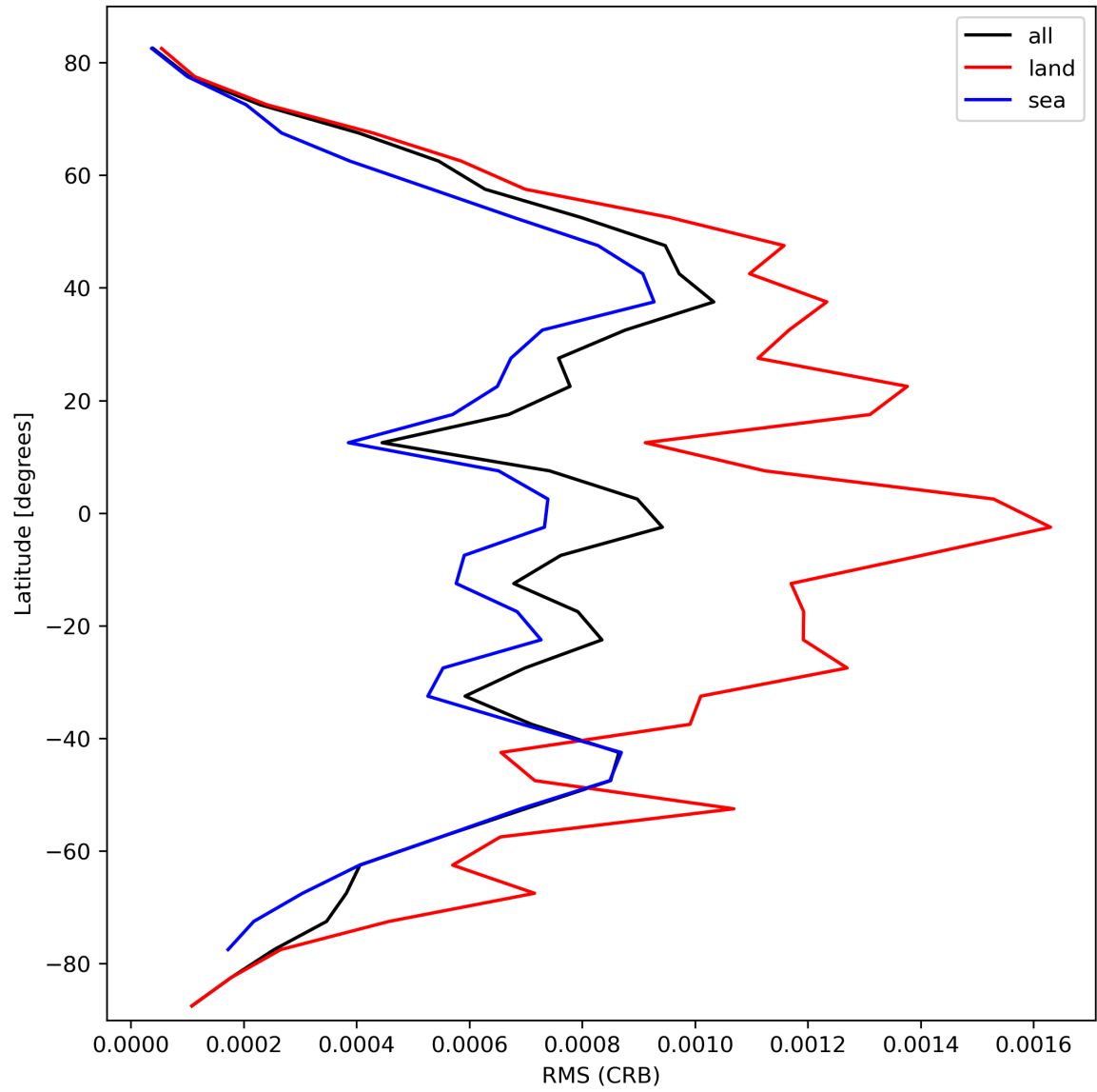
Figure 32: Zonal average of “RMS (CRB)” for 2024-03-07 to 2024-03-09.
