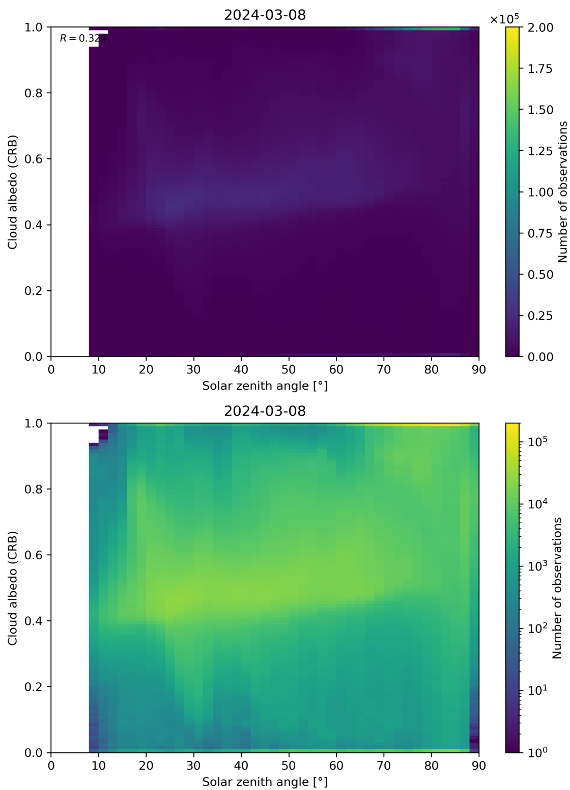
Figure 98: Scatter density plot of “Solar zenith angle” against “Cloud albedo (CRB)” for 2024-03-07 to 2024-03-09.
