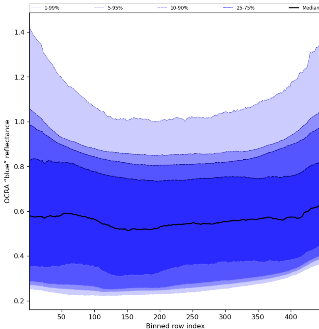
Figure 67: Along track statistics of “OCRA “blue” reflectance” for 2024-03-07 to 2024-03-09
