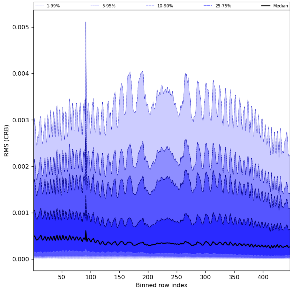
Figure 64: Along track statistics of “RMS (CRB)” for 2024-03-07 to 2024-03-09
