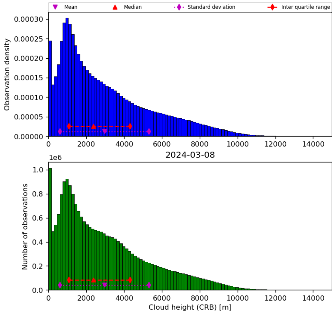
Figure 43: Histogram of “Cloud height (CRB)” for 2024-03-07 to 2024-03-09
