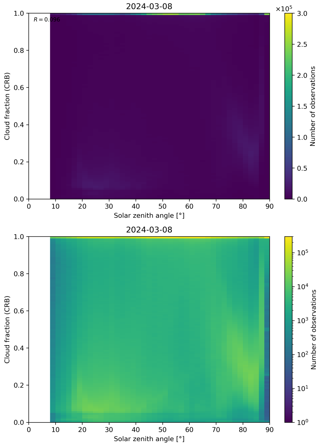
Figure 101: Scatter density plot of “Solar zenith angle” against “Cloud fraction (CRB)” for 2024-03-07 to 2024-03-09.
