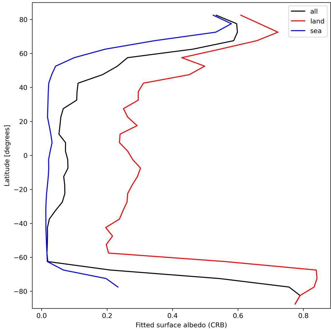
Figure 30: Zonal average of “Fitted surface albedo (CRB)” for 2024-03-07 to 2024-03-09.
