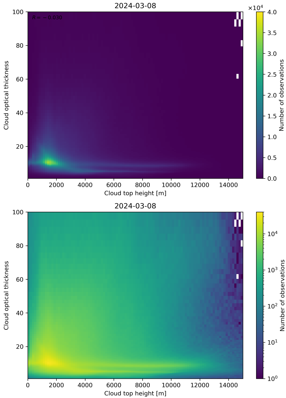
Figure 90: Scatter density plot of “Cloud top height” against “Cloud optical thickness” for 2024-03-07 to 2024-03-09.
