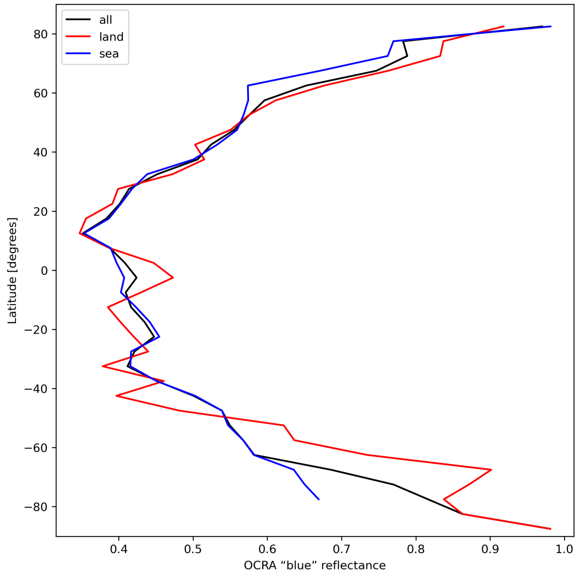
Figure 35: Zonal average of “OCRA “blue” reflectance” for 2024-03-07 to 2024-03-09.
