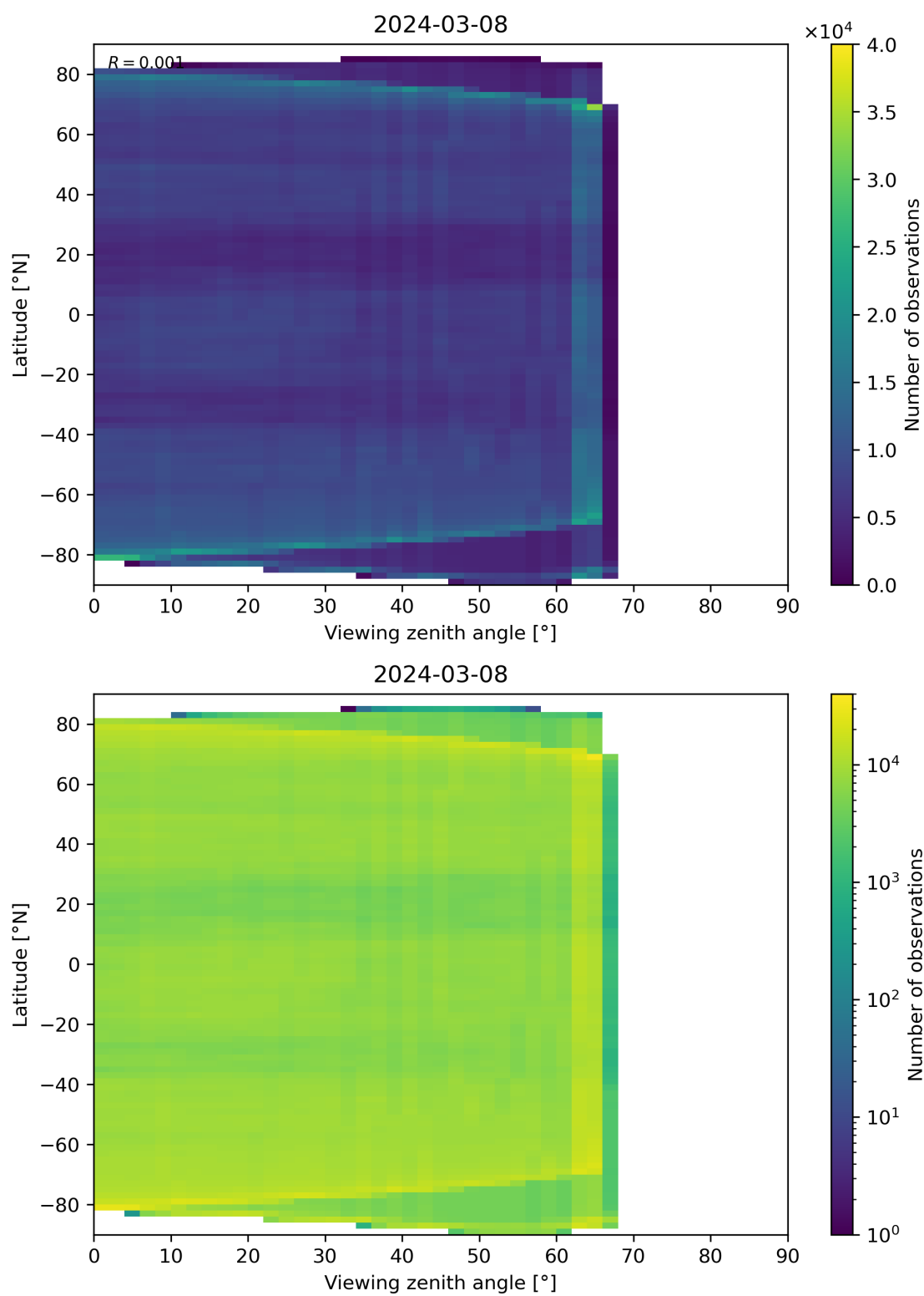
Figure 113: Scatter density plot of “Viewing zenith angle” against “Latitude” for 2024-03-07 to 2024-03-09.
