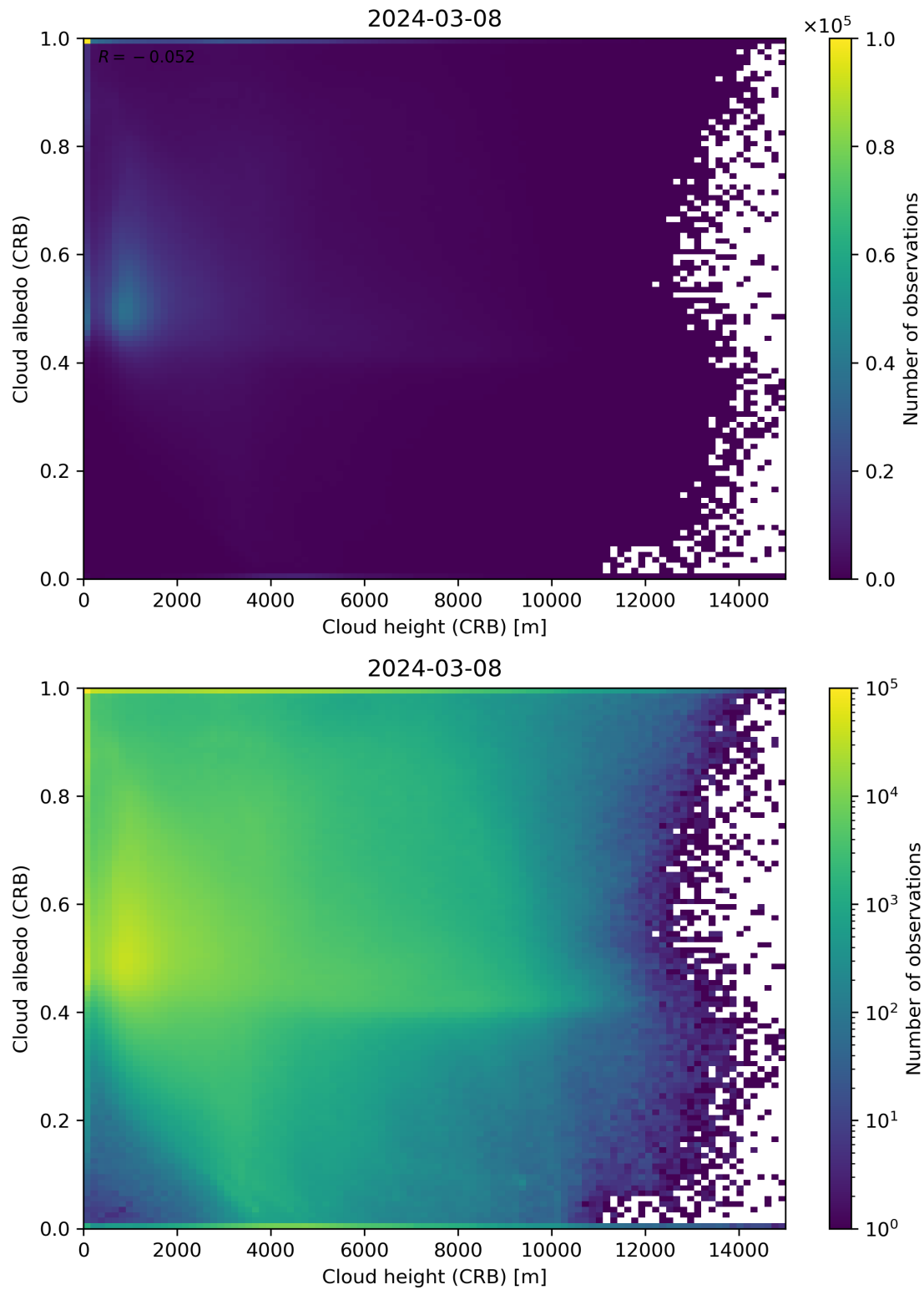
Figure 80: Scatter density plot of “Cloud height (CRB)” against “Cloud albedo (CRB)” for 2024-03-07 to 2024-03-09.
