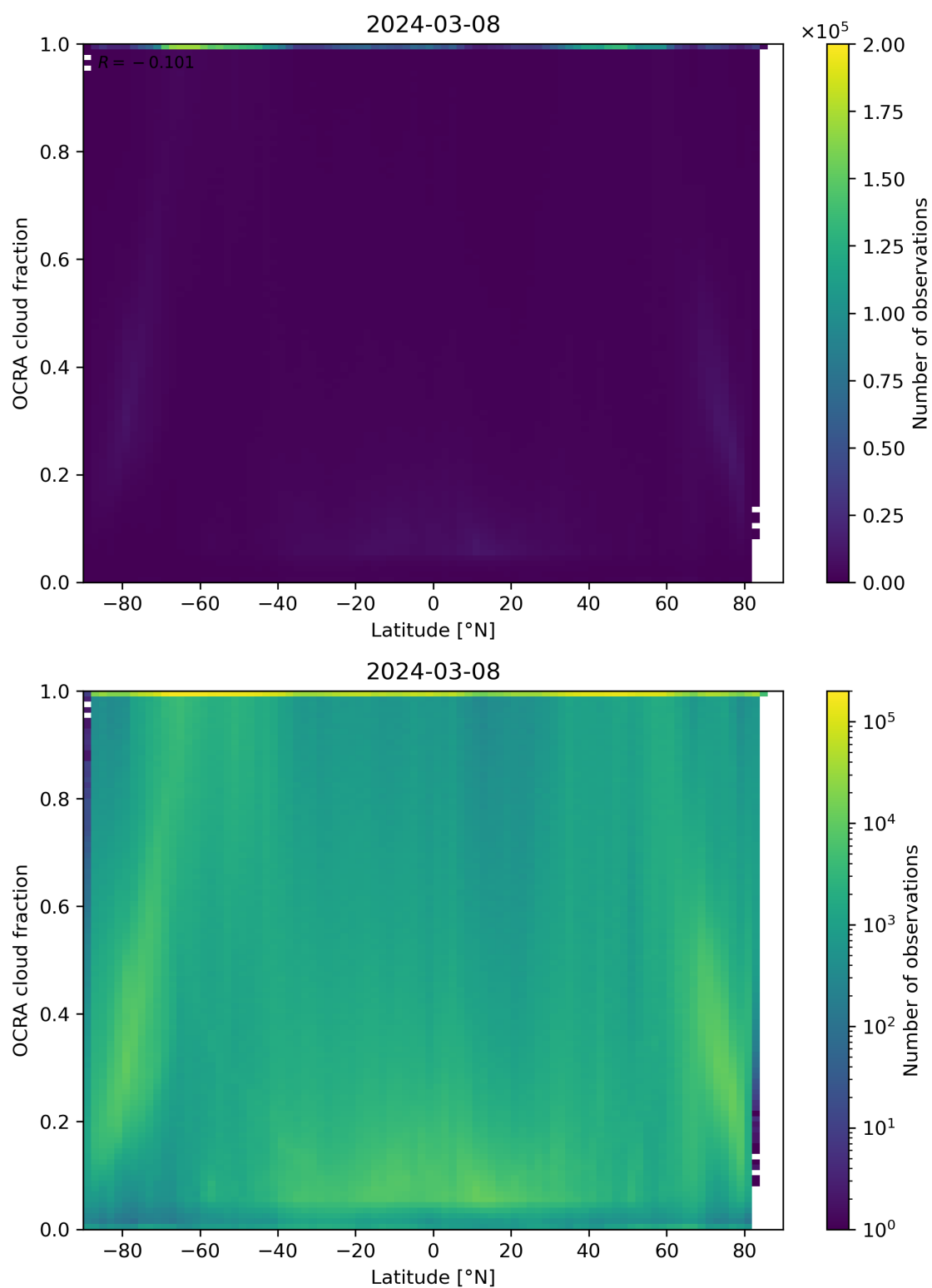
Figure 93: Scatter density plot of “Latitude” against “OCRA cloud fraction” for 2024-03-07 to 2024-03-09.
