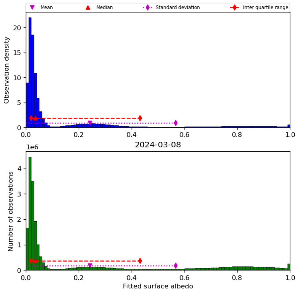
Figure 45: Histogram of “Fitted surface albedo” for 2024-03-07 to 2024-03-09
