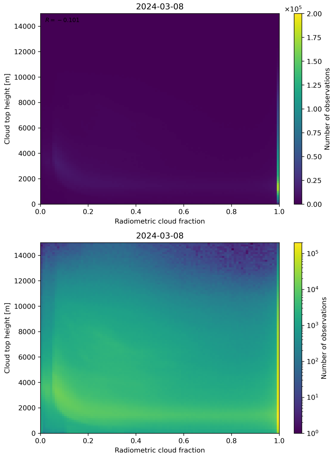
Figure 76: Scatter density plot of “Radiometric cloud fraction” against “Cloud top height” for 2024-03-07 to 2024-03-09.
