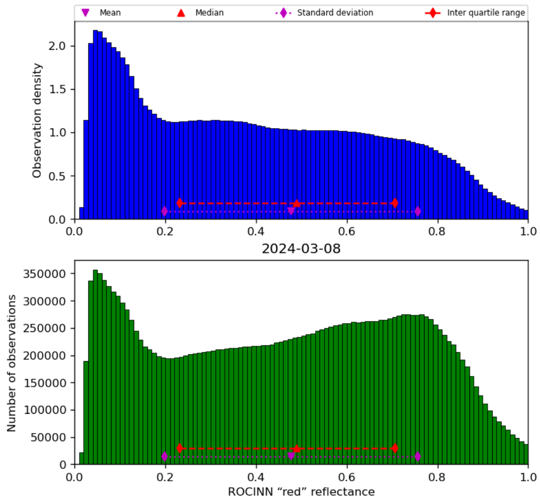
Figure 53: Histogram of “ROCINN “red” reflectance” for 2024-03-07 to 2024-03-09
