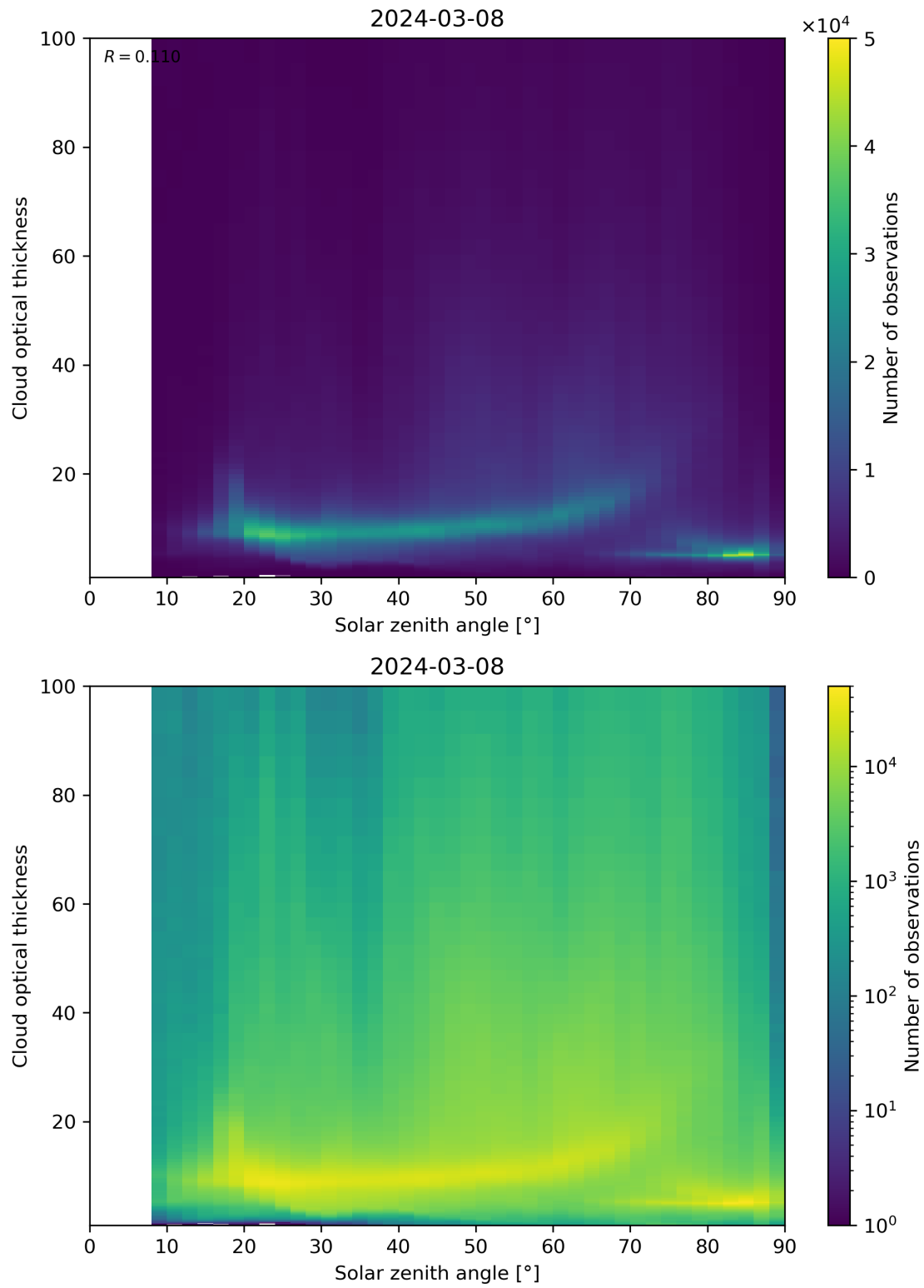
Figure 103: Scatter density plot of “Solar zenith angle” against “Cloud optical thickness” for 2024-03-07 to 2024-03-09.
