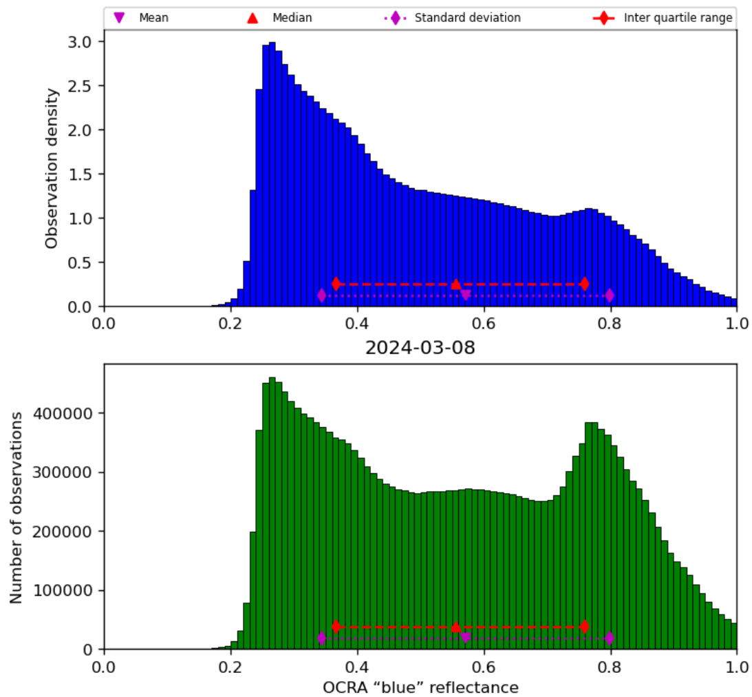
Figure 51: Histogram of “OCRA “blue” reflectance” for 2024-03-07 to 2024-03-09
