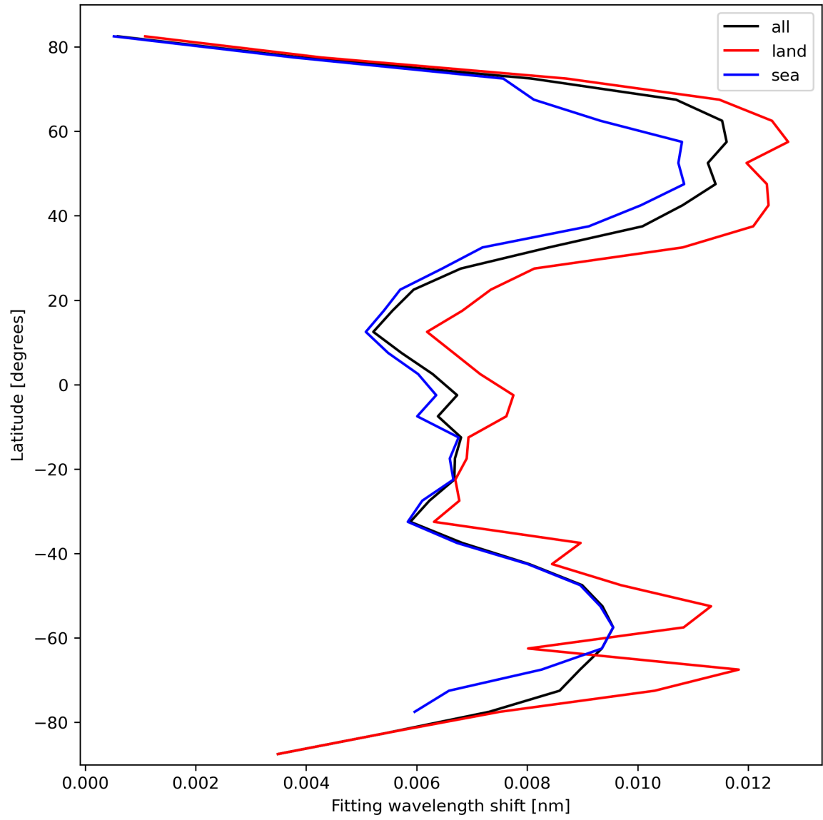
Figure 33: Zonal average of “Fitting wavelength shift” for 2024-03-07 to 2024-03-09.
