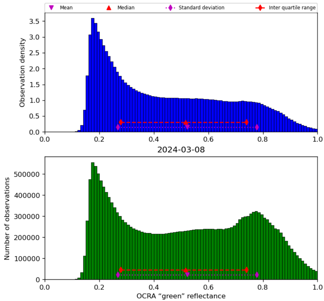
Figure 52: Histogram of “OCRA “green” reflectance” for 2024-03-07 to 2024-03-09
