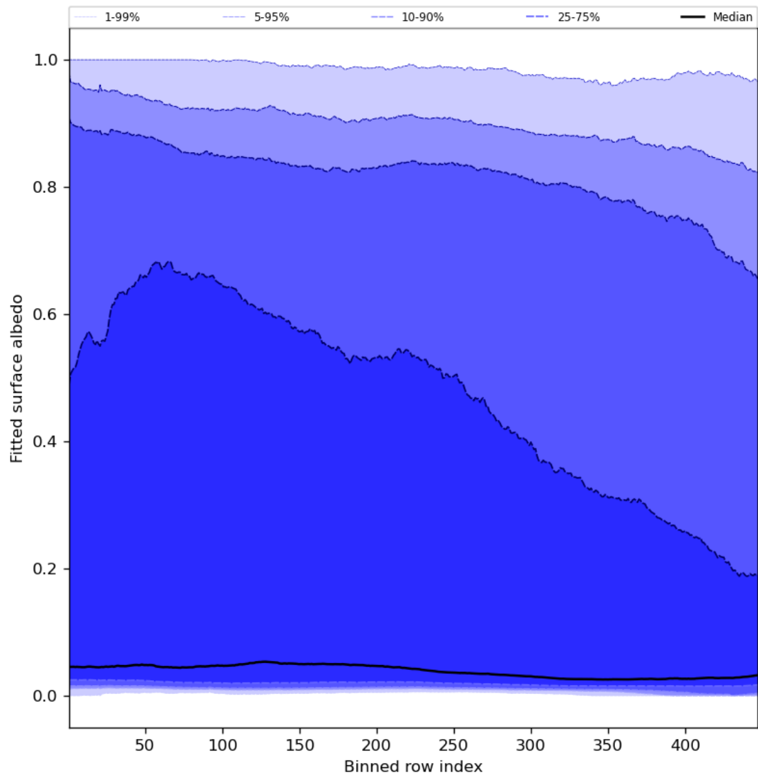
Figure 61: Along track statistics of “Fitted surface albedo” for 2024-03-07 to 2024-03-09
