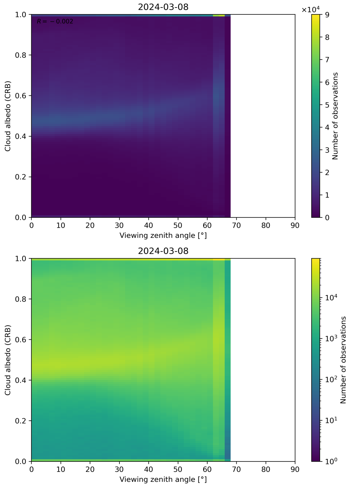
Figure 106: Scatter density plot of “Viewing zenith angle” against “Cloud albedo (CRB)” for 2024-03-07 to 2024-03-09.
