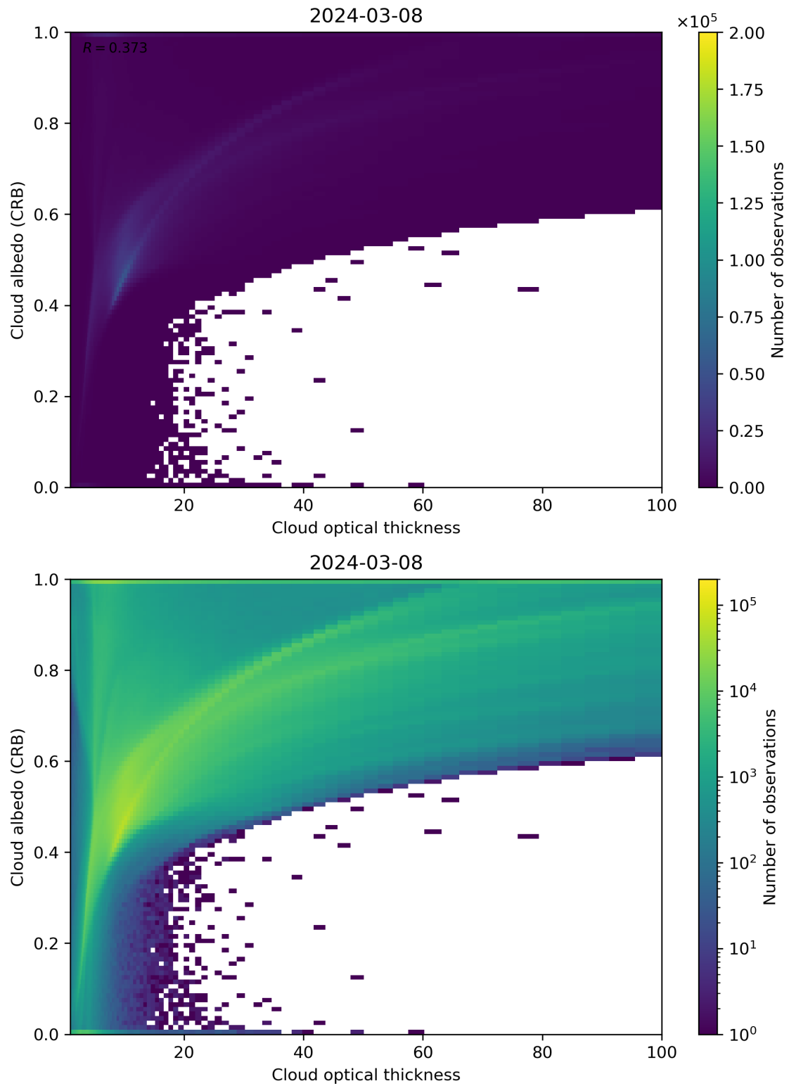
Figure 82: Scatter density plot of “Cloud optical thickness” against “Cloud albedo (CRB)” for 2024-03-07 to 2024-03-09.
