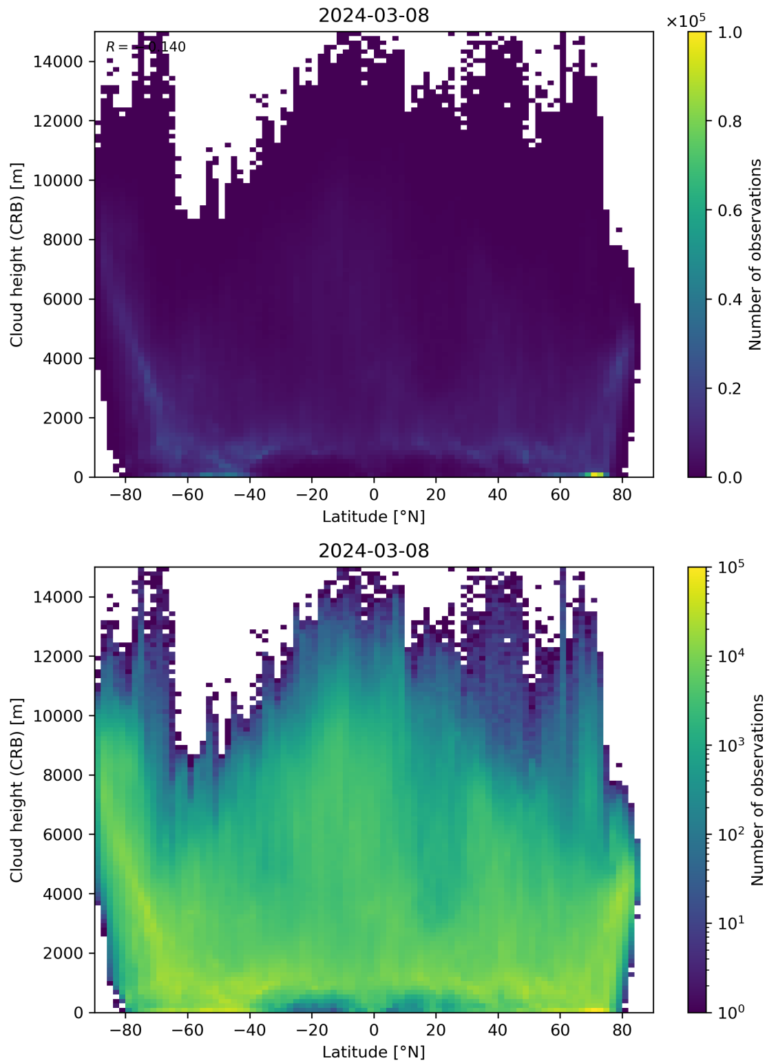
Figure 95: Scatter density plot of “Latitude” against “Cloud height (CRB)” for 2024-03-07 to 2024-03-09.
