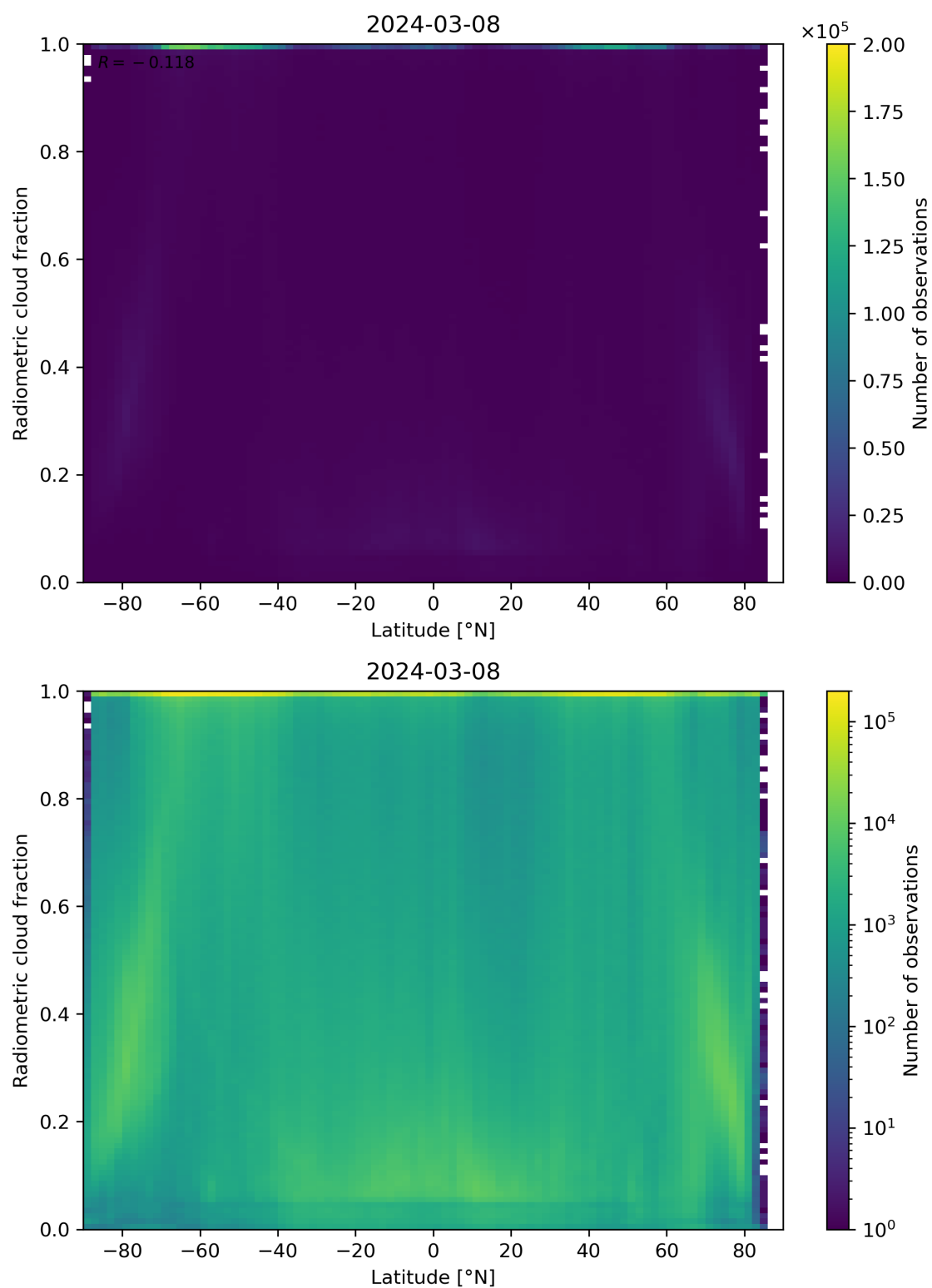
Figure 92: Scatter density plot of “Latitude” against “Radiometric cloud fraction” for 2024-03-07 to 2024-03-09.
