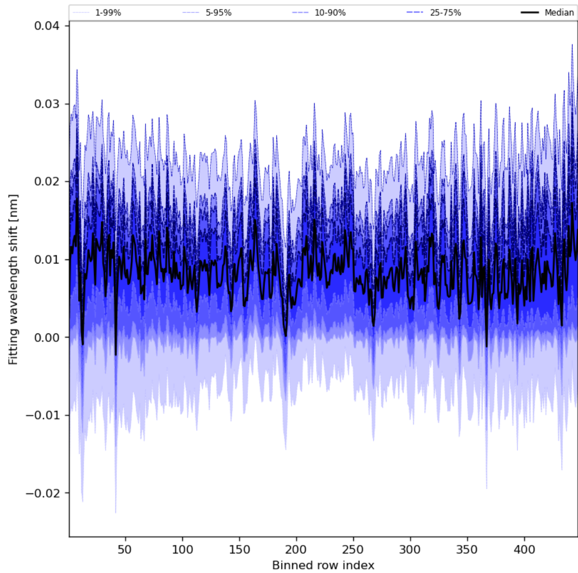
Figure 65: Along track statistics of “Fitting wavelength shift” for 2024-03-07 to 2024-03-09
