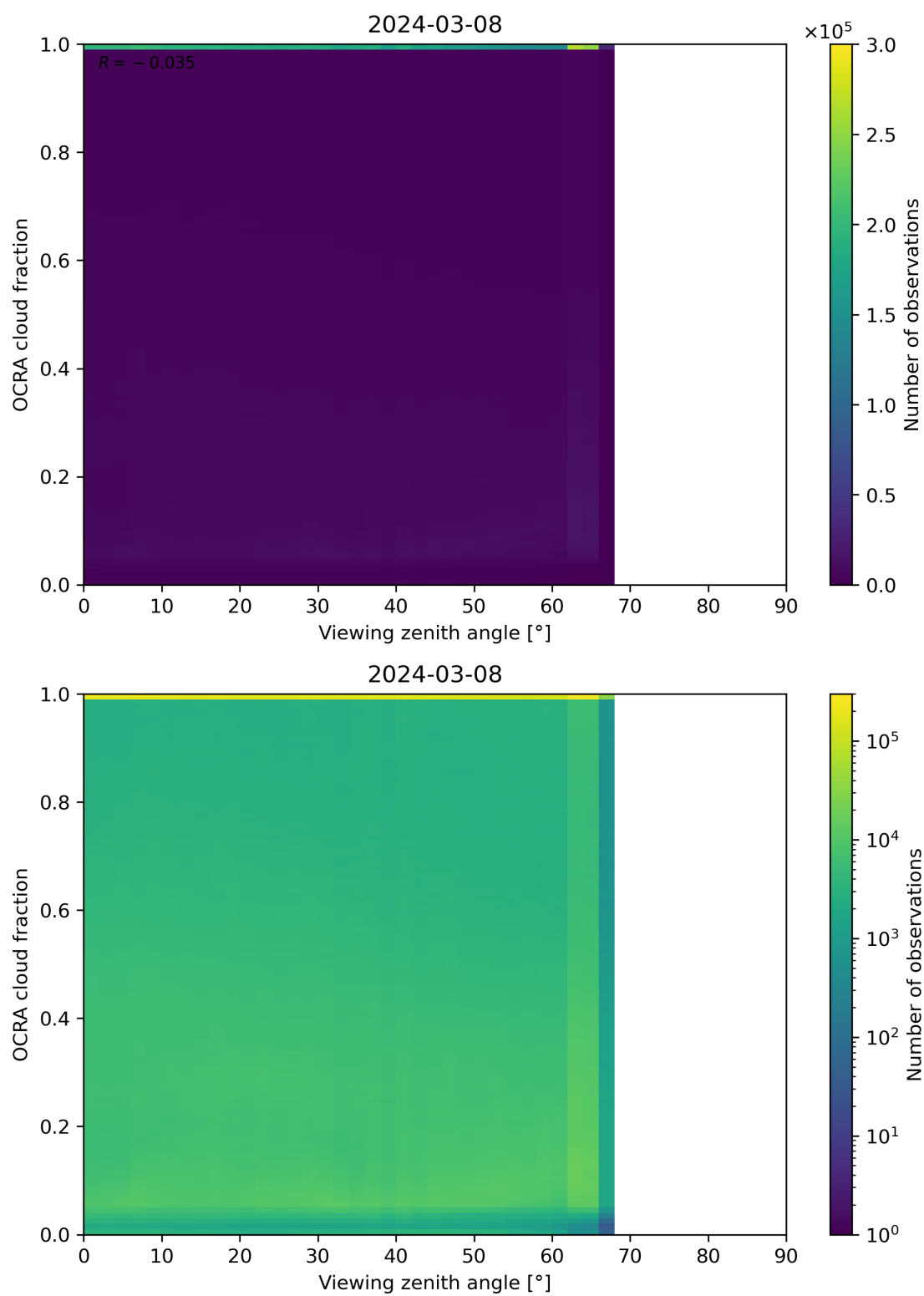
Figure 108: Scatter density plot of “Viewing zenith angle” against “OCRA cloud fraction” for 2024-03-07 to 2024-03-09.
