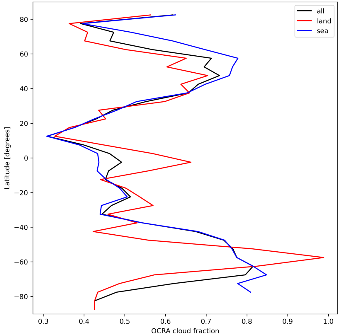
Figure 34: Zonal average of “OCRA cloud fraction” for 2024-03-07 to 2024-03-09.
