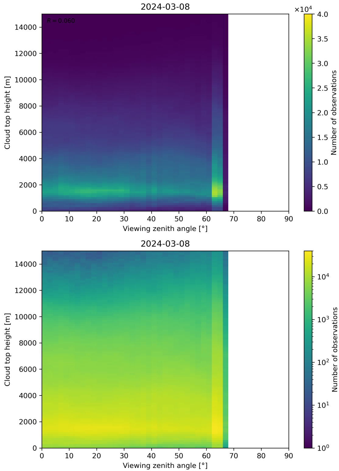
Figure 112: Scatter density plot of “Viewing zenith angle” against “Cloud top height” for 2024-03-07 to 2024-03-09.
