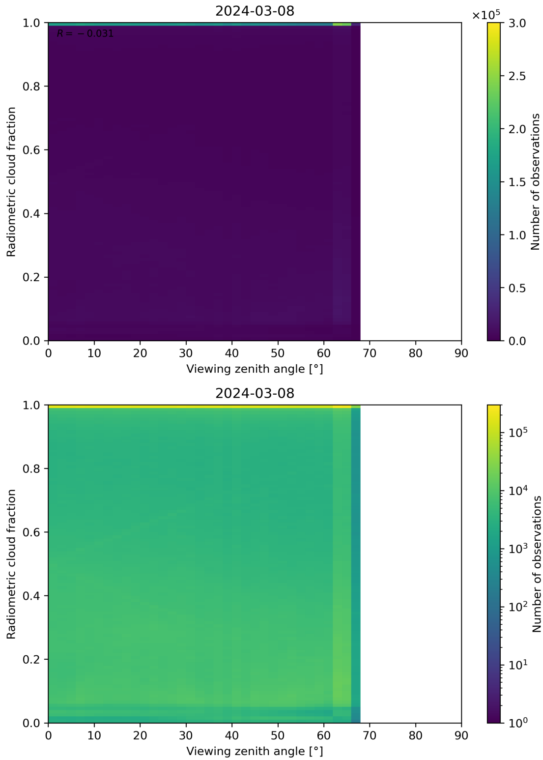
Figure 107: Scatter density plot of “Viewing zenith angle” against “Radiometric cloud fraction” for 2024-03-07 to 2024-03-09.
