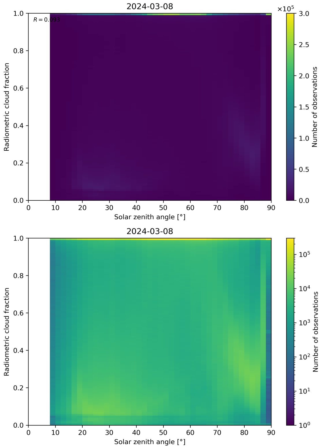
Figure 99: Scatter density plot of “Solar zenith angle” against “Radiometric cloud fraction” for 2024-03-07 to 2024-03-09.
