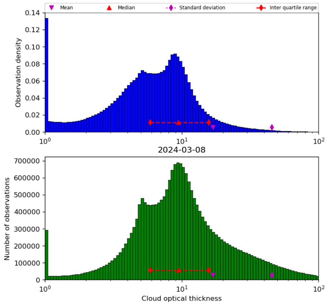
Figure 41: Histogram of “Cloud optical thickness” for 2024-03-07 to 2024-03-09
