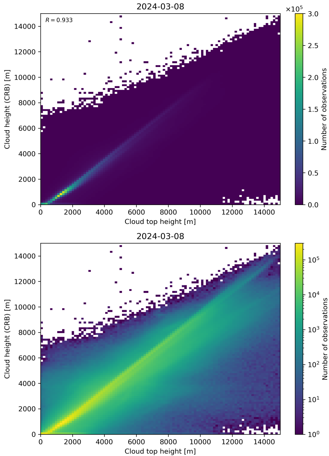
Figure 89: Scatter density plot of “Cloud top height” against “Cloud height (CRB)” for 2024-03-07 to 2024-03-09.
