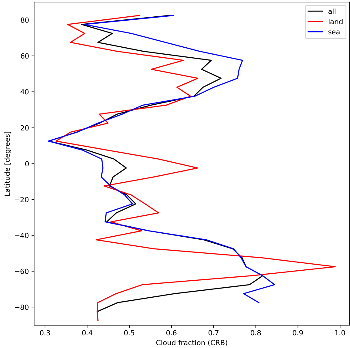
Figure 26: Zonal average of “Cloud fraction (CRB)” for 2024-03-07 to 2024-03-09.
