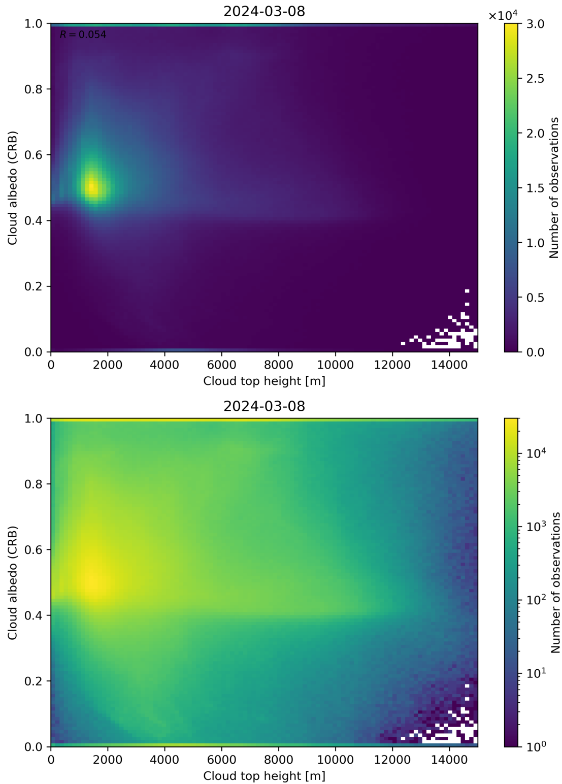
Figure 86: Scatter density plot of “Cloud top height” against “Cloud albedo (CRB)” for 2024-03-07 to 2024-03-09.
