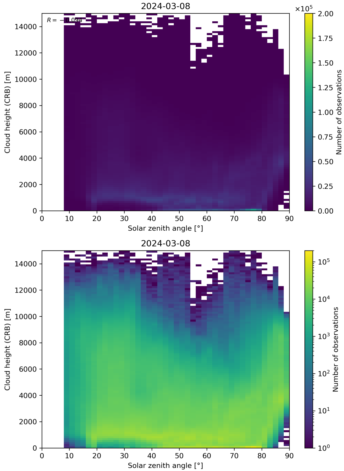
Figure 102: Scatter density plot of “Solar zenith angle” against “Cloud height (CRB)” for 2024-03-07 to 2024-03-09.
