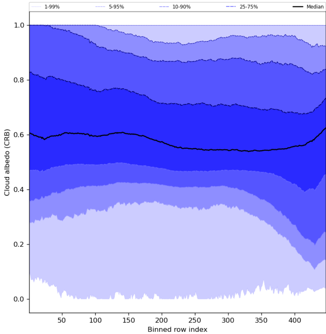
Figure 60: Along track statistics of “Cloud albedo (CRB)” for 2024-03-07 to 2024-03-09
