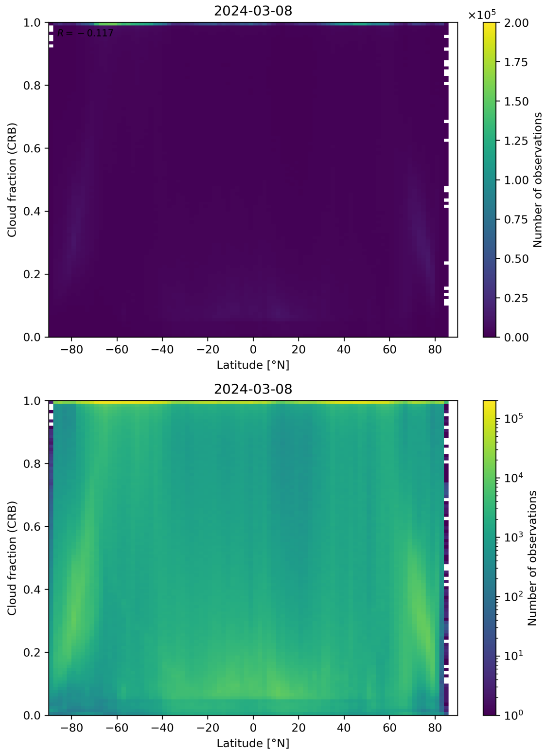
Figure 94: Scatter density plot of “Latitude” against “Cloud fraction (CRB)” for 2024-03-07 to 2024-03-09.
