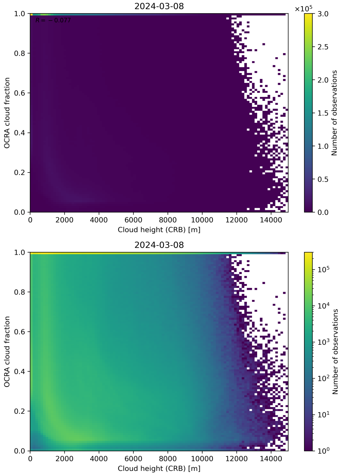
Figure 81: Scatter density plot of “Cloud height (CRB)” against “OCRA cloud fraction” for 2024-03-07 to 2024-03-09.
