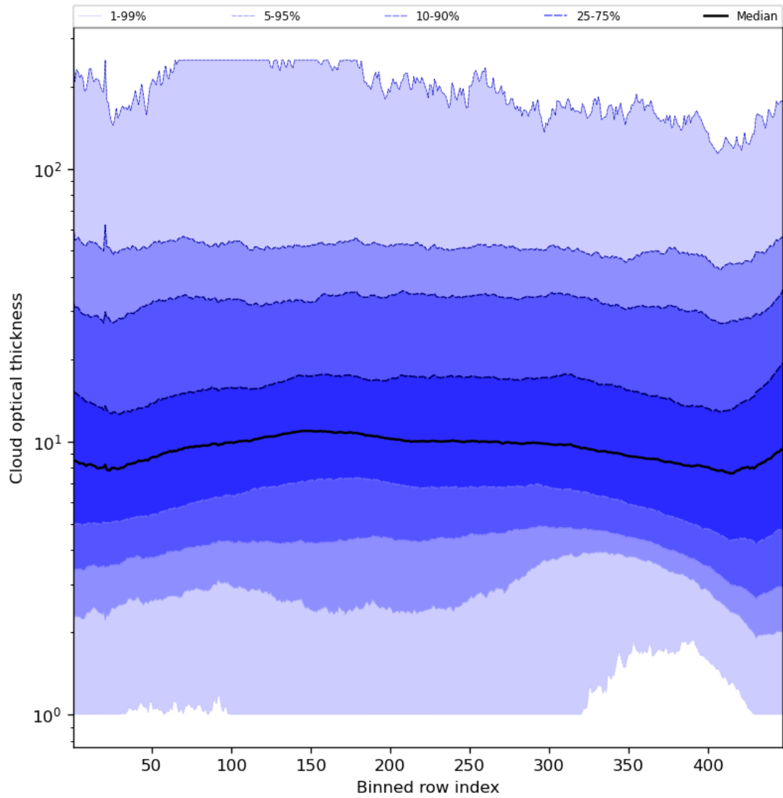
Figure 57: Along track statistics of “Cloud optical thickness” for 2024-03-07 to 2024-03-09
