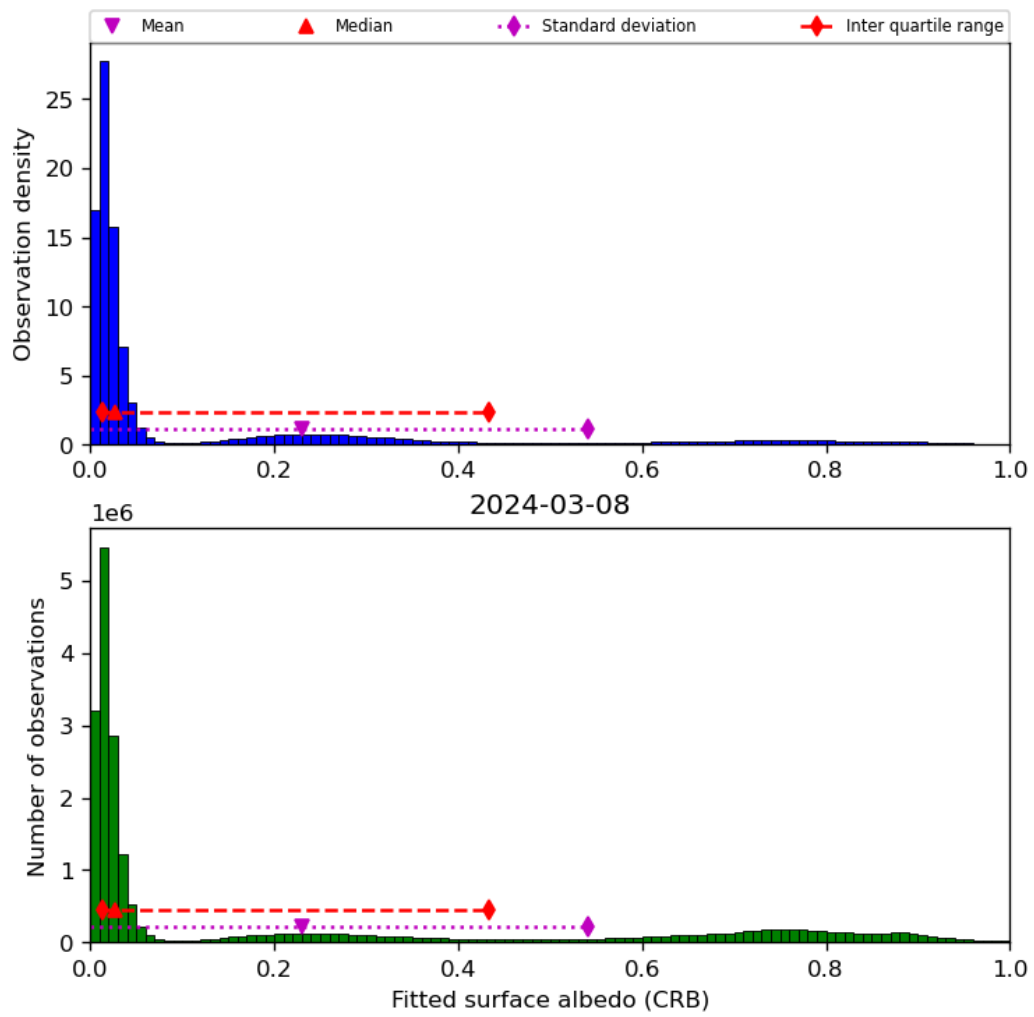
Figure 46: Histogram of “Fitted surface albedo (CRB)” for 2024-03-07 to 2024-03-09
