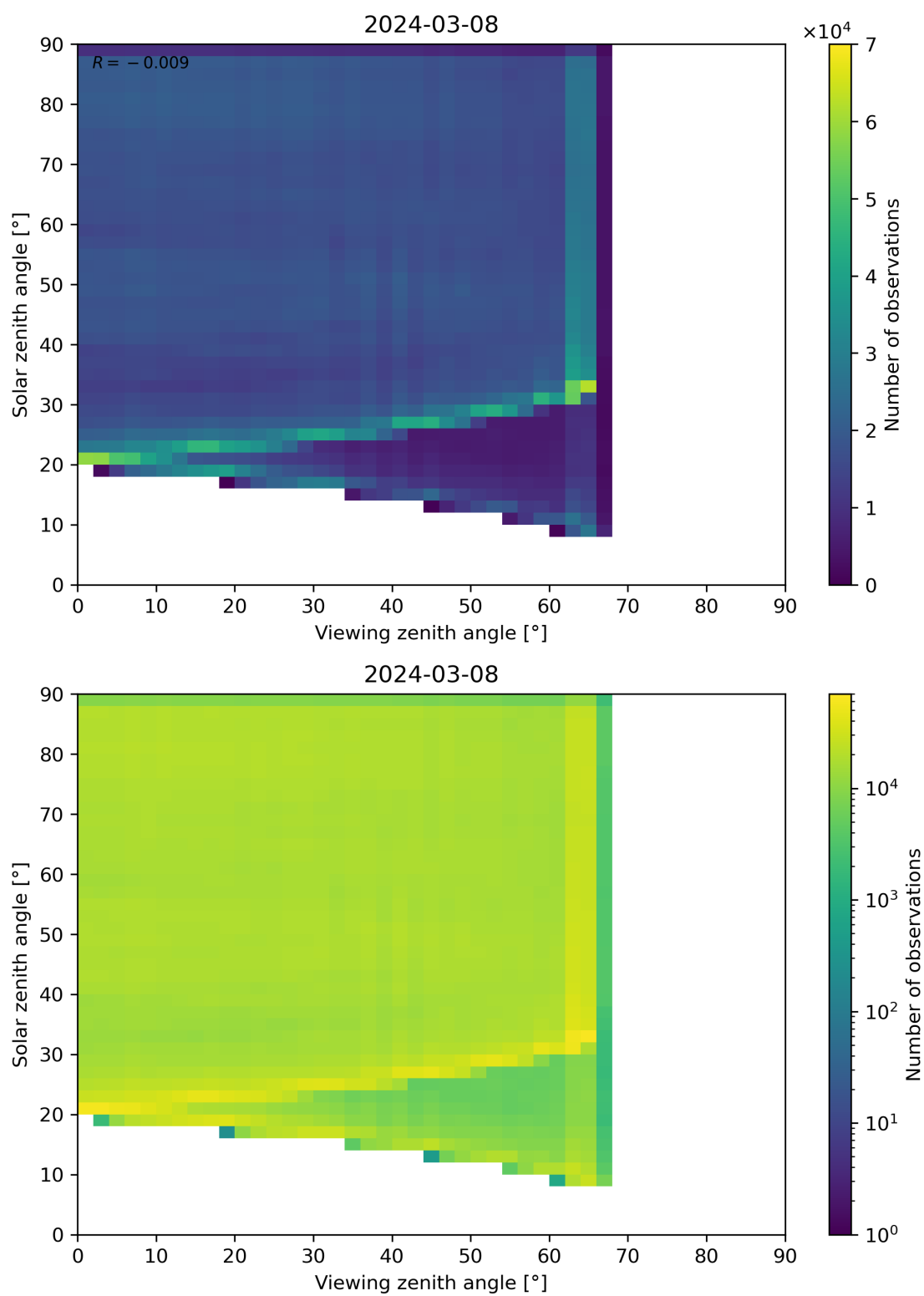
Figure 114: Scatter density plot of “Viewing zenith angle” against “Solar zenith angle” for 2024-03-07 to 2024-03-09.
