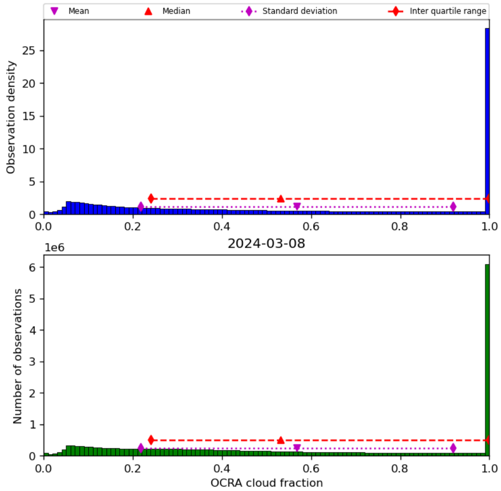
Figure 50: Histogram of “OCRA cloud fraction” for 2024-03-07 to 2024-03-09
