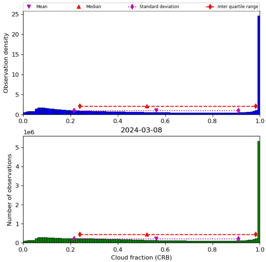
Figure 42: Histogram of “Cloud fraction (CRB)” for 2024-03-07 to 2024-03-09
