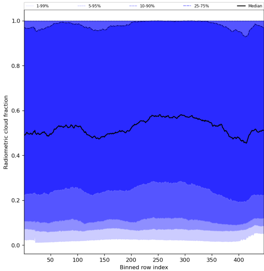
Figure 55: Along track statistics of “Radiometric cloud fraction” for 2024-03-07 to 2024-03-09
