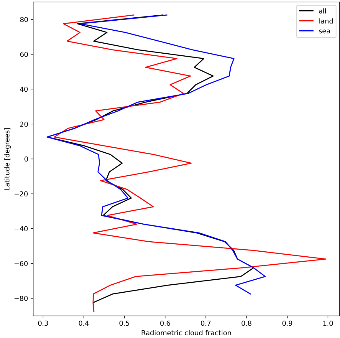
Figure 23: Zonal average of “Radiometric cloud fraction” for 2024-03-07 to 2024-03-09.
