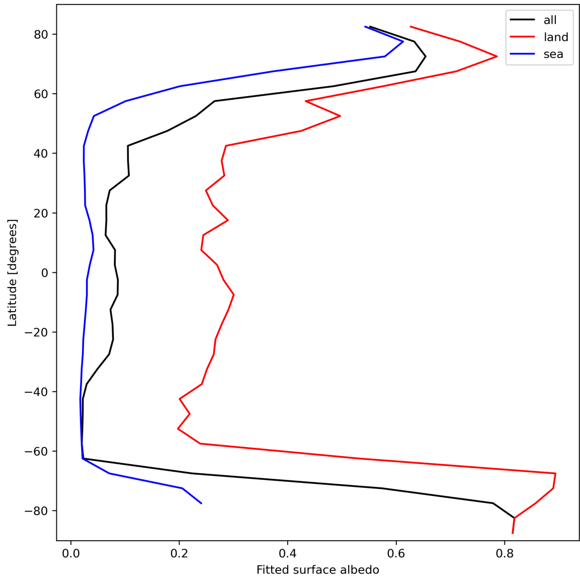
Figure 29: Zonal average of “Fitted surface albedo” for 2024-03-07 to 2024-03-09.
