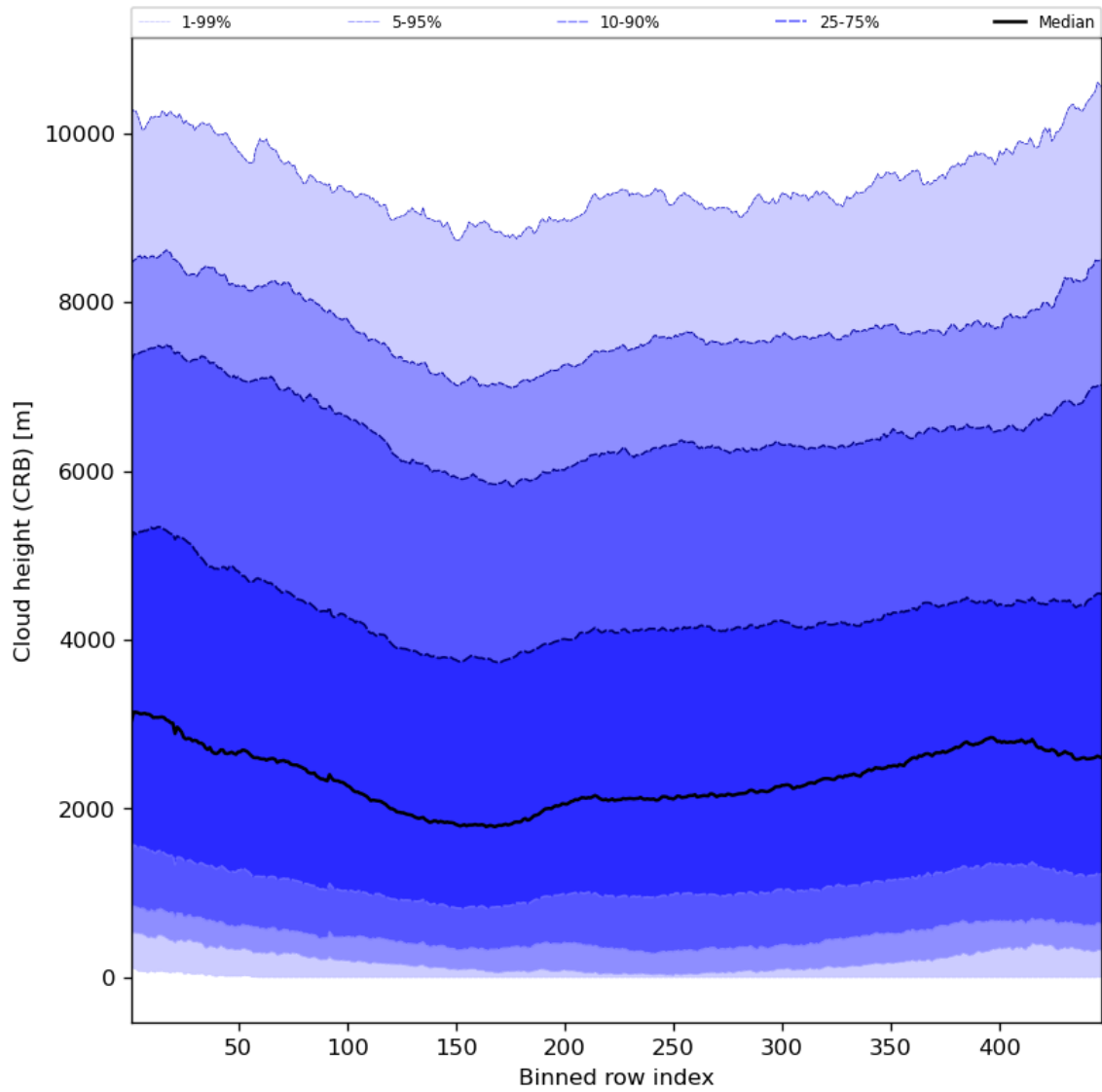
Figure 59: Along track statistics of “Cloud height (CRB)” for 2024-03-07 to 2024-03-09
