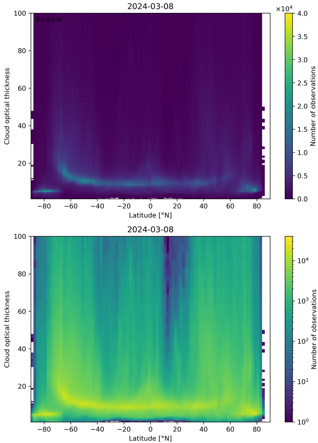
Figure 96: Scatter density plot of “Latitude” against “Cloud optical thickness” for 2024-03-07 to 2024-03-09.
