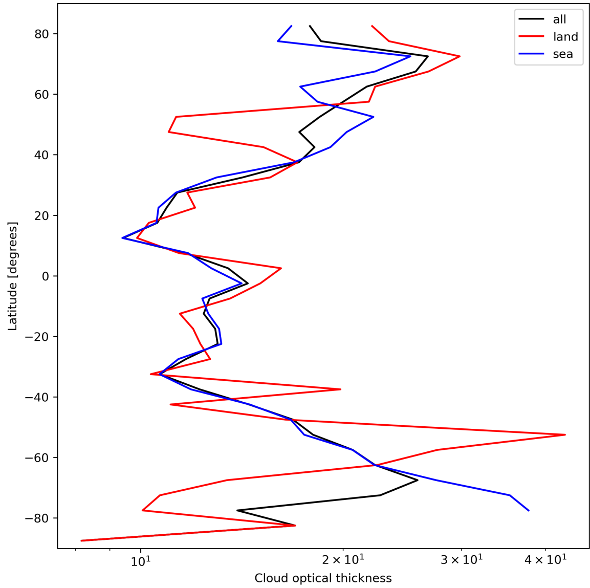
Figure 25: Zonal average of “Cloud optical thickness” for 2024-03-07 to 2024-03-09.
