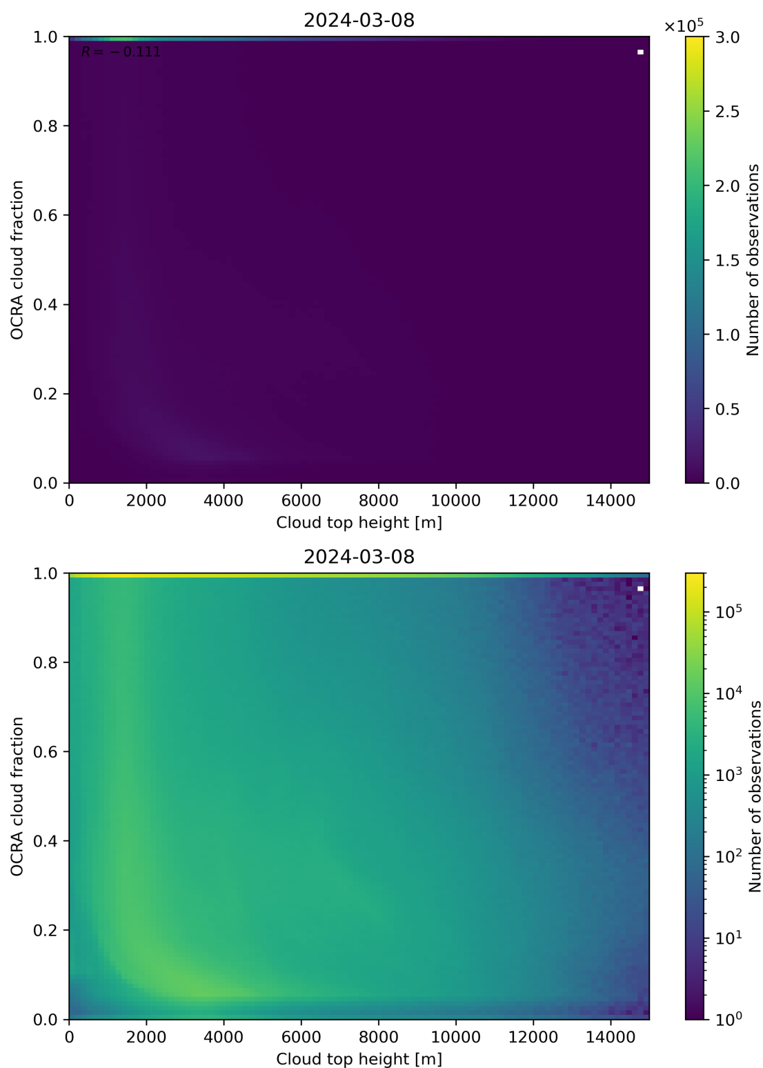
Figure 87: Scatter density plot of “Cloud top height” against “OCRA cloud fraction” for 2024-03-07 to 2024-03-09.
