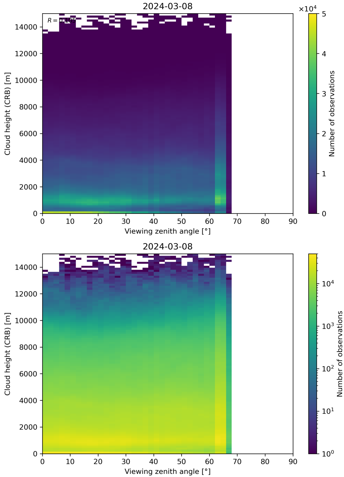
Figure 110: Scatter density plot of “Viewing zenith angle” against “Cloud height (CRB)” for 2024-03-07 to 2024-03-09.
