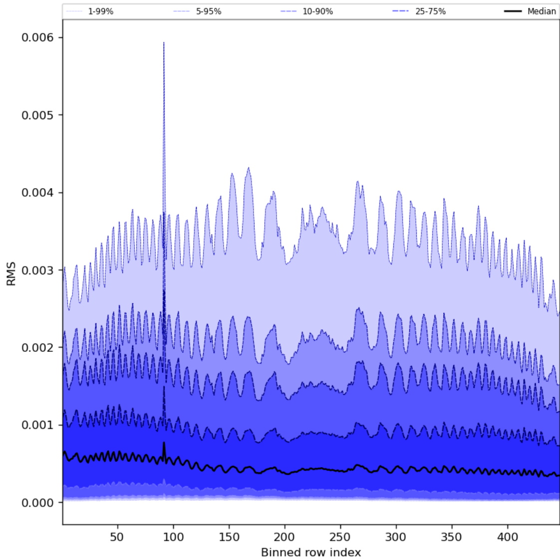
Figure 63: Along track statistics of “RMS” for 2024-03-10 to 2024-03-12
