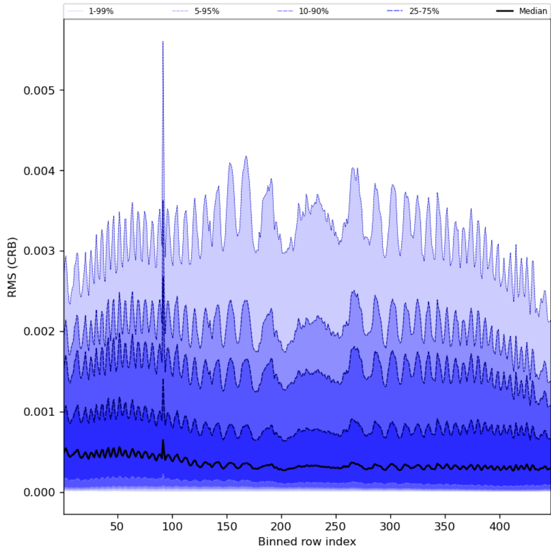
Figure 64: Along track statistics of “RMS (CRB)” for 2024-03-10 to 2024-03-12
