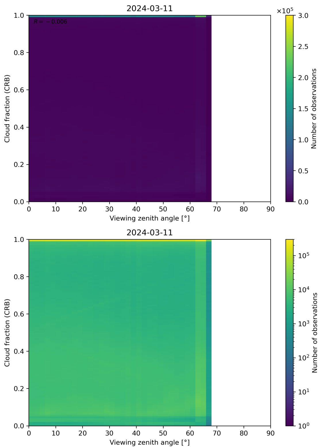
Figure 109: Scatter density plot of “Viewing zenith angle” against “Cloud fraction (CRB)” for 2024-03-10 to 2024-03-12.
