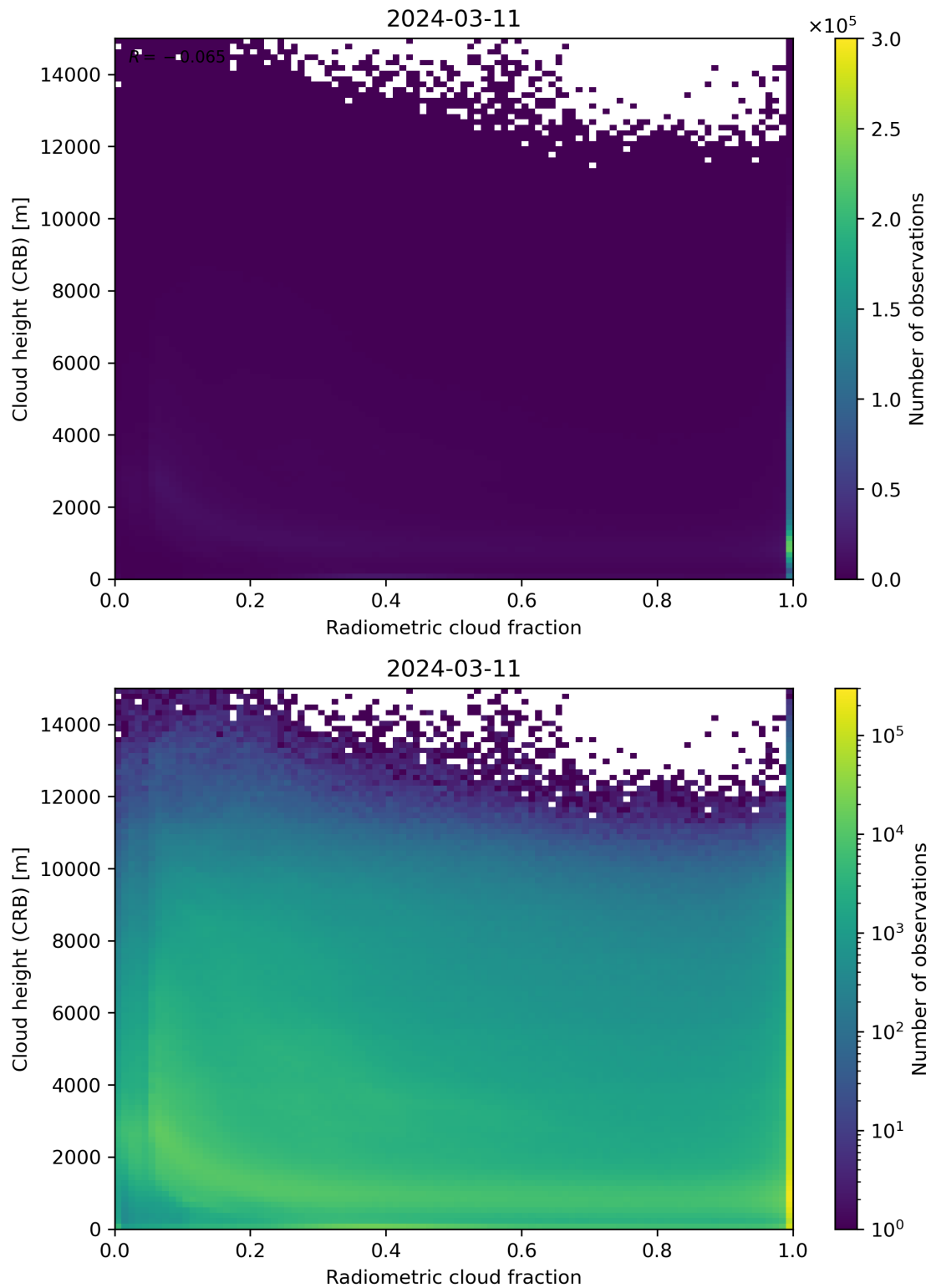
Figure 74: Scatter density plot of “Radiometric cloud fraction” against “Cloud height (CRB)” for 2024-03-10 to 2024-03-12.
