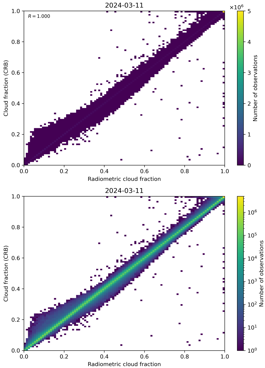
Figure 73: Scatter density plot of “Radiometric cloud fraction” against “Cloud fraction (CRB)” for 2024-03-10 to 2024-03-12.
