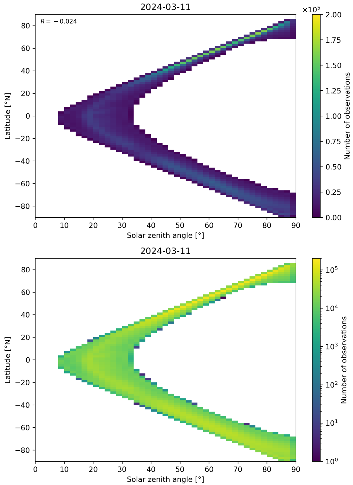
Figure 105: Scatter density plot of “Solar zenith angle” against “Latitude” for 2024-03-10 to 2024-03-12.
