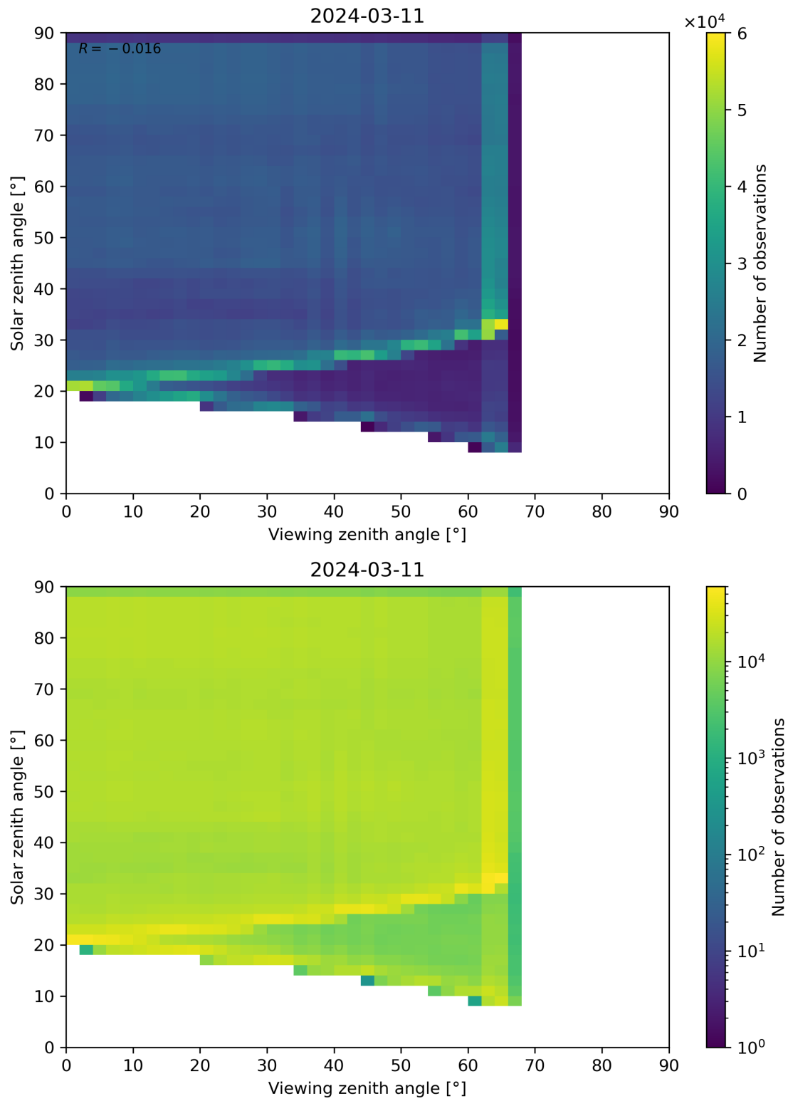
Figure 114: Scatter density plot of “Viewing zenith angle” against “Solar zenith angle” for 2024-03-10 to 2024-03-12.
