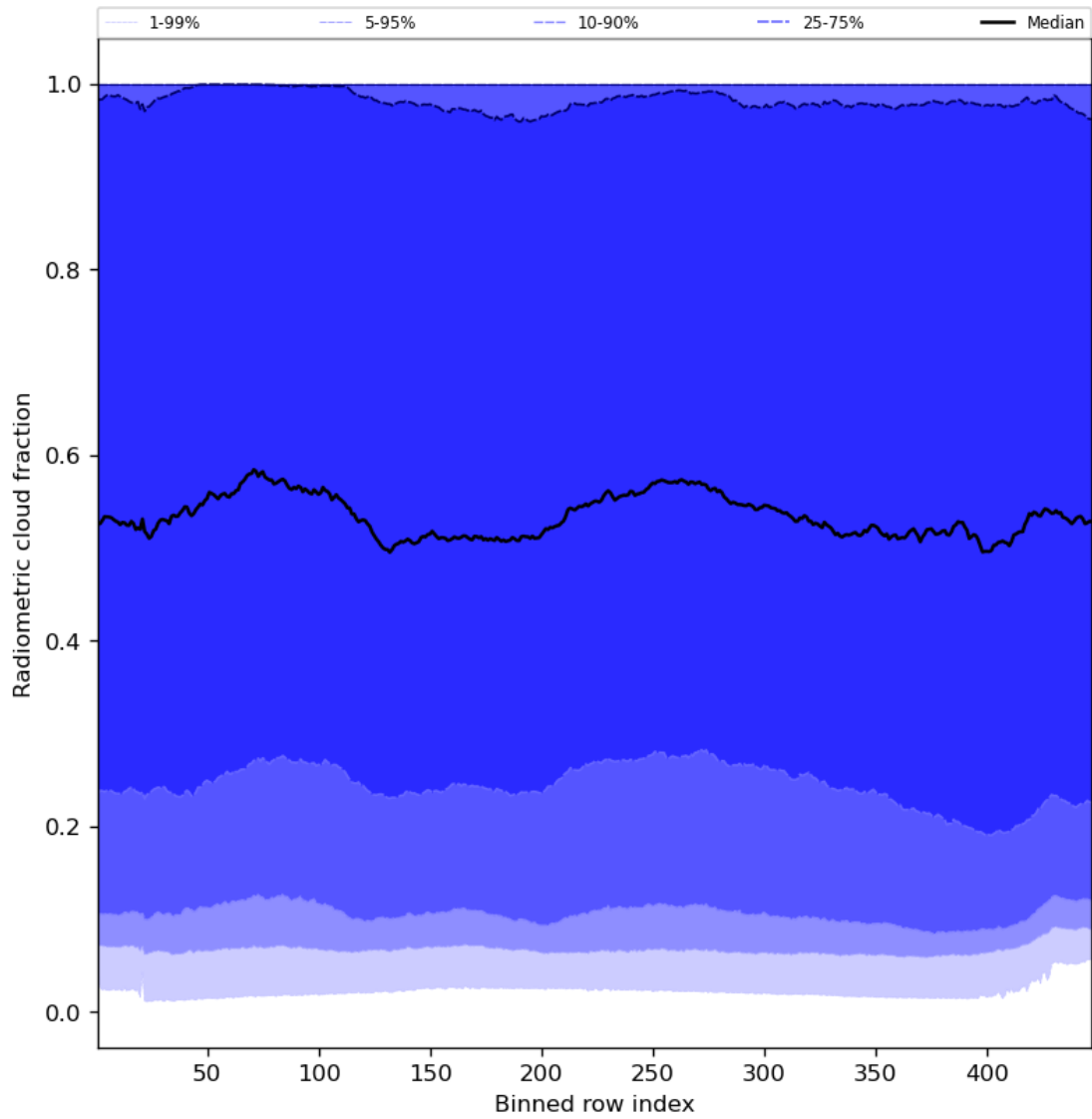
Figure 55: Along track statistics of “Radiometric cloud fraction” for 2024-03-10 to 2024-03-12
