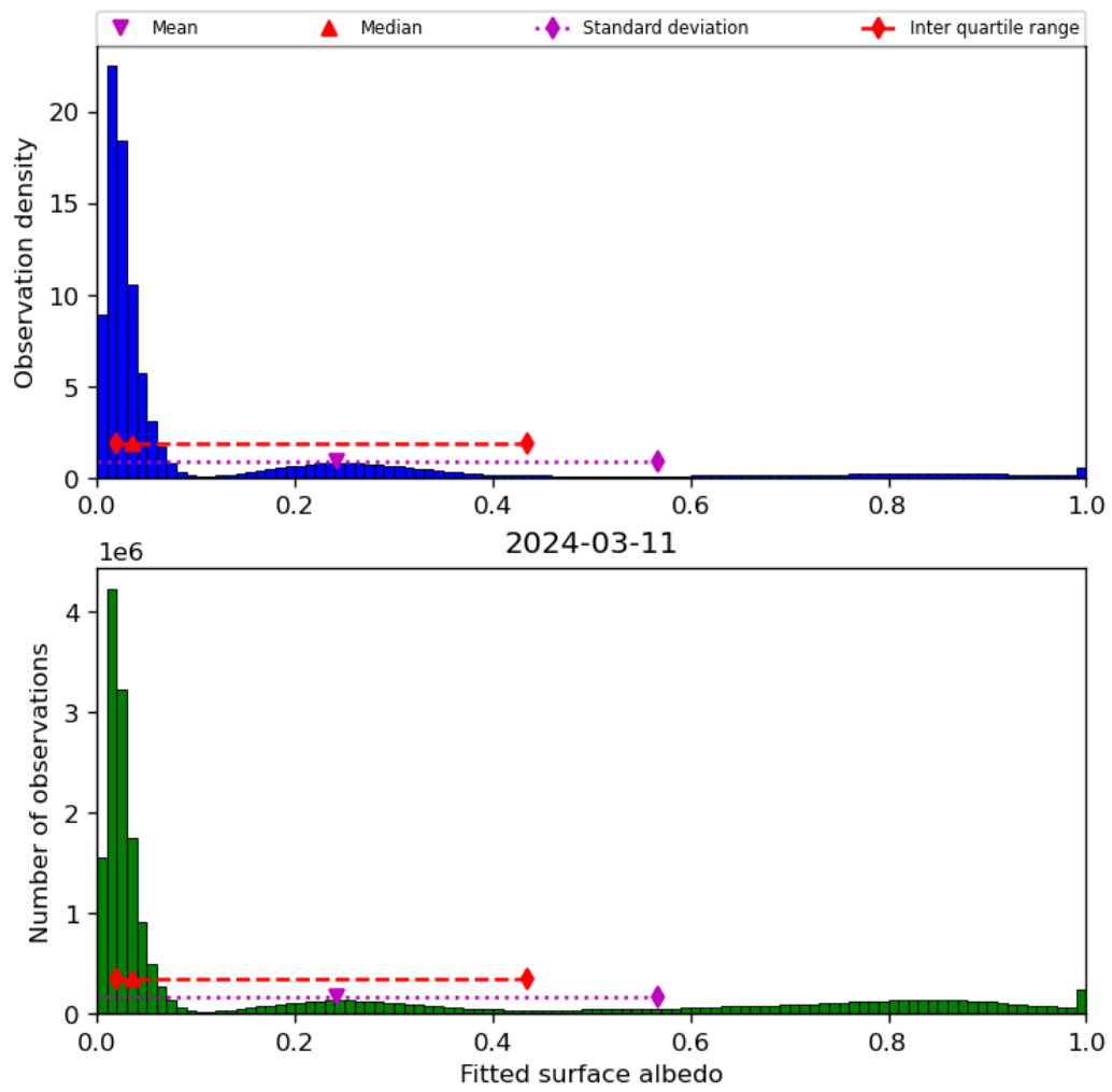
Figure 45: Histogram of “Fitted surface albedo” for 2024-03-10 to 2024-03-12
