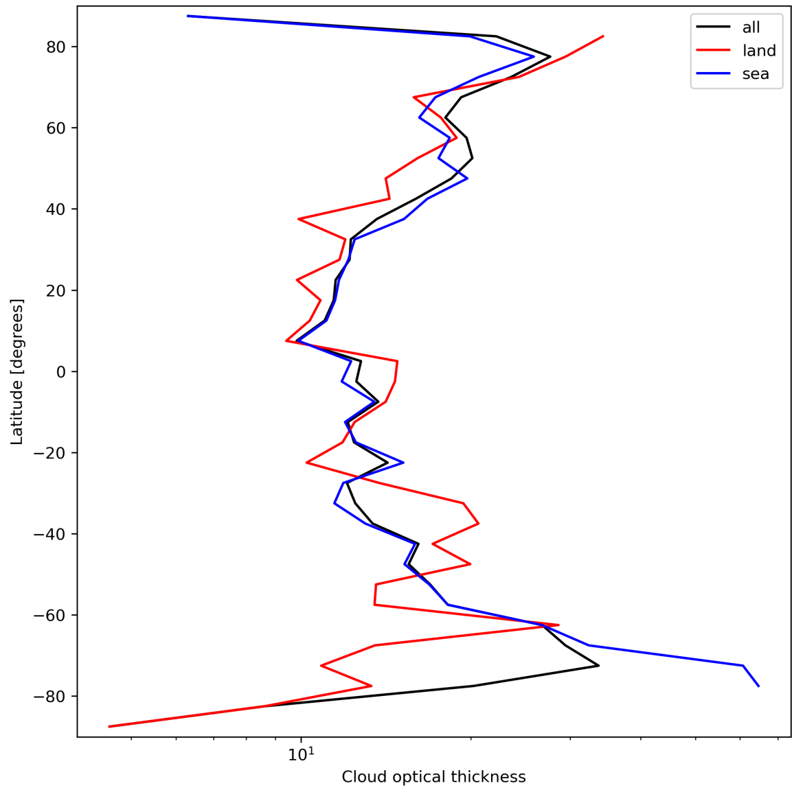
Figure 25: Zonal average of “Cloud optical thickness” for 2024-03-10 to 2024-03-12.
