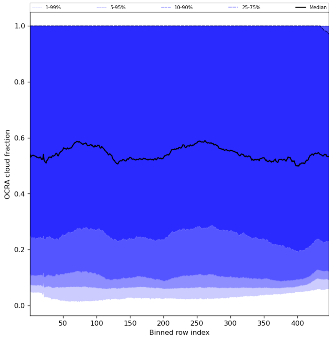
Figure 66: Along track statistics of “OCRA cloud fraction” for 2024-03-10 to 2024-03-12
