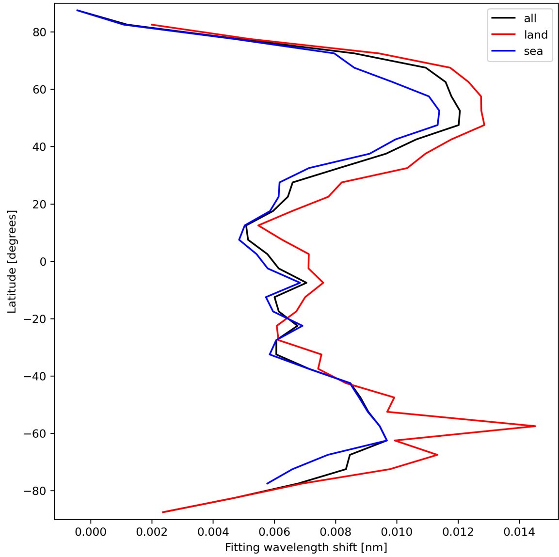
Figure 33: Zonal average of “Fitting wavelength shift” for 2024-03-10 to 2024-03-12.
