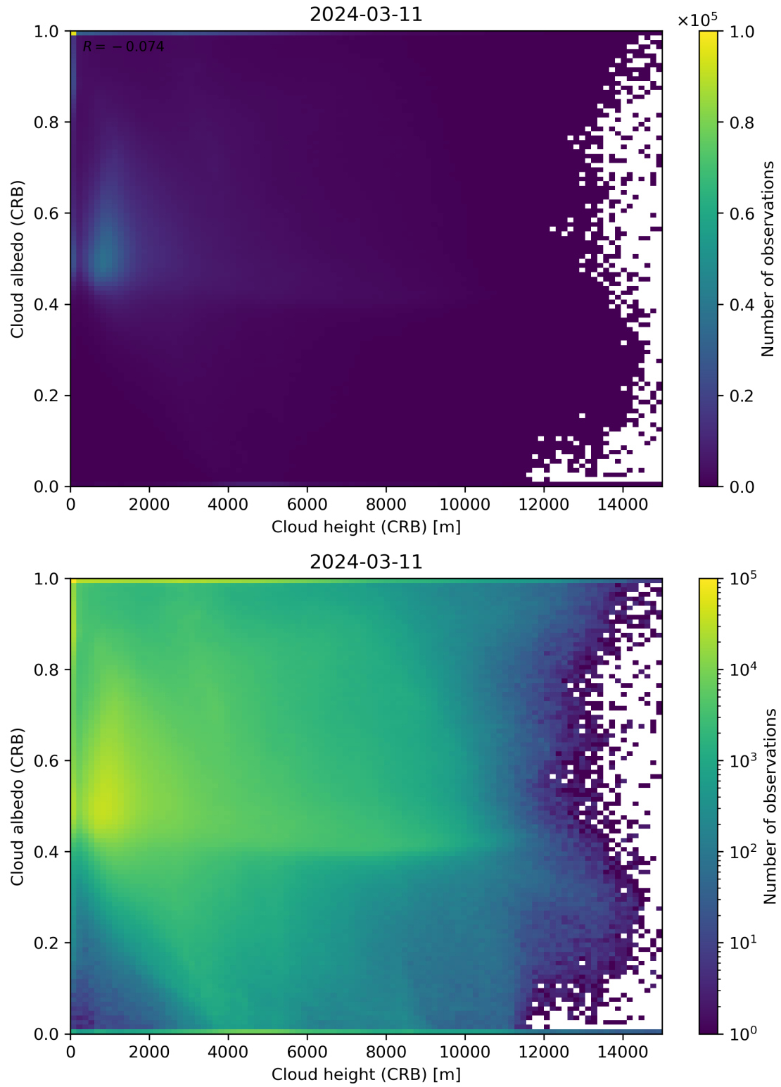
Figure 80: Scatter density plot of “Cloud height (CRB)” against “Cloud albedo (CRB)” for 2024-03-10 to 2024-03-12.
