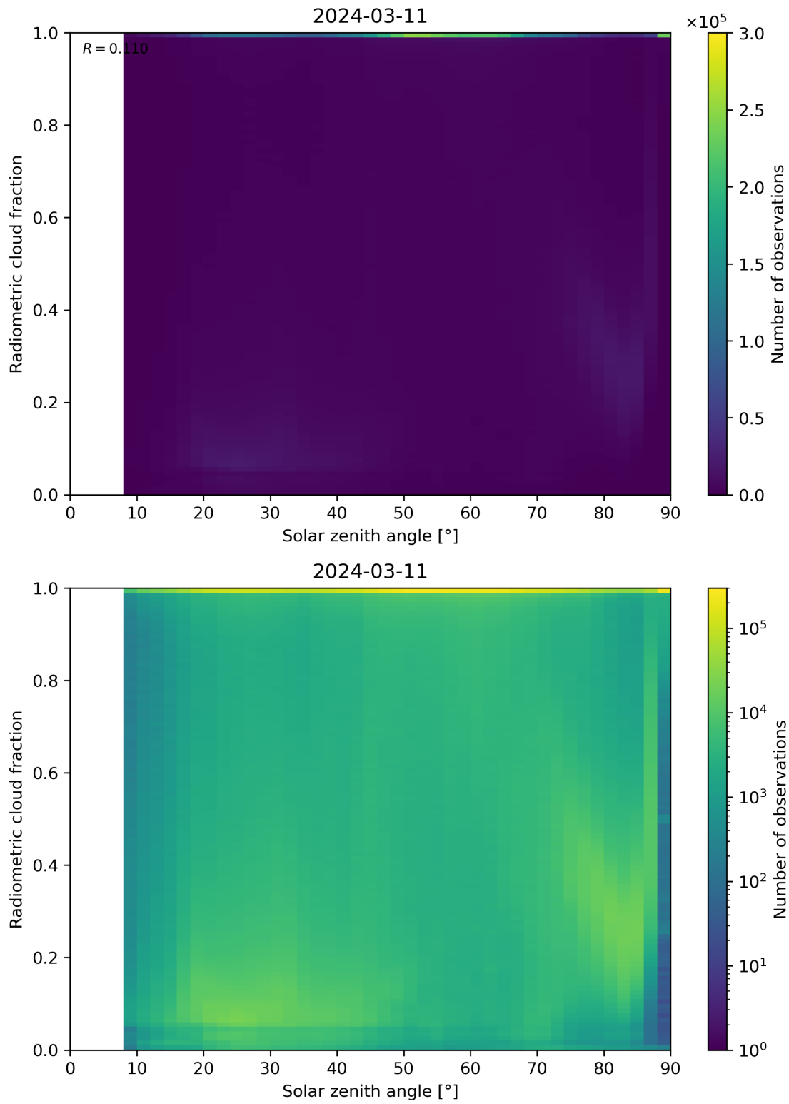
Figure 99: Scatter density plot of “Solar zenith angle” against “Radiometric cloud fraction” for 2024-03-10 to 2024-03-12.
