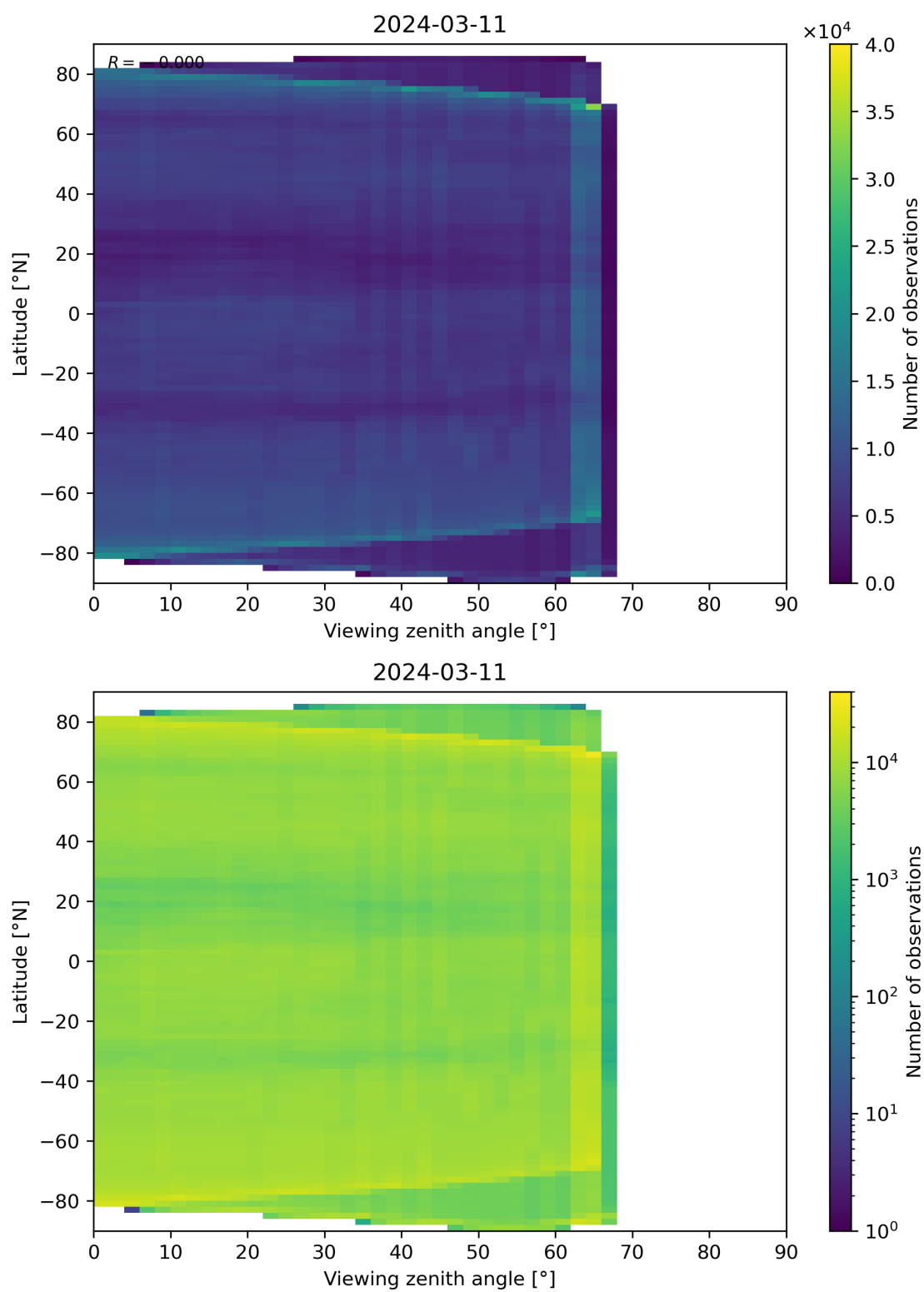
Figure 113: Scatter density plot of “Viewing zenith angle” against “Latitude” for 2024-03-10 to 2024-03-12.
