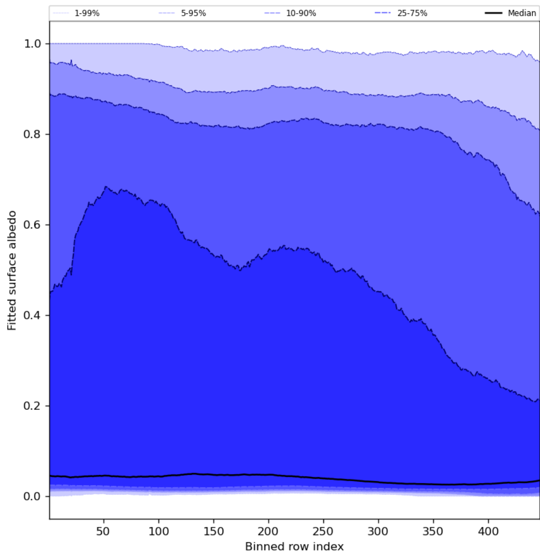
Figure 61: Along track statistics of “Fitted surface albedo” for 2024-03-10 to 2024-03-12
