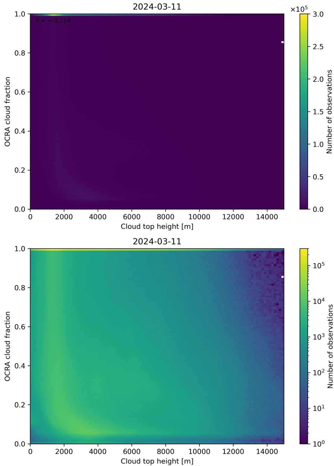
Figure 87: Scatter density plot of “Cloud top height” against “OCRA cloud fraction” for 2024-03-10 to 2024-03-12.
