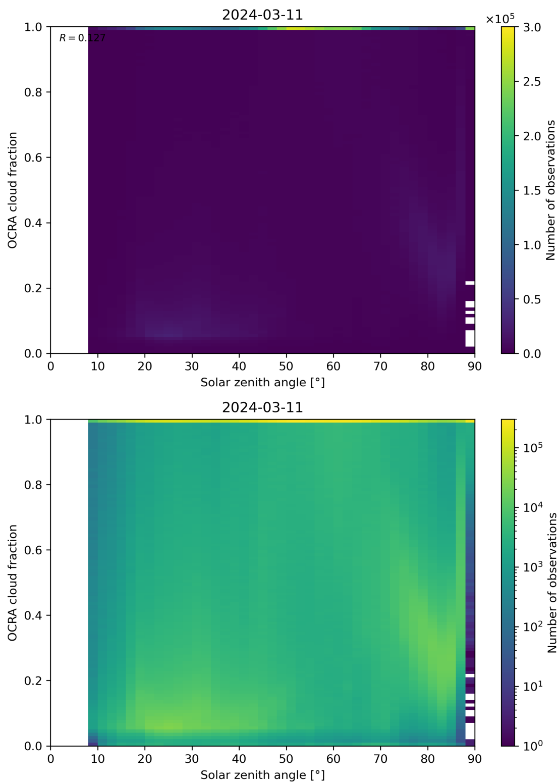
Figure 100: Scatter density plot of “Solar zenith angle” against “OCRA cloud fraction” for 2024-03-10 to 2024-03-12.
