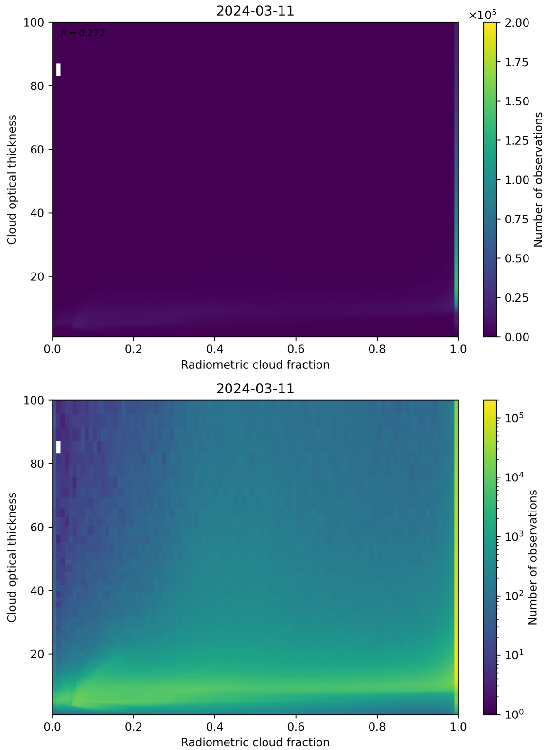
Figure 75: Scatter density plot of “Radiometric cloud fraction” against “Cloud optical thickness” for 2024-03-10 to 2024-03-12.
