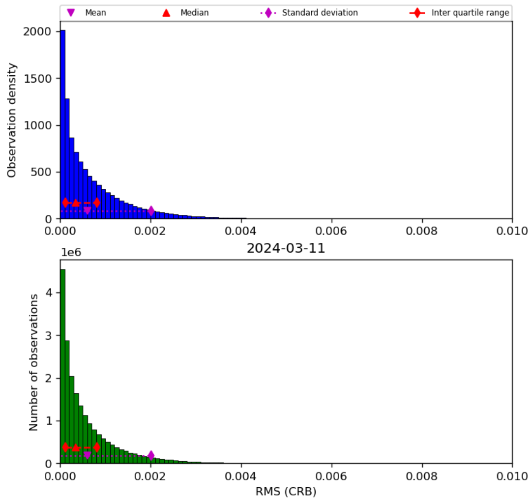
Figure 48: Histogram of “RMS (CRB)” for 2024-03-10 to 2024-03-12
