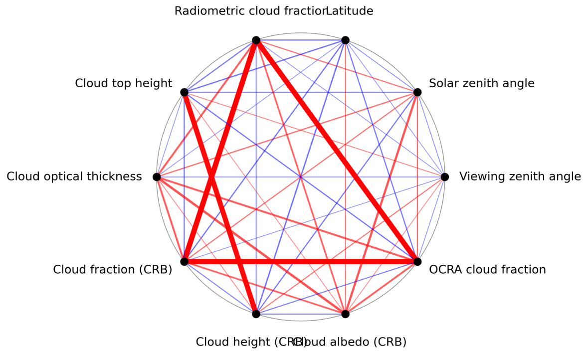
Figure 1: Map of correlation graph for 2024-03-10 to 2024-03-12.
