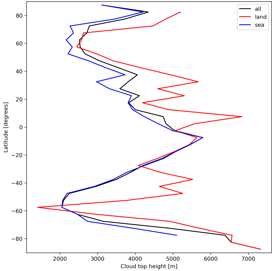
Figure 24: Zonal average of “Cloud top height” for 2024-03-10 to 2024-03-12.
