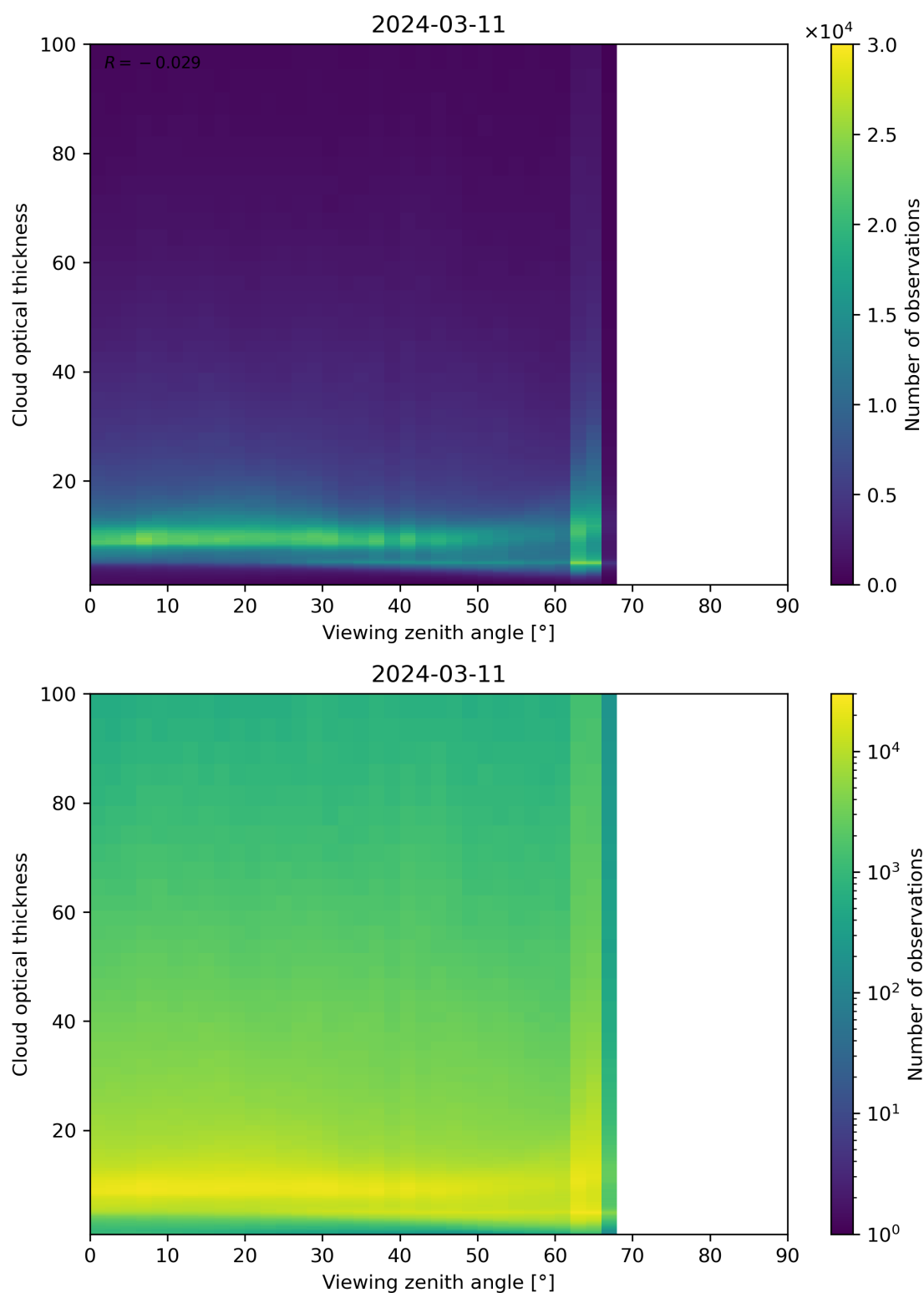
Figure 111: Scatter density plot of “Viewing zenith angle” against “Cloud optical thickness” for 2024-03-10 to 2024-03-12.
