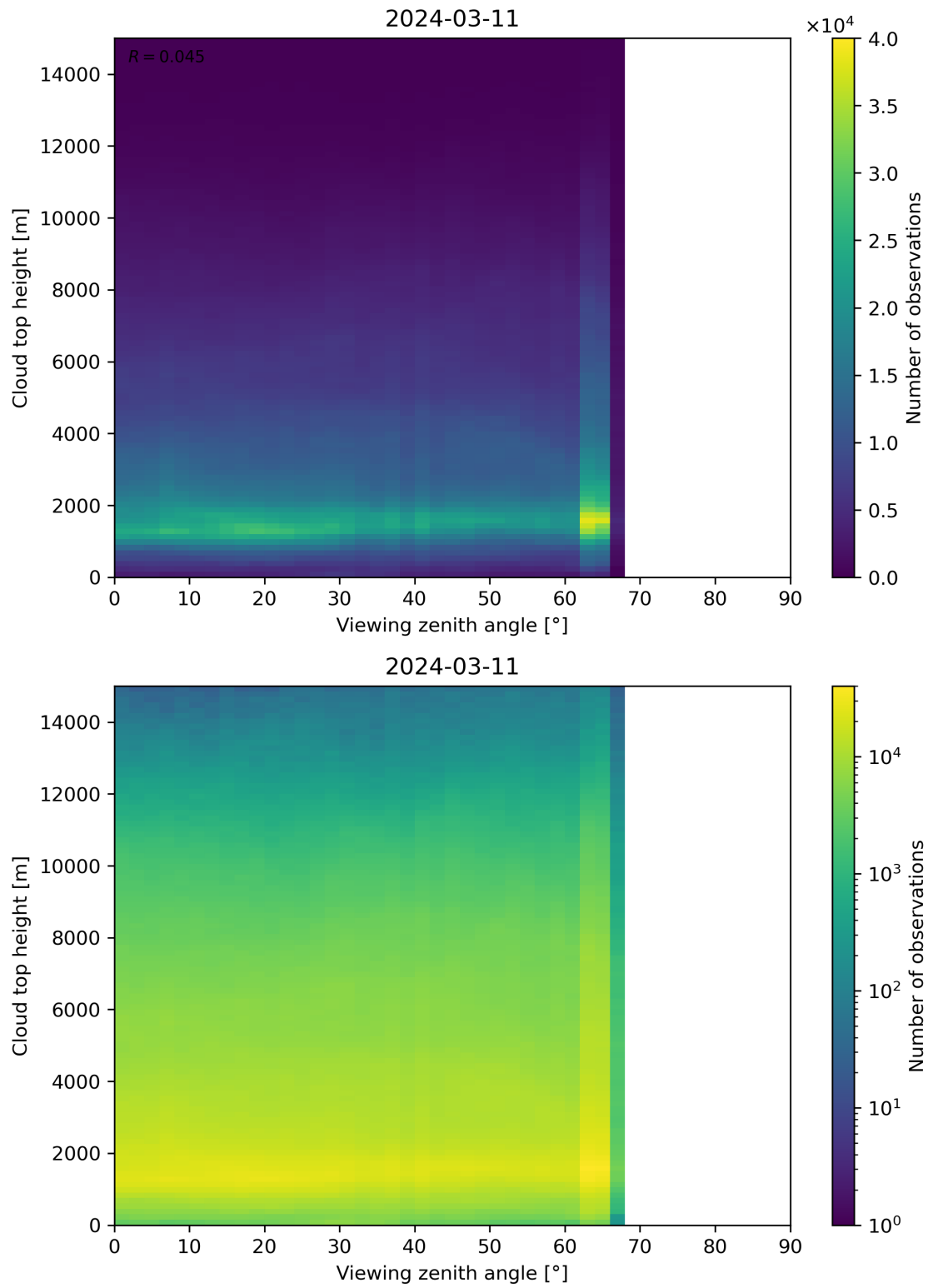
Figure 112: Scatter density plot of “Viewing zenith angle” against “Cloud top height” for 2024-03-10 to 2024-03-12.
