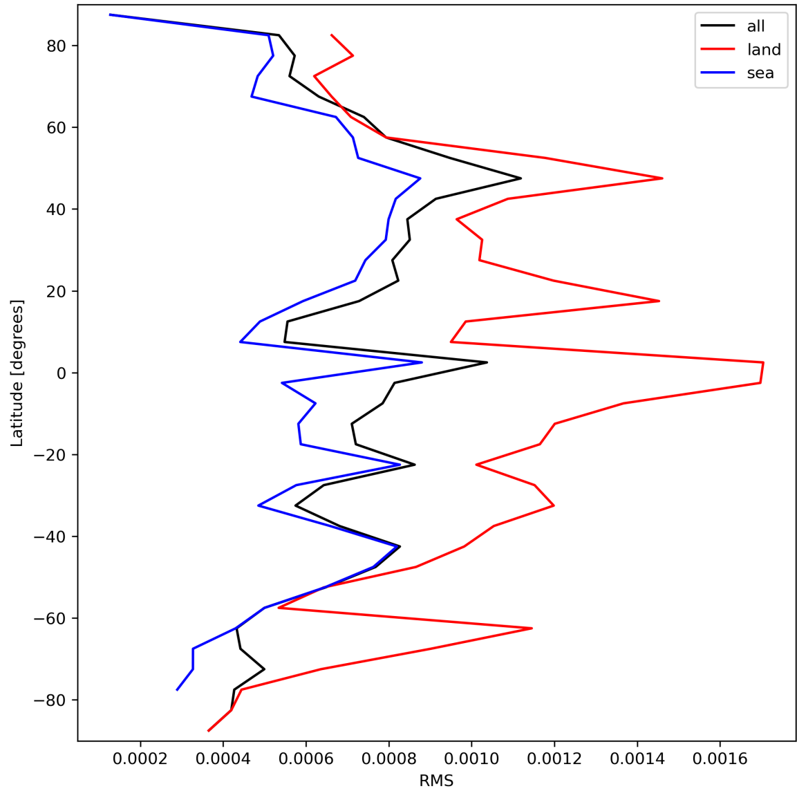
Figure 31: Zonal average of “RMS” for 2024-03-10 to 2024-03-12.
