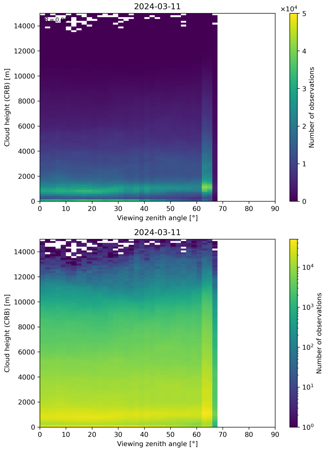
Figure 110: Scatter density plot of “Viewing zenith angle” against “Cloud height (CRB)” for 2024-03-10 to 2024-03-12.
