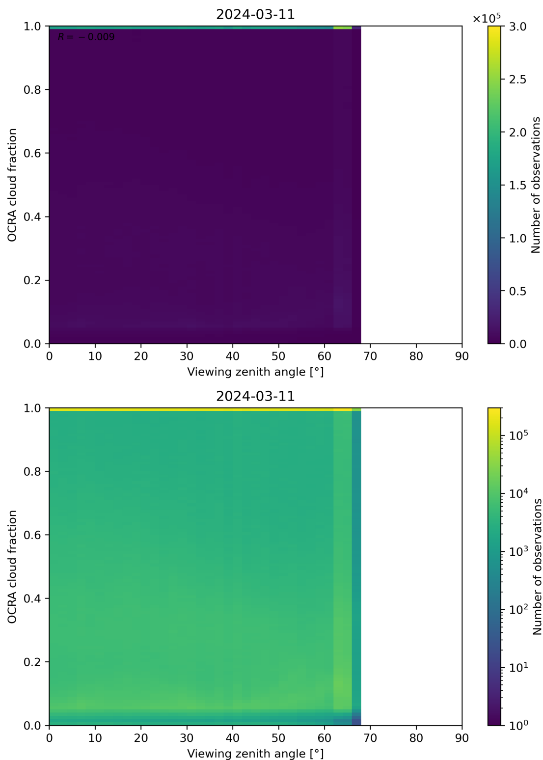
Figure 108: Scatter density plot of “Viewing zenith angle” against “OCRA cloud fraction” for 2024-03-10 to 2024-03-12.
