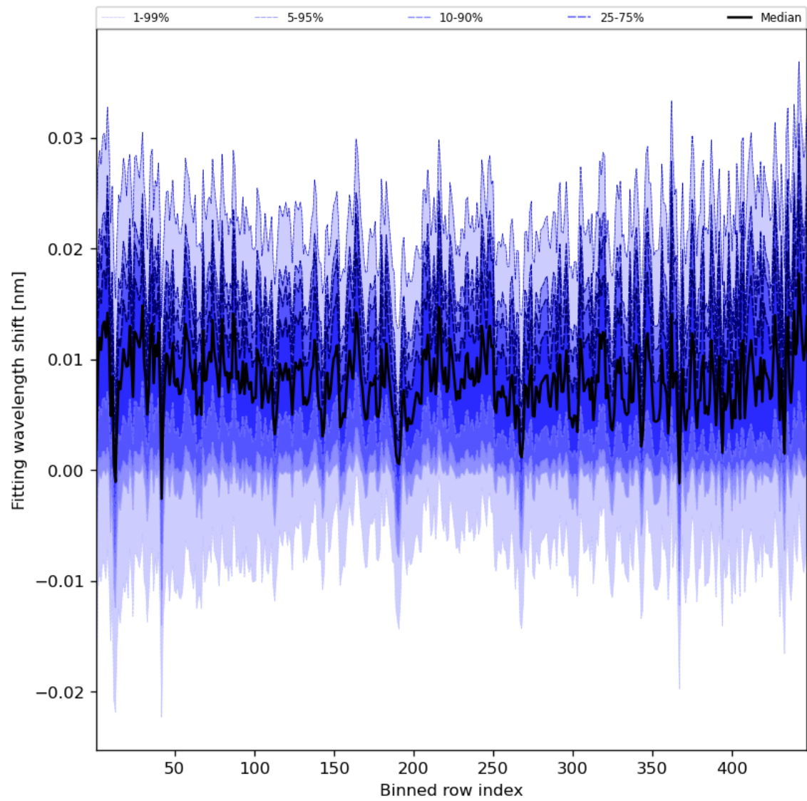
Figure 65: Along track statistics of “Fitting wavelength shift” for 2024-03-10 to 2024-03-12
