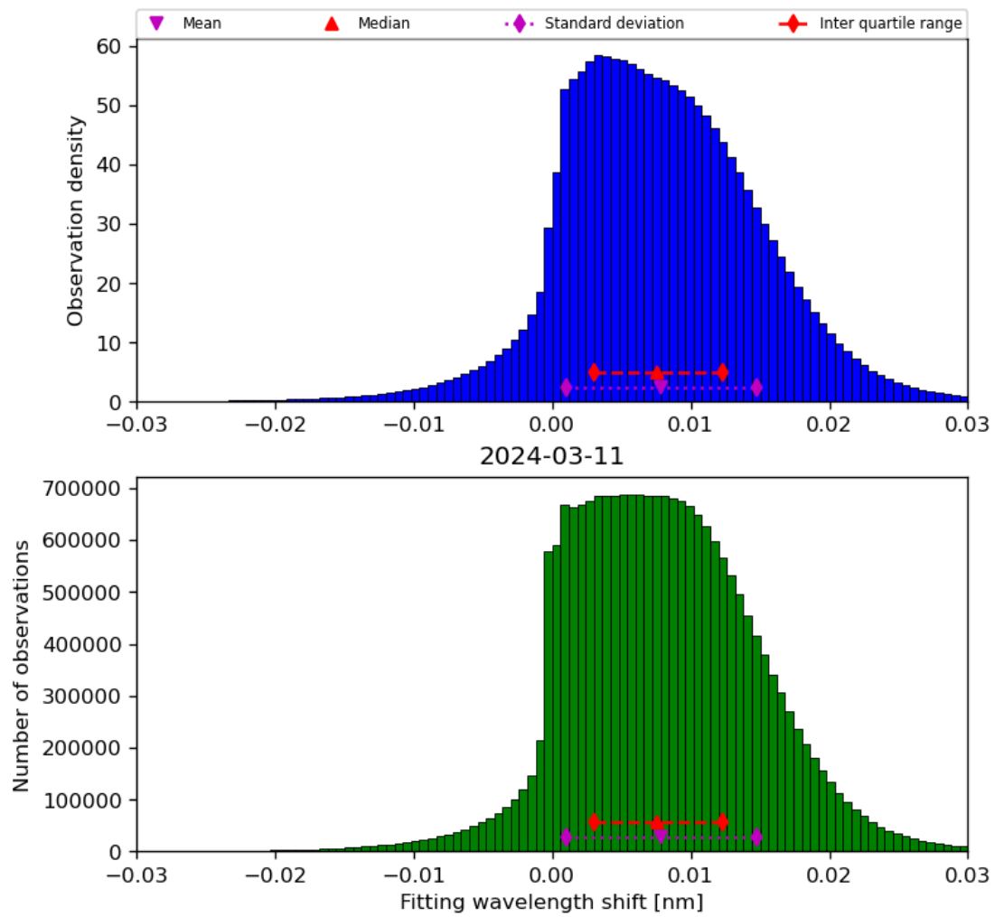
Figure 49: Histogram of “Fitting wavelength shift” for 2024-03-10 to 2024-03-12
