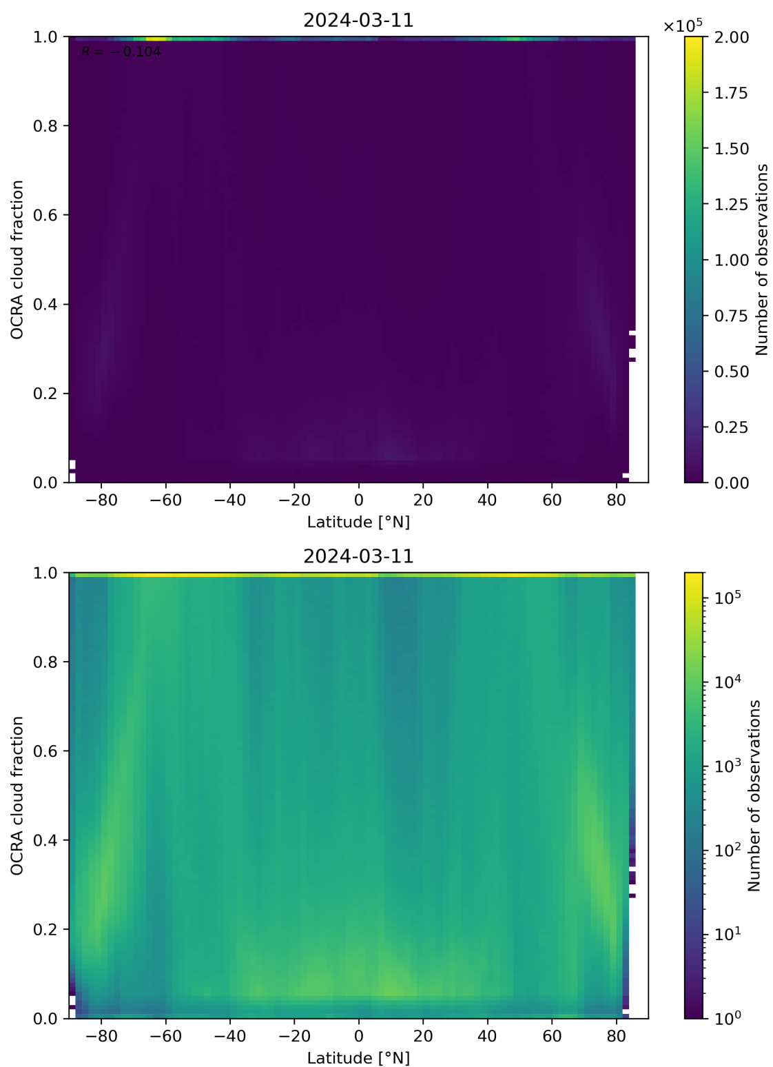
Figure 93: Scatter density plot of “Latitude” against “OCRA cloud fraction” for 2024-03-10 to 2024-03-12.
