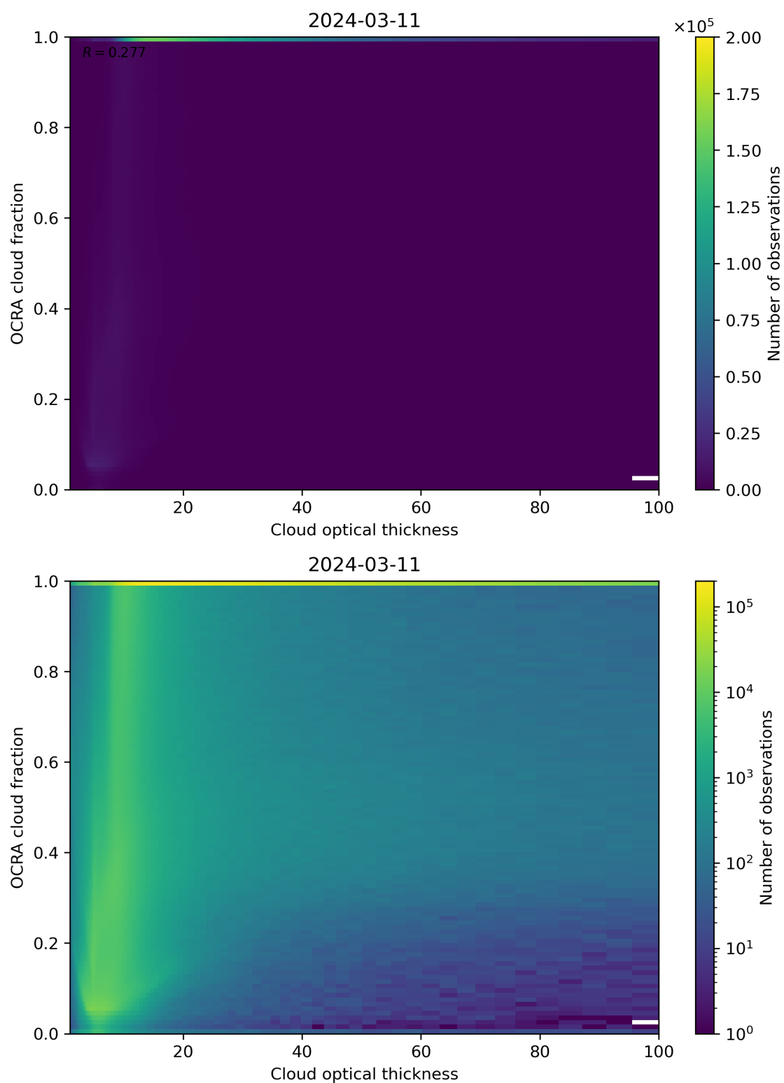
Figure 83: Scatter density plot of “Cloud optical thickness” against “OCRA cloud fraction” for 2024-03-10 to 2024-03-12.
