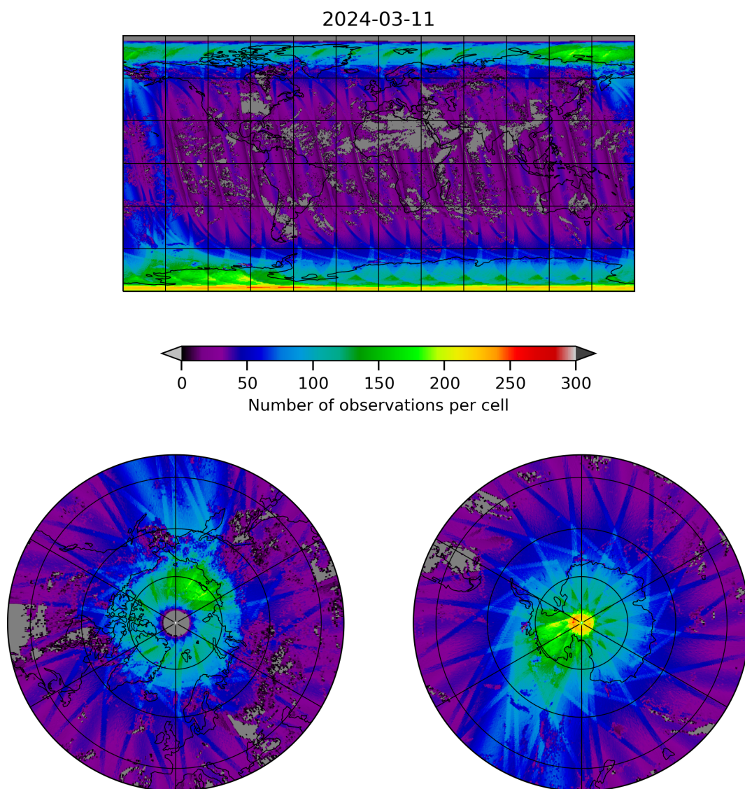
Figure 21: Map of the number of observations for 2024-03-10 to 2024-03-12
