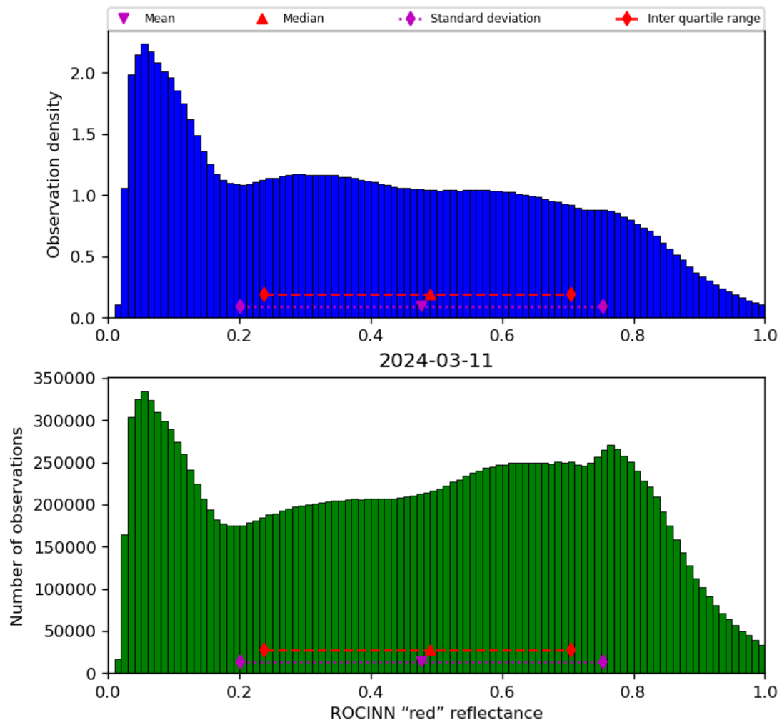
Figure 53: Histogram of “ROCINN “red” reflectance” for 2024-03-10 to 2024-03-12
