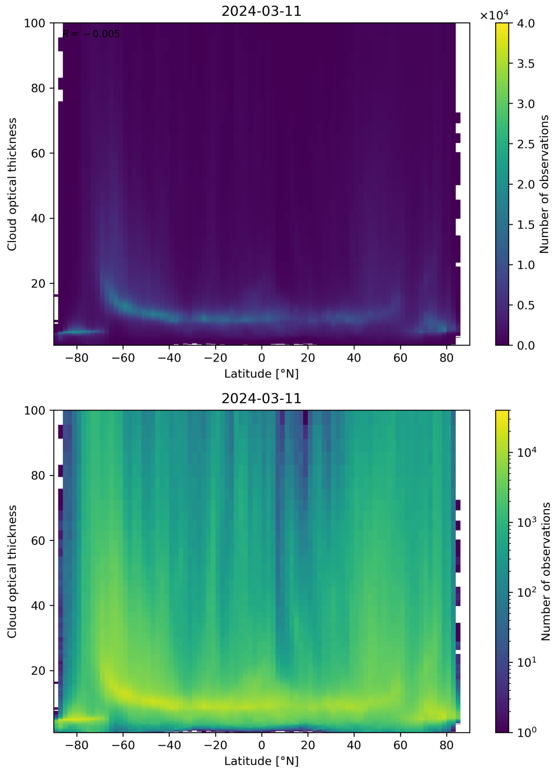
Figure 96: Scatter density plot of “Latitude” against “Cloud optical thickness” for 2024-03-10 to 2024-03-12.
