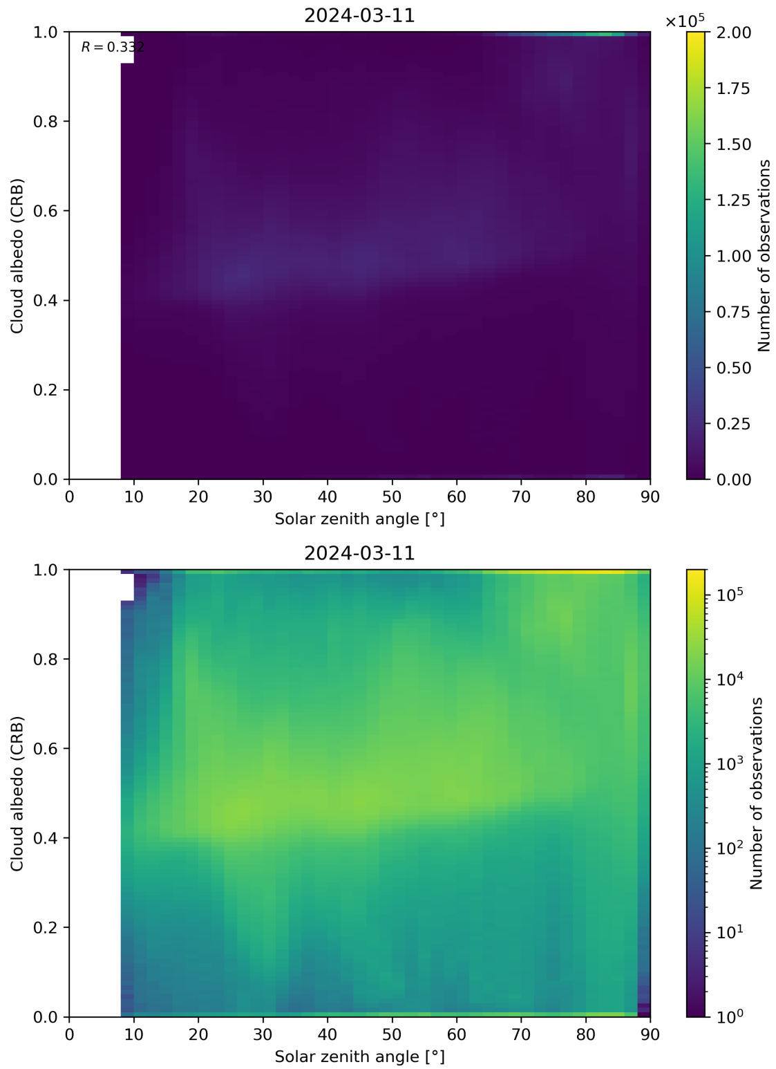
Figure 98: Scatter density plot of “Solar zenith angle” against “Cloud albedo (CRB)” for 2024-03-10 to 2024-03-12.
