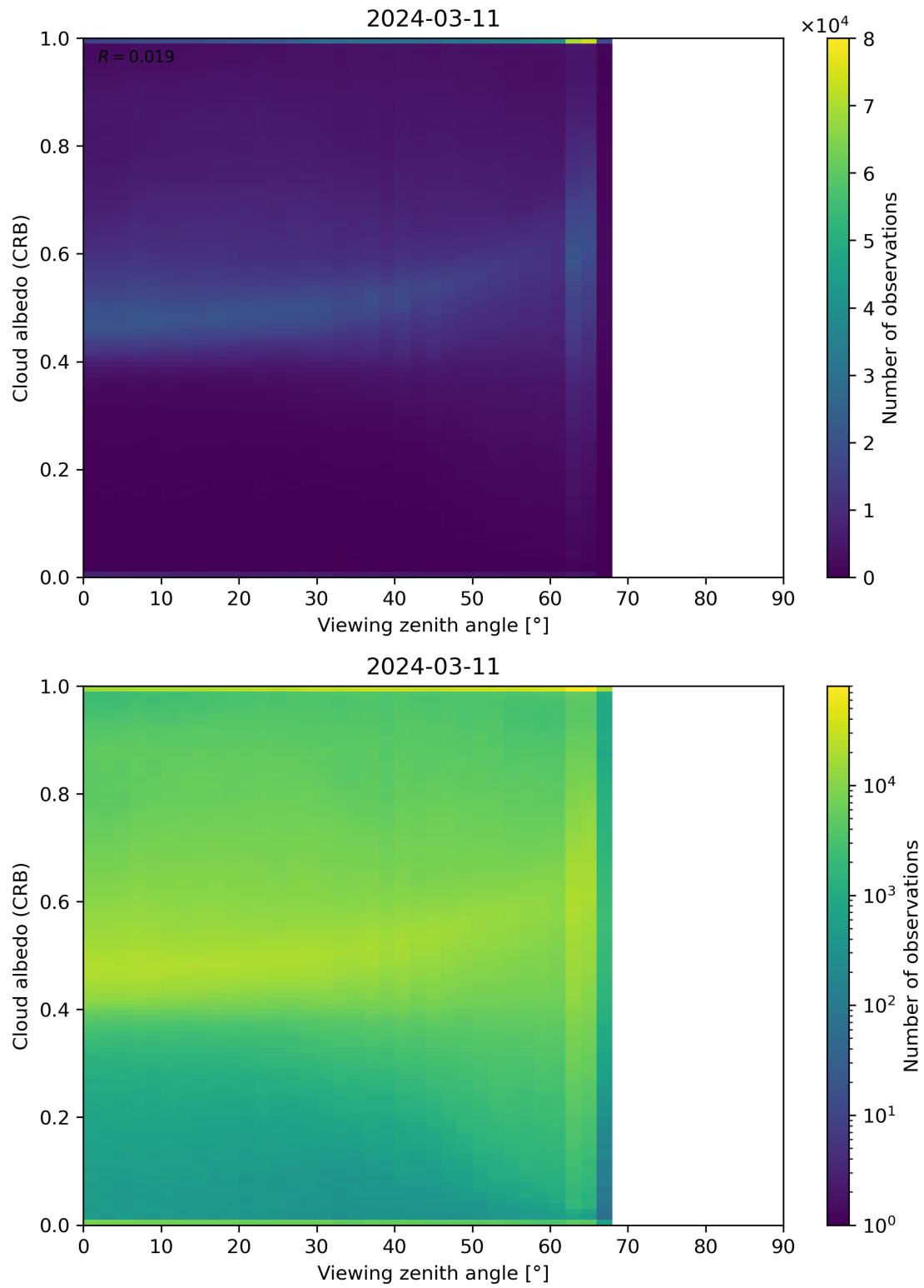
Figure 106: Scatter density plot of “Viewing zenith angle” against “Cloud albedo (CRB)” for 2024-03-10 to 2024-03-12.
