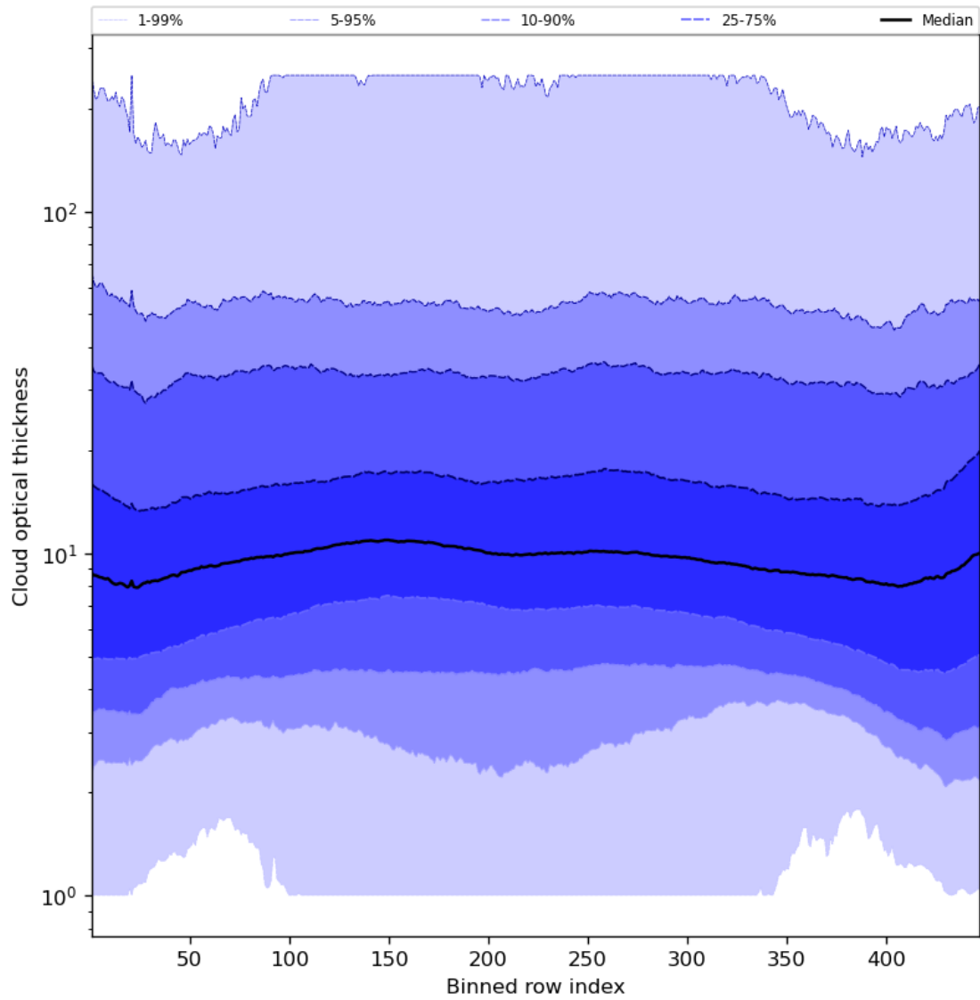
Figure 57: Along track statistics of “Cloud optical thickness” for 2024-03-10 to 2024-03-12
