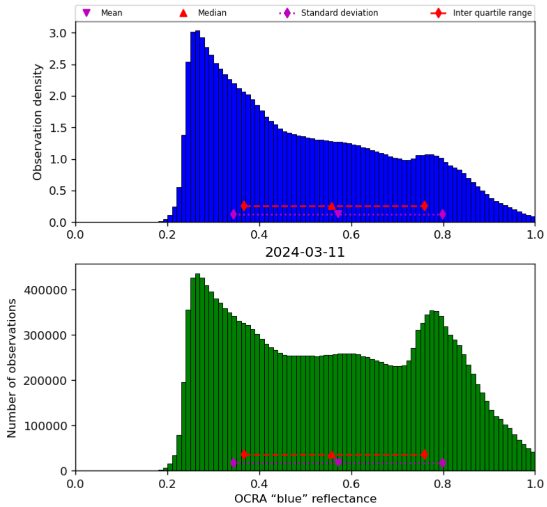
Figure 51: Histogram of “OCRA “blue” reflectance” for 2024-03-10 to 2024-03-12
