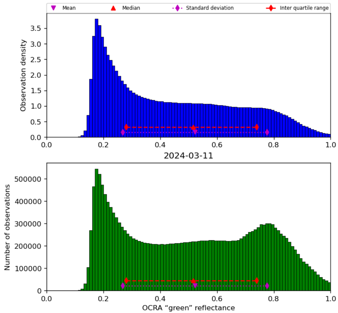
Figure 52: Histogram of “OCRA “green” reflectance” for 2024-03-10 to 2024-03-12
