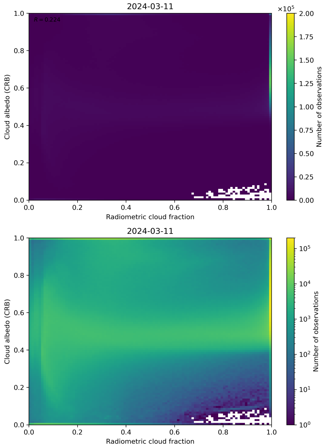
Figure 71: Scatter density plot of “Radiometric cloud fraction” against “Cloud albedo (CRB)” for 2024-03-10 to 2024-03-12.
