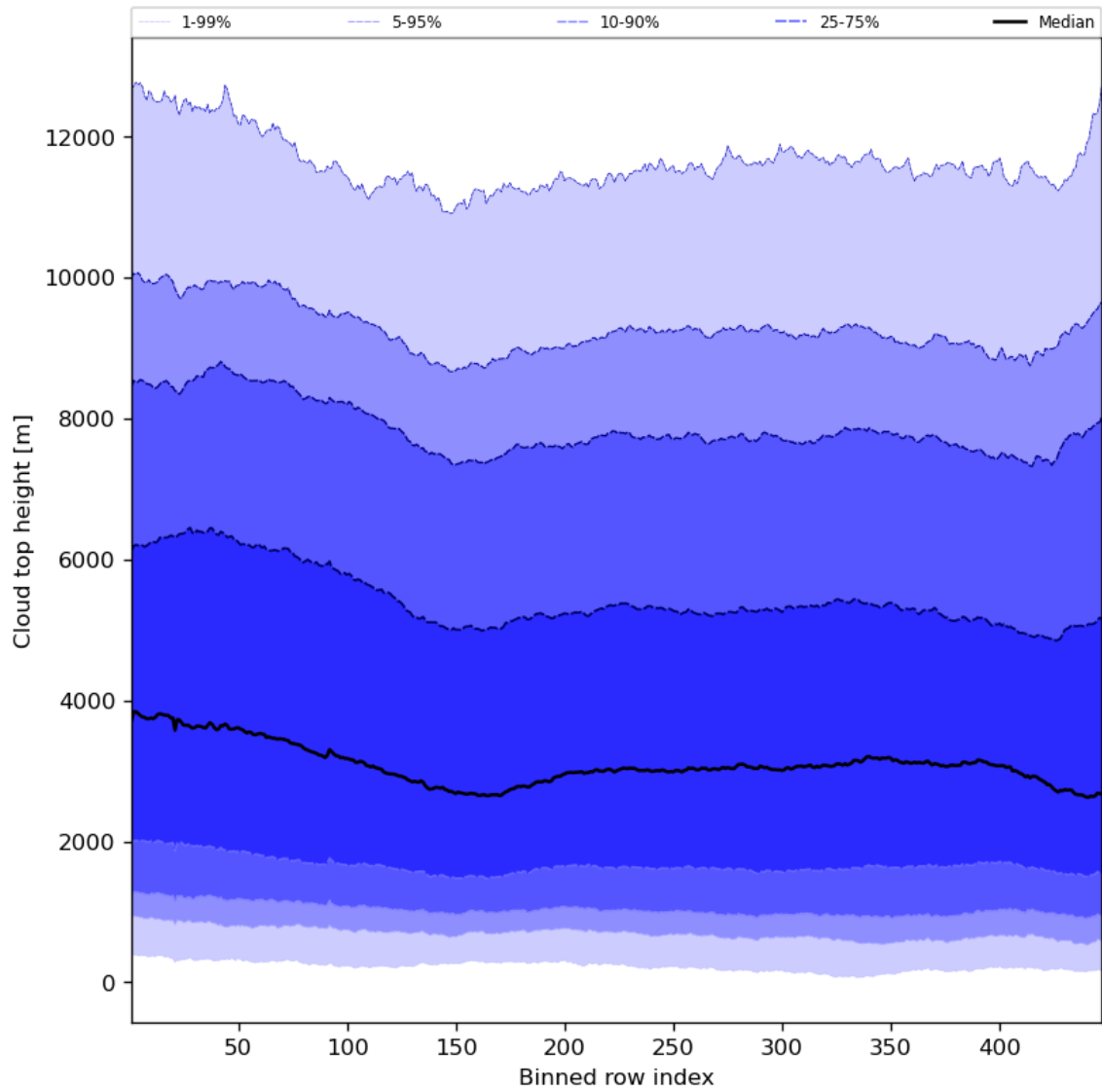
Figure 56: Along track statistics of “Cloud top height” for 2024-03-10 to 2024-03-12
