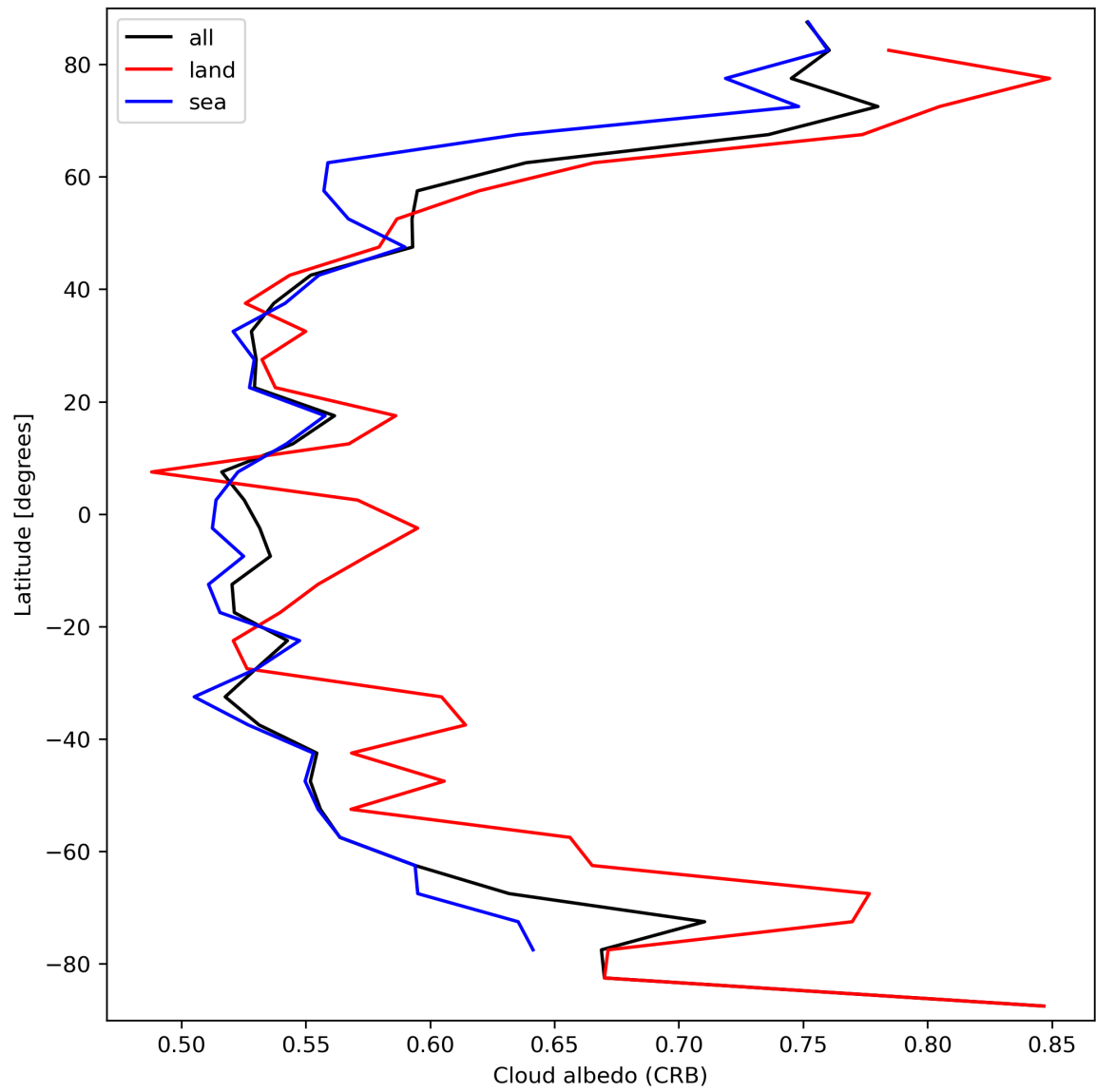
Figure 28: Zonal average of “Cloud albedo (CRB)” for 2024-03-10 to 2024-03-12.
