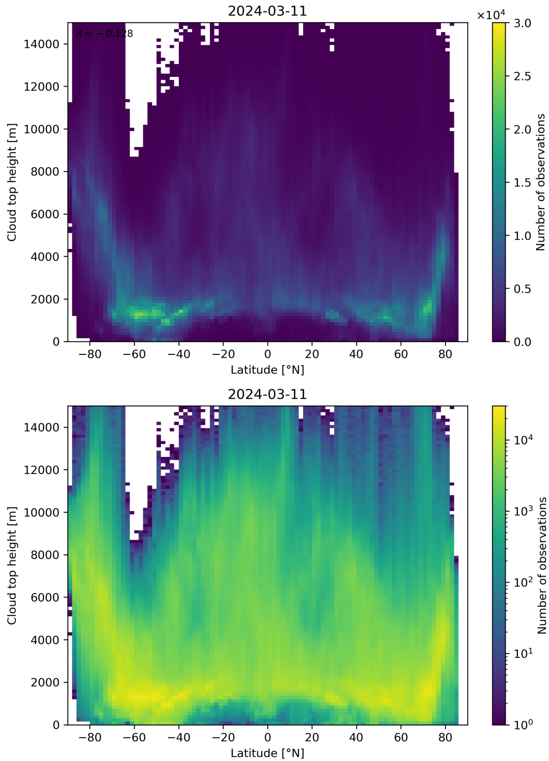
Figure 97: Scatter density plot of “Latitude” against “Cloud top height” for 2024-03-10 to 2024-03-12.
