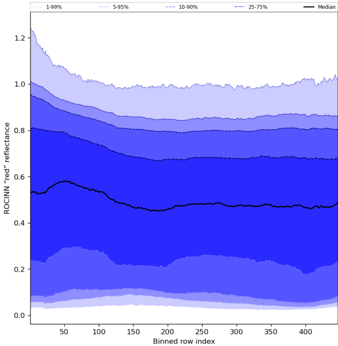
Figure 69: Along track statistics of “ROCINN “red” reflectance” for 2024-03-10 to 2024-03-12
