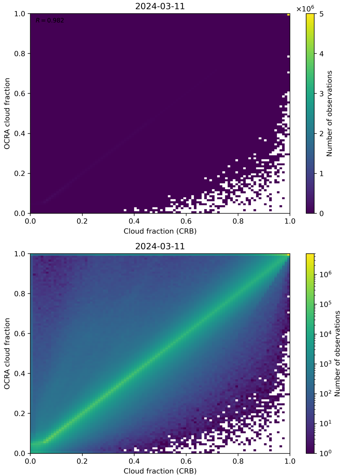
Figure 78: Scatter density plot of “Cloud fraction (CRB)” against “OCRA cloud fraction” for 2024-03-10 to 2024-03-12.
