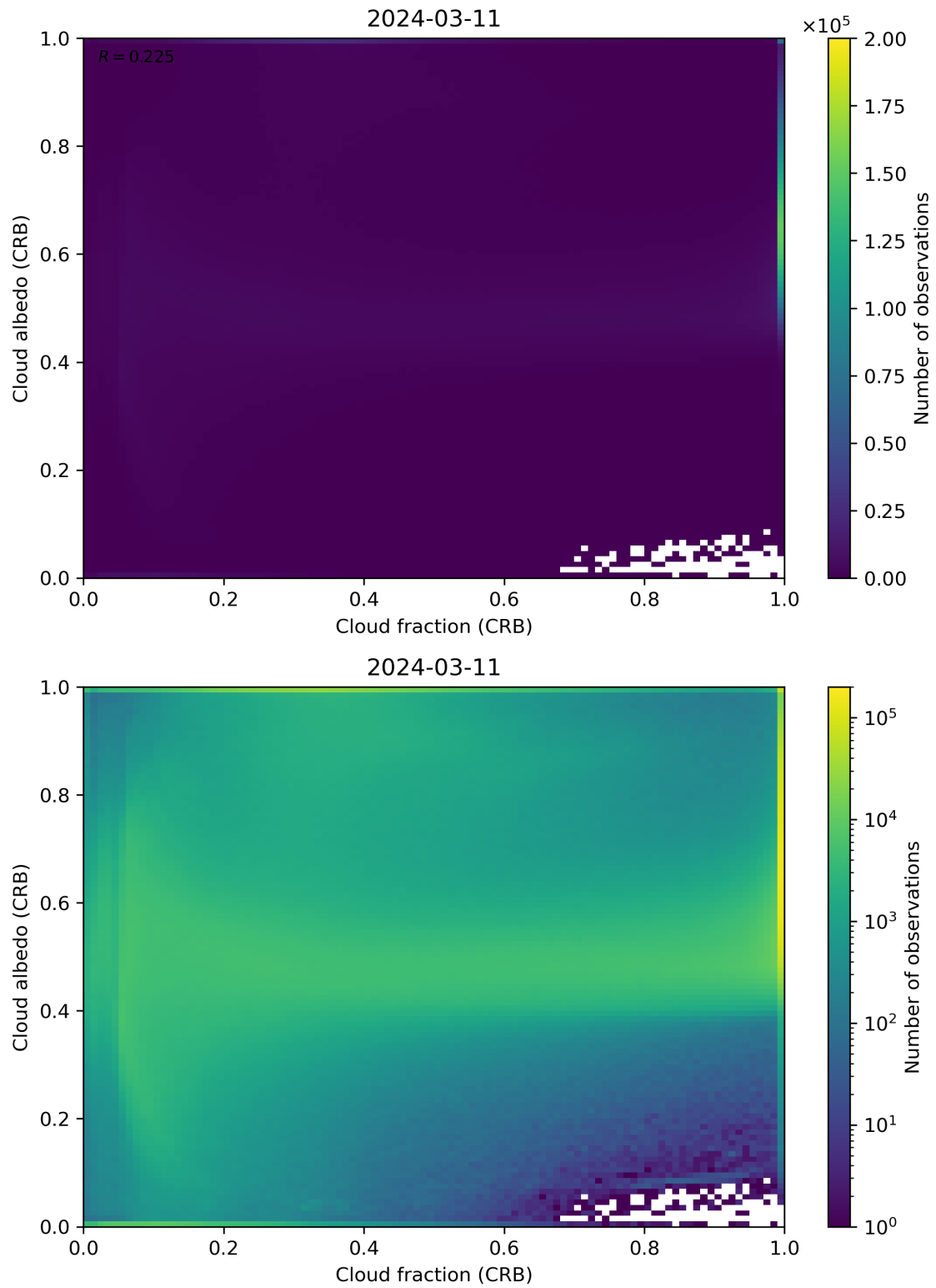
Figure 77: Scatter density plot of “Cloud fraction (CRB)” against “Cloud albedo (CRB)” for 2024-03-10 to 2024-03-12.
