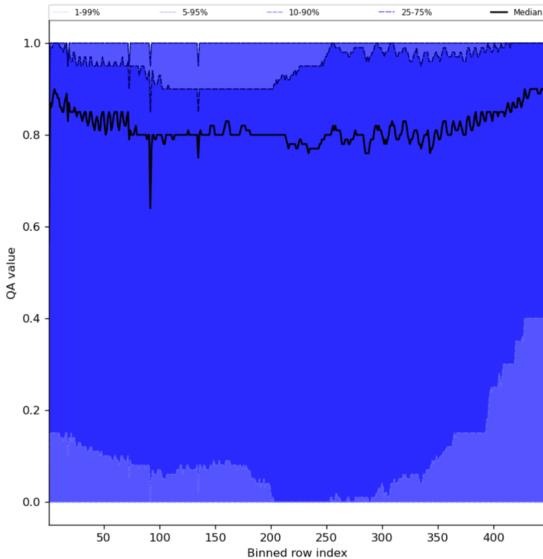
Figure 54: Along track statistics of “QA value” for 2024-03-10 to 2024-03-12
