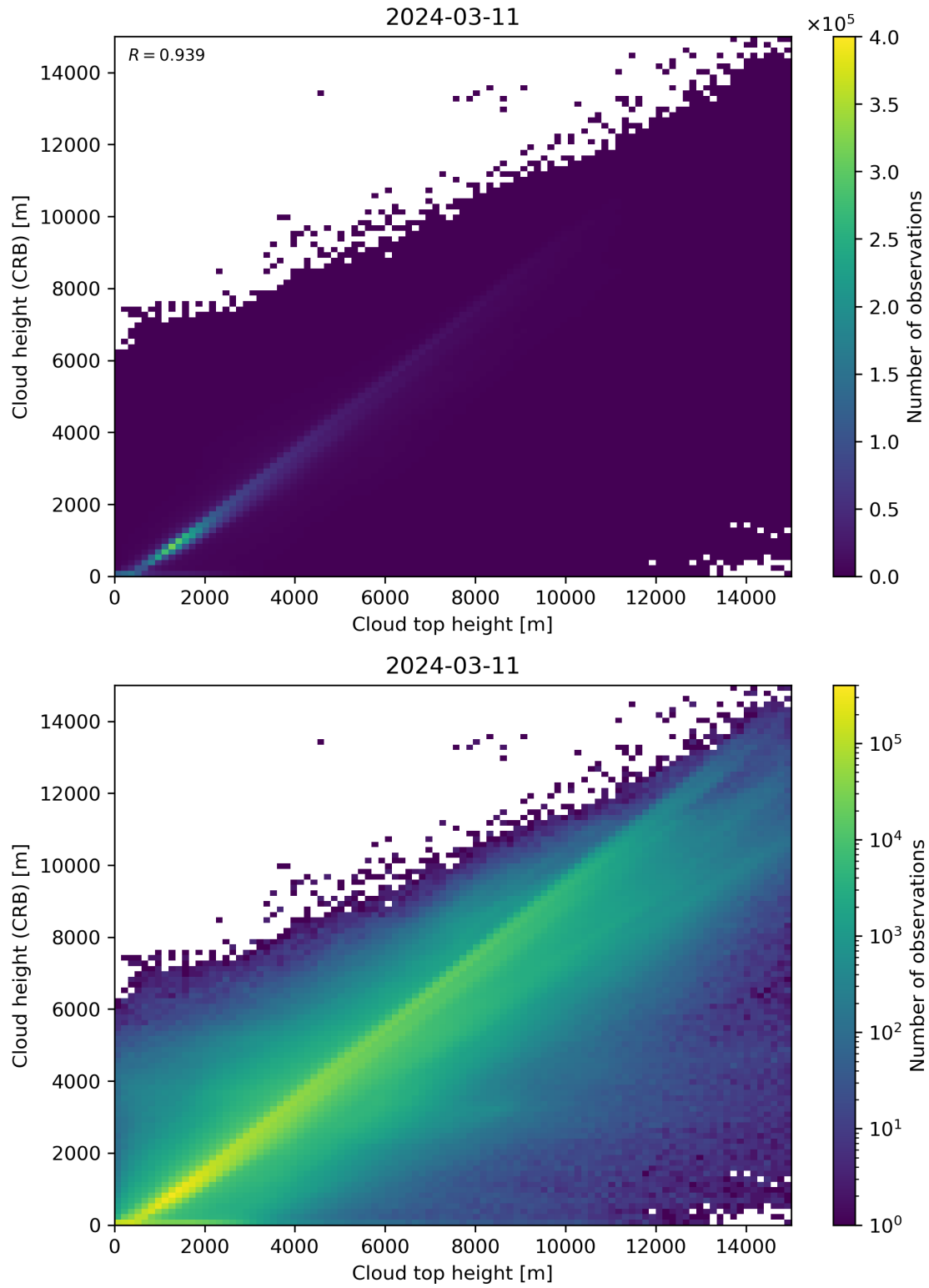
Figure 89: Scatter density plot of “Cloud top height” against “Cloud height (CRB)” for 2024-03-10 to 2024-03-12.
