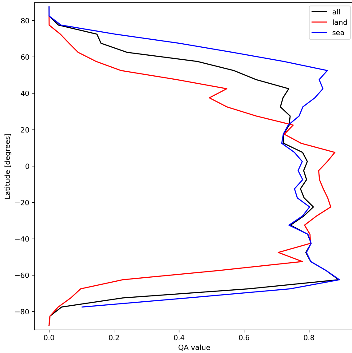
Figure 22: Zonal average of “QA value” for 2024-03-10 to 2024-03-12.
