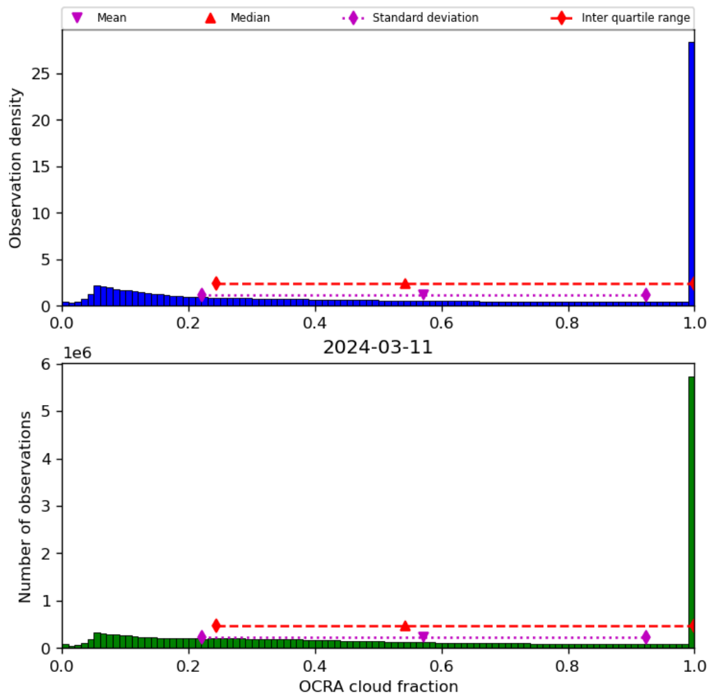
Figure 50: Histogram of “OCRA cloud fraction” for 2024-03-10 to 2024-03-12
