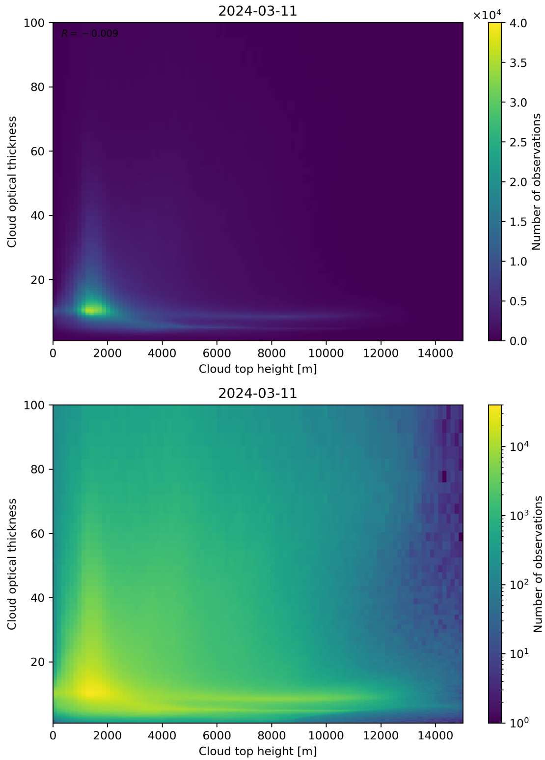
Figure 90: Scatter density plot of “Cloud top height” against “Cloud optical thickness” for 2024-03-10 to 2024-03-12.
