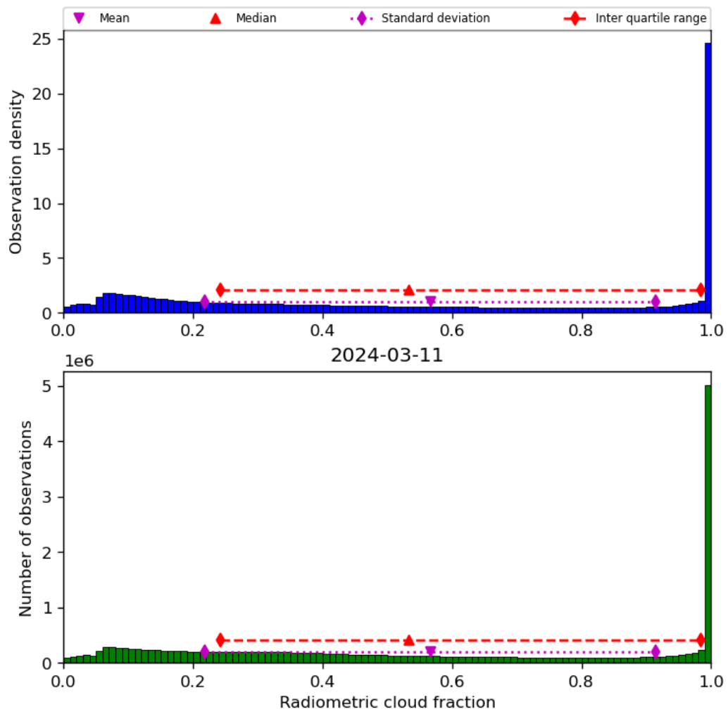
Figure 39: Histogram of “Radiometric cloud fraction” for 2024-03-10 to 2024-03-12
