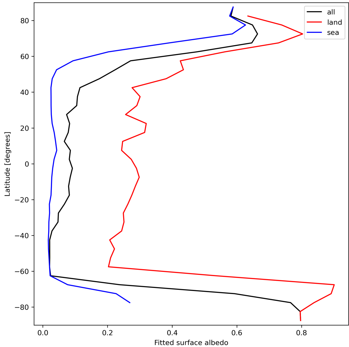
Figure 29: Zonal average of “Fitted surface albedo” for 2024-03-10 to 2024-03-12.
