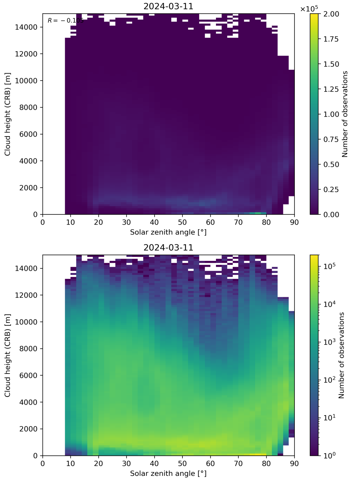
Figure 102: Scatter density plot of “Solar zenith angle” against “Cloud height (CRB)” for 2024-03-10 to 2024-03-12.
