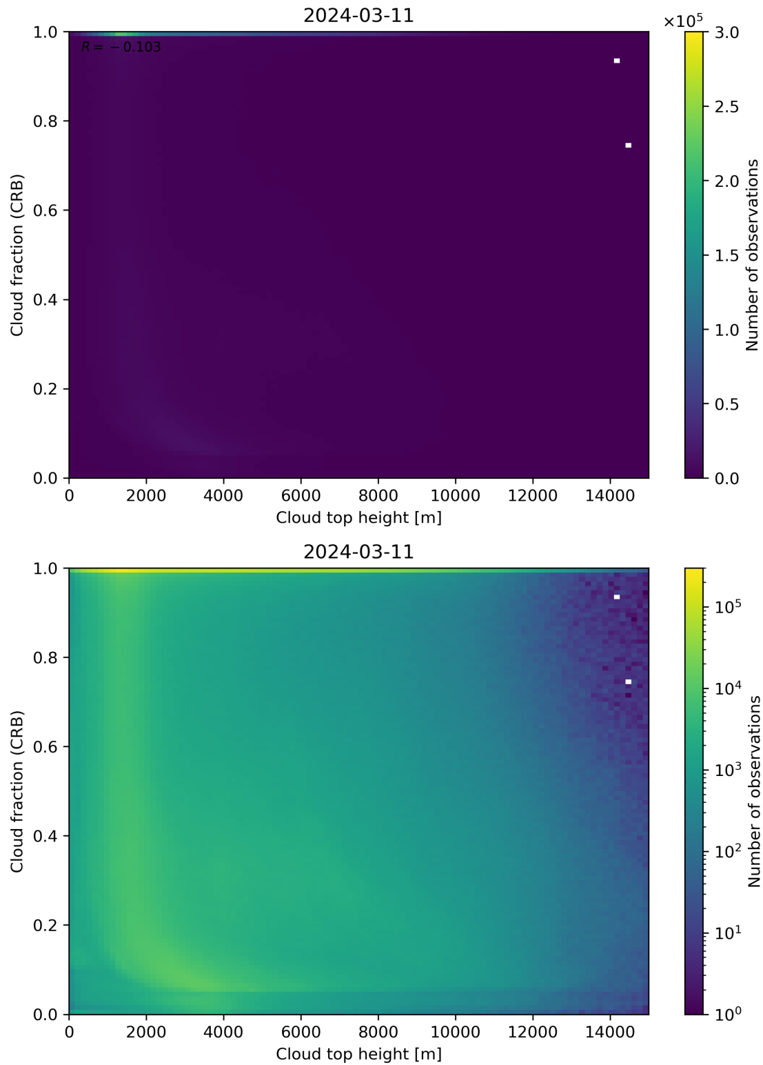
Figure 88: Scatter density plot of “Cloud top height” against “Cloud fraction (CRB)” for 2024-03-10 to 2024-03-12.
