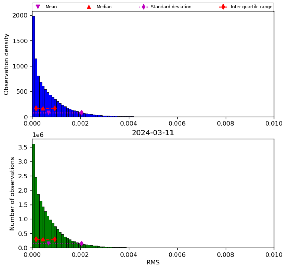
Figure 47: Histogram of “RMS” for 2024-03-10 to 2024-03-12
