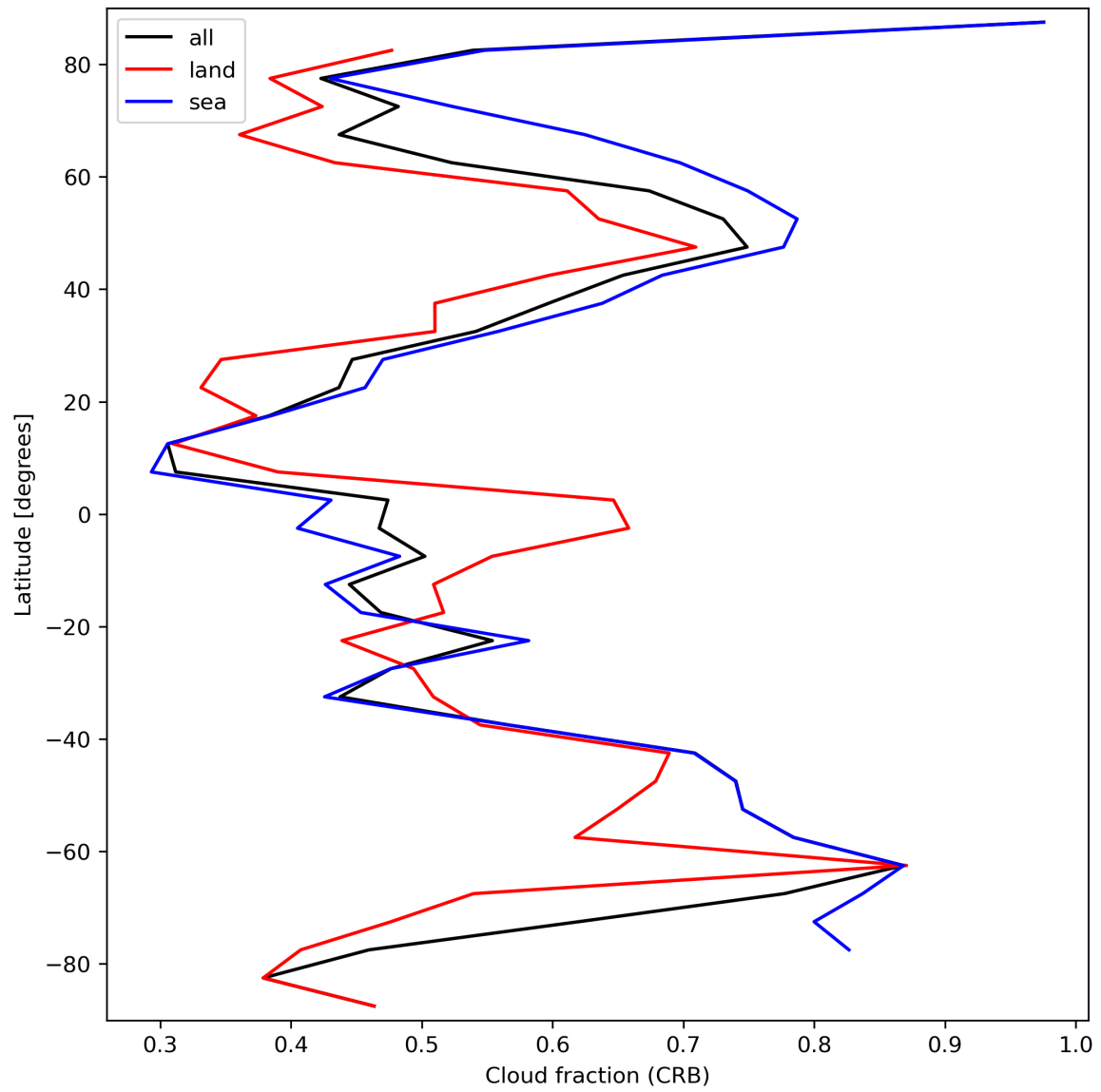
Figure 26: Zonal average of “Cloud fraction (CRB)” for 2024-03-10 to 2024-03-12.
