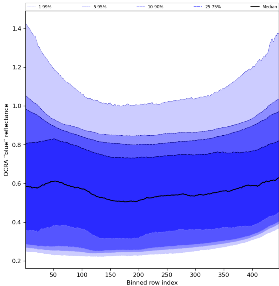
Figure 67: Along track statistics of "OCRA "blue" reflectance" for 2024-03-10 to 2024-03-12
