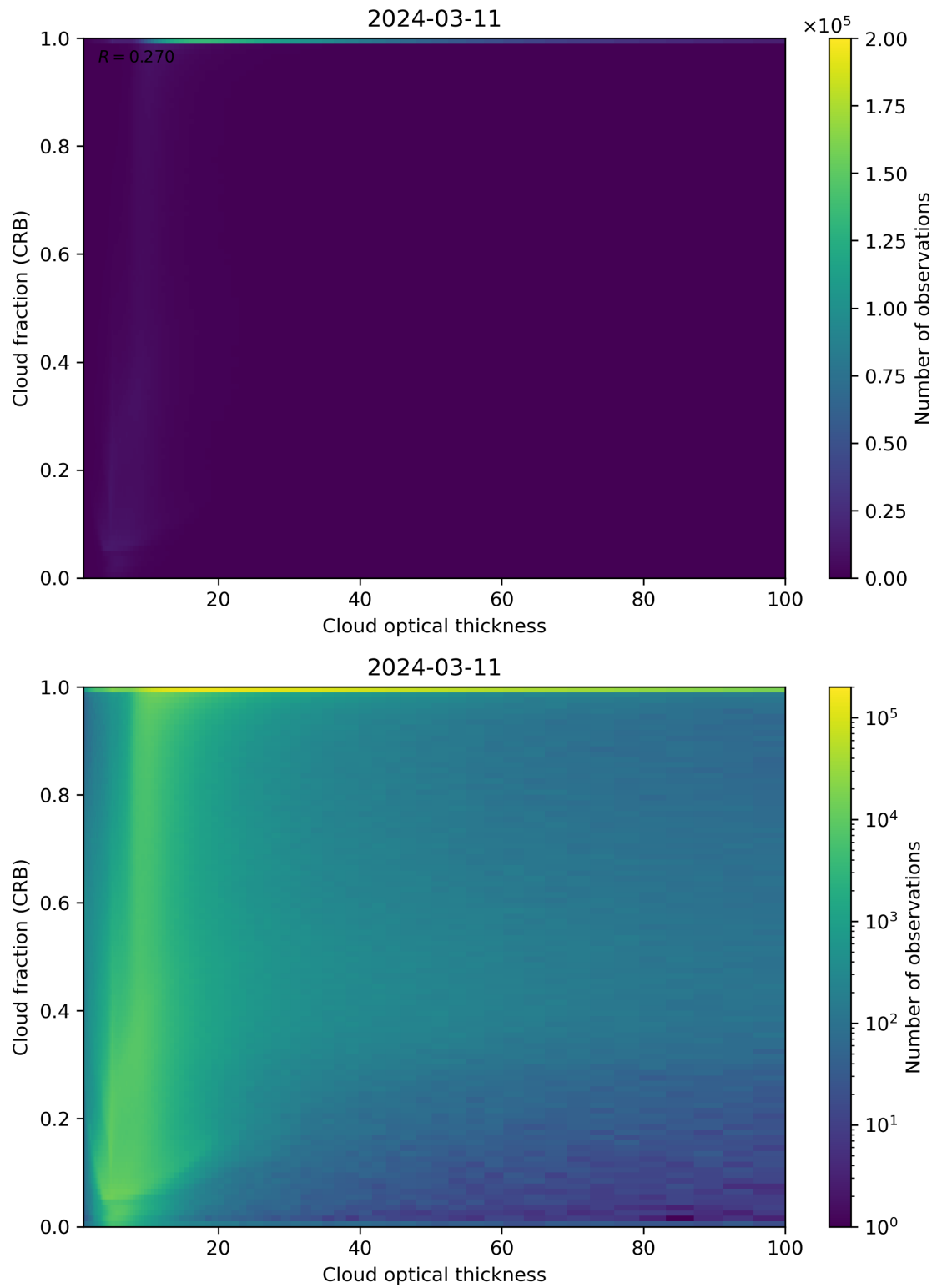
Figure 84: Scatter density plot of “Cloud optical thickness” against “Cloud fraction (CRB)” for 2024-03-10 to 2024-03-12.
