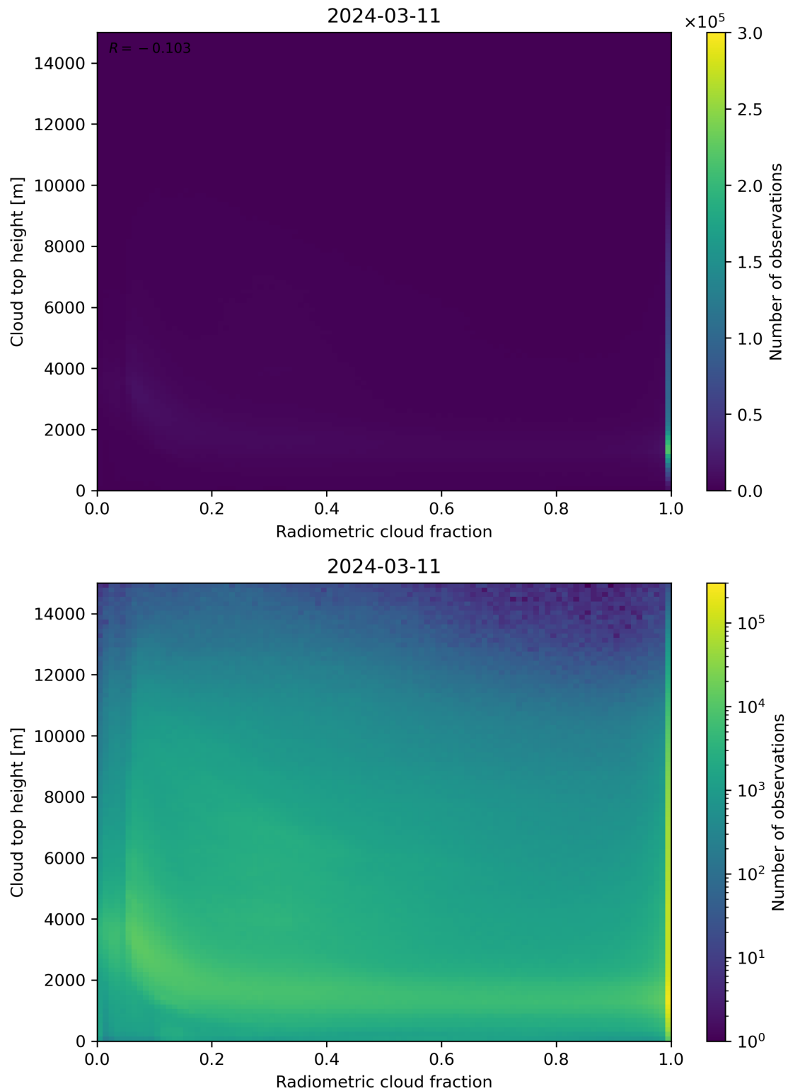
Figure 76: Scatter density plot of “Radiometric cloud fraction” against “Cloud top height” for 2024-03-10 to 2024-03-12.
