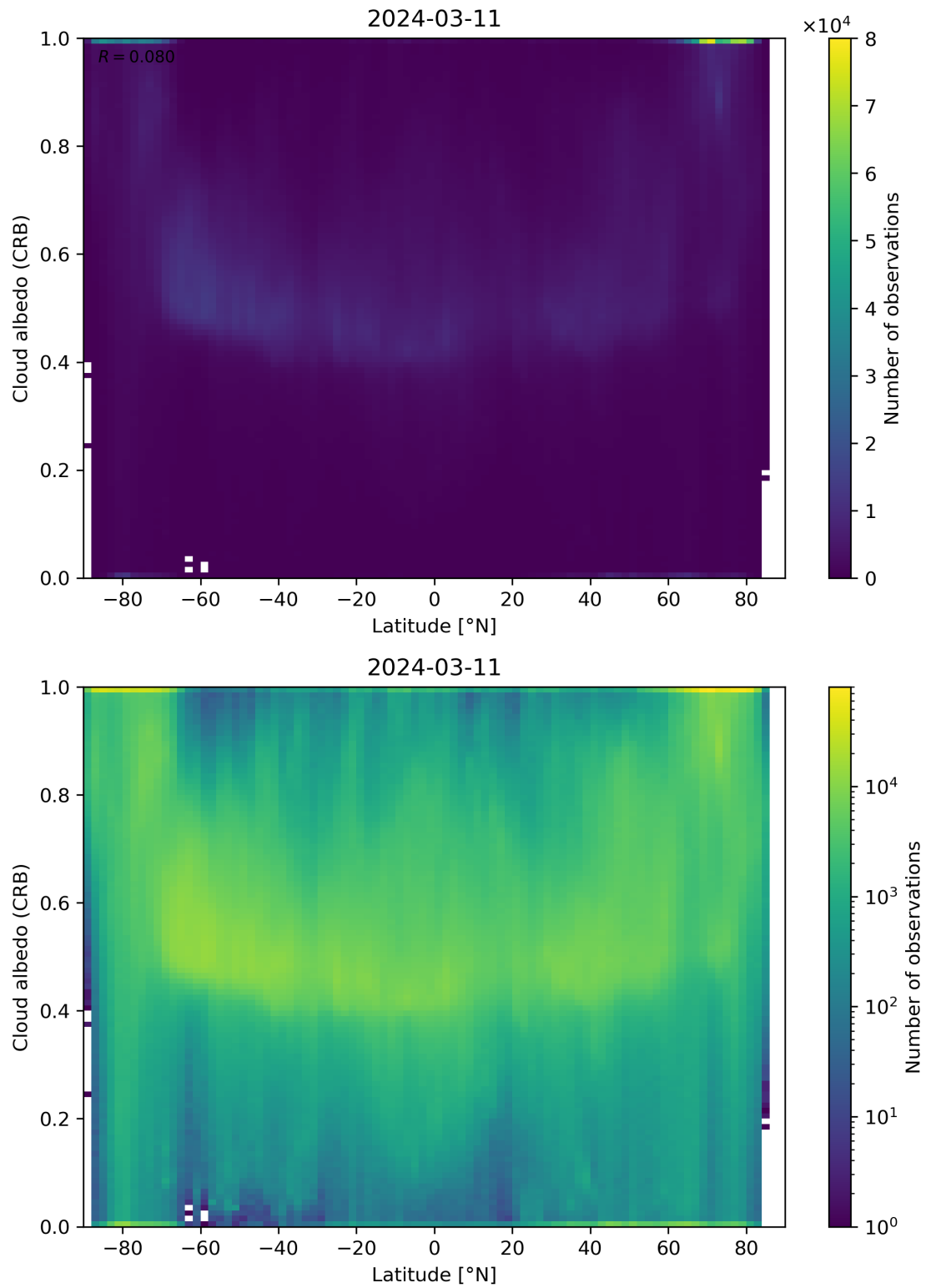
Figure 91: Scatter density plot of “Latitude” against “Cloud albedo (CRB)” for 2024-03-10 to 2024-03-12.
