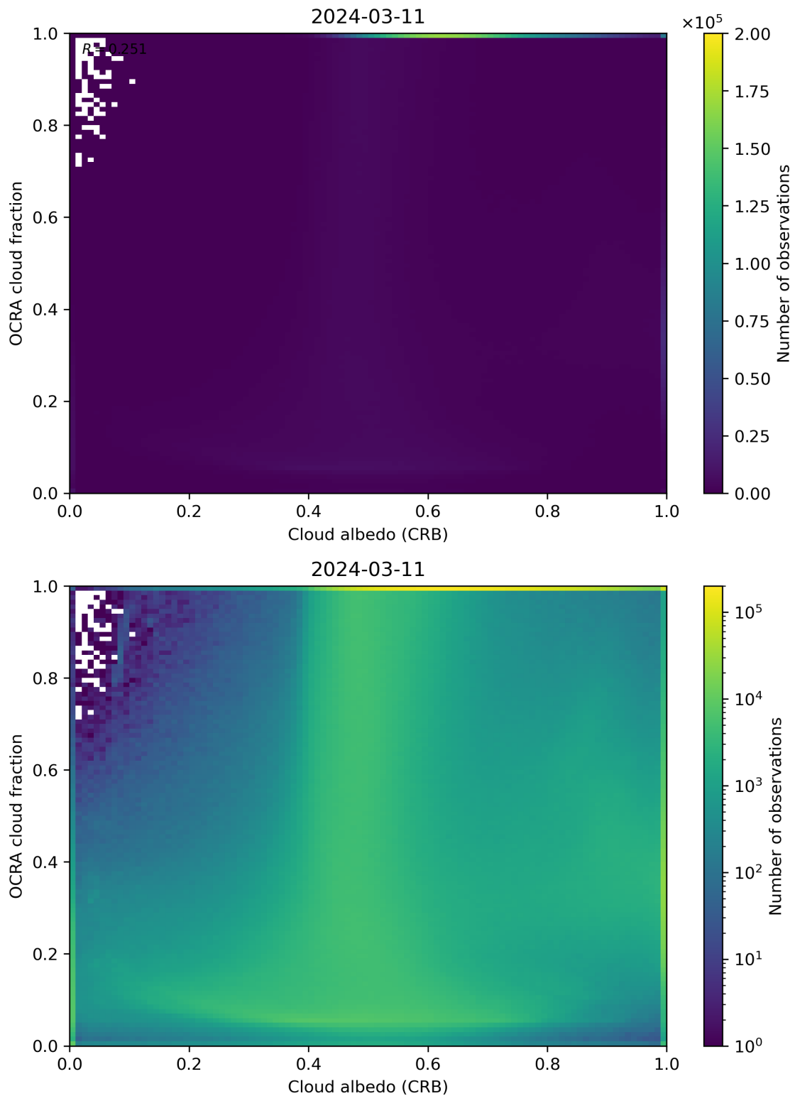
Figure 70: Scatter density plot of “Cloud albedo (CRB)” against “OCRA cloud fraction” for 2024-03-10 to 2024-03-12.
