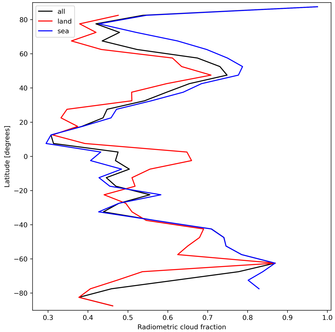
Figure 23: Zonal average of “Radiometric cloud fraction” for 2024-03-10 to 2024-03-12.
