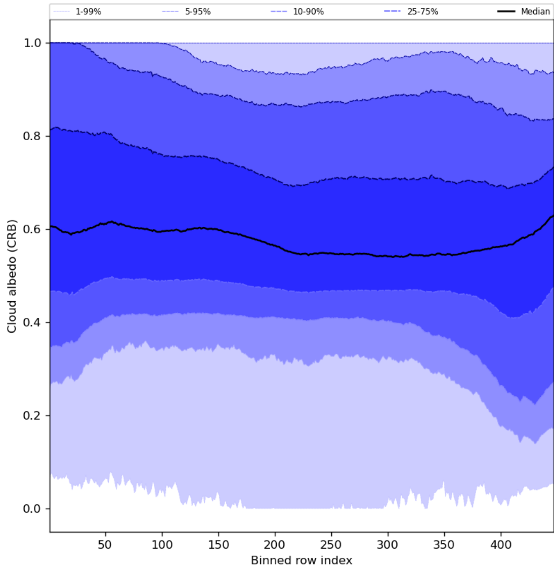
Figure 60: Along track statistics of “Cloud albedo (CRB)” for 2024-03-10 to 2024-03-12
