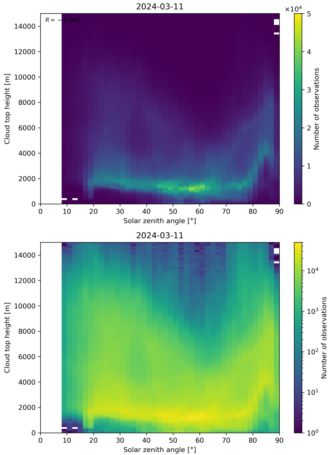
Figure 104: Scatter density plot of “Solar zenith angle” against “Cloud top height” for 2024-03-10 to 2024-03-12.
