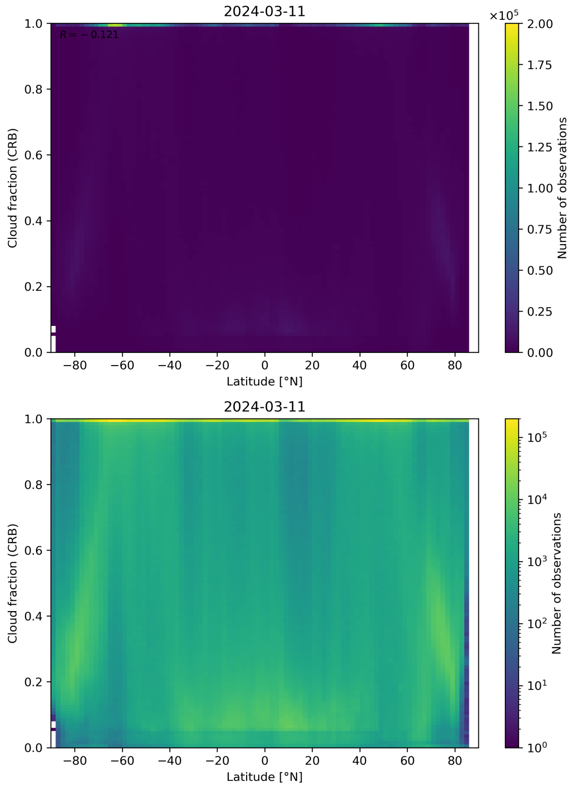
Figure 94: Scatter density plot of “Latitude” against “Cloud fraction (CRB)” for 2024-03-10 to 2024-03-12.
