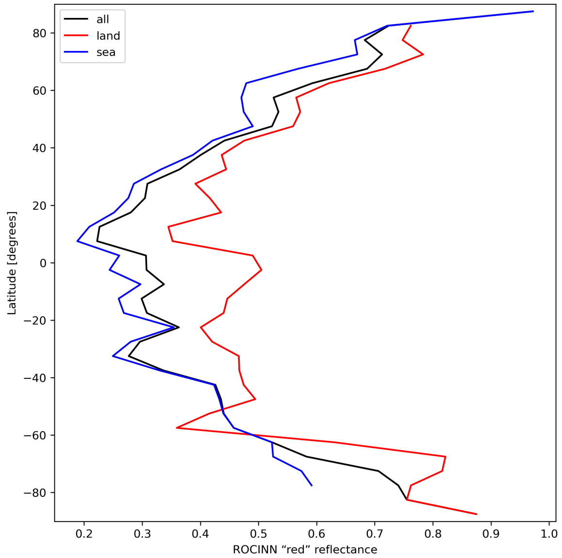
Figure 37: Zonal average of “ROCINN “red” reflectance” for 2024-03-10 to 2024-03-12.
