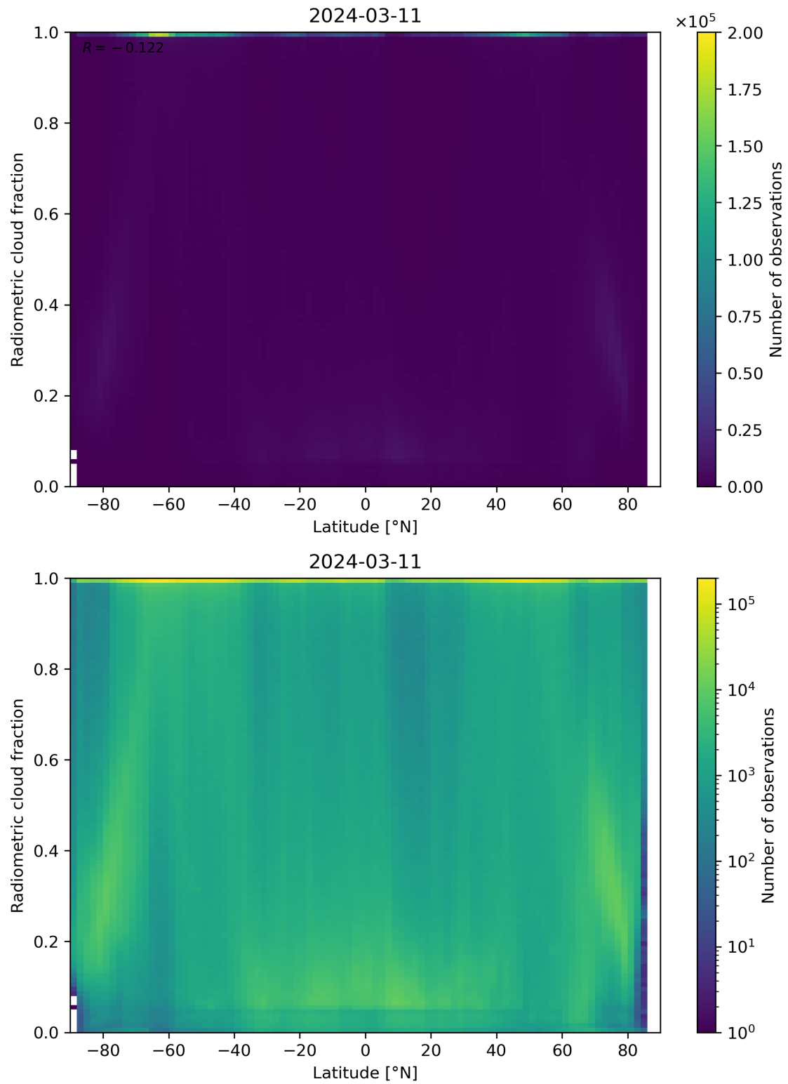
Figure 92: Scatter density plot of “Latitude” against “Radiometric cloud fraction” for 2024-03-10 to 2024-03-12.
