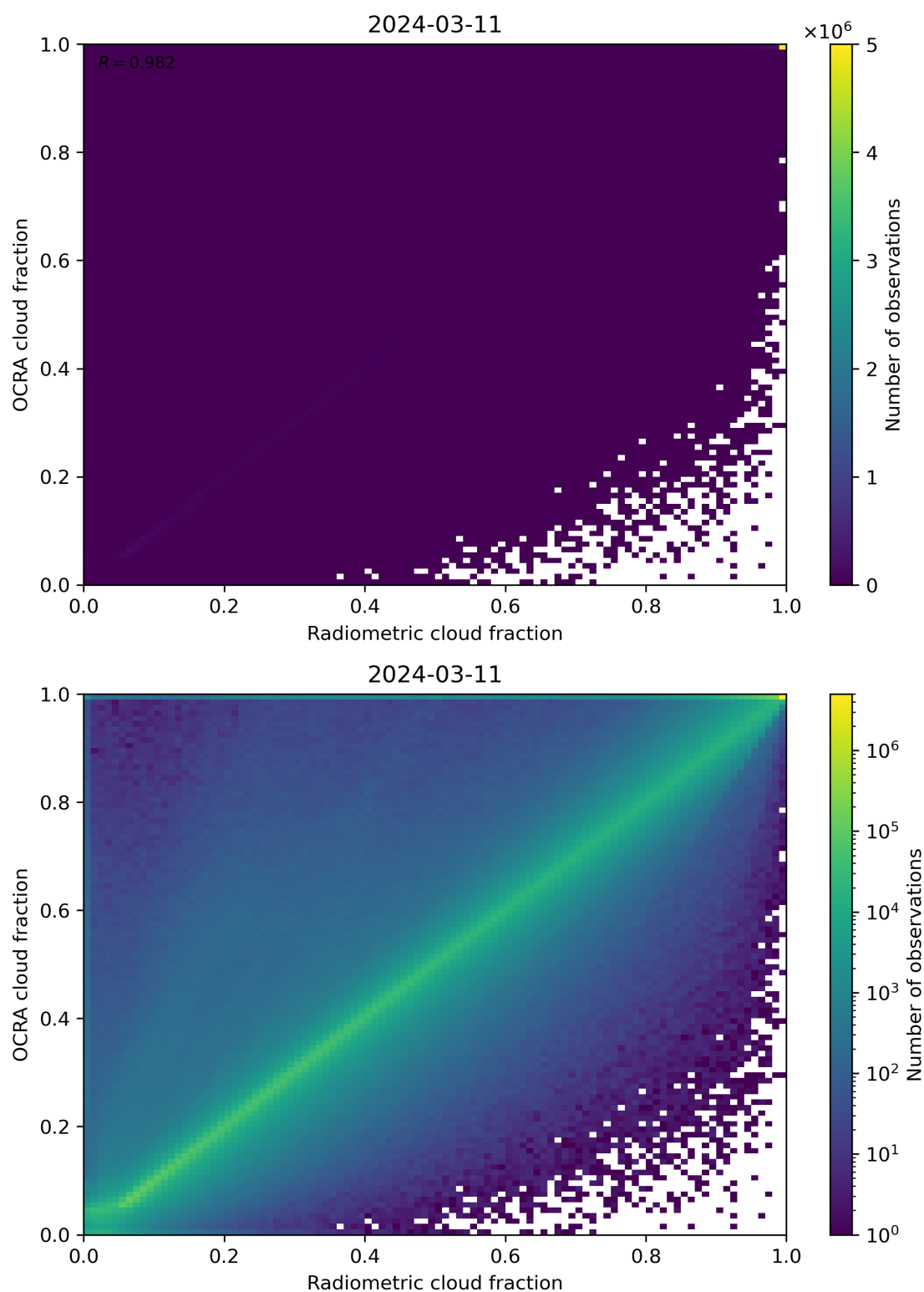
Figure 72: Scatter density plot of “Radiometric cloud fraction” against “OCRA cloud fraction” for 2024-03-10 to 2024-03-12.
