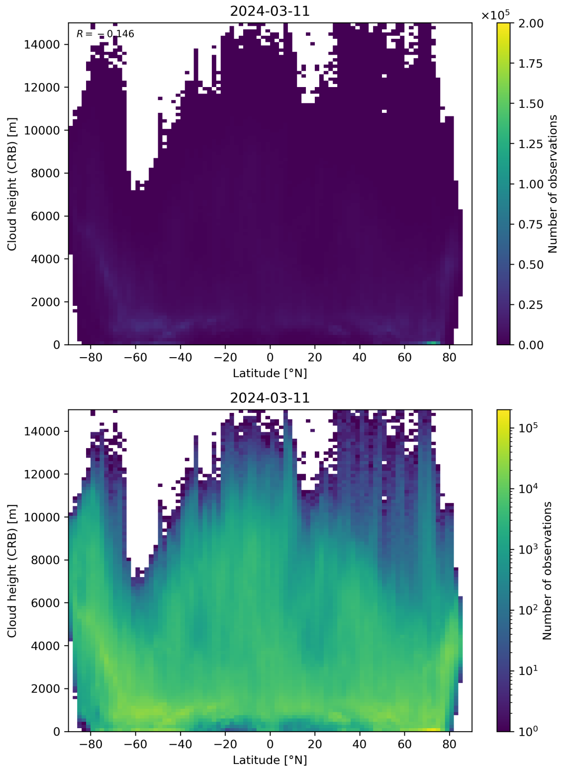
Figure 95: Scatter density plot of “Latitude” against “Cloud height (CRB)” for 2024-03-10 to 2024-03-12.
