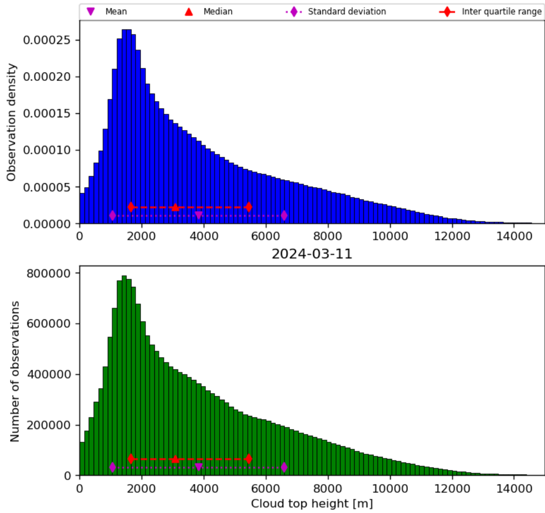
Figure 40: Histogram of “Cloud top height” for 2024-03-10 to 2024-03-12
