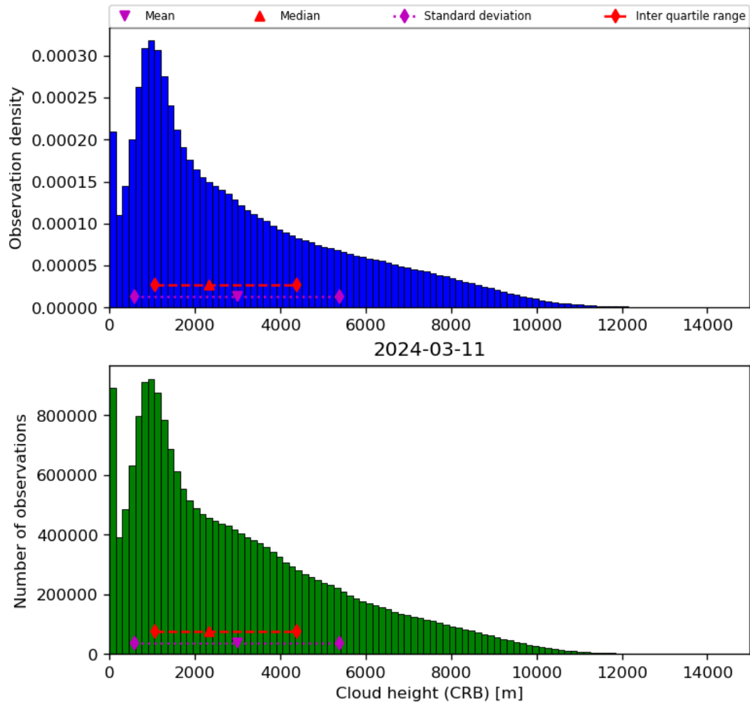
Figure 43: Histogram of “Cloud height (CRB)” for 2024-03-10 to 2024-03-12
