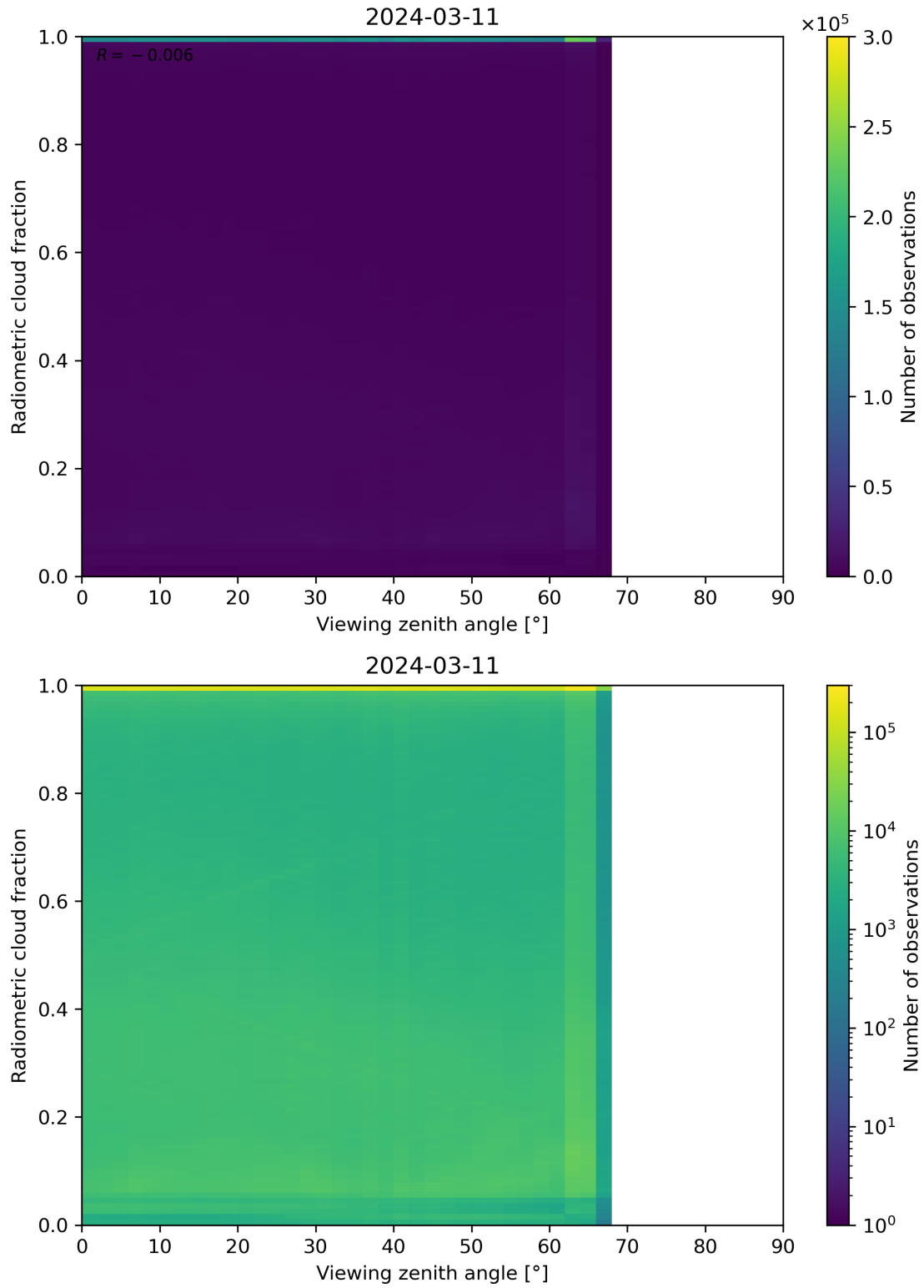
Figure 107: Scatter density plot of “Viewing zenith angle” against “Radiometric cloud fraction” for 2024-03-10 to 2024-03-12.
