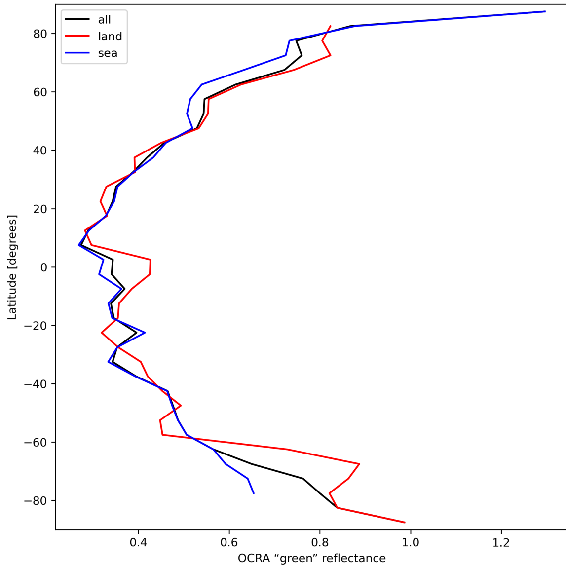
Figure 36: Zonal average of “OCRA “green” reflectance” for 2024-03-10 to 2024-03-12.
