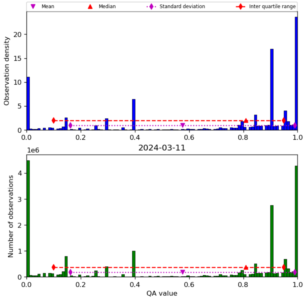
Figure 38: Histogram of “QA value” for 2024-03-10 to 2024-03-12
