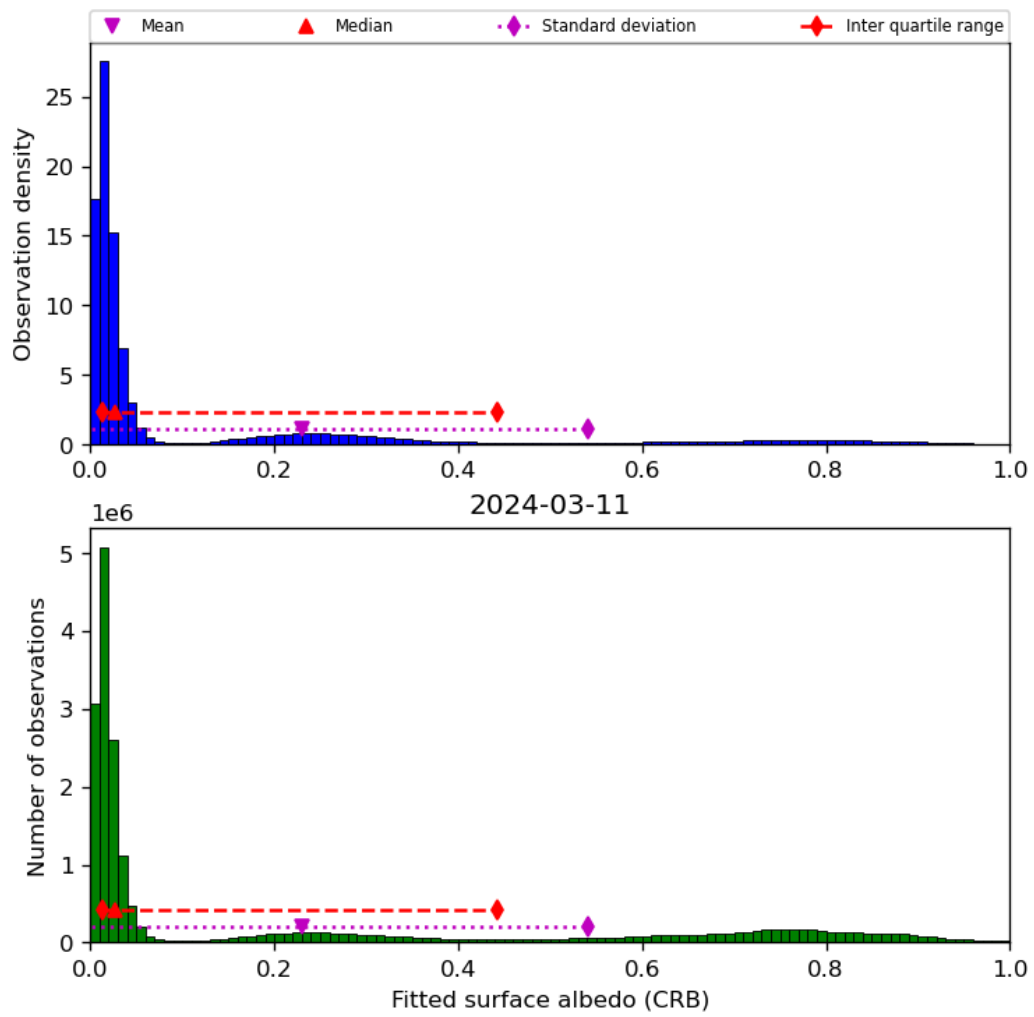
Figure 46: Histogram of “Fitted surface albedo (CRB)” for 2024-03-10 to 2024-03-12
