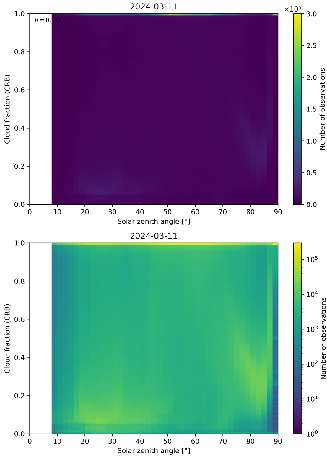
Figure 101: Scatter density plot of “Solar zenith angle” against “Cloud fraction (CRB)” for 2024-03-10 to 2024-03-12.
