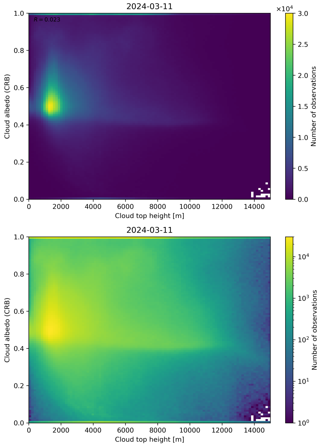
Figure 86: Scatter density plot of “Cloud top height” against “Cloud albedo (CRB)” for 2024-03-10 to 2024-03-12.
