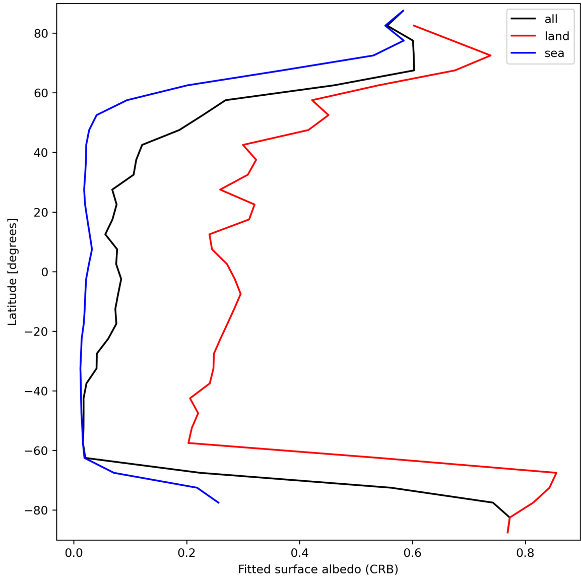
Figure 30: Zonal average of “Fitted surface albedo (CRB)” for 2024-03-10 to 2024-03-12.
