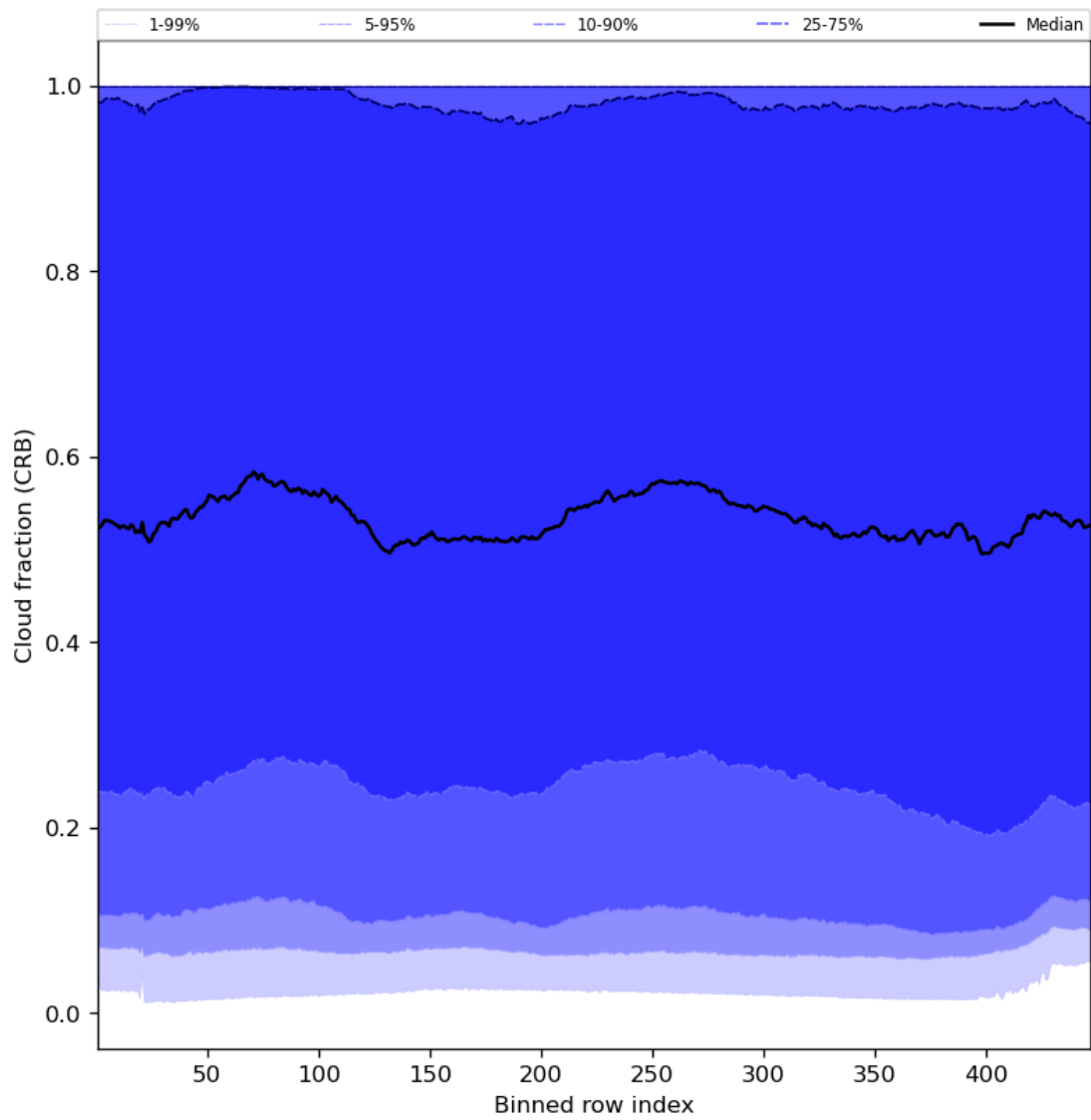
Figure 58: Along track statistics of “Cloud fraction (CRB)” for 2024-03-10 to 2024-03-12
