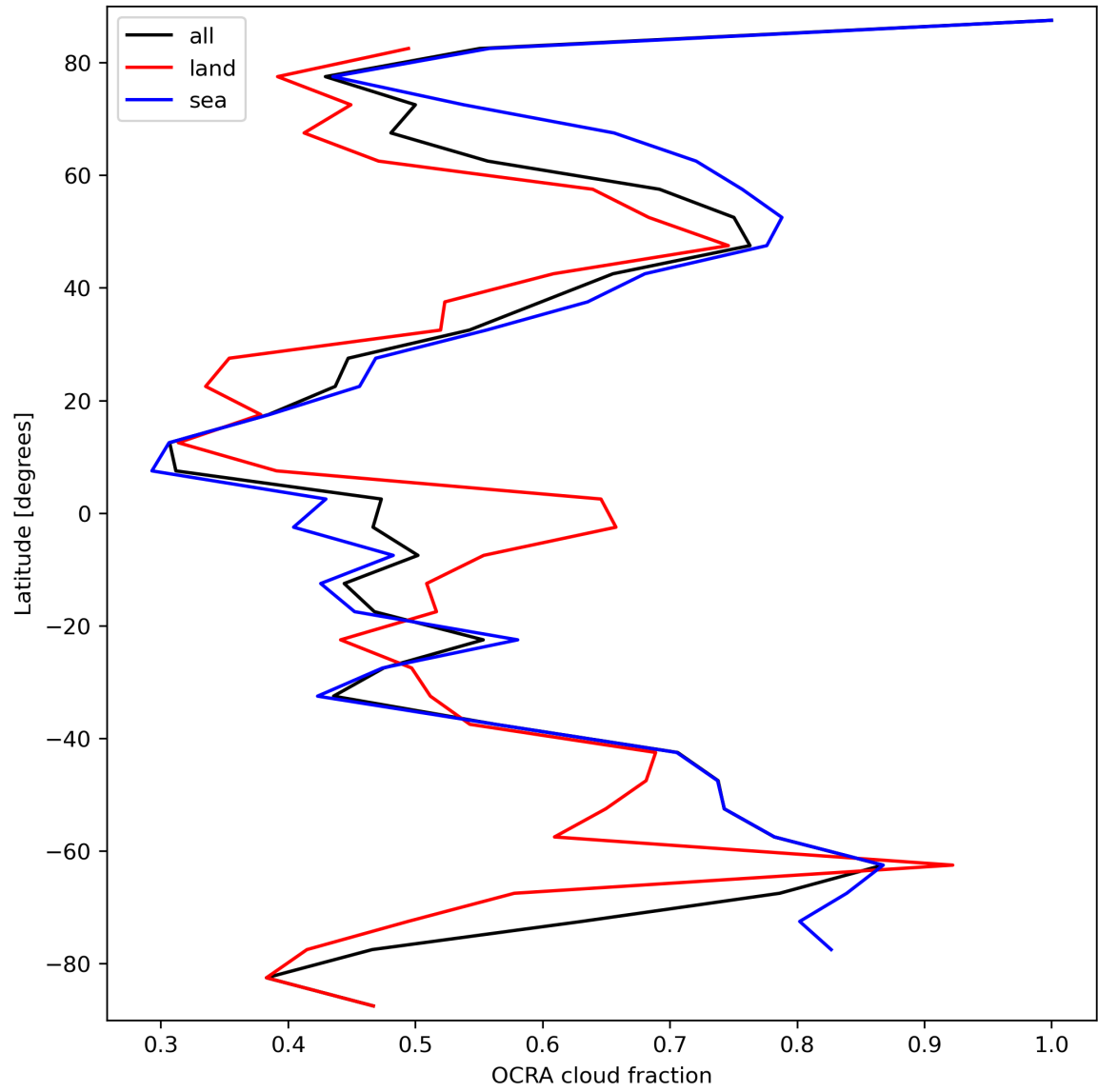
Figure 34: Zonal average of “OCRA cloud fraction” for 2024-03-10 to 2024-03-12.
