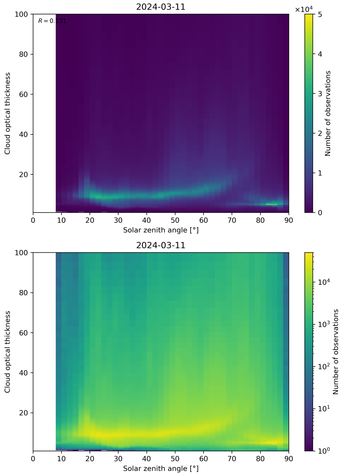
Figure 103: Scatter density plot of “Solar zenith angle” against “Cloud optical thickness” for 2024-03-10 to 2024-03-12.
