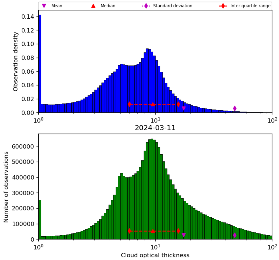
Figure 41: Histogram of “Cloud optical thickness” for 2024-03-10 to 2024-03-12
