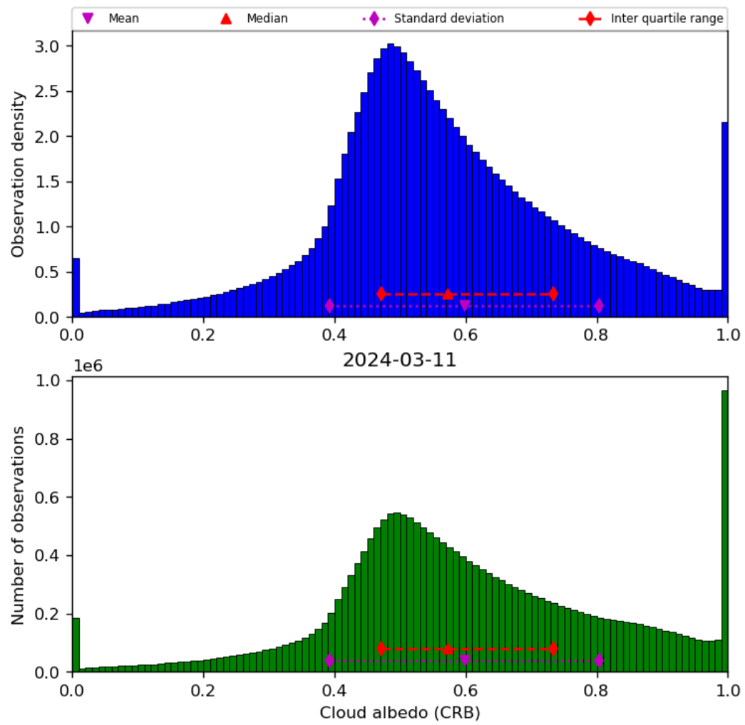
Figure 44: Histogram of “Cloud albedo (CRB)” for 2024-03-10 to 2024-03-12
