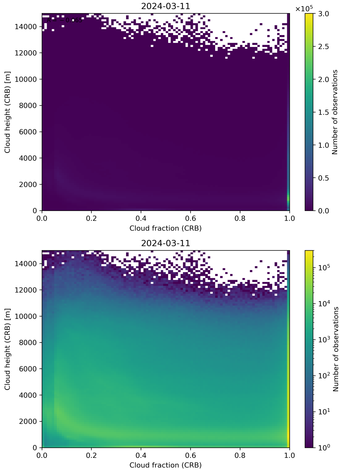
Figure 79: Scatter density plot of “Cloud fraction (CRB)” against “Cloud height (CRB)” for 2024-03-10 to 2024-03-12.
