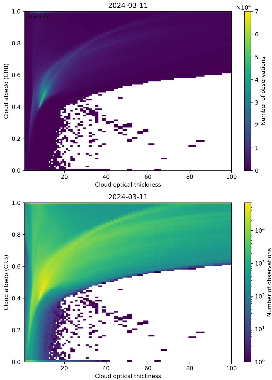
Figure 82: Scatter density plot of “Cloud optical thickness” against “Cloud albedo (CRB)” for 2024-03-10 to 2024-03-12.
