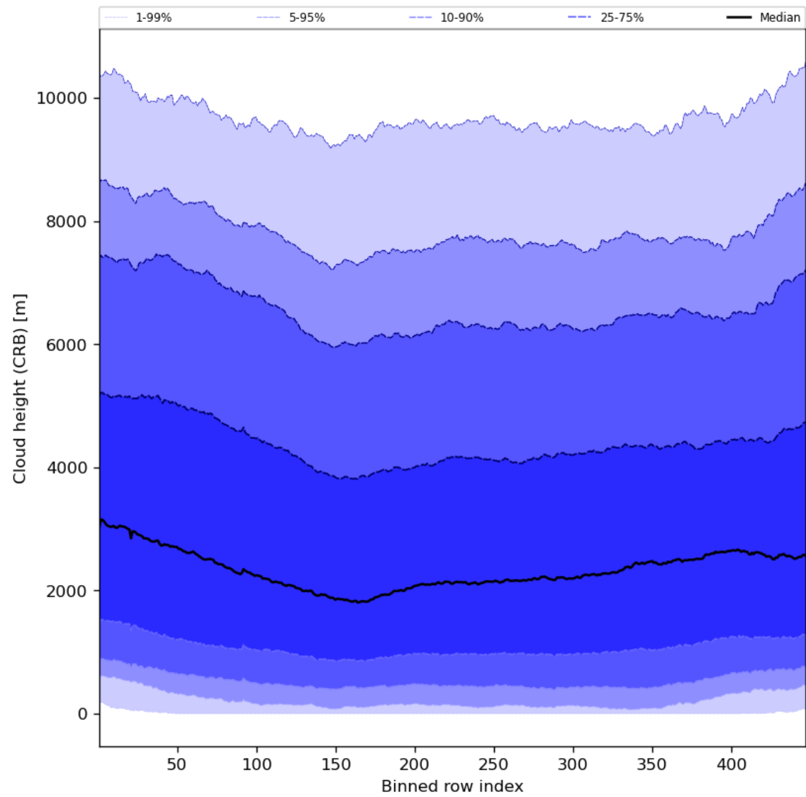
Figure 59: Along track statistics of “Cloud height (CRB)” for 2024-03-10 to 2024-03-12
