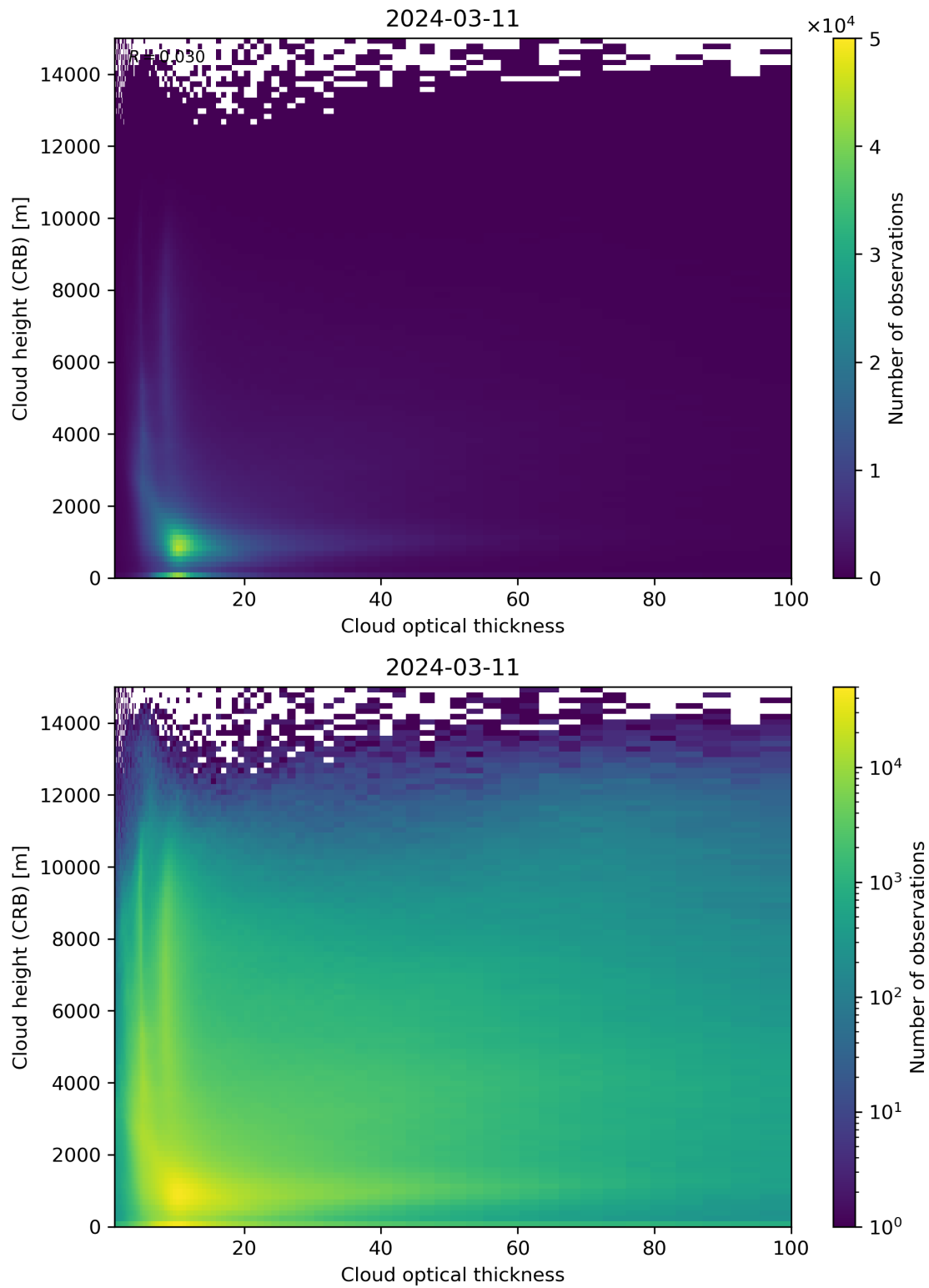
Figure 85: Scatter density plot of “Cloud optical thickness” against “Cloud height (CRB)” for 2024-03-10 to 2024-03-12.
