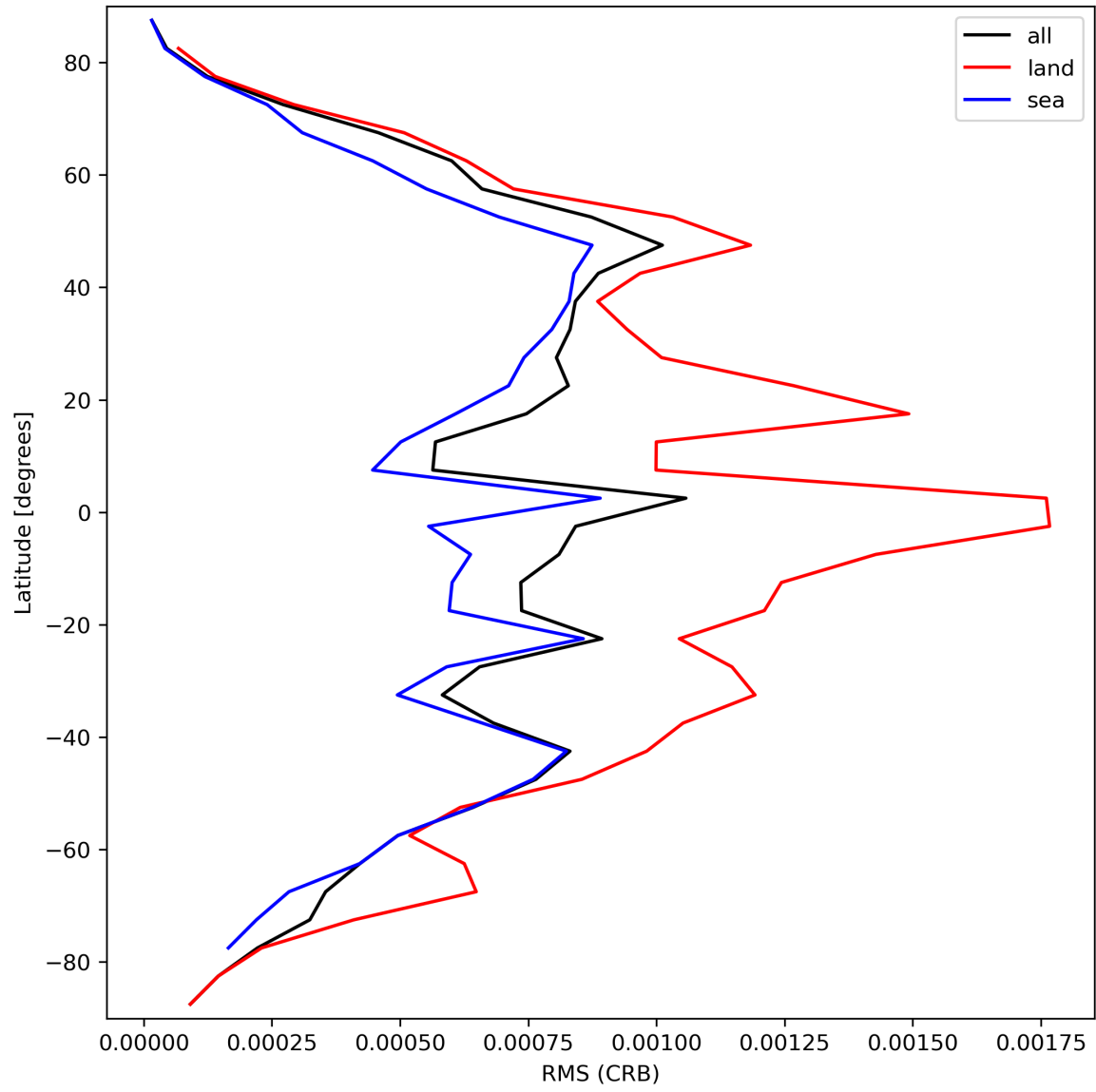
Figure 32: Zonal average of “RMS (CRB)” for 2024-03-10 to 2024-03-12.
