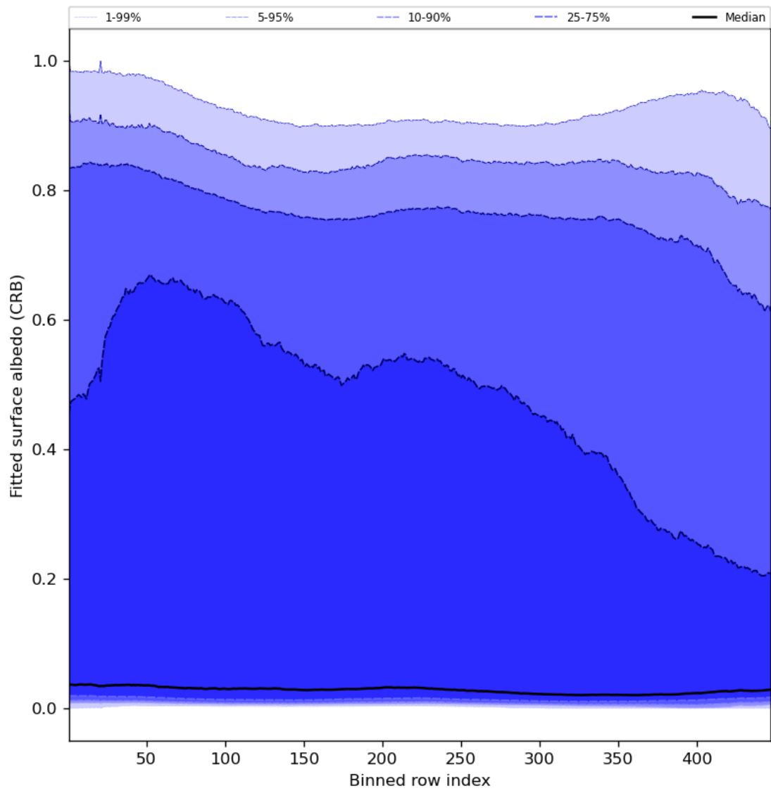
Figure 62: Along track statistics of “Fitted surface albedo (CRB)” for 2024-03-10 to 2024-03-12
