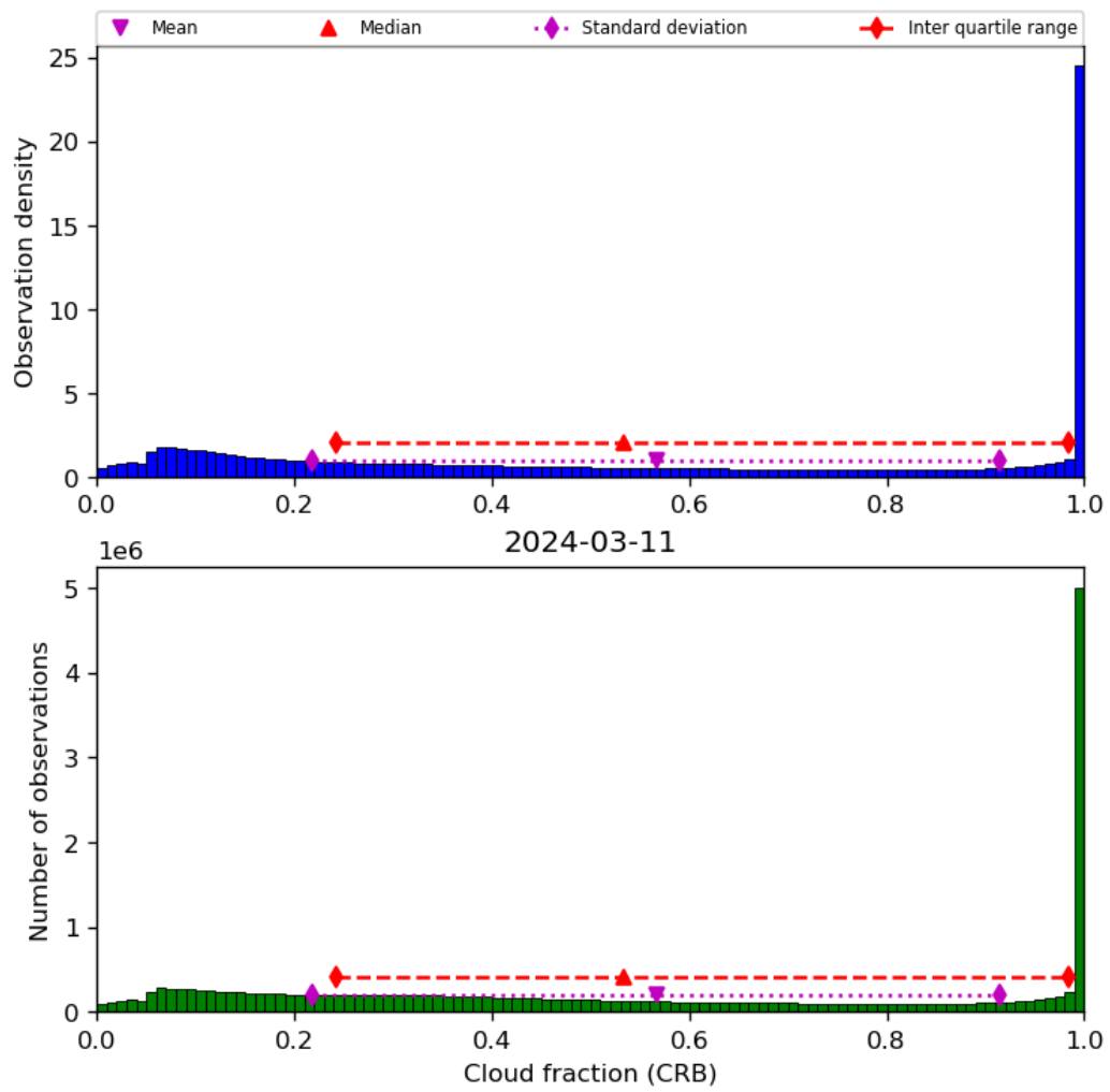
Figure 42: Histogram of “Cloud fraction (CRB)” for 2024-03-10 to 2024-03-12
