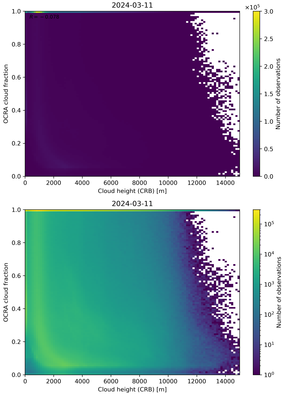
Figure 81: Scatter density plot of “Cloud height (CRB)” against “OCRA cloud fraction” for 2024-03-10 to 2024-03-12.
