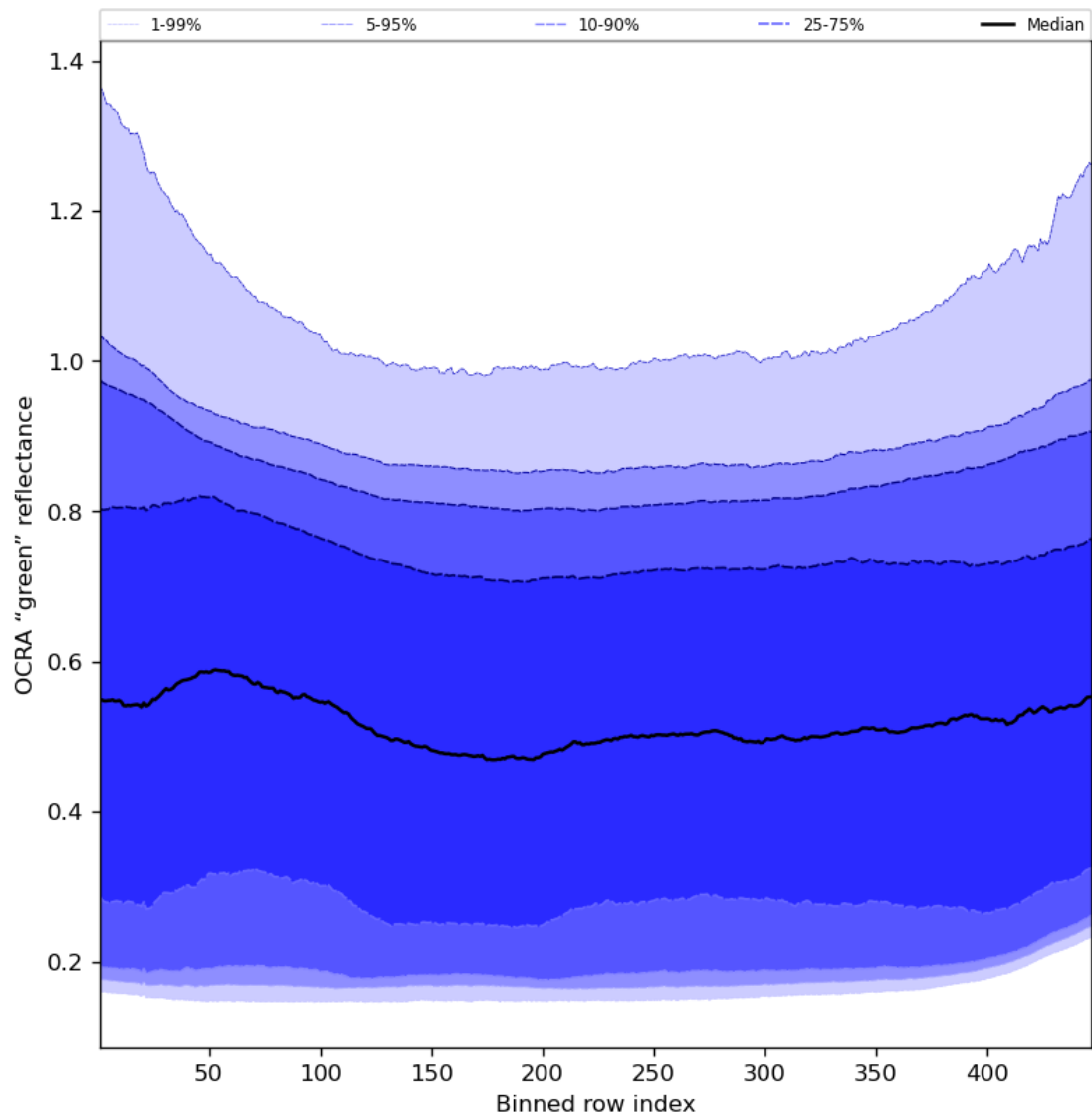
Figure 68: Along track statistics of "OCRA "green" reflectance" for 2024-03-10 to 2024-03-12
