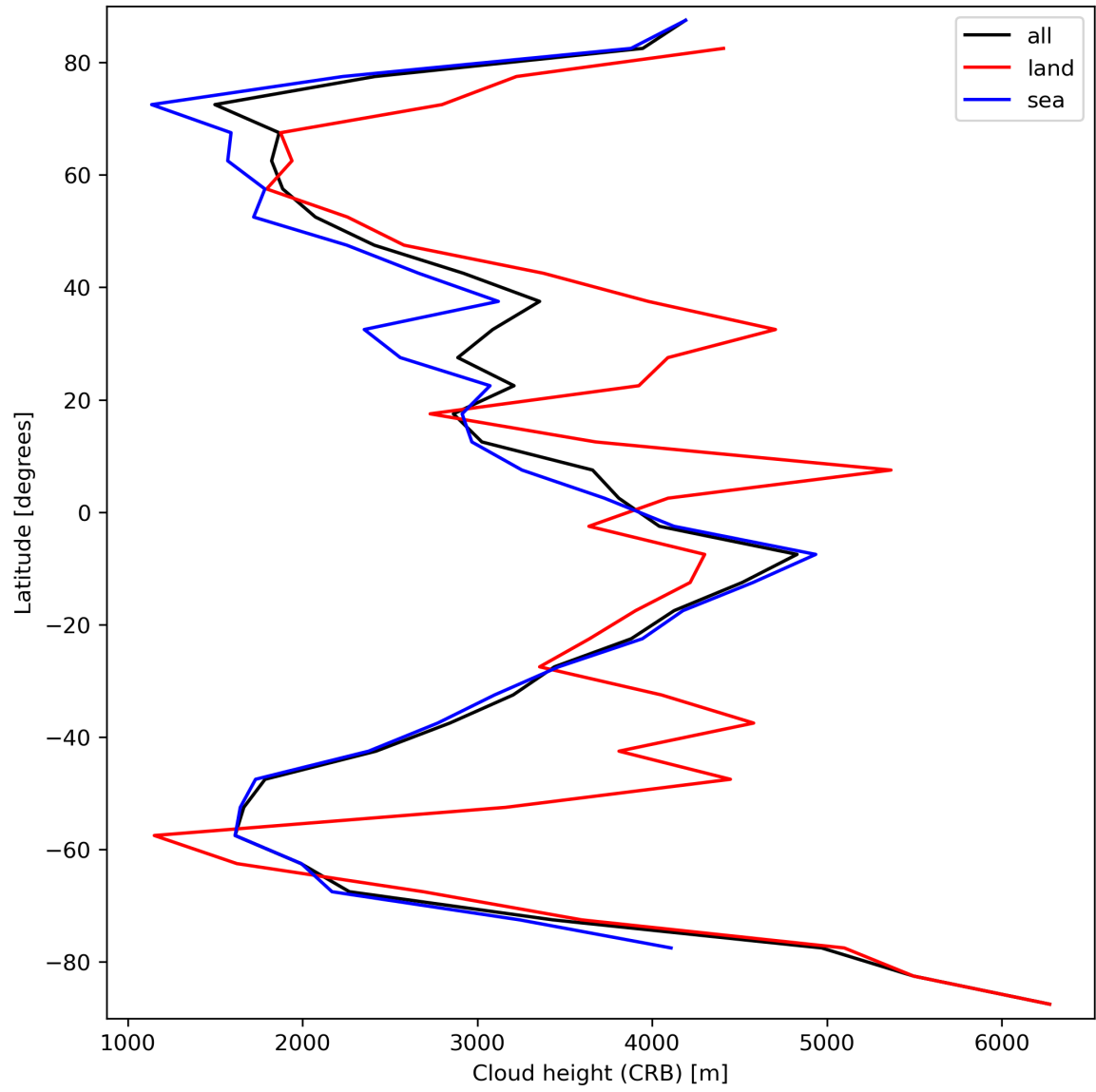
Figure 27: Zonal average of “Cloud height (CRB)” for 2024-03-10 to 2024-03-12.
