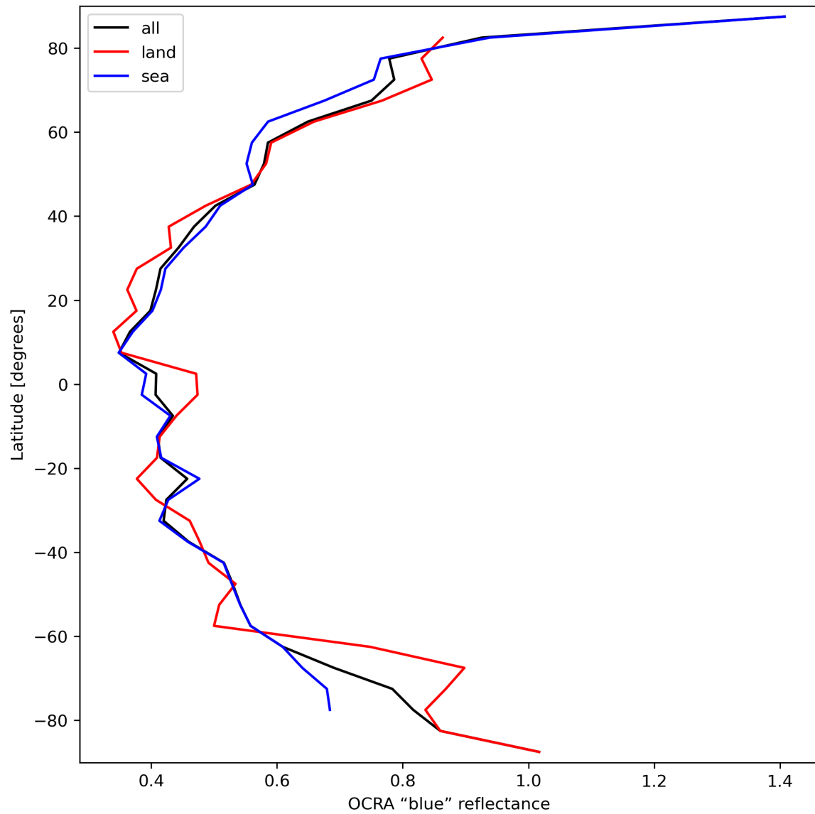
Figure 35: Zonal average of “OCRA “blue” reflectance” for 2024-03-10 to 2024-03-12.
