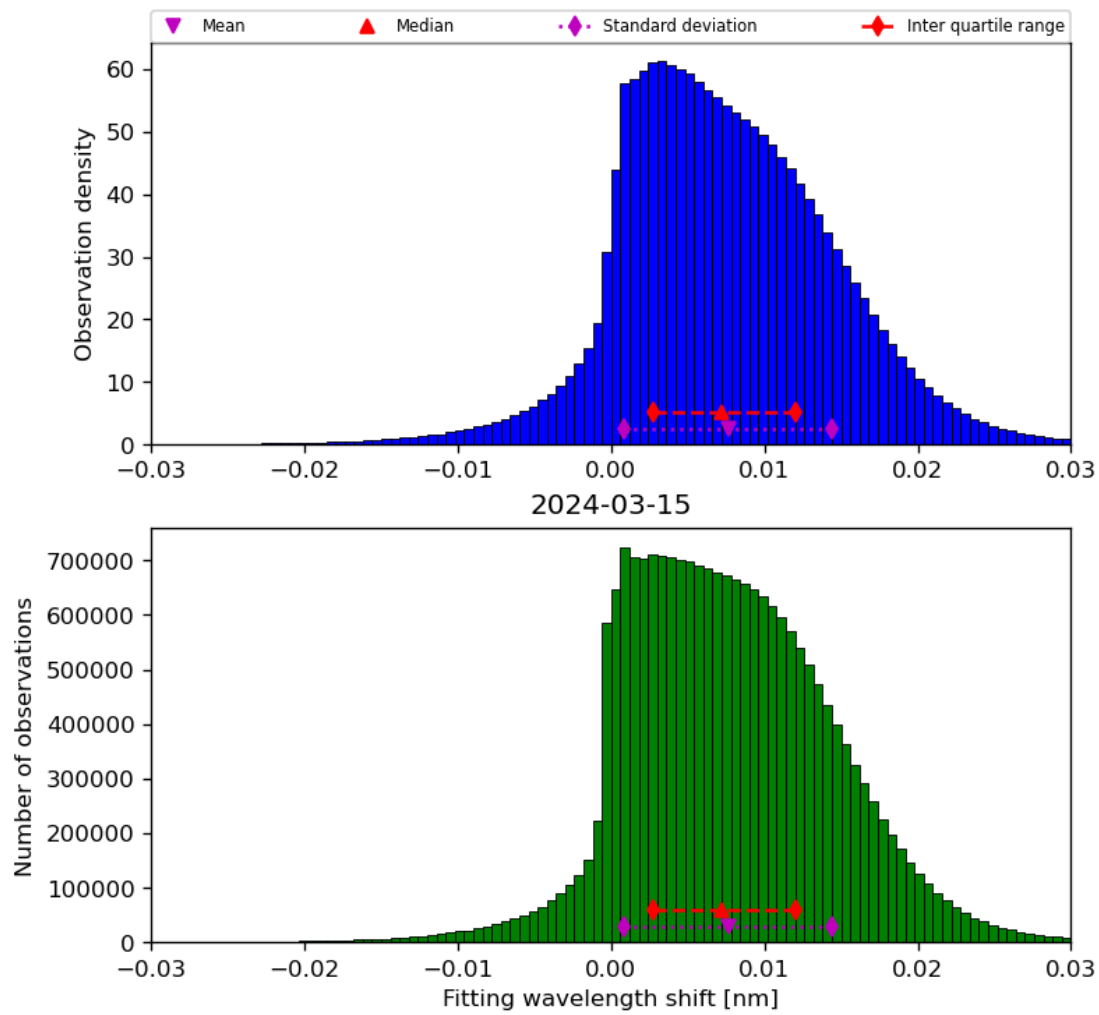
Figure 49: Histogram of “Fitting wavelength shift” for 2024-03-14 to 2024-03-16
