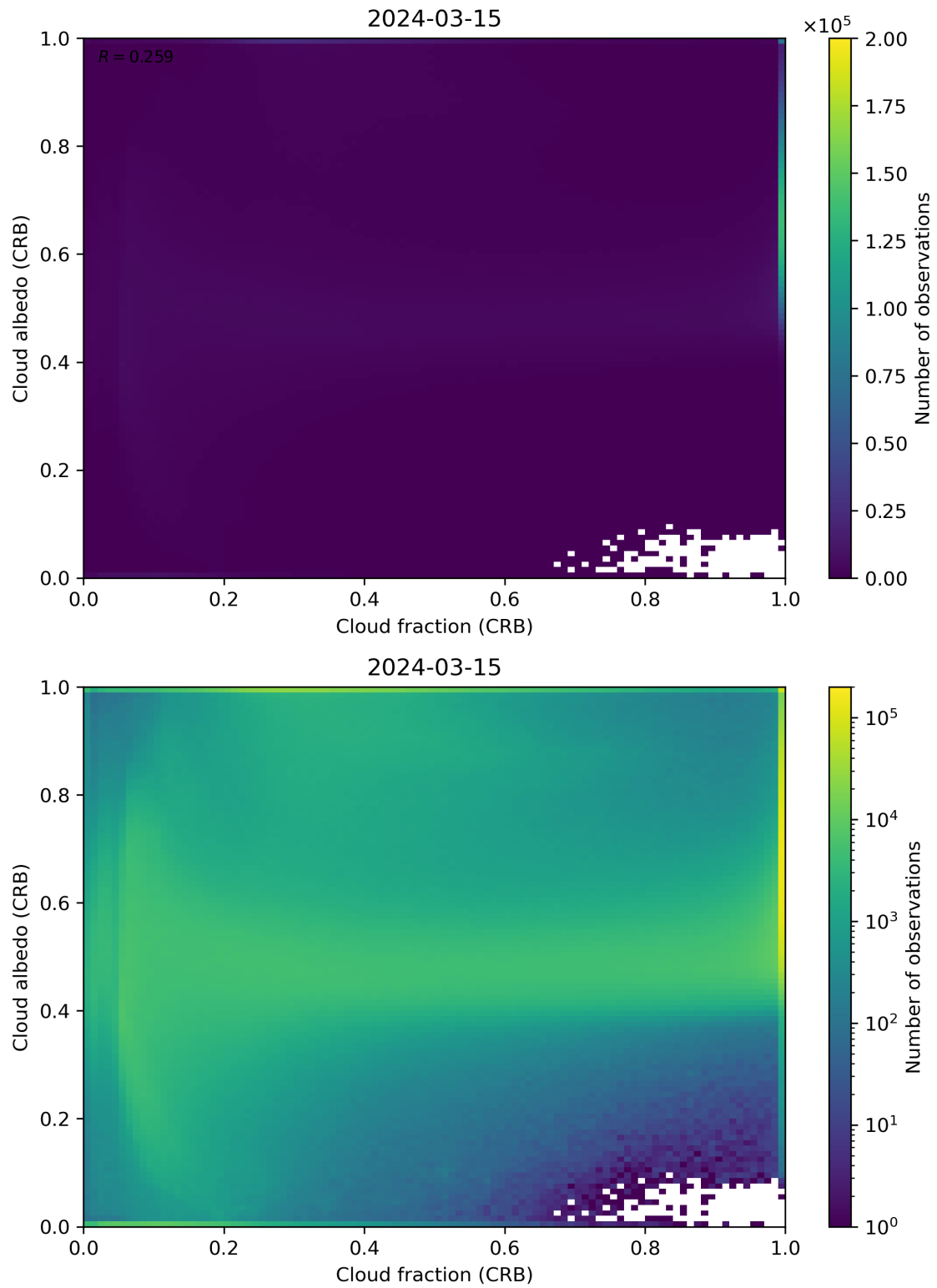
Figure 77: Scatter density plot of “Cloud fraction (CRB)” against “Cloud albedo (CRB)” for 2024-03-14 to 2024-03-16.
