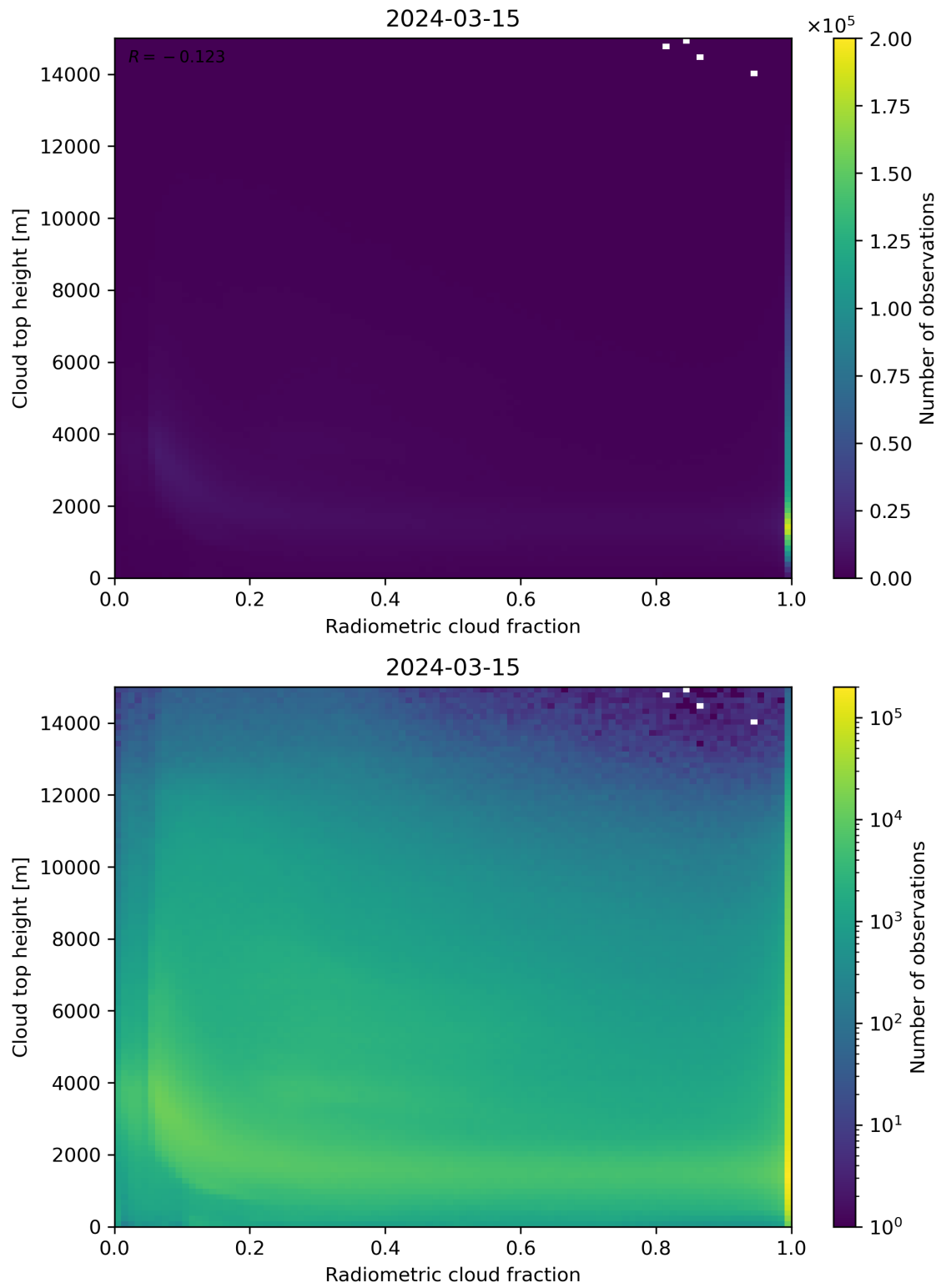
Figure 76: Scatter density plot of “Radiometric cloud fraction” against “Cloud top height” for 2024-03-14 to 2024-03-16.
