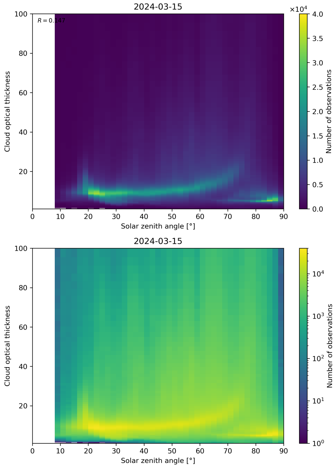
Figure 103: Scatter density plot of “Solar zenith angle” against “Cloud optical thickness” for 2024-03-14 to 2024-03-16.
