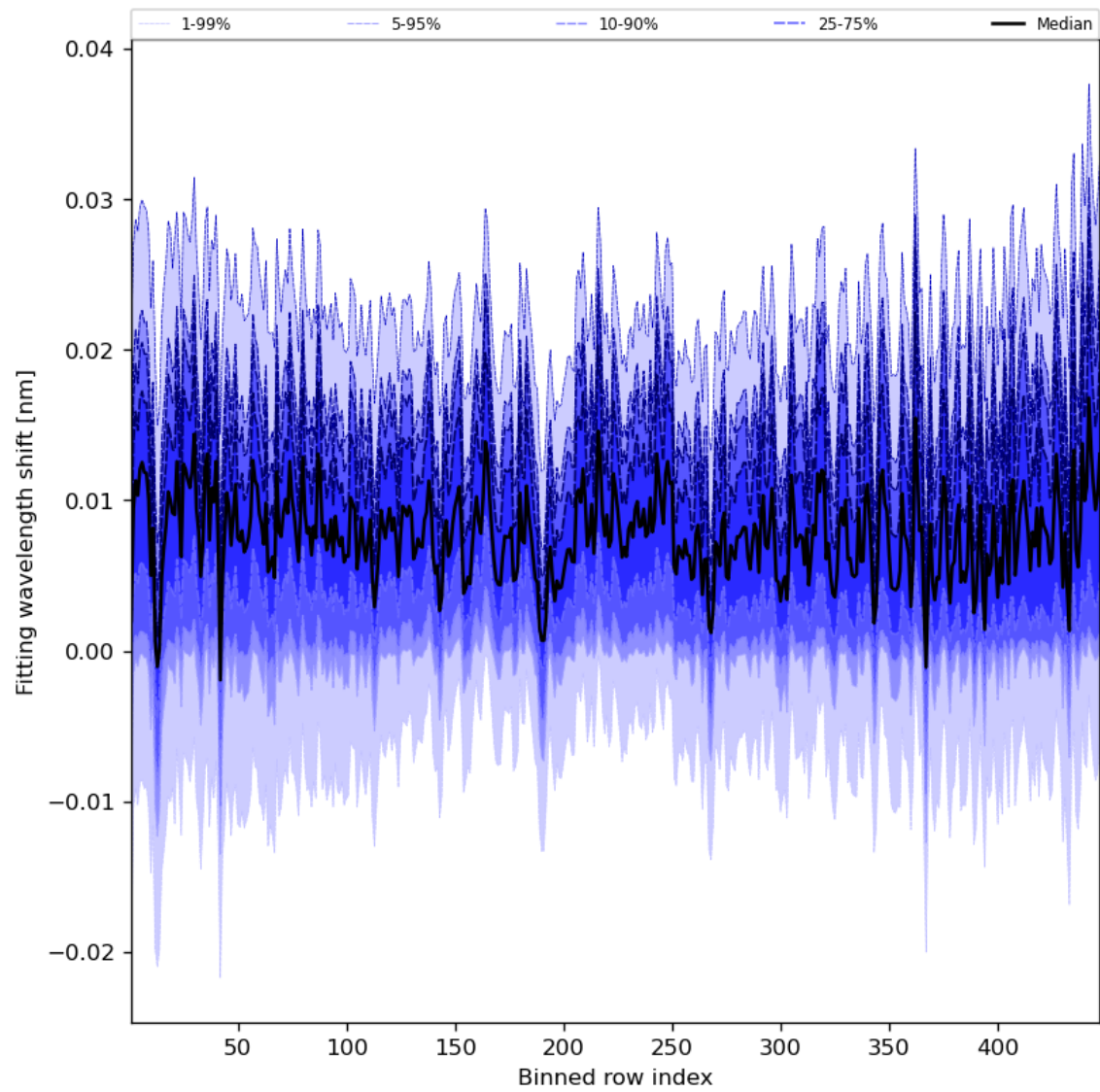
Figure 65: Along track statistics of “Fitting wavelength shift” for 2024-03-14 to 2024-03-16
