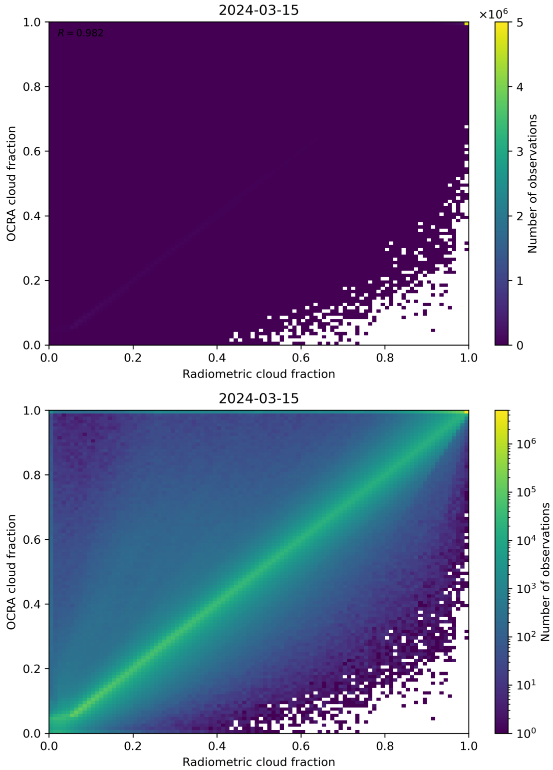
Figure 72: Scatter density plot of “Radiometric cloud fraction” against “OCRA cloud fraction” for 2024-03-14 to 2024-03-16.
