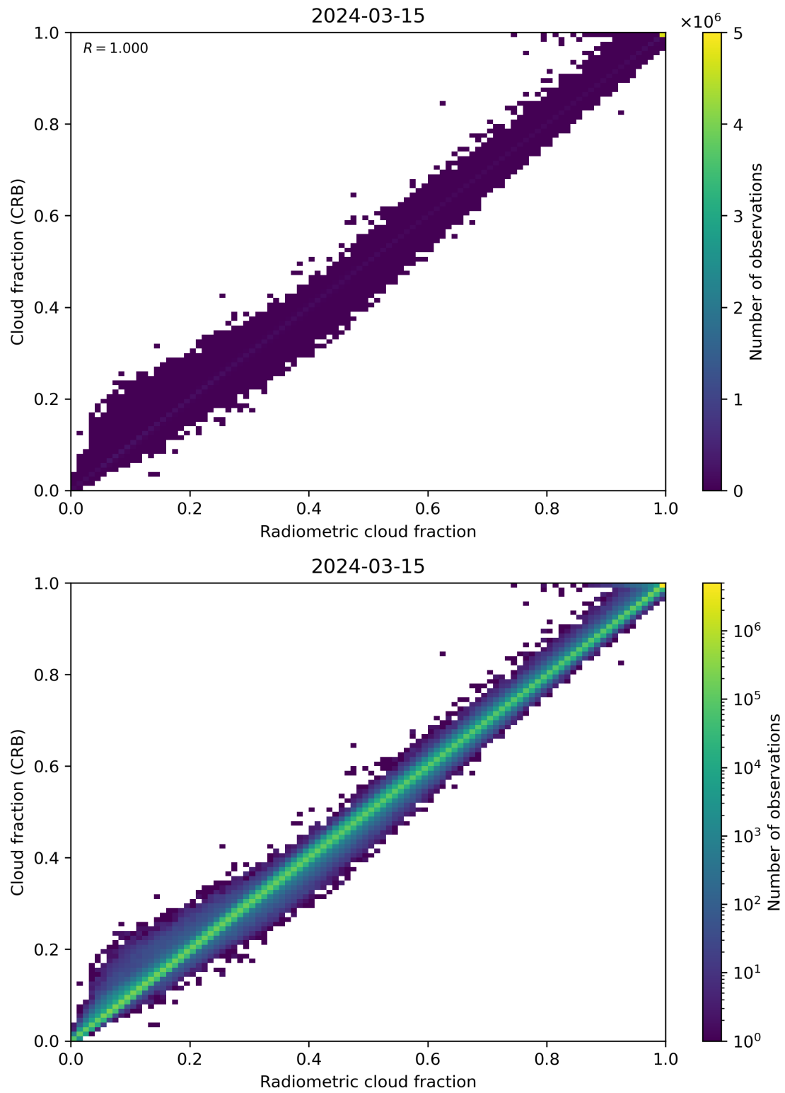
Figure 73: Scatter density plot of “Radiometric cloud fraction” against “Cloud fraction (CRB)” for 2024-03-14 to 2024-03-16.
