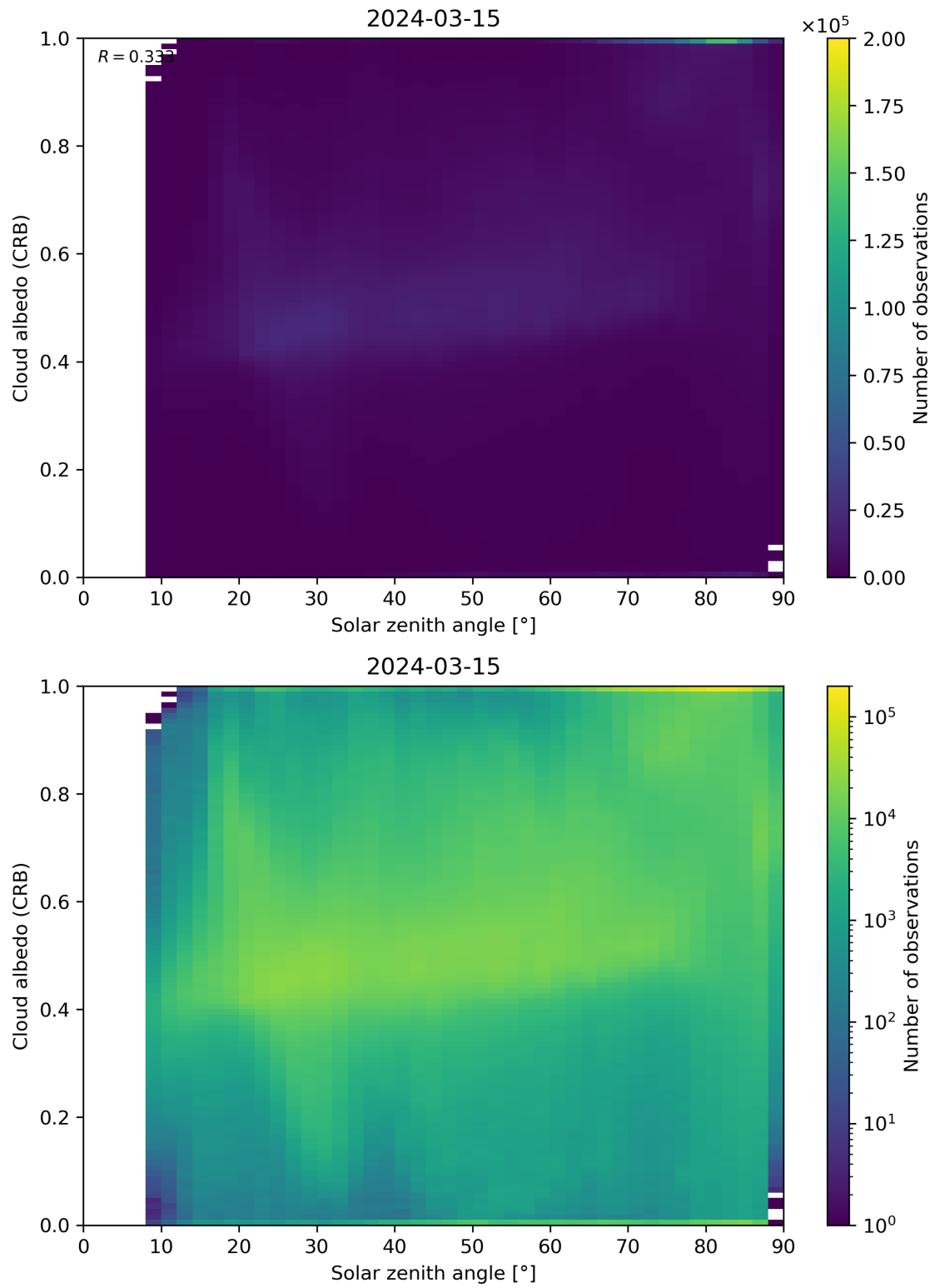
Figure 98: Scatter density plot of “Solar zenith angle” against “Cloud albedo (CRB)” for 2024-03-14 to 2024-03-16.
