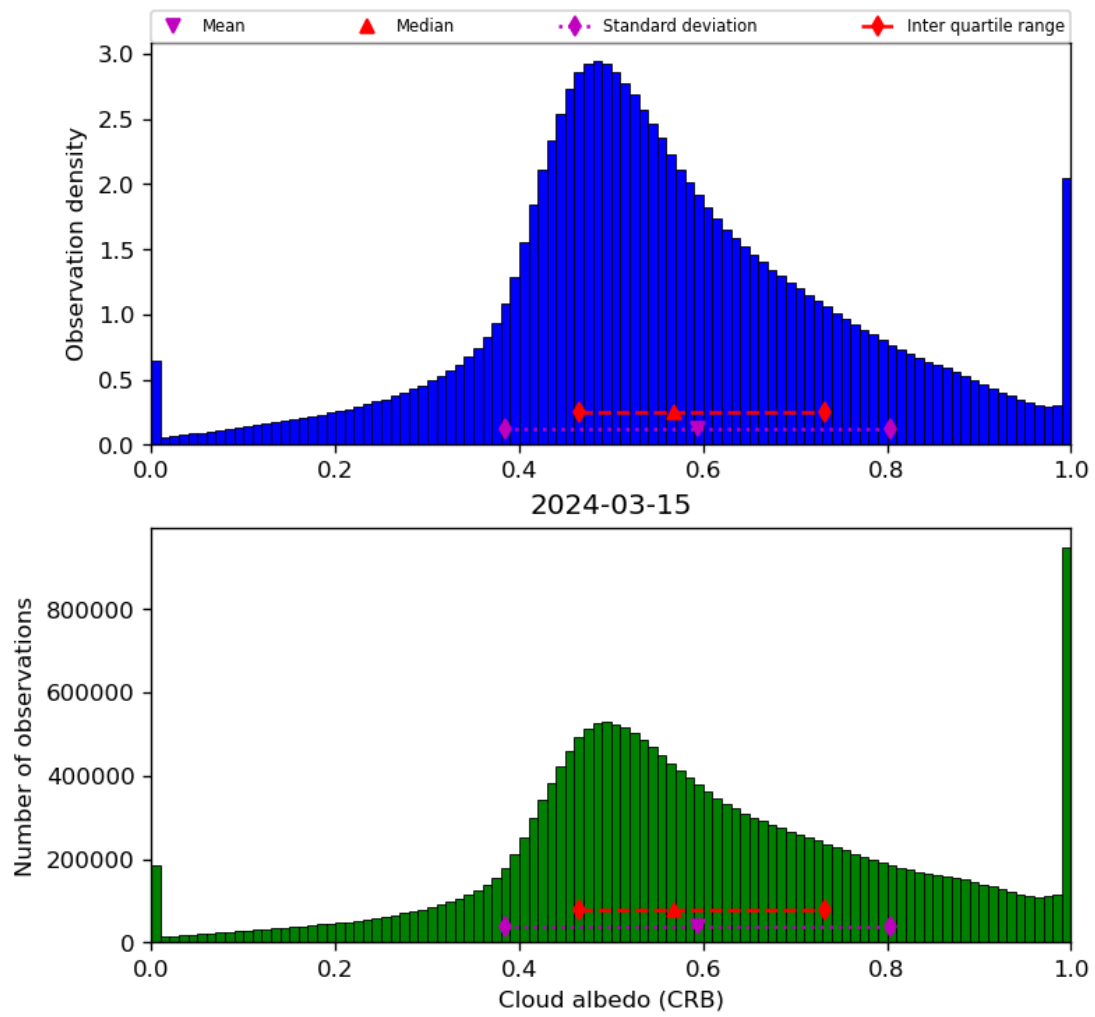
Figure 44: Histogram of “Cloud albedo (CRB)” for 2024-03-14 to 2024-03-16
