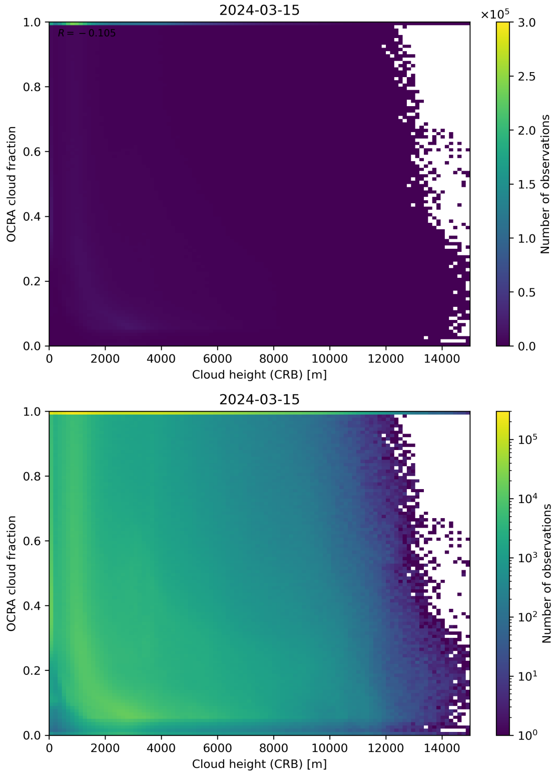
Figure 81: Scatter density plot of “Cloud height (CRB)” against “OCRA cloud fraction” for 2024-03-14 to 2024-03-16.
