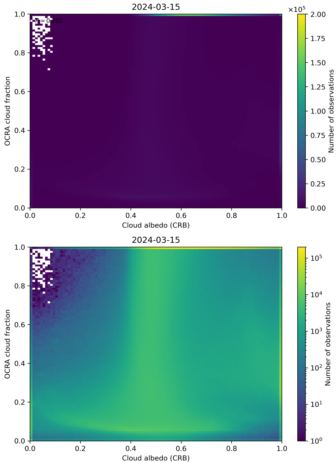
Figure 70: Scatter density plot of “Cloud albedo (CRB)” against “OCRA cloud fraction” for 2024-03-14 to 2024-03-16.
