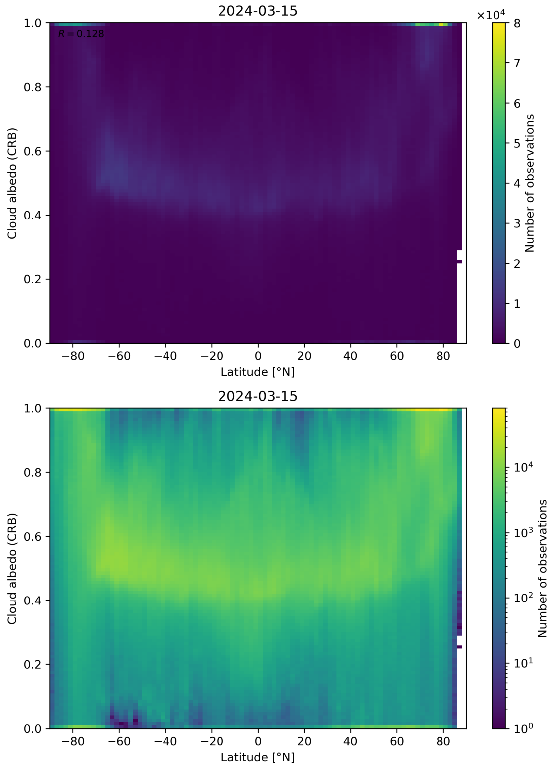
Figure 91: Scatter density plot of “Latitude” against “Cloud albedo (CRB)” for 2024-03-14 to 2024-03-16.
