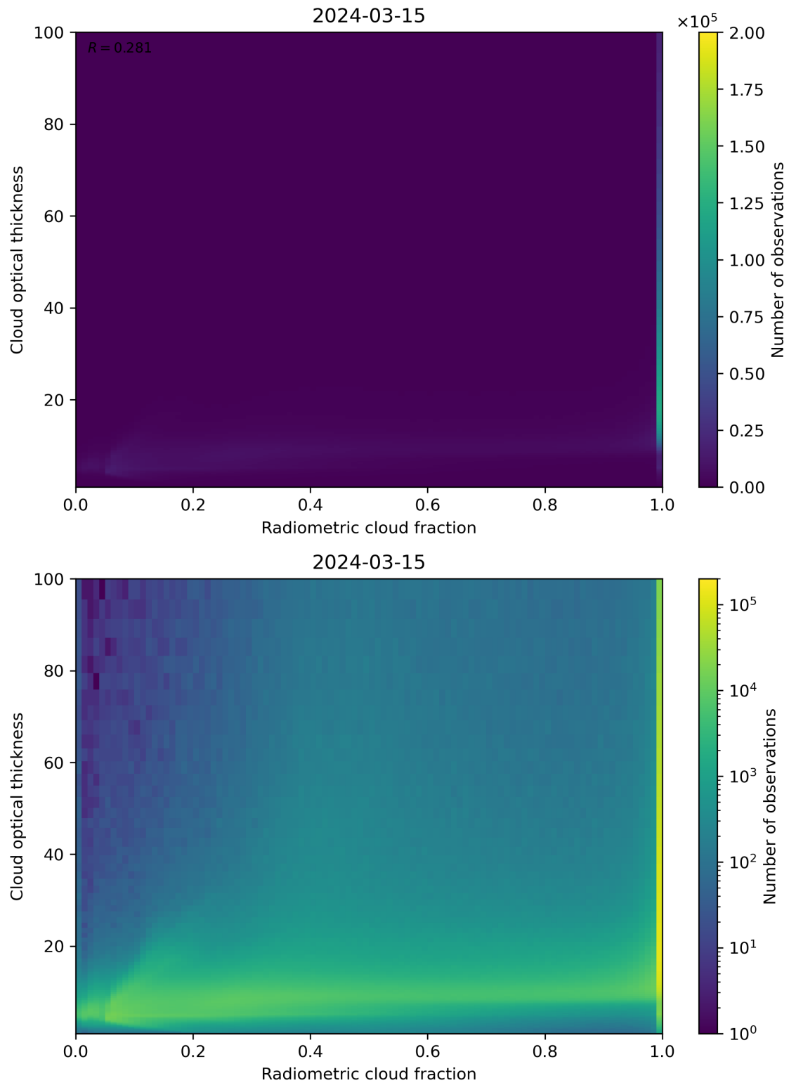
Figure 75: Scatter density plot of “Radiometric cloud fraction” against “Cloud optical thickness” for 2024-03-14 to 2024-03-16.
