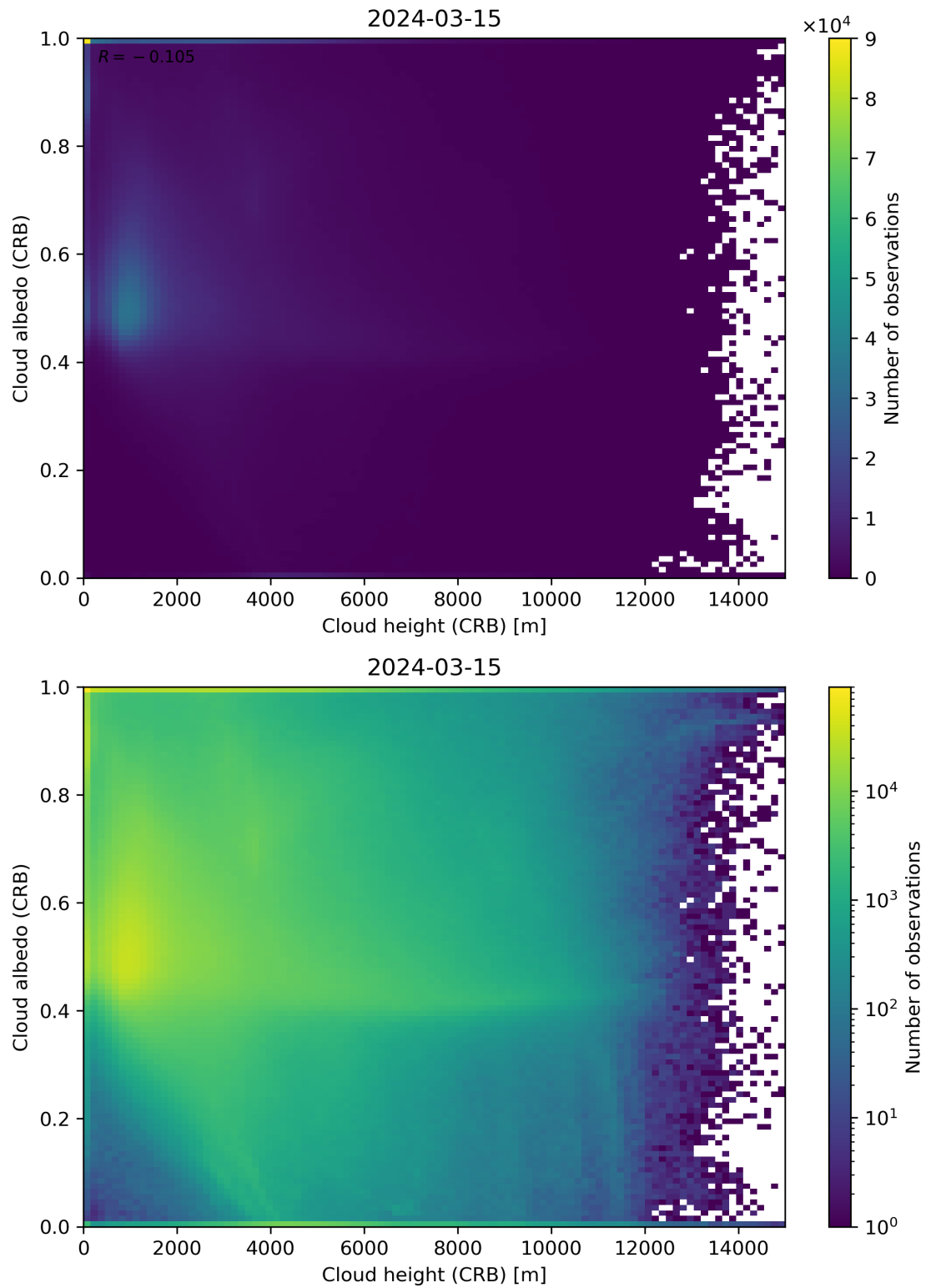
Figure 80: Scatter density plot of “Cloud height (CRB)” against “Cloud albedo (CRB)” for 2024-03-14 to 2024-03-16.
