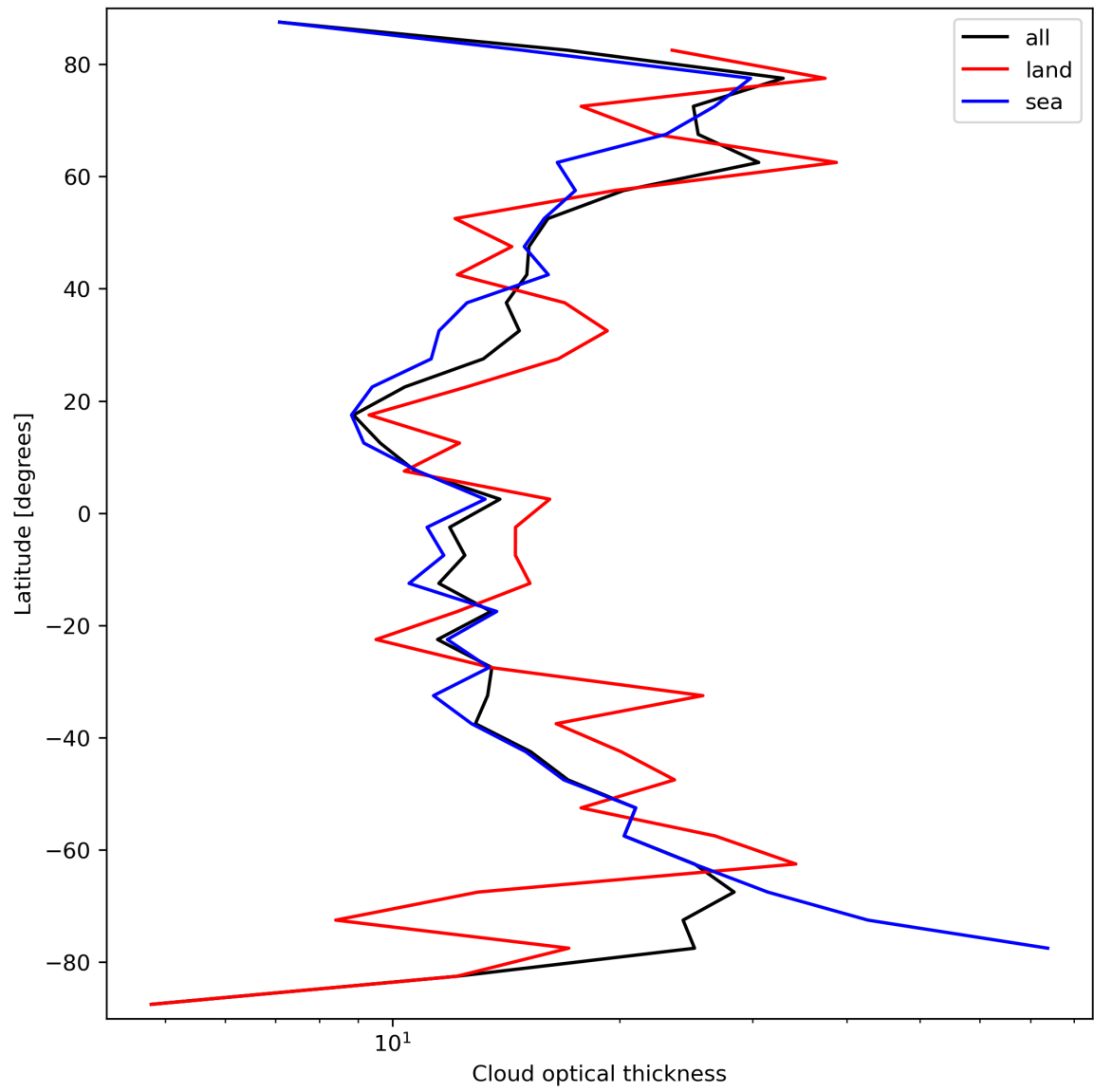
Figure 25: Zonal average of “Cloud optical thickness” for 2024-03-14 to 2024-03-16.
