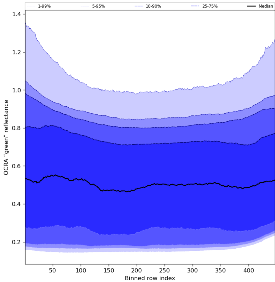
Figure 68: Along track statistics of "OCRA "green" reflectance" for 2024-03-14 to 2024-03-16
