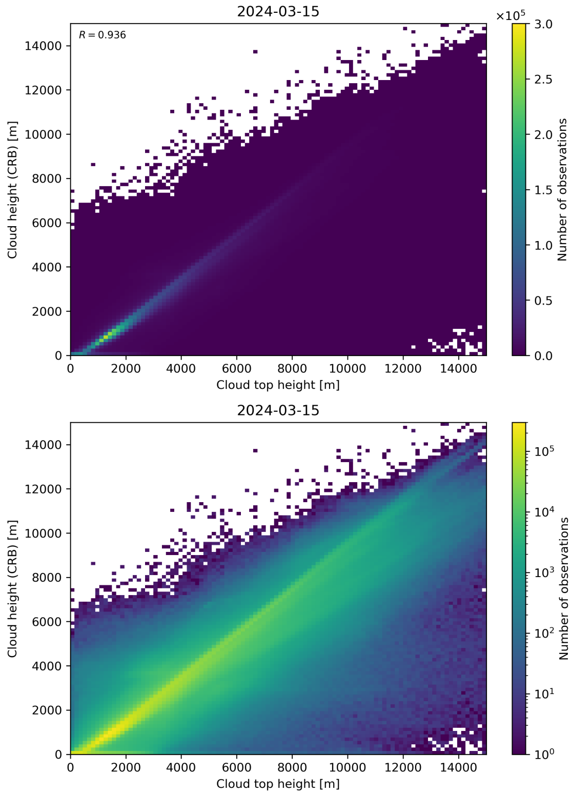
Figure 89: Scatter density plot of “Cloud top height” against “Cloud height (CRB)” for 2024-03-14 to 2024-03-16.
