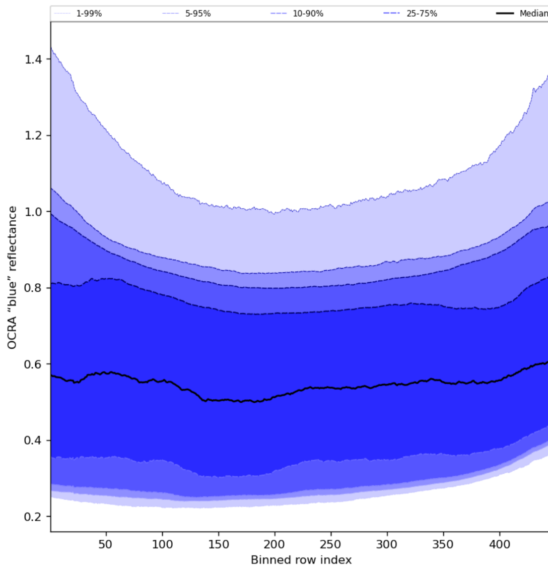
Figure 67: Along track statistics of “OCRA “blue” reflectance” for 2024-03-14 to 2024-03-16
