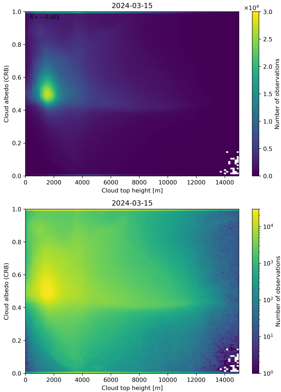
Figure 86: Scatter density plot of “Cloud top height” against “Cloud albedo (CRB)” for 2024-03-14 to 2024-03-16.
