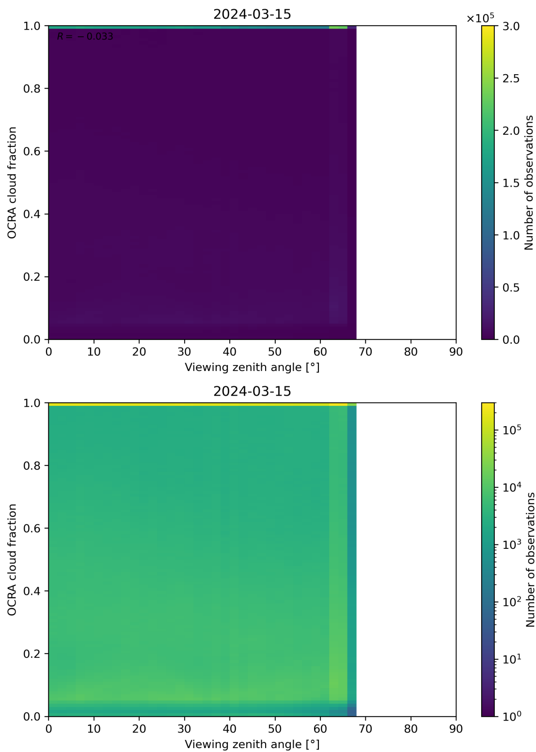
Figure 108: Scatter density plot of “Viewing zenith angle” against “OCRA cloud fraction” for 2024-03-14 to 2024-03-16.
