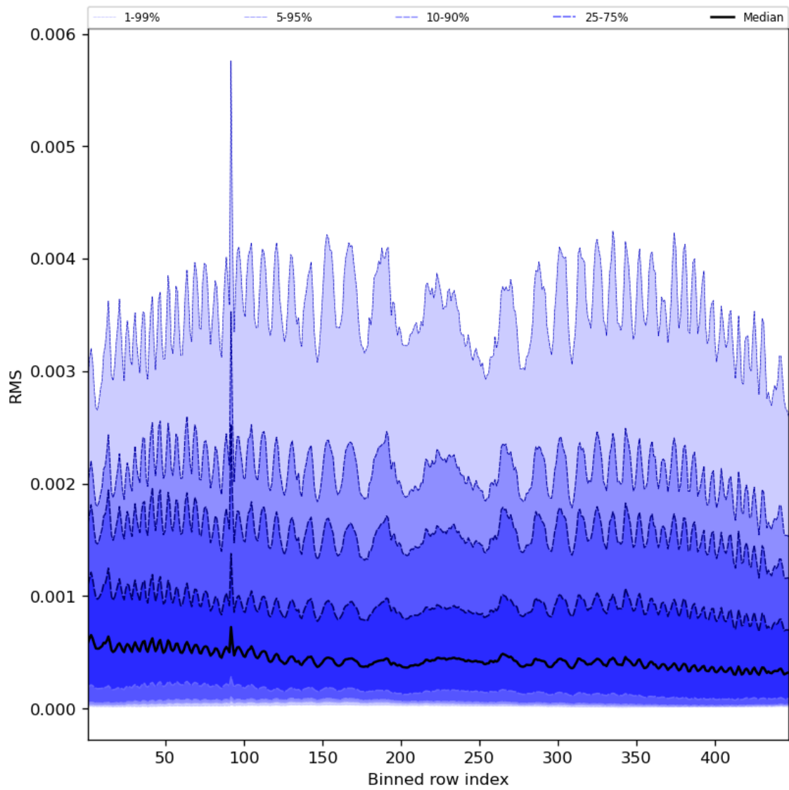
Figure 63: Along track statistics of “RMS” for 2024-03-14 to 2024-03-16
