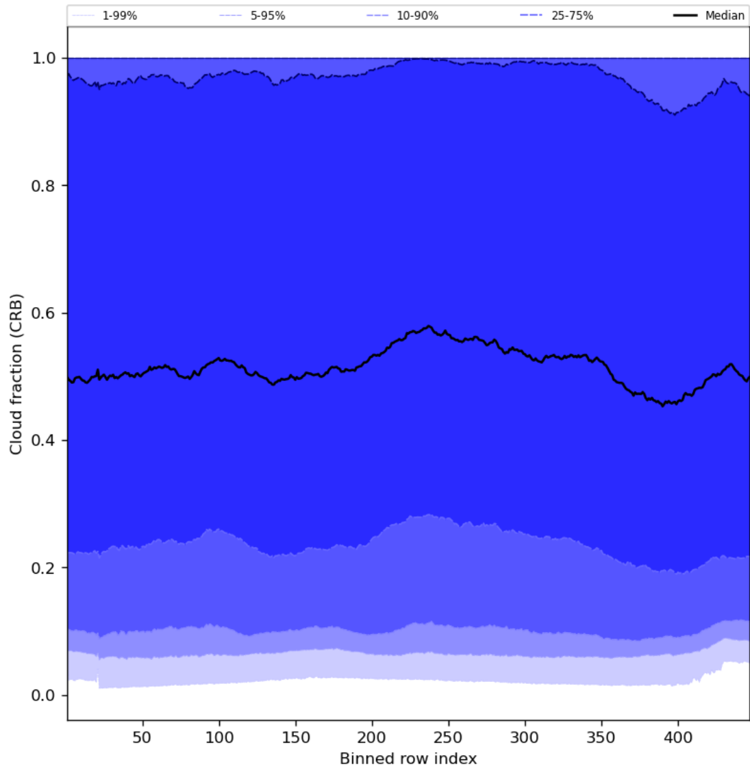
Figure 58: Along track statistics of “Cloud fraction (CRB)” for 2024-03-14 to 2024-03-16
