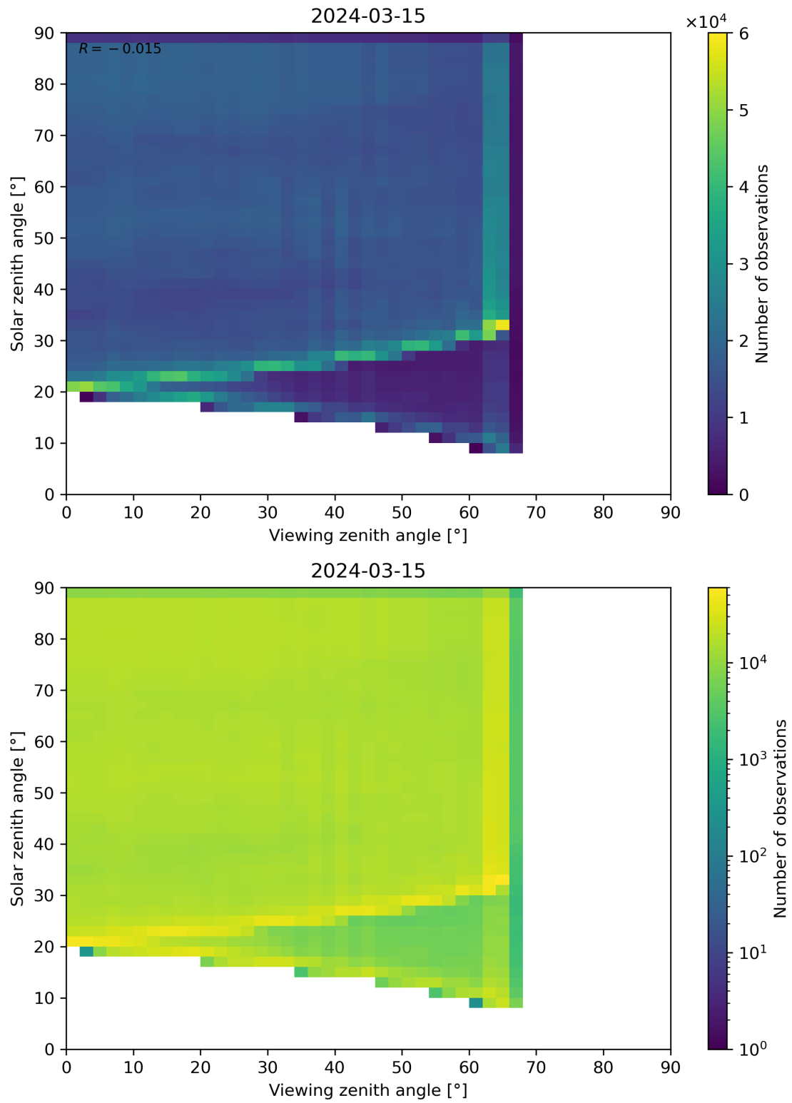
Figure 114: Scatter density plot of “Viewing zenith angle” against “Solar zenith angle” for 2024-03-14 to 2024-03-16.
