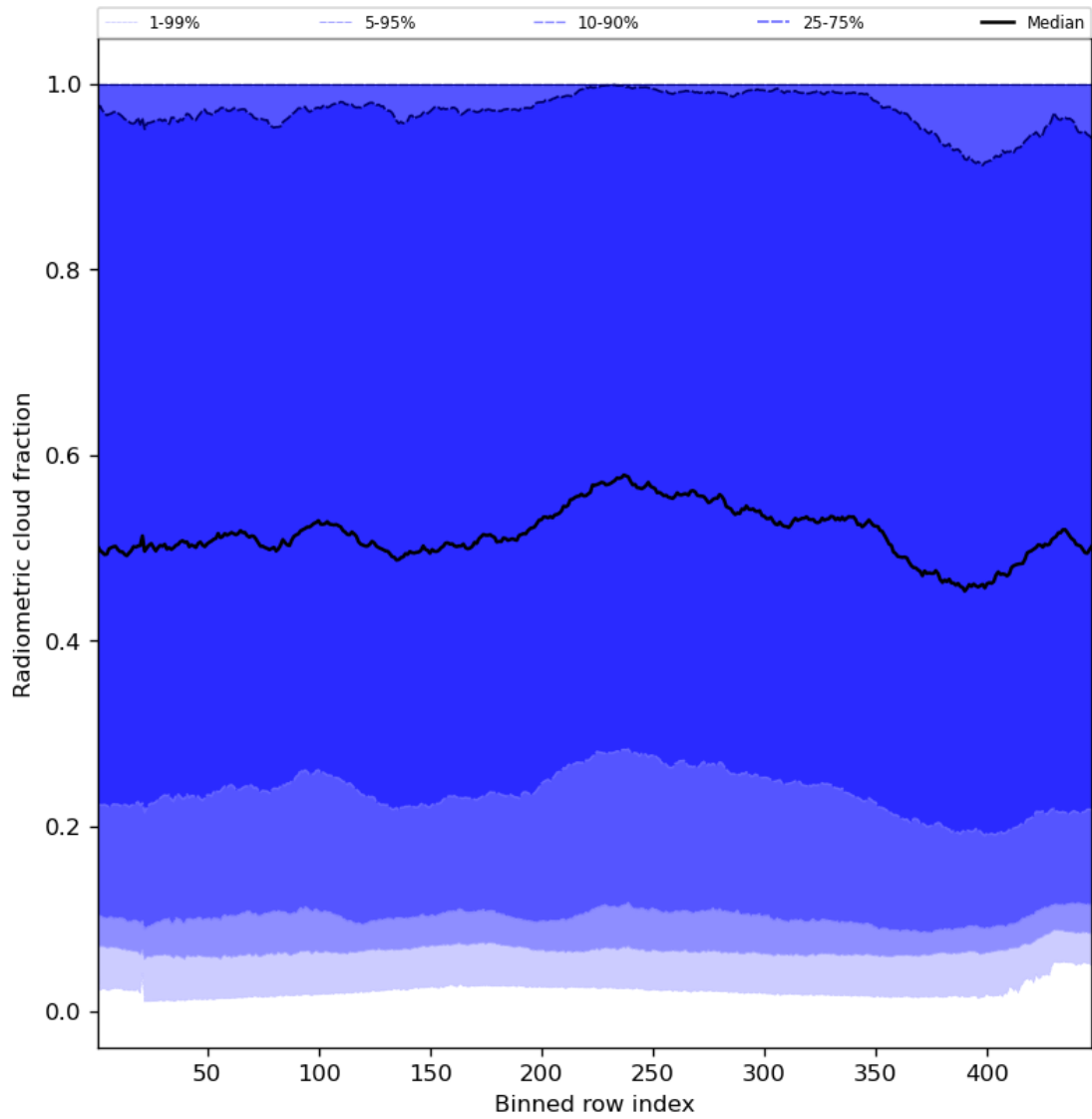
Figure 55: Along track statistics of “Radiometric cloud fraction” for 2024-03-14 to 2024-03-16
