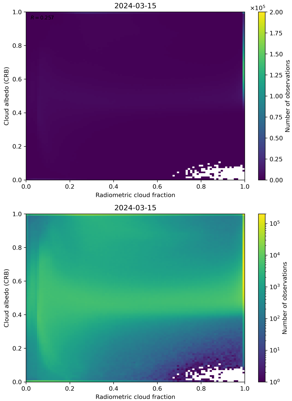
Figure 71: Scatter density plot of “Radiometric cloud fraction” against “Cloud albedo (CRB)” for 2024-03-14 to 2024-03-16.
