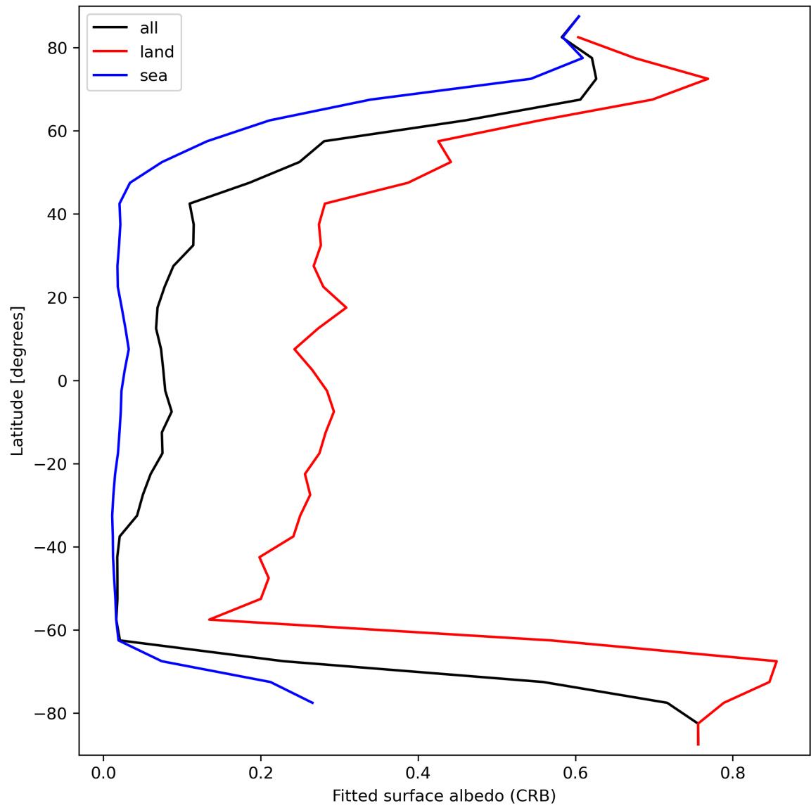
Figure 30: Zonal average of “Fitted surface albedo (CRB)” for 2024-03-14 to 2024-03-16.
