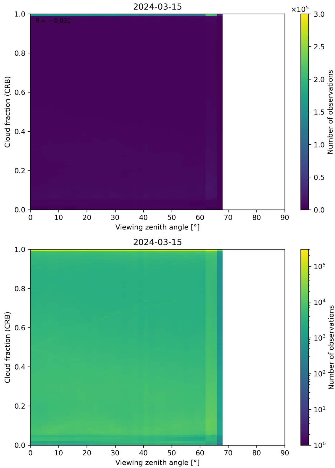
Figure 109: Scatter density plot of “Viewing zenith angle” against “Cloud fraction (CRB)” for 2024-03-14 to 2024-03-16.
