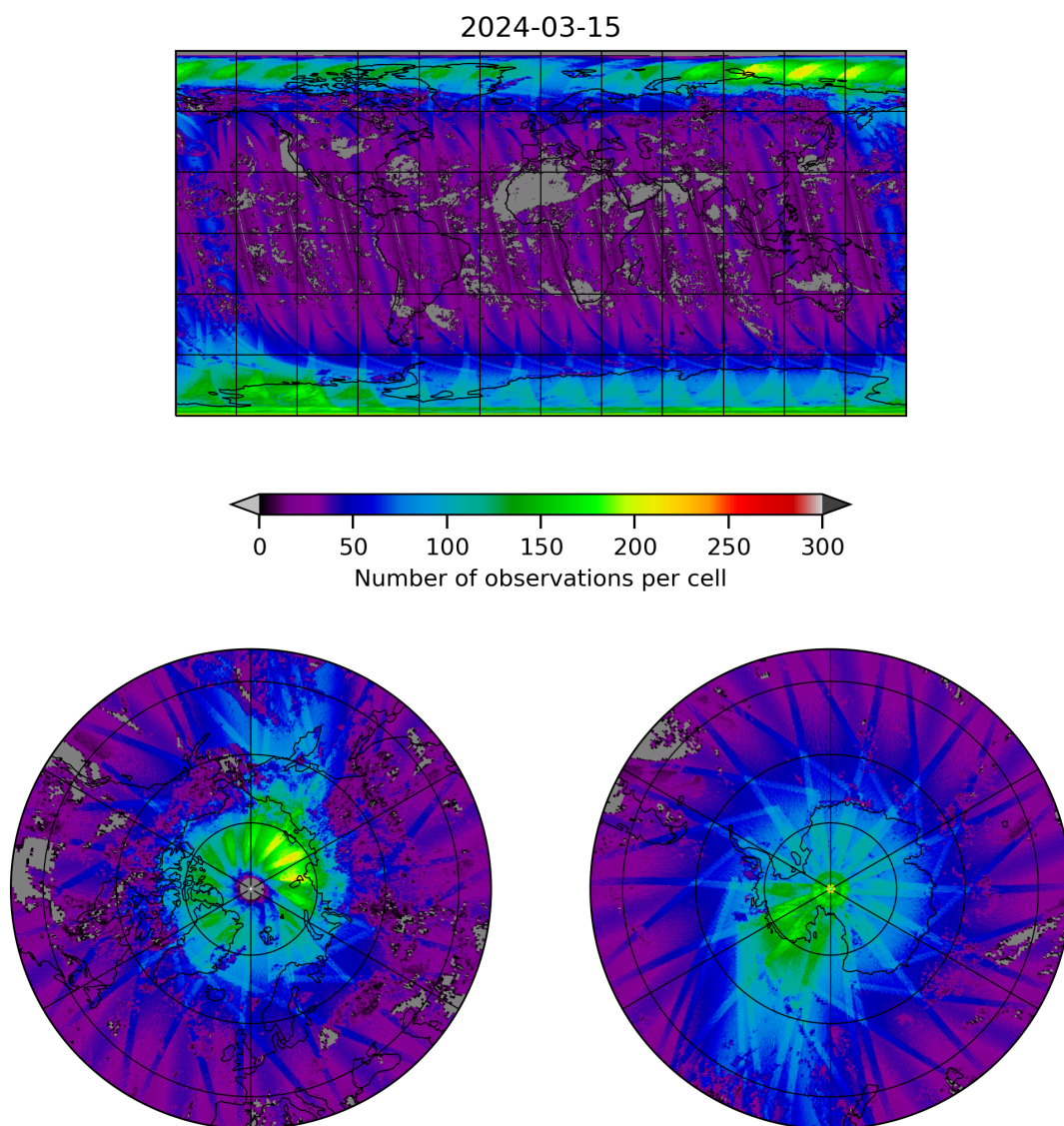
Figure 21: Map of the number of observations for 2024-03-14 to 2024-03-16
