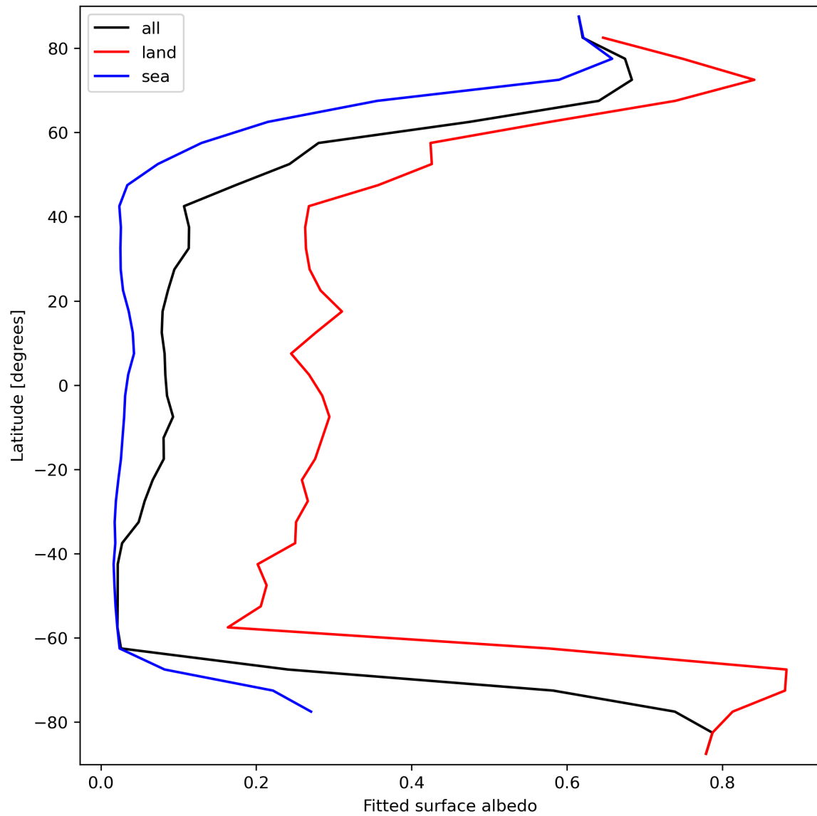
Figure 29: Zonal average of “Fitted surface albedo” for 2024-03-14 to 2024-03-16.
