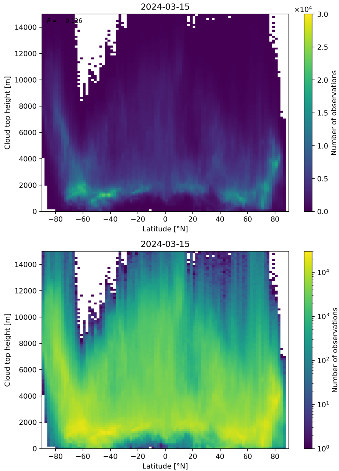
Figure 97: Scatter density plot of “Latitude” against “Cloud top height” for 2024-03-14 to 2024-03-16.
