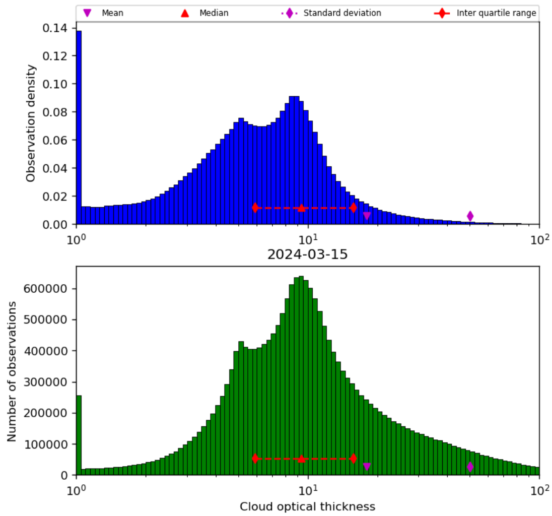
Figure 41: Histogram of “Cloud optical thickness” for 2024-03-14 to 2024-03-16
