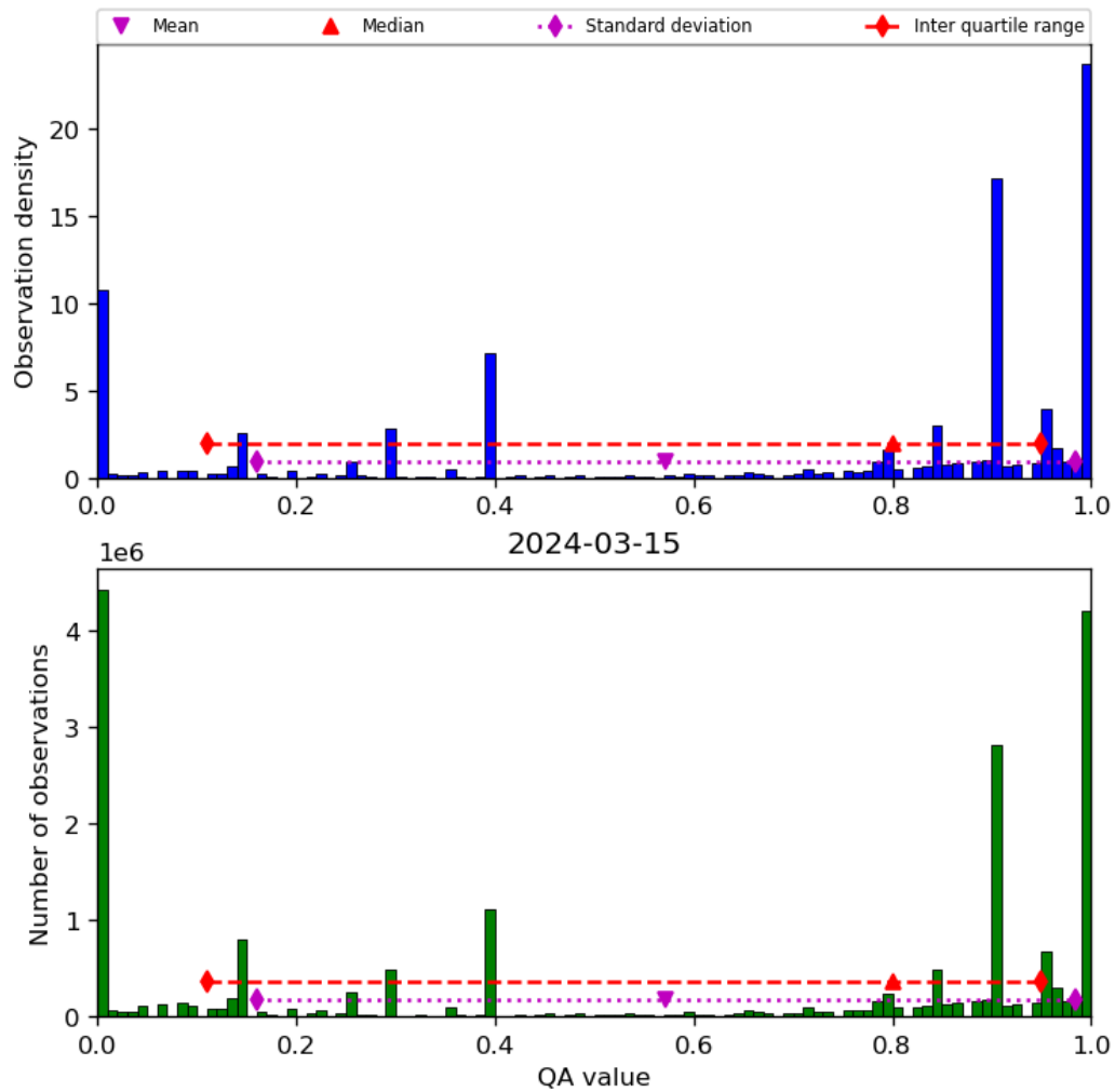
Figure 38: Histogram of “QA value” for 2024-03-14 to 2024-03-16
