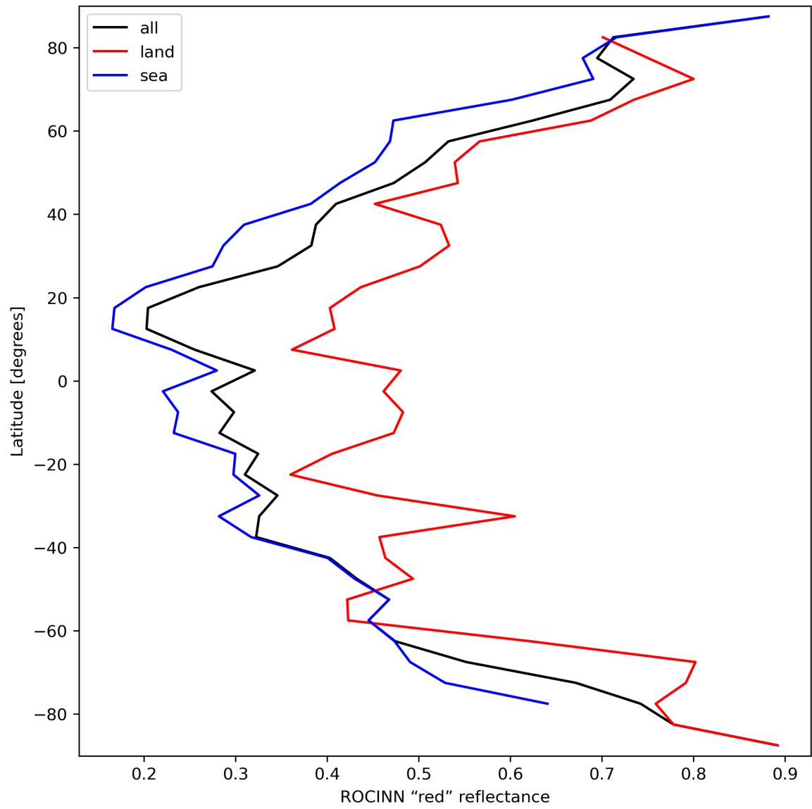
Figure 37: Zonal average of “ROCINN “red” reflectance” for 2024-03-14 to 2024-03-16.
