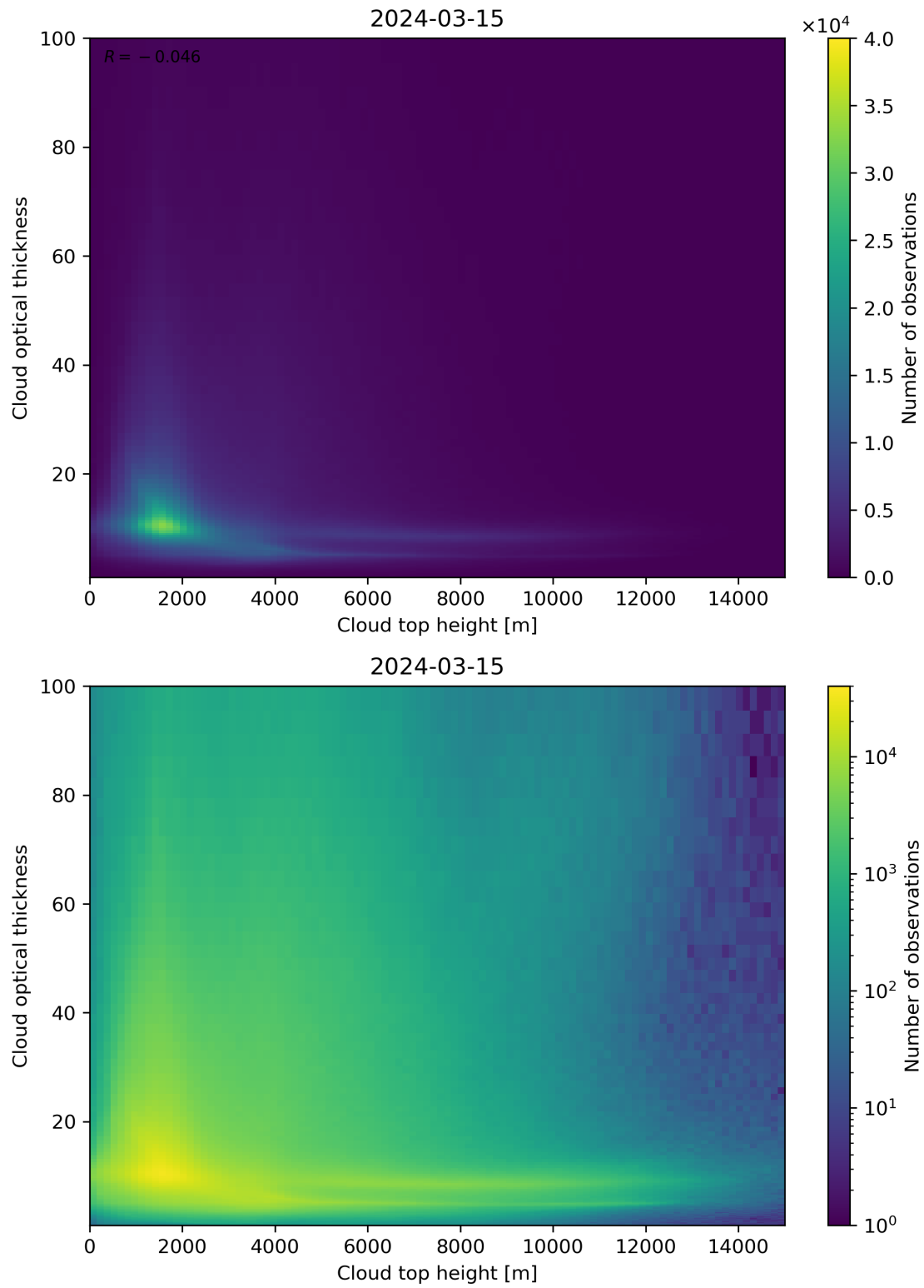
Figure 90: Scatter density plot of “Cloud top height” against “Cloud optical thickness” for 2024-03-14 to 2024-03-16.
