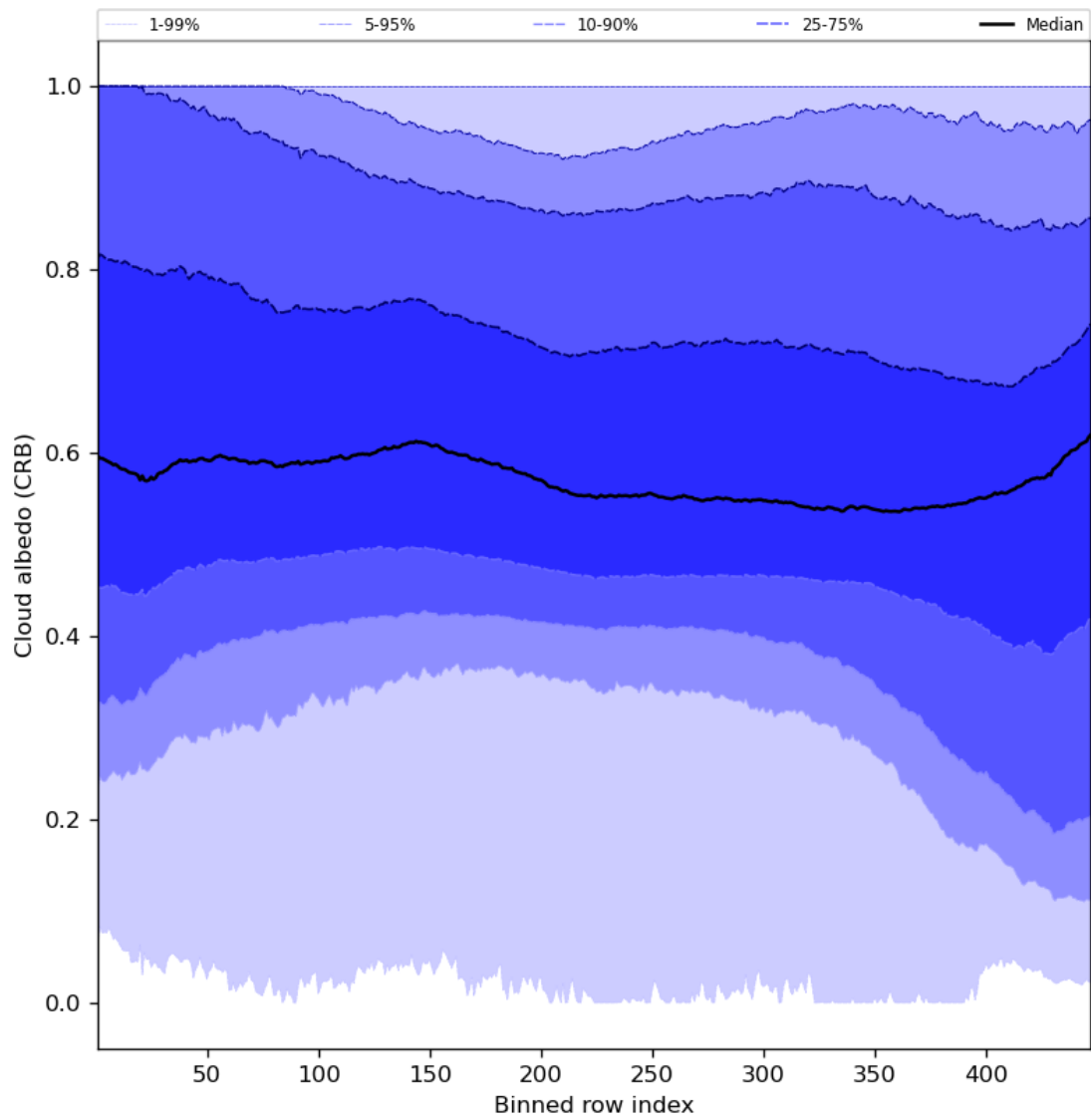
Figure 60: Along track statistics of “Cloud albedo (CRB)” for 2024-03-14 to 2024-03-16
