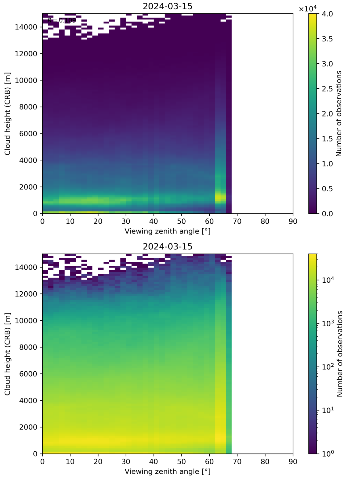
Figure 110: Scatter density plot of “Viewing zenith angle” against “Cloud height (CRB)” for 2024-03-14 to 2024-03-16.
