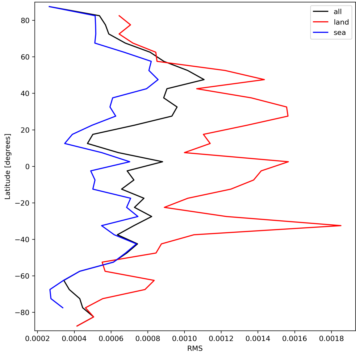
Figure 31: Zonal average of “RMS” for 2024-03-14 to 2024-03-16.
