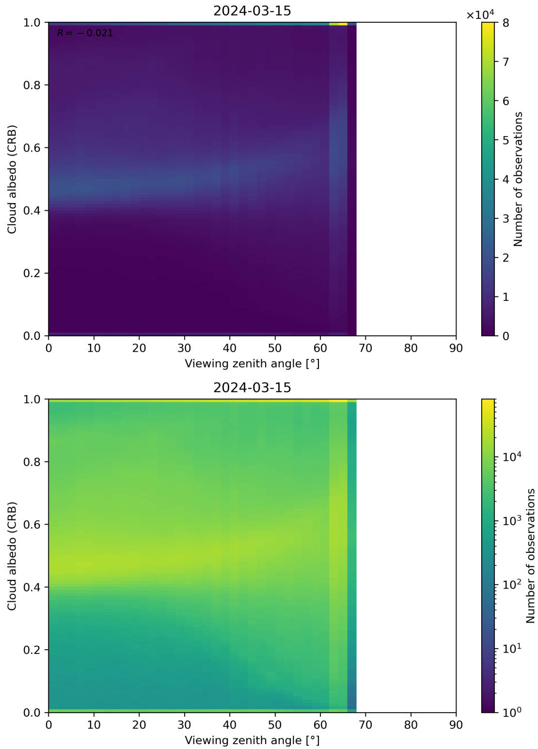
Figure 106: Scatter density plot of “Viewing zenith angle” against “Cloud albedo (CRB)” for 2024-03-14 to 2024-03-16.
