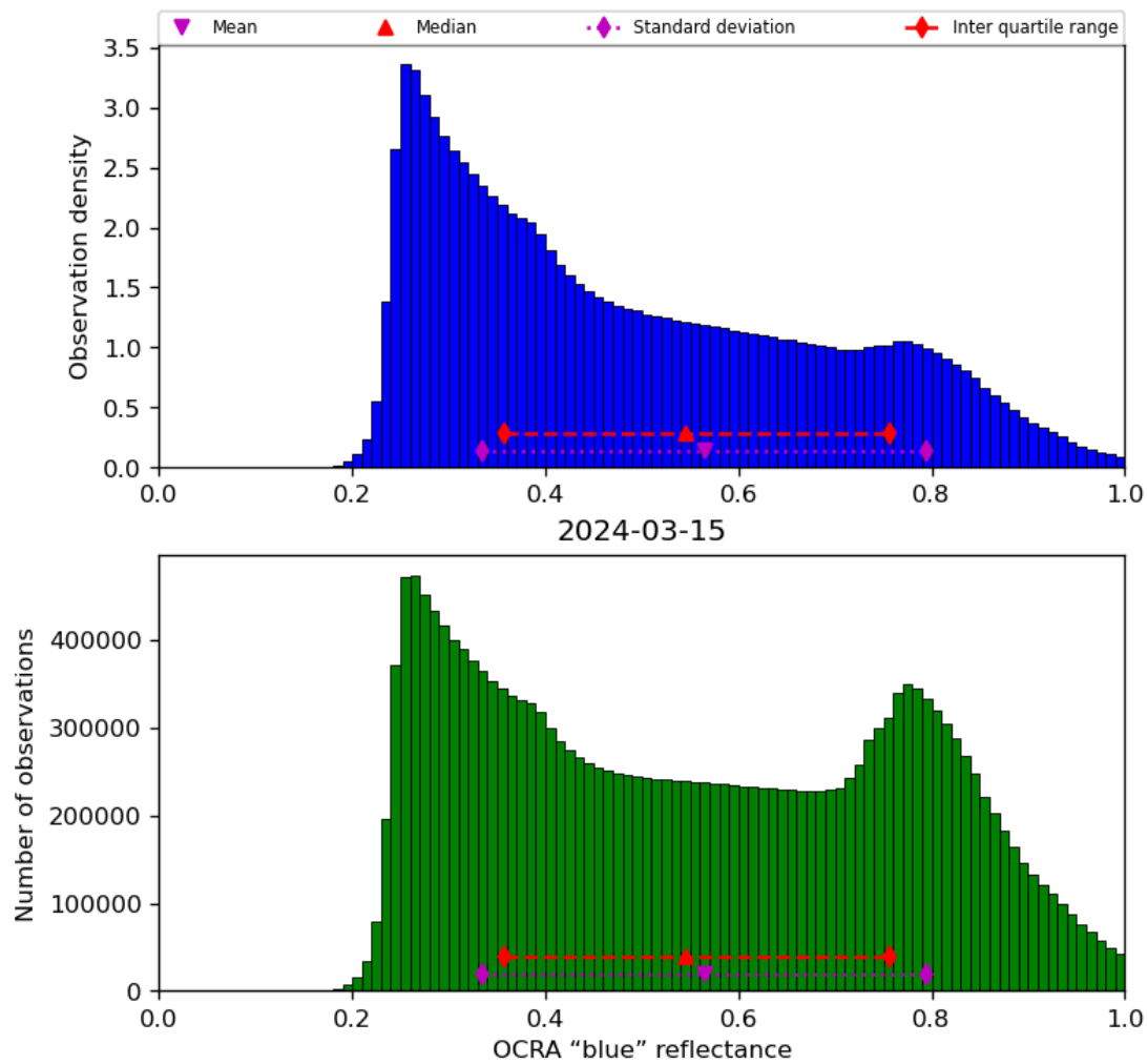
Figure 51: Histogram of “OCRA “blue” reflectance” for 2024-03-14 to 2024-03-16
