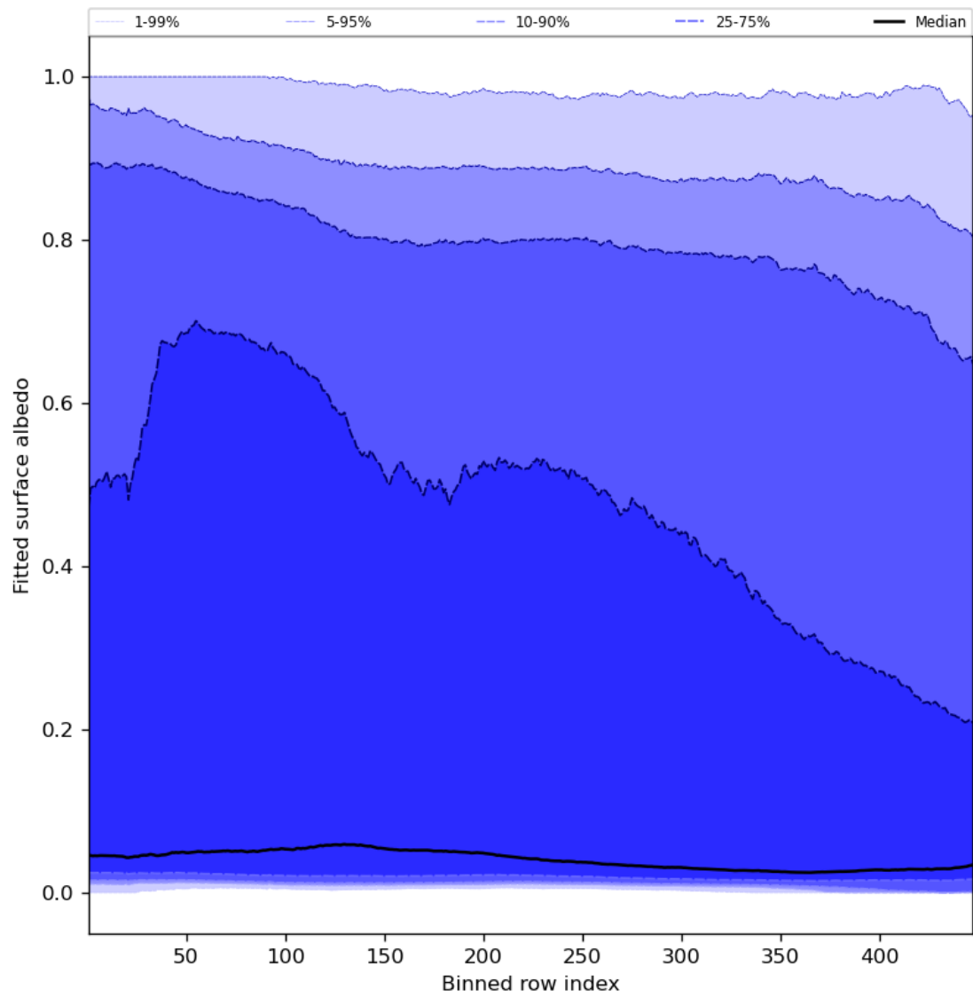
Figure 61: Along track statistics of “Fitted surface albedo” for 2024-03-14 to 2024-03-16
