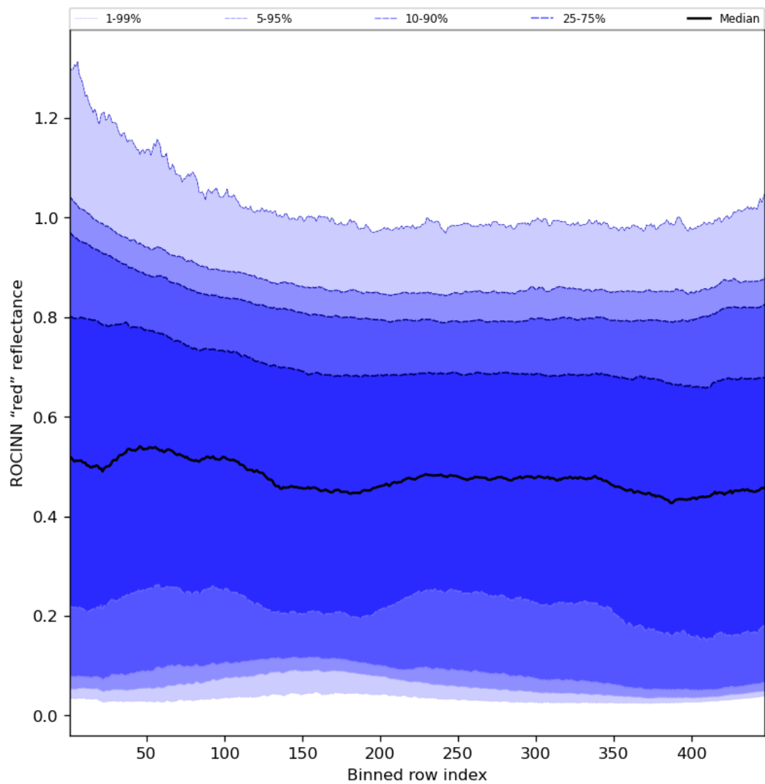
Figure 69: Along track statistics of “ROCINN “red” reflectance” for 2024-03-14 to 2024-03-16
