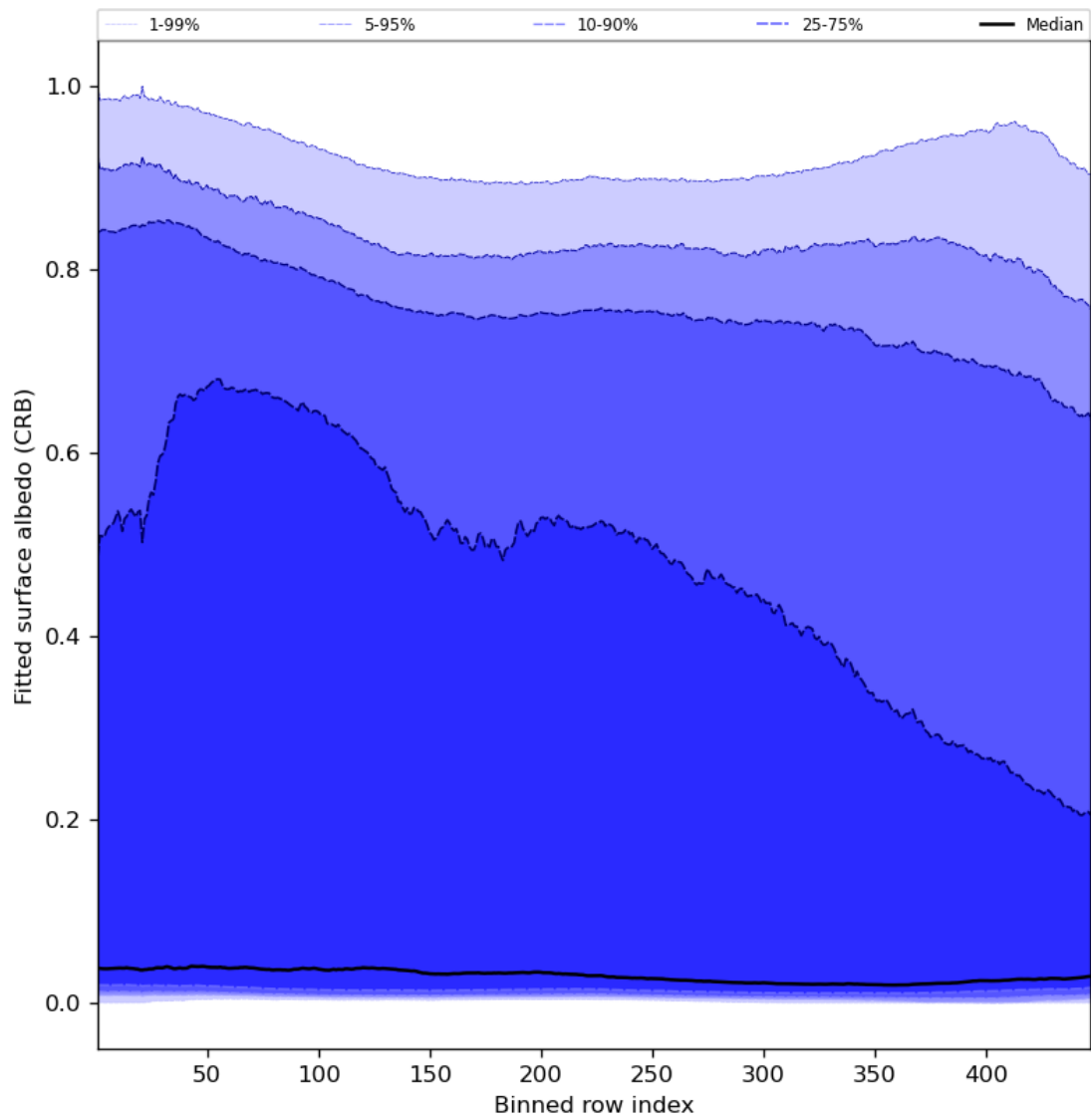
Figure 62: Along track statistics of “Fitted surface albedo (CRB)” for 2024-03-14 to 2024-03-16
