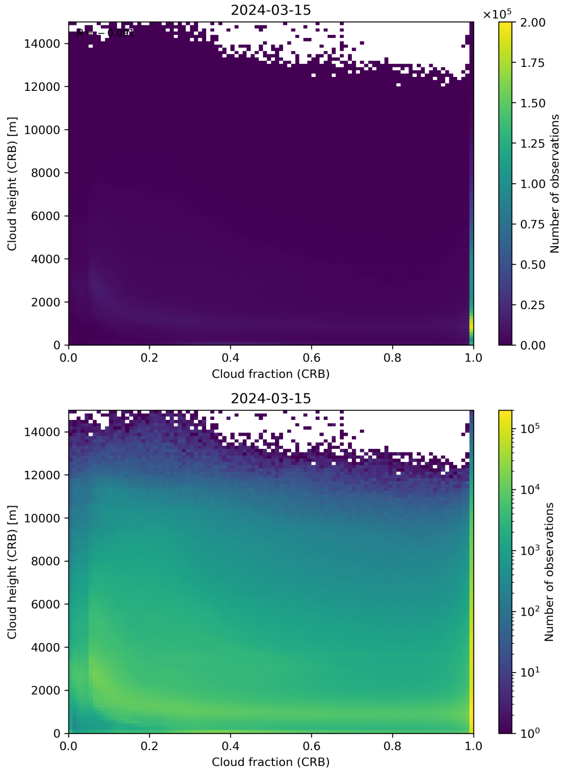
Figure 79: Scatter density plot of “Cloud fraction (CRB)” against “Cloud height (CRB)” for 2024-03-14 to 2024-03-16.
