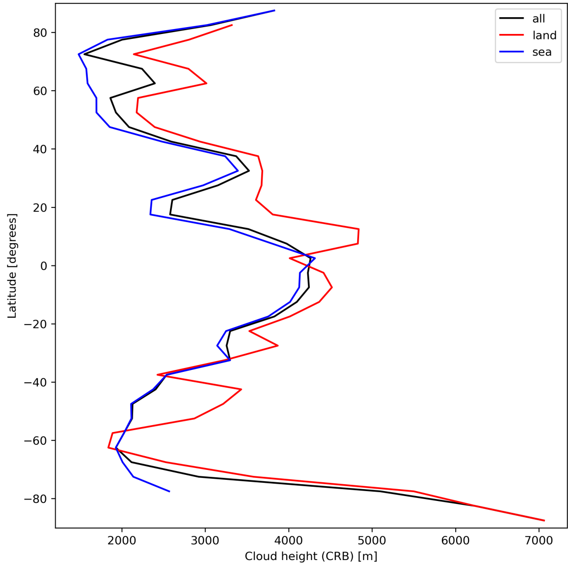
Figure 27: Zonal average of “Cloud height (CRB)” for 2024-03-14 to 2024-03-16.
