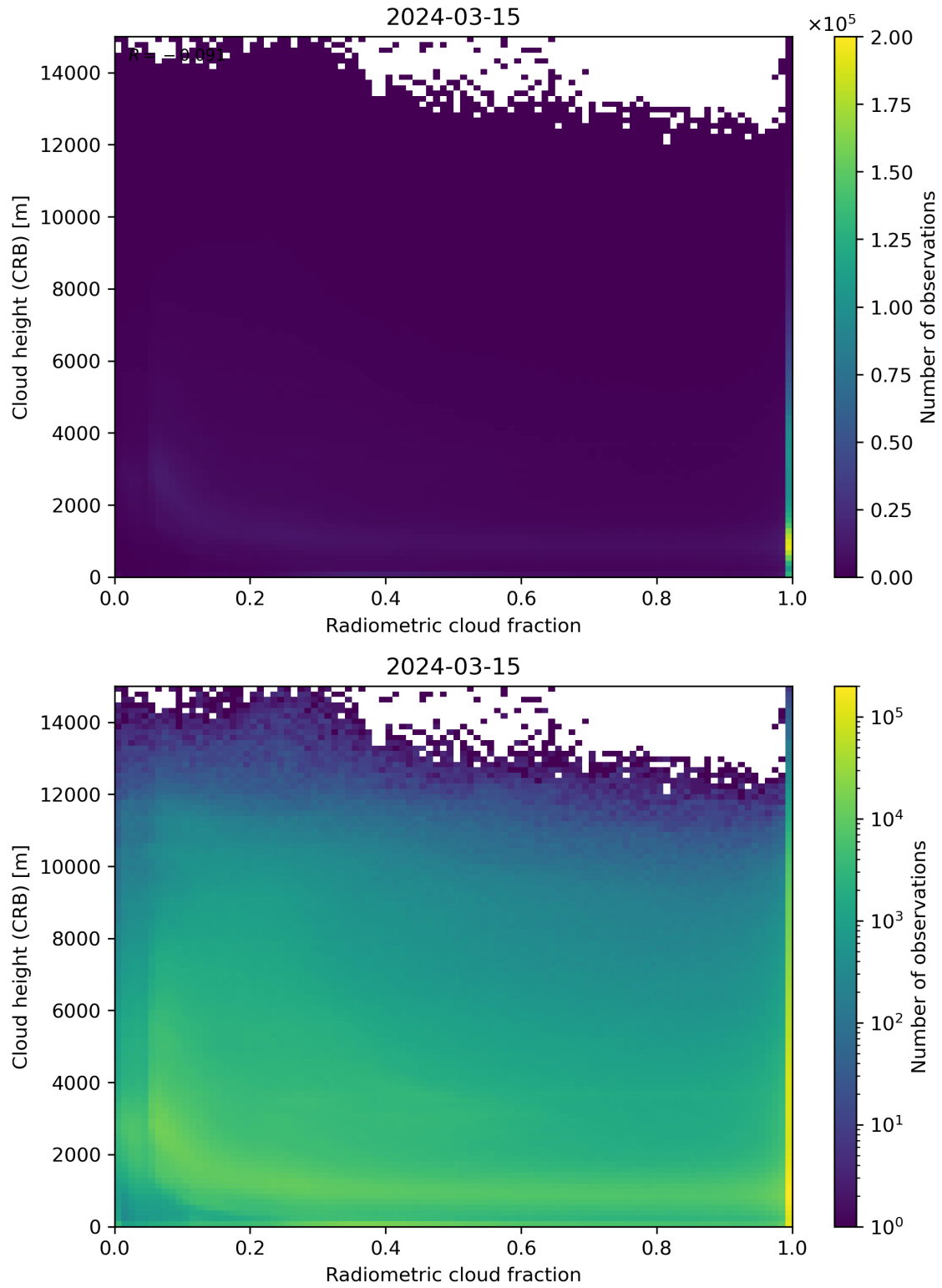
Figure 74: Scatter density plot of “Radiometric cloud fraction” against “Cloud height (CRB)” for 2024-03-14 to 2024-03-16.
