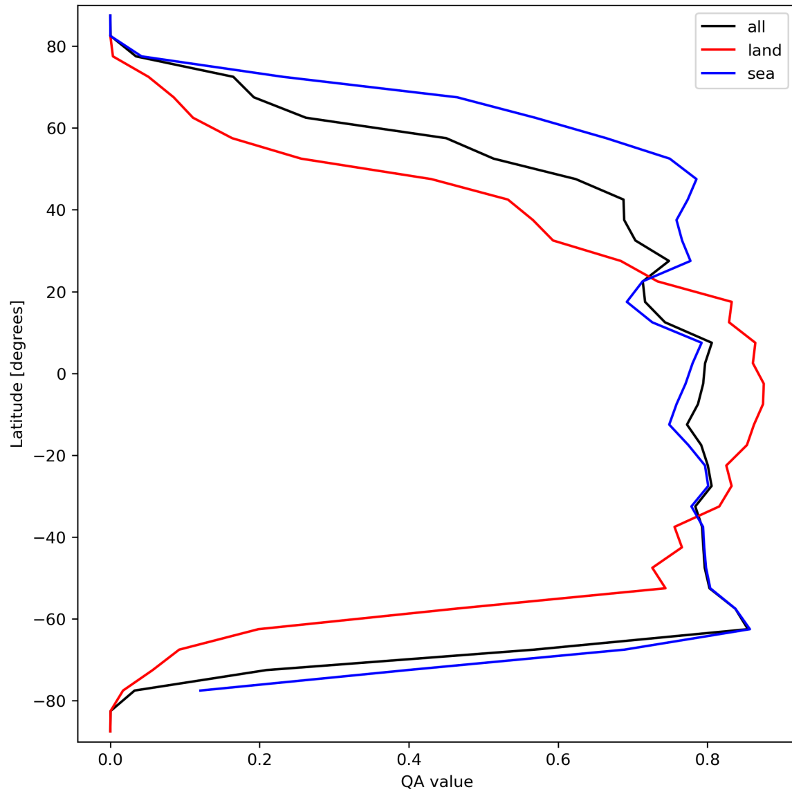
Figure 22: Zonal average of “QA value” for 2024-03-14 to 2024-03-16.
