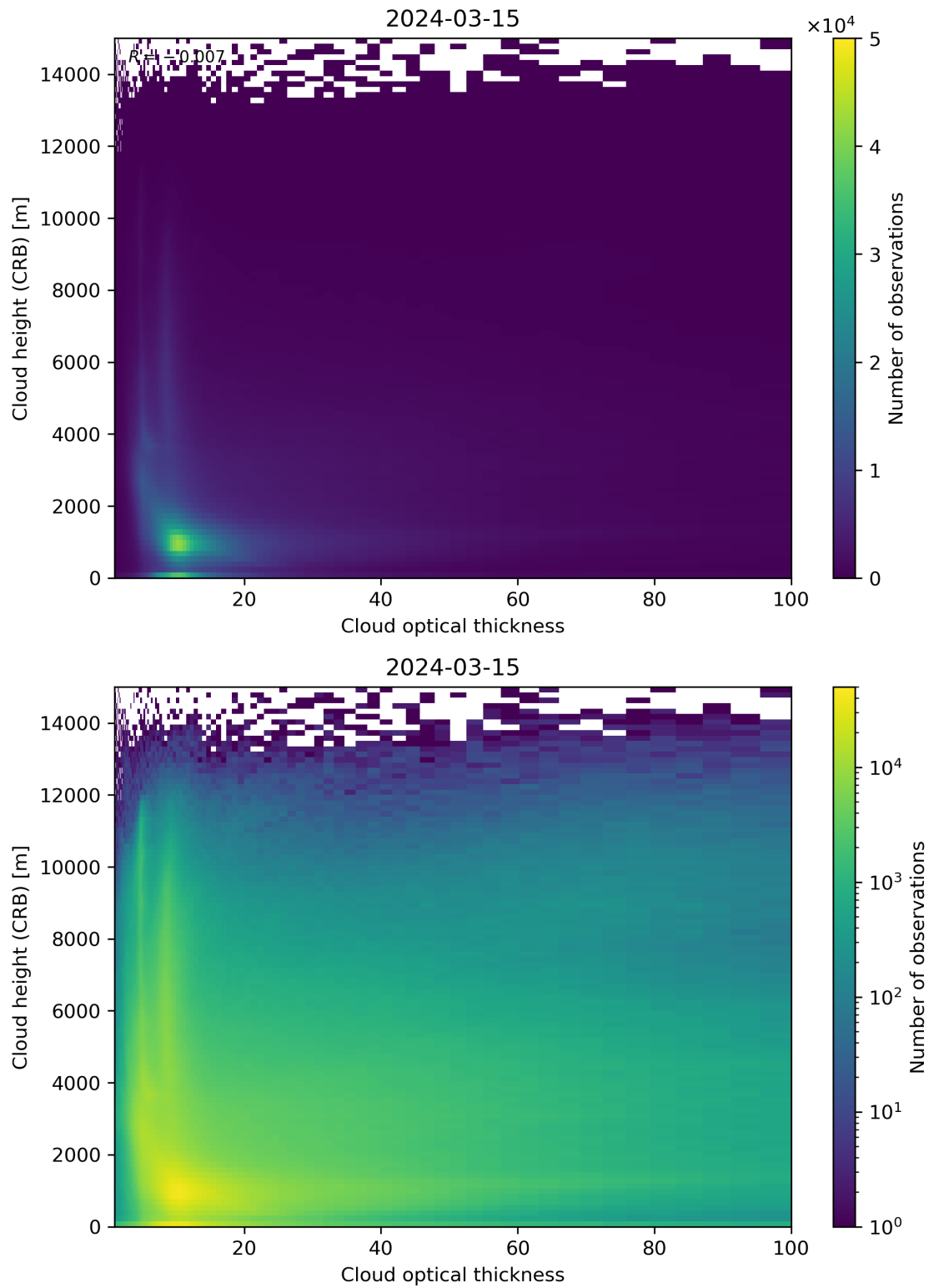
Figure 85: Scatter density plot of “Cloud optical thickness” against “Cloud height (CRB)” for 2024-03-14 to 2024-03-16.
