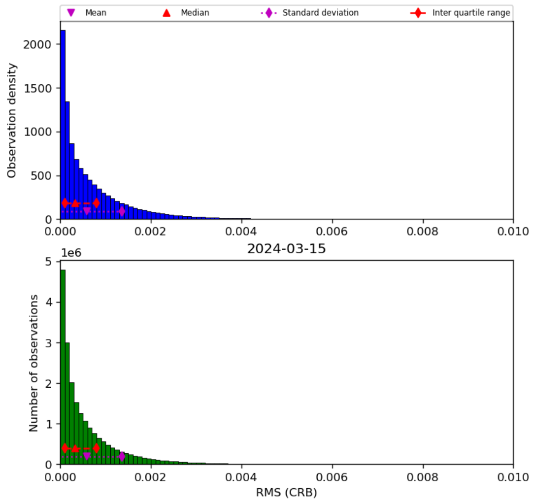
Figure 48: Histogram of “RMS (CRB)” for 2024-03-14 to 2024-03-16
