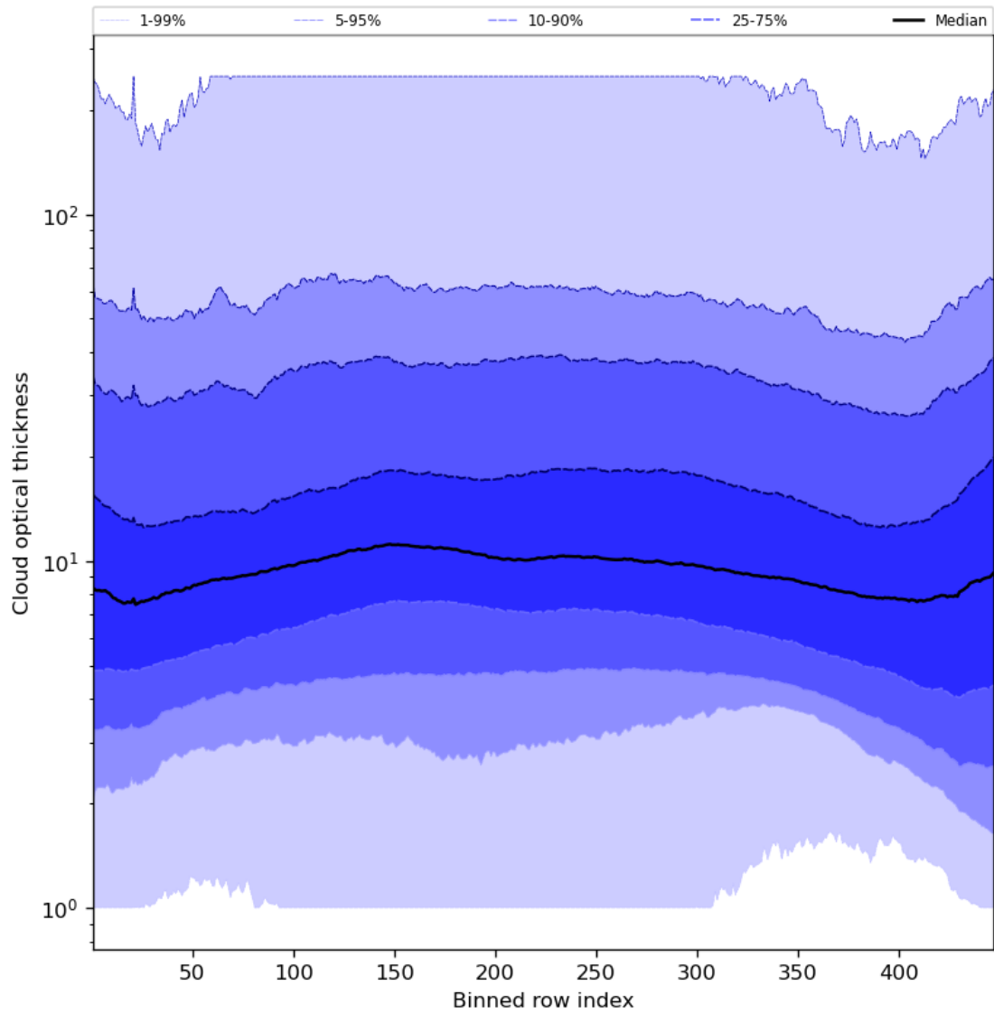
Figure 57: Along track statistics of “Cloud optical thickness” for 2024-03-14 to 2024-03-16
