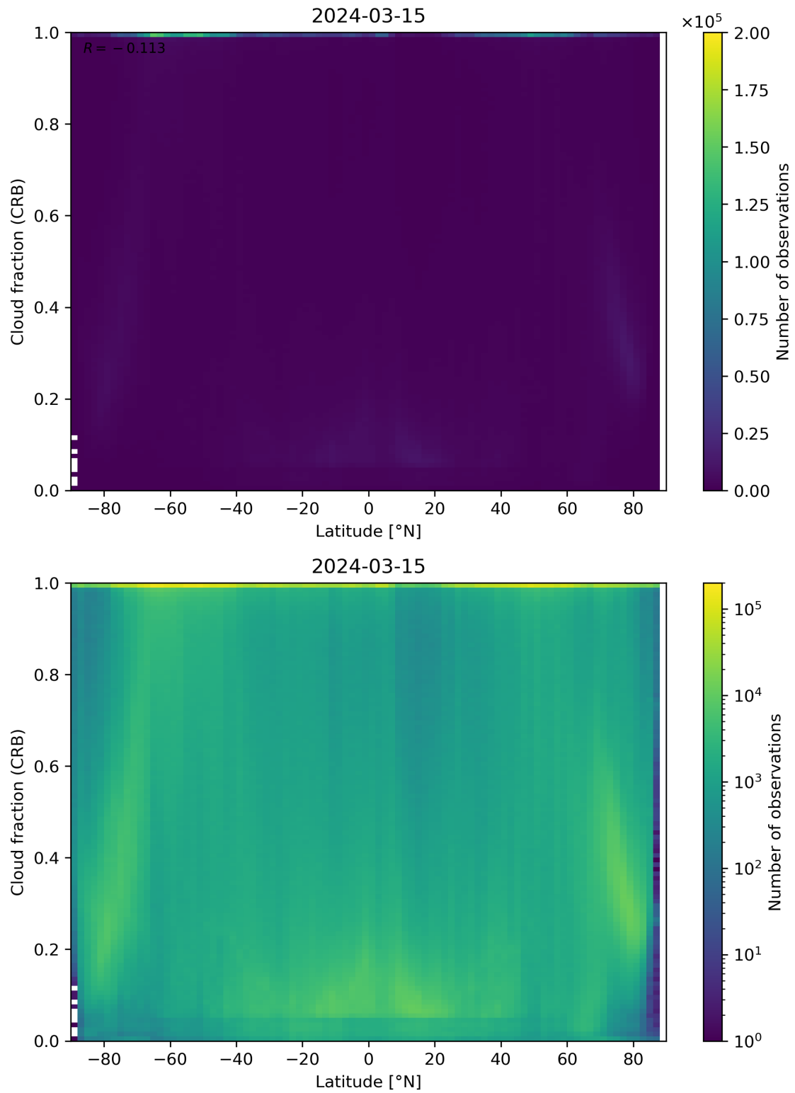
Figure 94: Scatter density plot of “Latitude” against “Cloud fraction (CRB)” for 2024-03-14 to 2024-03-16.
