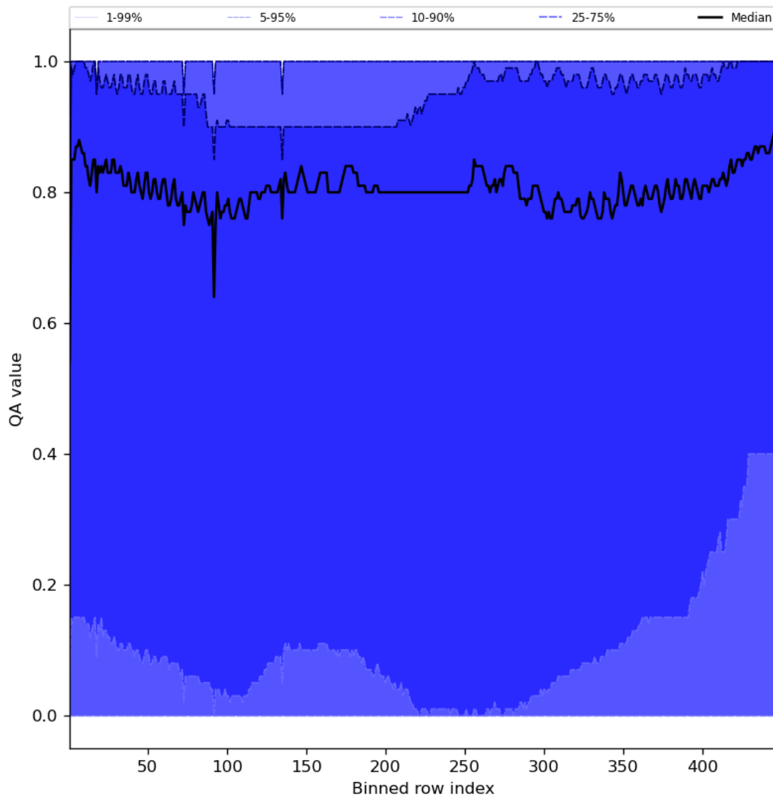
Figure 54: Along track statistics of “QA value” for 2024-03-14 to 2024-03-16
