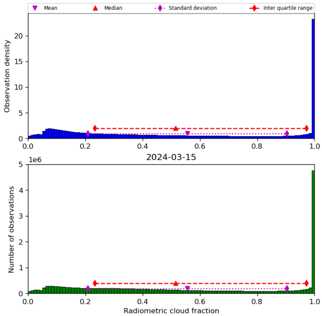
Figure 39: Histogram of “Radiometric cloud fraction” for 2024-03-14 to 2024-03-16
