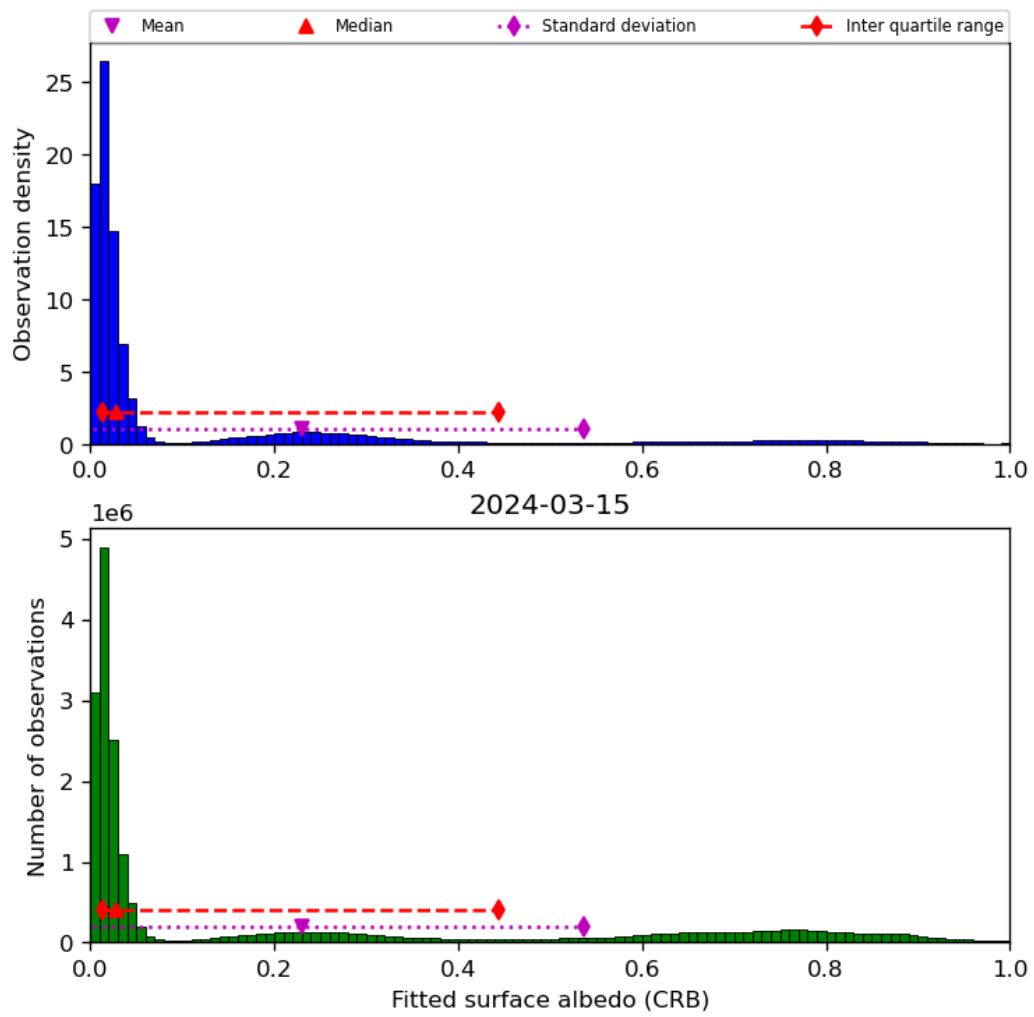
Figure 46: Histogram of “Fitted surface albedo (CRB)” for 2024-03-14 to 2024-03-16
