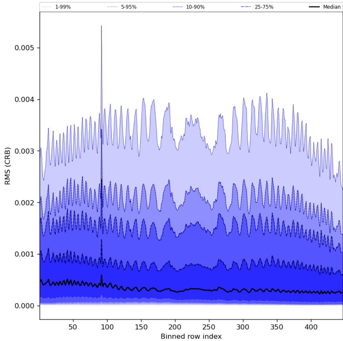
Figure 64: Along track statistics of “RMS (CRB)” for 2024-03-14 to 2024-03-16
