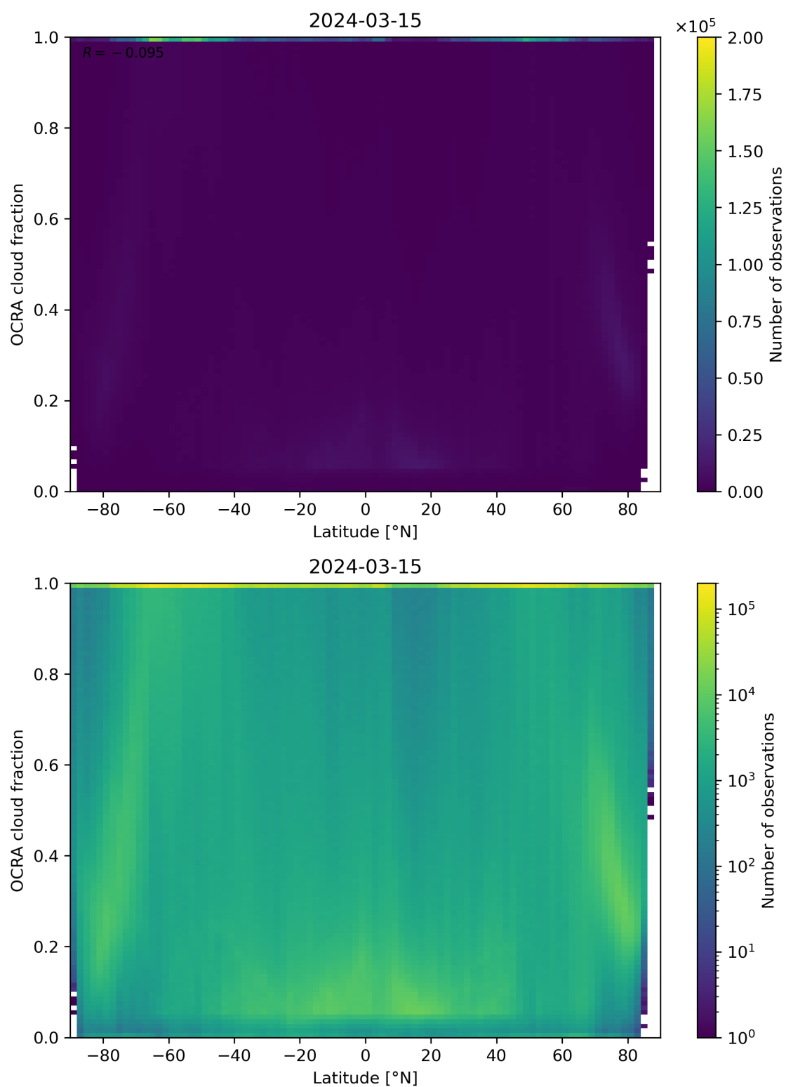
Figure 93: Scatter density plot of “Latitude” against “OCRA cloud fraction” for 2024-03-14 to 2024-03-16.
