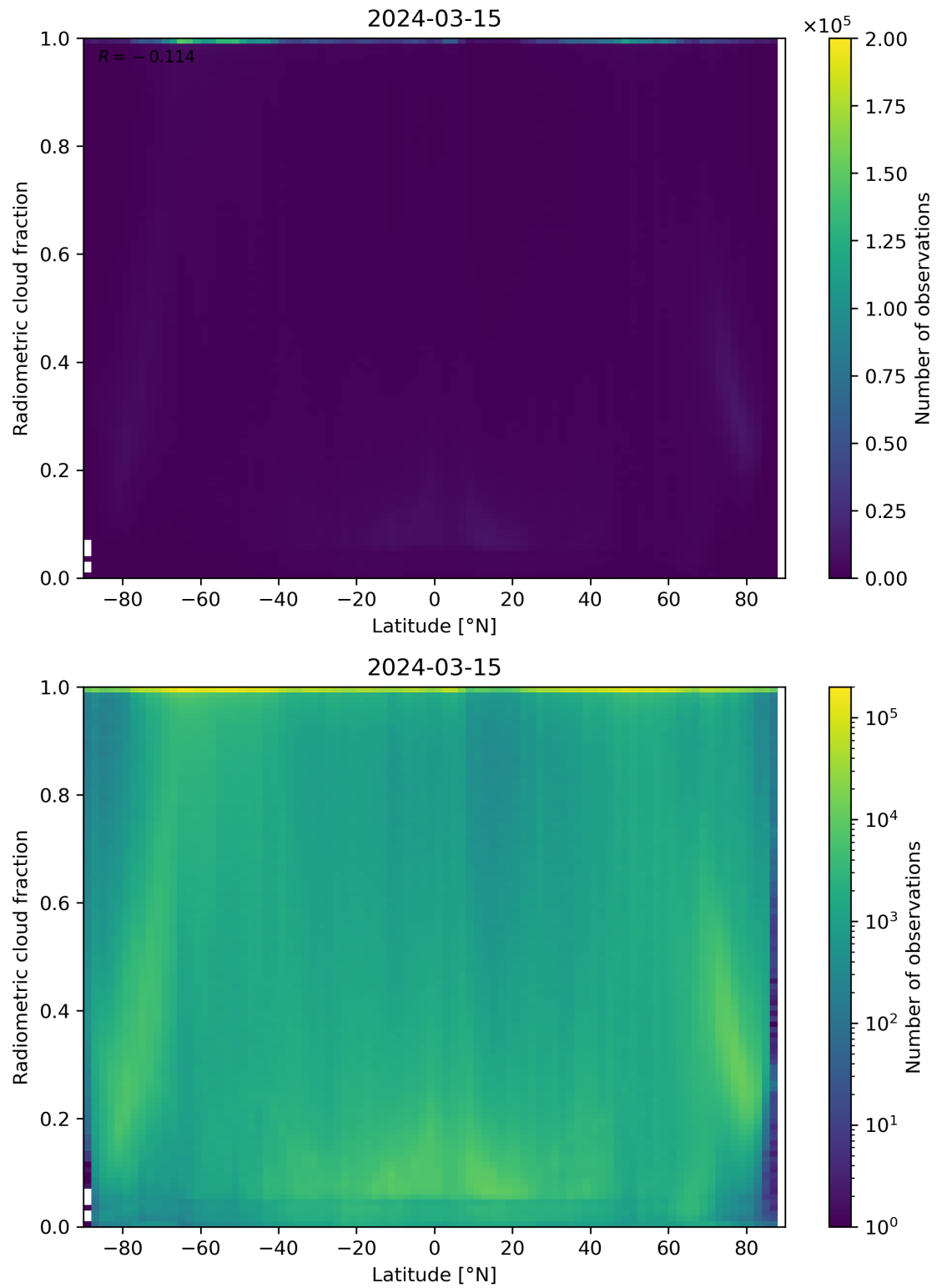
Figure 92: Scatter density plot of “Latitude” against “Radiometric cloud fraction” for 2024-03-14 to 2024-03-16.
