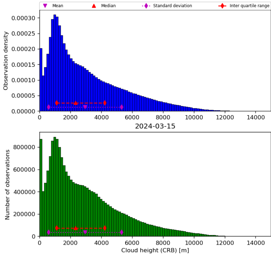
Figure 43: Histogram of “Cloud height (CRB)” for 2024-03-14 to 2024-03-16
