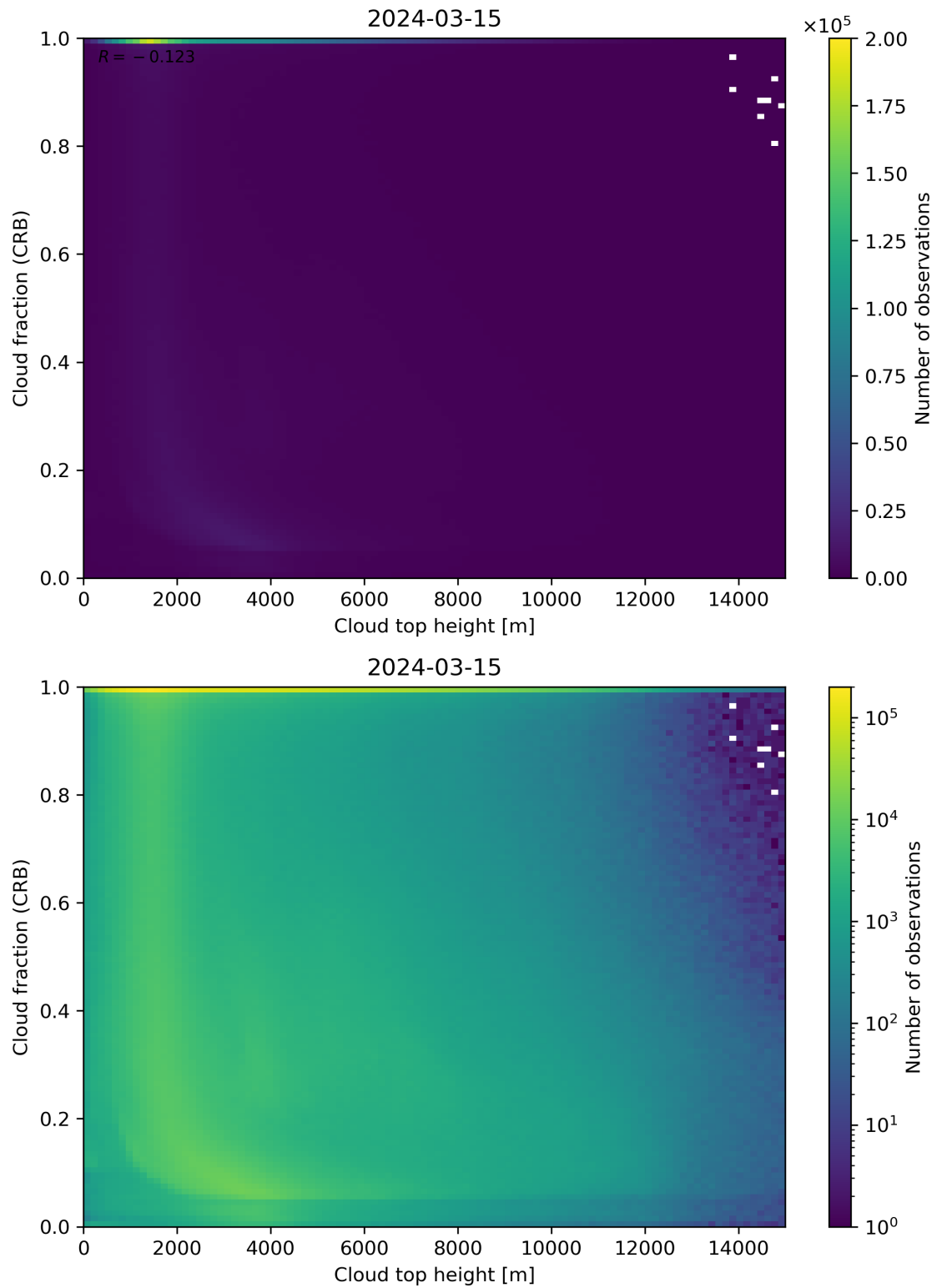
Figure 88: Scatter density plot of “Cloud top height” against “Cloud fraction (CRB)” for 2024-03-14 to 2024-03-16.
