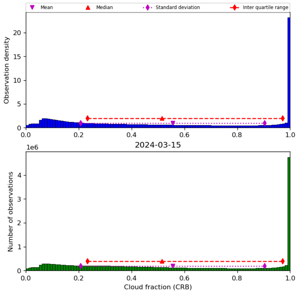
Figure 42: Histogram of “Cloud fraction (CRB)” for 2024-03-14 to 2024-03-16
