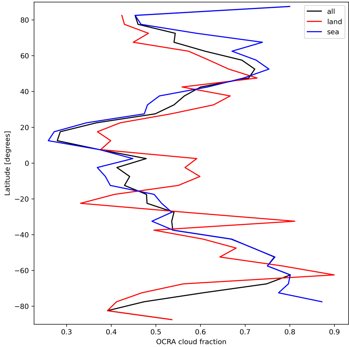
Figure 34: Zonal average of “OCRA cloud fraction” for 2024-03-14 to 2024-03-16.
