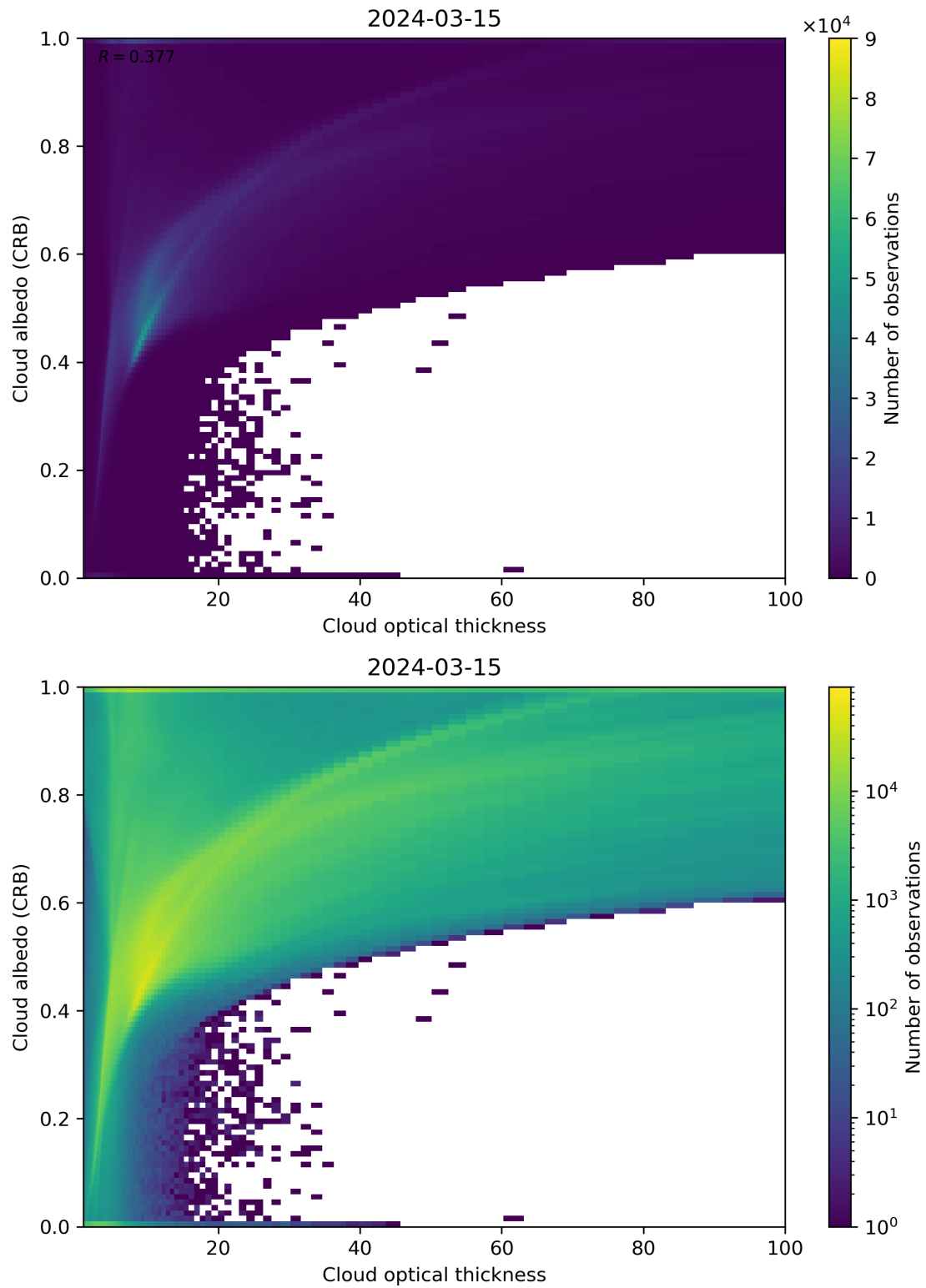
Figure 82: Scatter density plot of “Cloud optical thickness” against “Cloud albedo (CRB)” for 2024-03-14 to 2024-03-16.
