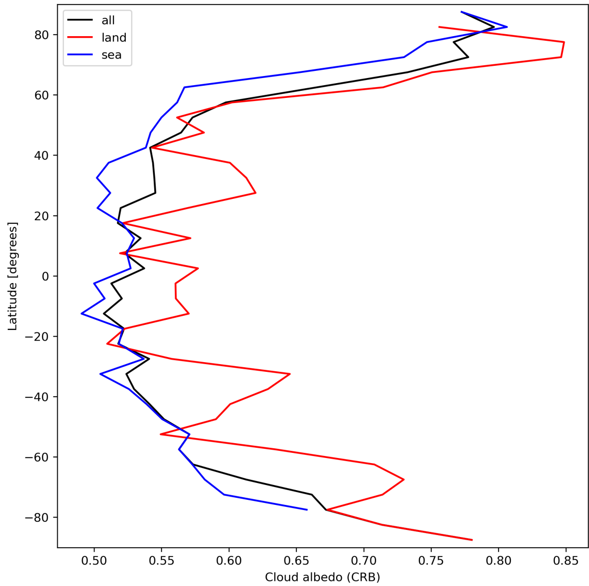
Figure 28: Zonal average of “Cloud albedo (CRB)” for 2024-03-14 to 2024-03-16.
