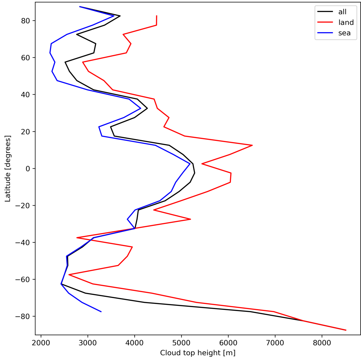
Figure 24: Zonal average of “Cloud top height” for 2024-03-14 to 2024-03-16.
