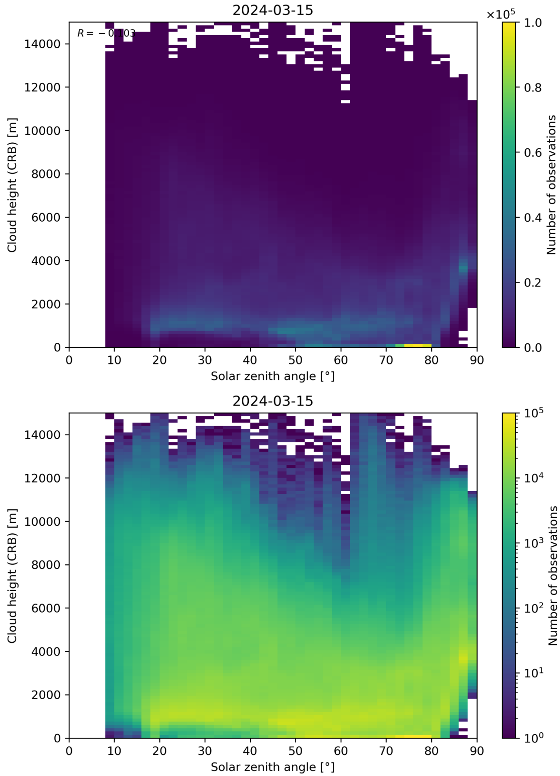
Figure 102: Scatter density plot of “Solar zenith angle” against “Cloud height (CRB)” for 2024-03-14 to 2024-03-16.
