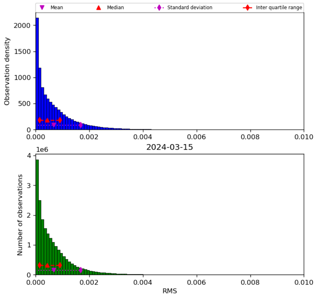
Figure 47: Histogram of “RMS” for 2024-03-14 to 2024-03-16
