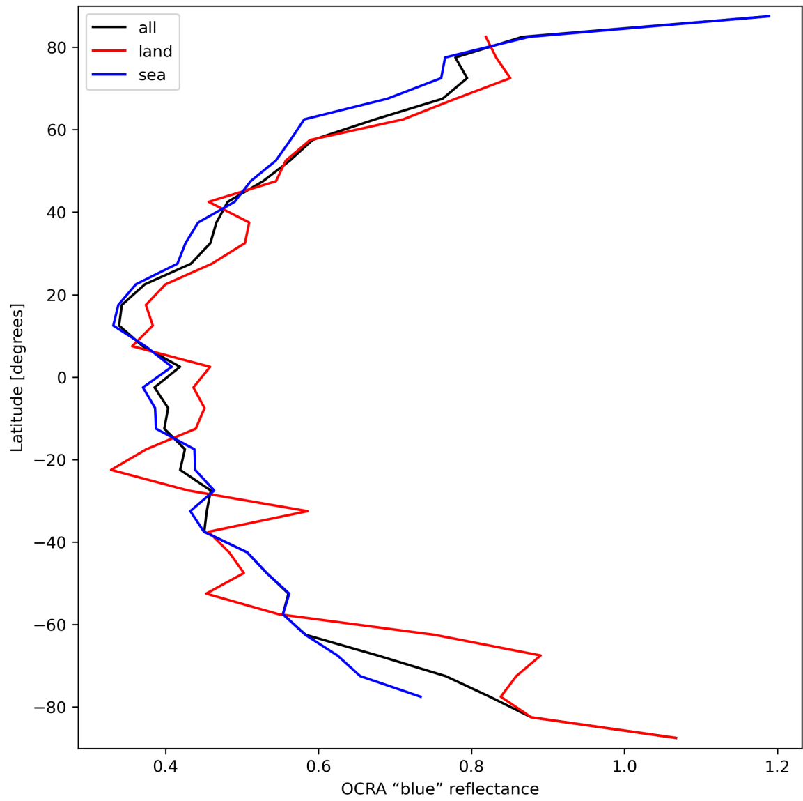
Figure 35: Zonal average of “OCRA “blue” reflectance” for 2024-03-14 to 2024-03-16.
