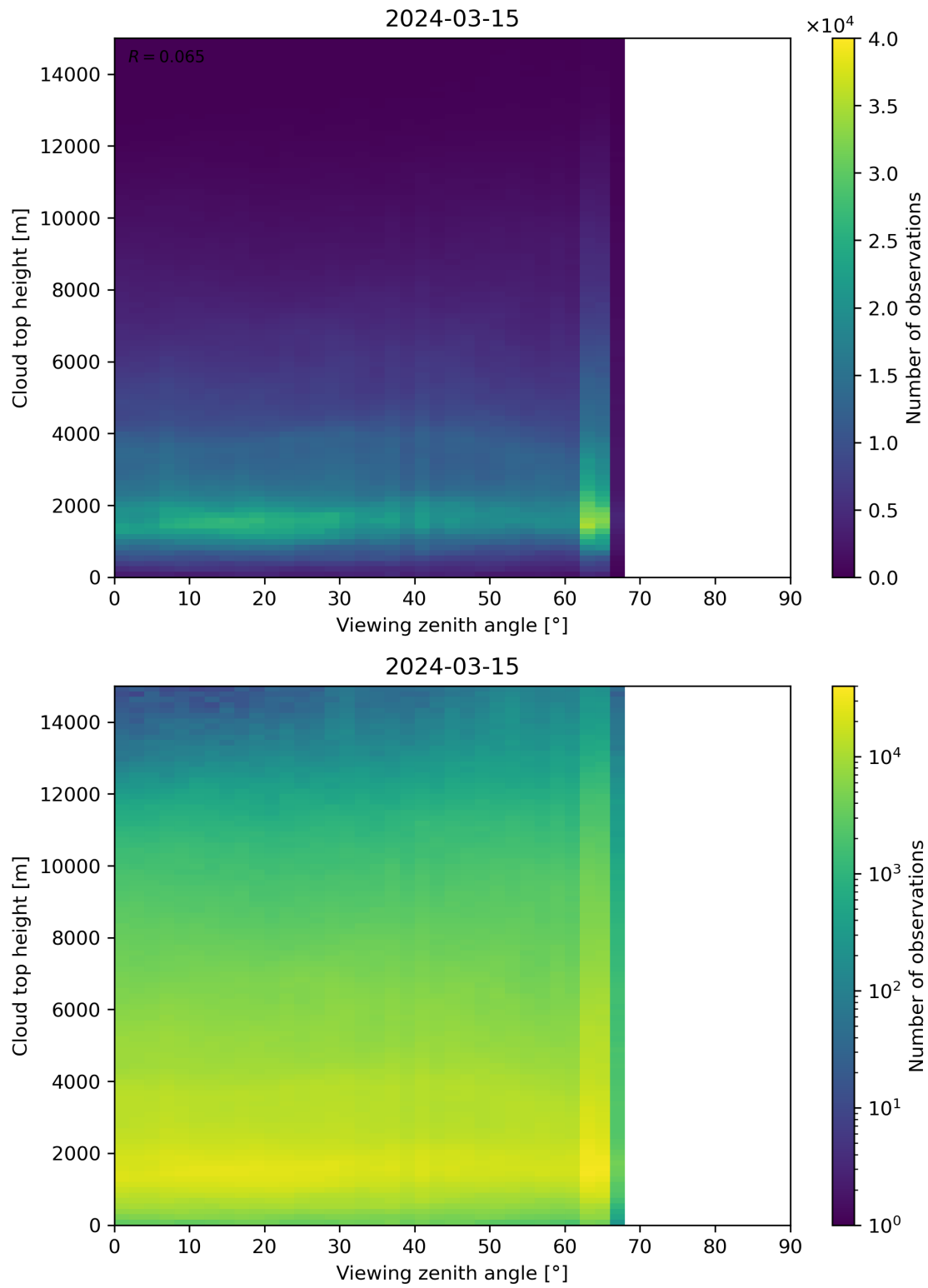
Figure 112: Scatter density plot of “Viewing zenith angle” against “Cloud top height” for 2024-03-14 to 2024-03-16.
