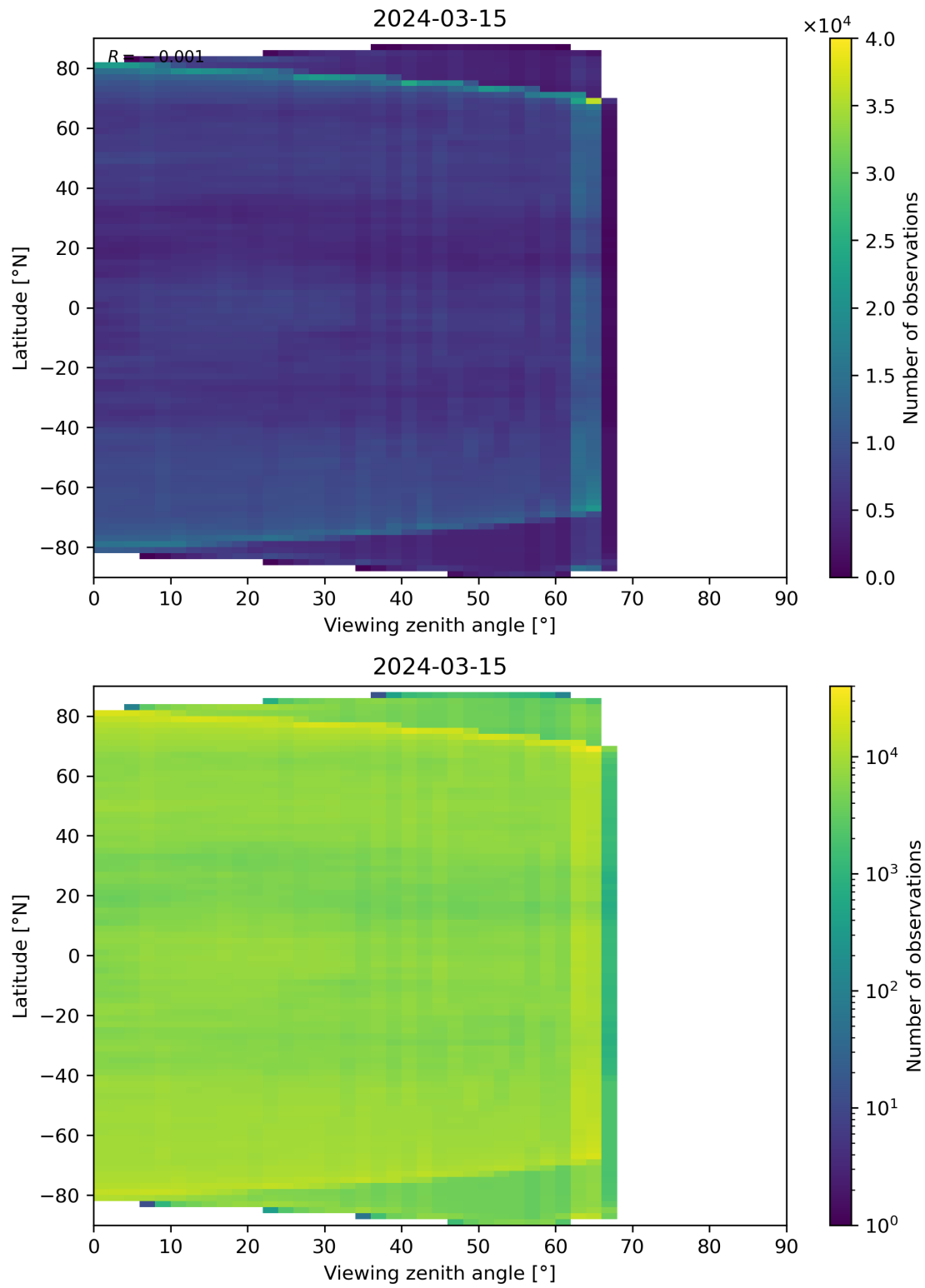
Figure 113: Scatter density plot of “Viewing zenith angle” against “Latitude” for 2024-03-14 to 2024-03-16.
