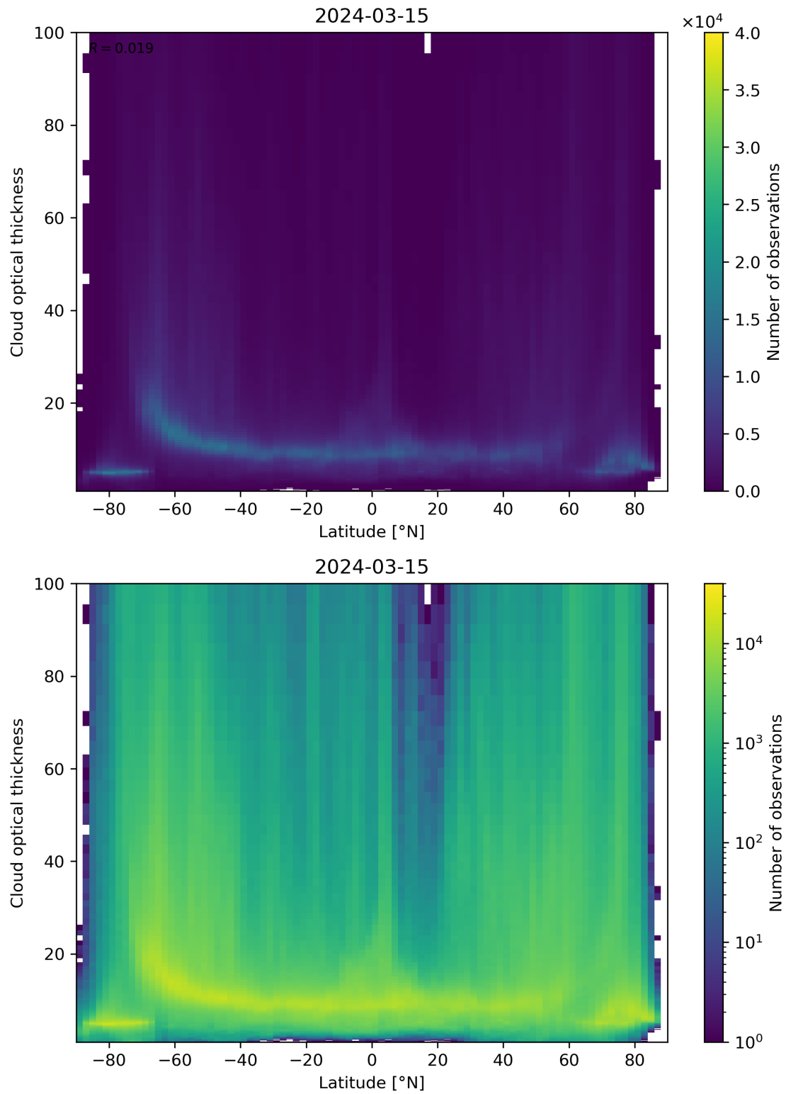
Figure 96: Scatter density plot of “Latitude” against “Cloud optical thickness” for 2024-03-14 to 2024-03-16.
