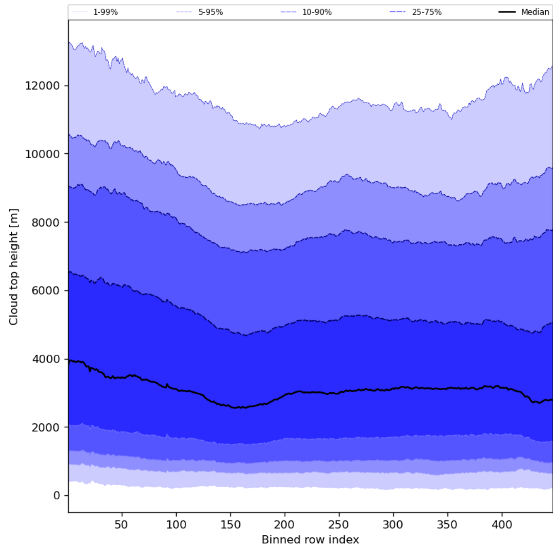
Figure 56: Along track statistics of “Cloud top height” for 2024-03-14 to 2024-03-16
