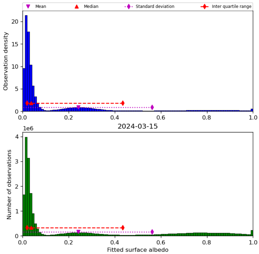
Figure 45: Histogram of “Fitted surface albedo” for 2024-03-14 to 2024-03-16
