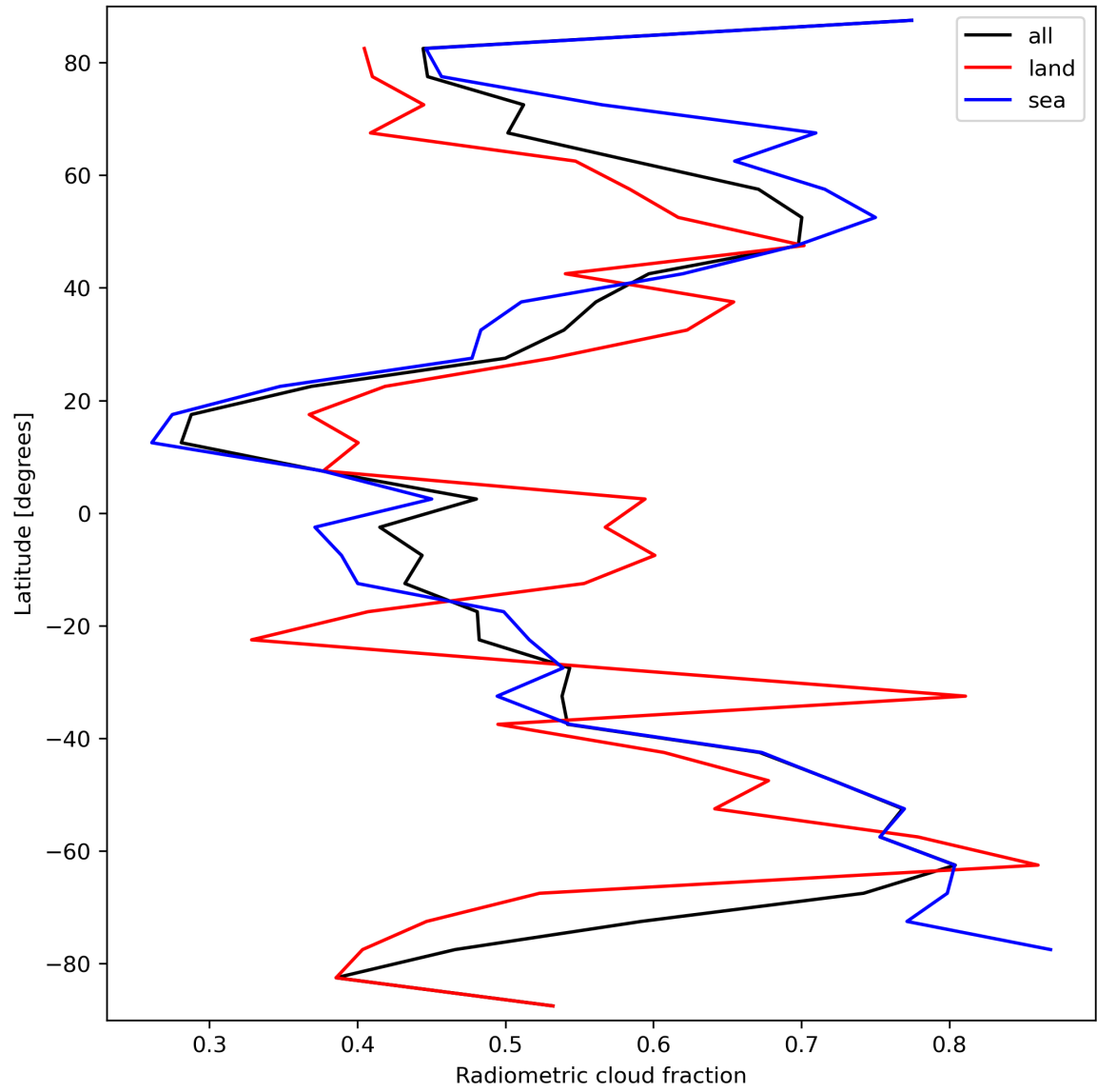
Figure 23: Zonal average of “Radiometric cloud fraction” for 2024-03-14 to 2024-03-16.
