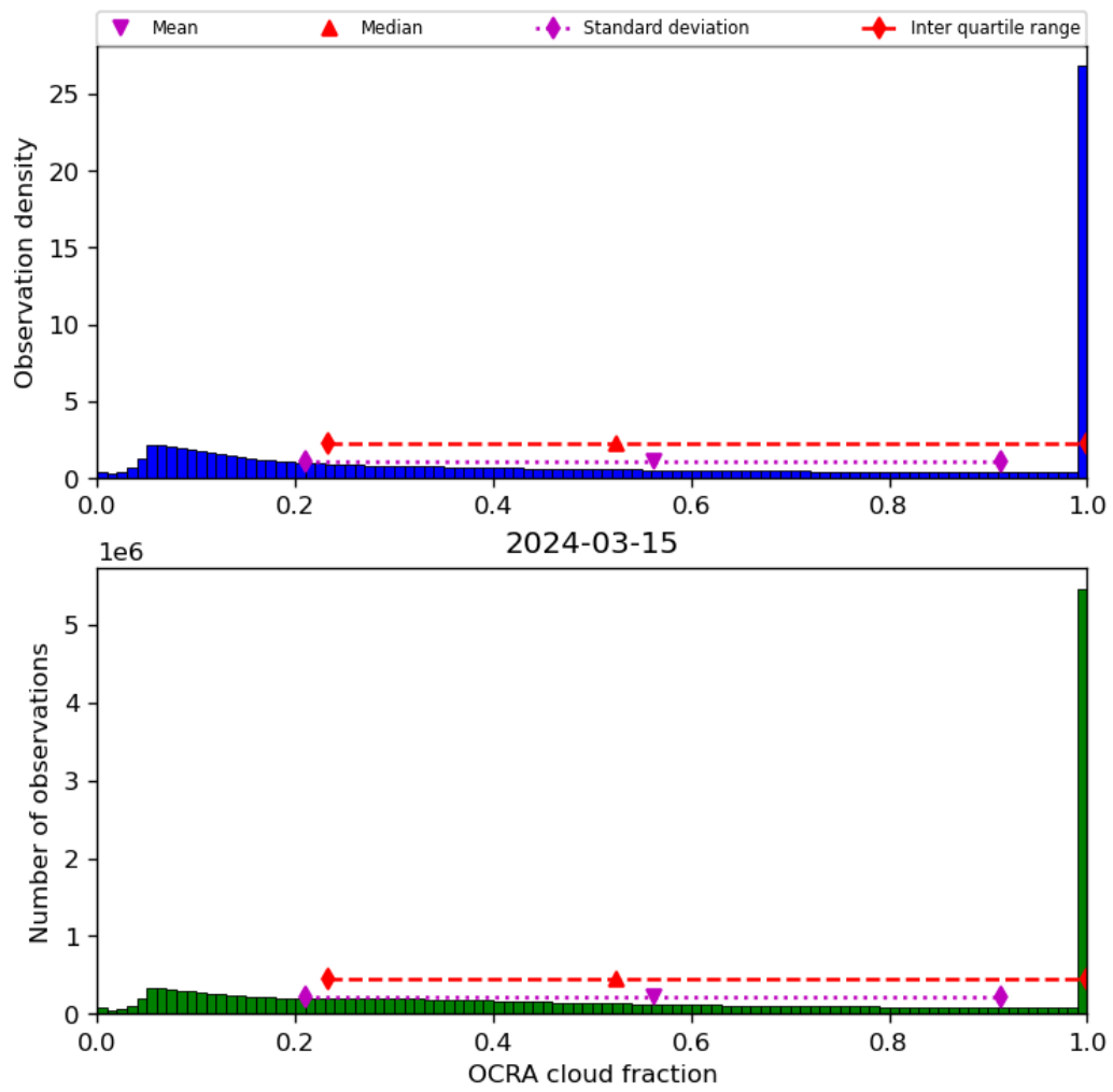
Figure 50: Histogram of “OCRA cloud fraction” for 2024-03-14 to 2024-03-16
