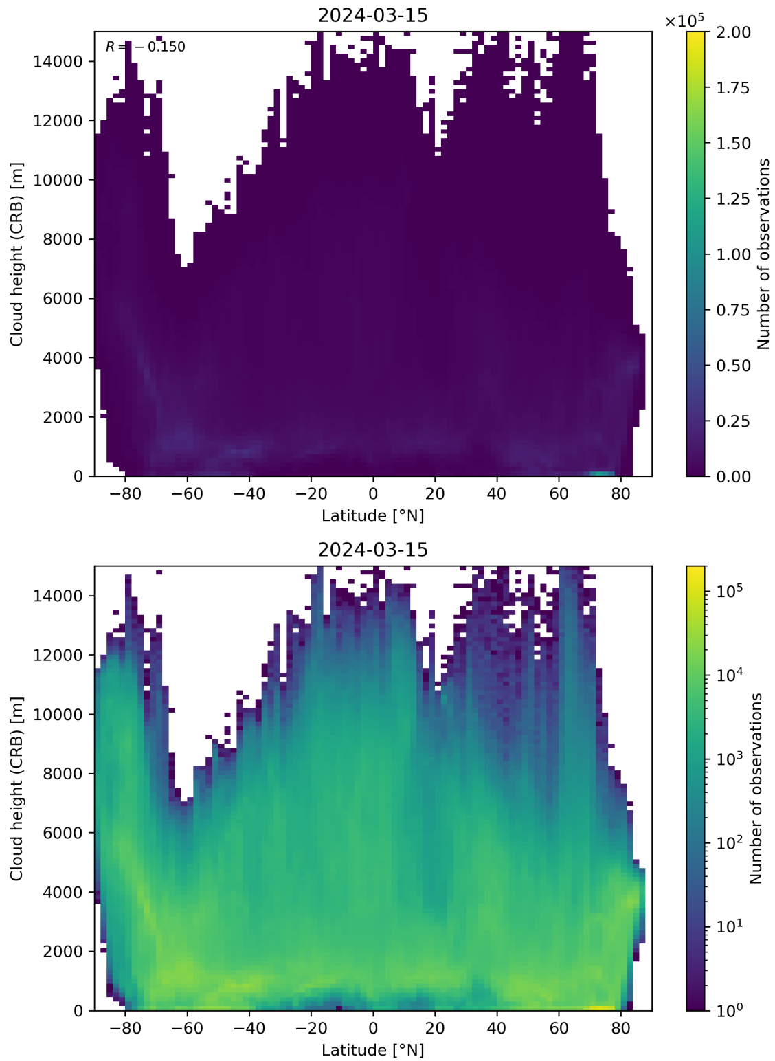
Figure 95: Scatter density plot of “Latitude” against “Cloud height (CRB)” for 2024-03-14 to 2024-03-16.
