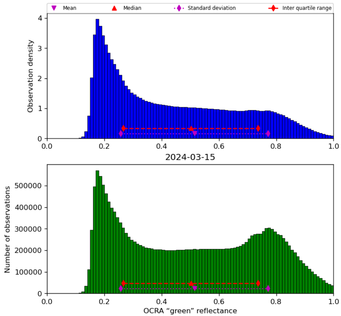
Figure 52: Histogram of “OCRA “green” reflectance” for 2024-03-14 to 2024-03-16
