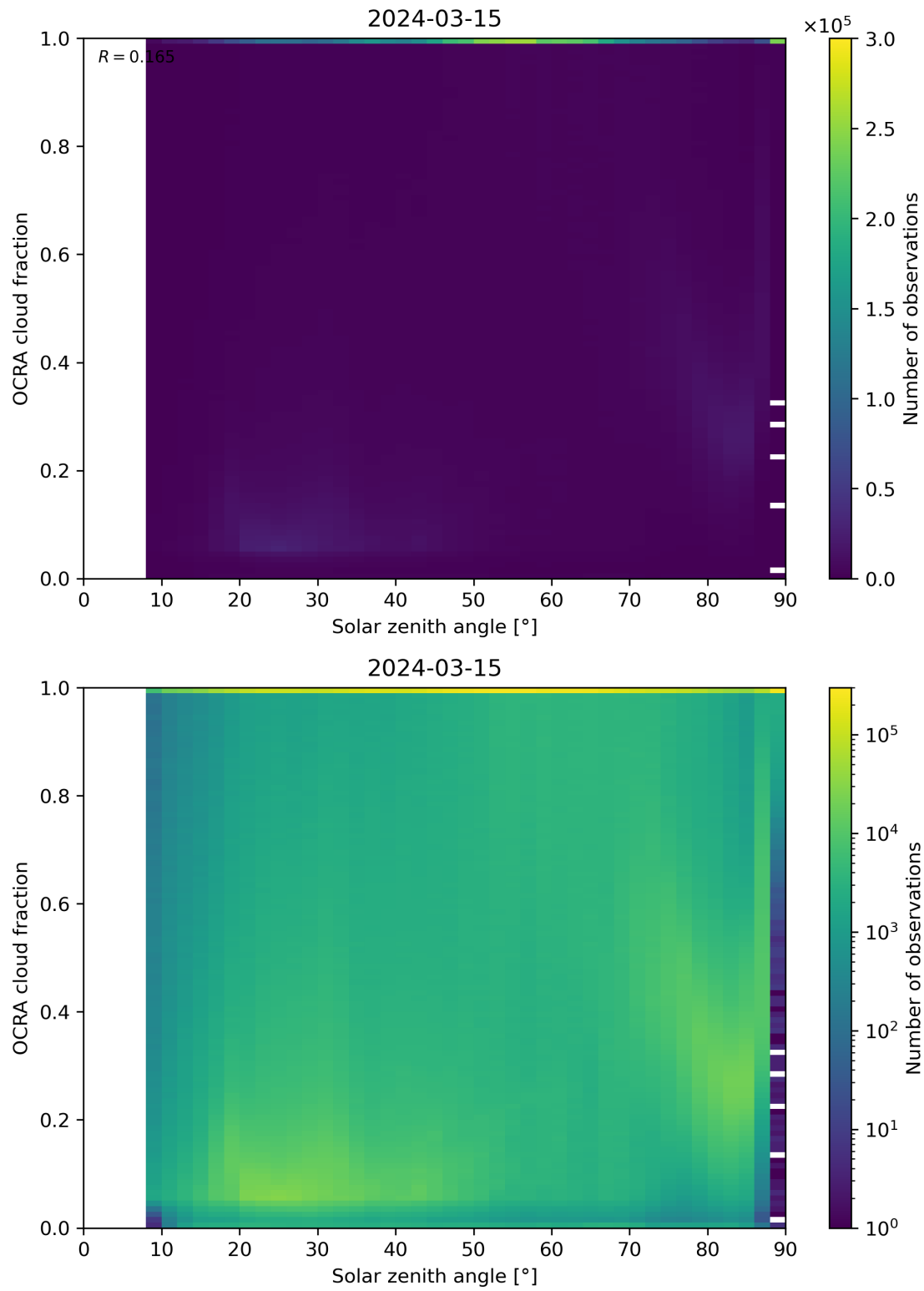
Figure 100: Scatter density plot of “Solar zenith angle” against “OCRA cloud fraction” for 2024-03-14 to 2024-03-16.
