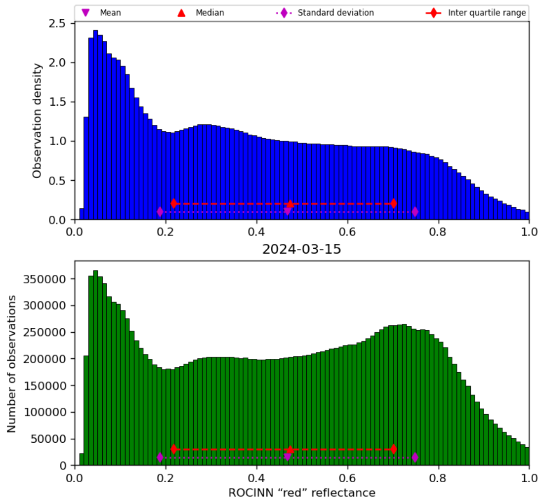
Figure 53: Histogram of “ROCINN “red” reflectance” for 2024-03-14 to 2024-03-16
