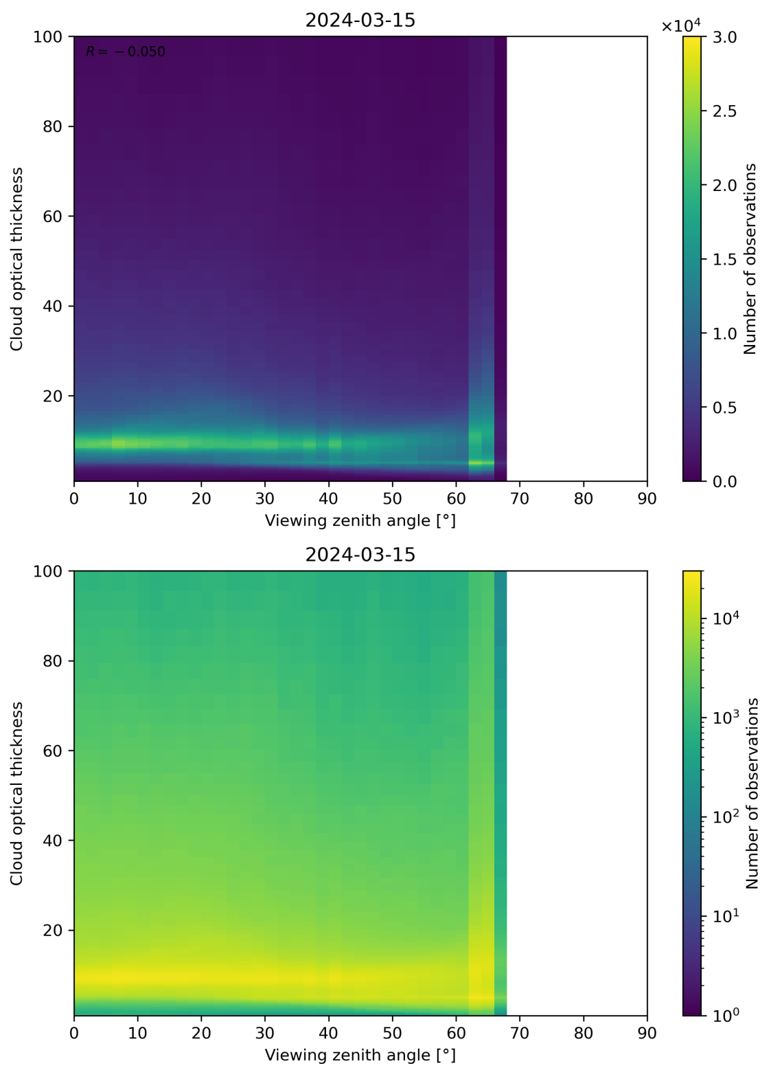
Figure 111: Scatter density plot of “Viewing zenith angle” against “Cloud optical thickness” for 2024-03-14 to 2024-03-16.
