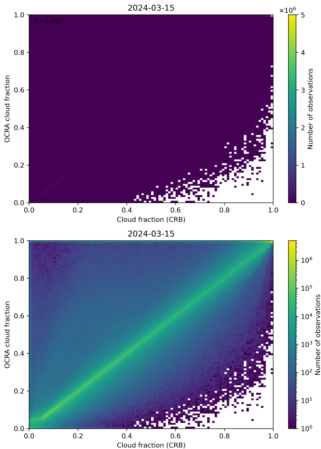
Figure 78: Scatter density plot of “Cloud fraction (CRB)” against “OCRA cloud fraction” for 2024-03-14 to 2024-03-16.
