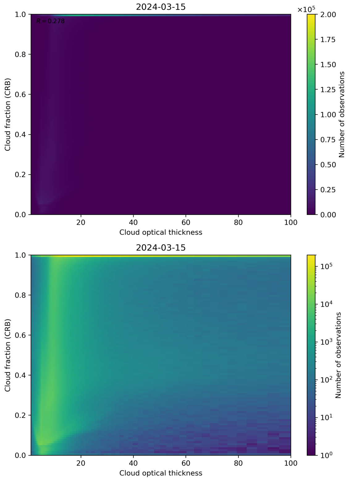
Figure 84: Scatter density plot of “Cloud optical thickness” against “Cloud fraction (CRB)” for 2024-03-14 to 2024-03-16.
