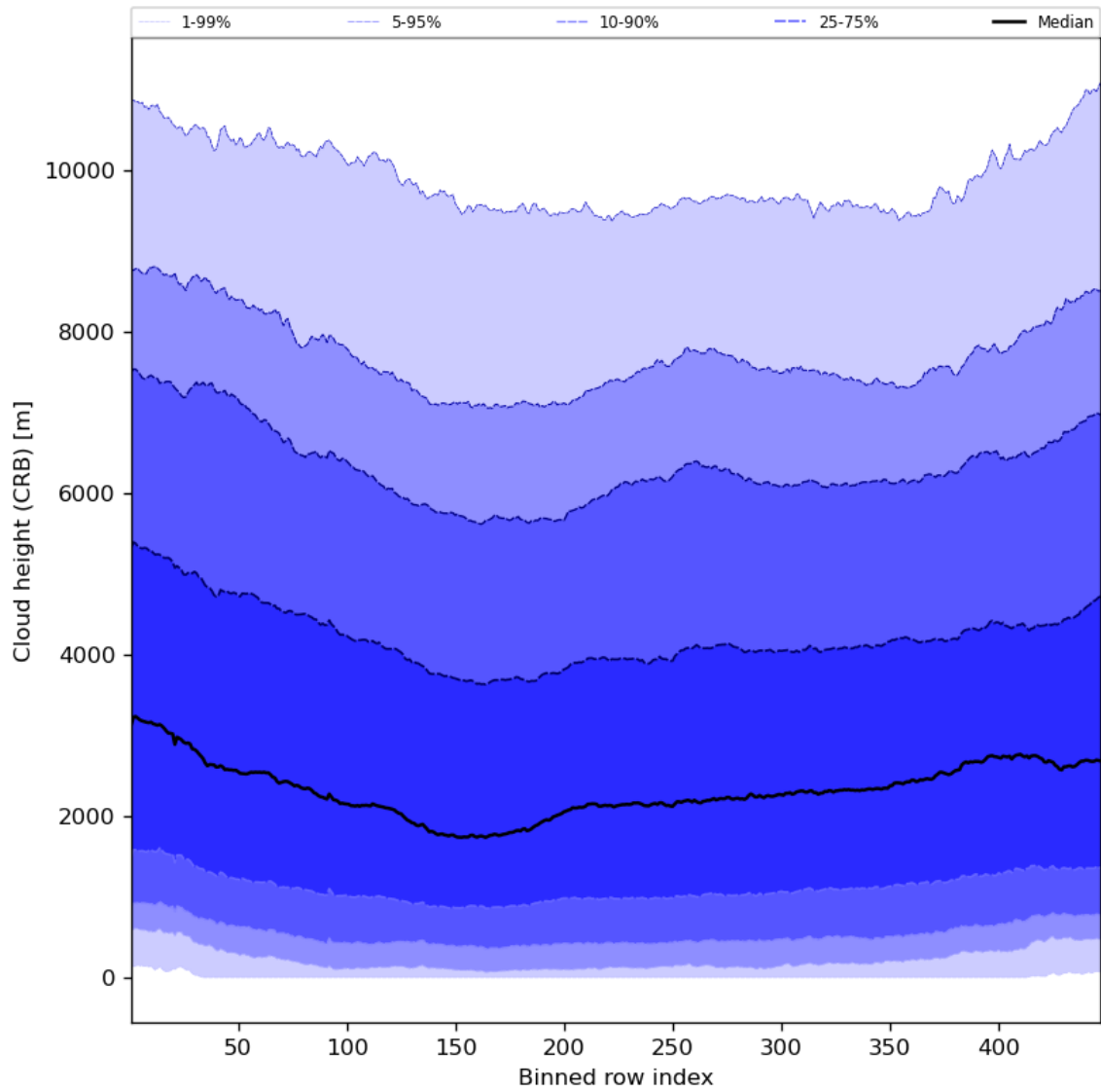
Figure 59: Along track statistics of “Cloud height (CRB)” for 2024-03-14 to 2024-03-16
