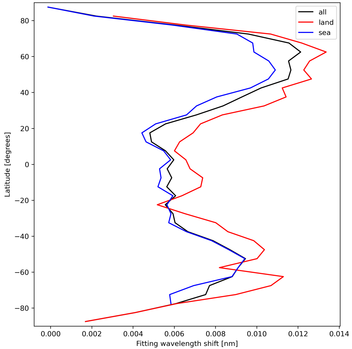
Figure 33: Zonal average of “Fitting wavelength shift” for 2024-03-14 to 2024-03-16.
