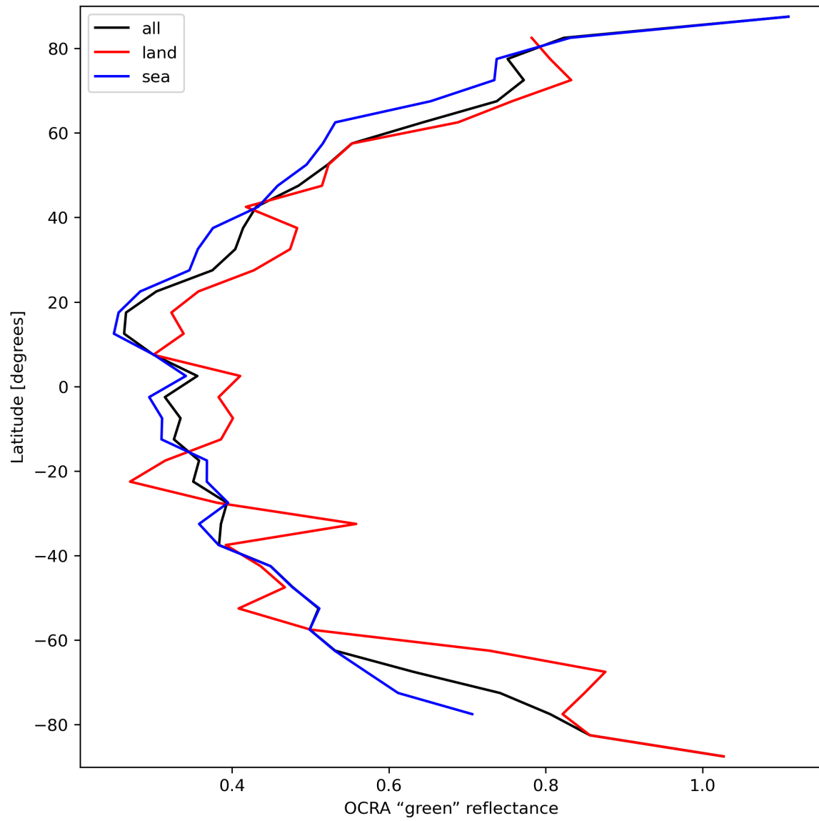
Figure 36: Zonal average of “OCRA “green” reflectance” for 2024-03-14 to 2024-03-16.
