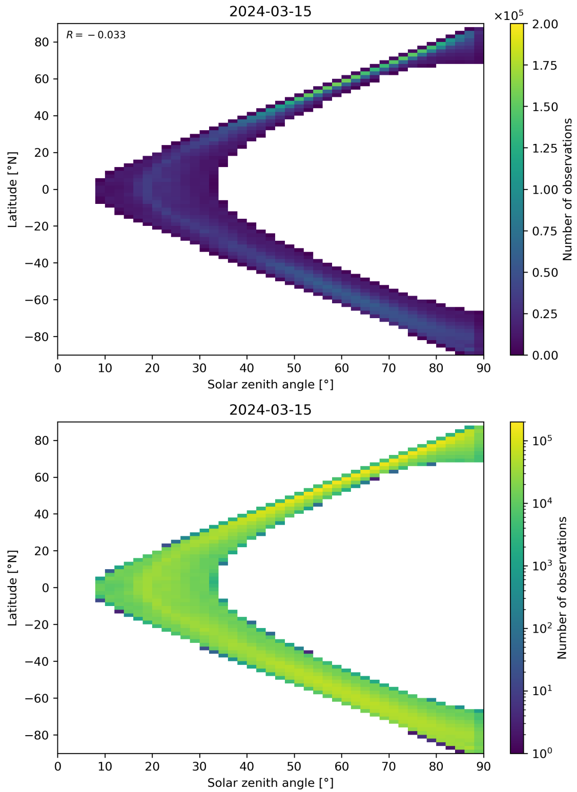
Figure 105: Scatter density plot of “Solar zenith angle” against “Latitude” for 2024-03-14 to 2024-03-16.
