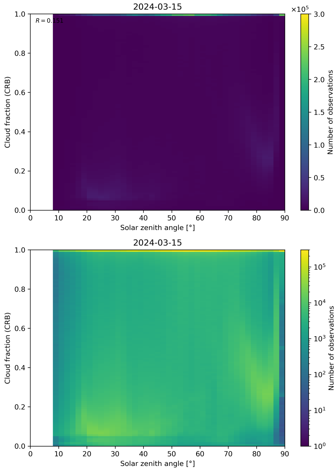
Figure 101: Scatter density plot of “Solar zenith angle” against “Cloud fraction (CRB)” for 2024-03-14 to 2024-03-16.
