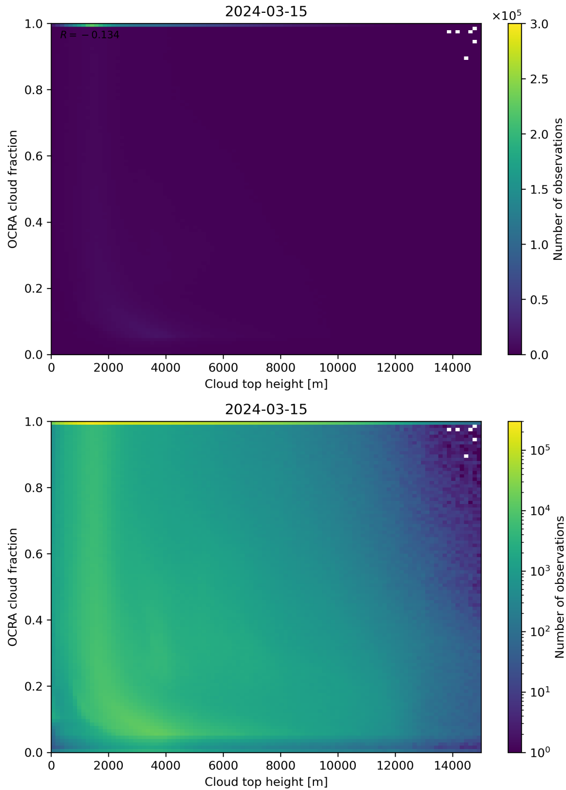
Figure 87: Scatter density plot of “Cloud top height” against “OCRA cloud fraction” for 2024-03-14 to 2024-03-16.
