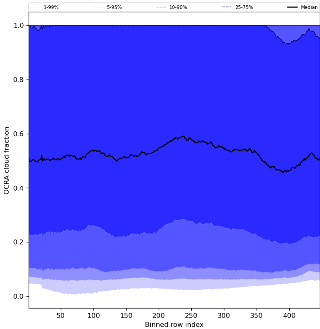
Figure 66: Along track statistics of “OCRA cloud fraction” for 2024-03-14 to 2024-03-16
