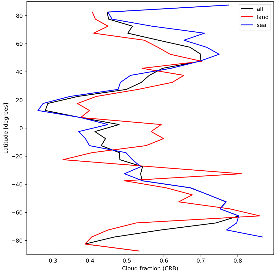
Figure 26: Zonal average of “Cloud fraction (CRB)” for 2024-03-14 to 2024-03-16.
