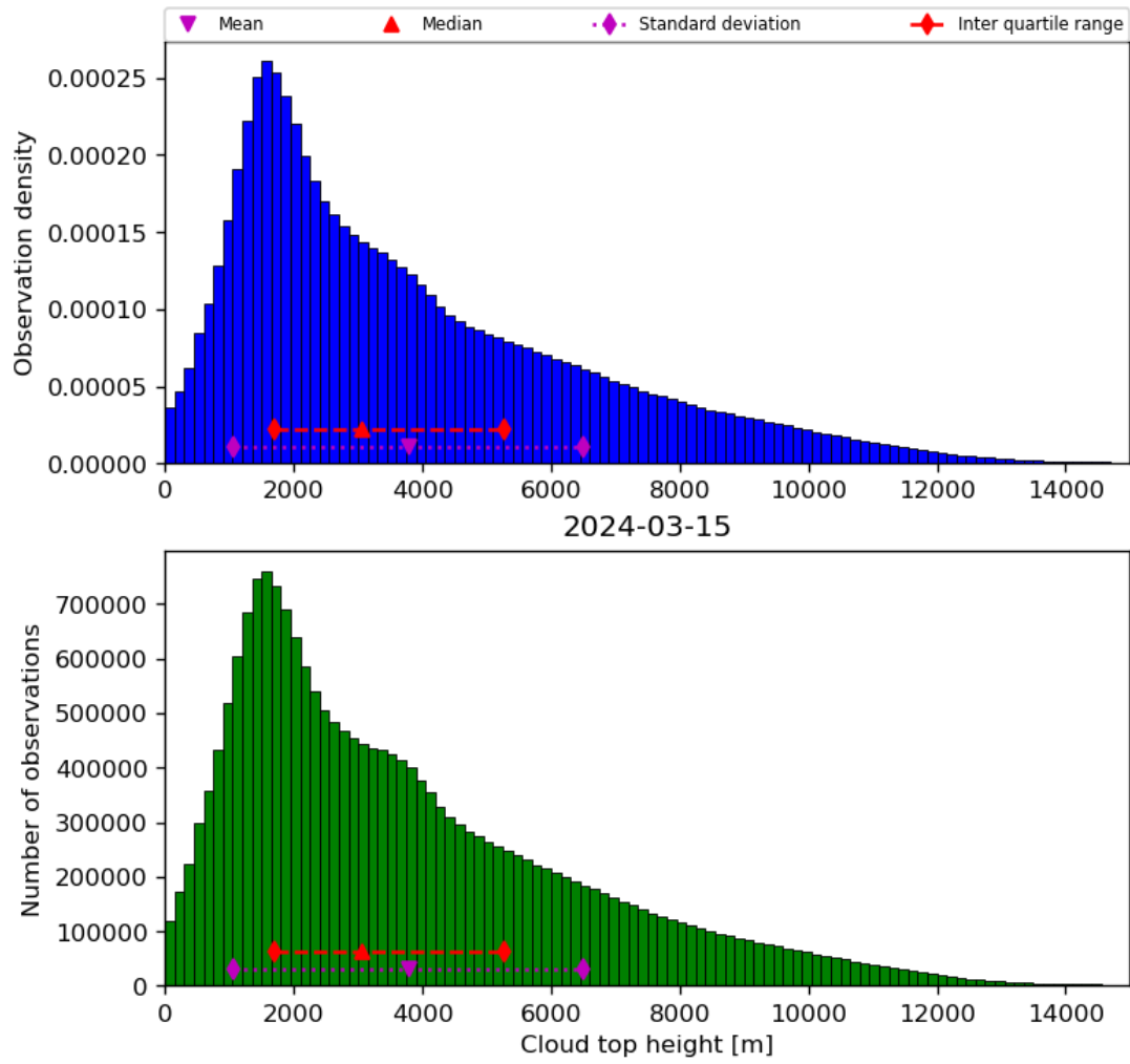
Figure 40: Histogram of “Cloud top height” for 2024-03-14 to 2024-03-16
