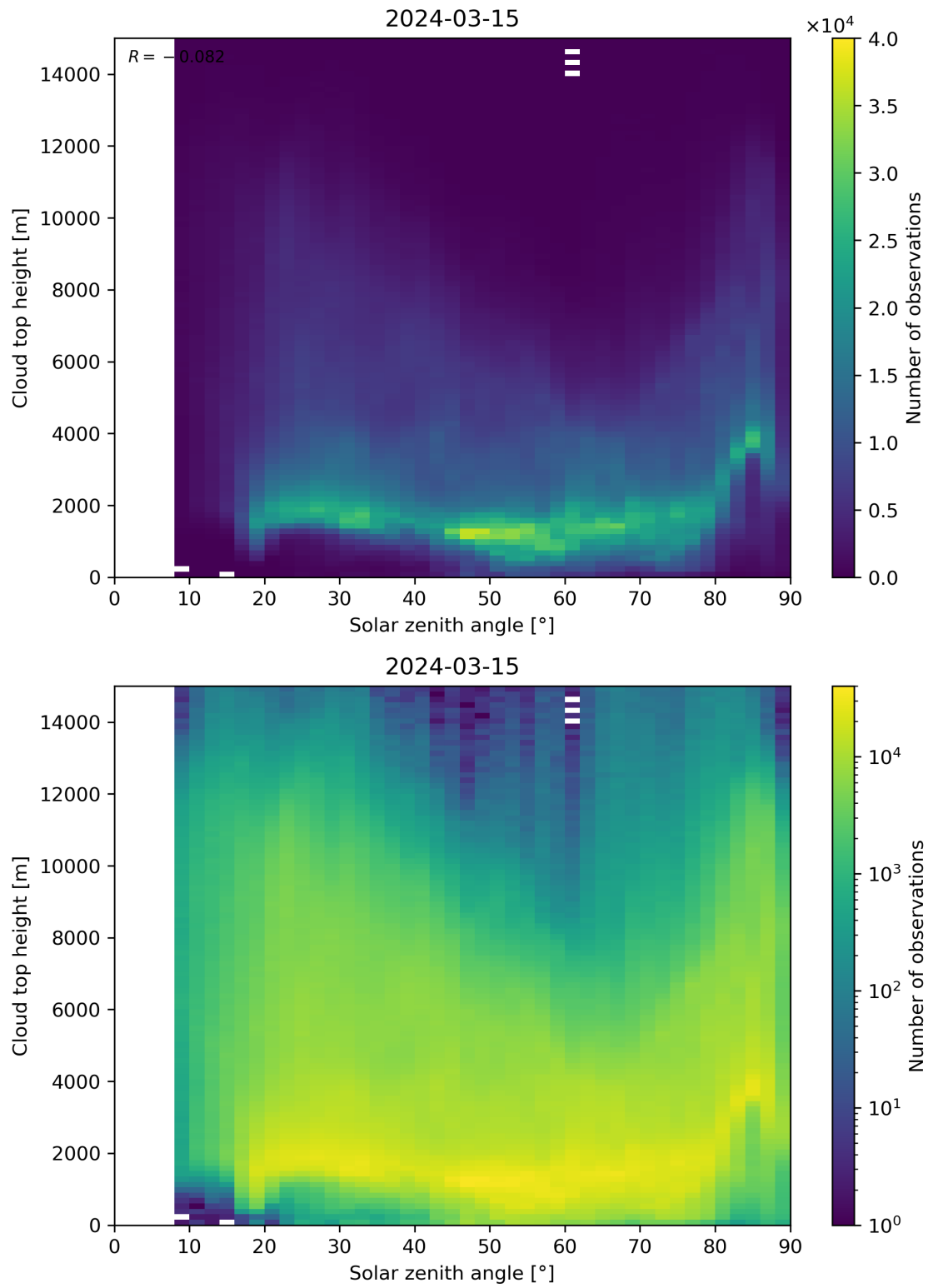
Figure 104: Scatter density plot of “Solar zenith angle” against “Cloud top height” for 2024-03-14 to 2024-03-16.
