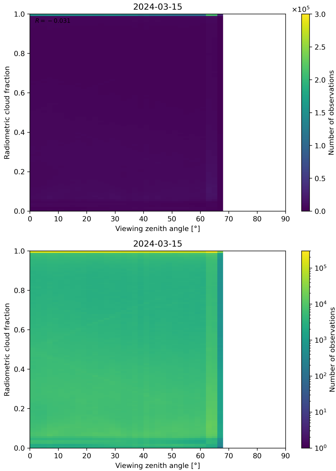
Figure 107: Scatter density plot of “Viewing zenith angle” against “Radiometric cloud fraction” for 2024-03-14 to 2024-03-16.
