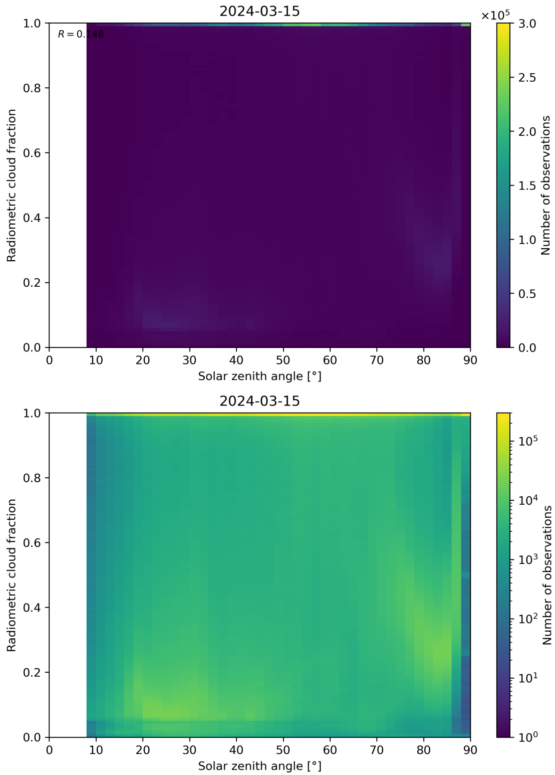
Figure 99: Scatter density plot of “Solar zenith angle” against “Radiometric cloud fraction” for 2024-03-14 to 2024-03-16.
