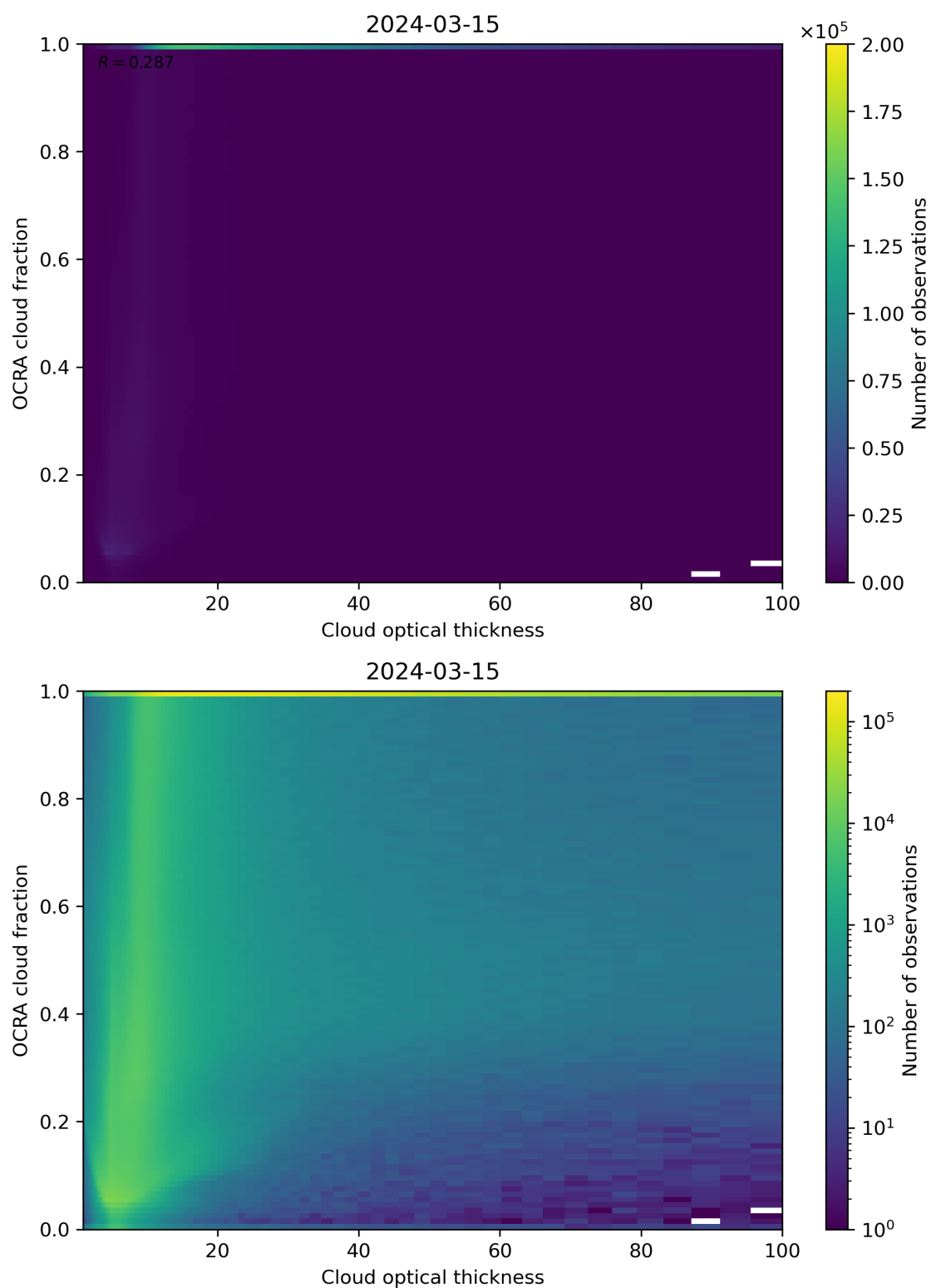
Figure 83: Scatter density plot of “Cloud optical thickness” against “OCRA cloud fraction” for 2024-03-14 to 2024-03-16.
