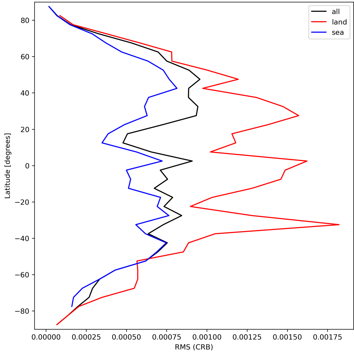
Figure 32: Zonal average of “RMS (CRB)” for 2024-03-14 to 2024-03-16.
