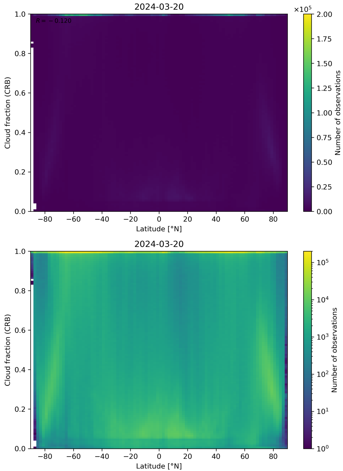
Figure 94: Scatter density plot of “Latitude” against “Cloud fraction (CRB)” for 2024-03-20 to 2024-03-21.
