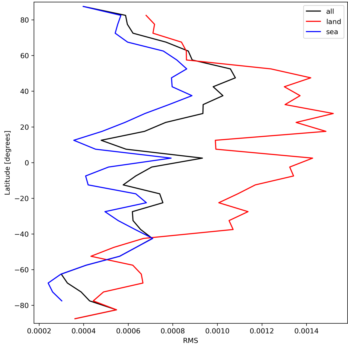
Figure 31: Zonal average of “RMS” for 2024-03-20 to 2024-03-21.
