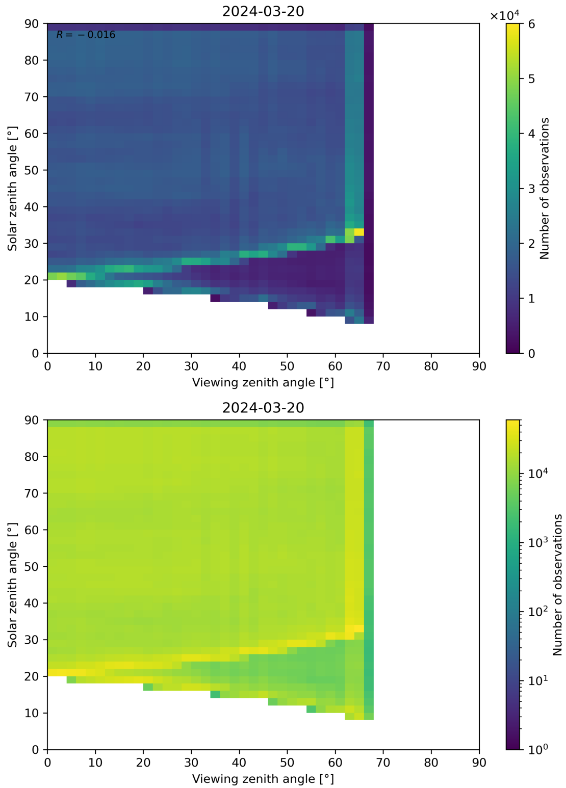
Figure 114: Scatter density plot of “Viewing zenith angle” against “Solar zenith angle” for 2024-03-20 to 2024-03-21.
