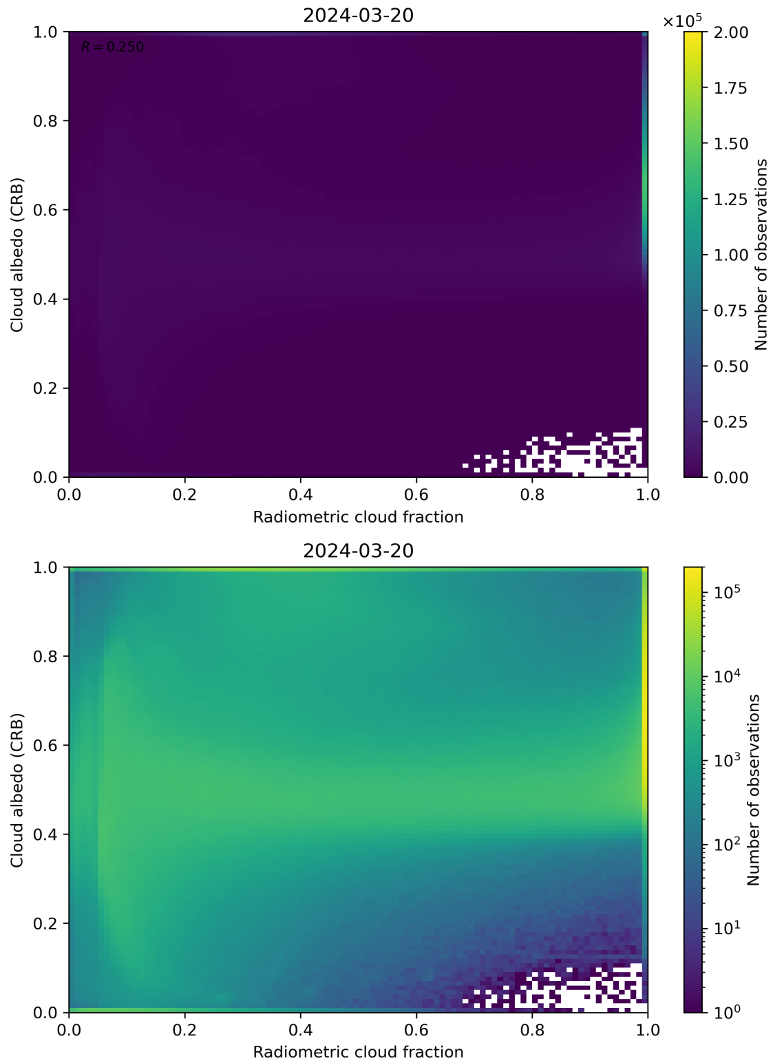
Figure 71: Scatter density plot of “Radiometric cloud fraction” against “Cloud albedo (CRB)” for 2024-03-20 to 2024-03-21.
