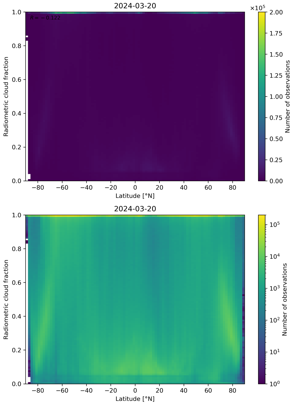
Figure 92: Scatter density plot of “Latitude” against “Radiometric cloud fraction” for 2024-03-20 to 2024-03-21.
