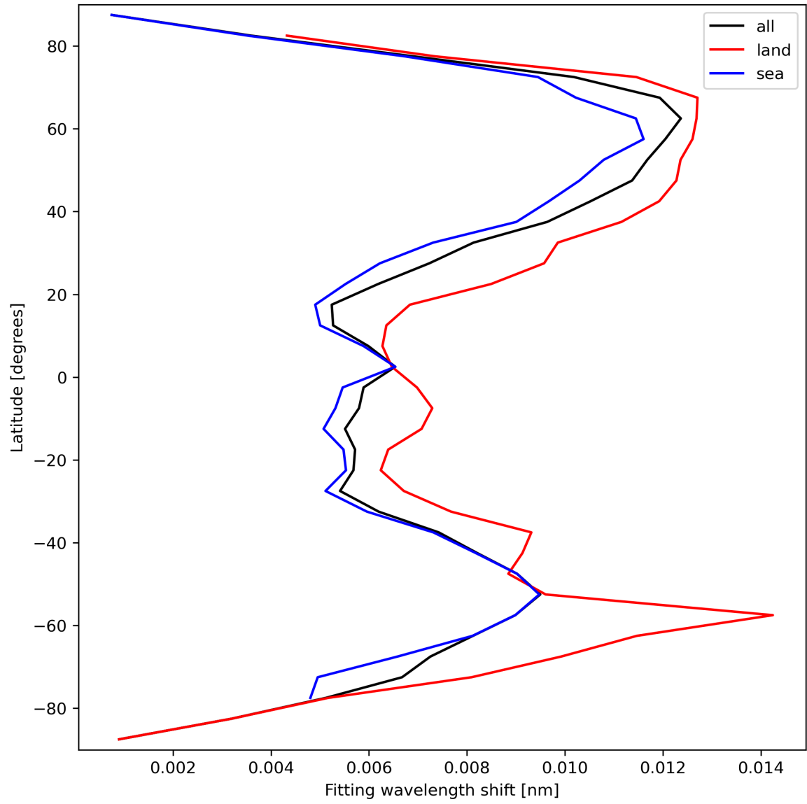
Figure 33: Zonal average of “Fitting wavelength shift” for 2024-03-20 to 2024-03-21.
