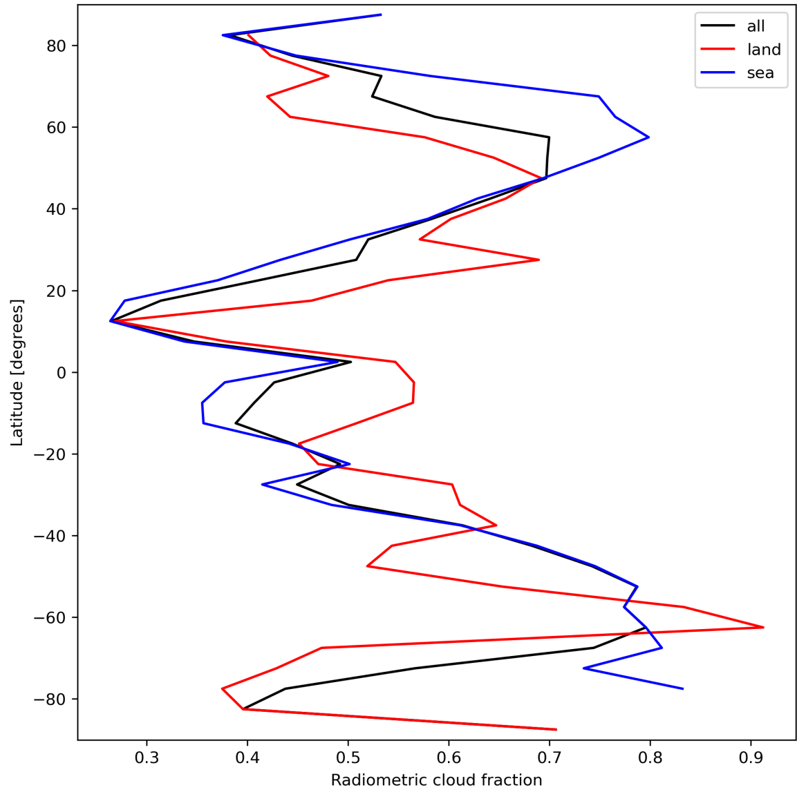
Figure 23: Zonal average of “Radiometric cloud fraction” for 2024-03-20 to 2024-03-21.
