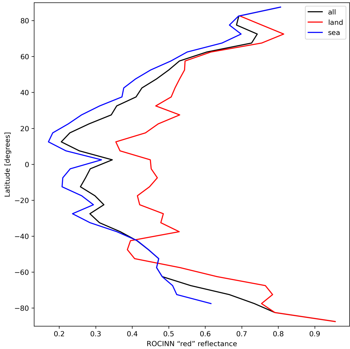
Figure 37: Zonal average of “ROCINN “red” reflectance” for 2024-03-20 to 2024-03-21.
