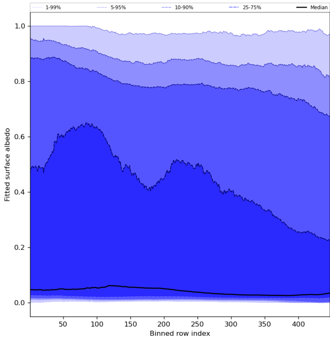
Figure 61: Along track statistics of “Fitted surface albedo” for 2024-03-20 to 2024-03-21
