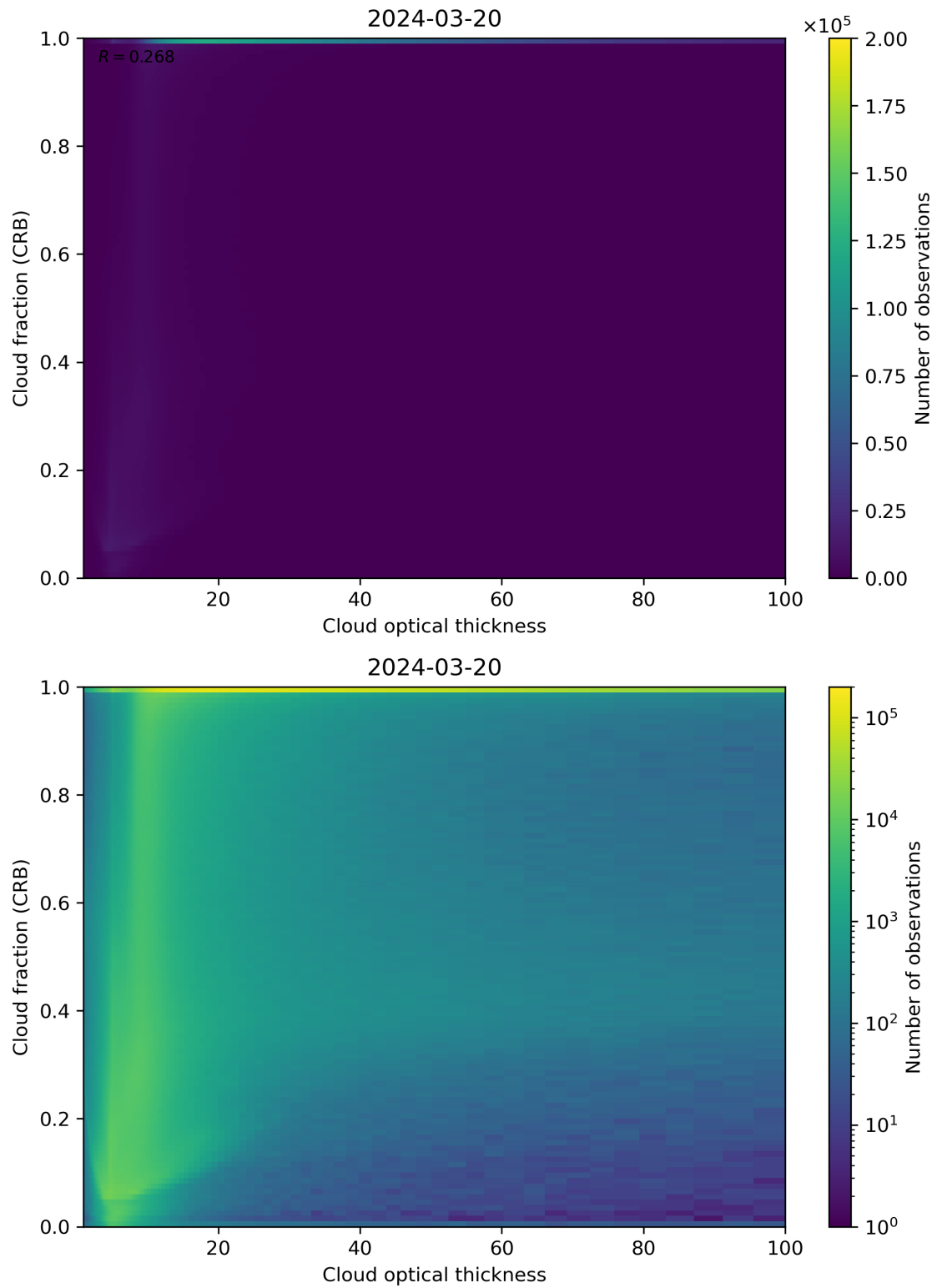
Figure 84: Scatter density plot of “Cloud optical thickness” against “Cloud fraction (CRB)” for 2024-03-20 to 2024-03-21.
