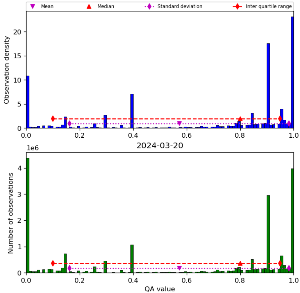
Figure 38: Histogram of “QA value” for 2024-03-20 to 2024-03-21
