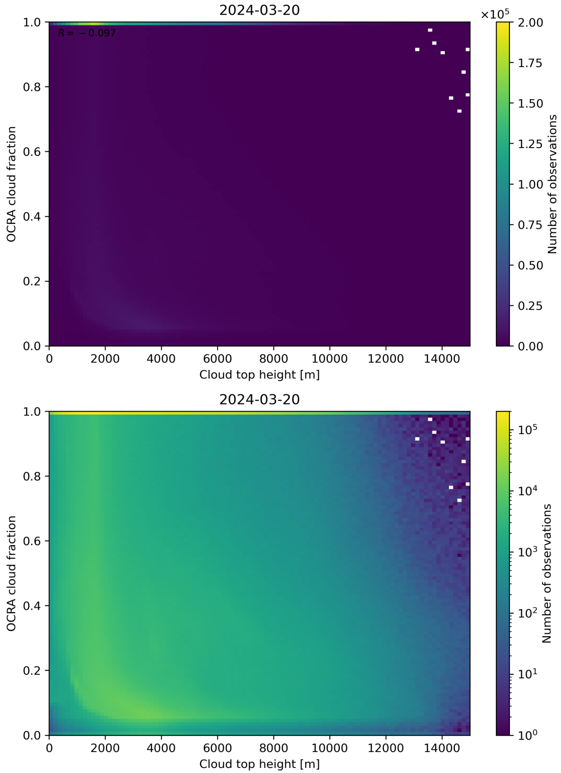
Figure 87: Scatter density plot of “Cloud top height” against “OCRA cloud fraction” for 2024-03-20 to 2024-03-21.
