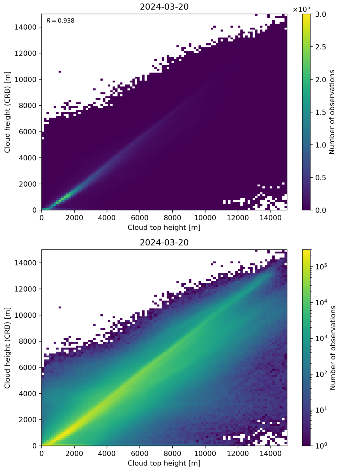
Figure 89: Scatter density plot of “Cloud top height” against “Cloud height (CRB)” for 2024-03-20 to 2024-03-21.
