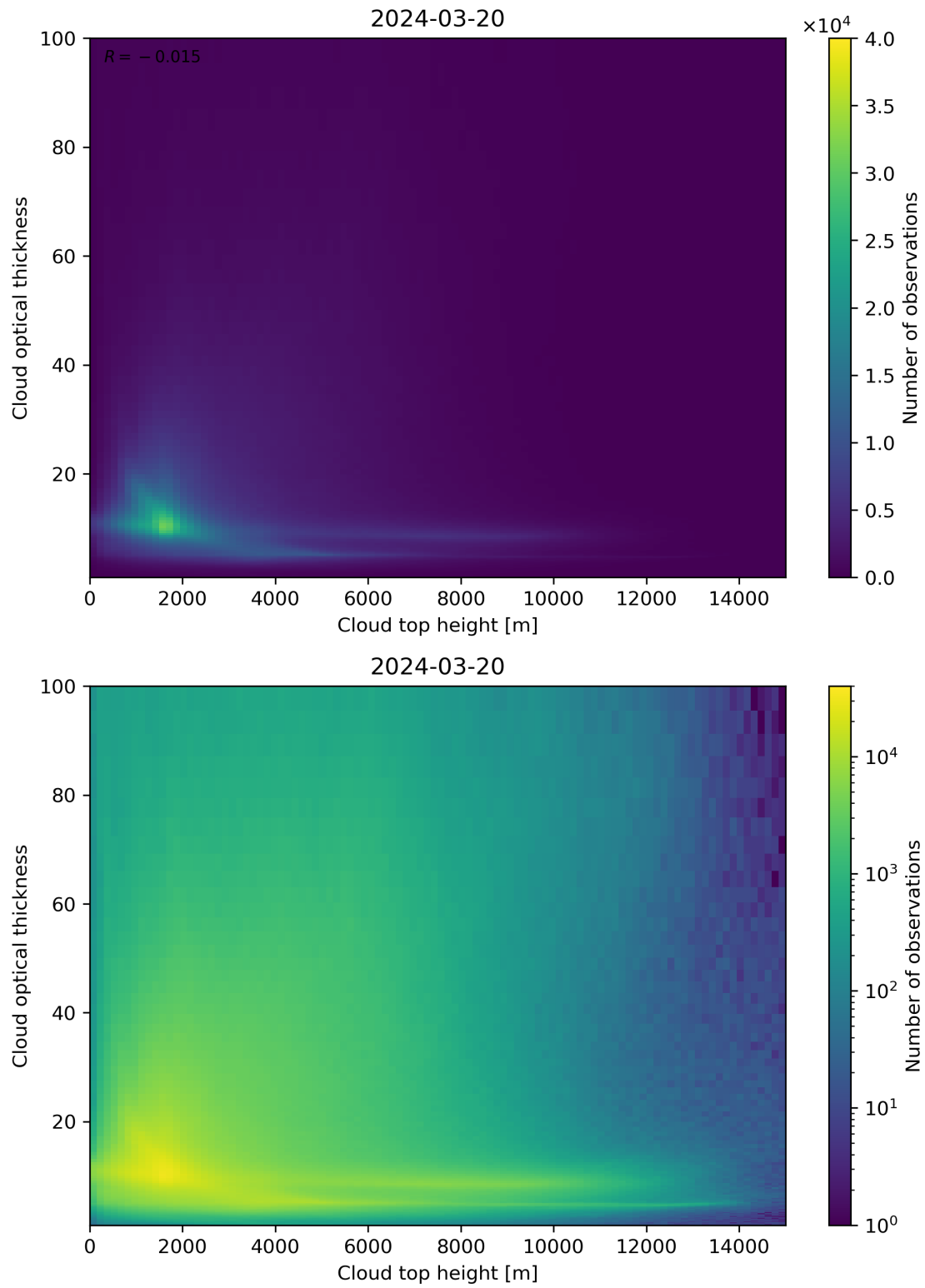
Figure 90: Scatter density plot of “Cloud top height” against “Cloud optical thickness” for 2024-03-20 to 2024-03-21.
