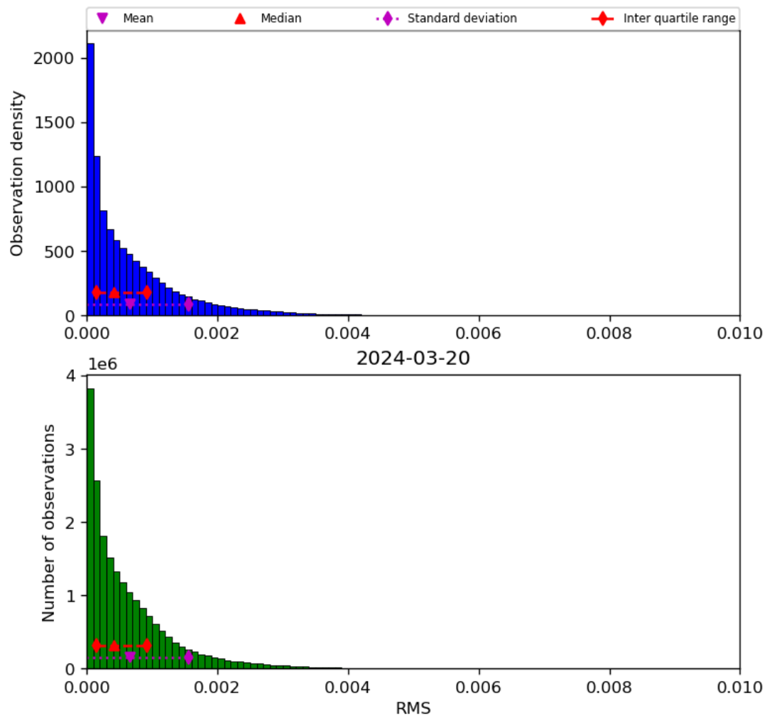
Figure 47: Histogram of “RMS” for 2024-03-20 to 2024-03-21
