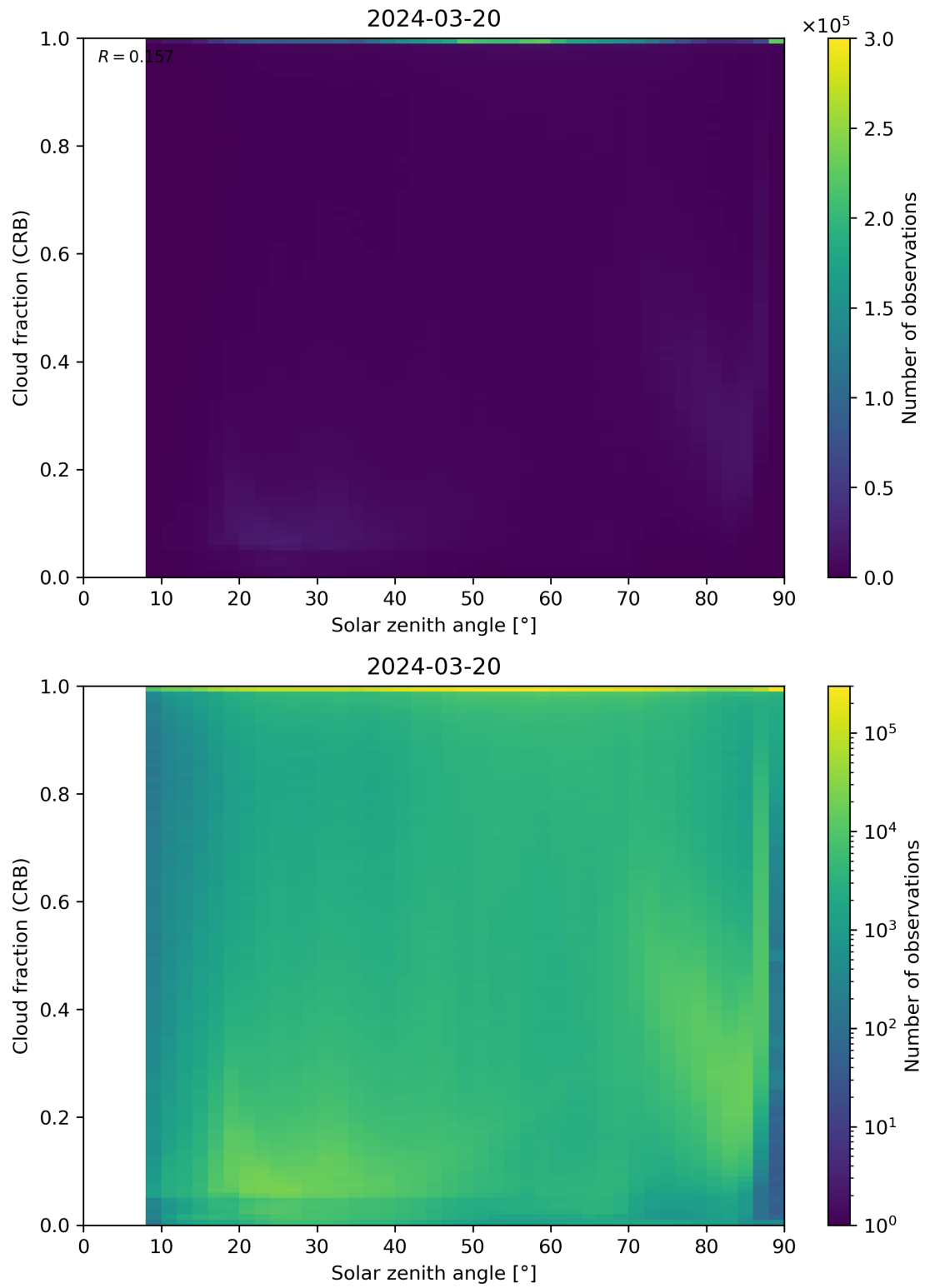
Figure 101: Scatter density plot of “Solar zenith angle” against “Cloud fraction (CRB)” for 2024-03-20 to 2024-03-21.
