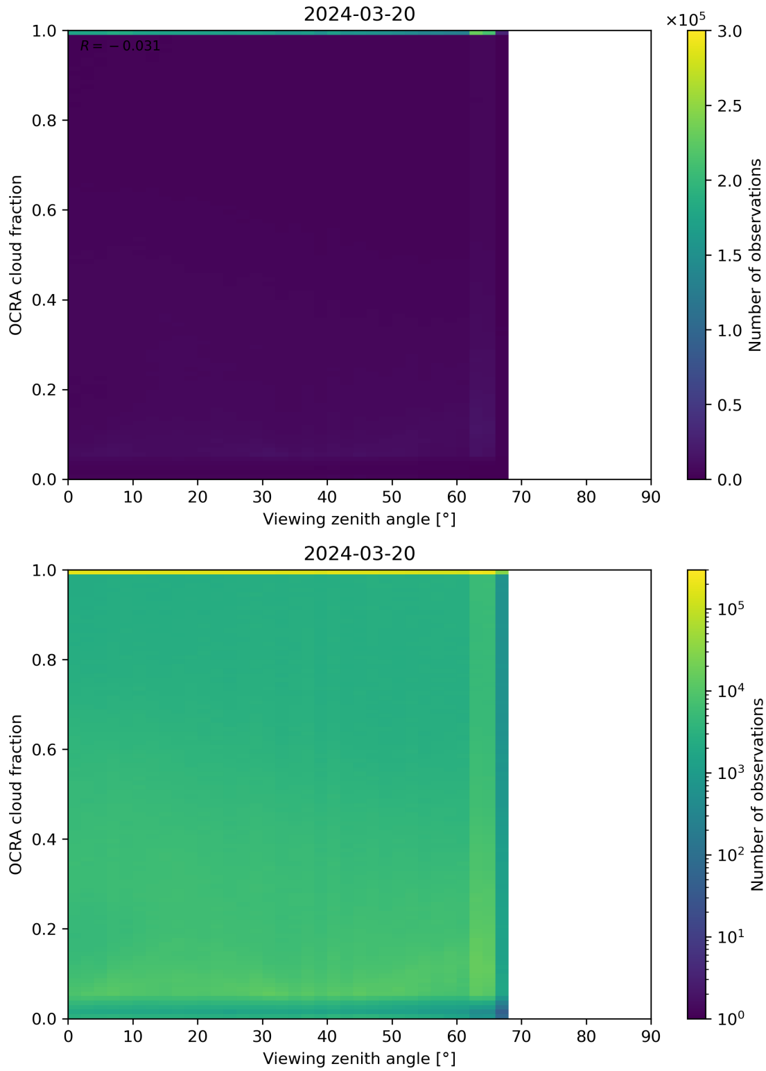
Figure 108: Scatter density plot of “Viewing zenith angle” against “OCRA cloud fraction” for 2024-03-20 to 2024-03-21.
