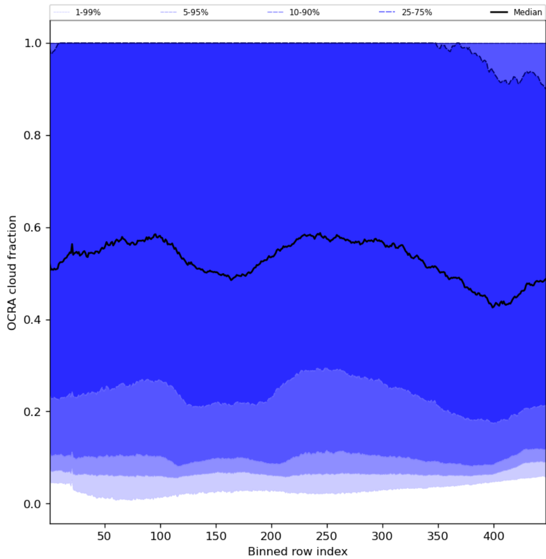
Figure 66: Along track statistics of “OCRA cloud fraction” for 2024-03-20 to 2024-03-21
