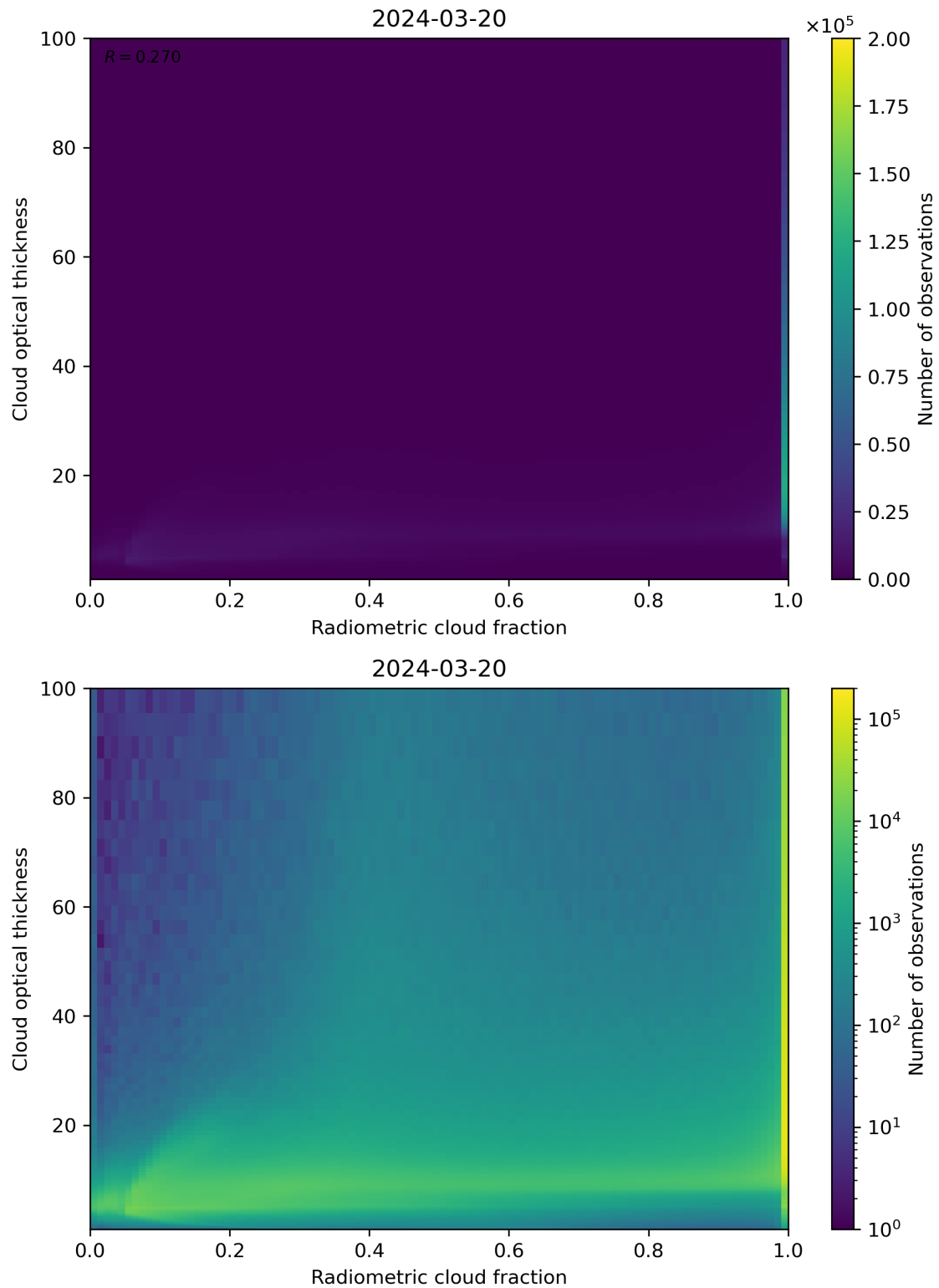
Figure 75: Scatter density plot of “Radiometric cloud fraction” against “Cloud optical thickness” for 2024-03-20 to 2024-03-21.
