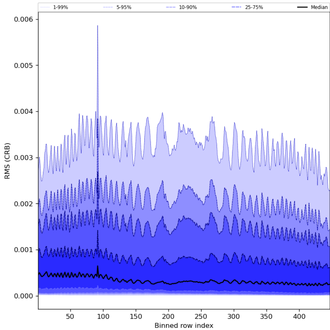
Figure 64: Along track statistics of “RMS (CRB)” for 2024-03-20 to 2024-03-21
