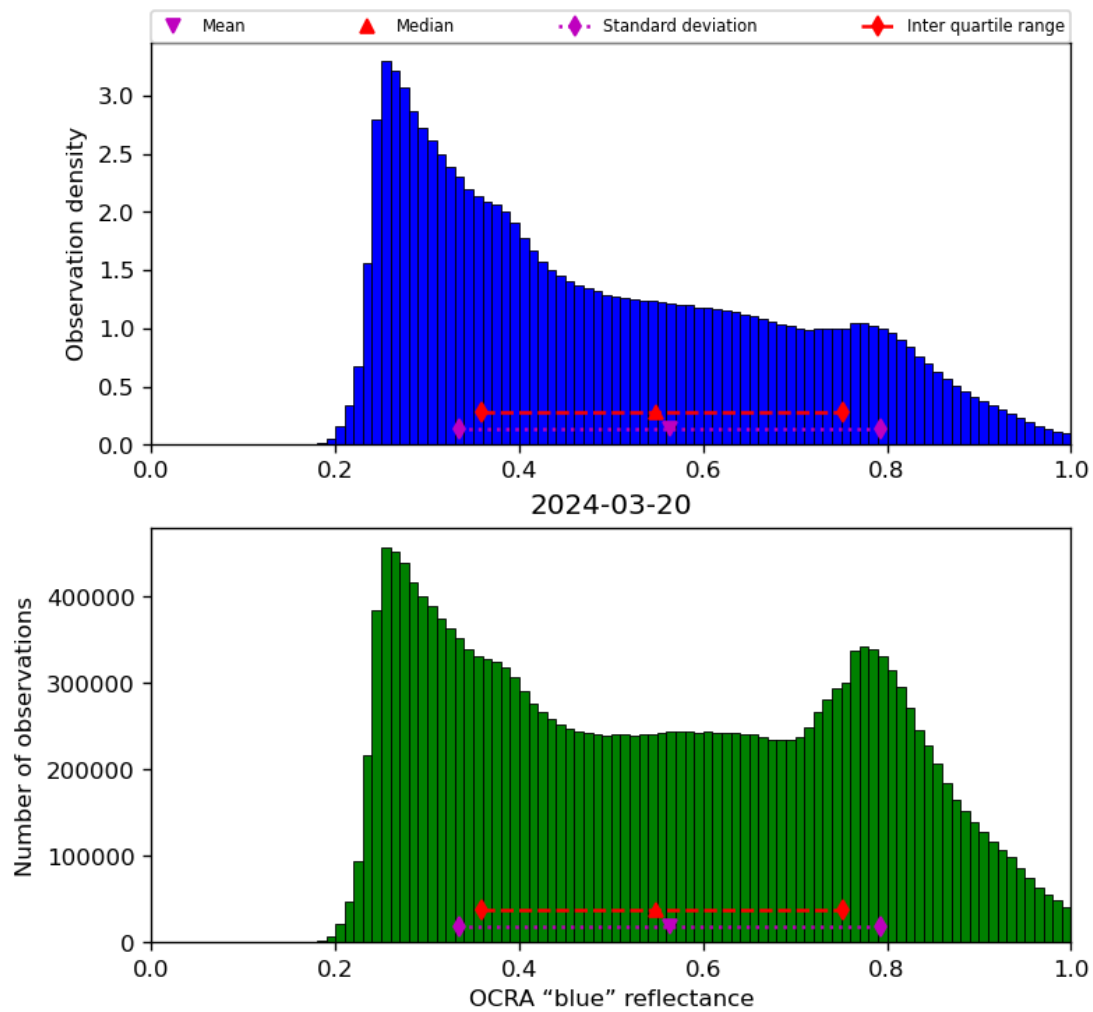
Figure 51: Histogram of “OCRA “blue” reflectance” for 2024-03-20 to 2024-03-21
