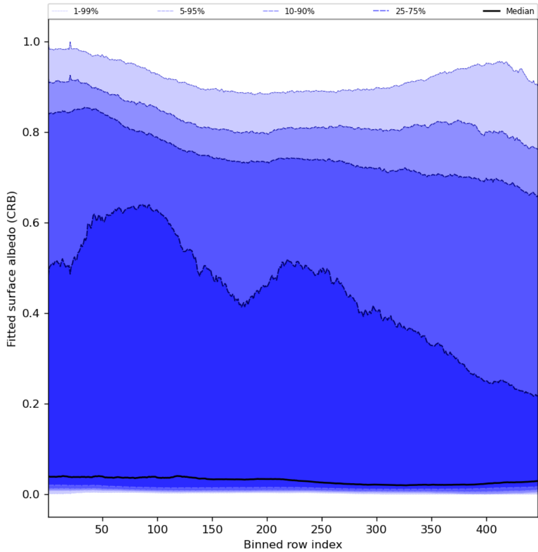
Figure 62: Along track statistics of “Fitted surface albedo (CRB)” for 2024-03-20 to 2024-03-21
