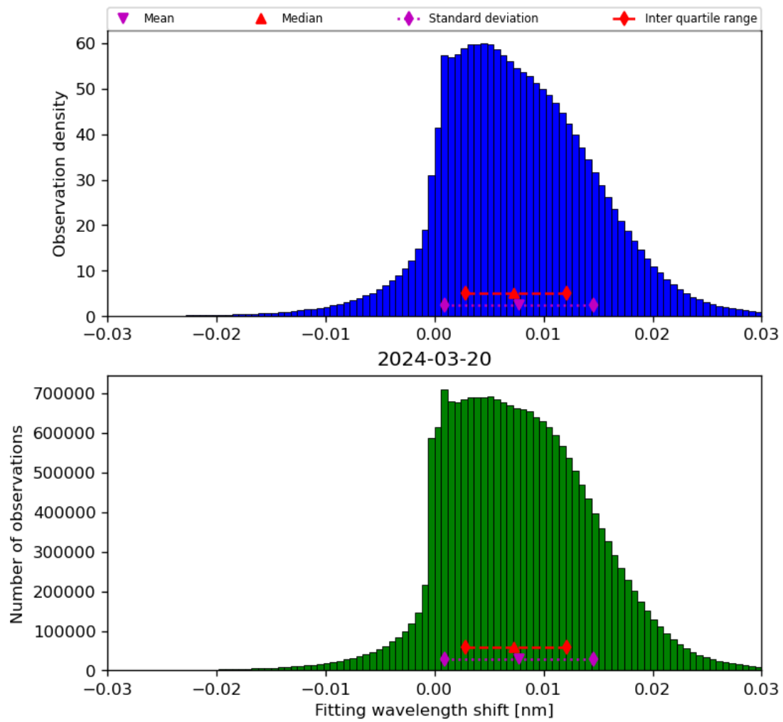
Figure 49: Histogram of “Fitting wavelength shift” for 2024-03-20 to 2024-03-21
