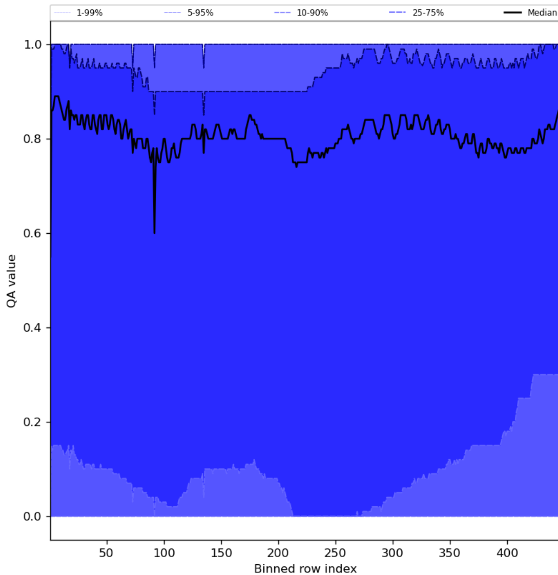
Figure 54: Along track statistics of “QA value” for 2024-03-20 to 2024-03-21
