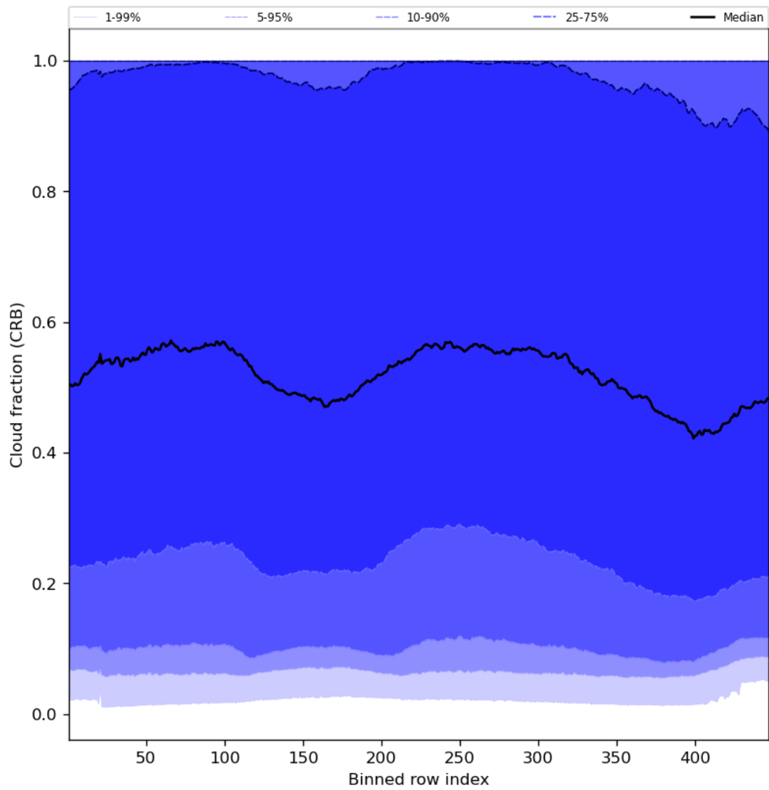
Figure 58: Along track statistics of “Cloud fraction (CRB)” for 2024-03-20 to 2024-03-21
