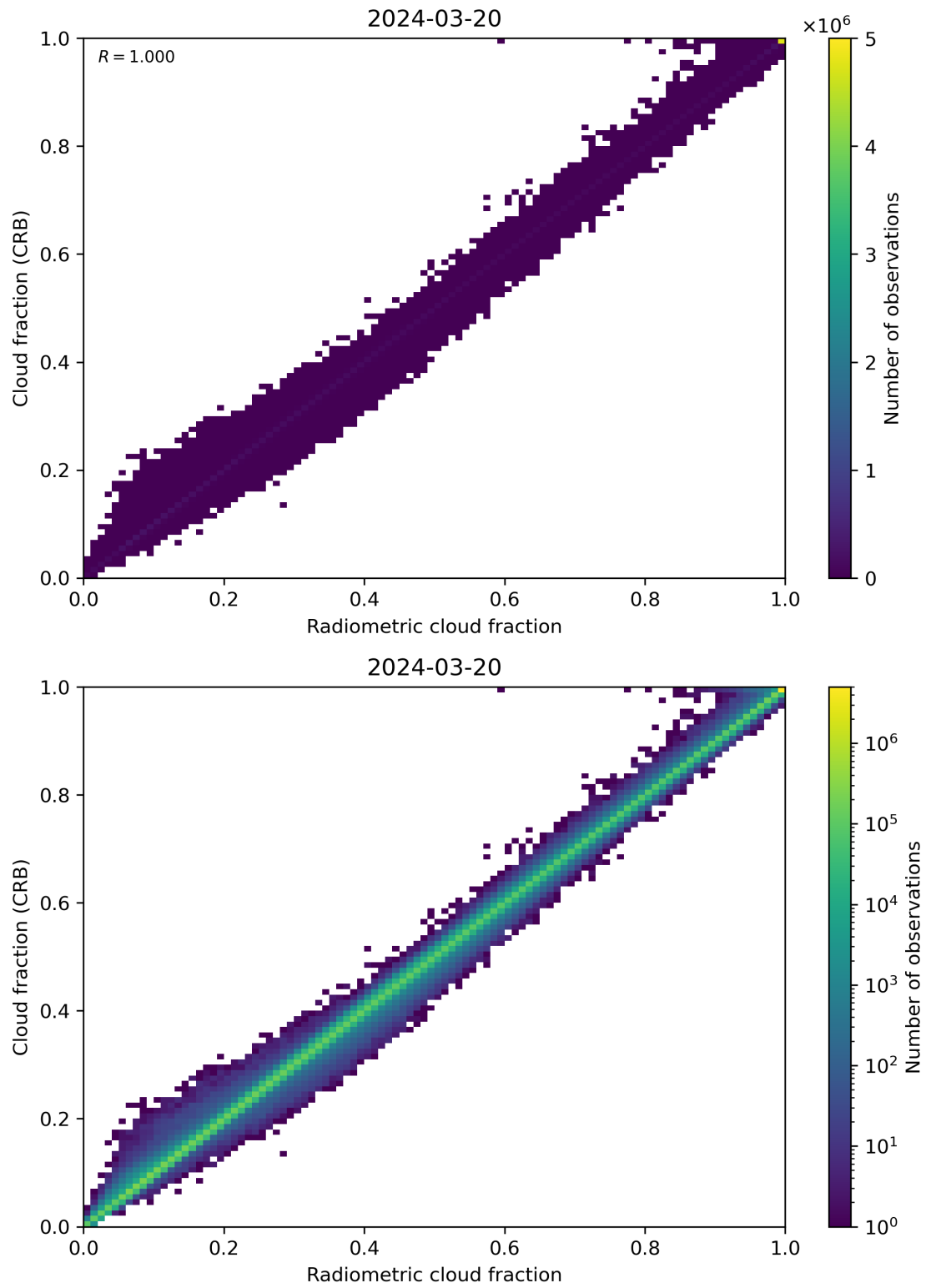
Figure 73: Scatter density plot of “Radiometric cloud fraction” against “Cloud fraction (CRB)” for 2024-03-20 to 2024-03-21.
