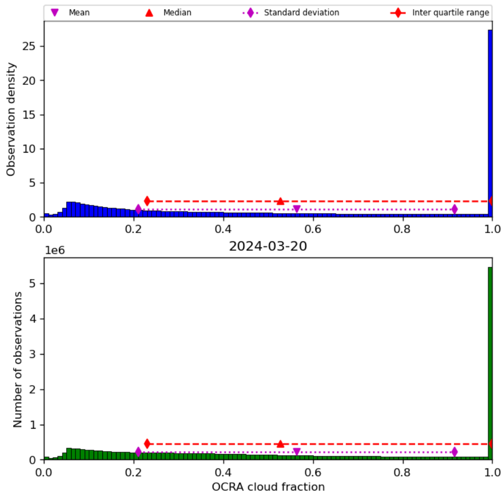
Figure 50: Histogram of “OCRA cloud fraction” for 2024-03-20 to 2024-03-21
