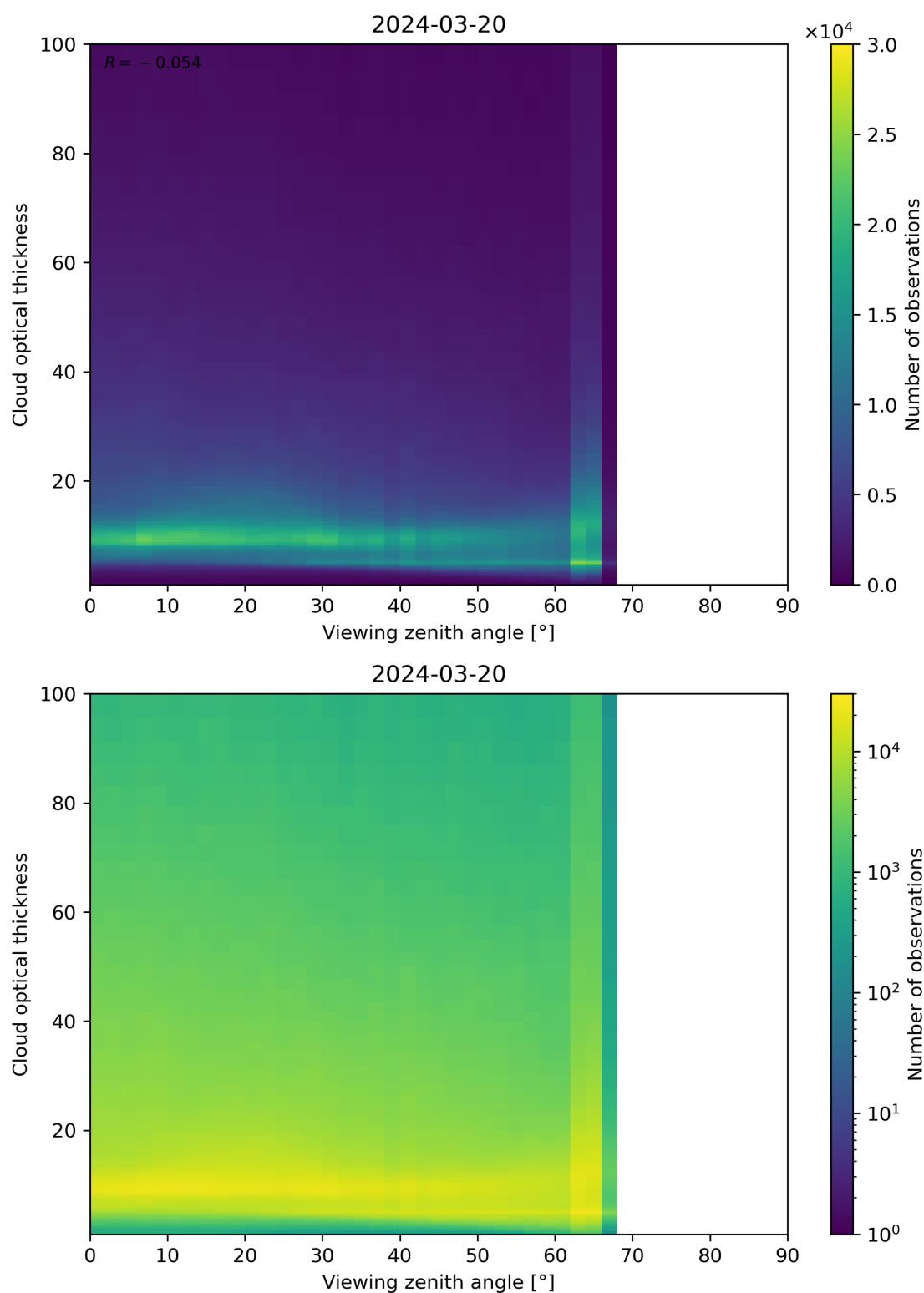
Figure 111: Scatter density plot of “Viewing zenith angle” against “Cloud optical thickness” for 2024-03-20 to 2024-03-21.
