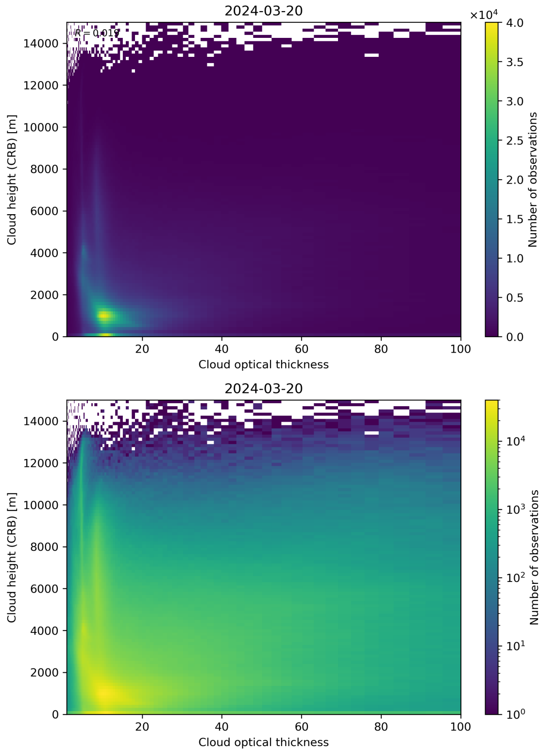
Figure 85: Scatter density plot of “Cloud optical thickness” against “Cloud height (CRB)” for 2024-03-20 to 2024-03-21.
