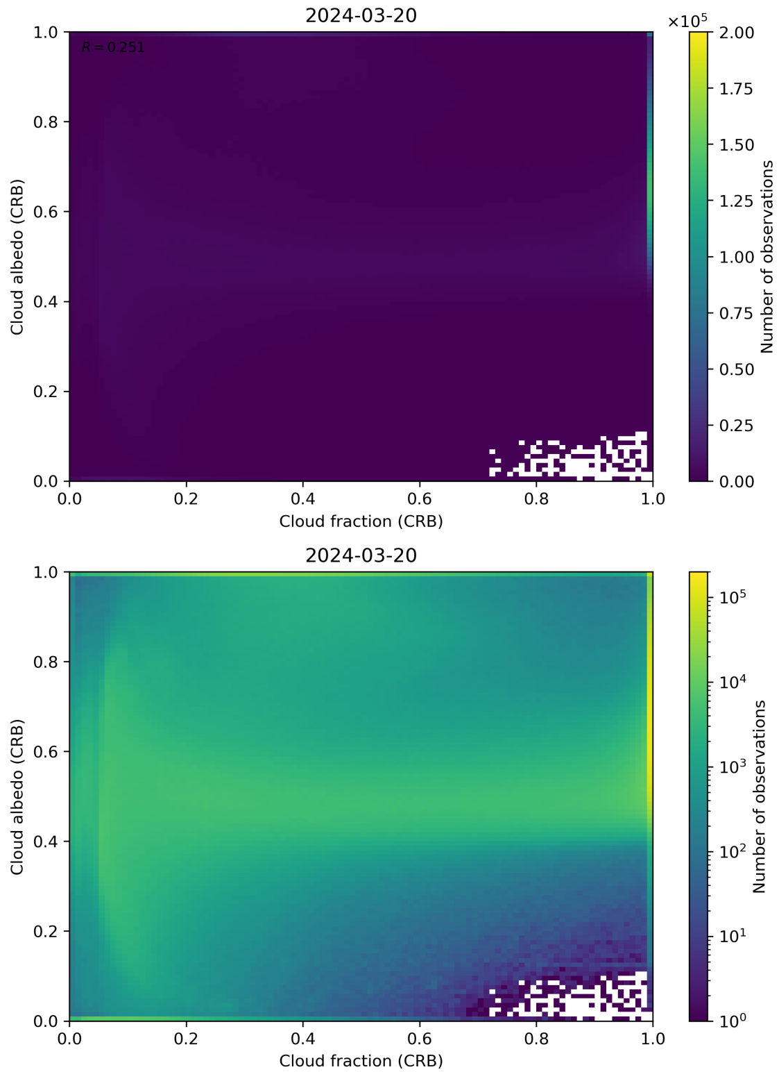
Figure 77: Scatter density plot of “Cloud fraction (CRB)” against “Cloud albedo (CRB)” for 2024-03-20 to 2024-03-21.
