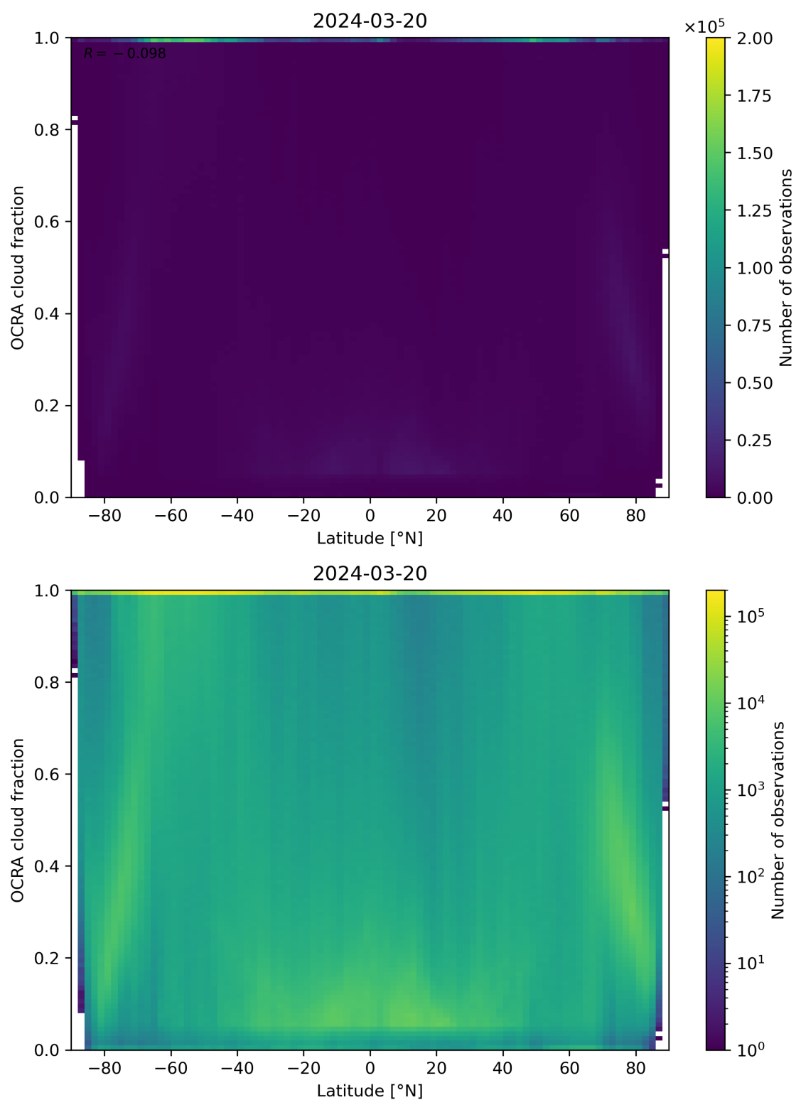
Figure 93: Scatter density plot of “Latitude” against “OCRA cloud fraction” for 2024-03-20 to 2024-03-21.
