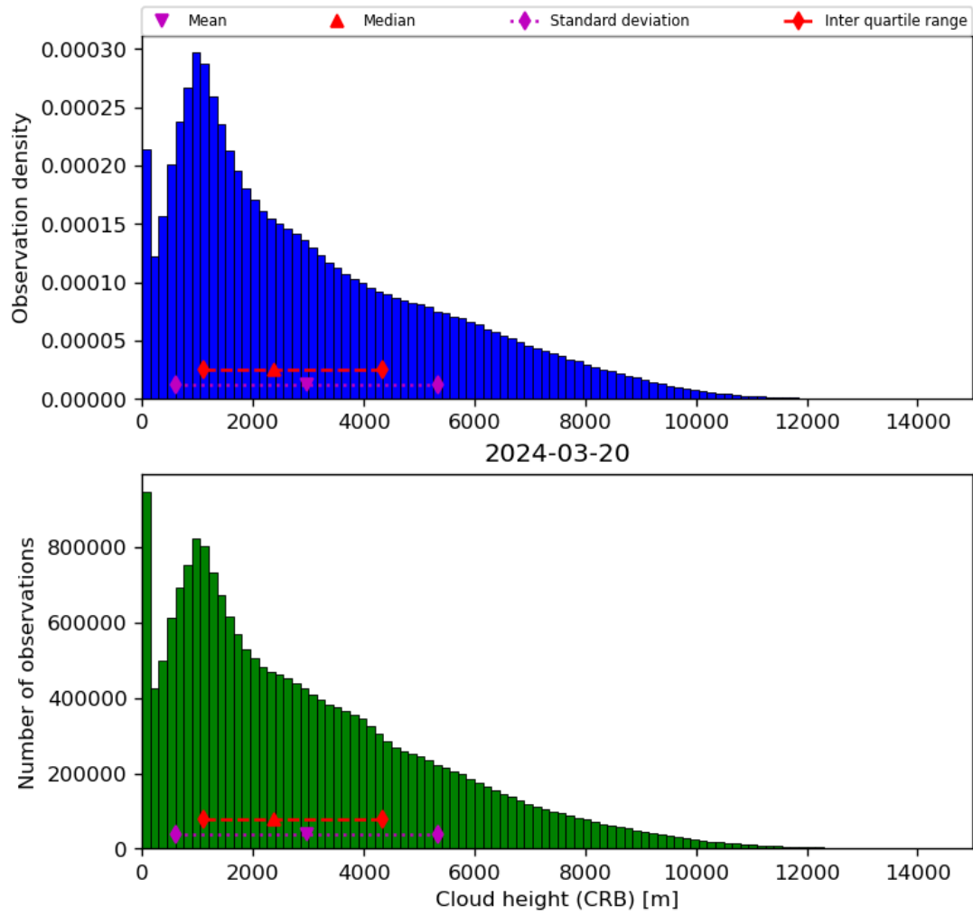
Figure 43: Histogram of “Cloud height (CRB)” for 2024-03-20 to 2024-03-21
