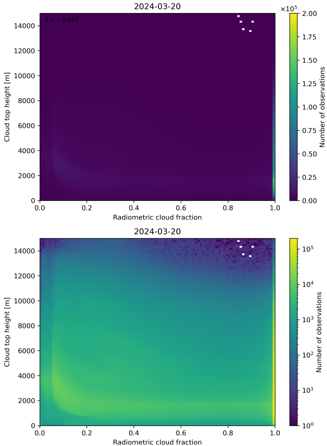
Figure 76: Scatter density plot of “Radiometric cloud fraction” against “Cloud top height” for 2024-03-20 to 2024-03-21.
