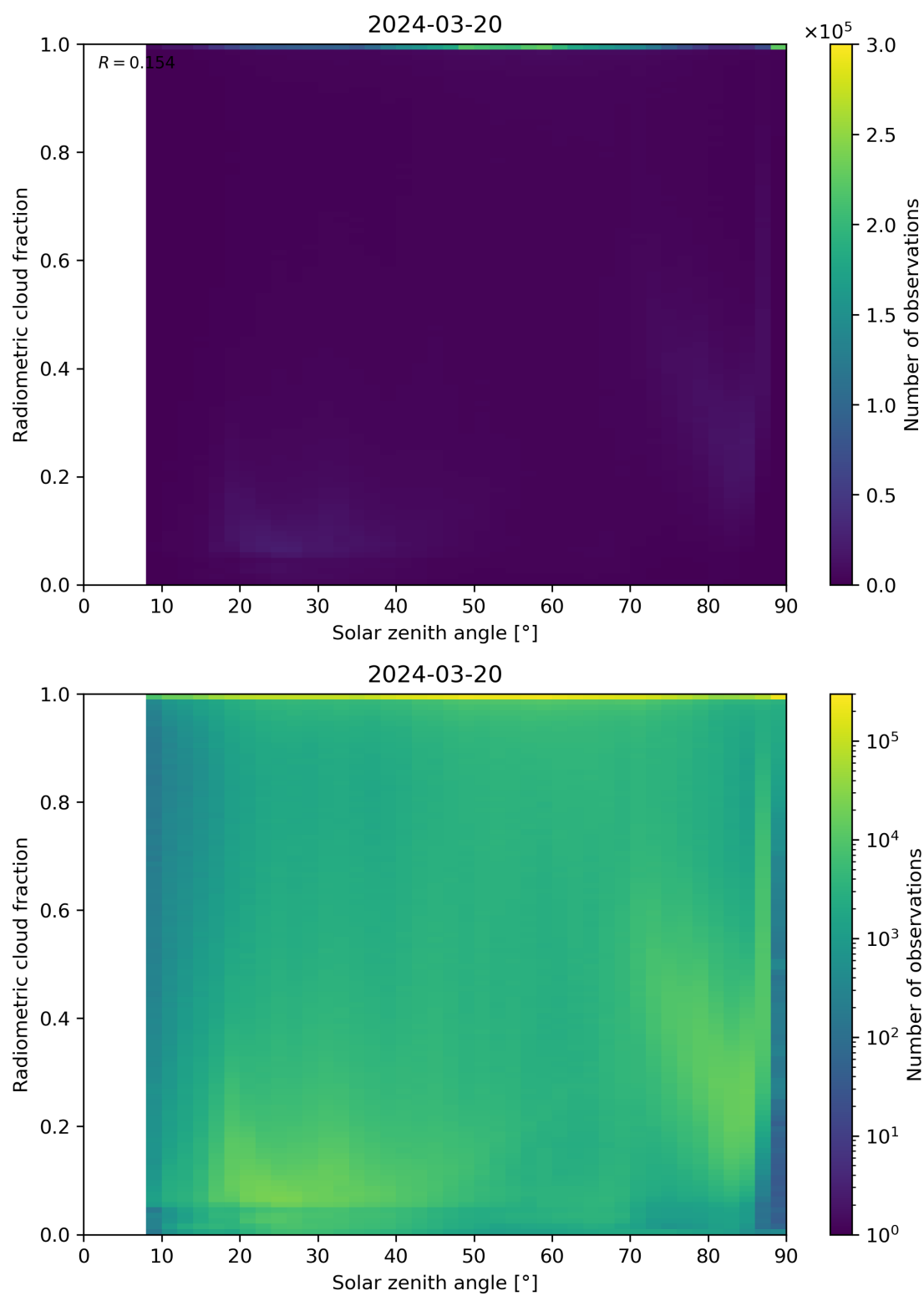
Figure 99: Scatter density plot of “Solar zenith angle” against “Radiometric cloud fraction” for 2024-03-20 to 2024-03-21.
