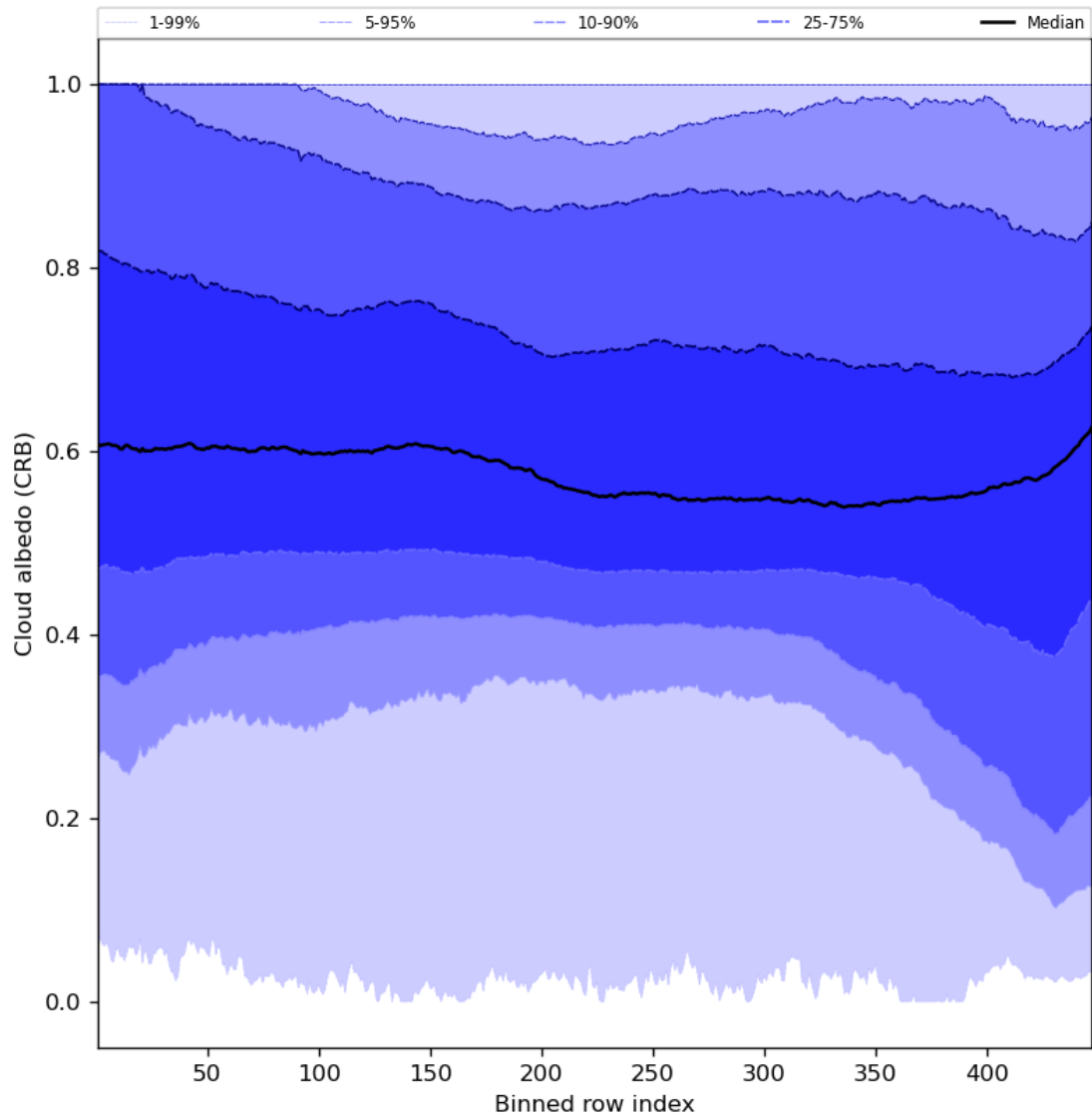
Figure 60: Along track statistics of “Cloud albedo (CRB)” for 2024-03-20 to 2024-03-21
