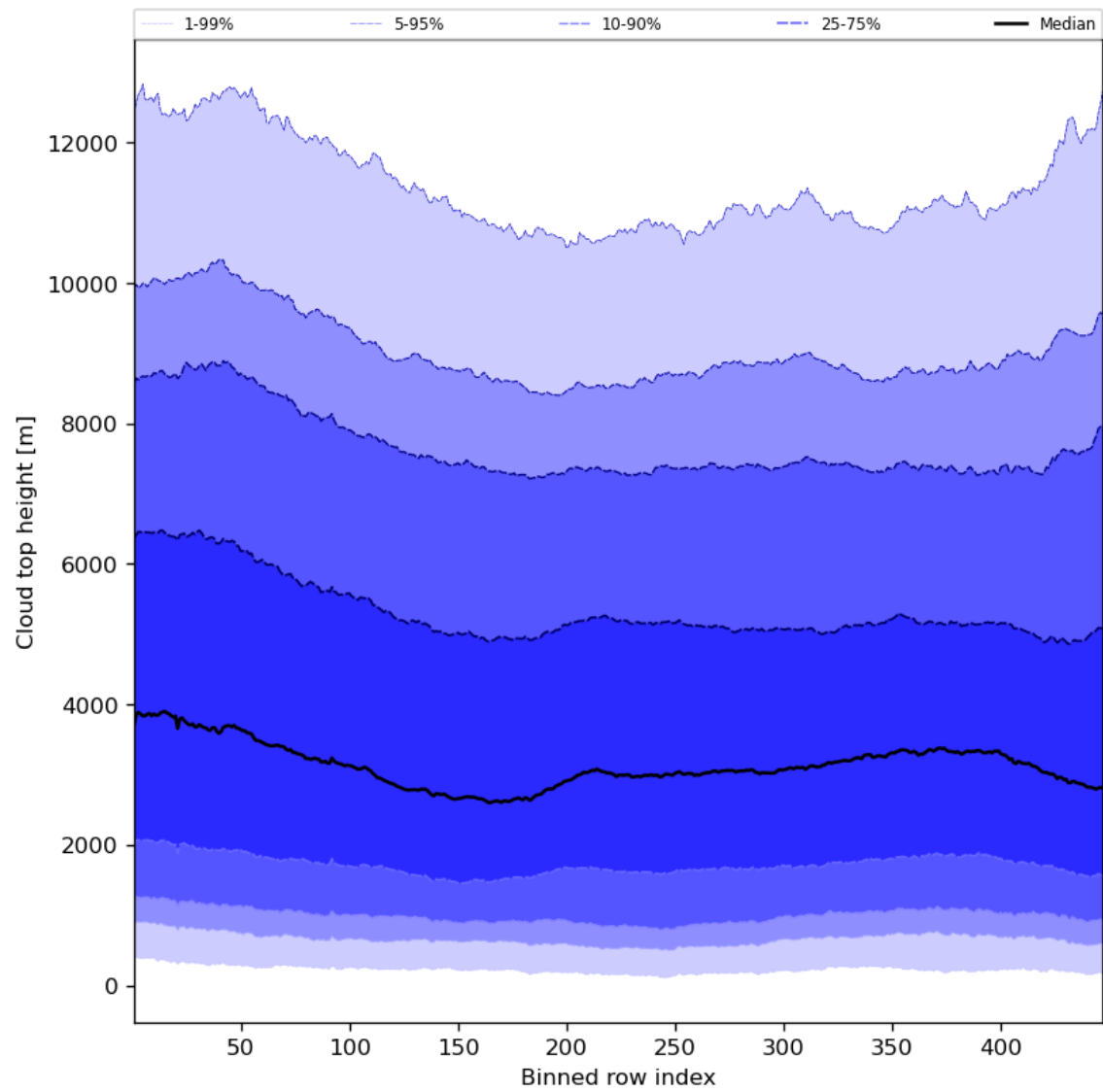
Figure 56: Along track statistics of “Cloud top height” for 2024-03-20 to 2024-03-21
