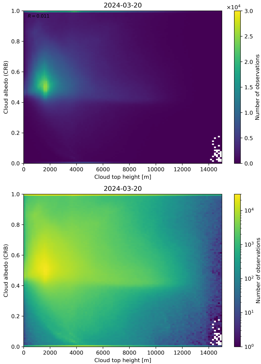
Figure 86: Scatter density plot of “Cloud top height” against “Cloud albedo (CRB)” for 2024-03-20 to 2024-03-21.
