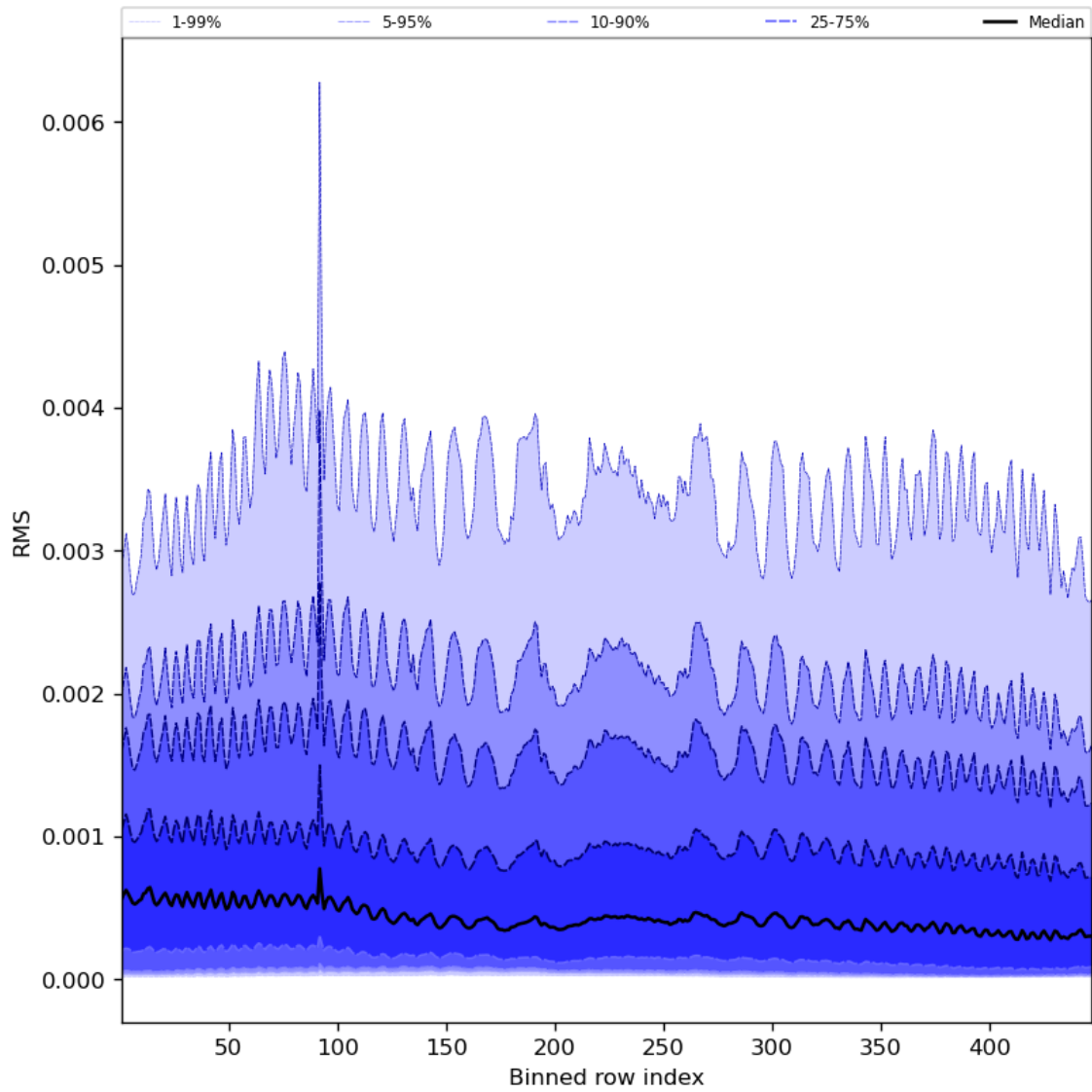
Figure 63: Along track statistics of “RMS” for 2024-03-20 to 2024-03-21
