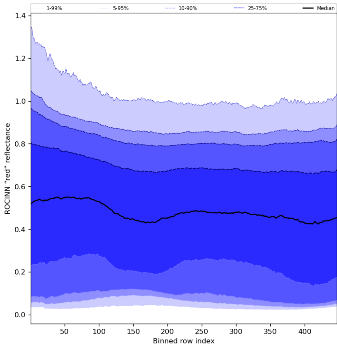
Figure 69: Along track statistics of “ROCINN “red” reflectance” for 2024-03-20 to 2024-03-21
