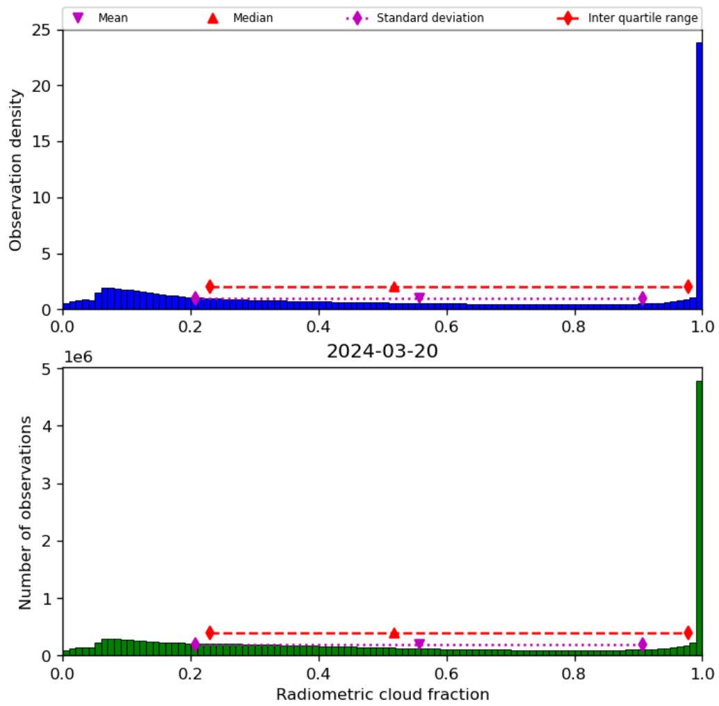
Figure 39: Histogram of “Radiometric cloud fraction” for 2024-03-20 to 2024-03-21
