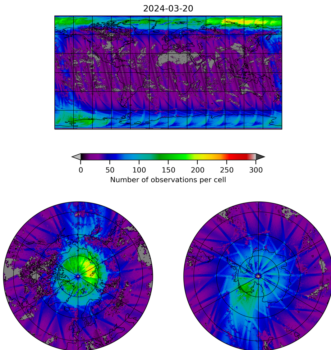
Figure 21: Map of the number of observations for 2024-03-20 to 2024-03-21
