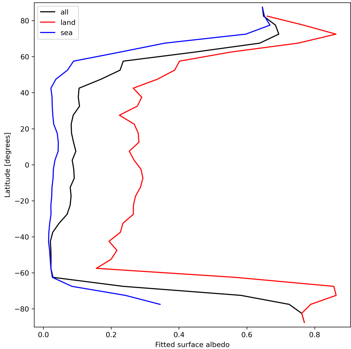
Figure 29: Zonal average of “Fitted surface albedo” for 2024-03-20 to 2024-03-21.
