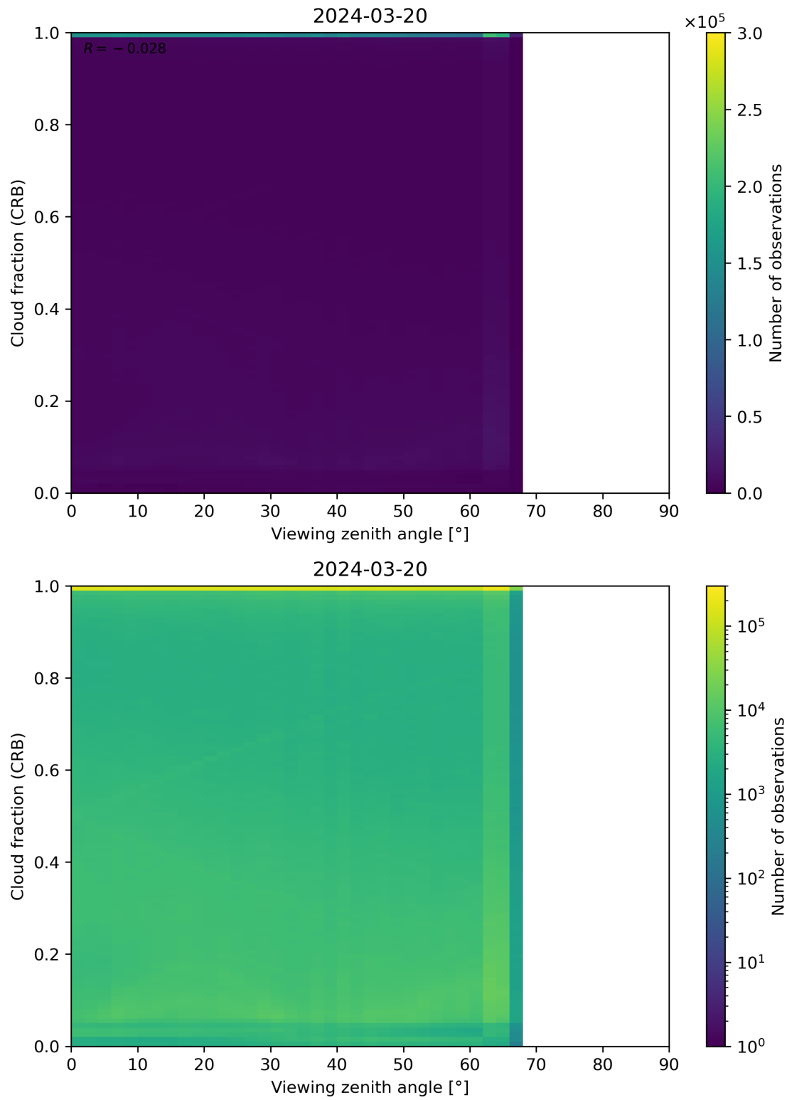
Figure 109: Scatter density plot of “Viewing zenith angle” against “Cloud fraction (CRB)” for 2024-03-20 to 2024-03-21.
