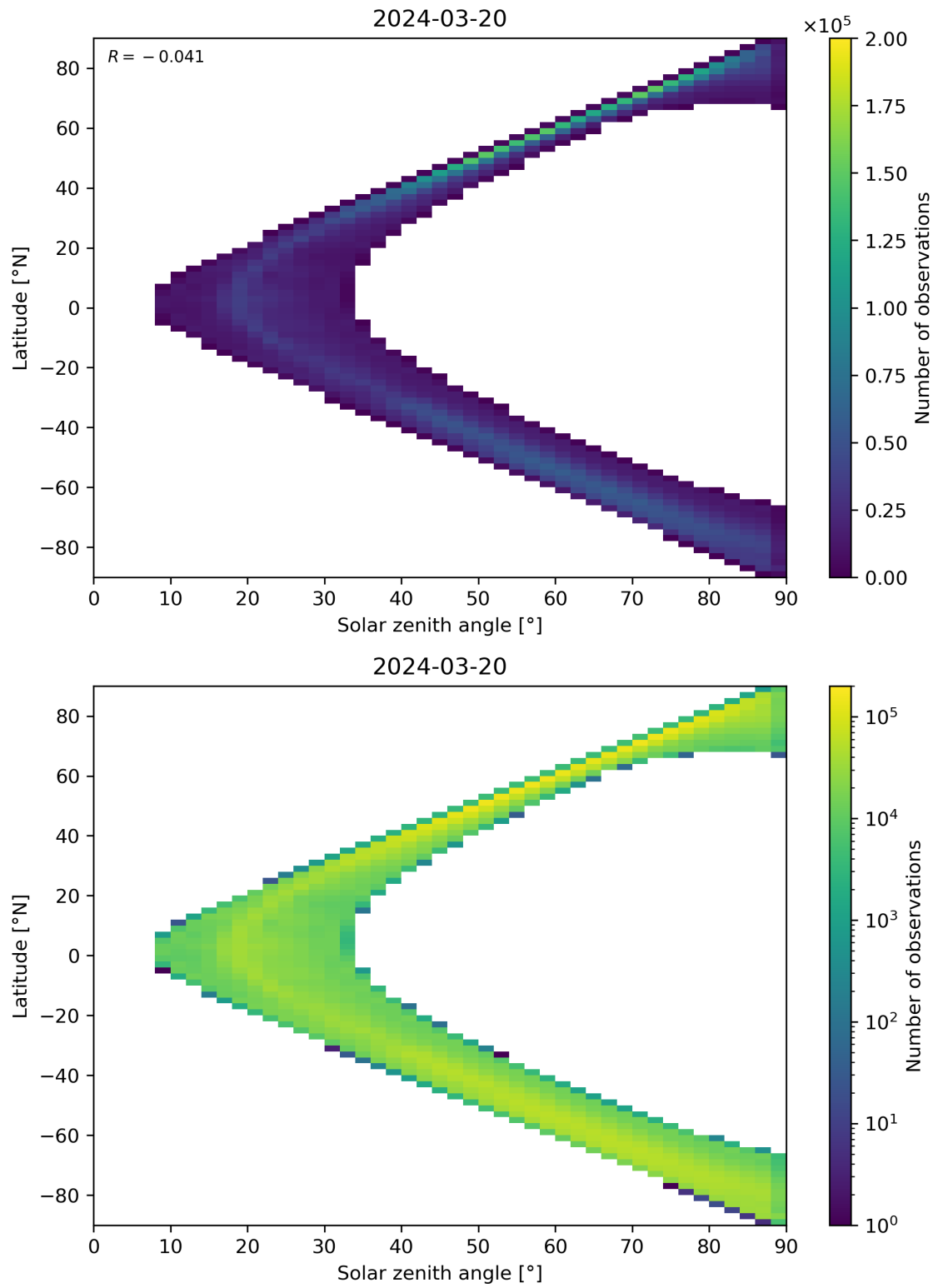
Figure 105: Scatter density plot of “Solar zenith angle” against “Latitude” for 2024-03-20 to 2024-03-21.
