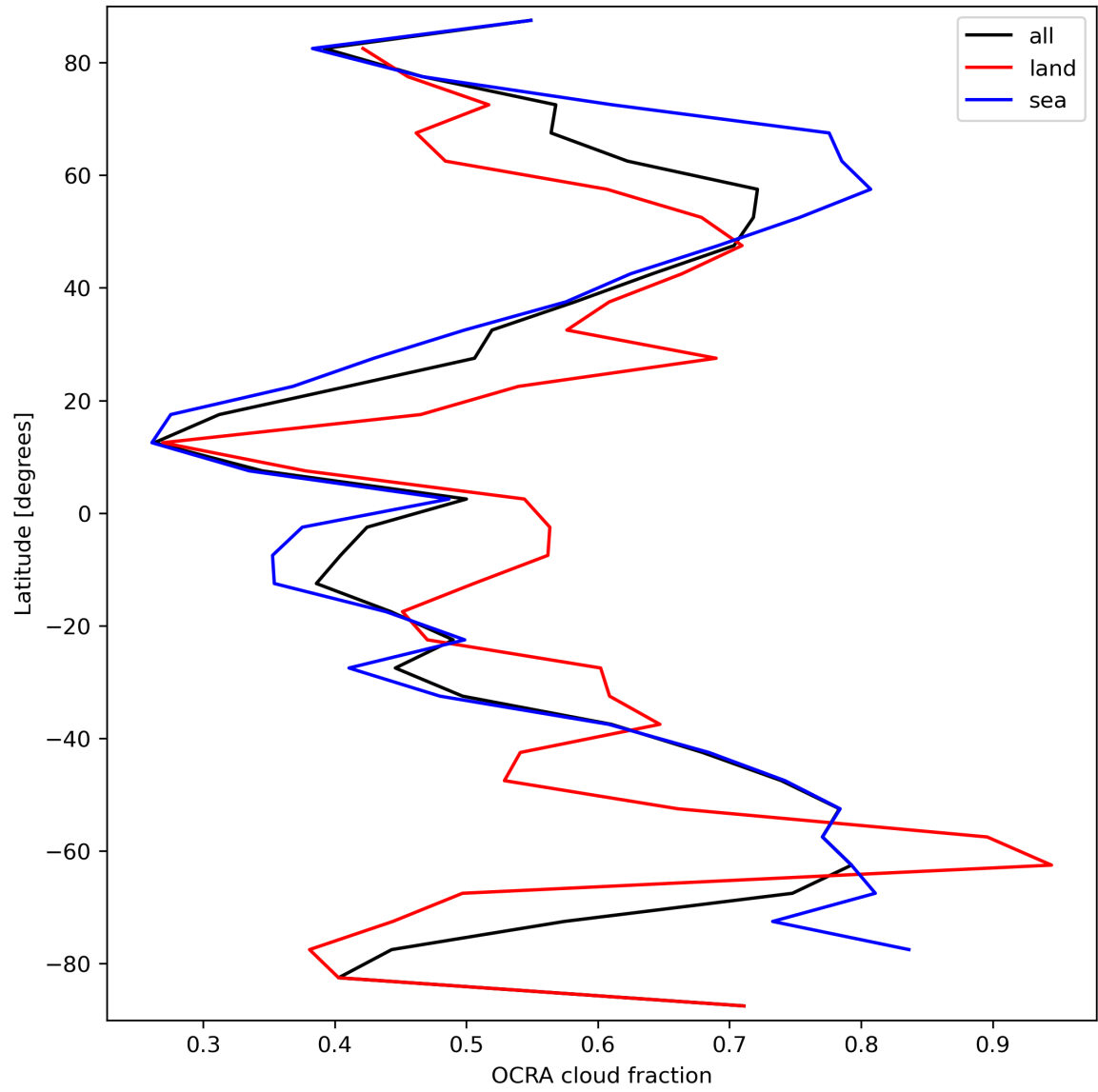
Figure 34: Zonal average of “OCRA cloud fraction” for 2024-03-20 to 2024-03-21.
