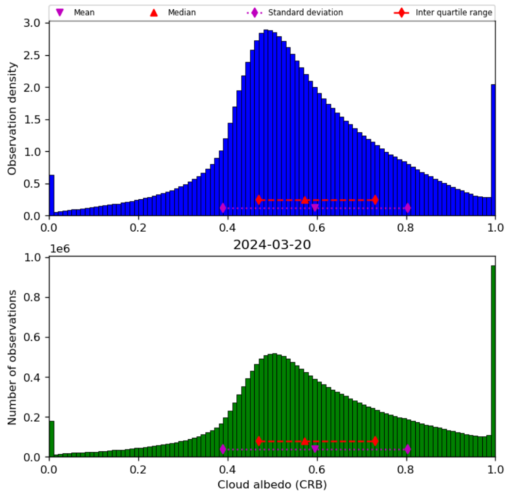
Figure 44: Histogram of “Cloud albedo (CRB)” for 2024-03-20 to 2024-03-21
