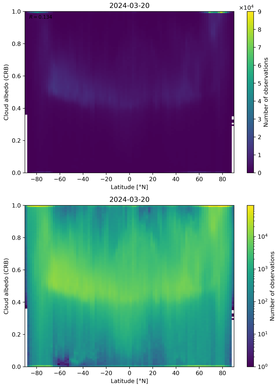
Figure 91: Scatter density plot of “Latitude” against “Cloud albedo (CRB)” for 2024-03-20 to 2024-03-21.
