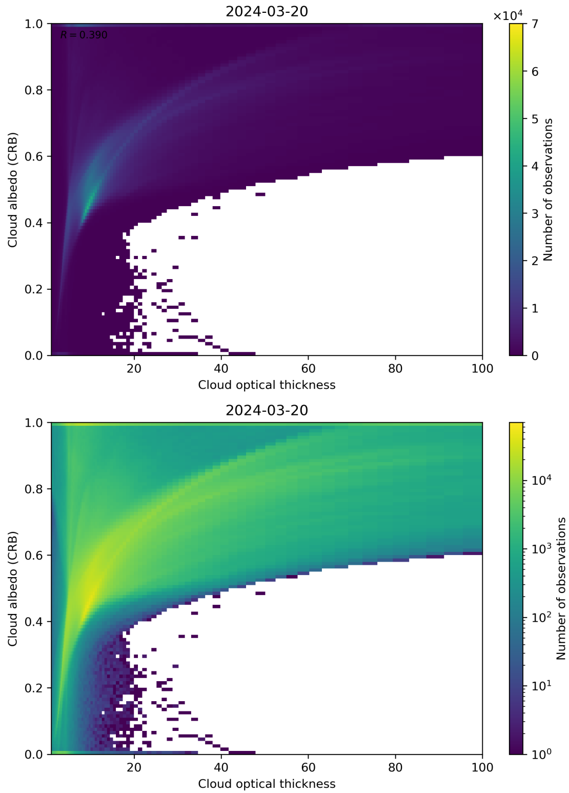
Figure 82: Scatter density plot of “Cloud optical thickness” against “Cloud albedo (CRB)” for 2024-03-20 to 2024-03-21.
