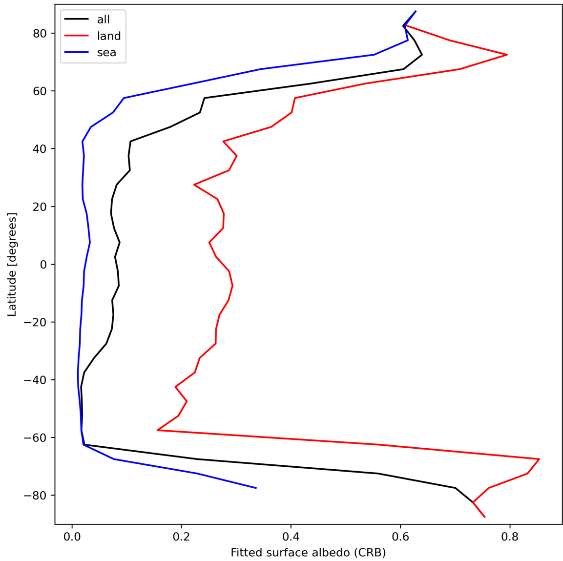
Figure 30: Zonal average of “Fitted surface albedo (CRB)” for 2024-03-20 to 2024-03-21.
