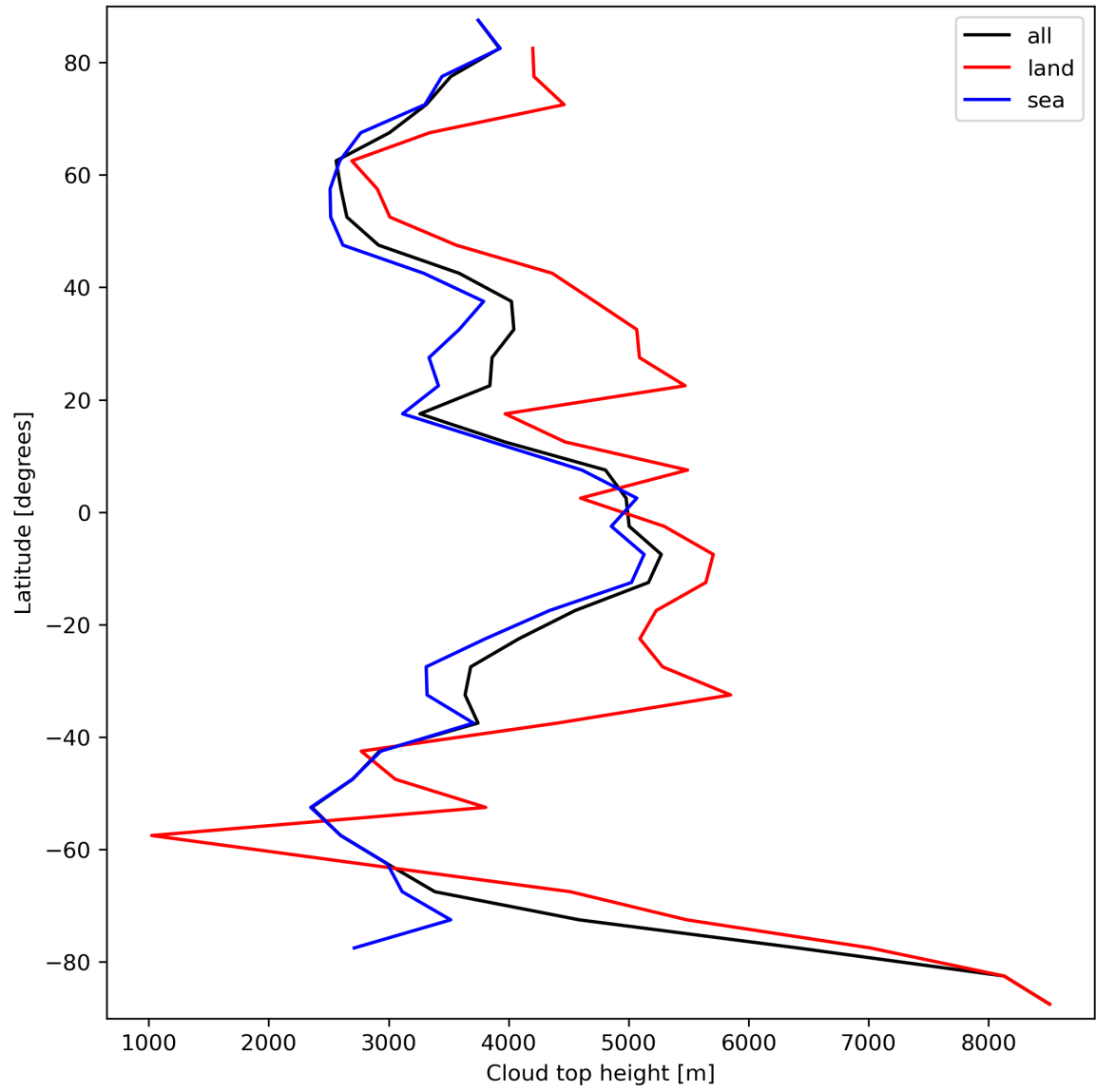
Figure 24: Zonal average of “Cloud top height” for 2024-03-20 to 2024-03-21.
