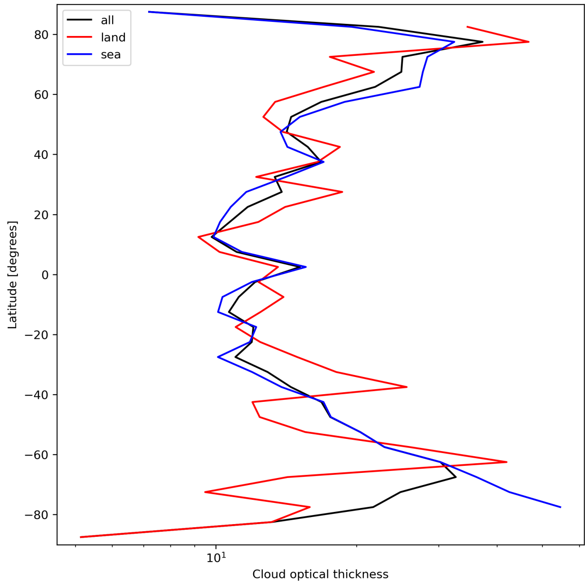
Figure 25: Zonal average of “Cloud optical thickness” for 2024-03-20 to 2024-03-21.
