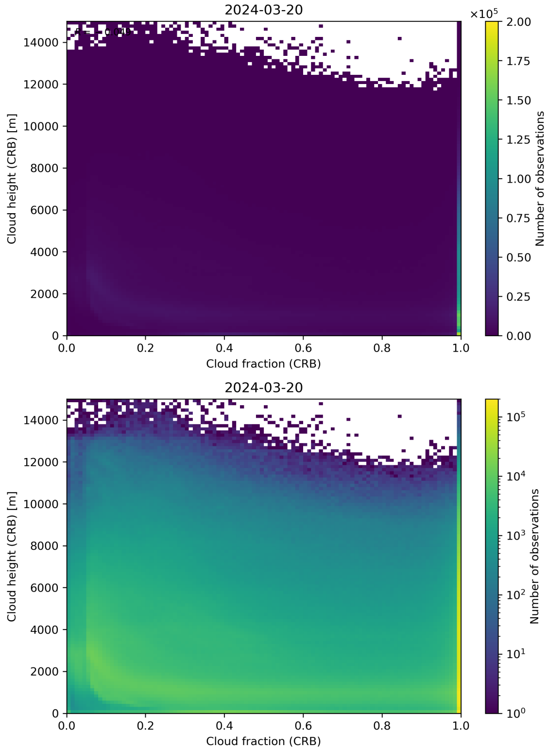
Figure 79: Scatter density plot of “Cloud fraction (CRB)” against “Cloud height (CRB)” for 2024-03-20 to 2024-03-21.
