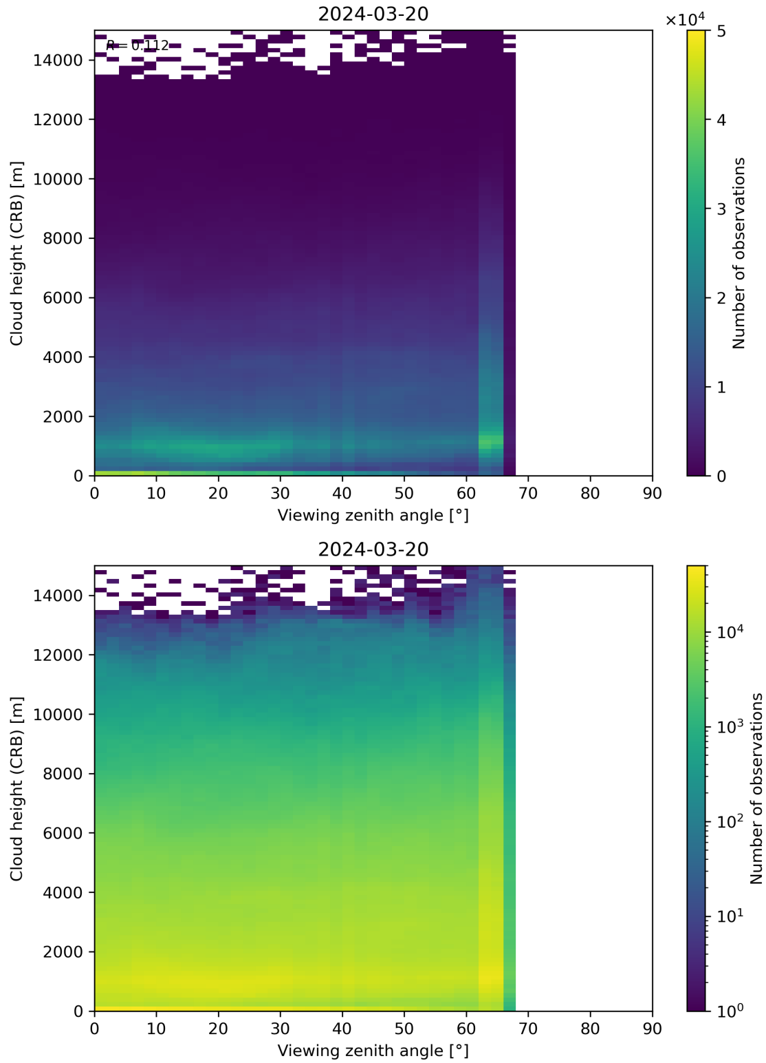
Figure 110: Scatter density plot of “Viewing zenith angle” against “Cloud height (CRB)” for 2024-03-20 to 2024-03-21.
