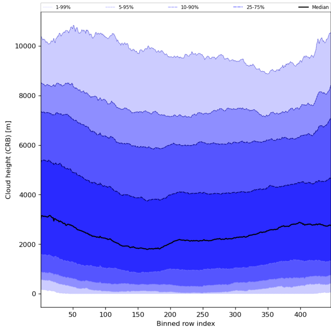
Figure 59: Along track statistics of “Cloud height (CRB)” for 2024-03-20 to 2024-03-21
