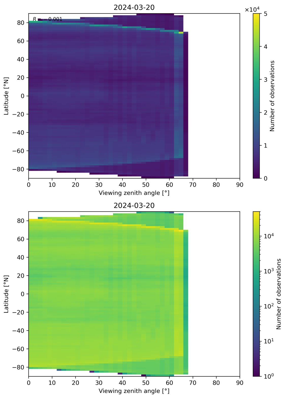
Figure 113: Scatter density plot of “Viewing zenith angle” against “Latitude” for 2024-03-20 to 2024-03-21.
