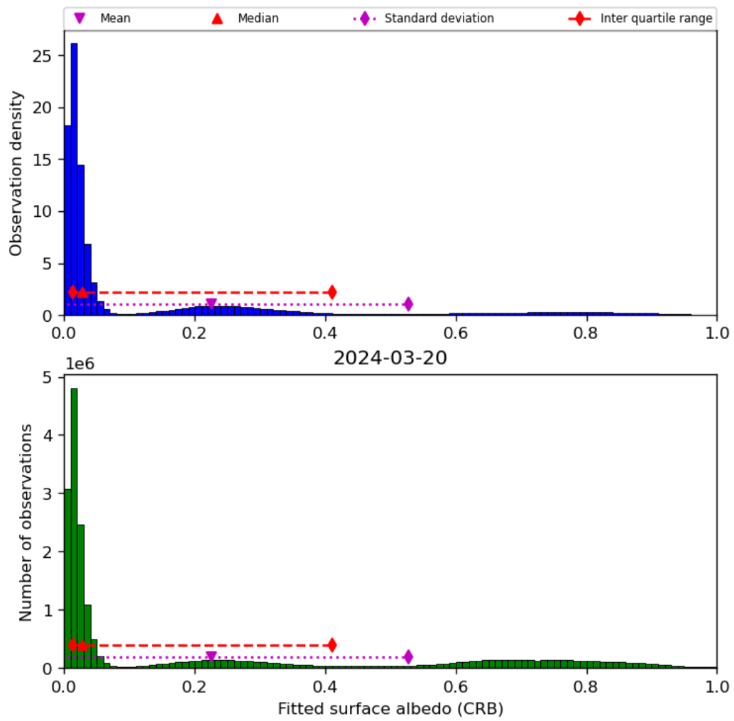
Figure 46: Histogram of “Fitted surface albedo (CRB)” for 2024-03-20 to 2024-03-21
