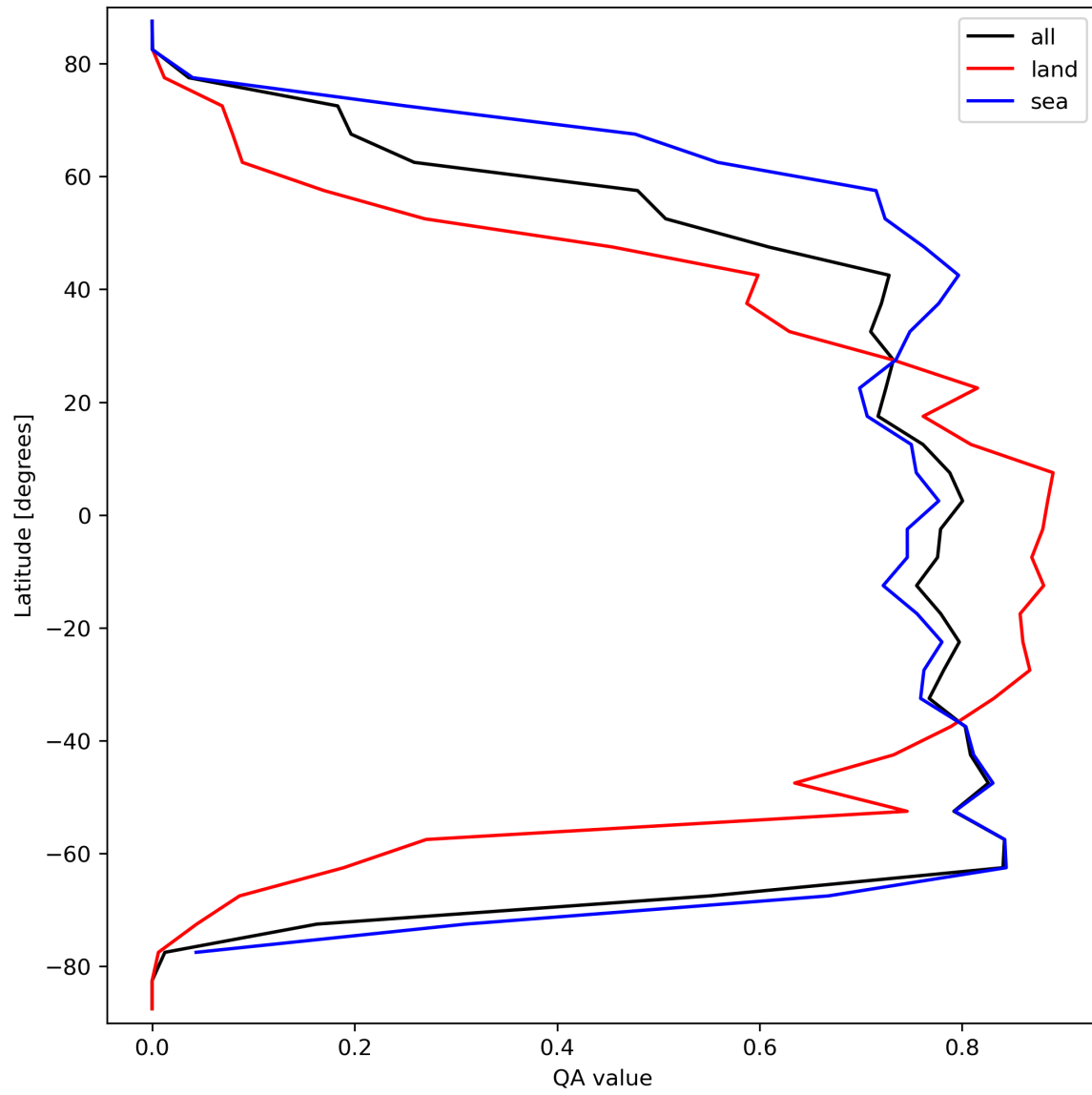
Figure 22: Zonal average of “QA value” for 2024-03-20 to 2024-03-21.
