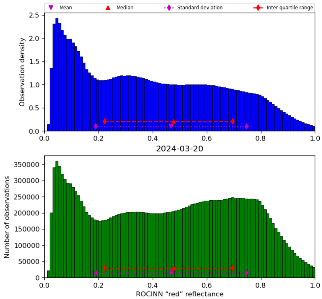
Figure 53: Histogram of “ROCINN “red” reflectance” for 2024-03-20 to 2024-03-21
