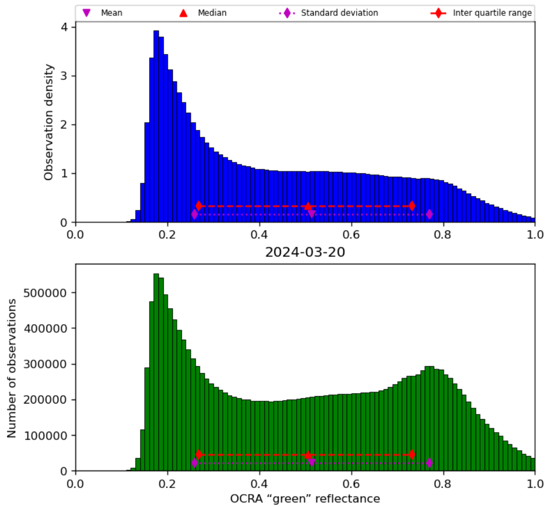
Figure 52: Histogram of “OCRA “green” reflectance” for 2024-03-20 to 2024-03-21
