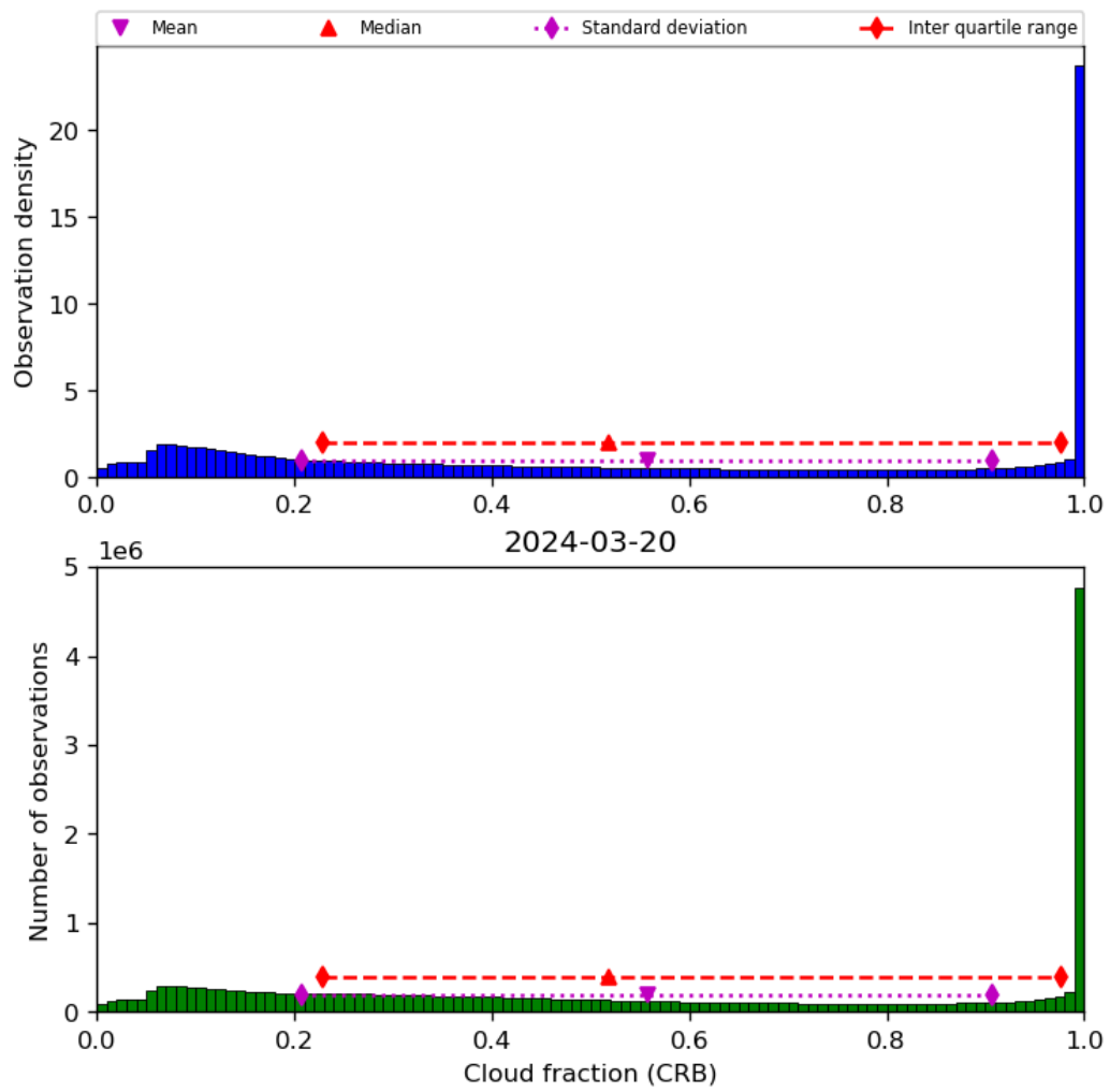
Figure 42: Histogram of “Cloud fraction (CRB)” for 2024-03-20 to 2024-03-21
