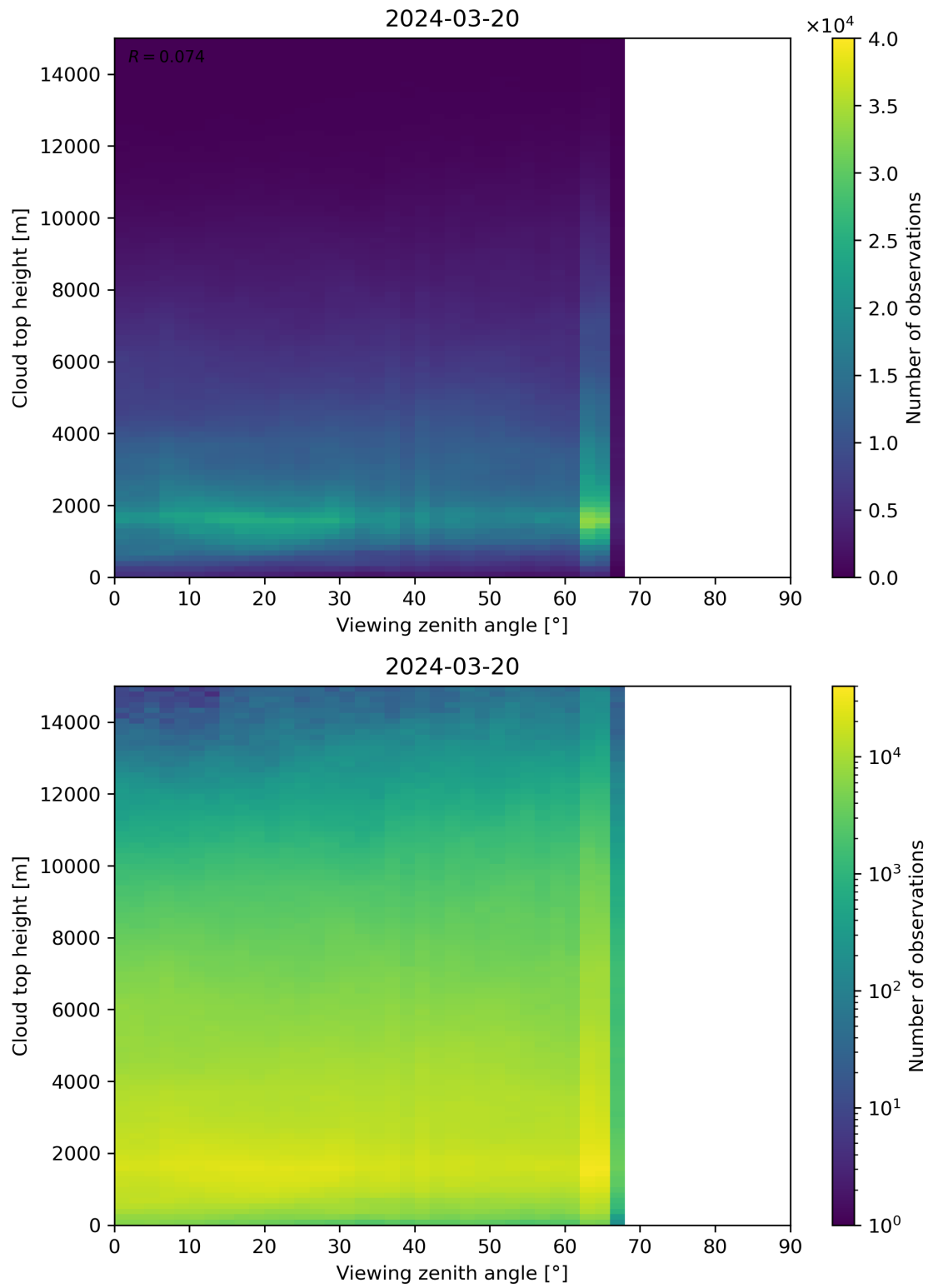
Figure 112: Scatter density plot of “Viewing zenith angle” against “Cloud top height” for 2024-03-20 to 2024-03-21.
