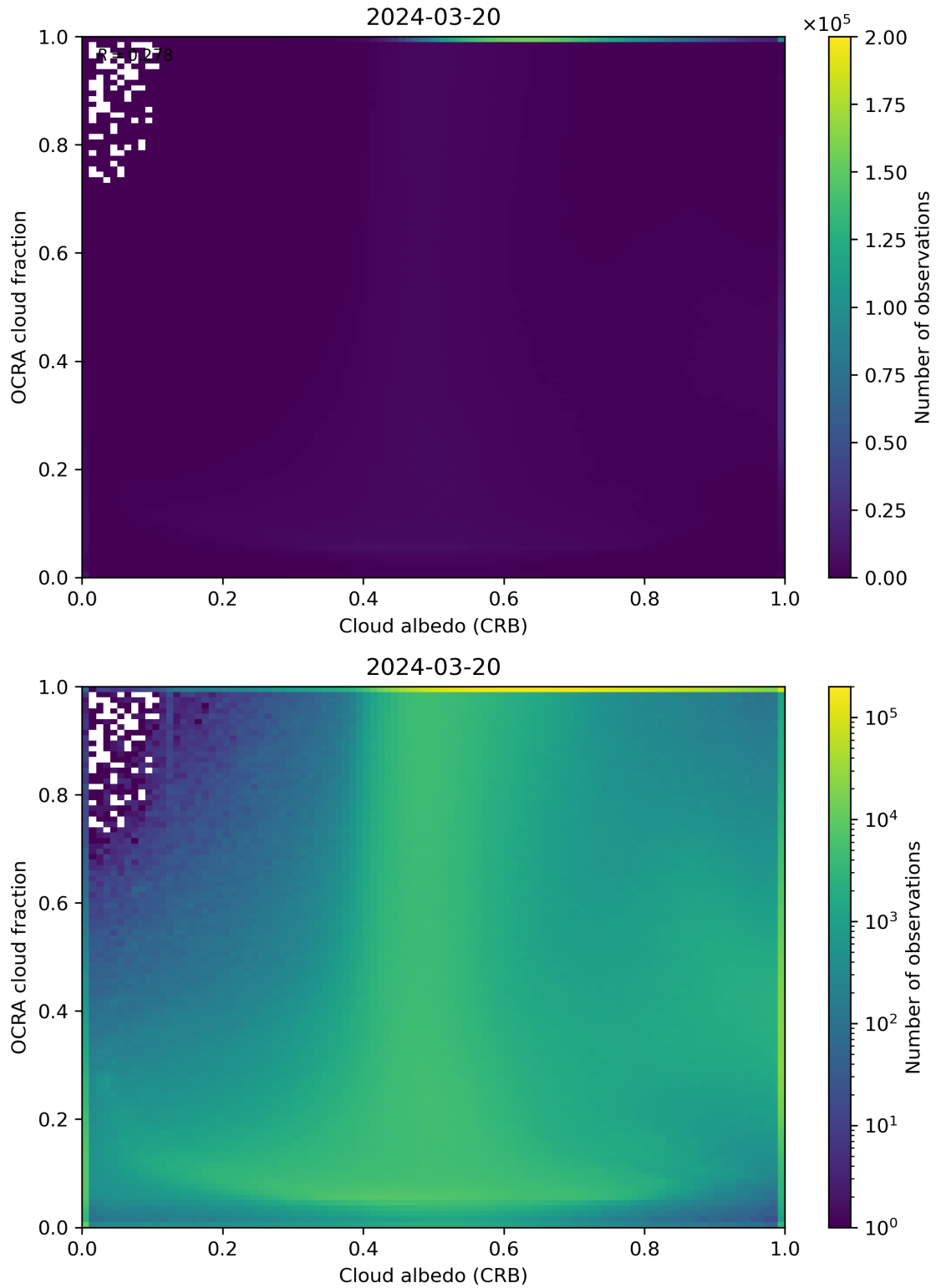
Figure 70: Scatter density plot of “Cloud albedo (CRB)” against “OCRA cloud fraction” for 2024-03-20 to 2024-03-21.
