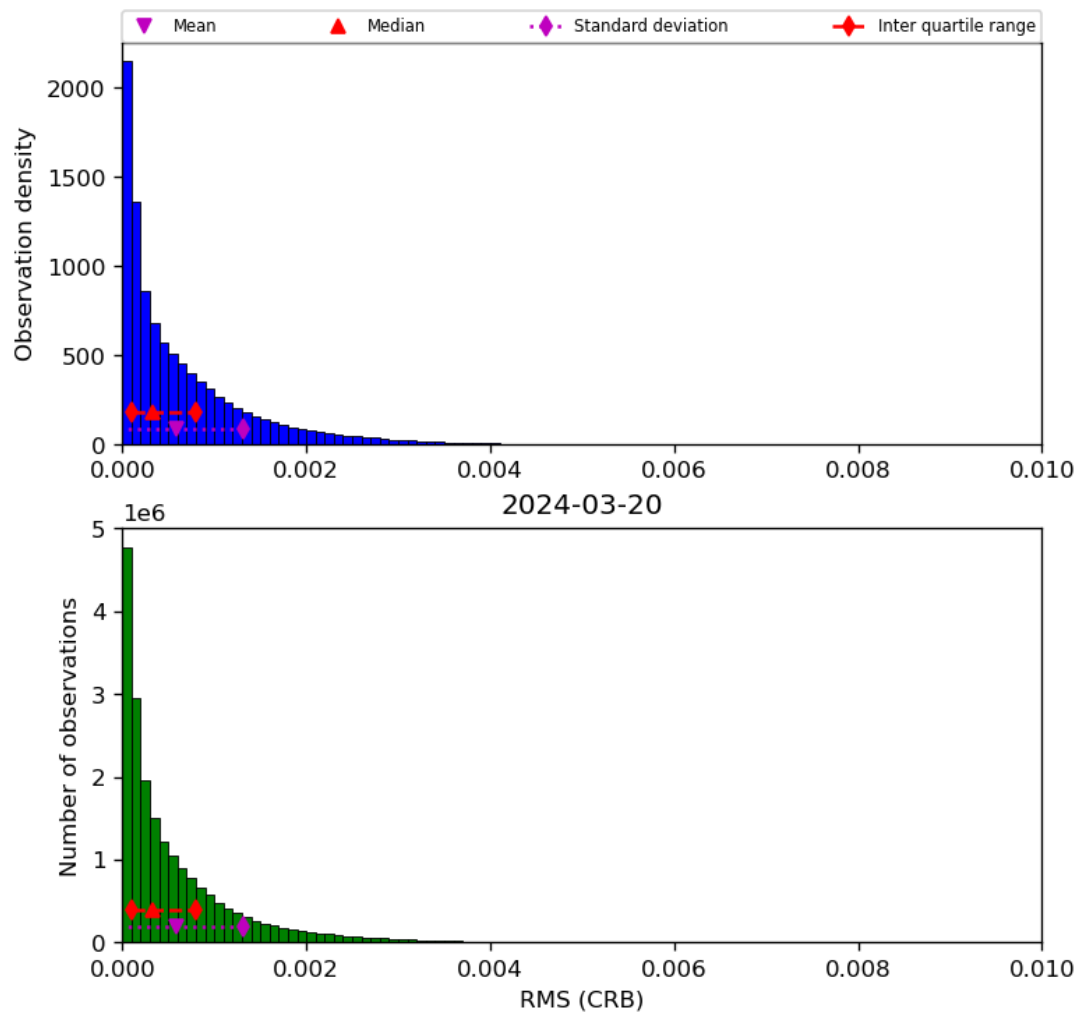
Figure 48: Histogram of “RMS (CRB)” for 2024-03-20 to 2024-03-21
