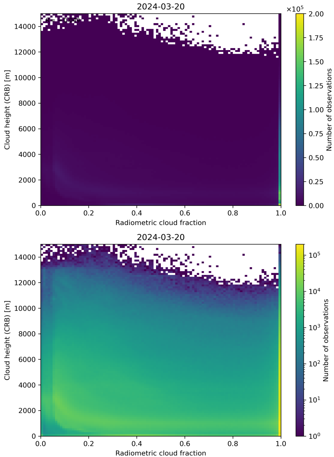
Figure 74: Scatter density plot of “Radiometric cloud fraction” against “Cloud height (CRB)” for 2024-03-20 to 2024-03-21.
