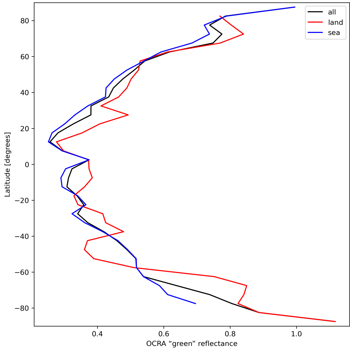
Figure 36: Zonal average of “OCRA “green” reflectance” for 2024-03-20 to 2024-03-21.
