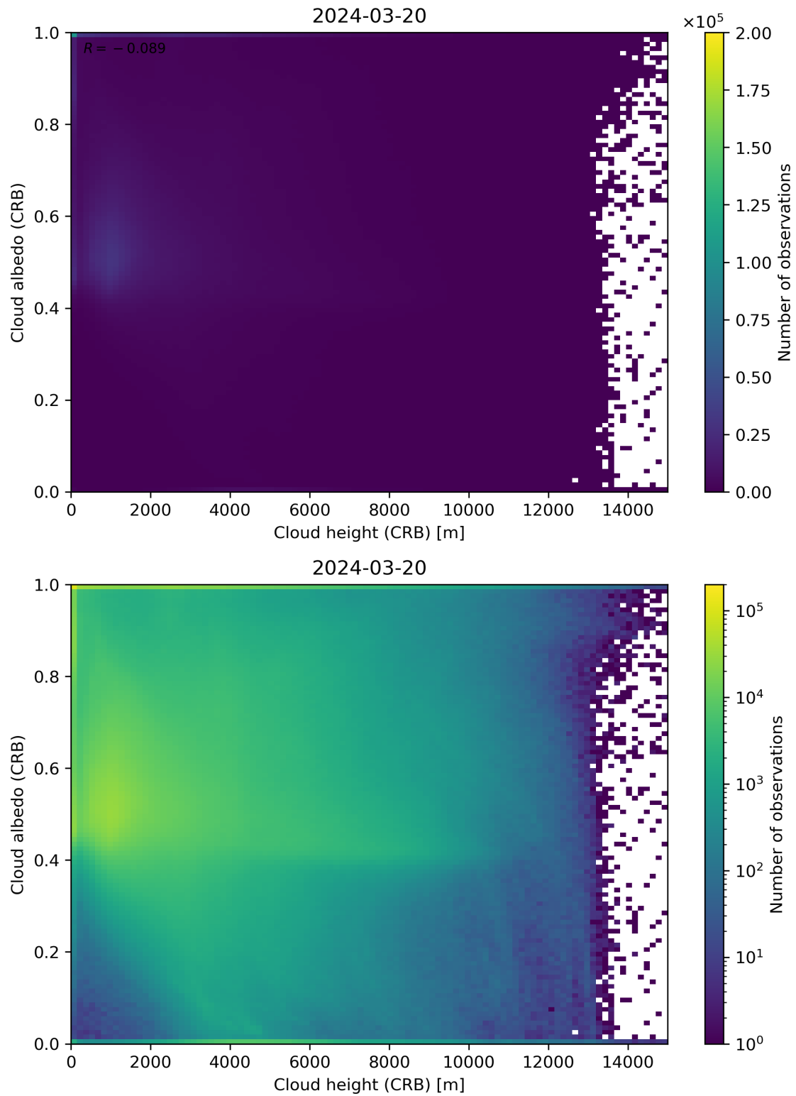
Figure 80: Scatter density plot of “Cloud height (CRB)” against “Cloud albedo (CRB)” for 2024-03-20 to 2024-03-21.
