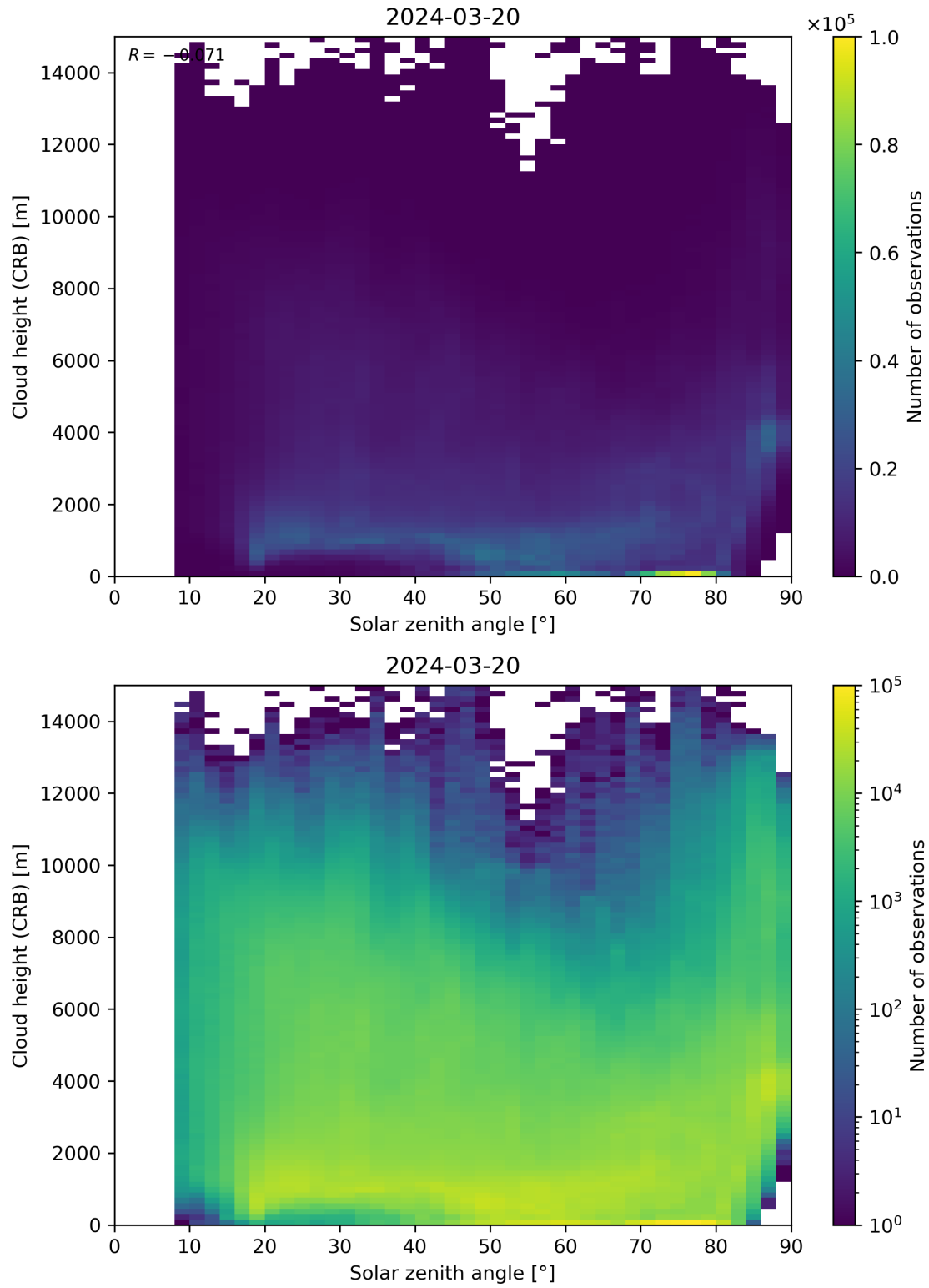
Figure 102: Scatter density plot of “Solar zenith angle” against “Cloud height (CRB)” for 2024-03-20 to 2024-03-21.
