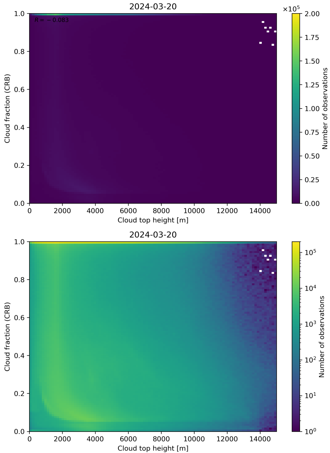
Figure 88: Scatter density plot of “Cloud top height” against “Cloud fraction (CRB)” for 2024-03-20 to 2024-03-21.
