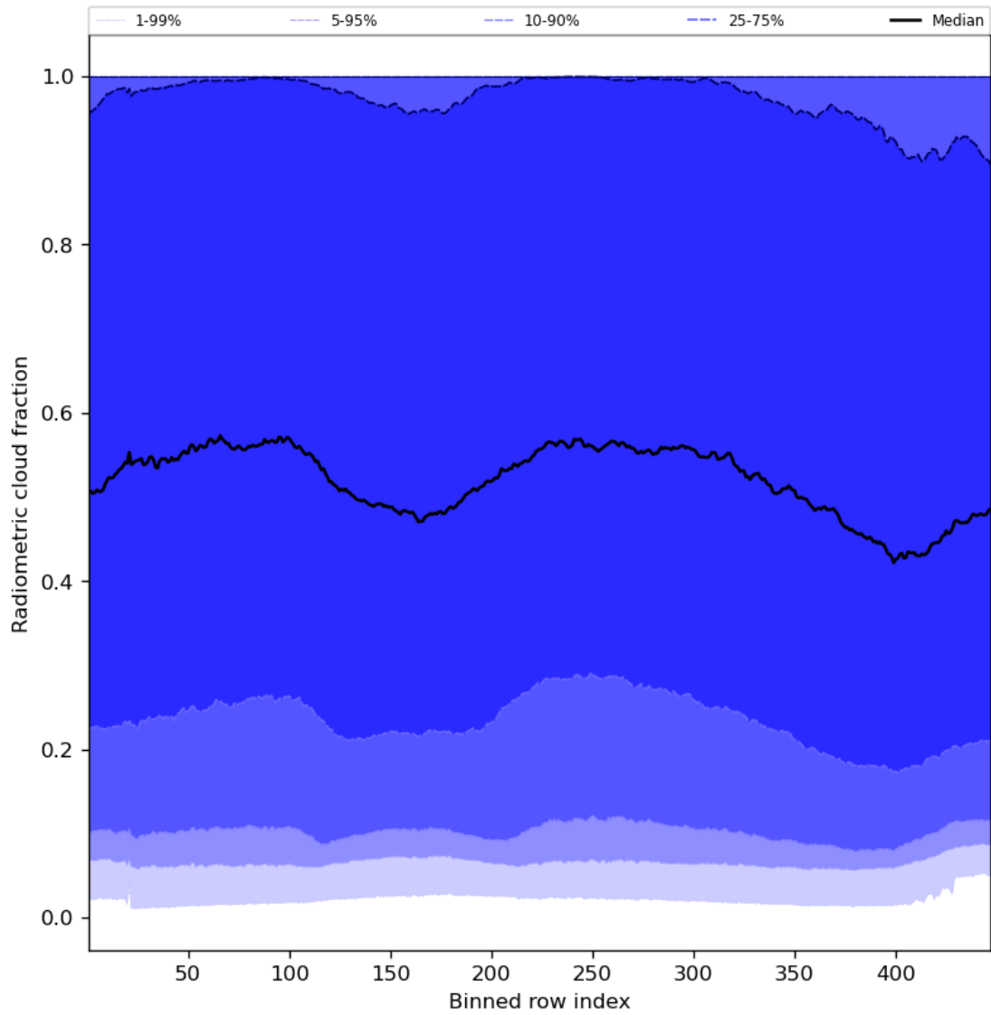
Figure 55: Along track statistics of “Radiometric cloud fraction” for 2024-03-20 to 2024-03-21
