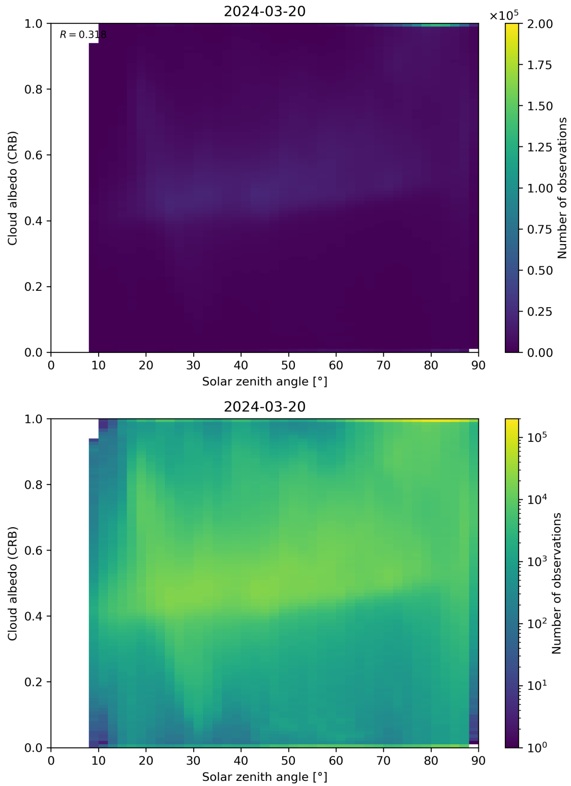
Figure 98: Scatter density plot of “Solar zenith angle” against “Cloud albedo (CRB)” for 2024-03-20 to 2024-03-21.
