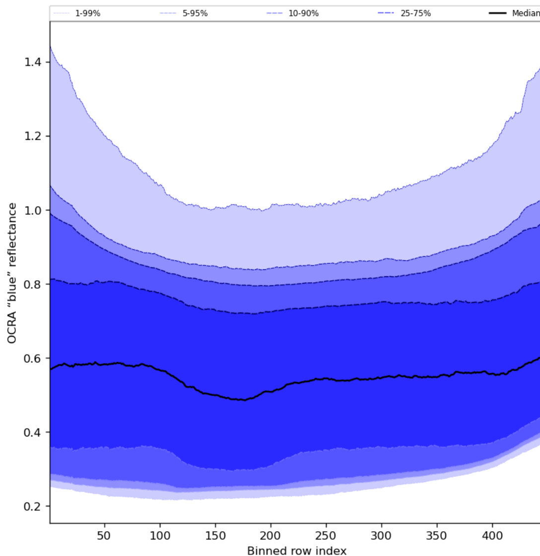
Figure 67: Along track statistics of “OCRA “blue” reflectance” for 2024-03-20 to 2024-03-21
