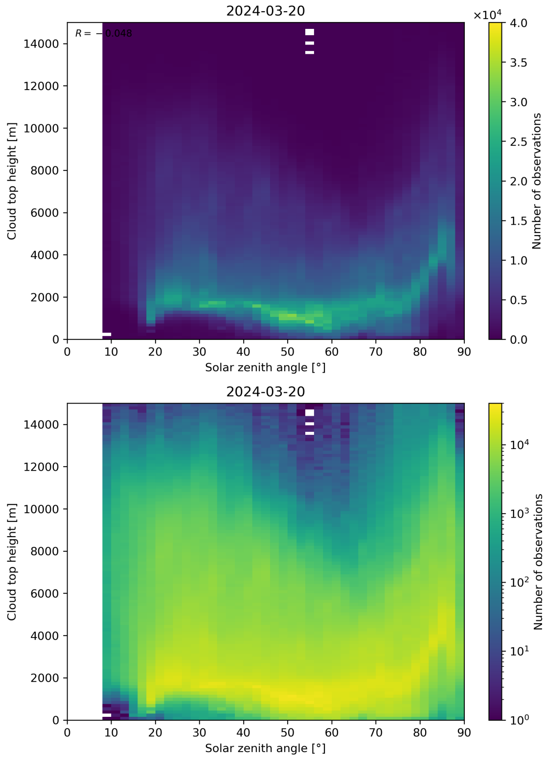
Figure 104: Scatter density plot of “Solar zenith angle” against “Cloud top height” for 2024-03-20 to 2024-03-21.
