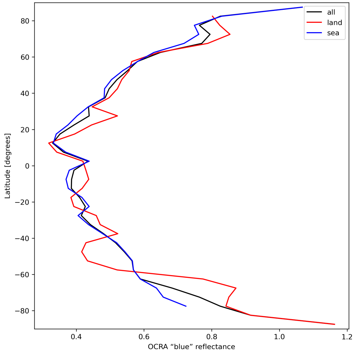
Figure 35: Zonal average of “OCRA “blue” reflectance” for 2024-03-20 to 2024-03-21.
