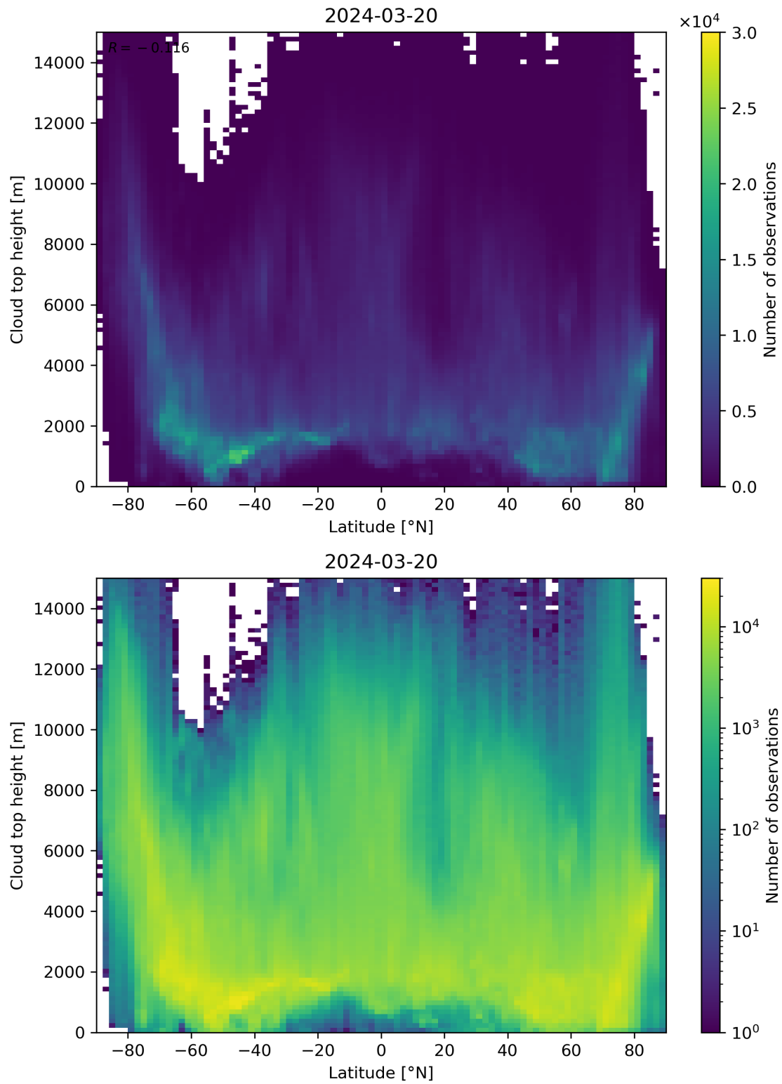
Figure 97: Scatter density plot of “Latitude” against “Cloud top height” for 2024-03-20 to 2024-03-21.
