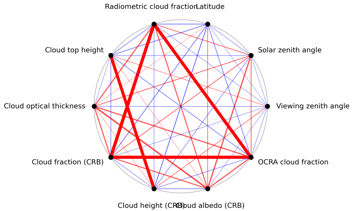
Figure 1: Map of correlation graph for 2024-03-20 to 2024-03-21.
