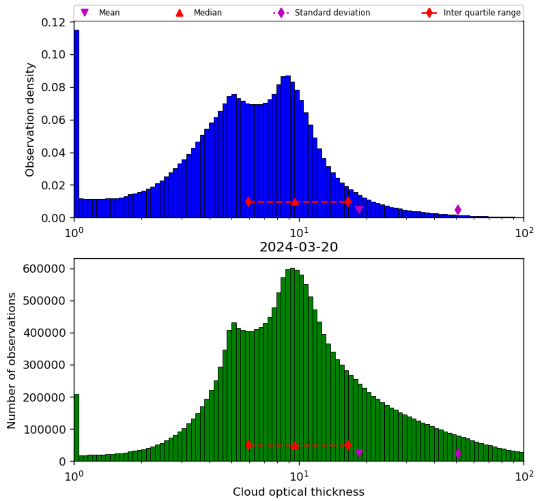
Figure 41: Histogram of “Cloud optical thickness” for 2024-03-20 to 2024-03-21
