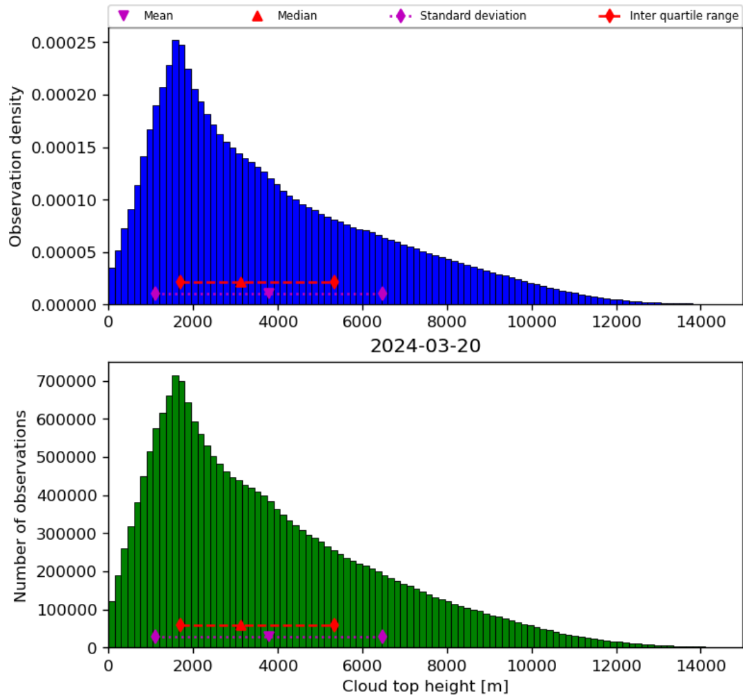
Figure 40: Histogram of “Cloud top height” for 2024-03-20 to 2024-03-21
