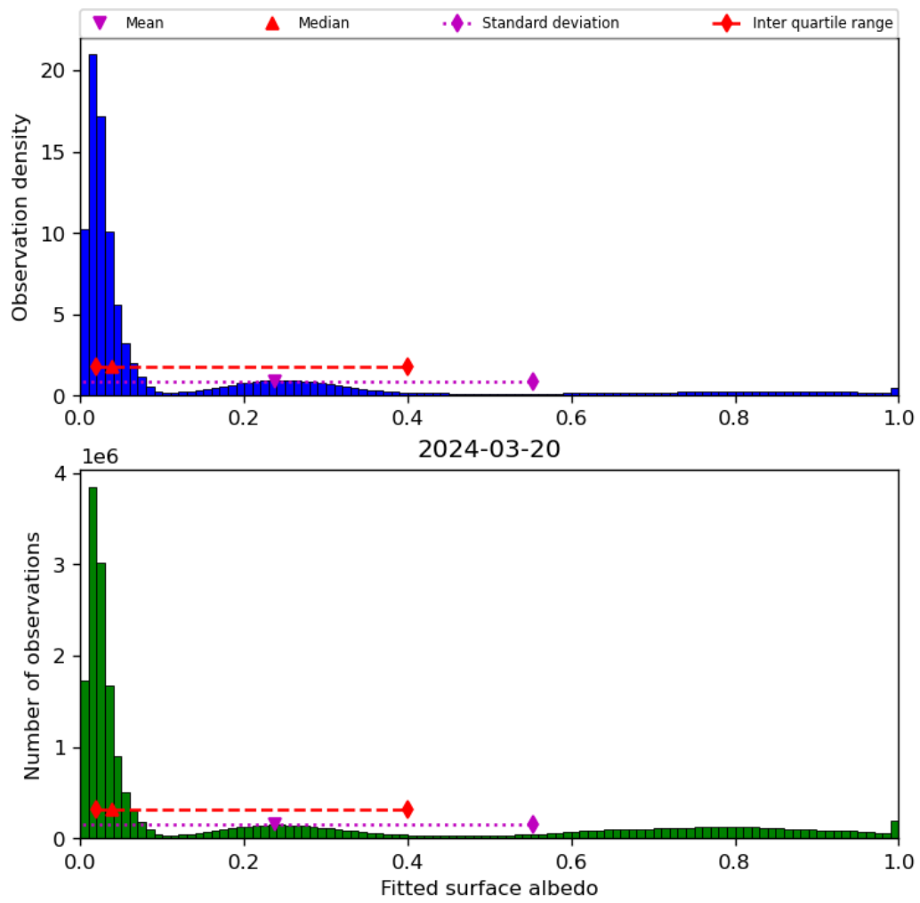
Figure 45: Histogram of “Fitted surface albedo” for 2024-03-20 to 2024-03-21
