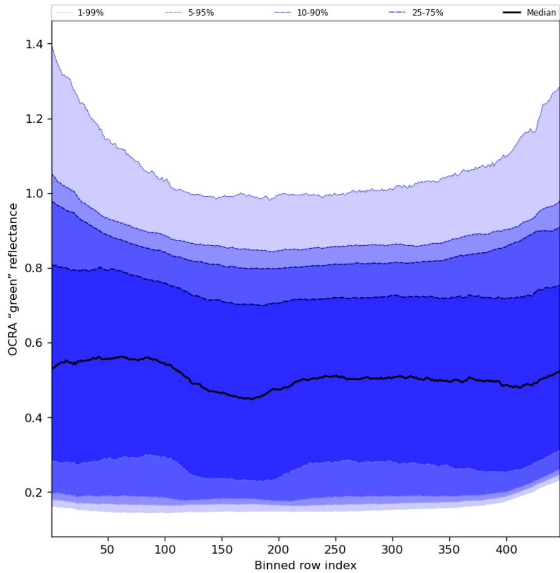
Figure 68: Along track statistics of “OCRA “green” reflectance” for 2024-03-20 to 2024-03-21
