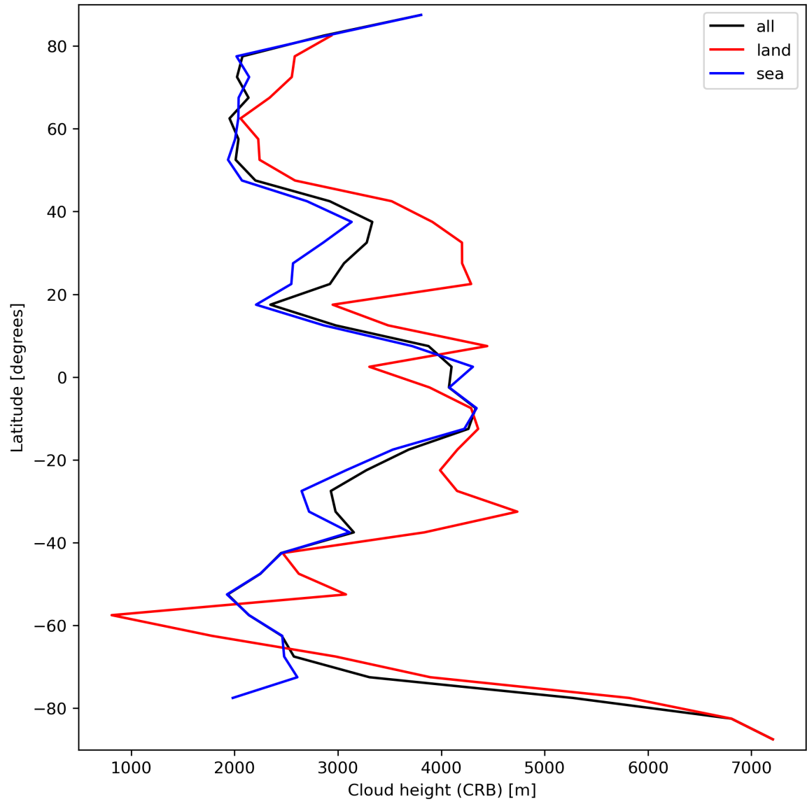
Figure 27: Zonal average of “Cloud height (CRB)” for 2024-03-20 to 2024-03-21.
