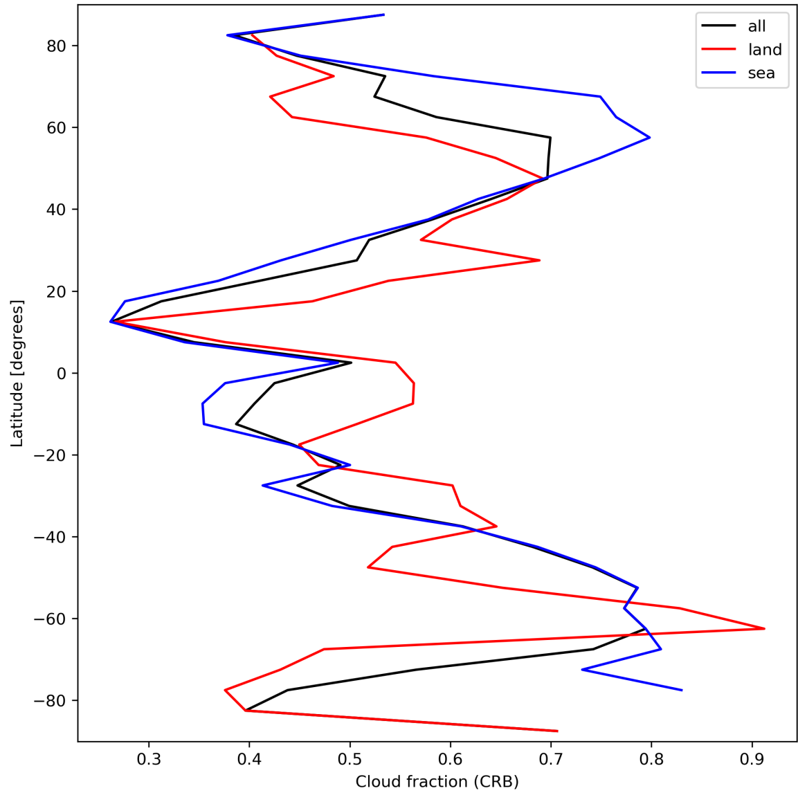
Figure 26: Zonal average of “Cloud fraction (CRB)” for 2024-03-20 to 2024-03-21.
