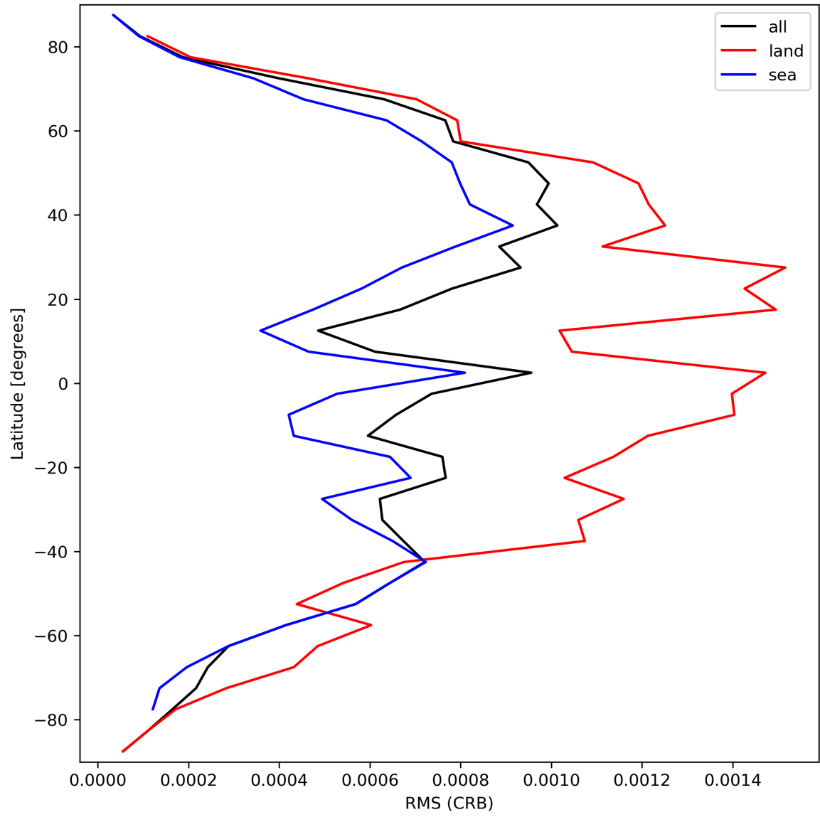
Figure 32: Zonal average of "RMS (CRB)" for 2024-03-20 to 2024-03-21.
