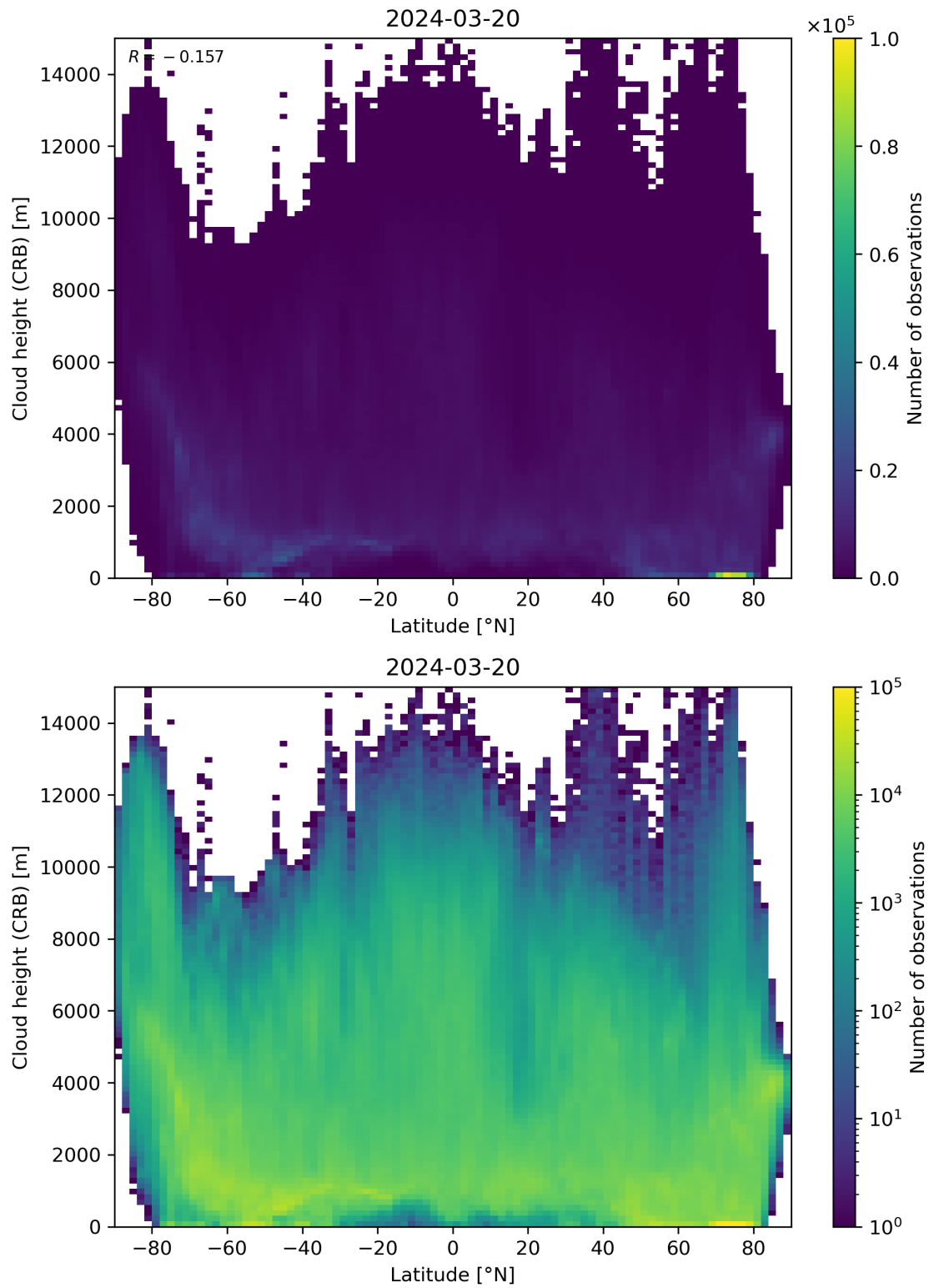
Figure 95: Scatter density plot of “Latitude” against “Cloud height (CRB)” for 2024-03-20 to 2024-03-21.
