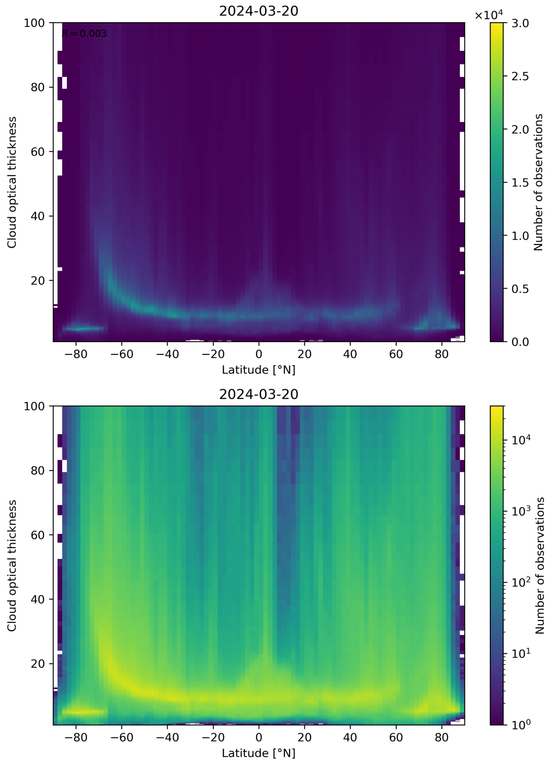
Figure 96: Scatter density plot of “Latitude” against “Cloud optical thickness” for 2024-03-20 to 2024-03-21.
