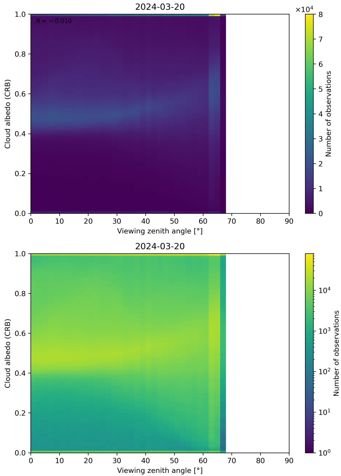
Figure 106: Scatter density plot of “Viewing zenith angle” against “Cloud albedo (CRB)” for 2024-03-20 to 2024-03-21.
