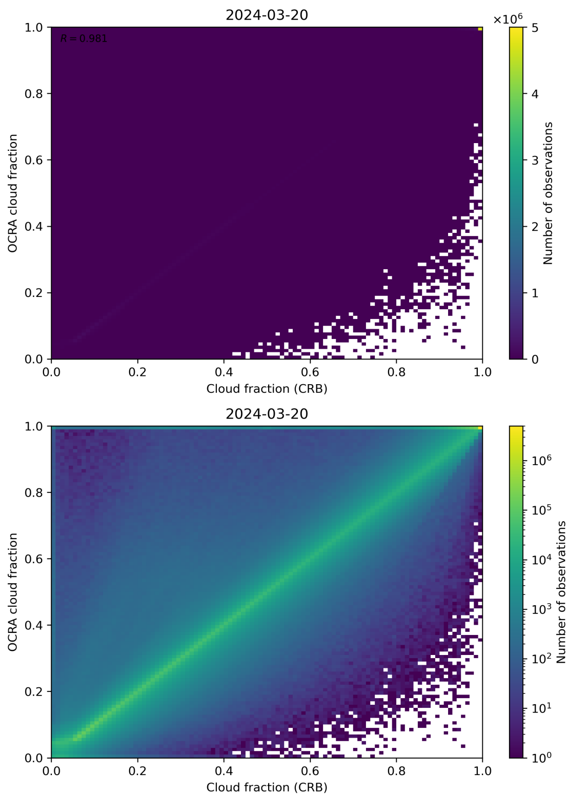
Figure 78: Scatter density plot of “Cloud fraction (CRB)” against “OCRA cloud fraction” for 2024-03-20 to 2024-03-21.
