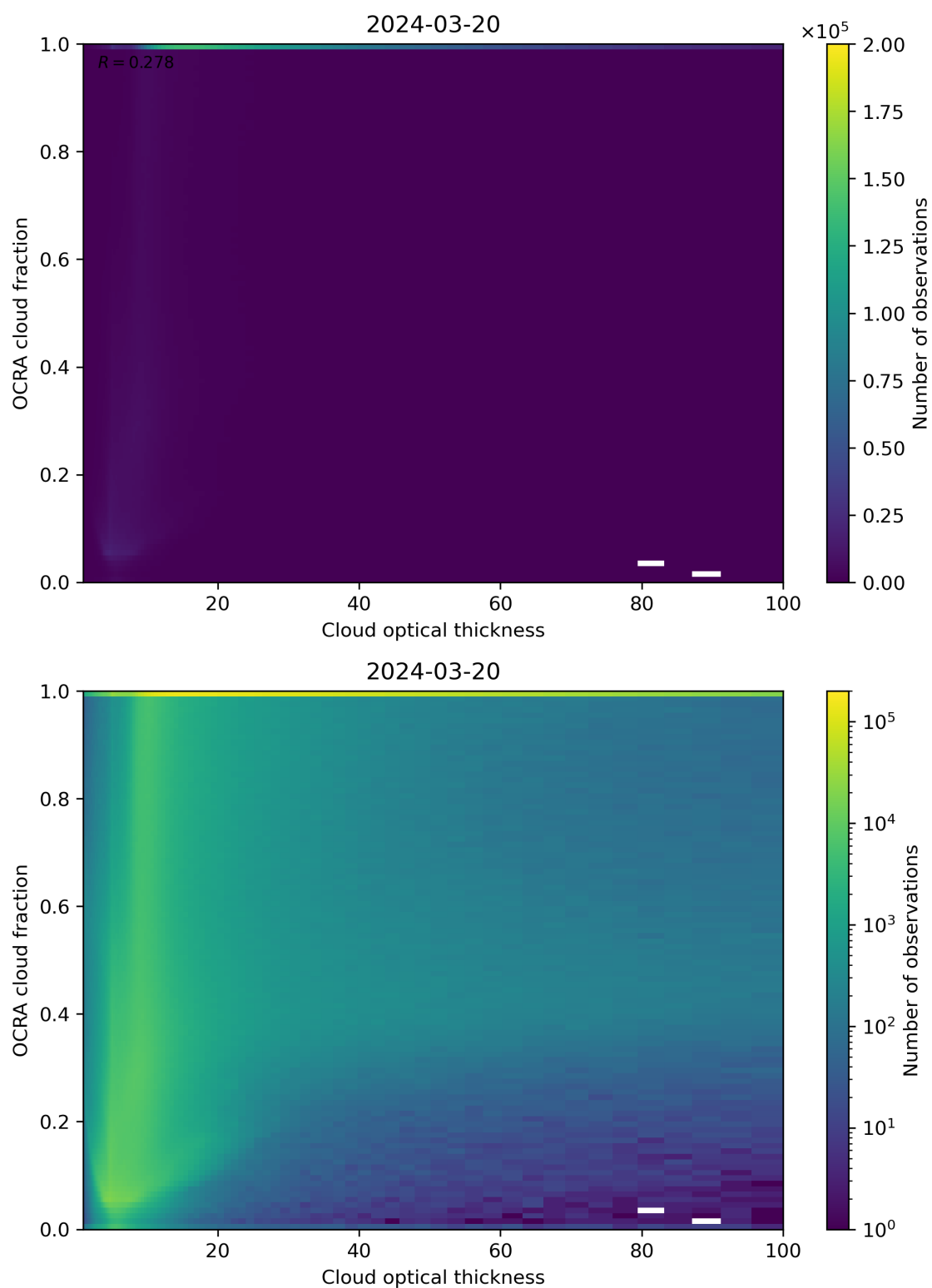
Figure 83: Scatter density plot of “Cloud optical thickness” against “OCRA cloud fraction” for 2024-03-20 to 2024-03-21.
