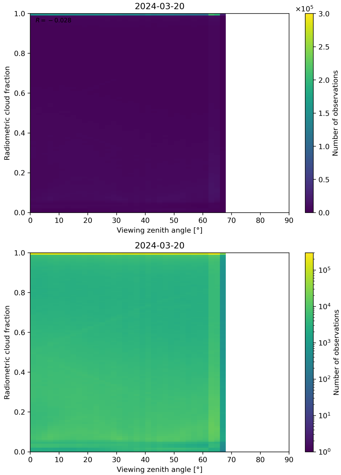
Figure 107: Scatter density plot of “Viewing zenith angle” against “Radiometric cloud fraction” for 2024-03-20 to 2024-03-21.
