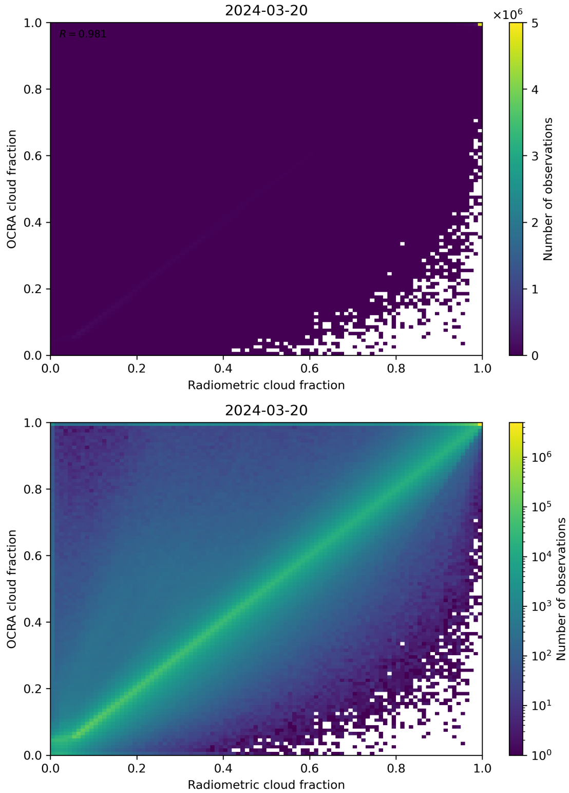
Figure 72: Scatter density plot of “Radiometric cloud fraction” against “OCRA cloud fraction” for 2024-03-20 to 2024-03-21.
