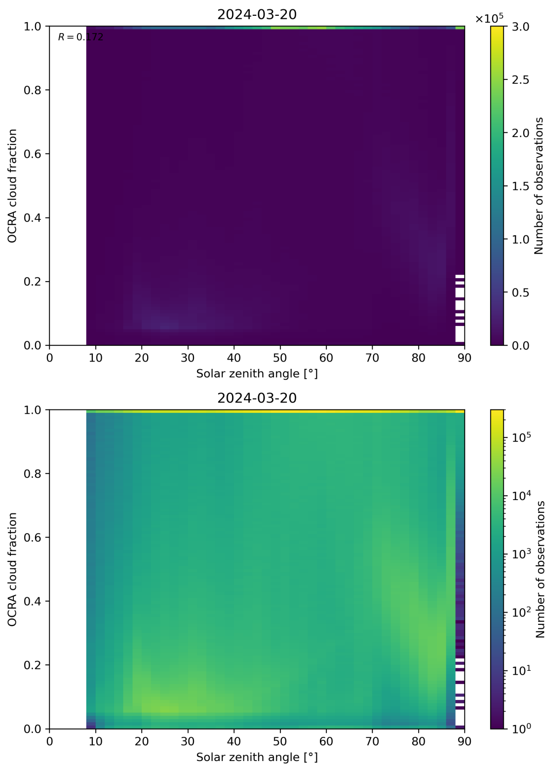
Figure 100: Scatter density plot of “Solar zenith angle” against “OCRA cloud fraction” for 2024-03-20 to 2024-03-21.
