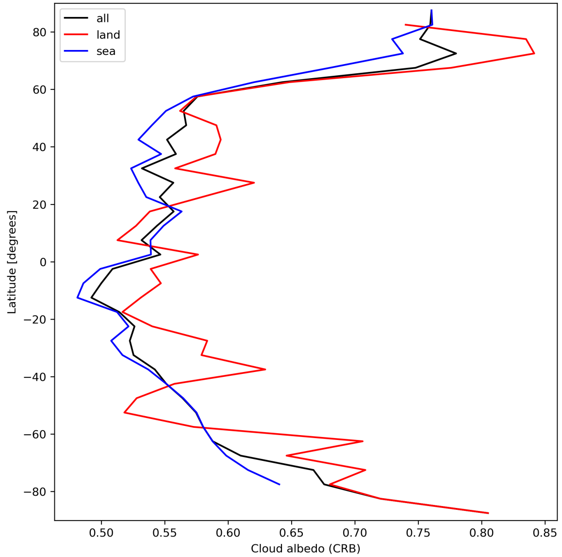
Figure 28: Zonal average of “Cloud albedo (CRB)” for 2024-03-20 to 2024-03-21.
