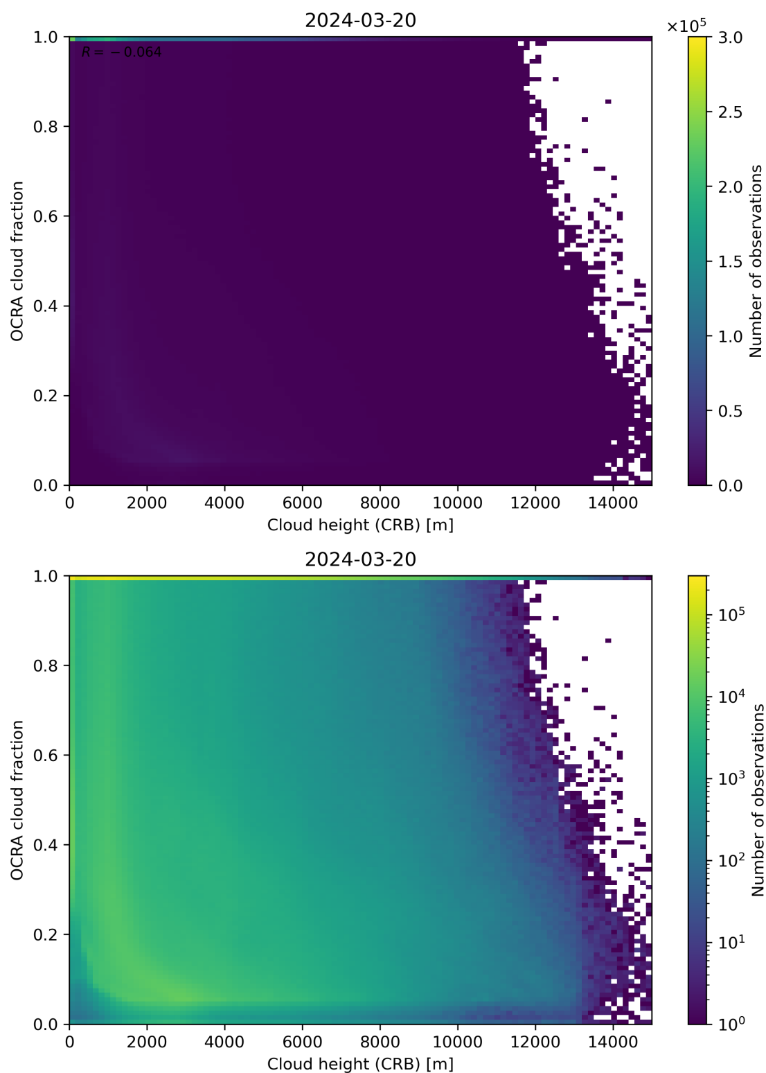
Figure 81: Scatter density plot of “Cloud height (CRB)” against “OCRA cloud fraction” for 2024-03-20 to 2024-03-21.
