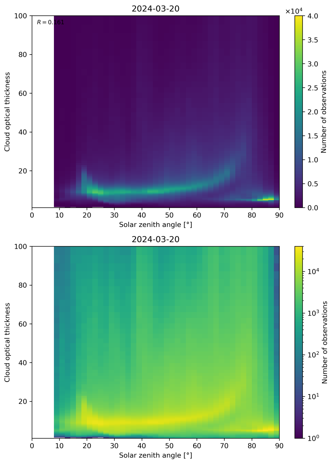
Figure 103: Scatter density plot of “Solar zenith angle” against “Cloud optical thickness” for 2024-03-20 to 2024-03-21.
