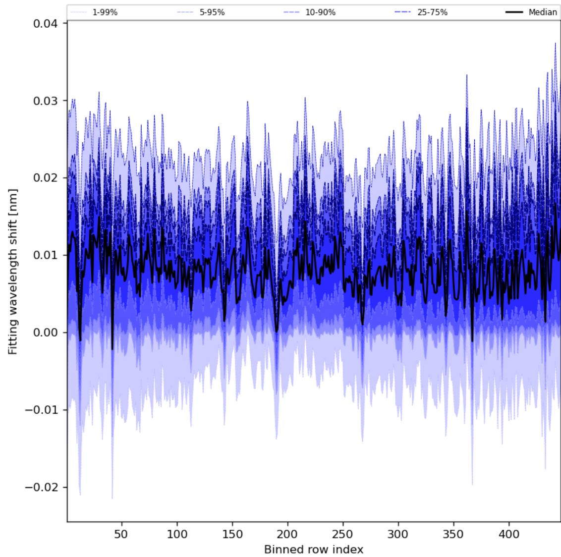
Figure 65: Along track statistics of “Fitting wavelength shift” for 2024-03-20 to 2024-03-21
