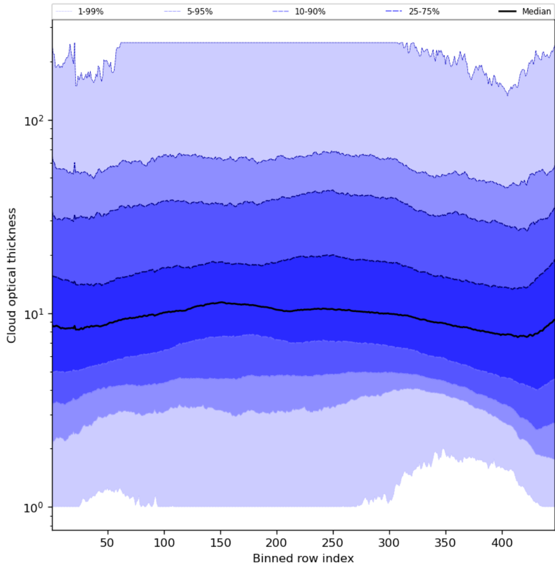
Figure 57: Along track statistics of “Cloud optical thickness” for 2024-03-20 to 2024-03-21
