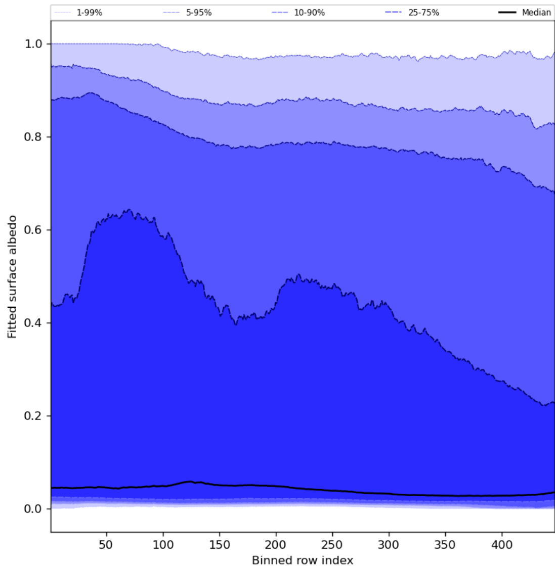
Figure 61: Along track statistics of “Fitted surface albedo” for 2024-03-20 to 2024-03-22
