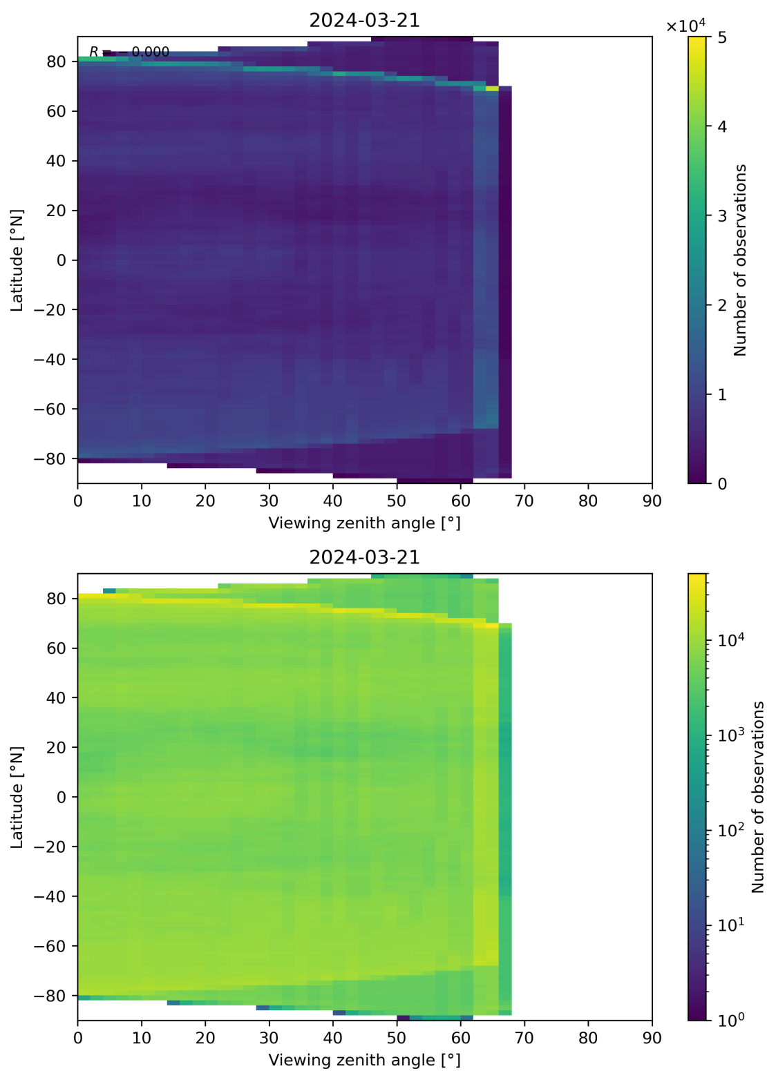
Figure 113: Scatter density plot of “Viewing zenith angle” against “Latitude” for 2024-03-20 to 2024-03-22.
