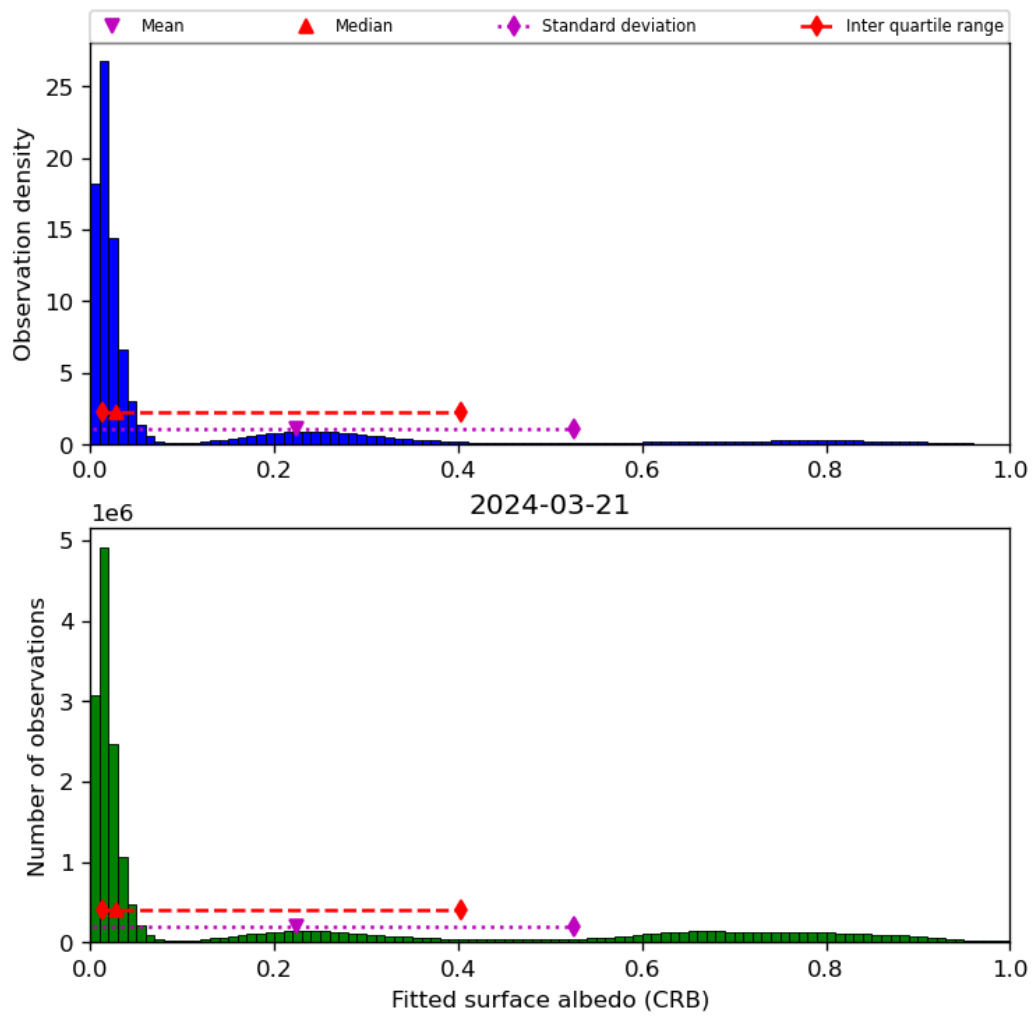
Figure 46: Histogram of “Fitted surface albedo (CRB)” for 2024-03-20 to 2024-03-22
