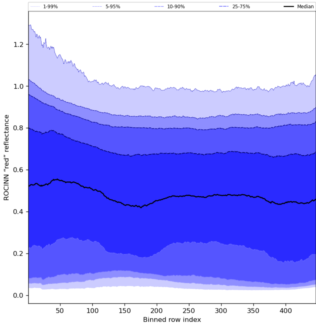
Figure 69: Along track statistics of “ROCINN “red” reflectance” for 2024-03-20 to 2024-03-22
