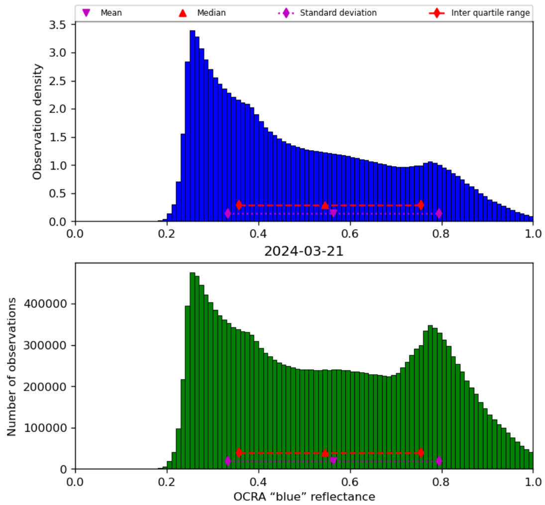
Figure 51: Histogram of “OCRA “blue” reflectance” for 2024-03-20 to 2024-03-22
