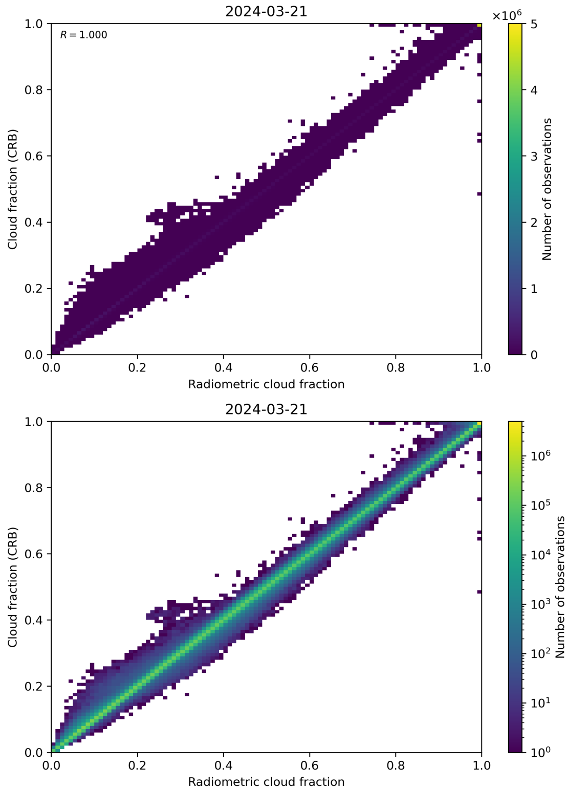
Figure 73: Scatter density plot of “Radiometric cloud fraction” against “Cloud fraction (CRB)” for 2024-03-20 to 2024-03-22.
