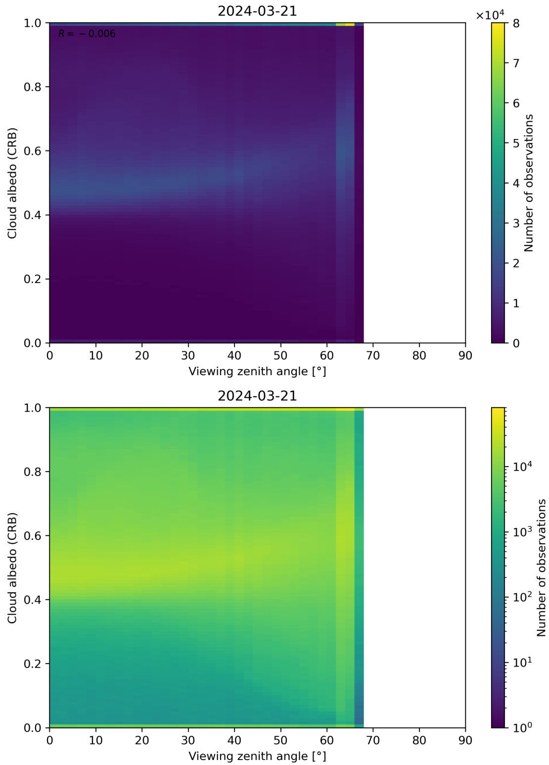
Figure 106: Scatter density plot of “Viewing zenith angle” against “Cloud albedo (CRB)” for 2024-03-20 to 2024-03-22.
