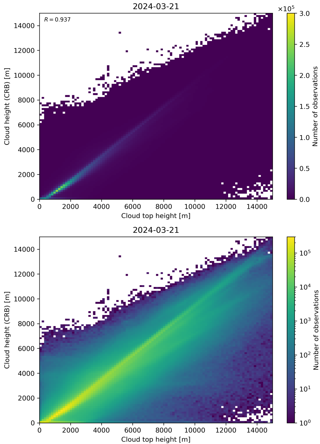
Figure 89: Scatter density plot of “Cloud top height” against “Cloud height (CRB)” for 2024-03-20 to 2024-03-22.
