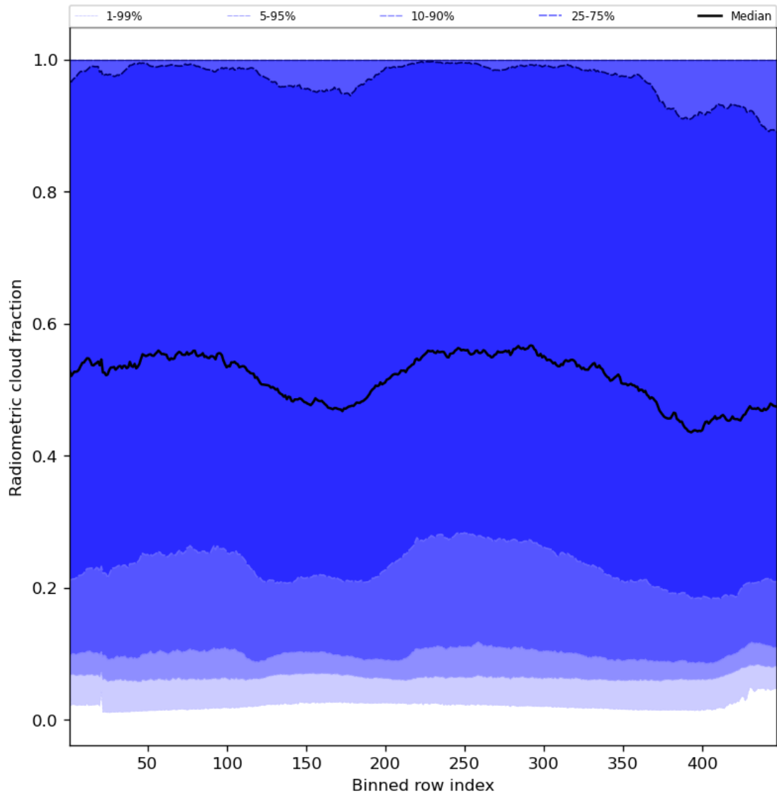
Figure 55: Along track statistics of “Radiometric cloud fraction” for 2024-03-20 to 2024-03-22
