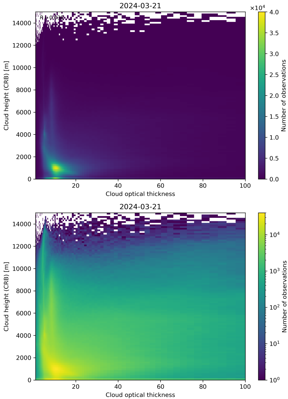
Figure 85: Scatter density plot of “Cloud optical thickness” against “Cloud height (CRB)” for 2024-03-20 to 2024-03-22.
