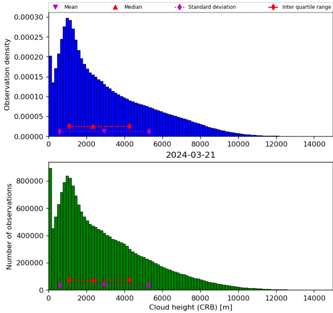
Figure 43: Histogram of “Cloud height (CRB)” for 2024-03-20 to 2024-03-22
