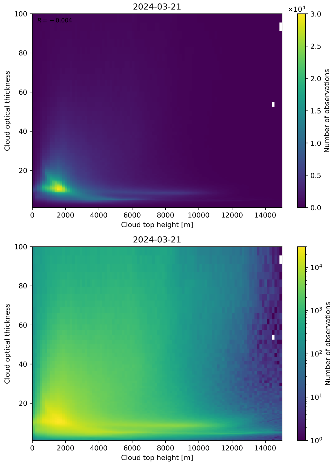
Figure 90: Scatter density plot of “Cloud top height” against “Cloud optical thickness” for 2024-03-20 to 2024-03-22.
