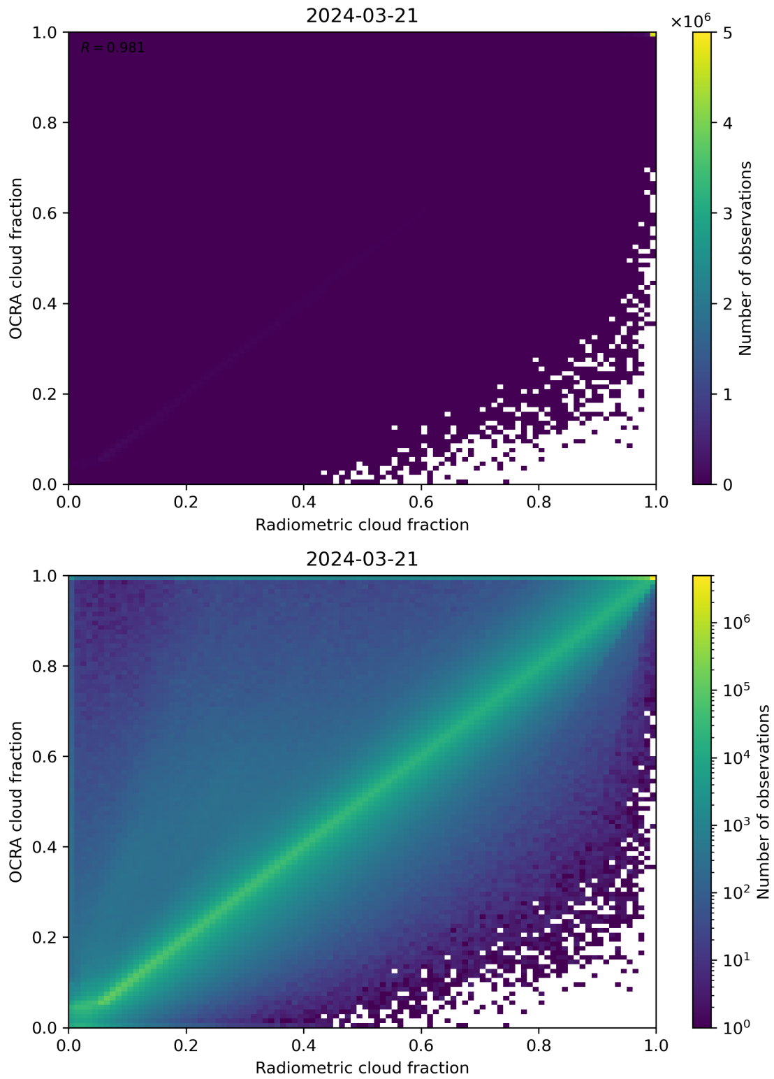
Figure 72: Scatter density plot of “Radiometric cloud fraction” against “OCRA cloud fraction” for 2024-03-20 to 2024-03-22.
