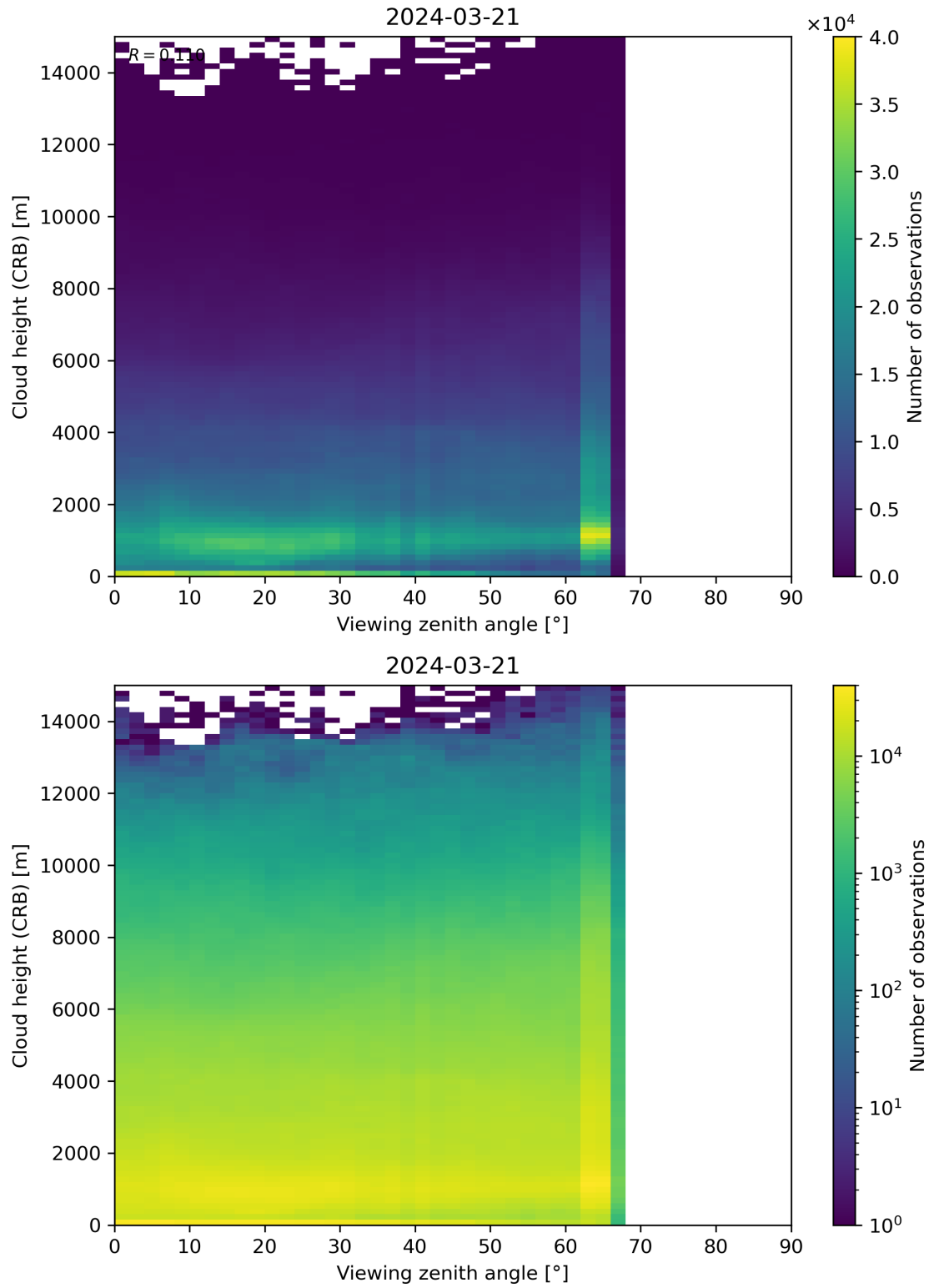
Figure 110: Scatter density plot of “Viewing zenith angle” against “Cloud height (CRB)” for 2024-03-20 to 2024-03-22.
