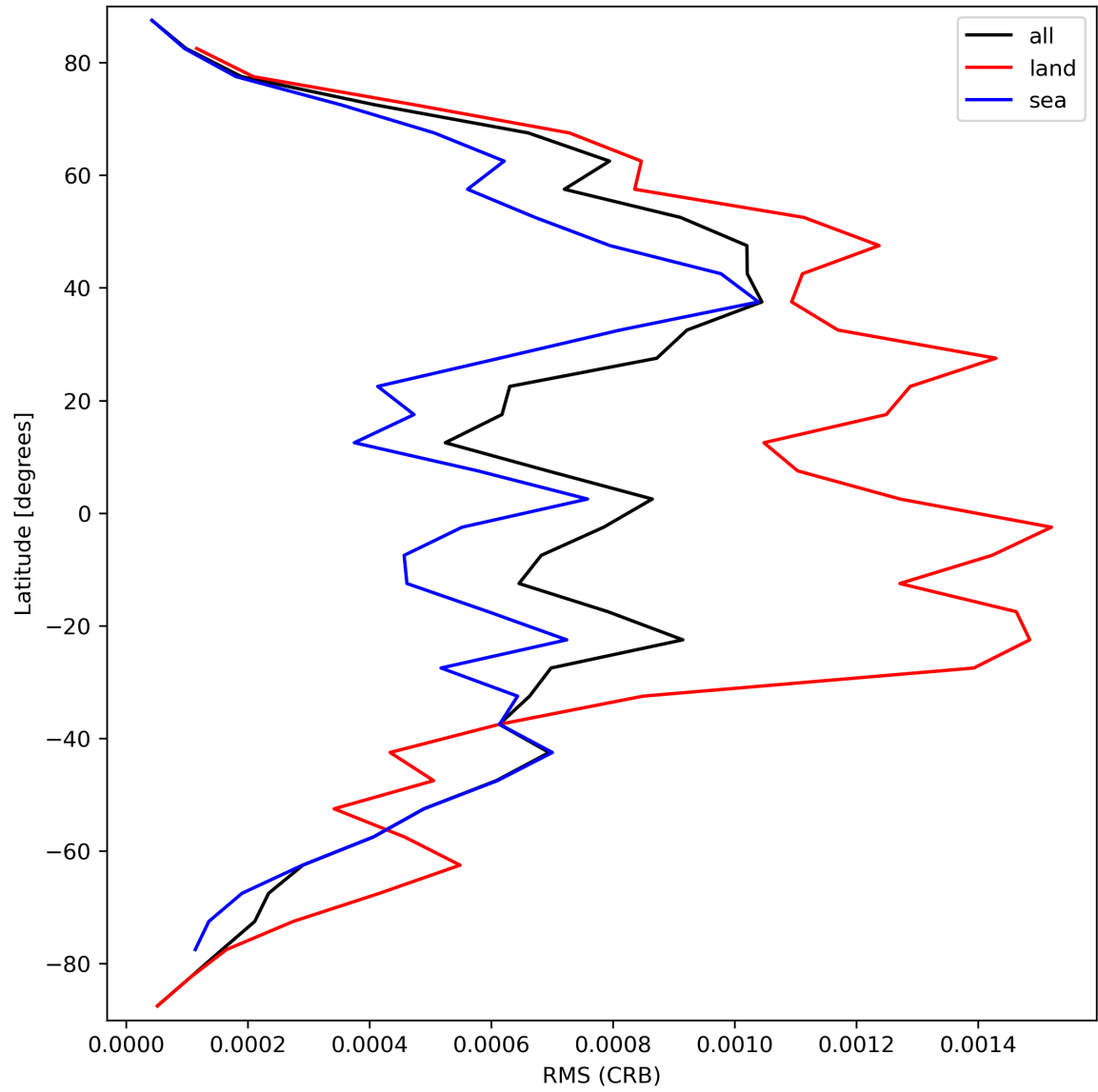
Figure 32: Zonal average of “RMS (CRB)” for 2024-03-20 to 2024-03-22.
