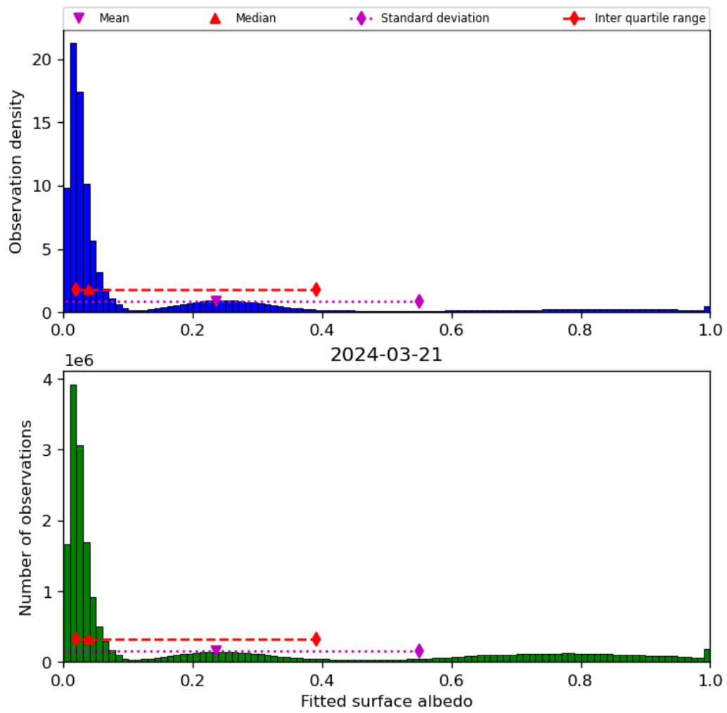
Figure 45: Histogram of “Fitted surface albedo” for 2024-03-20 to 2024-03-22
