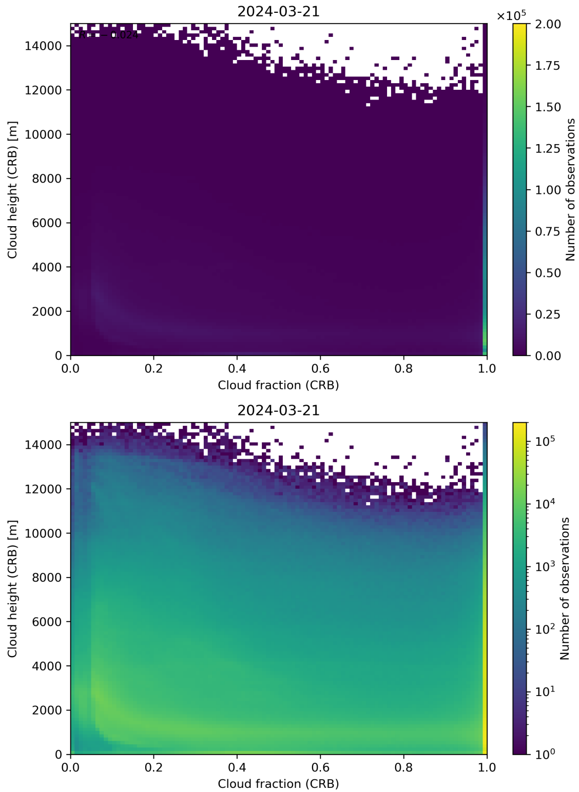
Figure 79: Scatter density plot of “Cloud fraction (CRB)” against “Cloud height (CRB)” for 2024-03-20 to 2024-03-22.
