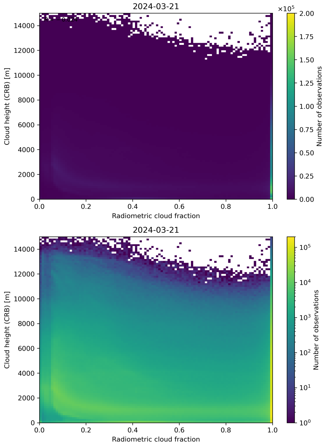
Figure 74: Scatter density plot of “Radiometric cloud fraction” against “Cloud height (CRB)” for 2024-03-20 to 2024-03-22.
