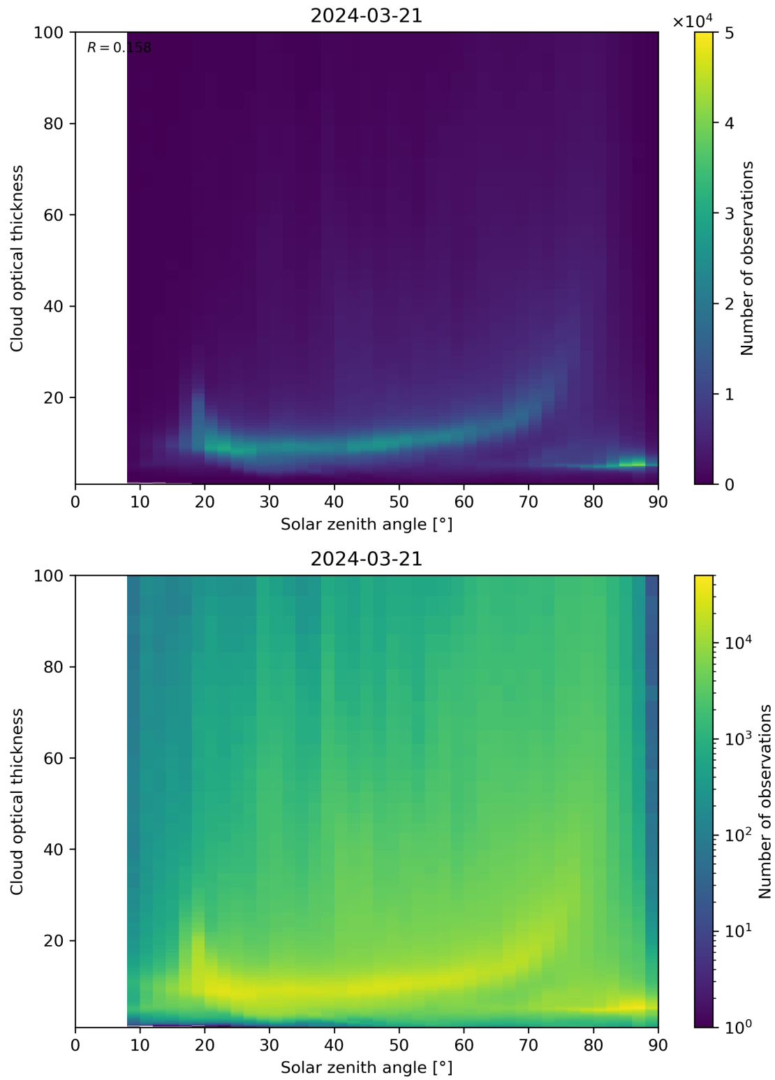
Figure 103: Scatter density plot of “Solar zenith angle” against “Cloud optical thickness” for 2024-03-20 to 2024-03-22.
