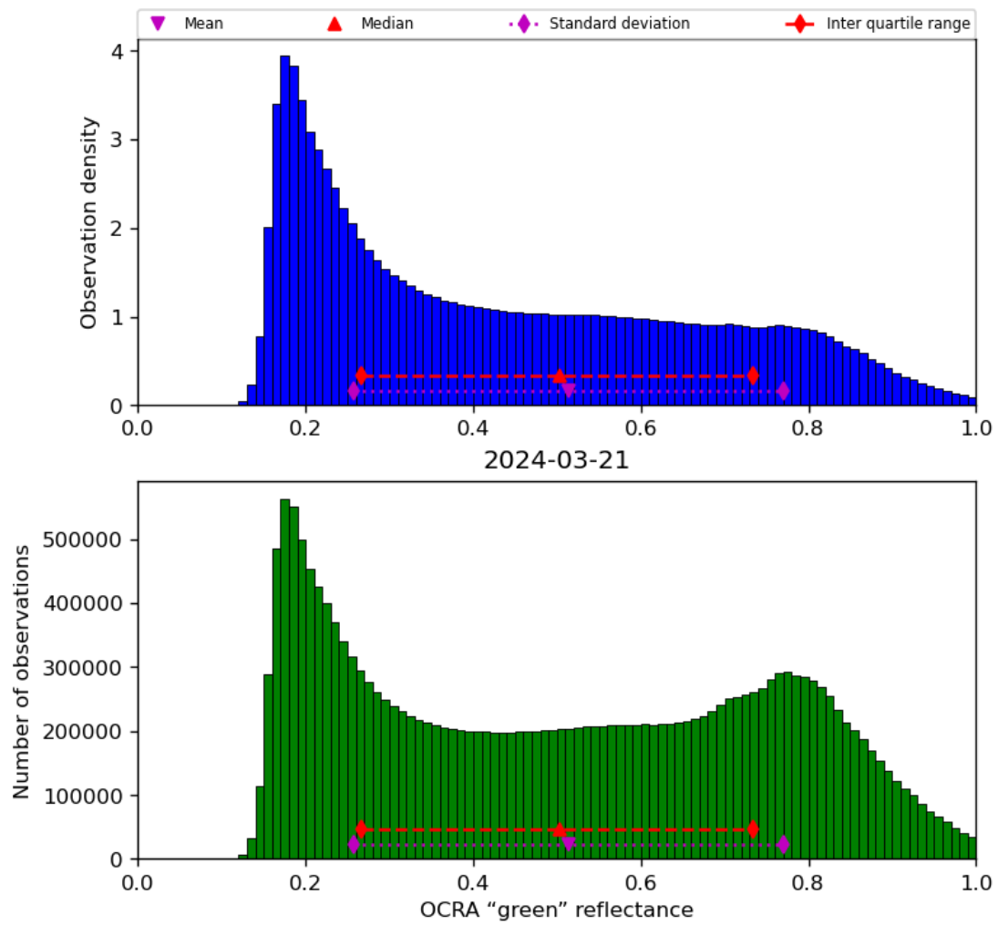
Figure 52: Histogram of “OCRA “green” reflectance” for 2024-03-20 to 2024-03-22
