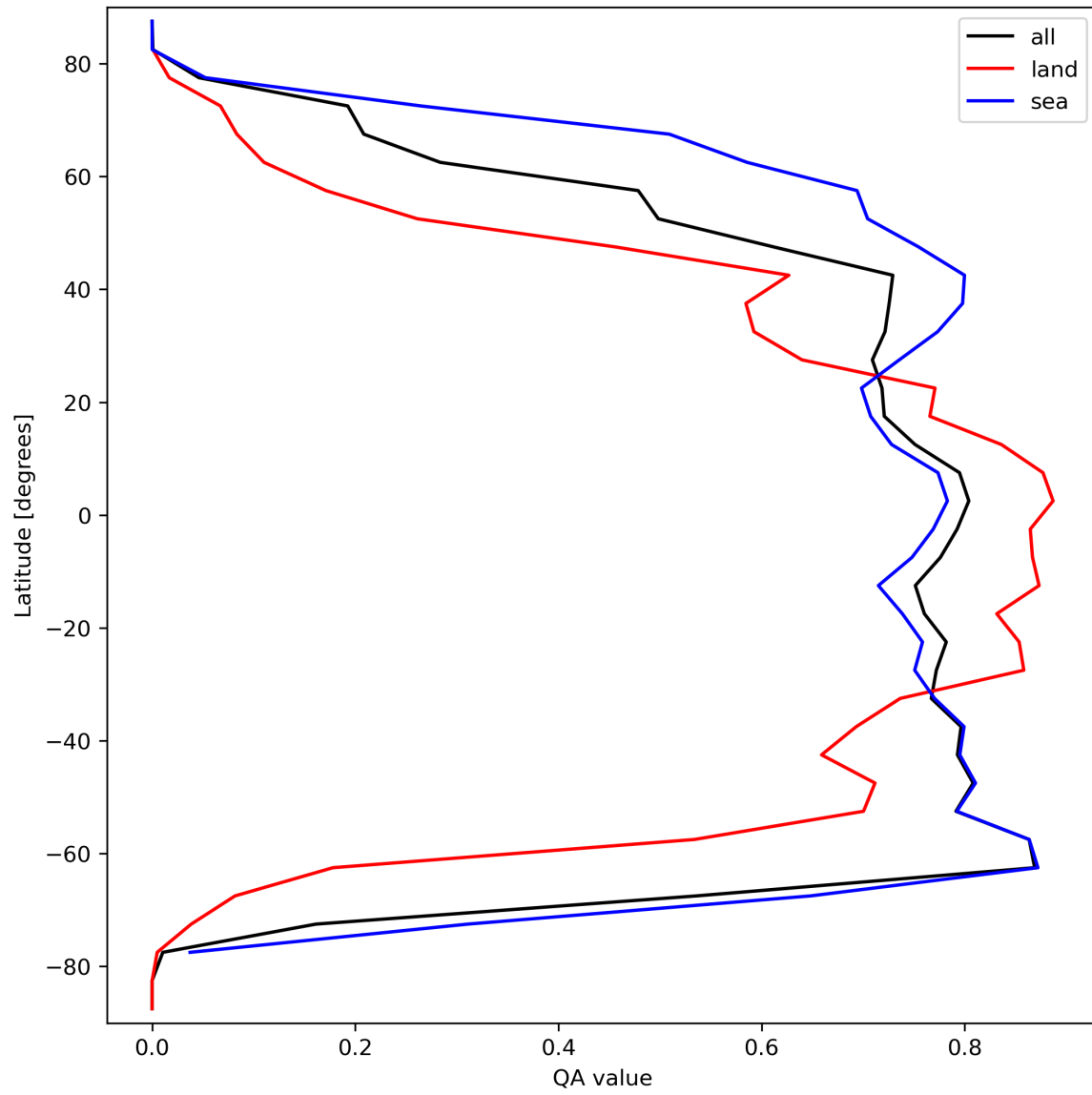
Figure 22: Zonal average of “QA value” for 2024-03-20 to 2024-03-22.
