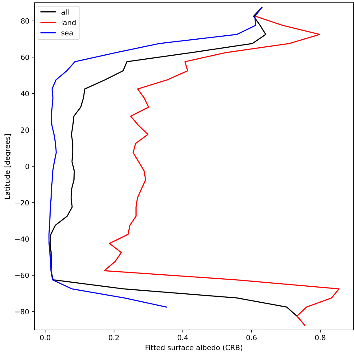
Figure 30: Zonal average of “Fitted surface albedo (CRB)” for 2024-03-20 to 2024-03-22.
