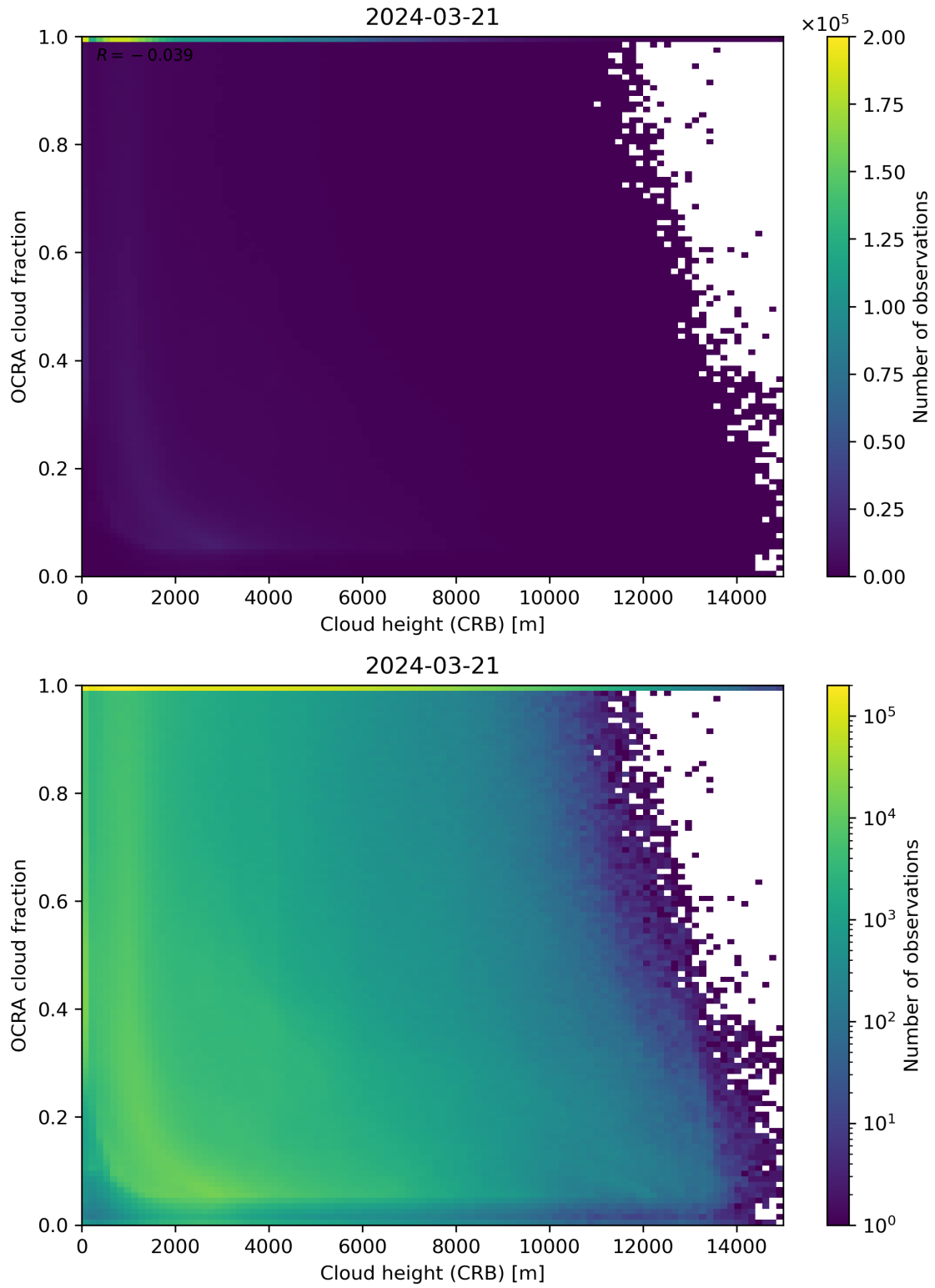
Figure 81: Scatter density plot of “Cloud height (CRB)” against “OCRA cloud fraction” for 2024-03-20 to 2024-03-22.
