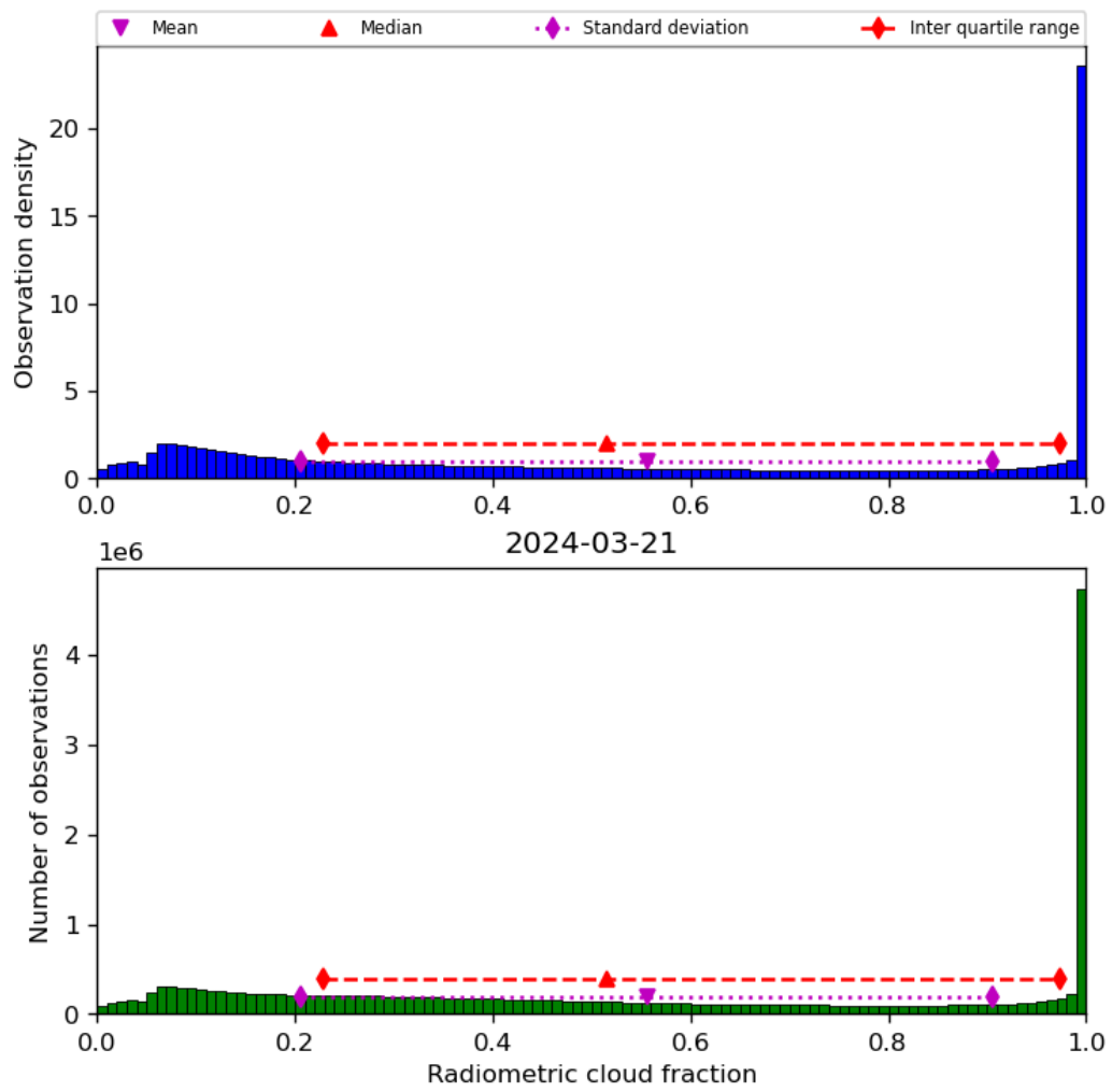
Figure 39: Histogram of “Radiometric cloud fraction” for 2024-03-20 to 2024-03-22
