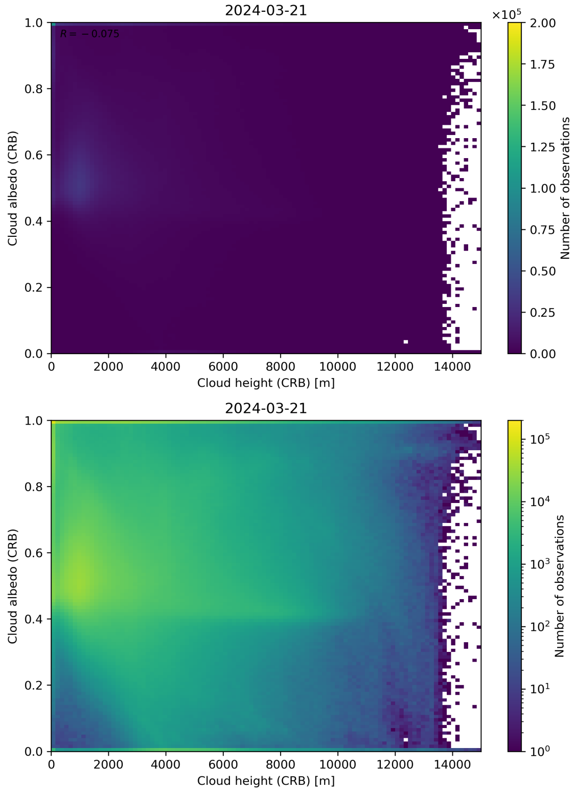
Figure 80: Scatter density plot of “Cloud height (CRB)” against “Cloud albedo (CRB)” for 2024-03-20 to 2024-03-22.
