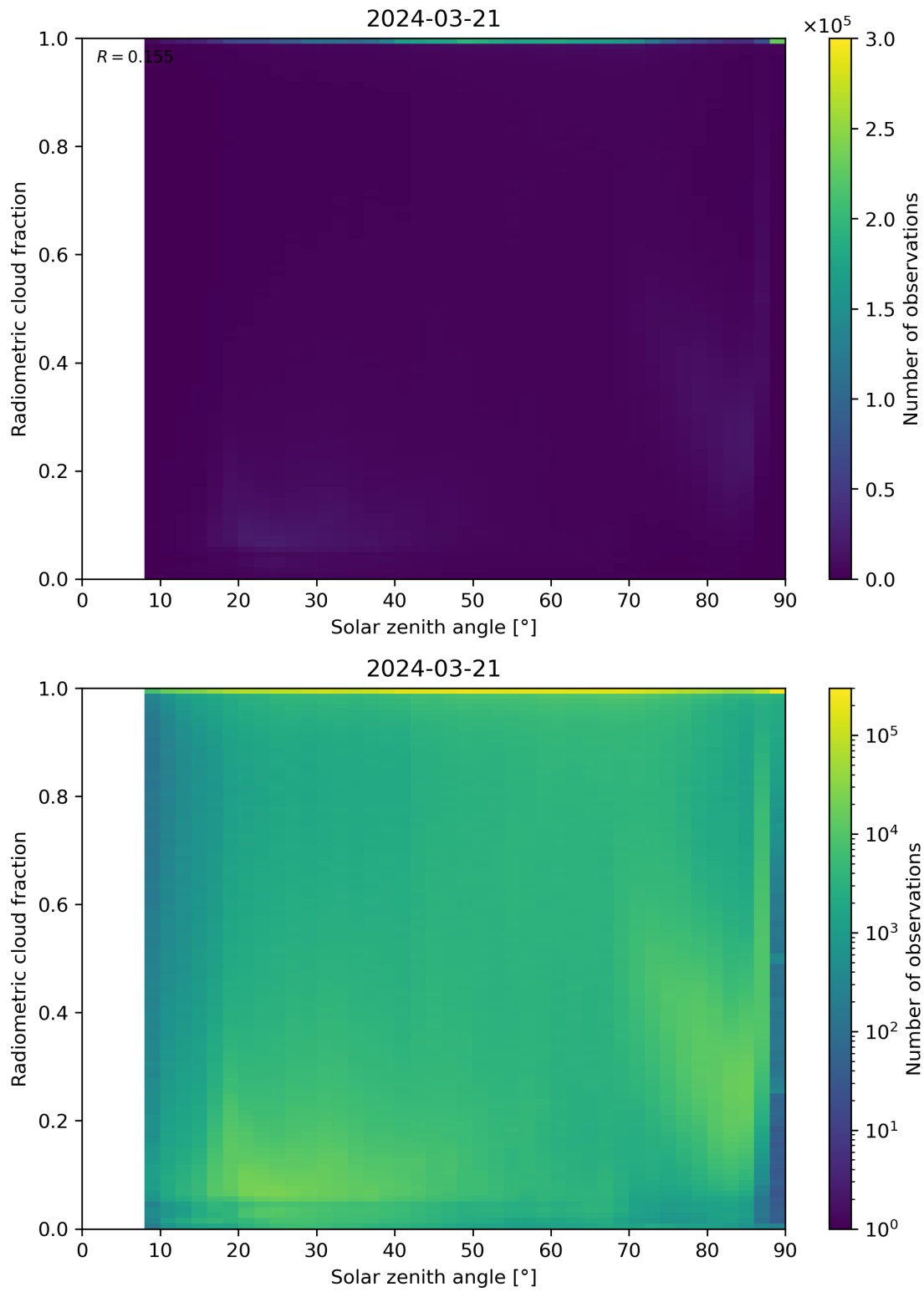
Figure 99: Scatter density plot of “Solar zenith angle” against “Radiometric cloud fraction” for 2024-03-20 to 2024-03-22.
