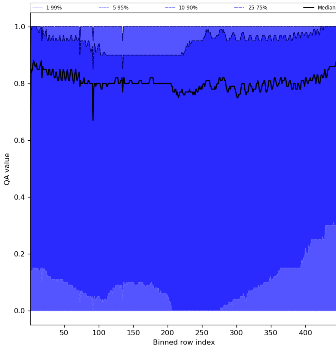
Figure 54: Along track statistics of “QA value” for 2024-03-20 to 2024-03-22
