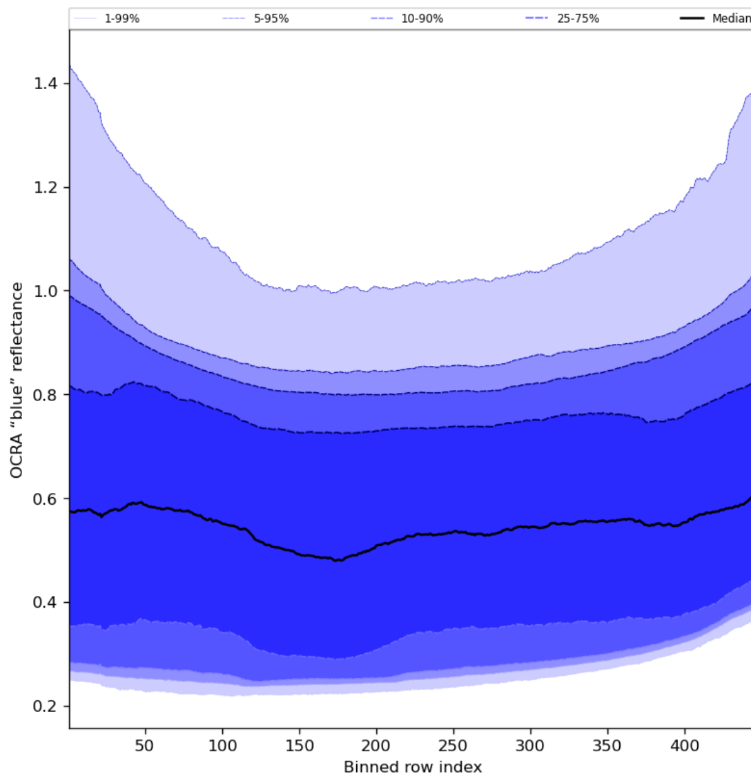
Figure 67: Along track statistics of “OCRA “blue” reflectance” for 2024-03-20 to 2024-03-22
