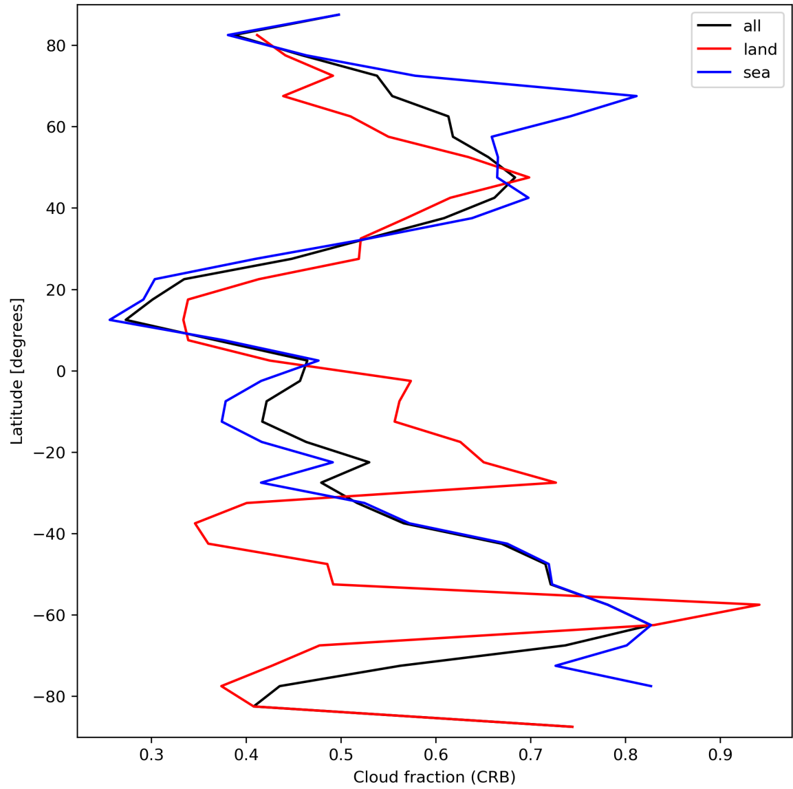
Figure 26: Zonal average of “Cloud fraction (CRB)” for 2024-03-20 to 2024-03-22.
