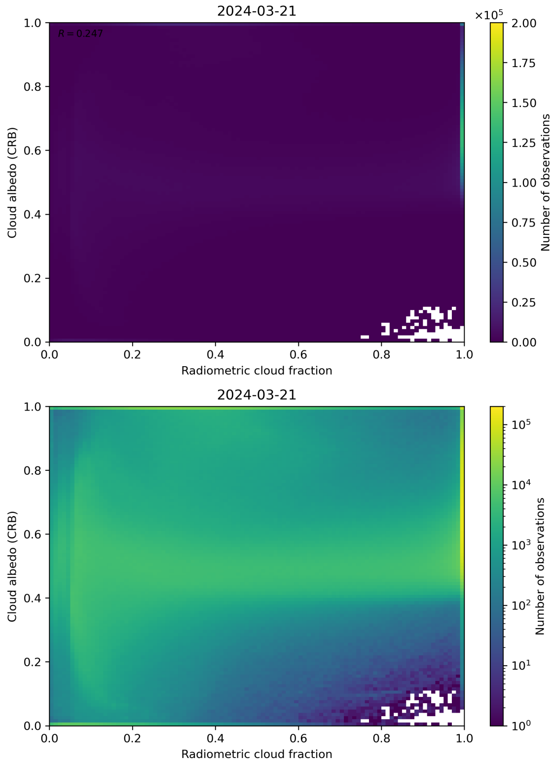
Figure 71: Scatter density plot of “Radiometric cloud fraction” against “Cloud albedo (CRB)” for 2024-03-20 to 2024-03-22.
