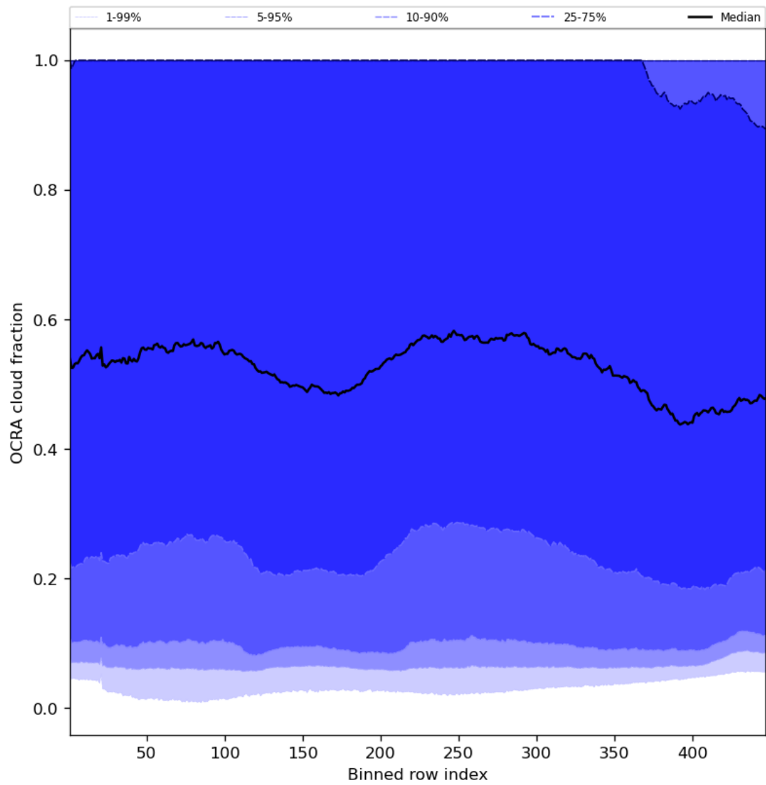
Figure 66: Along track statistics of “OCRA cloud fraction” for 2024-03-20 to 2024-03-22
