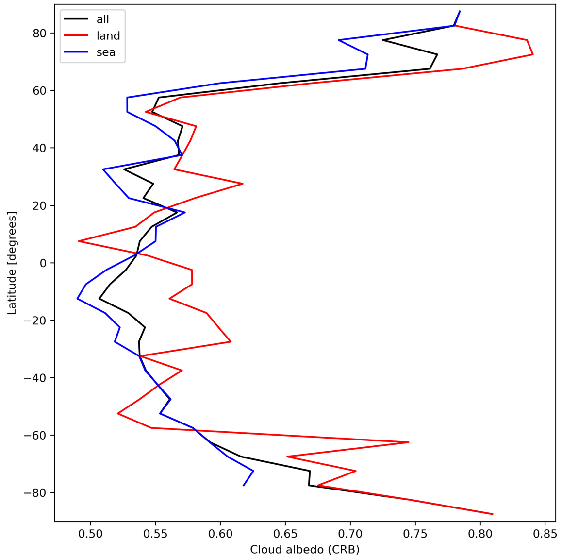
Figure 28: Zonal average of “Cloud albedo (CRB)” for 2024-03-20 to 2024-03-22.
