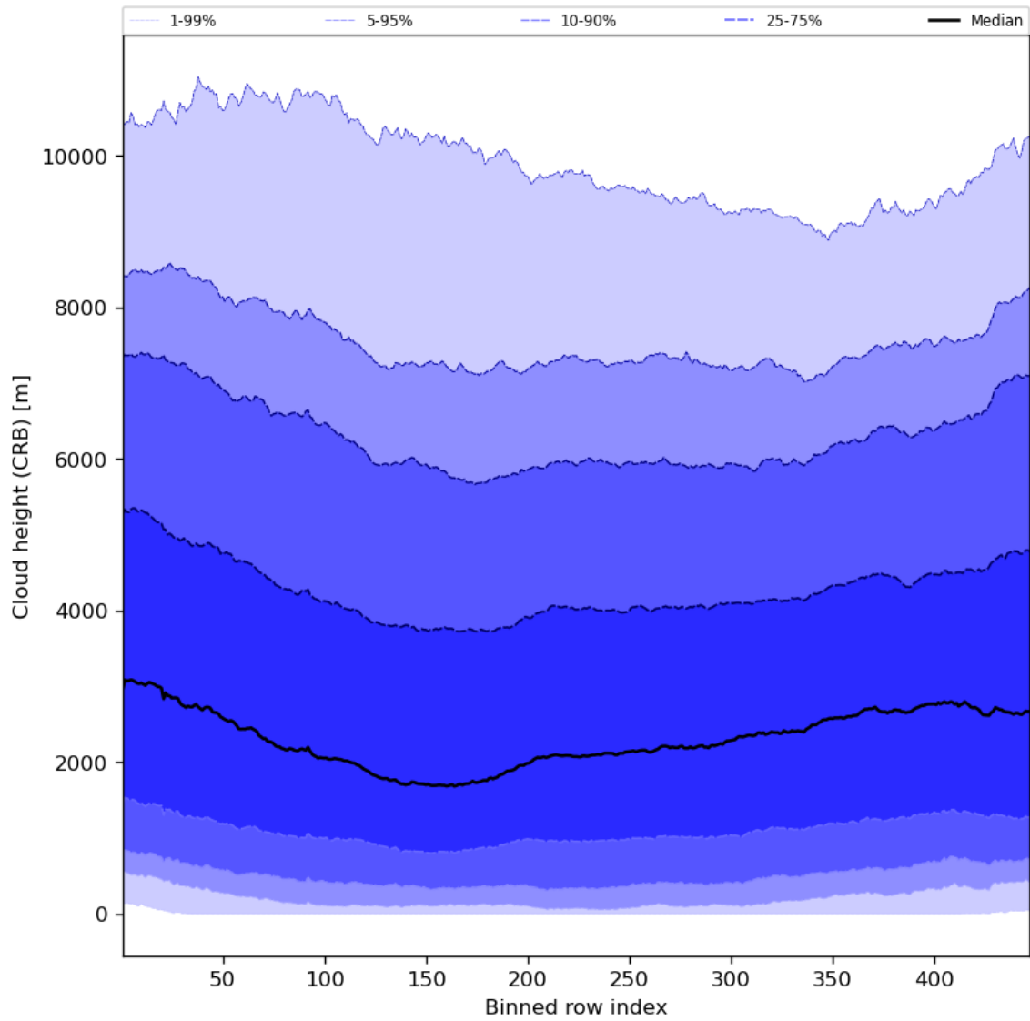
Figure 59: Along track statistics of “Cloud height (CRB)” for 2024-03-20 to 2024-03-22
