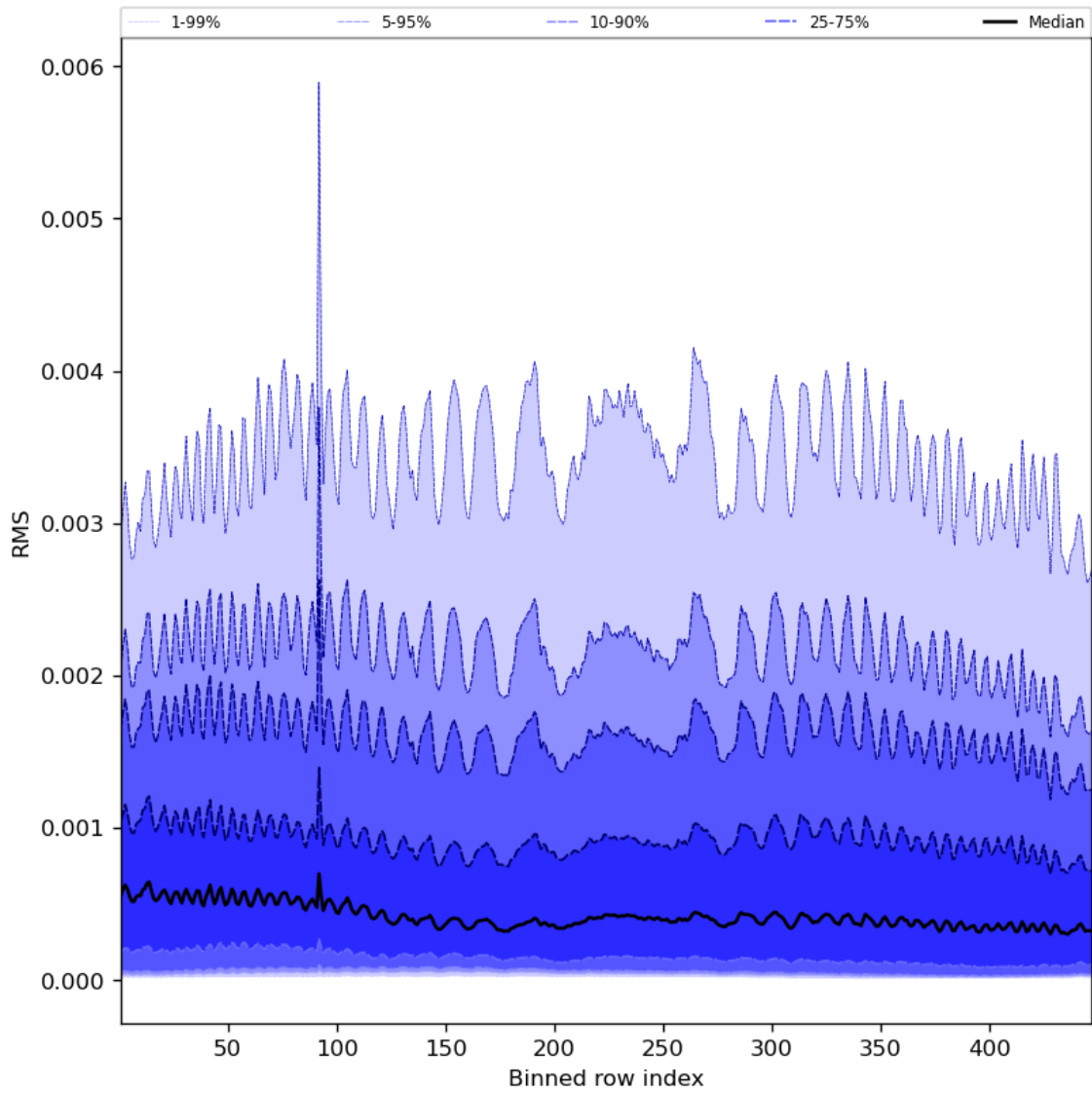
Figure 63: Along track statistics of “RMS” for 2024-03-20 to 2024-03-22
