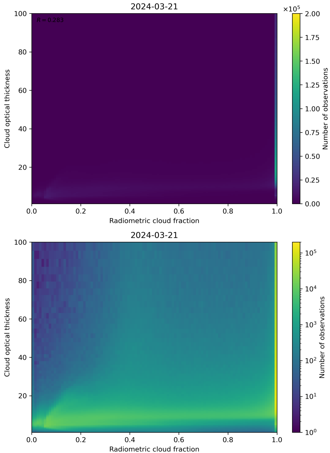
Figure 75: Scatter density plot of “Radiometric cloud fraction” against “Cloud optical thickness” for 2024-03-20 to 2024-03-22.
