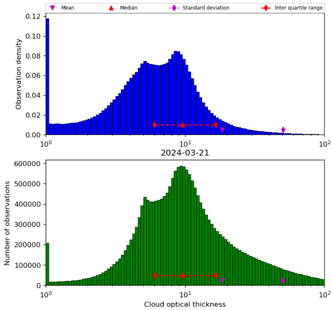
Figure 41: Histogram of “Cloud optical thickness” for 2024-03-20 to 2024-03-22
