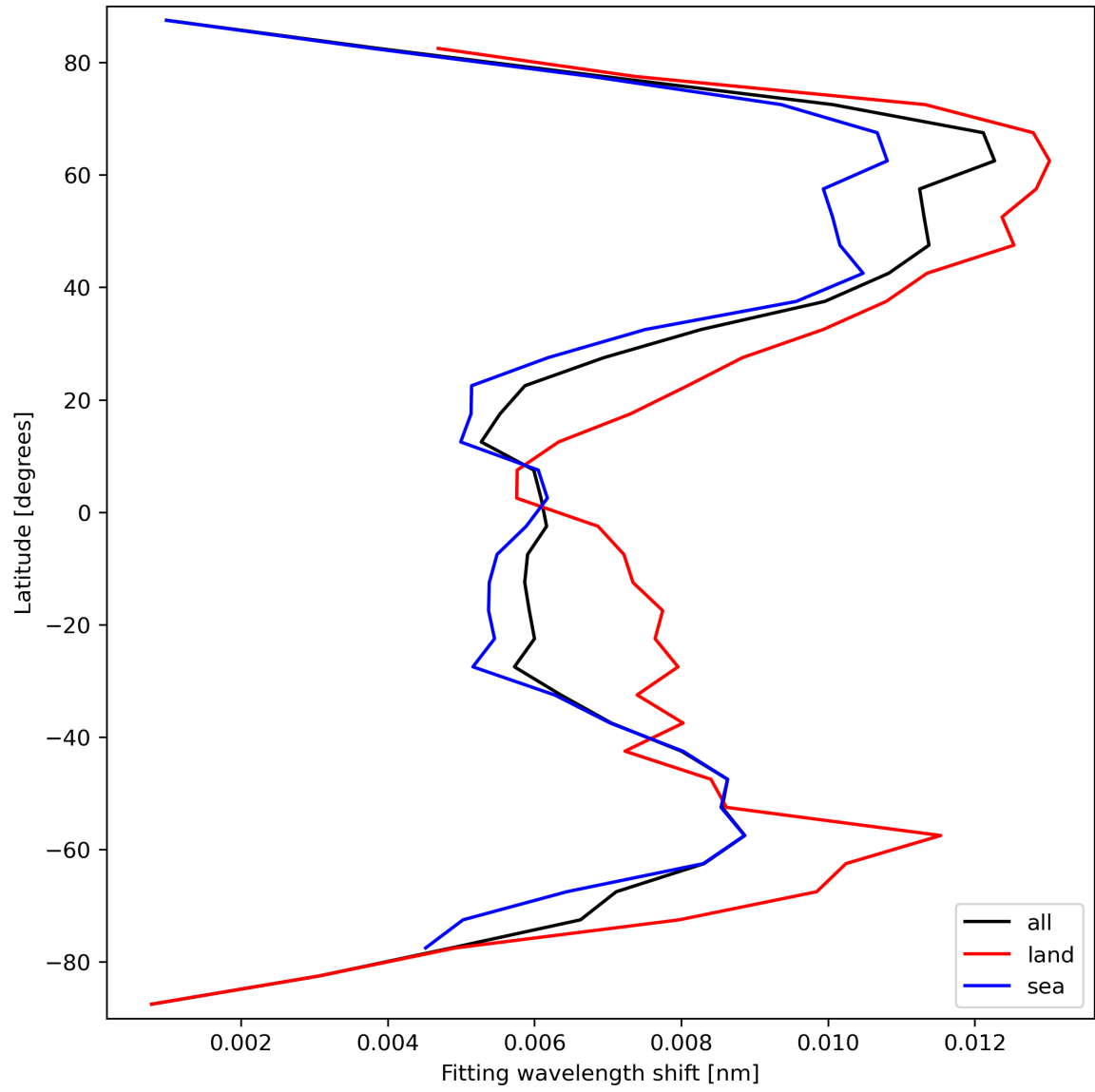
Figure 33: Zonal average of “Fitting wavelength shift” for 2024-03-20 to 2024-03-22.
