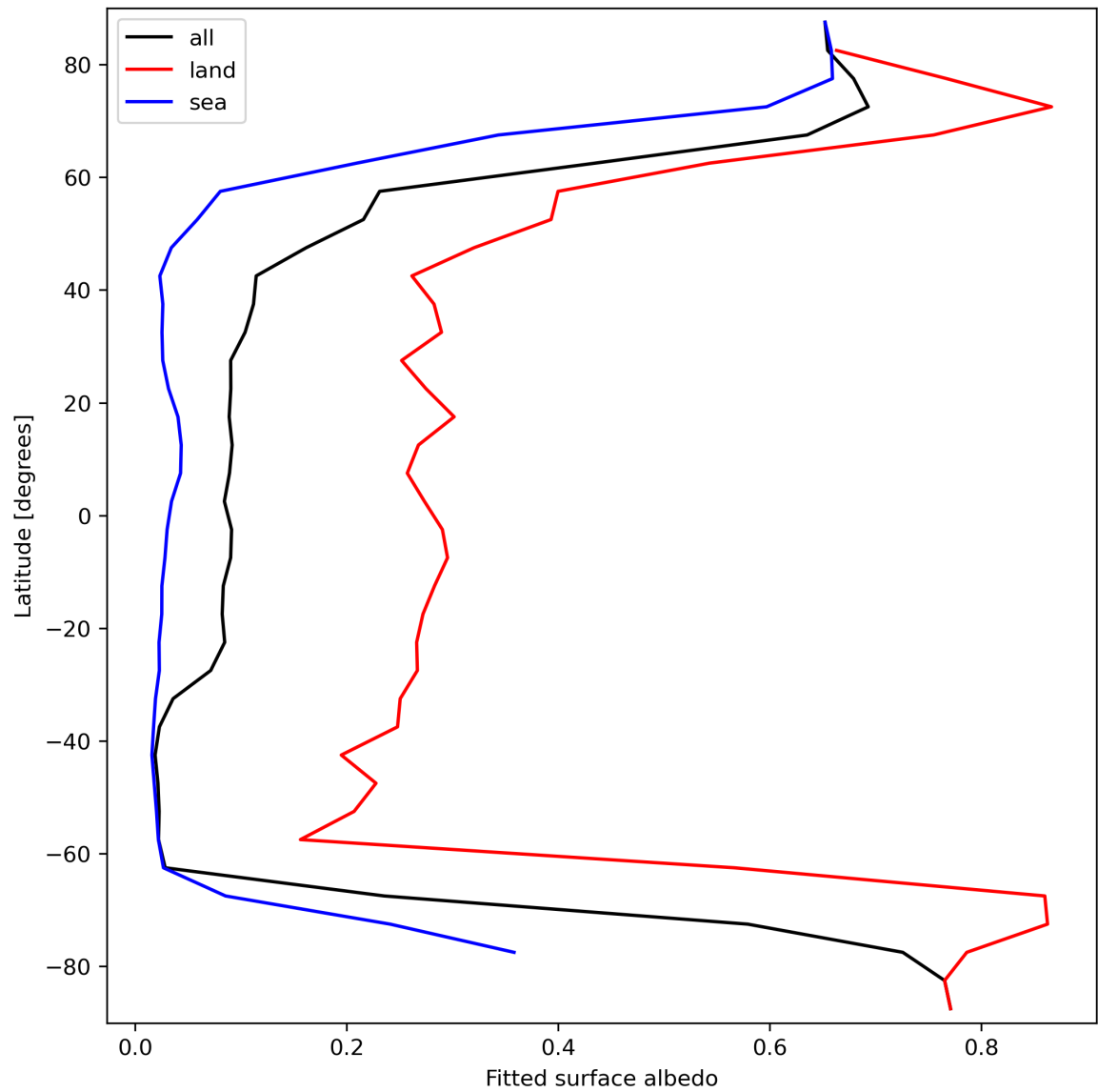
Figure 29: Zonal average of “Fitted surface albedo” for 2024-03-20 to 2024-03-22.
