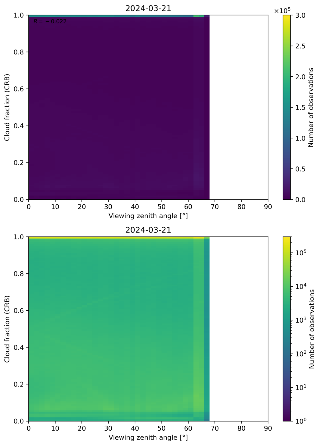
Figure 109: Scatter density plot of “Viewing zenith angle” against “Cloud fraction (CRB)” for 2024-03-20 to 2024-03-22.
