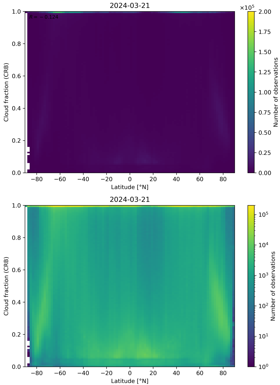
Figure 94: Scatter density plot of “Latitude” against “Cloud fraction (CRB)” for 2024-03-20 to 2024-03-22.
