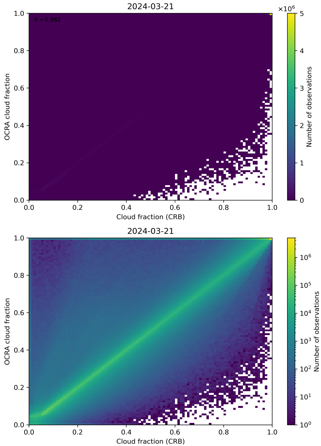
Figure 78: Scatter density plot of “Cloud fraction (CRB)” against “OCRA cloud fraction” for 2024-03-20 to 2024-03-22.
