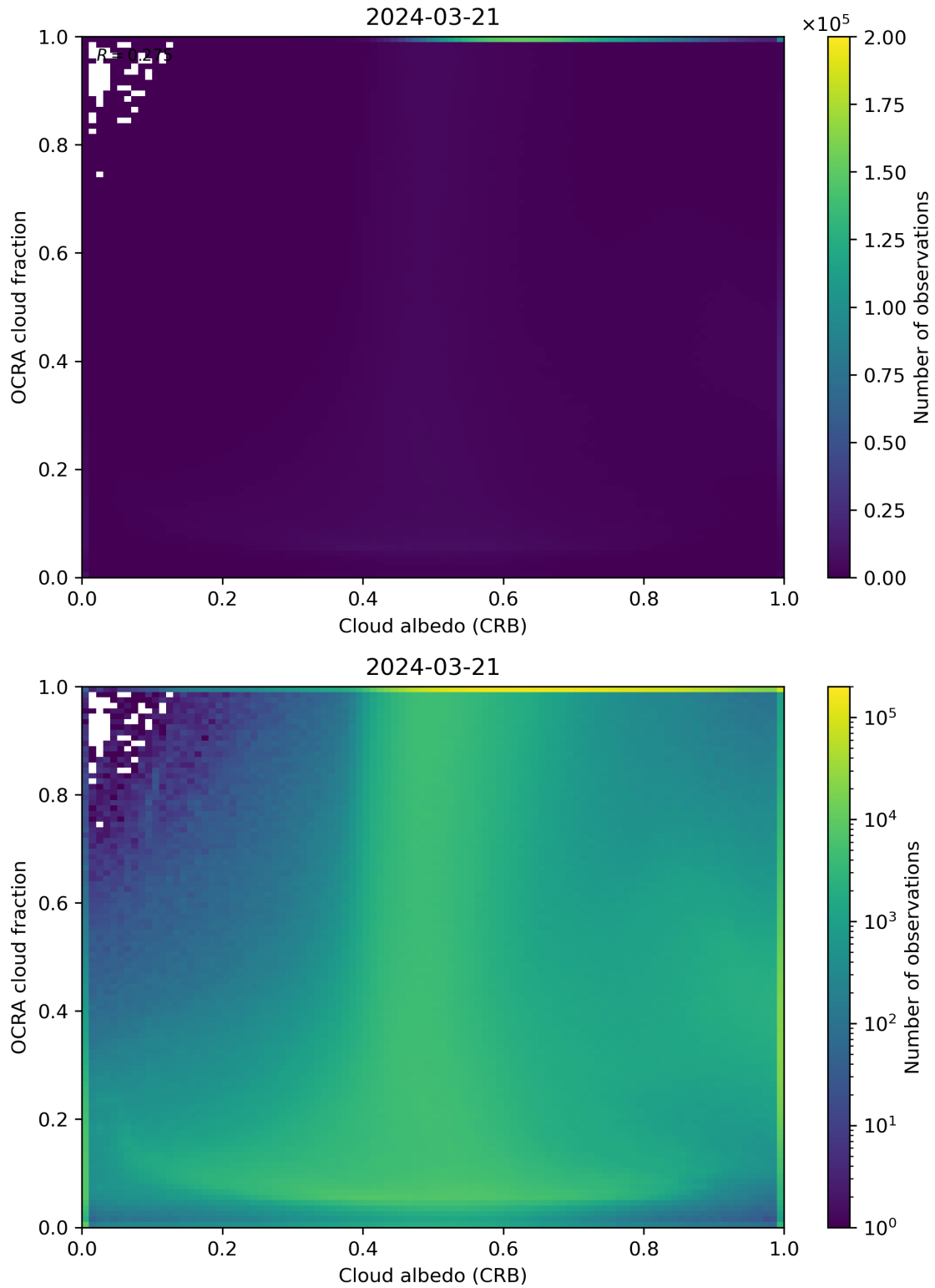
Figure 70: Scatter density plot of “Cloud albedo (CRB)” against “OCRA cloud fraction” for 2024-03-20 to 2024-03-22.
