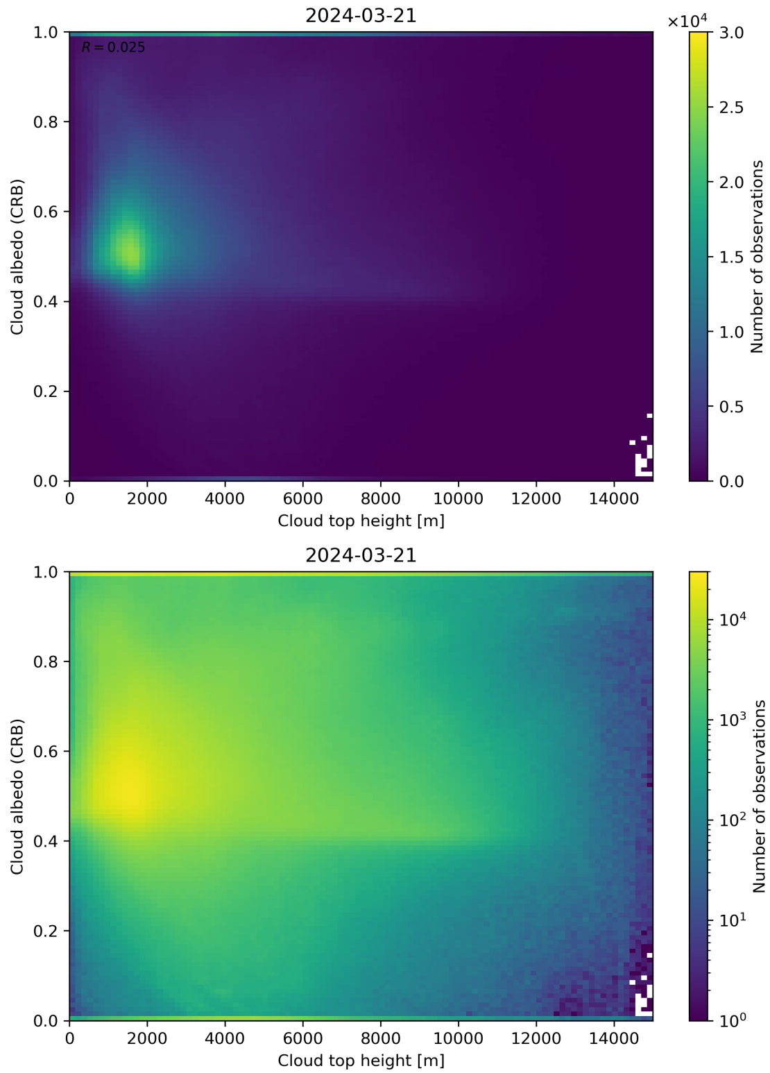
Figure 86: Scatter density plot of “Cloud top height” against “Cloud albedo (CRB)” for 2024-03-20 to 2024-03-22.
