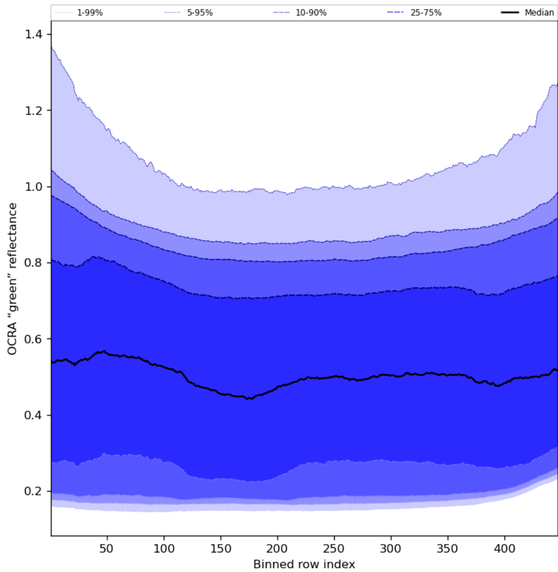
Figure 68: Along track statistics of "OCRA "green" reflectance" for 2024-03-20 to 2024-03-22
