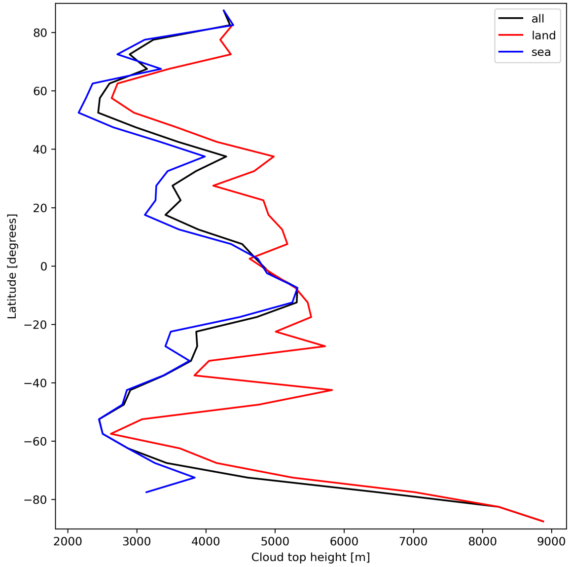
Figure 24: Zonal average of “Cloud top height” for 2024-03-20 to 2024-03-22.
