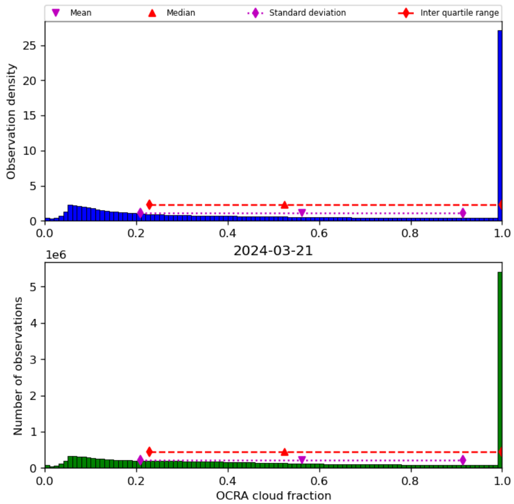
Figure 50: Histogram of “OCRA cloud fraction” for 2024-03-20 to 2024-03-22
