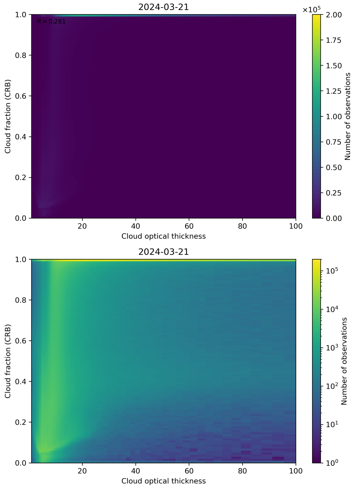
Figure 84: Scatter density plot of “Cloud optical thickness” against “Cloud fraction (CRB)” for 2024-03-20 to 2024-03-22.
