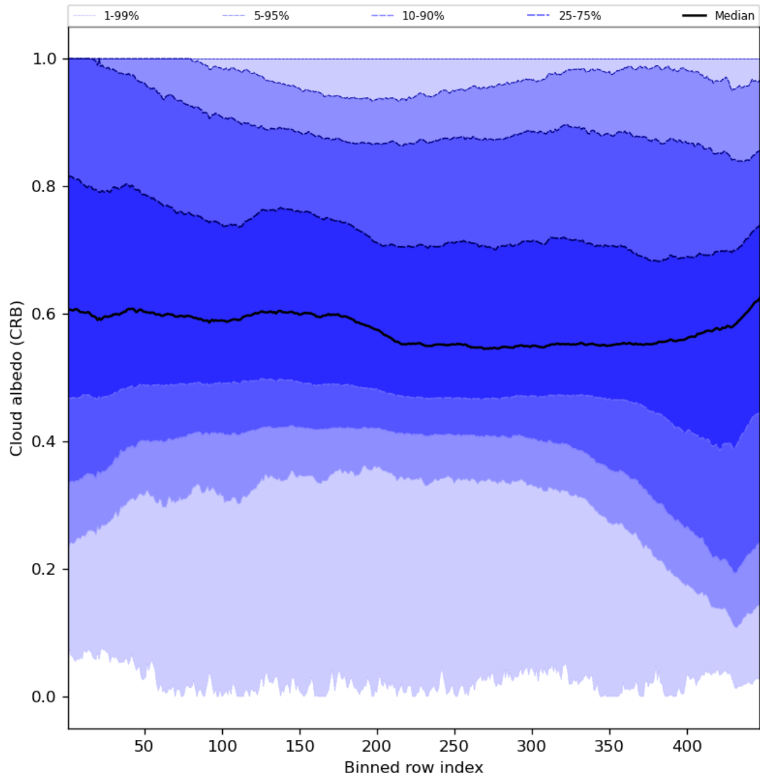
Figure 60: Along track statistics of “Cloud albedo (CRB)” for 2024-03-20 to 2024-03-22
