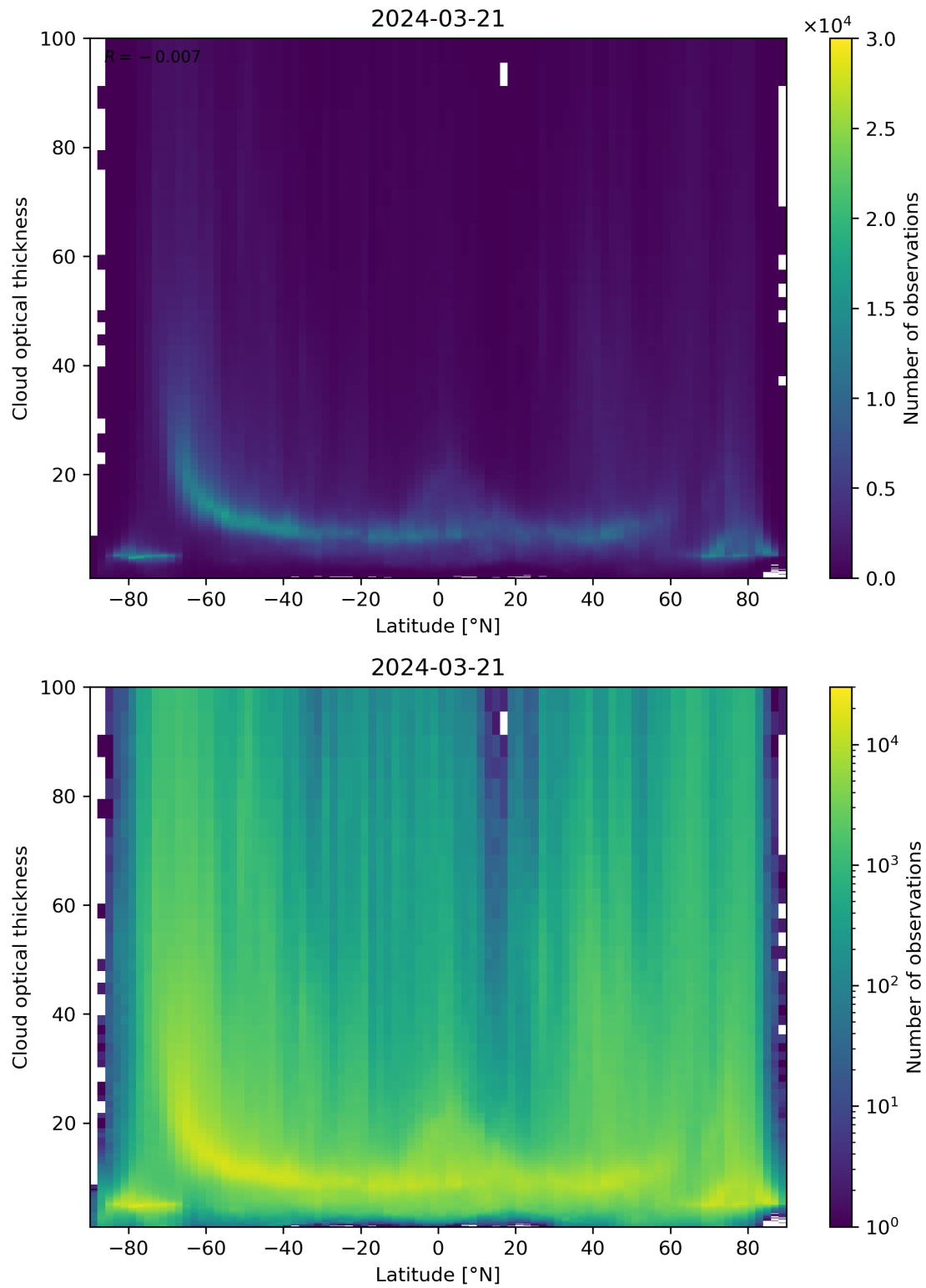
Figure 96: Scatter density plot of “Latitude” against “Cloud optical thickness” for 2024-03-20 to 2024-03-22.
