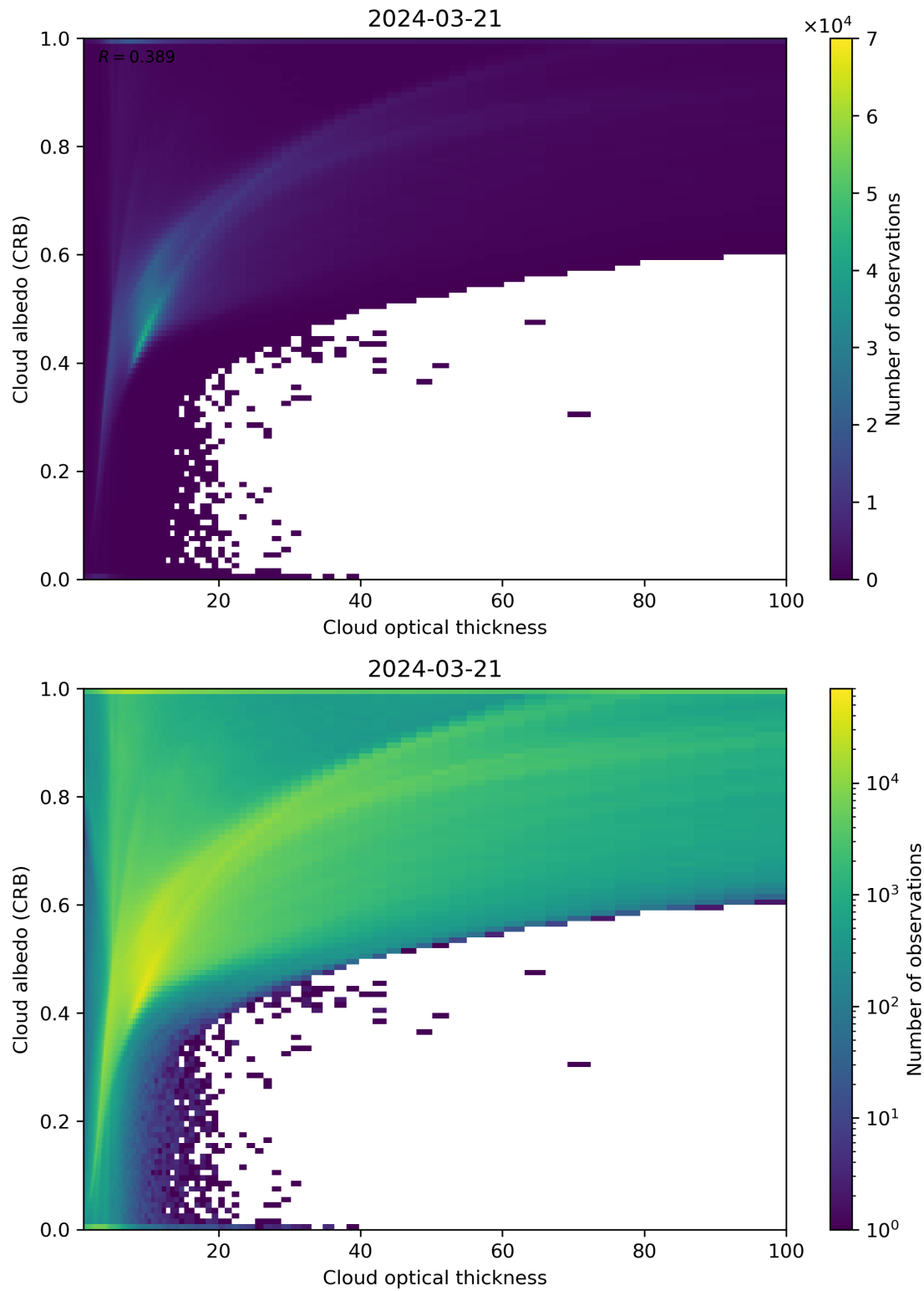
Figure 82: Scatter density plot of “Cloud optical thickness” against “Cloud albedo (CRB)” for 2024-03-20 to 2024-03-22.
