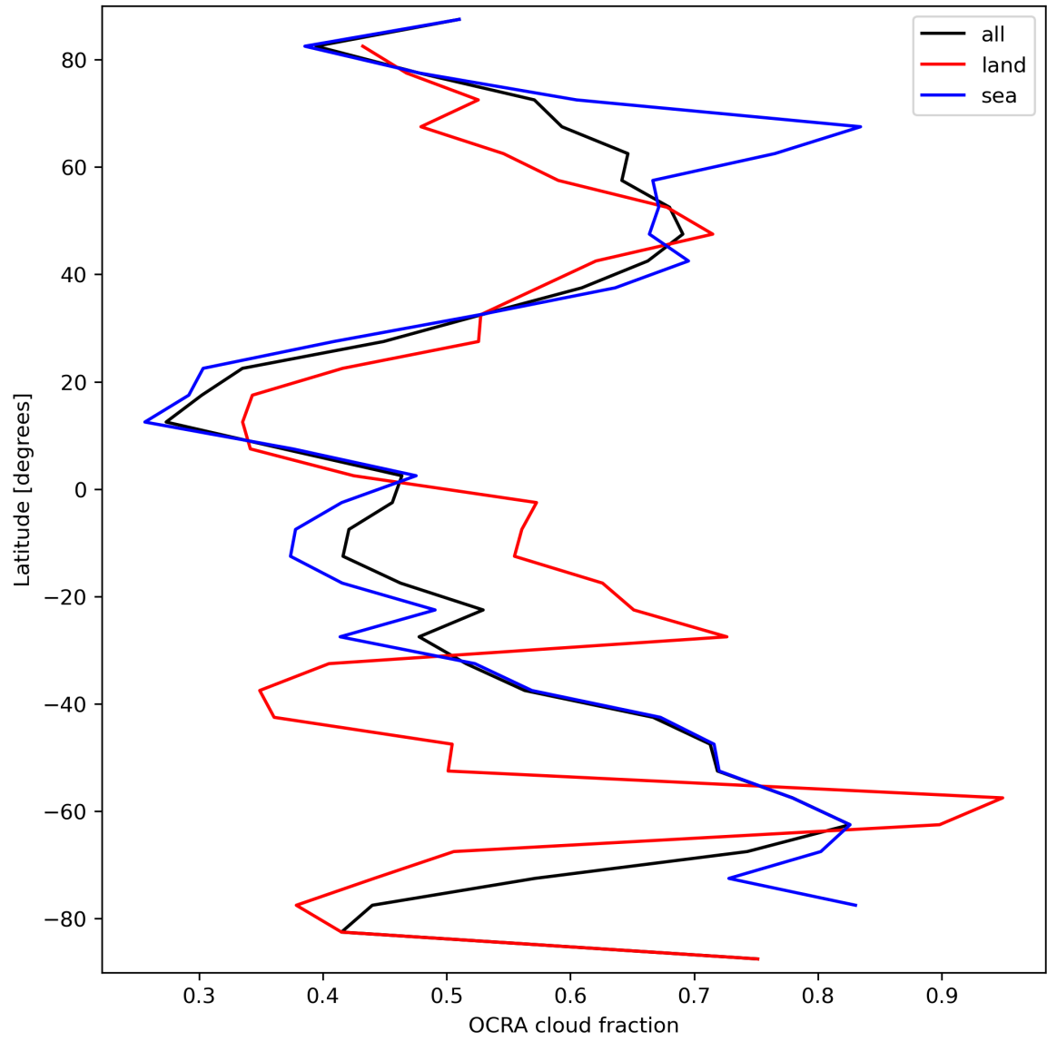
Figure 34: Zonal average of “OCRA cloud fraction” for 2024-03-20 to 2024-03-22.
