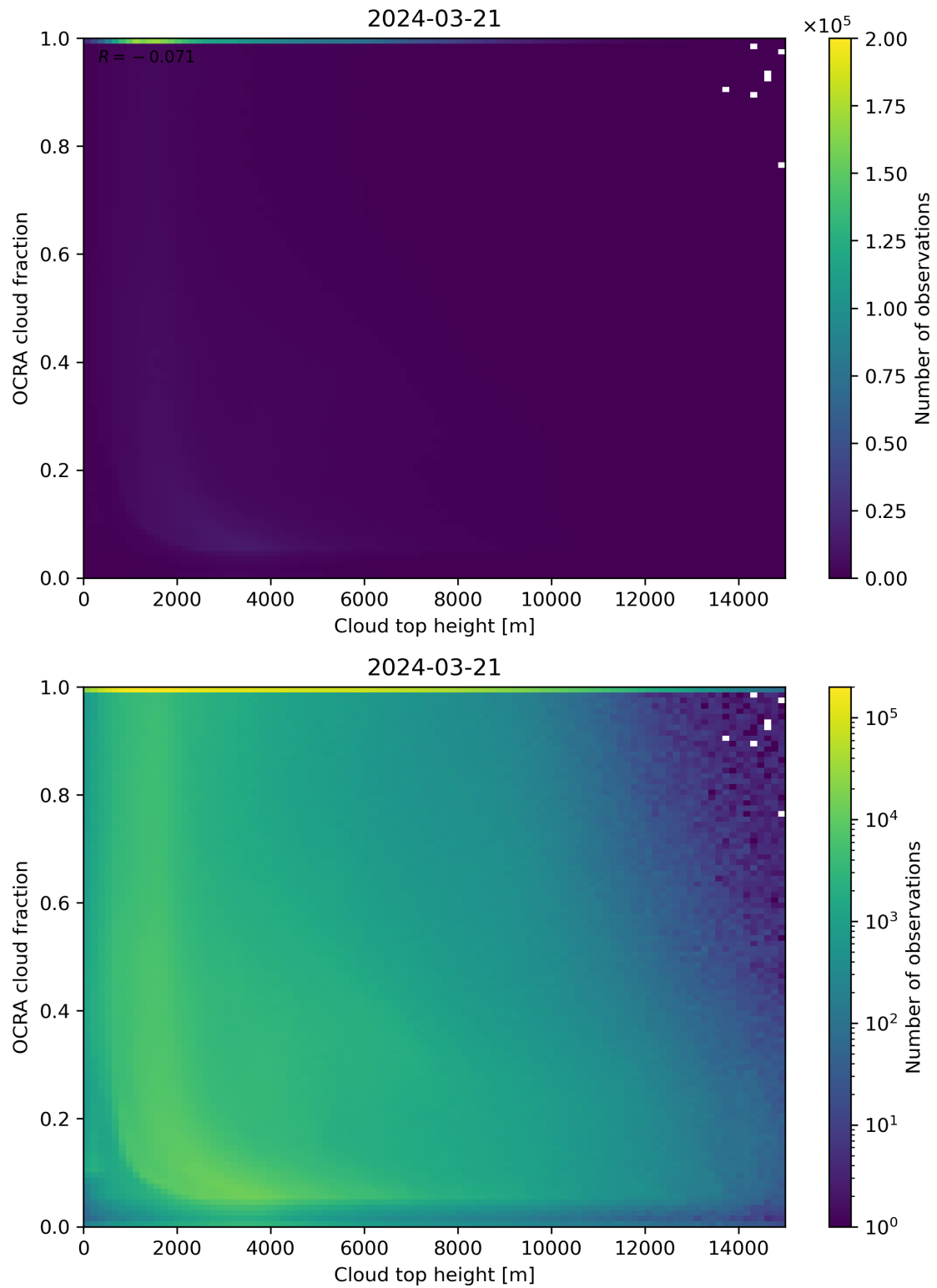
Figure 87: Scatter density plot of “Cloud top height” against “OCRA cloud fraction” for 2024-03-20 to 2024-03-22.
