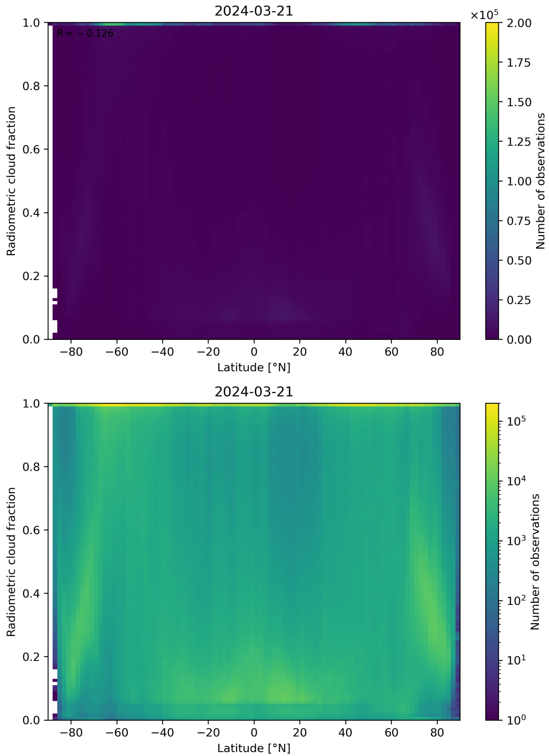
Figure 92: Scatter density plot of “Latitude” against “Radiometric cloud fraction” for 2024-03-20 to 2024-03-22.
