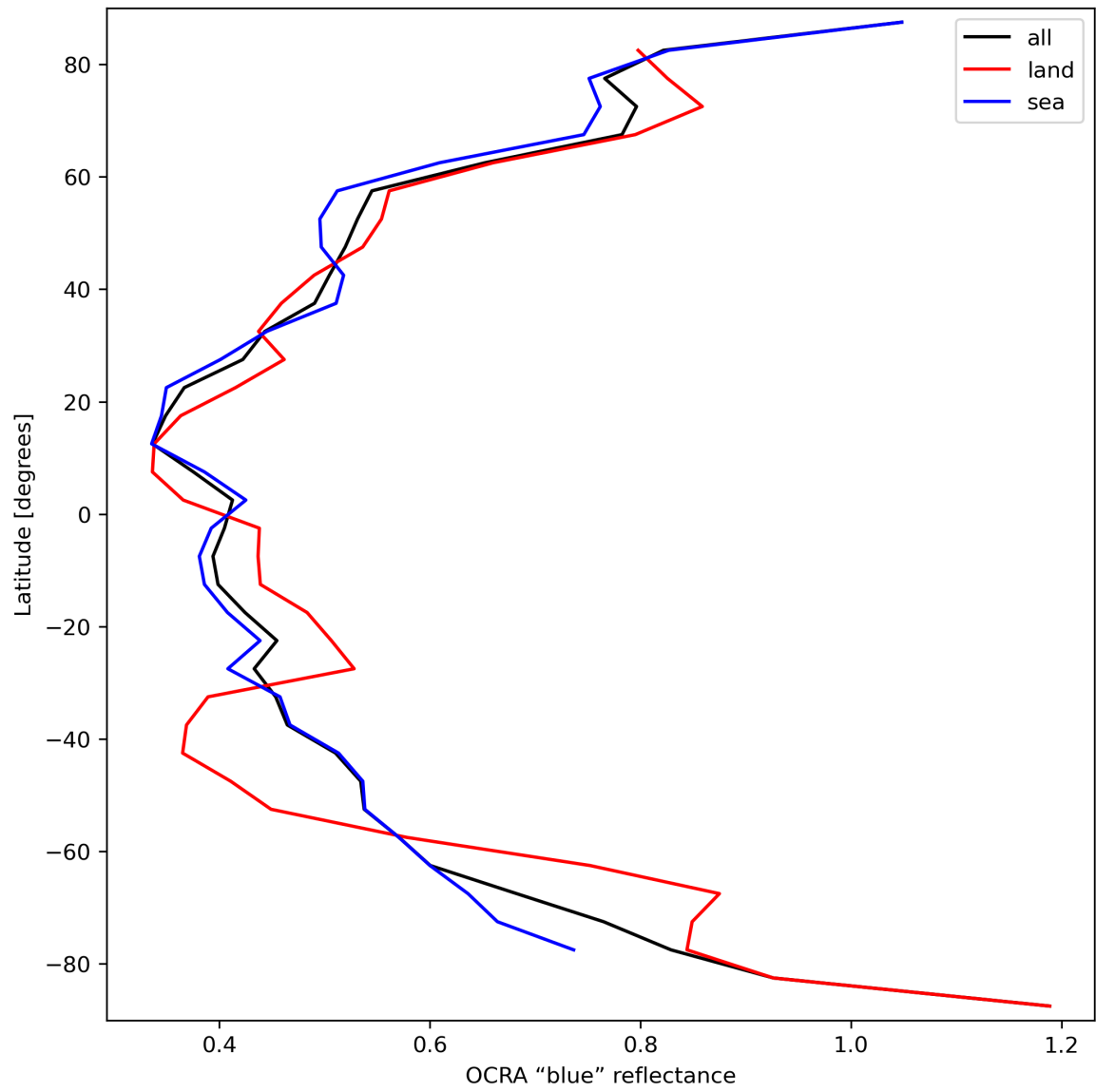
Figure 35: Zonal average of “OCRA “blue” reflectance” for 2024-03-20 to 2024-03-22.
