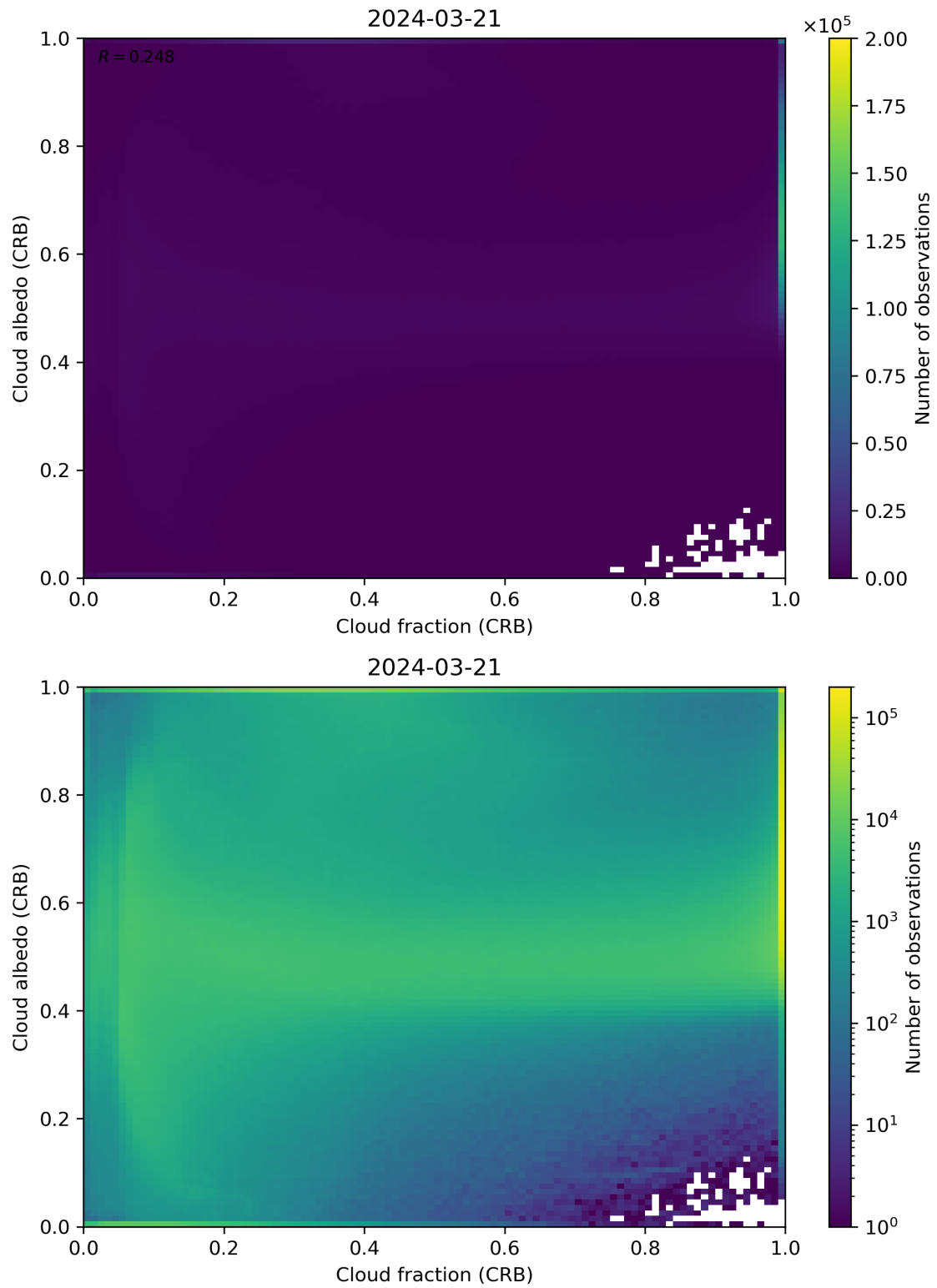
Figure 77: Scatter density plot of “Cloud fraction (CRB)” against “Cloud albedo (CRB)” for 2024-03-20 to 2024-03-22.
