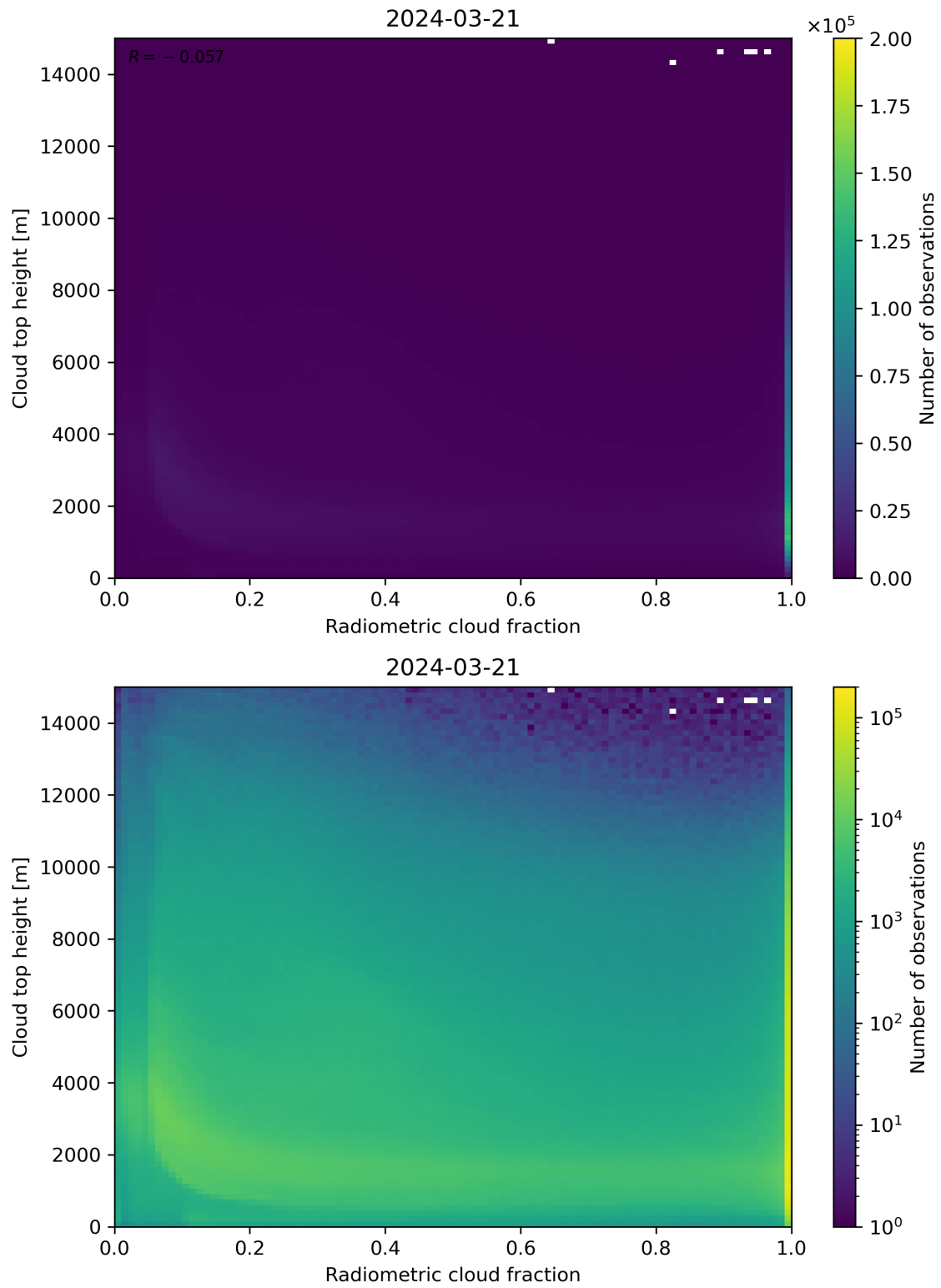
Figure 76: Scatter density plot of “Radiometric cloud fraction” against “Cloud top height” for 2024-03-20 to 2024-03-22.
