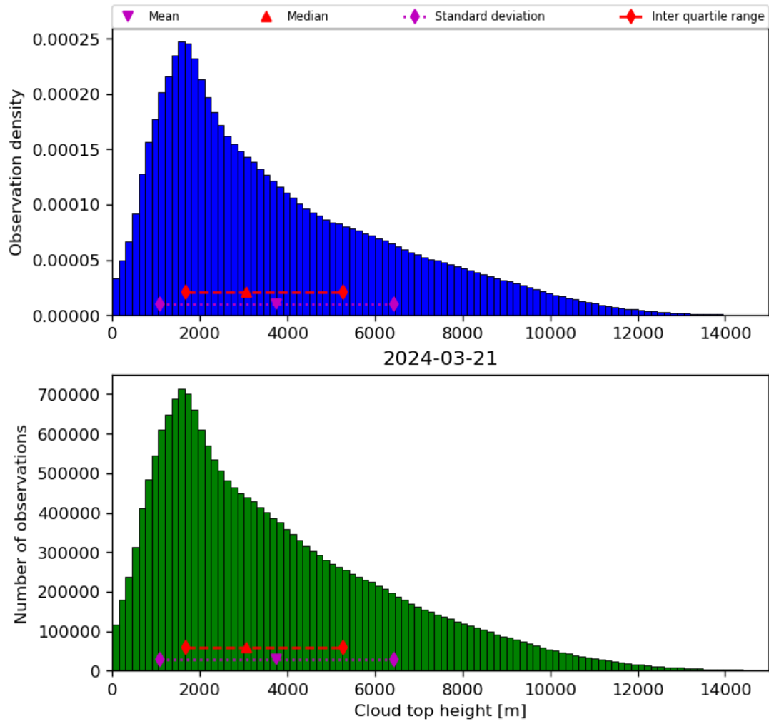
Figure 40: Histogram of “Cloud top height” for 2024-03-20 to 2024-03-22
