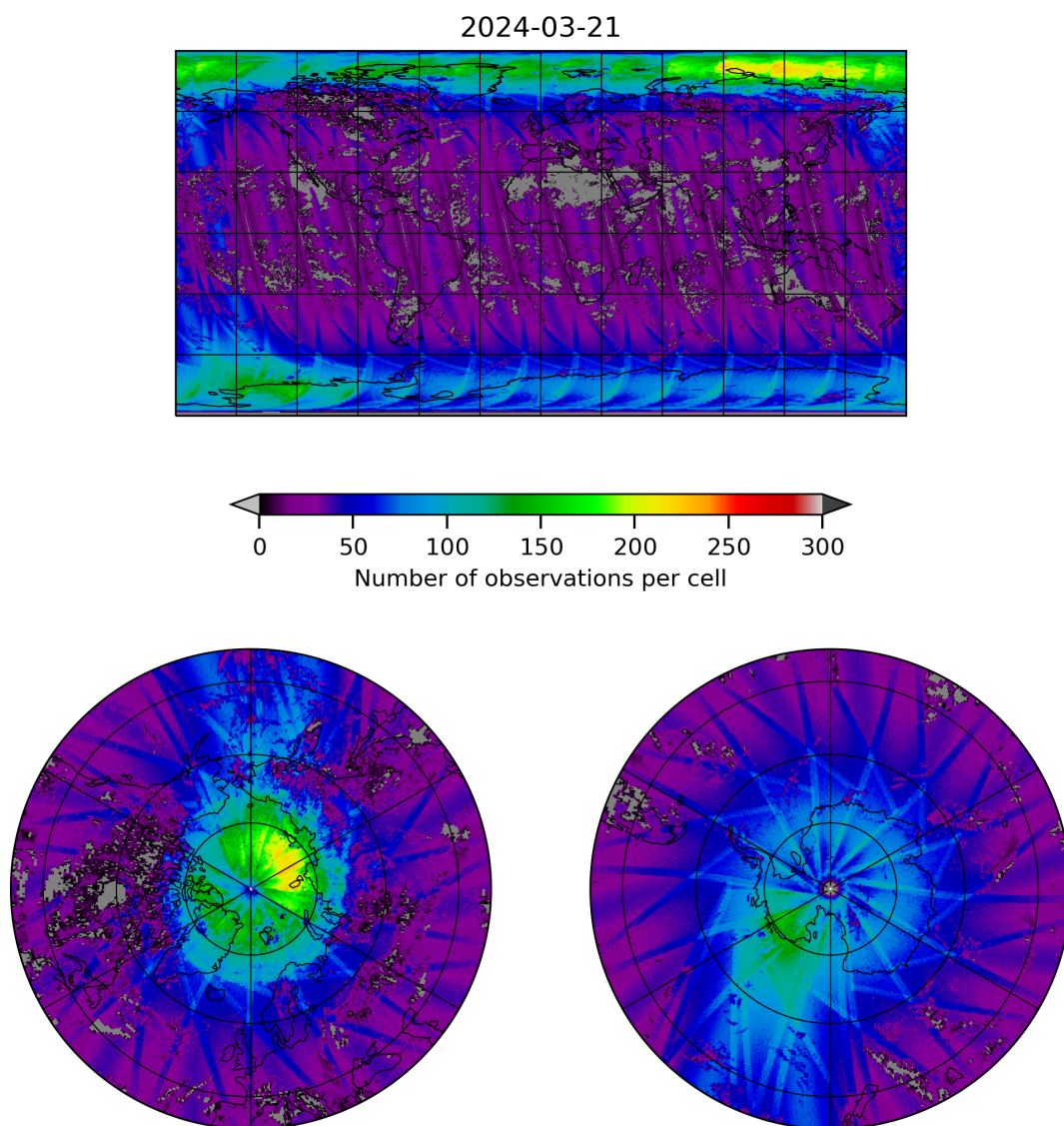
Figure 21: Map of the number of observations for 2024-03-20 to 2024-03-22
