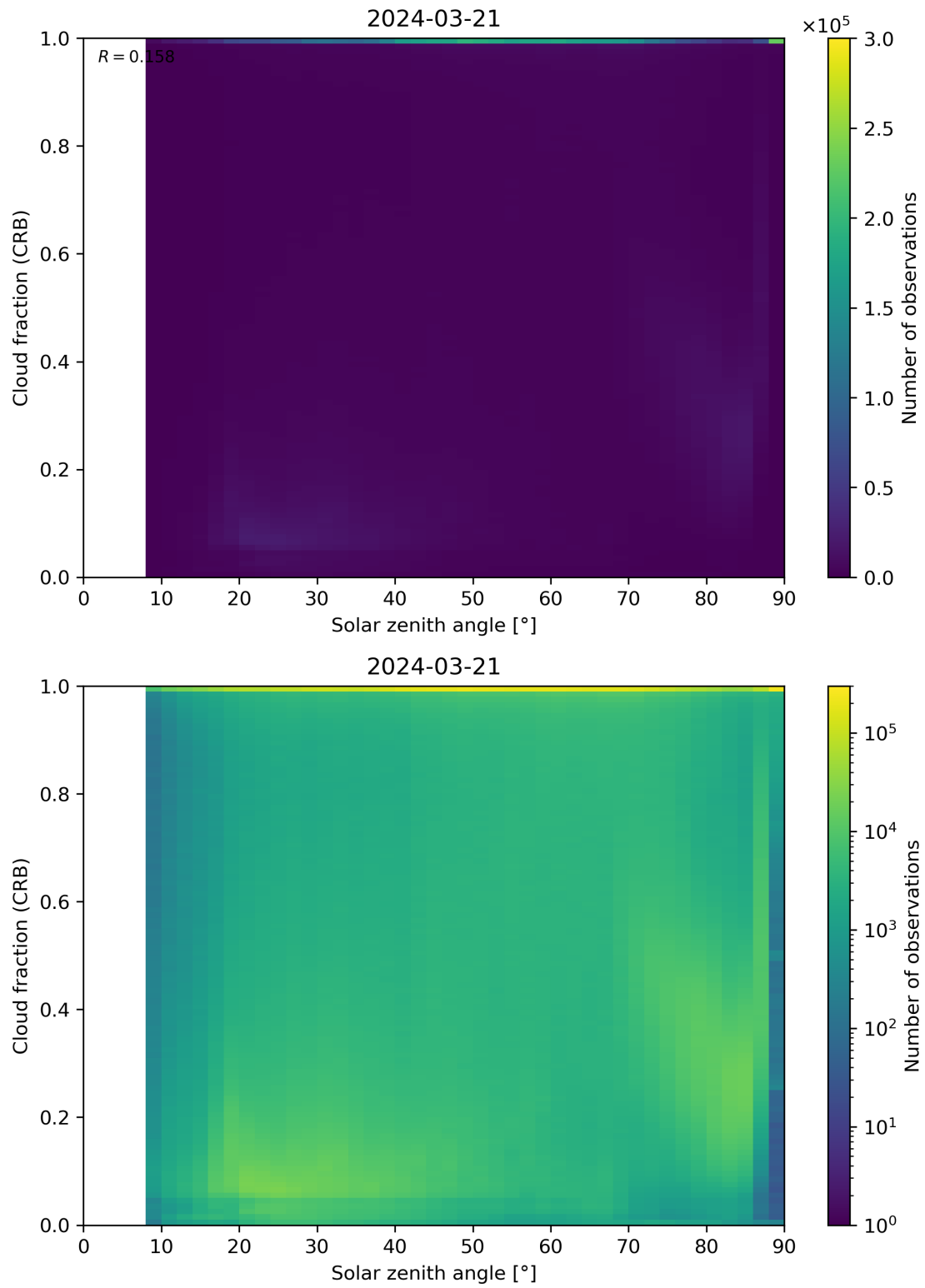
Figure 101: Scatter density plot of “Solar zenith angle” against “Cloud fraction (CRB)” for 2024-03-20 to 2024-03-22.
