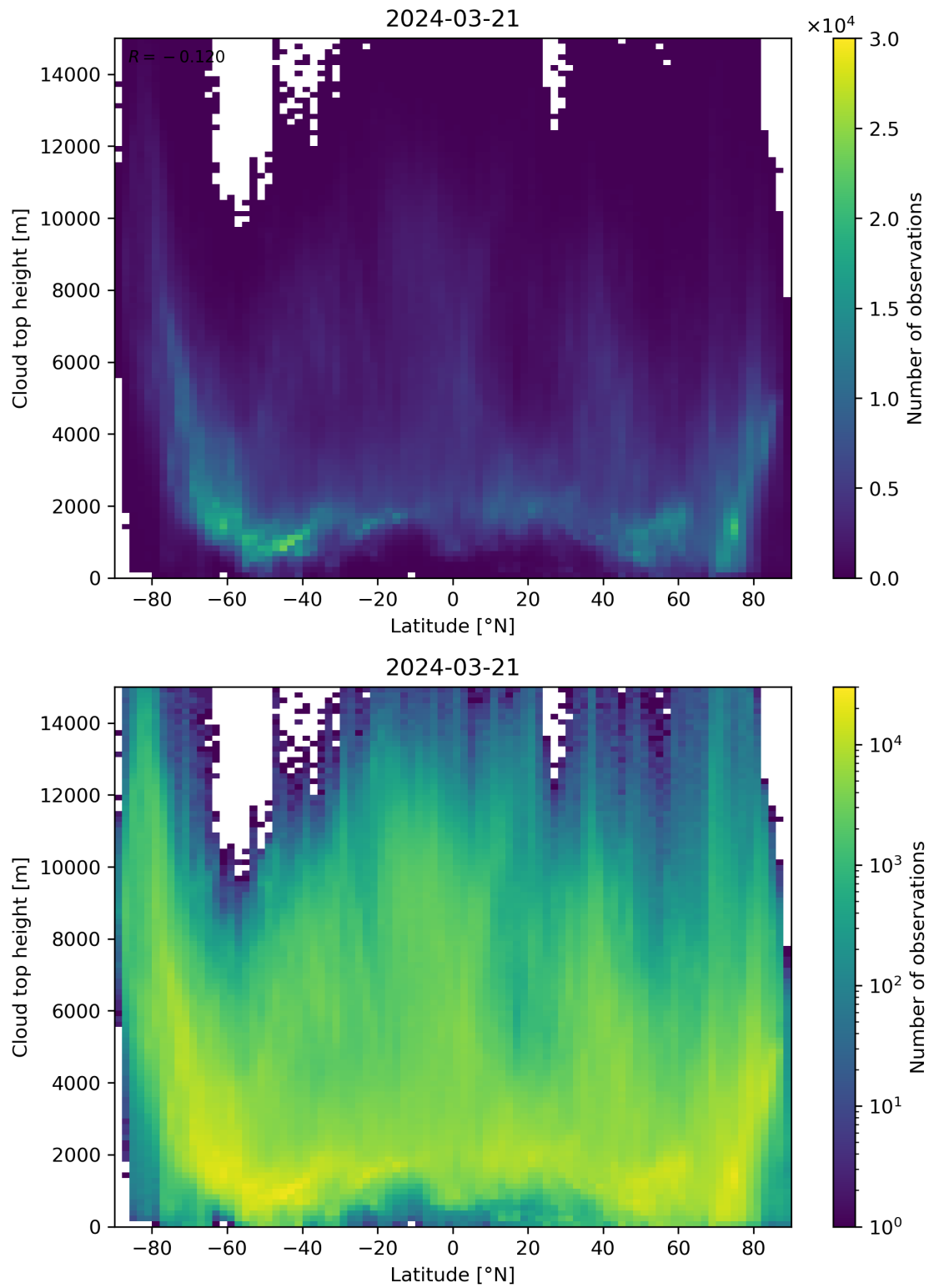
Figure 97: Scatter density plot of “Latitude” against “Cloud top height” for 2024-03-20 to 2024-03-22.
