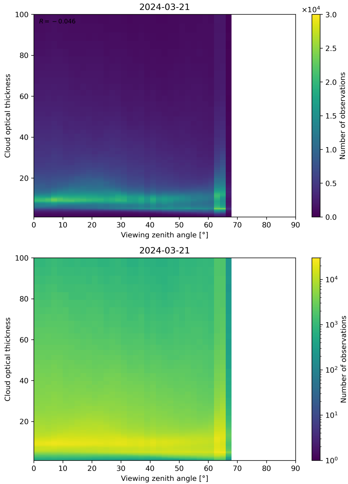
Figure 111: Scatter density plot of “Viewing zenith angle” against “Cloud optical thickness” for 2024-03-20 to 2024-03-22.
