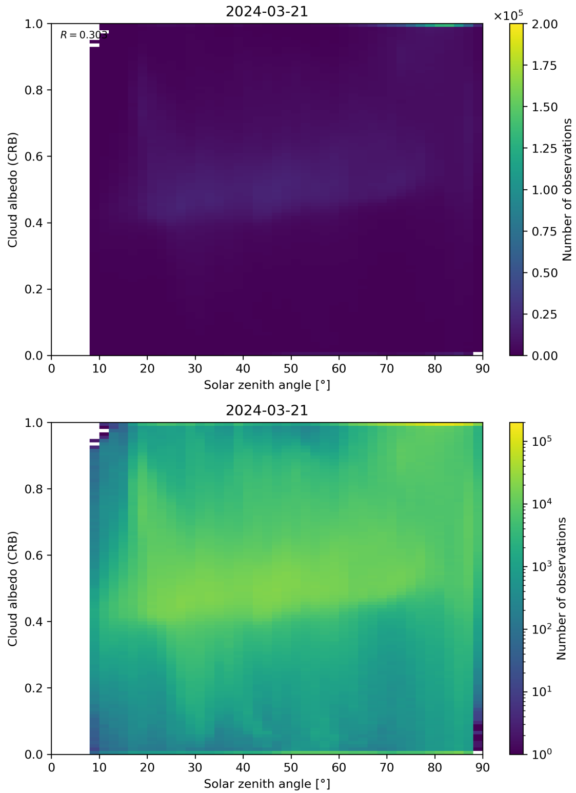
Figure 98: Scatter density plot of “Solar zenith angle” against “Cloud albedo (CRB)” for 2024-03-20 to 2024-03-22.
