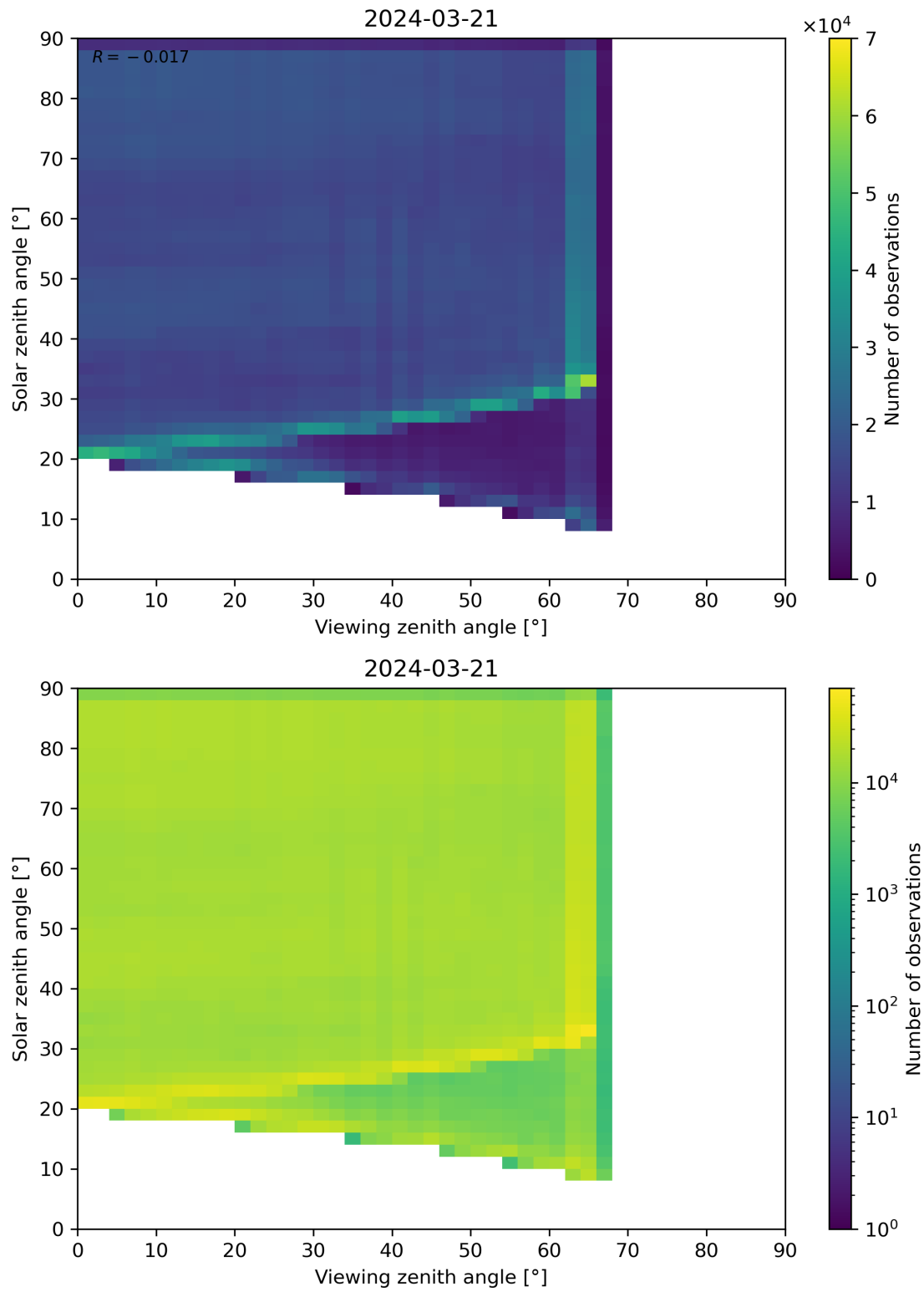
Figure 114: Scatter density plot of “Viewing zenith angle” against “Solar zenith angle” for 2024-03-20 to 2024-03-22.
