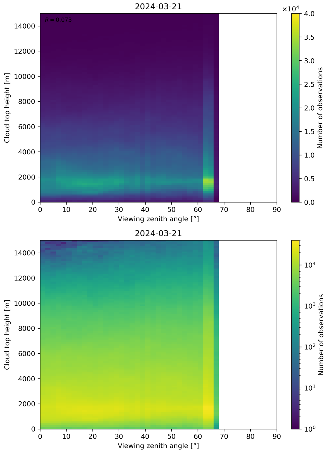
Figure 112: Scatter density plot of “Viewing zenith angle” against “Cloud top height” for 2024-03-20 to 2024-03-22.
