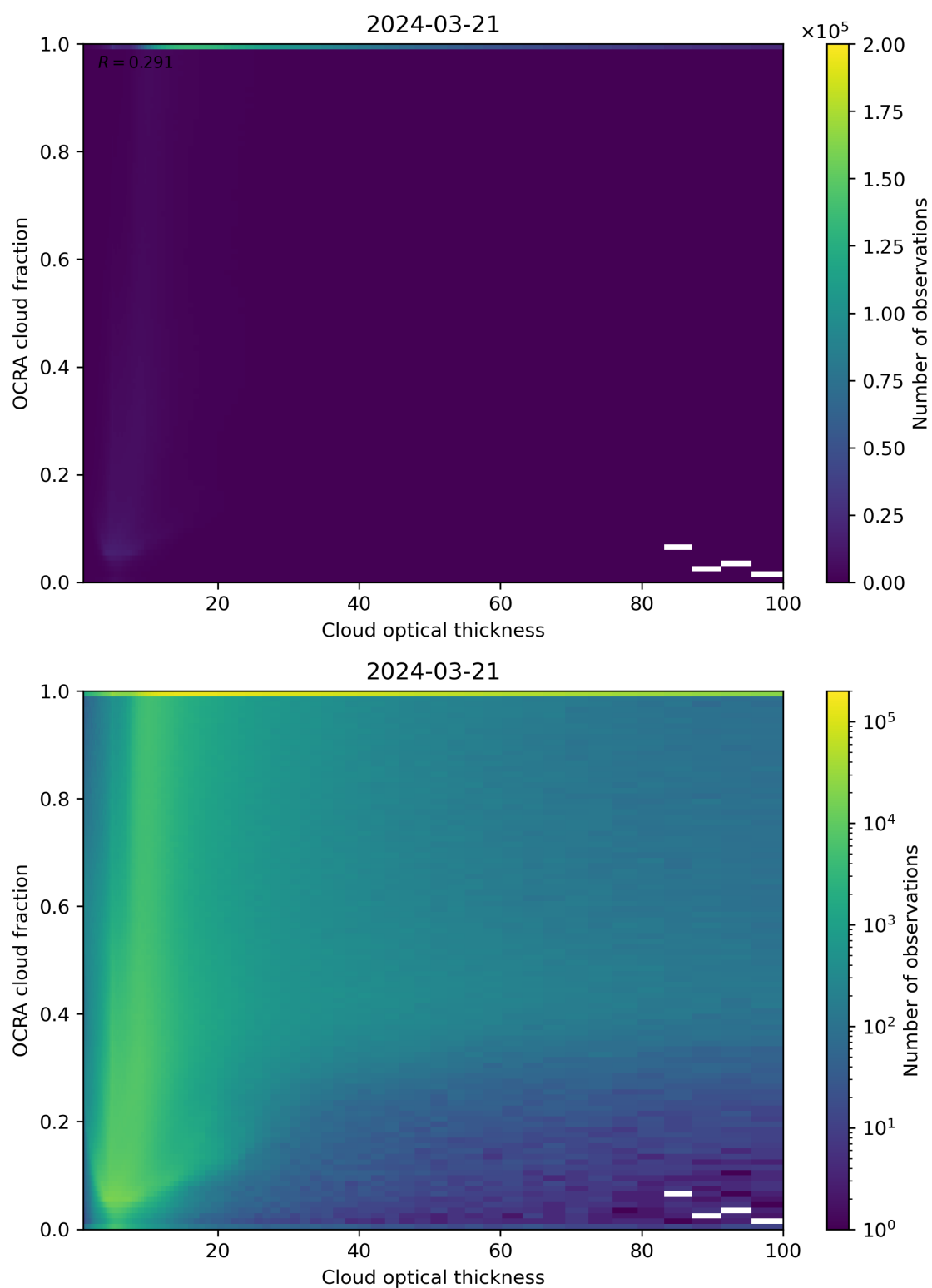
Figure 83: Scatter density plot of “Cloud optical thickness” against “OCRA cloud fraction” for 2024-03-20 to 2024-03-22.
