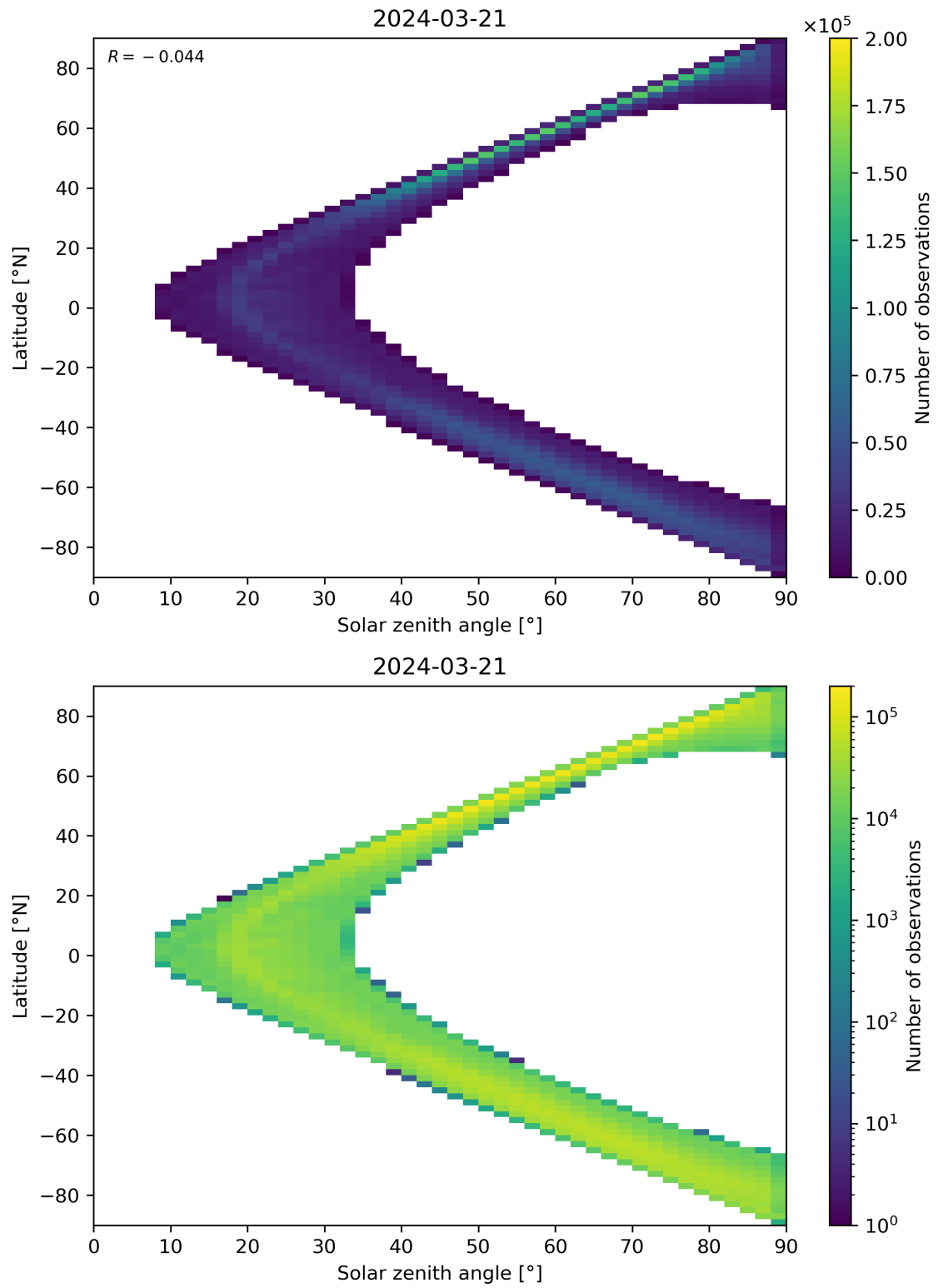
Figure 105: Scatter density plot of “Solar zenith angle” against “Latitude” for 2024-03-20 to 2024-03-22.
