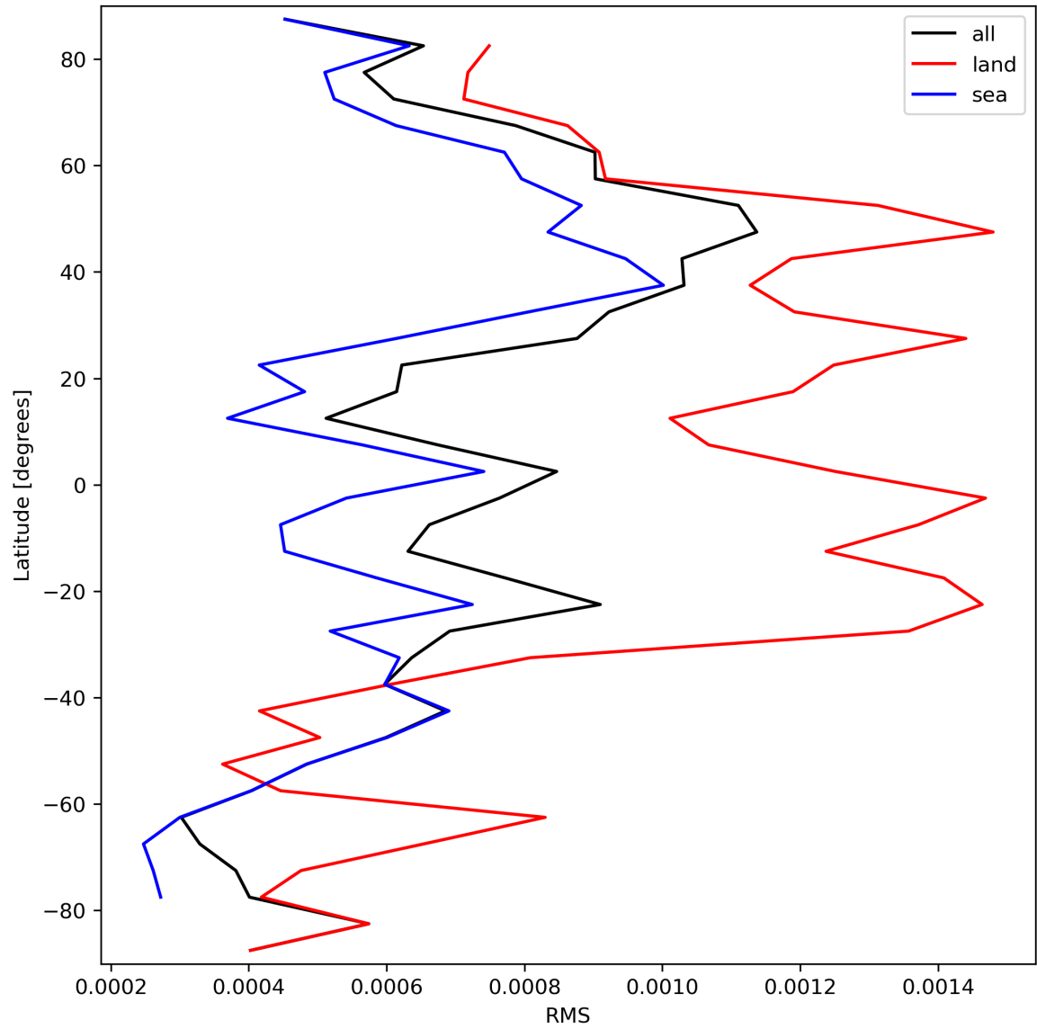
Figure 31: Zonal average of “RMS” for 2024-03-20 to 2024-03-22.
