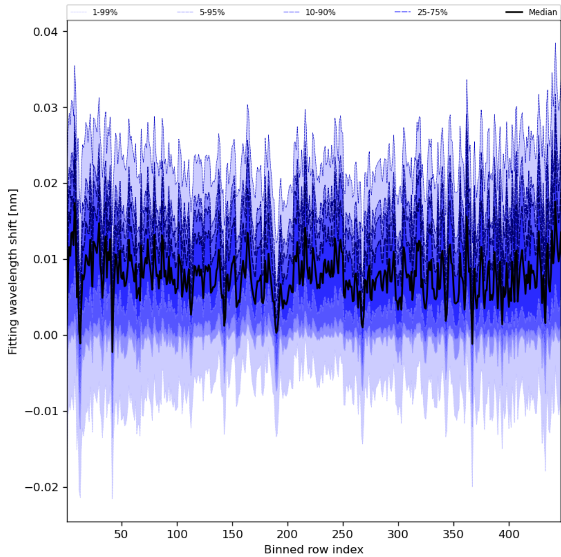
Figure 65: Along track statistics of “Fitting wavelength shift” for 2024-03-20 to 2024-03-22
