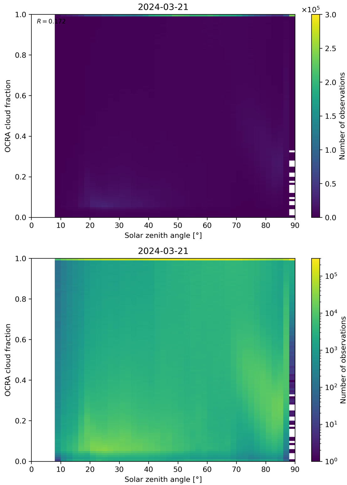
Figure 100: Scatter density plot of “Solar zenith angle” against “OCRA cloud fraction” for 2024-03-20 to 2024-03-22.
