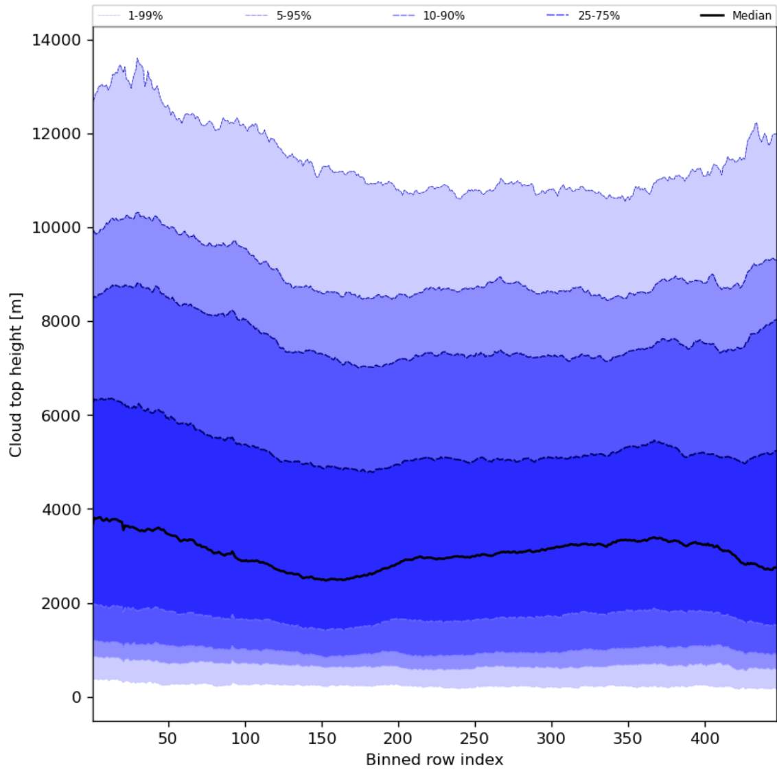
Figure 56: Along track statistics of “Cloud top height” for 2024-03-20 to 2024-03-22
