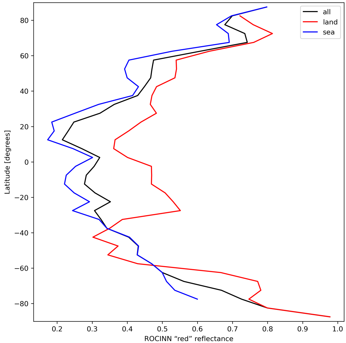
Figure 37: Zonal average of “ROCINN “red” reflectance” for 2024-03-20 to 2024-03-22.
