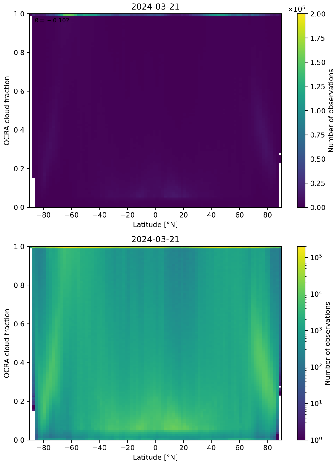
Figure 93: Scatter density plot of “Latitude” against “OCRA cloud fraction” for 2024-03-20 to 2024-03-22.
