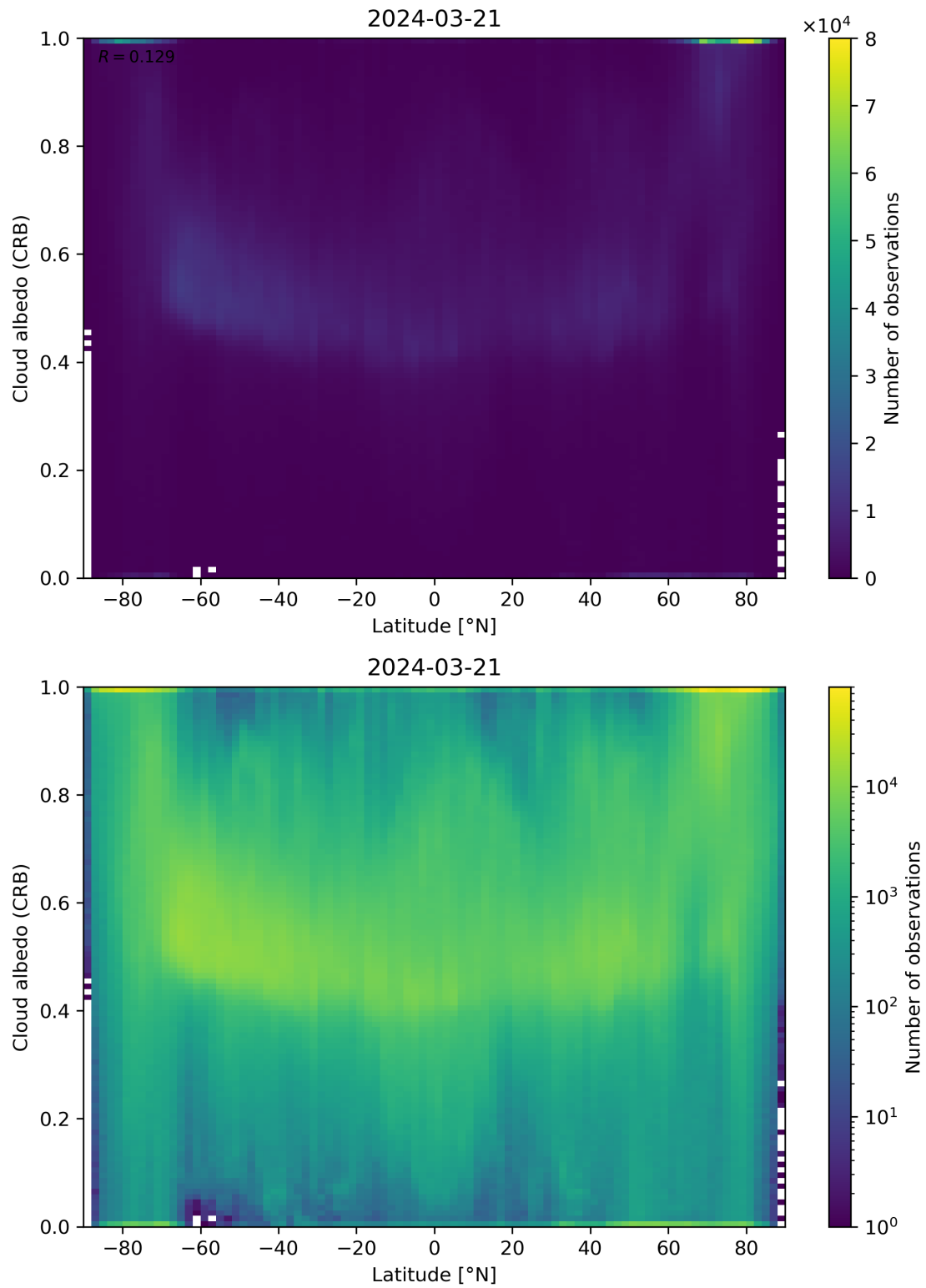
Figure 91: Scatter density plot of “Latitude” against “Cloud albedo (CRB)” for 2024-03-20 to 2024-03-22.
