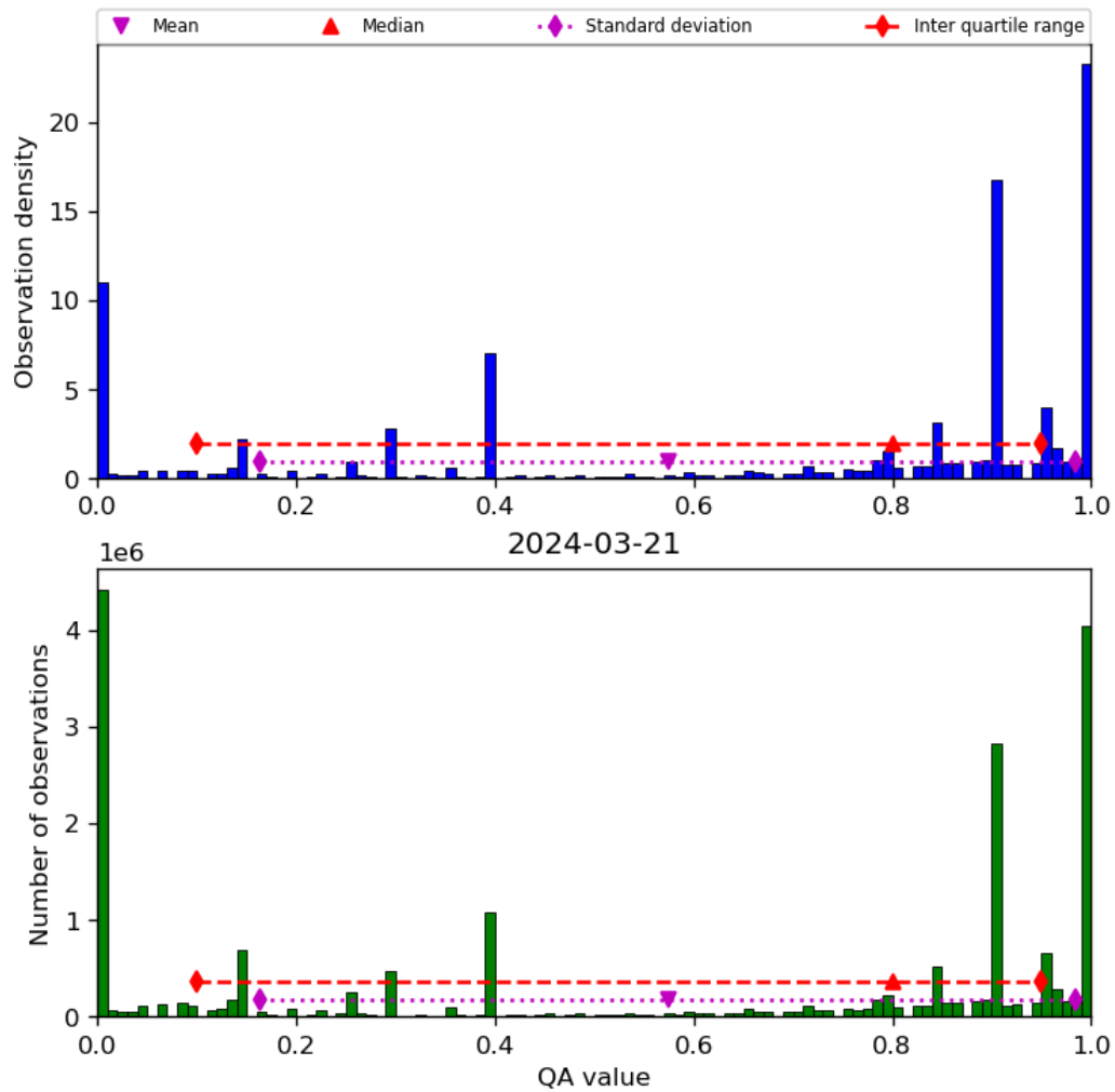
Figure 38: Histogram of “QA value” for 2024-03-20 to 2024-03-22
