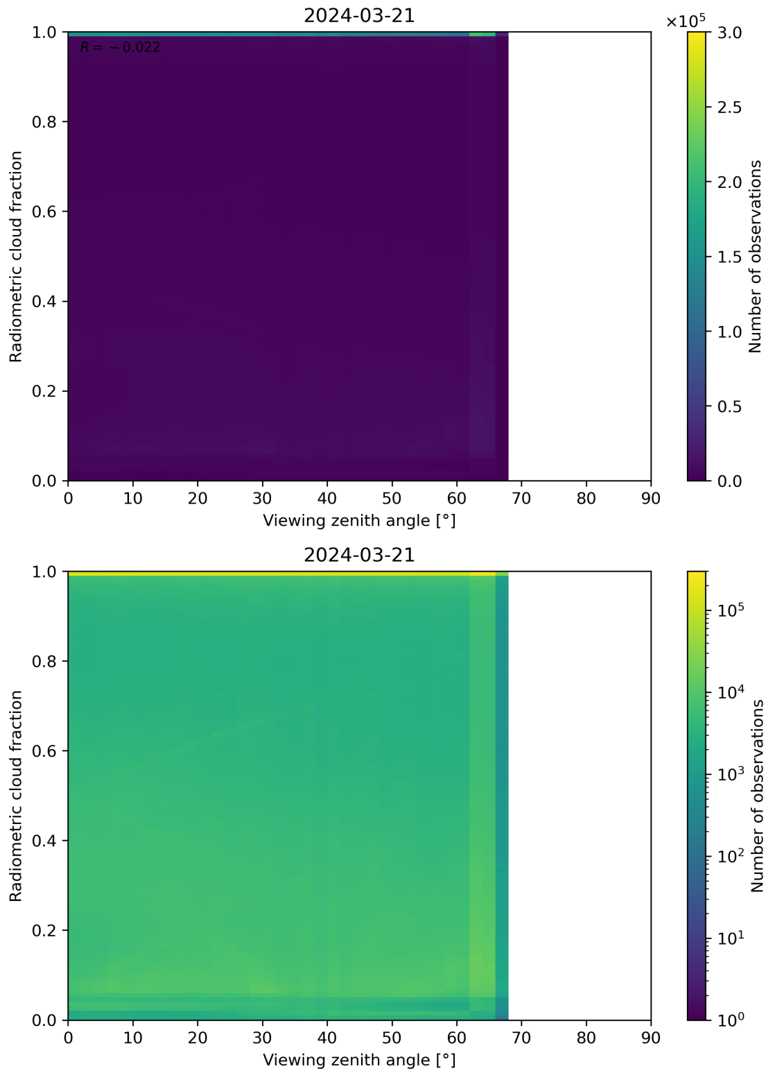
Figure 107: Scatter density plot of “Viewing zenith angle” against “Radiometric cloud fraction” for 2024-03-20 to 2024-03-22.
