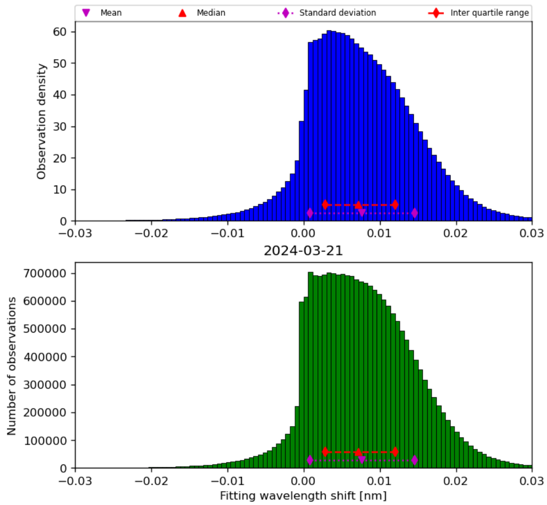
Figure 49: Histogram of “Fitting wavelength shift” for 2024-03-20 to 2024-03-22
