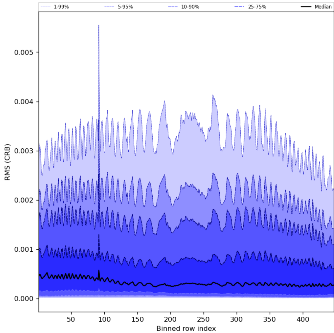
Figure 64: Along track statistics of “RMS (CRB)” for 2024-03-20 to 2024-03-22
