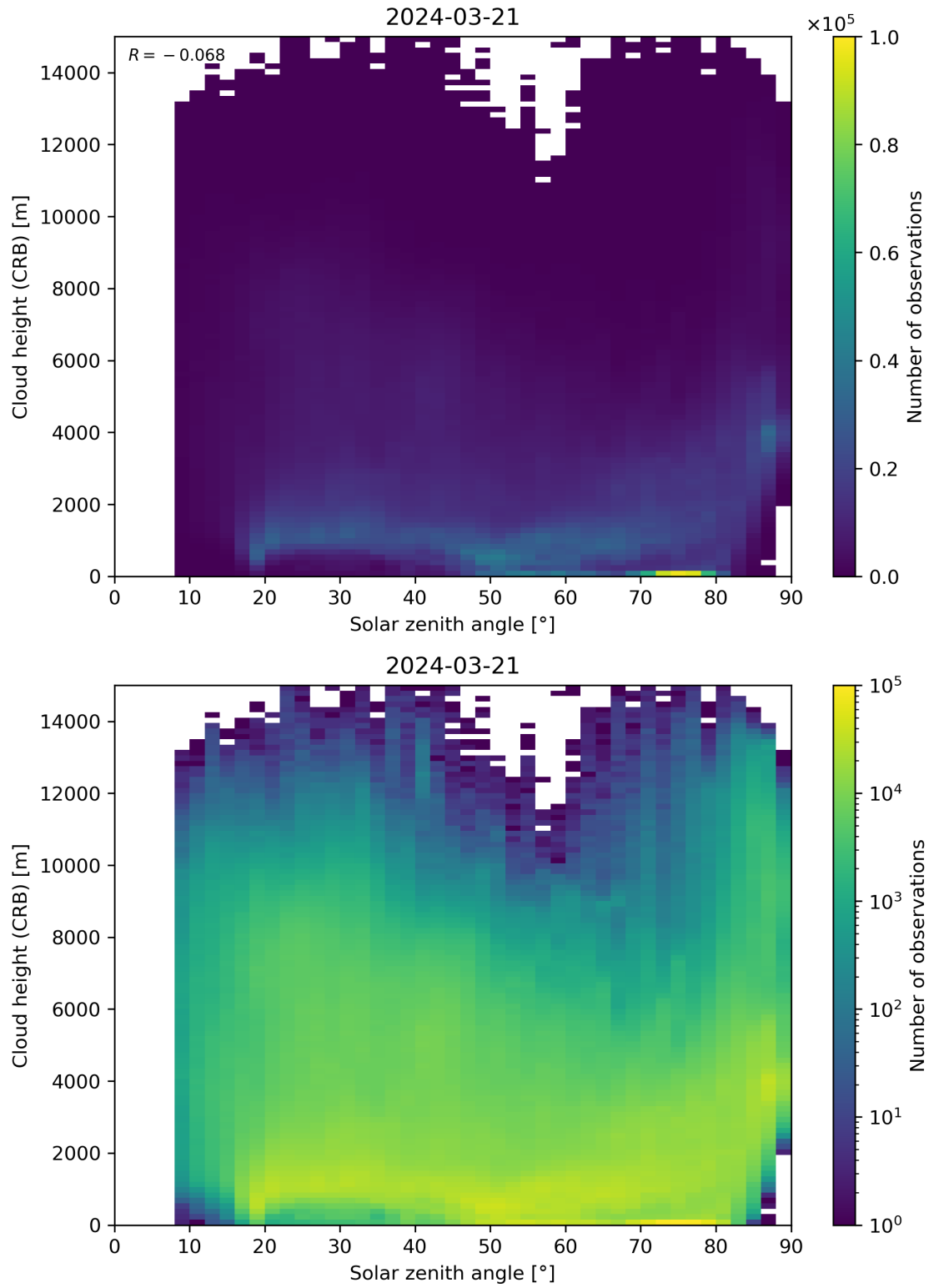
Figure 102: Scatter density plot of “Solar zenith angle” against “Cloud height (CRB)” for 2024-03-20 to 2024-03-22.
