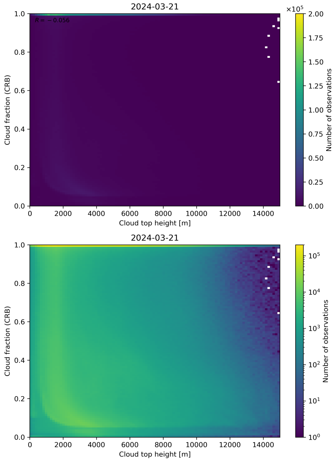
Figure 88: Scatter density plot of “Cloud top height” against “Cloud fraction (CRB)” for 2024-03-20 to 2024-03-22.
