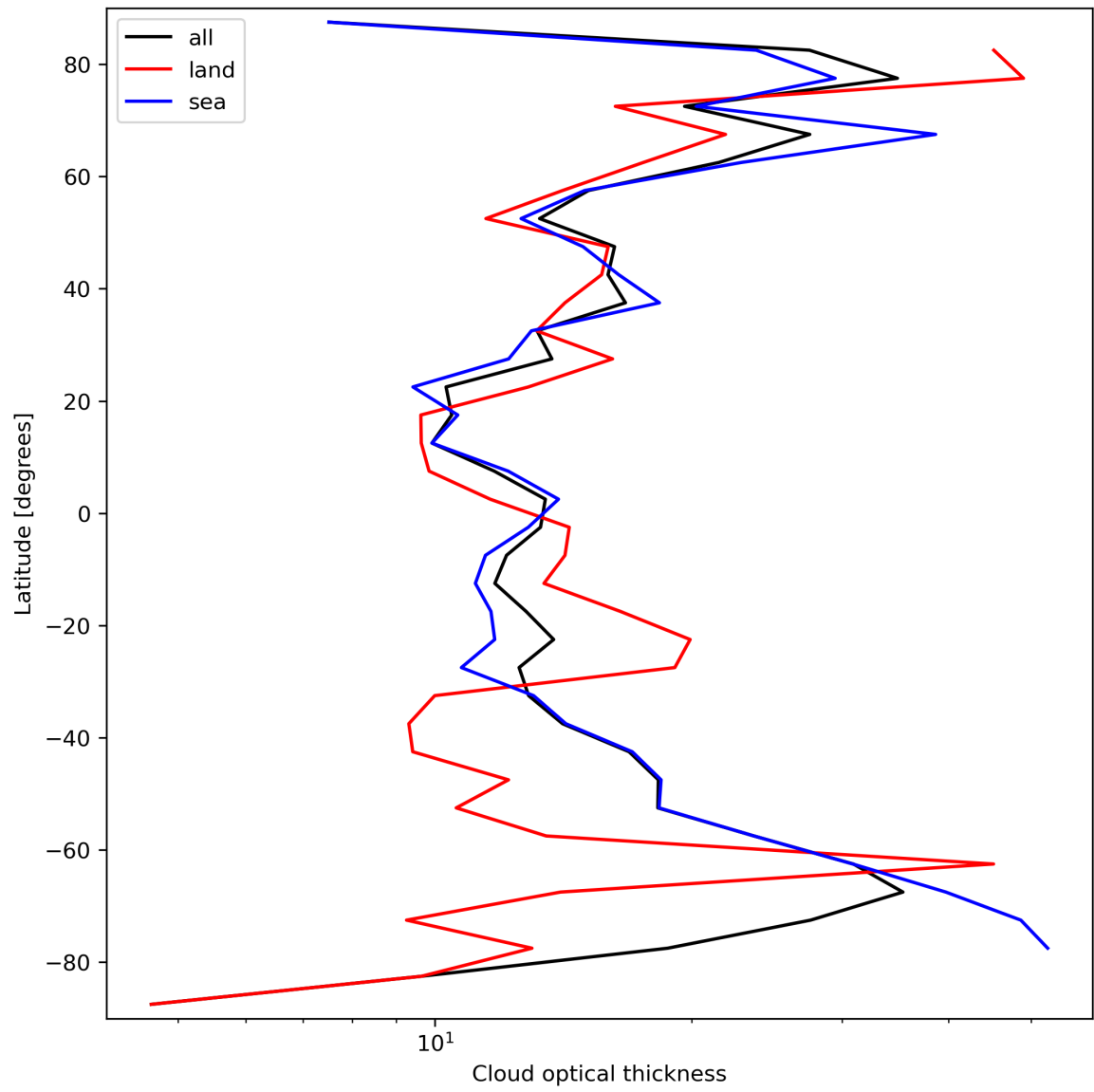
Figure 25: Zonal average of “Cloud optical thickness” for 2024-03-20 to 2024-03-22.
