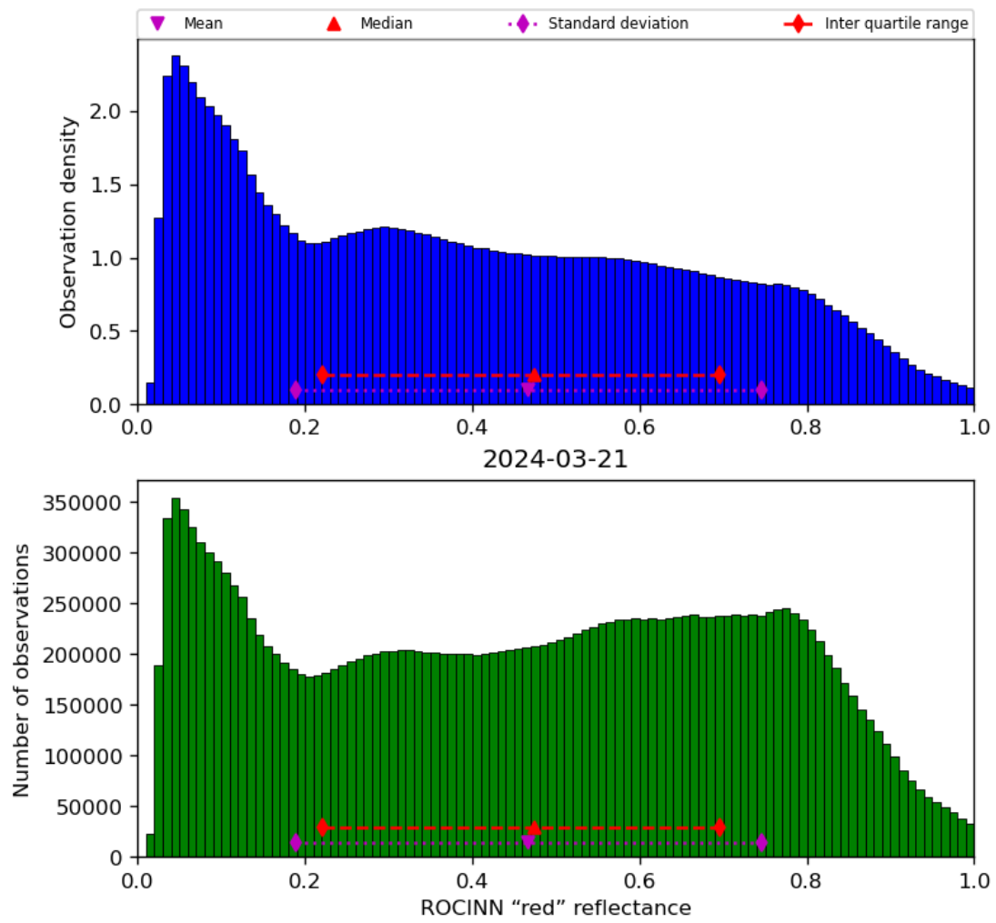
Figure 53: Histogram of “ROCINN “red” reflectance” for 2024-03-20 to 2024-03-22
