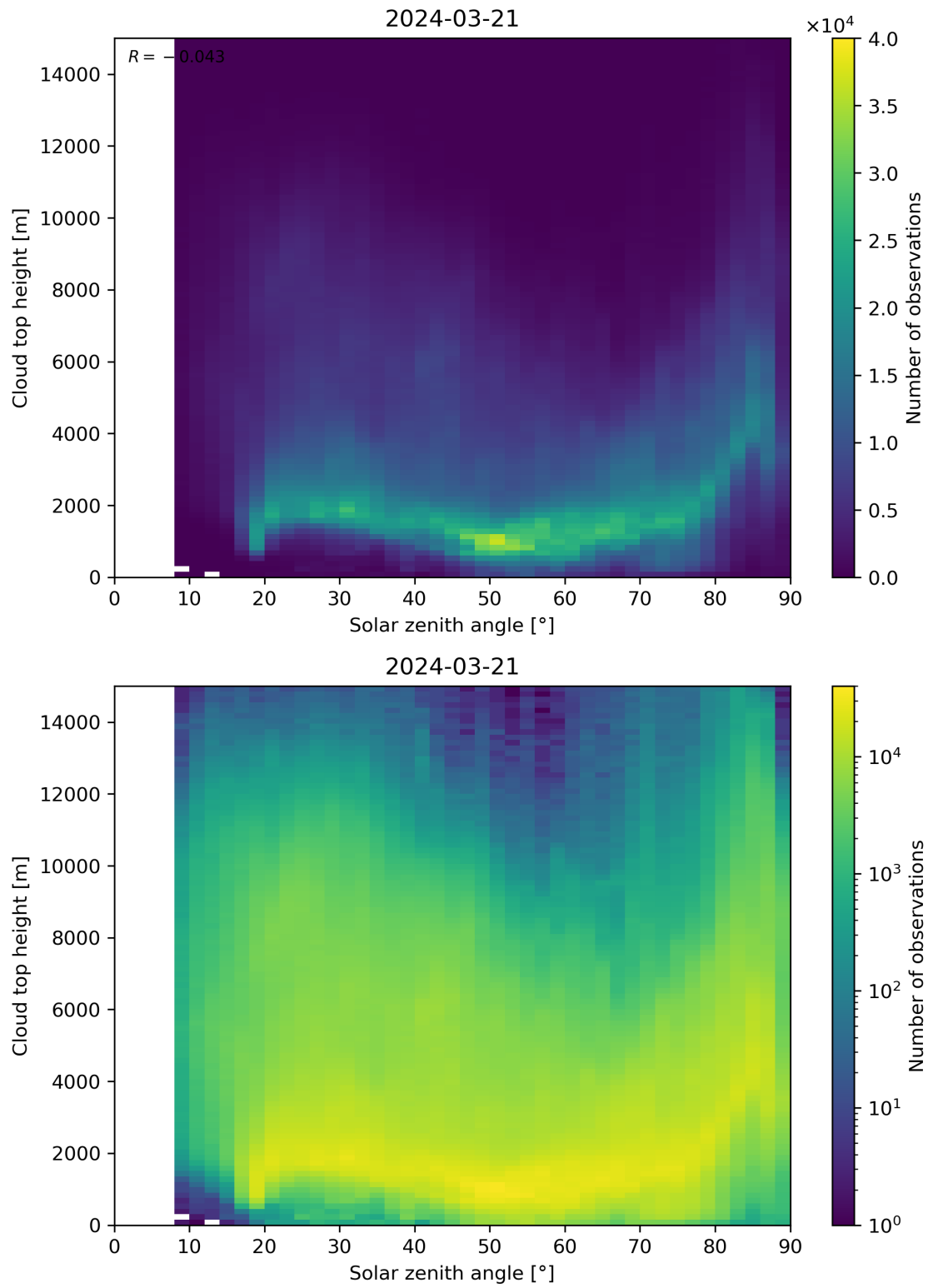
Figure 104: Scatter density plot of “Solar zenith angle” against “Cloud top height” for 2024-03-20 to 2024-03-22.
