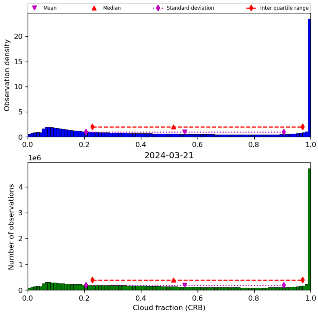
Figure 42: Histogram of “Cloud fraction (CRB)” for 2024-03-20 to 2024-03-22
