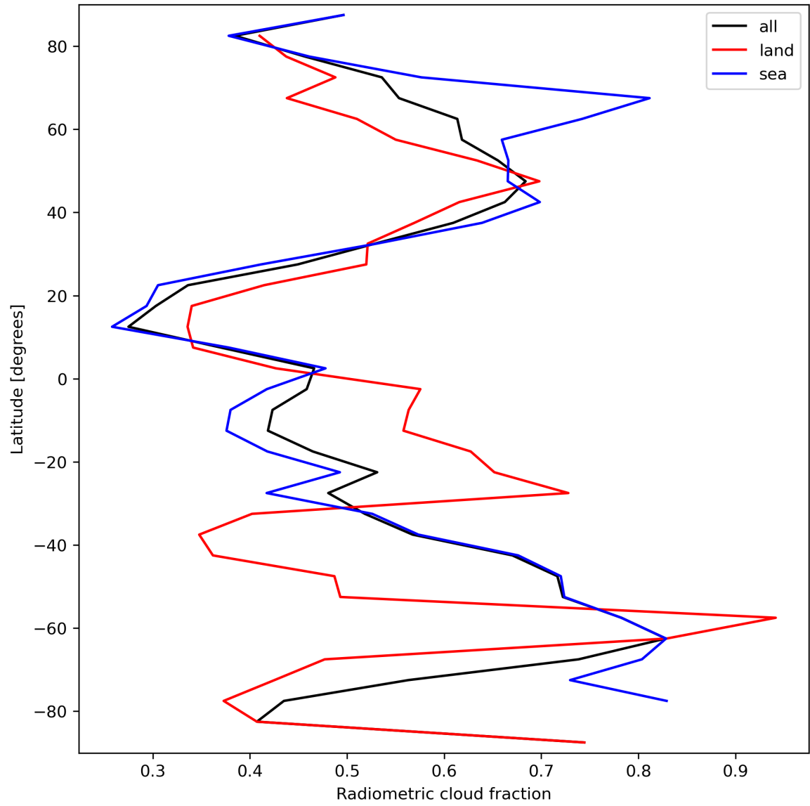
Figure 23: Zonal average of “Radiometric cloud fraction” for 2024-03-20 to 2024-03-22.
