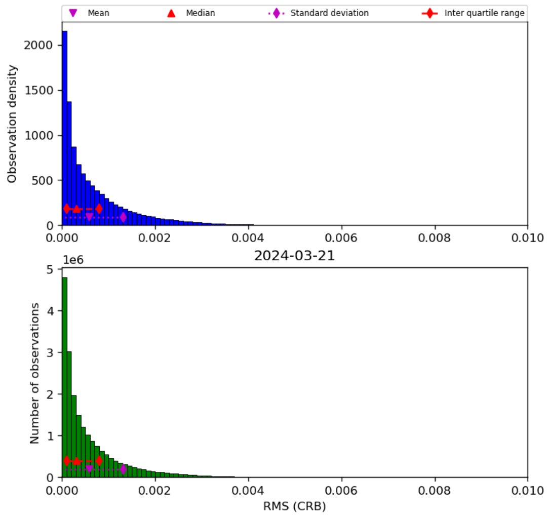
Figure 48: Histogram of “RMS (CRB)” for 2024-03-20 to 2024-03-22
