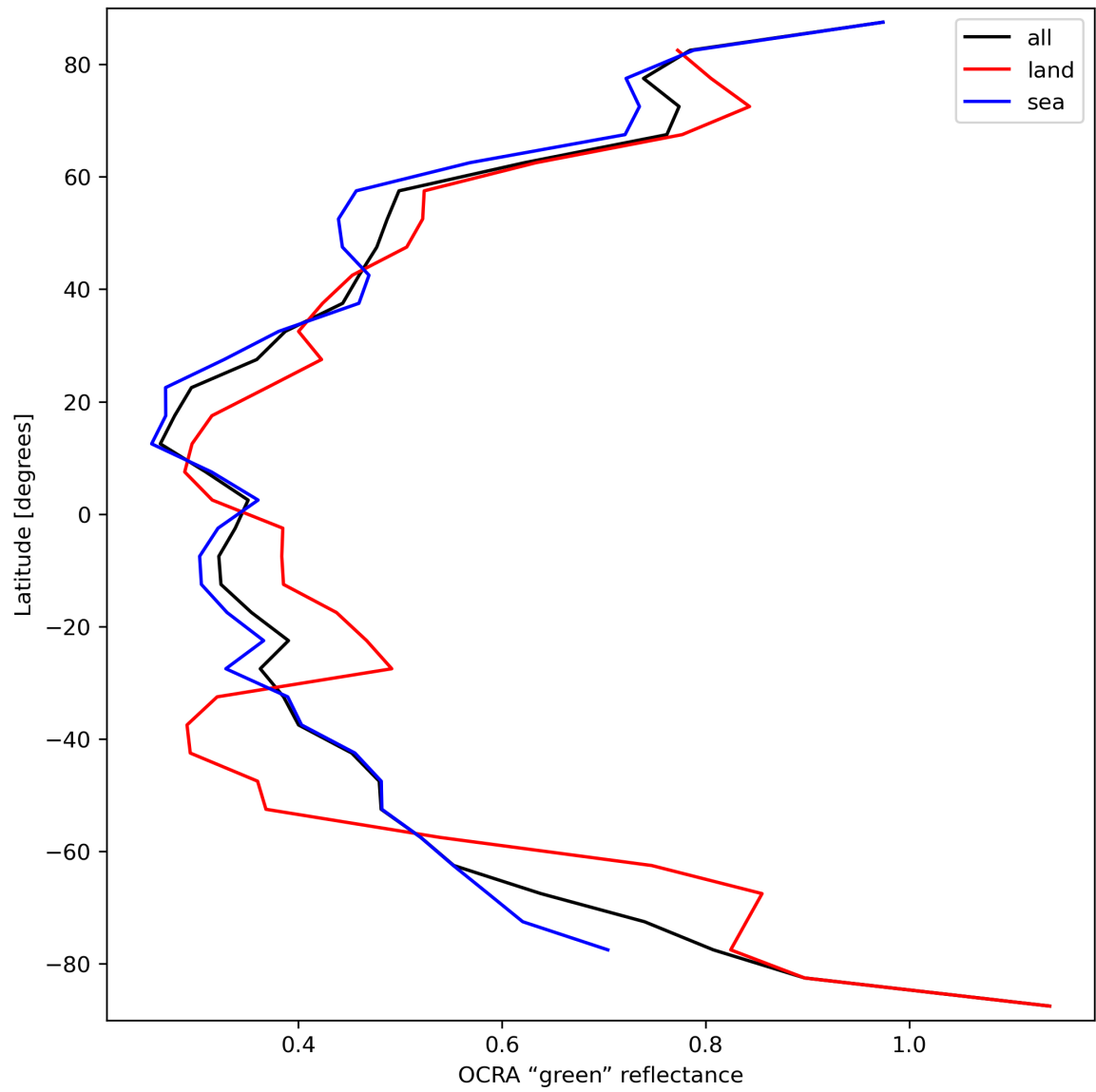
Figure 36: Zonal average of “OCRA “green” reflectance” for 2024-03-20 to 2024-03-22.
