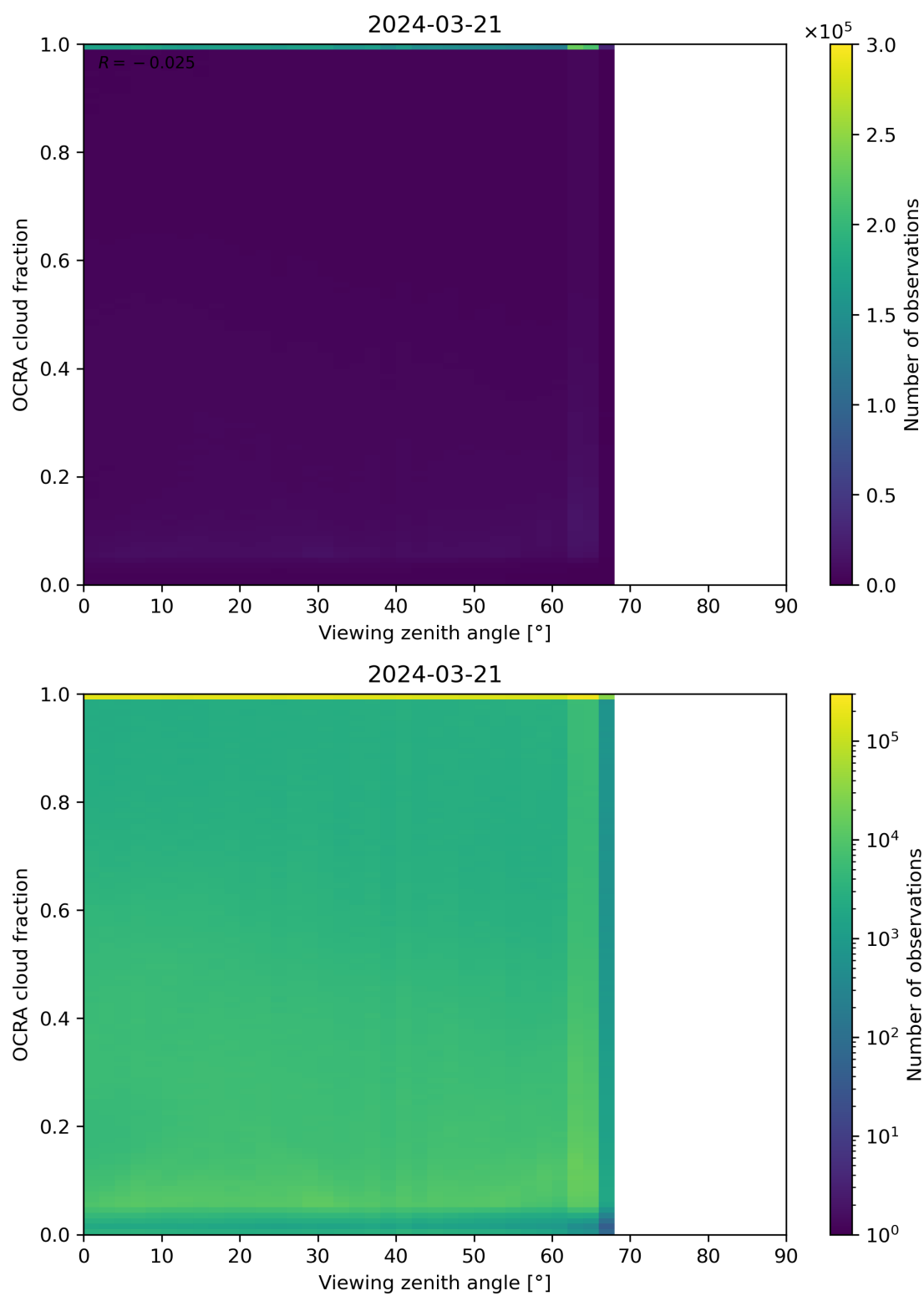
Figure 108: Scatter density plot of “Viewing zenith angle” against “OCRA cloud fraction” for 2024-03-20 to 2024-03-22.
