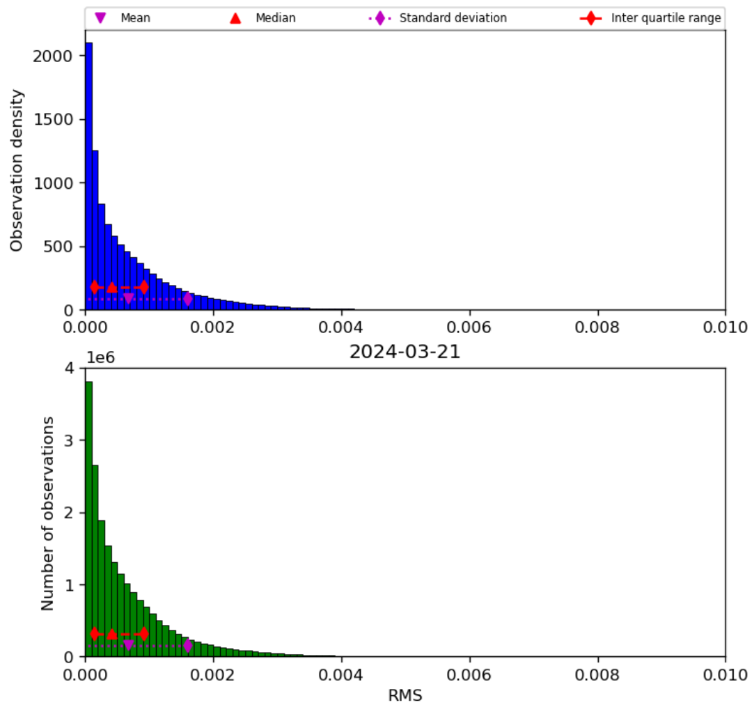
Figure 47: Histogram of “RMS” for 2024-03-20 to 2024-03-22
