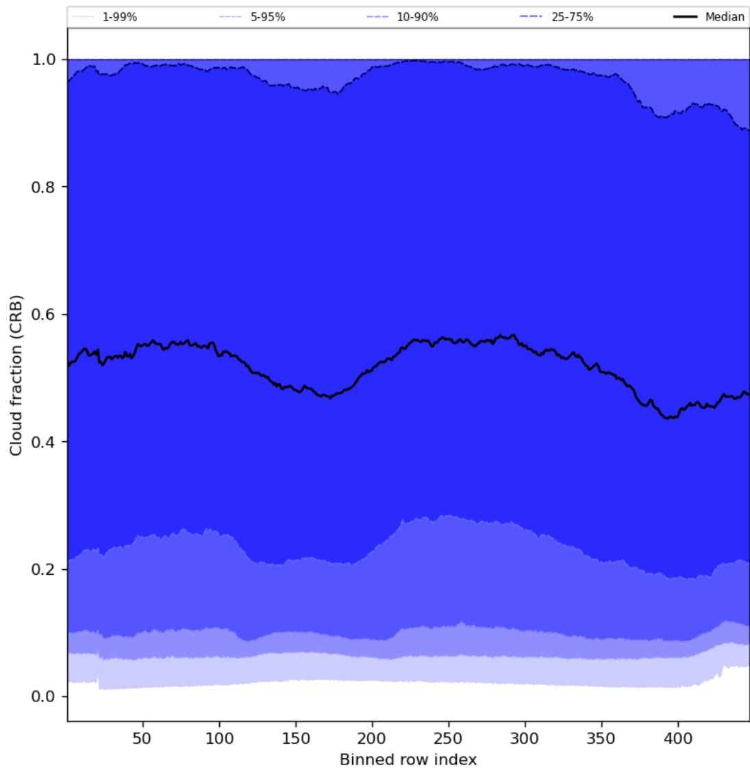
Figure 58: Along track statistics of “Cloud fraction (CRB)” for 2024-03-20 to 2024-03-22
