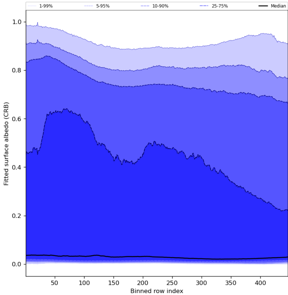
Figure 62: Along track statistics of “Fitted surface albedo (CRB)” for 2024-03-20 to 2024-03-22
