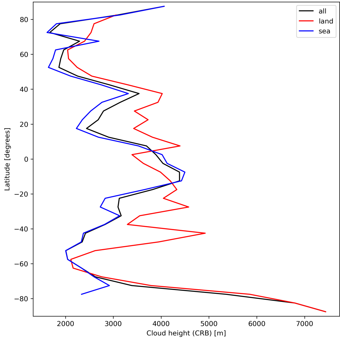
Figure 27: Zonal average of “Cloud height (CRB)” for 2024-03-20 to 2024-03-22.
