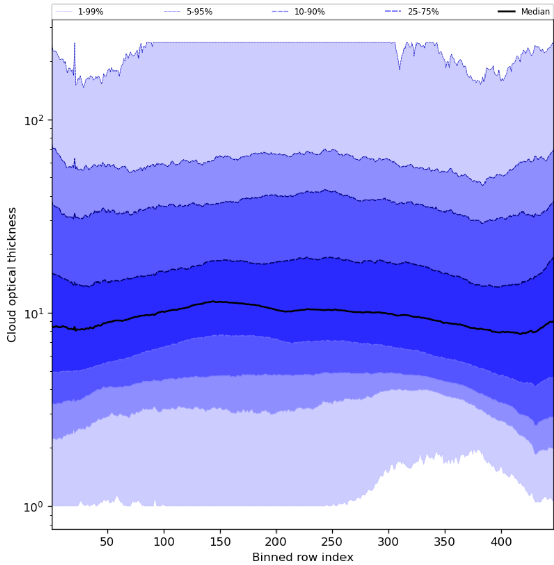
Figure 57: Along track statistics of “Cloud optical thickness” for 2024-03-20 to 2024-03-22
