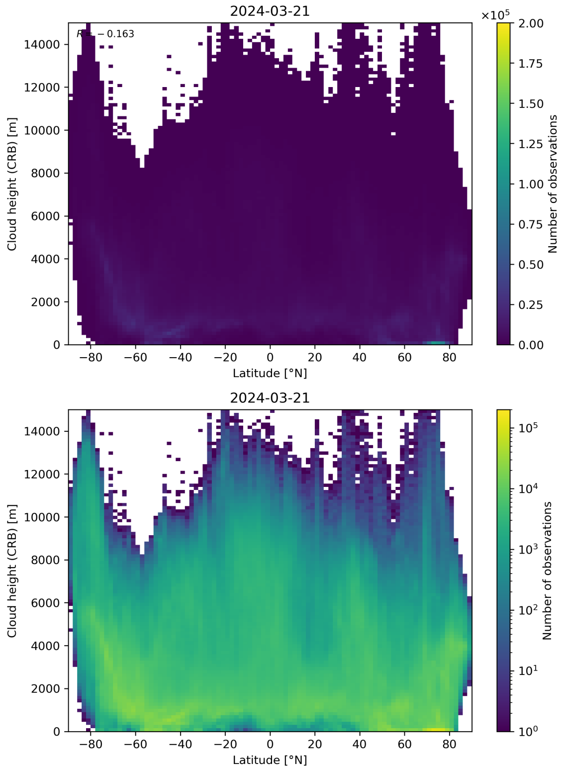
Figure 95: Scatter density plot of “Latitude” against “Cloud height (CRB)” for 2024-03-20 to 2024-03-22.
