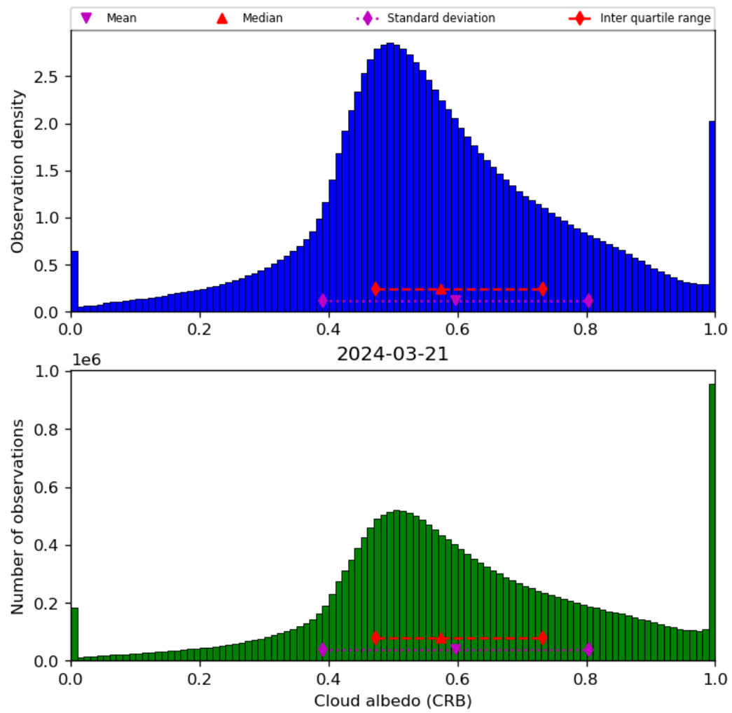
Figure 44: Histogram of “Cloud albedo (CRB)” for 2024-03-20 to 2024-03-22
