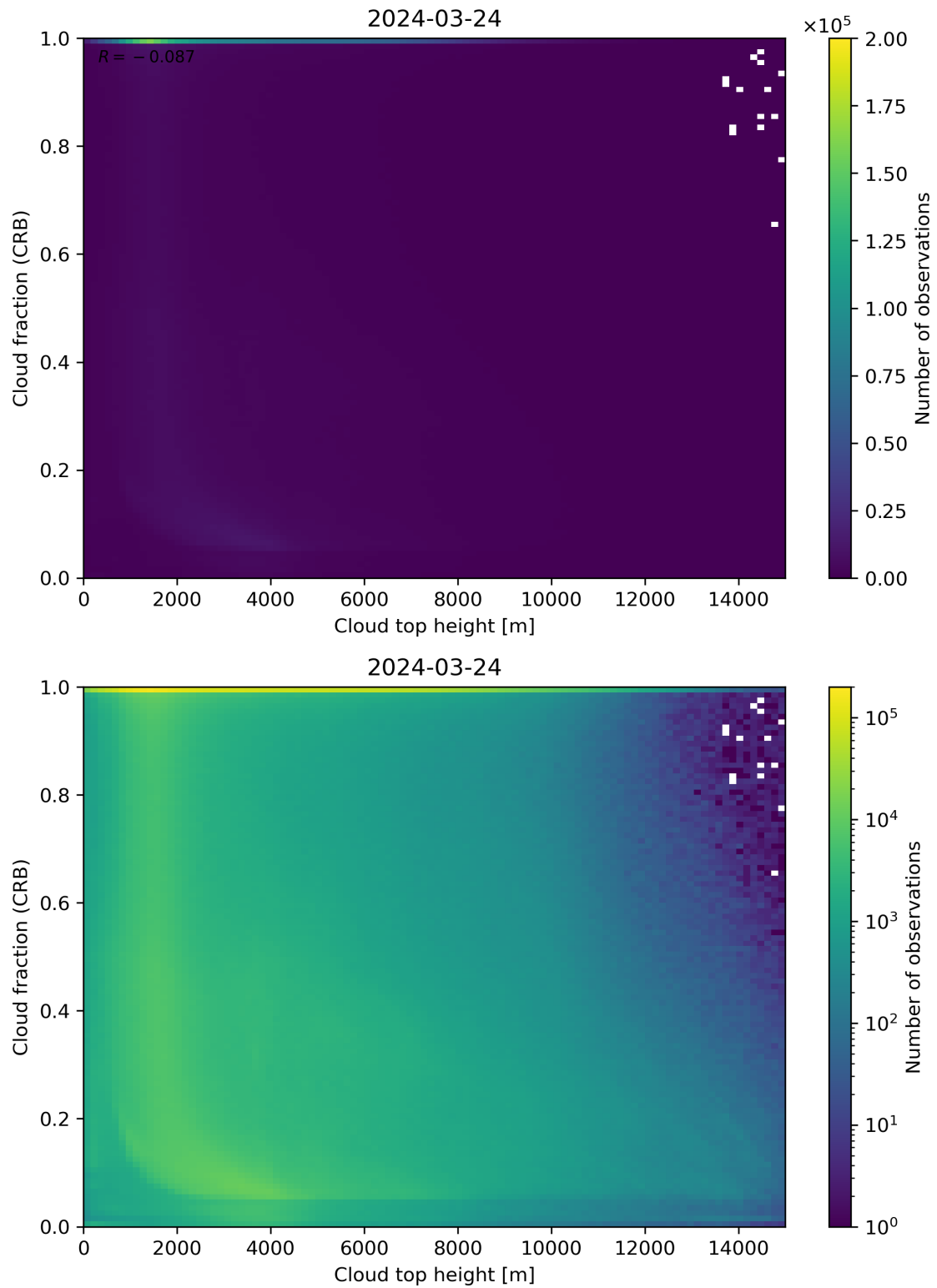
Figure 88: Scatter density plot of “Cloud top height” against “Cloud fraction (CRB)” for 2024-03-23 to 2024-03-25.
