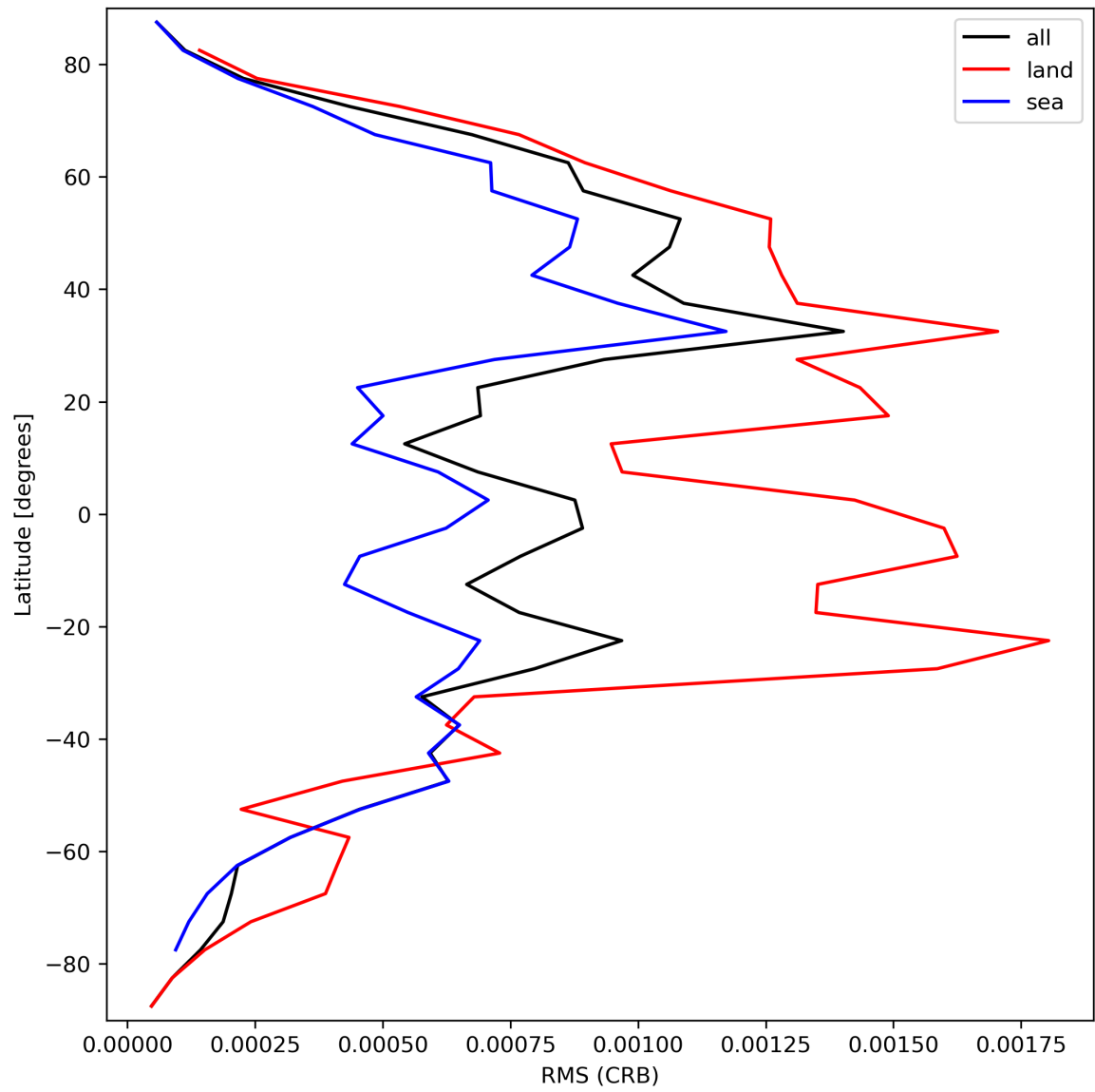
Figure 32: Zonal average of “RMS (CRB)” for 2024-03-23 to 2024-03-25.
