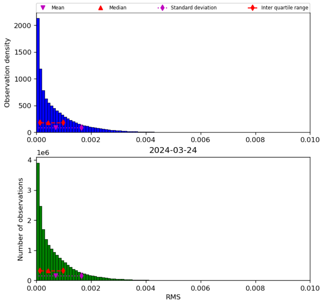
Figure 47: Histogram of “RMS” for 2024-03-23 to 2024-03-25
