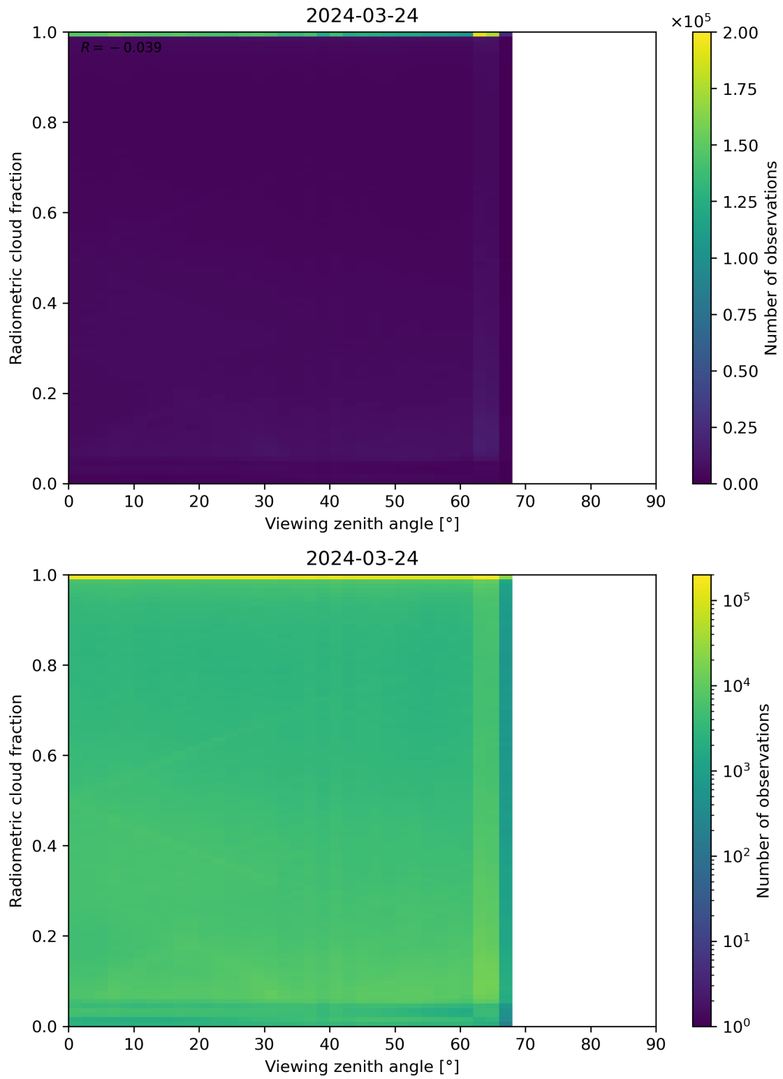
Figure 107: Scatter density plot of “Viewing zenith angle” against “Radiometric cloud fraction” for 2024-03-23 to 2024-03-25.
