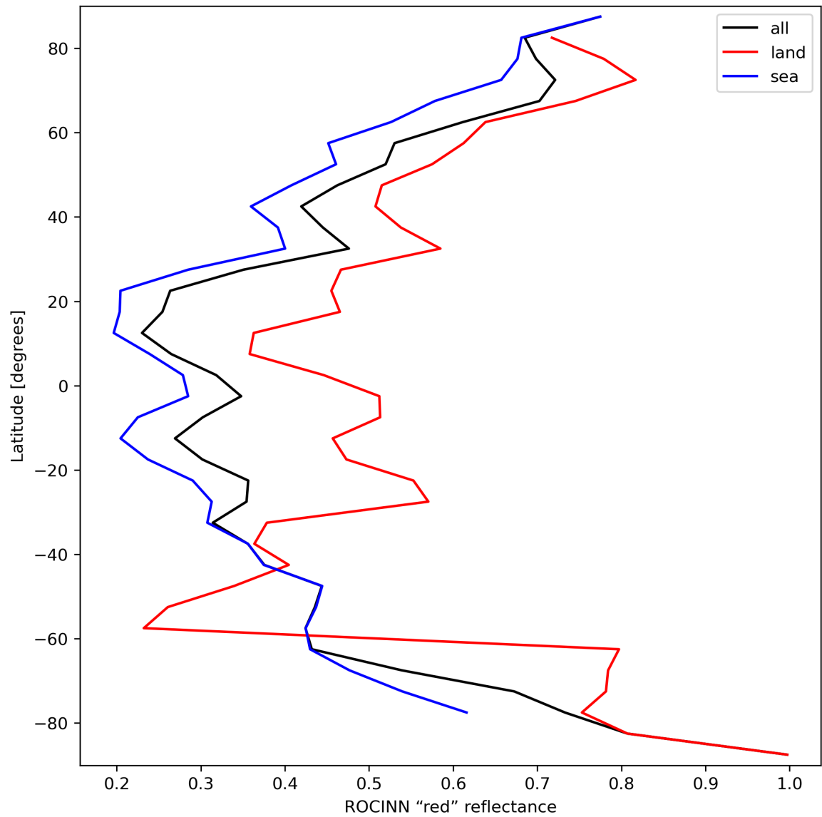
Figure 37: Zonal average of “ROCINN “red” reflectance” for 2024-03-23 to 2024-03-25.
