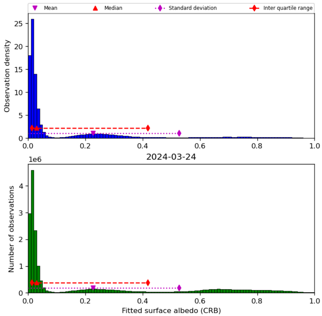
Figure 46: Histogram of “Fitted surface albedo (CRB)” for 2024-03-23 to 2024-03-25
