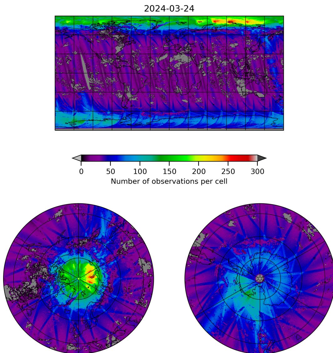
Figure 21: Map of the number of observations for 2024-03-23 to 2024-03-25
