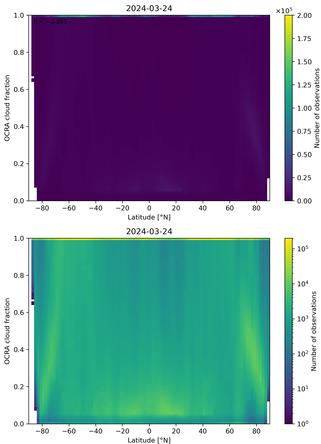
Figure 93: Scatter density plot of “Latitude” against “OCRA cloud fraction” for 2024-03-23 to 2024-03-25.
