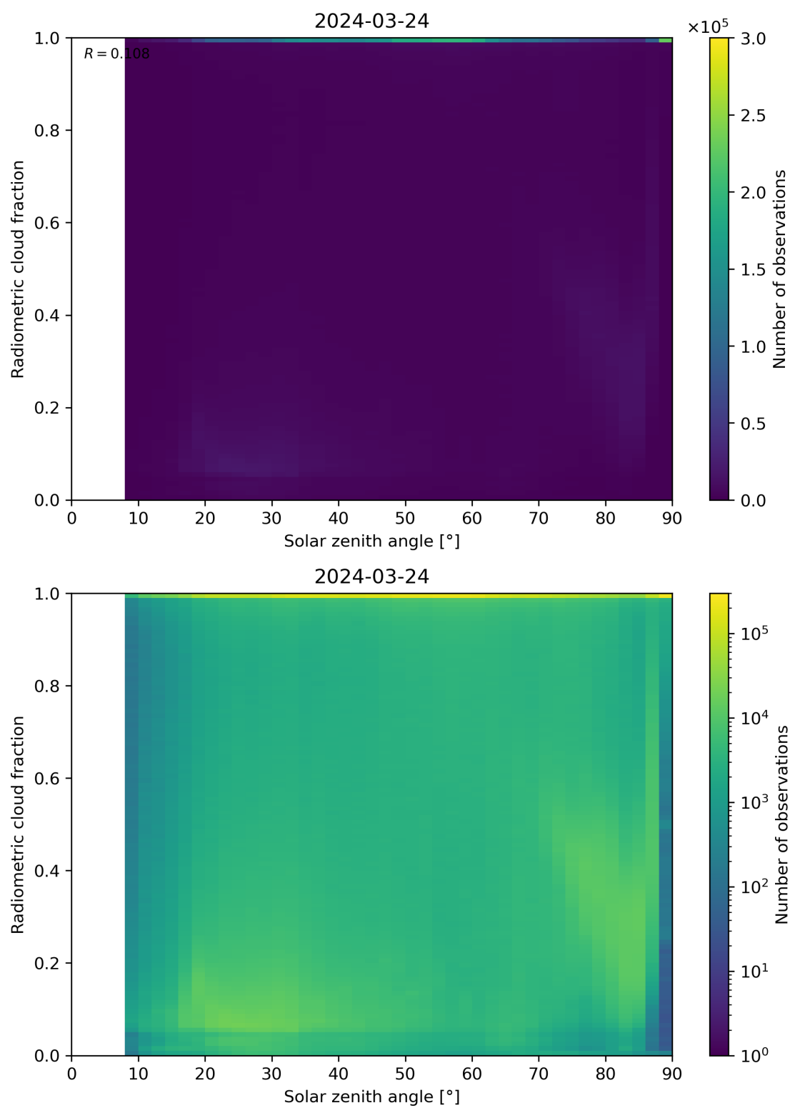
Figure 99: Scatter density plot of “Solar zenith angle” against “Radiometric cloud fraction” for 2024-03-23 to 2024-03-25.
