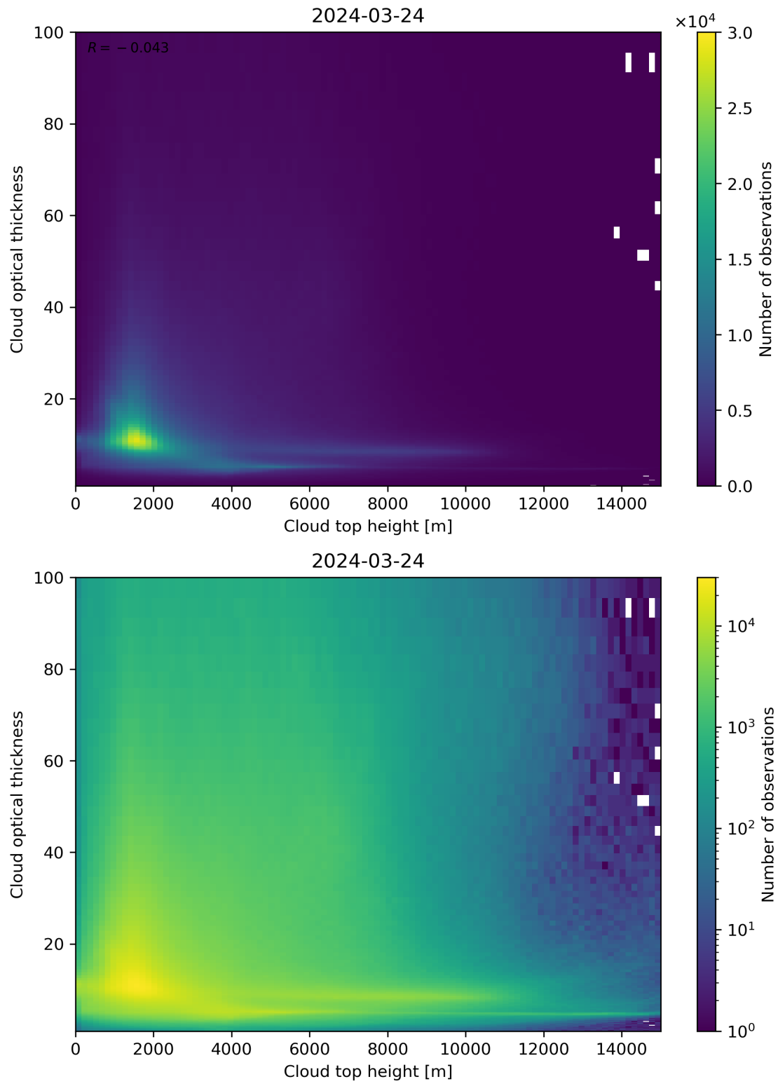
Figure 90: Scatter density plot of “Cloud top height” against “Cloud optical thickness” for 2024-03-23 to 2024-03-25.
