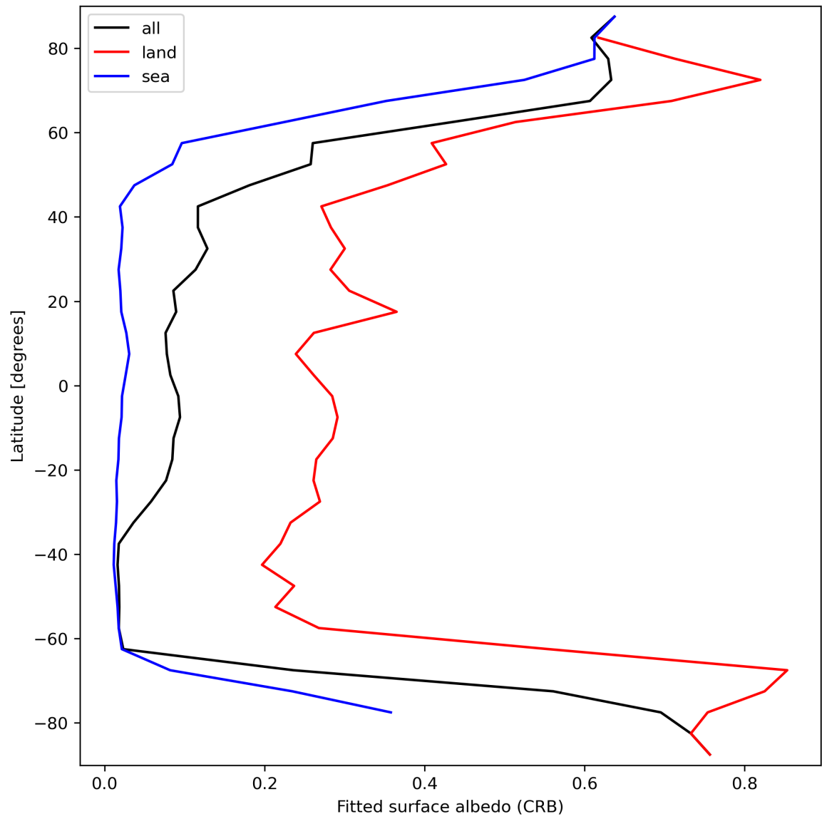
Figure 30: Zonal average of “Fitted surface albedo (CRB)” for 2024-03-23 to 2024-03-25.
