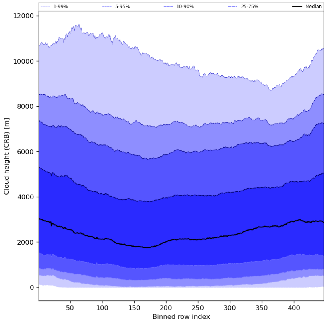
Figure 59: Along track statistics of “Cloud height (CRB)” for 2024-03-23 to 2024-03-25
