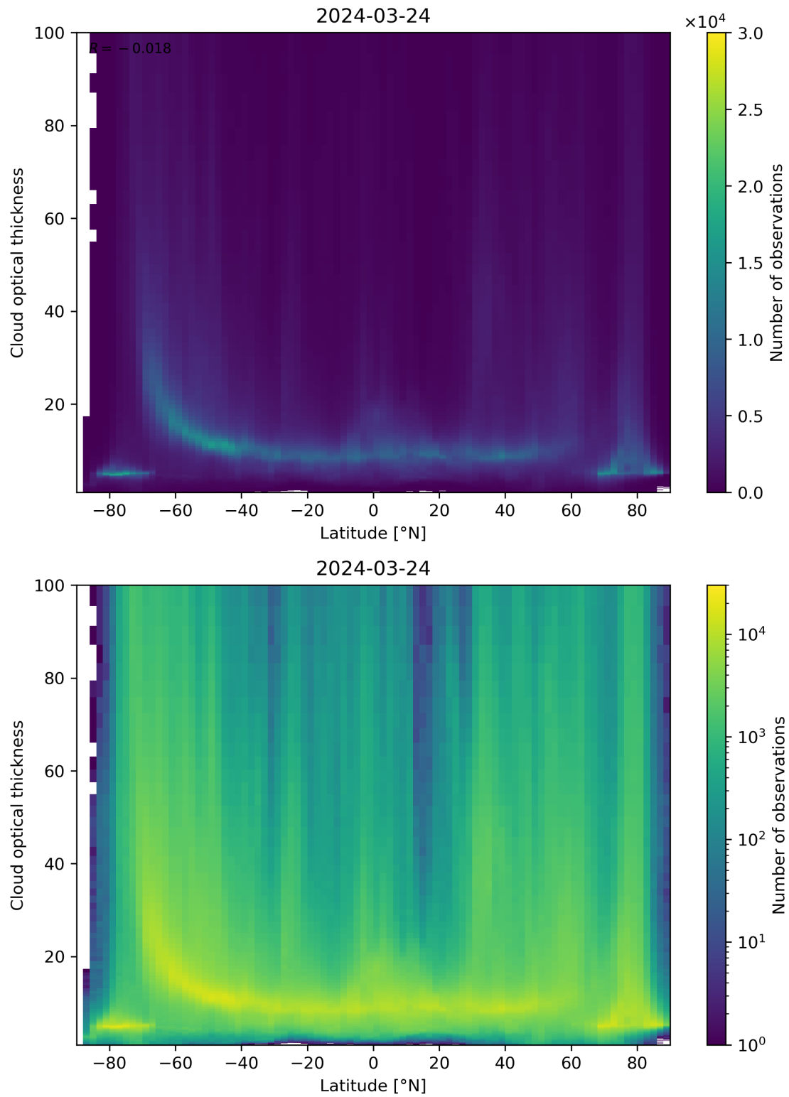
Figure 96: Scatter density plot of “Latitude” against “Cloud optical thickness” for 2024-03-23 to 2024-03-25.
