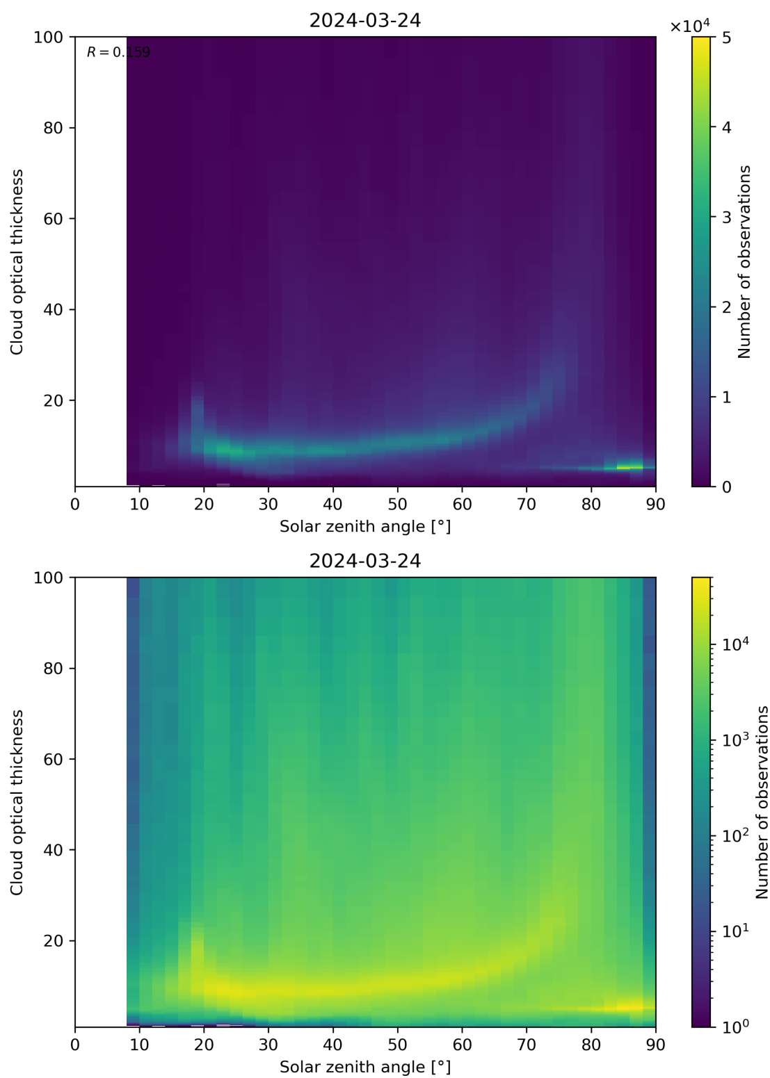
Figure 103: Scatter density plot of “Solar zenith angle” against “Cloud optical thickness” for 2024-03-23 to 2024-03-25.
