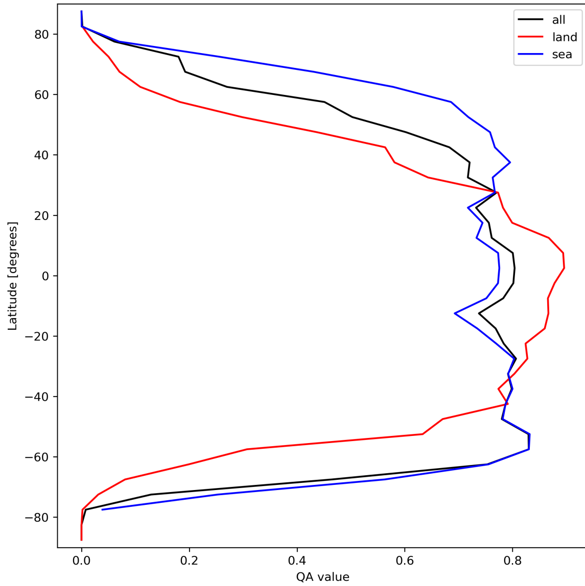
Figure 22: Zonal average of “QA value” for 2024-03-23 to 2024-03-25.
