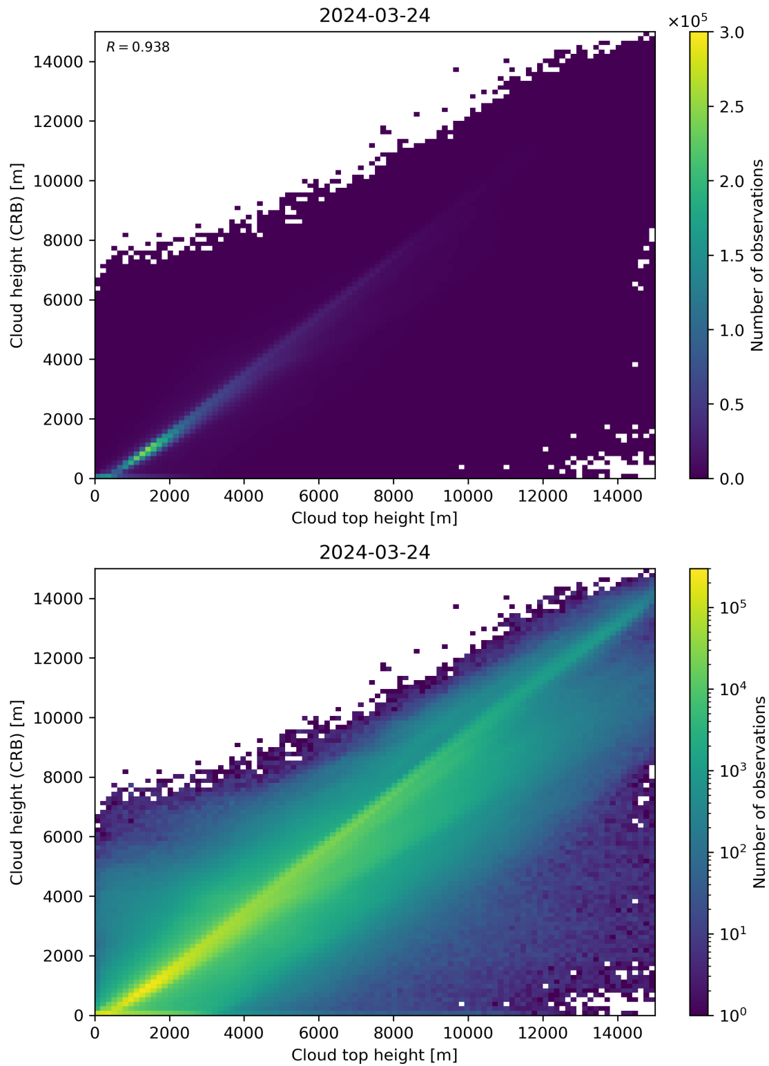
Figure 89: Scatter density plot of “Cloud top height” against “Cloud height (CRB)” for 2024-03-23 to 2024-03-25.
