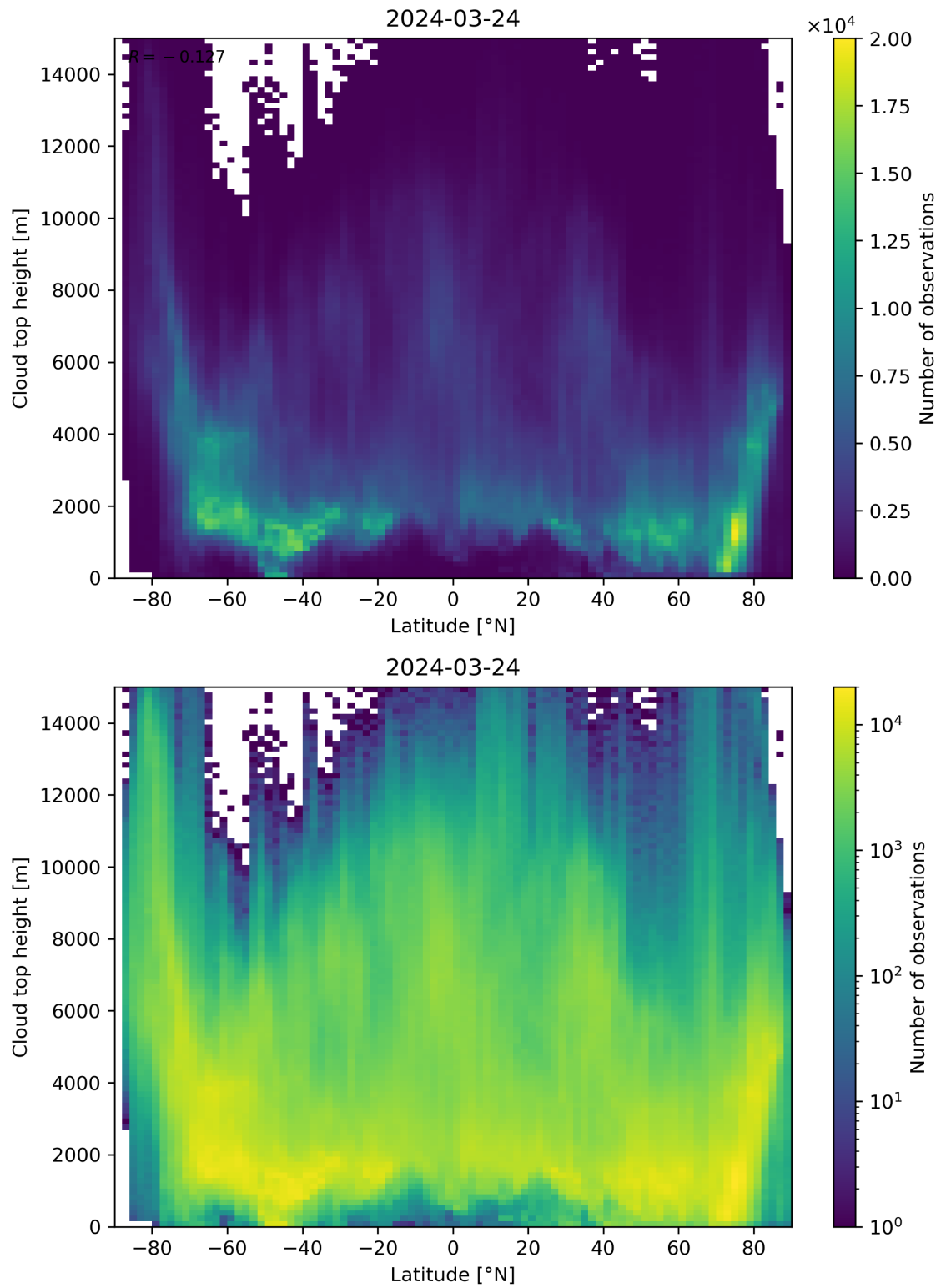
Figure 97: Scatter density plot of “Latitude” against “Cloud top height” for 2024-03-23 to 2024-03-25.
