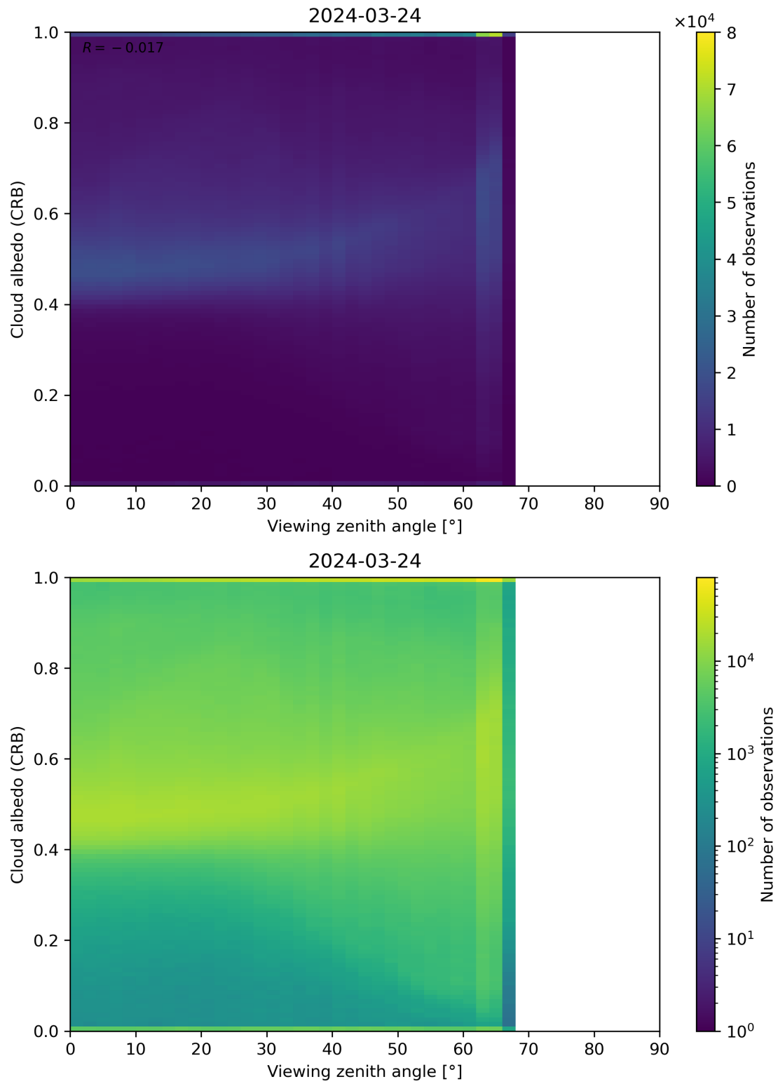
Figure 106: Scatter density plot of “Viewing zenith angle” against “Cloud albedo (CRB)” for 2024-03-23 to 2024-03-25.
