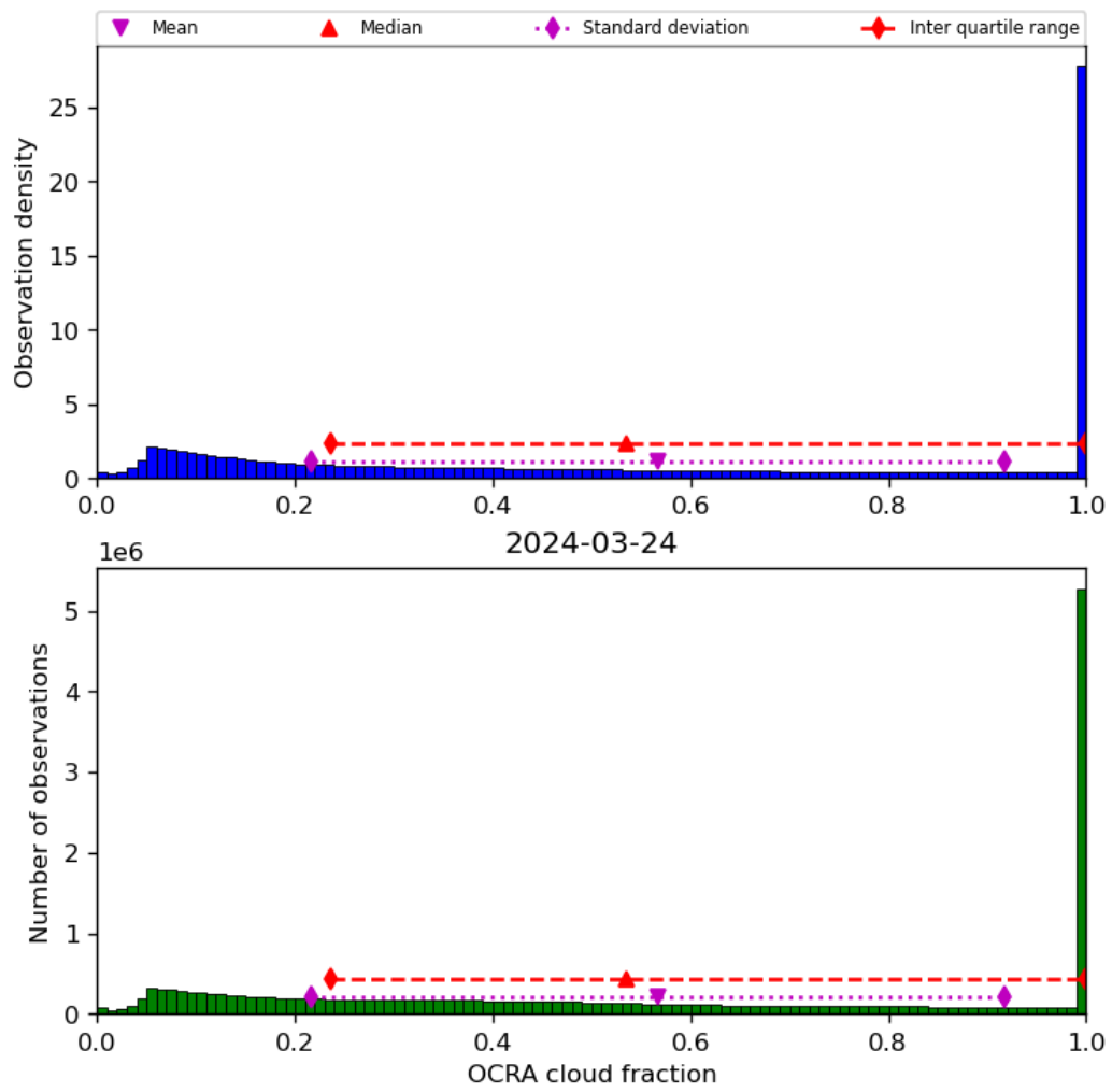
Figure 50: Histogram of “OCRA cloud fraction” for 2024-03-23 to 2024-03-25
