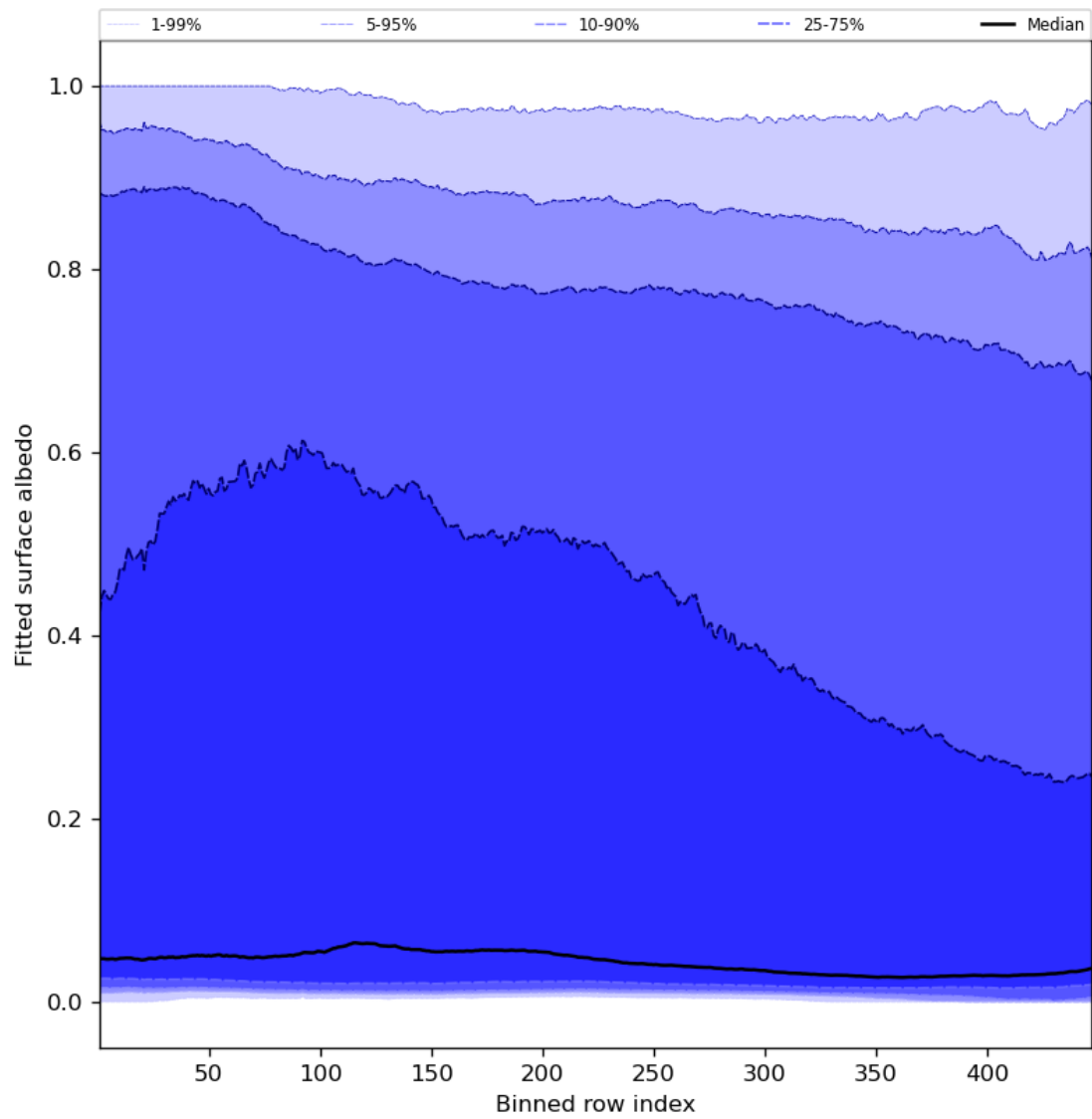
Figure 61: Along track statistics of “Fitted surface albedo” for 2024-03-23 to 2024-03-25
