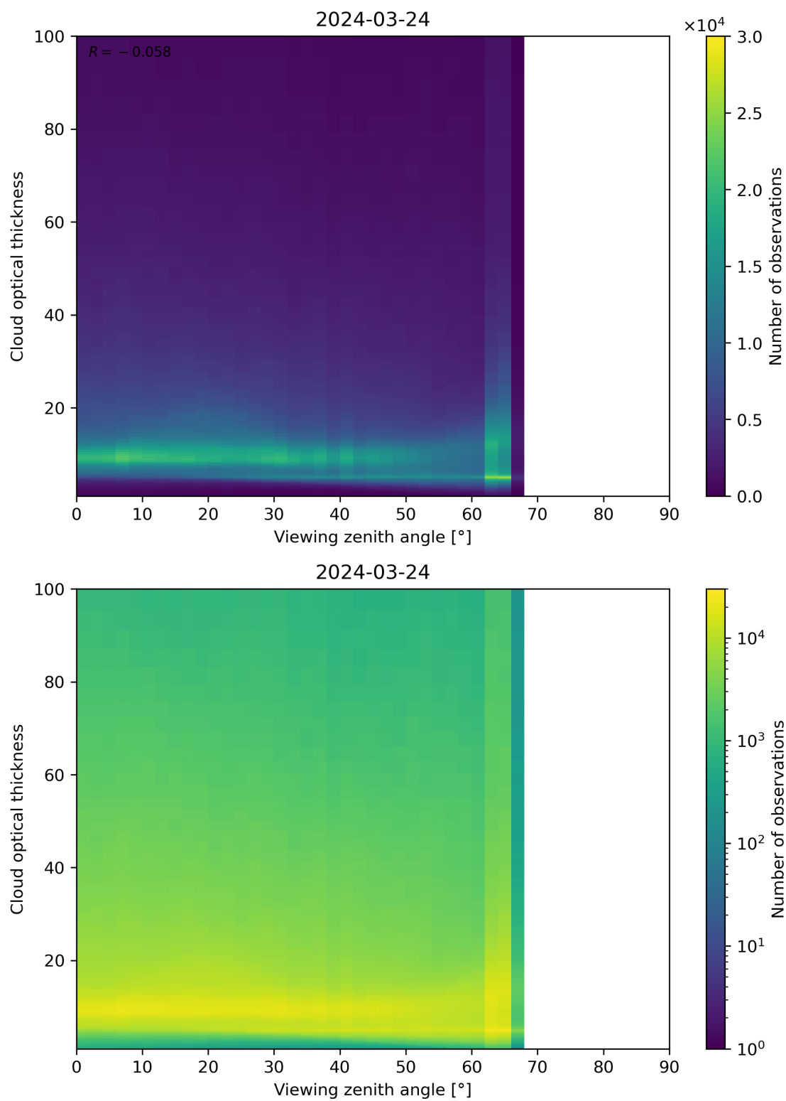
Figure 111: Scatter density plot of “Viewing zenith angle” against “Cloud optical thickness” for 2024-03-23 to 2024-03-25.
