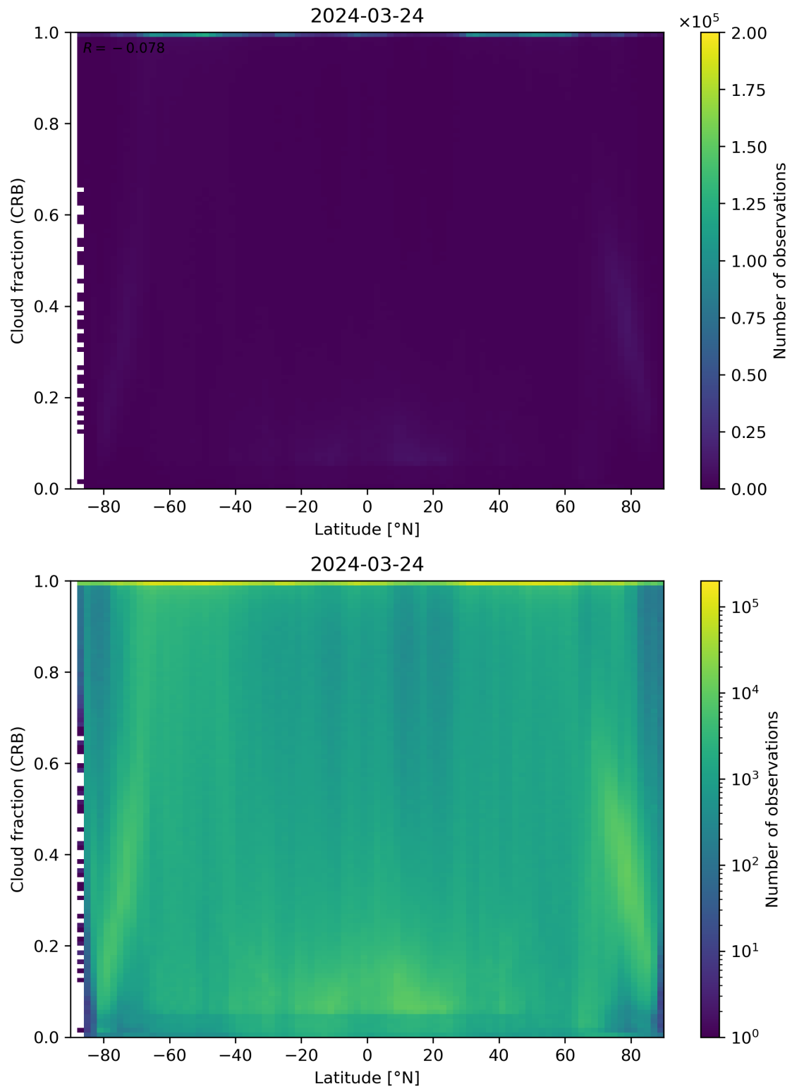
Figure 94: Scatter density plot of “Latitude” against “Cloud fraction (CRB)” for 2024-03-23 to 2024-03-25.
