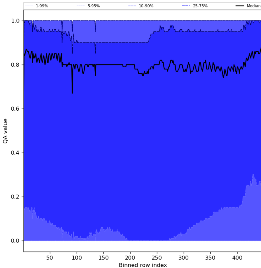
Figure 54: Along track statistics of “QA value” for 2024-03-23 to 2024-03-25
