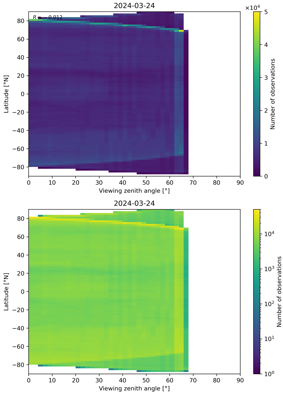
Figure 113: Scatter density plot of “Viewing zenith angle” against “Latitude” for 2024-03-23 to 2024-03-25.
