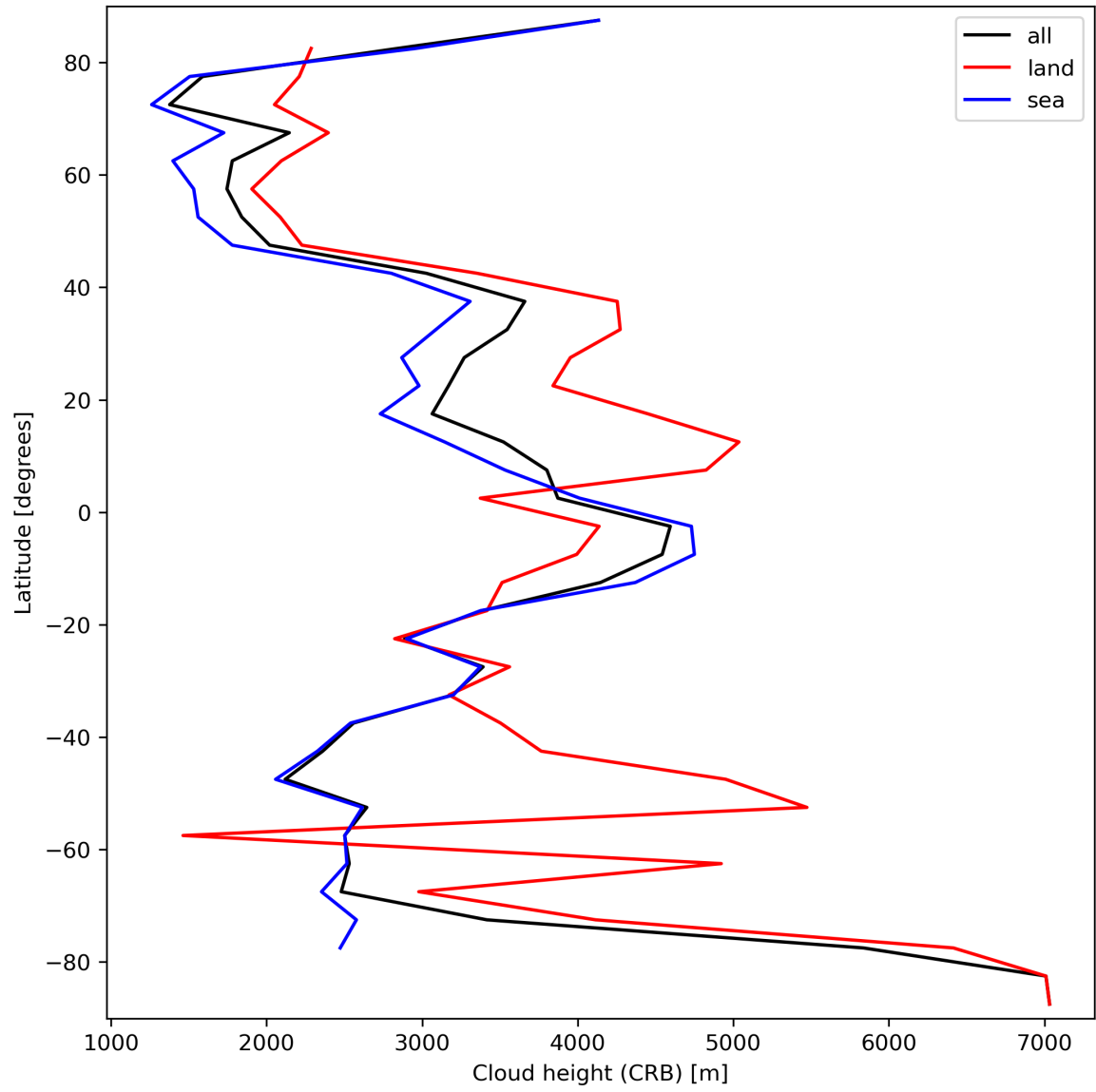
Figure 27: Zonal average of “Cloud height (CRB)” for 2024-03-23 to 2024-03-25.
