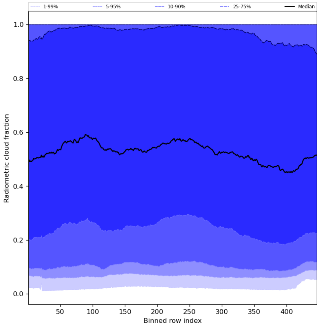
Figure 55: Along track statistics of “Radiometric cloud fraction” for 2024-03-23 to 2024-03-25
