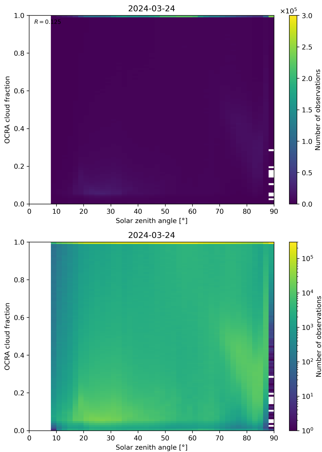
Figure 100: Scatter density plot of “Solar zenith angle” against “OCRA cloud fraction” for 2024-03-23 to 2024-03-25.
