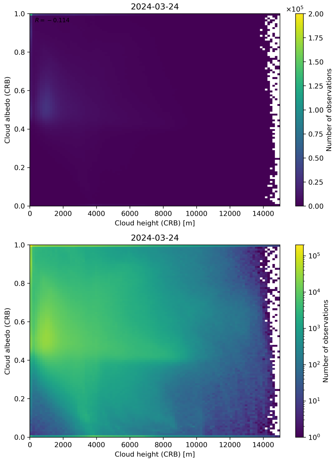
Figure 80: Scatter density plot of “Cloud height (CRB)” against “Cloud albedo (CRB)” for 2024-03-23 to 2024-03-25.
