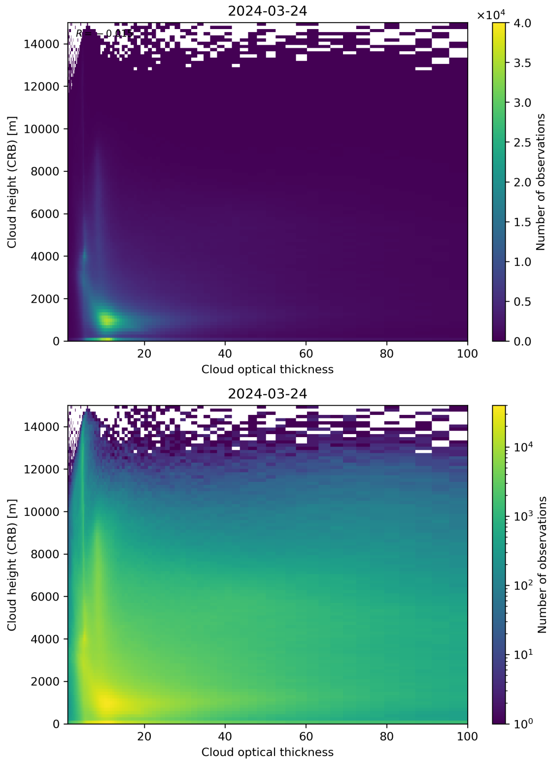
Figure 85: Scatter density plot of “Cloud optical thickness” against “Cloud height (CRB)” for 2024-03-23 to 2024-03-25.
