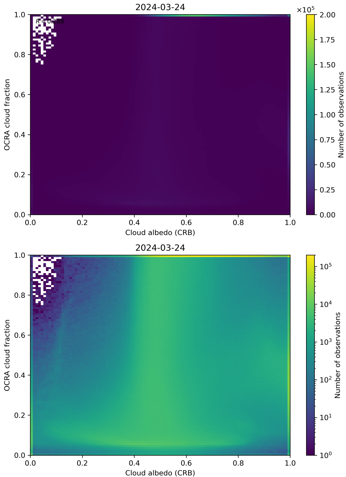
Figure 70: Scatter density plot of “Cloud albedo (CRB)” against “OCRA cloud fraction” for 2024-03-23 to 2024-03-25.
