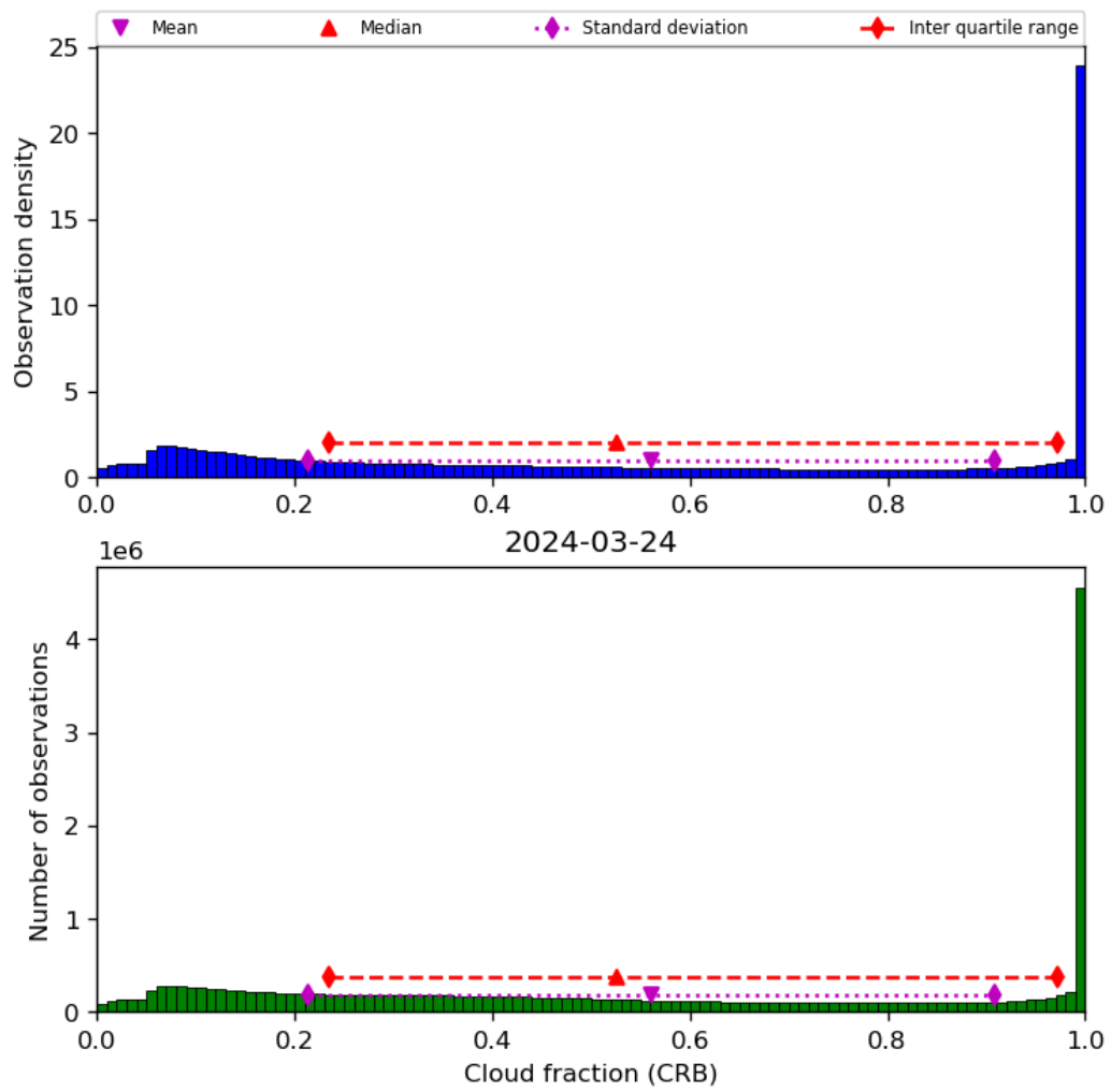
Figure 42: Histogram of “Cloud fraction (CRB)” for 2024-03-23 to 2024-03-25
