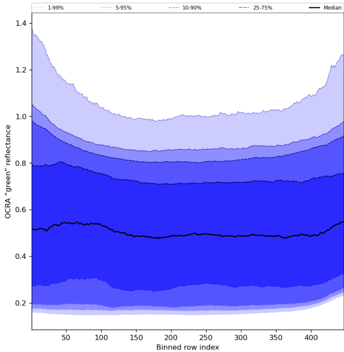
Figure 68: Along track statistics of “OCRA “green” reflectance” for 2024-03-23 to 2024-03-25
