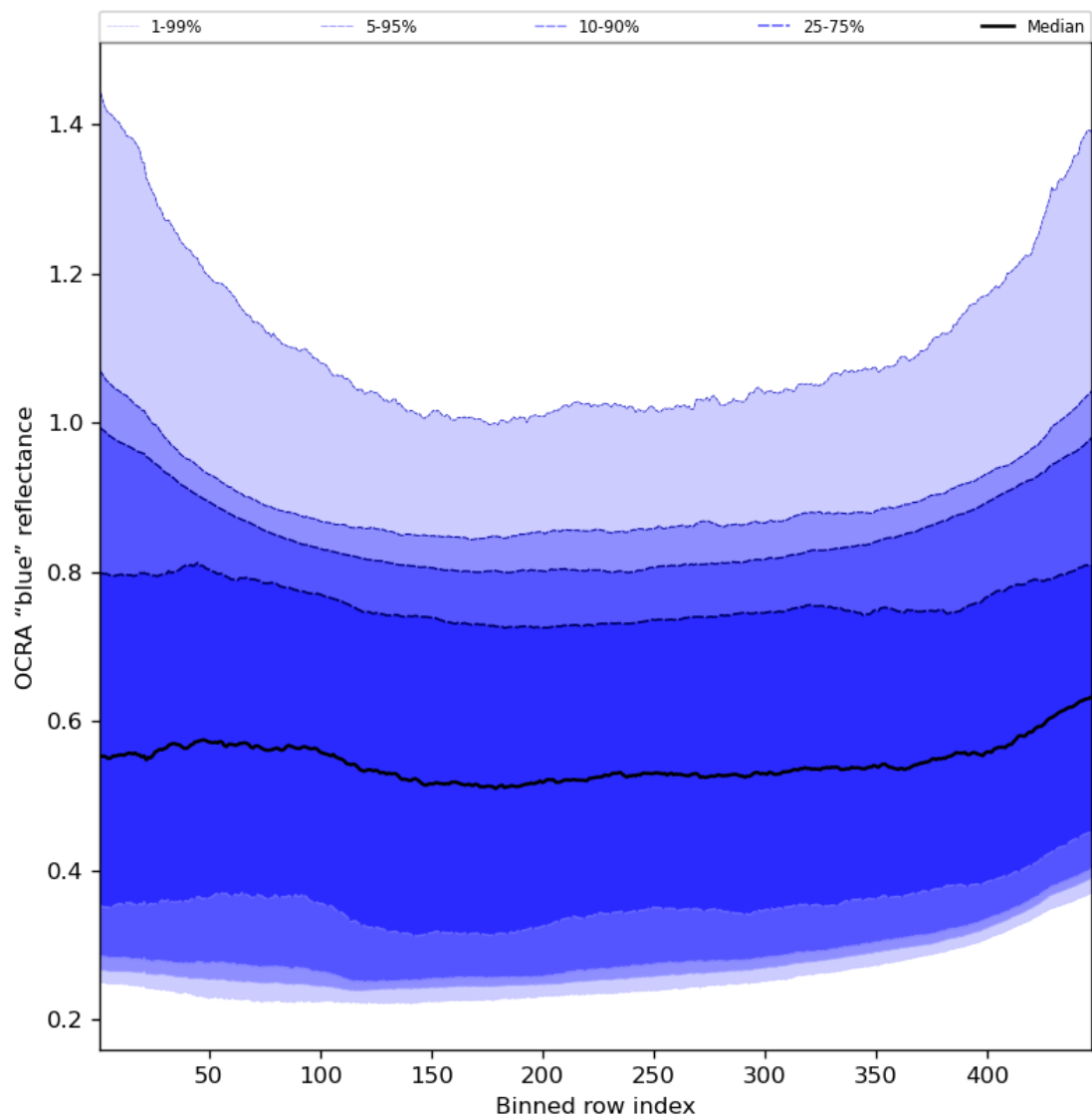
Figure 67: Along track statistics of "OCRA "blue" reflectance" for 2024-03-23 to 2024-03-25
