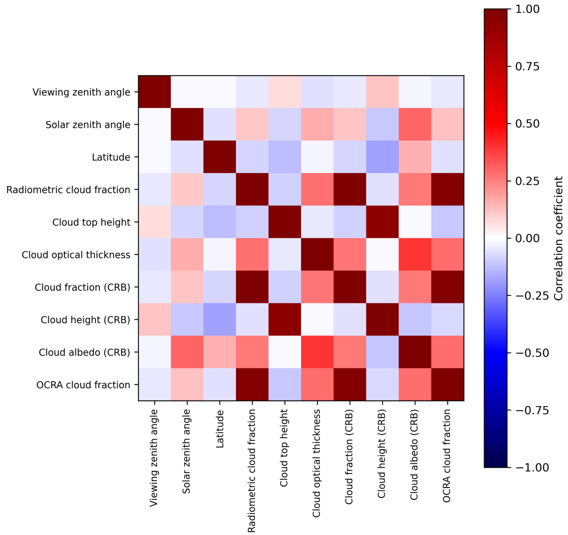
Figure 2: Map of correlation matrix for 2024-03-23 to 2024-03-25.
