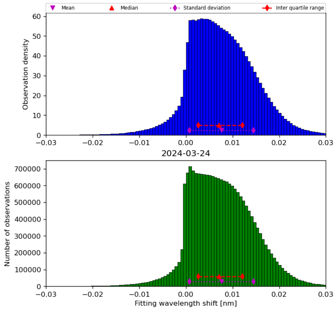
Figure 49: Histogram of “Fitting wavelength shift” for 2024-03-23 to 2024-03-25
