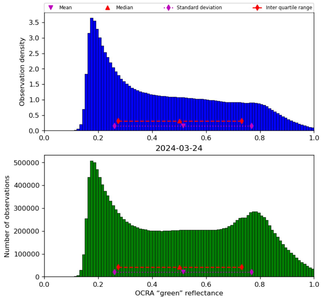
Figure 52: Histogram of “OCRA “green” reflectance” for 2024-03-23 to 2024-03-25
