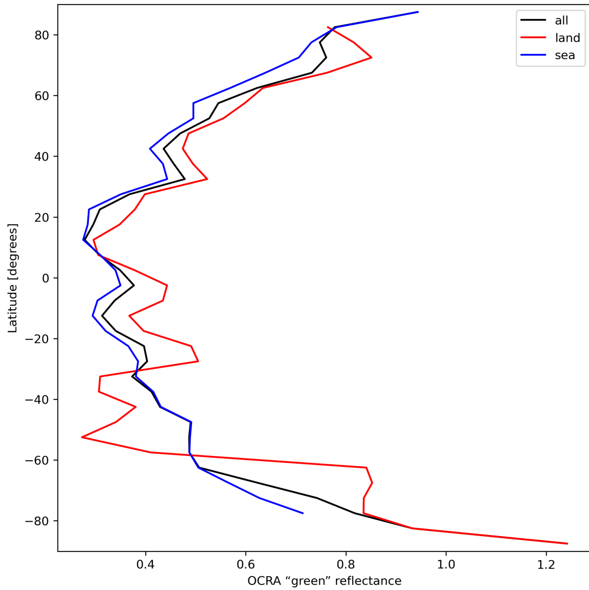
Figure 36: Zonal average of “OCRA “green” reflectance” for 2024-03-23 to 2024-03-25.
