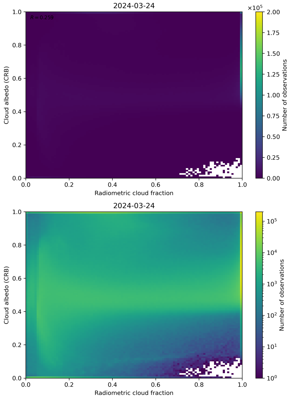
Figure 71: Scatter density plot of “Radiometric cloud fraction” against “Cloud albedo (CRB)” for 2024-03-23 to 2024-03-25.
