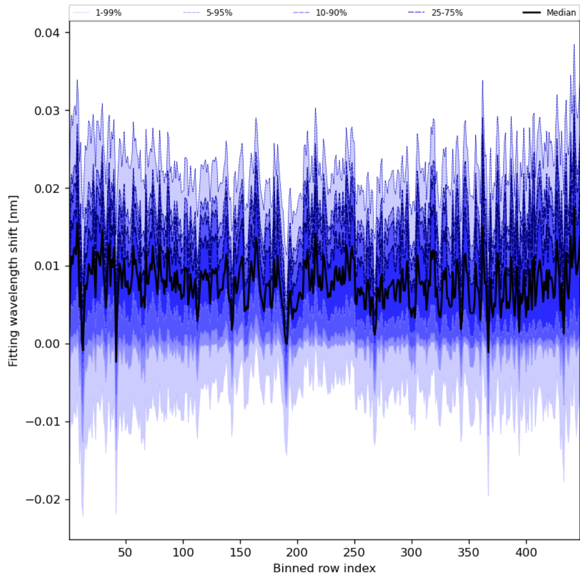
Figure 65: Along track statistics of “Fitting wavelength shift” for 2024-03-23 to 2024-03-25
