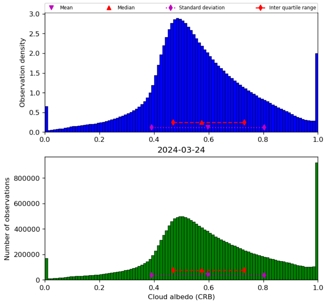
Figure 44: Histogram of “Cloud albedo (CRB)” for 2024-03-23 to 2024-03-25
