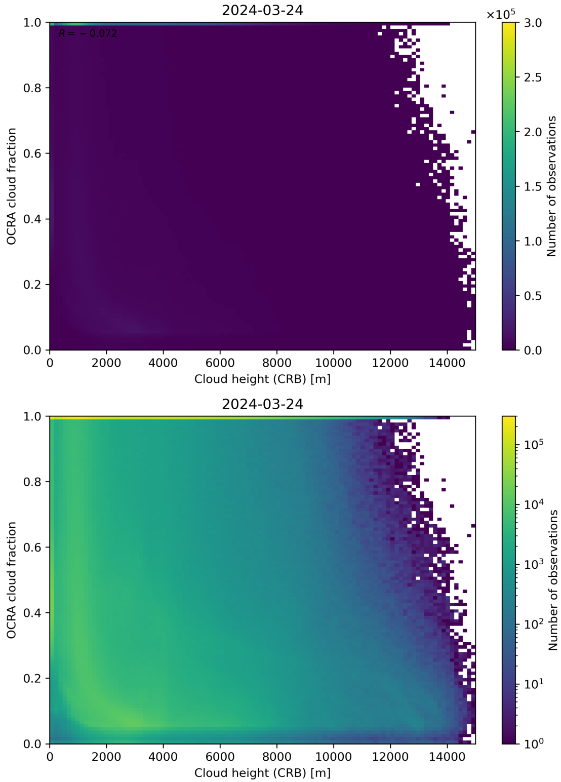
Figure 81: Scatter density plot of “Cloud height (CRB)” against “OCRA cloud fraction” for 2024-03-23 to 2024-03-25.
