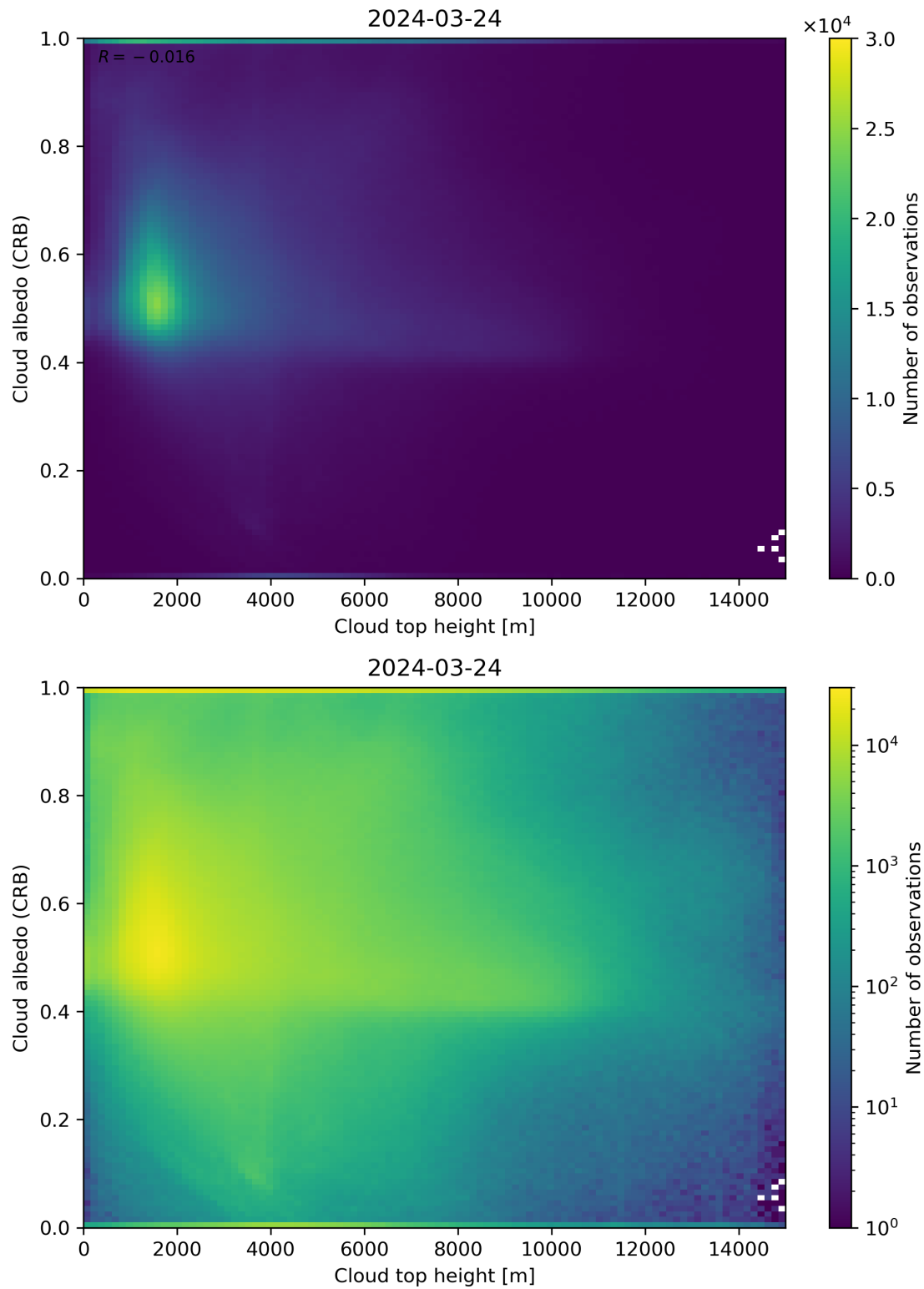
Figure 86: Scatter density plot of “Cloud top height” against “Cloud albedo (CRB)” for 2024-03-23 to 2024-03-25.
