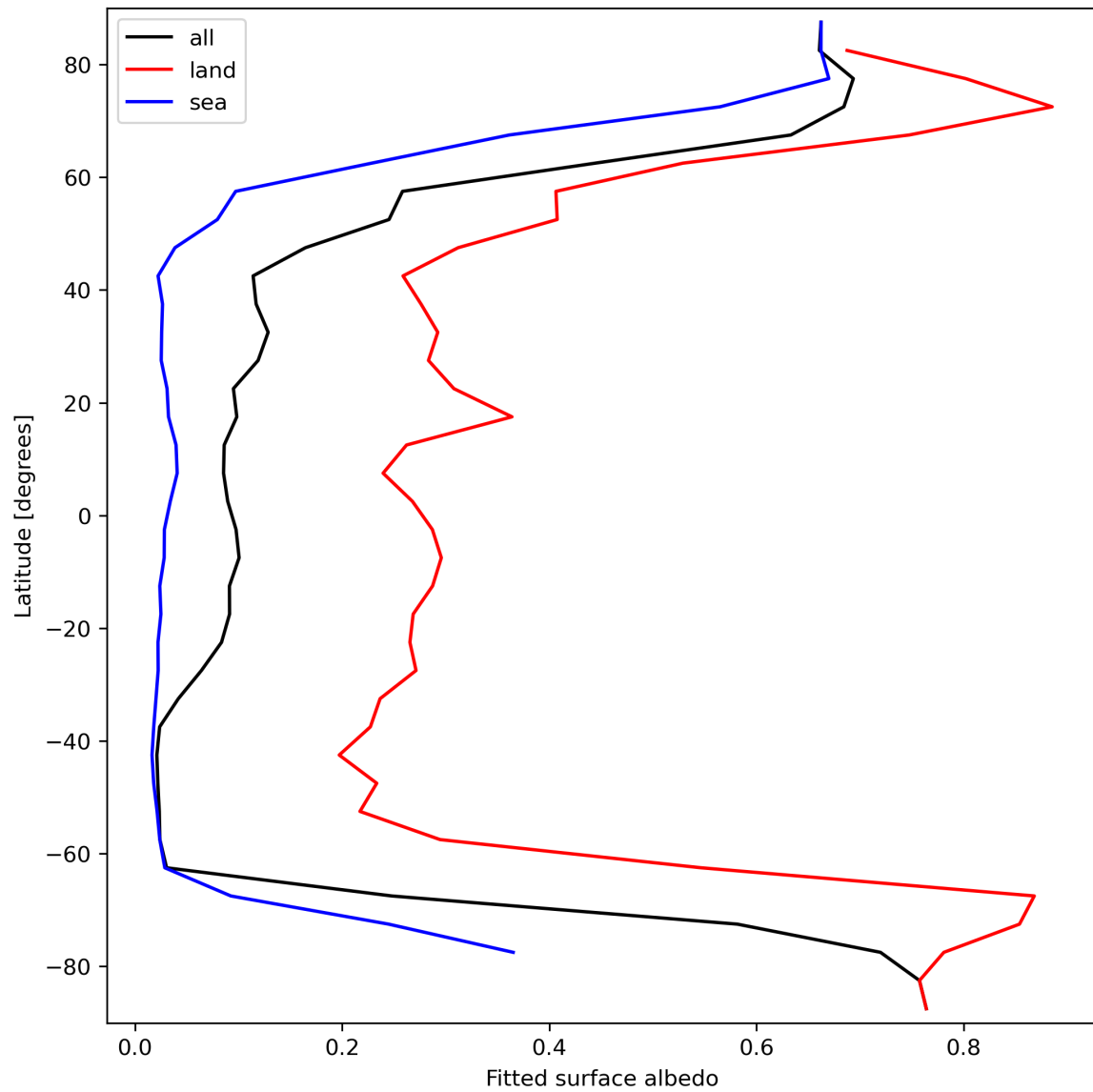
Figure 29: Zonal average of “Fitted surface albedo” for 2024-03-23 to 2024-03-25.
