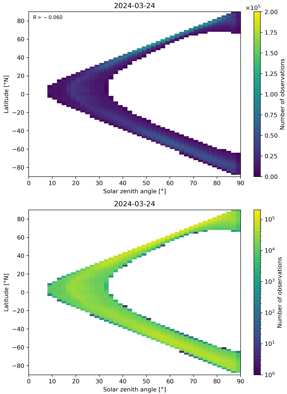
Figure 105: Scatter density plot of “Solar zenith angle” against “Latitude” for 2024-03-23 to 2024-03-25.
