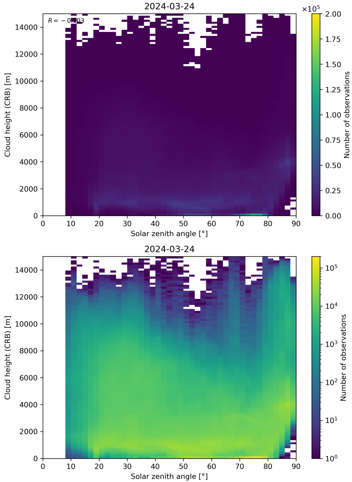
Figure 102: Scatter density plot of “Solar zenith angle” against “Cloud height (CRB)” for 2024-03-23 to 2024-03-25.
