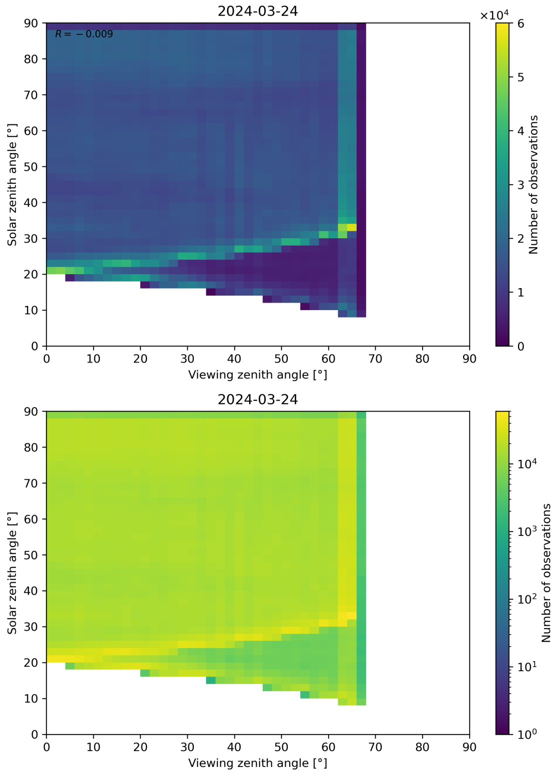
Figure 114: Scatter density plot of “Viewing zenith angle” against “Solar zenith angle” for 2024-03-23 to 2024-03-25.
