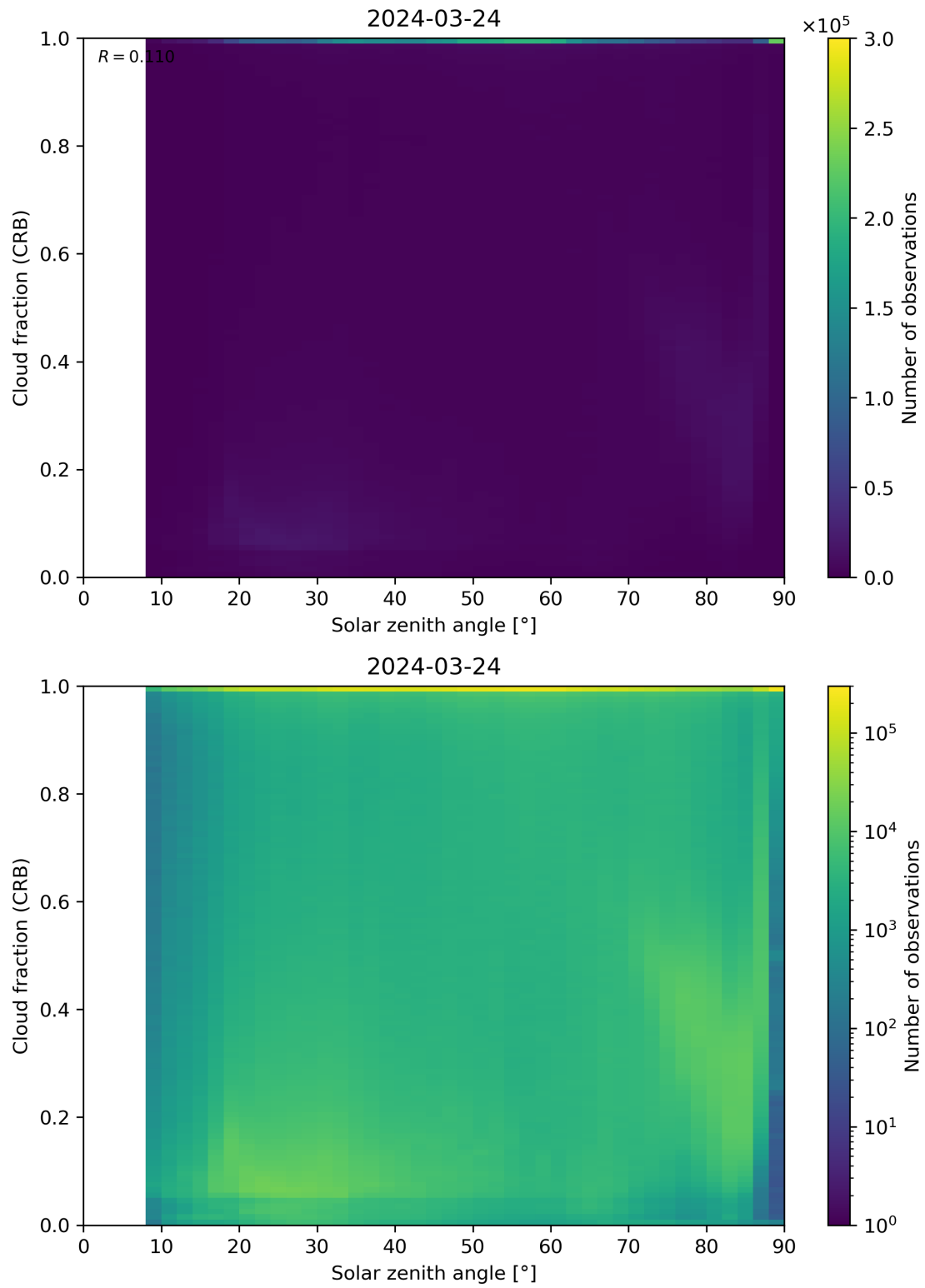
Figure 101: Scatter density plot of “Solar zenith angle” against “Cloud fraction (CRB)” for 2024-03-23 to 2024-03-25.
