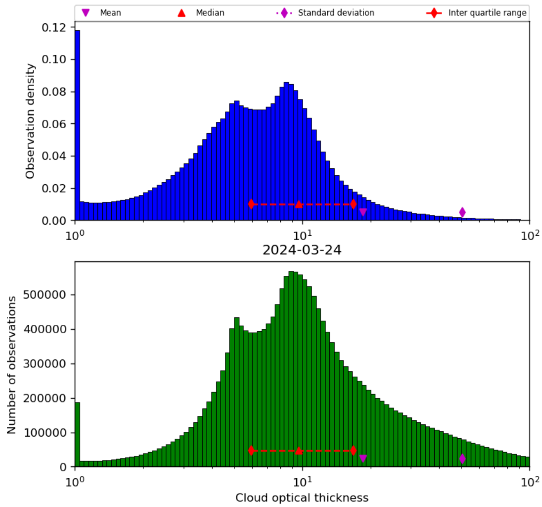
Figure 41: Histogram of “Cloud optical thickness” for 2024-03-23 to 2024-03-25
