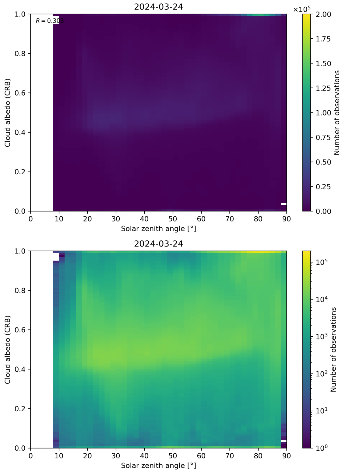
Figure 98: Scatter density plot of “Solar zenith angle” against “Cloud albedo (CRB)” for 2024-03-23 to 2024-03-25.
