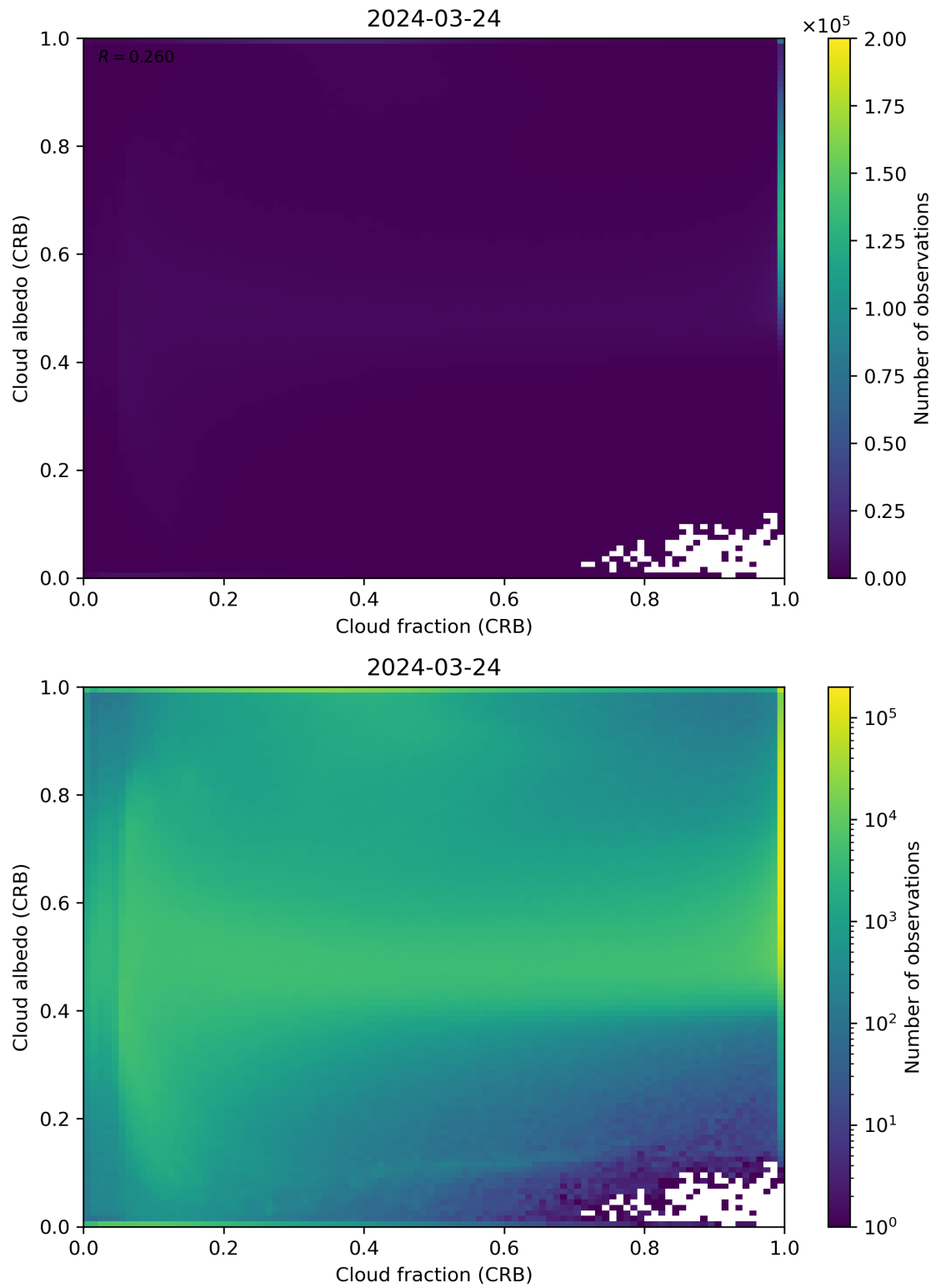
Figure 77: Scatter density plot of “Cloud fraction (CRB)” against “Cloud albedo (CRB)” for 2024-03-23 to 2024-03-25.
