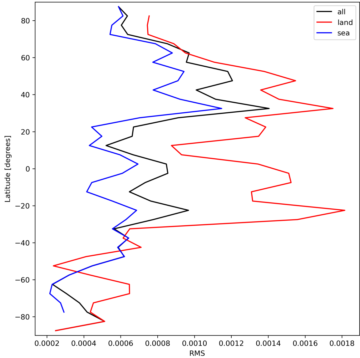
Figure 31: Zonal average of “RMS” for 2024-03-23 to 2024-03-25.
