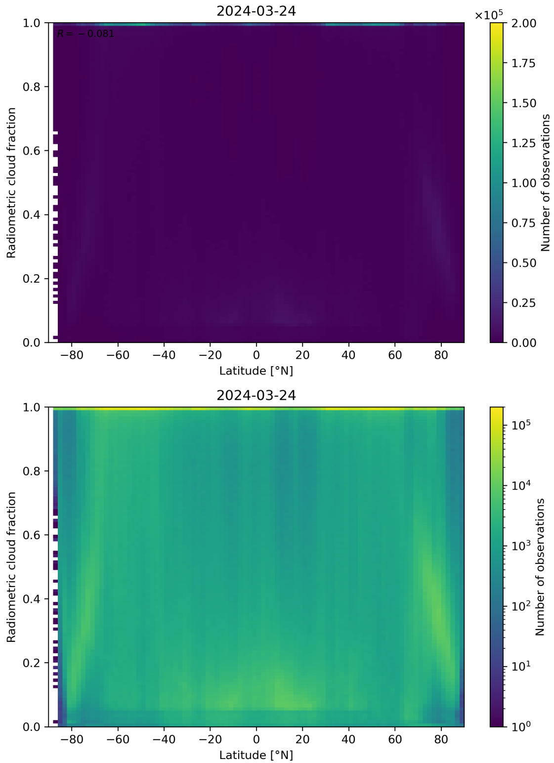
Figure 92: Scatter density plot of “Latitude” against “Radiometric cloud fraction” for 2024-03-23 to 2024-03-25.
