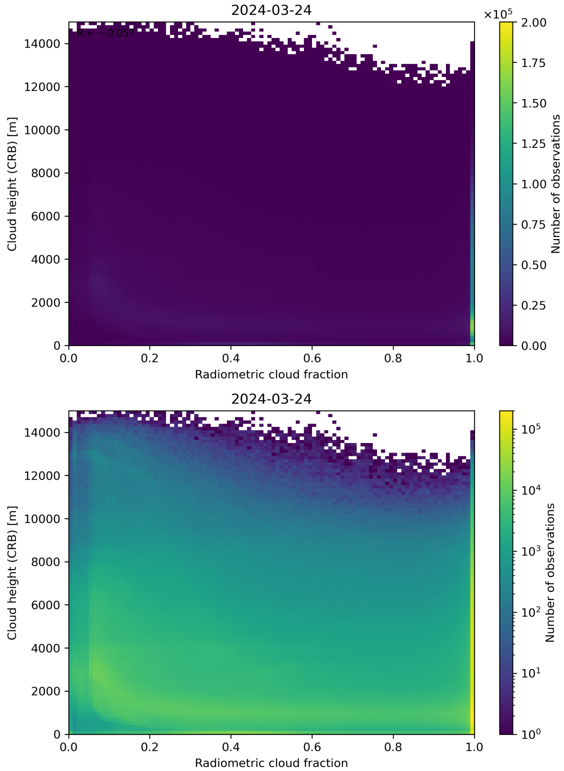
Figure 74: Scatter density plot of “Radiometric cloud fraction” against “Cloud height (CRB)” for 2024-03-23 to 2024-03-25.
