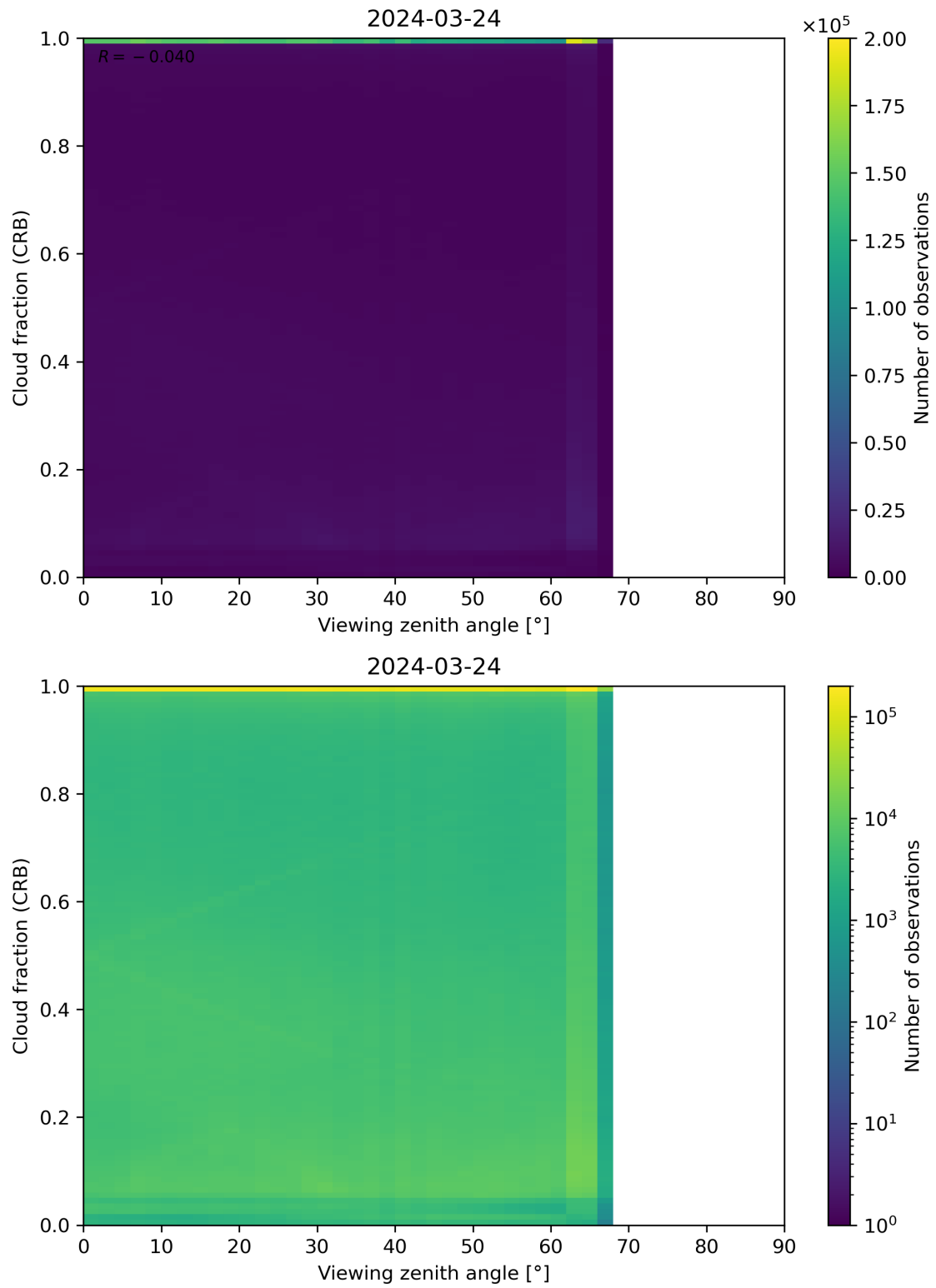
Figure 109: Scatter density plot of “Viewing zenith angle” against “Cloud fraction (CRB)” for 2024-03-23 to 2024-03-25.
