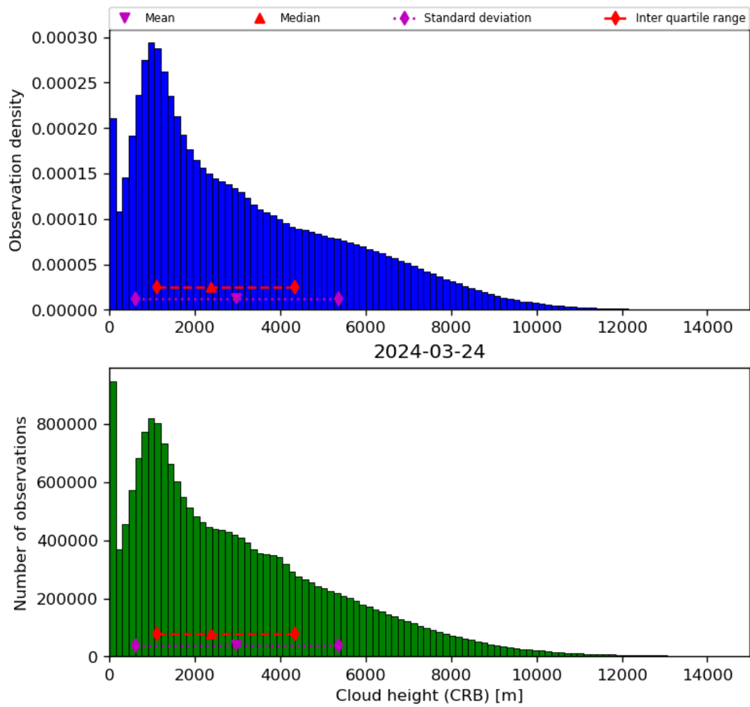
Figure 43: Histogram of “Cloud height (CRB)” for 2024-03-23 to 2024-03-25
