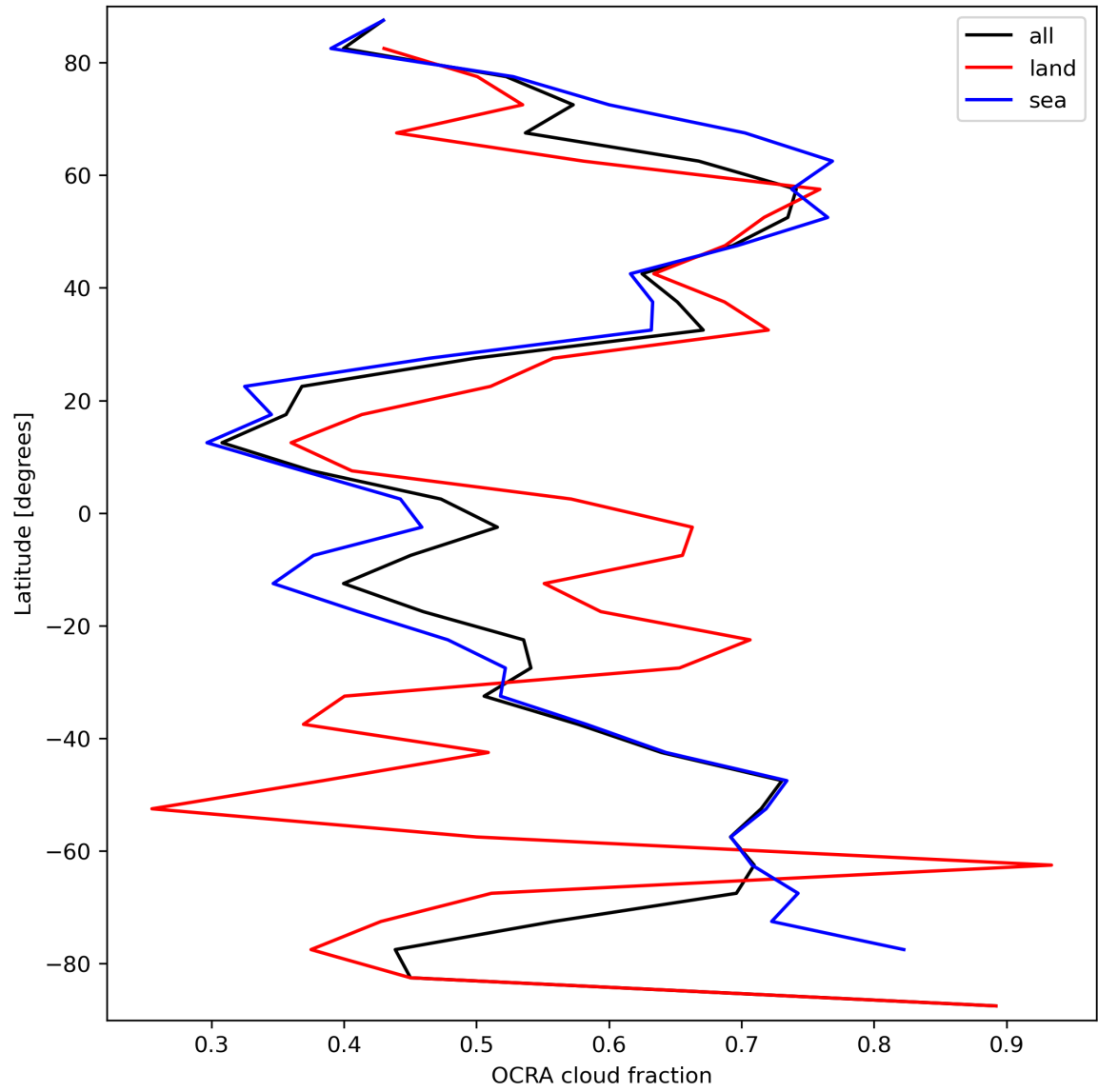
Figure 34: Zonal average of “OCRA cloud fraction” for 2024-03-23 to 2024-03-25.
