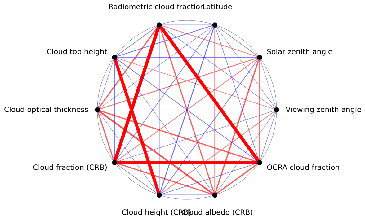
Figure 1: Map of correlation graph for 2024-03-23 to 2024-03-25.
