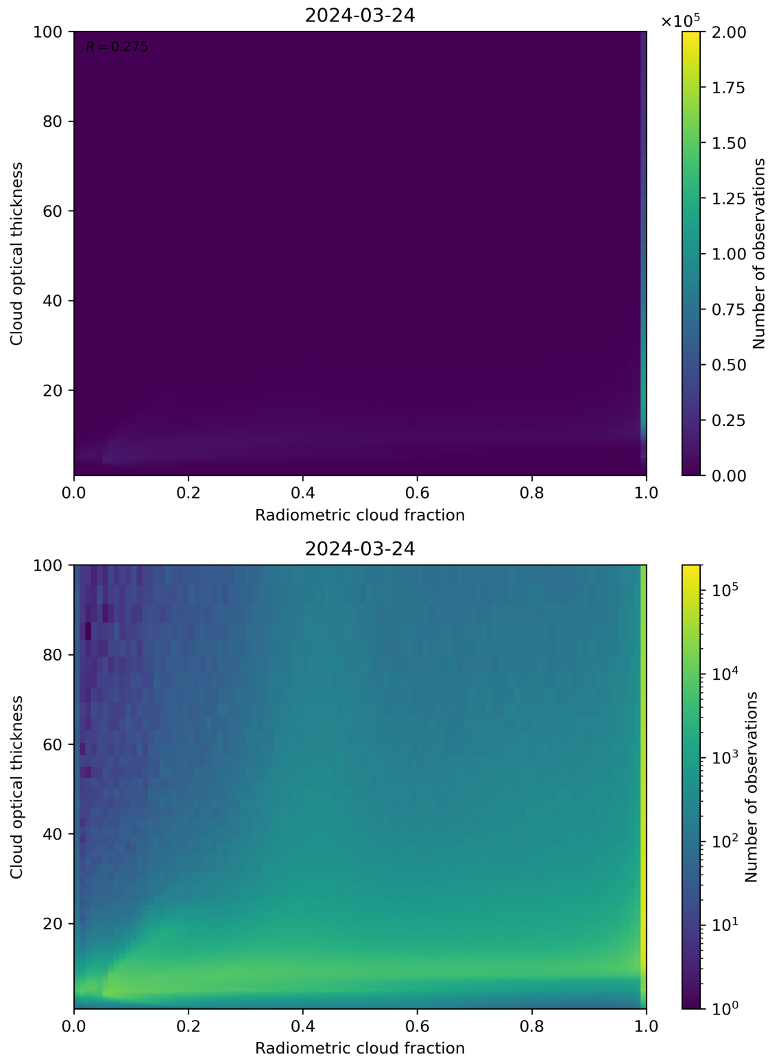
Figure 75: Scatter density plot of “Radiometric cloud fraction” against “Cloud optical thickness” for 2024-03-23 to 2024-03-25.
