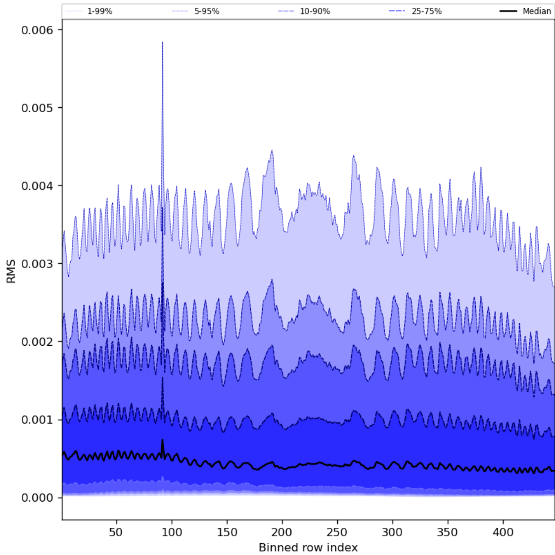
Figure 63: Along track statistics of “RMS” for 2024-03-23 to 2024-03-25
