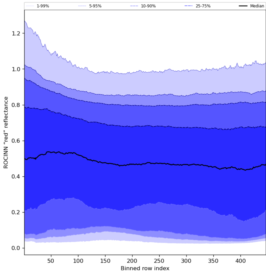
Figure 69: Along track statistics of “ROCINN “red” reflectance” for 2024-03-23 to 2024-03-25
