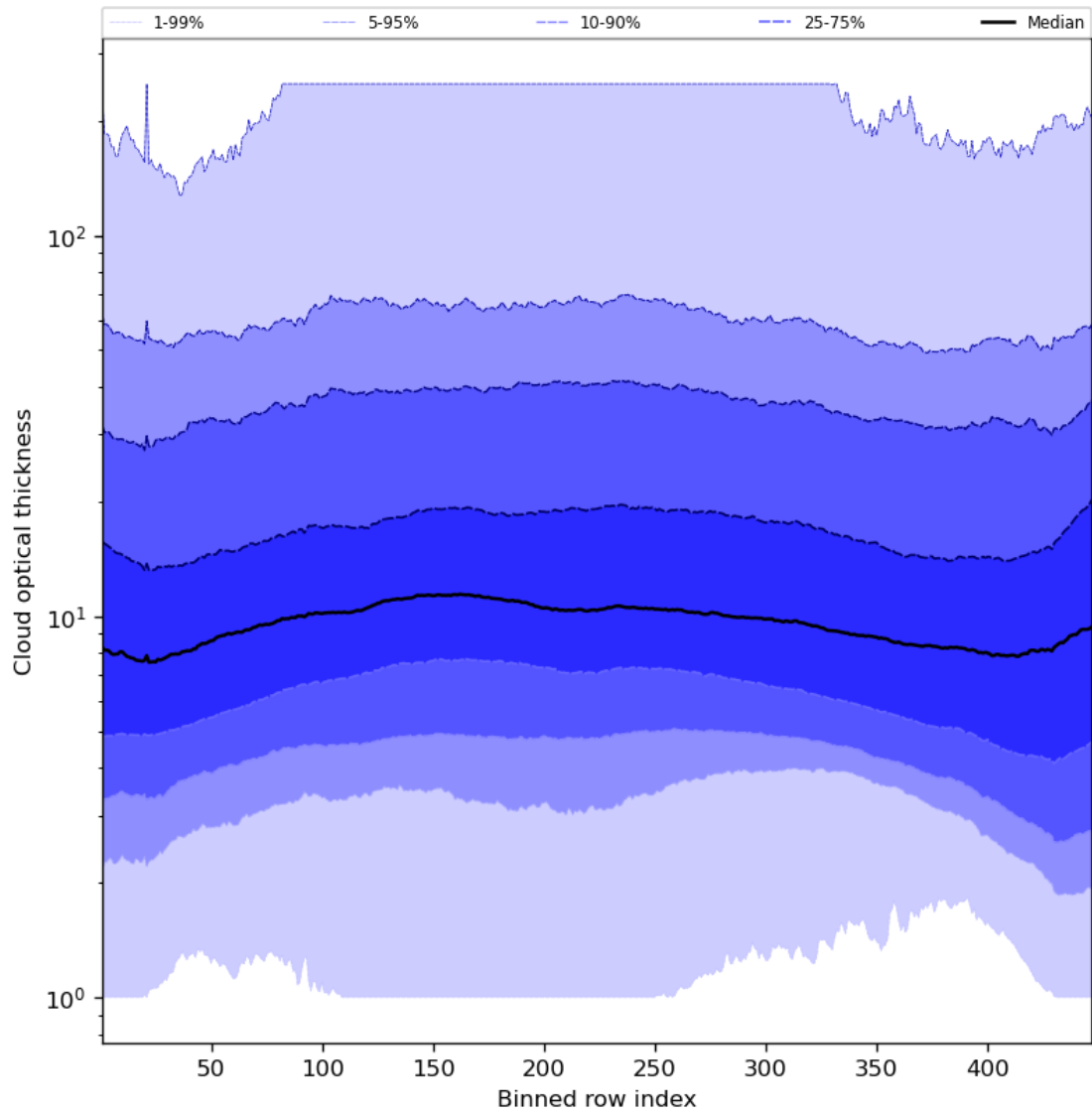
Figure 57: Along track statistics of “Cloud optical thickness” for 2024-03-23 to 2024-03-25
