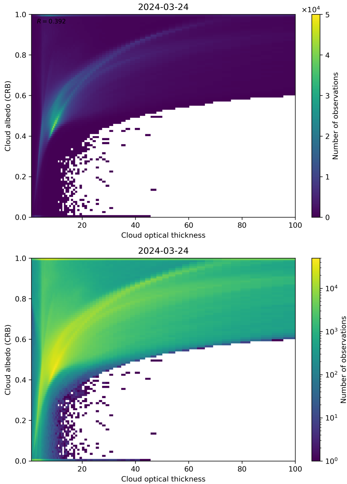
Figure 82: Scatter density plot of “Cloud optical thickness” against “Cloud albedo (CRB)” for 2024-03-23 to 2024-03-25.
