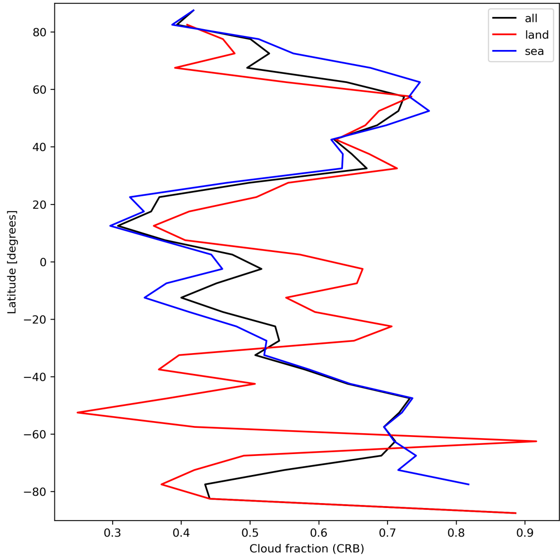
Figure 26: Zonal average of “Cloud fraction (CRB)” for 2024-03-23 to 2024-03-25.
