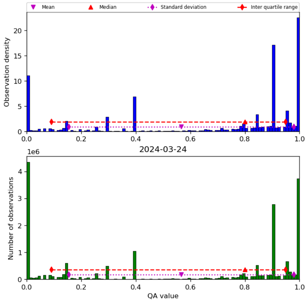
Figure 38: Histogram of “QA value” for 2024-03-23 to 2024-03-25
