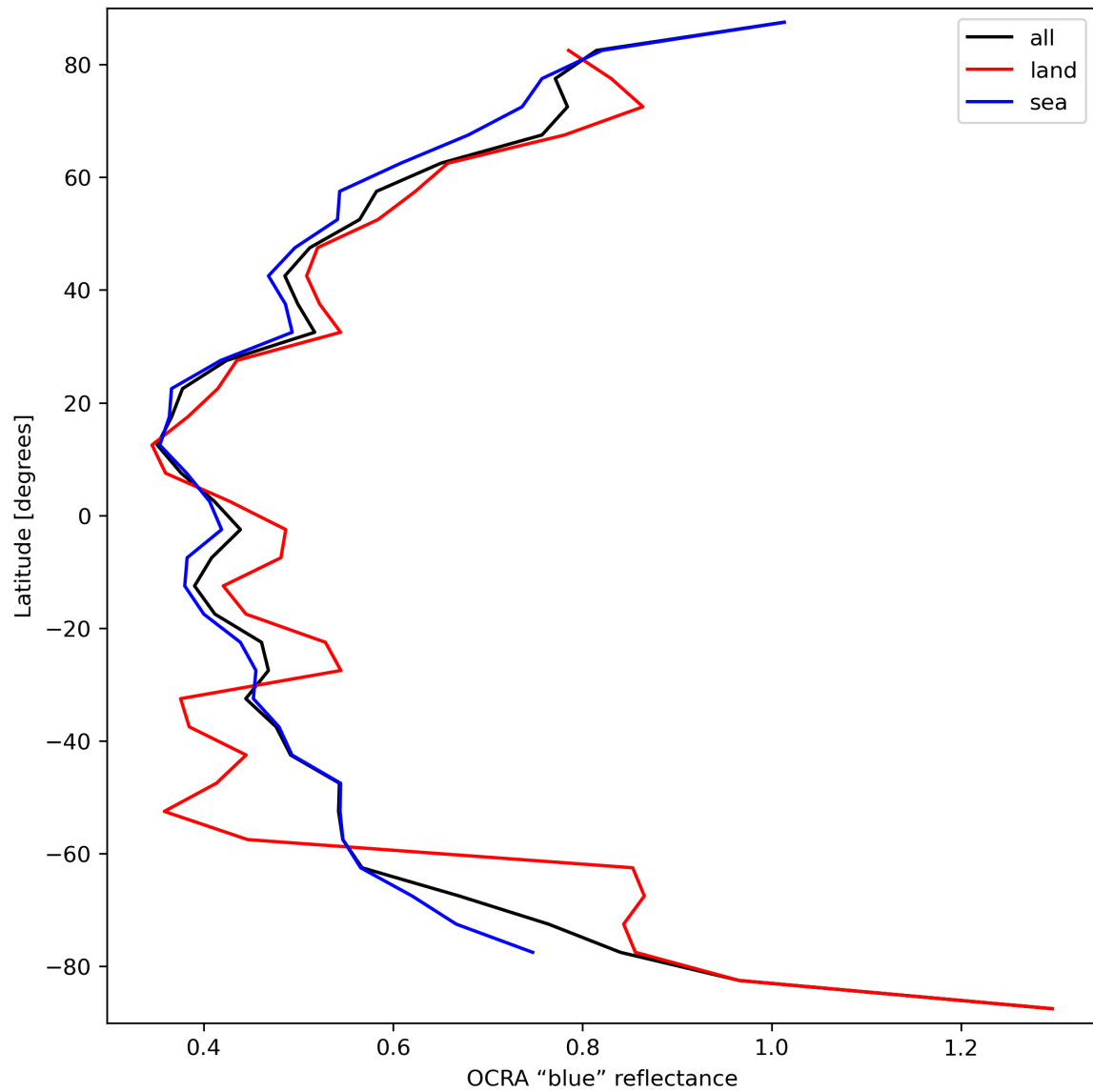
Figure 35: Zonal average of “OCRA “blue” reflectance” for 2024-03-23 to 2024-03-25.
