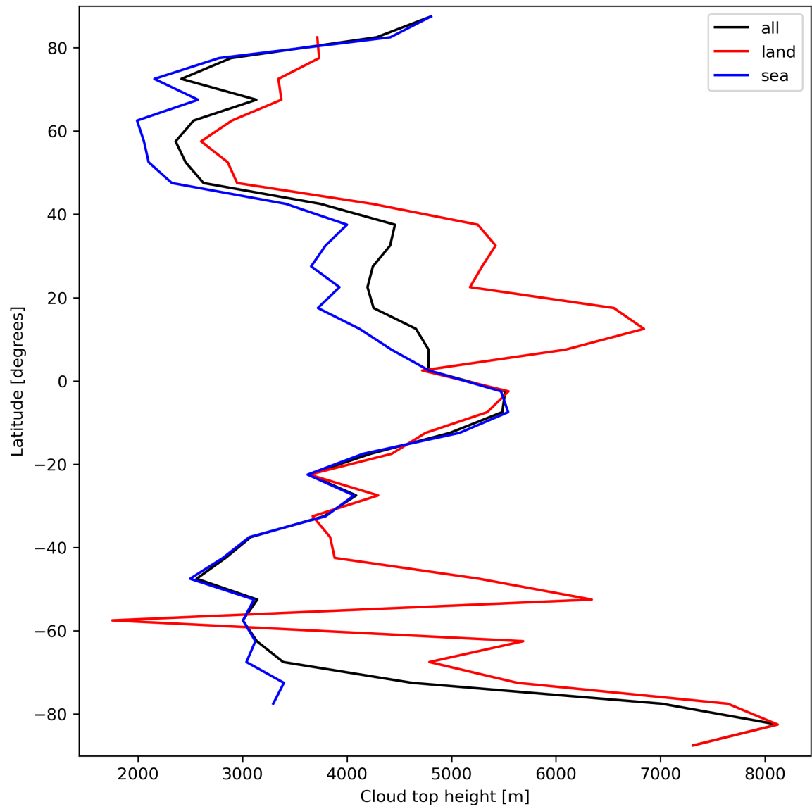
Figure 24: Zonal average of “Cloud top height” for 2024-03-23 to 2024-03-25.
