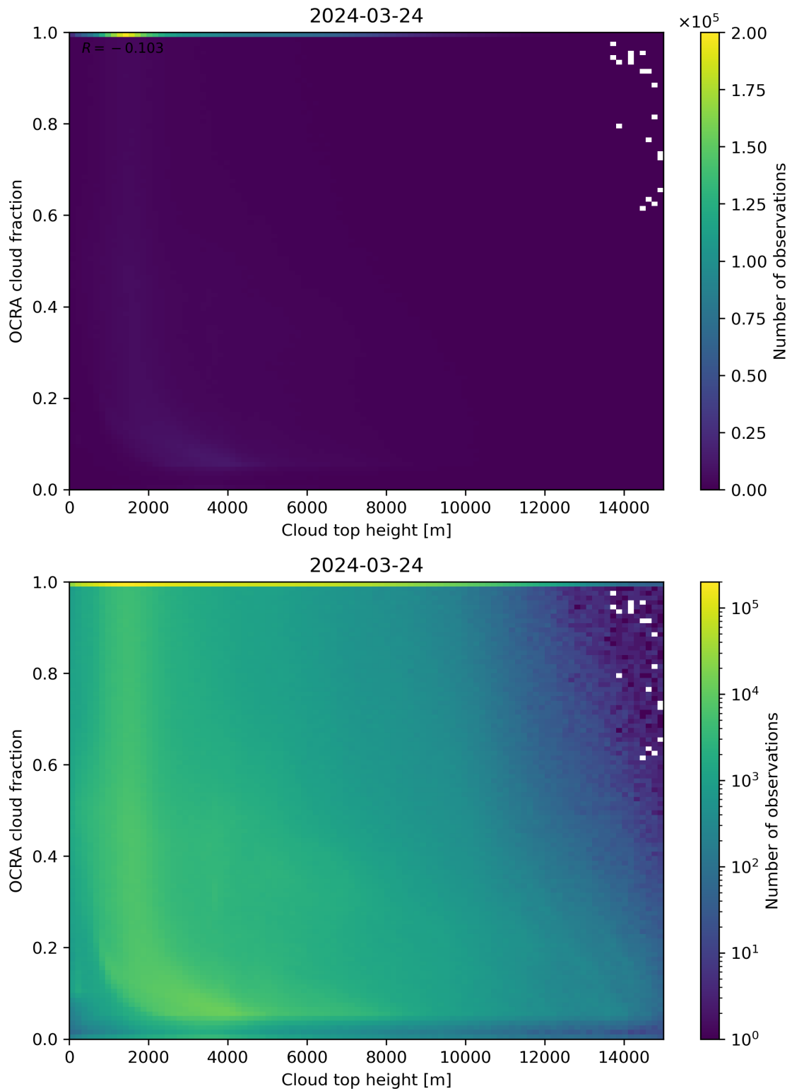
Figure 87: Scatter density plot of “Cloud top height” against “OCRA cloud fraction” for 2024-03-23 to 2024-03-25.
