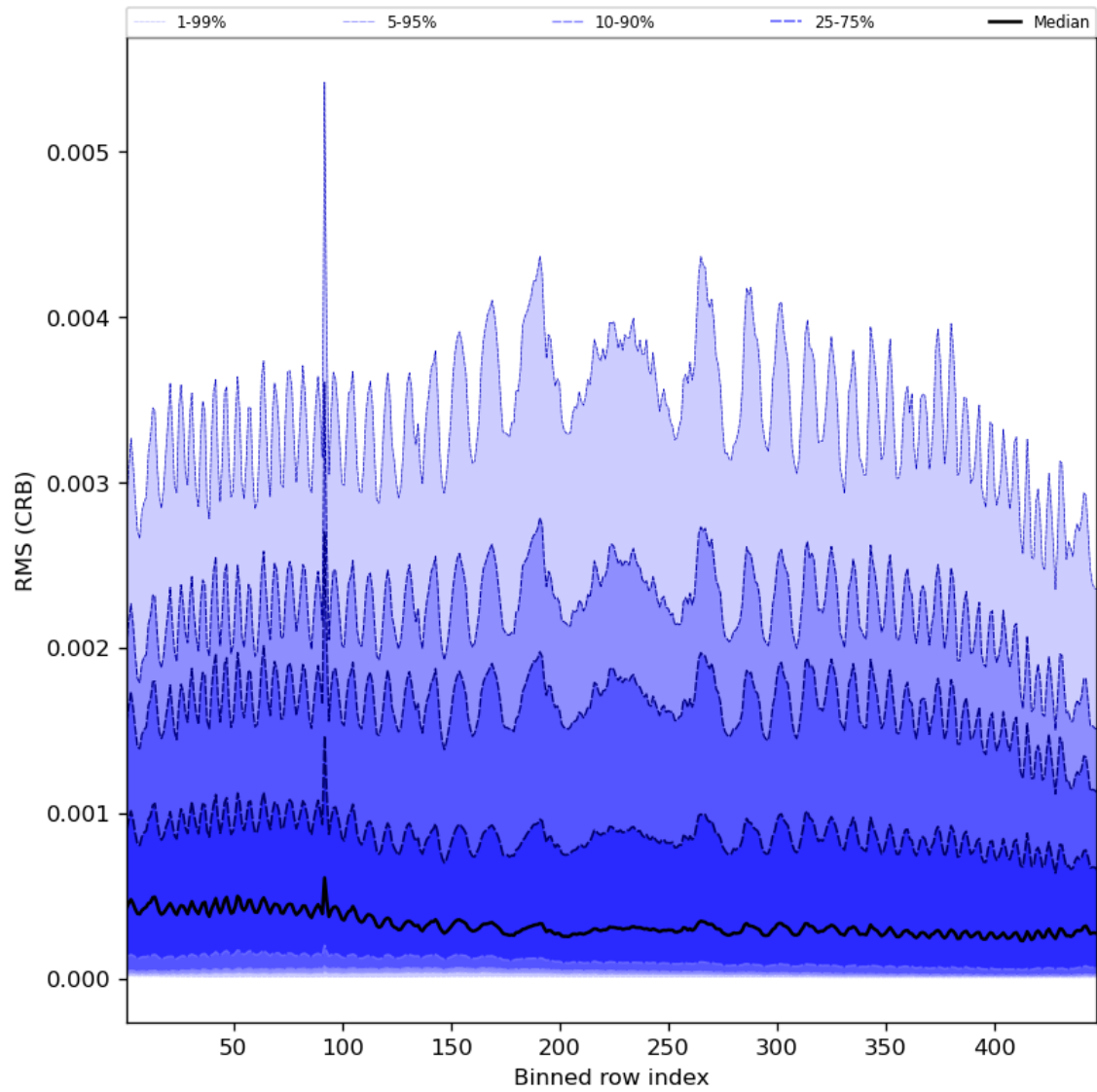
Figure 64: Along track statistics of “RMS (CRB)” for 2024-03-23 to 2024-03-25
