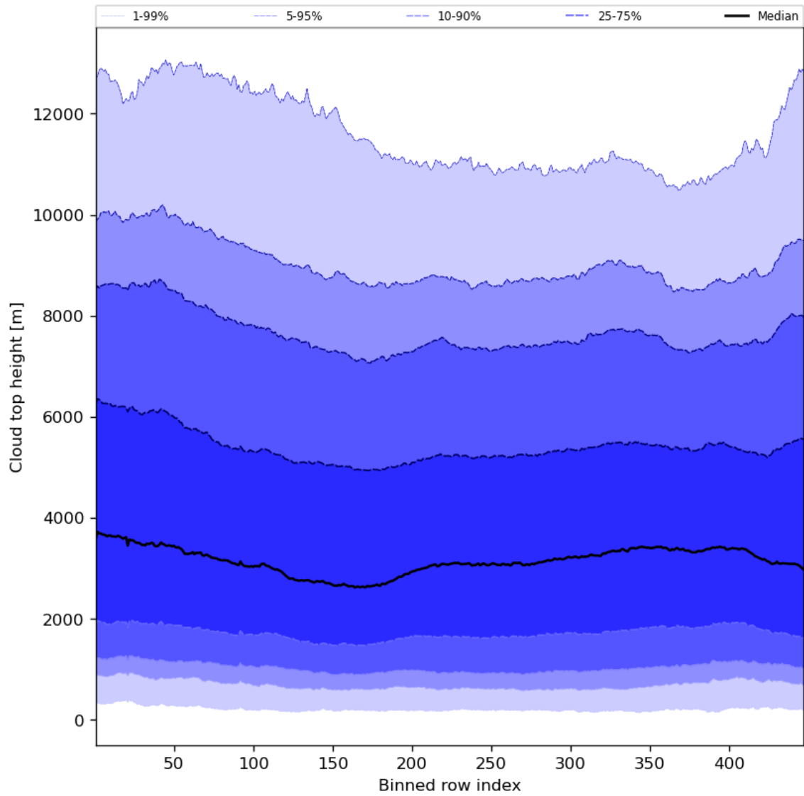
Figure 56: Along track statistics of “Cloud top height” for 2024-03-23 to 2024-03-25
