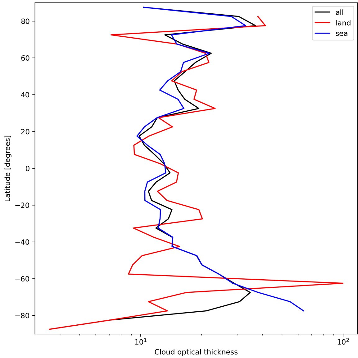
Figure 25: Zonal average of “Cloud optical thickness” for 2024-03-23 to 2024-03-25.
