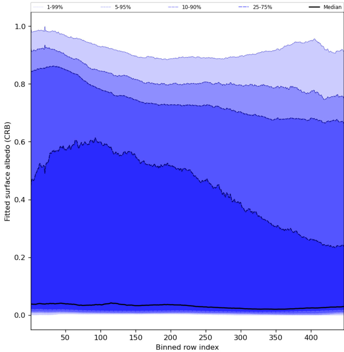
Figure 62: Along track statistics of “Fitted surface albedo (CRB)” for 2024-03-23 to 2024-03-25
