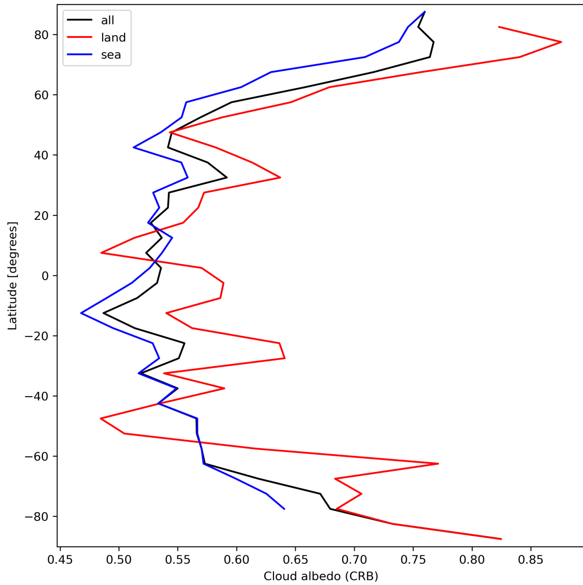
Figure 28: Zonal average of “Cloud albedo (CRB)” for 2024-03-23 to 2024-03-25.
