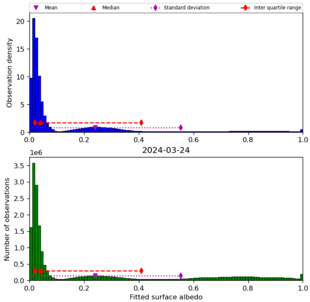
Figure 45: Histogram of “Fitted surface albedo” for 2024-03-23 to 2024-03-25
