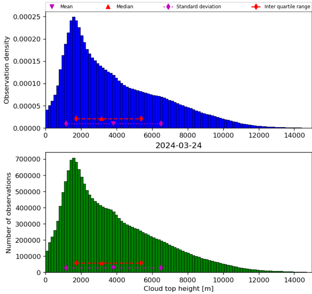
Figure 40: Histogram of “Cloud top height” for 2024-03-23 to 2024-03-25
