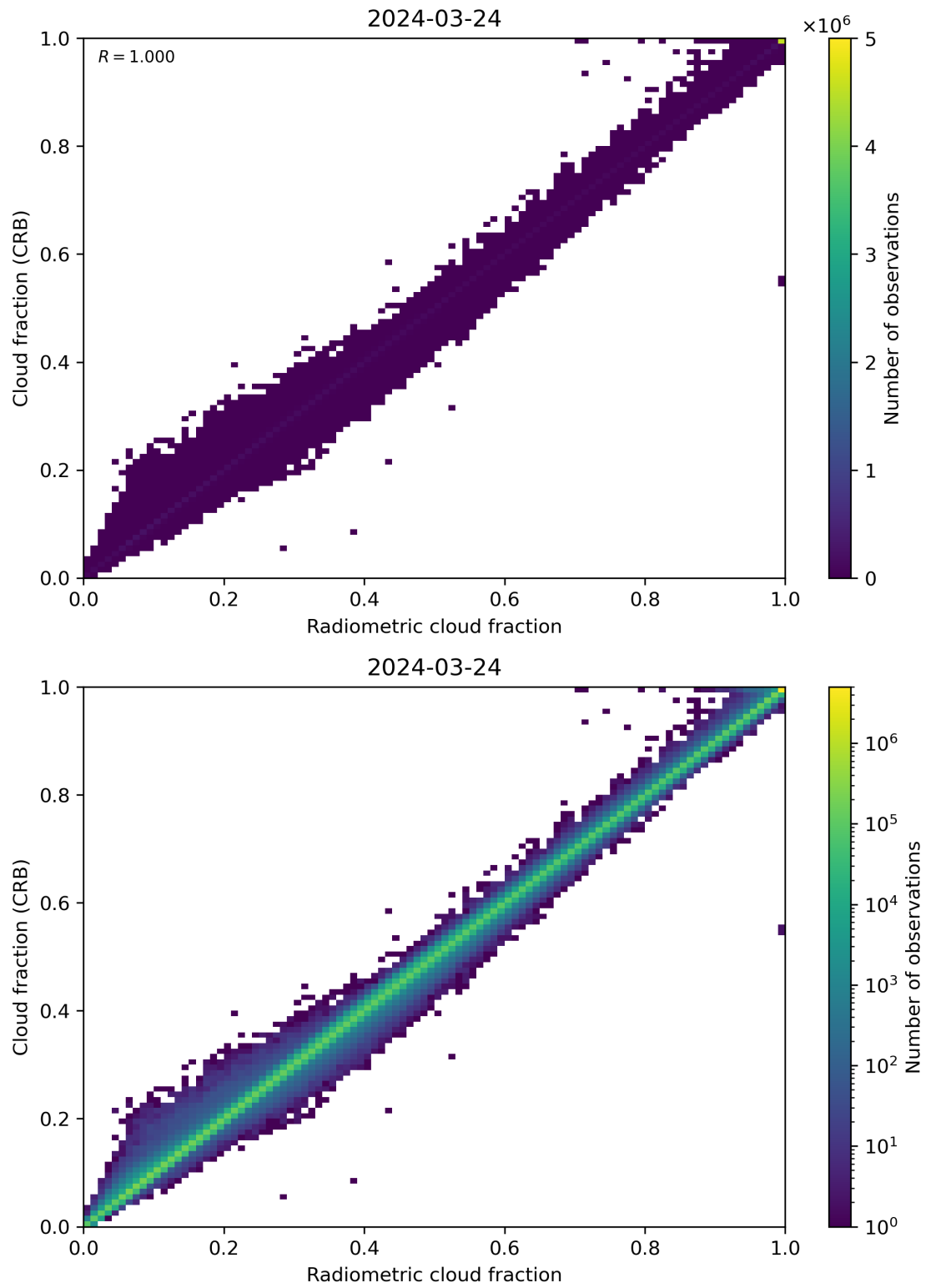
Figure 73: Scatter density plot of “Radiometric cloud fraction” against “Cloud fraction (CRB)” for 2024-03-23 to 2024-03-25.
