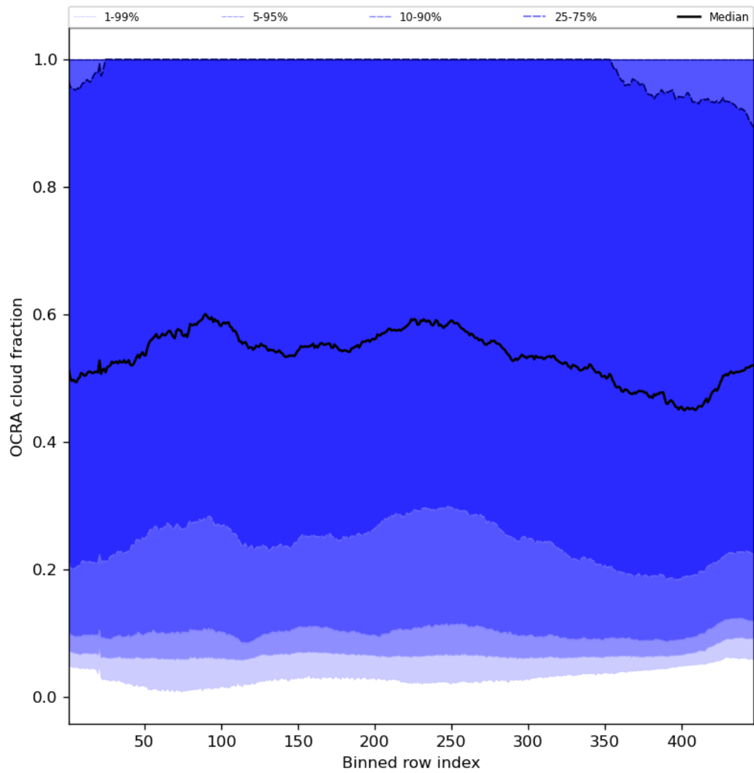
Figure 66: Along track statistics of “OCRA cloud fraction” for 2024-03-23 to 2024-03-25
