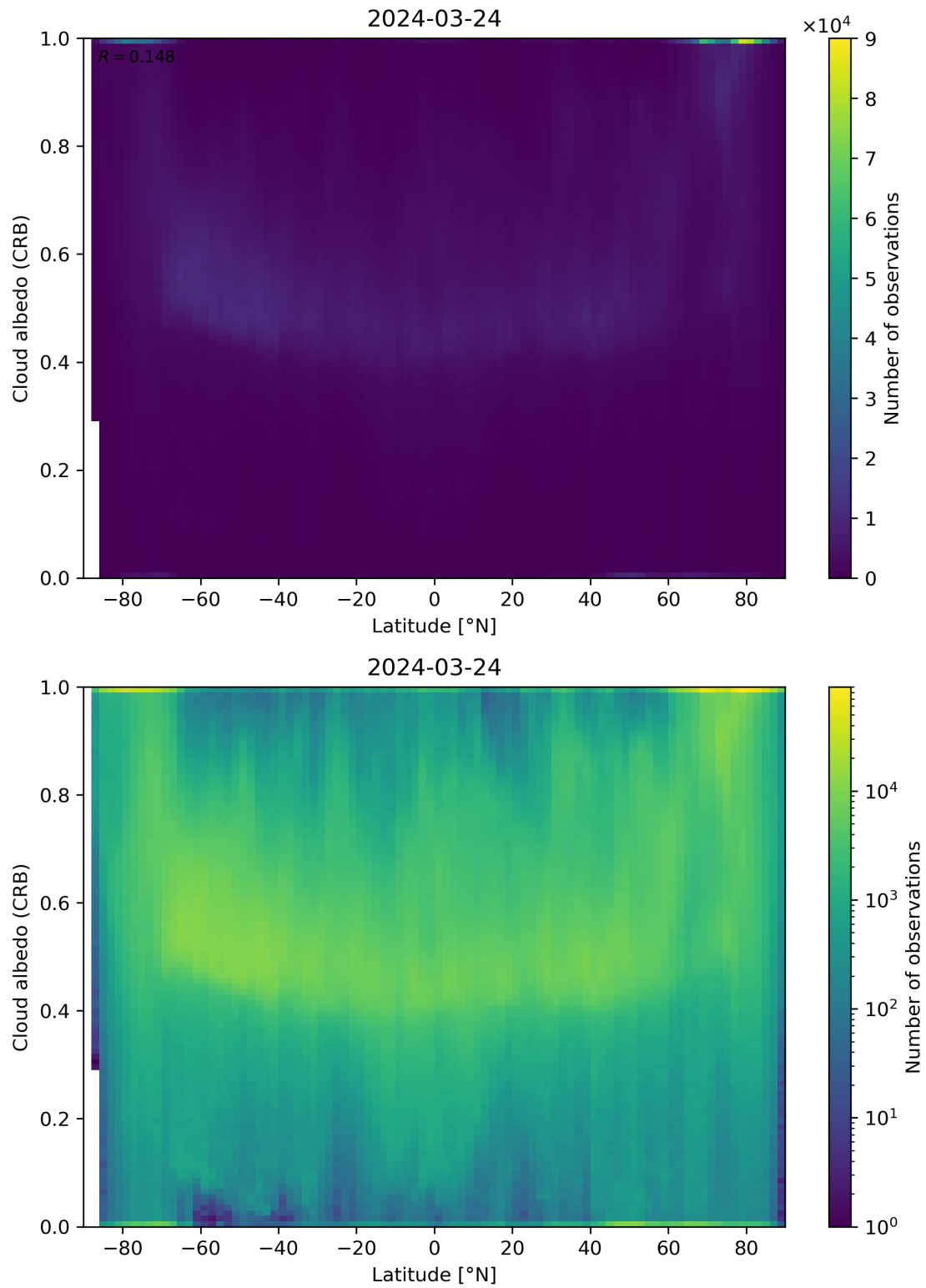
Figure 91: Scatter density plot of “Latitude” against “Cloud albedo (CRB)” for 2024-03-23 to 2024-03-25.
