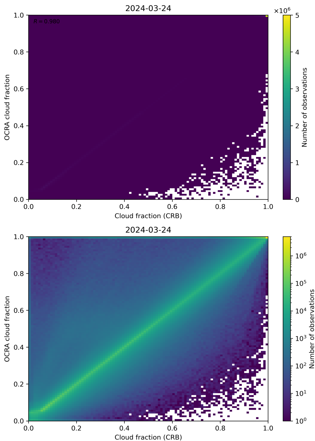
Figure 78: Scatter density plot of “Cloud fraction (CRB)” against “OCRA cloud fraction” for 2024-03-23 to 2024-03-25.
