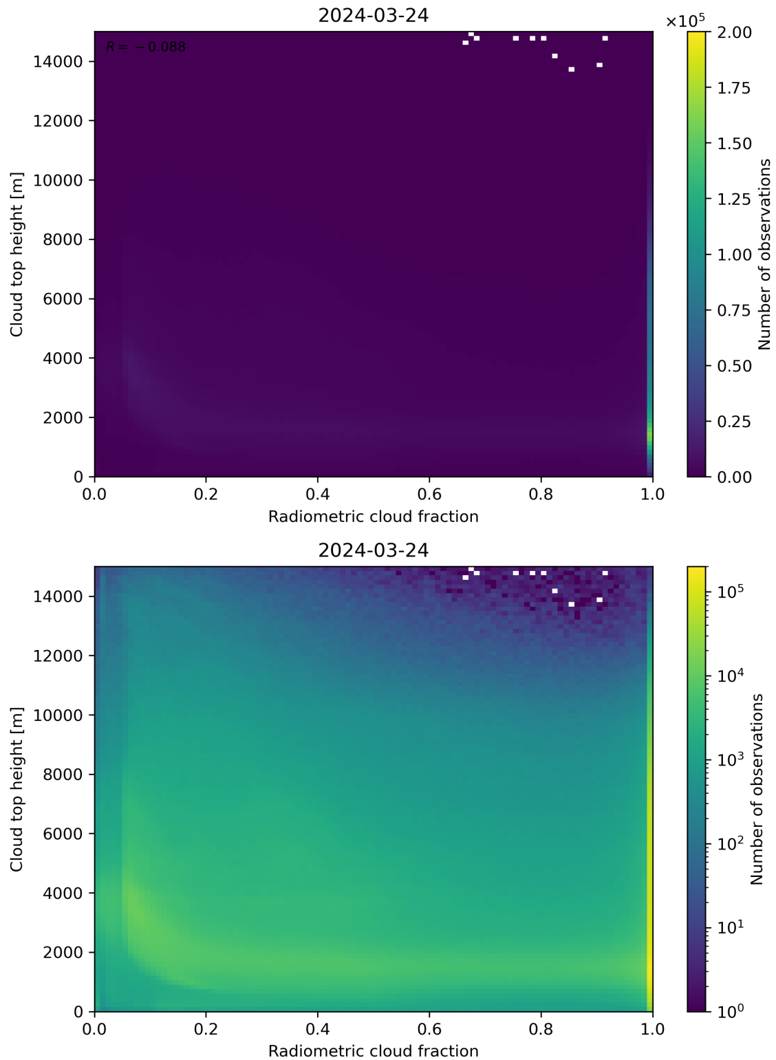
Figure 76: Scatter density plot of “Radiometric cloud fraction” against “Cloud top height” for 2024-03-23 to 2024-03-25.
