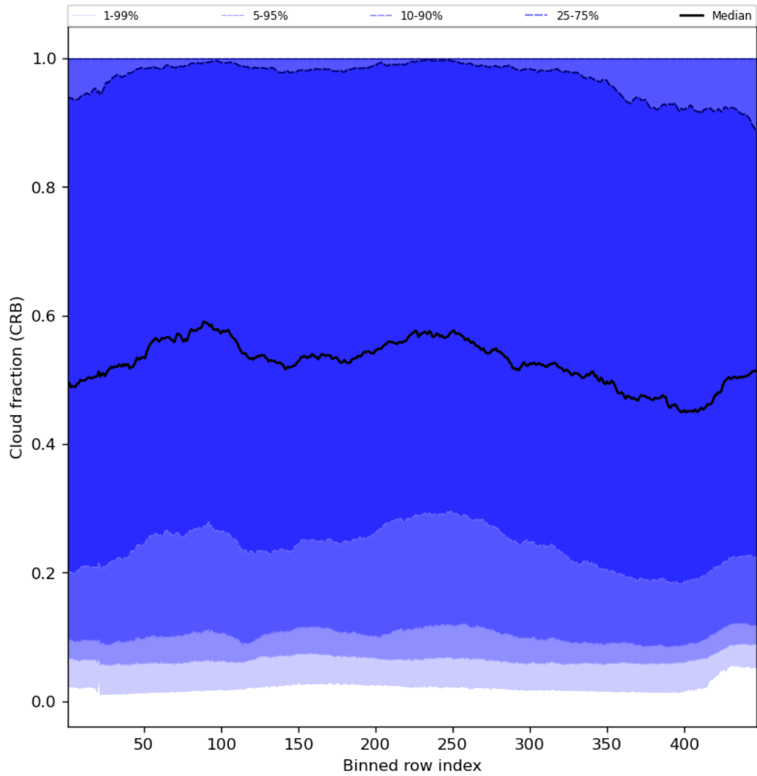
Figure 58: Along track statistics of “Cloud fraction (CRB)” for 2024-03-23 to 2024-03-25
