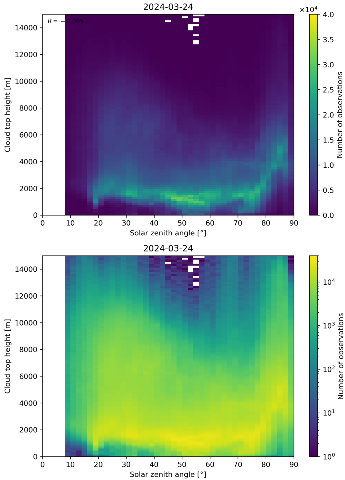
Figure 104: Scatter density plot of “Solar zenith angle” against “Cloud top height” for 2024-03-23 to 2024-03-25.
