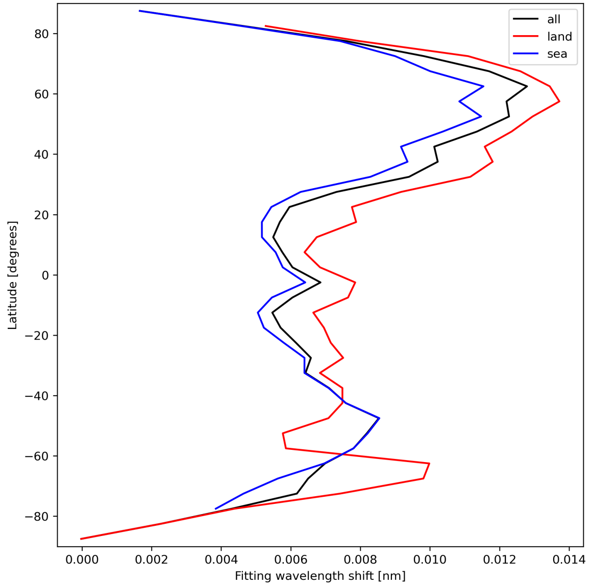
Figure 33: Zonal average of “Fitting wavelength shift” for 2024-03-23 to 2024-03-25.
