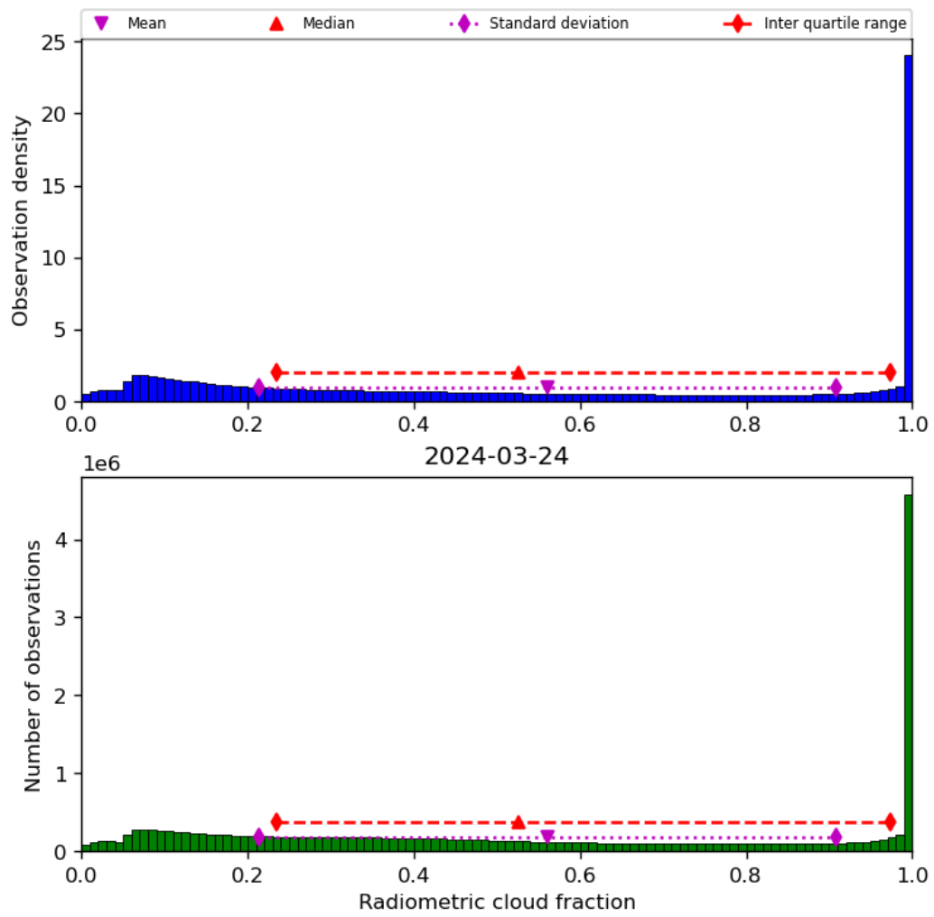
Figure 39: Histogram of “Radiometric cloud fraction” for 2024-03-23 to 2024-03-25
