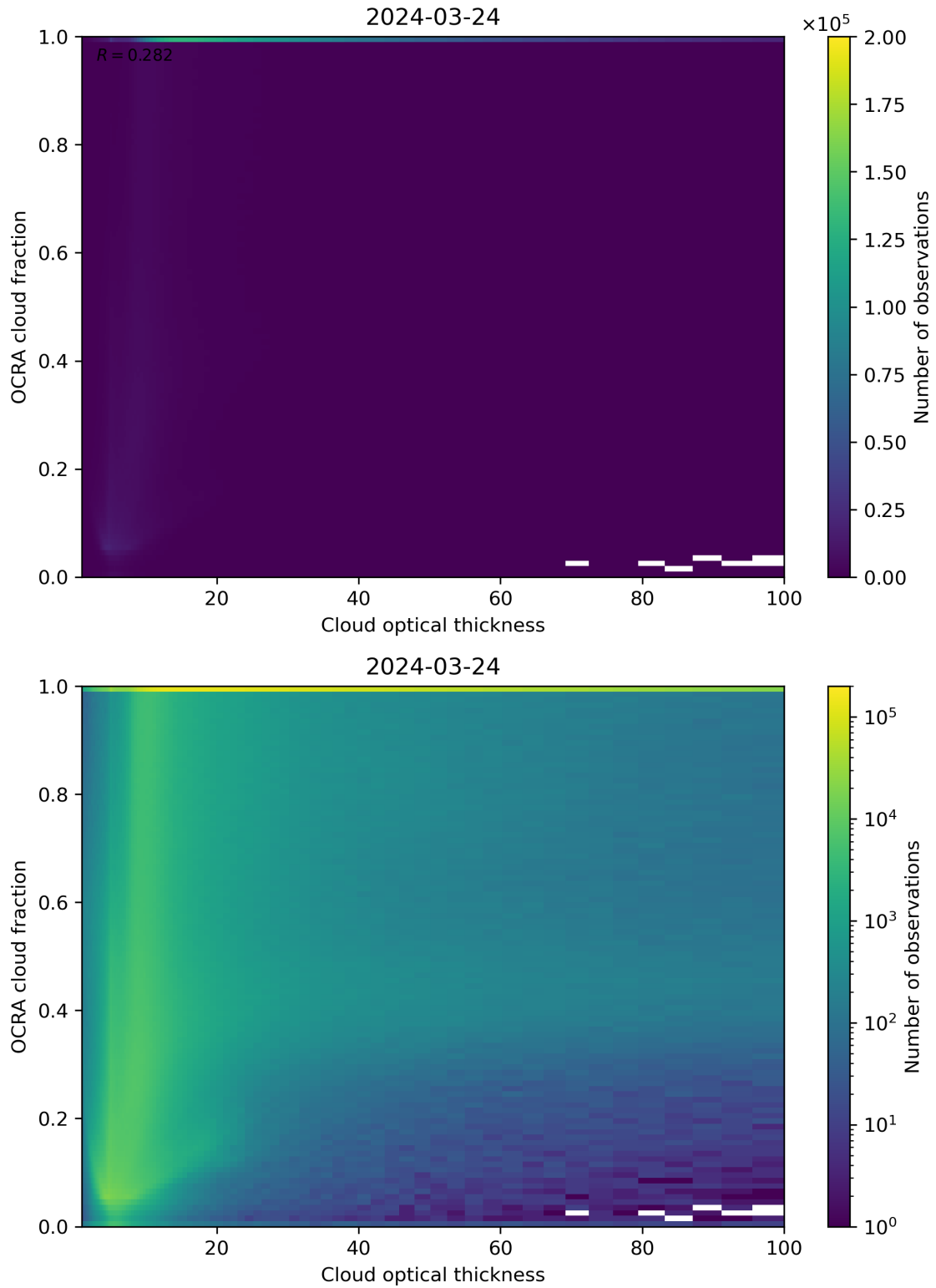
Figure 83: Scatter density plot of “Cloud optical thickness” against “OCRA cloud fraction” for 2024-03-23 to 2024-03-25.
