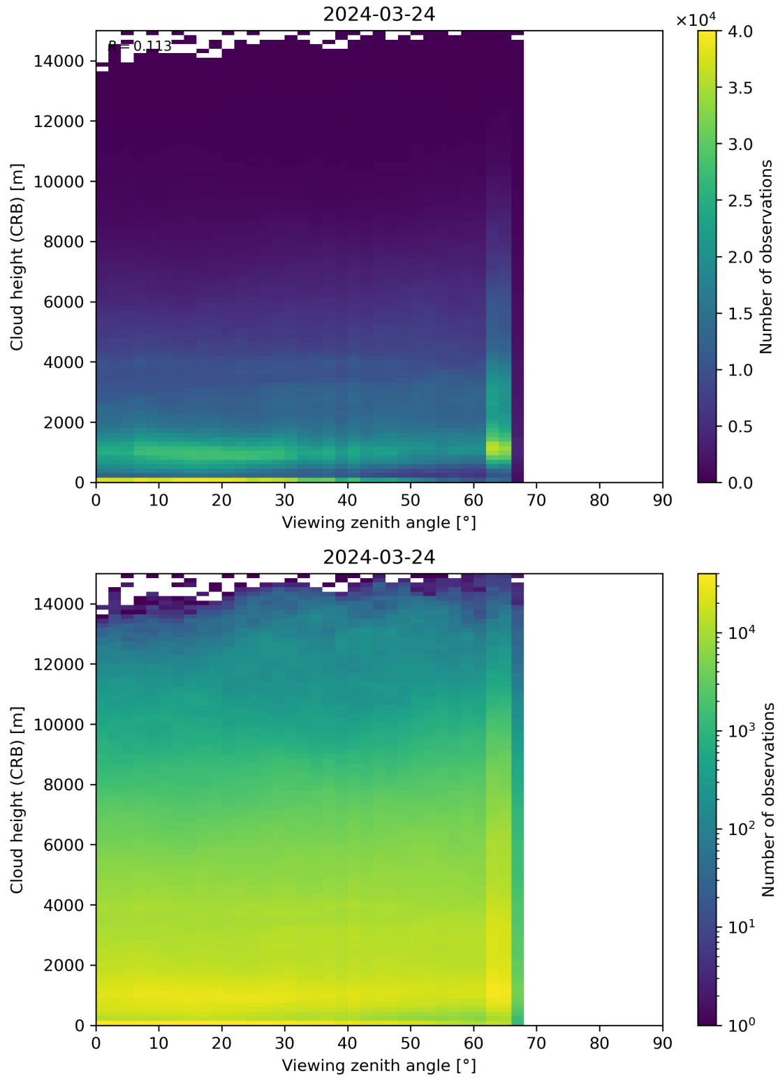
Figure 110: Scatter density plot of “Viewing zenith angle” against “Cloud height (CRB)” for 2024-03-23 to 2024-03-25.
