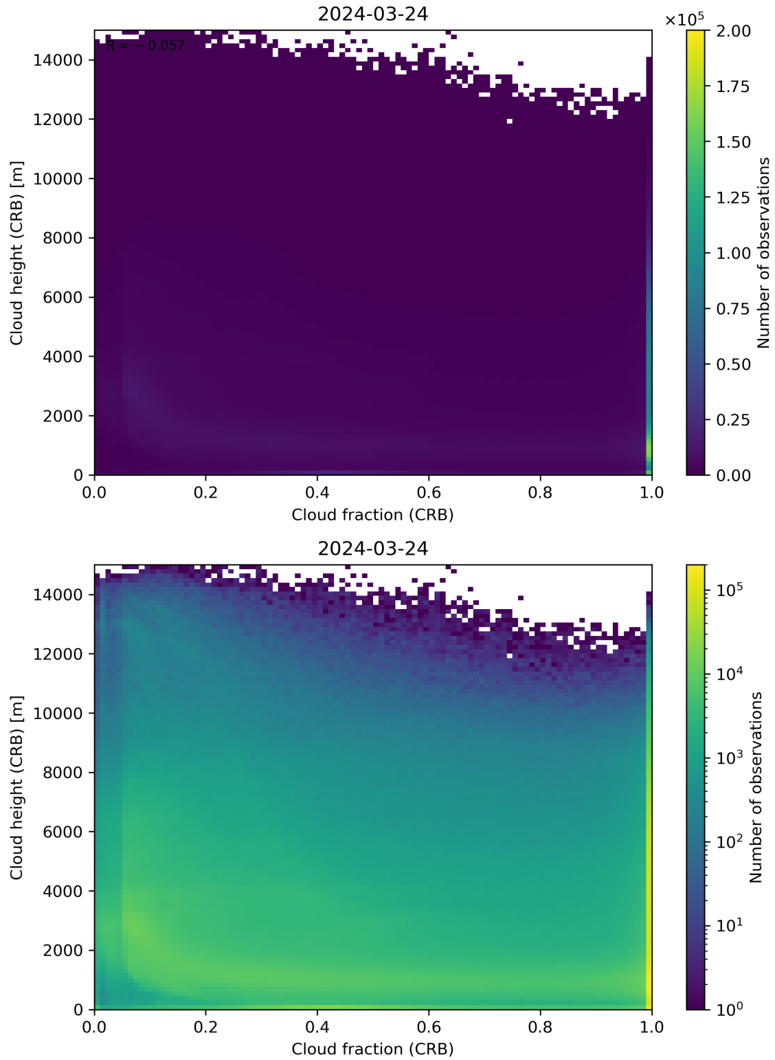
Figure 79: Scatter density plot of “Cloud fraction (CRB)” against “Cloud height (CRB)” for 2024-03-23 to 2024-03-25.
