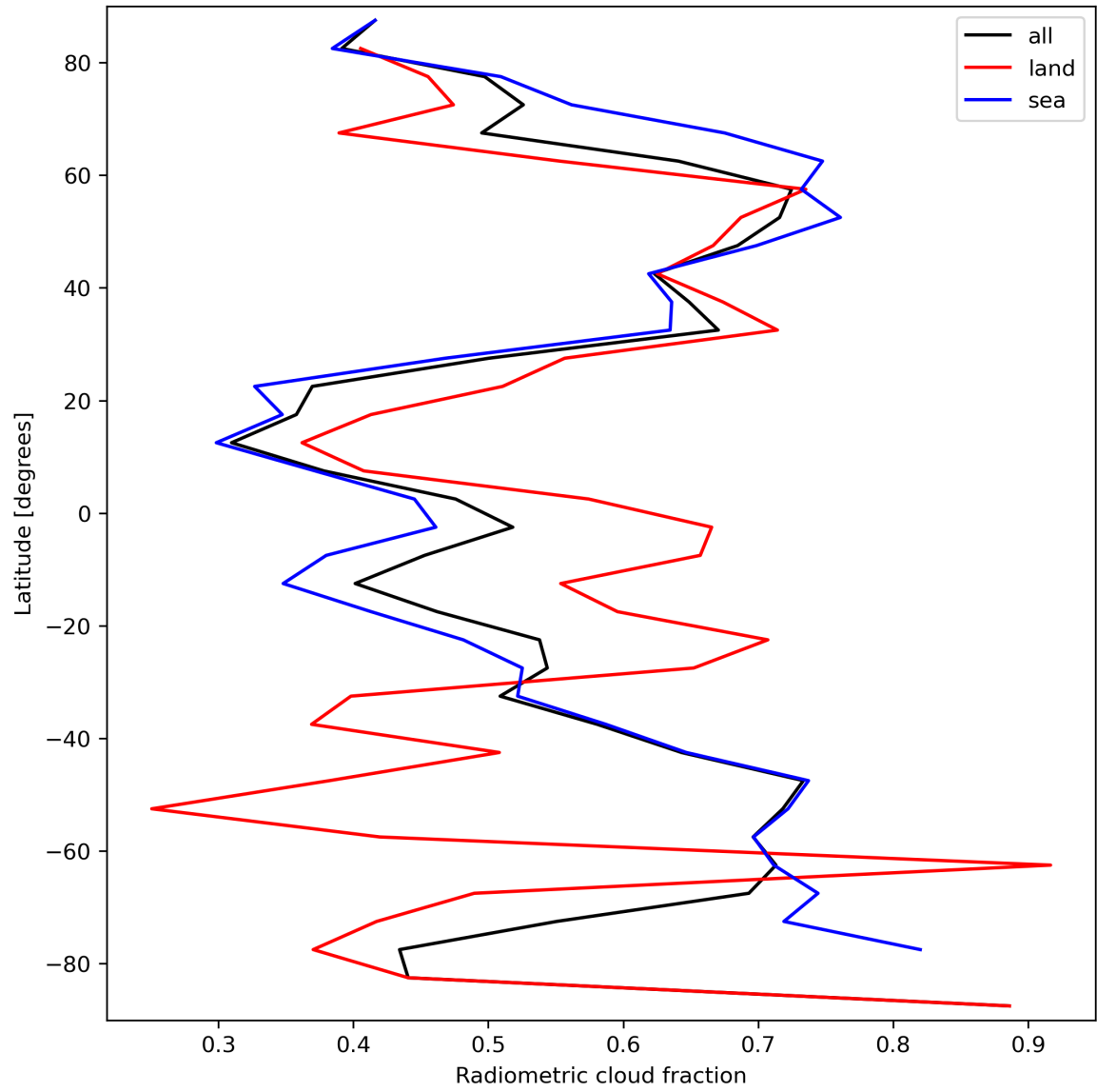
Figure 23: Zonal average of “Radiometric cloud fraction” for 2024-03-23 to 2024-03-25.
