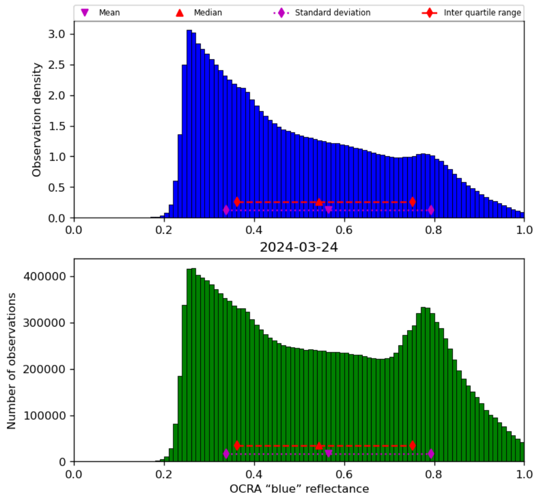
Figure 51: Histogram of “OCRA “blue” reflectance” for 2024-03-23 to 2024-03-25
