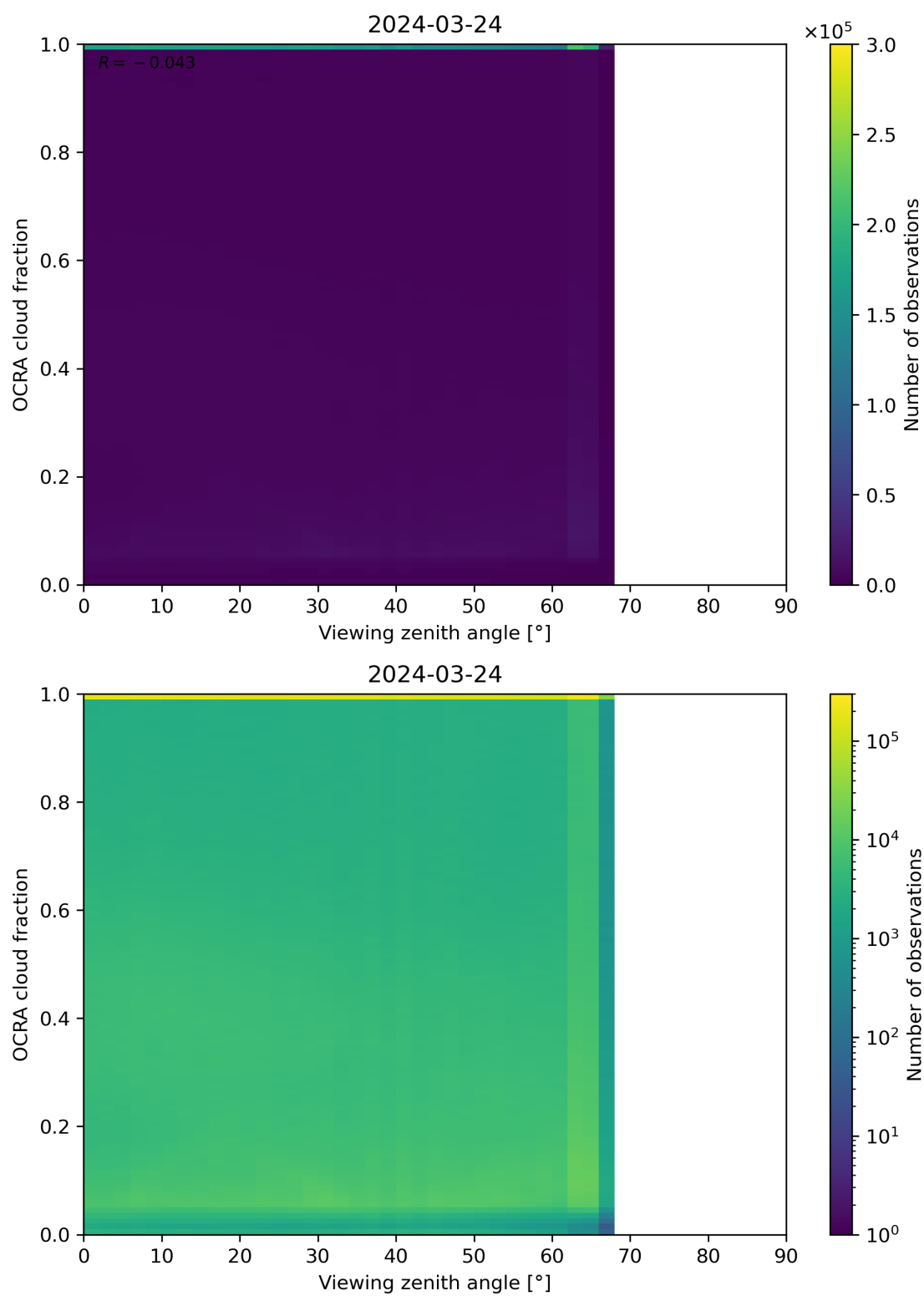
Figure 108: Scatter density plot of “Viewing zenith angle” against “OCRA cloud fraction” for 2024-03-23 to 2024-03-25.
