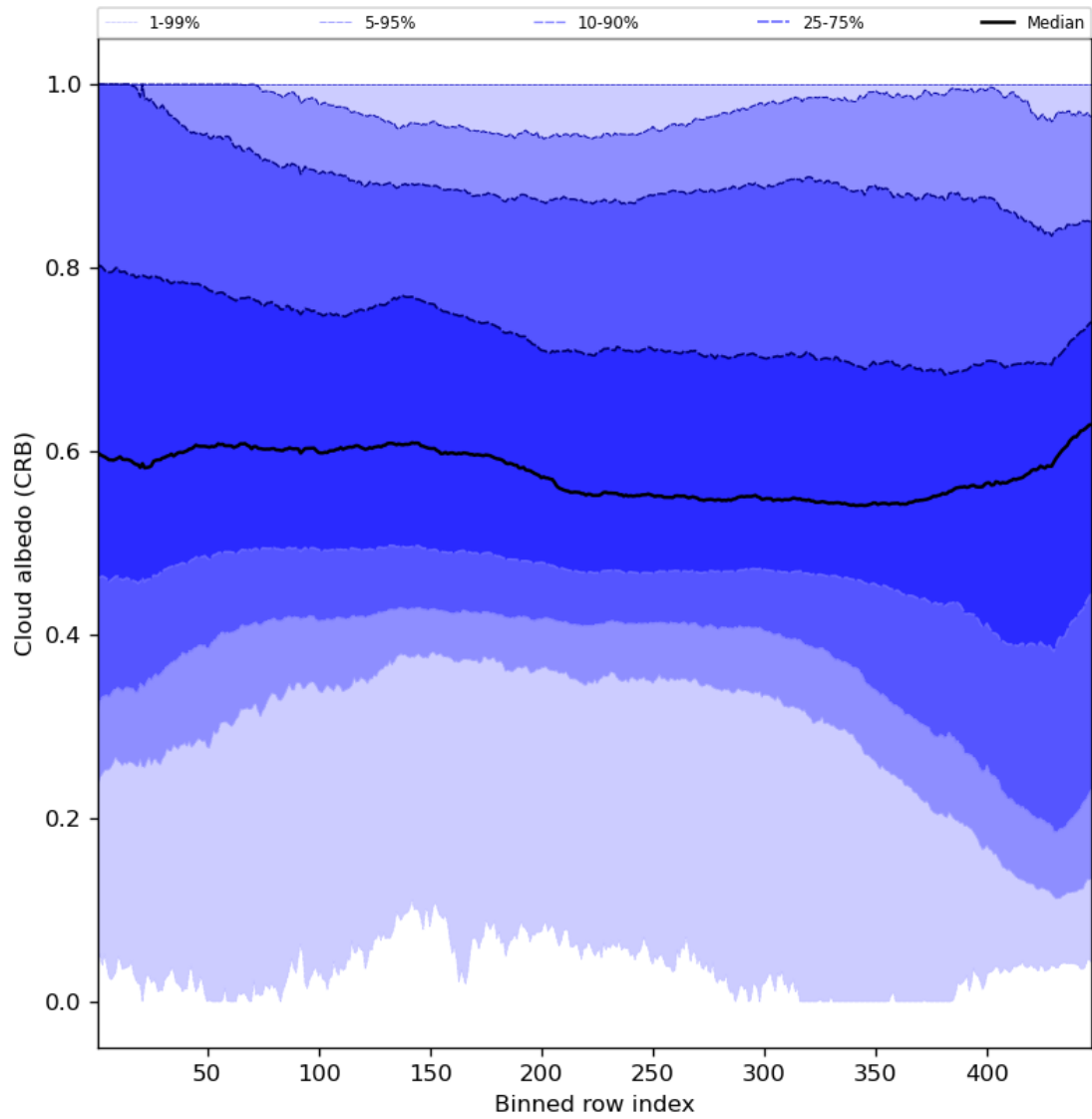
Figure 60: Along track statistics of “Cloud albedo (CRB)” for 2024-03-23 to 2024-03-25
