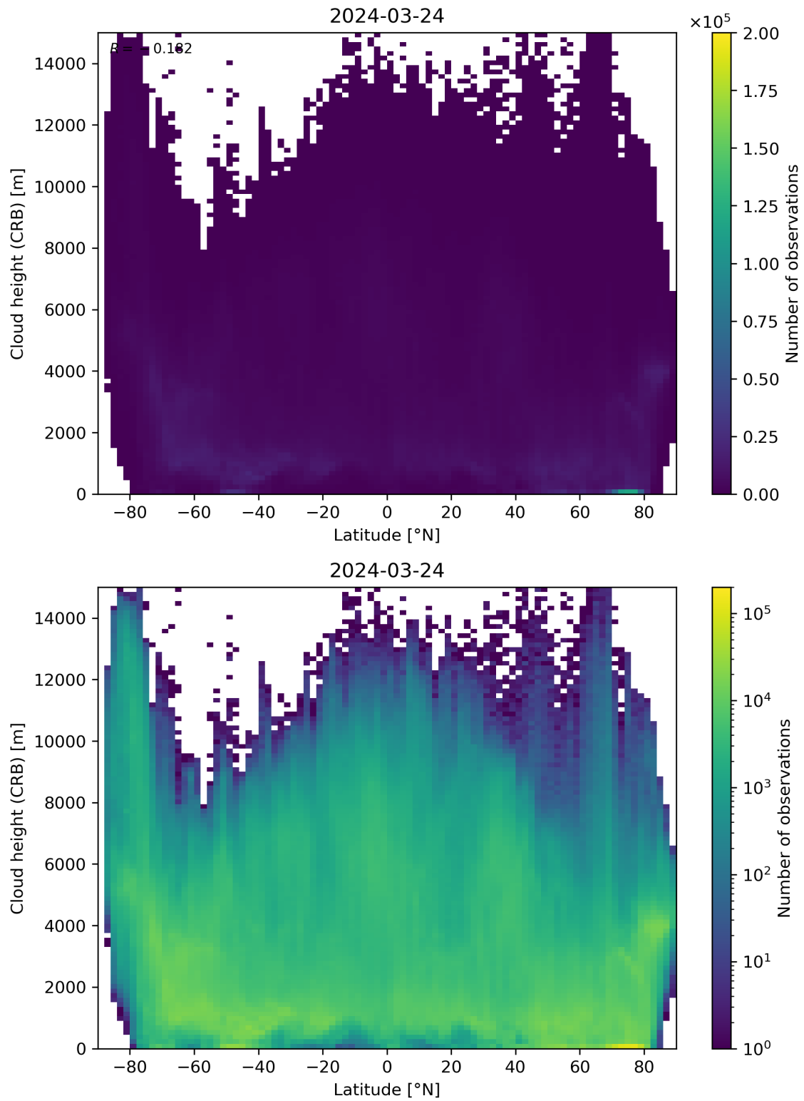
Figure 95: Scatter density plot of “Latitude” against “Cloud height (CRB)” for 2024-03-23 to 2024-03-25.
