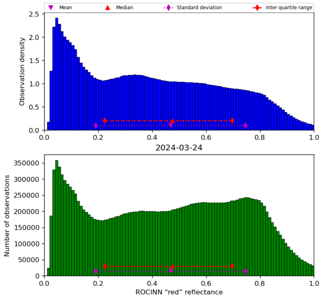
Figure 53: Histogram of “ROCINN “red” reflectance” for 2024-03-23 to 2024-03-25
