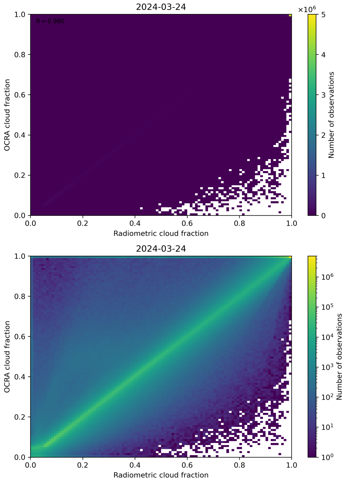
Figure 72: Scatter density plot of “Radiometric cloud fraction” against “OCRA cloud fraction” for 2024-03-23 to 2024-03-25.
