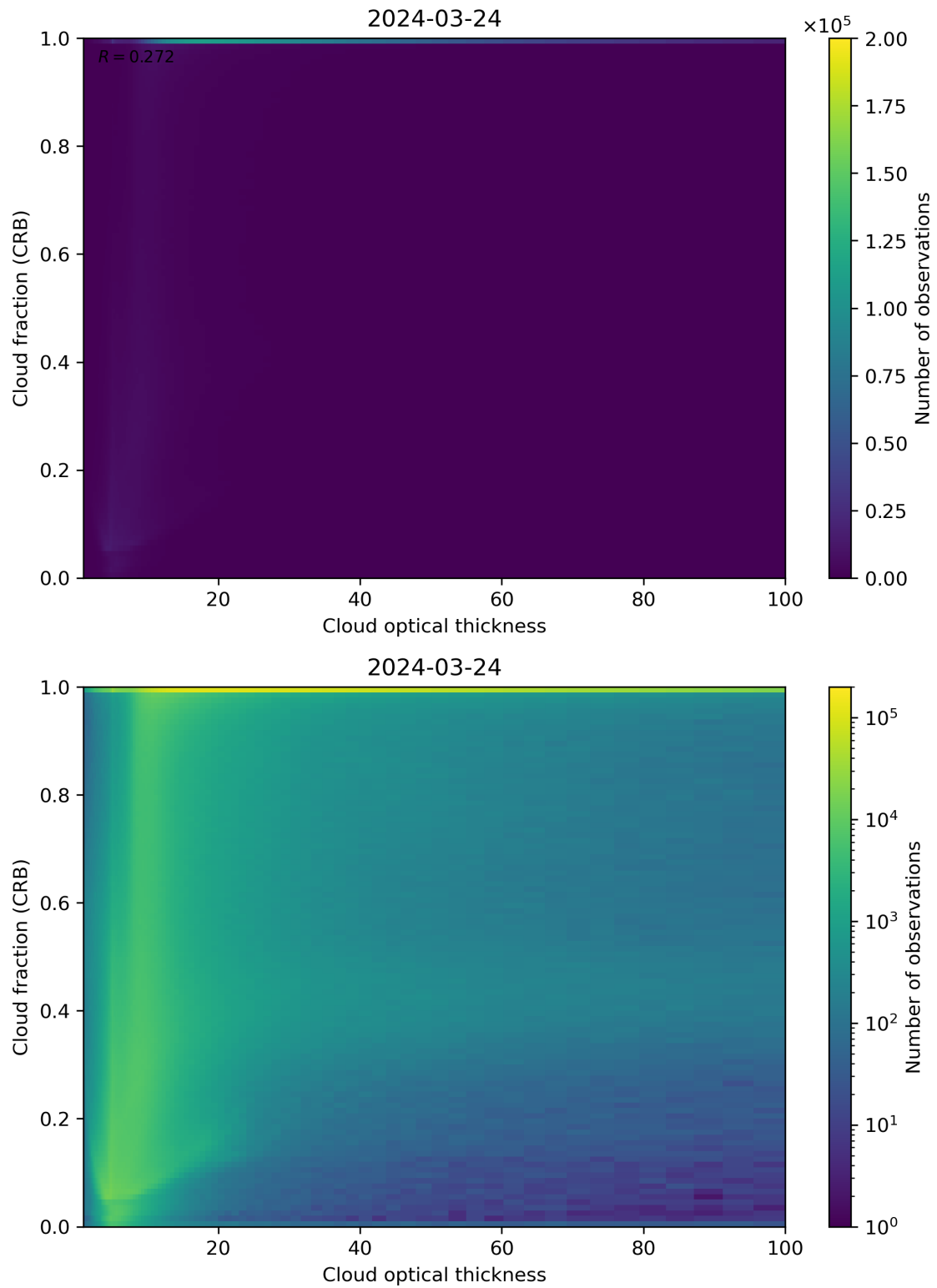
Figure 84: Scatter density plot of “Cloud optical thickness” against “Cloud fraction (CRB)” for 2024-03-23 to 2024-03-25.
