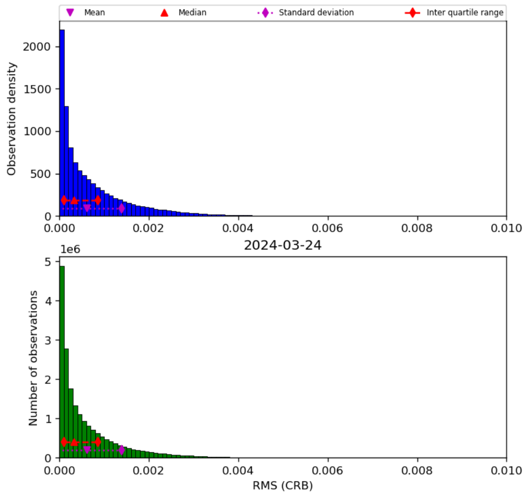
Figure 48: Histogram of “RMS (CRB)” for 2024-03-23 to 2024-03-25
