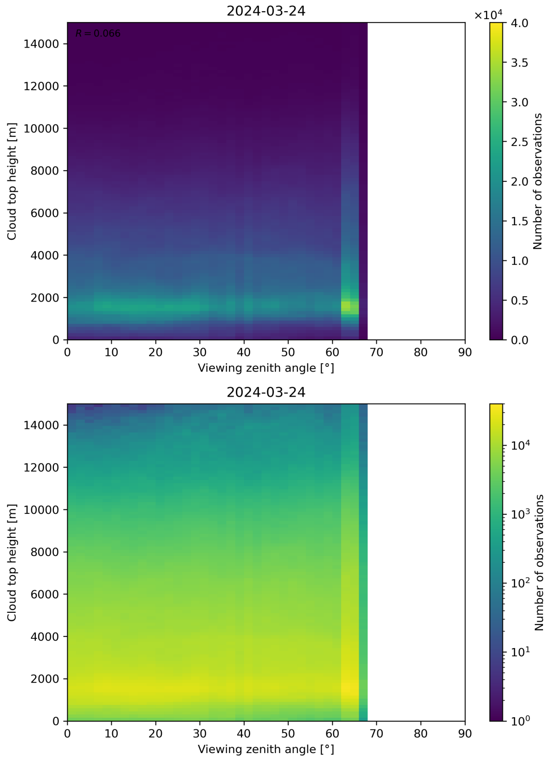
Figure 112: Scatter density plot of “Viewing zenith angle” against “Cloud top height” for 2024-03-23 to 2024-03-25.
