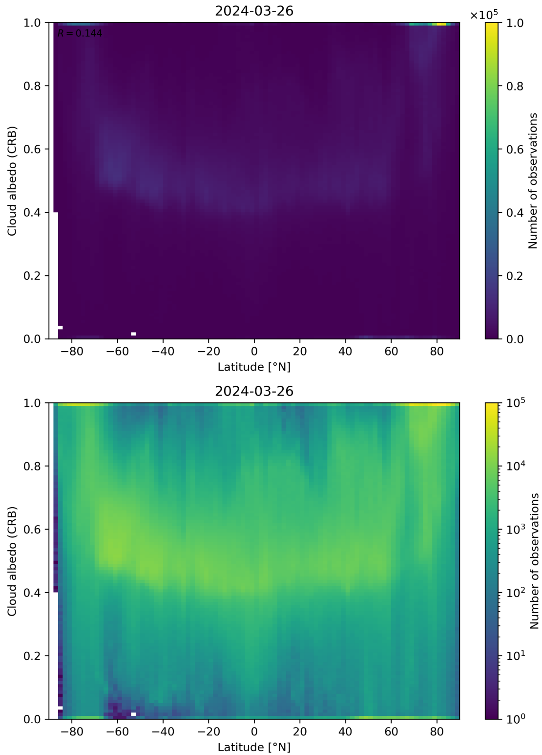
Figure 91: Scatter density plot of “Latitude” against “Cloud albedo (CRB)” for 2024-03-25 to 2024-03-27.
