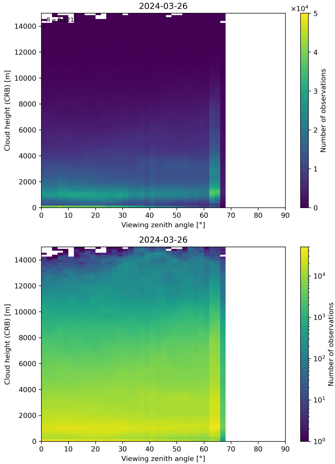
Figure 110: Scatter density plot of “Viewing zenith angle” against “Cloud height (CRB)” for 2024-03-25 to 2024-03-27.
