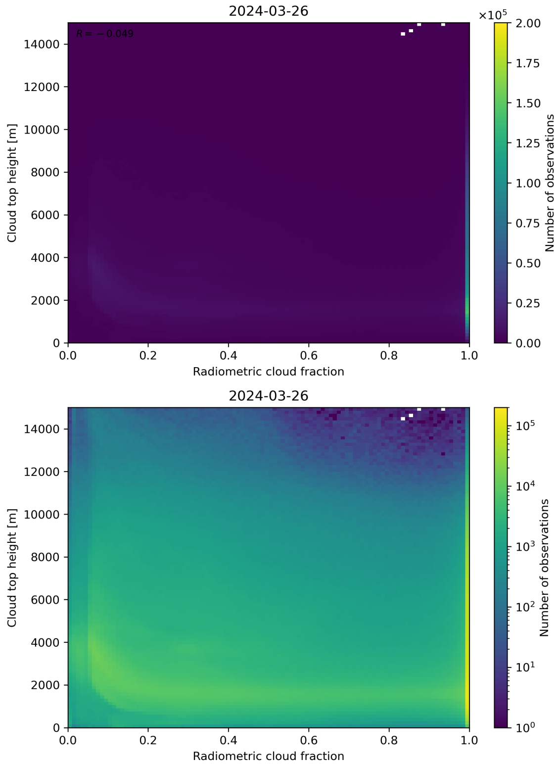
Figure 76: Scatter density plot of “Radiometric cloud fraction” against “Cloud top height” for 2024-03-25 to 2024-03-27.
