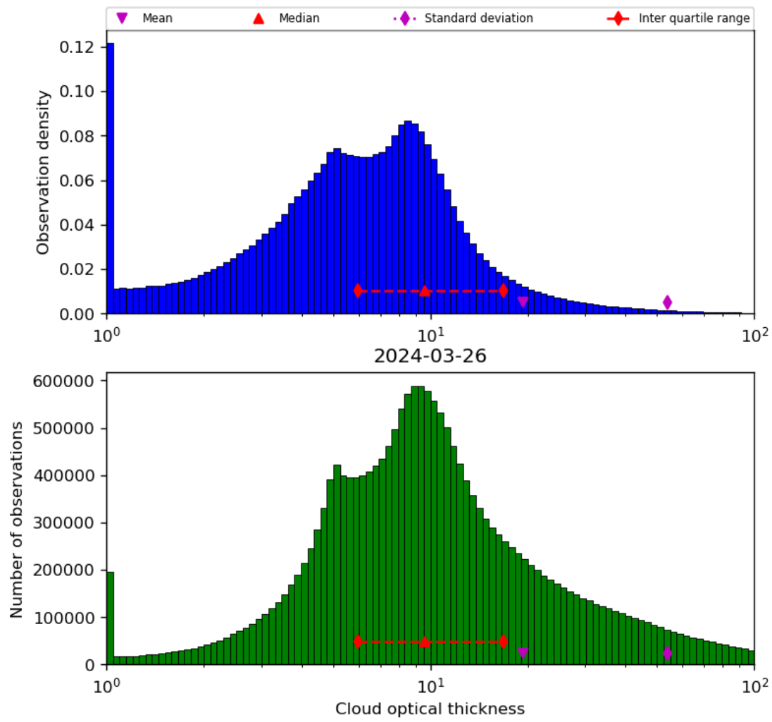
Figure 41: Histogram of “Cloud optical thickness” for 2024-03-25 to 2024-03-27
