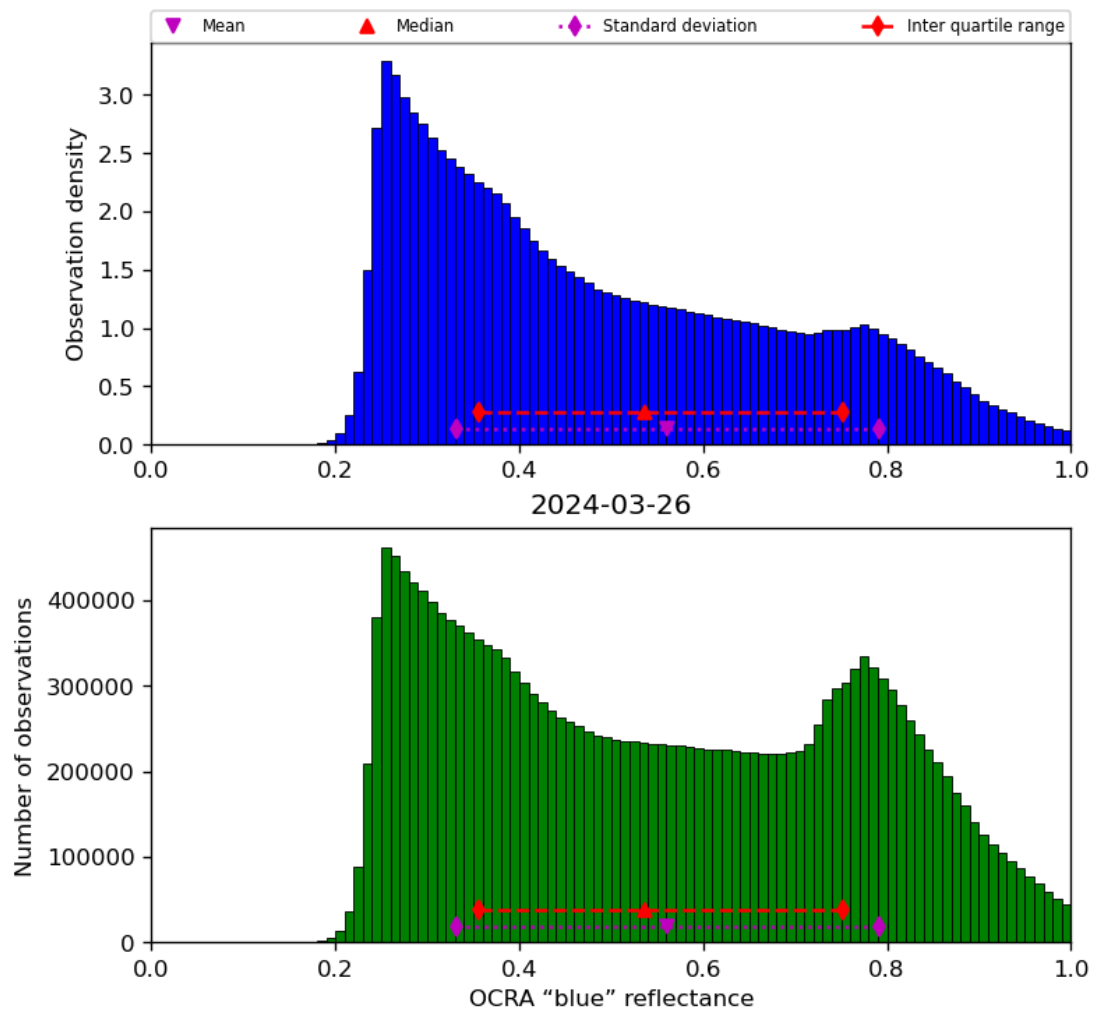
Figure 51: Histogram of “OCRA “blue” reflectance” for 2024-03-25 to 2024-03-27
