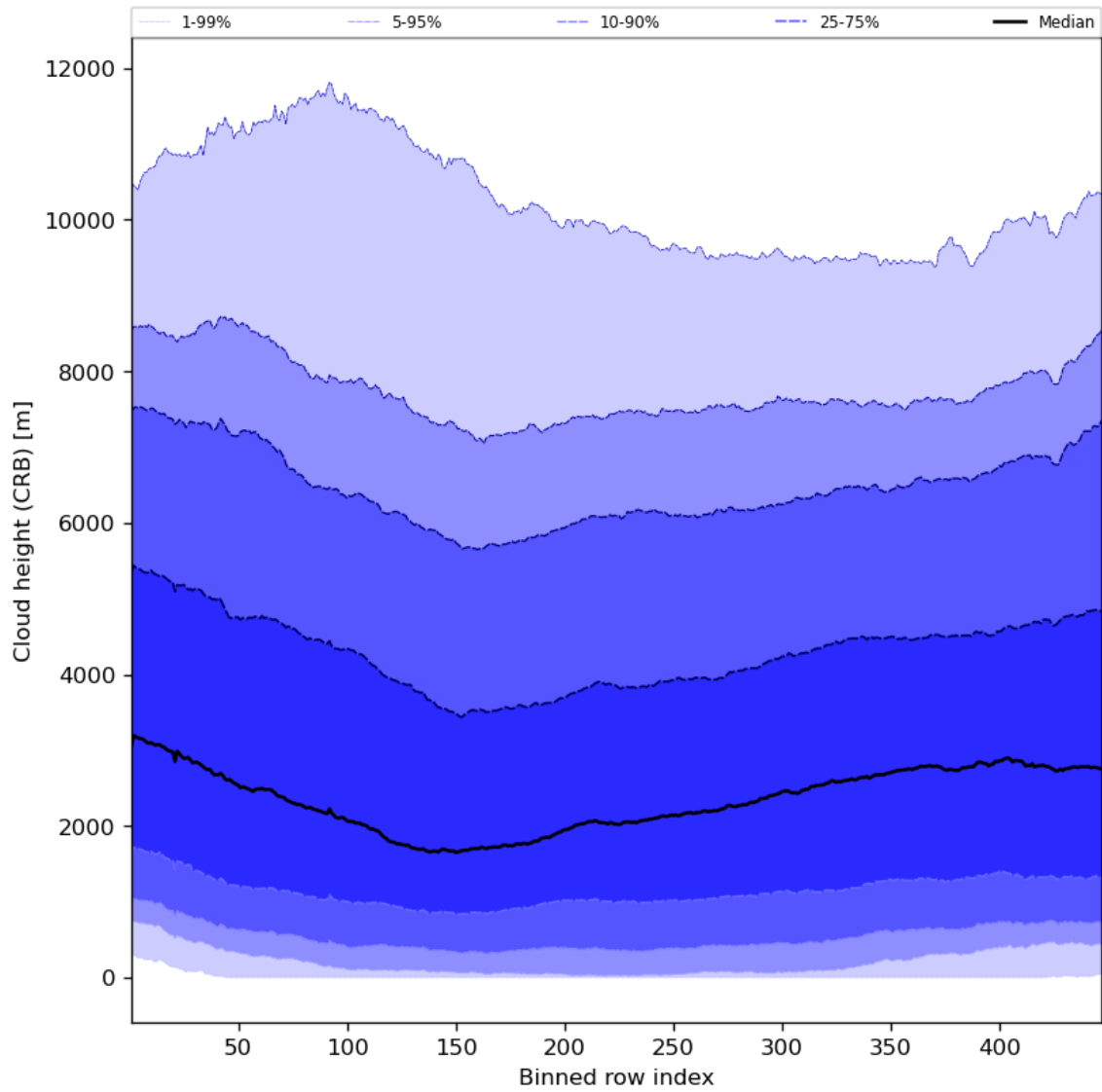
Figure 59: Along track statistics of “Cloud height (CRB)” for 2024-03-25 to 2024-03-27
