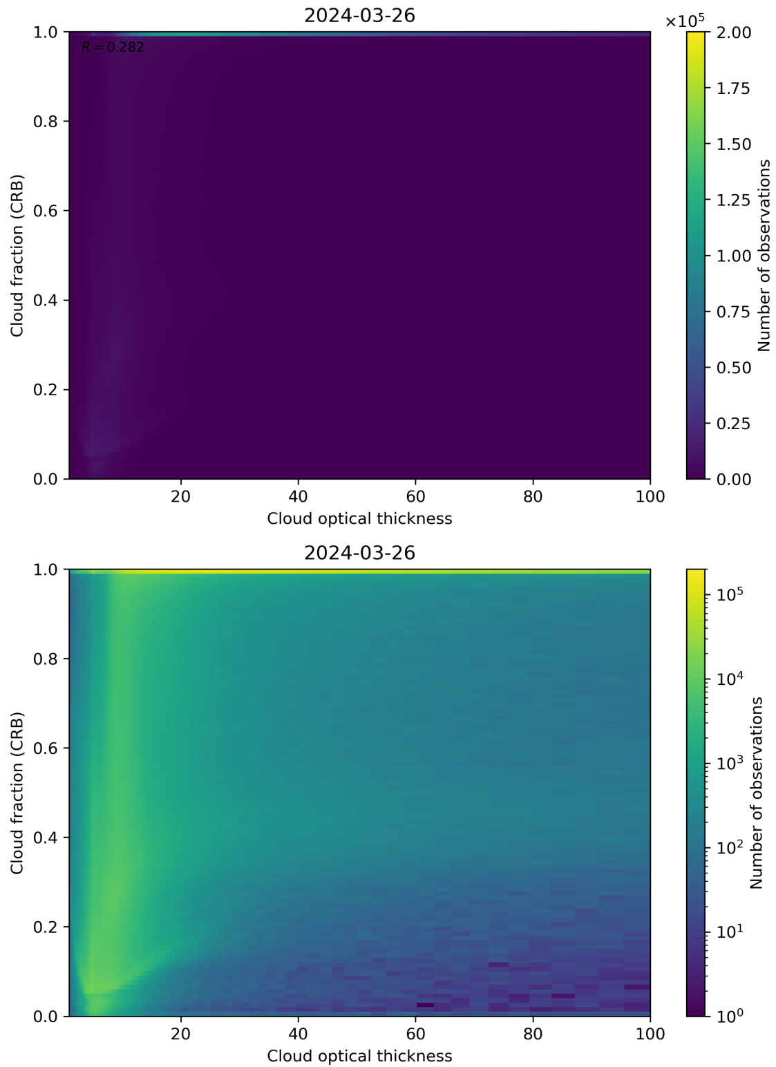
Figure 84: Scatter density plot of “Cloud optical thickness” against “Cloud fraction (CRB)” for 2024-03-25 to 2024-03-27.
