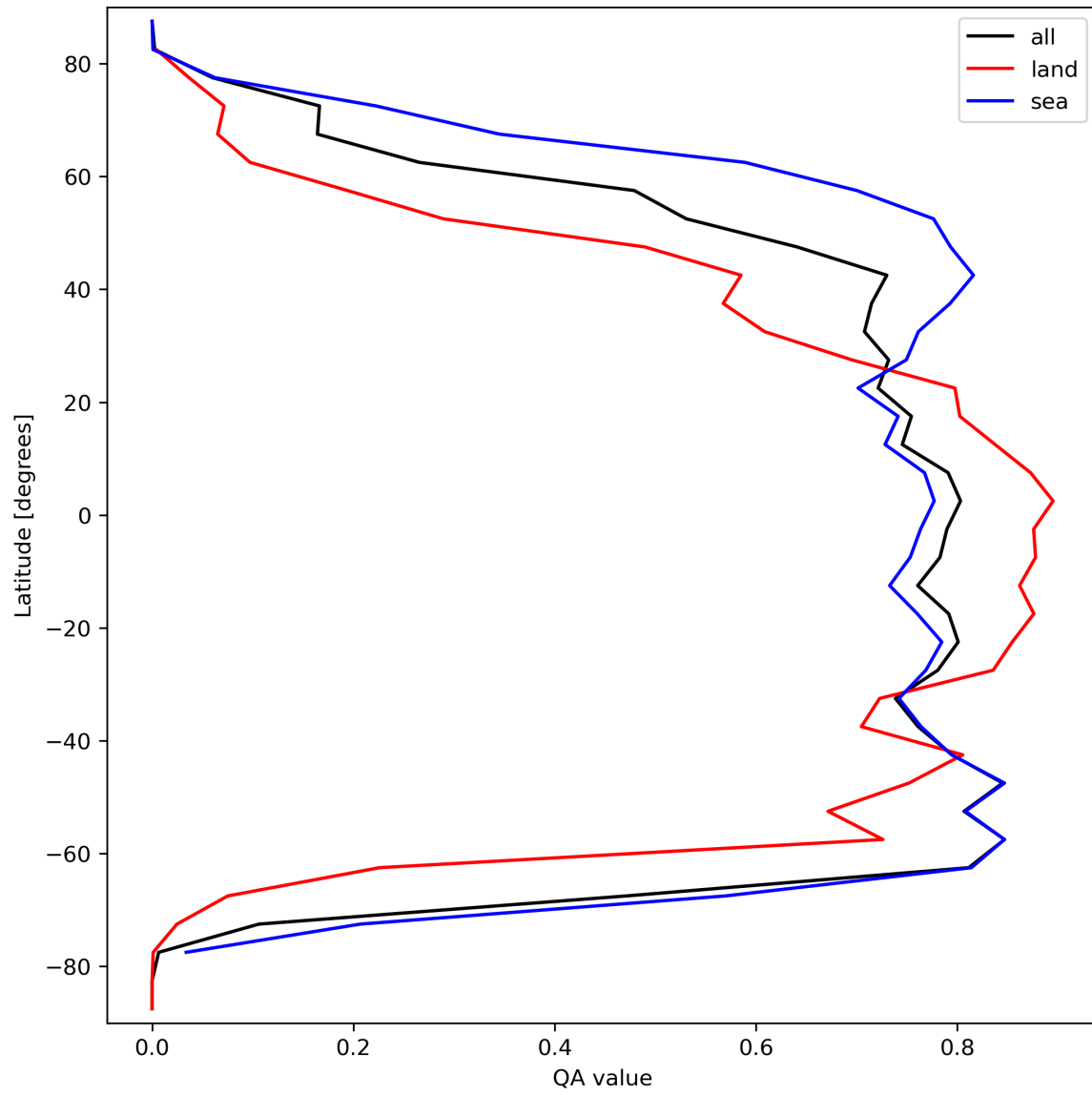
Figure 22: Zonal average of “QA value” for 2024-03-25 to 2024-03-27.
