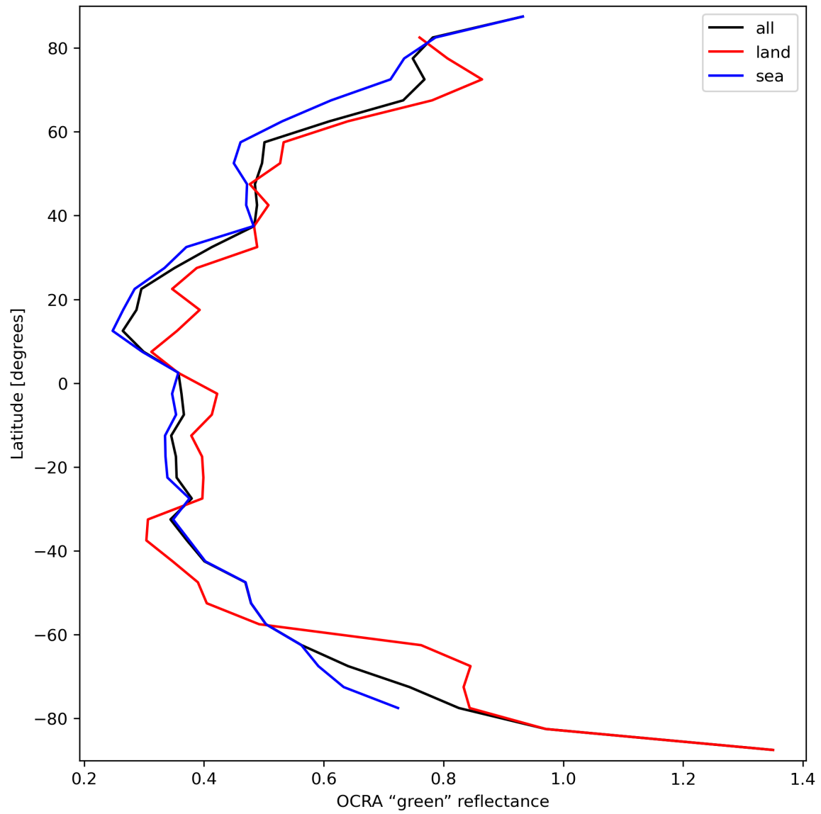
Figure 36: Zonal average of “OCRA “green” reflectance” for 2024-03-25 to 2024-03-27.
