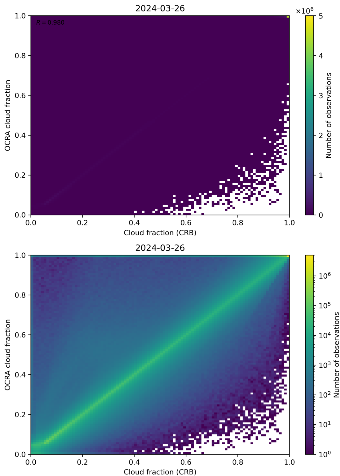
Figure 78: Scatter density plot of “Cloud fraction (CRB)” against “OCRA cloud fraction” for 2024-03-25 to 2024-03-27.
