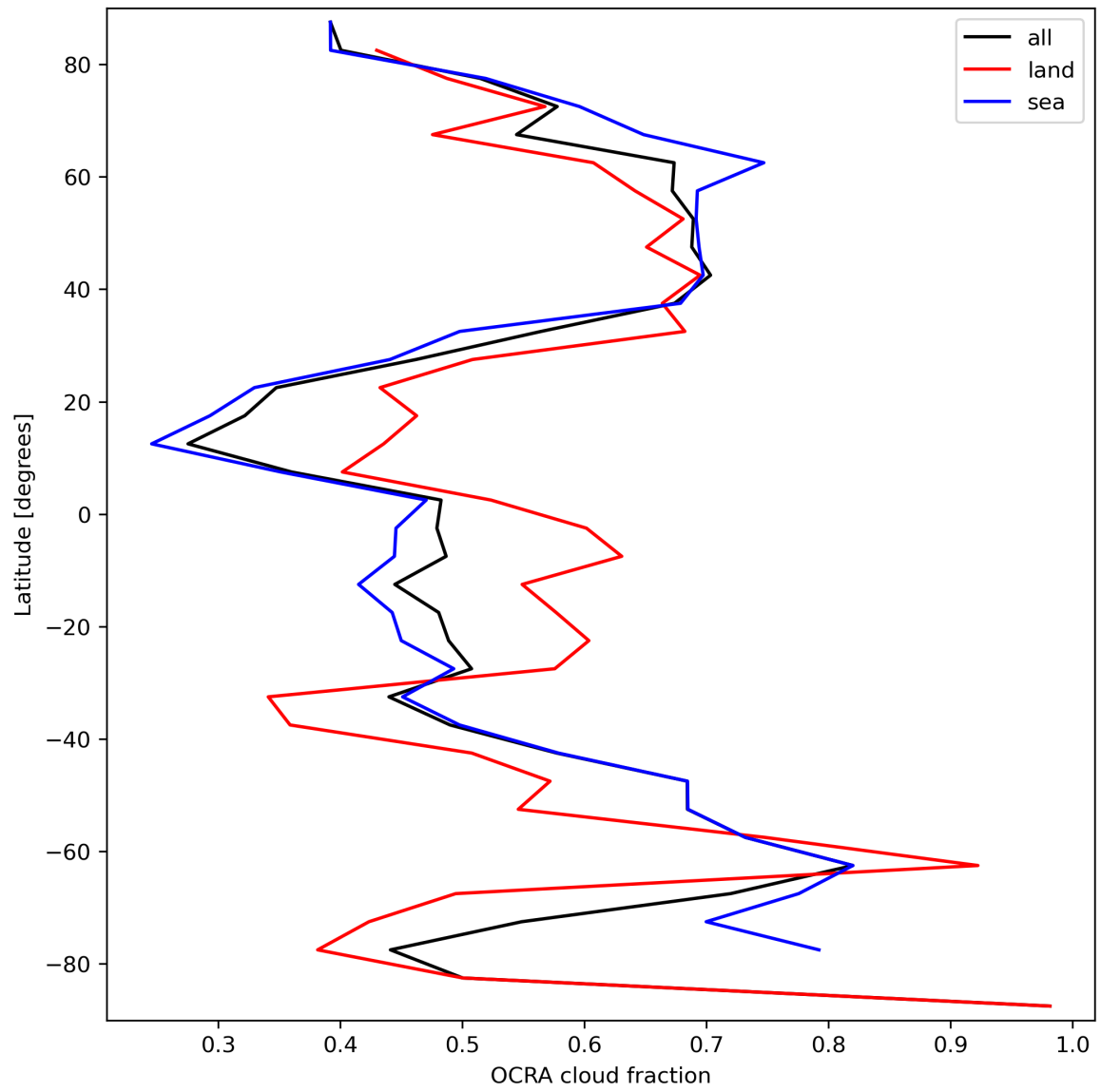
Figure 34: Zonal average of “OCRA cloud fraction” for 2024-03-25 to 2024-03-27.
