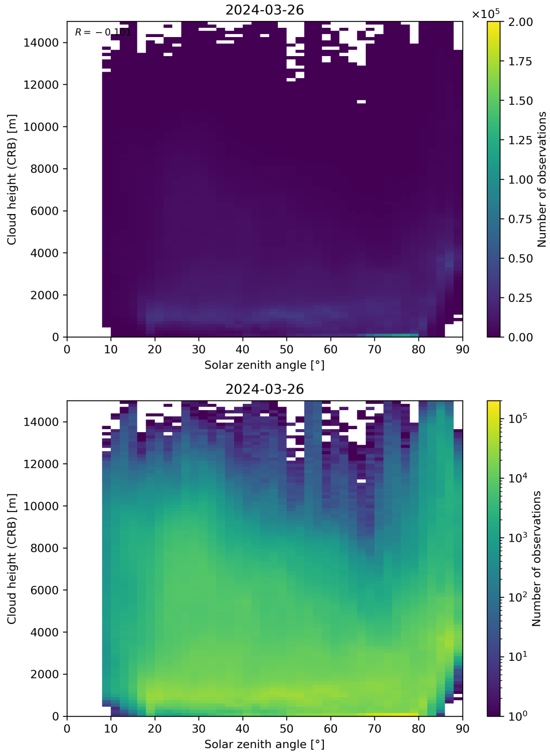
Figure 102: Scatter density plot of “Solar zenith angle” against “Cloud height (CRB)” for 2024-03-25 to 2024-03-27.
