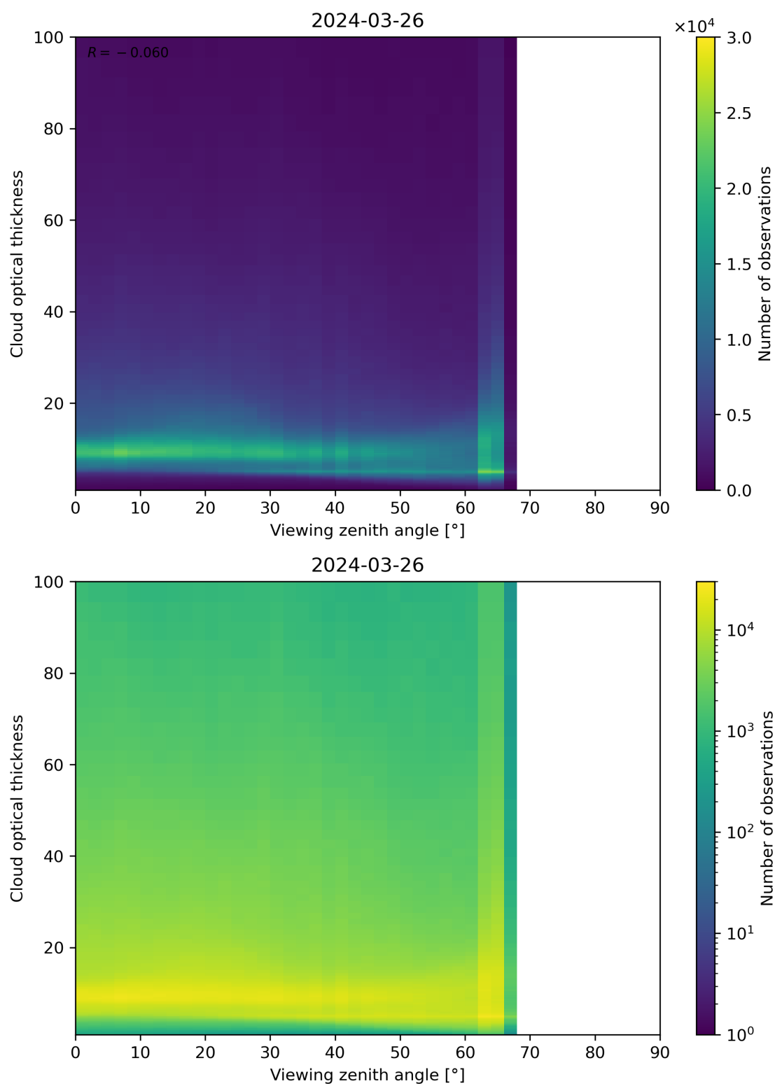
Figure 111: Scatter density plot of “Viewing zenith angle” against “Cloud optical thickness” for 2024-03-25 to 2024-03-27.
