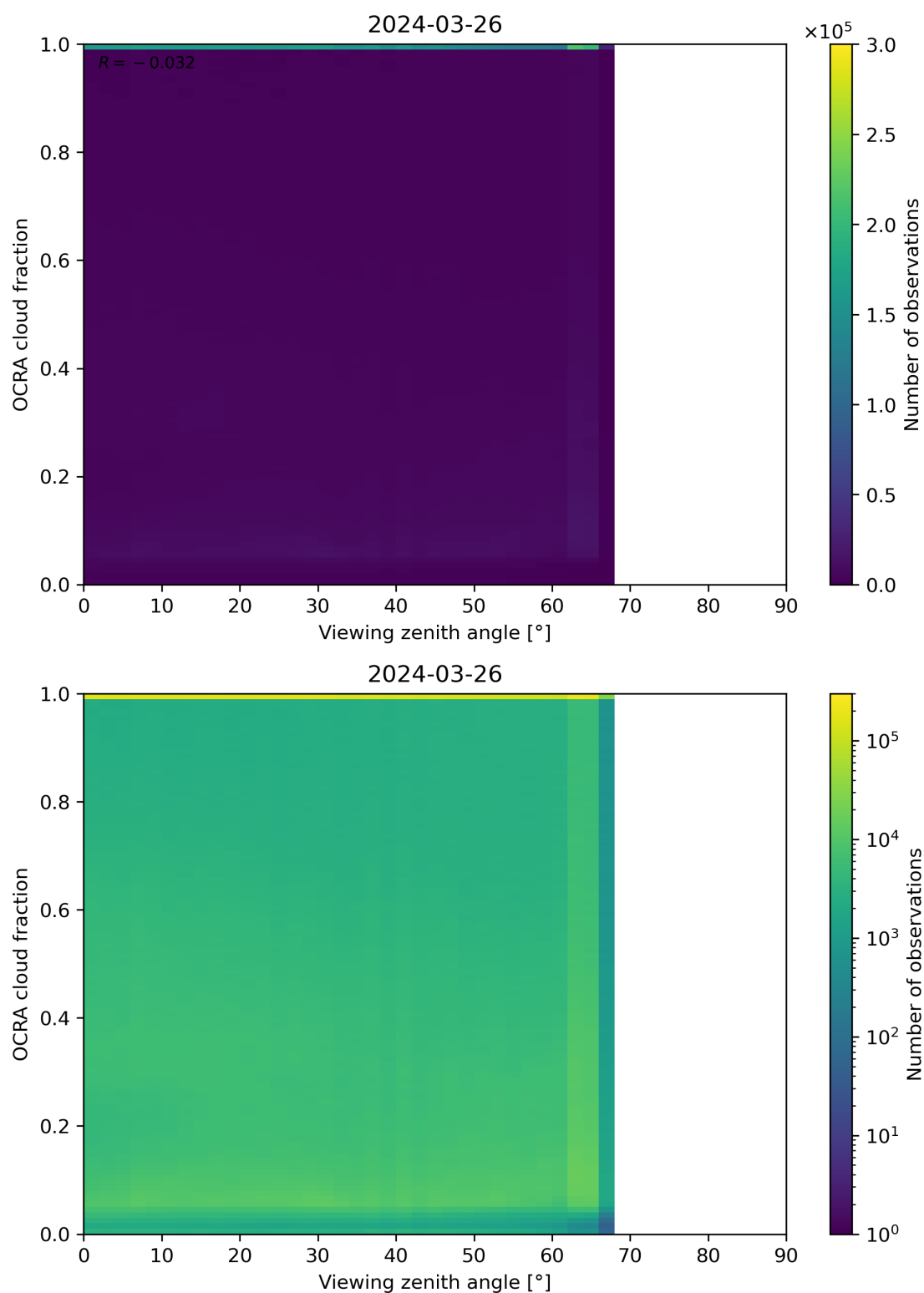
Figure 108: Scatter density plot of “Viewing zenith angle” against “OCRA cloud fraction” for 2024-03-25 to 2024-03-27.
