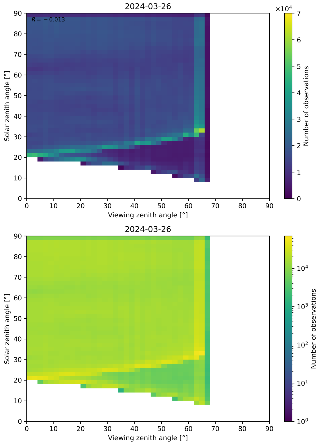
Figure 114: Scatter density plot of “Viewing zenith angle” against “Solar zenith angle” for 2024-03-25 to 2024-03-27.
