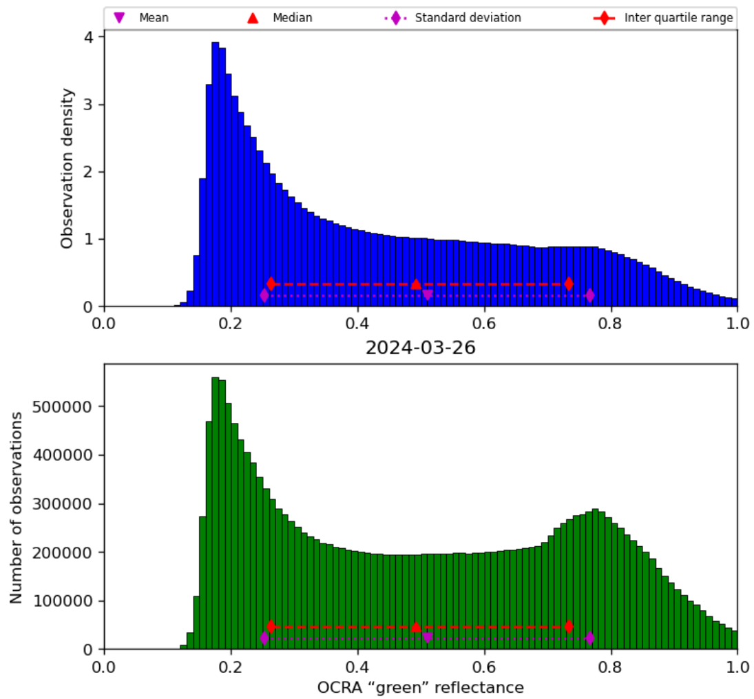
Figure 52: Histogram of “OCRA “green” reflectance” for 2024-03-25 to 2024-03-27
