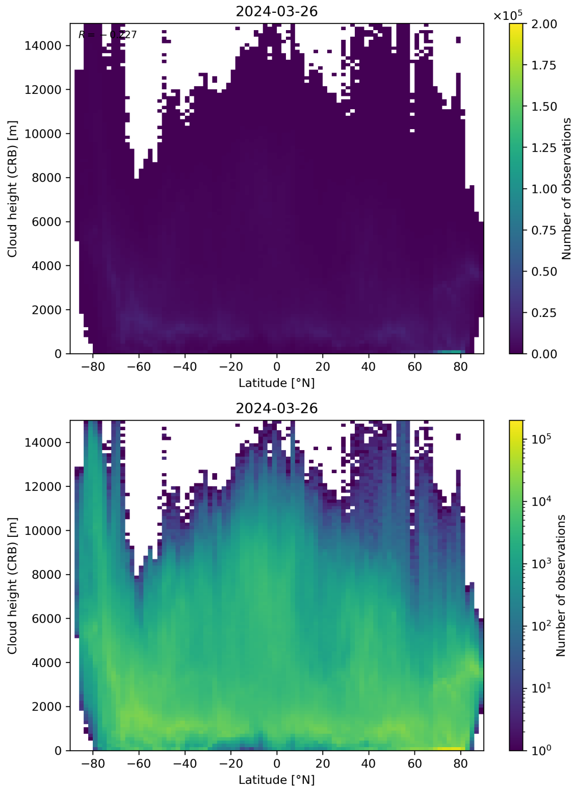
Figure 95: Scatter density plot of “Latitude” against “Cloud height (CRB)” for 2024-03-25 to 2024-03-27.
