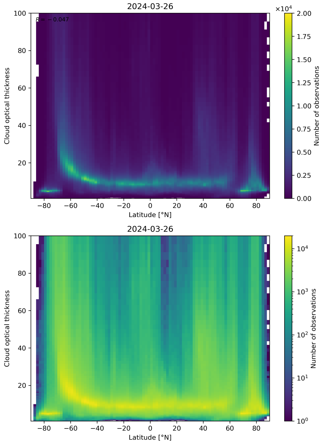
Figure 96: Scatter density plot of “Latitude” against “Cloud optical thickness” for 2024-03-25 to 2024-03-27.
