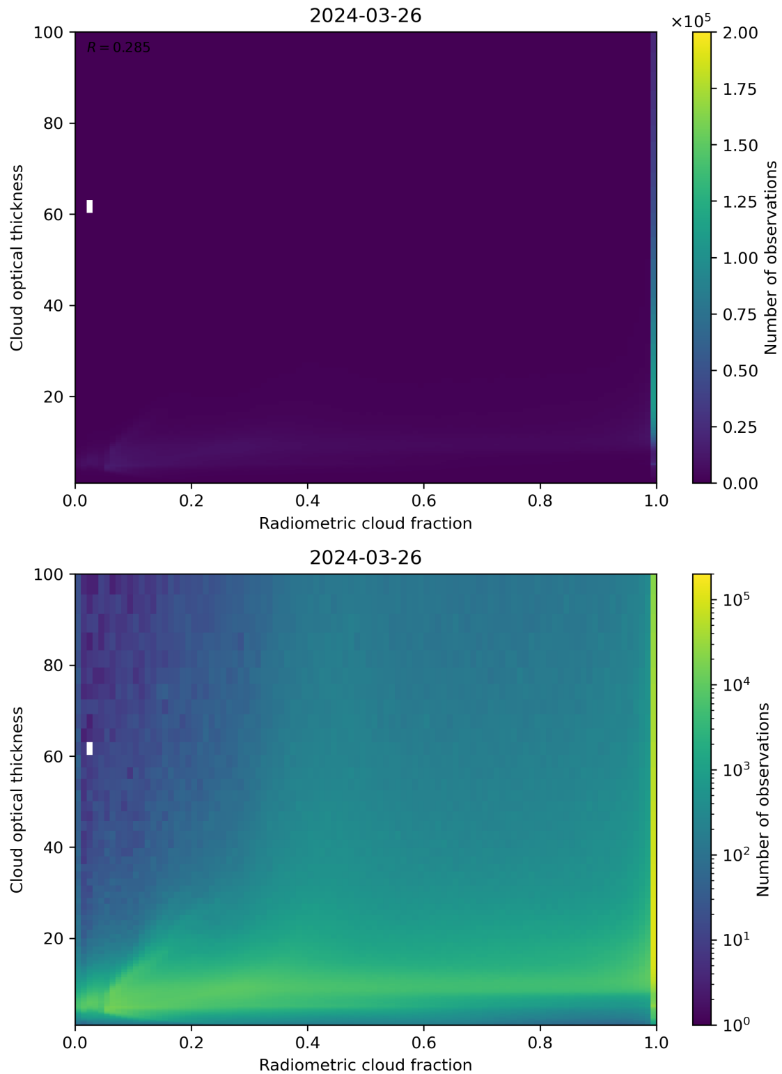
Figure 75: Scatter density plot of “Radiometric cloud fraction” against “Cloud optical thickness” for 2024-03-25 to 2024-03-27.
