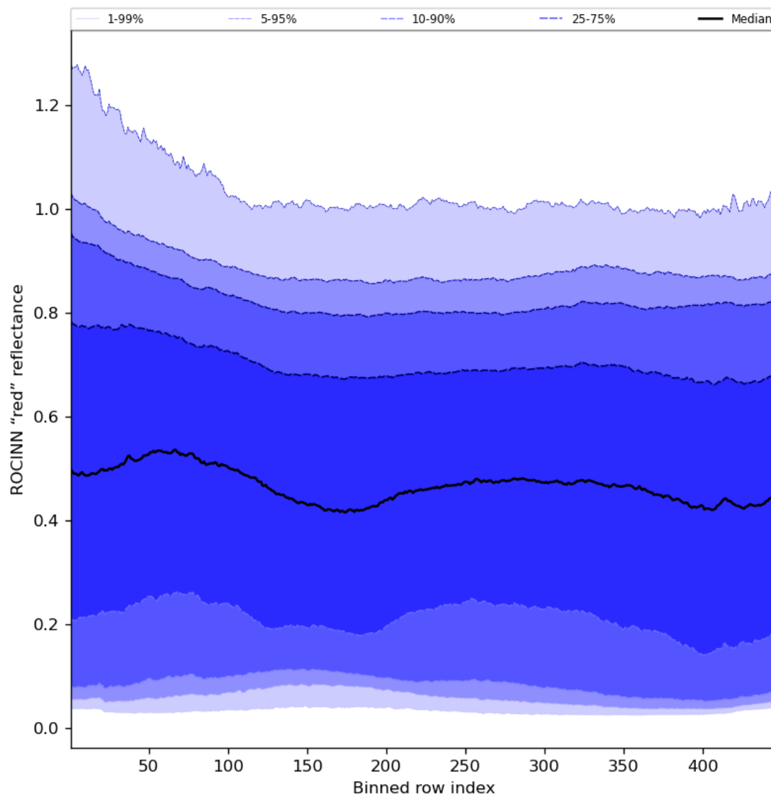
Figure 69: Along track statistics of “ROCINN “red” reflectance” for 2024-03-25 to 2024-03-27
