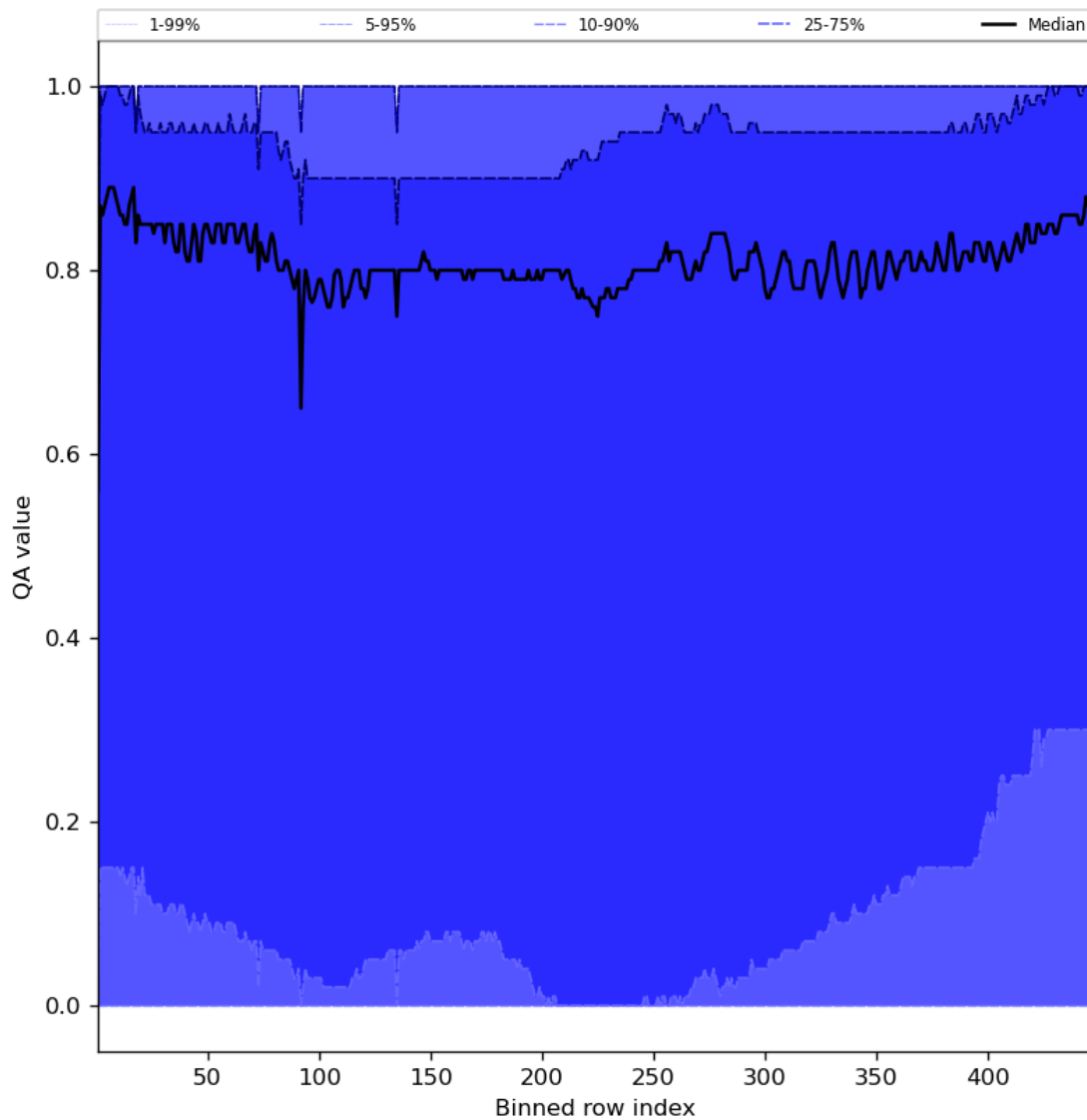
Figure 54: Along track statistics of “QA value” for 2024-03-25 to 2024-03-27
