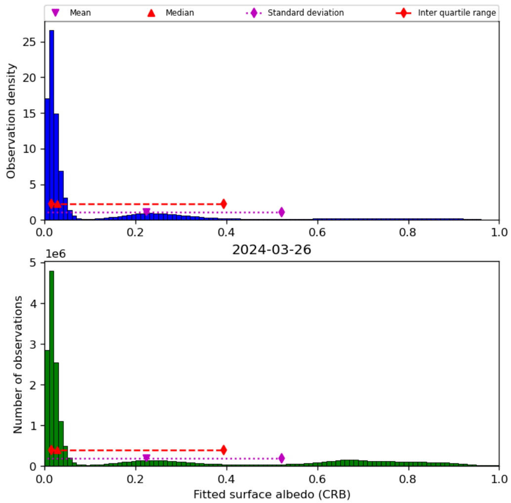
Figure 46: Histogram of “Fitted surface albedo (CRB)” for 2024-03-25 to 2024-03-27
