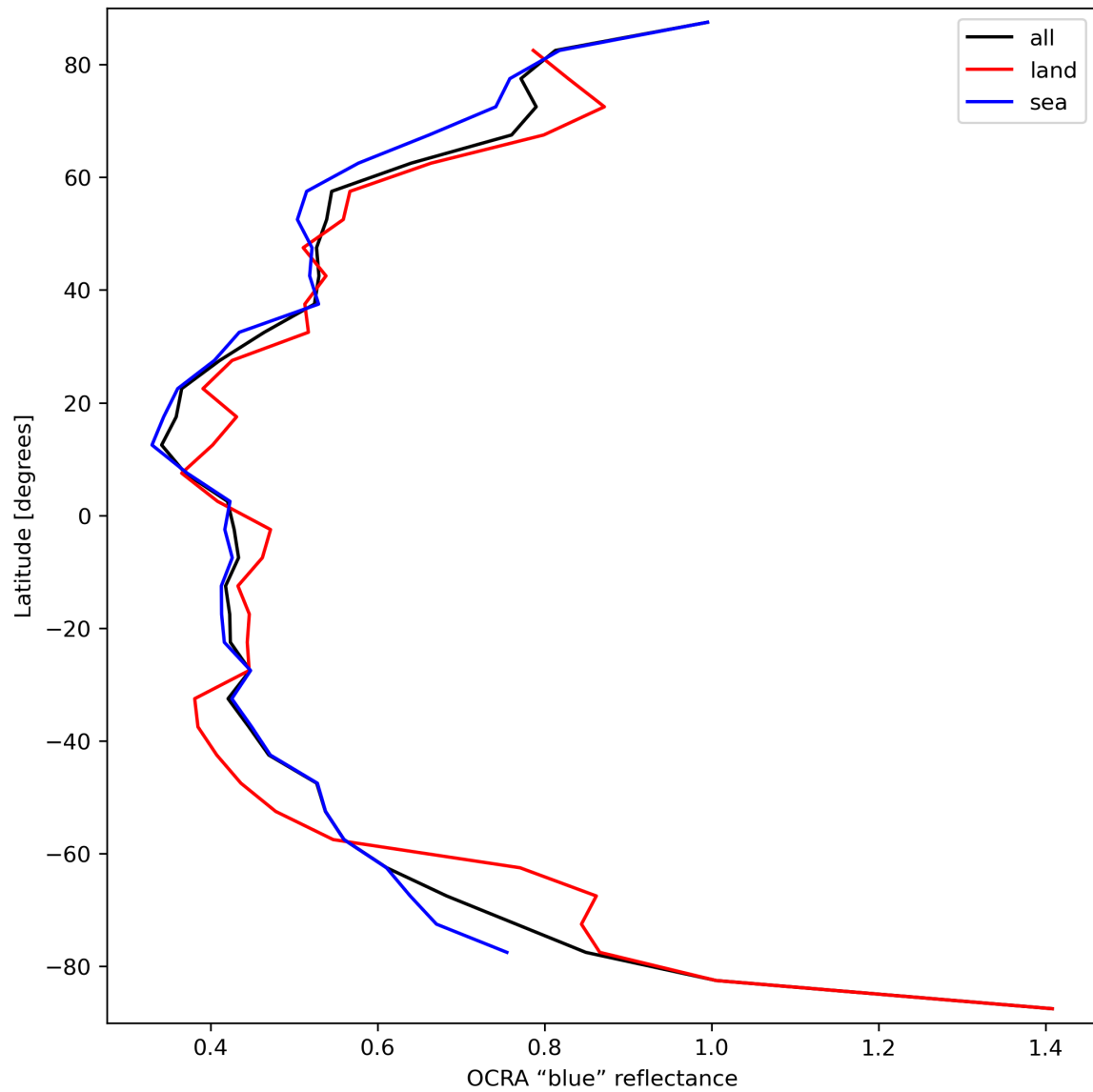
Figure 35: Zonal average of “OCRA “blue” reflectance” for 2024-03-25 to 2024-03-27.
