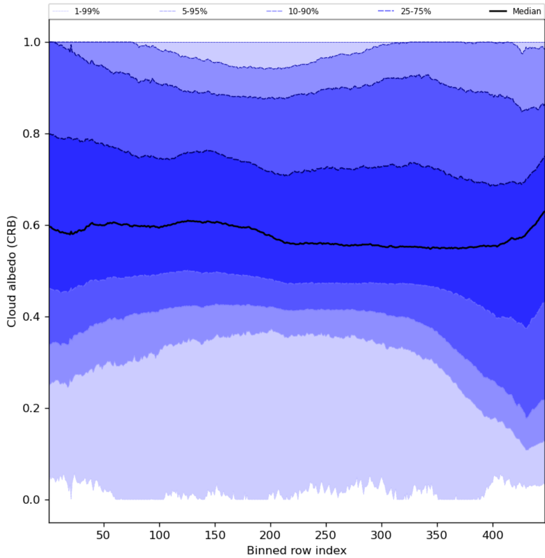
Figure 60: Along track statistics of “Cloud albedo (CRB)” for 2024-03-25 to 2024-03-27
