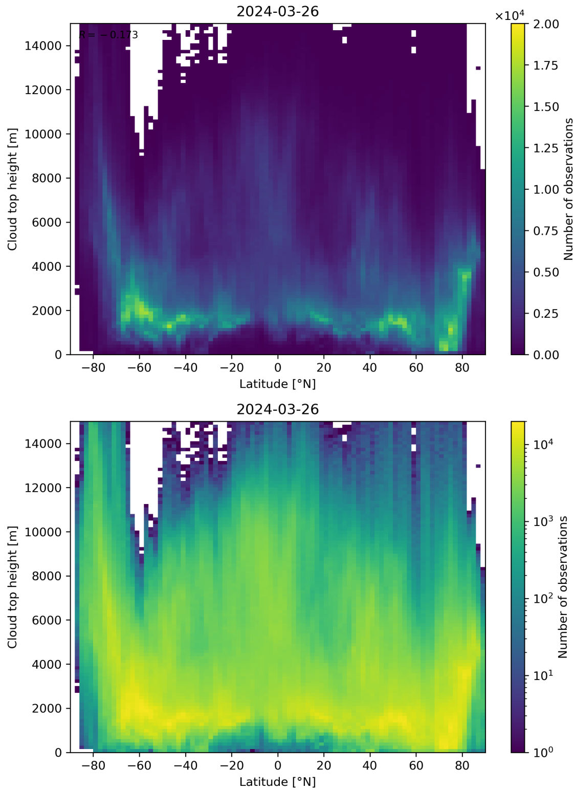
Figure 97: Scatter density plot of “Latitude” against “Cloud top height” for 2024-03-25 to 2024-03-27.
