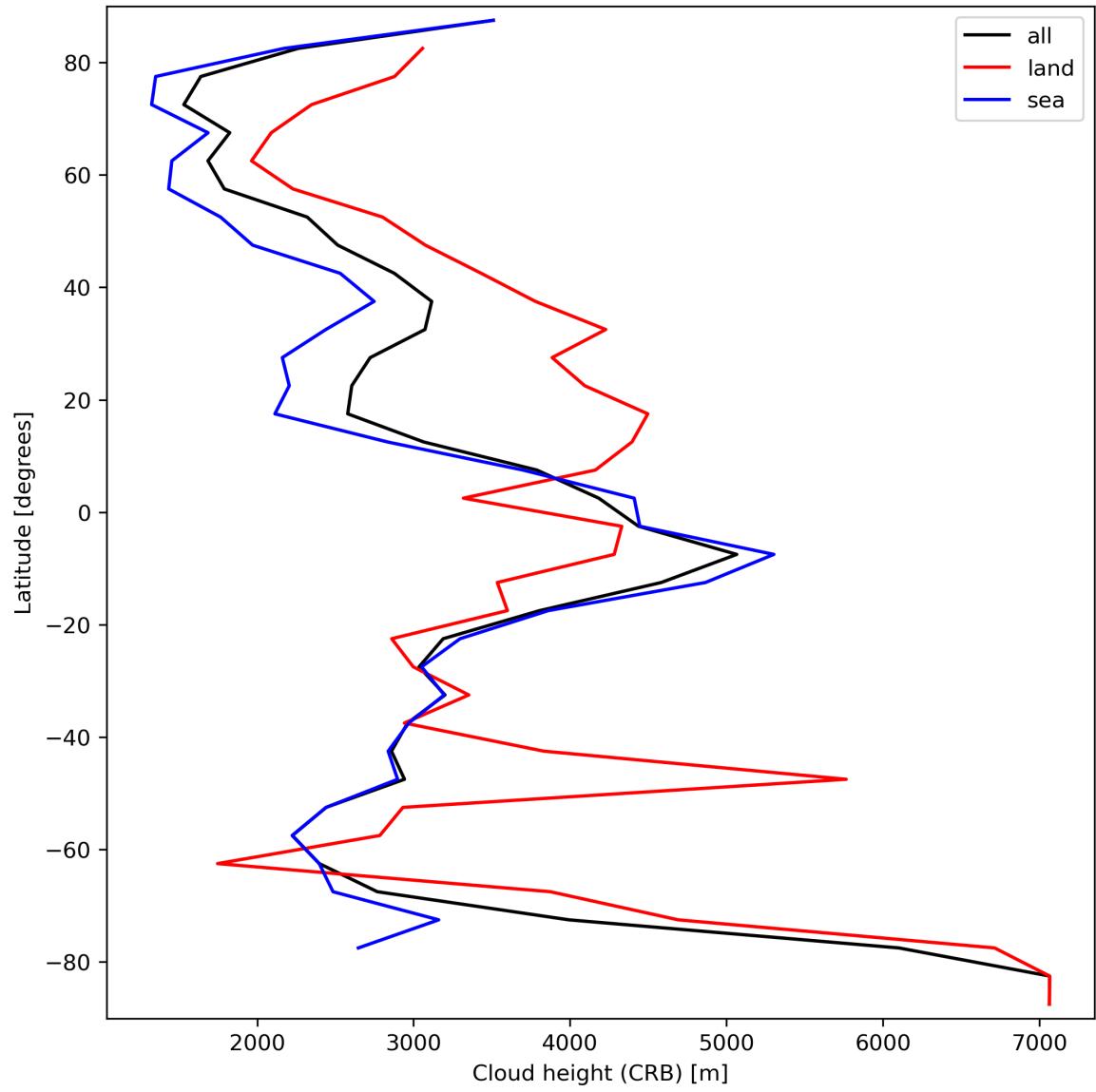
Figure 27: Zonal average of “Cloud height (CRB)” for 2024-03-25 to 2024-03-27.
