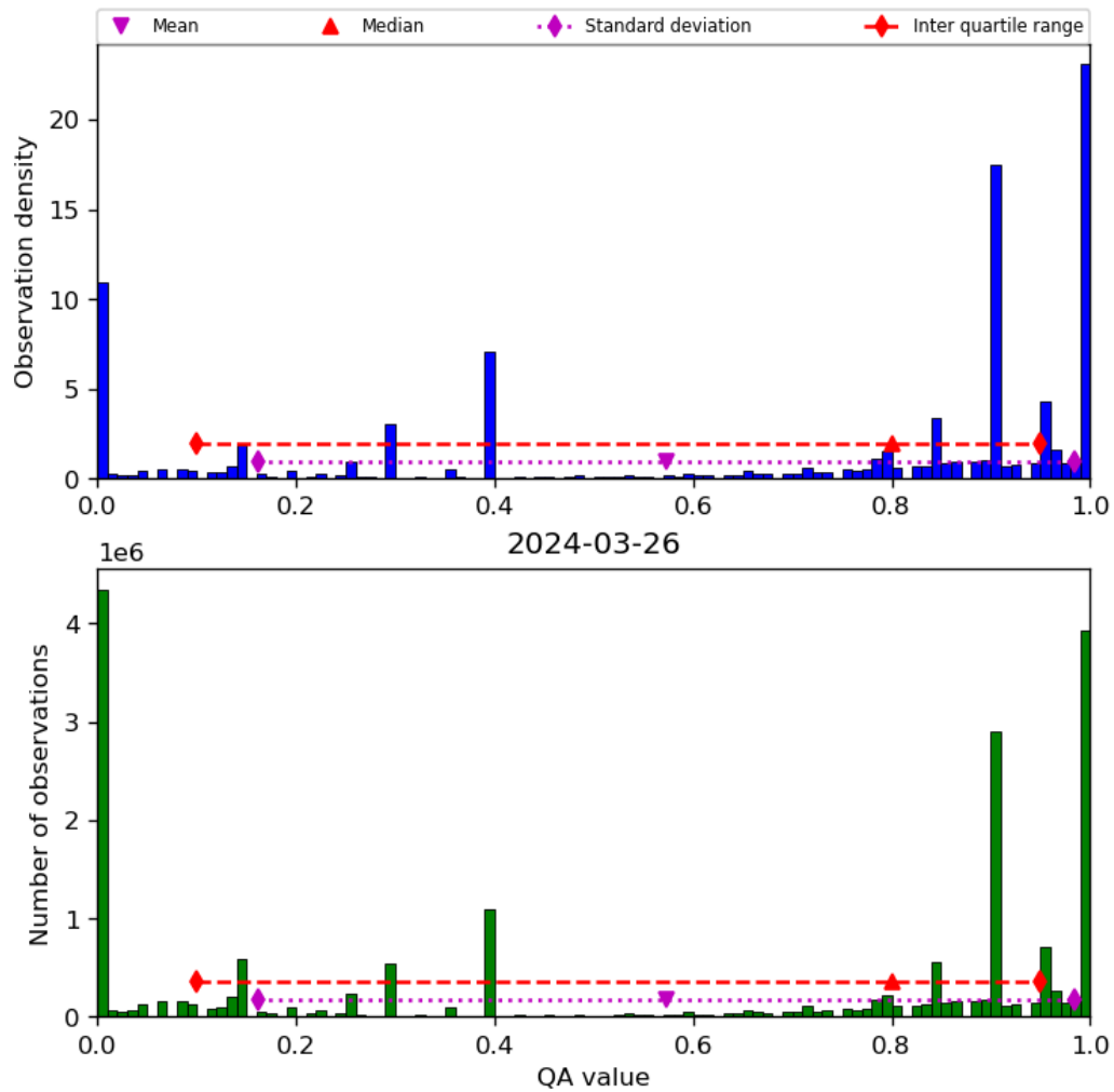
Figure 38: Histogram of “QA value” for 2024-03-25 to 2024-03-27
