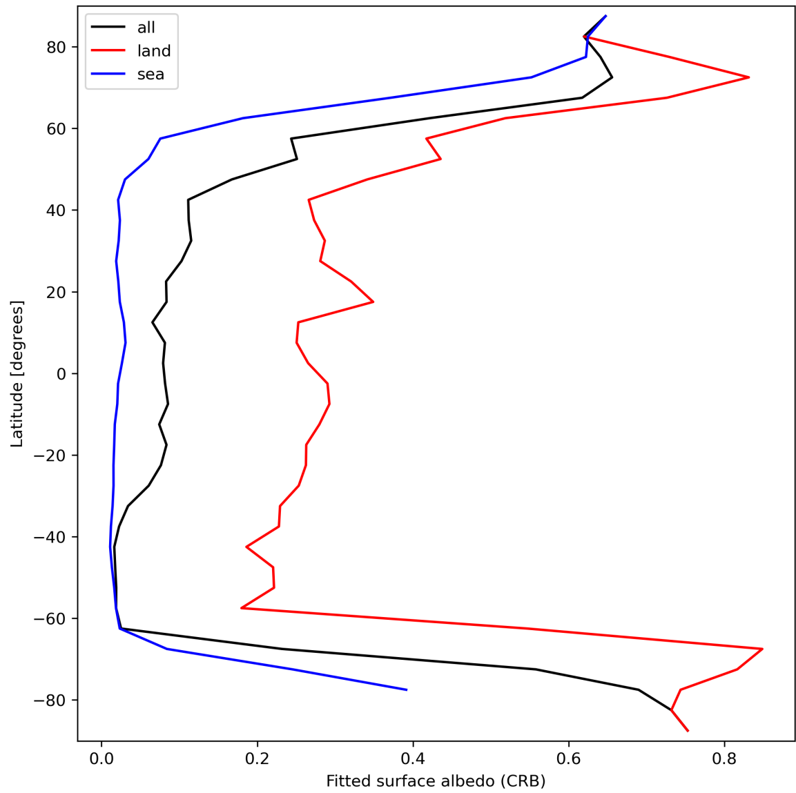
Figure 30: Zonal average of “Fitted surface albedo (CRB)” for 2024-03-25 to 2024-03-27.
