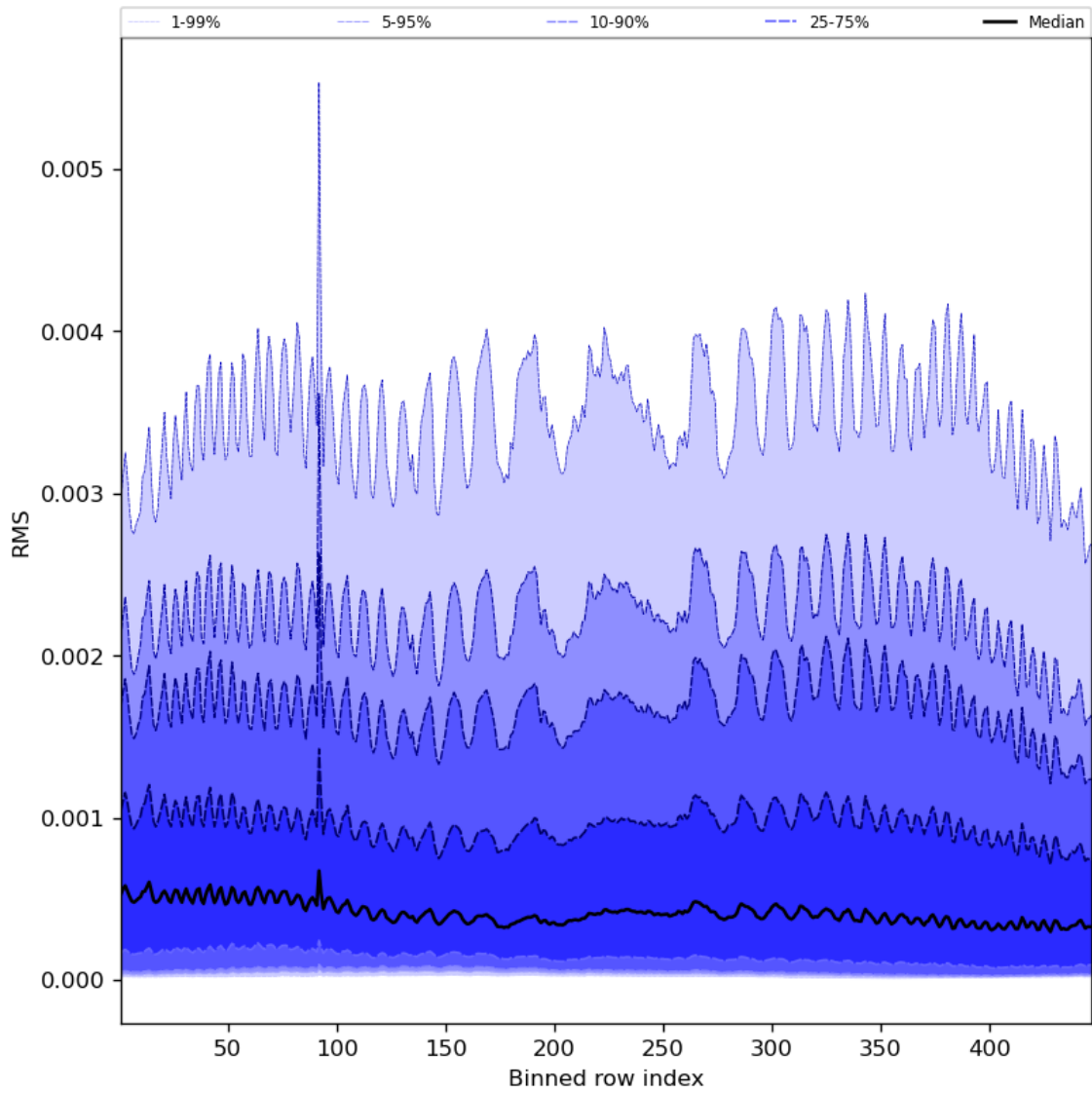
Figure 63: Along track statistics of “RMS” for 2024-03-25 to 2024-03-27
