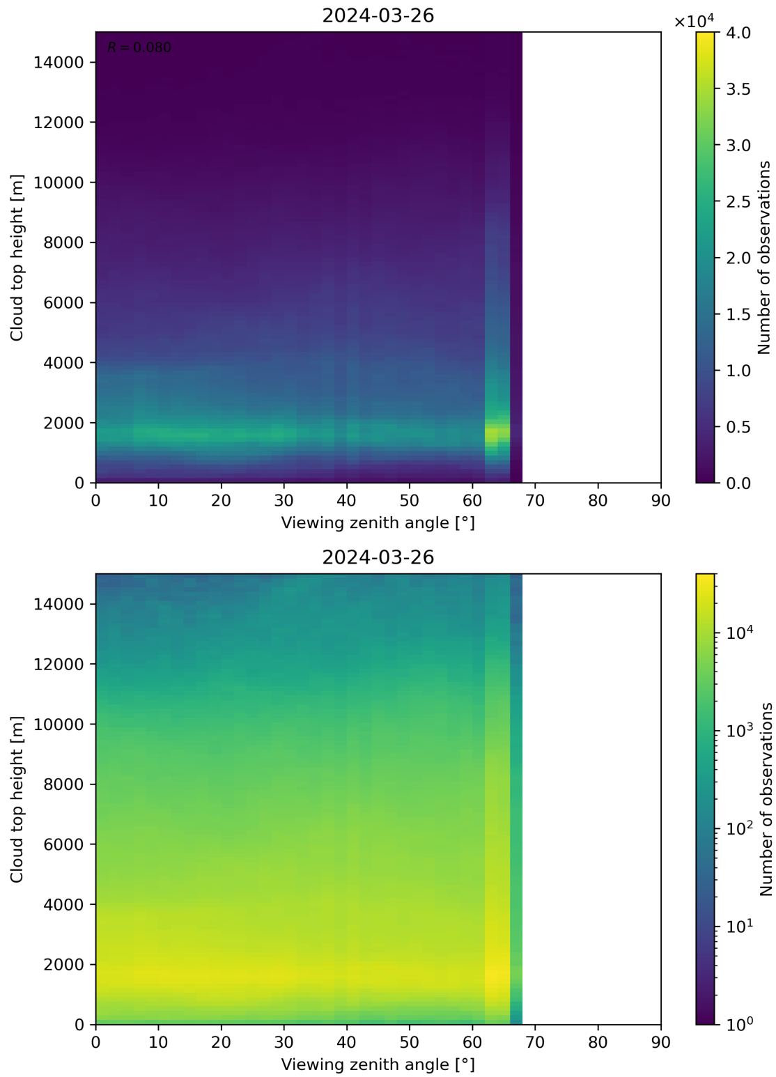
Figure 112: Scatter density plot of “Viewing zenith angle” against “Cloud top height” for 2024-03-25 to 2024-03-27.
