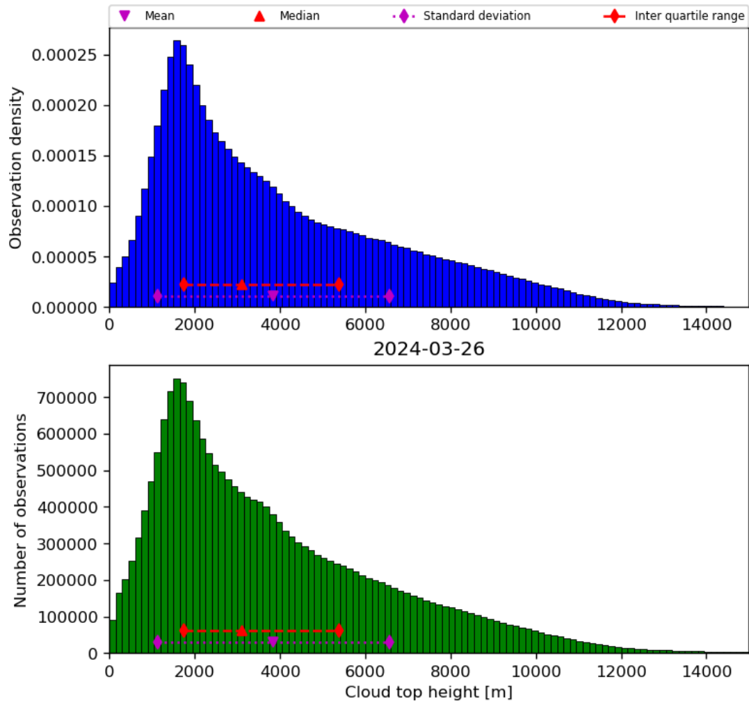
Figure 40: Histogram of “Cloud top height” for 2024-03-25 to 2024-03-27
