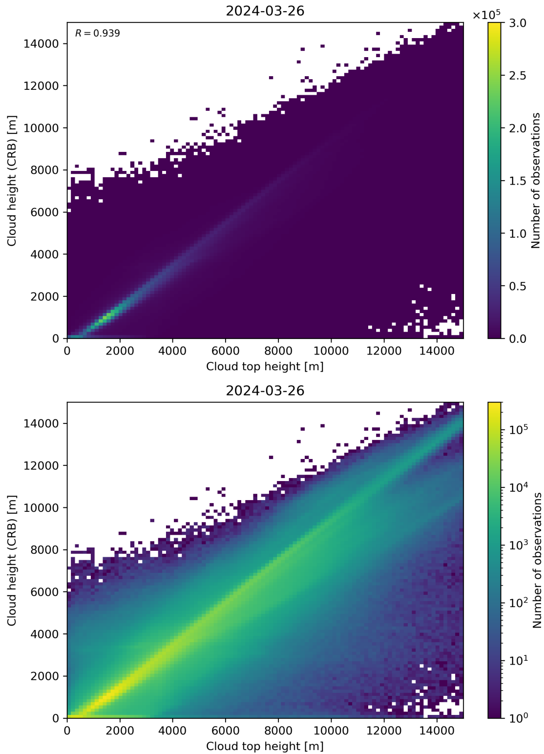
Figure 89: Scatter density plot of “Cloud top height” against “Cloud height (CRB)” for 2024-03-25 to 2024-03-27.
