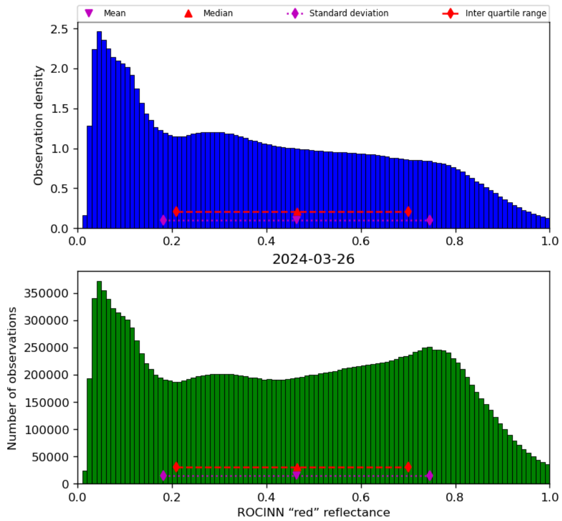
Figure 53: Histogram of “ROCINN “red” reflectance” for 2024-03-25 to 2024-03-27
