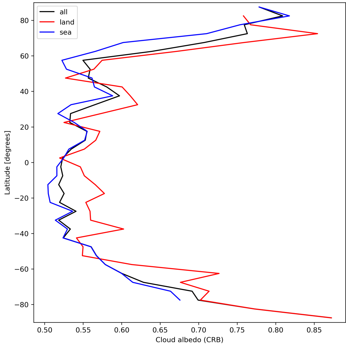
Figure 28: Zonal average of “Cloud albedo (CRB)” for 2024-03-25 to 2024-03-27.
