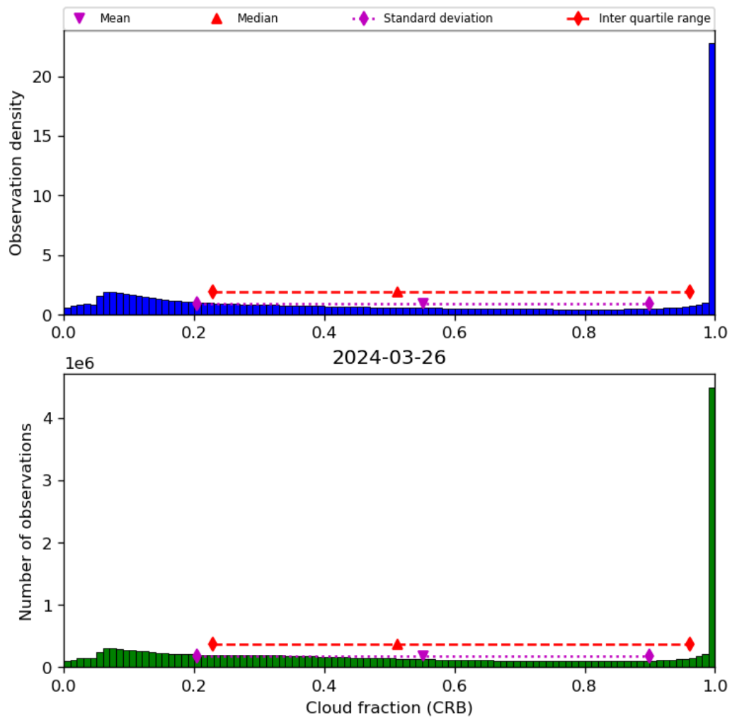
Figure 42: Histogram of “Cloud fraction (CRB)” for 2024-03-25 to 2024-03-27
