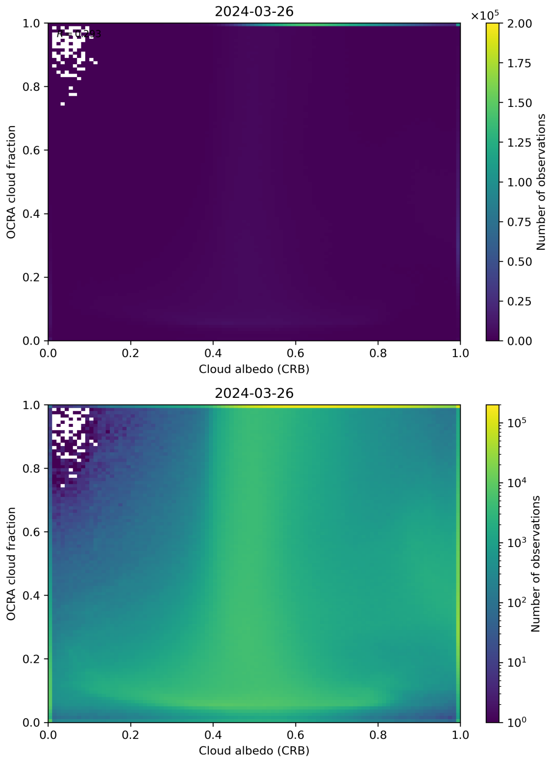
Figure 70: Scatter density plot of “Cloud albedo (CRB)” against “OCRA cloud fraction” for 2024-03-25 to 2024-03-27.
