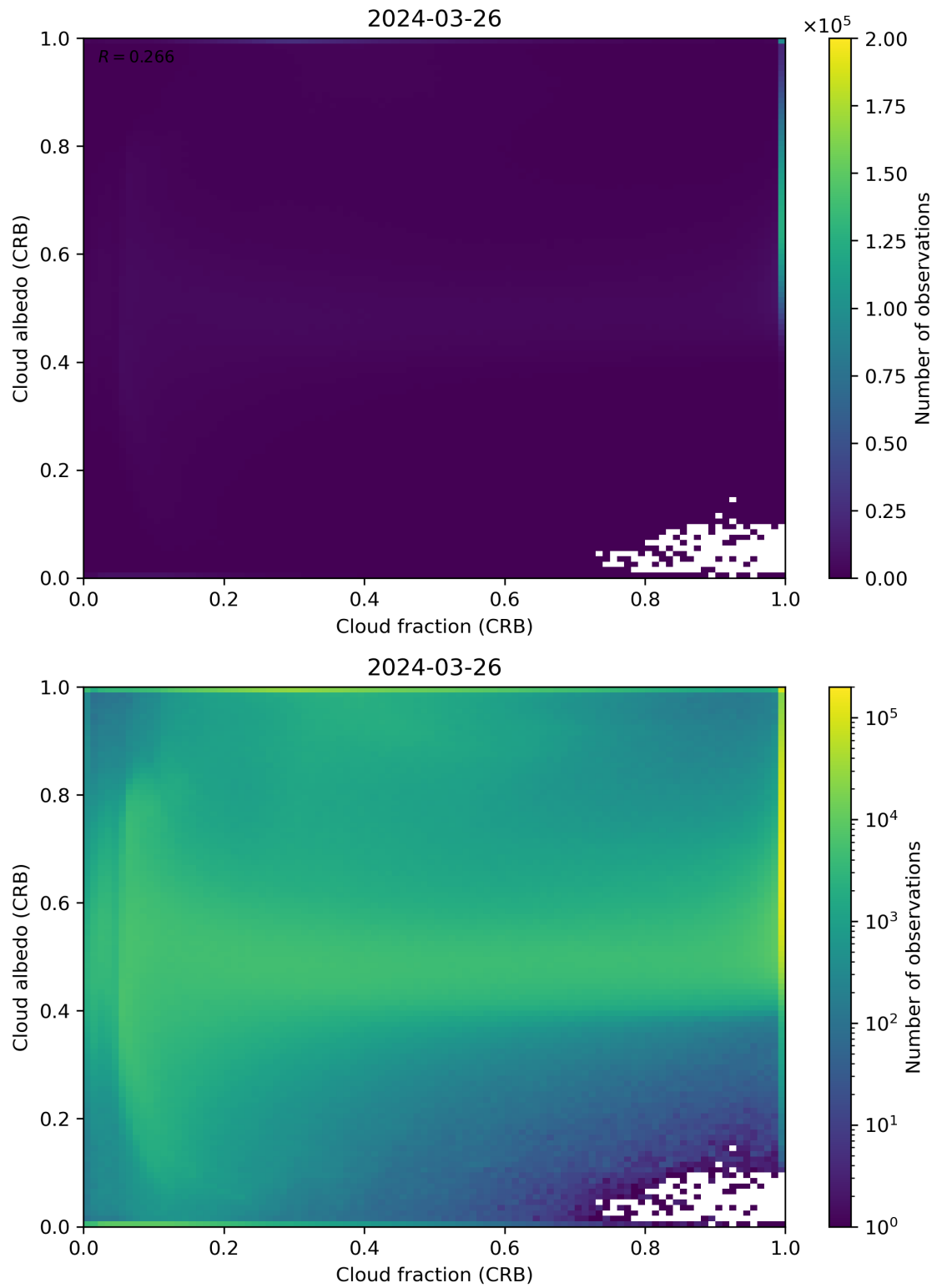
Figure 77: Scatter density plot of “Cloud fraction (CRB)” against “Cloud albedo (CRB)” for 2024-03-25 to 2024-03-27.
