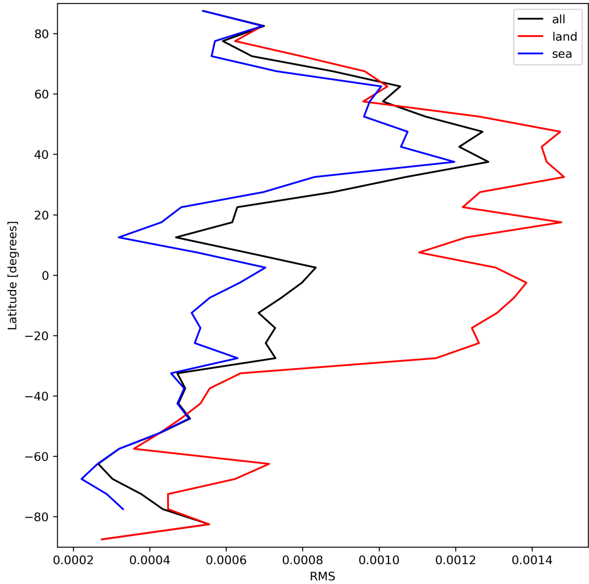
Figure 31: Zonal average of “RMS” for 2024-03-25 to 2024-03-27.
