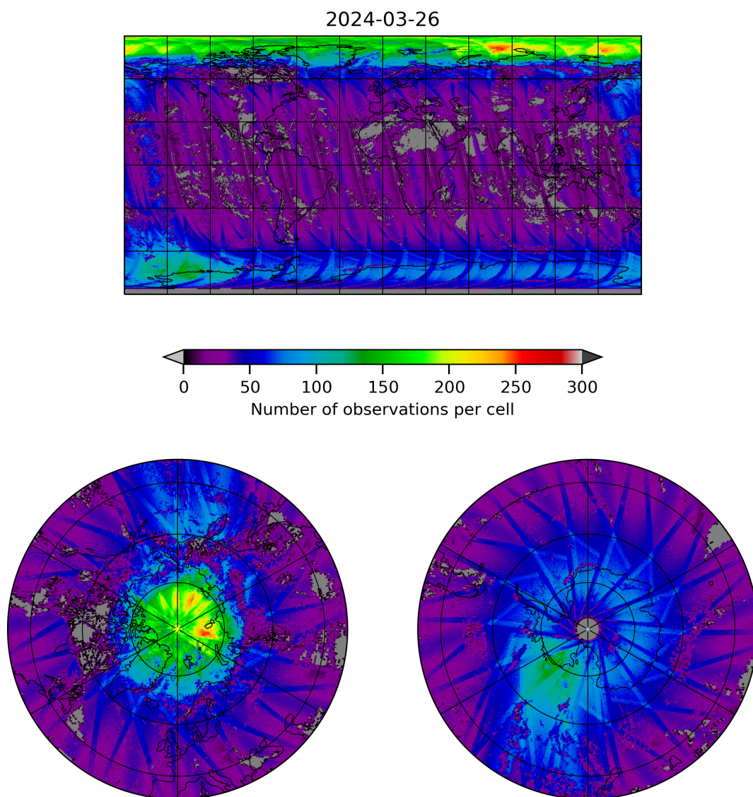
Figure 21: Map of the number of observations for 2024-03-25 to 2024-03-27
