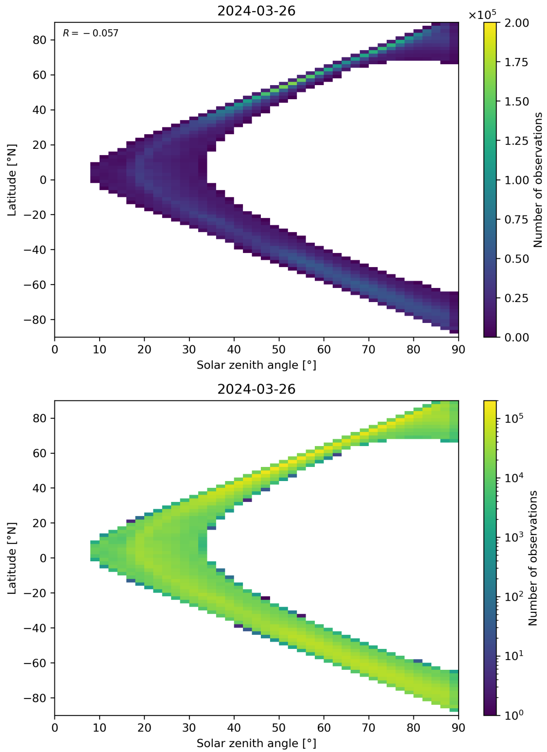
Figure 105: Scatter density plot of “Solar zenith angle” against “Latitude” for 2024-03-25 to 2024-03-27.
