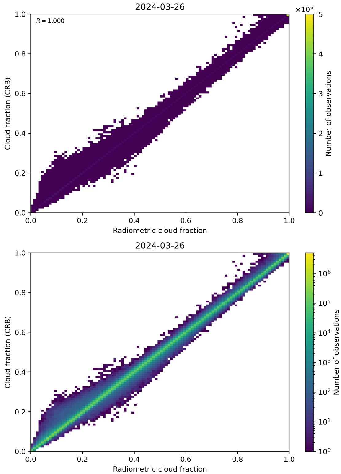
Figure 73: Scatter density plot of “Radiometric cloud fraction” against “Cloud fraction (CRB)” for 2024-03-25 to 2024-03-27.
