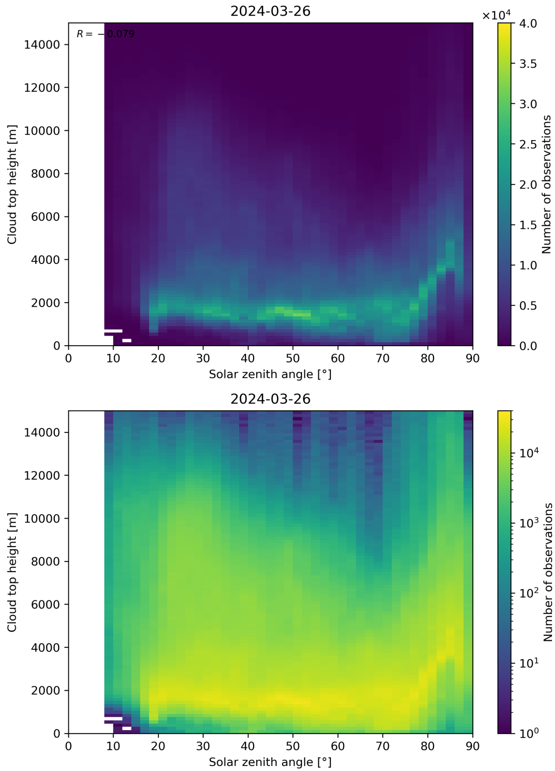
Figure 104: Scatter density plot of “Solar zenith angle” against “Cloud top height” for 2024-03-25 to 2024-03-27.
