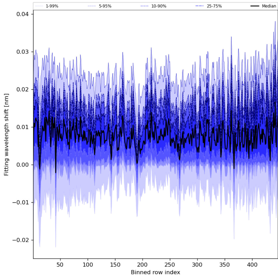
Figure 65: Along track statistics of “Fitting wavelength shift” for 2024-03-25 to 2024-03-27
