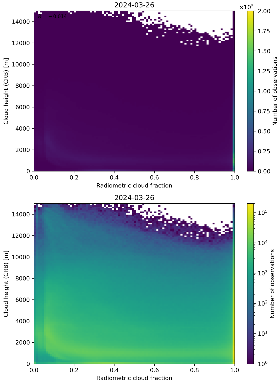
Figure 74: Scatter density plot of “Radiometric cloud fraction” against “Cloud height (CRB)” for 2024-03-25 to 2024-03-27.
