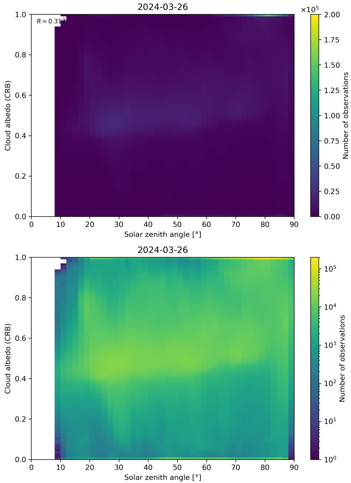
Figure 98: Scatter density plot of “Solar zenith angle” against “Cloud albedo (CRB)” for 2024-03-25 to 2024-03-27.
