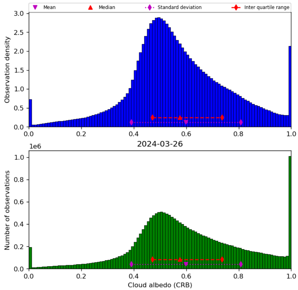
Figure 44: Histogram of “Cloud albedo (CRB)” for 2024-03-25 to 2024-03-27
