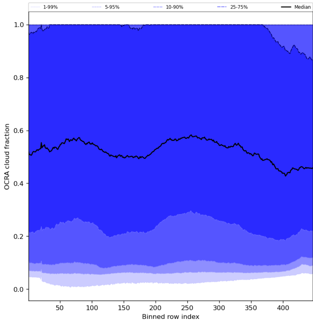
Figure 66: Along track statistics of “OCRA cloud fraction” for 2024-03-25 to 2024-03-27
