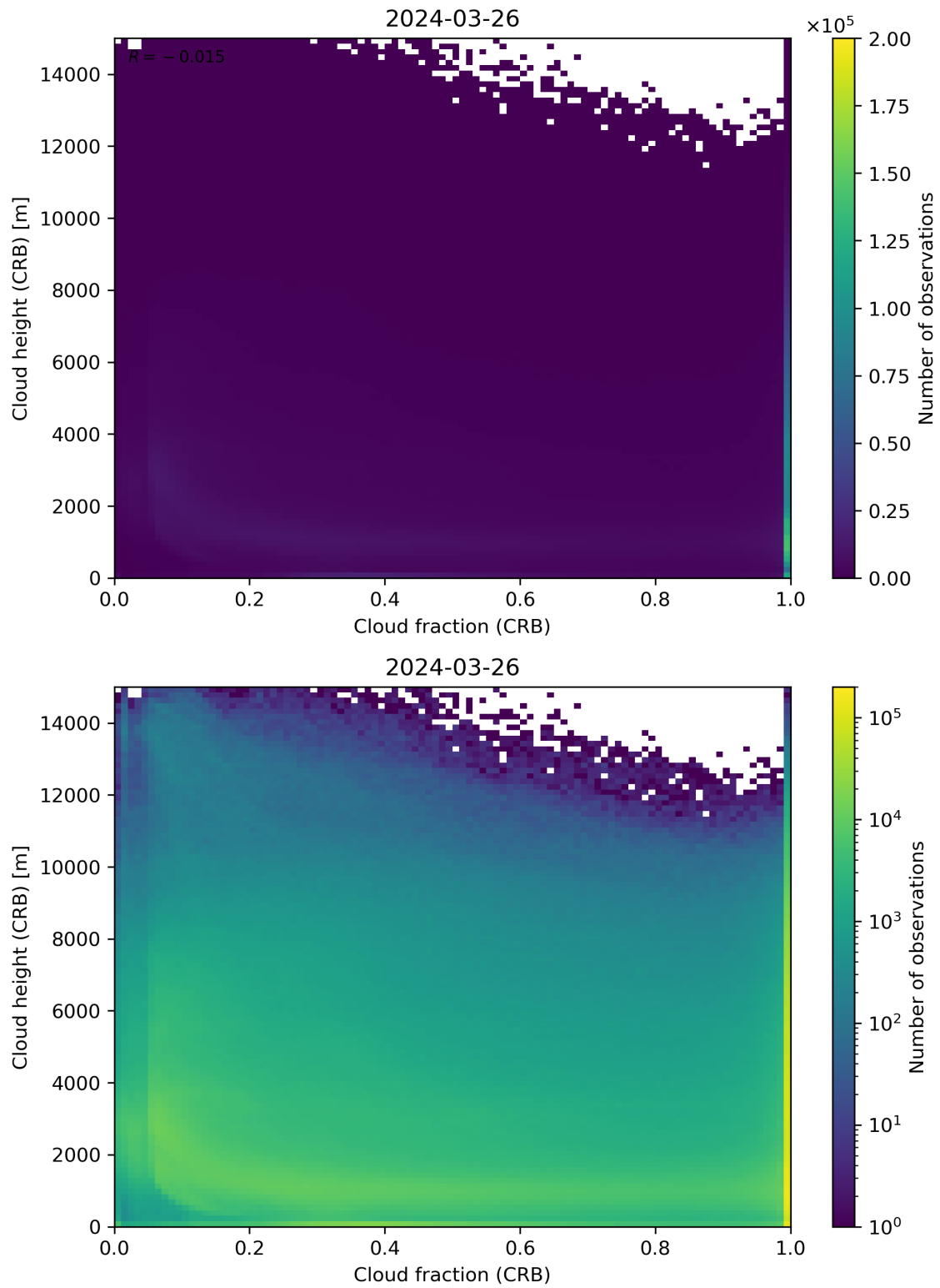
Figure 79: Scatter density plot of “Cloud fraction (CRB)” against “Cloud height (CRB)” for 2024-03-25 to 2024-03-27.
