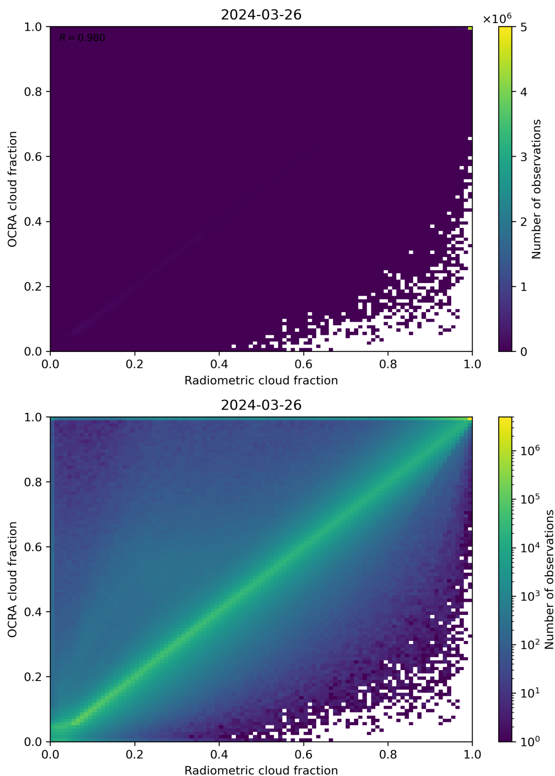
Figure 72: Scatter density plot of “Radiometric cloud fraction” against “OCRA cloud fraction” for 2024-03-25 to 2024-03-27.
