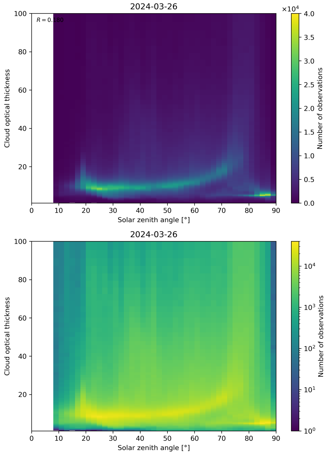
Figure 103: Scatter density plot of “Solar zenith angle” against “Cloud optical thickness” for 2024-03-25 to 2024-03-27.
