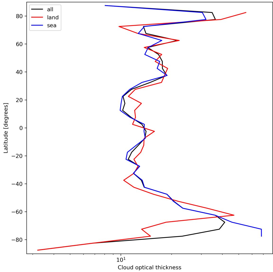
Figure 25: Zonal average of “Cloud optical thickness” for 2024-03-25 to 2024-03-27.
