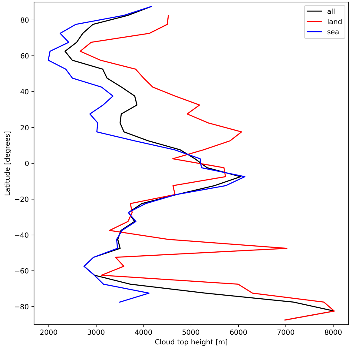
Figure 24: Zonal average of “Cloud top height” for 2024-03-25 to 2024-03-27.
