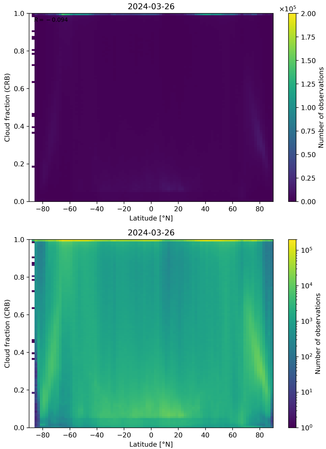
Figure 94: Scatter density plot of “Latitude” against “Cloud fraction (CRB)” for 2024-03-25 to 2024-03-27.
