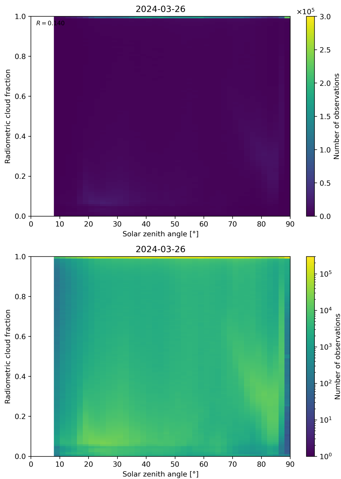
Figure 99: Scatter density plot of “Solar zenith angle” against “Radiometric cloud fraction” for 2024-03-25 to 2024-03-27.
