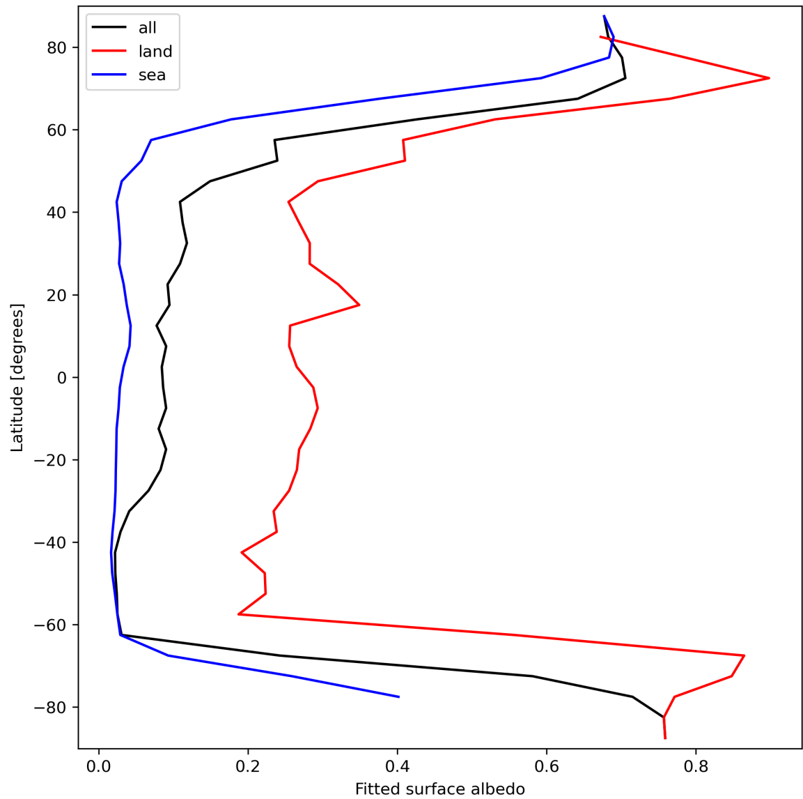
Figure 29: Zonal average of “Fitted surface albedo” for 2024-03-25 to 2024-03-27.
