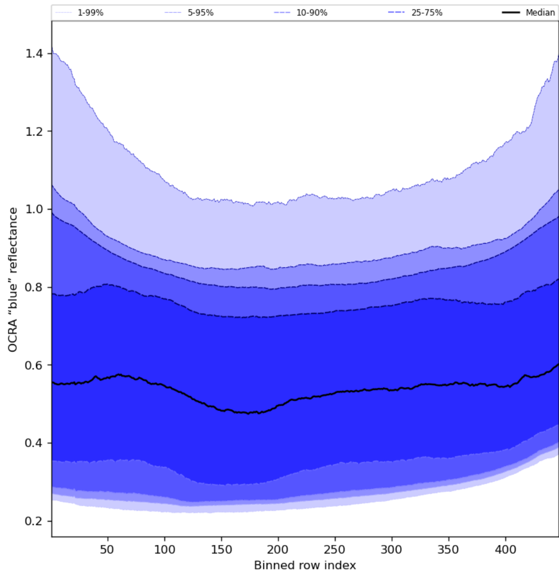
Figure 67: Along track statistics of “OCRA “blue” reflectance” for 2024-03-25 to 2024-03-27
