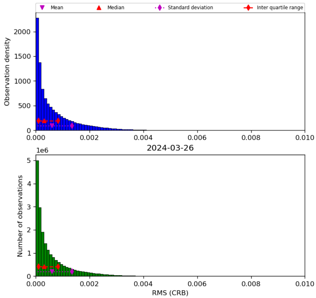
Figure 48: Histogram of “RMS (CRB)” for 2024-03-25 to 2024-03-27
