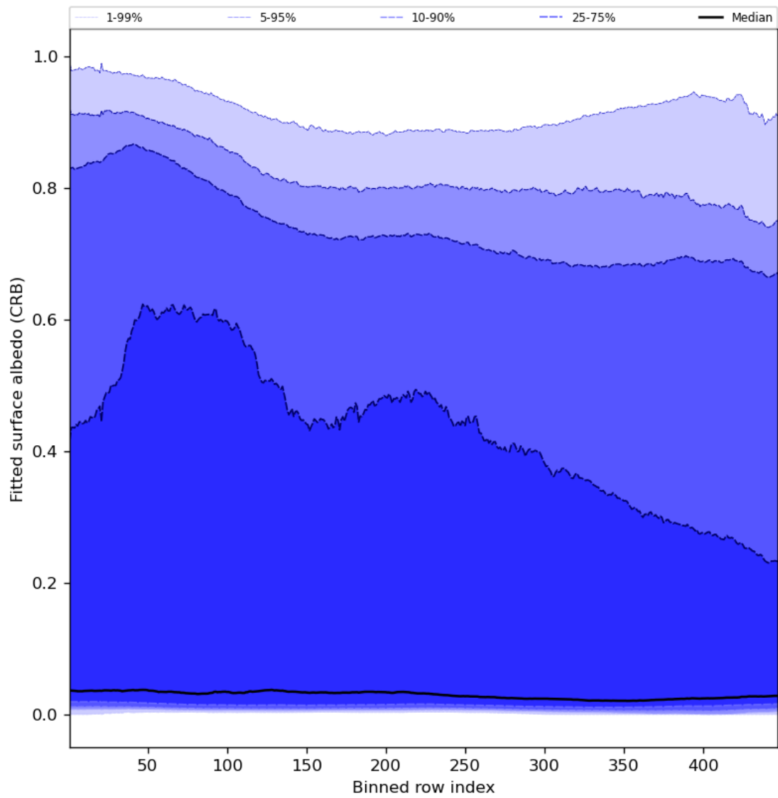
Figure 62: Along track statistics of “Fitted surface albedo (CRB)” for 2024-03-25 to 2024-03-27
