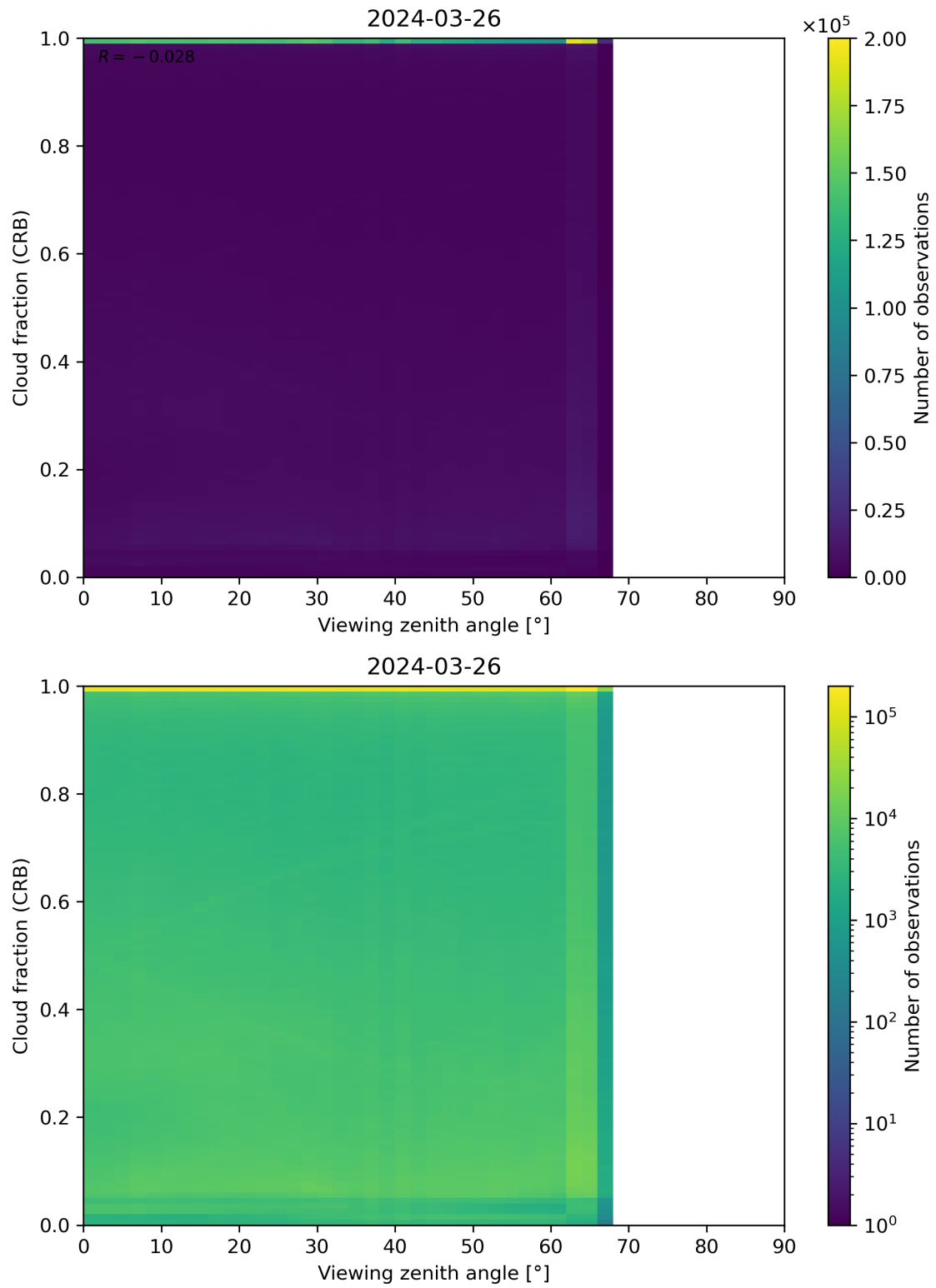
Figure 109: Scatter density plot of “Viewing zenith angle” against “Cloud fraction (CRB)” for 2024-03-25 to 2024-03-27.
