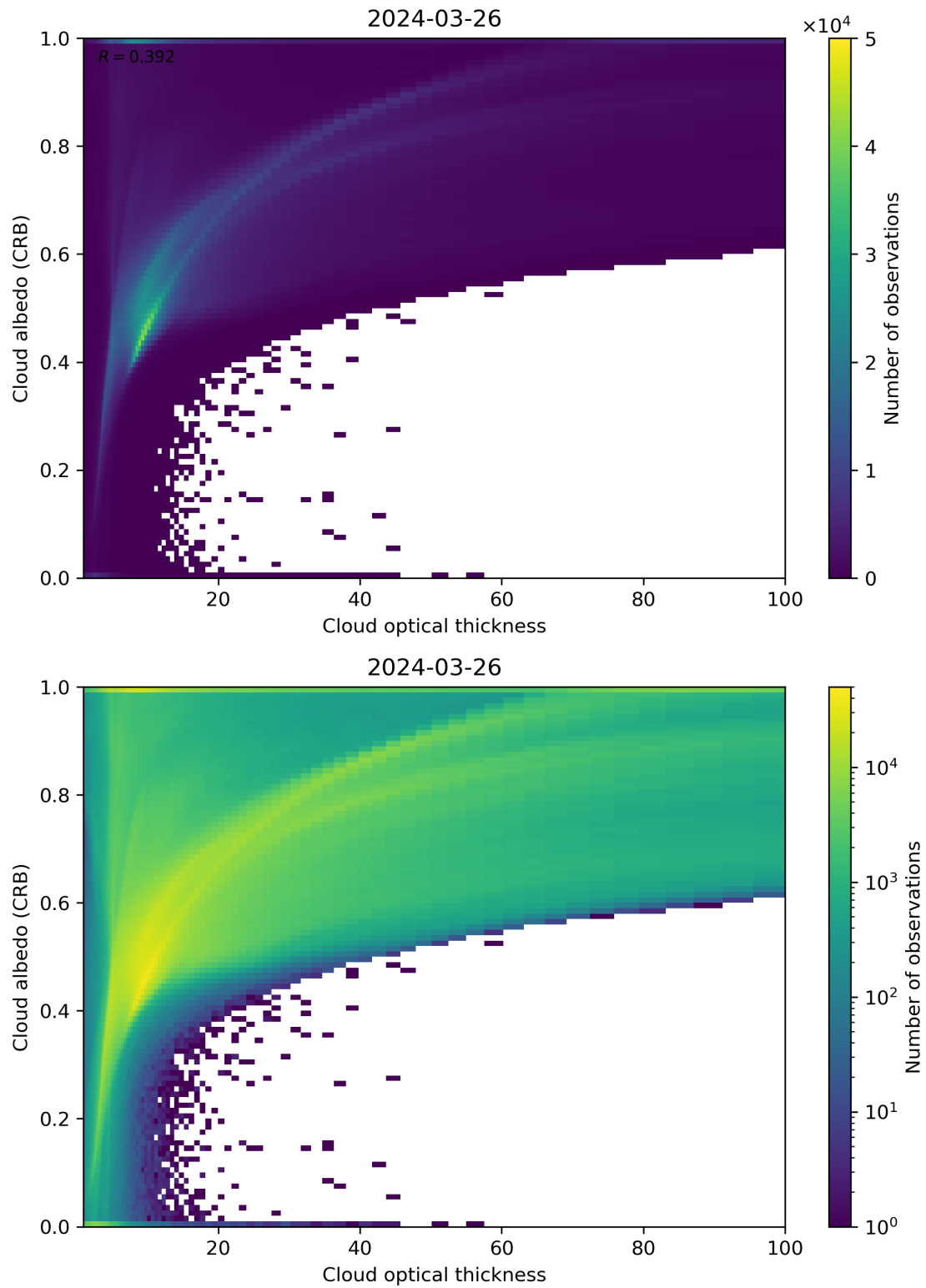
Figure 82: Scatter density plot of “Cloud optical thickness” against “Cloud albedo (CRB)” for 2024-03-25 to 2024-03-27.
