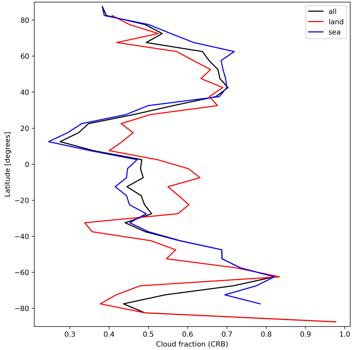
Figure 26: Zonal average of “Cloud fraction (CRB)” for 2024-03-25 to 2024-03-27.
