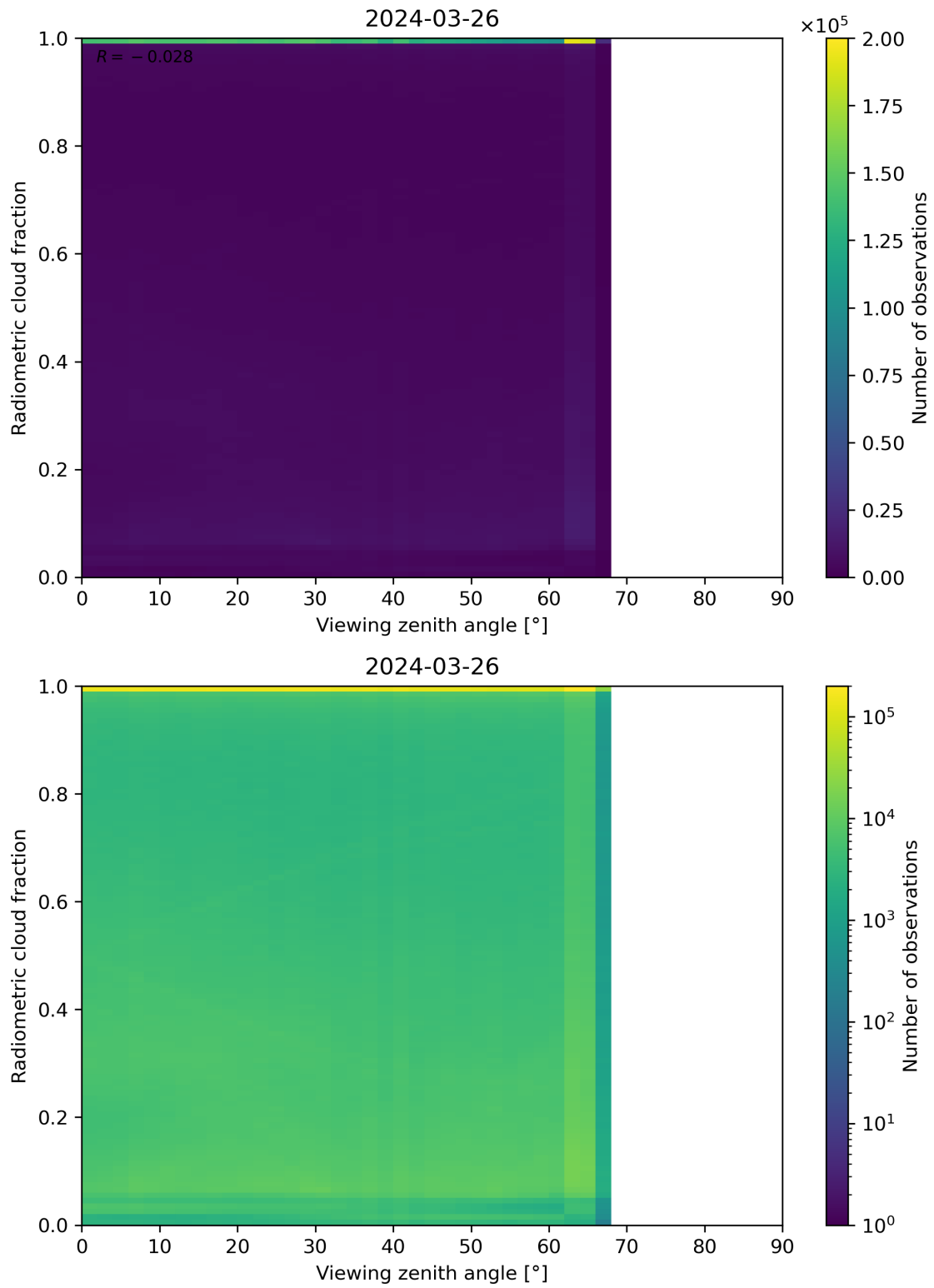
Figure 107: Scatter density plot of “Viewing zenith angle” against “Radiometric cloud fraction” for 2024-03-25 to 2024-03-27.
