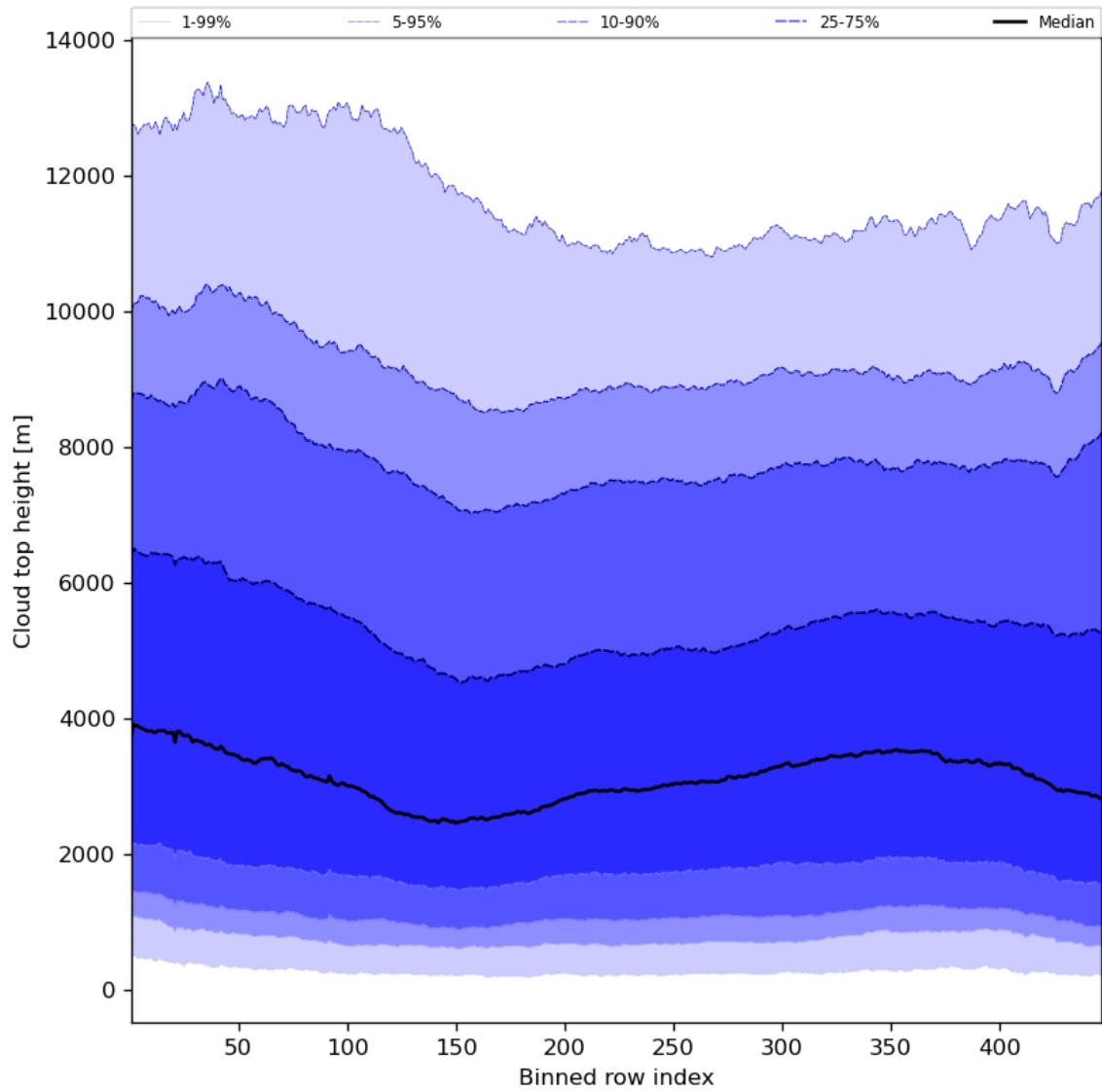
Figure 56: Along track statistics of “Cloud top height” for 2024-03-25 to 2024-03-27
