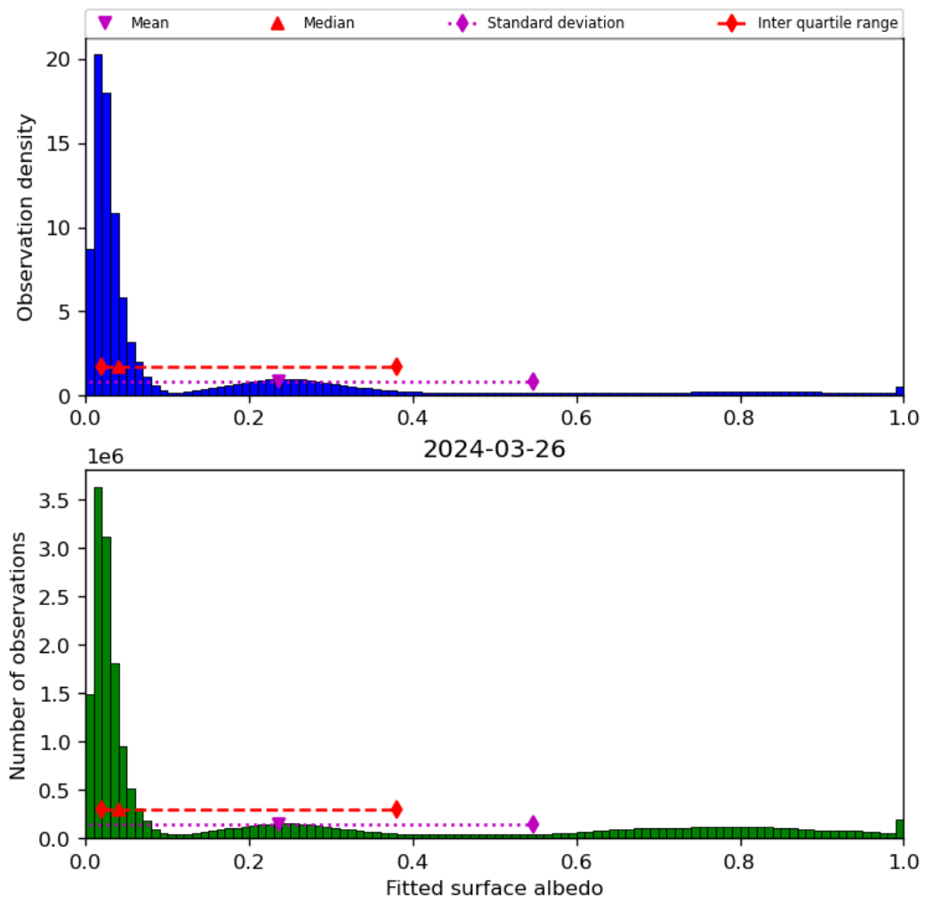
Figure 45: Histogram of “Fitted surface albedo” for 2024-03-25 to 2024-03-27
