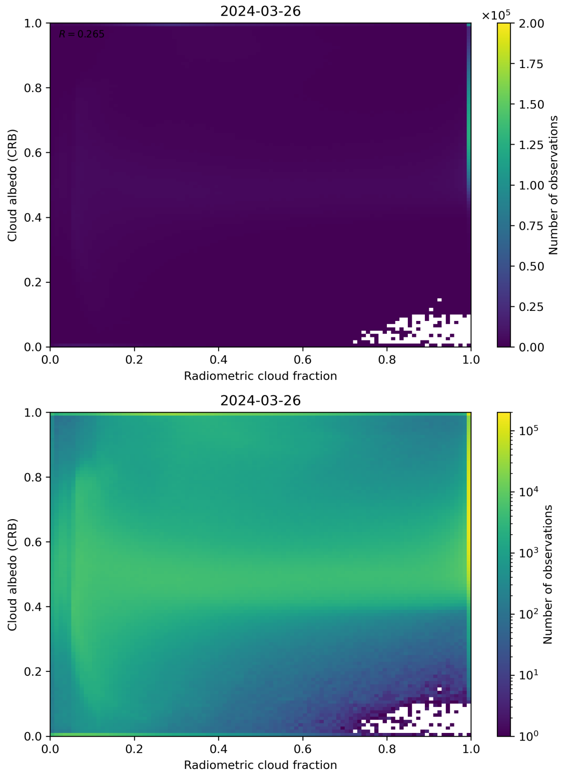
Figure 71: Scatter density plot of “Radiometric cloud fraction” against “Cloud albedo (CRB)” for 2024-03-25 to 2024-03-27.
