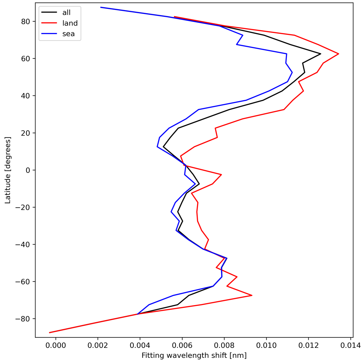
Figure 33: Zonal average of “Fitting wavelength shift” for 2024-03-25 to 2024-03-27.
