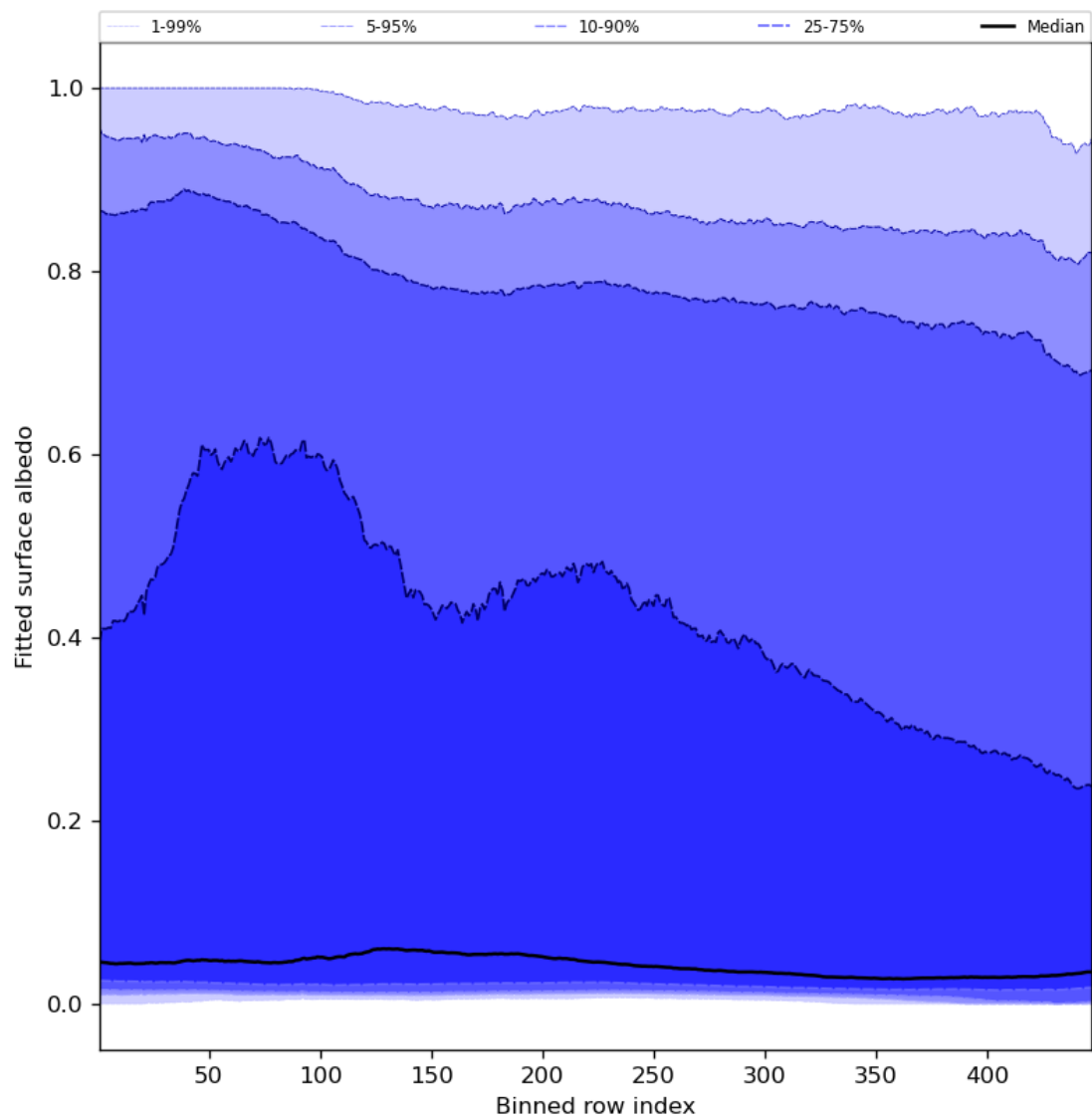
Figure 61: Along track statistics of “Fitted surface albedo” for 2024-03-25 to 2024-03-27
