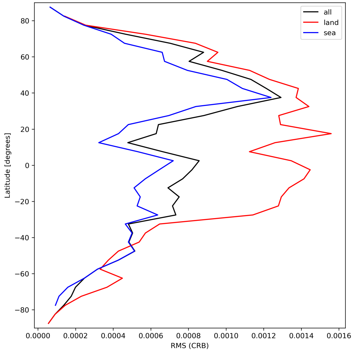
Figure 32: Zonal average of “RMS (CRB)” for 2024-03-25 to 2024-03-27.
