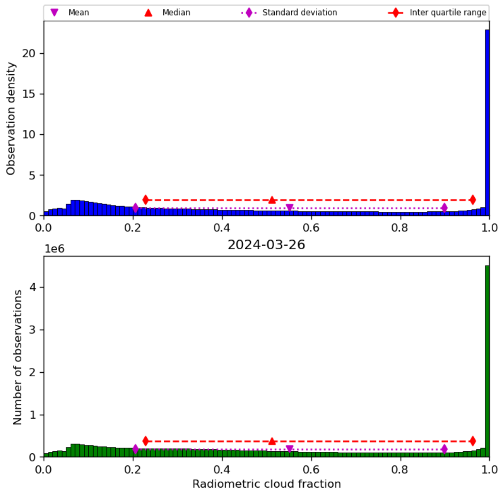
Figure 39: Histogram of “Radiometric cloud fraction” for 2024-03-25 to 2024-03-27
