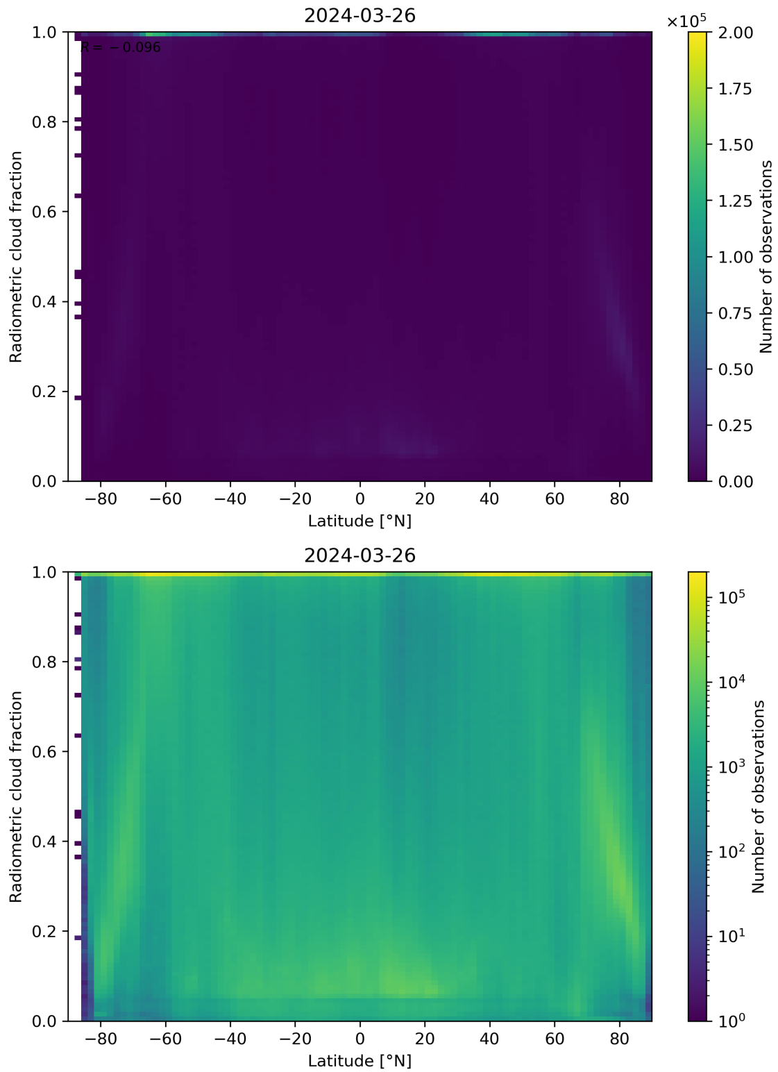
Figure 92: Scatter density plot of “Latitude” against “Radiometric cloud fraction” for 2024-03-25 to 2024-03-27.
