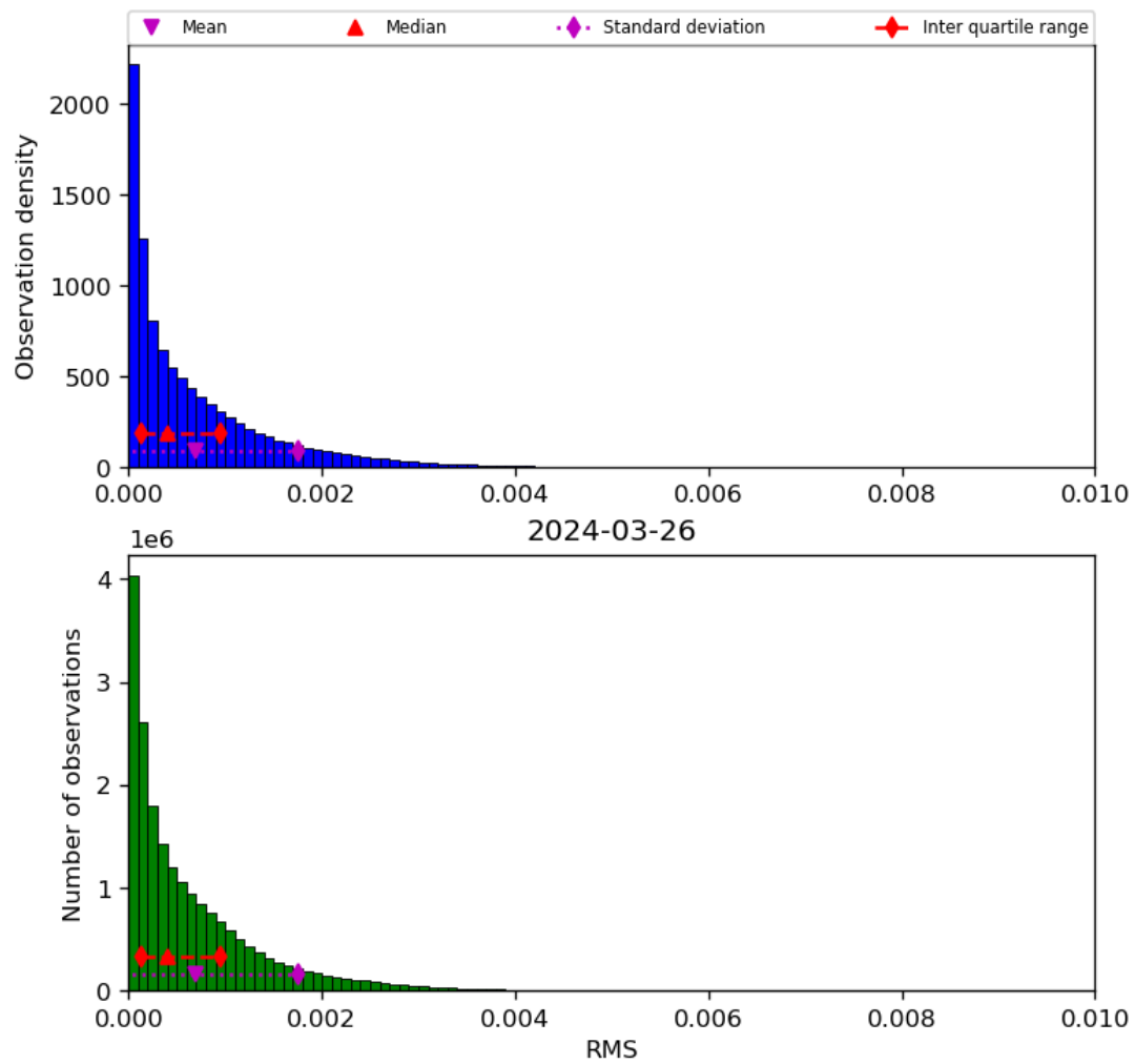
Figure 47: Histogram of “RMS” for 2024-03-25 to 2024-03-27
