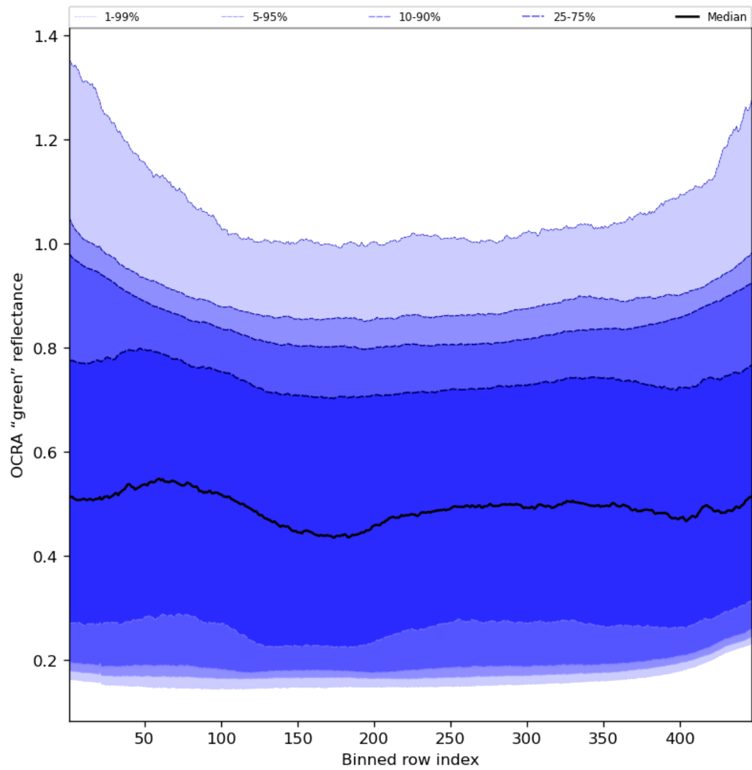
Figure 68: Along track statistics of “OCRA “green” reflectance” for 2024-03-25 to 2024-03-27
