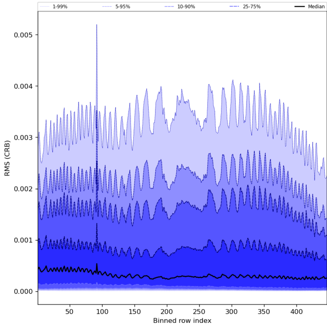
Figure 64: Along track statistics of “RMS (CRB)” for 2024-03-25 to 2024-03-27
