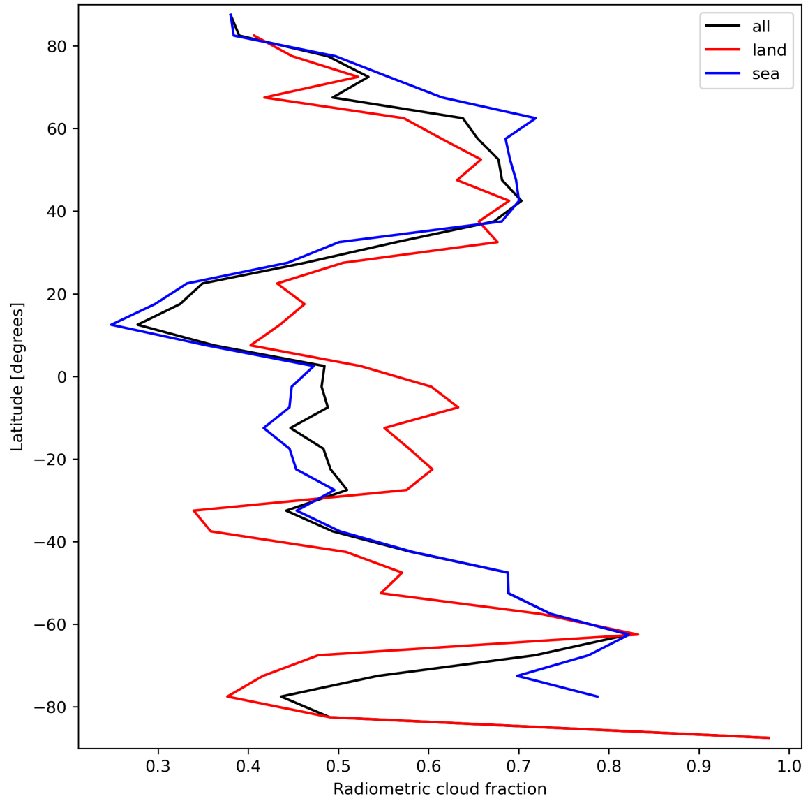
Figure 23: Zonal average of “Radiometric cloud fraction” for 2024-03-25 to 2024-03-27.
