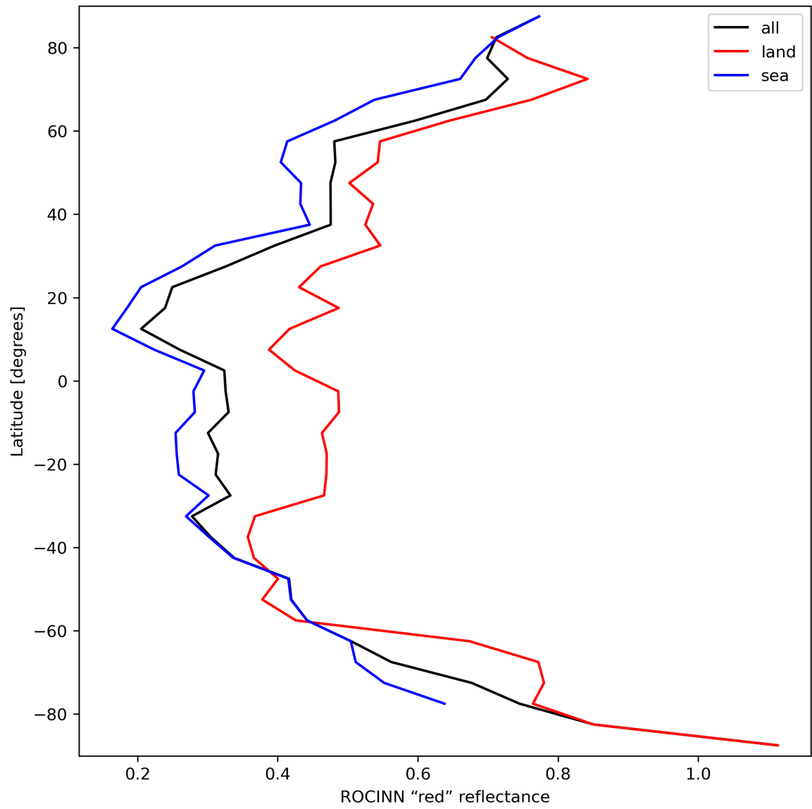
Figure 37: Zonal average of “ROCINN “red” reflectance” for 2024-03-25 to 2024-03-27.
