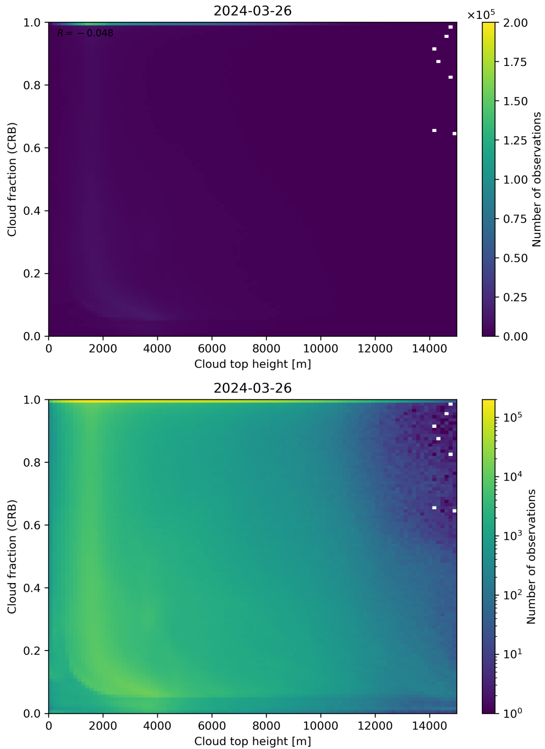
Figure 88: Scatter density plot of “Cloud top height” against “Cloud fraction (CRB)” for 2024-03-25 to 2024-03-27.
