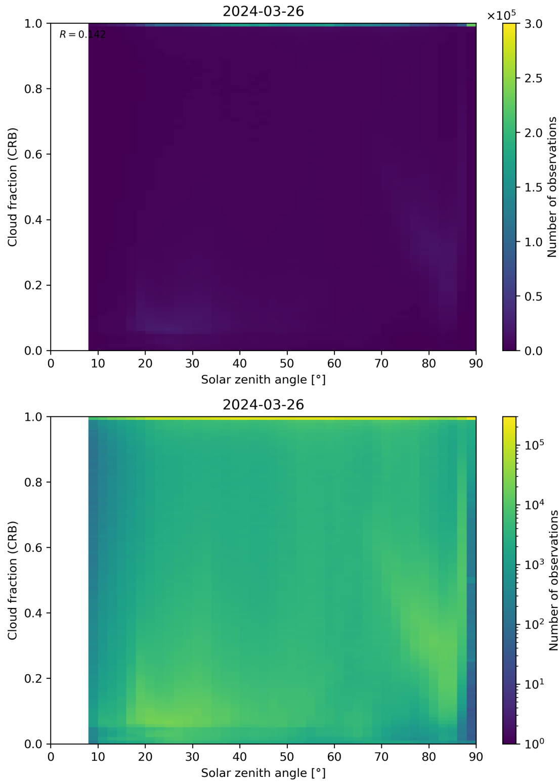
Figure 101: Scatter density plot of “Solar zenith angle” against “Cloud fraction (CRB)” for 2024-03-25 to 2024-03-27.
