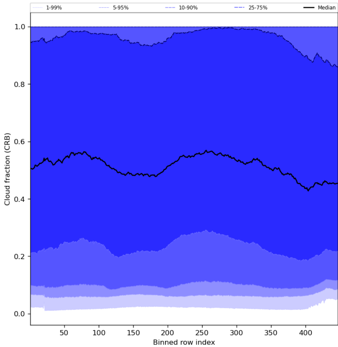
Figure 58: Along track statistics of “Cloud fraction (CRB)” for 2024-03-25 to 2024-03-27
