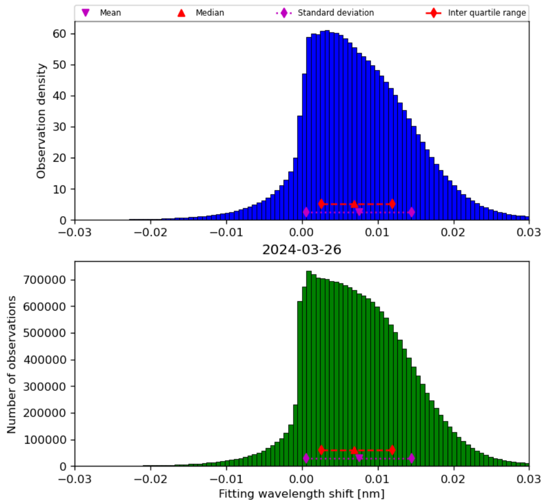
Figure 49: Histogram of “Fitting wavelength shift” for 2024-03-25 to 2024-03-27
