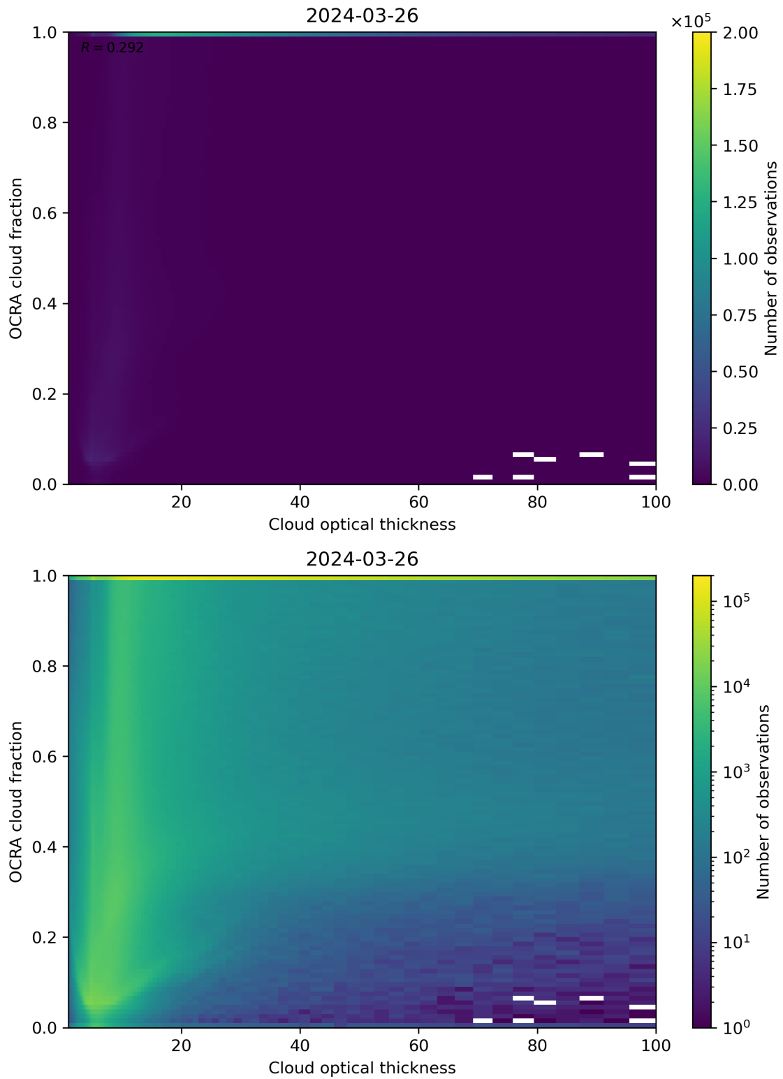
Figure 83: Scatter density plot of “Cloud optical thickness” against “OCRA cloud fraction” for 2024-03-25 to 2024-03-27.
