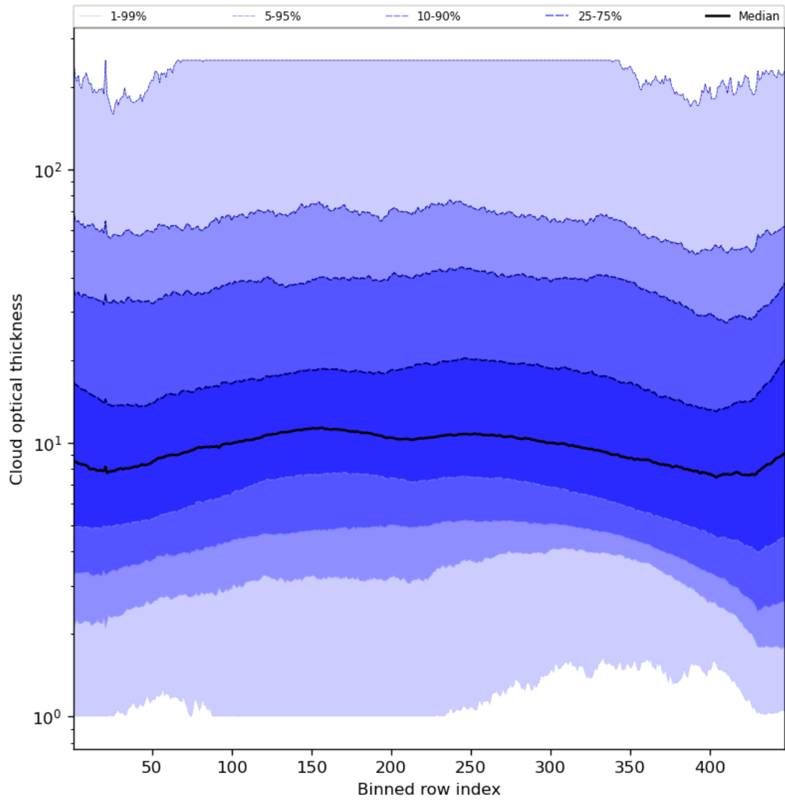
Figure 57: Along track statistics of “Cloud optical thickness” for 2024-03-25 to 2024-03-27
