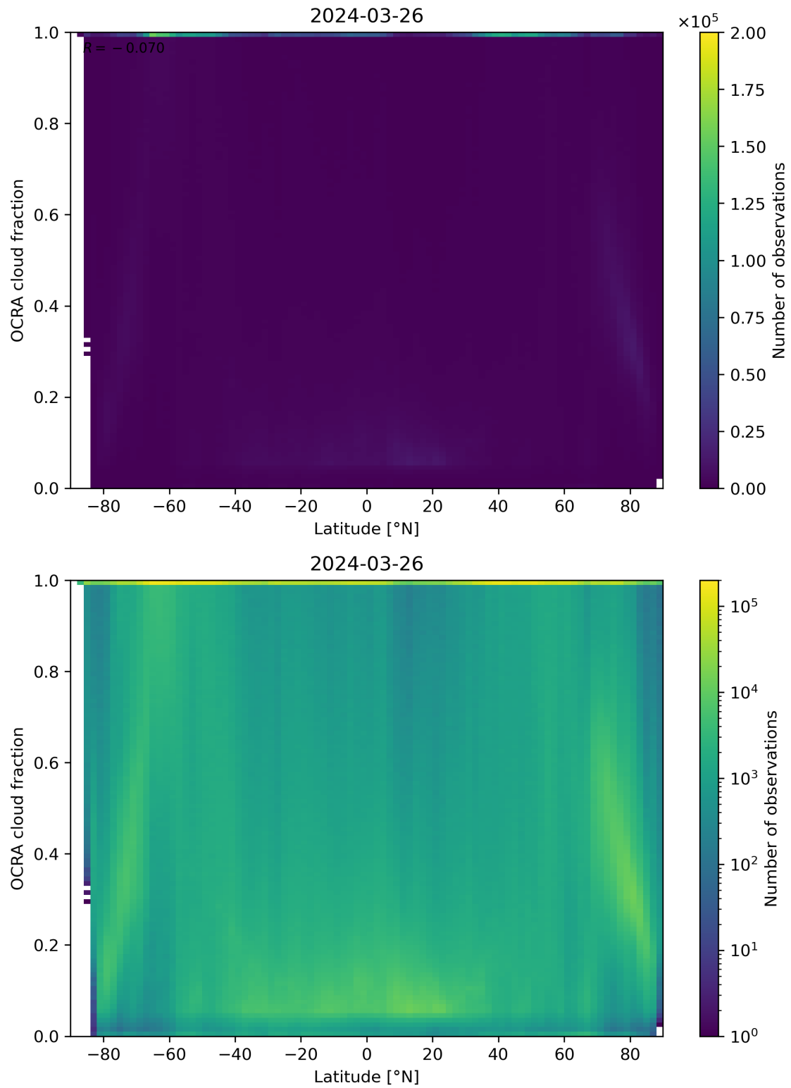
Figure 93: Scatter density plot of “Latitude” against “OCRA cloud fraction” for 2024-03-25 to 2024-03-27.
