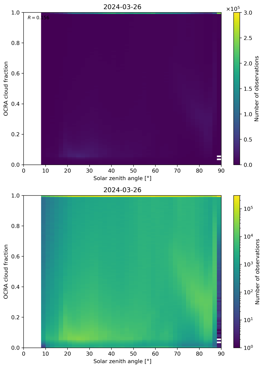
Figure 100: Scatter density plot of “Solar zenith angle” against “OCRA cloud fraction” for 2024-03-25 to 2024-03-27.
