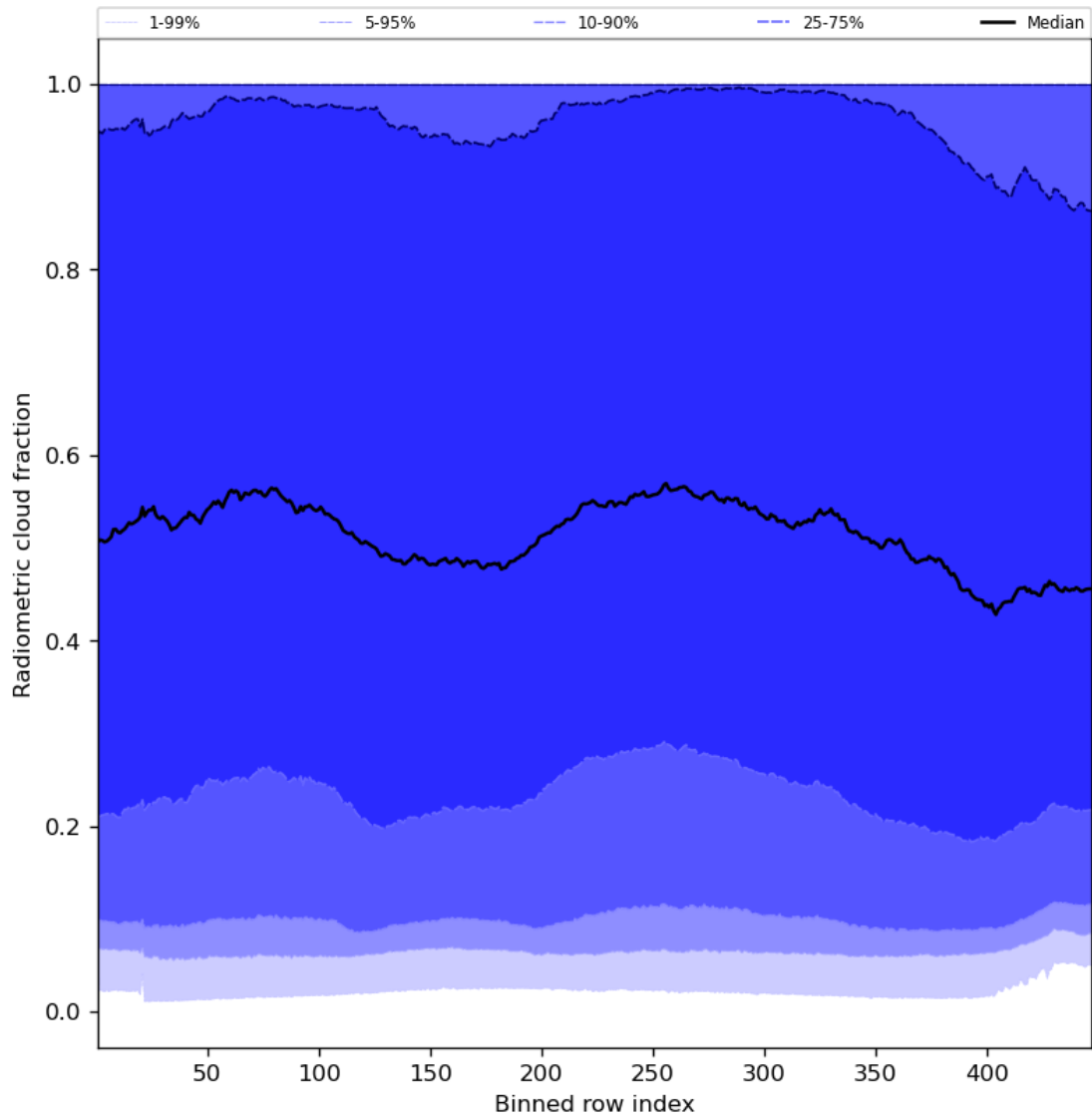
Figure 55: Along track statistics of “Radiometric cloud fraction” for 2024-03-25 to 2024-03-27
