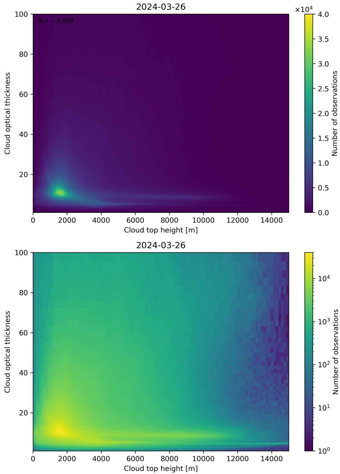
Figure 90: Scatter density plot of “Cloud top height” against “Cloud optical thickness” for 2024-03-25 to 2024-03-27.
