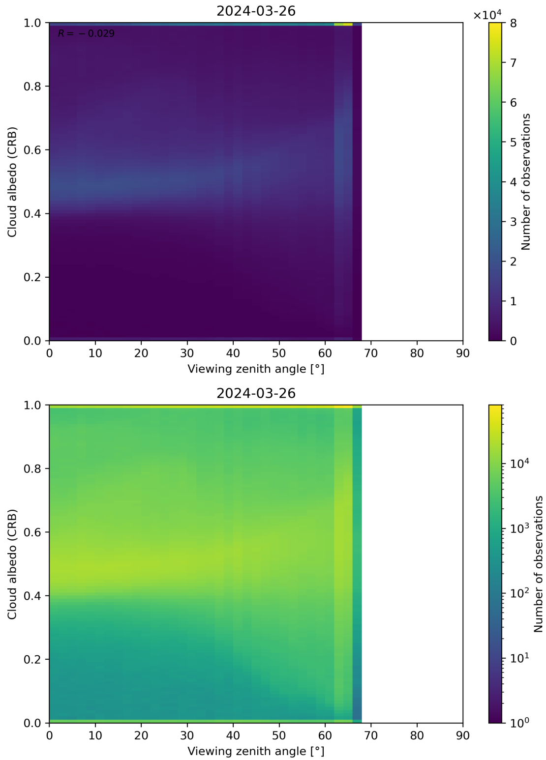
Figure 106: Scatter density plot of “Viewing zenith angle” against “Cloud albedo (CRB)” for 2024-03-25 to 2024-03-27.
