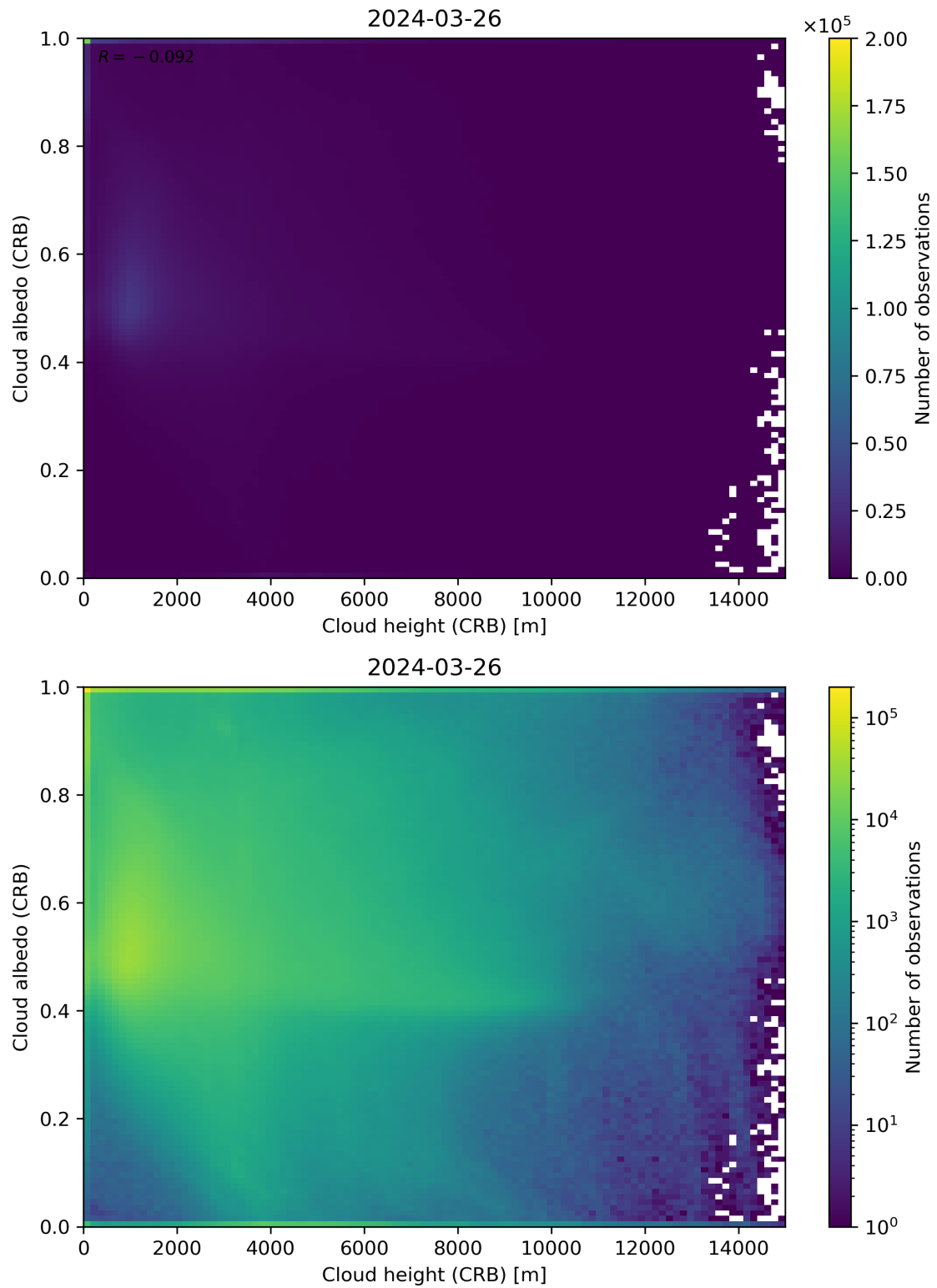
Figure 80: Scatter density plot of “Cloud height (CRB)” against “Cloud albedo (CRB)” for 2024-03-25 to 2024-03-27.
