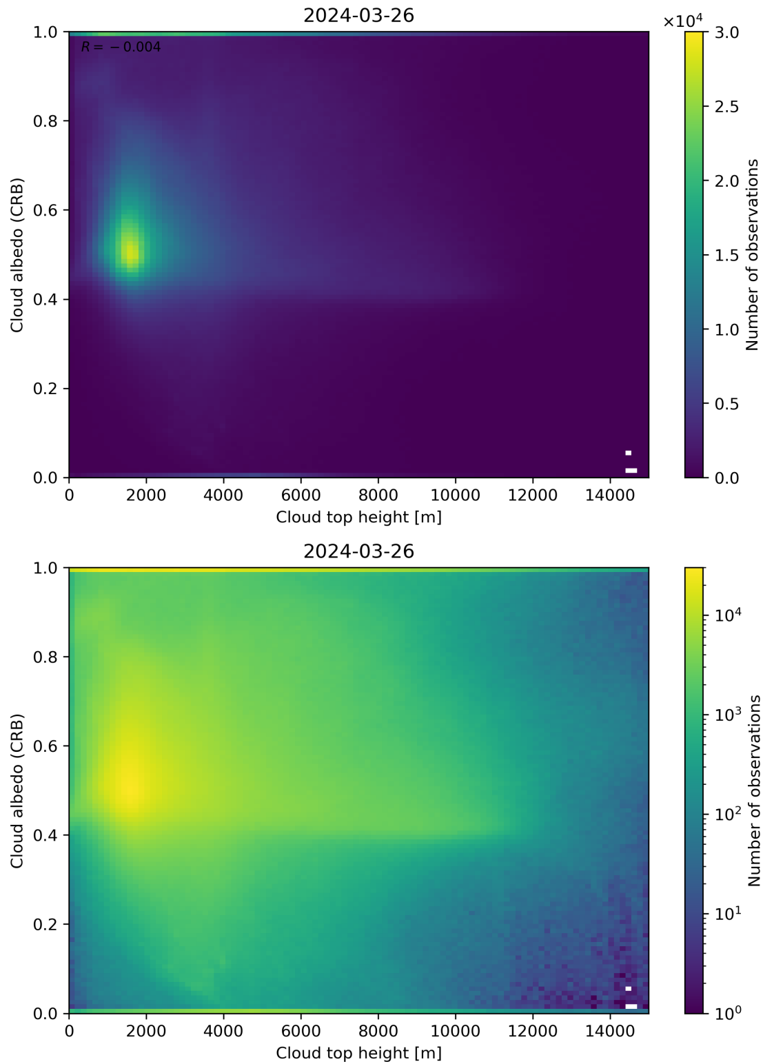
Figure 86: Scatter density plot of “Cloud top height” against “Cloud albedo (CRB)” for 2024-03-25 to 2024-03-27.
