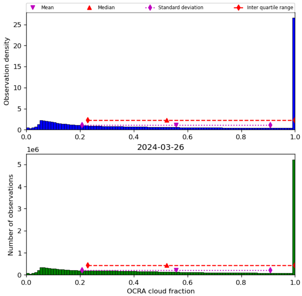
Figure 50: Histogram of “OCRA cloud fraction” for 2024-03-25 to 2024-03-27
