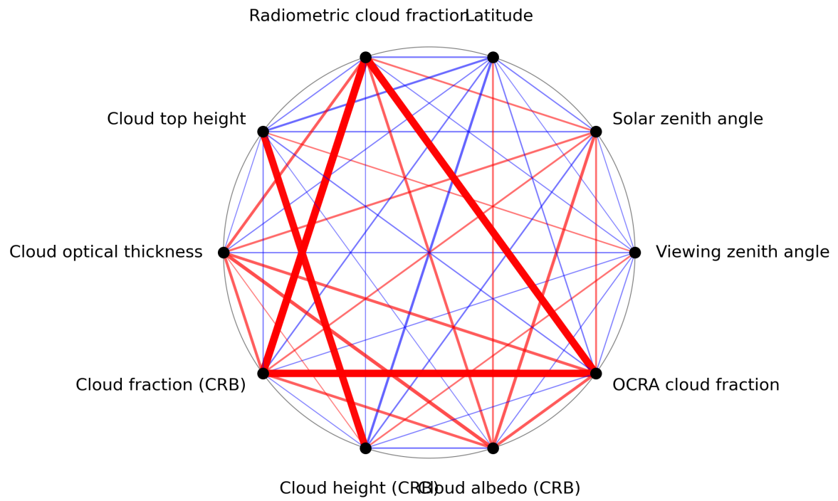
Figure 1: Map of correlation graph for 2024-03-25 to 2024-03-27.
