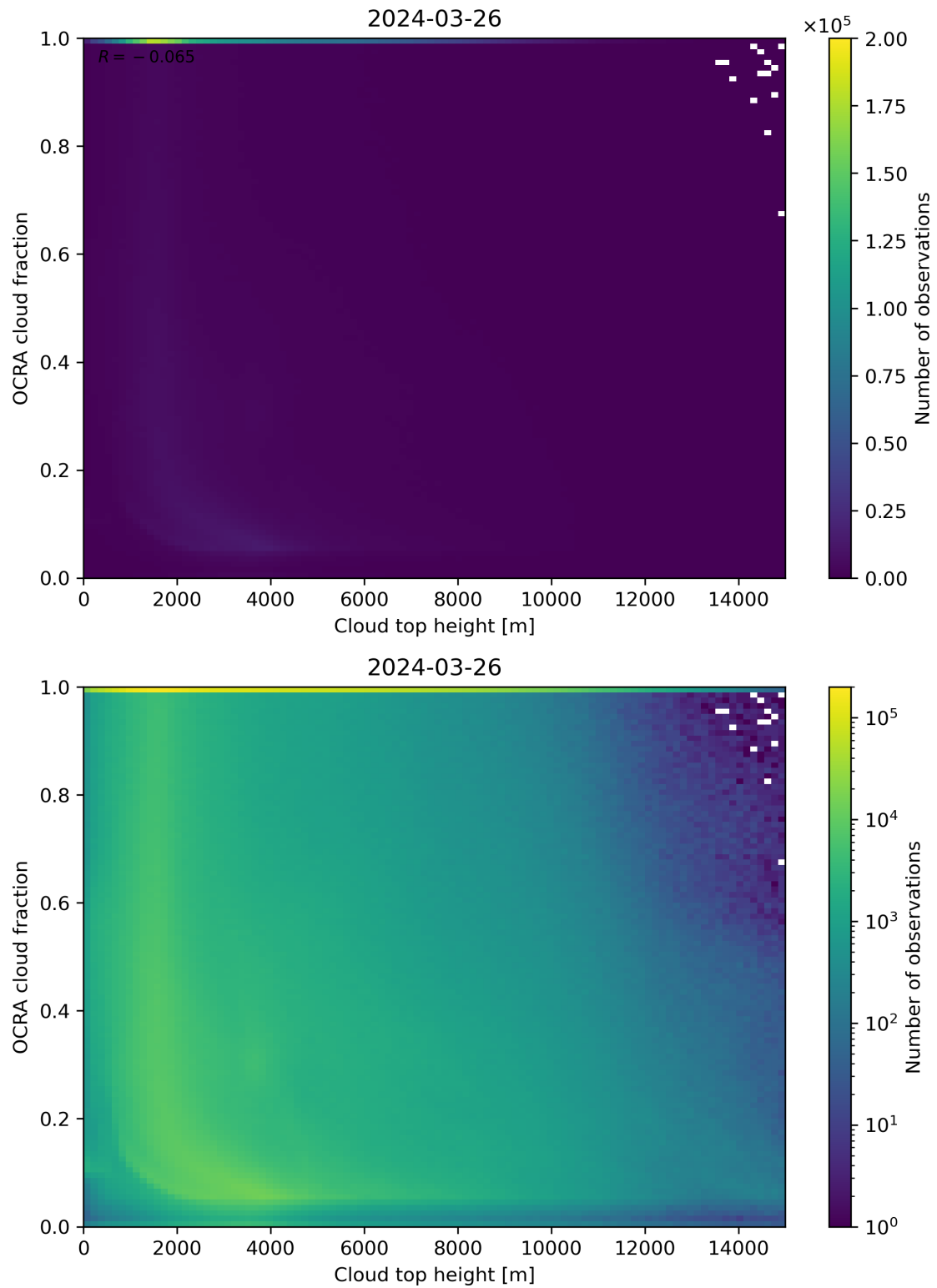
Figure 87: Scatter density plot of “Cloud top height” against “OCRA cloud fraction” for 2024-03-25 to 2024-03-27.
