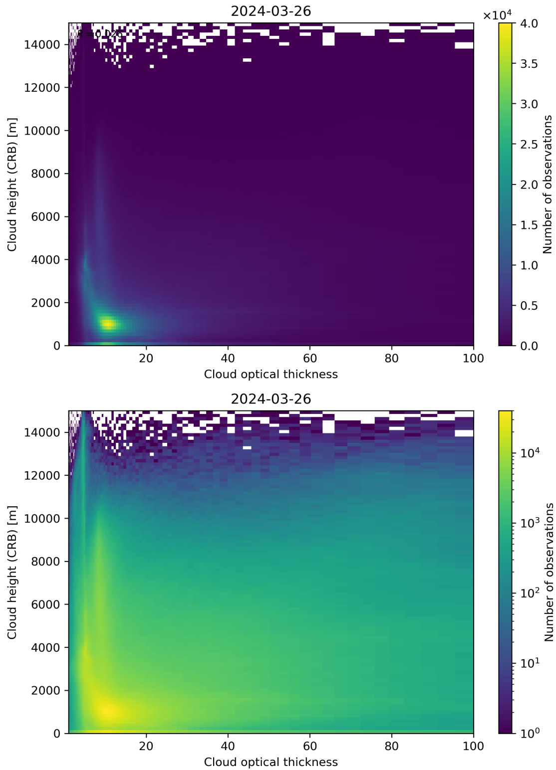
Figure 85: Scatter density plot of “Cloud optical thickness” against “Cloud height (CRB)” for 2024-03-25 to 2024-03-27.
