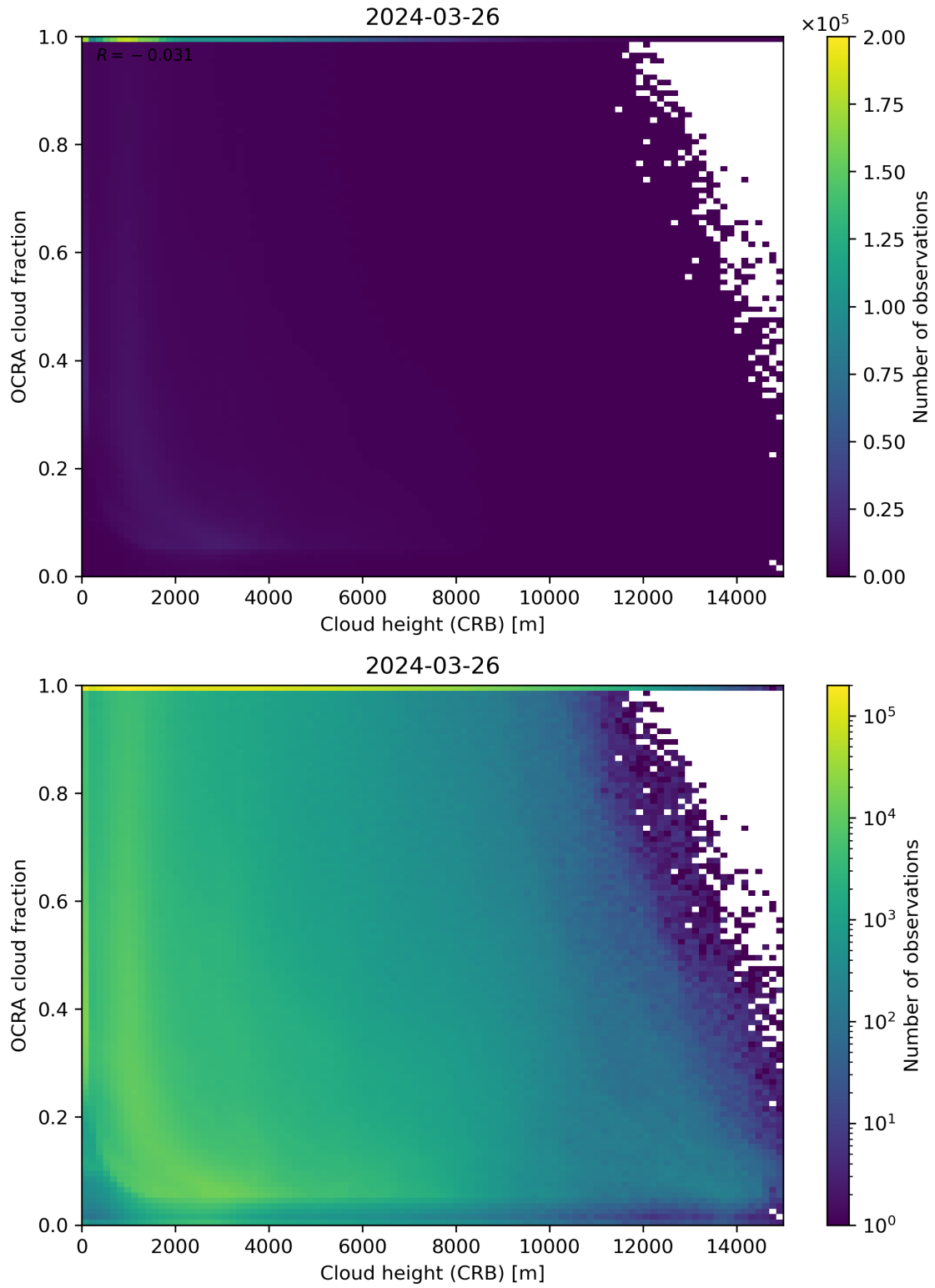
Figure 81: Scatter density plot of “Cloud height (CRB)” against “OCRA cloud fraction” for 2024-03-25 to 2024-03-27.
