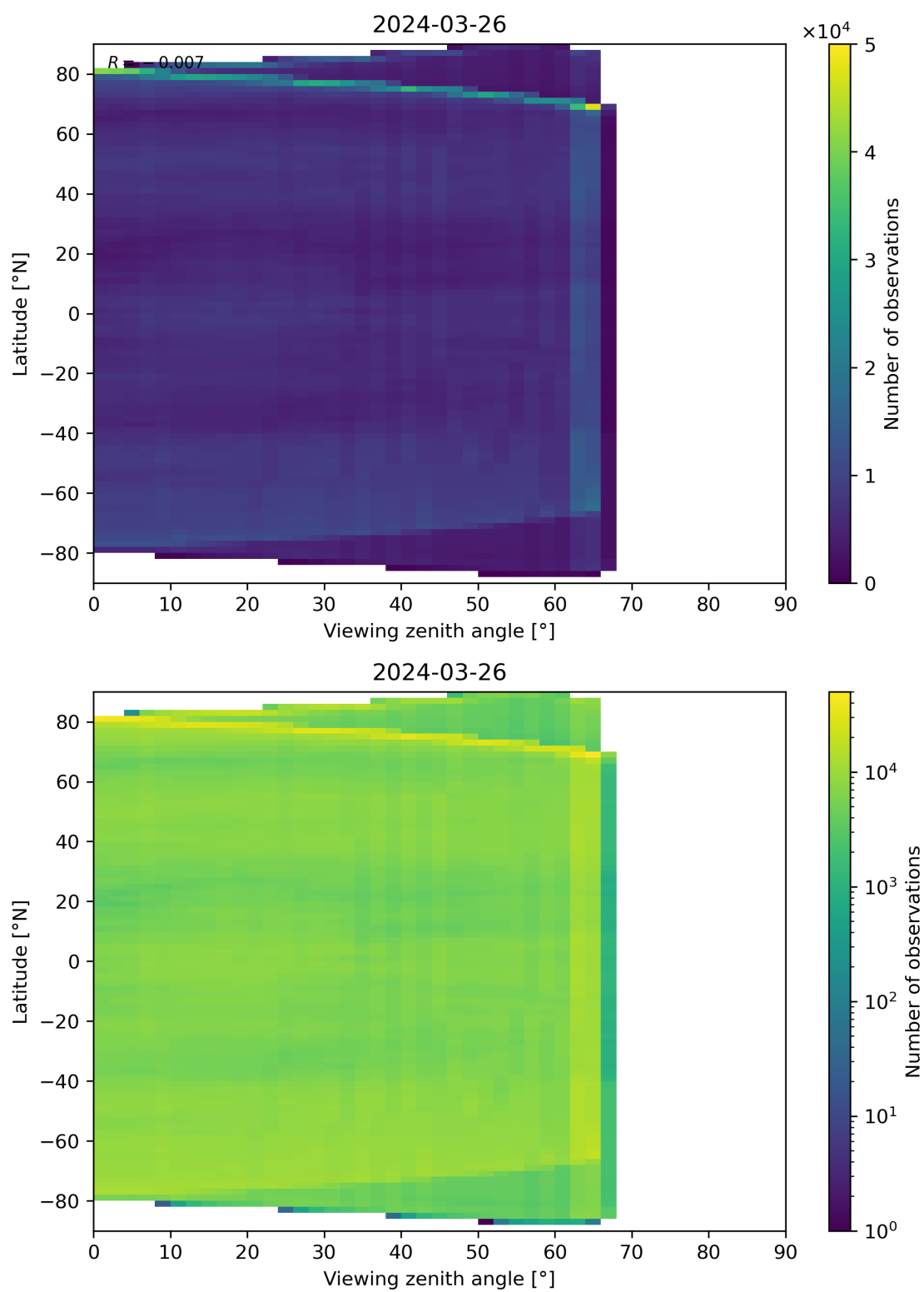
Figure 113: Scatter density plot of “Viewing zenith angle” against “Latitude” for 2024-03-25 to 2024-03-27.
