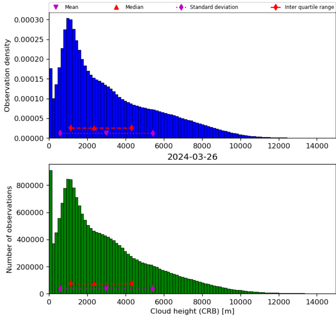
Figure 43: Histogram of “Cloud height (CRB)” for 2024-03-25 to 2024-03-27
