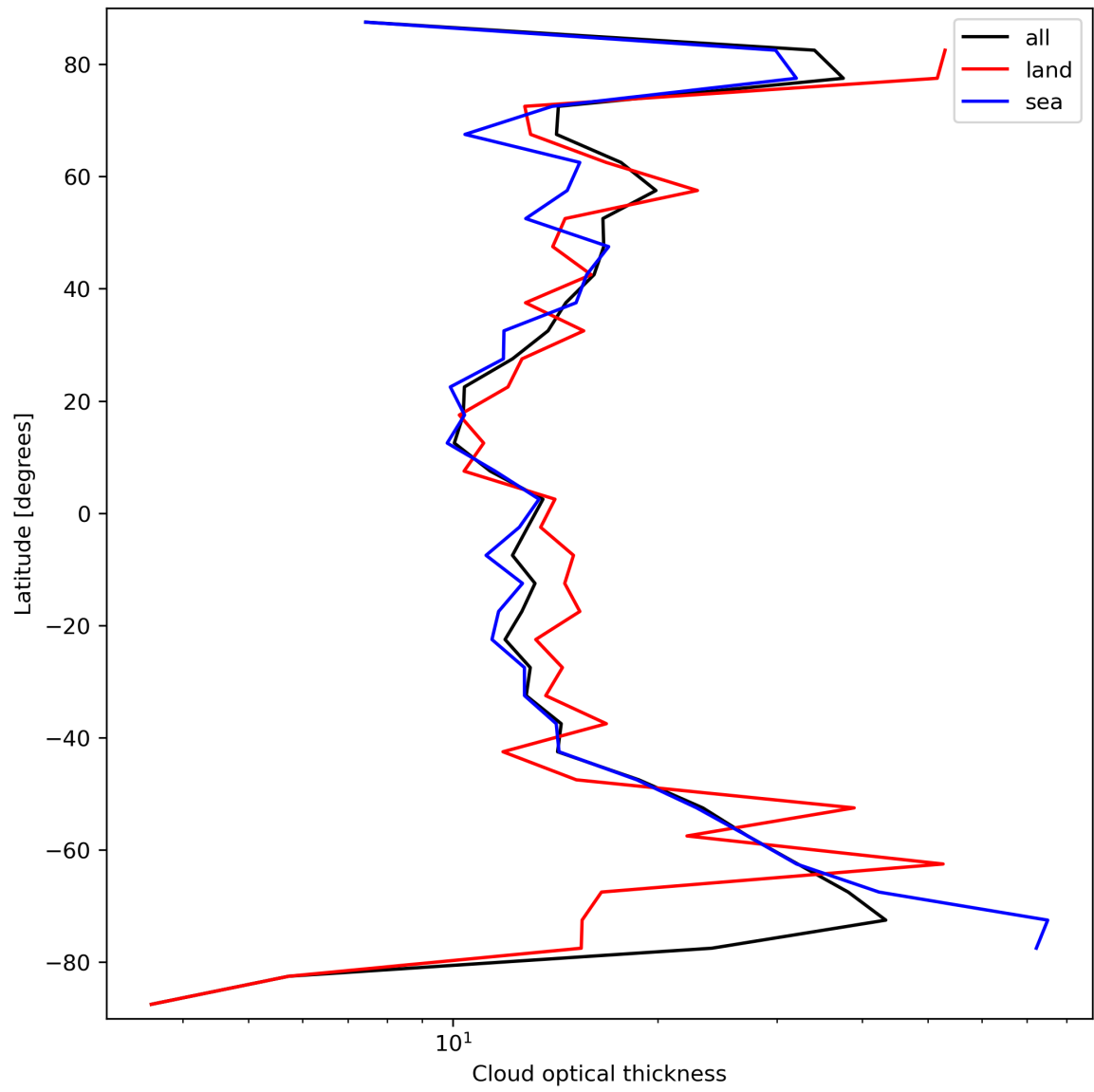
Figure 25: Zonal average of “Cloud optical thickness” for 2024-03-26 to 2024-03-28.
