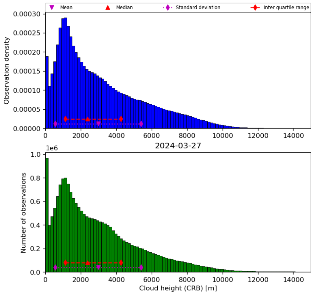
Figure 43: Histogram of “Cloud height (CRB)” for 2024-03-26 to 2024-03-28
