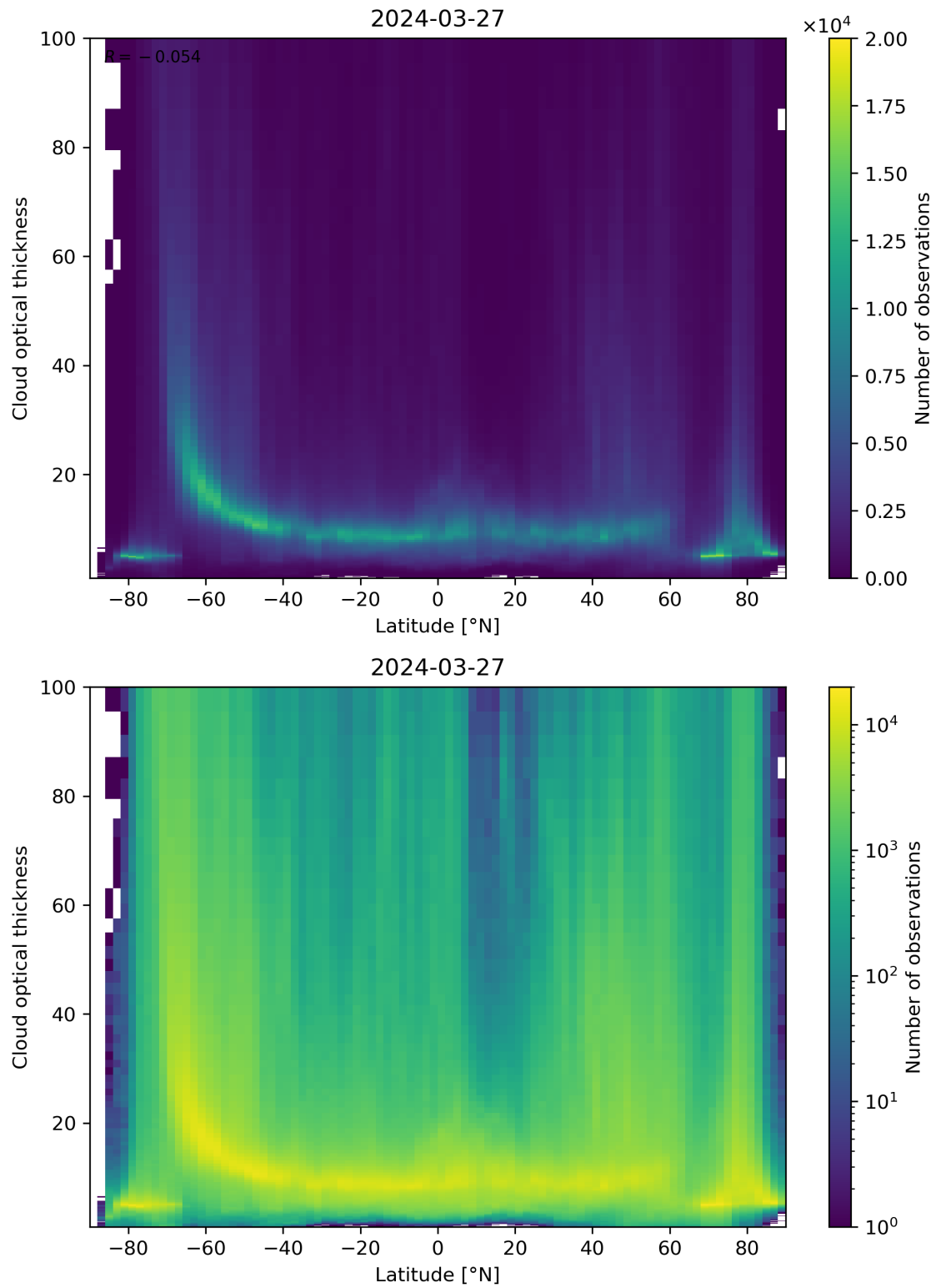
Figure 96: Scatter density plot of “Latitude” against “Cloud optical thickness” for 2024-03-26 to 2024-03-28.
