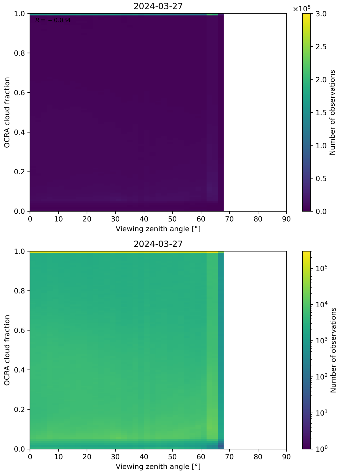
Figure 108: Scatter density plot of “Viewing zenith angle” against “OCRA cloud fraction” for 2024-03-26 to 2024-03-28.
