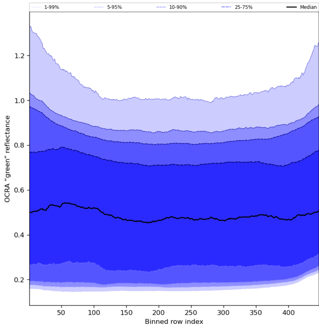
Figure 68: Along track statistics of "OCRA "green" reflectance" for 2024-03-26 to 2024-03-28
