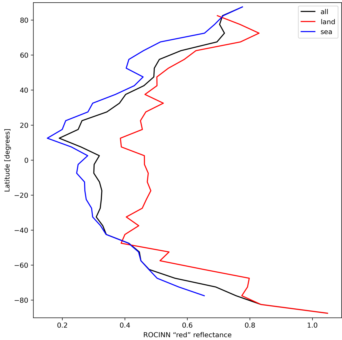
Figure 37: Zonal average of "ROCINN "red" reflectance" for 2024-03-26 to 2024-03-28.
