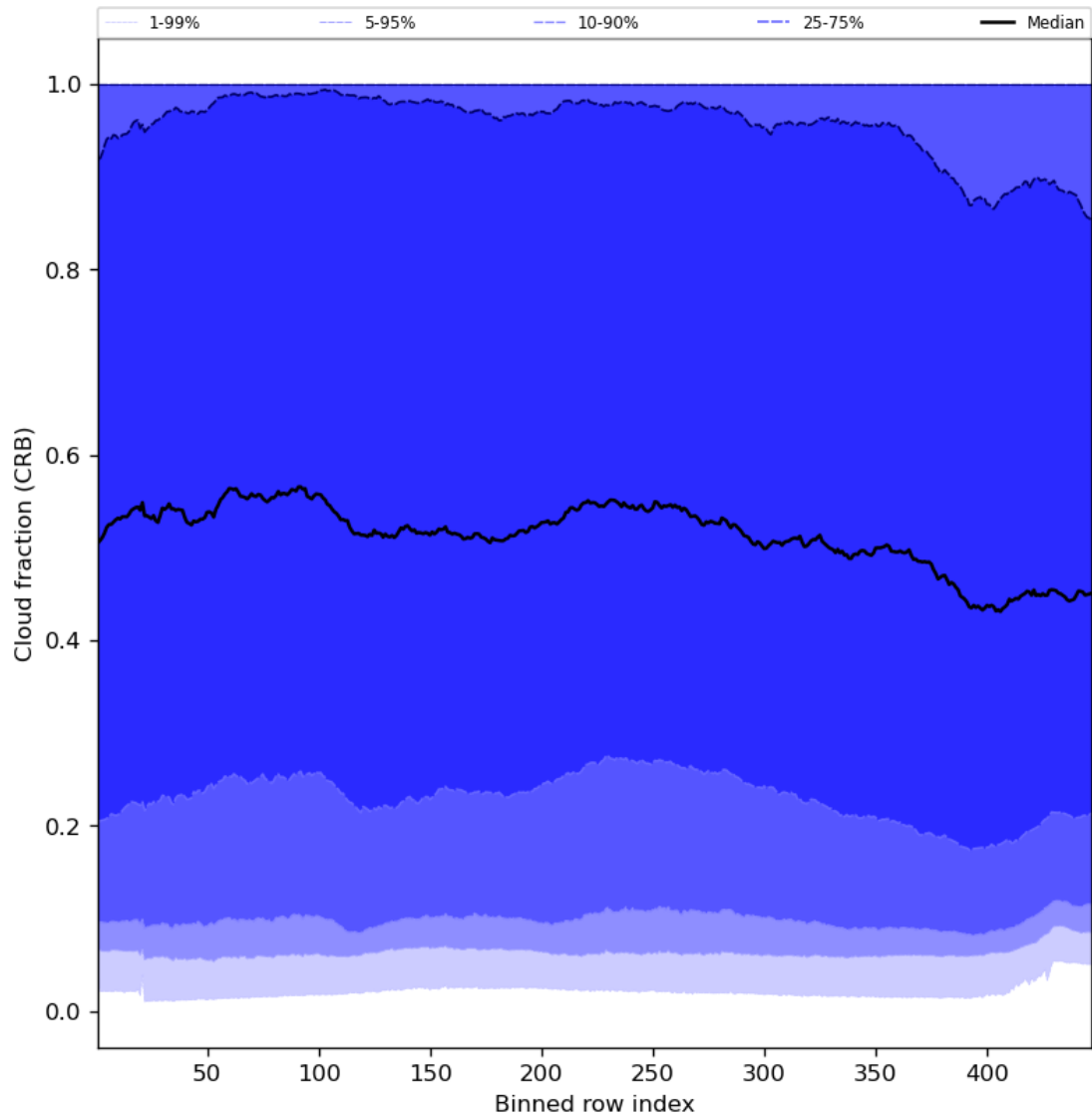
Figure 58: Along track statistics of “Cloud fraction (CRB)” for 2024-03-26 to 2024-03-28
