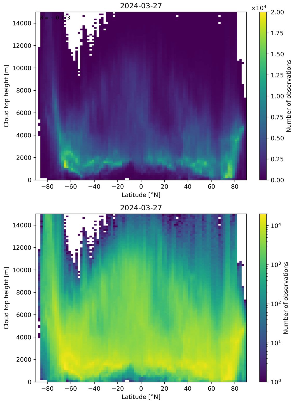
Figure 97: Scatter density plot of “Latitude” against “Cloud top height” for 2024-03-26 to 2024-03-28.
