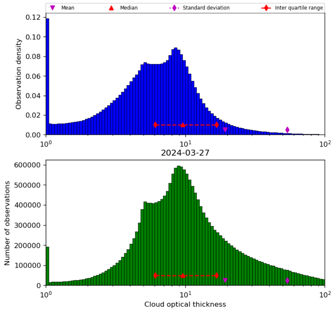
Figure 41: Histogram of “Cloud optical thickness” for 2024-03-26 to 2024-03-28
