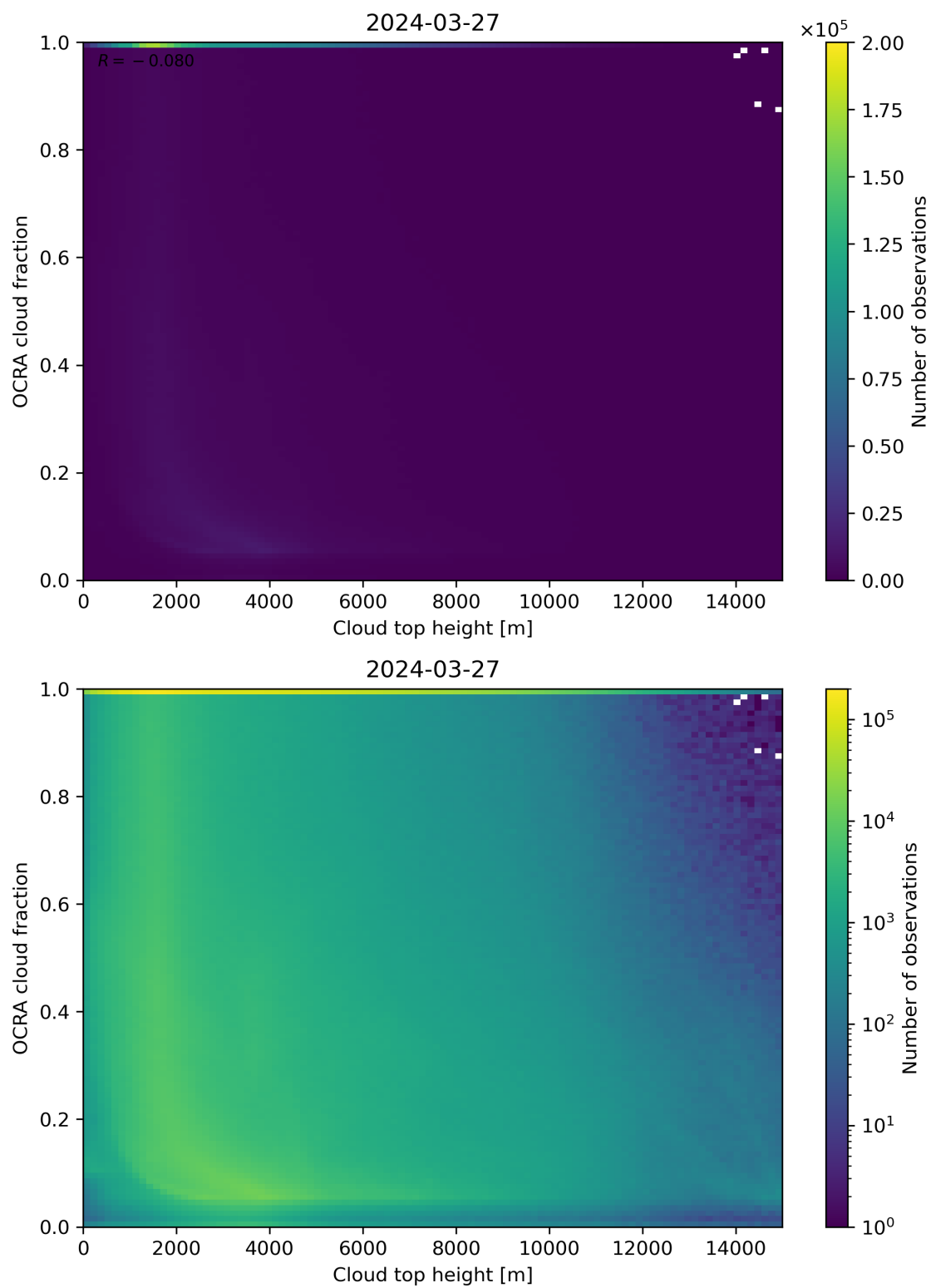
Figure 87: Scatter density plot of “Cloud top height” against “OCRA cloud fraction” for 2024-03-26 to 2024-03-28.
