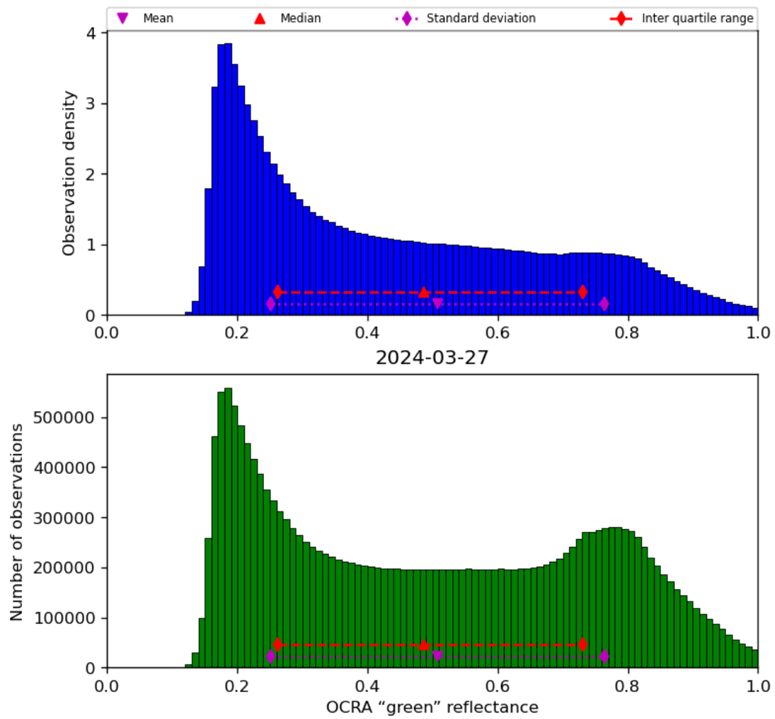
Figure 52: Histogram of “OCRA “green” reflectance” for 2024-03-26 to 2024-03-28
