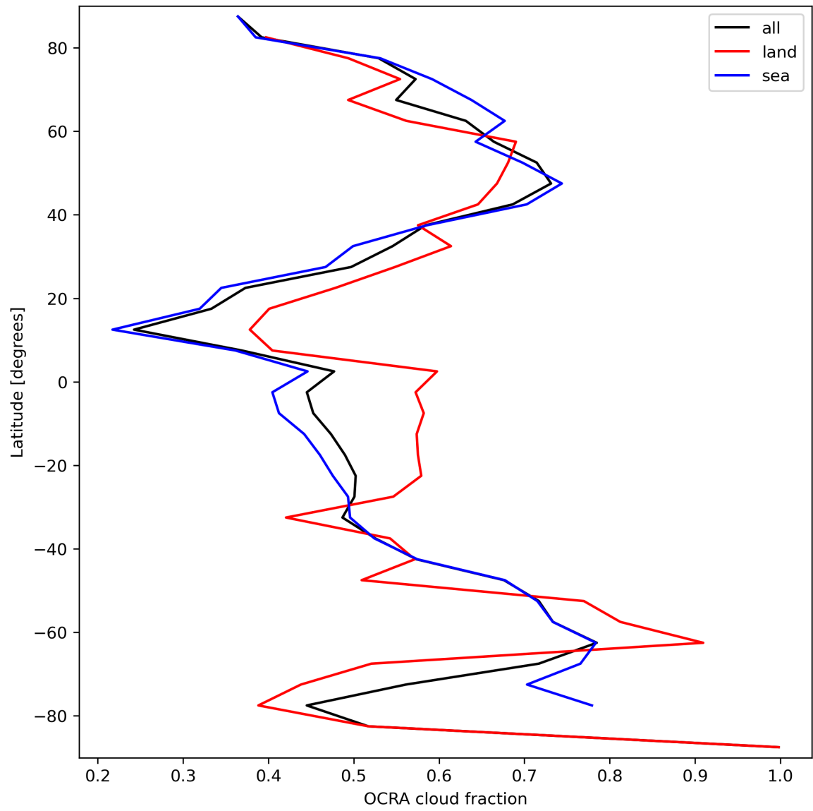
Figure 34: Zonal average of “OCRA cloud fraction” for 2024-03-26 to 2024-03-28.
