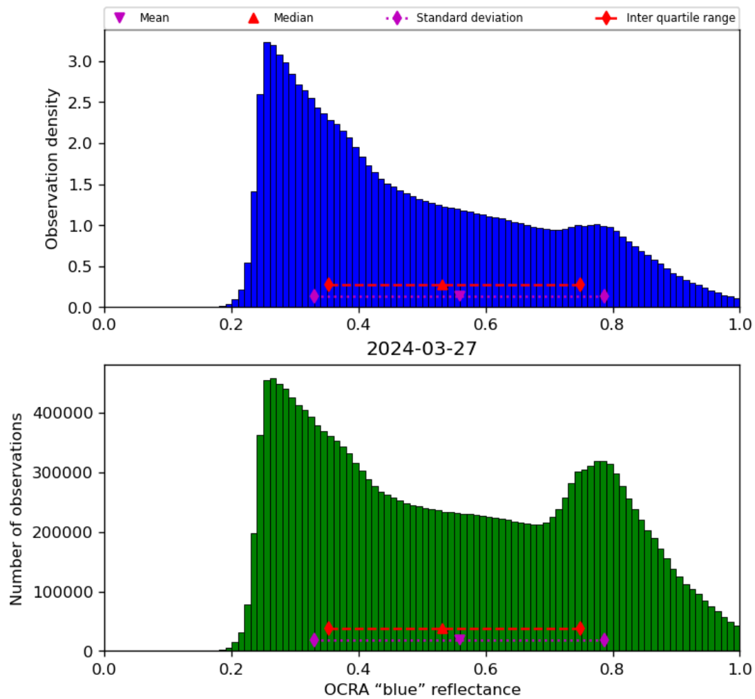
Figure 51: Histogram of “OCRA “blue” reflectance” for 2024-03-26 to 2024-03-28
