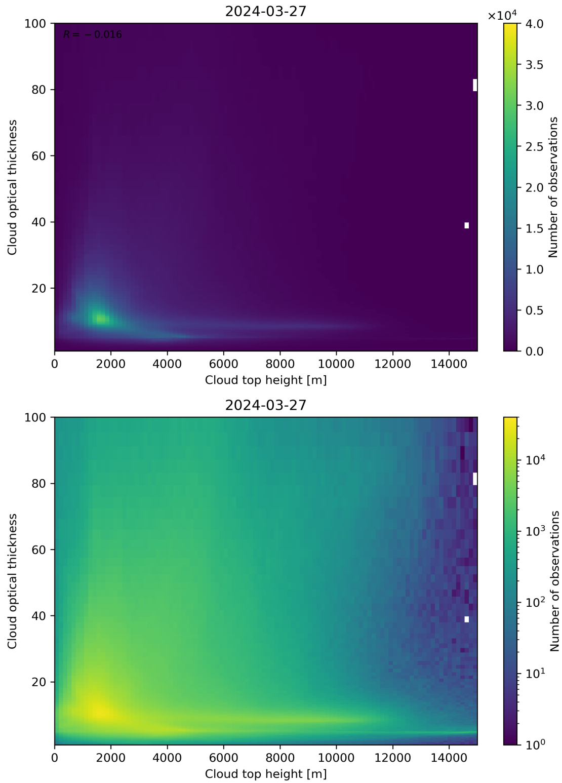
Figure 90: Scatter density plot of “Cloud top height” against “Cloud optical thickness” for 2024-03-26 to 2024-03-28.
