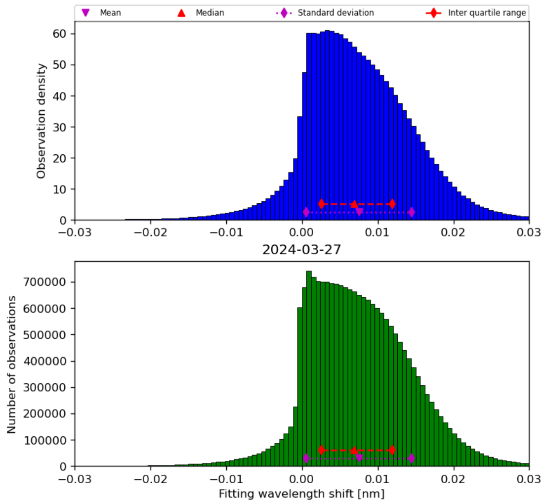
Figure 49: Histogram of “Fitting wavelength shift” for 2024-03-26 to 2024-03-28
