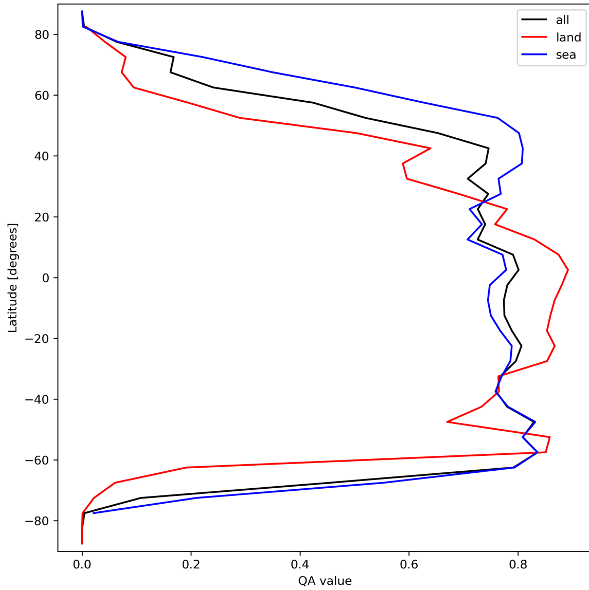
Figure 22: Zonal average of “QA value” for 2024-03-26 to 2024-03-28.
