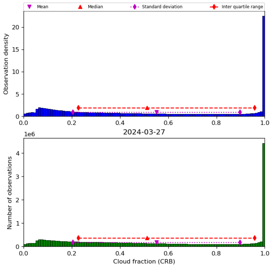
Figure 42: Histogram of “Cloud fraction (CRB)” for 2024-03-26 to 2024-03-28
