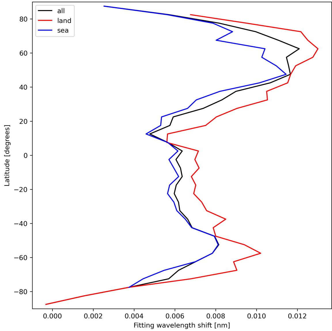
Figure 33: Zonal average of “Fitting wavelength shift” for 2024-03-26 to 2024-03-28.
