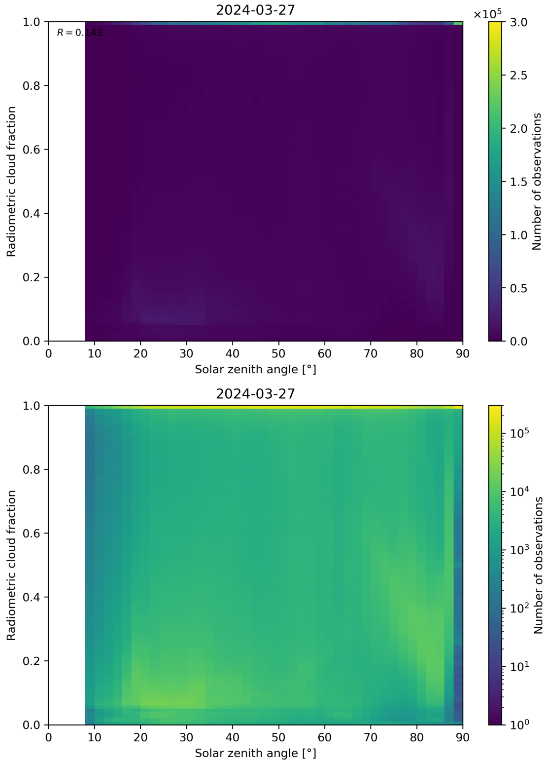
Figure 99: Scatter density plot of “Solar zenith angle” against “Radiometric cloud fraction” for 2024-03-26 to 2024-03-28.
