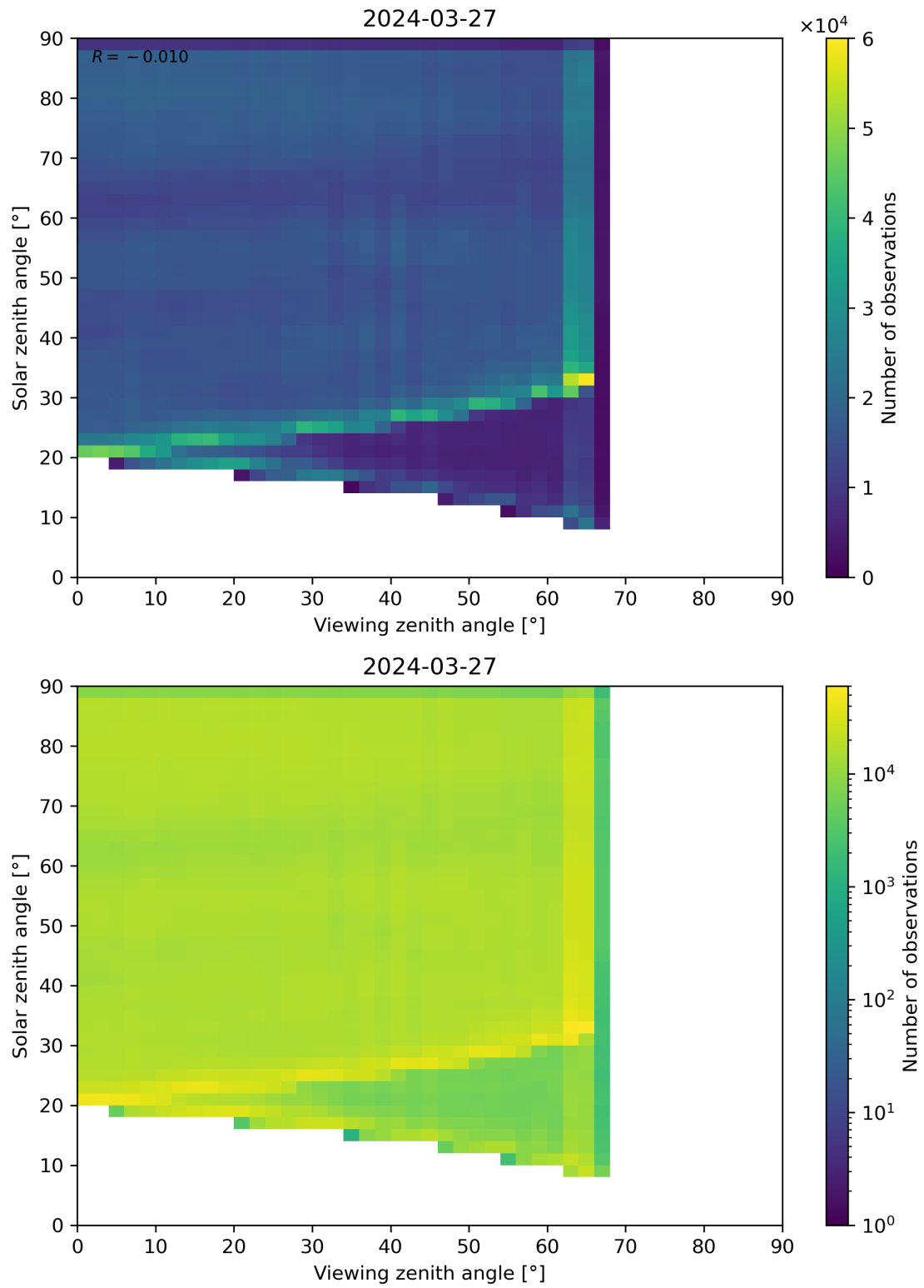
Figure 114: Scatter density plot of “Viewing zenith angle” against “Solar zenith angle” for 2024-03-26 to 2024-03-28.
