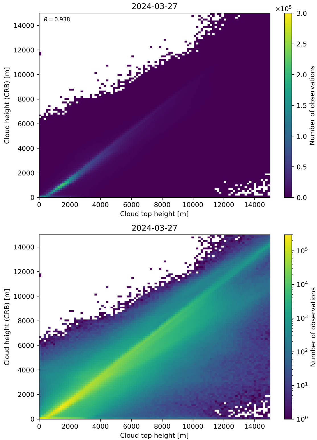
Figure 89: Scatter density plot of “Cloud top height” against “Cloud height (CRB)” for 2024-03-26 to 2024-03-28.
