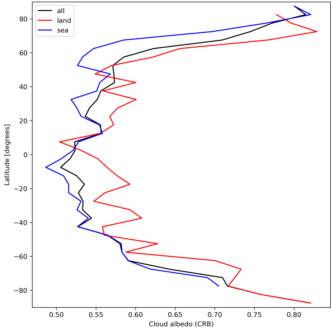
Figure 28: Zonal average of “Cloud albedo (CRB)” for 2024-03-26 to 2024-03-28.
