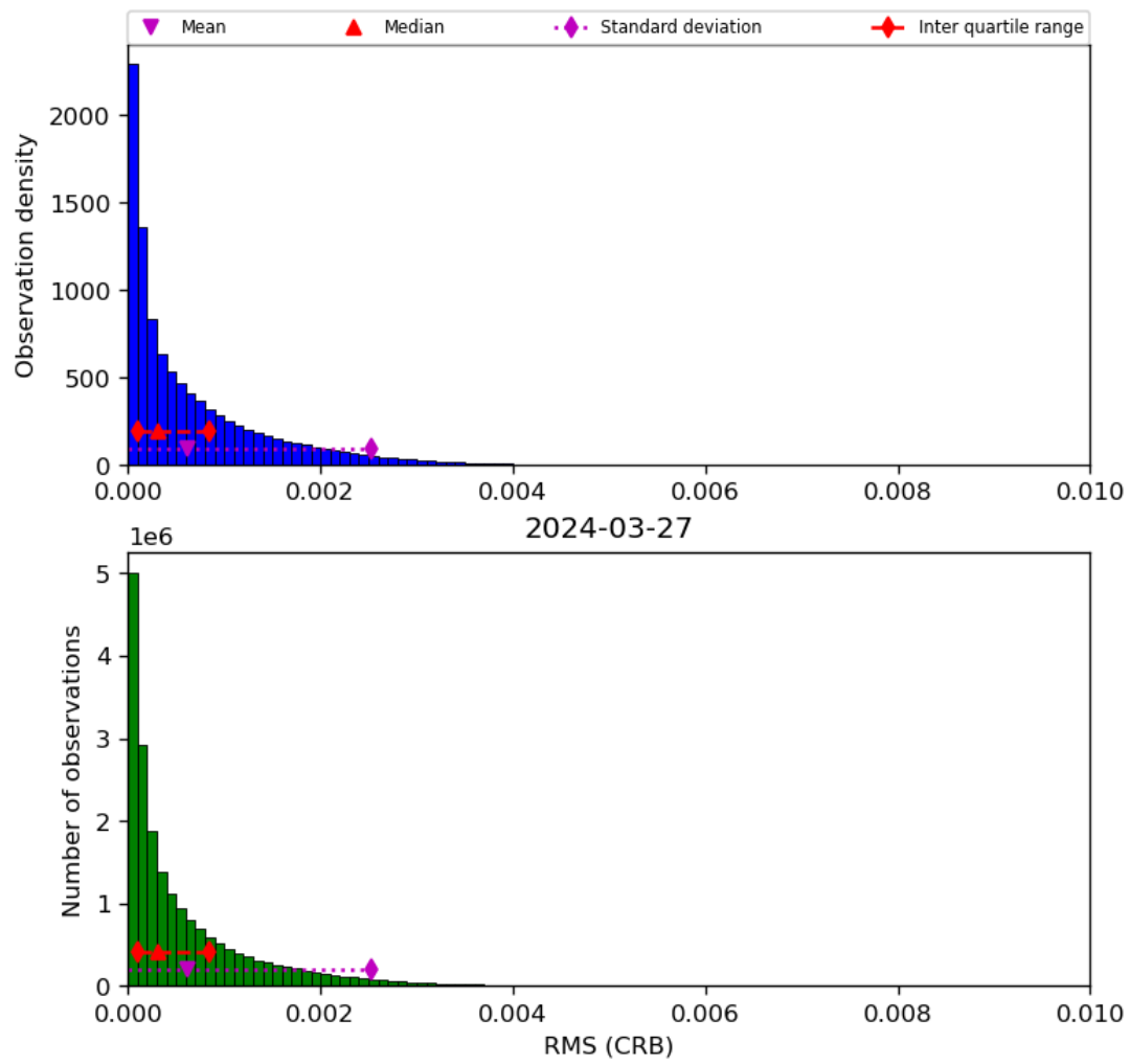
Figure 48: Histogram of “RMS (CRB)” for 2024-03-26 to 2024-03-28
