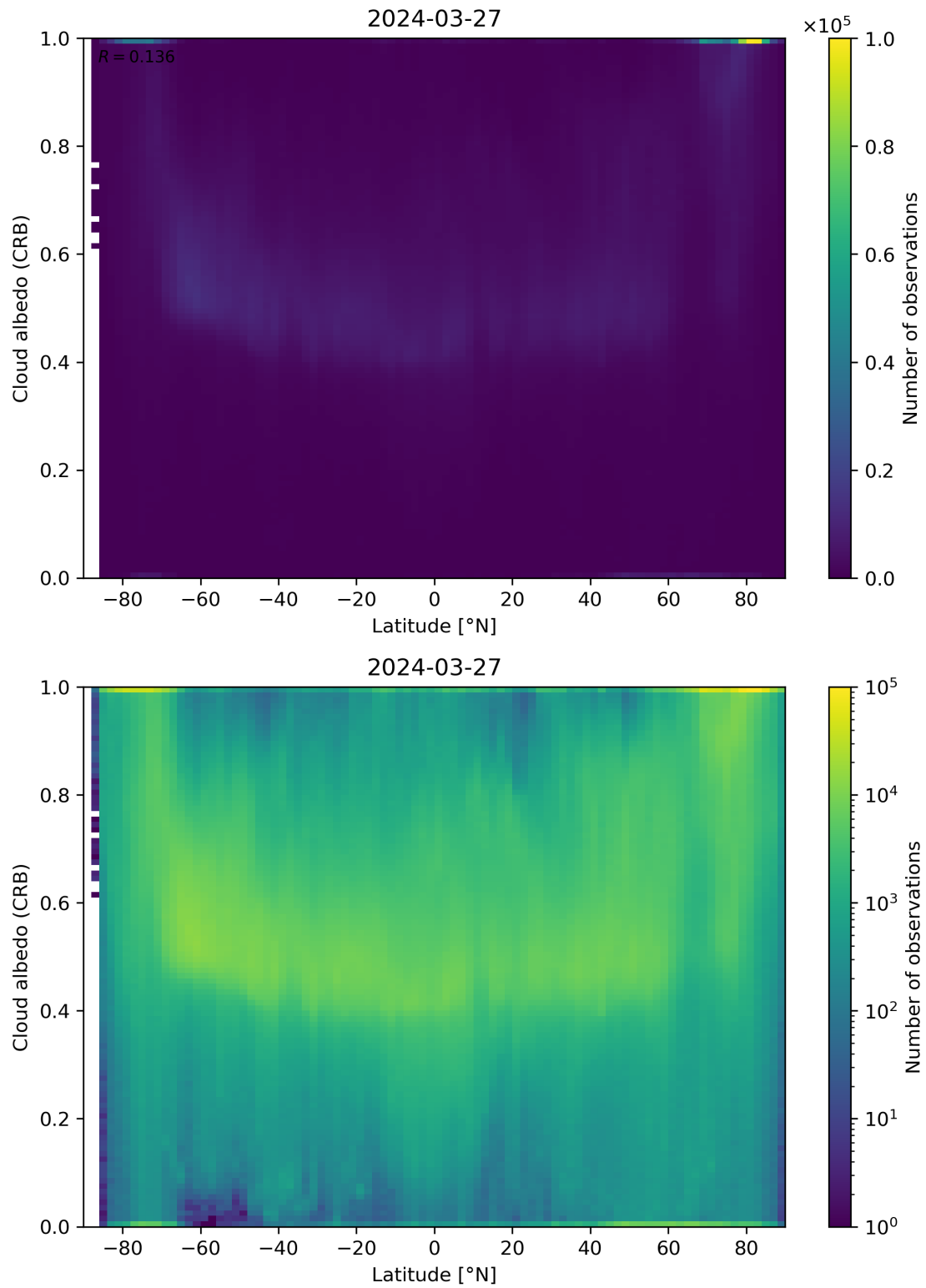
Figure 91: Scatter density plot of “Latitude” against “Cloud albedo (CRB)” for 2024-03-26 to 2024-03-28.
