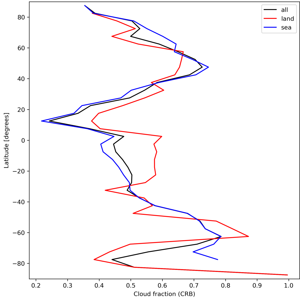
Figure 26: Zonal average of “Cloud fraction (CRB)” for 2024-03-26 to 2024-03-28.
