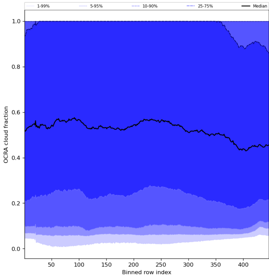
Figure 66: Along track statistics of “OCRA cloud fraction” for 2024-03-26 to 2024-03-28
