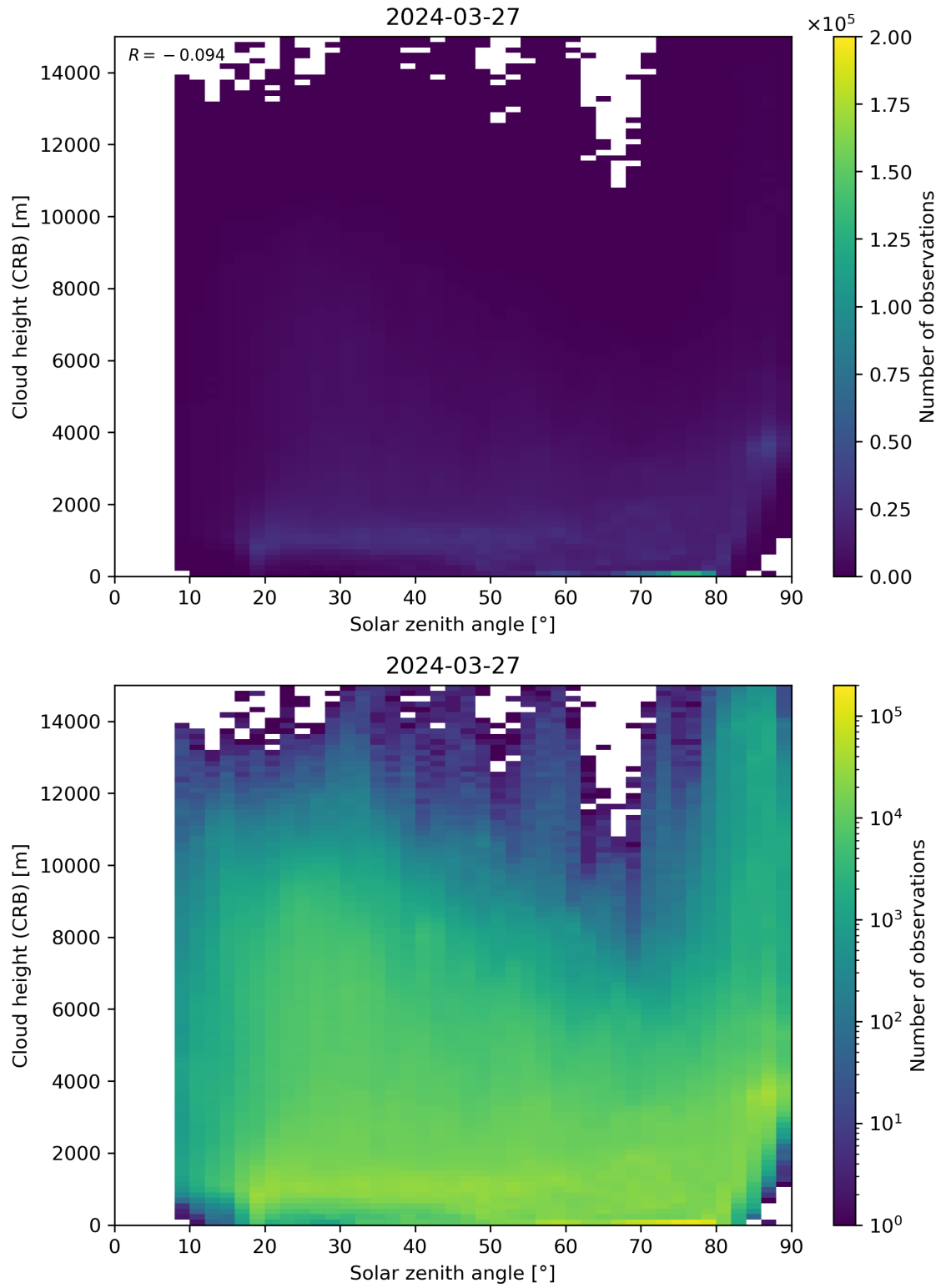
Figure 102: Scatter density plot of “Solar zenith angle” against “Cloud height (CRB)” for 2024-03-26 to 2024-03-28.
