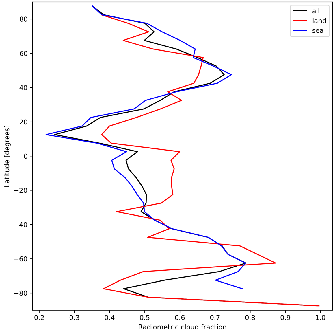
Figure 23: Zonal average of “Radiometric cloud fraction” for 2024-03-26 to 2024-03-28.
