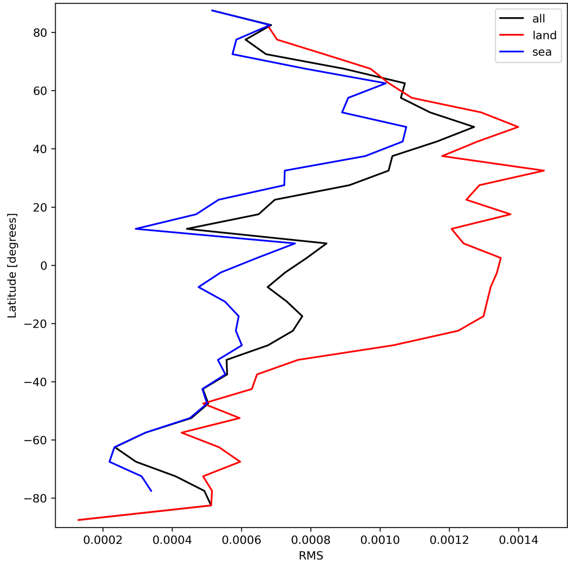
Figure 31: Zonal average of “RMS” for 2024-03-26 to 2024-03-28.
