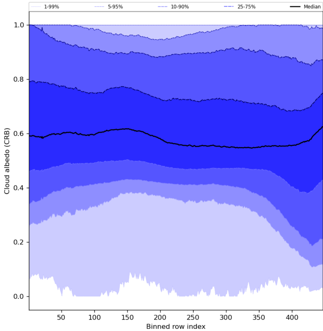
Figure 60: Along track statistics of “Cloud albedo (CRB)” for 2024-03-26 to 2024-03-28
