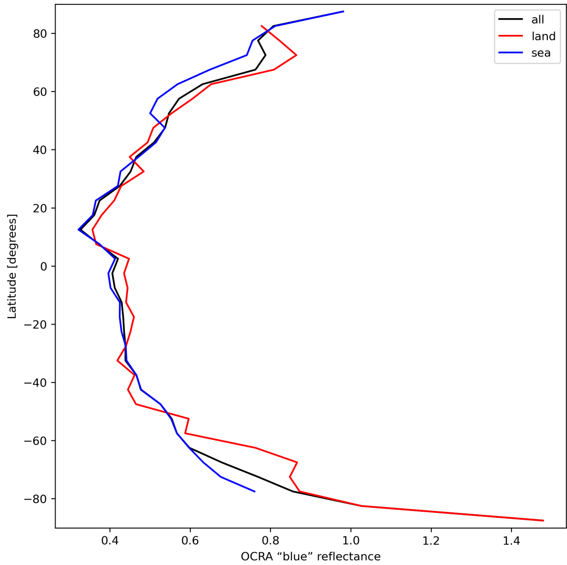
Figure 35: Zonal average of "OCRA "blue" reflectance" for 2024-03-26 to 2024-03-28.
