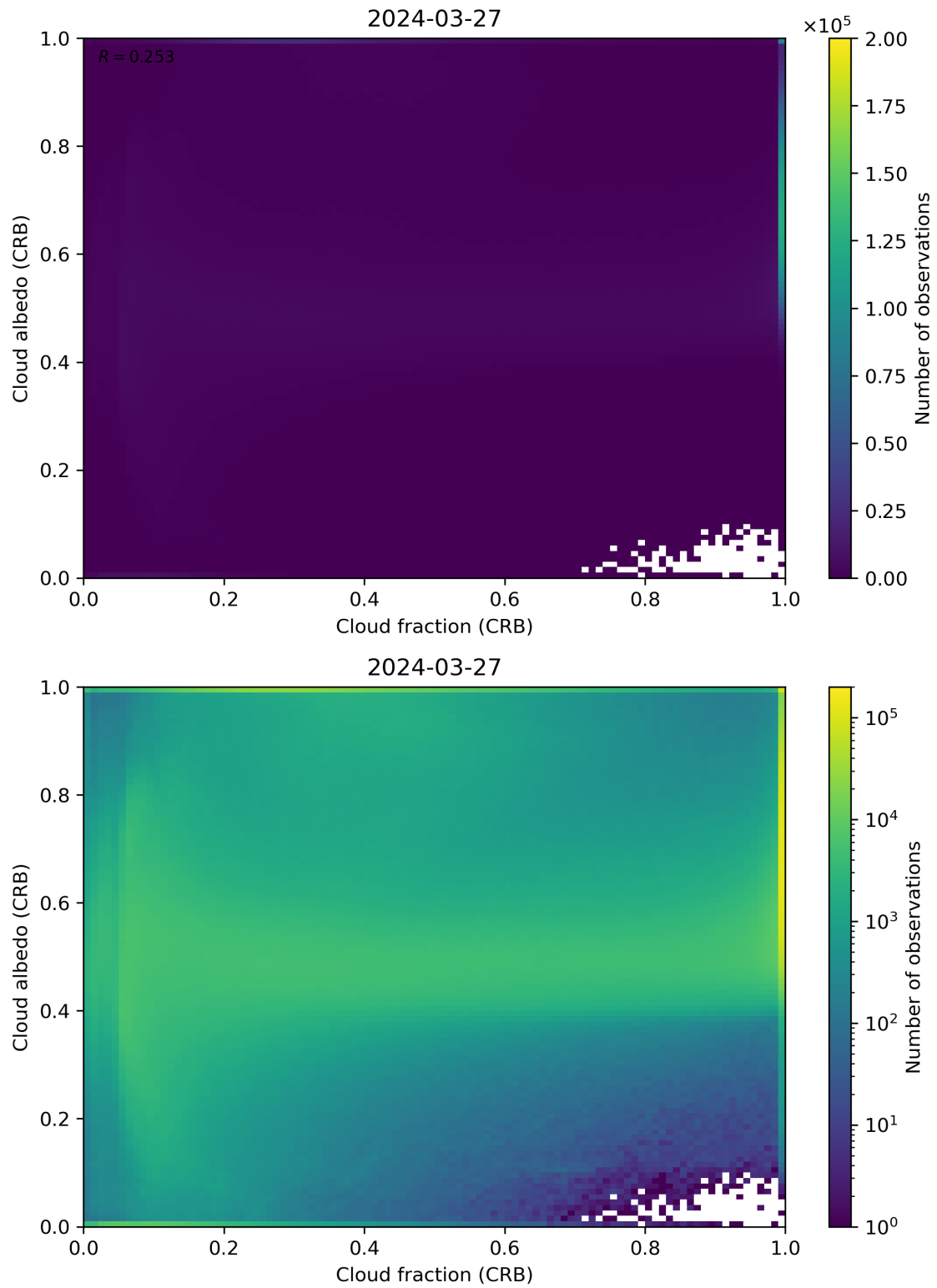
Figure 77: Scatter density plot of “Cloud fraction (CRB)” against “Cloud albedo (CRB)” for 2024-03-26 to 2024-03-28.
