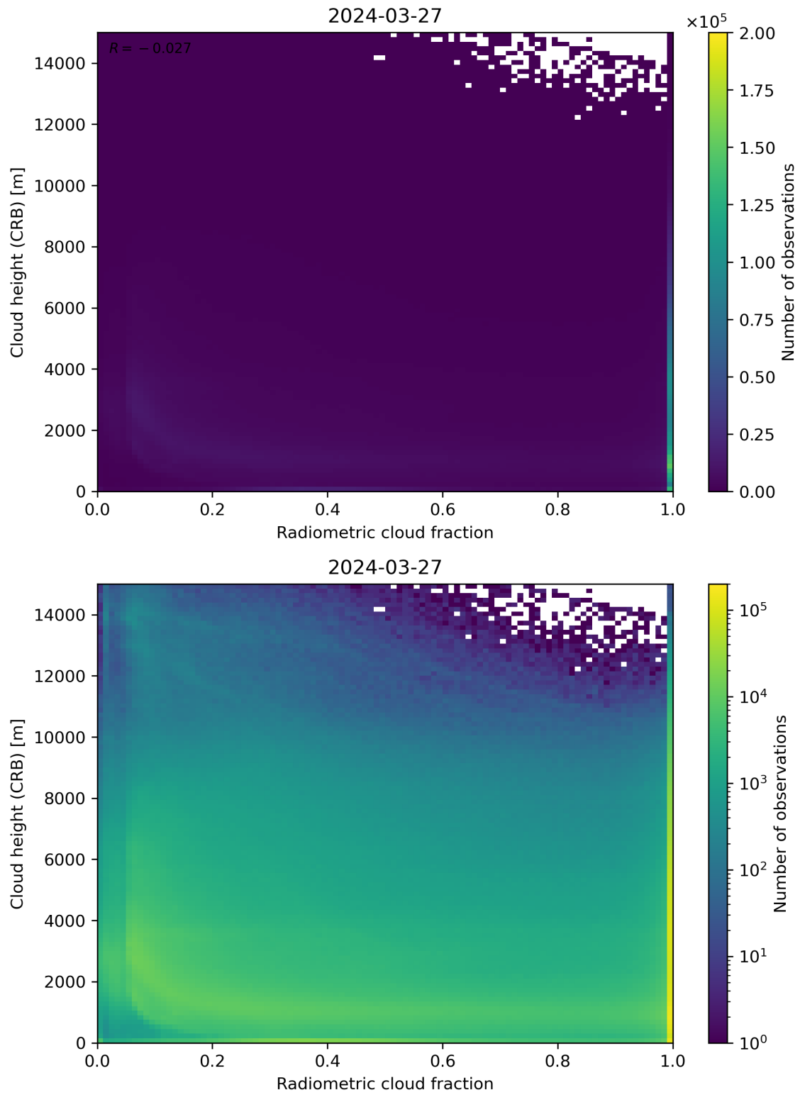
Figure 74: Scatter density plot of “Radiometric cloud fraction” against “Cloud height (CRB)” for 2024-03-26 to 2024-03-28.
