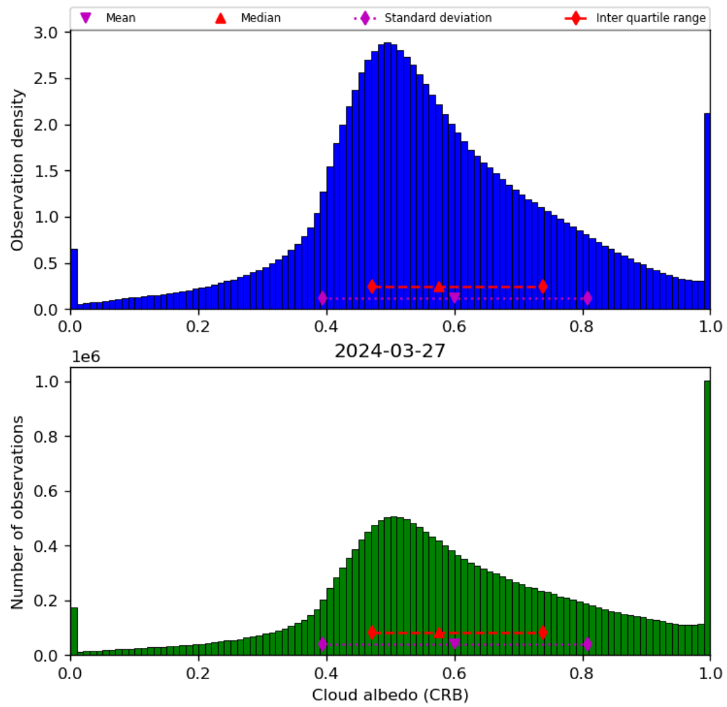
Figure 44: Histogram of “Cloud albedo (CRB)” for 2024-03-26 to 2024-03-28
