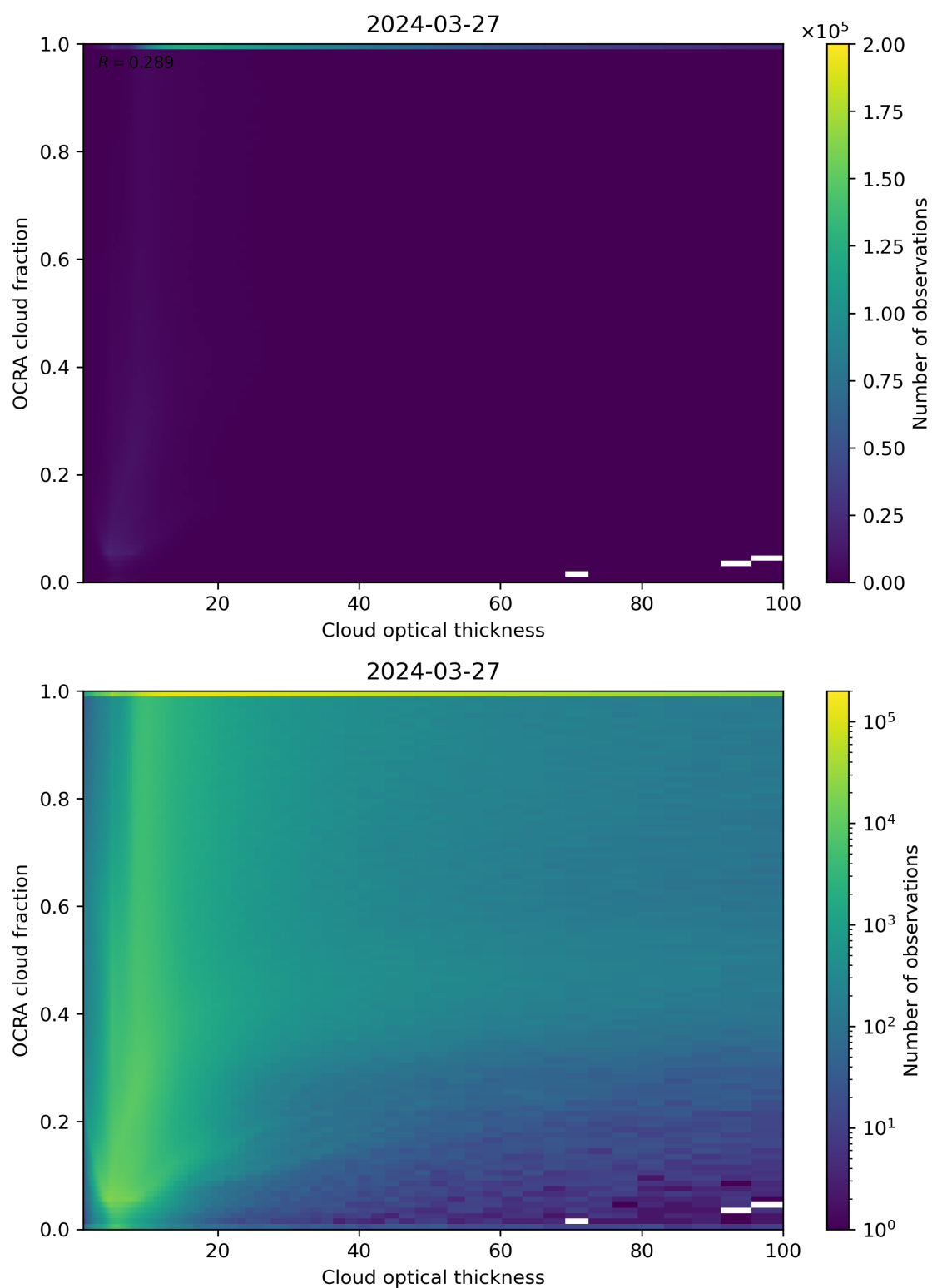
Figure 83: Scatter density plot of “Cloud optical thickness” against “OCRA cloud fraction” for 2024-03-26 to 2024-03-28.
