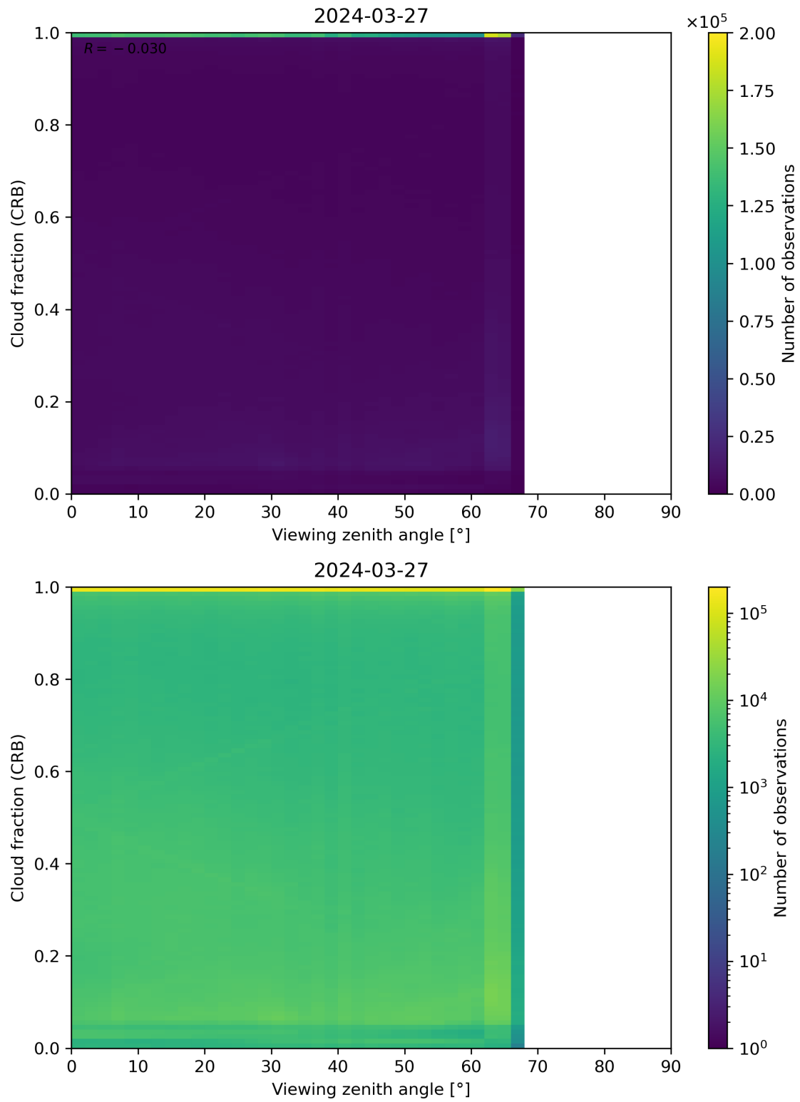
Figure 109: Scatter density plot of “Viewing zenith angle” against “Cloud fraction (CRB)” for 2024-03-26 to 2024-03-28.
