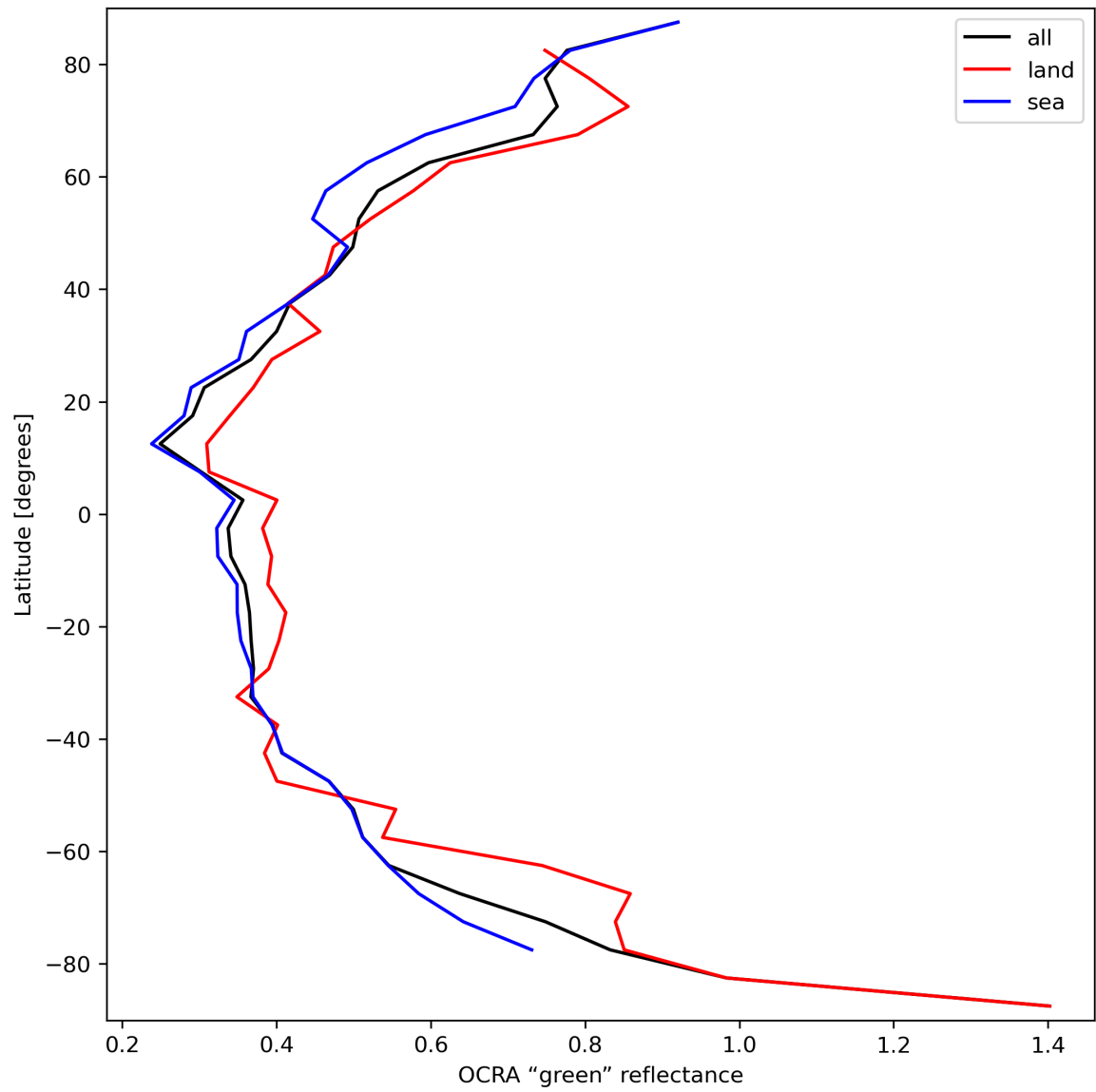
Figure 36: Zonal average of “OCRA “green” reflectance” for 2024-03-26 to 2024-03-28.
