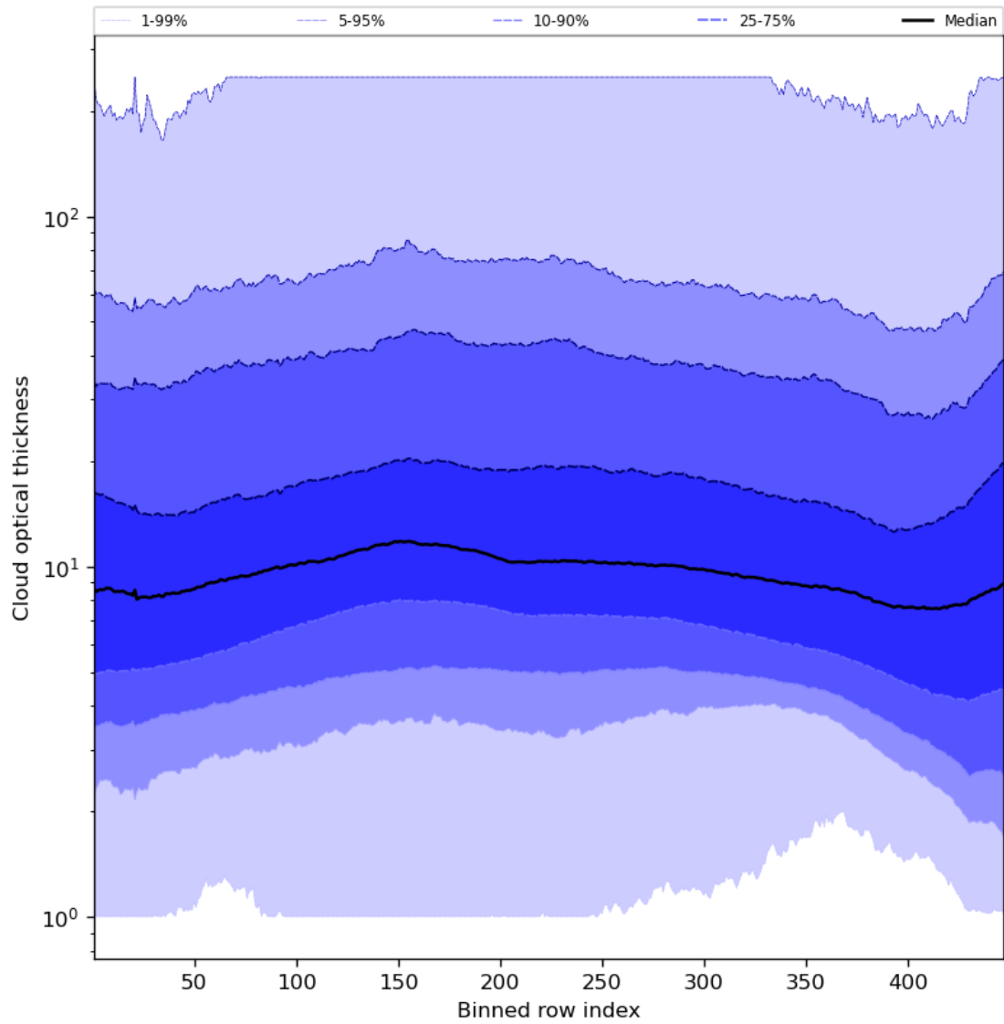
Figure 57: Along track statistics of “Cloud optical thickness” for 2024-03-26 to 2024-03-28
