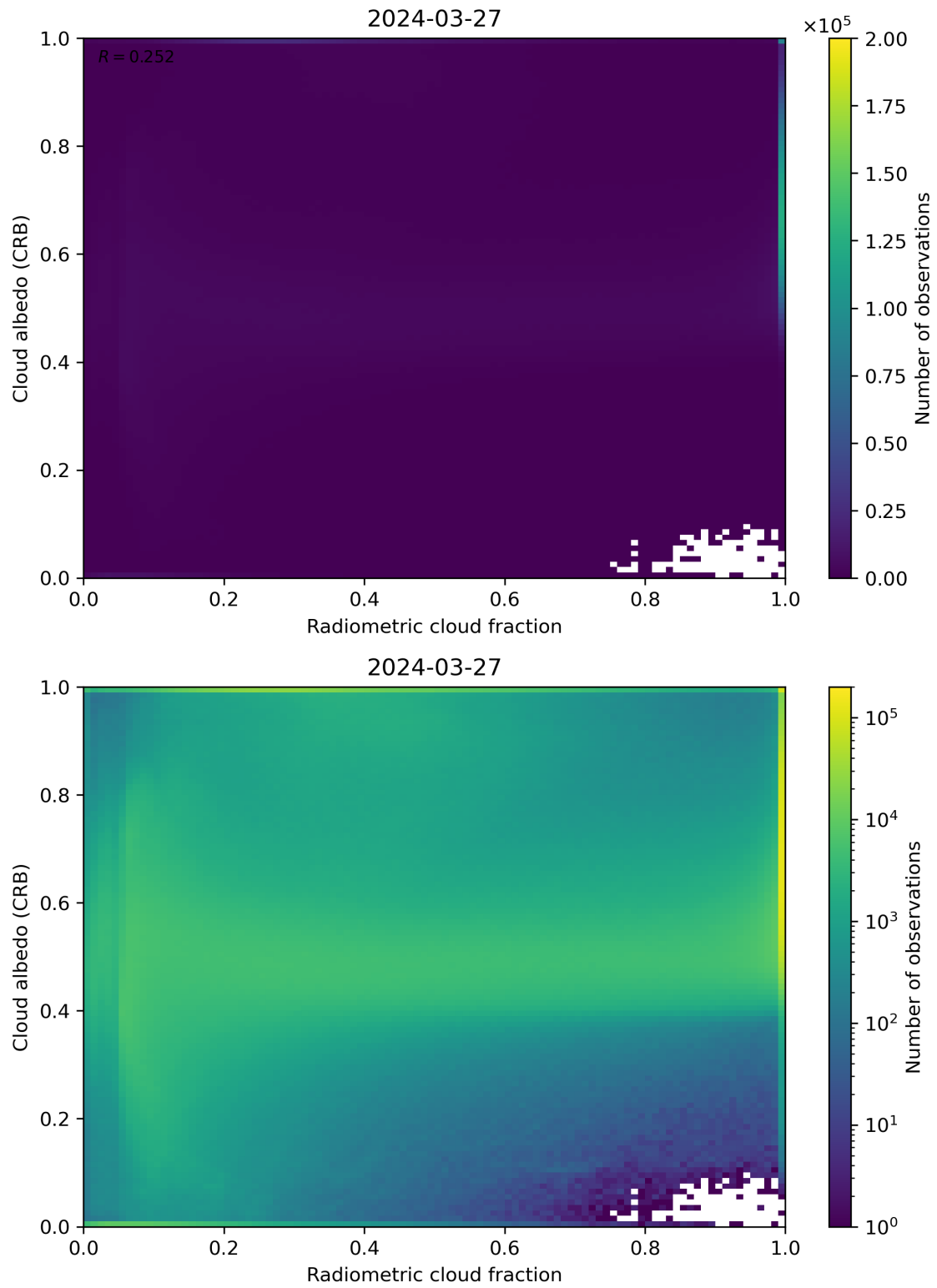
Figure 71: Scatter density plot of “Radiometric cloud fraction” against “Cloud albedo (CRB)” for 2024-03-26 to 2024-03-28.
