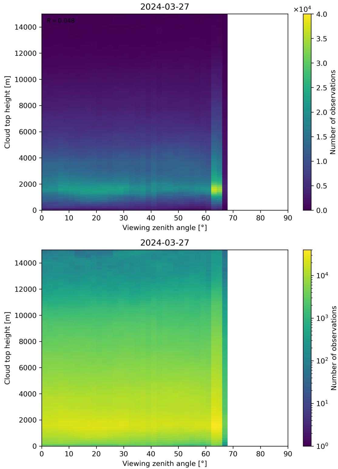
Figure 112: Scatter density plot of “Viewing zenith angle” against “Cloud top height” for 2024-03-26 to 2024-03-28.
