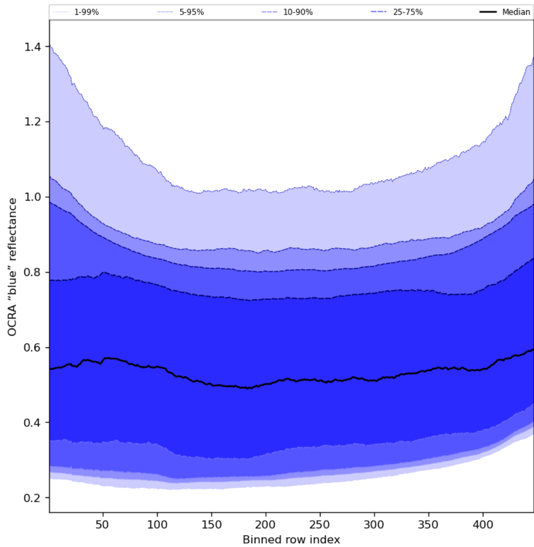
Figure 67: Along track statistics of “OCRA “blue” reflectance” for 2024-03-26 to 2024-03-28
