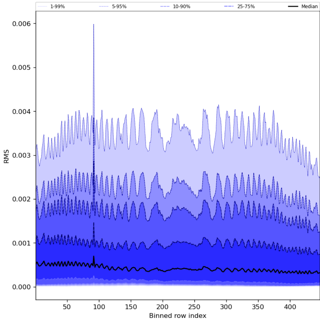
Figure 63: Along track statistics of “RMS” for 2024-03-26 to 2024-03-28
