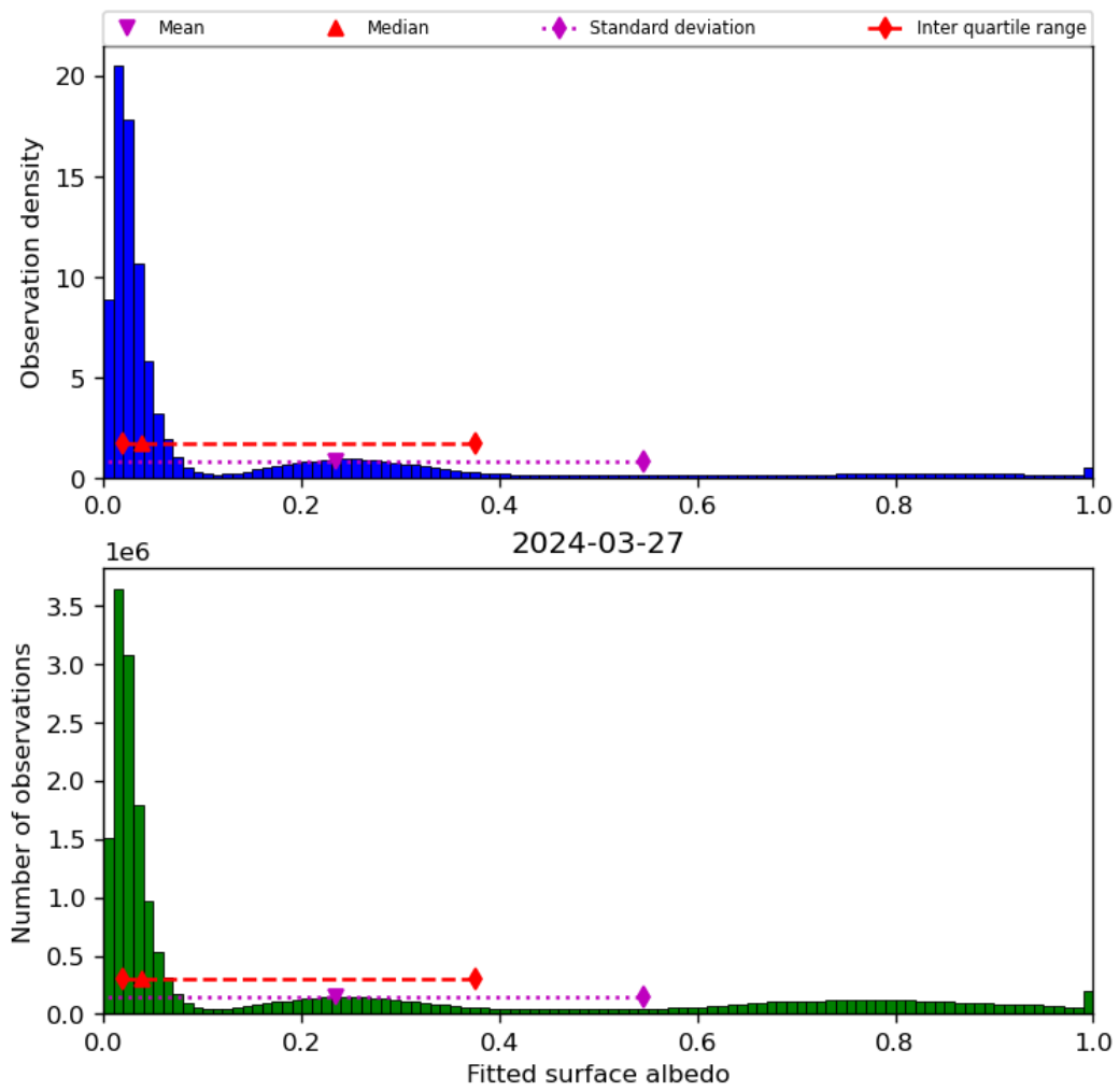
Figure 45: Histogram of “Fitted surface albedo” for 2024-03-26 to 2024-03-28
