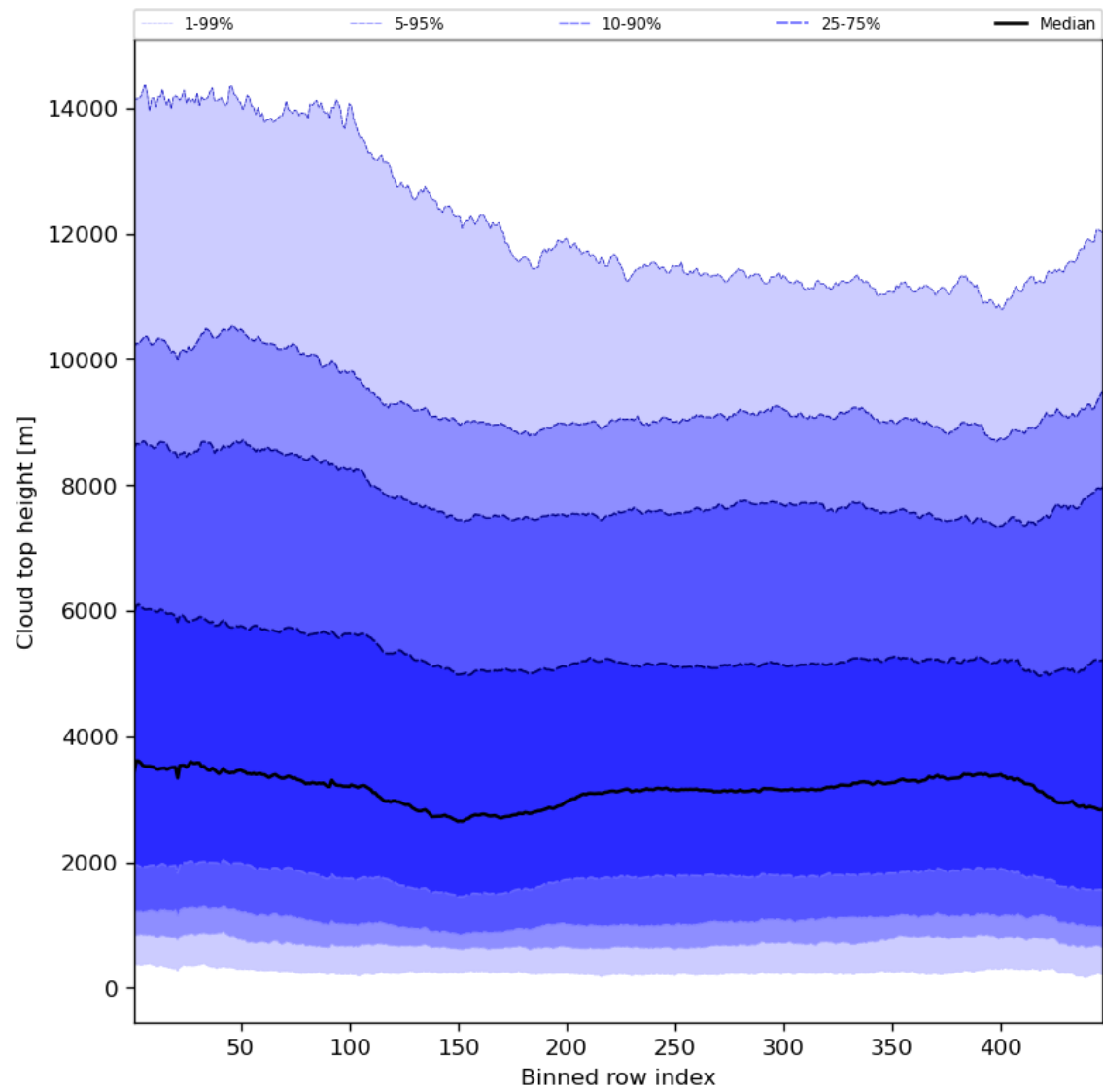
Figure 56: Along track statistics of “Cloud top height” for 2024-03-26 to 2024-03-28
