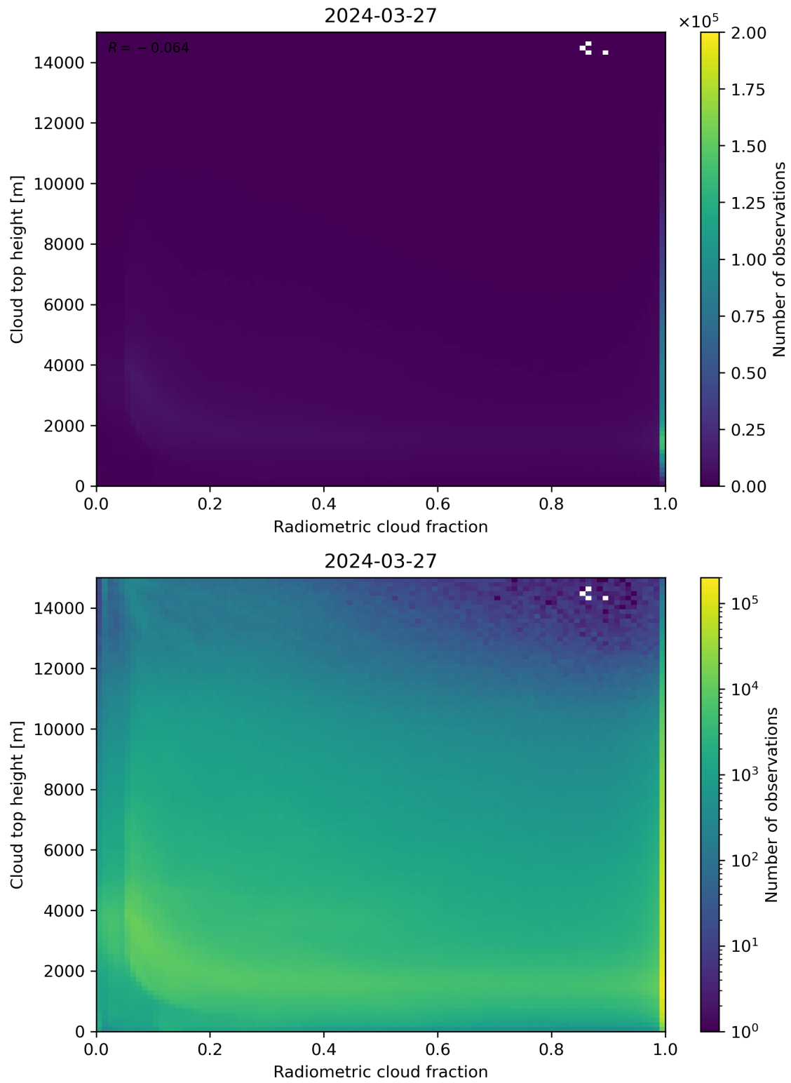
Figure 76: Scatter density plot of “Radiometric cloud fraction” against “Cloud top height” for 2024-03-26 to 2024-03-28.
