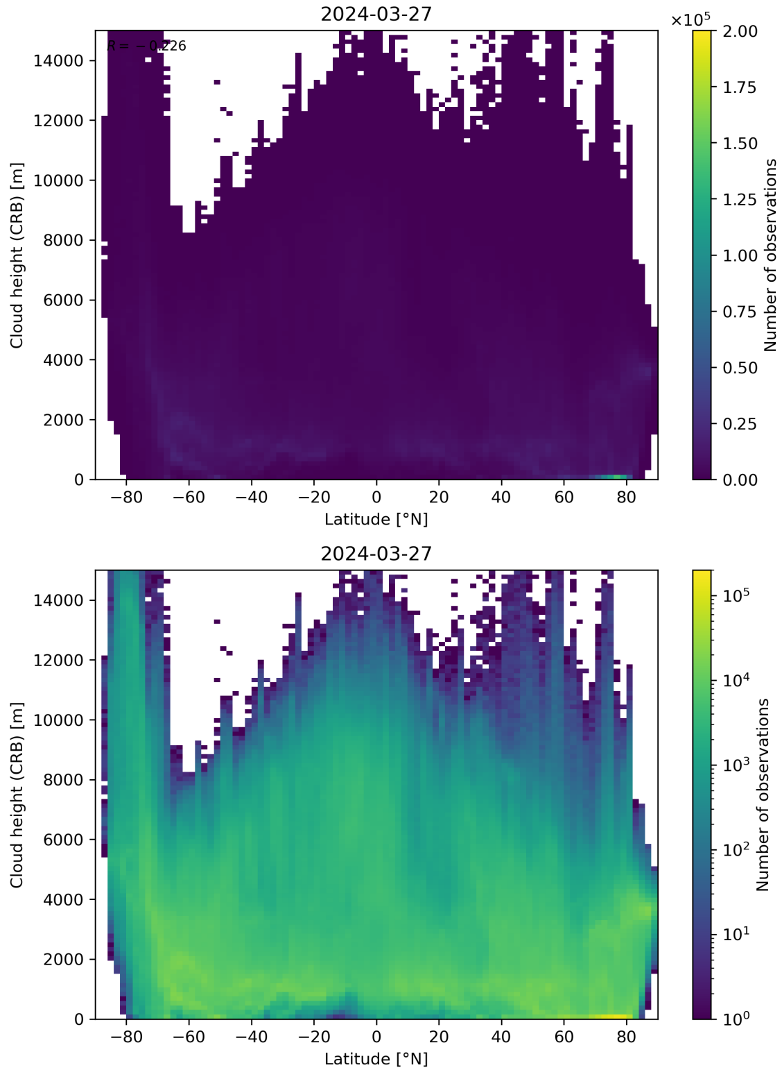
Figure 95: Scatter density plot of “Latitude” against “Cloud height (CRB)” for 2024-03-26 to 2024-03-28.
