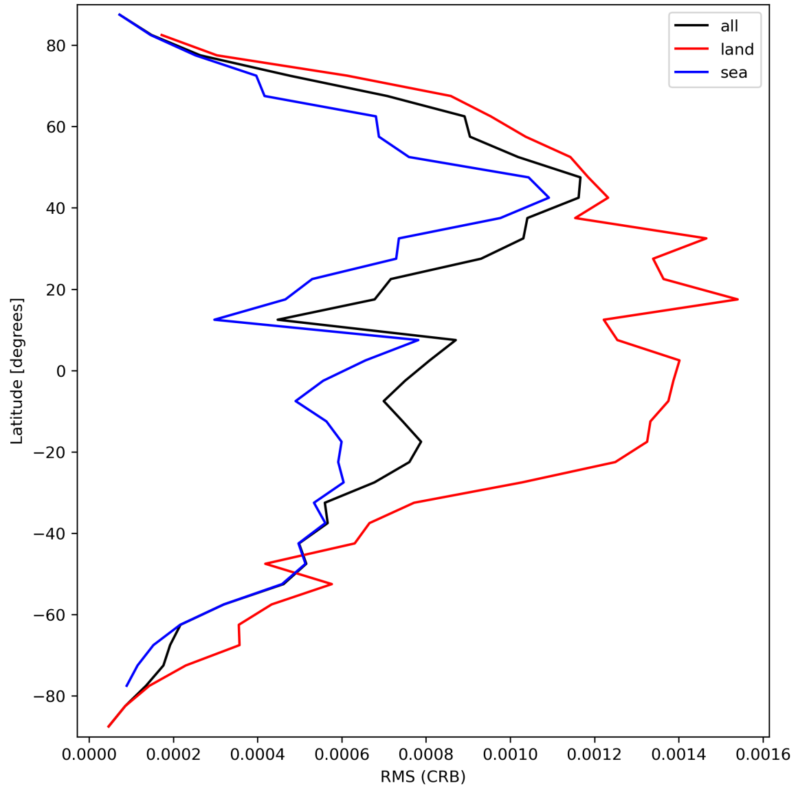
Figure 32: Zonal average of “RMS (CRB)” for 2024-03-26 to 2024-03-28.
