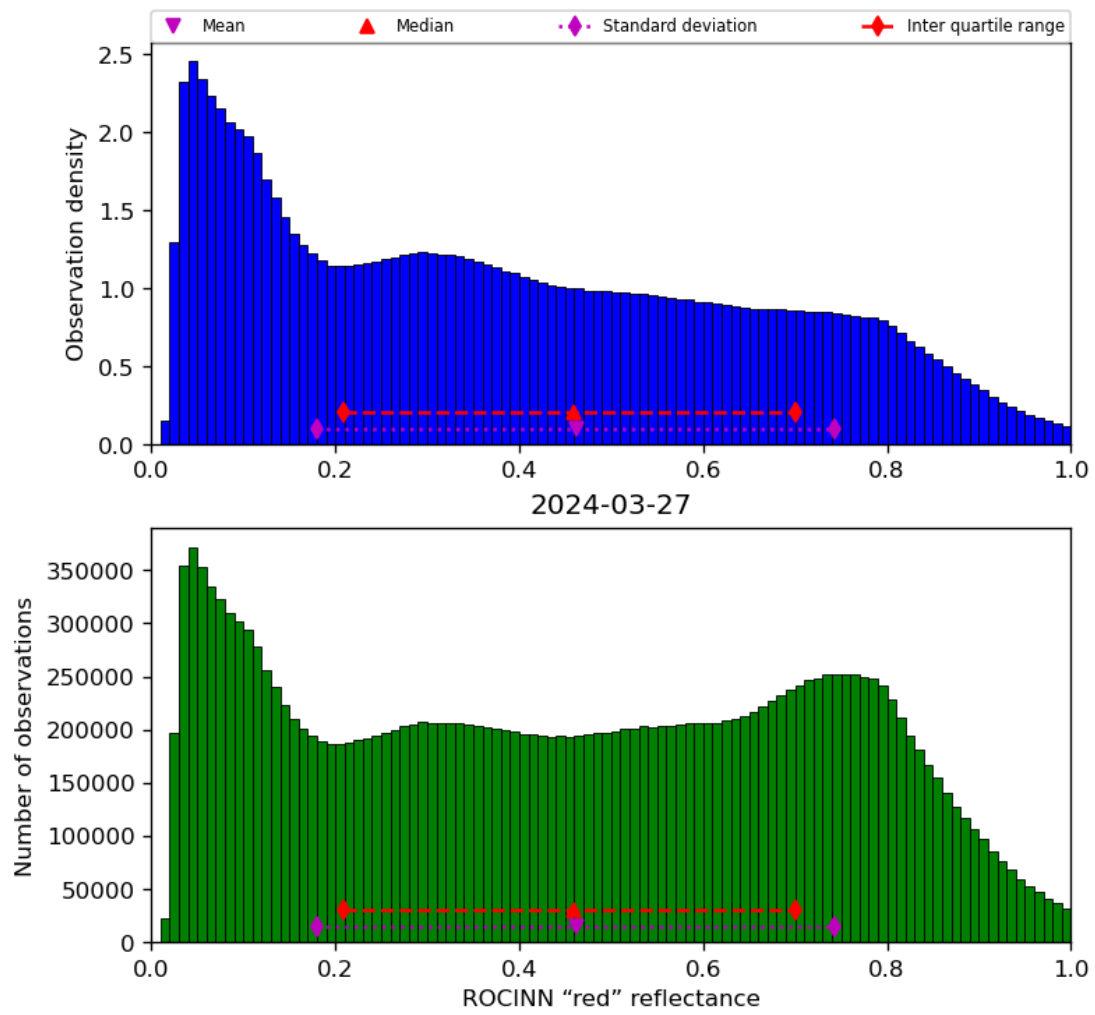
Figure 53: Histogram of “ROCINN “red” reflectance” for 2024-03-26 to 2024-03-28
