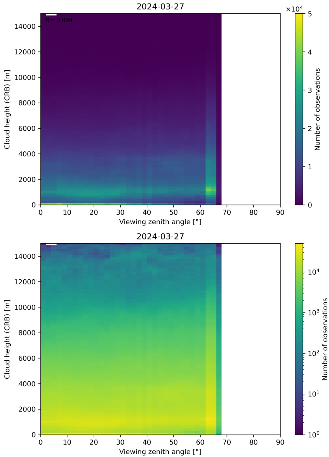
Figure 110: Scatter density plot of “Viewing zenith angle” against “Cloud height (CRB)” for 2024-03-26 to 2024-03-28.
