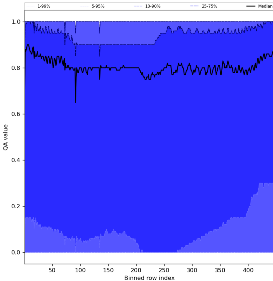
Figure 54: Along track statistics of “QA value” for 2024-03-26 to 2024-03-28
