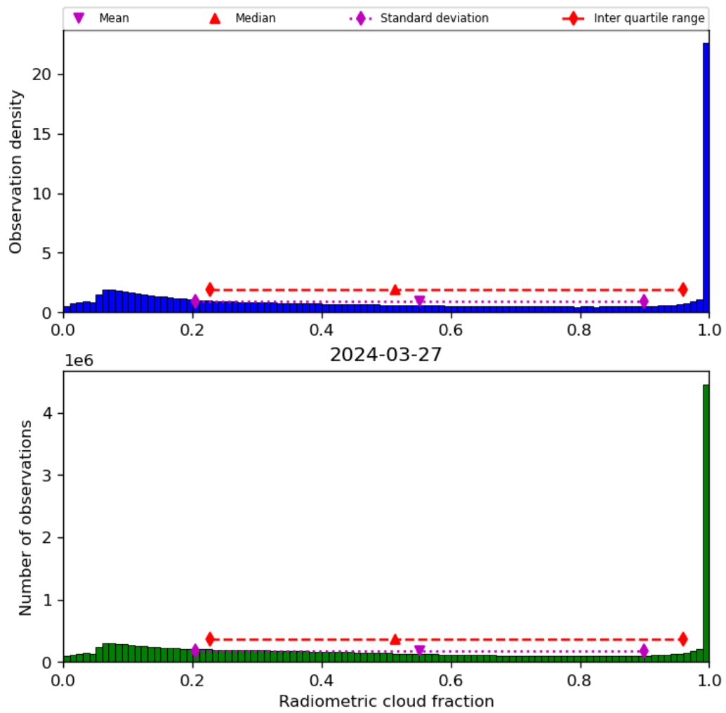
Figure 39: Histogram of “Radiometric cloud fraction” for 2024-03-26 to 2024-03-28
