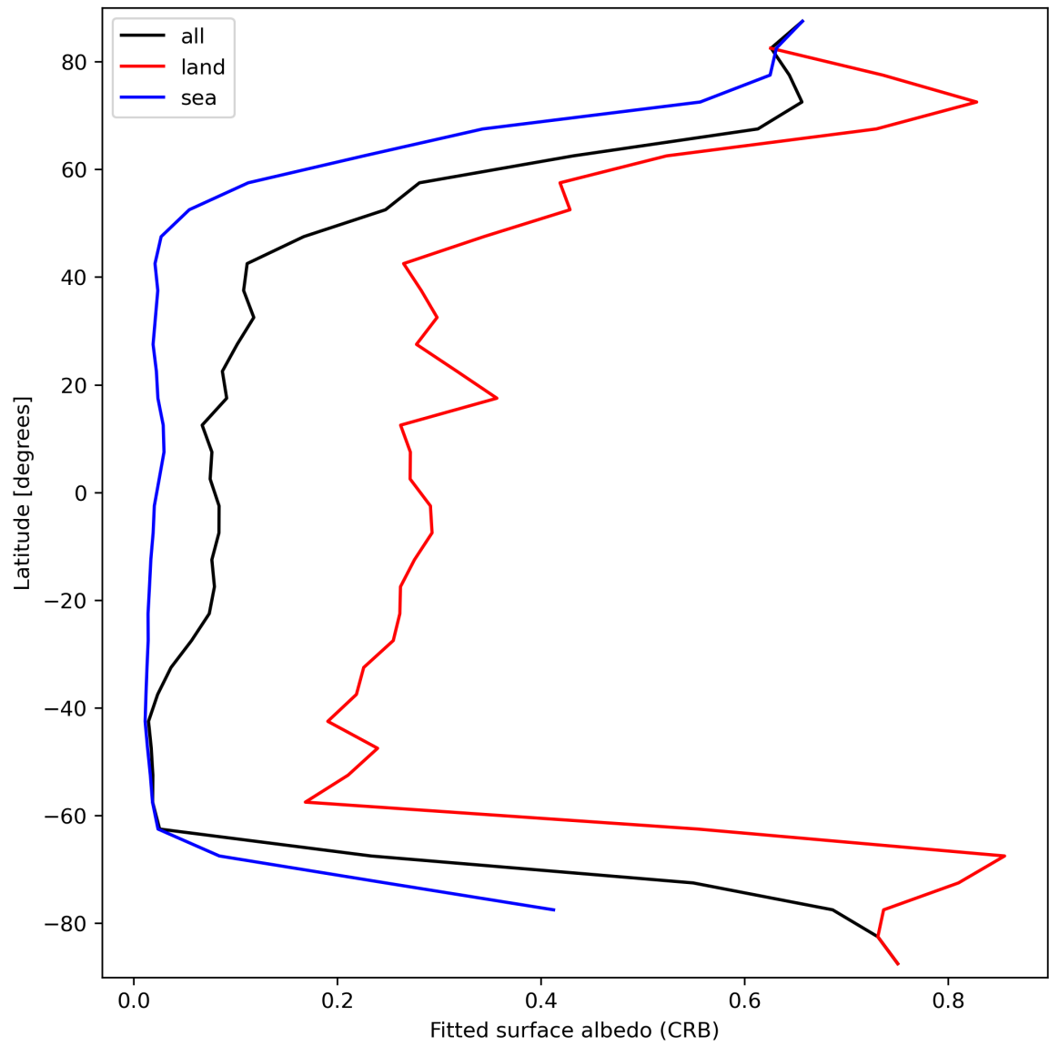
Figure 30: Zonal average of “Fitted surface albedo (CRB)” for 2024-03-26 to 2024-03-28.
