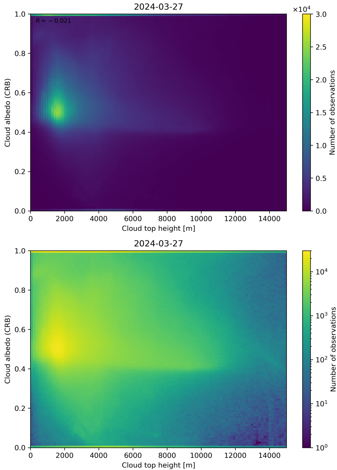
Figure 86: Scatter density plot of “Cloud top height” against “Cloud albedo (CRB)” for 2024-03-26 to 2024-03-28.
