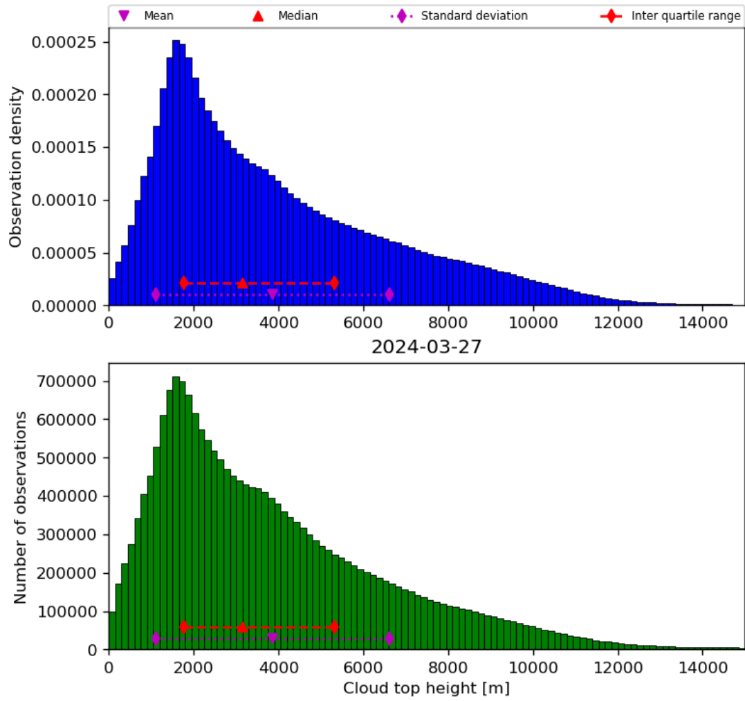
Figure 40: Histogram of “Cloud top height” for 2024-03-26 to 2024-03-28
