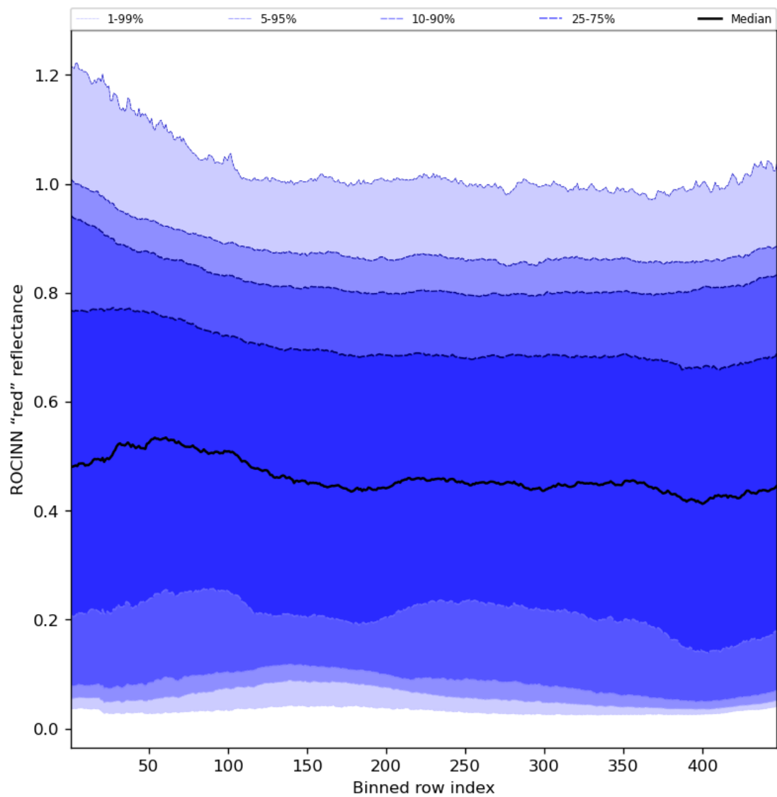
Figure 69: Along track statistics of “ROCINN “red” reflectance” for 2024-03-26 to 2024-03-28
