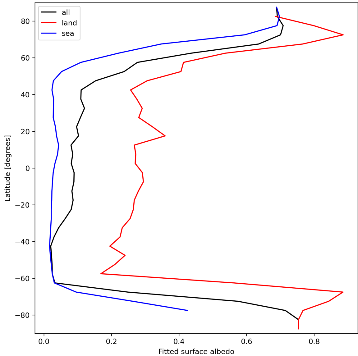
Figure 29: Zonal average of “Fitted surface albedo” for 2024-03-26 to 2024-03-28.
