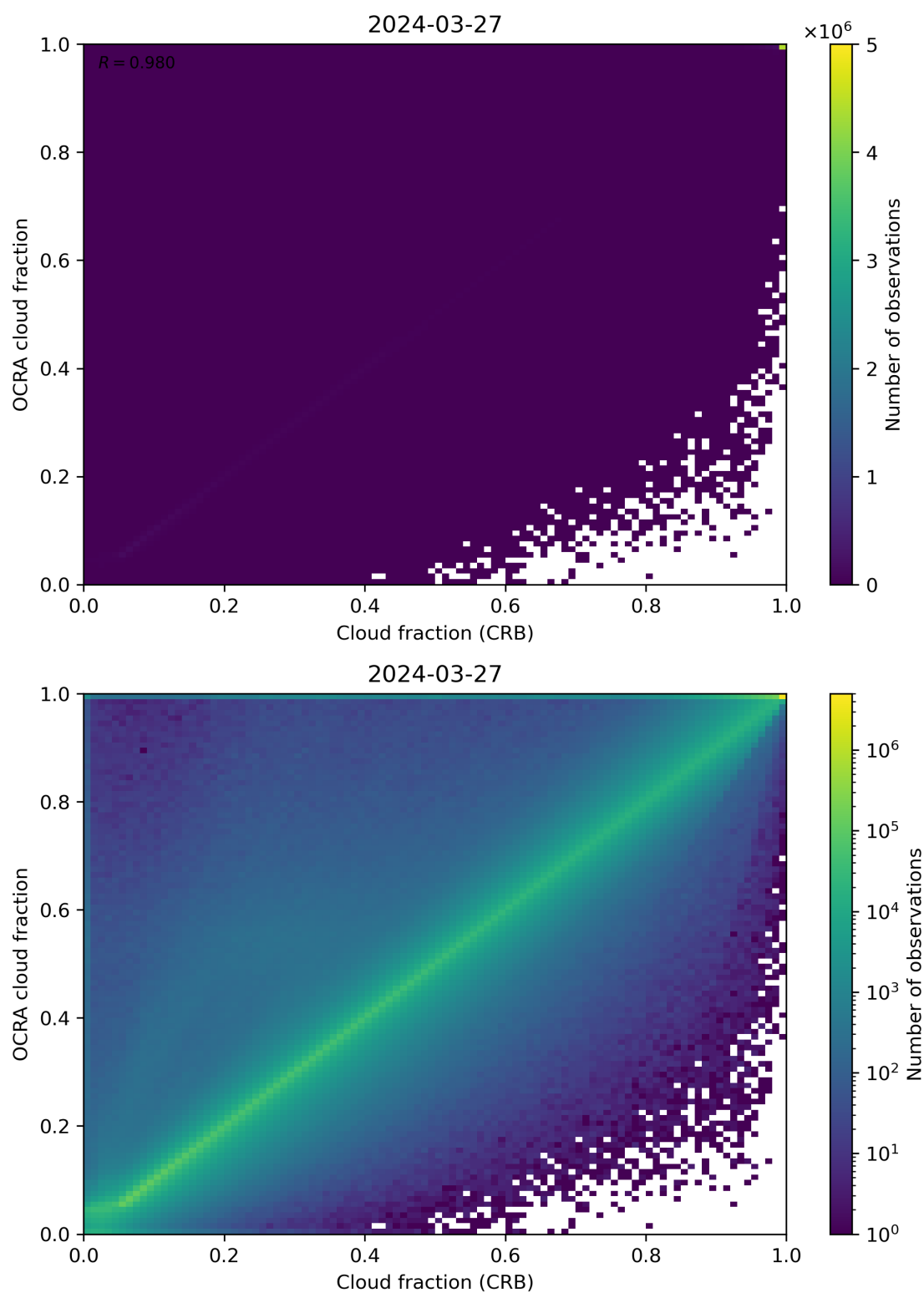
Figure 78: Scatter density plot of “Cloud fraction (CRB)” against “OCRA cloud fraction” for 2024-03-26 to 2024-03-28.
