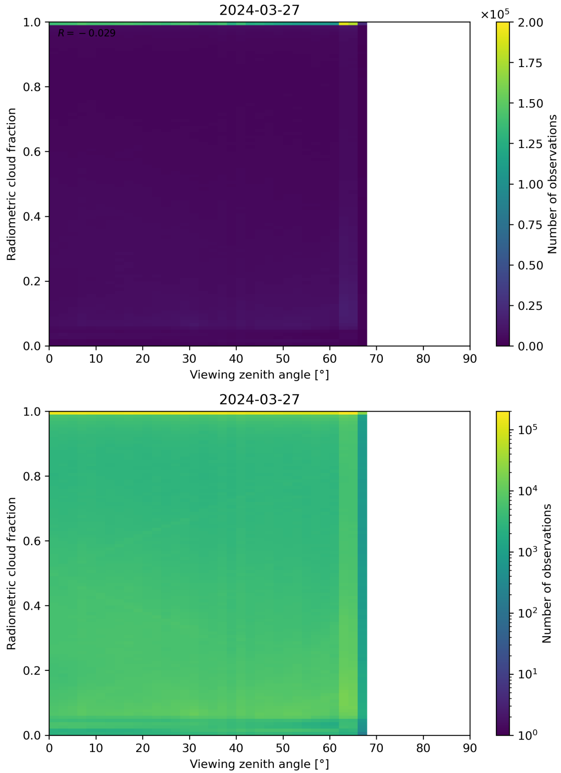
Figure 107: Scatter density plot of “Viewing zenith angle” against “Radiometric cloud fraction” for 2024-03-26 to 2024-03-28.
