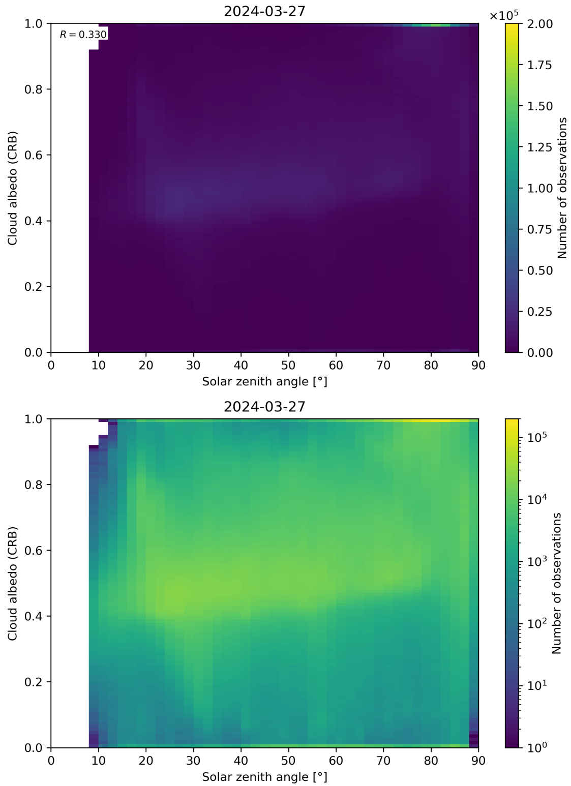
Figure 98: Scatter density plot of “Solar zenith angle” against “Cloud albedo (CRB)” for 2024-03-26 to 2024-03-28.
