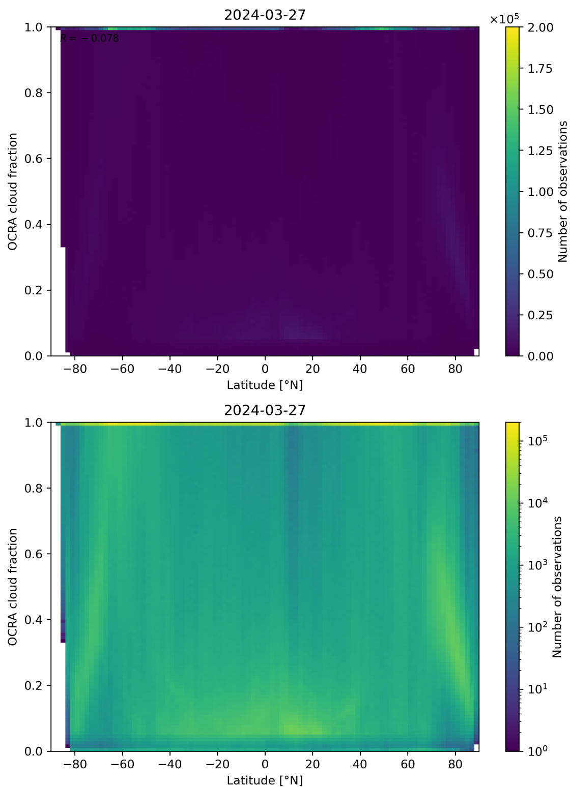
Figure 93: Scatter density plot of “Latitude” against “OCRA cloud fraction” for 2024-03-26 to 2024-03-28.
