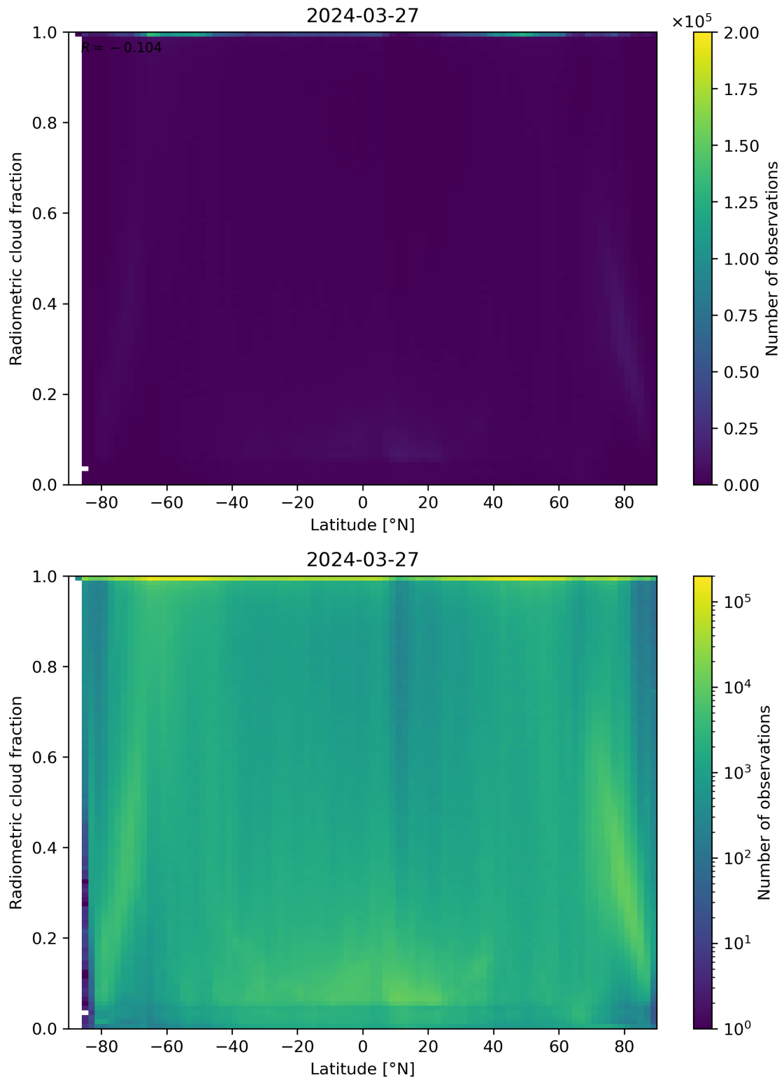
Figure 92: Scatter density plot of “Latitude” against “Radiometric cloud fraction” for 2024-03-26 to 2024-03-28.
