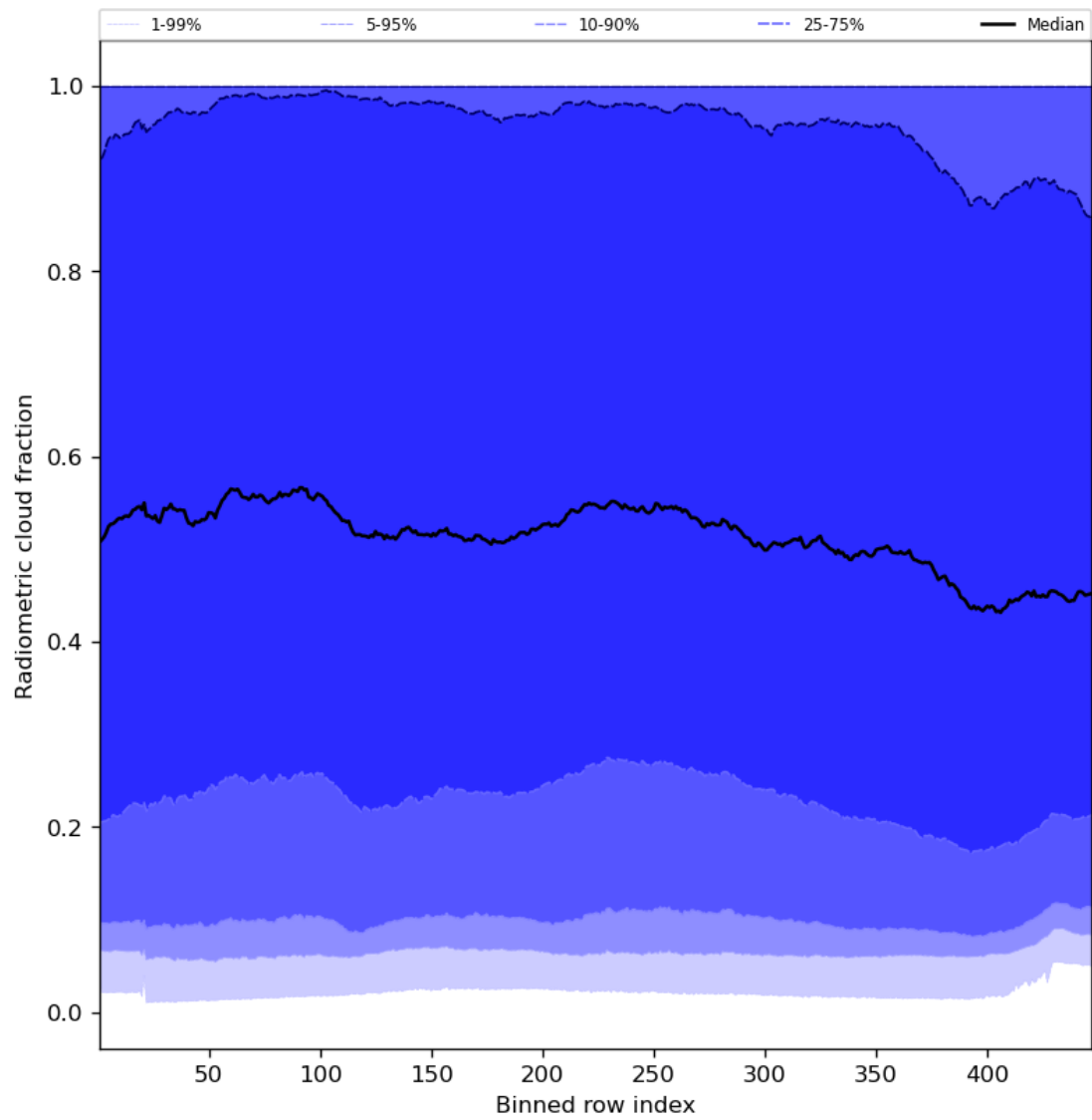
Figure 55: Along track statistics of “Radiometric cloud fraction” for 2024-03-26 to 2024-03-28
