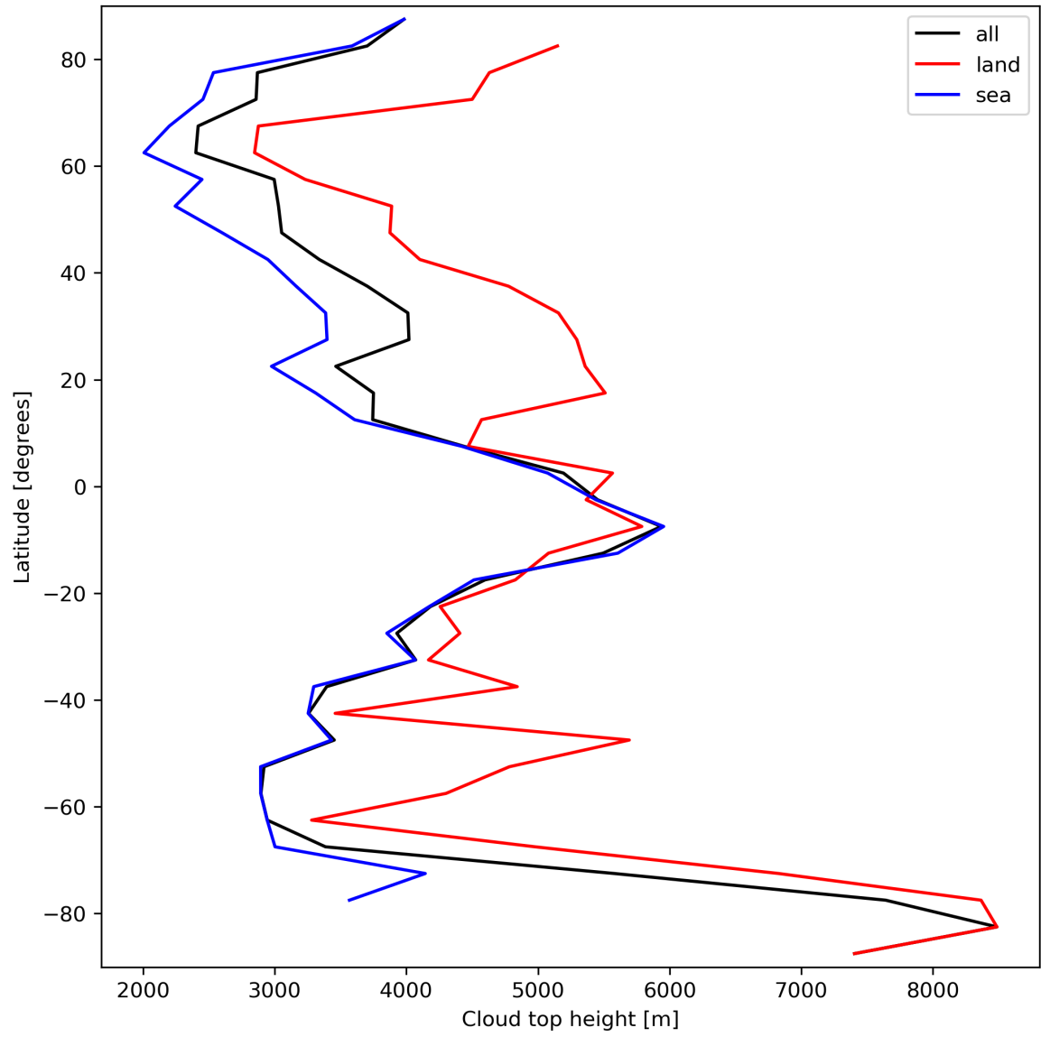
Figure 24: Zonal average of “Cloud top height” for 2024-03-26 to 2024-03-28.
