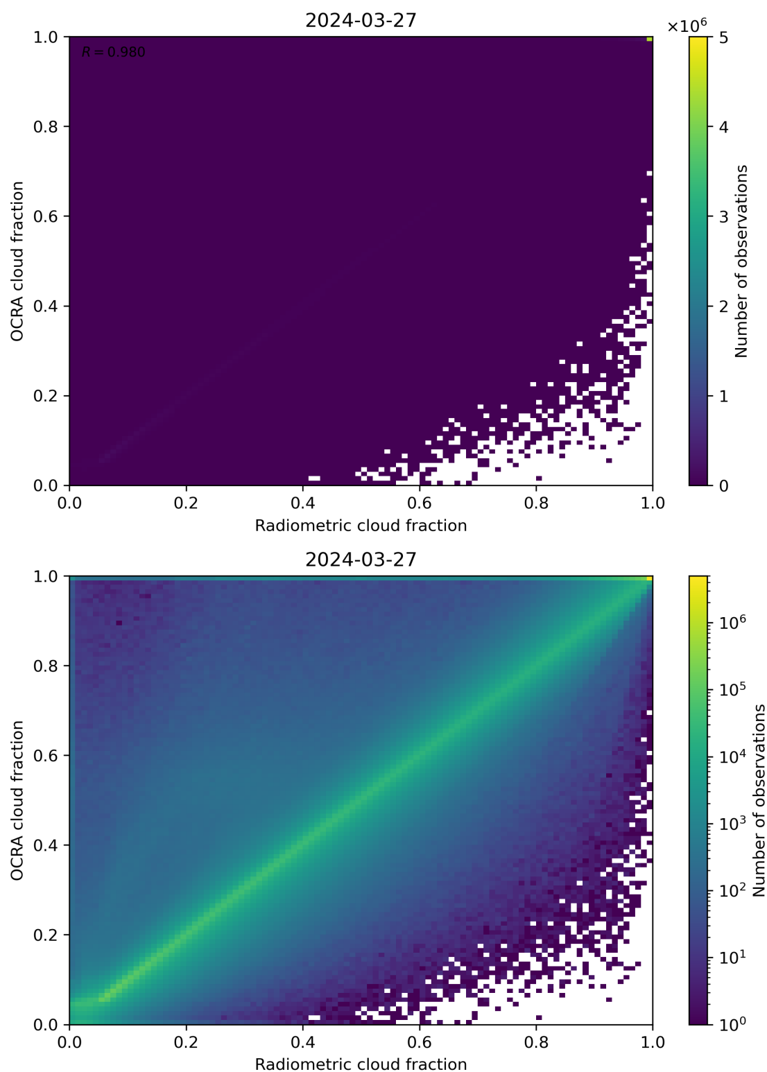
Figure 72: Scatter density plot of “Radiometric cloud fraction” against “OCRA cloud fraction” for 2024-03-26 to 2024-03-28.
