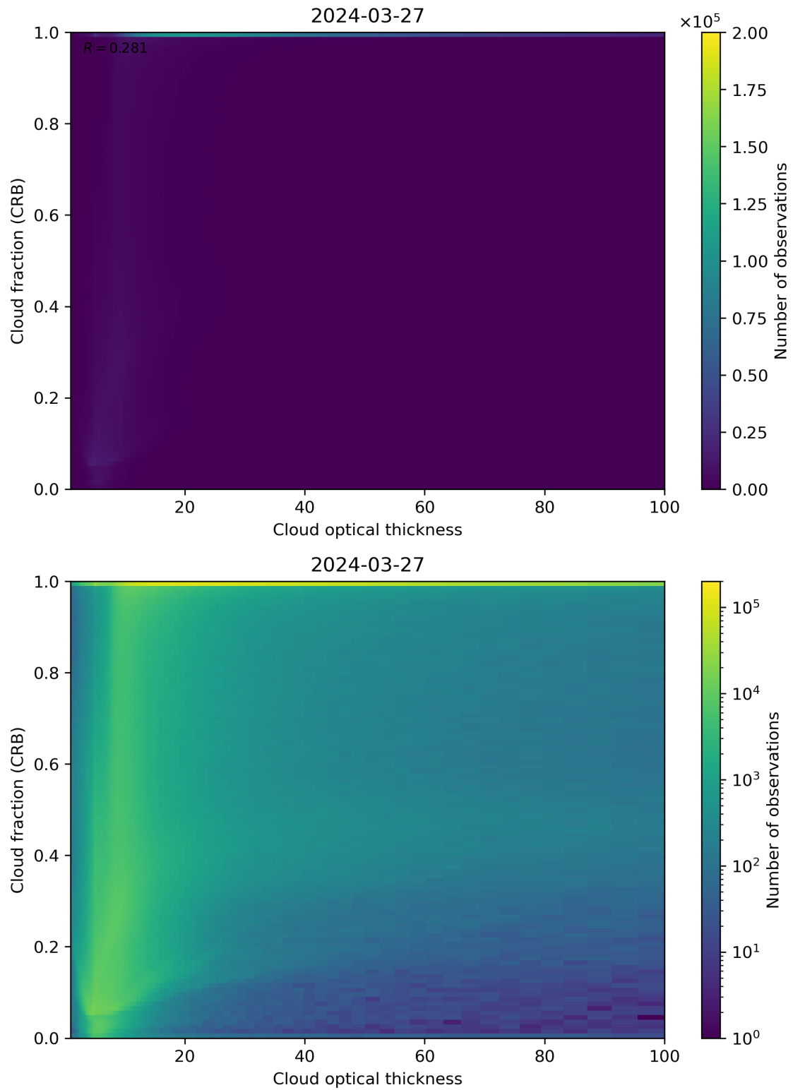
Figure 84: Scatter density plot of “Cloud optical thickness” against “Cloud fraction (CRB)” for 2024-03-26 to 2024-03-28.
