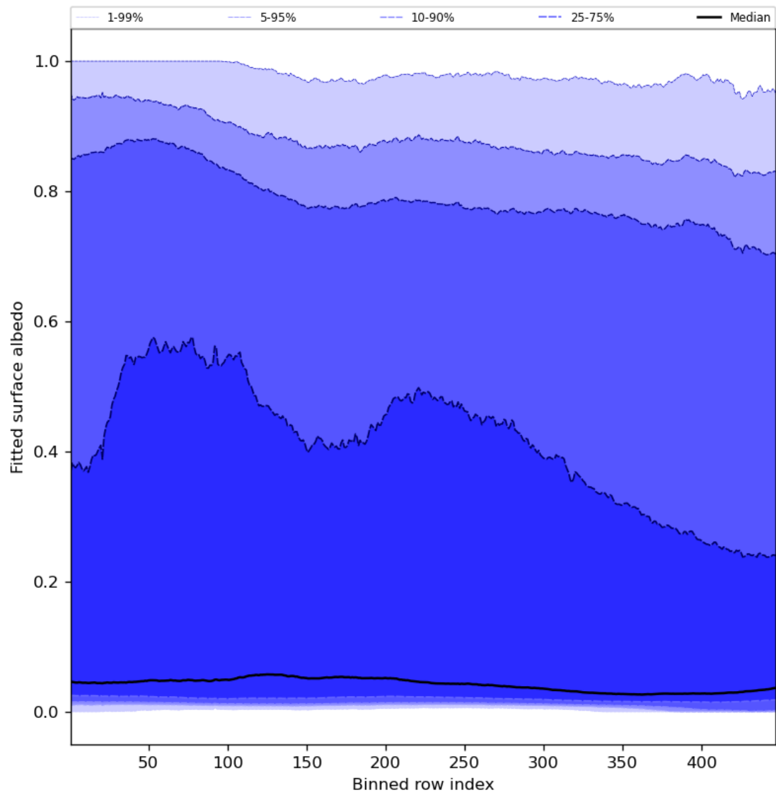
Figure 61: Along track statistics of “Fitted surface albedo” for 2024-03-26 to 2024-03-28
