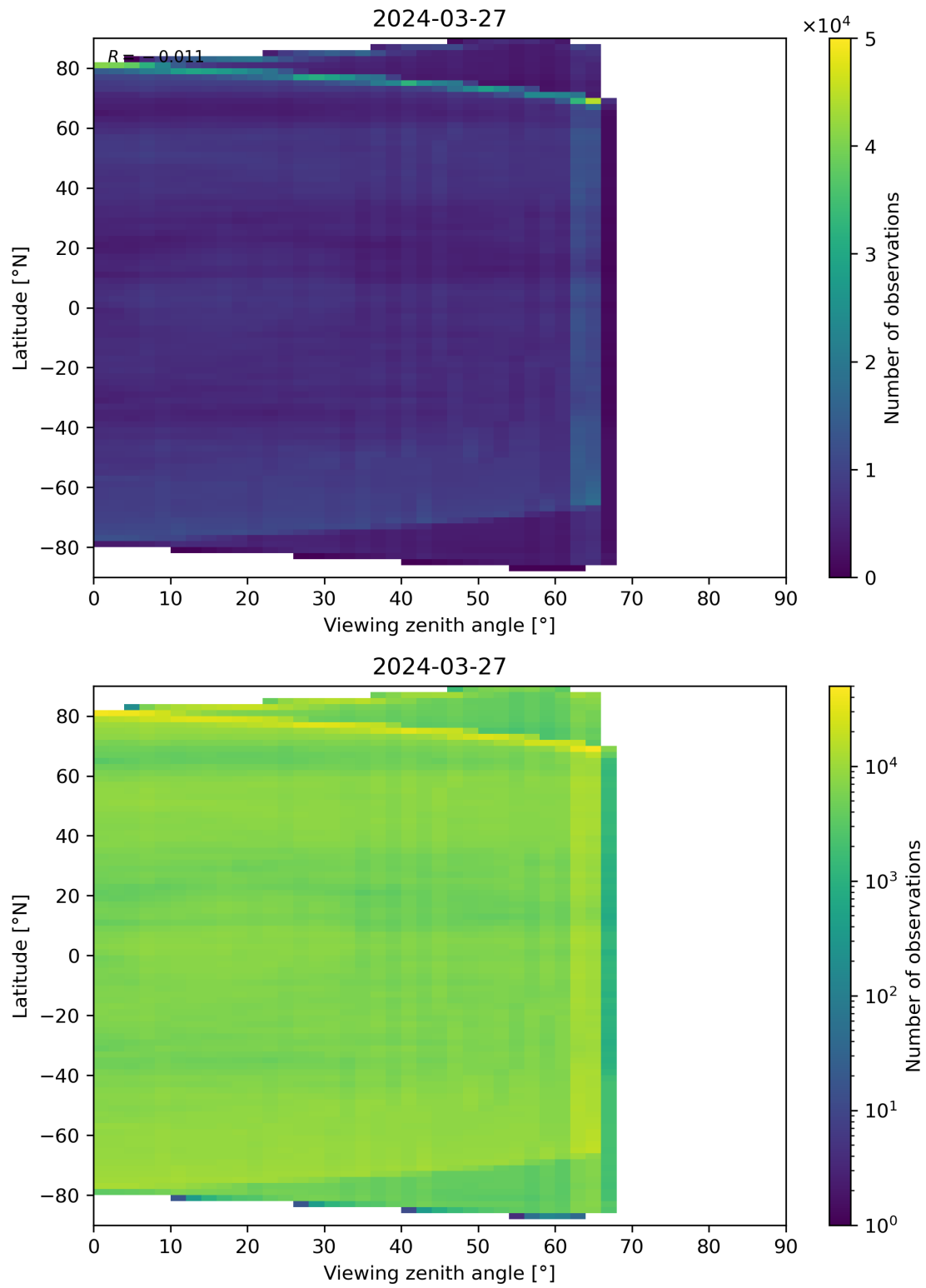
Figure 113: Scatter density plot of “Viewing zenith angle” against “Latitude” for 2024-03-26 to 2024-03-28.
