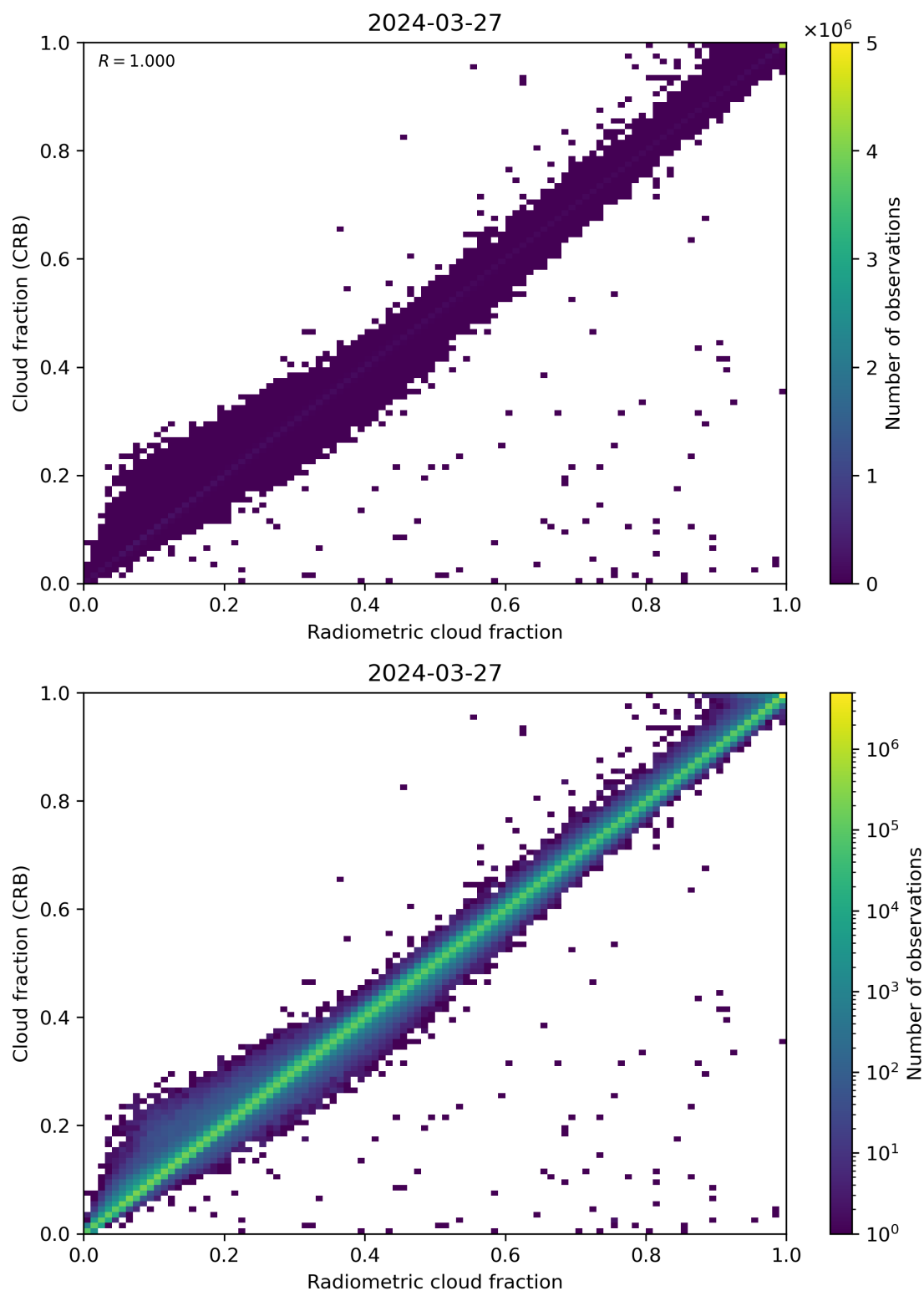
Figure 73: Scatter density plot of “Radiometric cloud fraction” against “Cloud fraction (CRB)” for 2024-03-26 to 2024-03-28.
