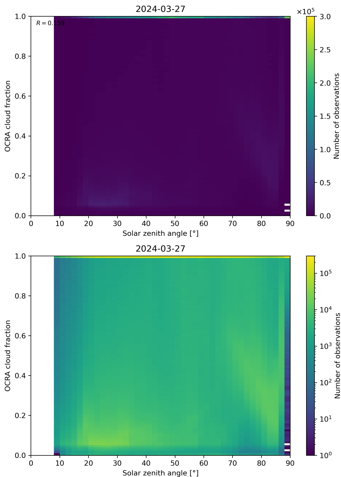
Figure 100: Scatter density plot of “Solar zenith angle” against “OCRA cloud fraction” for 2024-03-26 to 2024-03-28.
