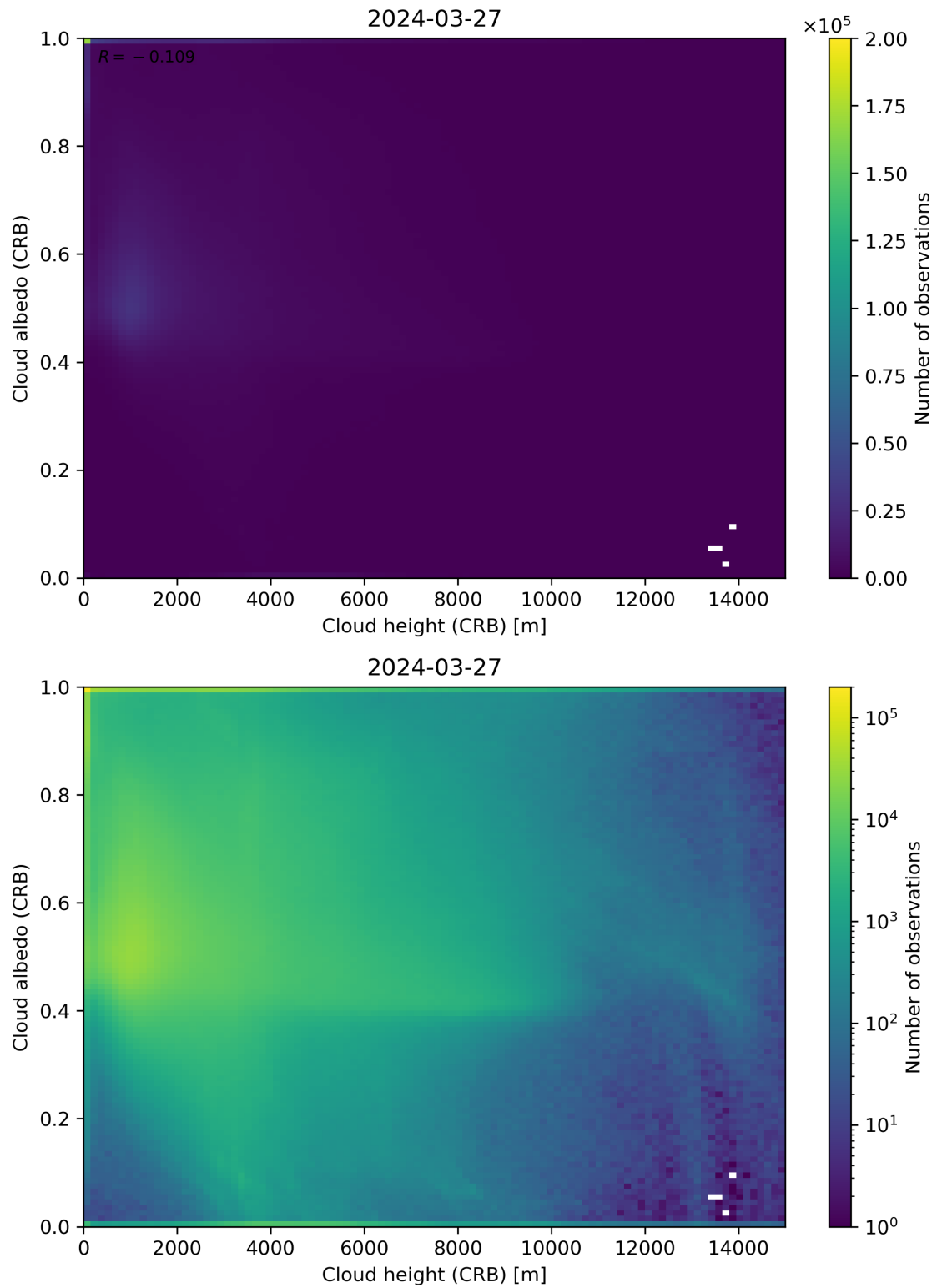
Figure 80: Scatter density plot of “Cloud height (CRB)” against “Cloud albedo (CRB)” for 2024-03-26 to 2024-03-28.
