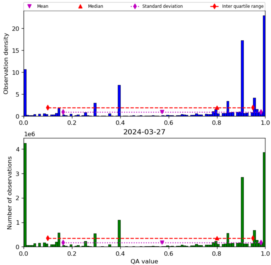
Figure 38: Histogram of “QA value” for 2024-03-26 to 2024-03-28
