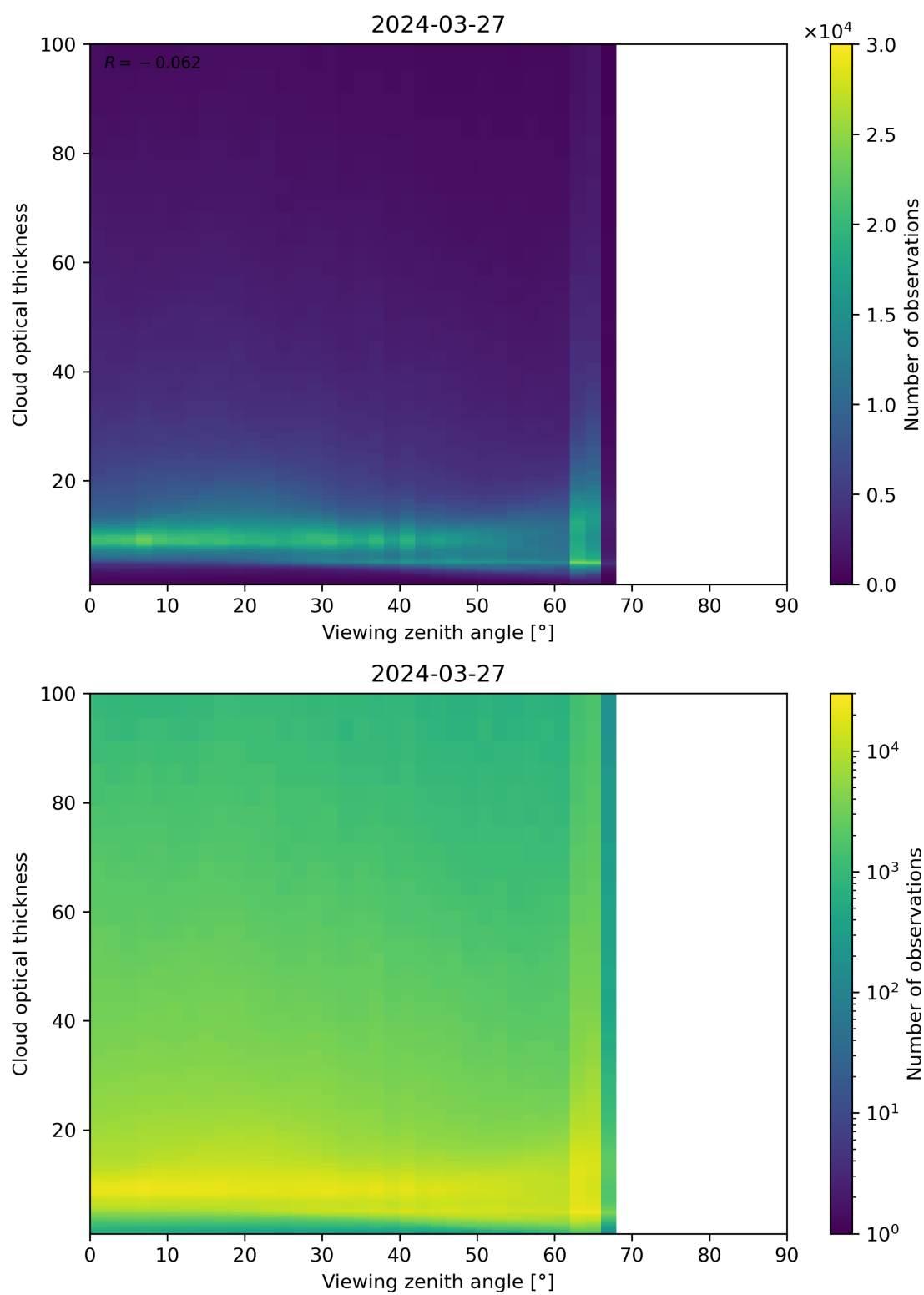
Figure 111: Scatter density plot of “Viewing zenith angle” against “Cloud optical thickness” for 2024-03-26 to 2024-03-28.
