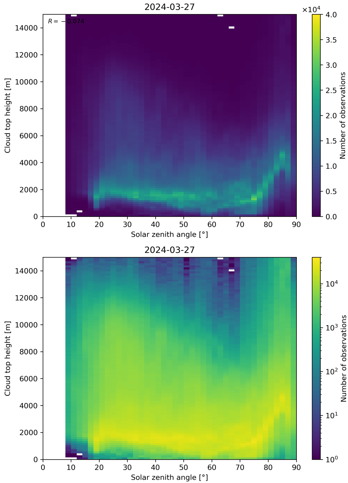
Figure 104: Scatter density plot of “Solar zenith angle” against “Cloud top height” for 2024-03-26 to 2024-03-28.
