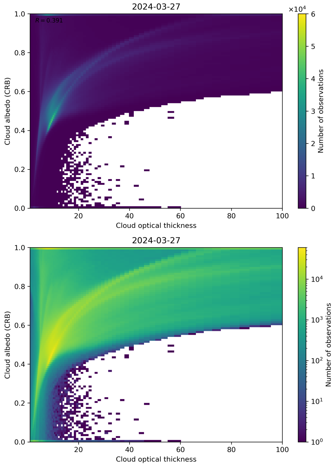
Figure 82: Scatter density plot of “Cloud optical thickness” against “Cloud albedo (CRB)” for 2024-03-26 to 2024-03-28.
