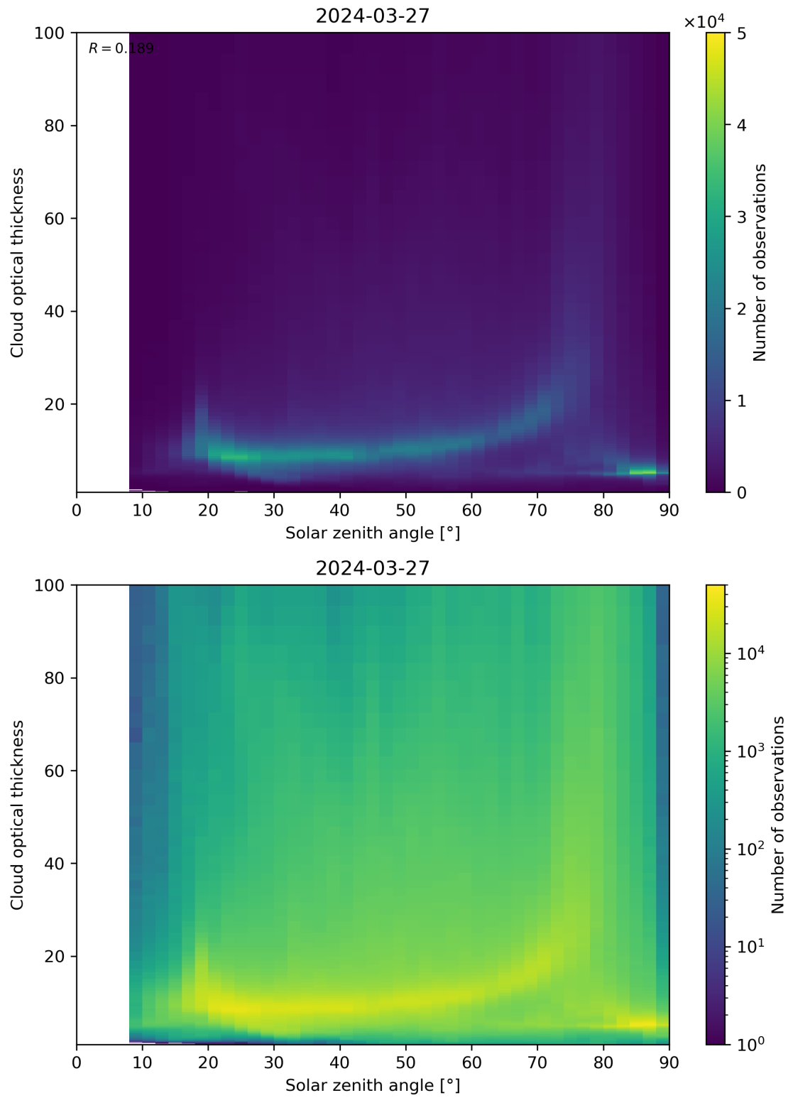
Figure 103: Scatter density plot of “Solar zenith angle” against “Cloud optical thickness” for 2024-03-26 to 2024-03-28.
