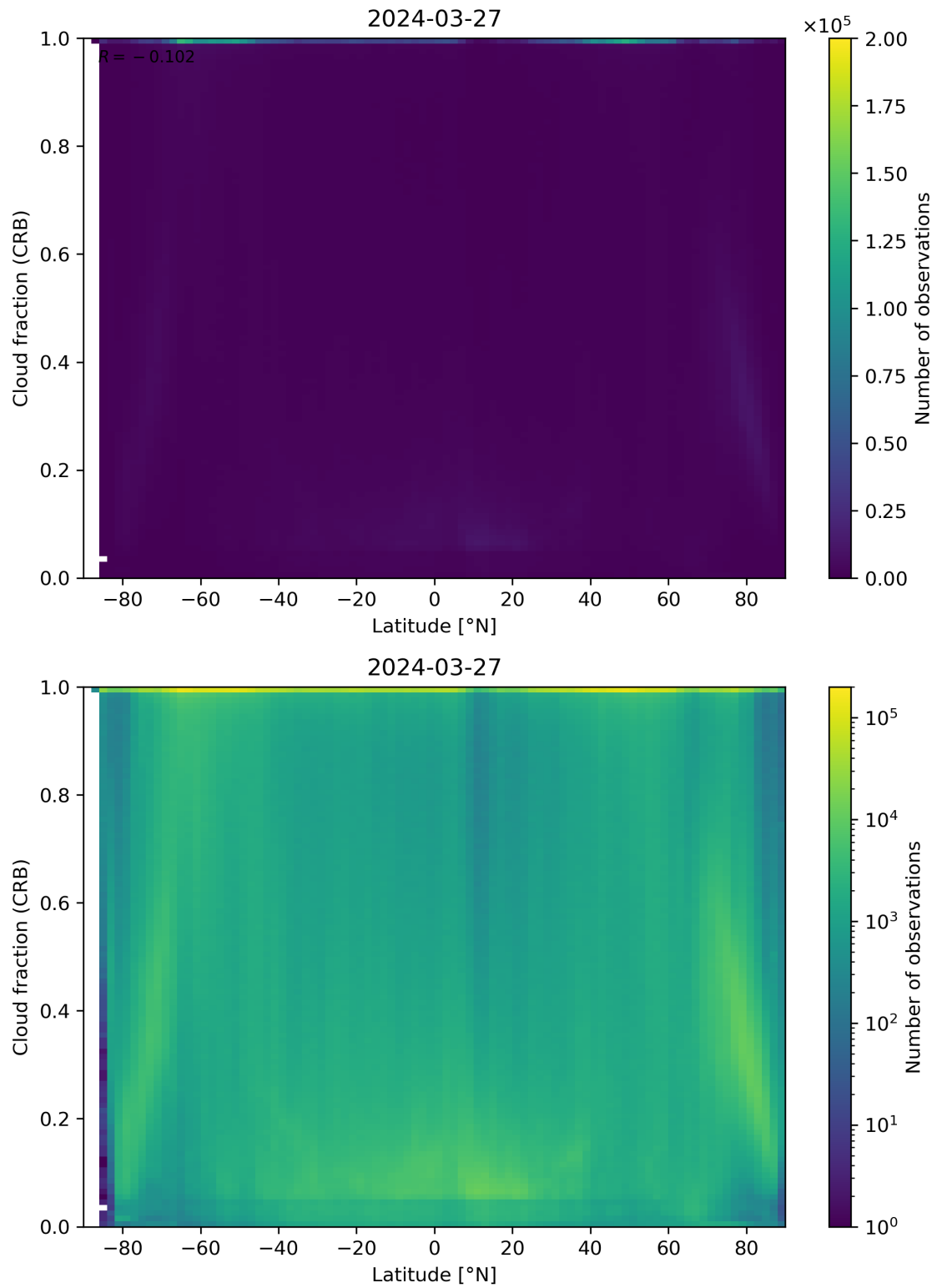
Figure 94: Scatter density plot of “Latitude” against “Cloud fraction (CRB)” for 2024-03-26 to 2024-03-28.
