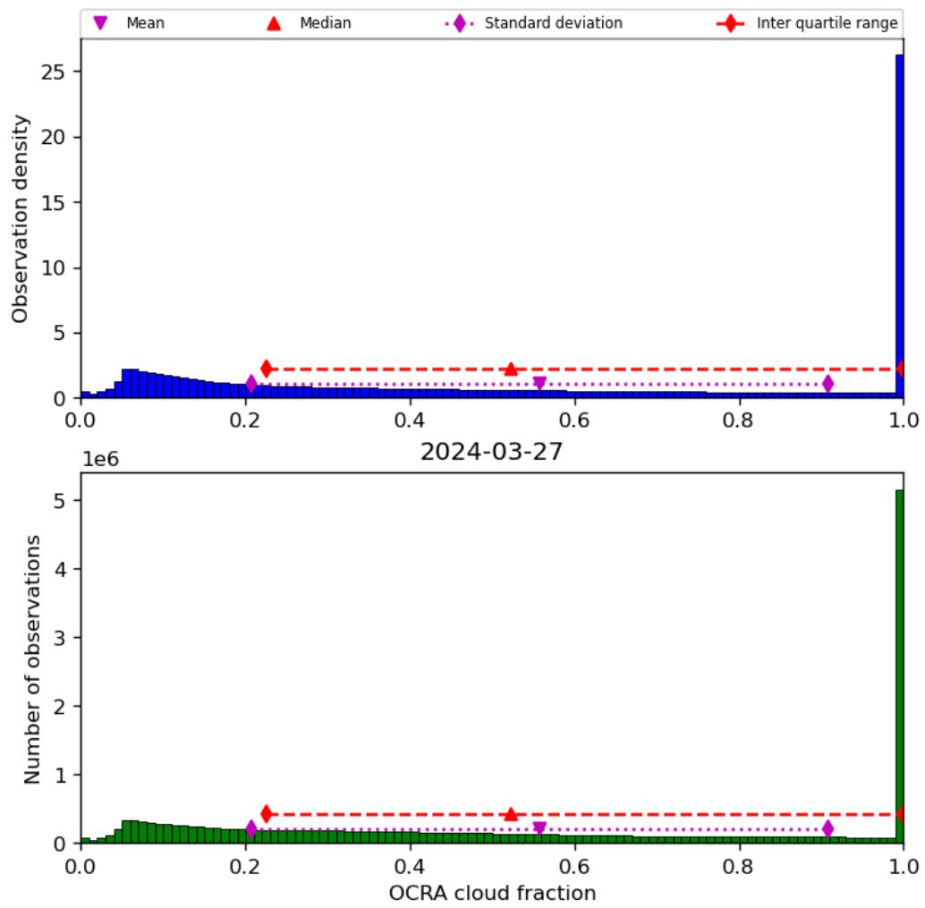
Figure 50: Histogram of “OCRA cloud fraction” for 2024-03-26 to 2024-03-28
