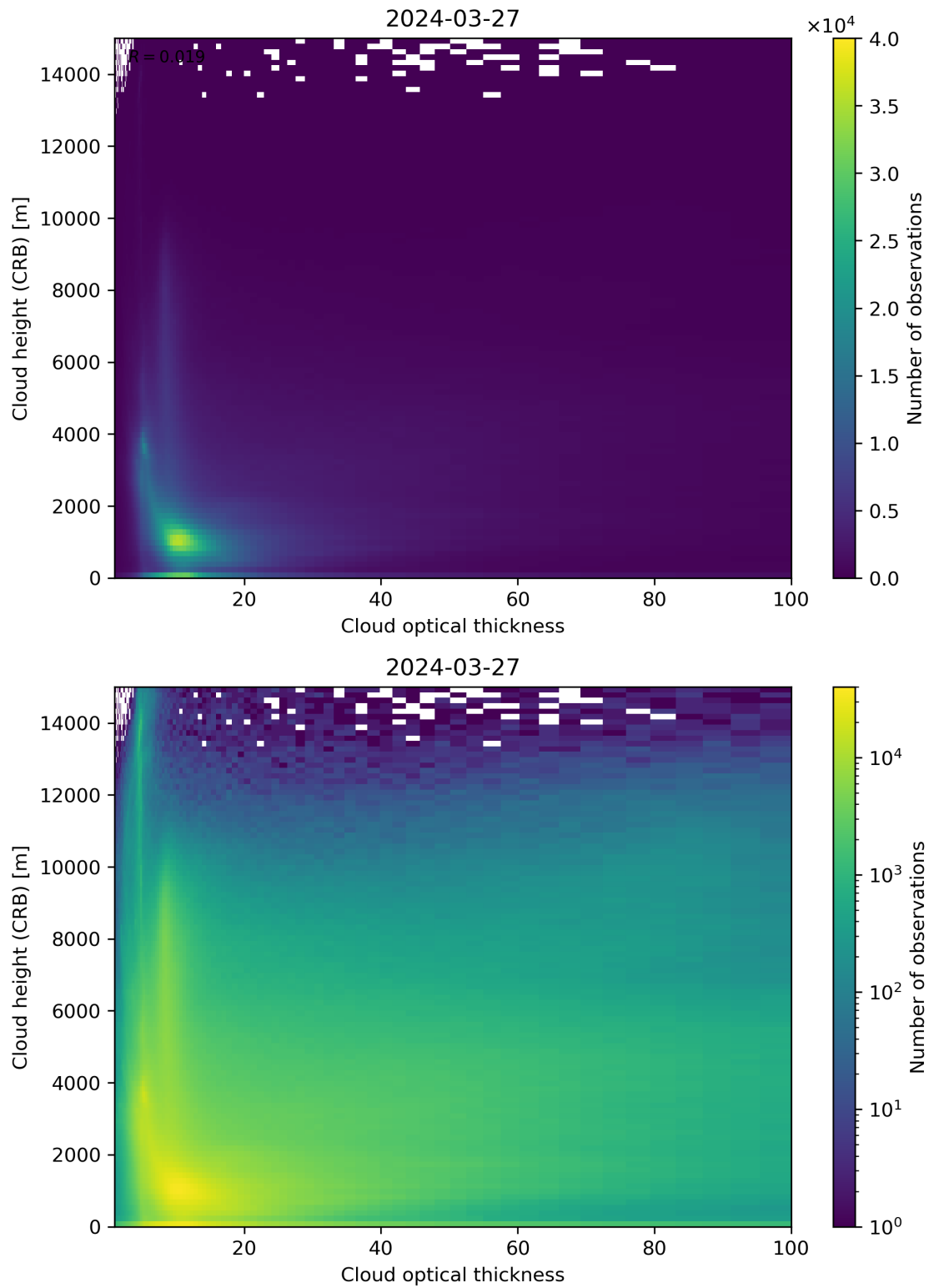
Figure 85: Scatter density plot of “Cloud optical thickness” against “Cloud height (CRB)” for 2024-03-26 to 2024-03-28.
