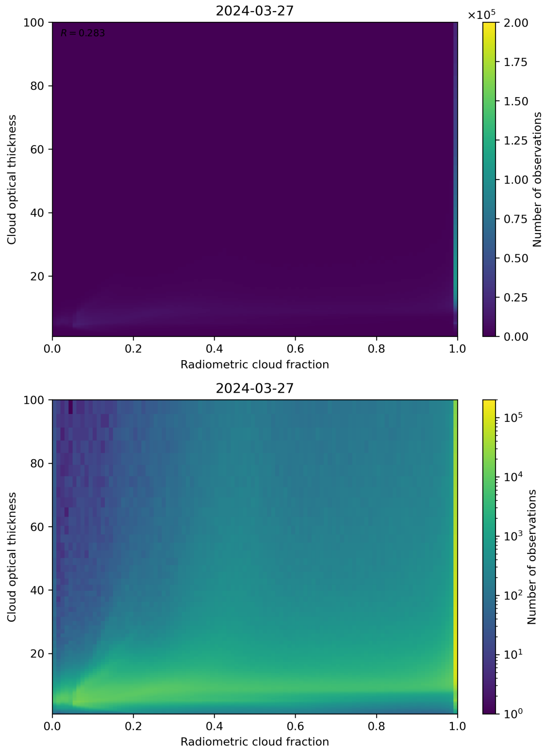
Figure 75: Scatter density plot of “Radiometric cloud fraction” against “Cloud optical thickness” for 2024-03-26 to 2024-03-28.
