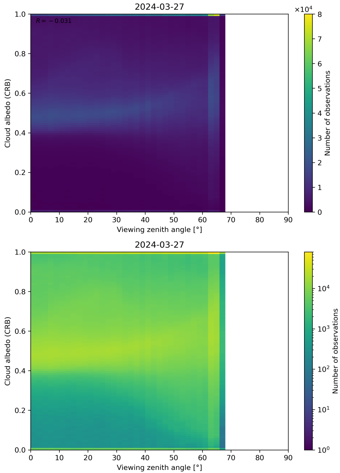
Figure 106: Scatter density plot of “Viewing zenith angle” against “Cloud albedo (CRB)” for 2024-03-26 to 2024-03-28.
