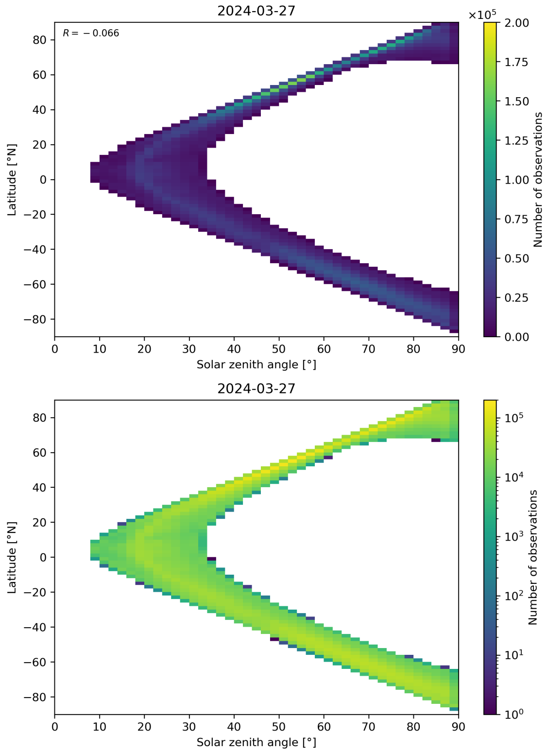
Figure 105: Scatter density plot of “Solar zenith angle” against “Latitude” for 2024-03-26 to 2024-03-28.
