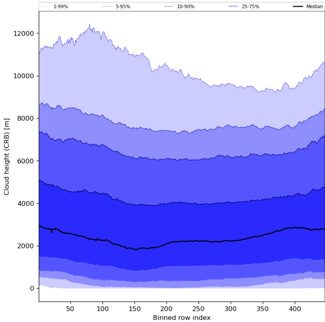
Figure 59: Along track statistics of “Cloud height (CRB)” for 2024-03-26 to 2024-03-28
