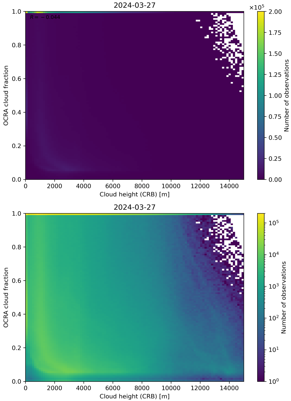
Figure 81: Scatter density plot of “Cloud height (CRB)” against “OCRA cloud fraction” for 2024-03-26 to 2024-03-28.
