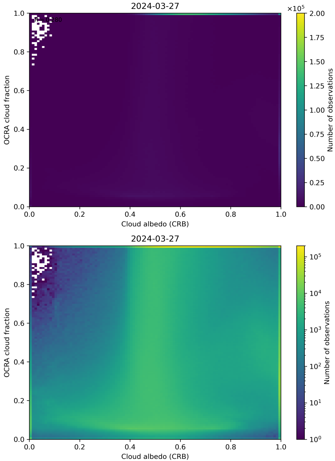
Figure 70: Scatter density plot of “Cloud albedo (CRB)” against “OCRA cloud fraction” for 2024-03-26 to 2024-03-28.
