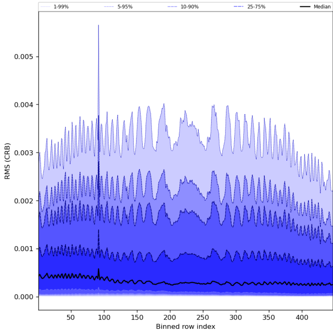
Figure 64: Along track statistics of “RMS (CRB)” for 2024-03-26 to 2024-03-28
