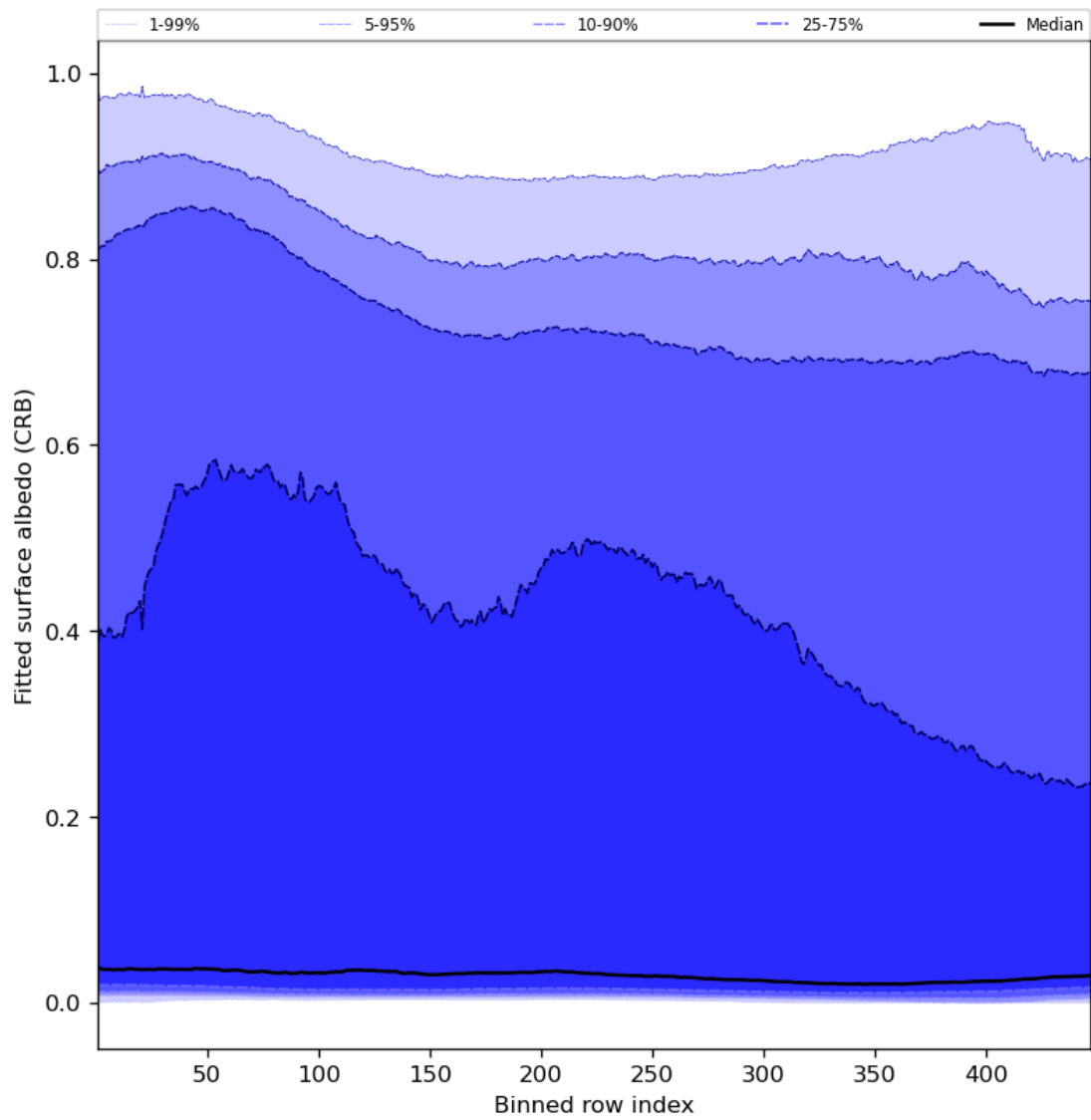
Figure 62: Along track statistics of “Fitted surface albedo (CRB)” for 2024-03-26 to 2024-03-28
