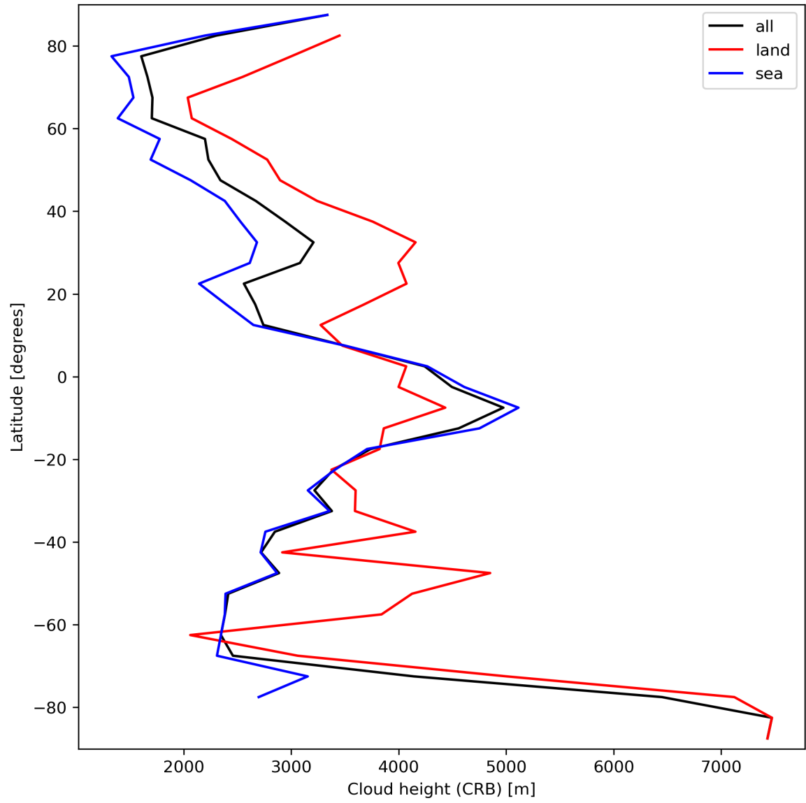
Figure 27: Zonal average of “Cloud height (CRB)” for 2024-03-26 to 2024-03-28.
