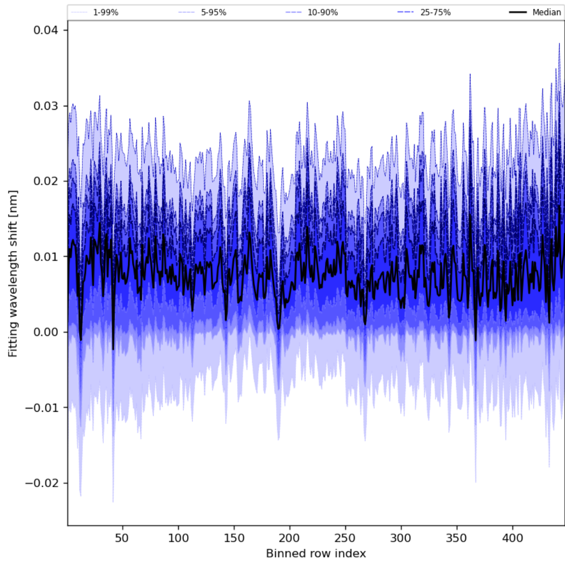
Figure 65: Along track statistics of “Fitting wavelength shift” for 2024-03-26 to 2024-03-28
