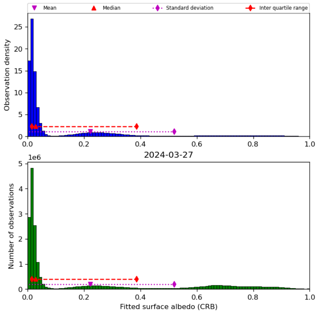
Figure 46: Histogram of “Fitted surface albedo (CRB)” for 2024-03-26 to 2024-03-28
