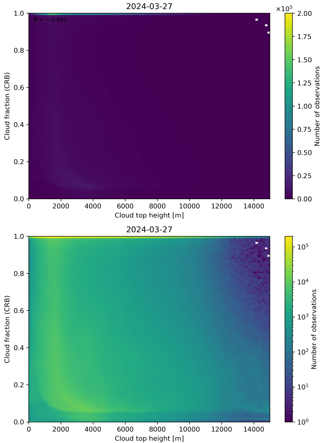
Figure 88: Scatter density plot of “Cloud top height” against “Cloud fraction (CRB)” for 2024-03-26 to 2024-03-28.
