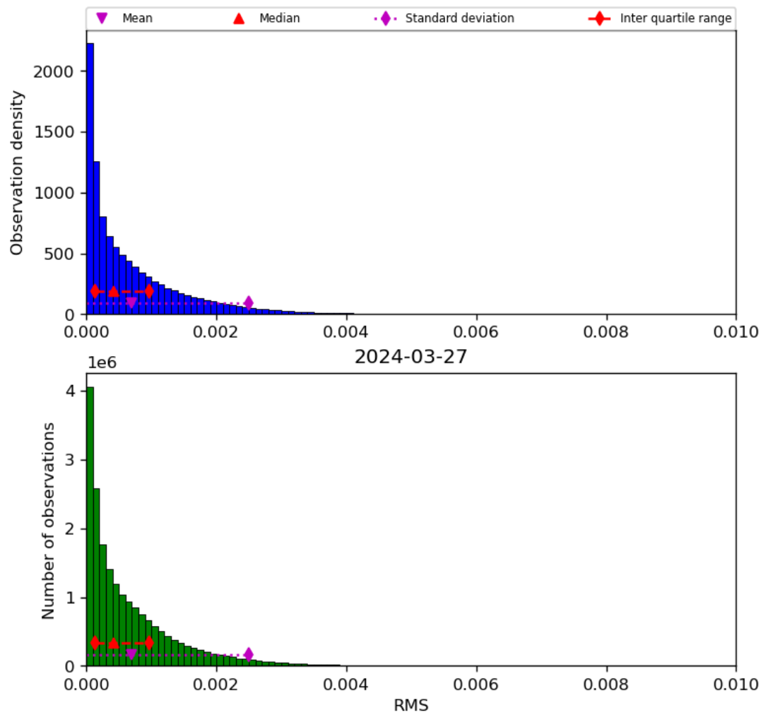
Figure 47: Histogram of “RMS” for 2024-03-26 to 2024-03-28
