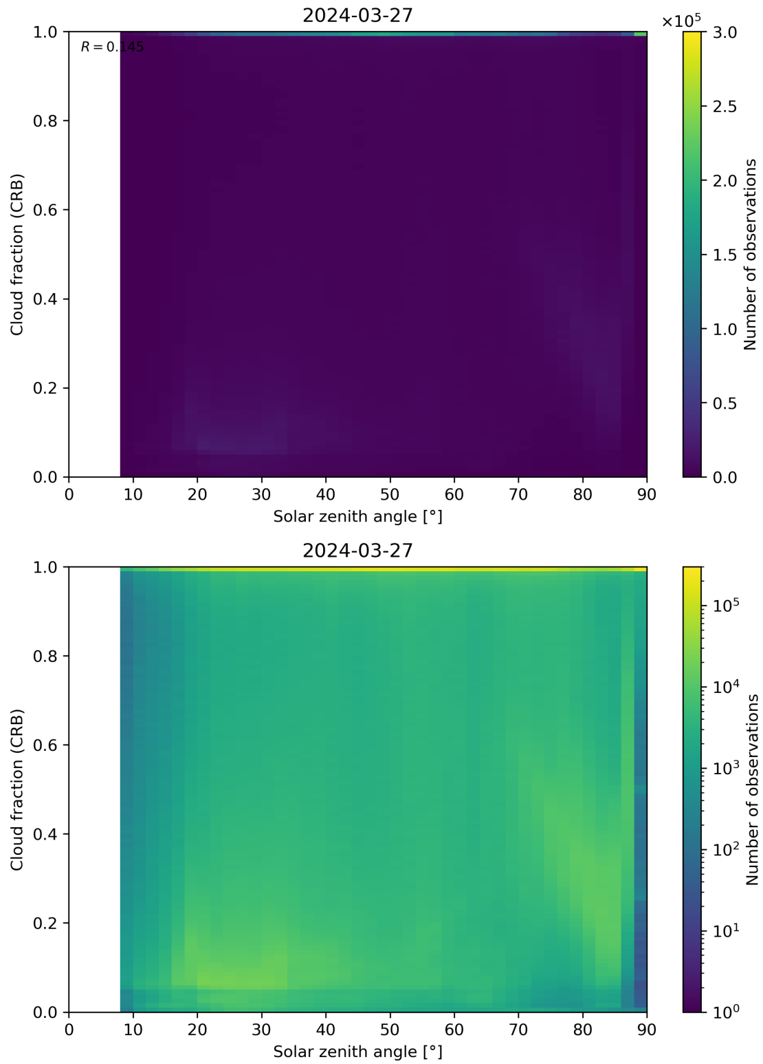
Figure 101: Scatter density plot of “Solar zenith angle” against “Cloud fraction (CRB)” for 2024-03-26 to 2024-03-28.
