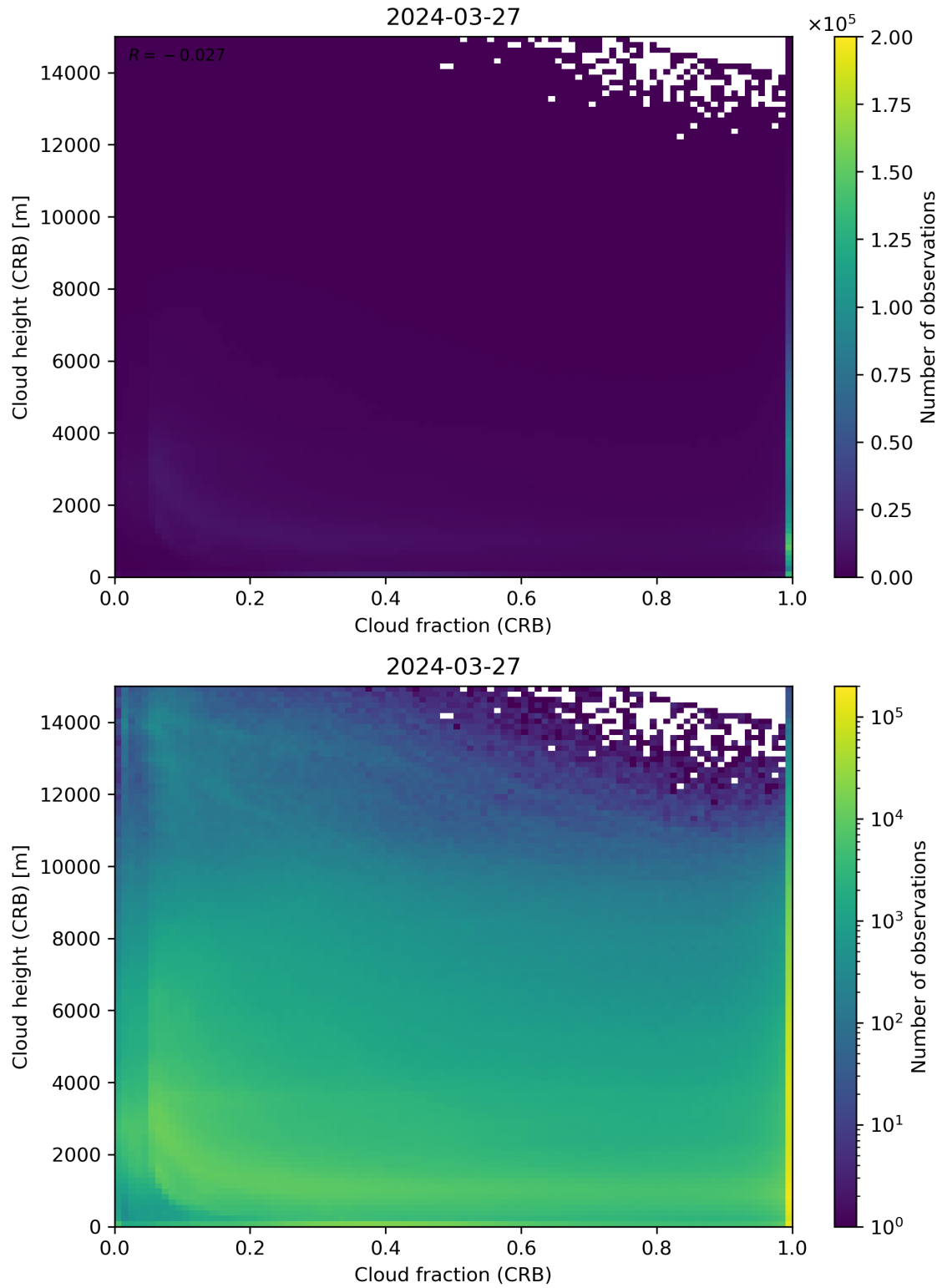
Figure 79: Scatter density plot of “Cloud fraction (CRB)” against “Cloud height (CRB)” for 2024-03-26 to 2024-03-28.
