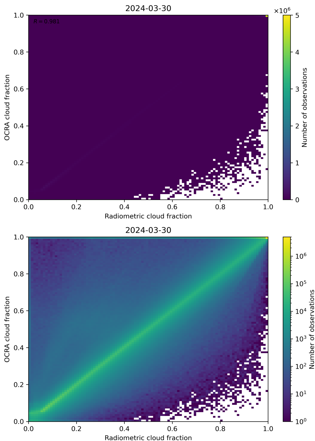
Figure 72: Scatter density plot of “Radiometric cloud fraction” against “OCRA cloud fraction” for 2024-03-30 to 2024-03-31.
