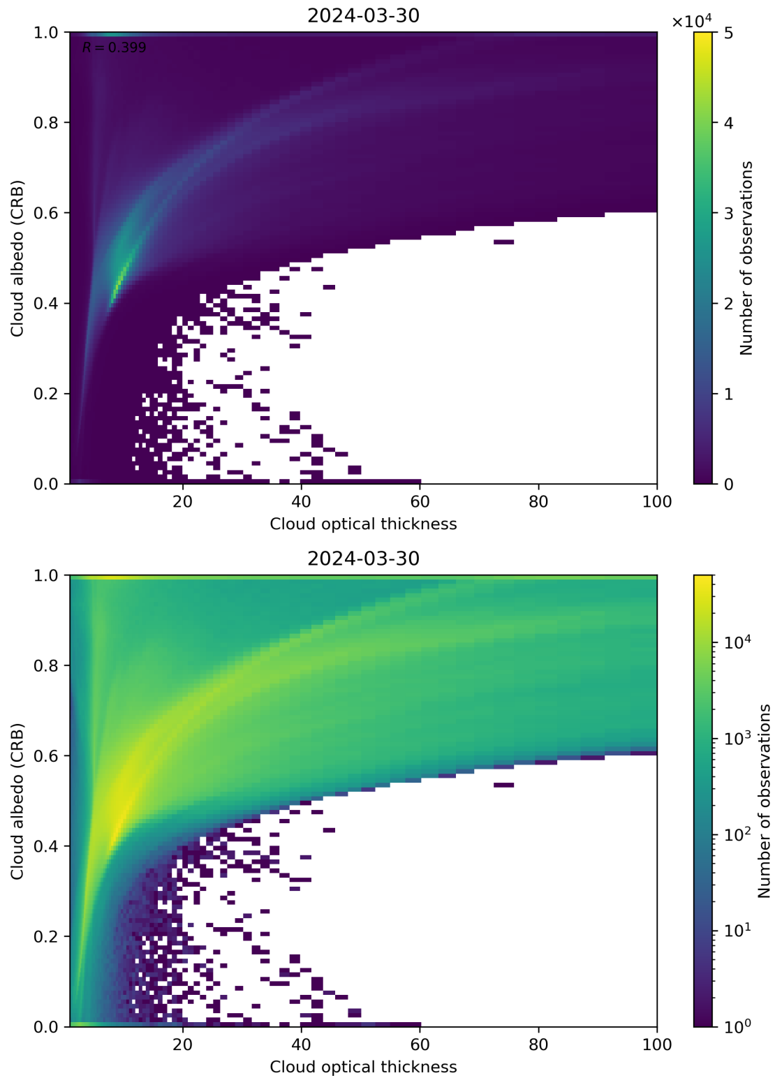
Figure 82: Scatter density plot of “Cloud optical thickness” against “Cloud albedo (CRB)” for 2024-03-30 to 2024-03-31.
