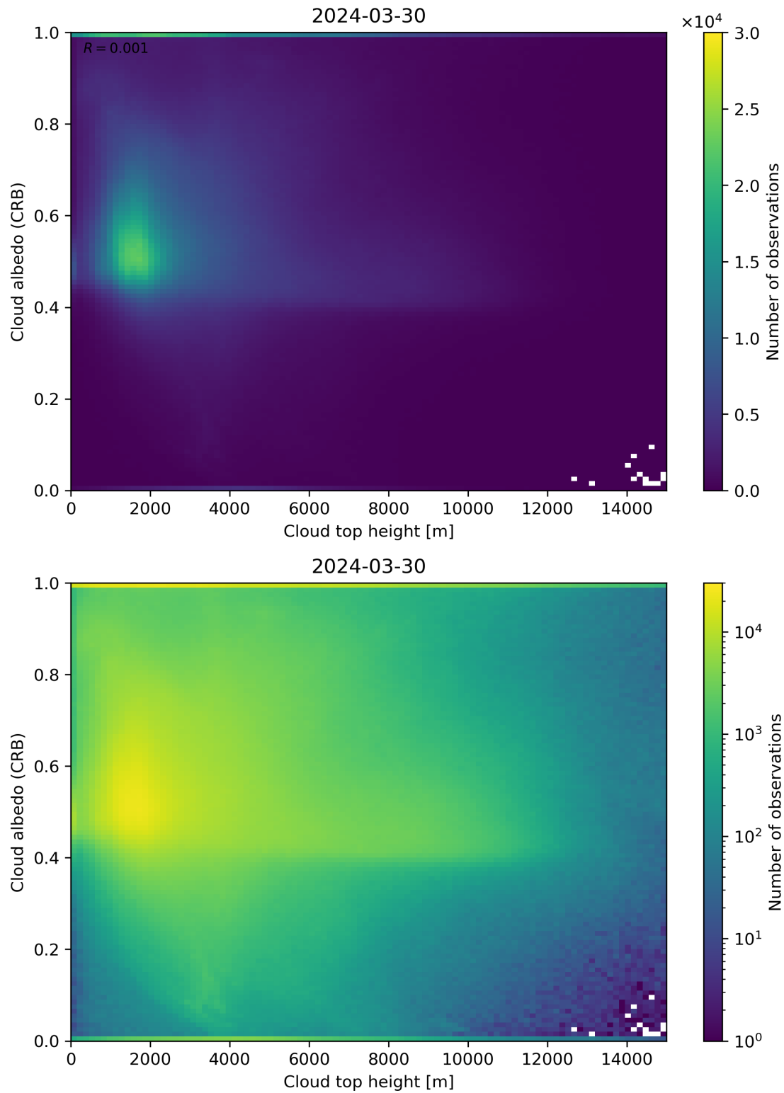
Figure 86: Scatter density plot of “Cloud top height” against “Cloud albedo (CRB)” for 2024-03-30 to 2024-03-31.
