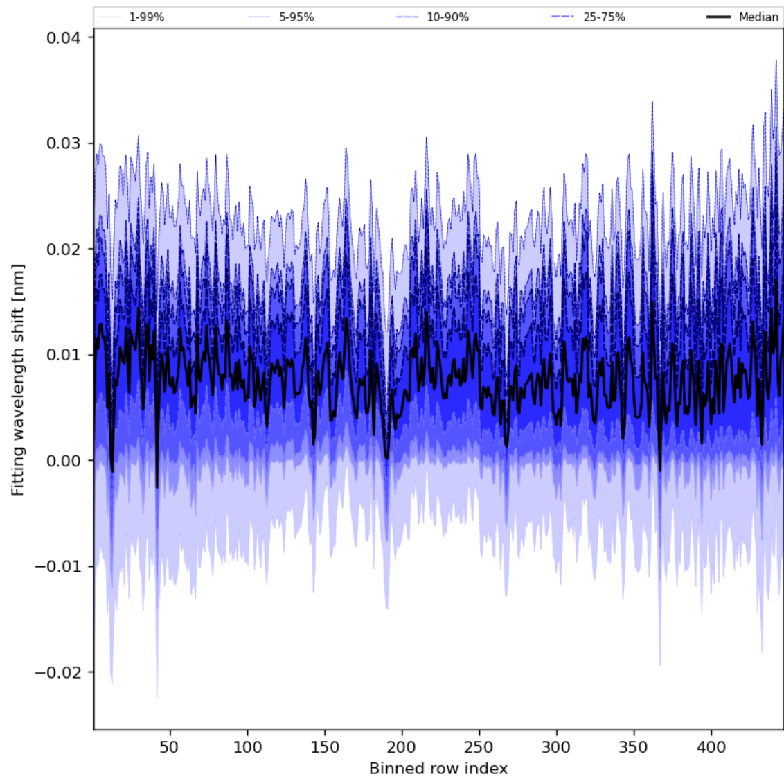
Figure 65: Along track statistics of “Fitting wavelength shift” for 2024-03-30 to 2024-03-31
