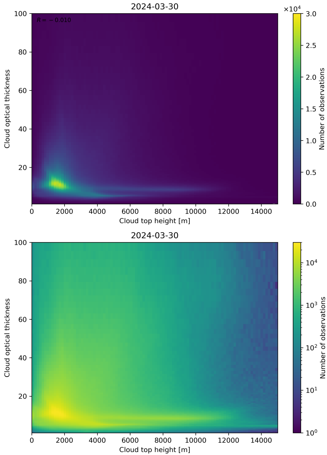
Figure 90: Scatter density plot of “Cloud top height” against “Cloud optical thickness” for 2024-03-30 to 2024-03-31.
