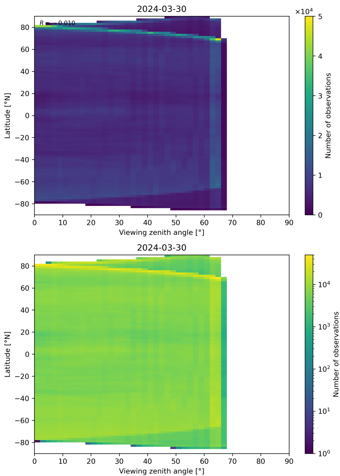
Figure 113: Scatter density plot of “Viewing zenith angle” against “Latitude” for 2024-03-30 to 2024-03-31.
