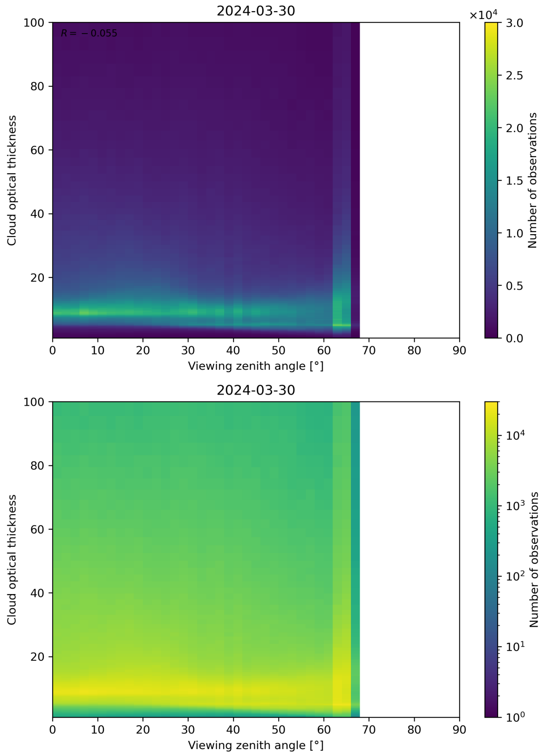
Figure 111: Scatter density plot of “Viewing zenith angle” against “Cloud optical thickness” for 2024-03-30 to 2024-03-31.
