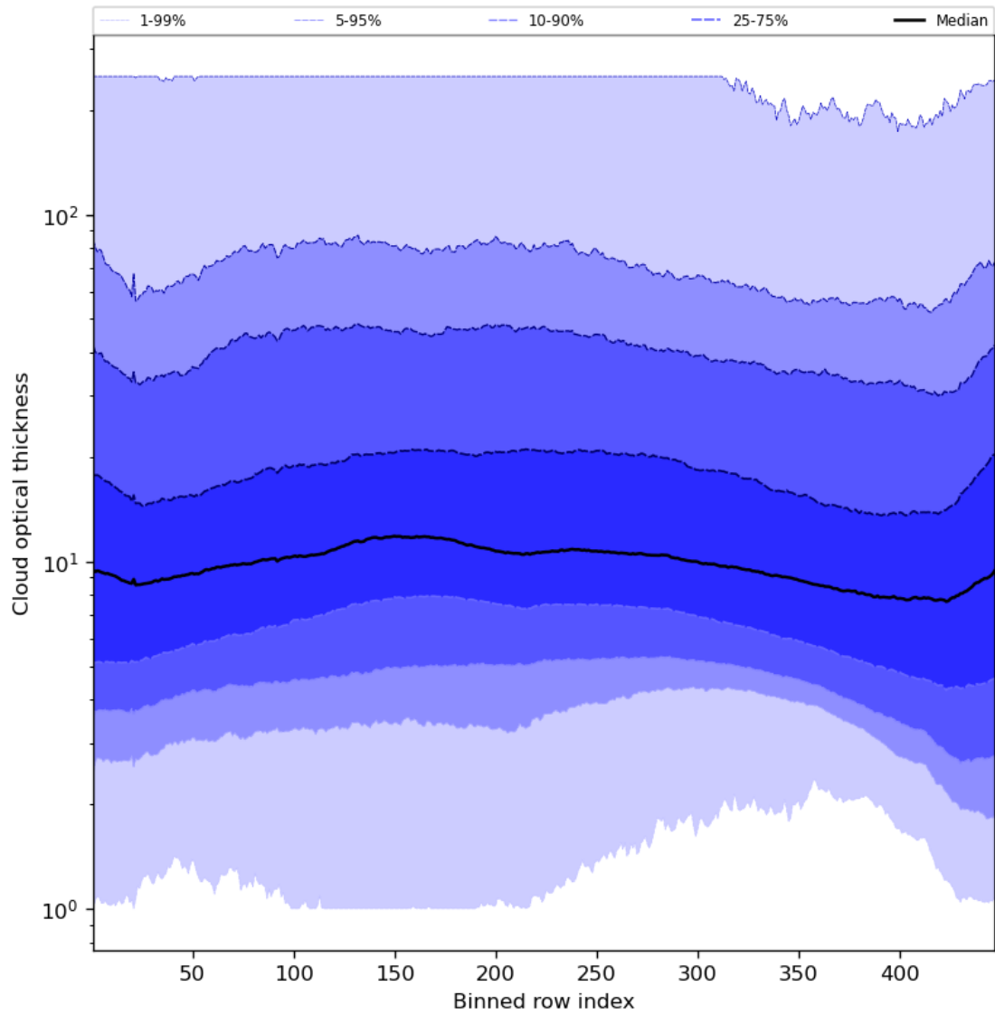
Figure 57: Along track statistics of “Cloud optical thickness” for 2024-03-30 to 2024-03-31
