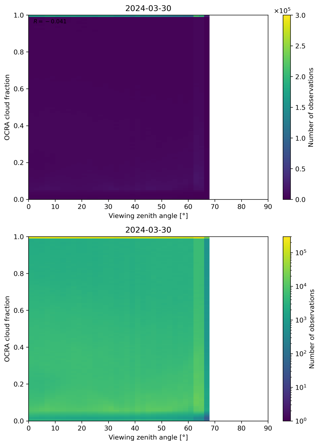
Figure 108: Scatter density plot of “Viewing zenith angle” against “OCRA cloud fraction” for 2024-03-30 to 2024-03-31.
