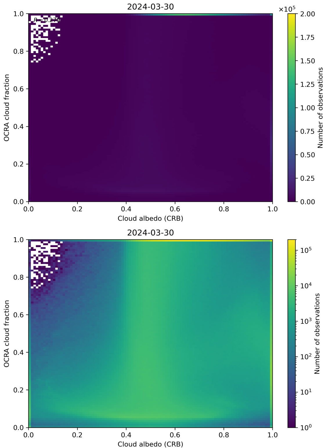
Figure 70: Scatter density plot of “Cloud albedo (CRB)” against “OCRA cloud fraction” for 2024-03-30 to 2024-03-31.
