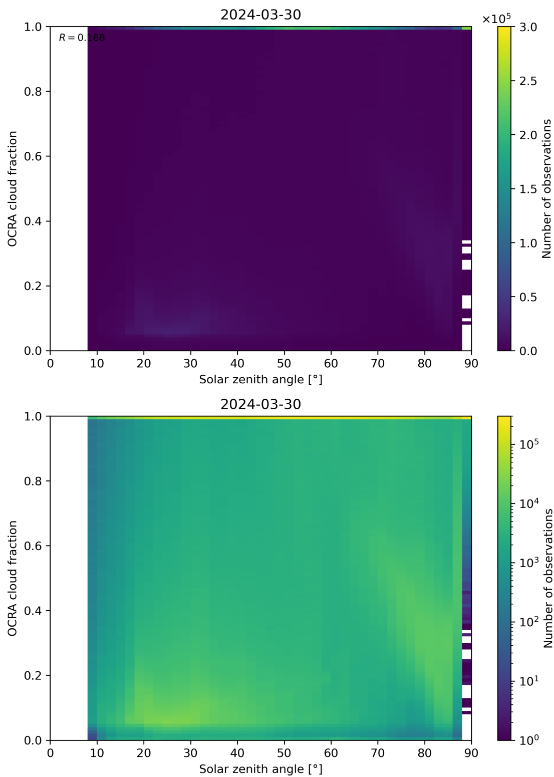
Figure 100: Scatter density plot of “Solar zenith angle” against “OCRA cloud fraction” for 2024-03-30 to 2024-03-31.
