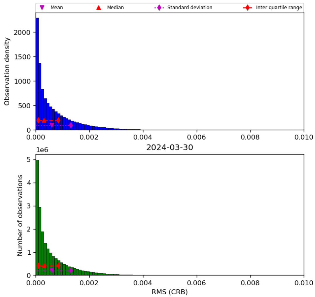
Figure 48: Histogram of “RMS (CRB)” for 2024-03-30 to 2024-03-31
