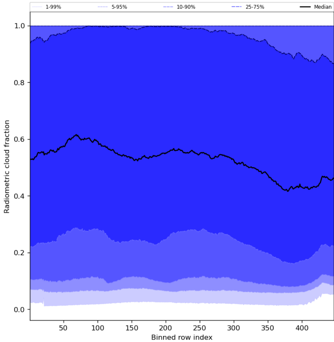
Figure 55: Along track statistics of “Radiometric cloud fraction” for 2024-03-30 to 2024-03-31
