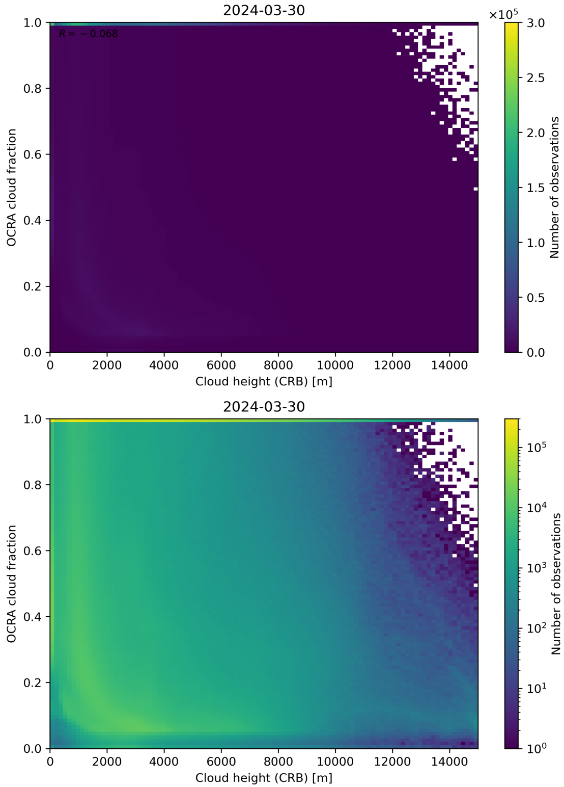
Figure 81: Scatter density plot of “Cloud height (CRB)” against “OCRA cloud fraction” for 2024-03-30 to 2024-03-31.
