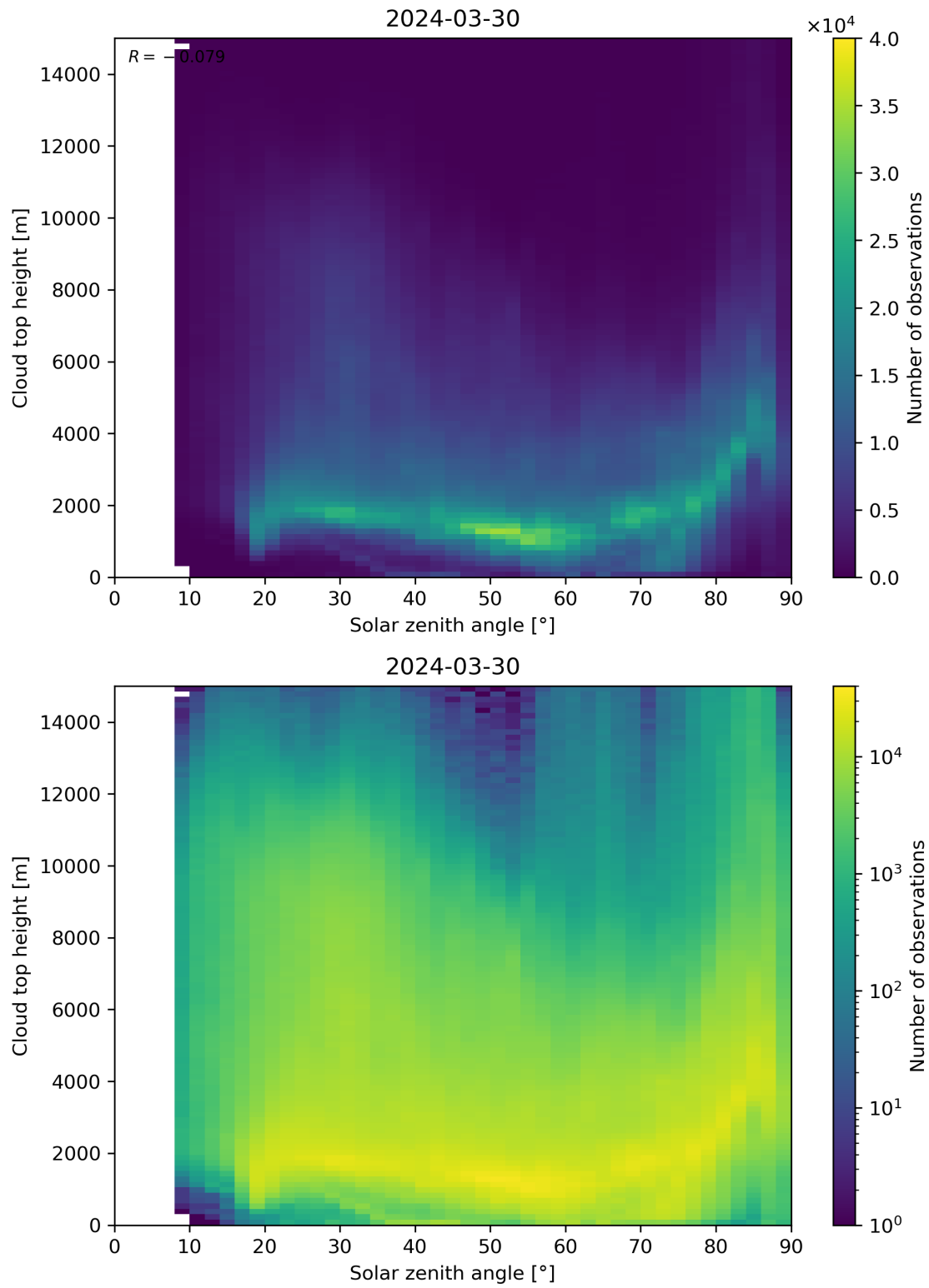
Figure 104: Scatter density plot of “Solar zenith angle” against “Cloud top height” for 2024-03-30 to 2024-03-31.
