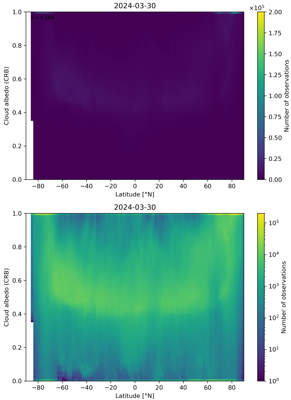
Figure 91: Scatter density plot of “Latitude” against “Cloud albedo (CRB)” for 2024-03-30 to 2024-03-31.
