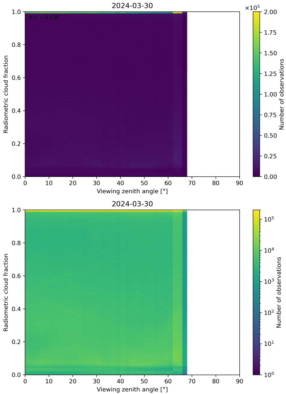
Figure 107: Scatter density plot of “Viewing zenith angle” against “Radiometric cloud fraction” for 2024-03-30 to 2024-03-31.
