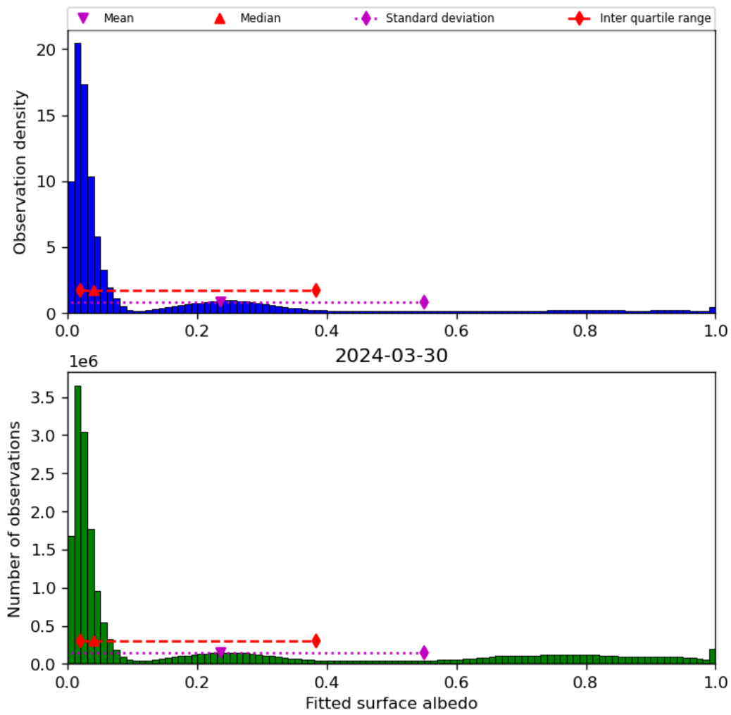
Figure 45: Histogram of “Fitted surface albedo” for 2024-03-30 to 2024-03-31
