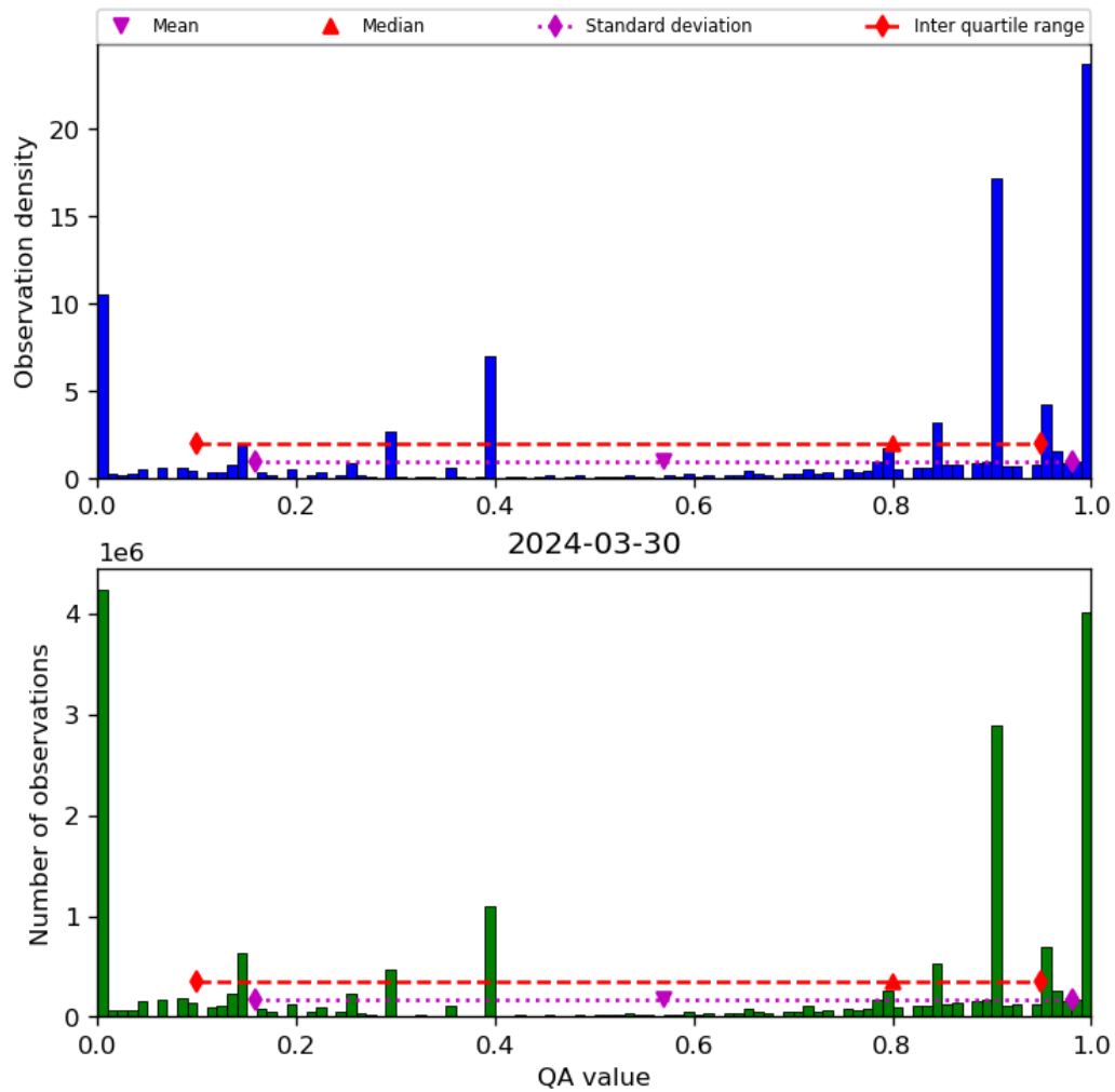
Figure 38: Histogram of “QA value” for 2024-03-30 to 2024-03-31
