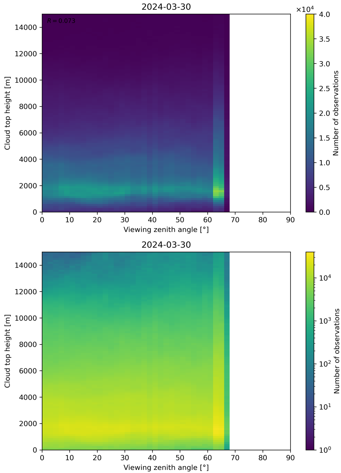
Figure 112: Scatter density plot of “Viewing zenith angle” against “Cloud top height” for 2024-03-30 to 2024-03-31.
