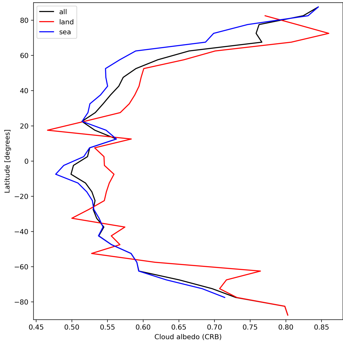
Figure 28: Zonal average of “Cloud albedo (CRB)” for 2024-03-30 to 2024-03-31.
