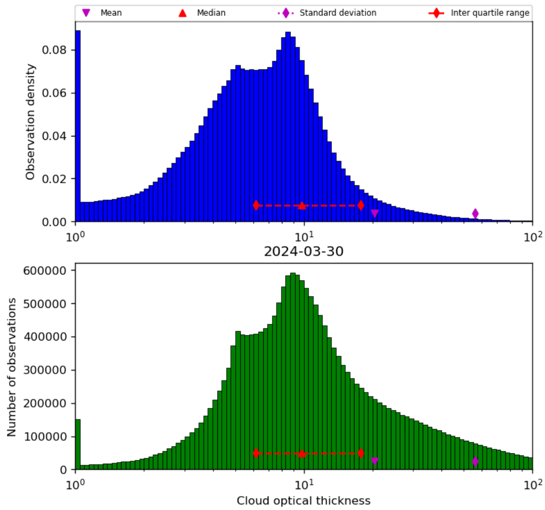
Figure 41: Histogram of “Cloud optical thickness” for 2024-03-30 to 2024-03-31
