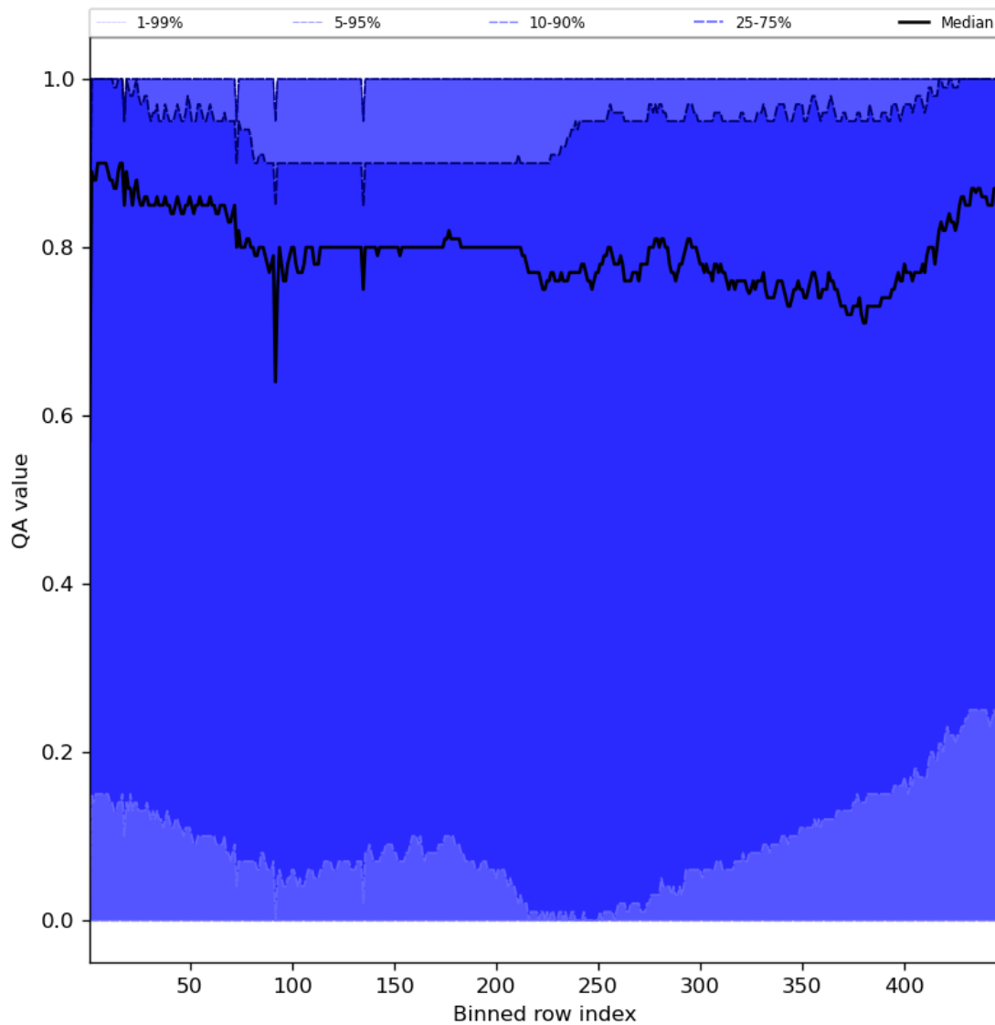
Figure 54: Along track statistics of “QA value” for 2024-03-30 to 2024-03-31
