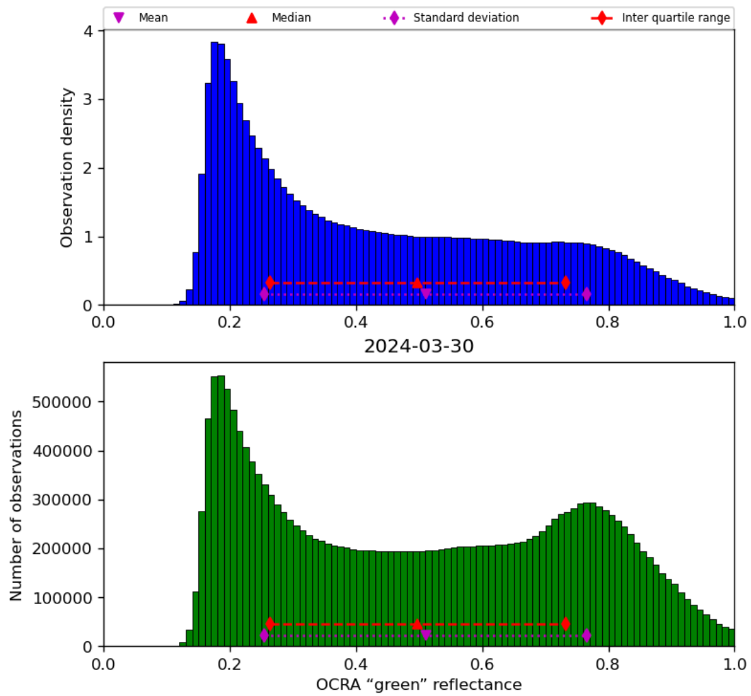
Figure 52: Histogram of “OCRA “green” reflectance” for 2024-03-30 to 2024-03-31
