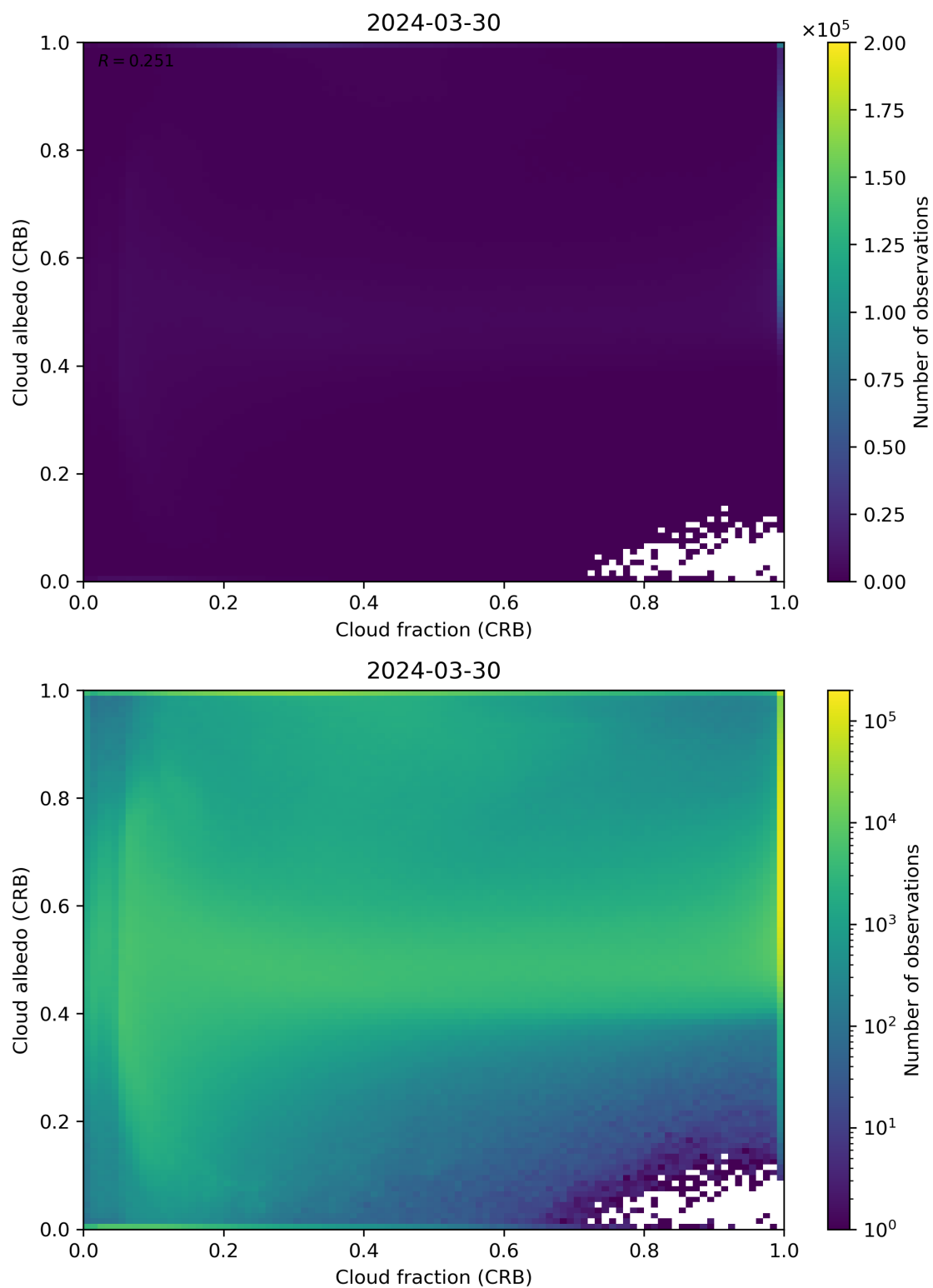
Figure 77: Scatter density plot of “Cloud fraction (CRB)” against “Cloud albedo (CRB)” for 2024-03-30 to 2024-03-31.
