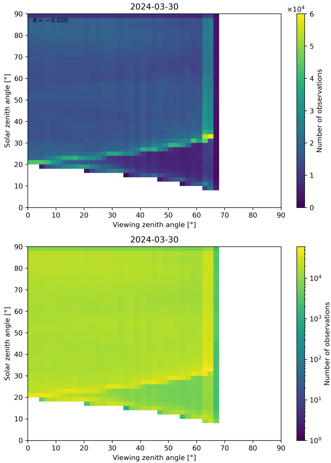
Figure 114: Scatter density plot of “Viewing zenith angle” against “Solar zenith angle” for 2024-03-30 to 2024-03-31.
