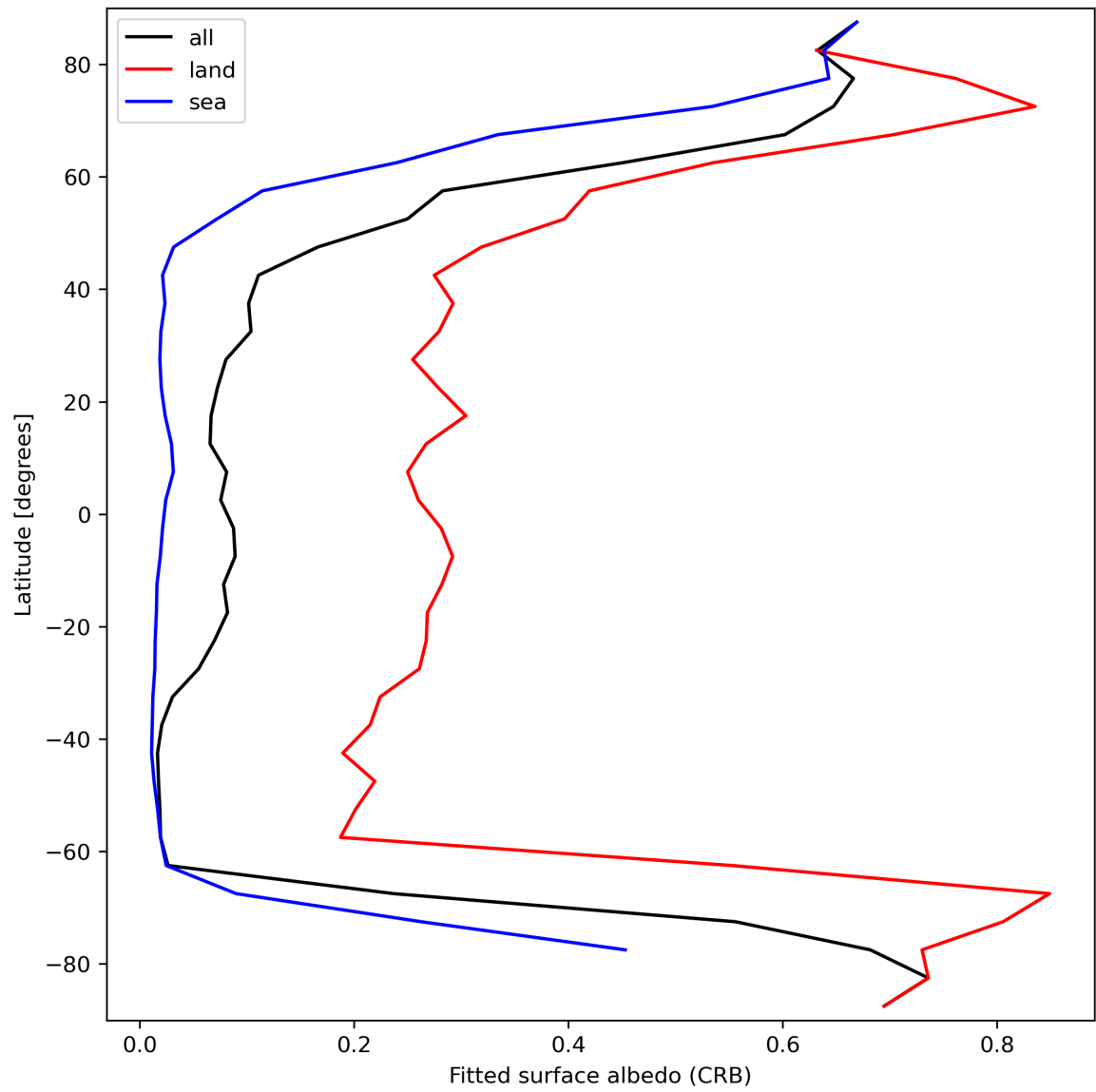
Figure 30: Zonal average of “Fitted surface albedo (CRB)” for 2024-03-30 to 2024-03-31.
