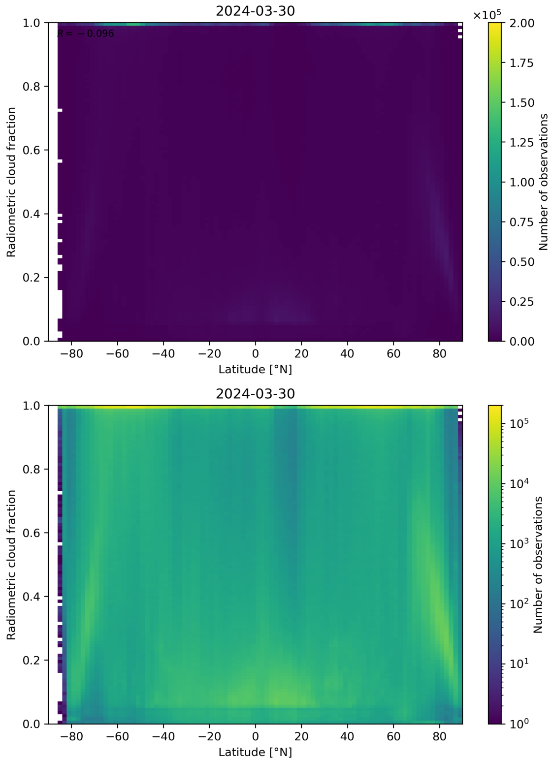
Figure 92: Scatter density plot of “Latitude” against “Radiometric cloud fraction” for 2024-03-30 to 2024-03-31.
