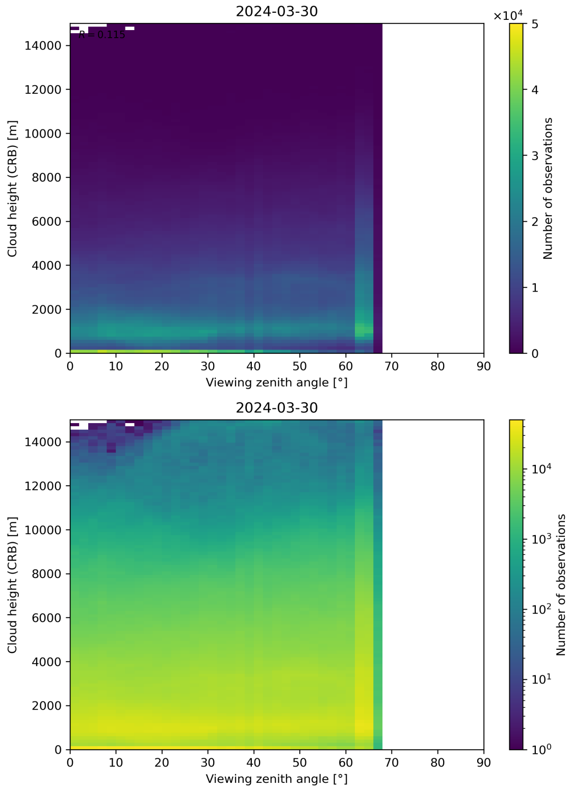
Figure 110: Scatter density plot of “Viewing zenith angle” against “Cloud height (CRB)” for 2024-03-30 to 2024-03-31.
