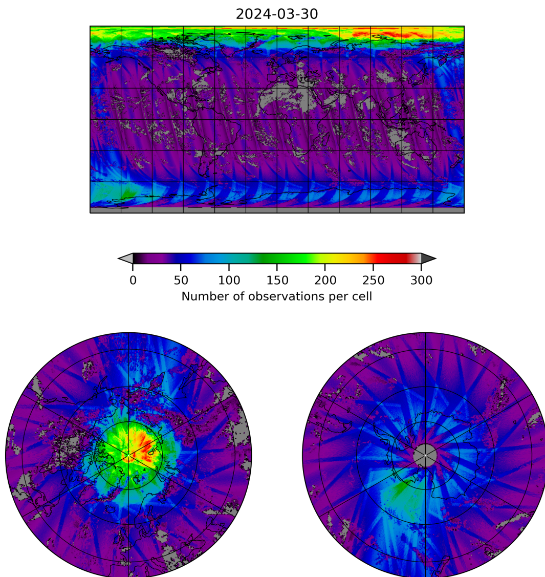
Figure 21: Map of the number of observations for 2024-03-30 to 2024-03-31
