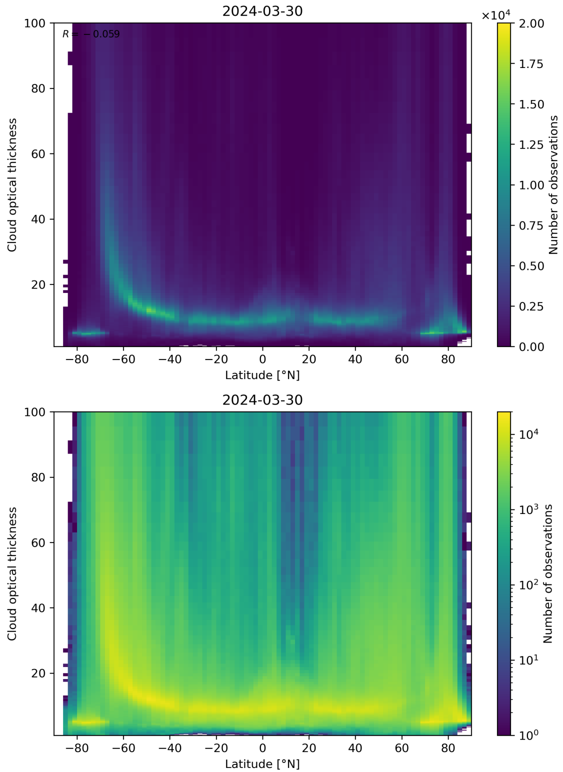
Figure 96: Scatter density plot of “Latitude” against “Cloud optical thickness” for 2024-03-30 to 2024-03-31.
