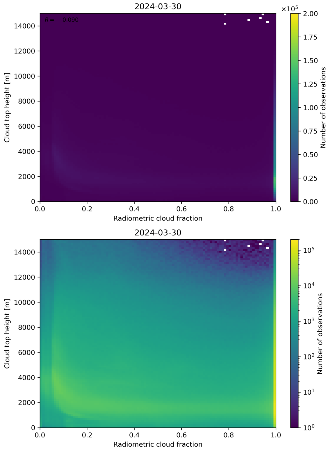
Figure 76: Scatter density plot of “Radiometric cloud fraction” against “Cloud top height” for 2024-03-30 to 2024-03-31.
