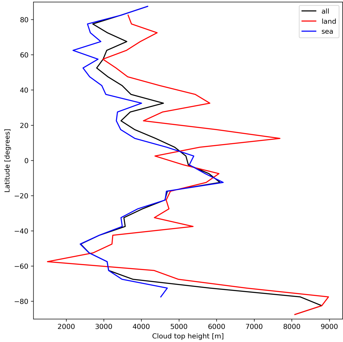
Figure 24: Zonal average of “Cloud top height” for 2024-03-30 to 2024-03-31.
