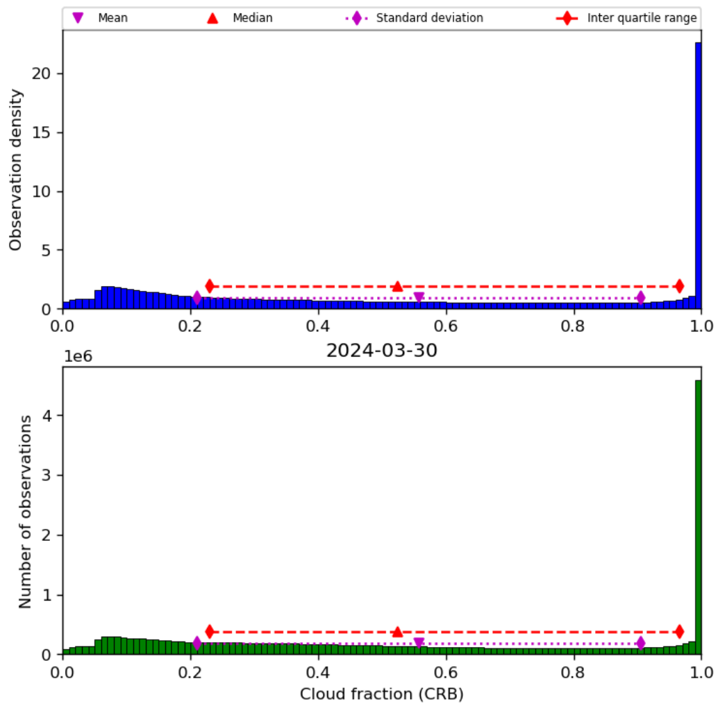
Figure 42: Histogram of “Cloud fraction (CRB)” for 2024-03-30 to 2024-03-31
