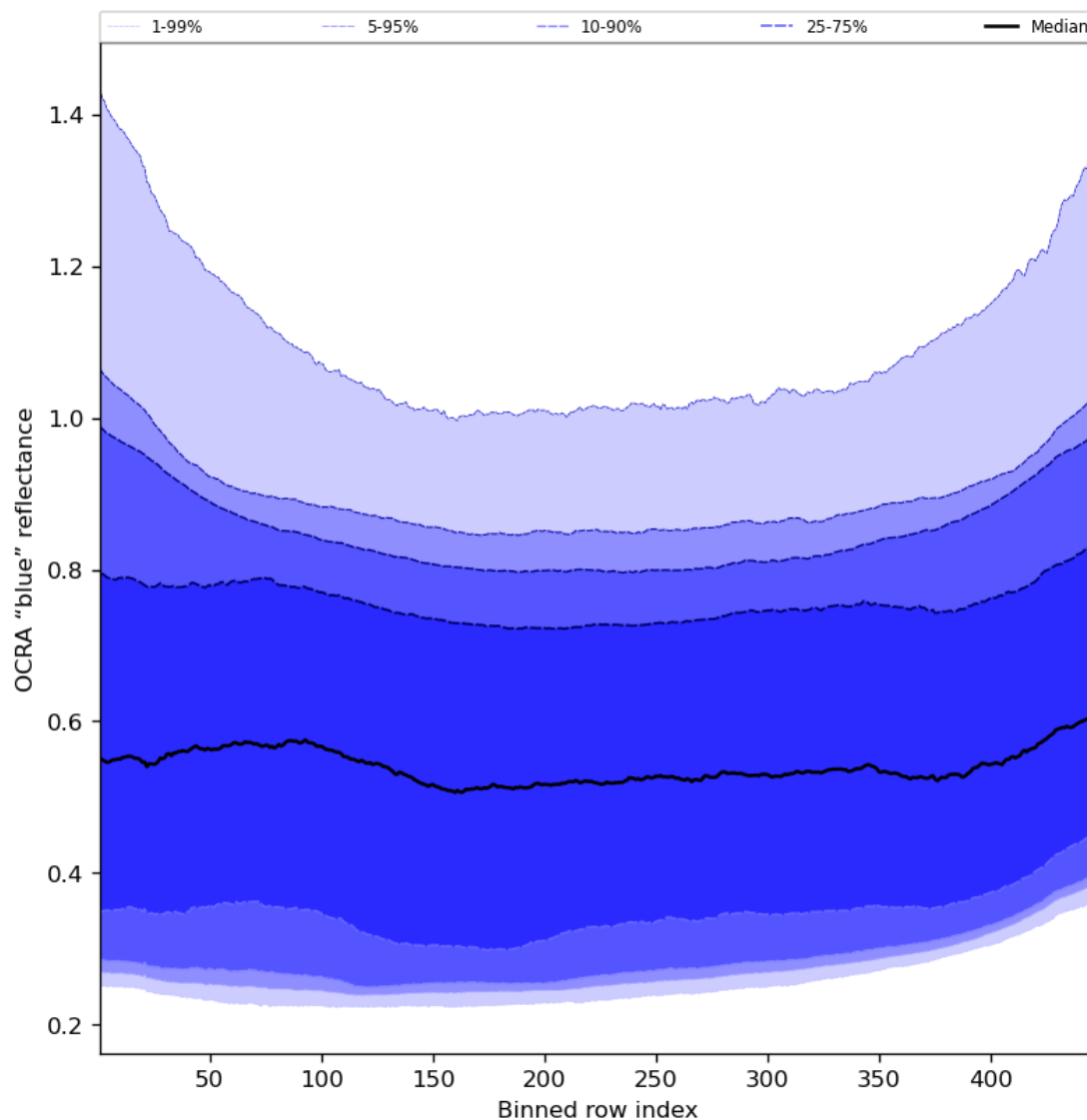
Figure 67: Along track statistics of “OCRA “blue” reflectance” for 2024-03-30 to 2024-03-31
