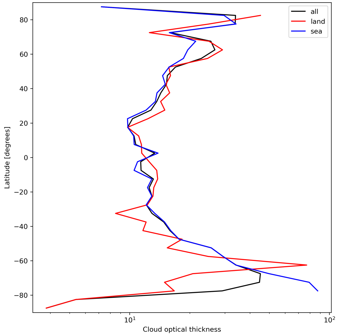
Figure 25: Zonal average of “Cloud optical thickness” for 2024-03-30 to 2024-03-31.
