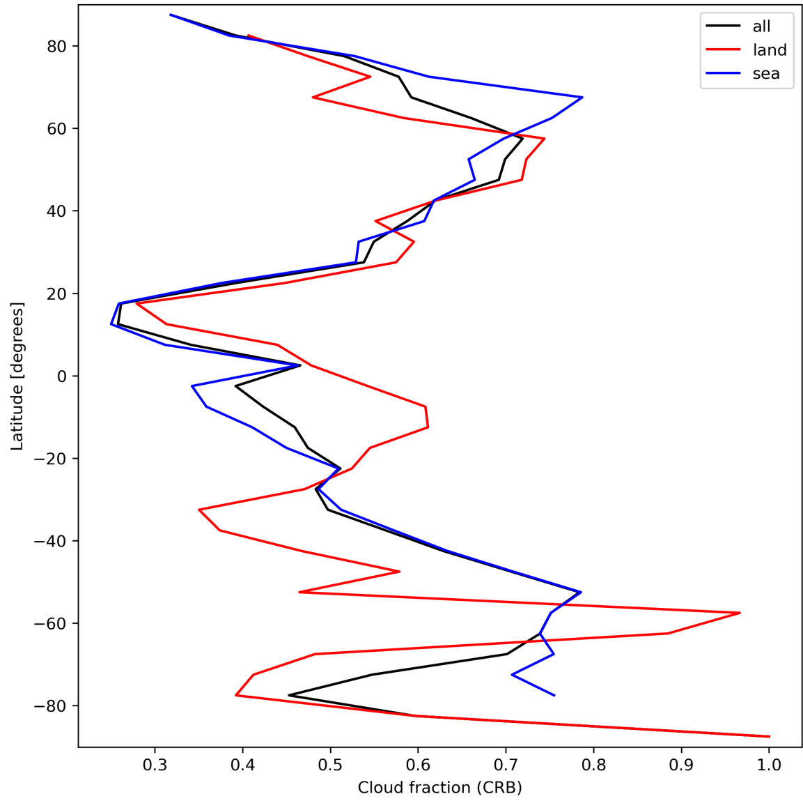
Figure 26: Zonal average of “Cloud fraction (CRB)” for 2024-03-30 to 2024-03-31.
