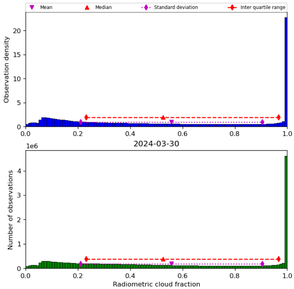
Figure 39: Histogram of “Radiometric cloud fraction” for 2024-03-30 to 2024-03-31
