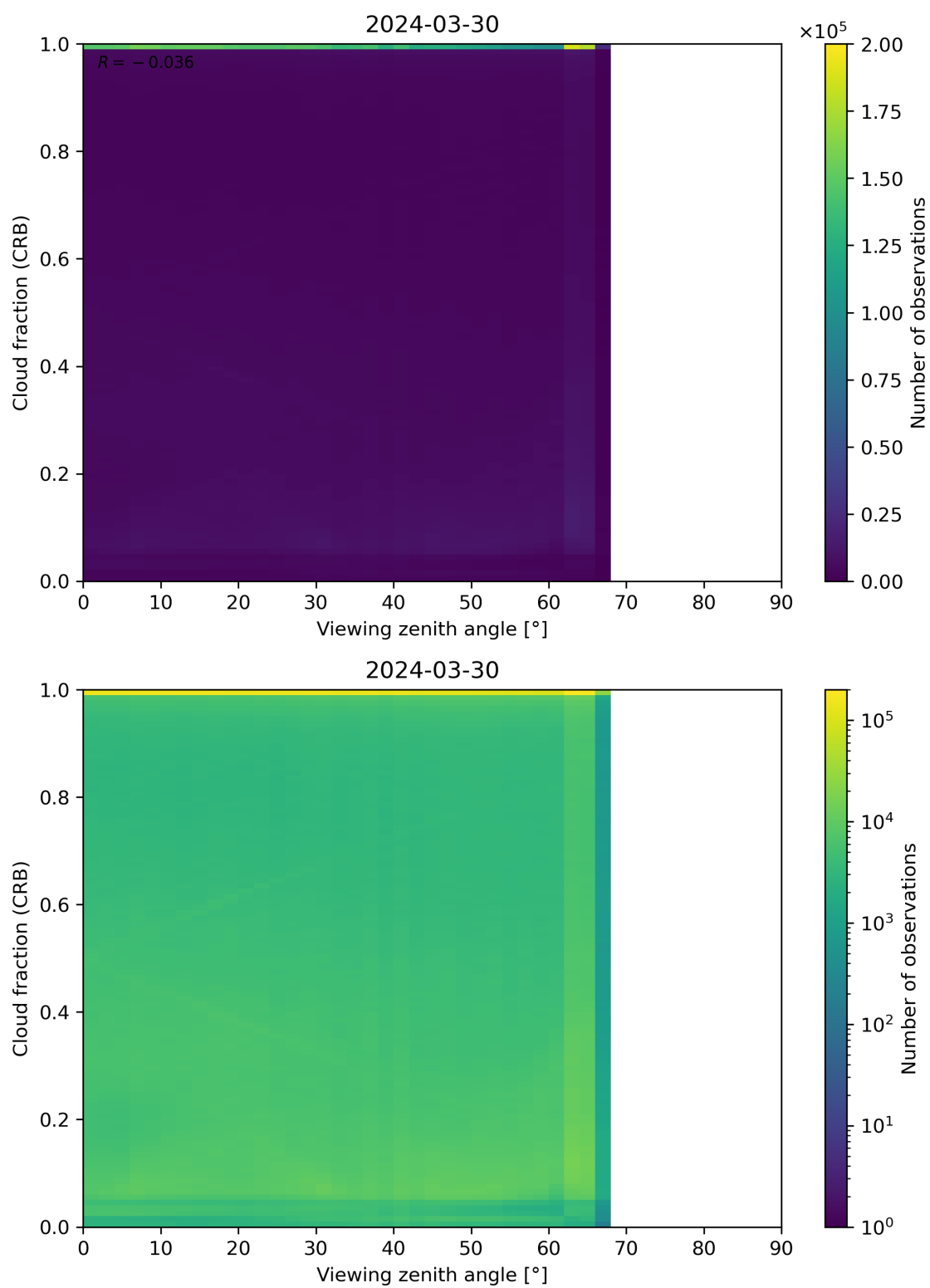
Figure 109: Scatter density plot of “Viewing zenith angle” against “Cloud fraction (CRB)” for 2024-03-30 to 2024-03-31.
