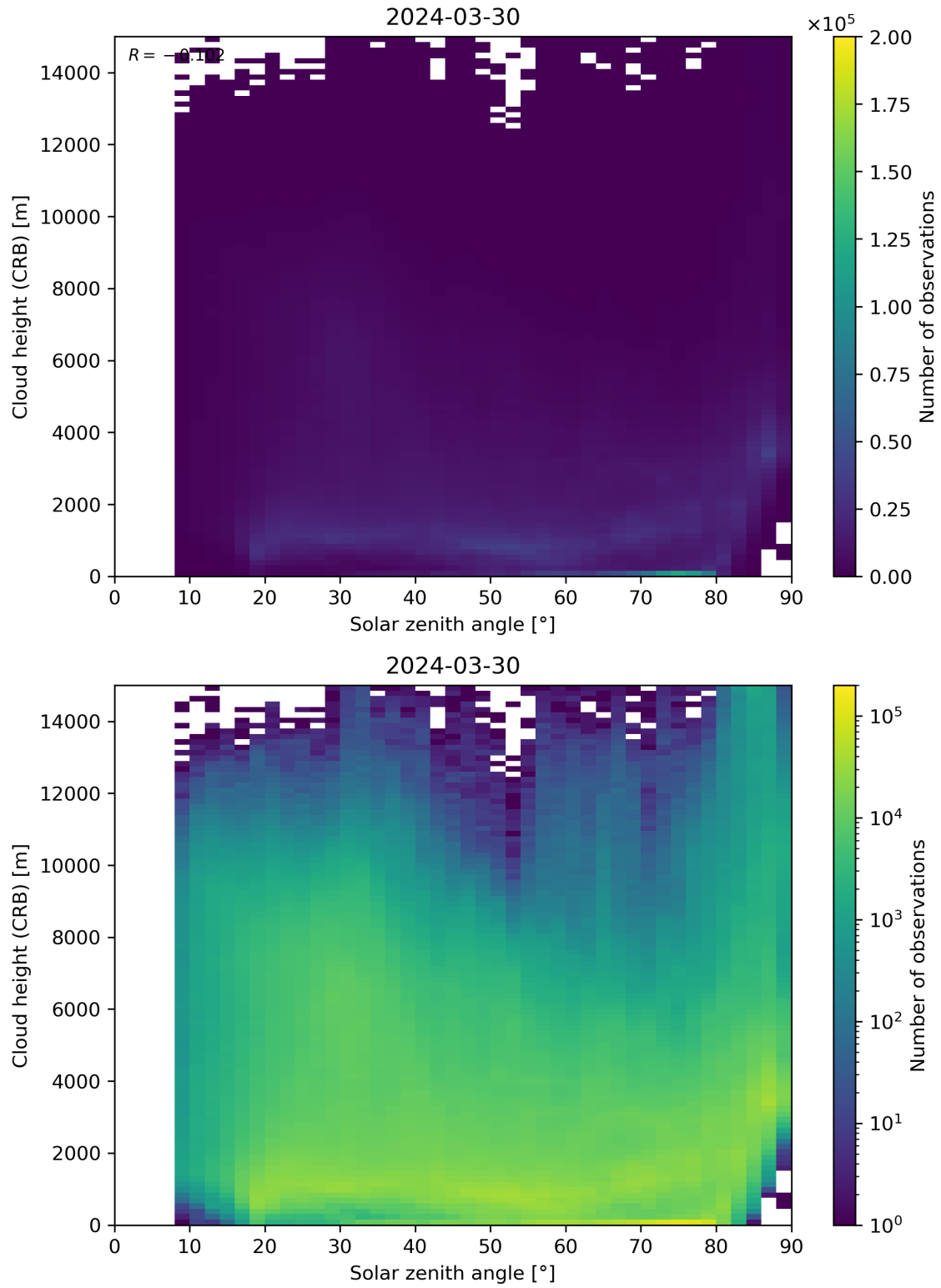
Figure 102: Scatter density plot of “Solar zenith angle” against “Cloud height (CRB)” for 2024-03-30 to 2024-03-31.
