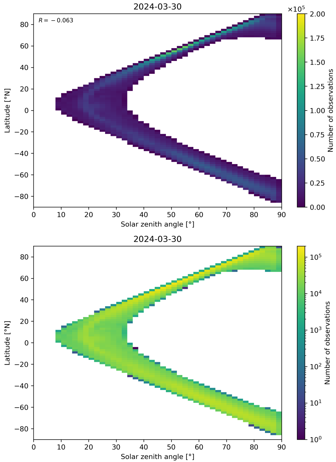
Figure 105: Scatter density plot of “Solar zenith angle” against “Latitude” for 2024-03-30 to 2024-03-31.
