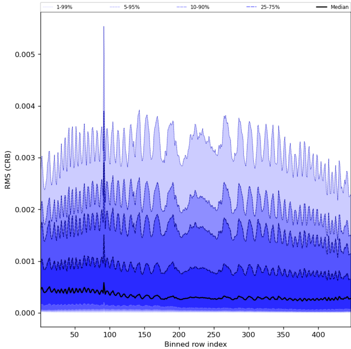
Figure 64: Along track statistics of “RMS (CRB)” for 2024-03-30 to 2024-03-31
