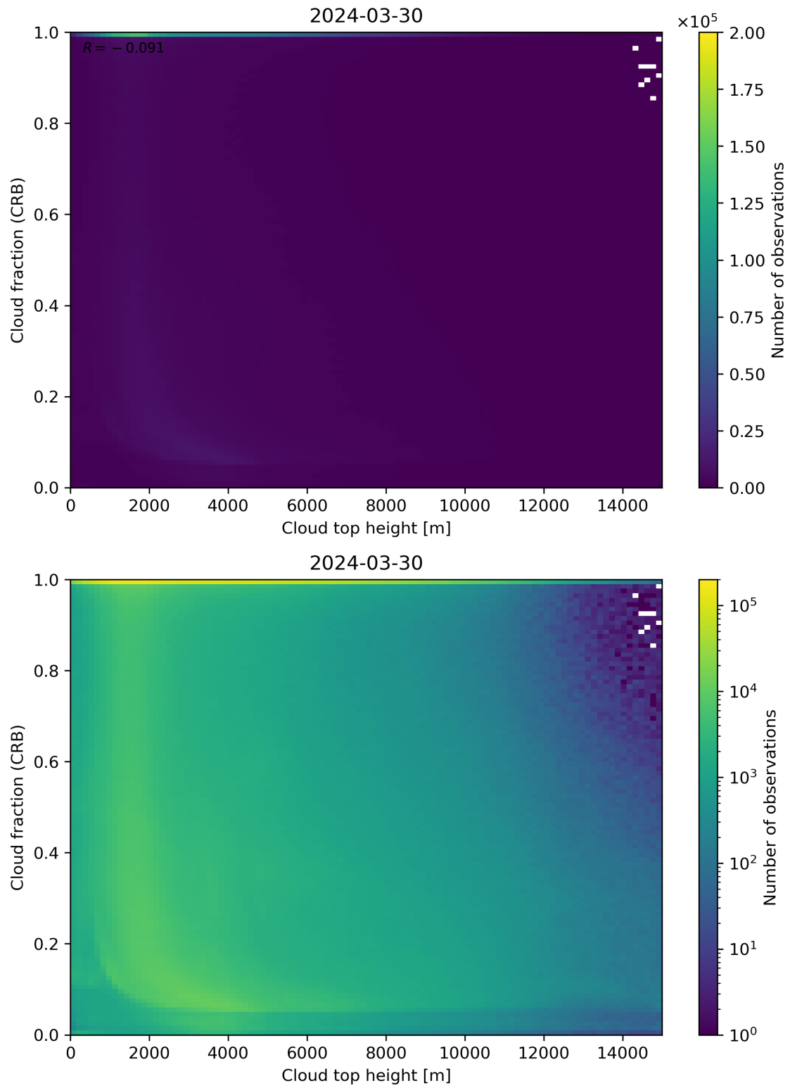
Figure 88: Scatter density plot of “Cloud top height” against “Cloud fraction (CRB)” for 2024-03-30 to 2024-03-31.
