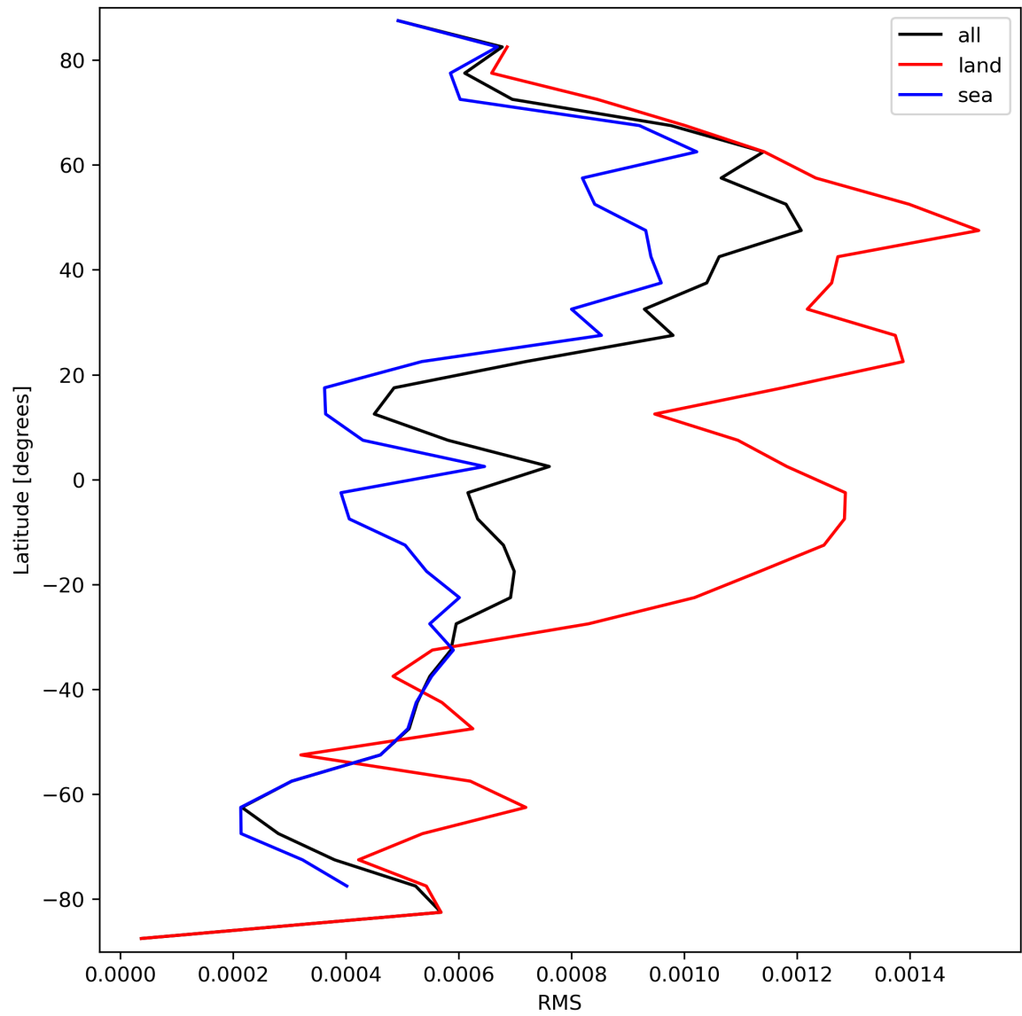
Figure 31: Zonal average of “RMS” for 2024-03-30 to 2024-03-31.
