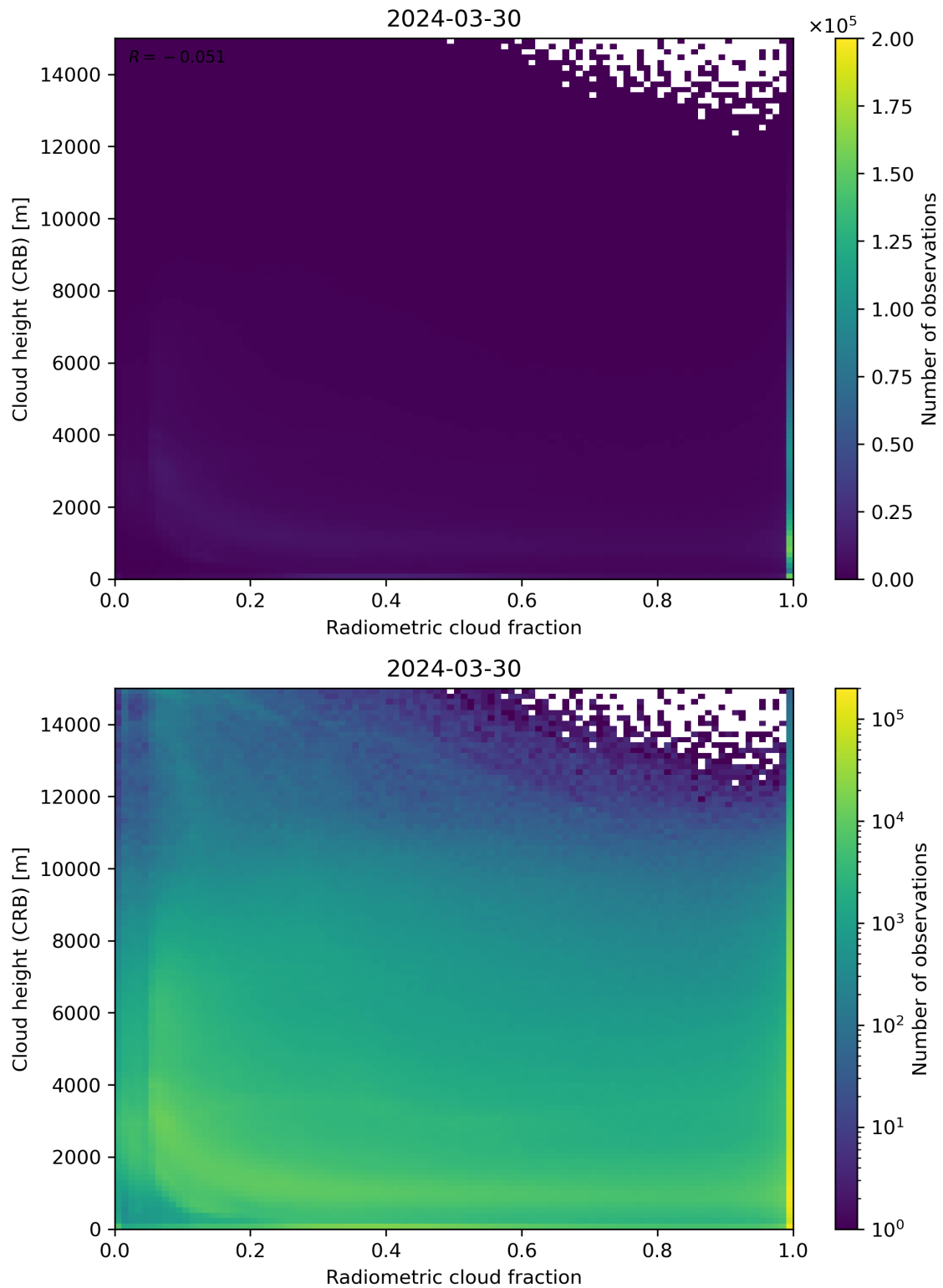
Figure 74: Scatter density plot of “Radiometric cloud fraction” against “Cloud height (CRB)” for 2024-03-30 to 2024-03-31.
