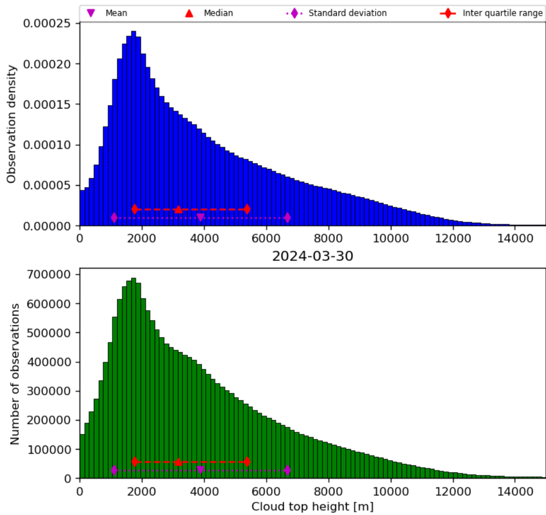
Figure 40: Histogram of “Cloud top height” for 2024-03-30 to 2024-03-31
