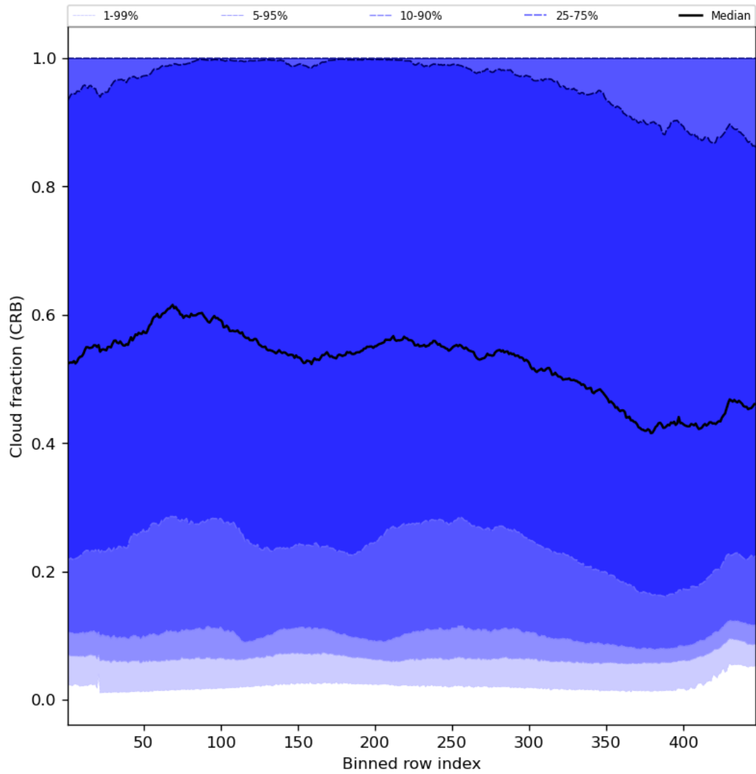
Figure 58: Along track statistics of “Cloud fraction (CRB)” for 2024-03-30 to 2024-03-31
