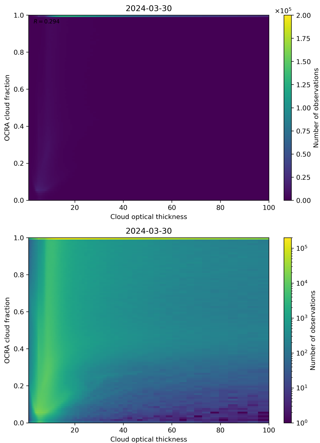
Figure 83: Scatter density plot of “Cloud optical thickness” against “OCRA cloud fraction” for 2024-03-30 to 2024-03-31.
