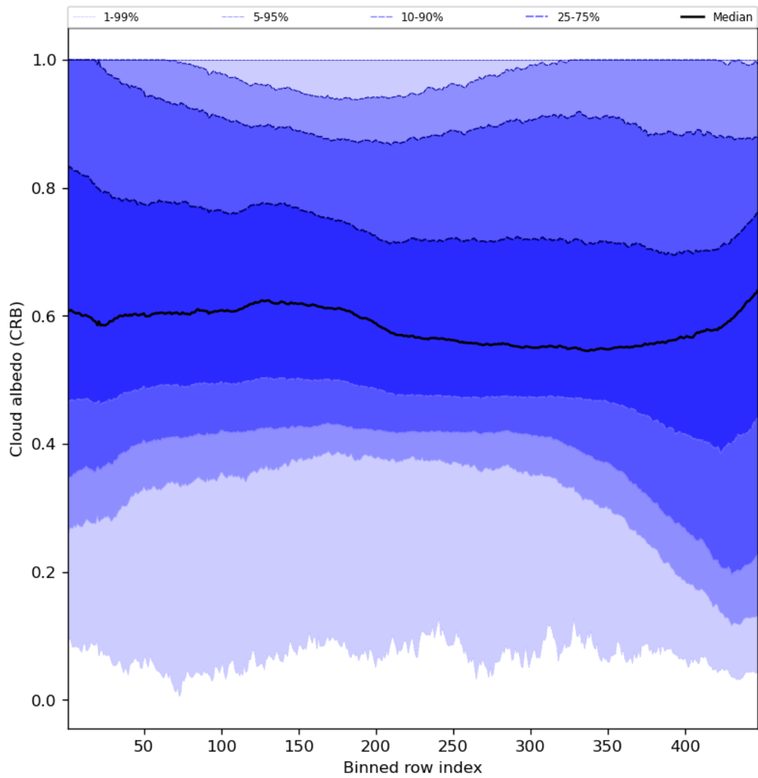
Figure 60: Along track statistics of “Cloud albedo (CRB)” for 2024-03-30 to 2024-03-31
