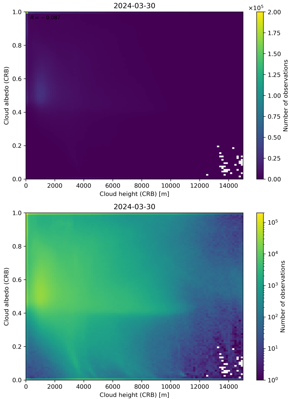
Figure 80: Scatter density plot of “Cloud height (CRB)” against “Cloud albedo (CRB)” for 2024-03-30 to 2024-03-31.
