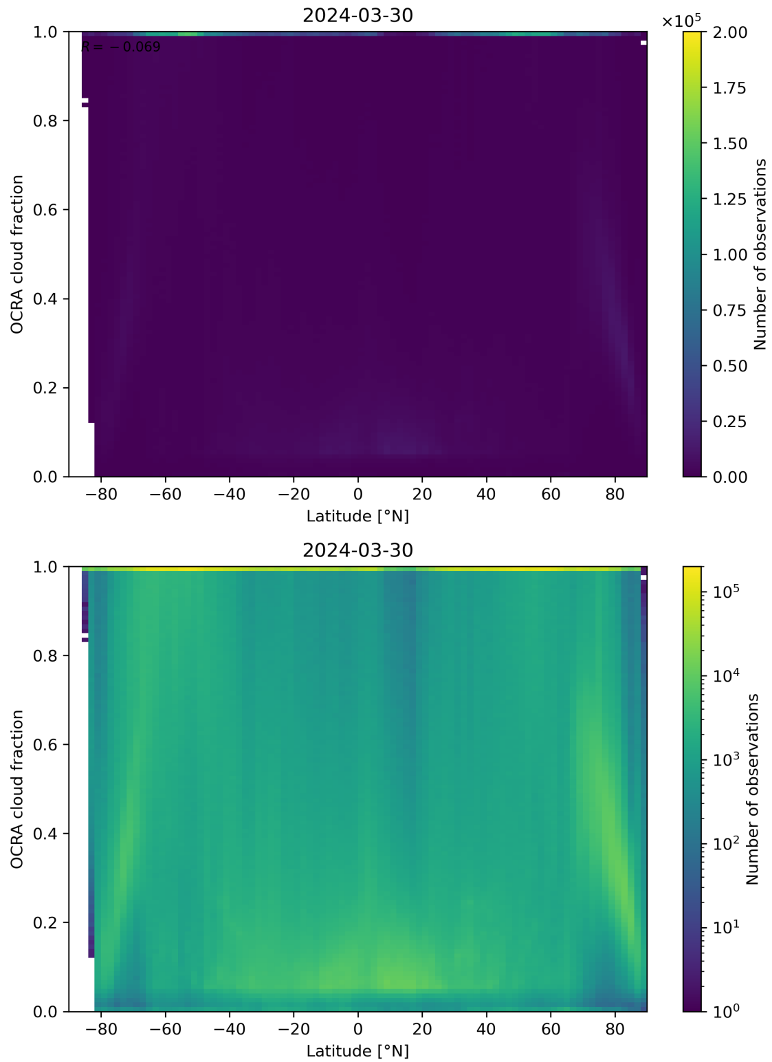
Figure 93: Scatter density plot of “Latitude” against “OCRA cloud fraction” for 2024-03-30 to 2024-03-31.
