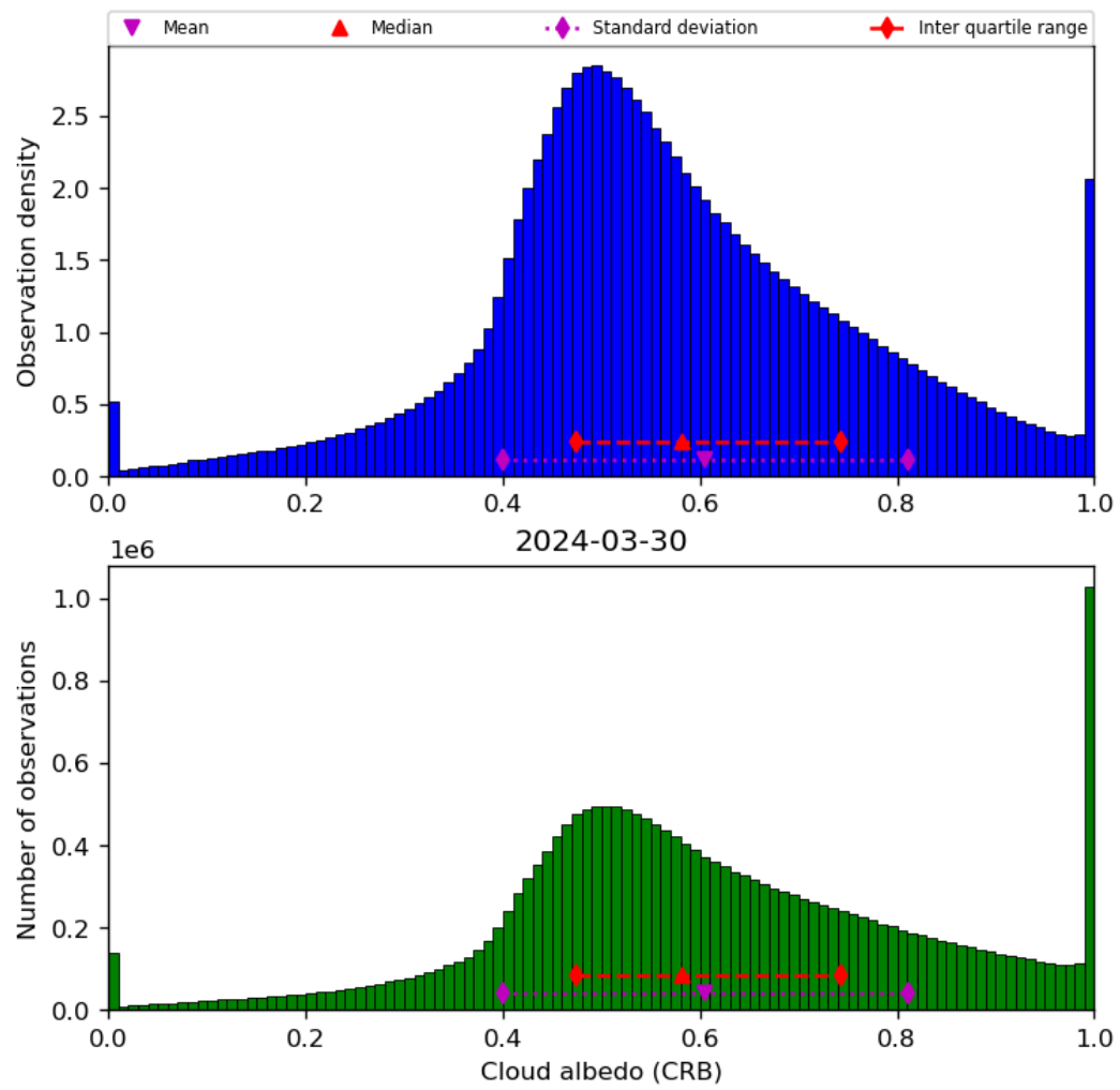
Figure 44: Histogram of “Cloud albedo (CRB)” for 2024-03-30 to 2024-03-31
