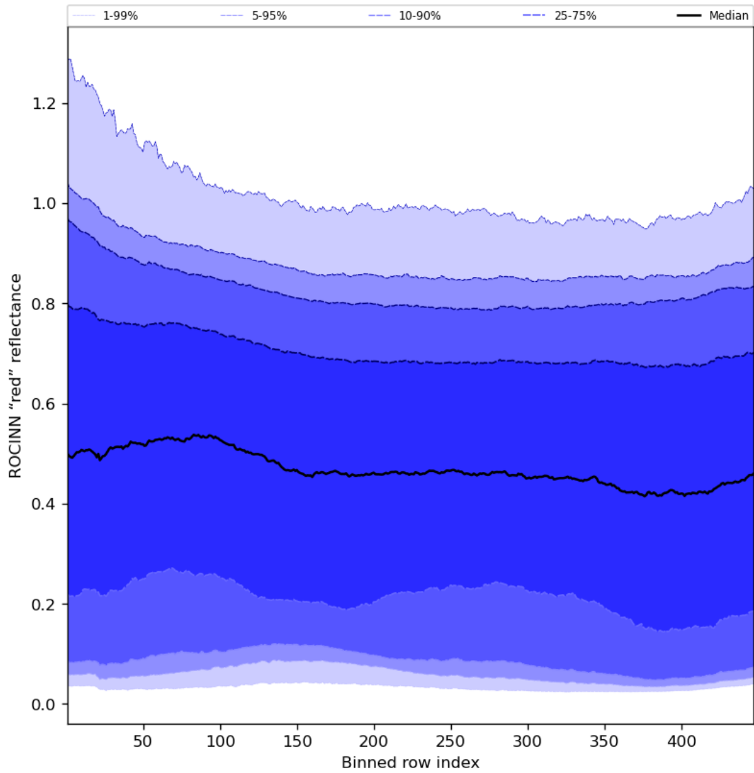
Figure 69: Along track statistics of “ROCINN “red” reflectance” for 2024-03-30 to 2024-03-31
