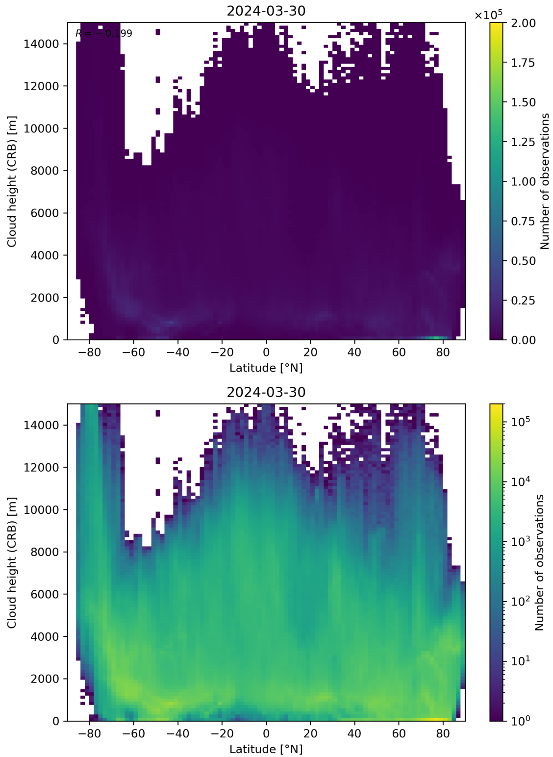
Figure 95: Scatter density plot of “Latitude” against “Cloud height (CRB)” for 2024-03-30 to 2024-03-31.
