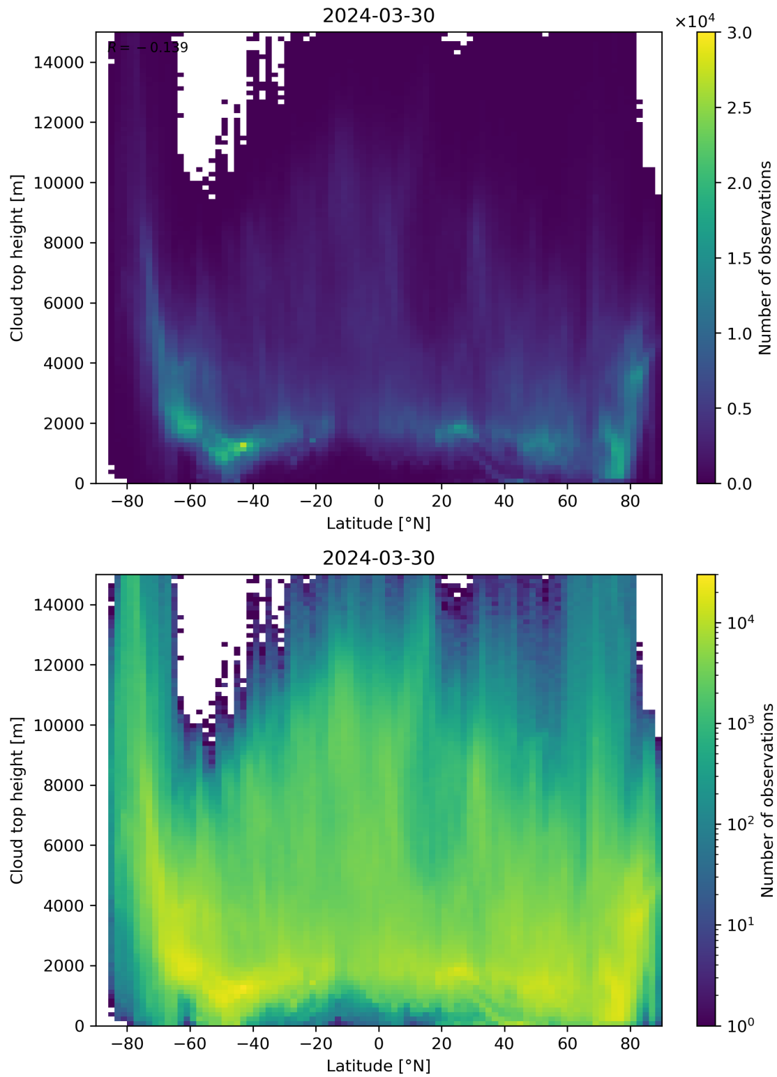
Figure 97: Scatter density plot of “Latitude” against “Cloud top height” for 2024-03-30 to 2024-03-31.
