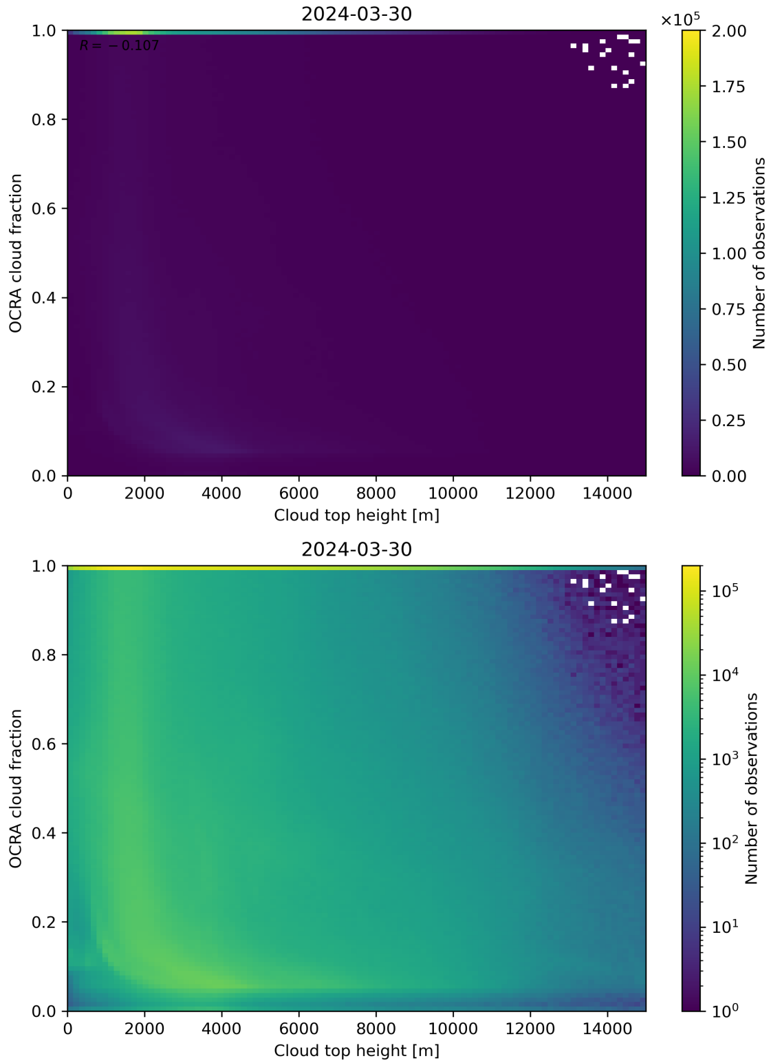
Figure 87: Scatter density plot of “Cloud top height” against “OCRA cloud fraction” for 2024-03-30 to 2024-03-31.
