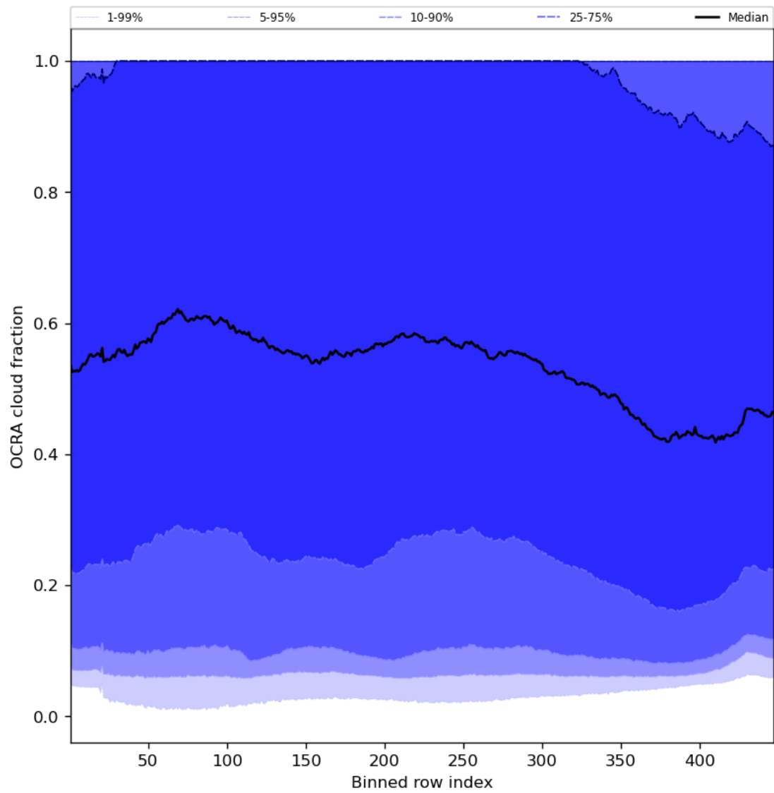
Figure 66: Along track statistics of “OCRA cloud fraction” for 2024-03-30 to 2024-03-31
