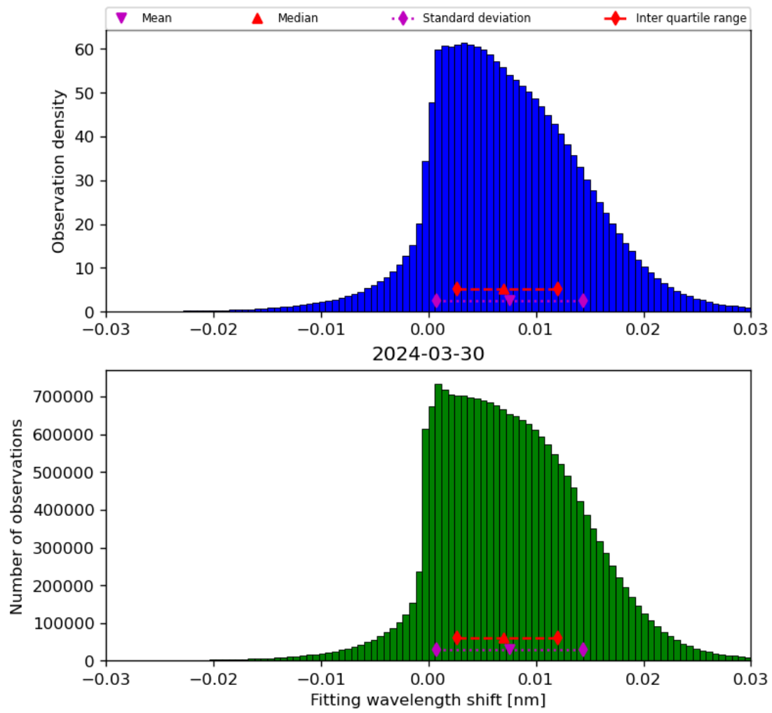
Figure 49: Histogram of “Fitting wavelength shift” for 2024-03-30 to 2024-03-31
