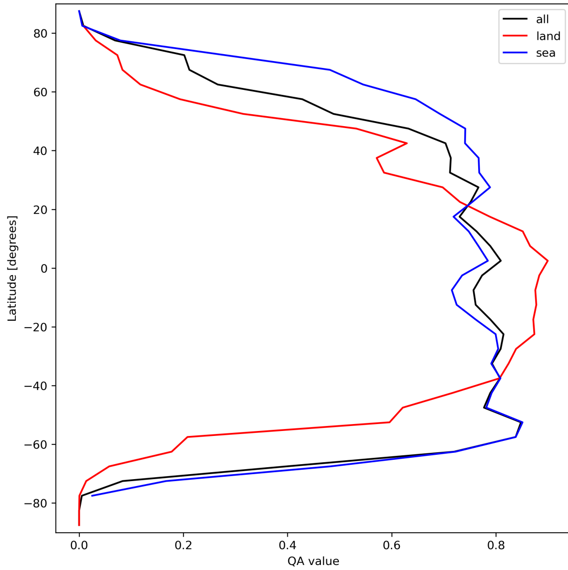
Figure 22: Zonal average of “QA value” for 2024-03-30 to 2024-03-31.
