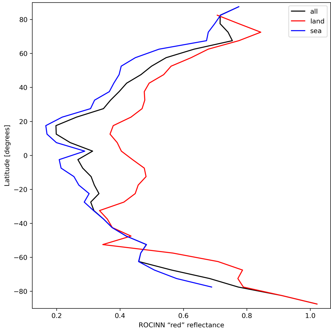
Figure 37: Zonal average of “ROCINN “red” reflectance” for 2024-03-30 to 2024-03-31.
