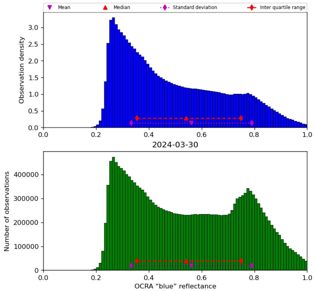
Figure 51: Histogram of “OCRA “blue” reflectance” for 2024-03-30 to 2024-03-31
