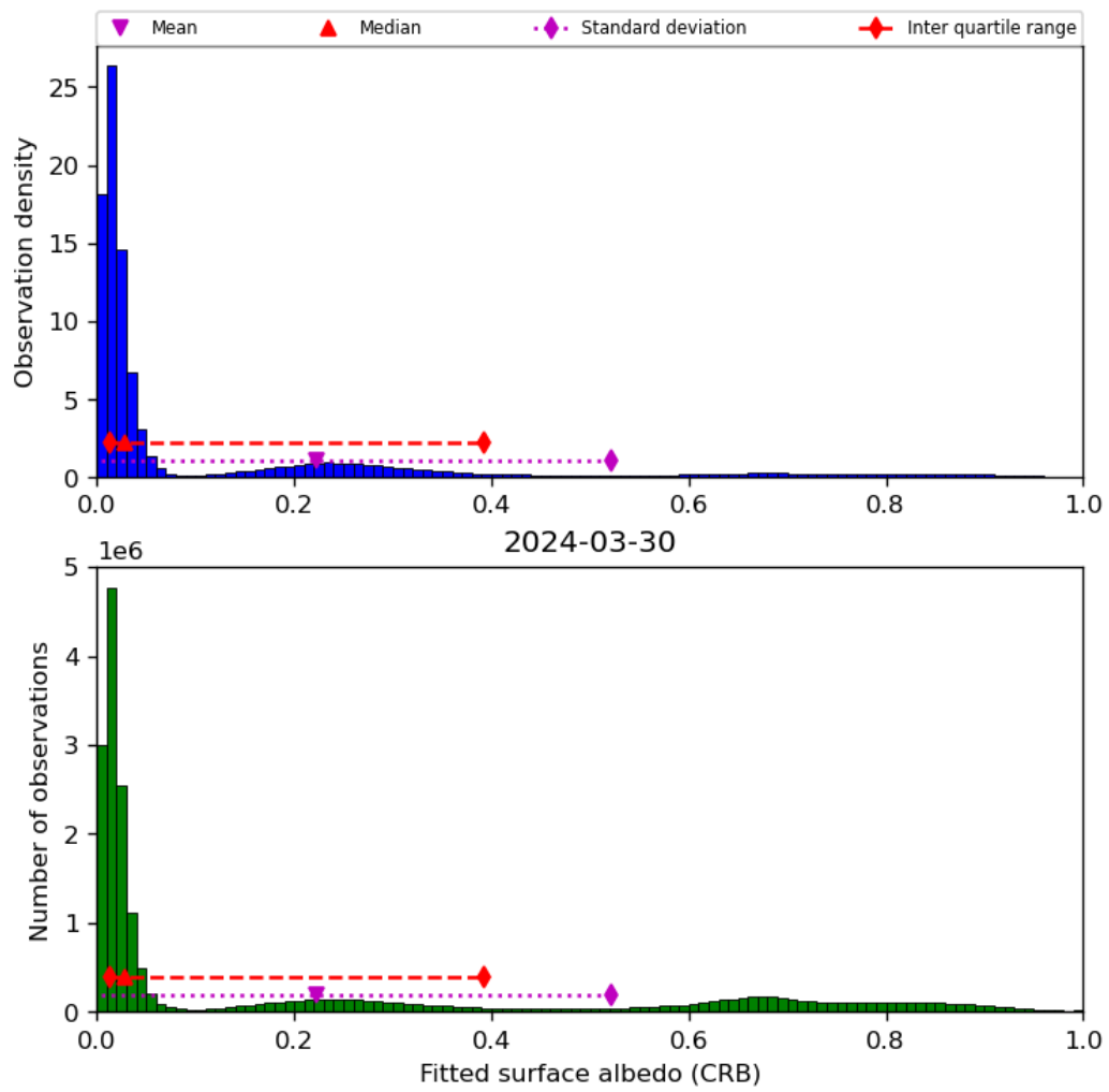
Figure 46: Histogram of “Fitted surface albedo (CRB)” for 2024-03-30 to 2024-03-31
