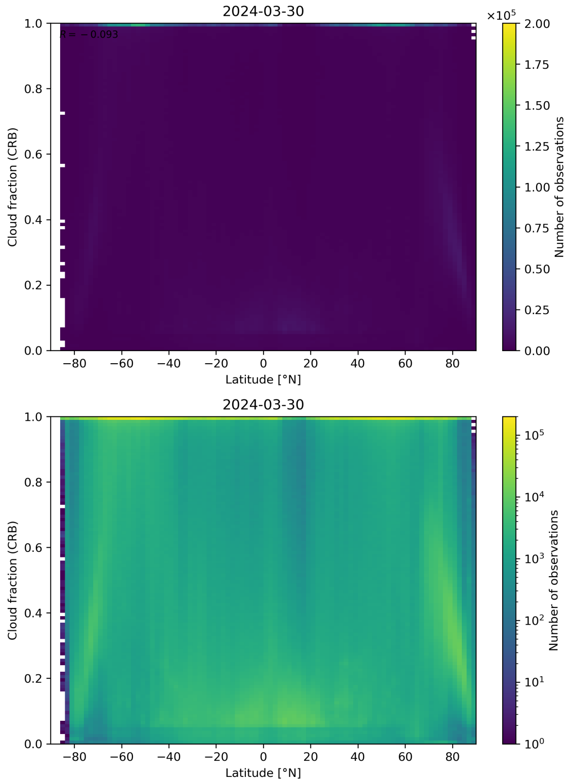
Figure 94: Scatter density plot of “Latitude” against “Cloud fraction (CRB)” for 2024-03-30 to 2024-03-31.
