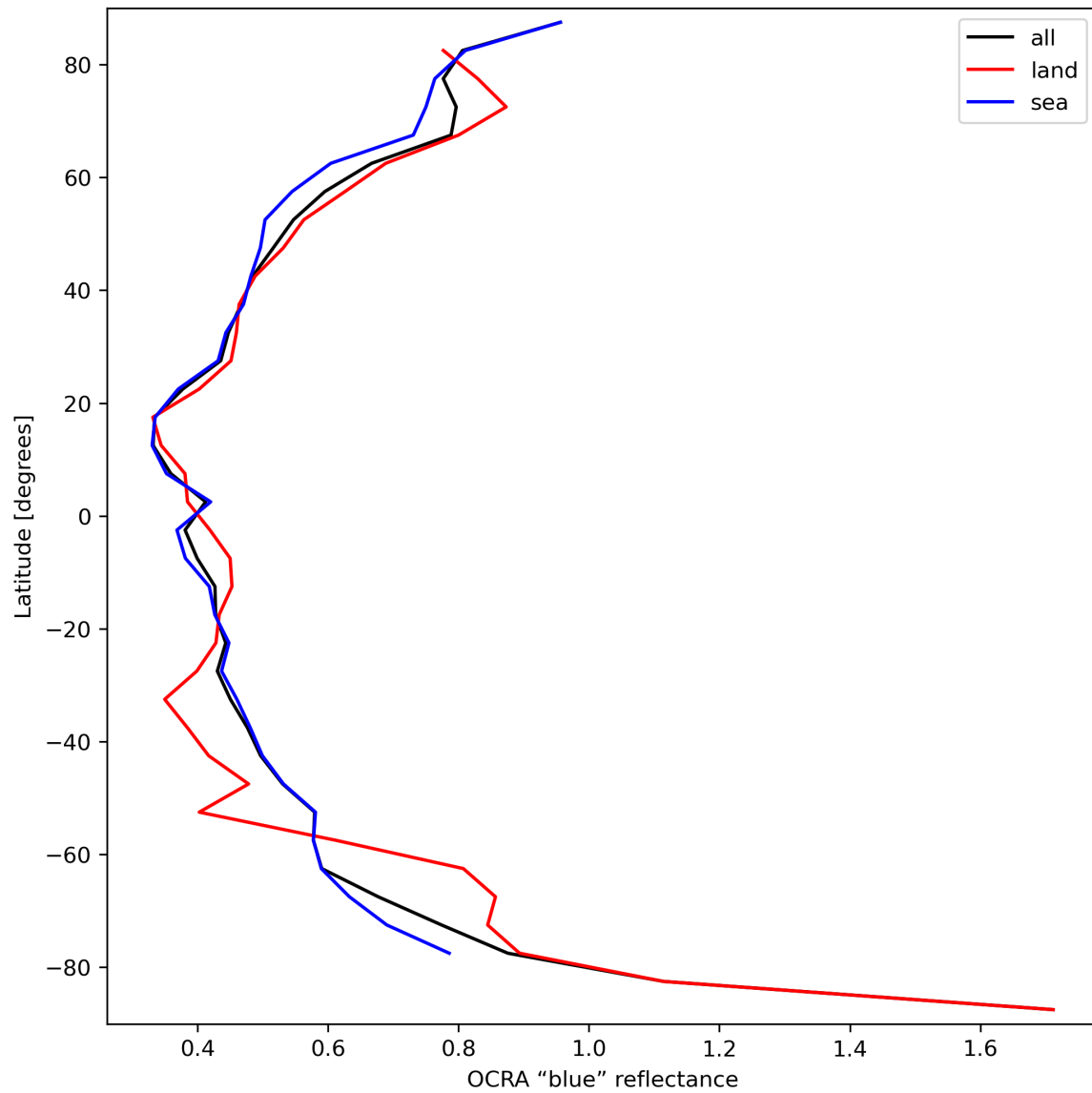
Figure 35: Zonal average of “OCRA “blue” reflectance” for 2024-03-30 to 2024-03-31.
