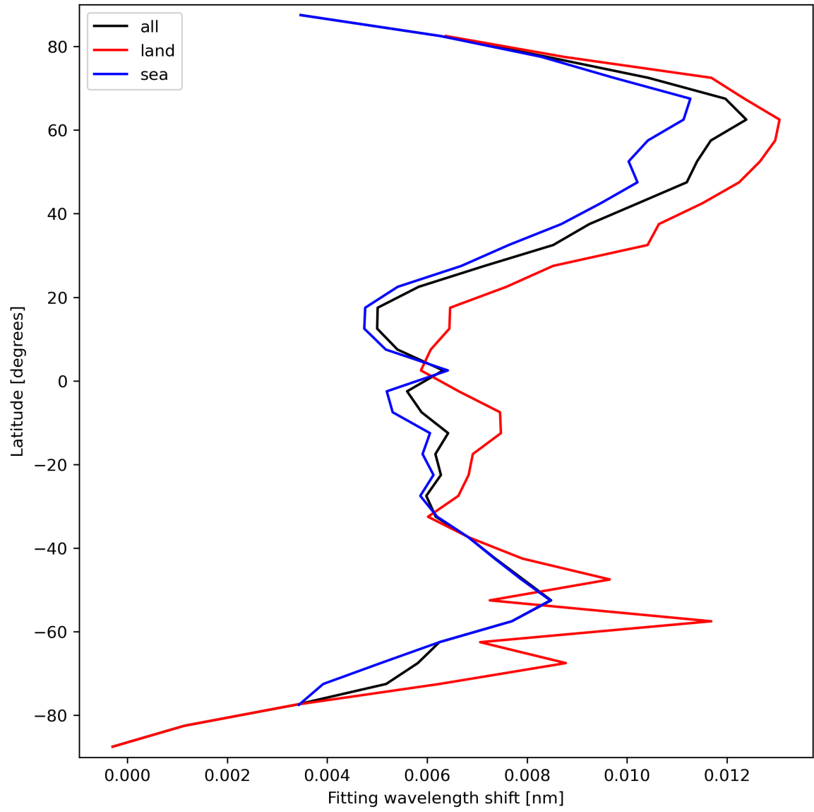
Figure 33: Zonal average of “Fitting wavelength shift” for 2024-03-30 to 2024-03-31.
