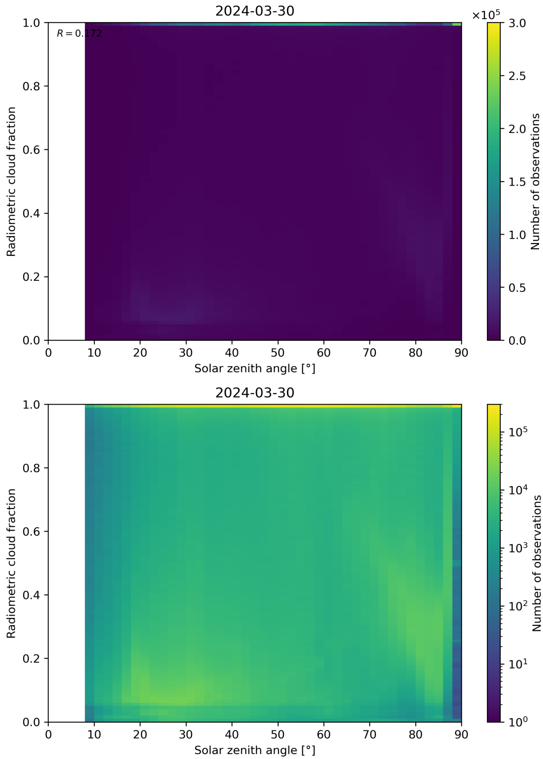
Figure 99: Scatter density plot of “Solar zenith angle” against “Radiometric cloud fraction” for 2024-03-30 to 2024-03-31.
