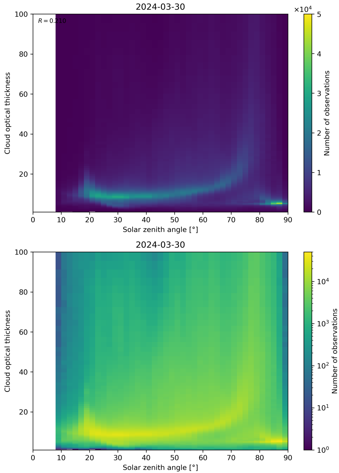
Figure 103: Scatter density plot of “Solar zenith angle” against “Cloud optical thickness” for 2024-03-30 to 2024-03-31.
