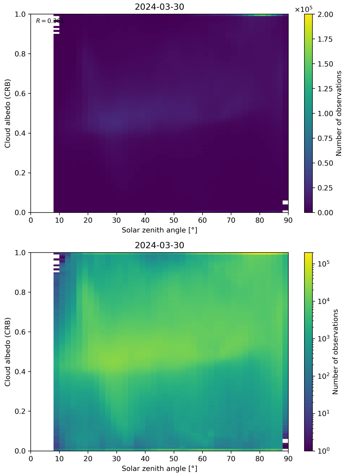
Figure 98: Scatter density plot of “Solar zenith angle” against “Cloud albedo (CRB)” for 2024-03-30 to 2024-03-31.
