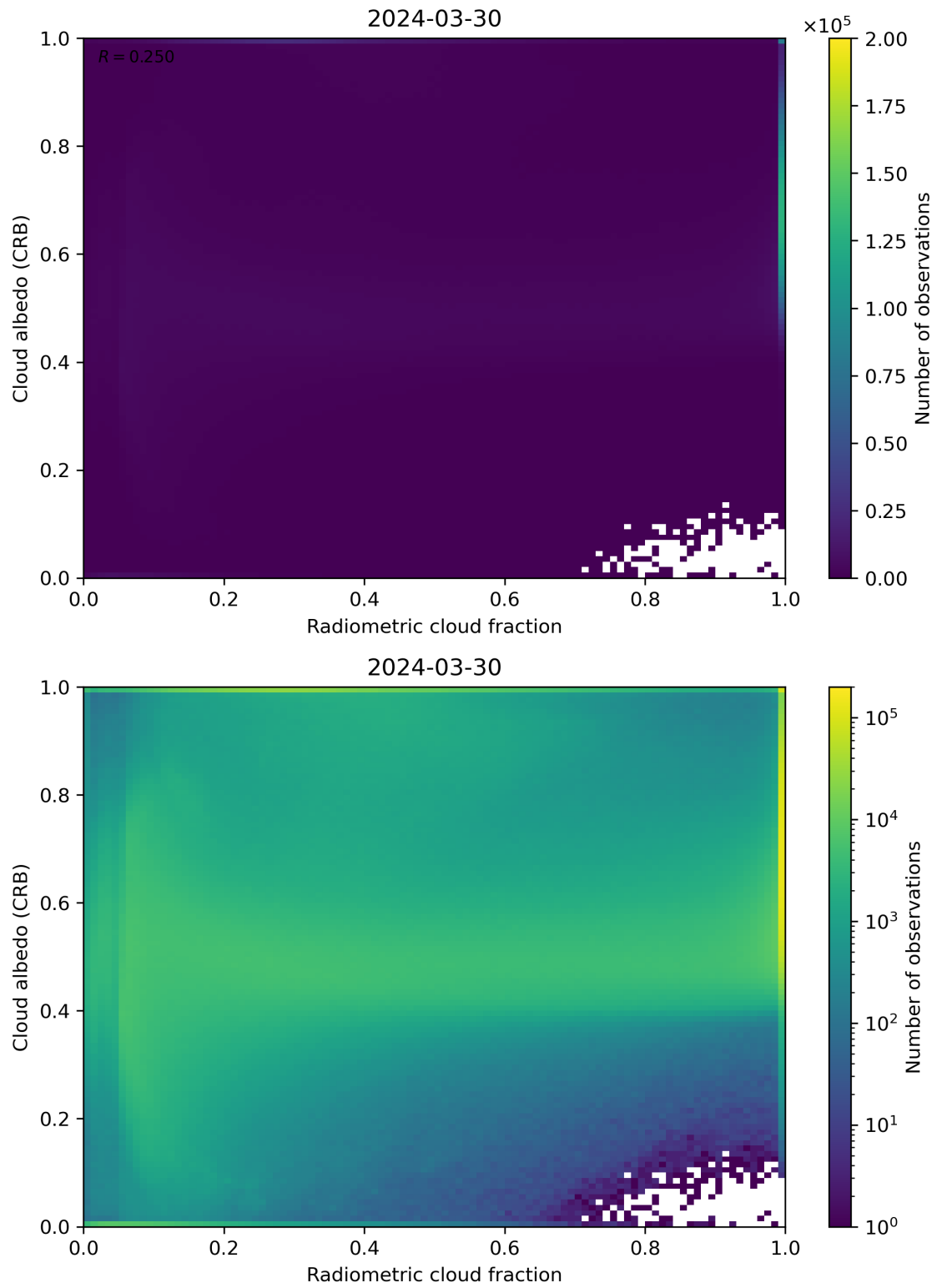
Figure 71: Scatter density plot of “Radiometric cloud fraction” against “Cloud albedo (CRB)” for 2024-03-30 to 2024-03-31.
