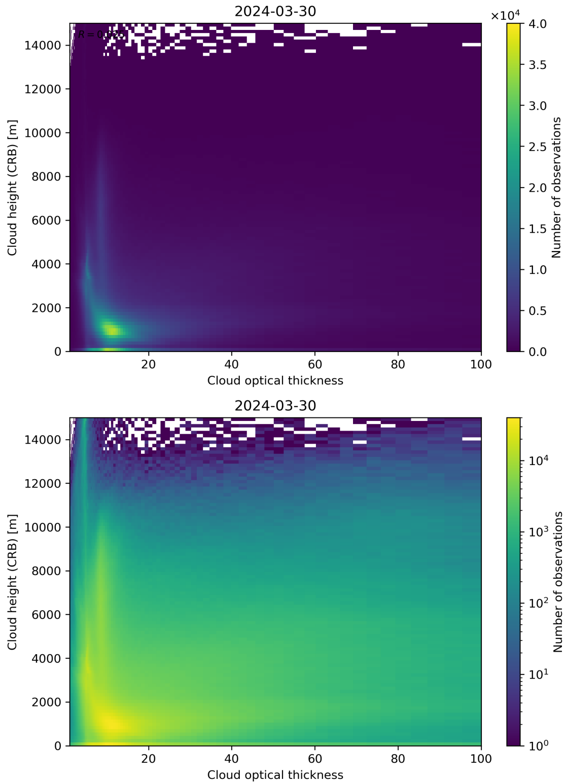
Figure 85: Scatter density plot of “Cloud optical thickness” against “Cloud height (CRB)” for 2024-03-30 to 2024-03-31.
