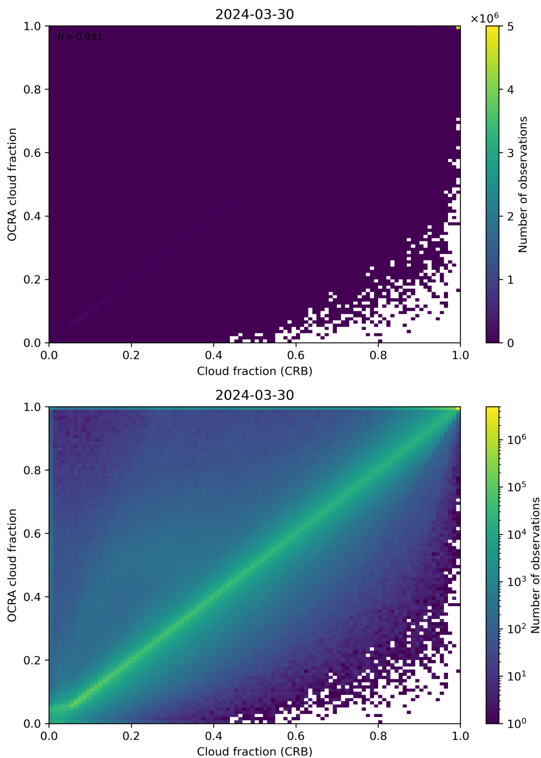
Figure 78: Scatter density plot of “Cloud fraction (CRB)” against “OCRA cloud fraction” for 2024-03-30 to 2024-03-31.
