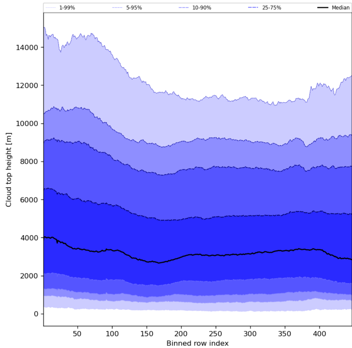
Figure 56: Along track statistics of “Cloud top height” for 2024-03-30 to 2024-03-31
