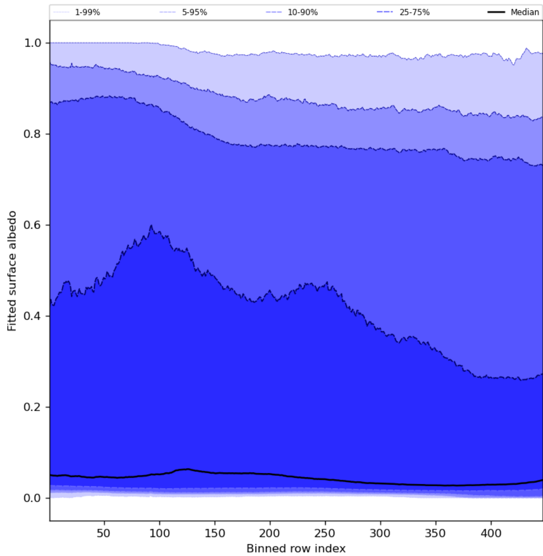
Figure 61: Along track statistics of “Fitted surface albedo” for 2024-03-30 to 2024-03-31
