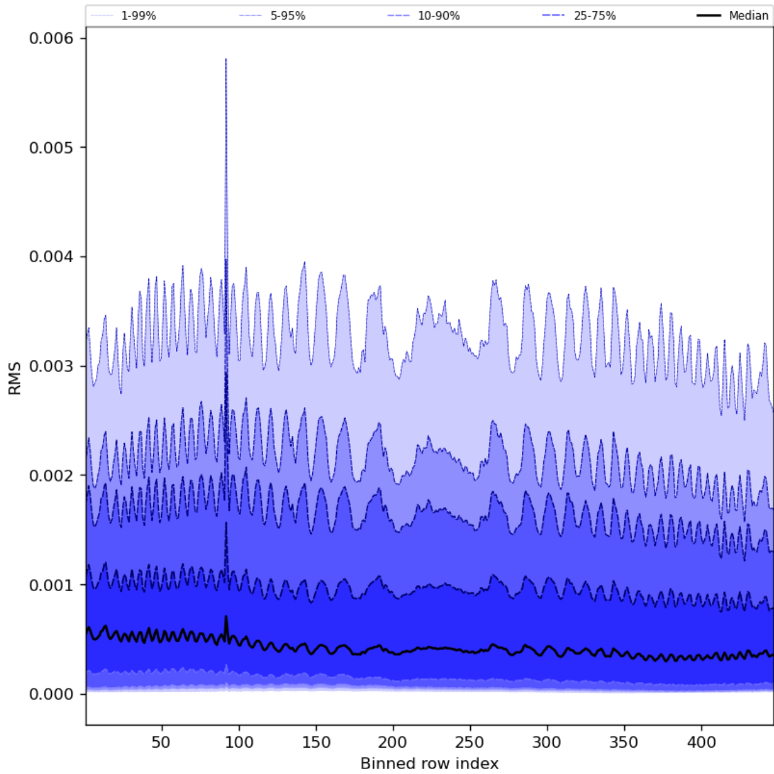
Figure 63: Along track statistics of “RMS” for 2024-03-30 to 2024-03-31
