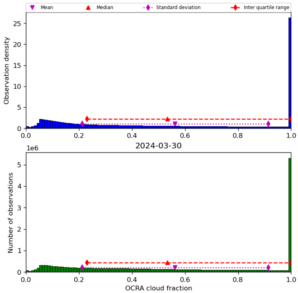
Figure 50: Histogram of “OCRA cloud fraction” for 2024-03-30 to 2024-03-31
