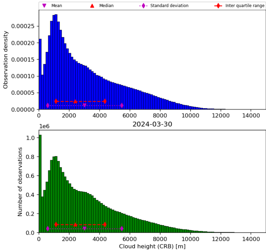
Figure 43: Histogram of “Cloud height (CRB)” for 2024-03-30 to 2024-03-31
