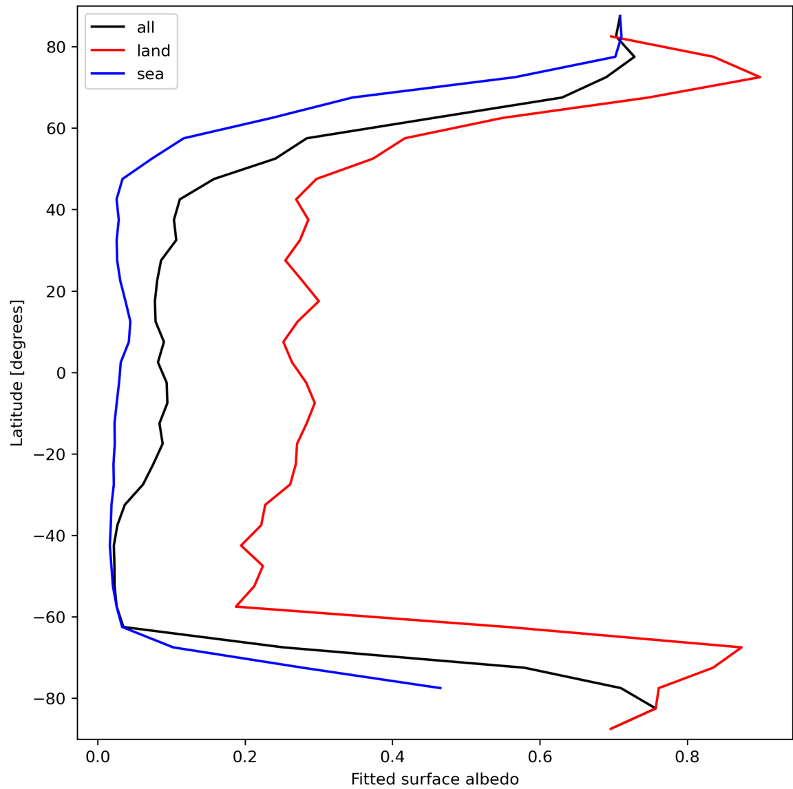
Figure 29: Zonal average of “Fitted surface albedo” for 2024-03-30 to 2024-03-31.
