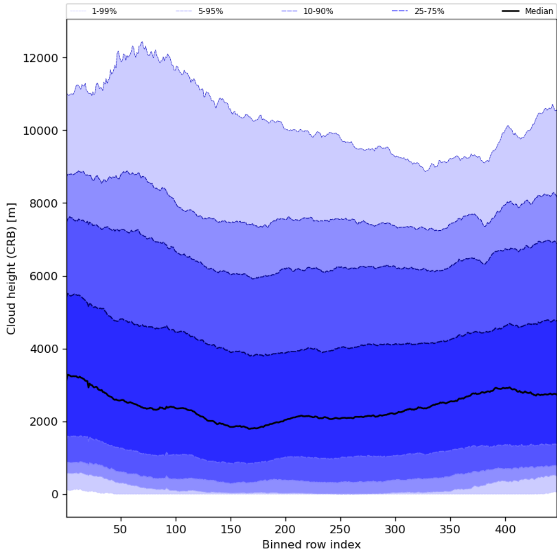
Figure 59: Along track statistics of “Cloud height (CRB)” for 2024-03-30 to 2024-03-31
