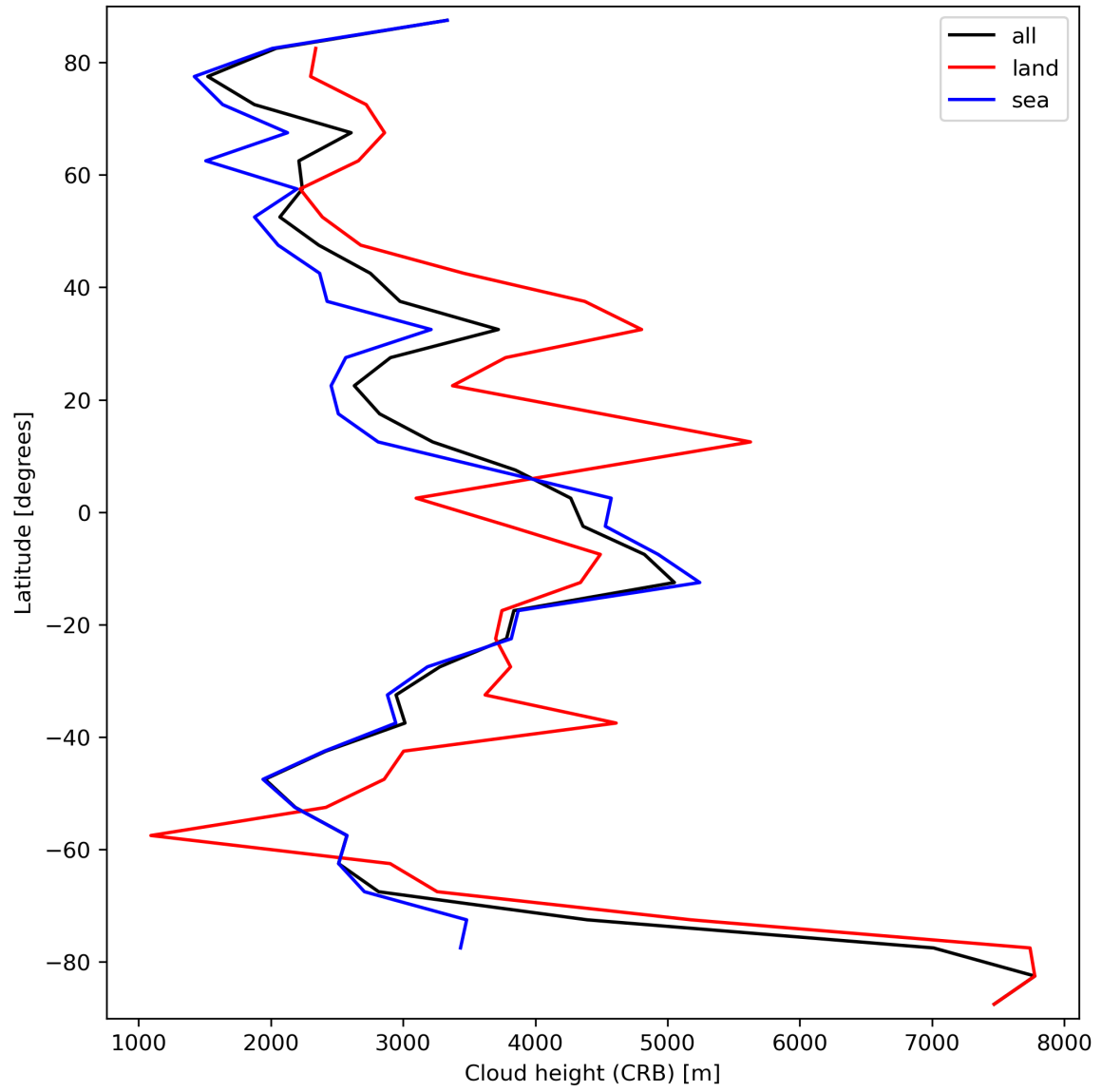
Figure 27: Zonal average of “Cloud height (CRB)” for 2024-03-30 to 2024-03-31.
