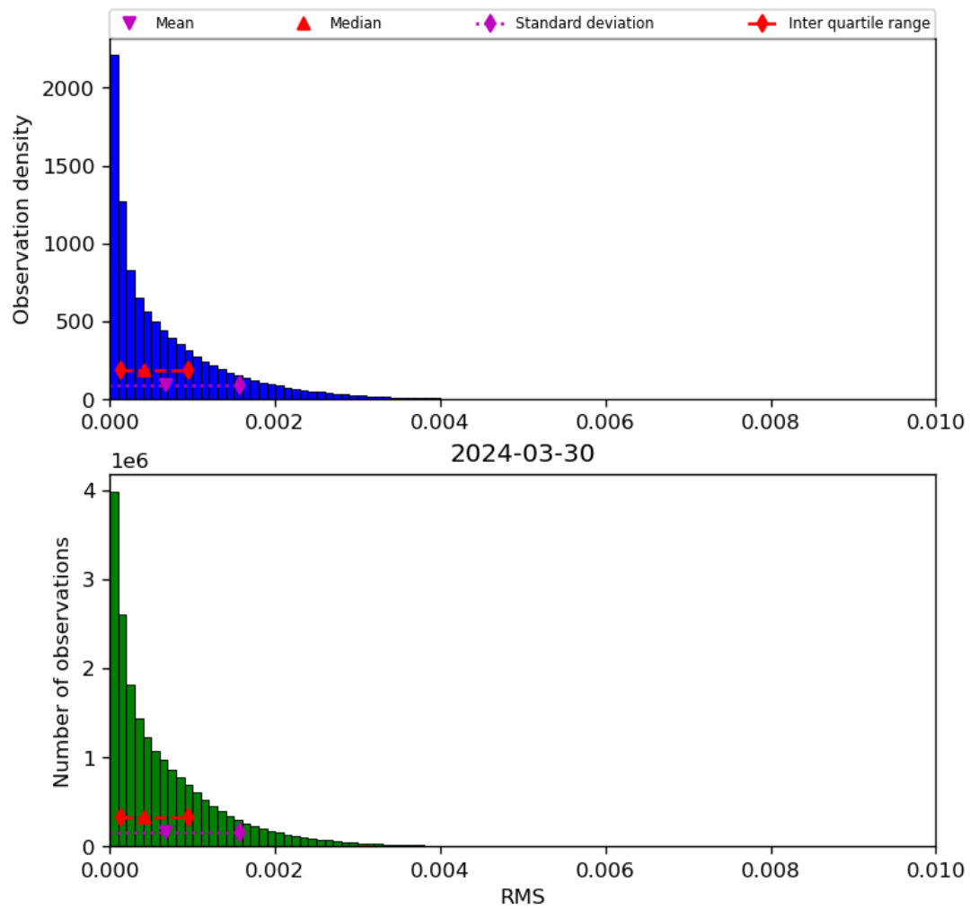
Figure 47: Histogram of “RMS” for 2024-03-30 to 2024-03-31
