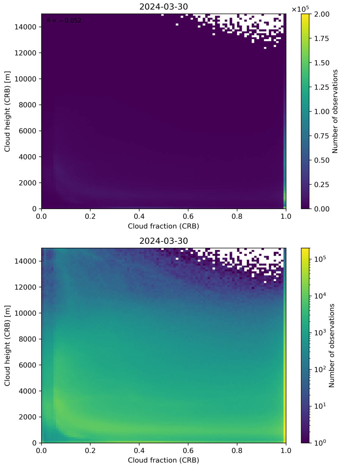
Figure 79: Scatter density plot of “Cloud fraction (CRB)” against “Cloud height (CRB)” for 2024-03-30 to 2024-03-31.
