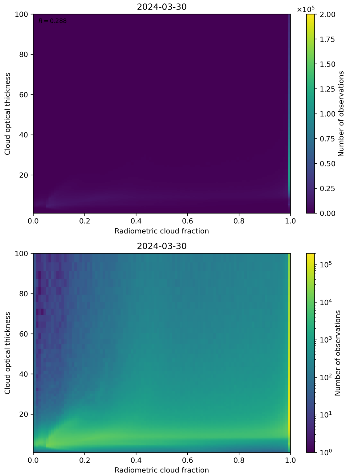
Figure 75: Scatter density plot of “Radiometric cloud fraction” against “Cloud optical thickness” for 2024-03-30 to 2024-03-31.
