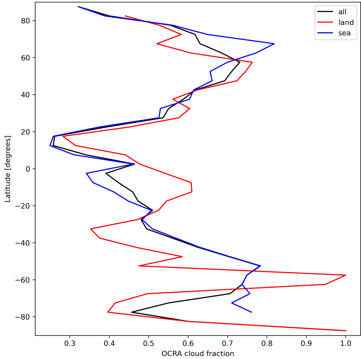
Figure 34: Zonal average of “OCRA cloud fraction” for 2024-03-30 to 2024-03-31.
