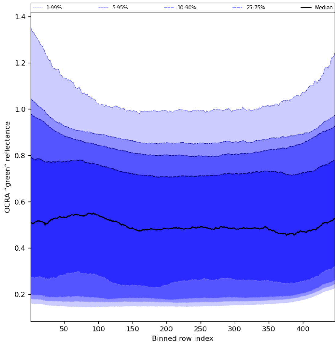
Figure 68: Along track statistics of "OCRA "green" reflectance" for 2024-03-30 to 2024-03-31
