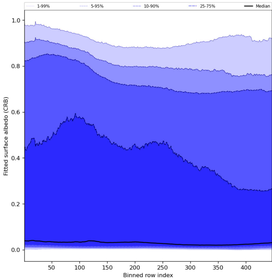
Figure 62: Along track statistics of “Fitted surface albedo (CRB)” for 2024-03-30 to 2024-03-31
