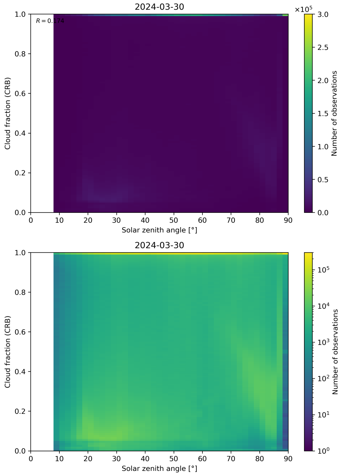
Figure 101: Scatter density plot of “Solar zenith angle” against “Cloud fraction (CRB)” for 2024-03-30 to 2024-03-31.
