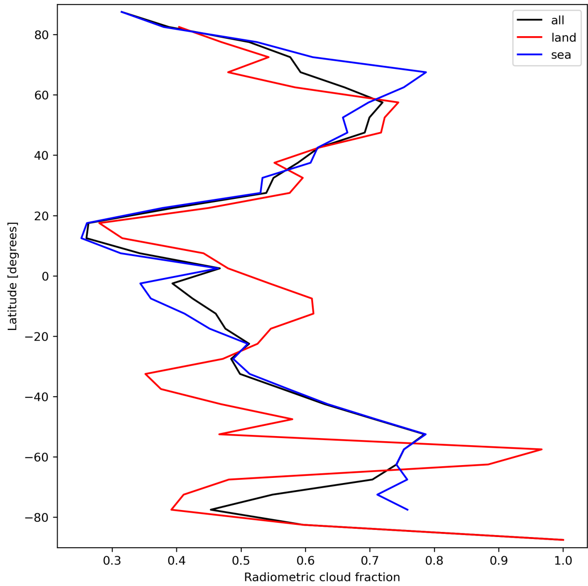
Figure 23: Zonal average of “Radiometric cloud fraction” for 2024-03-30 to 2024-03-31.
