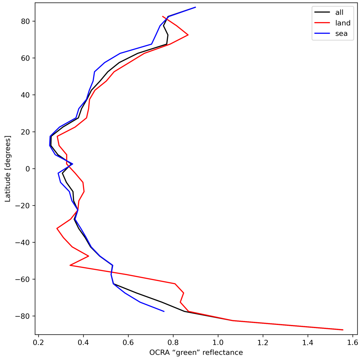
Figure 36: Zonal average of “OCRA “green” reflectance” for 2024-03-30 to 2024-03-31.
