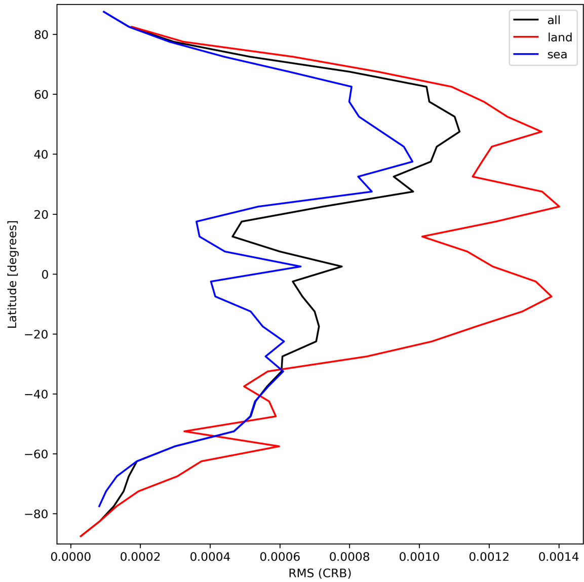
Figure 32: Zonal average of “RMS (CRB)” for 2024-03-30 to 2024-03-31.
