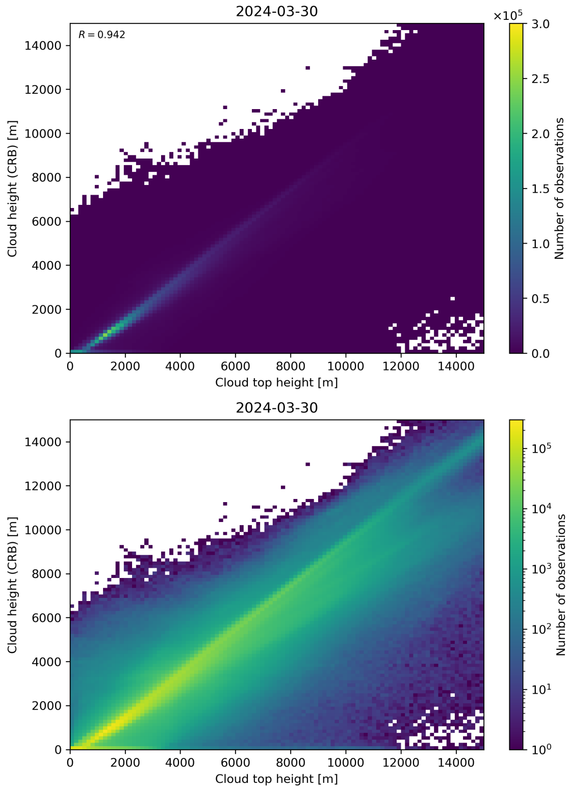
Figure 89: Scatter density plot of “Cloud top height” against “Cloud height (CRB)” for 2024-03-30 to 2024-03-31.
