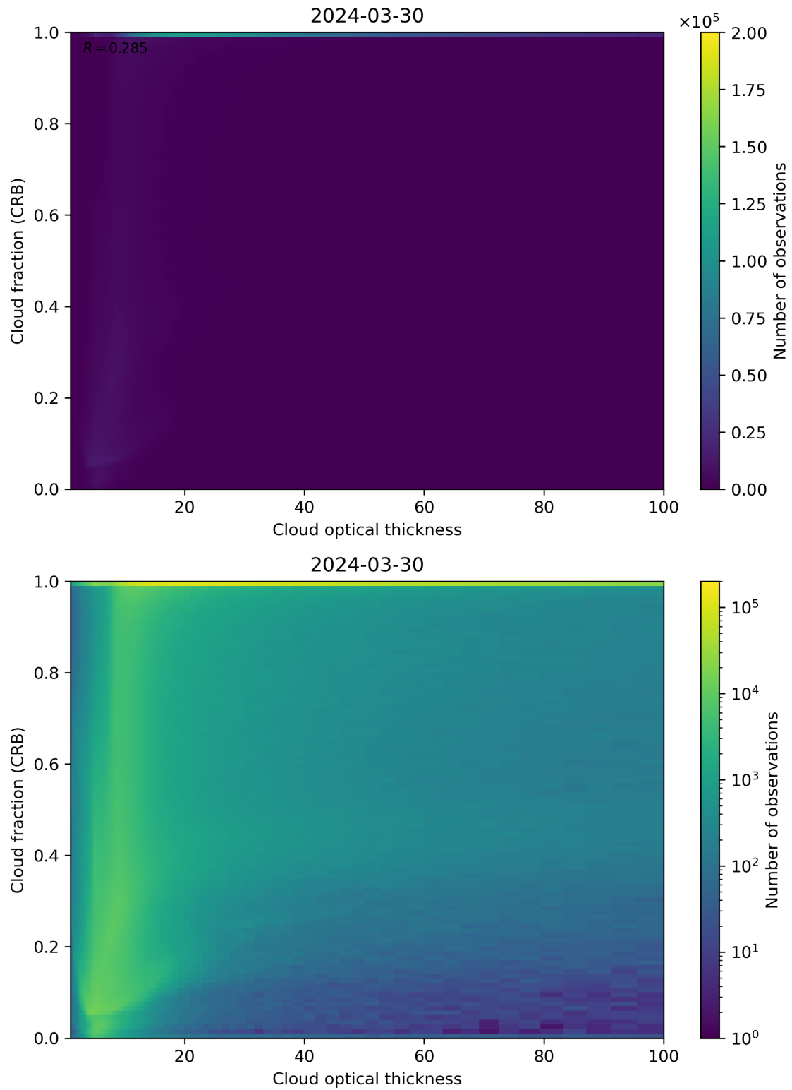
Figure 84: Scatter density plot of “Cloud optical thickness” against “Cloud fraction (CRB)” for 2024-03-30 to 2024-03-31.
