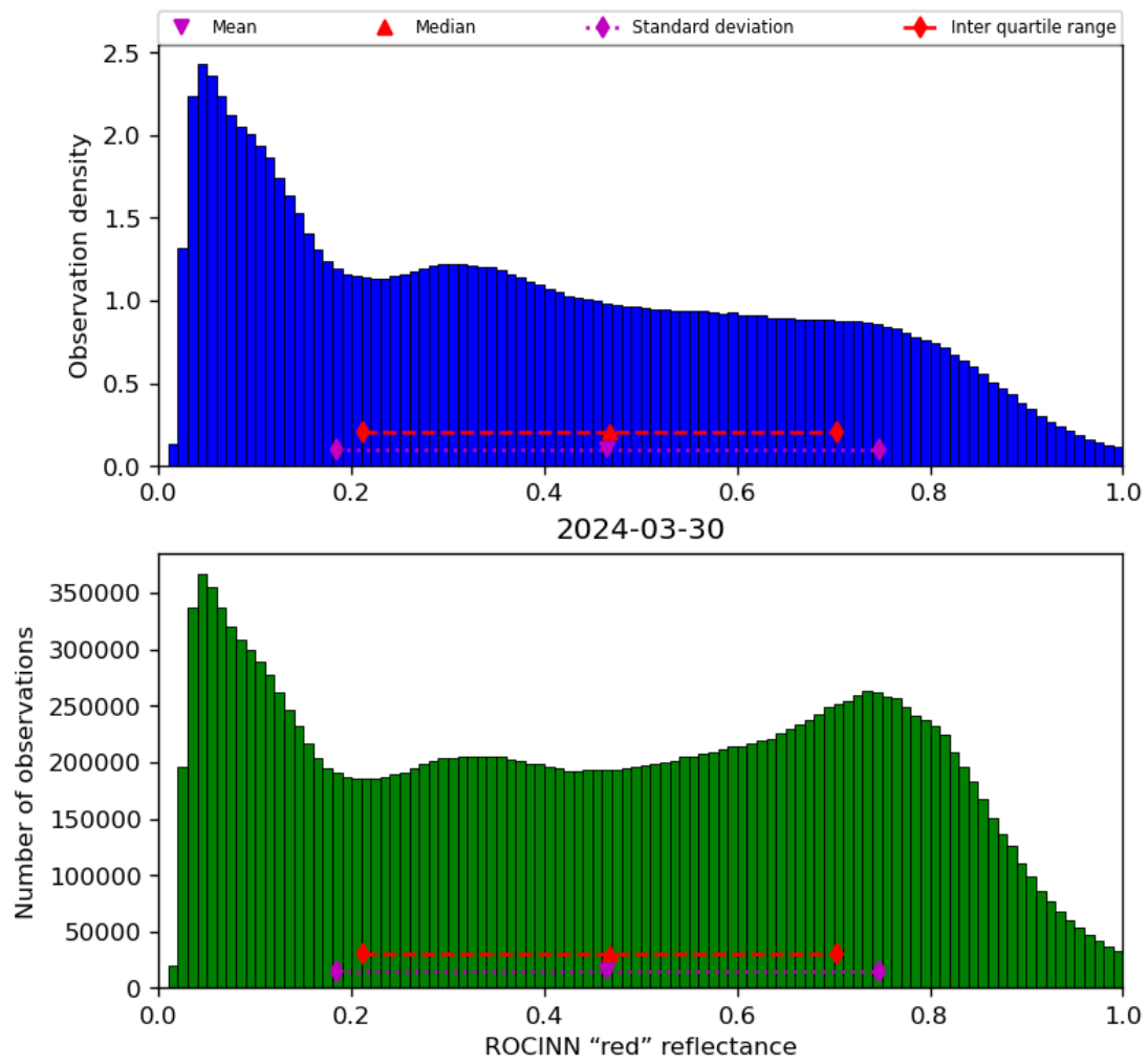
Figure 53: Histogram of “ROCINN “red” reflectance” for 2024-03-30 to 2024-03-31
