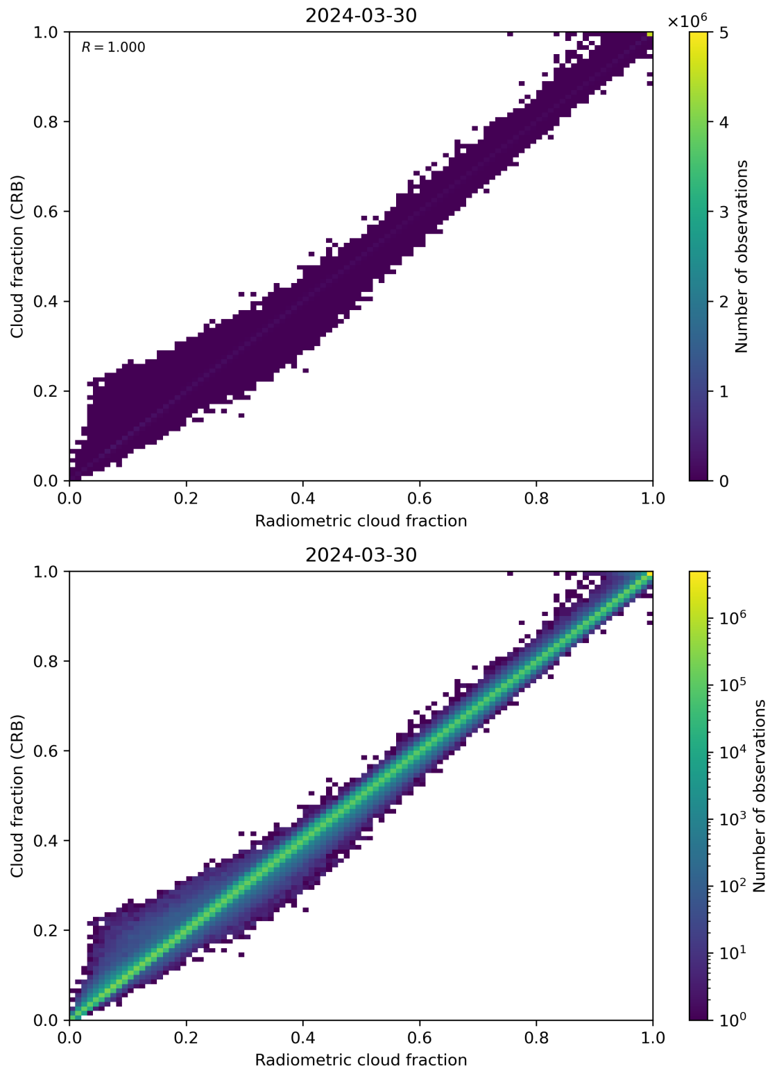
Figure 73: Scatter density plot of “Radiometric cloud fraction” against “Cloud fraction (CRB)” for 2024-03-30 to 2024-03-31.
