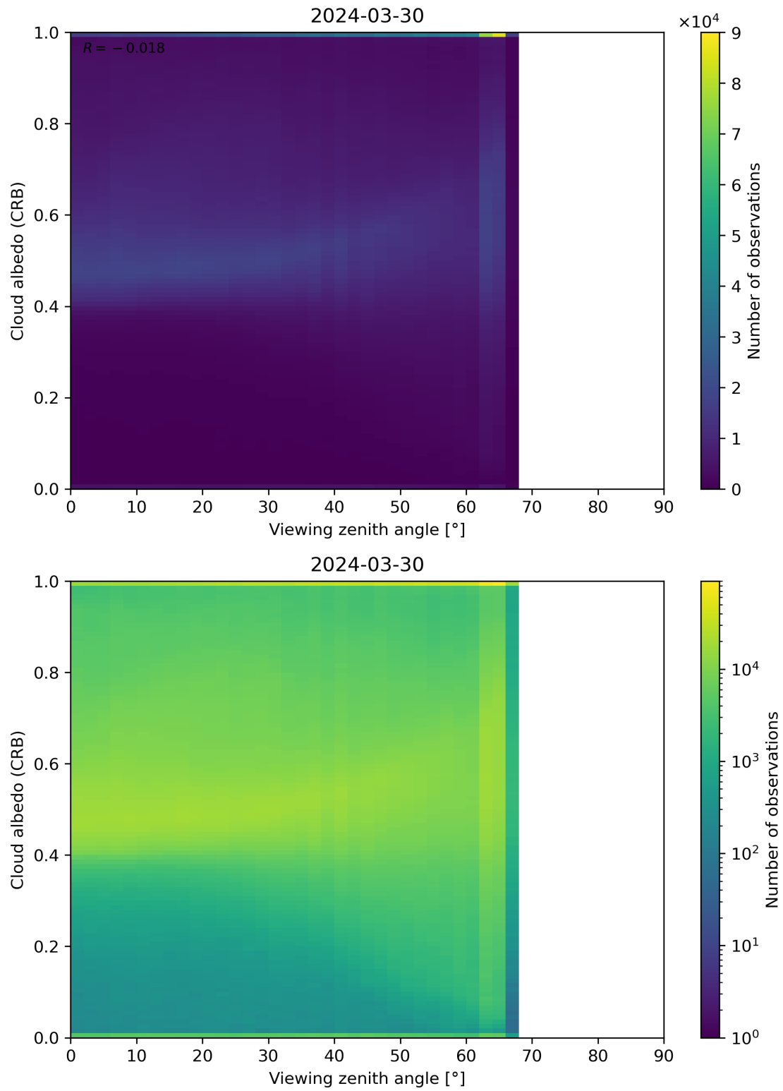
Figure 106: Scatter density plot of “Viewing zenith angle” against “Cloud albedo (CRB)” for 2024-03-30 to 2024-03-31.
