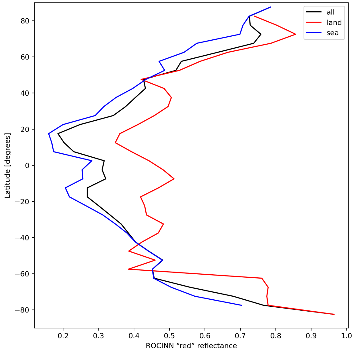
Figure 37: Zonal average of “ROCINN “red” reflectance” for 2024-03-31 to 2024-04-02.
