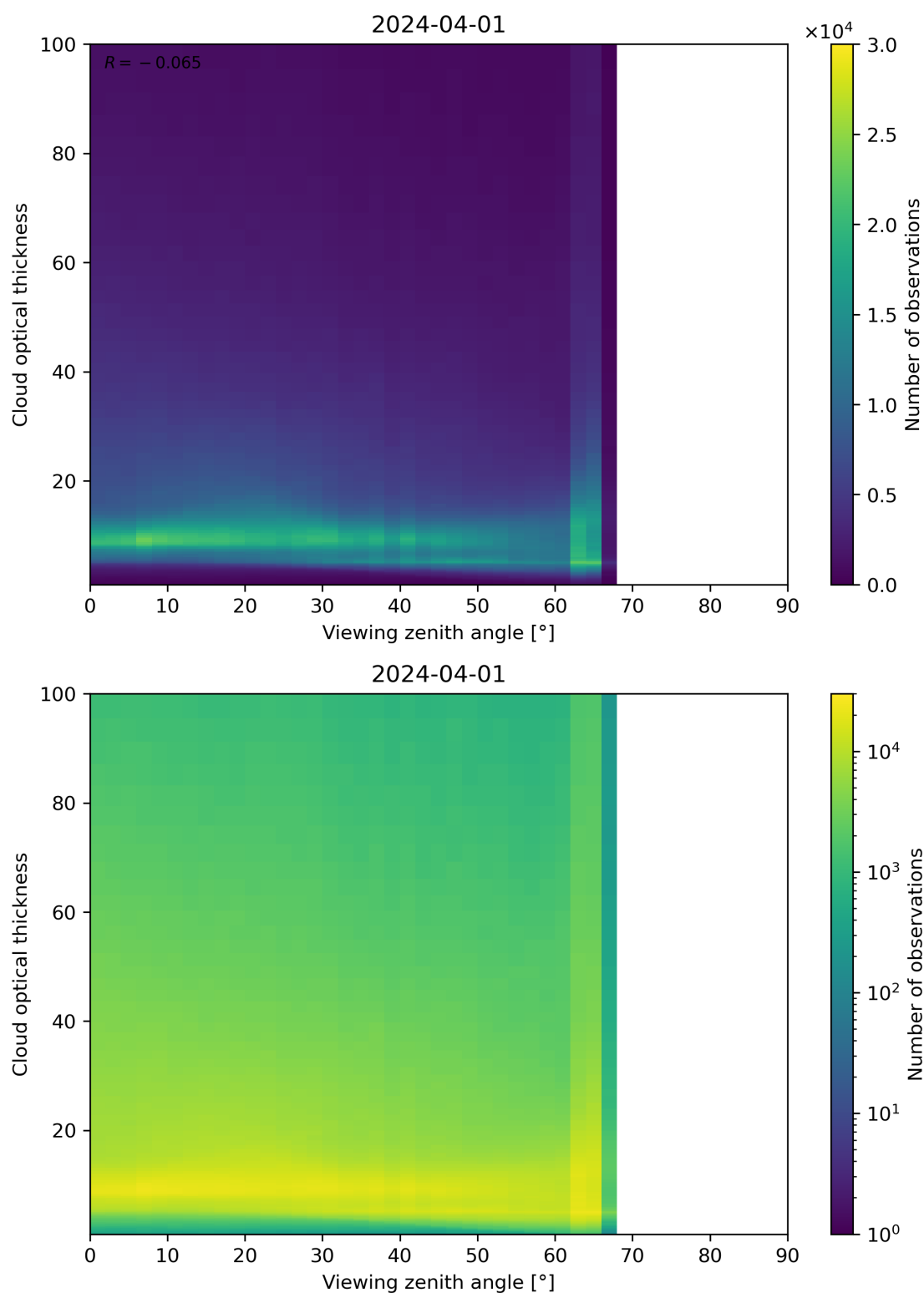
Figure 111: Scatter density plot of “Viewing zenith angle” against “Cloud optical thickness” for 2024-03-31 to 2024-04-02.
