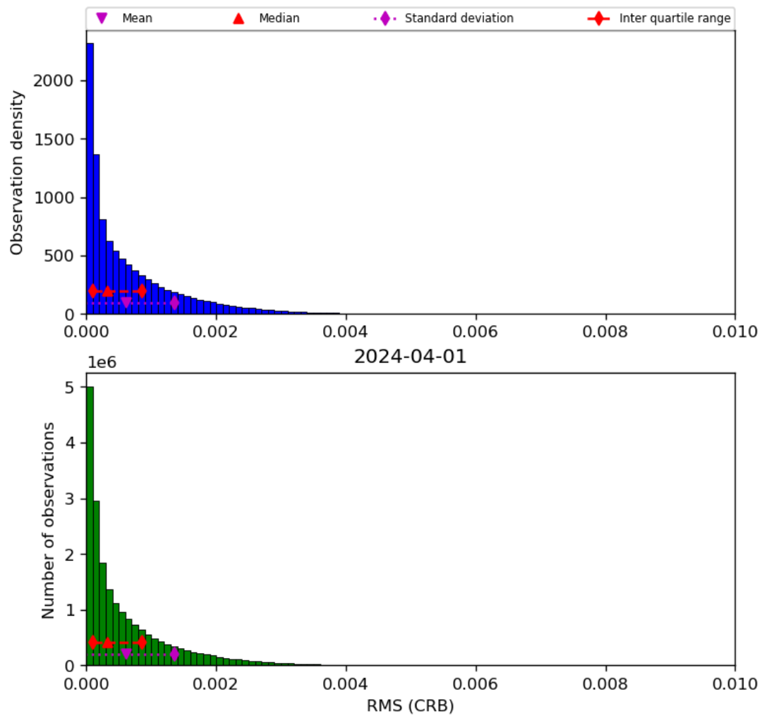
Figure 48: Histogram of “RMS (CRB)” for 2024-03-31 to 2024-04-02
