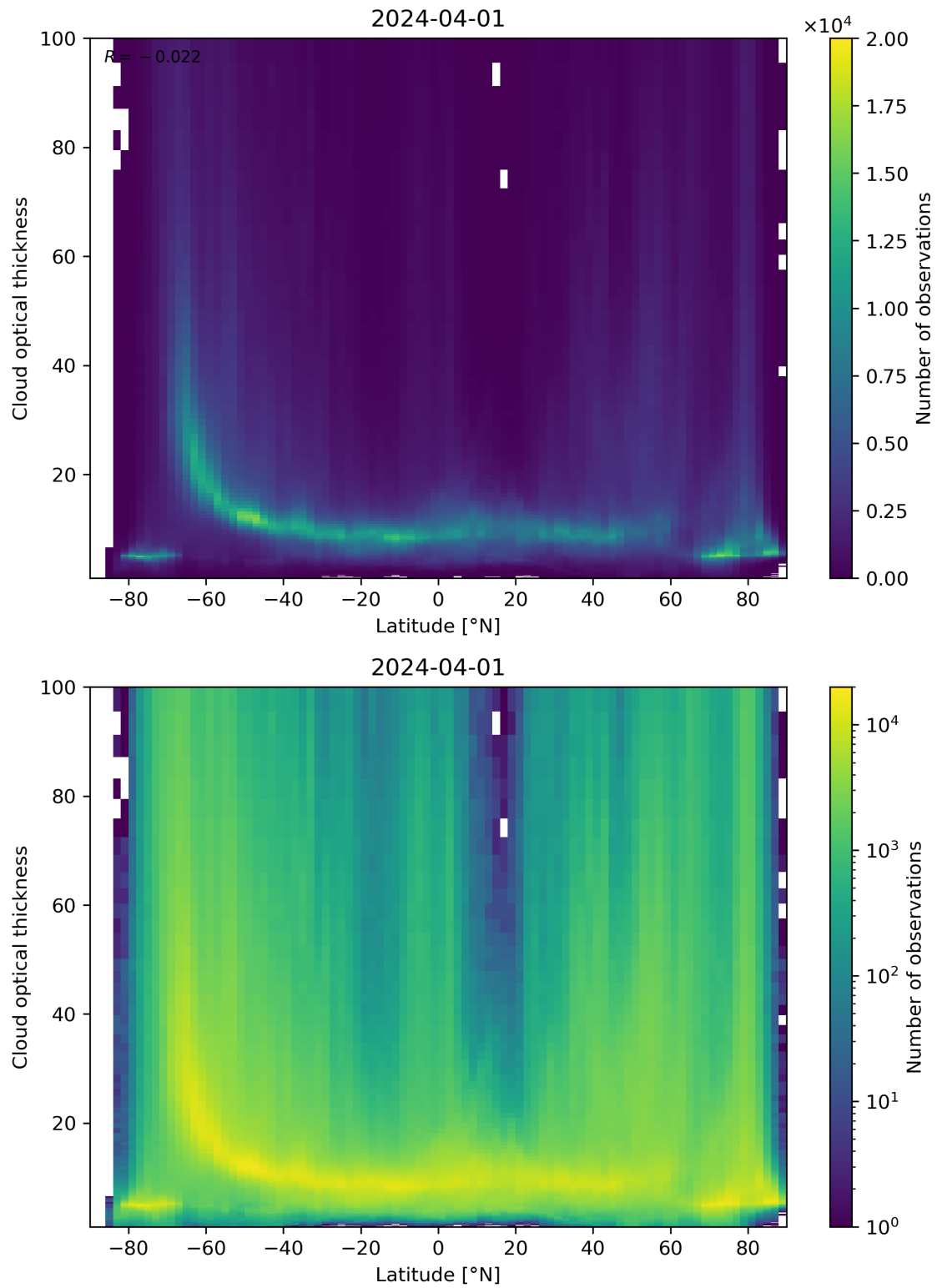
Figure 96: Scatter density plot of “Latitude” against “Cloud optical thickness” for 2024-03-31 to 2024-04-02.
