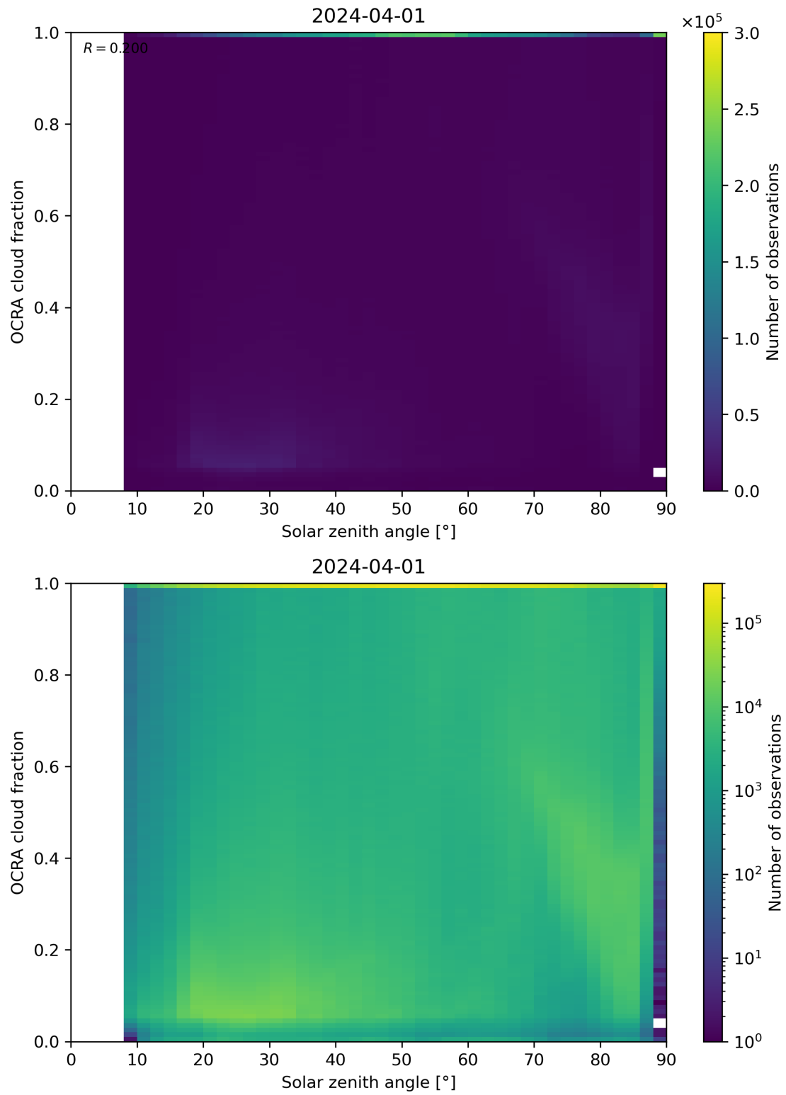
Figure 100: Scatter density plot of “Solar zenith angle” against “OCRA cloud fraction” for 2024-03-31 to 2024-04-02.
