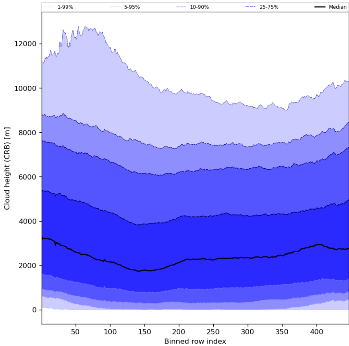
Figure 59: Along track statistics of “Cloud height (CRB)” for 2024-03-31 to 2024-04-02
