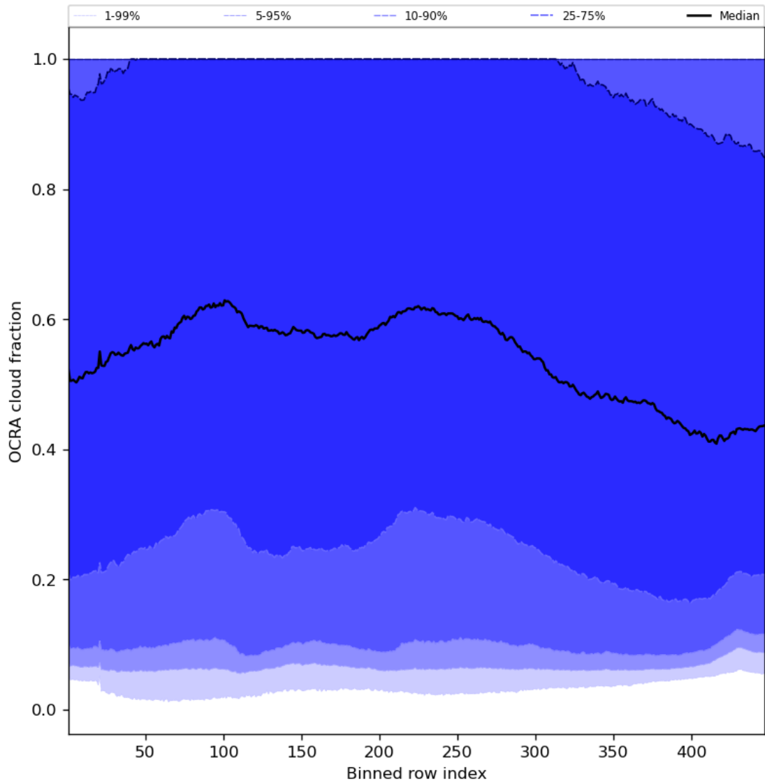
Figure 66: Along track statistics of “OCRA cloud fraction” for 2024-03-31 to 2024-04-02
