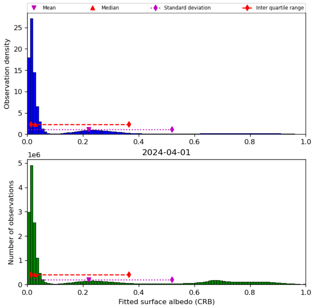
Figure 46: Histogram of “Fitted surface albedo (CRB)” for 2024-03-31 to 2024-04-02
