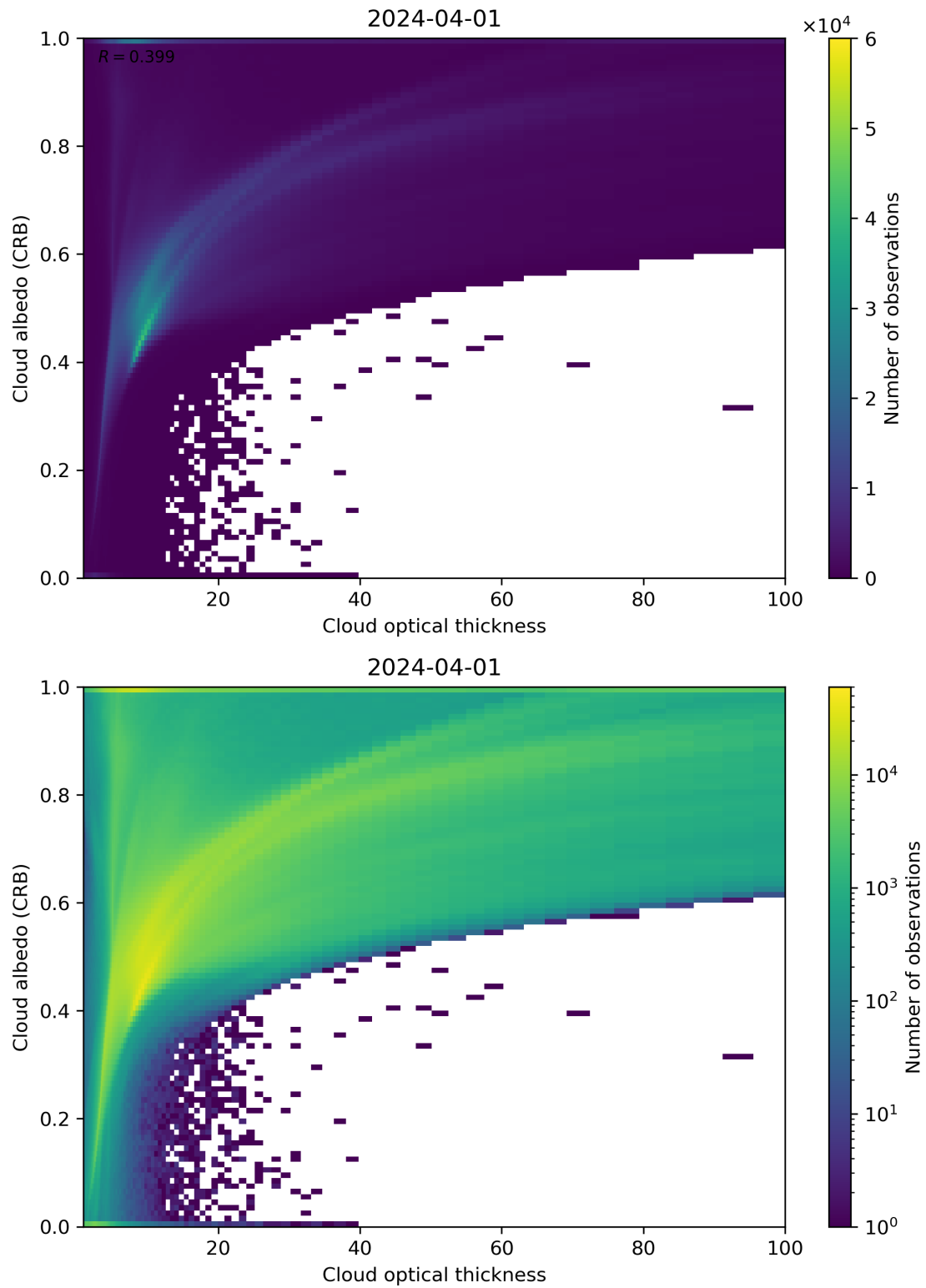
Figure 82: Scatter density plot of “Cloud optical thickness” against “Cloud albedo (CRB)” for 2024-03-31 to 2024-04-02.
