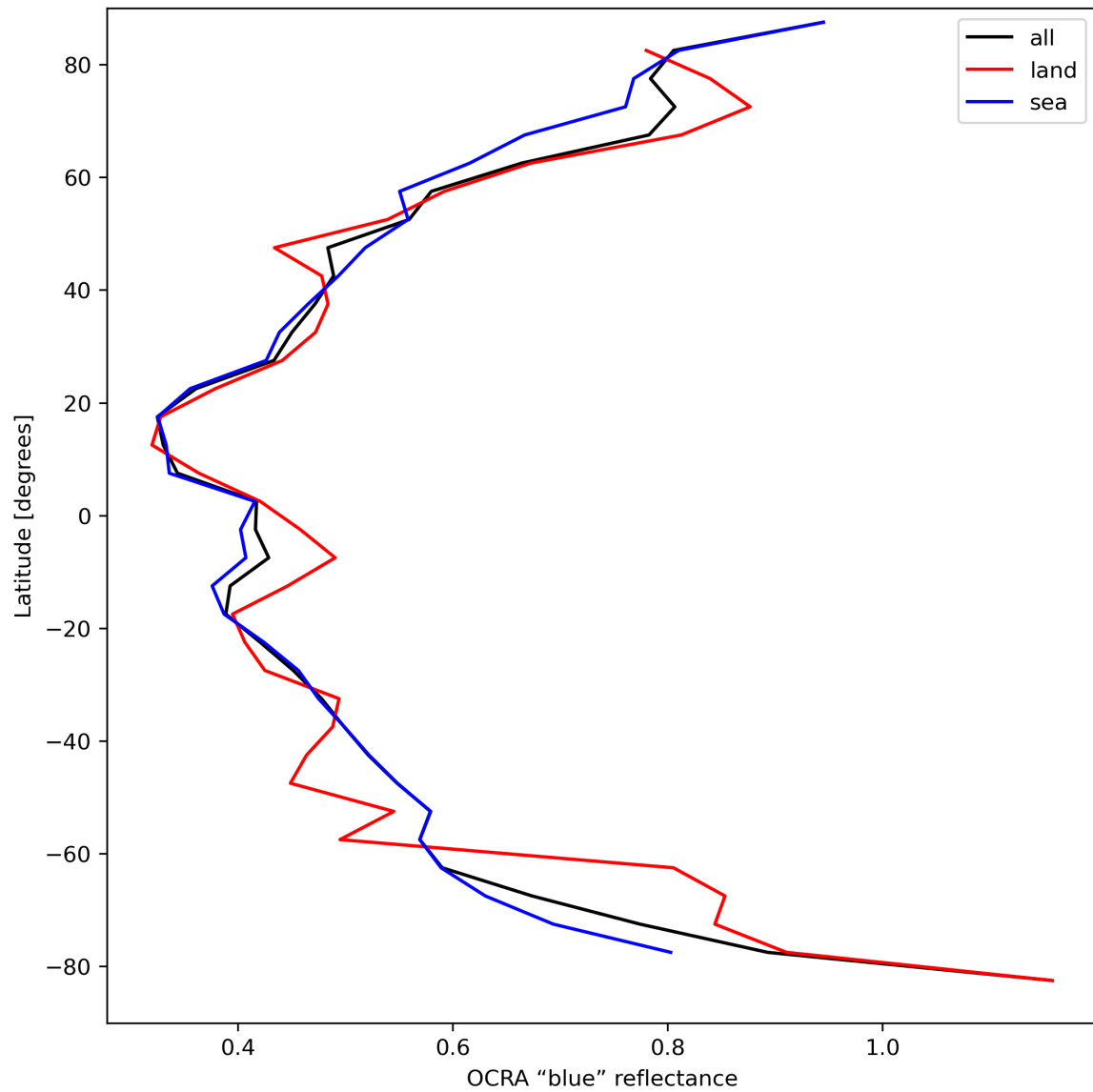
Figure 35: Zonal average of “OCRA “blue” reflectance” for 2024-03-31 to 2024-04-02.
