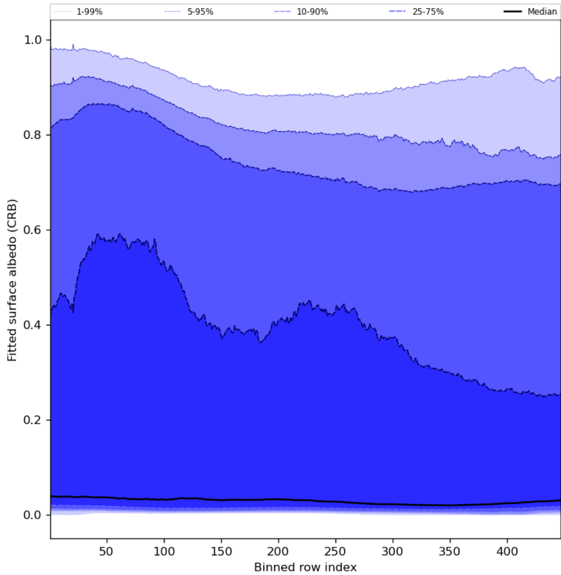
Figure 62: Along track statistics of “Fitted surface albedo (CRB)” for 2024-03-31 to 2024-04-02
