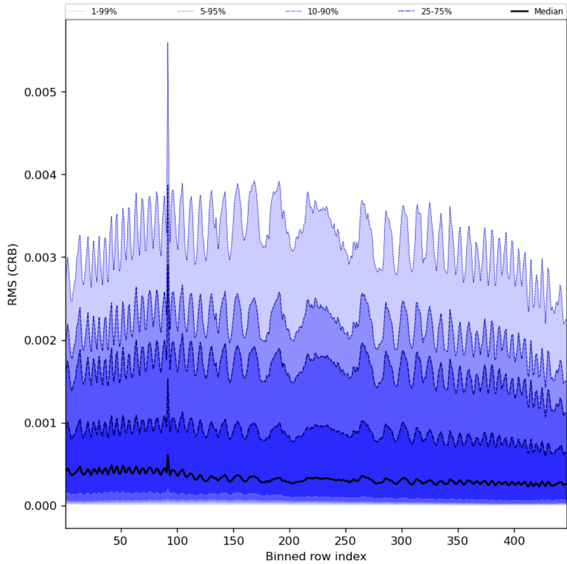
Figure 64: Along track statistics of “RMS (CRB)” for 2024-03-31 to 2024-04-02
