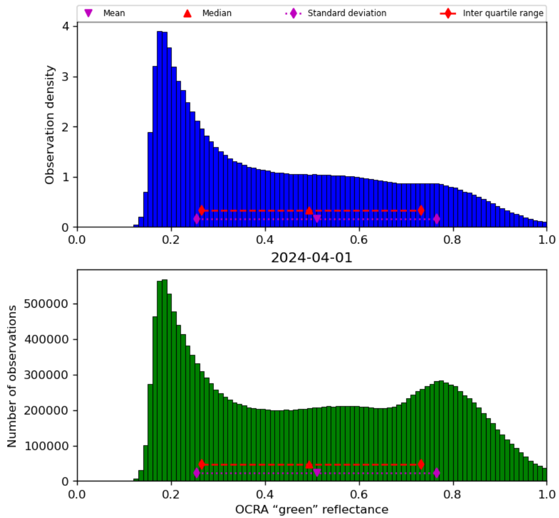
Figure 52: Histogram of “OCRA “green” reflectance” for 2024-03-31 to 2024-04-02
