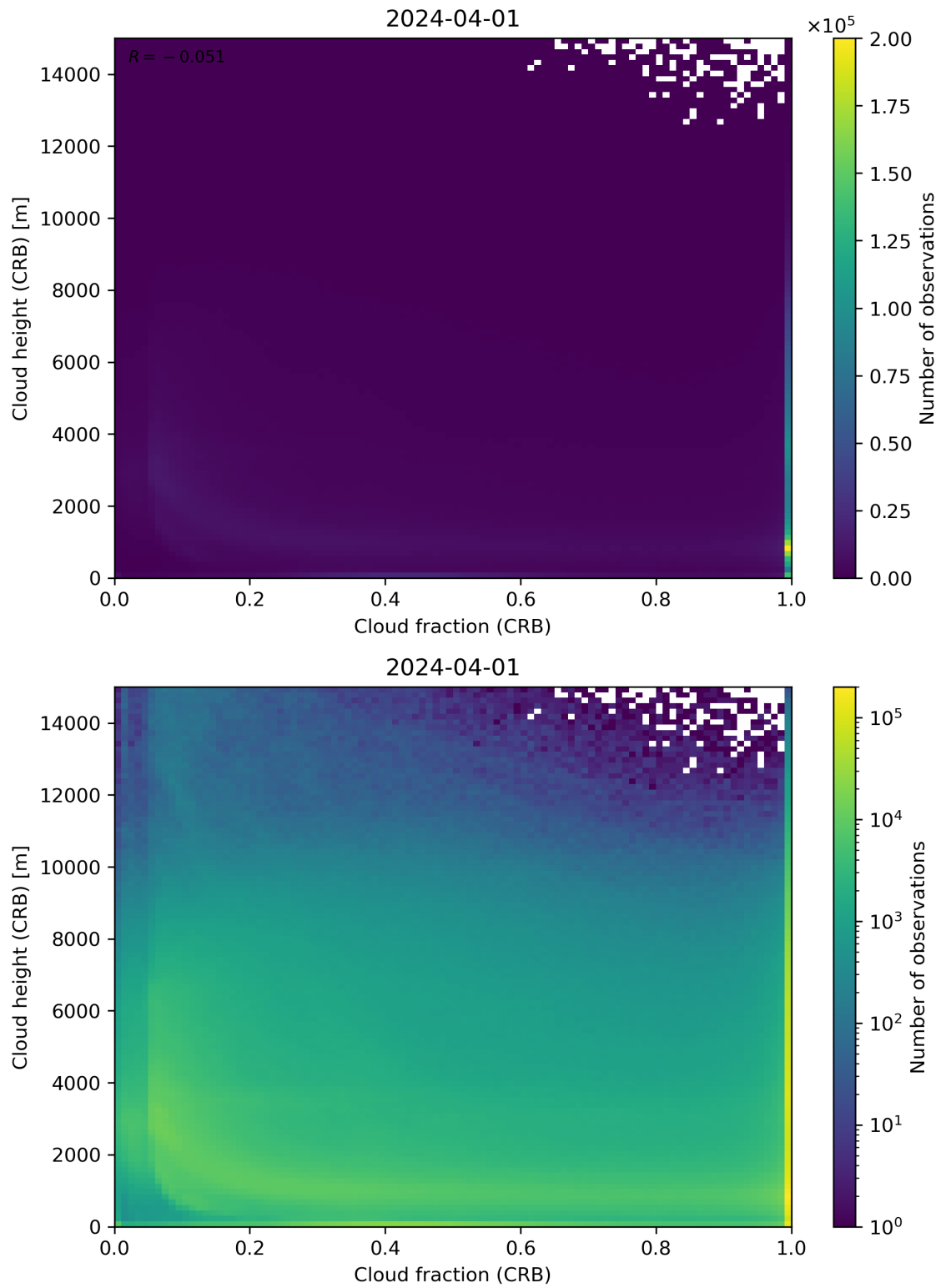
Figure 79: Scatter density plot of “Cloud fraction (CRB)” against “Cloud height (CRB)” for 2024-03-31 to 2024-04-02.
