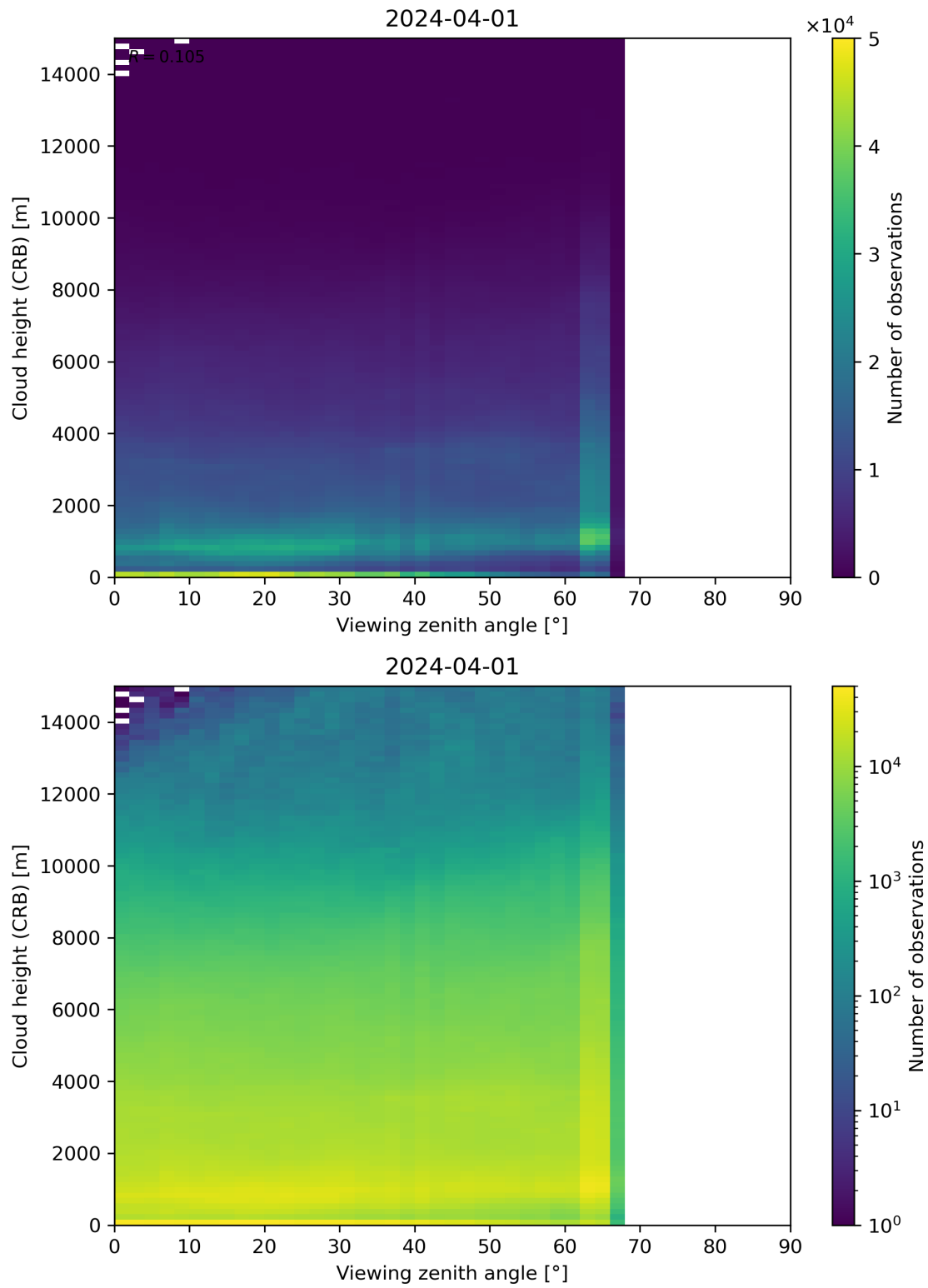
Figure 110: Scatter density plot of “Viewing zenith angle” against “Cloud height (CRB)” for 2024-03-31 to 2024-04-02.
