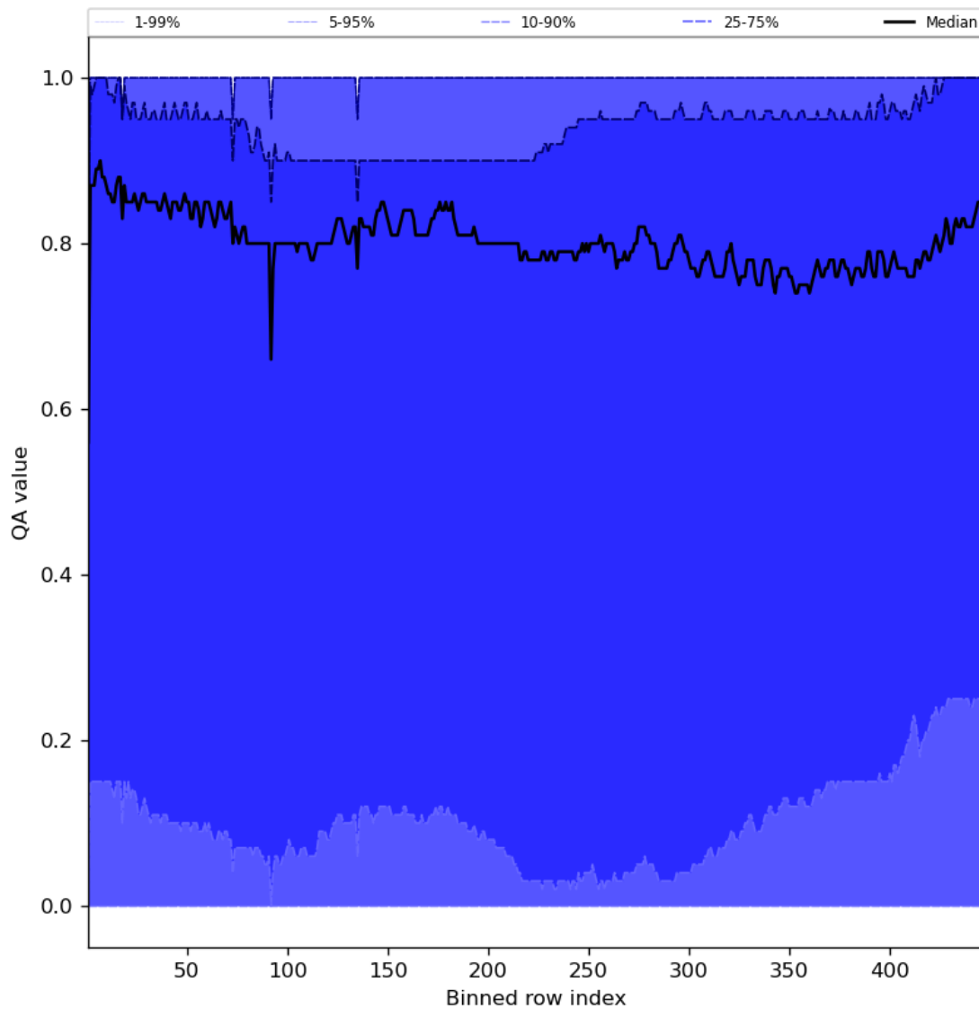
Figure 54: Along track statistics of “QA value” for 2024-03-31 to 2024-04-02
