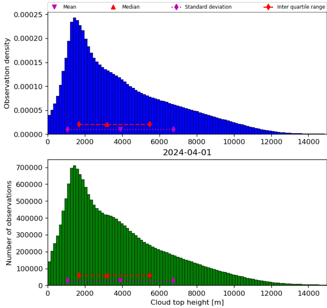
Figure 40: Histogram of “Cloud top height” for 2024-03-31 to 2024-04-02
