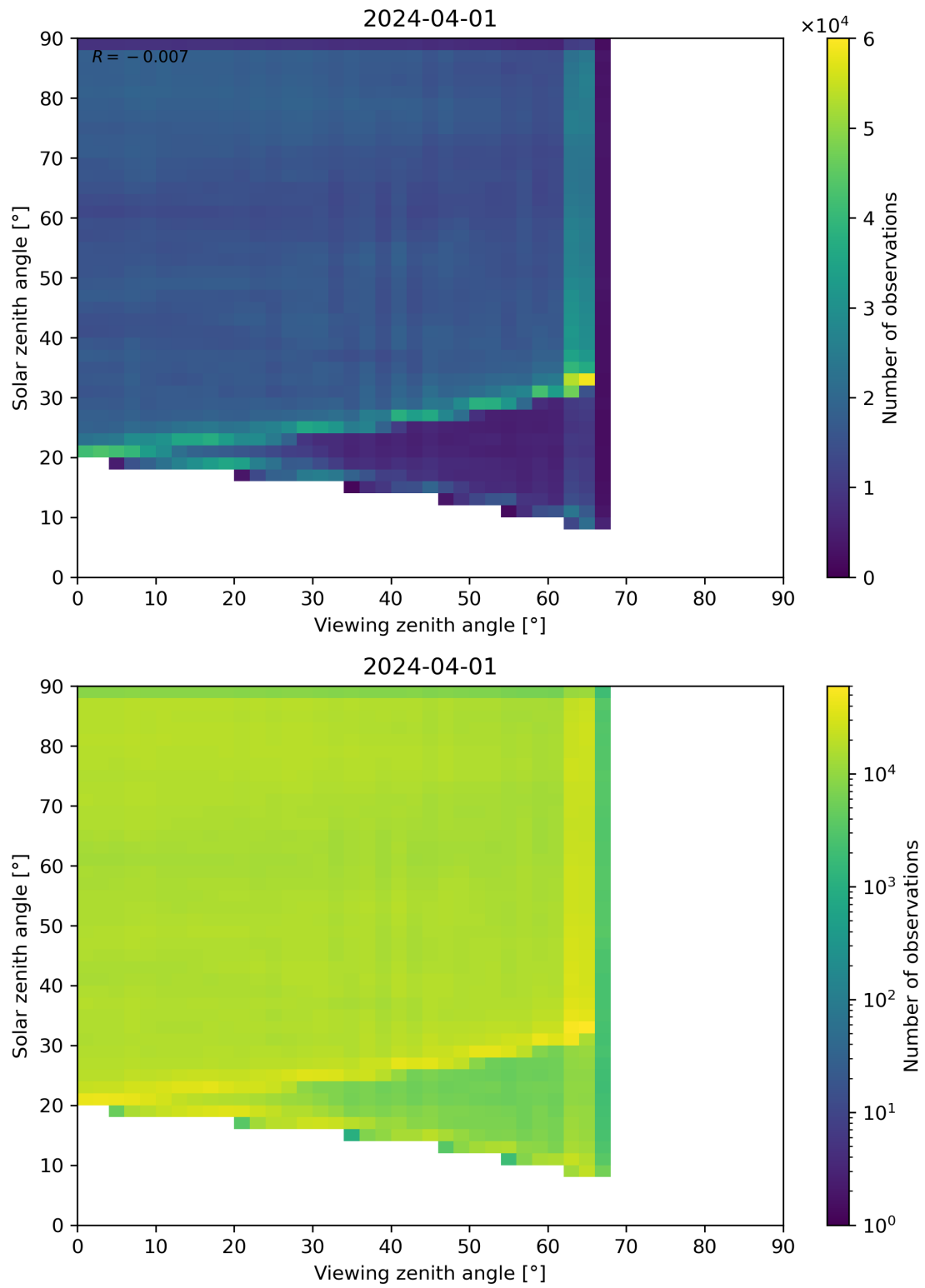
Figure 114: Scatter density plot of “Viewing zenith angle” against “Solar zenith angle” for 2024-03-31 to 2024-04-02.
