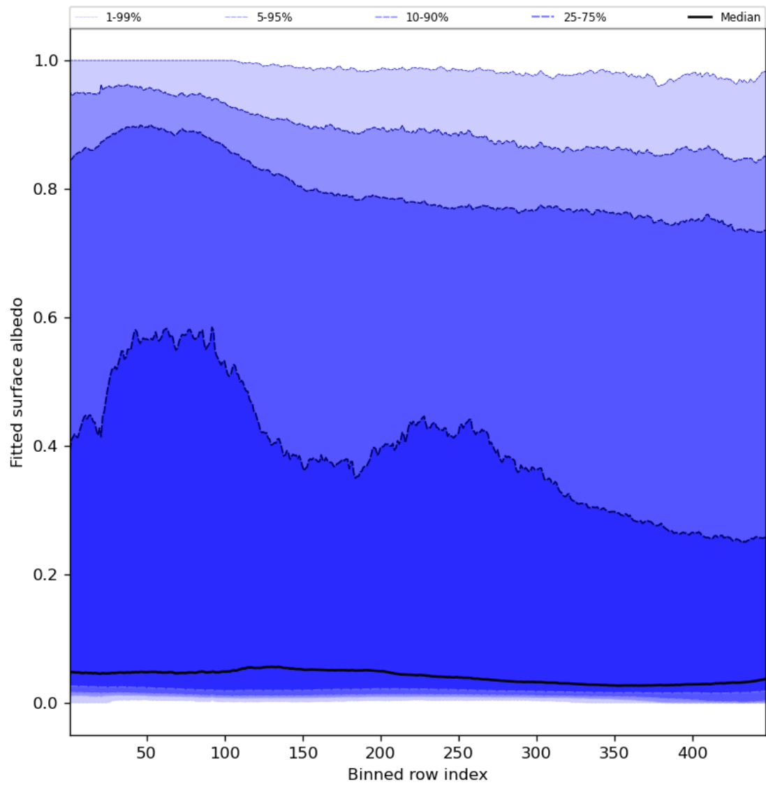
Figure 61: Along track statistics of “Fitted surface albedo” for 2024-03-31 to 2024-04-02
