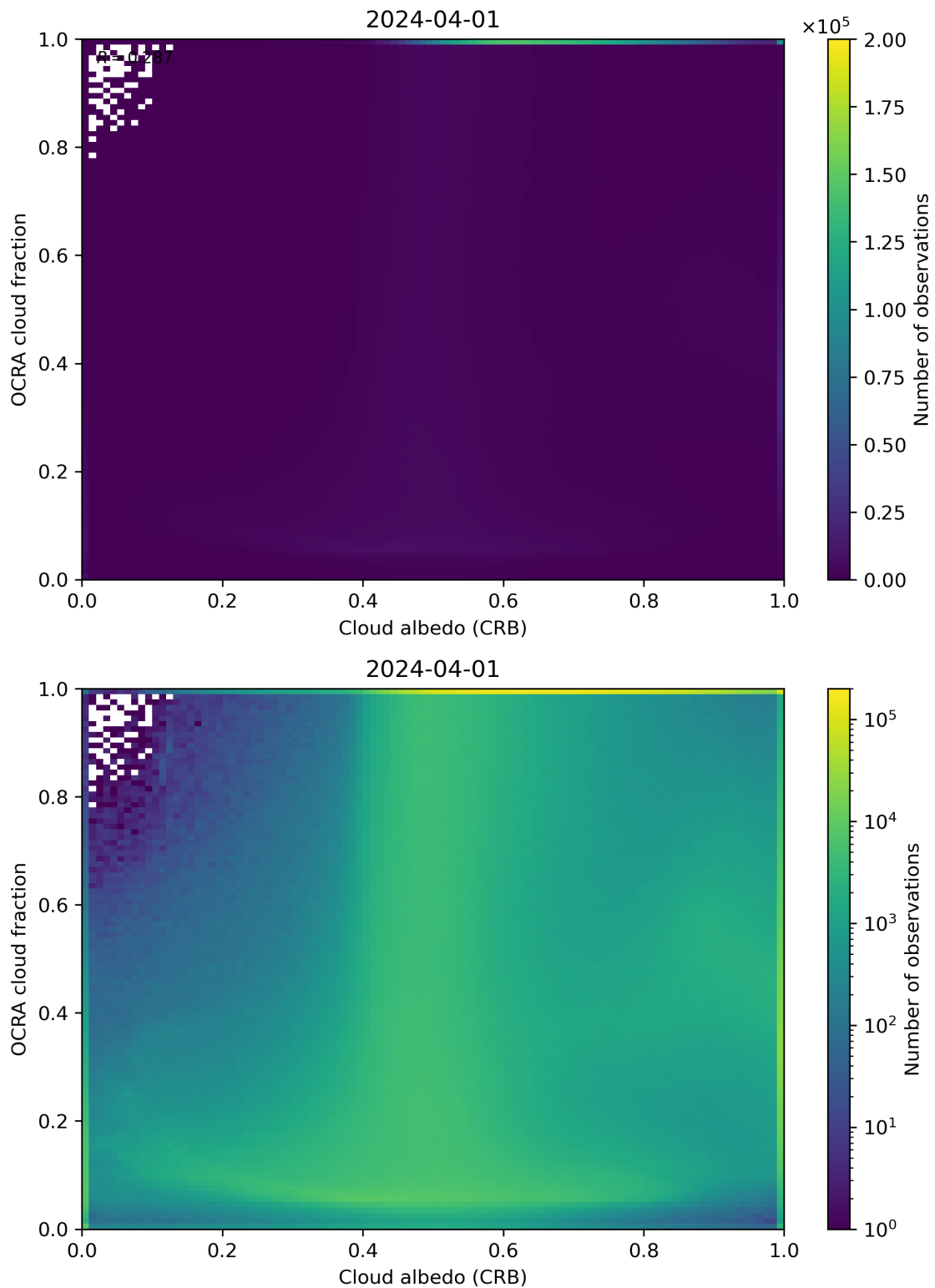
Figure 70: Scatter density plot of “Cloud albedo (CRB)” against “OCRA cloud fraction” for 2024-03-31 to 2024-04-02.
