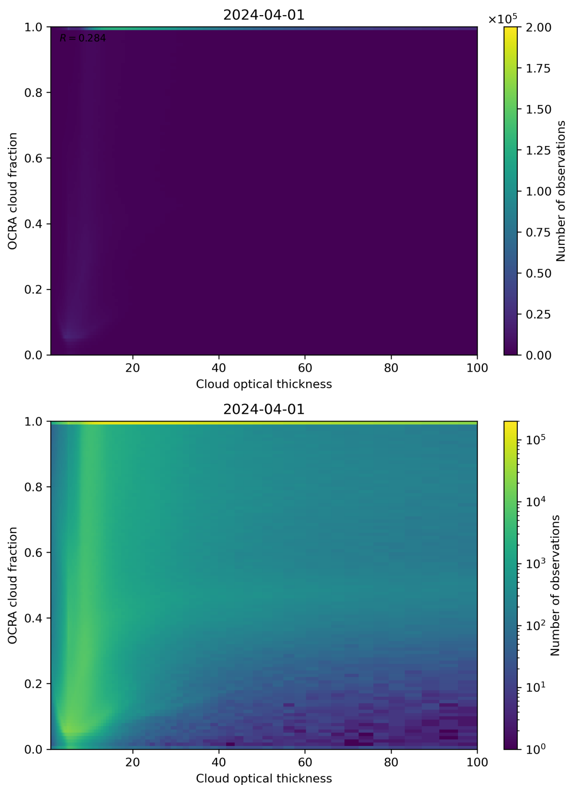
Figure 83: Scatter density plot of “Cloud optical thickness” against “OCRA cloud fraction” for 2024-03-31 to 2024-04-02.
