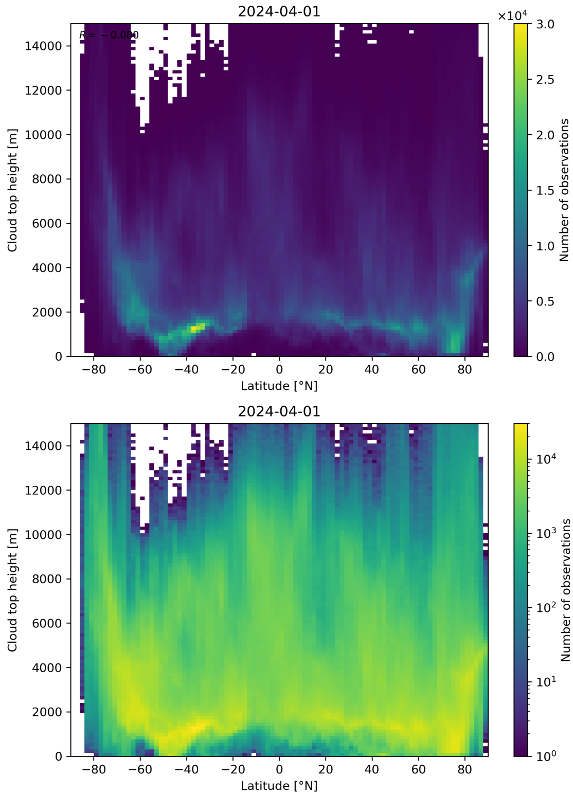
Figure 97: Scatter density plot of “Latitude” against “Cloud top height” for 2024-03-31 to 2024-04-02.
