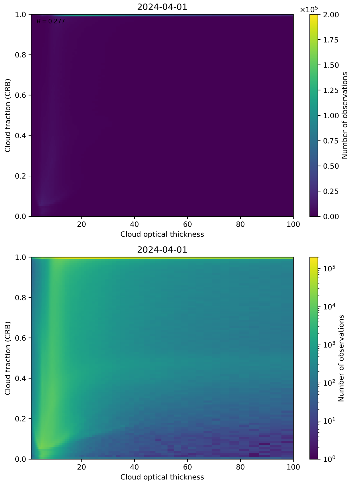
Figure 84: Scatter density plot of “Cloud optical thickness” against “Cloud fraction (CRB)” for 2024-03-31 to 2024-04-02.
