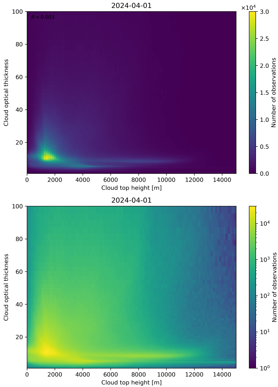
Figure 90: Scatter density plot of “Cloud top height” against “Cloud optical thickness” for 2024-03-31 to 2024-04-02.
