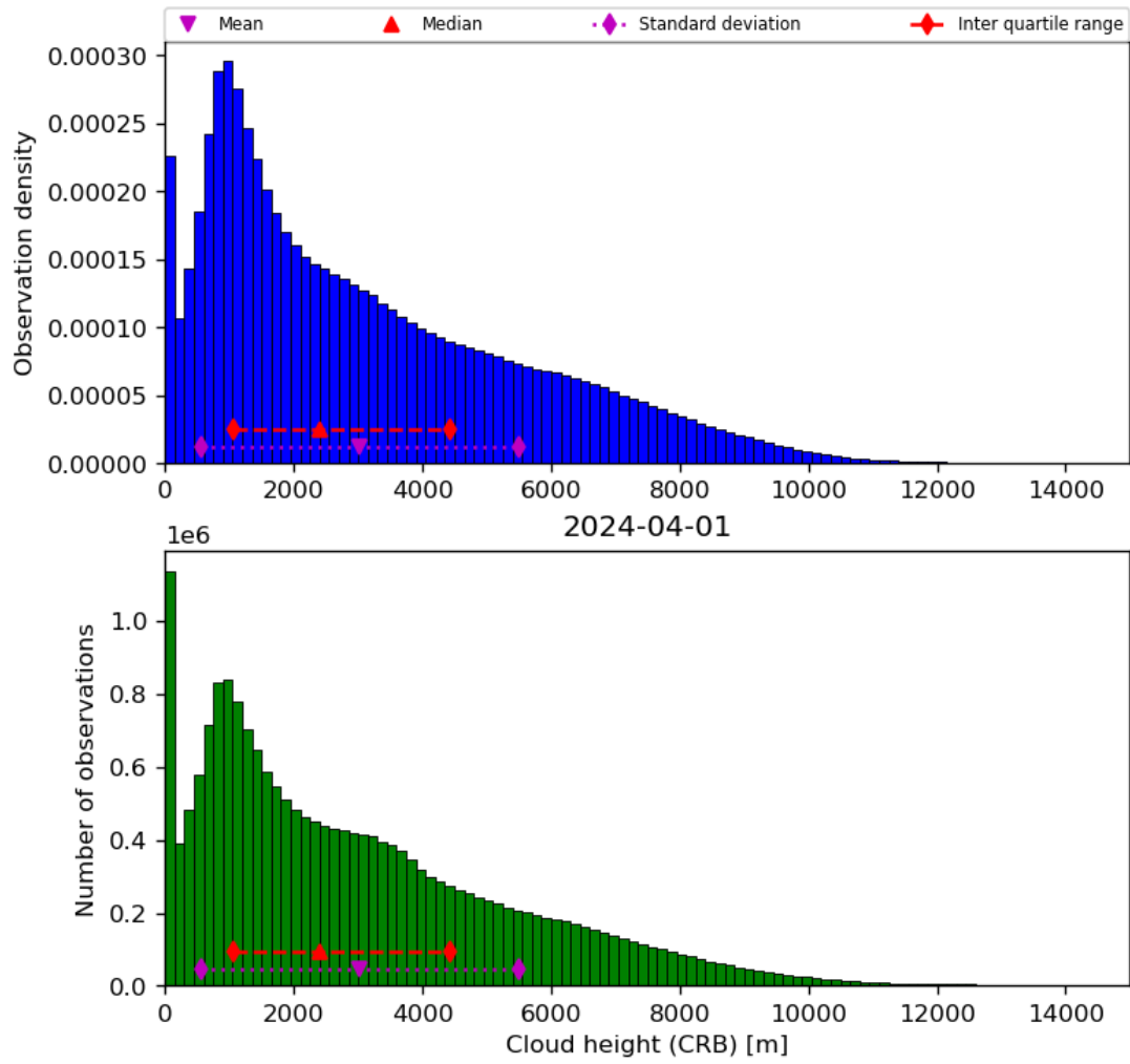
Figure 43: Histogram of “Cloud height (CRB)” for 2024-03-31 to 2024-04-02
