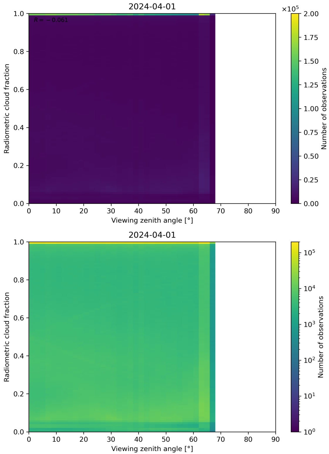
Figure 107: Scatter density plot of “Viewing zenith angle” against “Radiometric cloud fraction” for 2024-03-31 to 2024-04-02.
