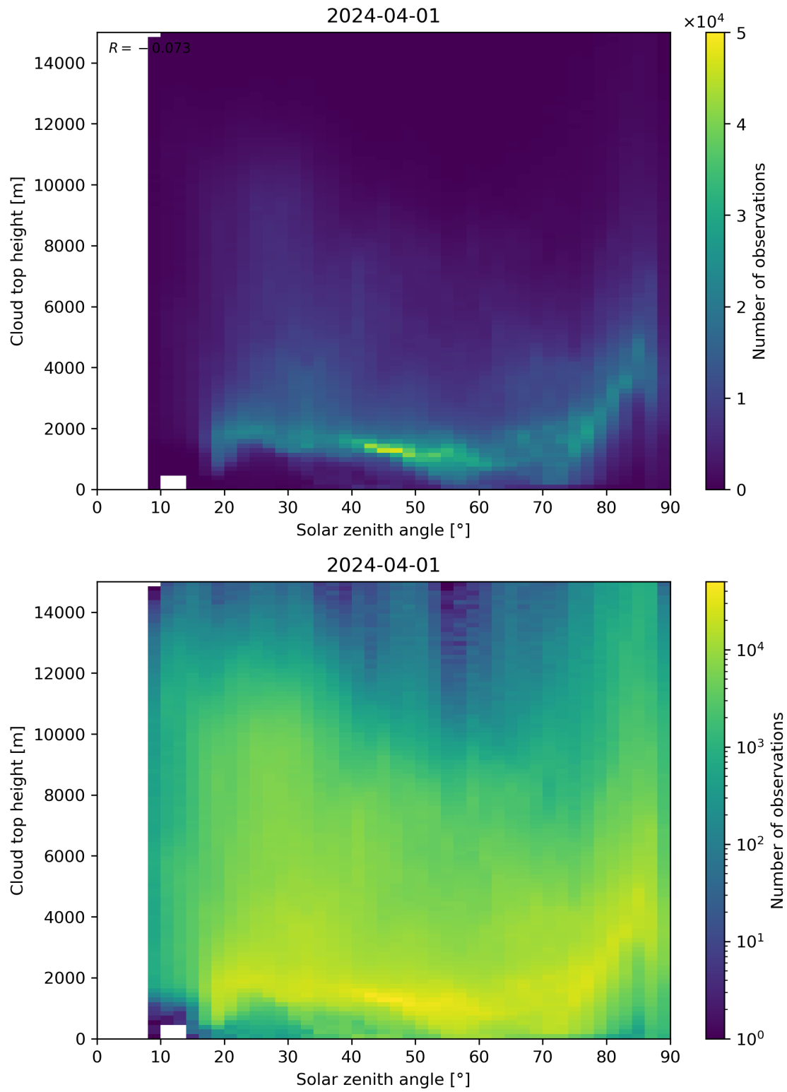
Figure 104: Scatter density plot of “Solar zenith angle” against “Cloud top height” for 2024-03-31 to 2024-04-02.
