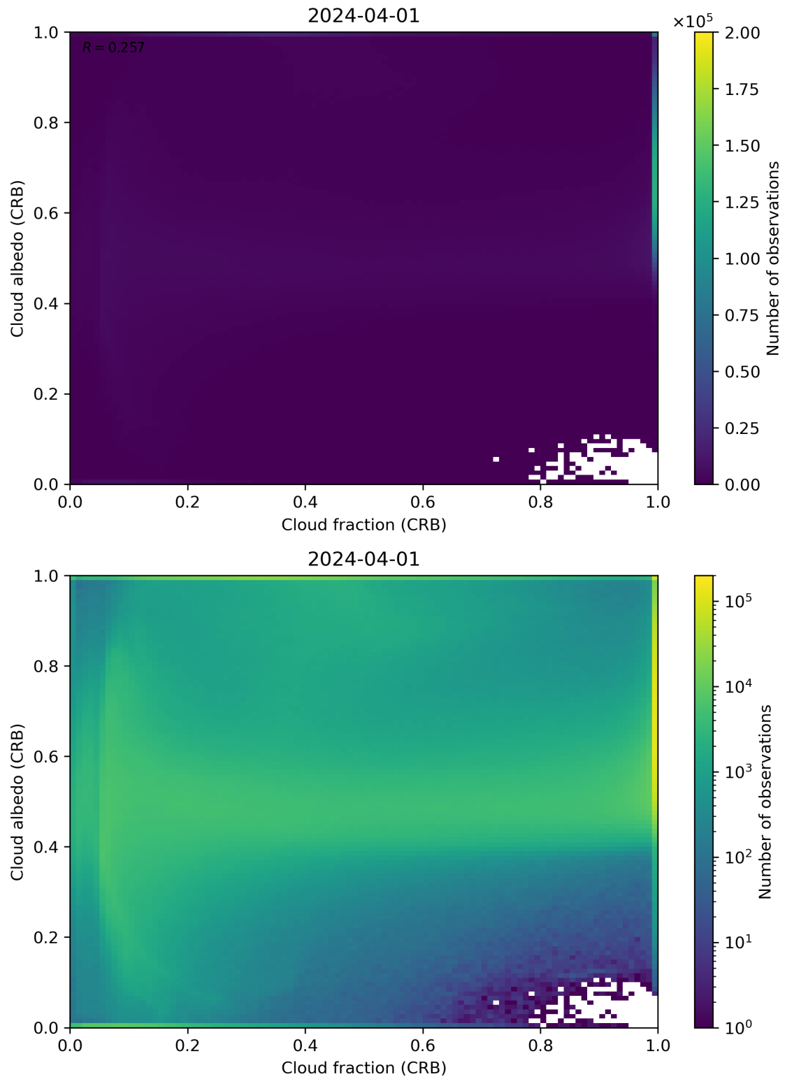
Figure 77: Scatter density plot of “Cloud fraction (CRB)” against “Cloud albedo (CRB)” for 2024-03-31 to 2024-04-02.
