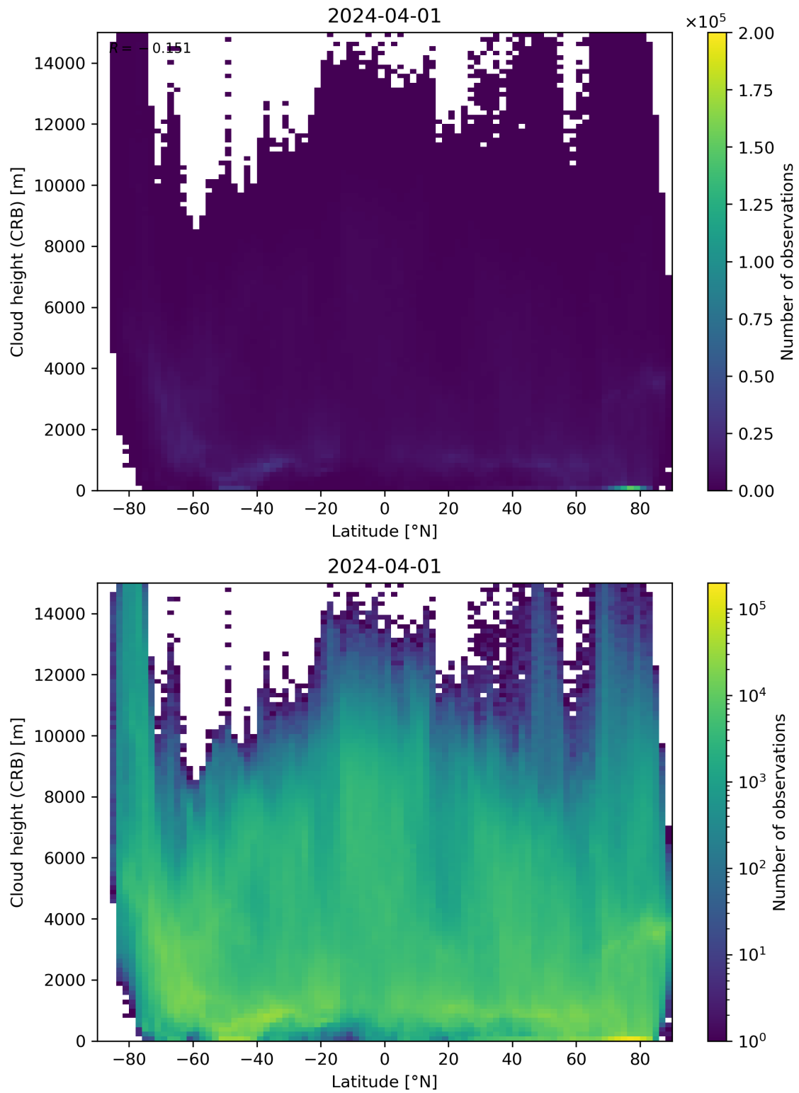
Figure 95: Scatter density plot of “Latitude” against “Cloud height (CRB)” for 2024-03-31 to 2024-04-02.
