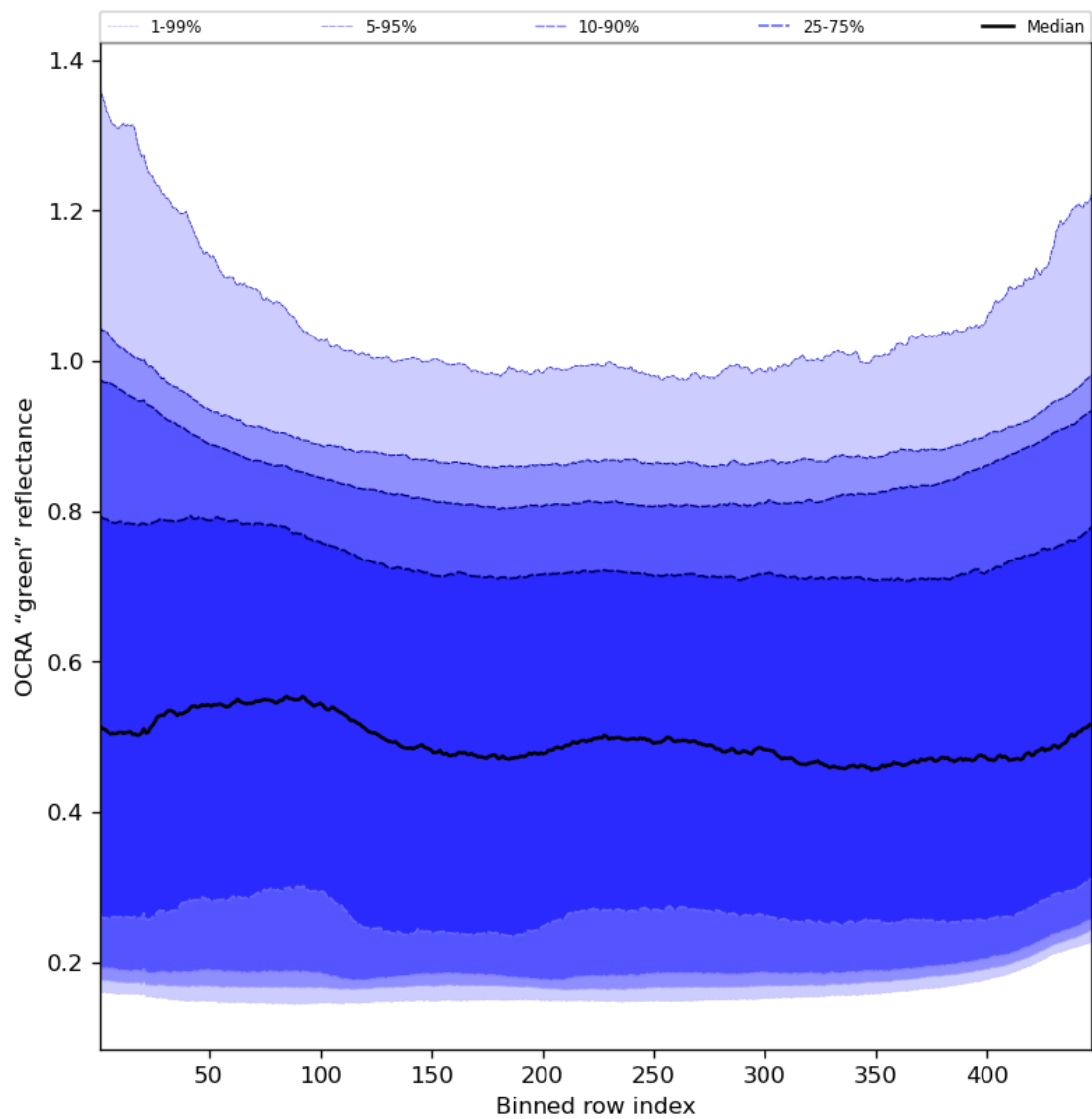
Figure 68: Along track statistics of “OCRA “green” reflectance” for 2024-03-31 to 2024-04-02
