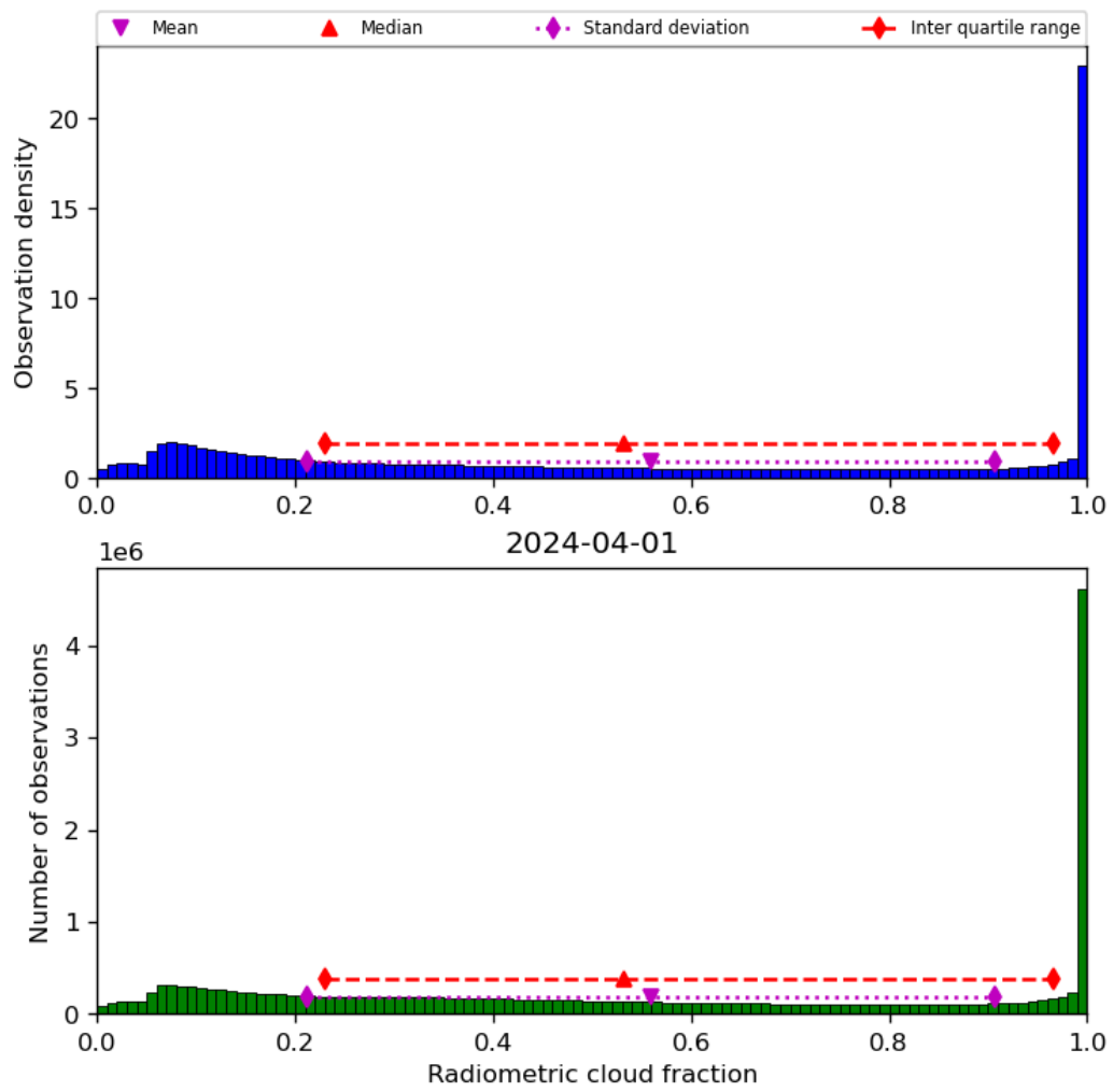
Figure 39: Histogram of “Radiometric cloud fraction” for 2024-03-31 to 2024-04-02
