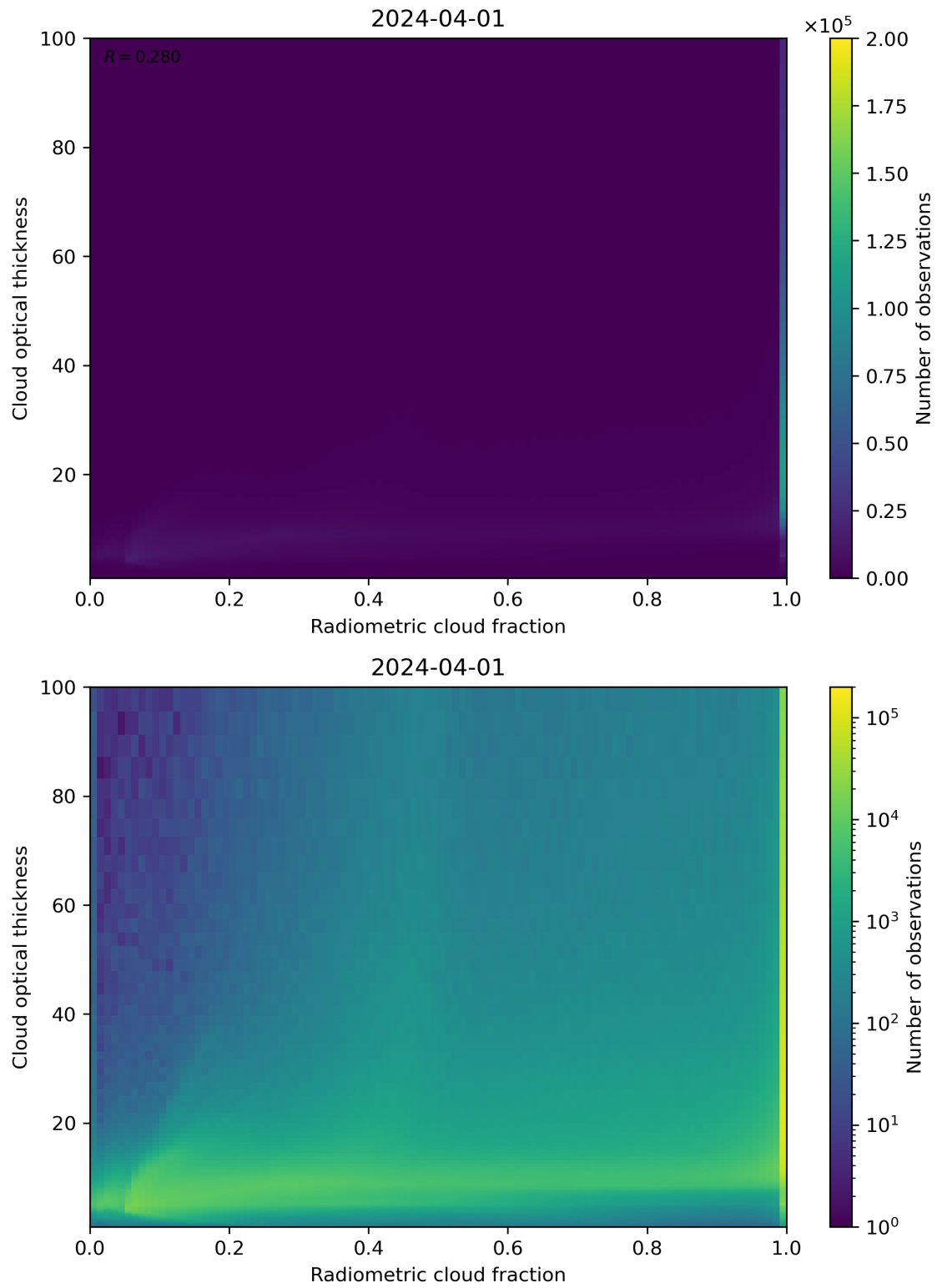
Figure 75: Scatter density plot of “Radiometric cloud fraction” against “Cloud optical thickness” for 2024-03-31 to 2024-04-02.
