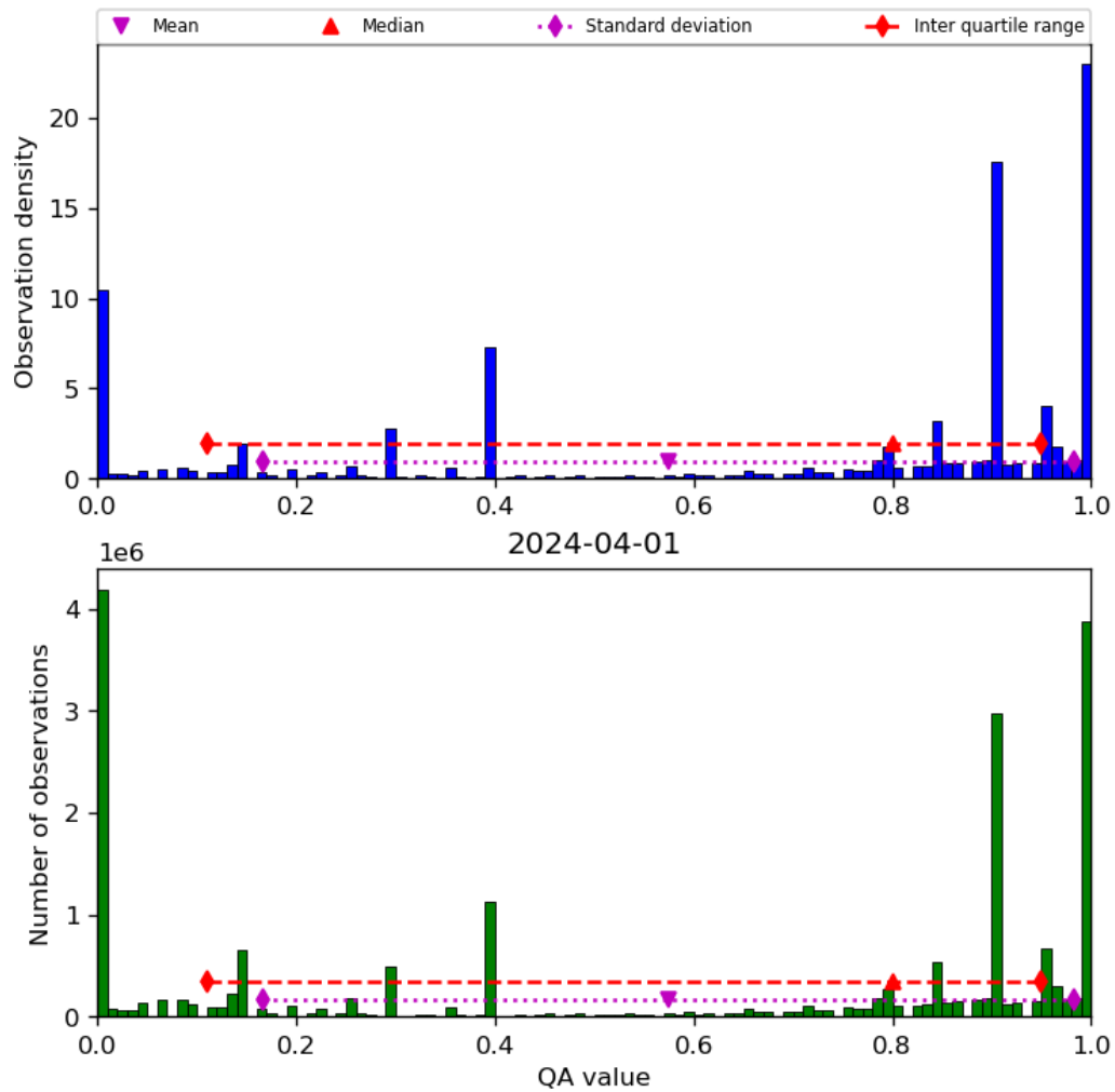
Figure 38: Histogram of “QA value” for 2024-03-31 to 2024-04-02
