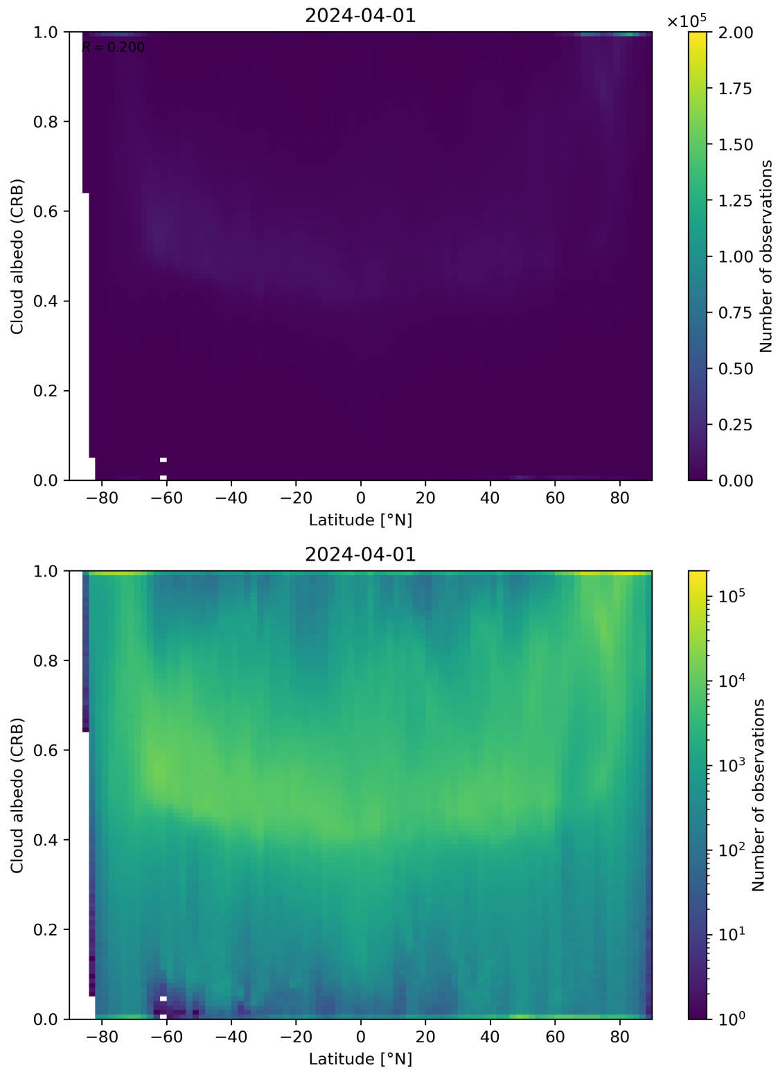
Figure 91: Scatter density plot of “Latitude” against “Cloud albedo (CRB)” for 2024-03-31 to 2024-04-02.
