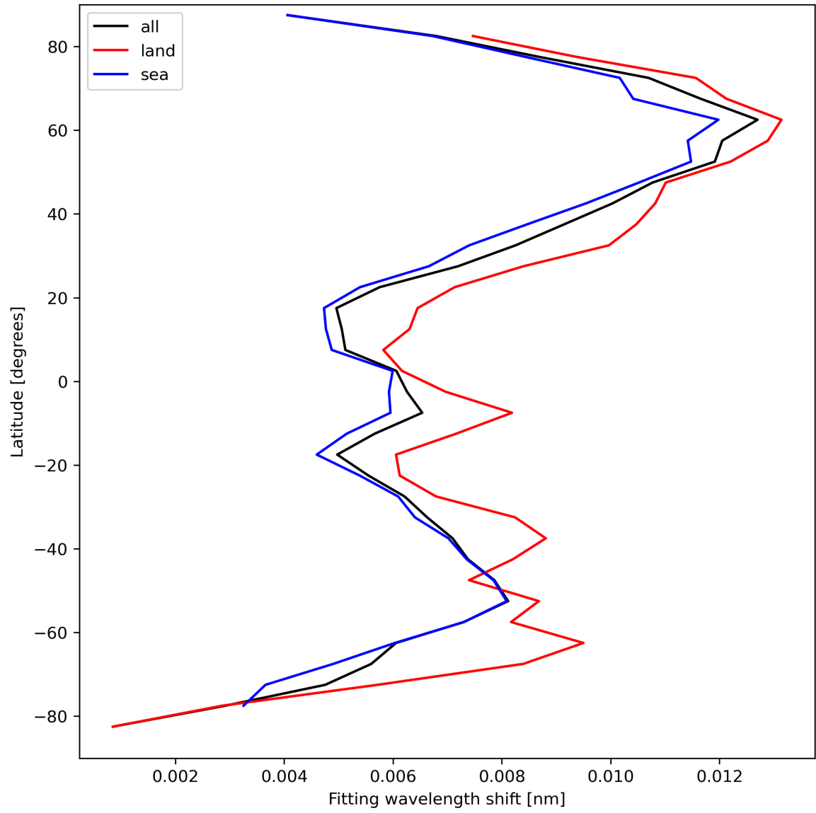
Figure 33: Zonal average of “Fitting wavelength shift” for 2024-03-31 to 2024-04-02.
