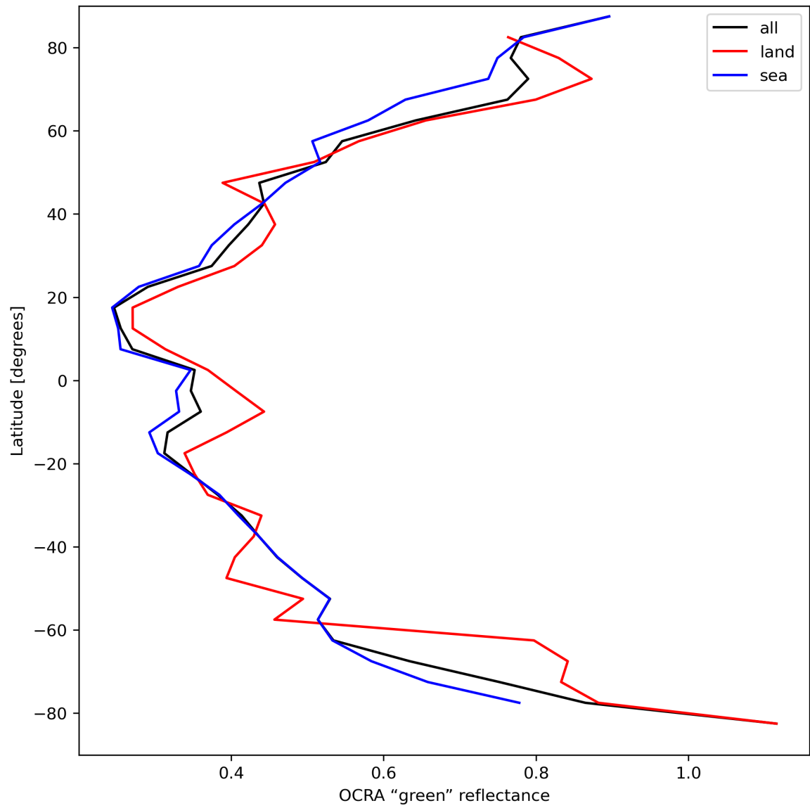
Figure 36: Zonal average of “OCRA “green” reflectance” for 2024-03-31 to 2024-04-02.
