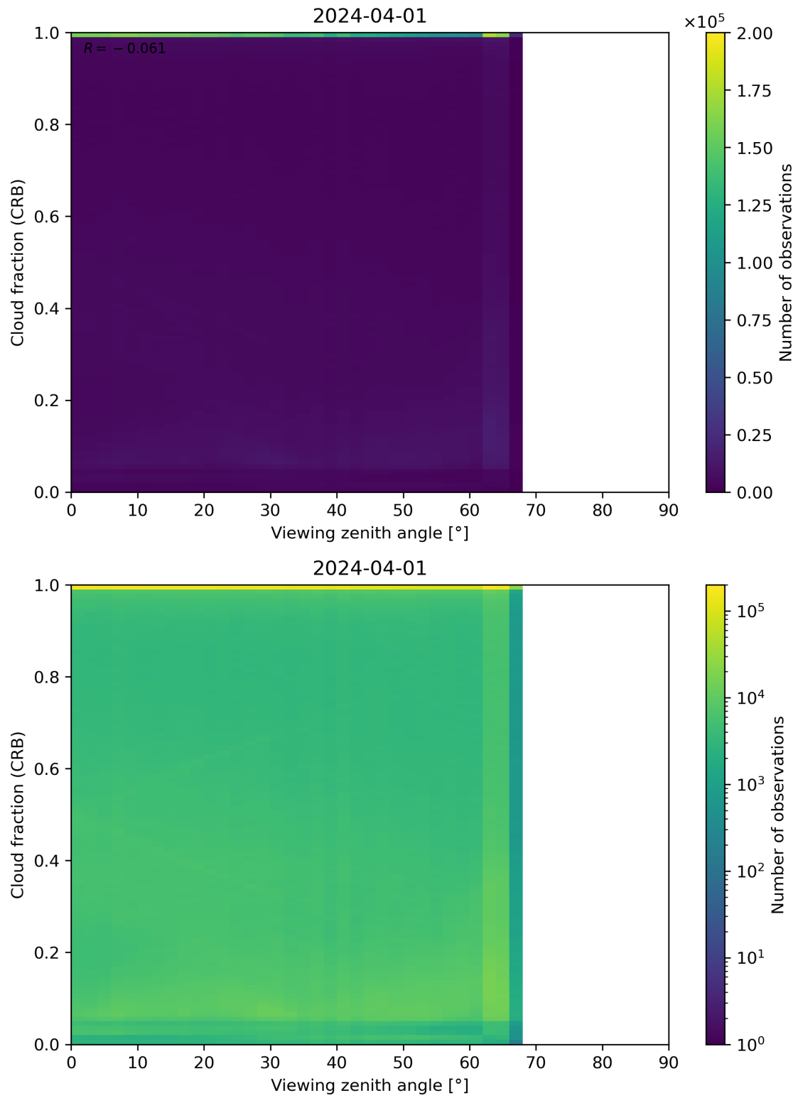
Figure 109: Scatter density plot of “Viewing zenith angle” against “Cloud fraction (CRB)” for 2024-03-31 to 2024-04-02.
