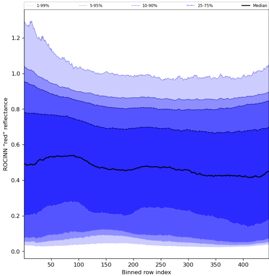
Figure 69: Along track statistics of “ROCINN “red” reflectance” for 2024-03-31 to 2024-04-02
