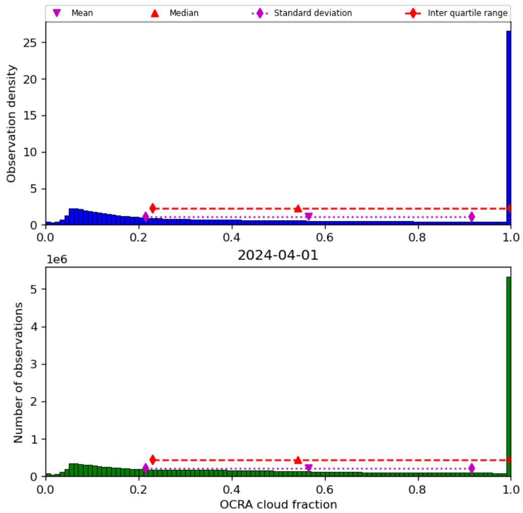
Figure 50: Histogram of “OCRA cloud fraction” for 2024-03-31 to 2024-04-02
