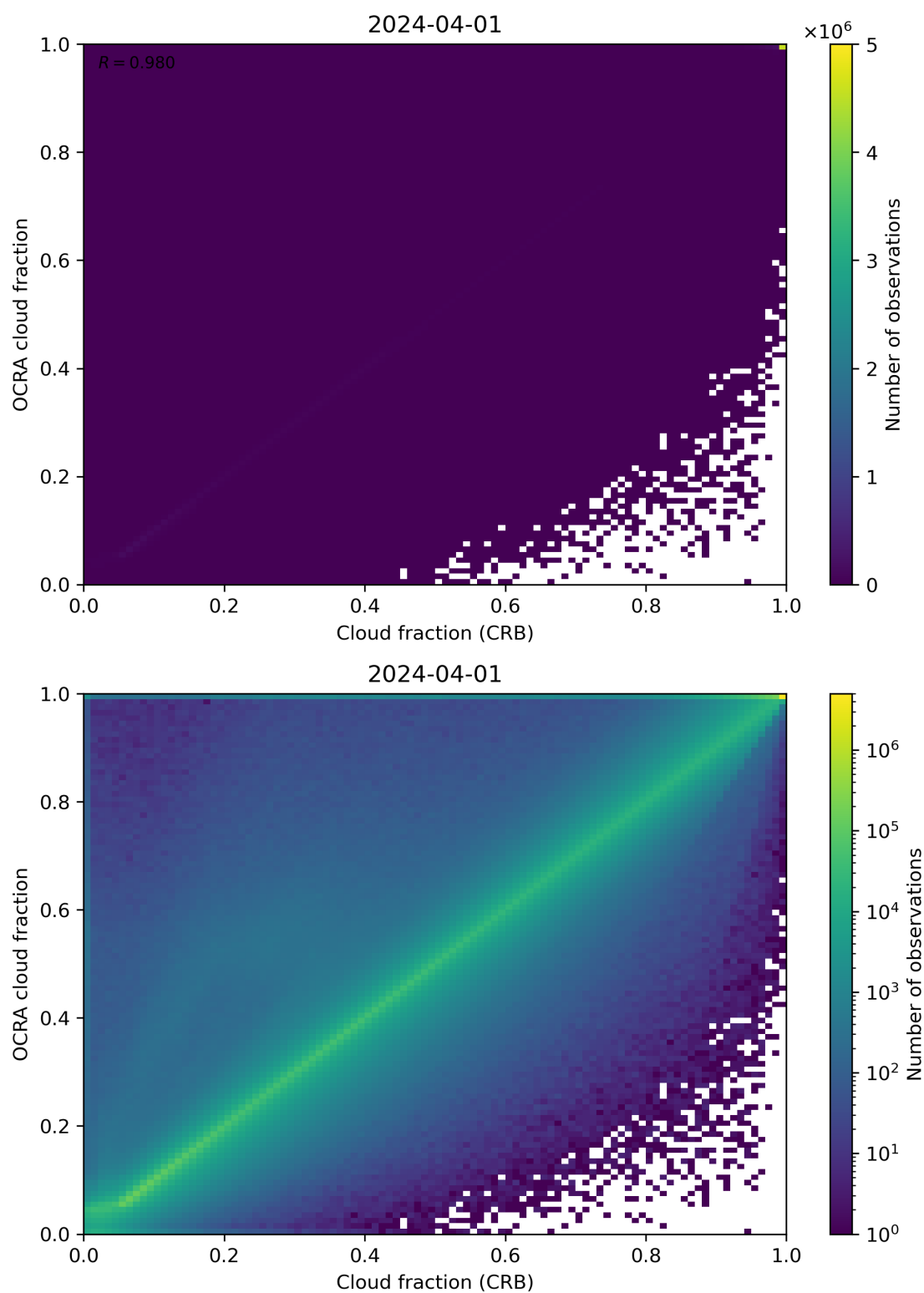
Figure 78: Scatter density plot of “Cloud fraction (CRB)” against “OCRA cloud fraction” for 2024-03-31 to 2024-04-02.
