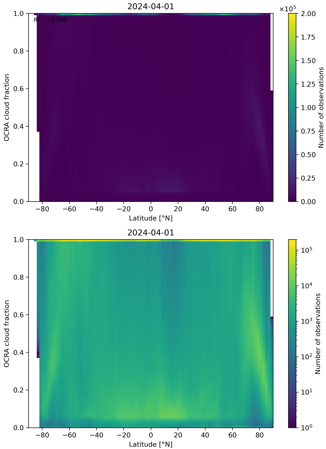
Figure 93: Scatter density plot of “Latitude” against “OCRA cloud fraction” for 2024-03-31 to 2024-04-02.
