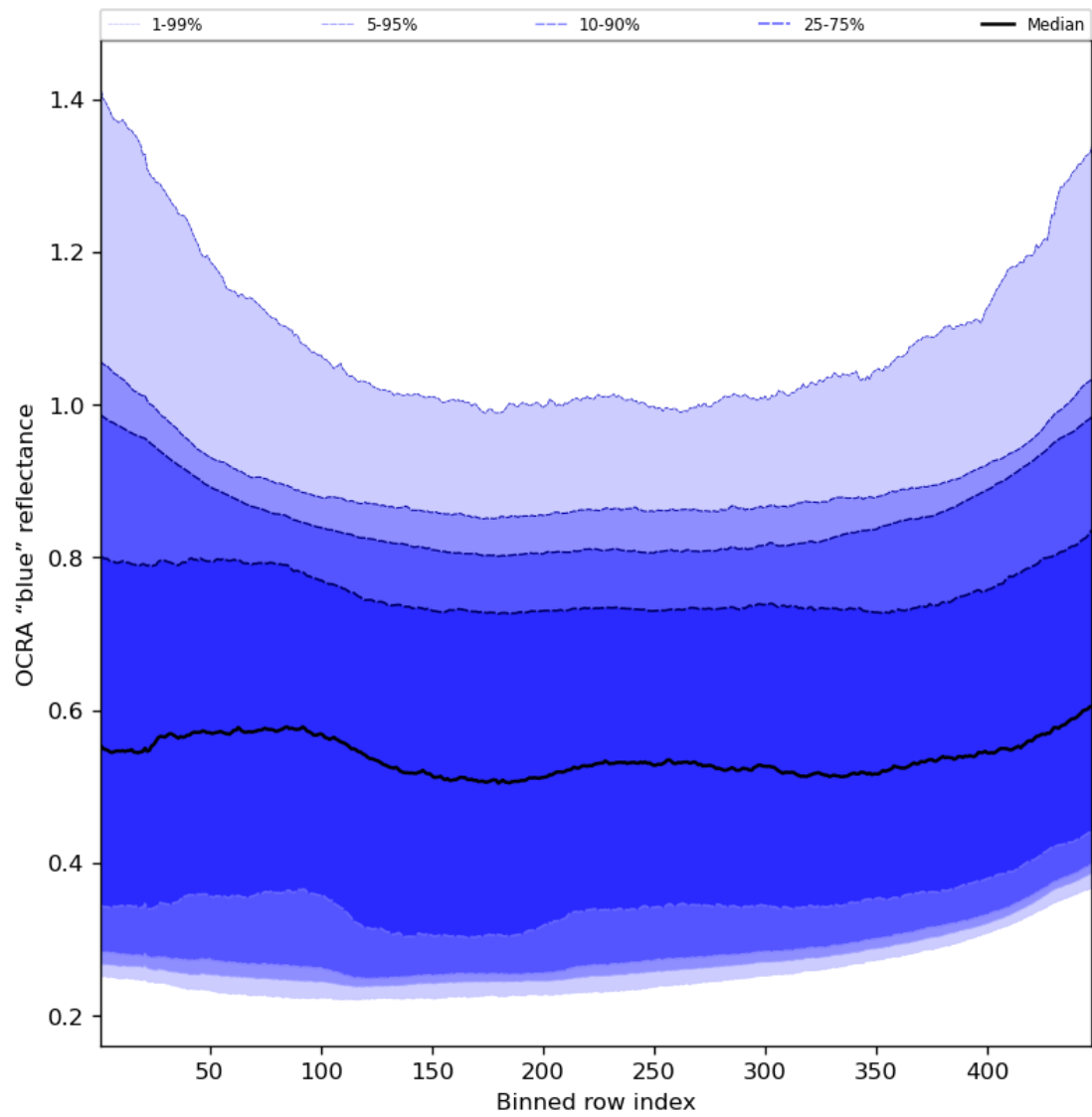
Figure 67: Along track statistics of “OCRA “blue” reflectance” for 2024-03-31 to 2024-04-02
