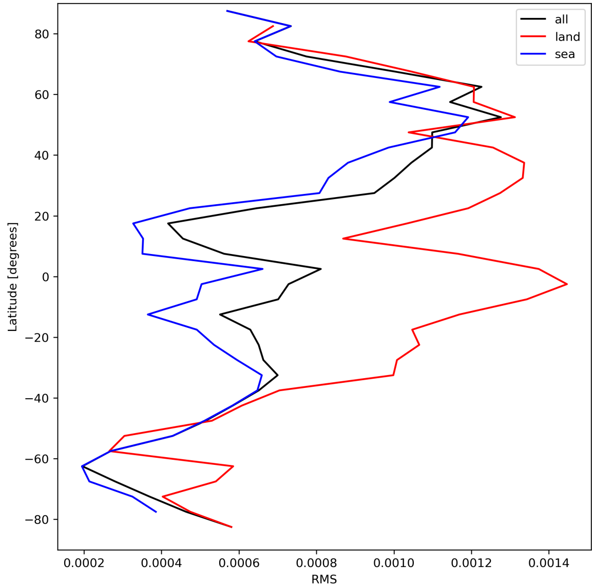
Figure 31: Zonal average of “RMS” for 2024-03-31 to 2024-04-02.
