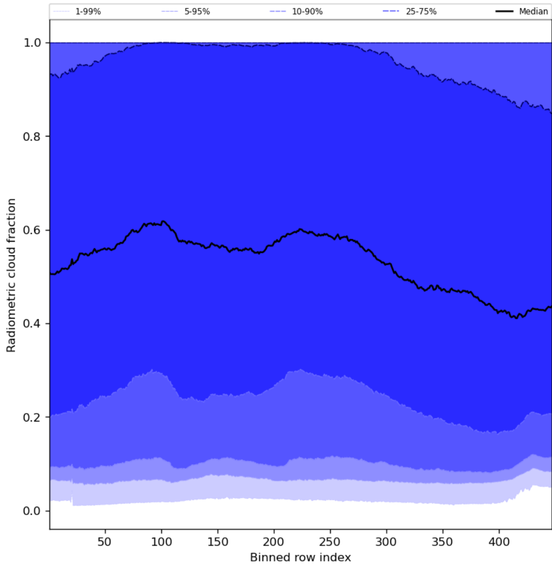
Figure 55: Along track statistics of “Radiometric cloud fraction” for 2024-03-31 to 2024-04-02
