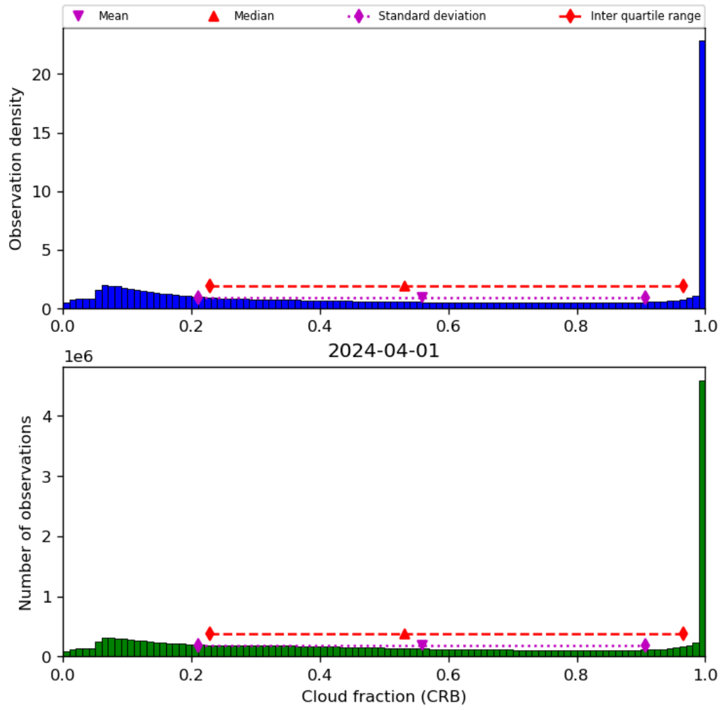
Figure 42: Histogram of “Cloud fraction (CRB)” for 2024-03-31 to 2024-04-02
