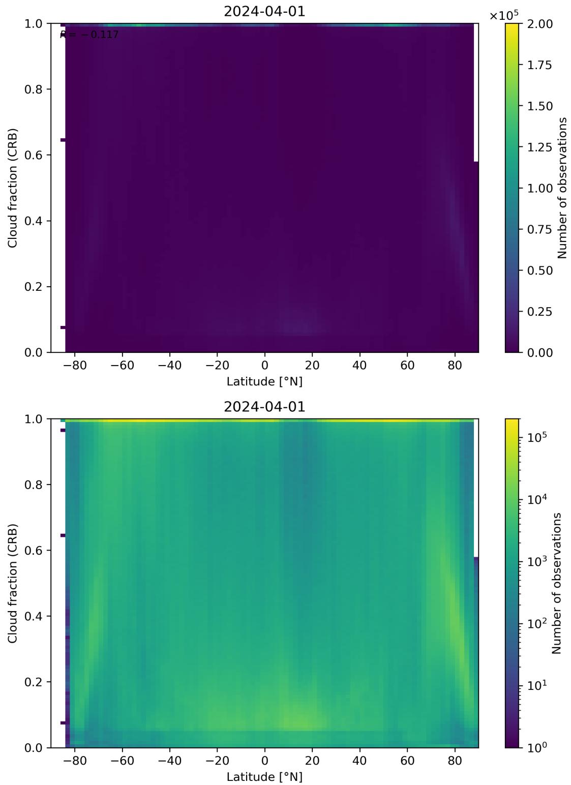
Figure 94: Scatter density plot of “Latitude” against “Cloud fraction (CRB)” for 2024-03-31 to 2024-04-02.
