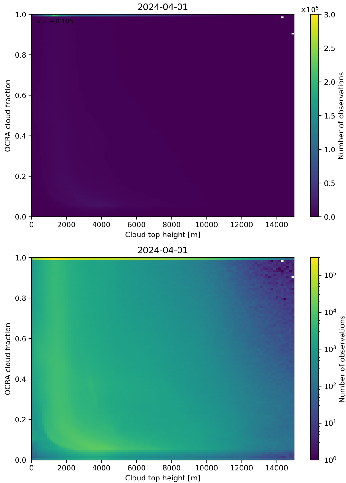
Figure 87: Scatter density plot of “Cloud top height” against “OCRA cloud fraction” for 2024-03-31 to 2024-04-02.
