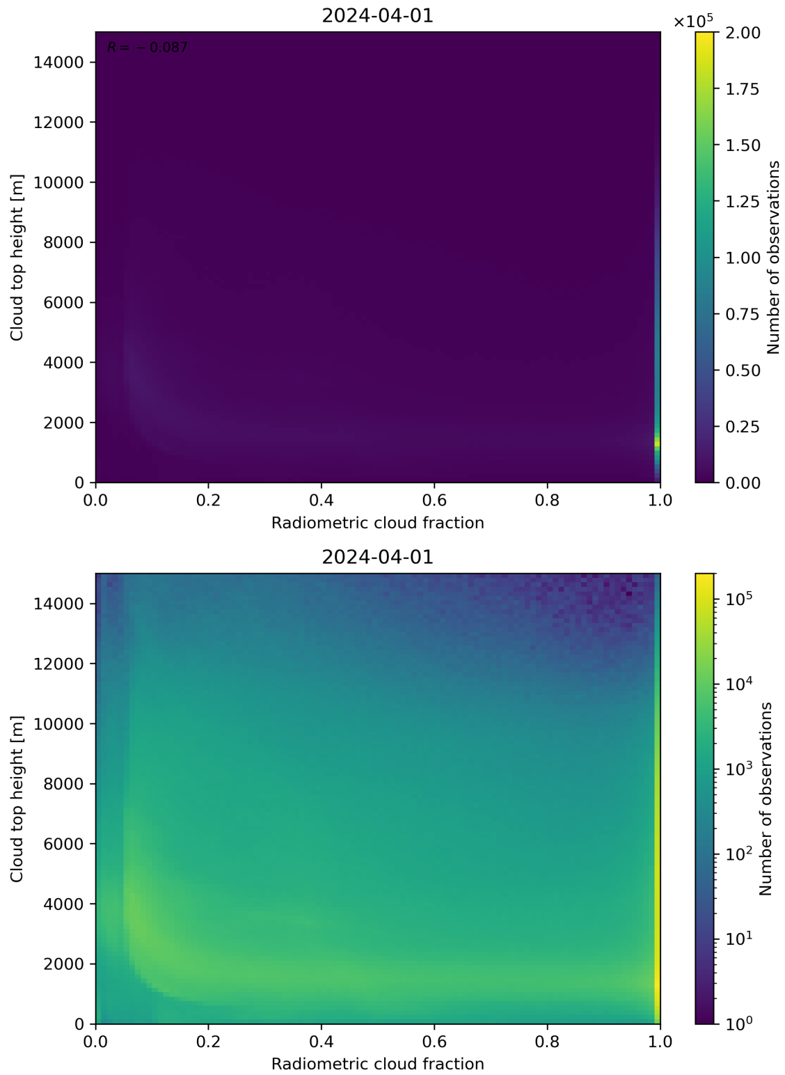
Figure 76: Scatter density plot of “Radiometric cloud fraction” against “Cloud top height” for 2024-03-31 to 2024-04-02.
