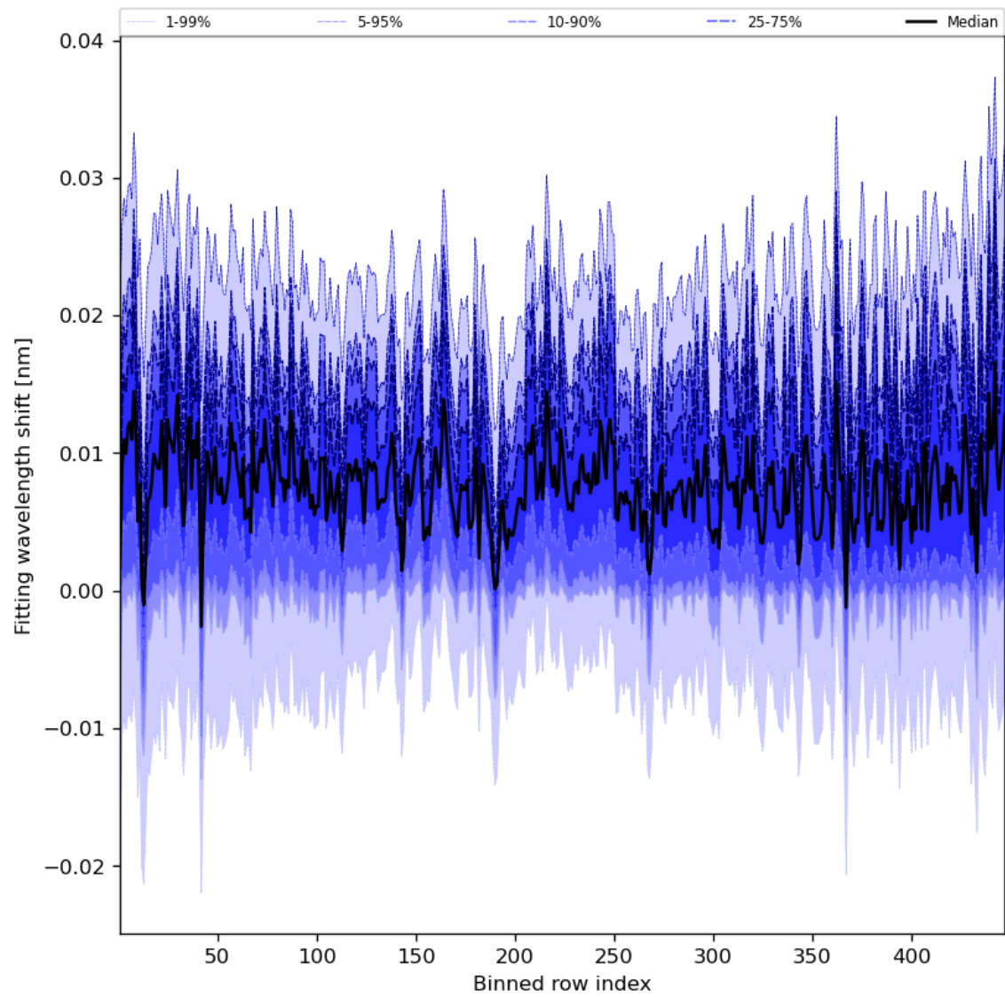
Figure 65: Along track statistics of “Fitting wavelength shift” for 2024-03-31 to 2024-04-02
