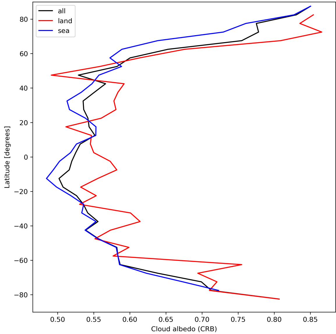
Figure 28: Zonal average of “Cloud albedo (CRB)” for 2024-03-31 to 2024-04-02.
