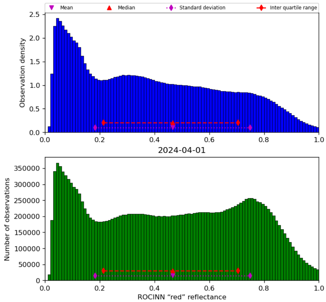
Figure 53: Histogram of “ROCINN “red” reflectance” for 2024-03-31 to 2024-04-02
