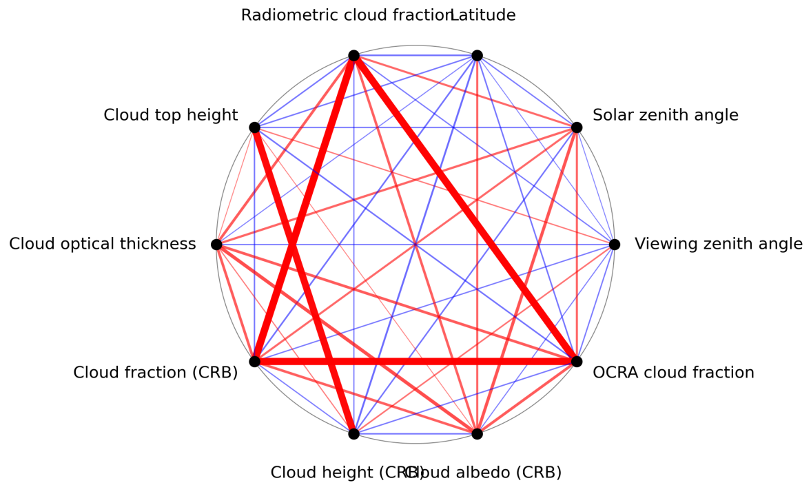
Figure 1: Map of correlation graph for 2024-03-31 to 2024-04-02.
