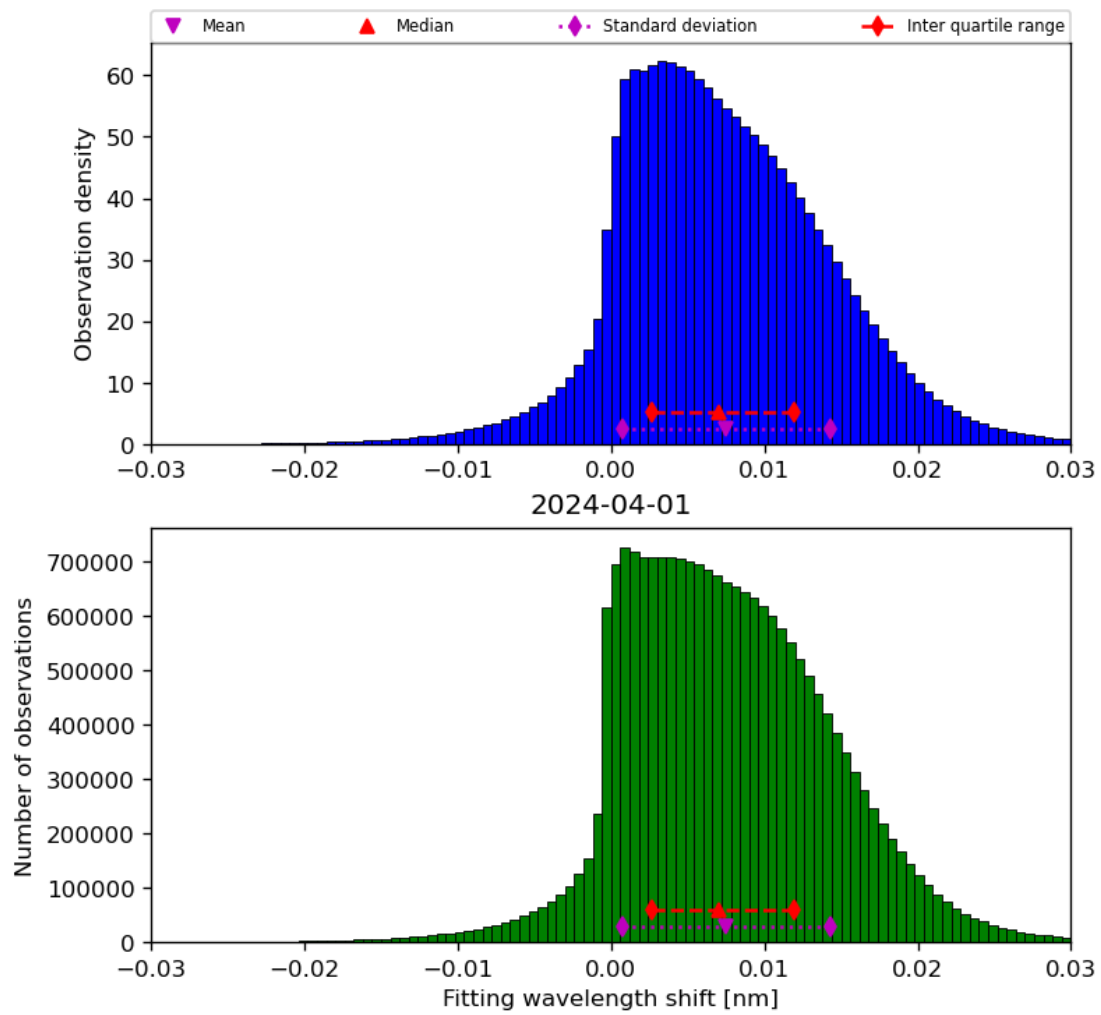
Figure 49: Histogram of “Fitting wavelength shift” for 2024-03-31 to 2024-04-02
