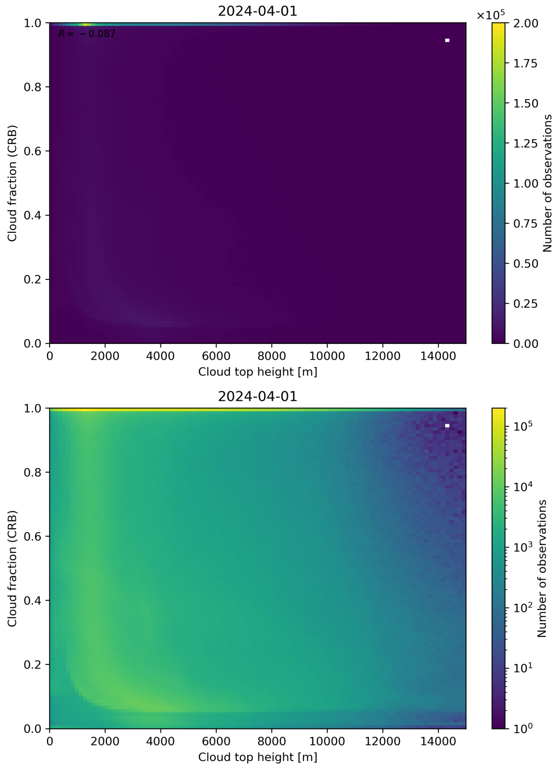
Figure 88: Scatter density plot of “Cloud top height” against “Cloud fraction (CRB)” for 2024-03-31 to 2024-04-02.
