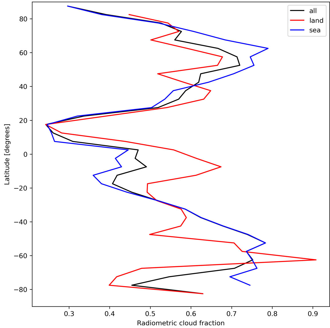
Figure 23: Zonal average of “Radiometric cloud fraction” for 2024-03-31 to 2024-04-02.
