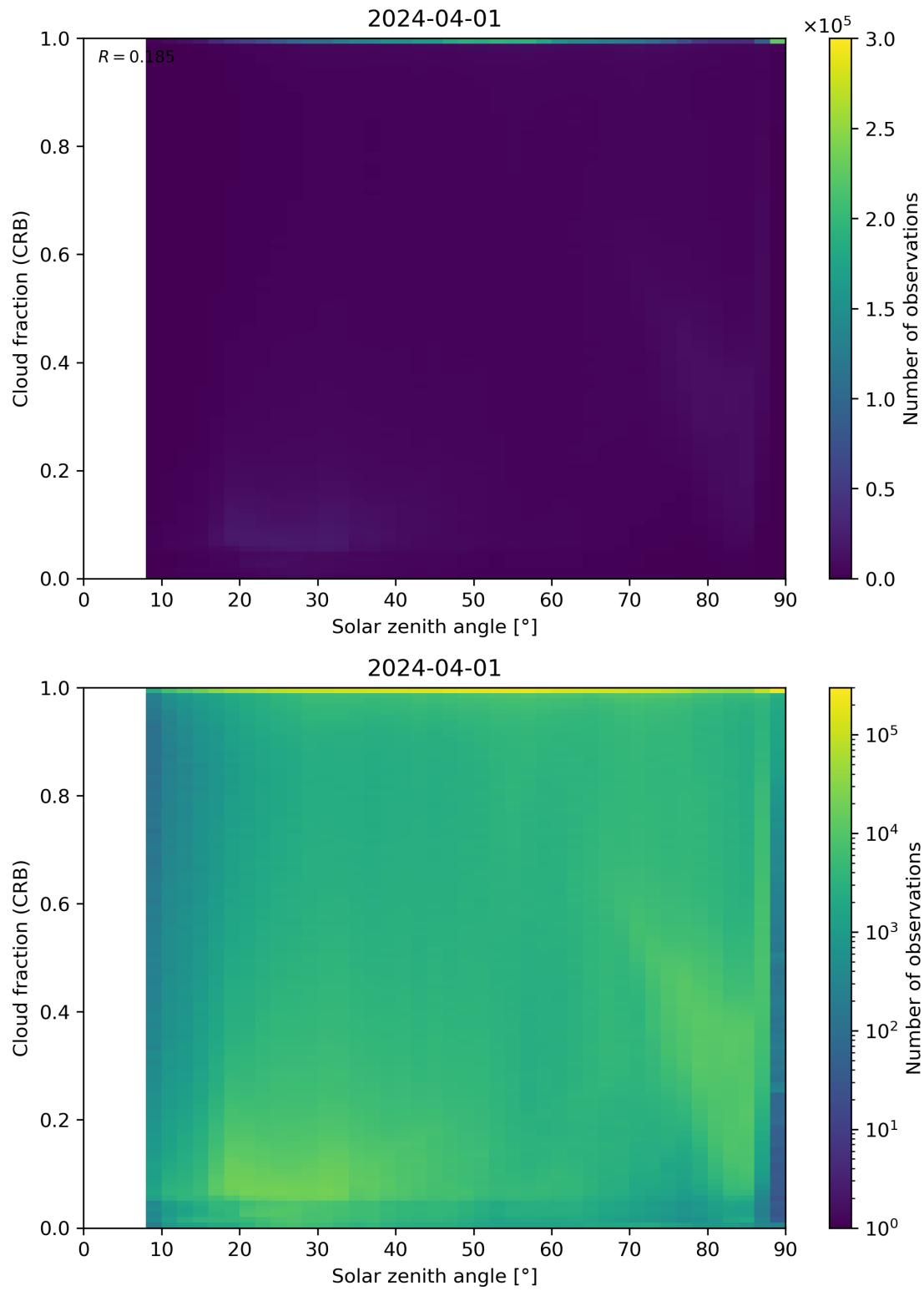
Figure 101: Scatter density plot of “Solar zenith angle” against “Cloud fraction (CRB)” for 2024-03-31 to 2024-04-02.
