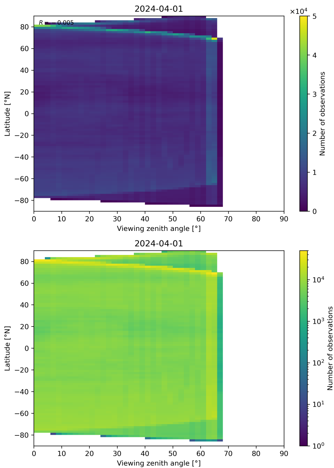
Figure 113: Scatter density plot of “Viewing zenith angle” against “Latitude” for 2024-03-31 to 2024-04-02.
