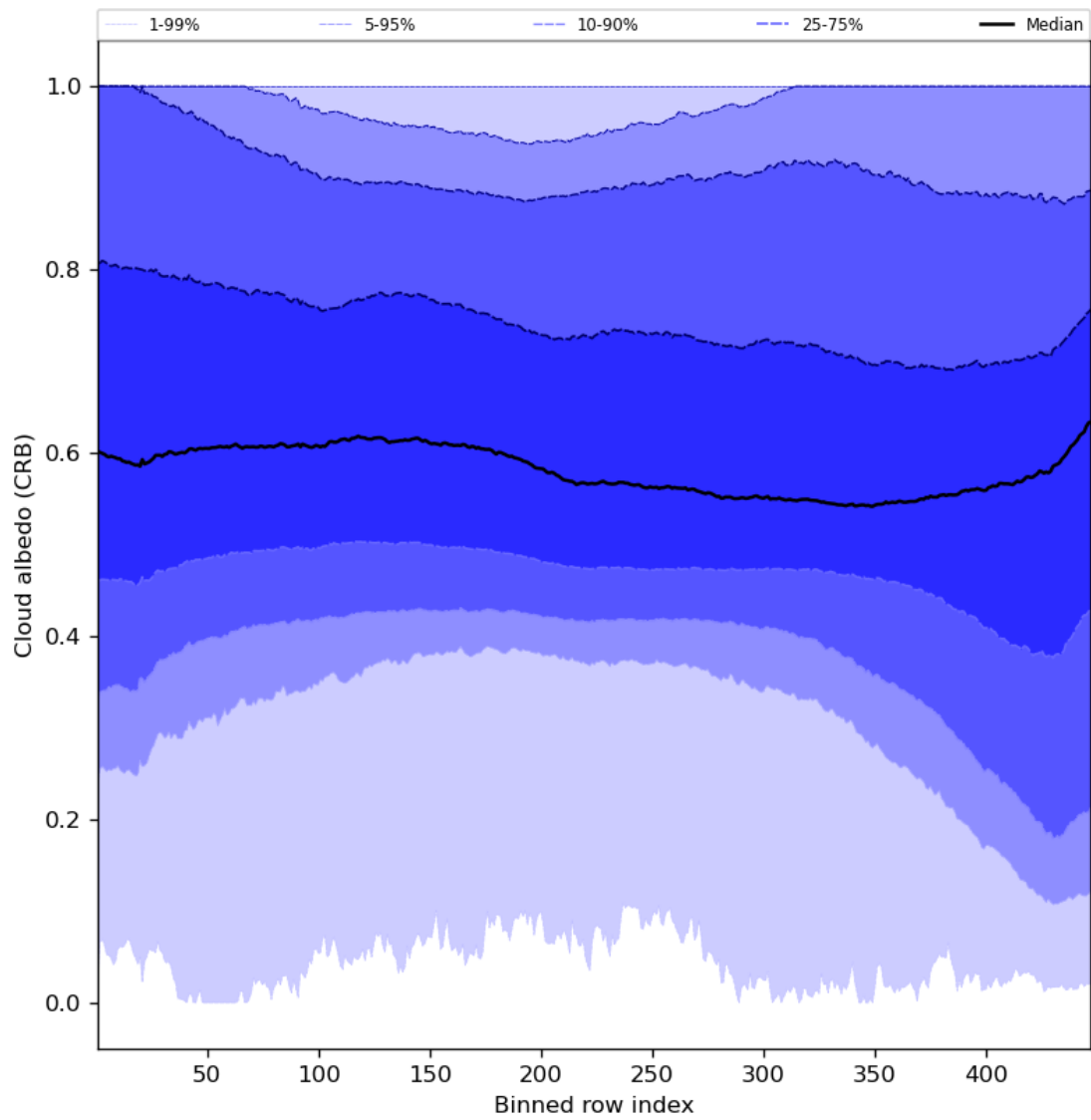
Figure 60: Along track statistics of “Cloud albedo (CRB)” for 2024-03-31 to 2024-04-02
