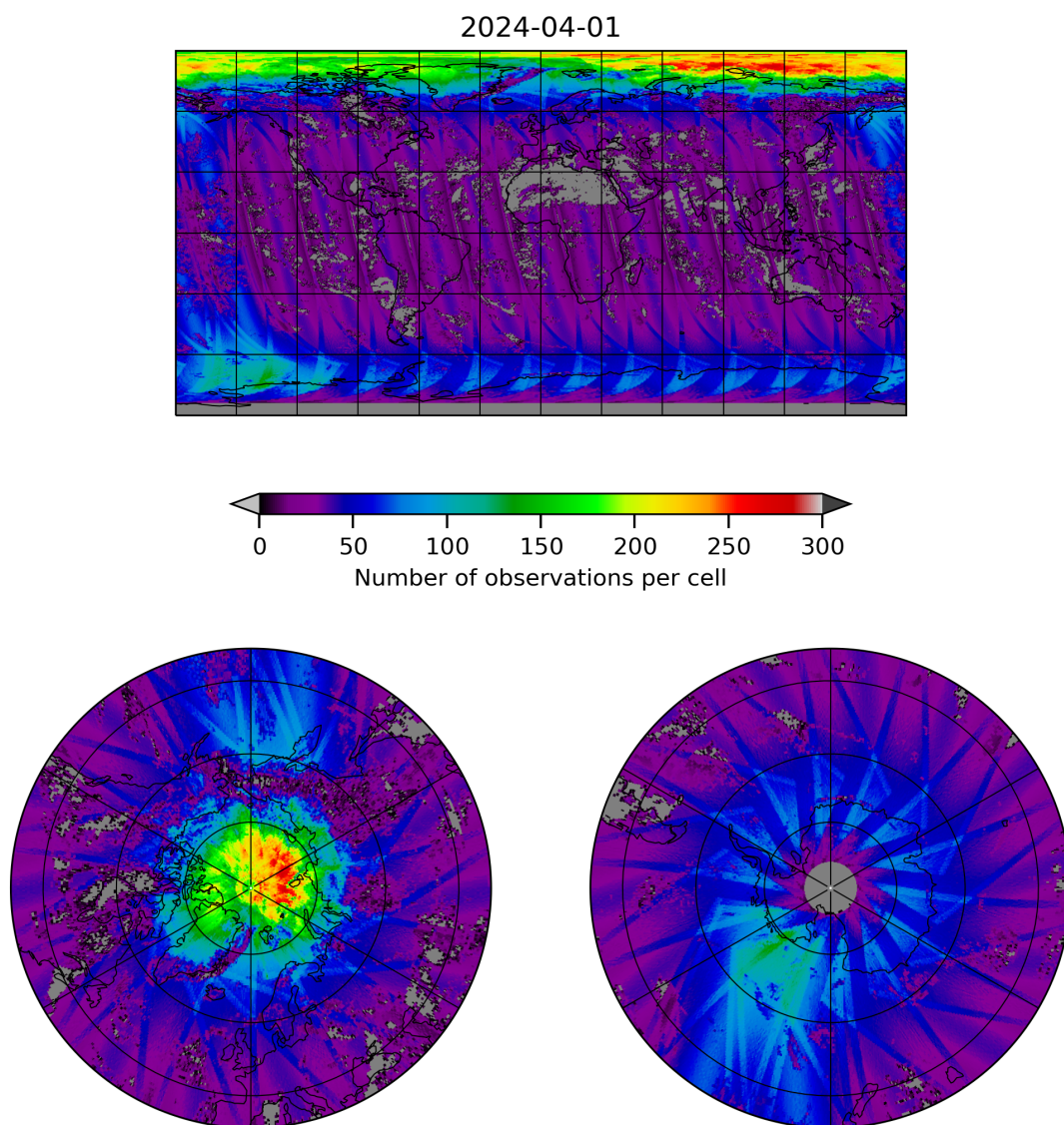
Figure 21: Map of the number of observations for 2024-03-31 to 2024-04-02
