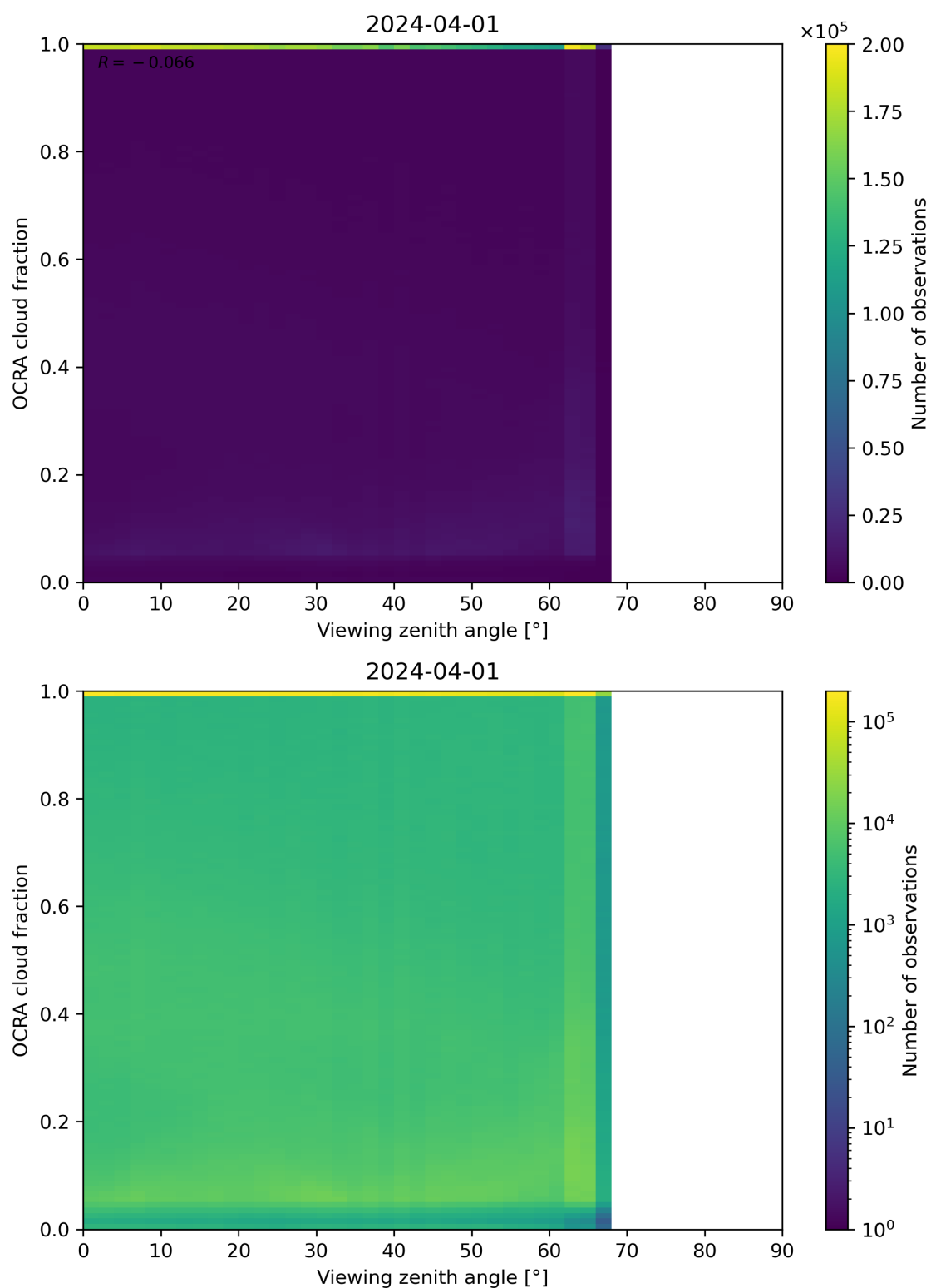
Figure 108: Scatter density plot of “Viewing zenith angle” against “OCRA cloud fraction” for 2024-03-31 to 2024-04-02.
