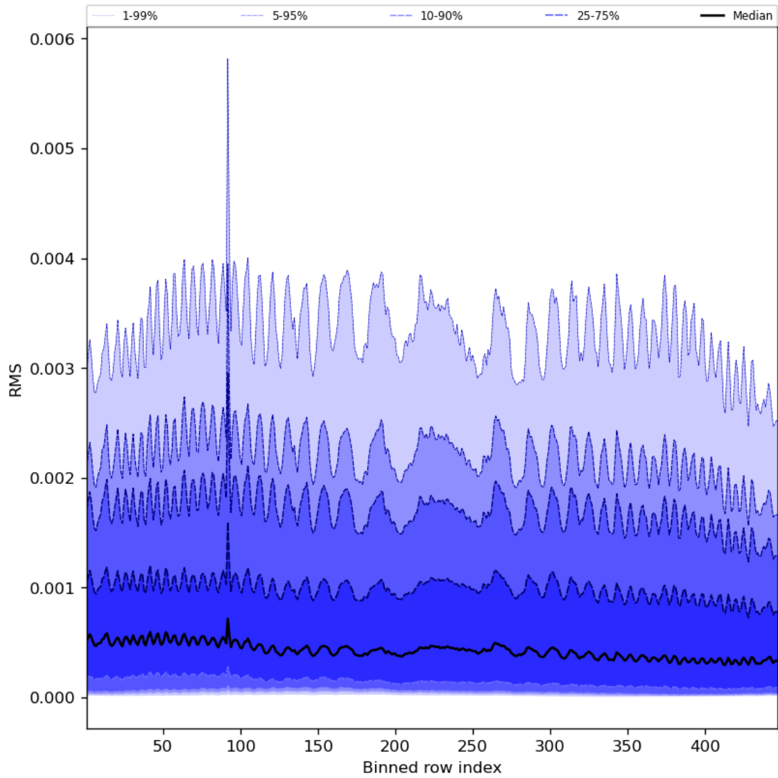
Figure 63: Along track statistics of “RMS” for 2024-03-31 to 2024-04-02
