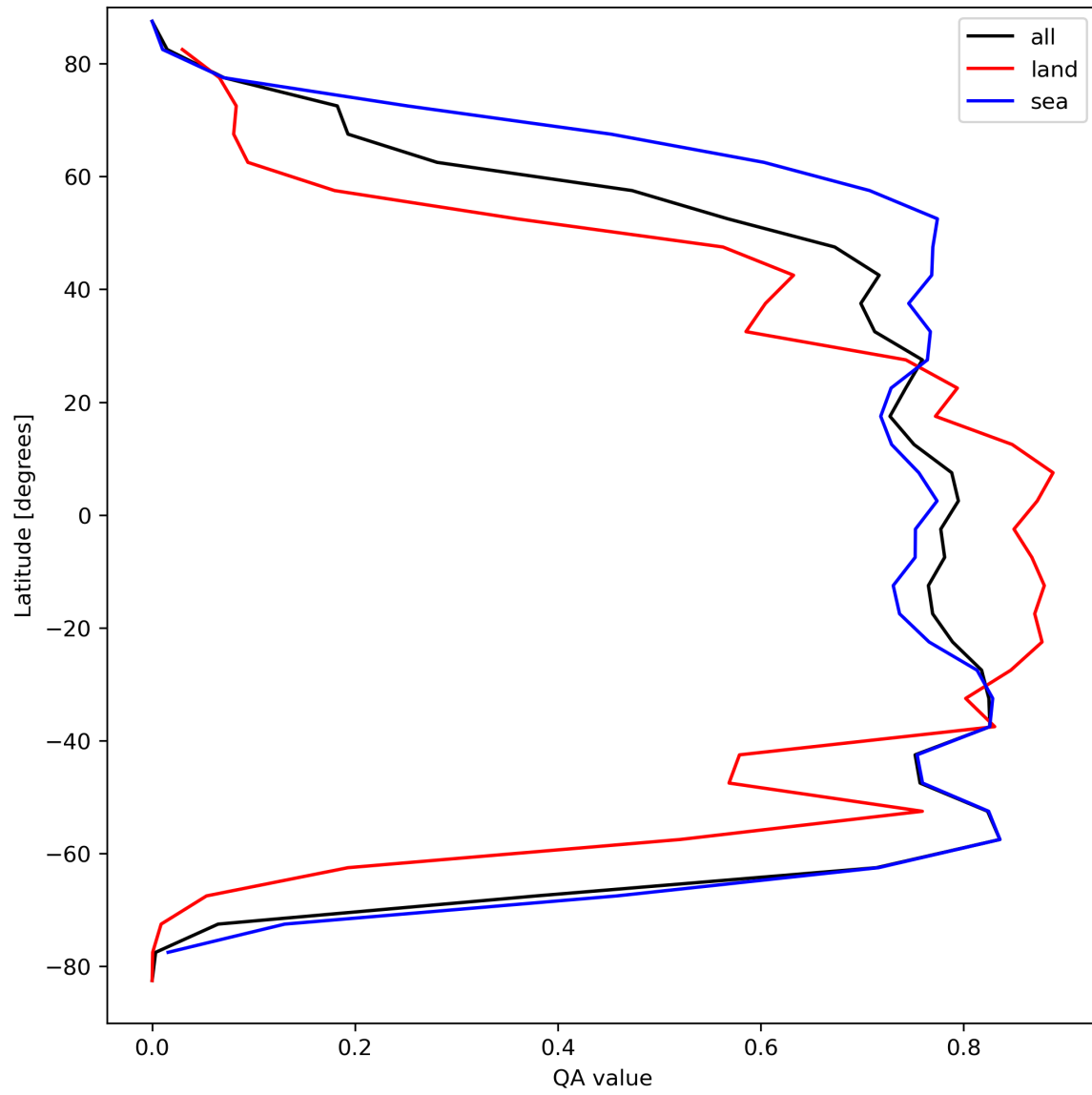
Figure 22: Zonal average of “QA value” for 2024-03-31 to 2024-04-02.
