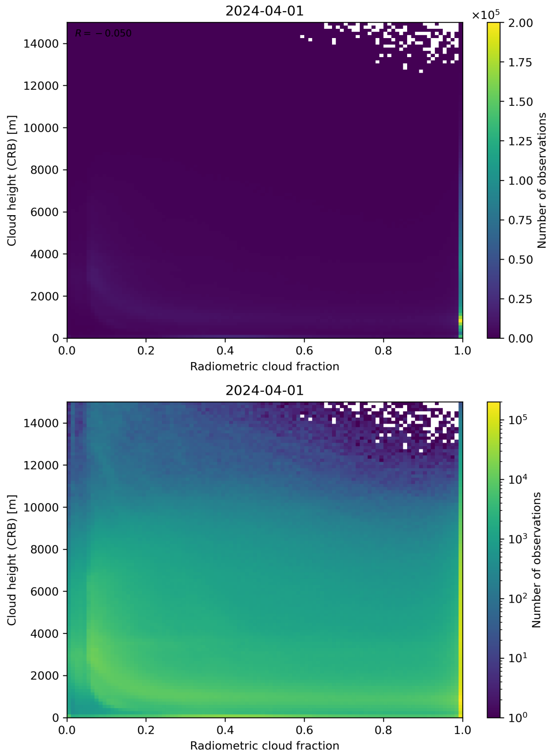
Figure 74: Scatter density plot of “Radiometric cloud fraction” against “Cloud height (CRB)” for 2024-03-31 to 2024-04-02.
