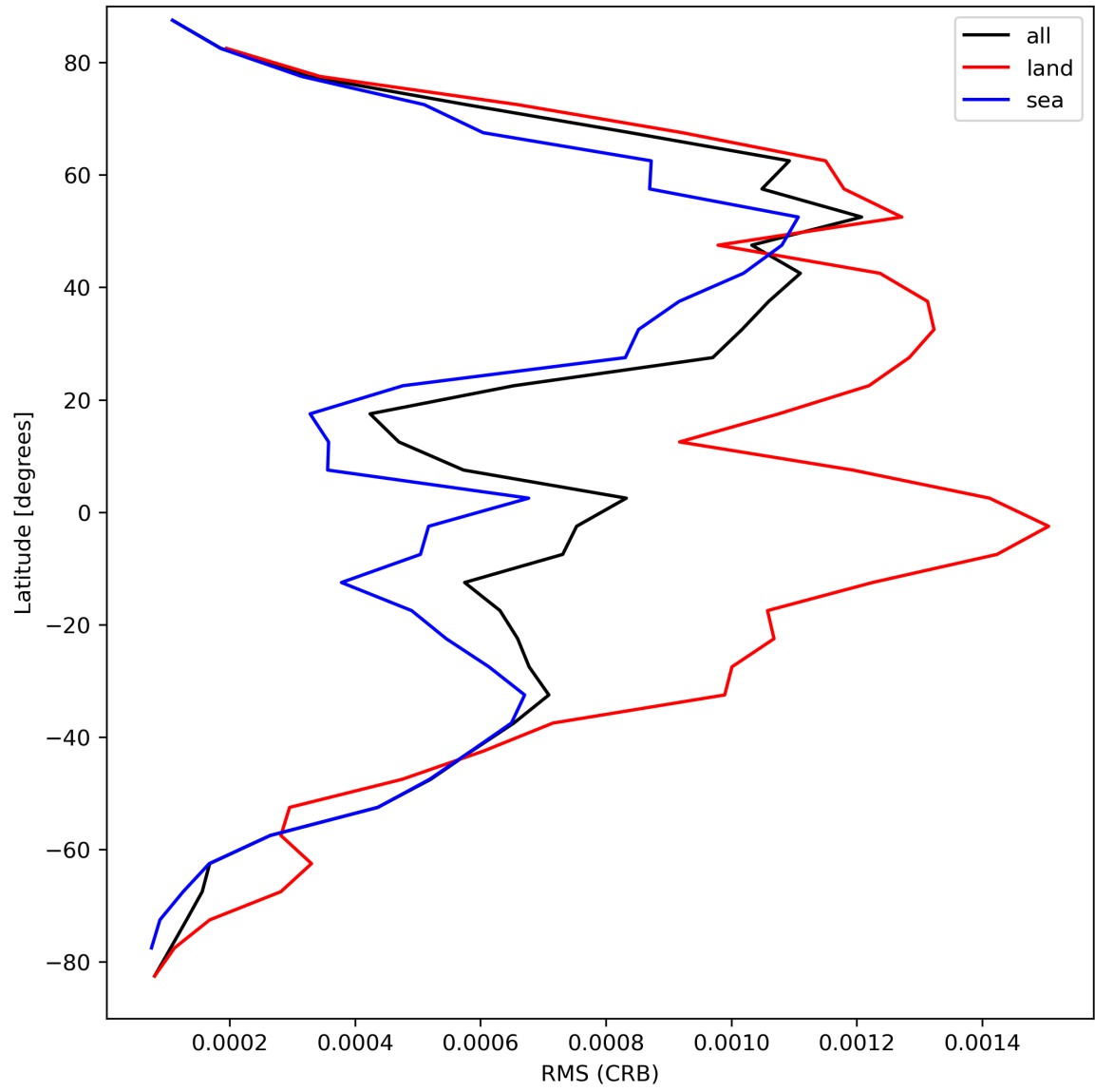
Figure 32: Zonal average of “RMS (CRB)” for 2024-03-31 to 2024-04-02.
