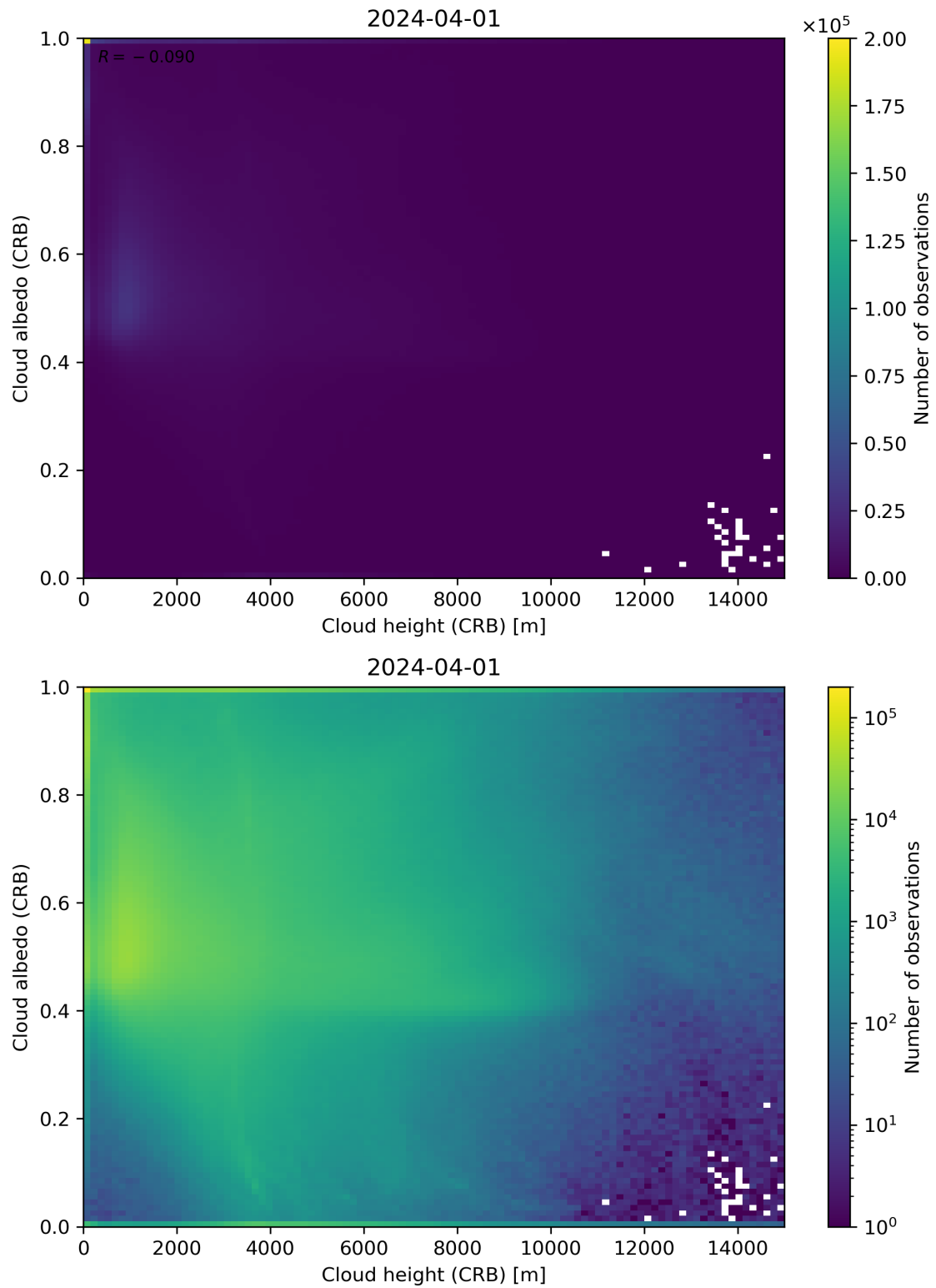
Figure 80: Scatter density plot of “Cloud height (CRB)” against “Cloud albedo (CRB)” for 2024-03-31 to 2024-04-02.
