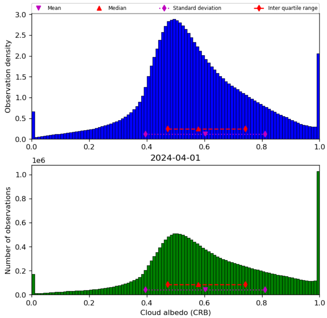
Figure 44: Histogram of “Cloud albedo (CRB)” for 2024-03-31 to 2024-04-02
