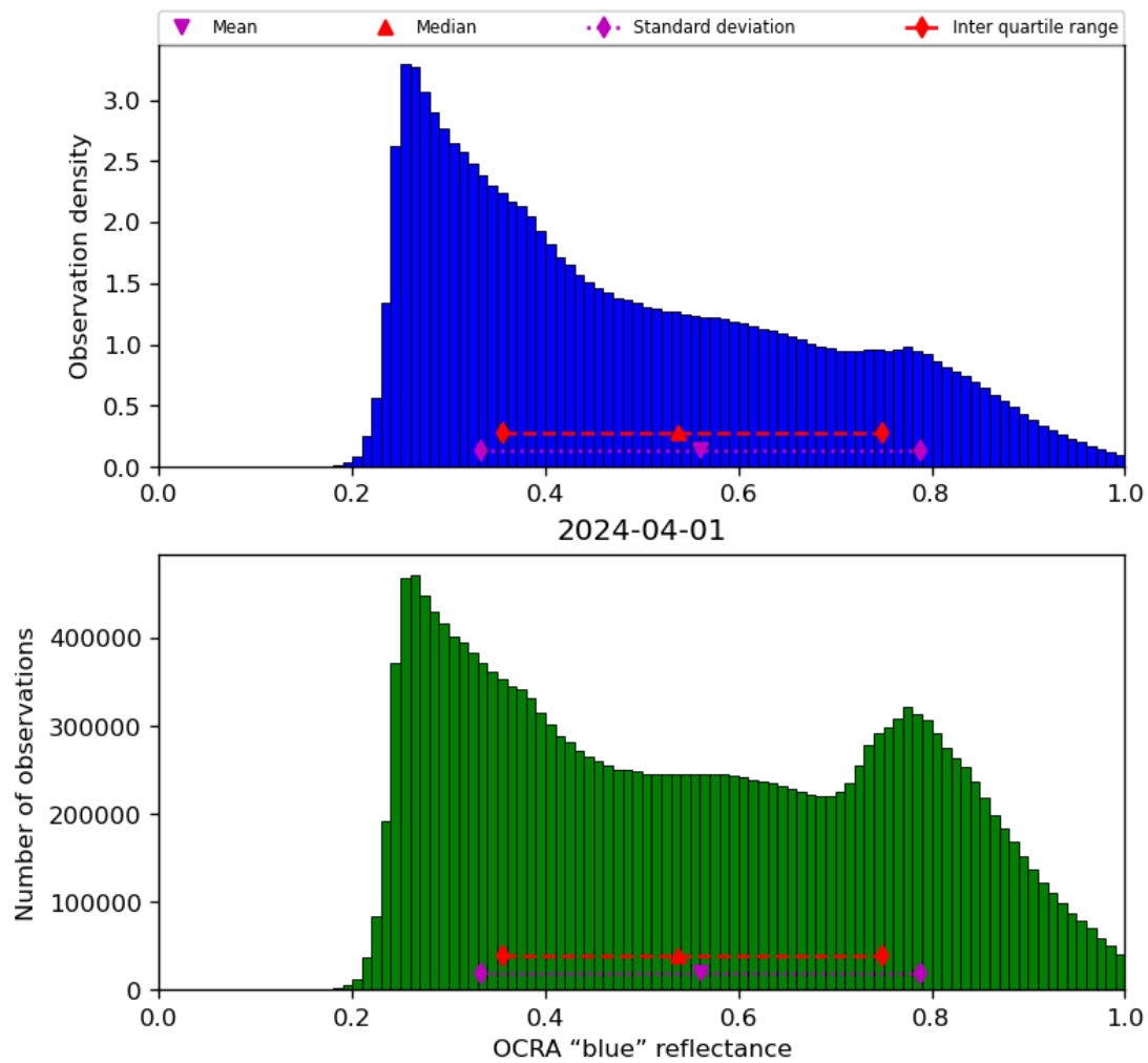
Figure 51: Histogram of “OCRA “blue” reflectance” for 2024-03-31 to 2024-04-02
