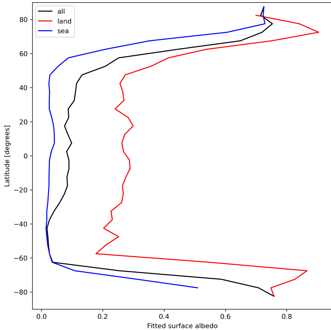
Figure 29: Zonal average of “Fitted surface albedo” for 2024-03-31 to 2024-04-02.
