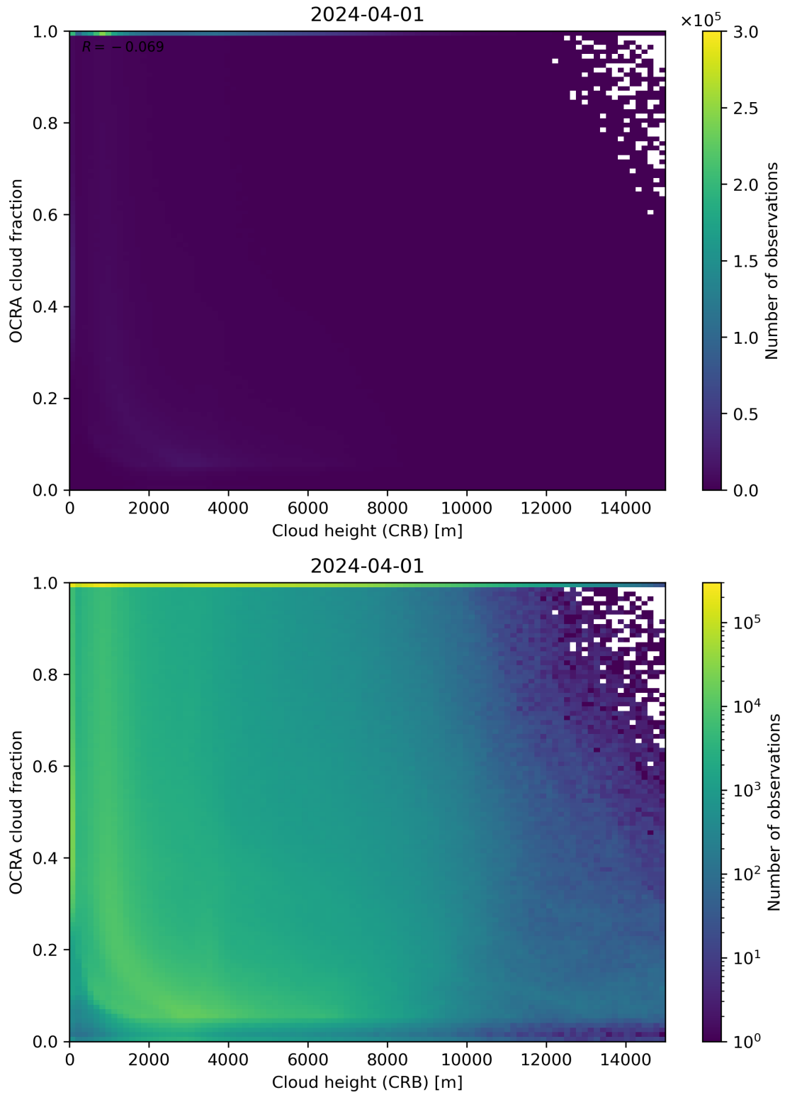
Figure 81: Scatter density plot of “Cloud height (CRB)” against “OCRA cloud fraction” for 2024-03-31 to 2024-04-02.
