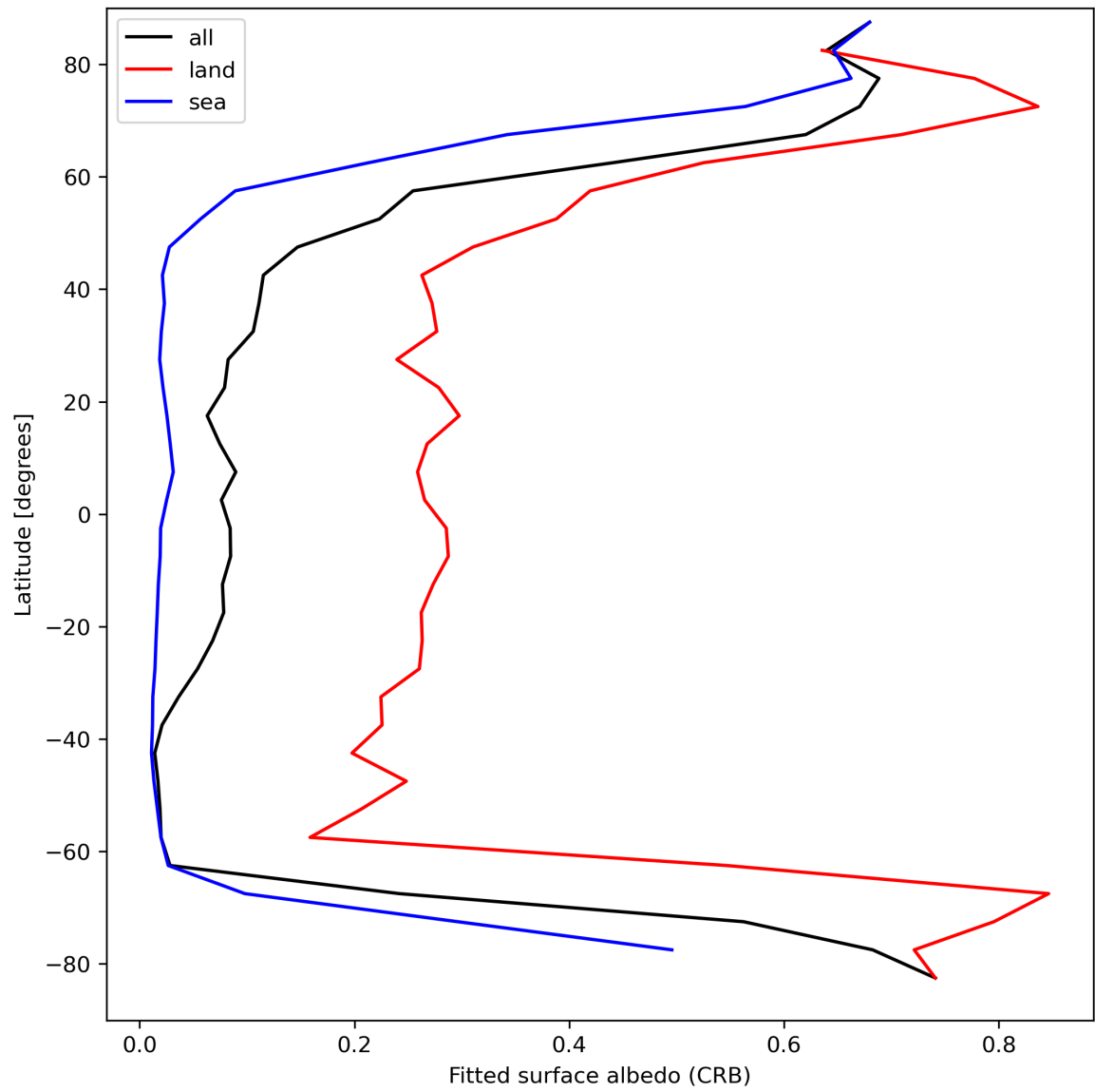
Figure 30: Zonal average of “Fitted surface albedo (CRB)” for 2024-03-31 to 2024-04-02.
