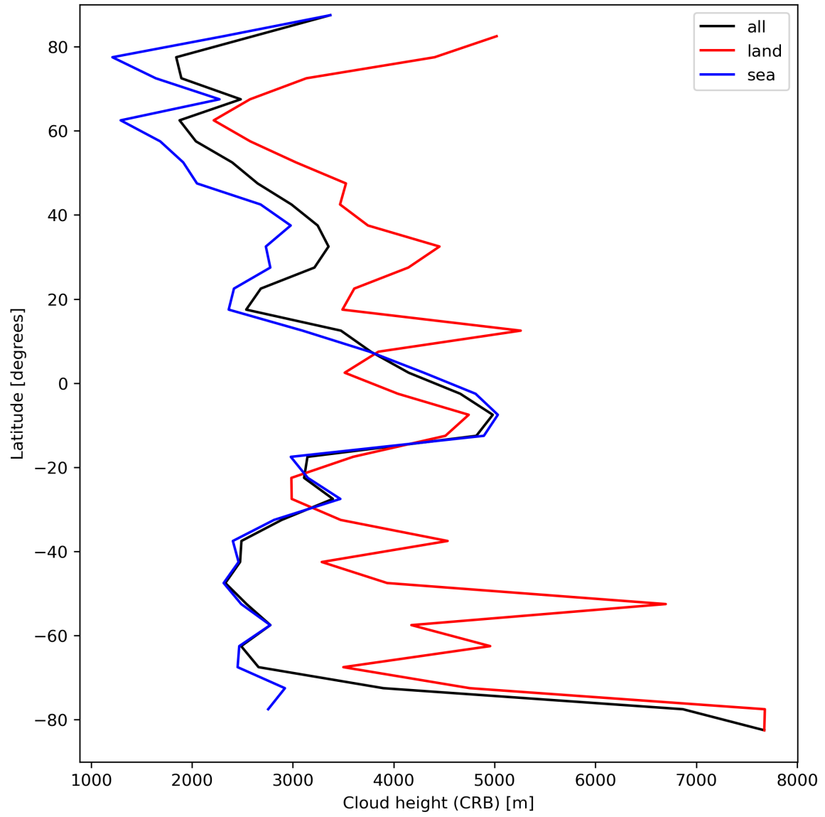
Figure 27: Zonal average of “Cloud height (CRB)” for 2024-03-31 to 2024-04-02.
