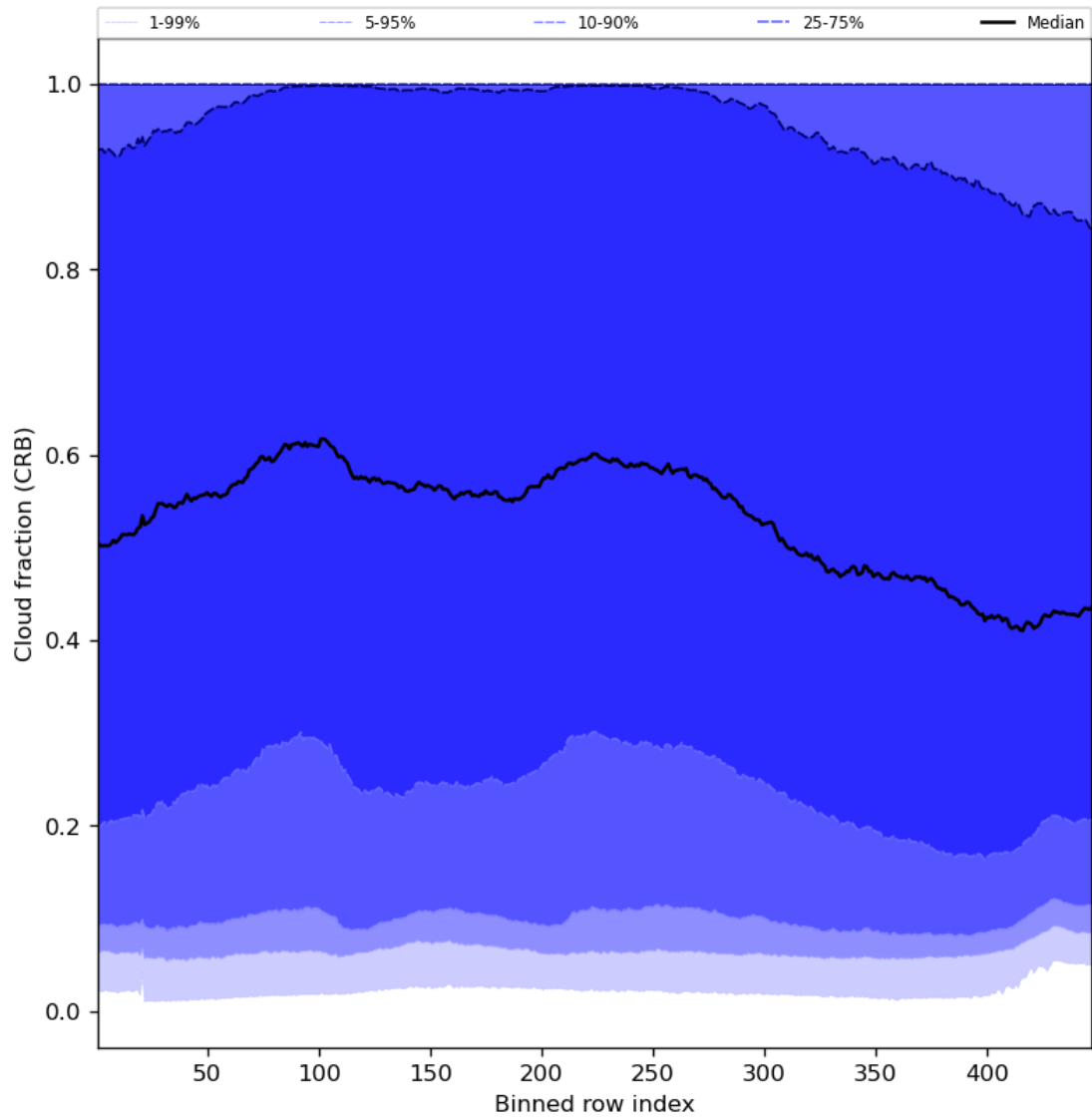
Figure 58: Along track statistics of “Cloud fraction (CRB)” for 2024-03-31 to 2024-04-02
