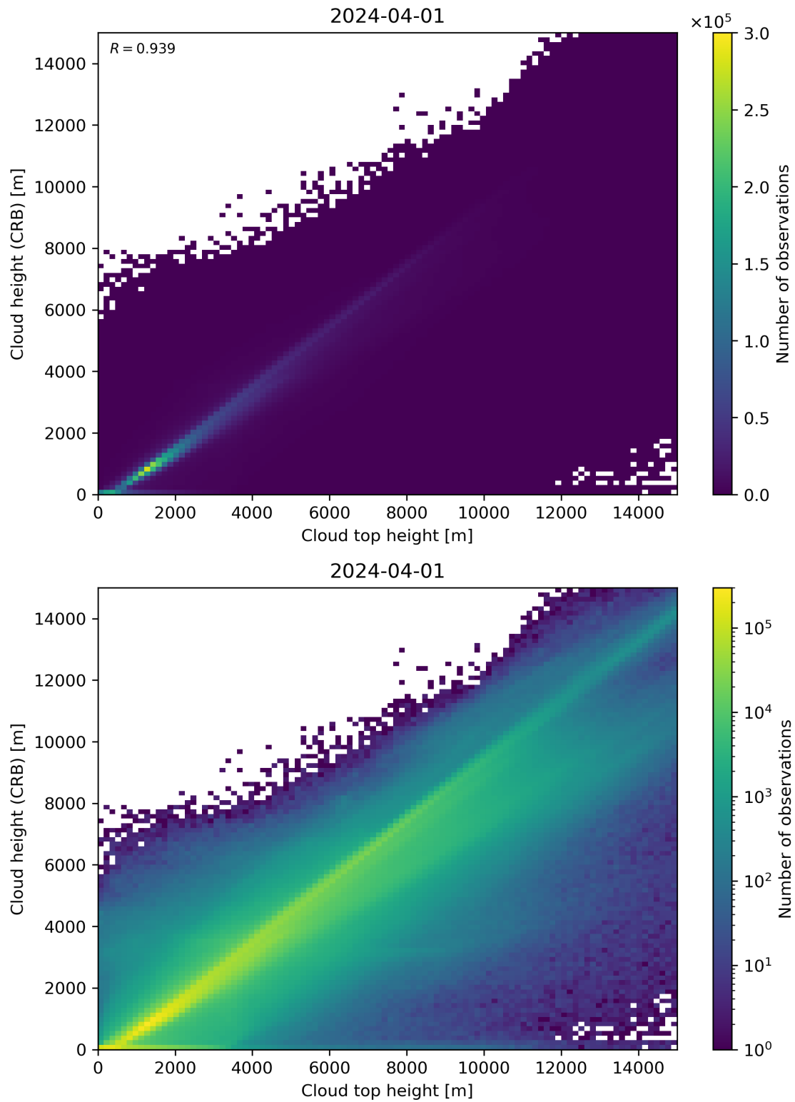
Figure 89: Scatter density plot of “Cloud top height” against “Cloud height (CRB)” for 2024-03-31 to 2024-04-02.
