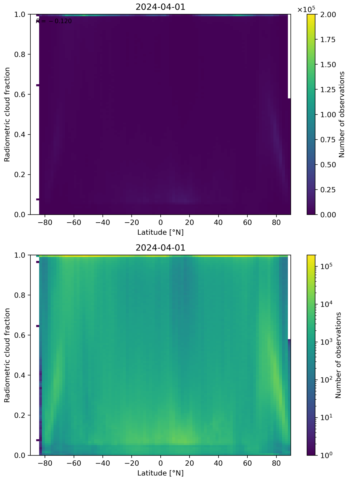
Figure 92: Scatter density plot of “Latitude” against “Radiometric cloud fraction” for 2024-03-31 to 2024-04-02.
