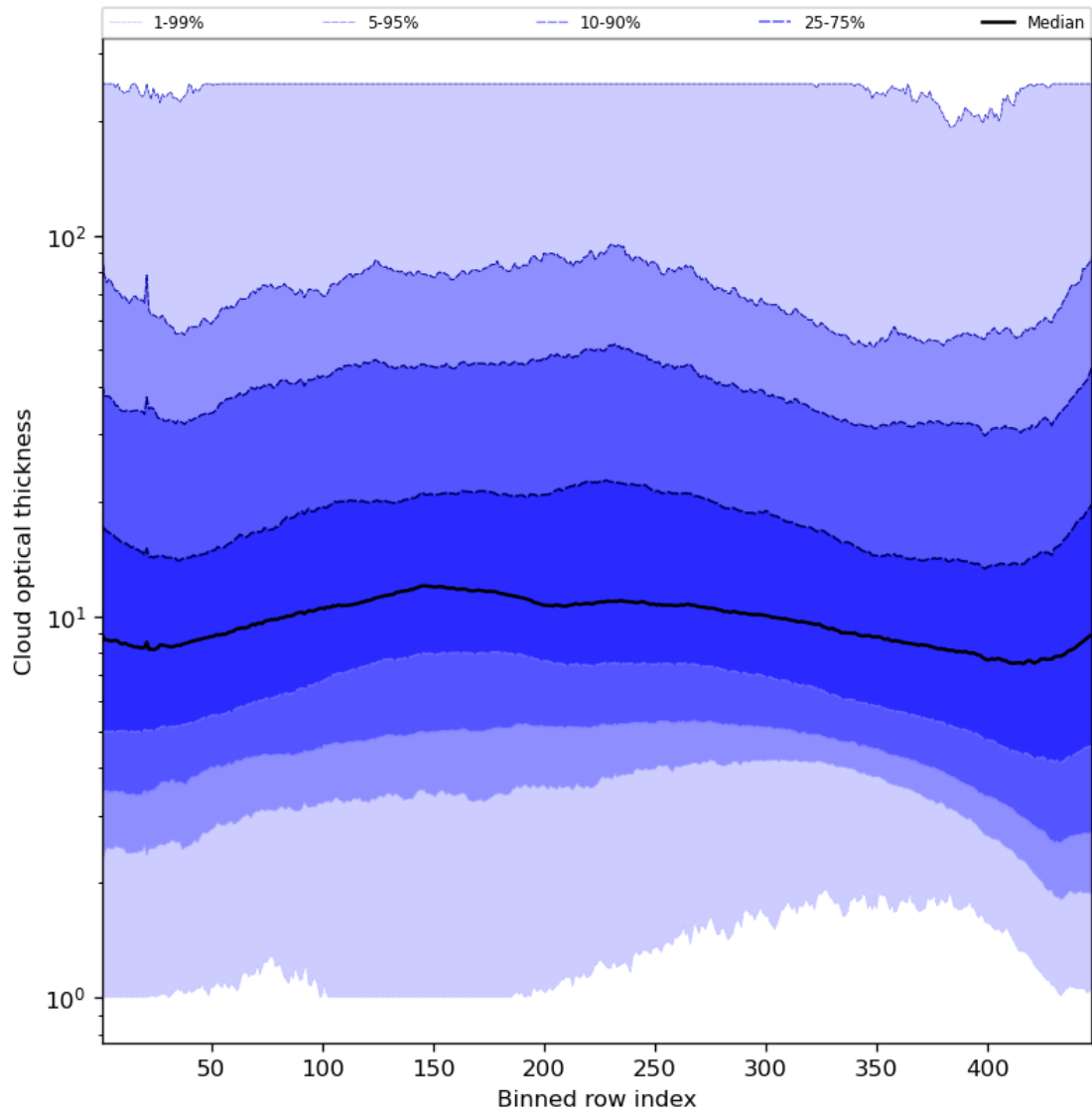
Figure 57: Along track statistics of “Cloud optical thickness” for 2024-03-31 to 2024-04-02
