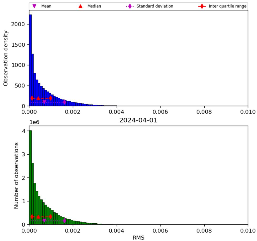
Figure 47: Histogram of “RMS” for 2024-03-31 to 2024-04-02
