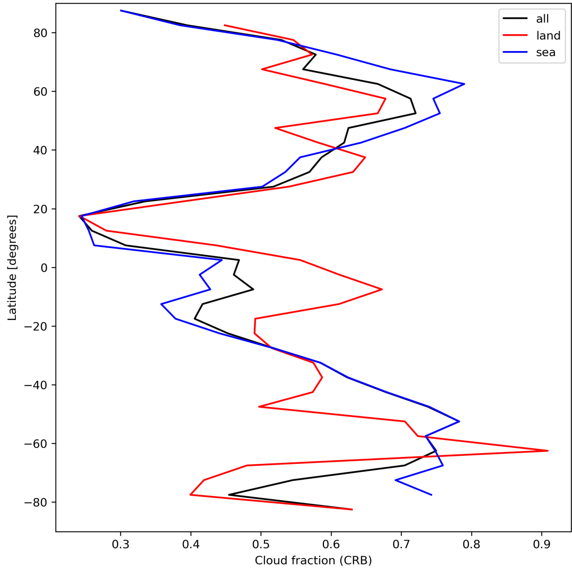
Figure 26: Zonal average of “Cloud fraction (CRB)” for 2024-03-31 to 2024-04-02.
