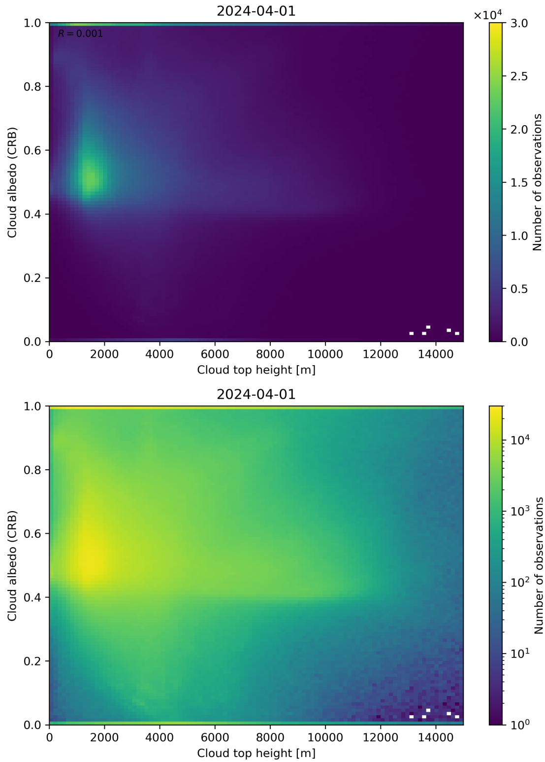
Figure 86: Scatter density plot of “Cloud top height” against “Cloud albedo (CRB)” for 2024-03-31 to 2024-04-02.
