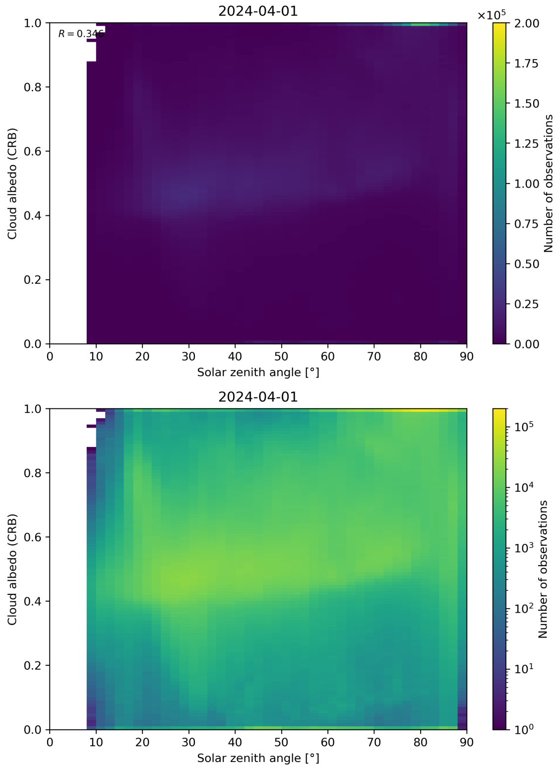
Figure 98: Scatter density plot of “Solar zenith angle” against “Cloud albedo (CRB)” for 2024-03-31 to 2024-04-02.
