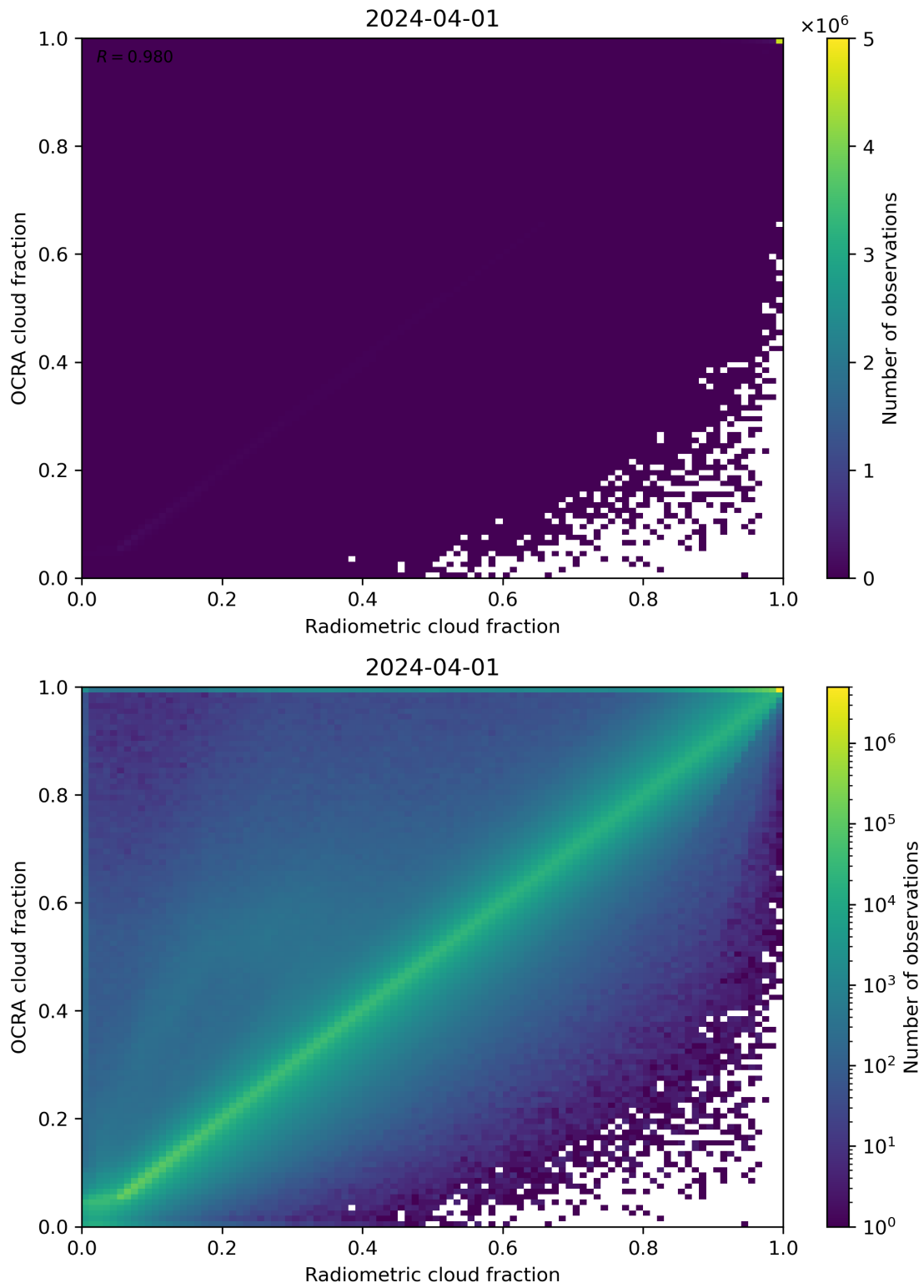
Figure 72: Scatter density plot of “Radiometric cloud fraction” against “OCRA cloud fraction” for 2024-03-31 to 2024-04-02.
