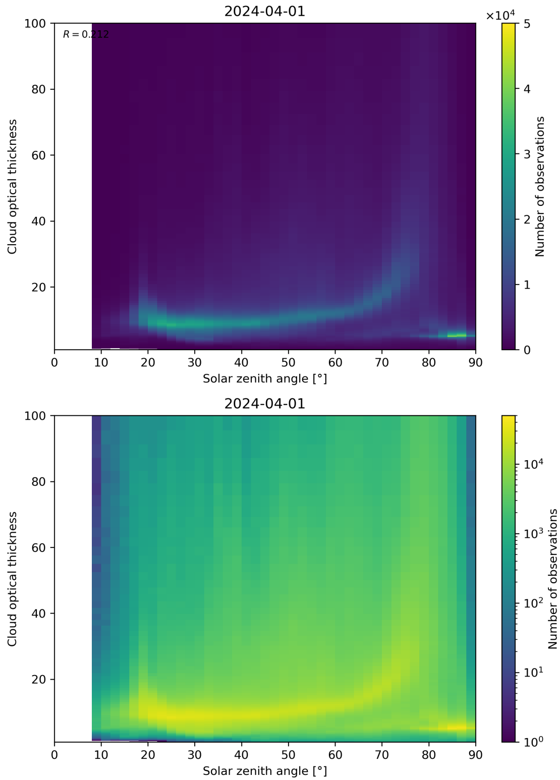
Figure 103: Scatter density plot of “Solar zenith angle” against “Cloud optical thickness” for 2024-03-31 to 2024-04-02.
