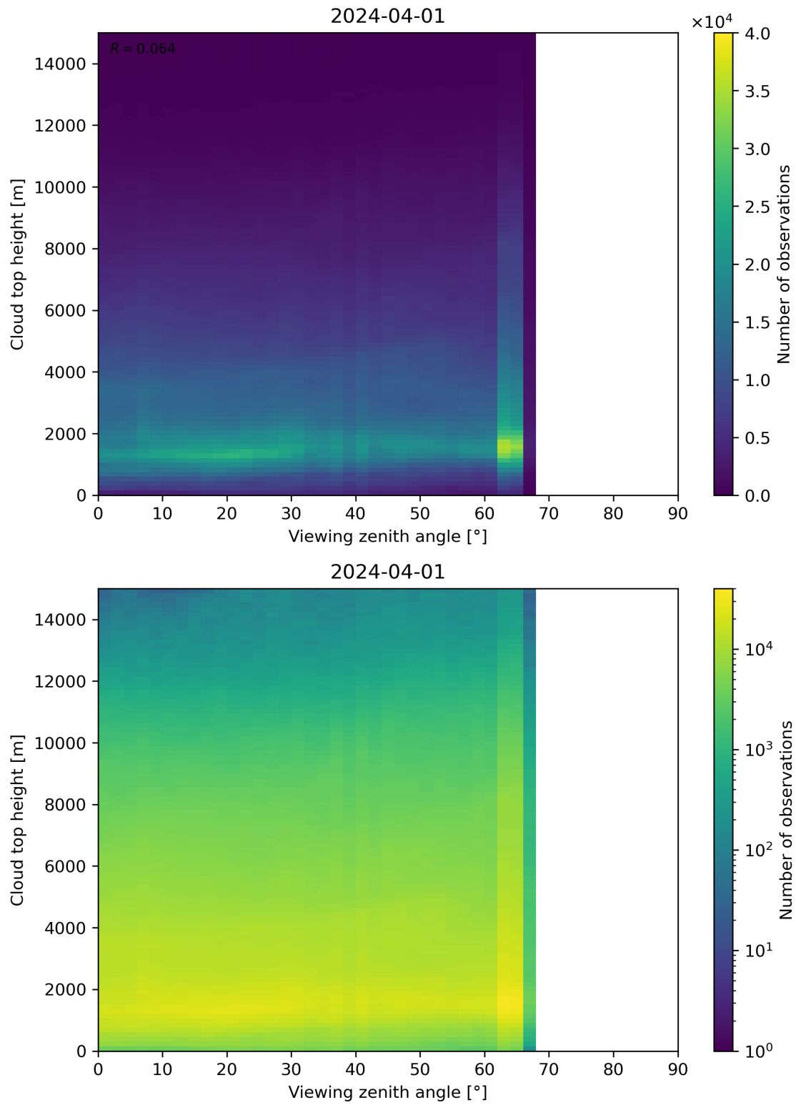
Figure 112: Scatter density plot of “Viewing zenith angle” against “Cloud top height” for 2024-03-31 to 2024-04-02.
