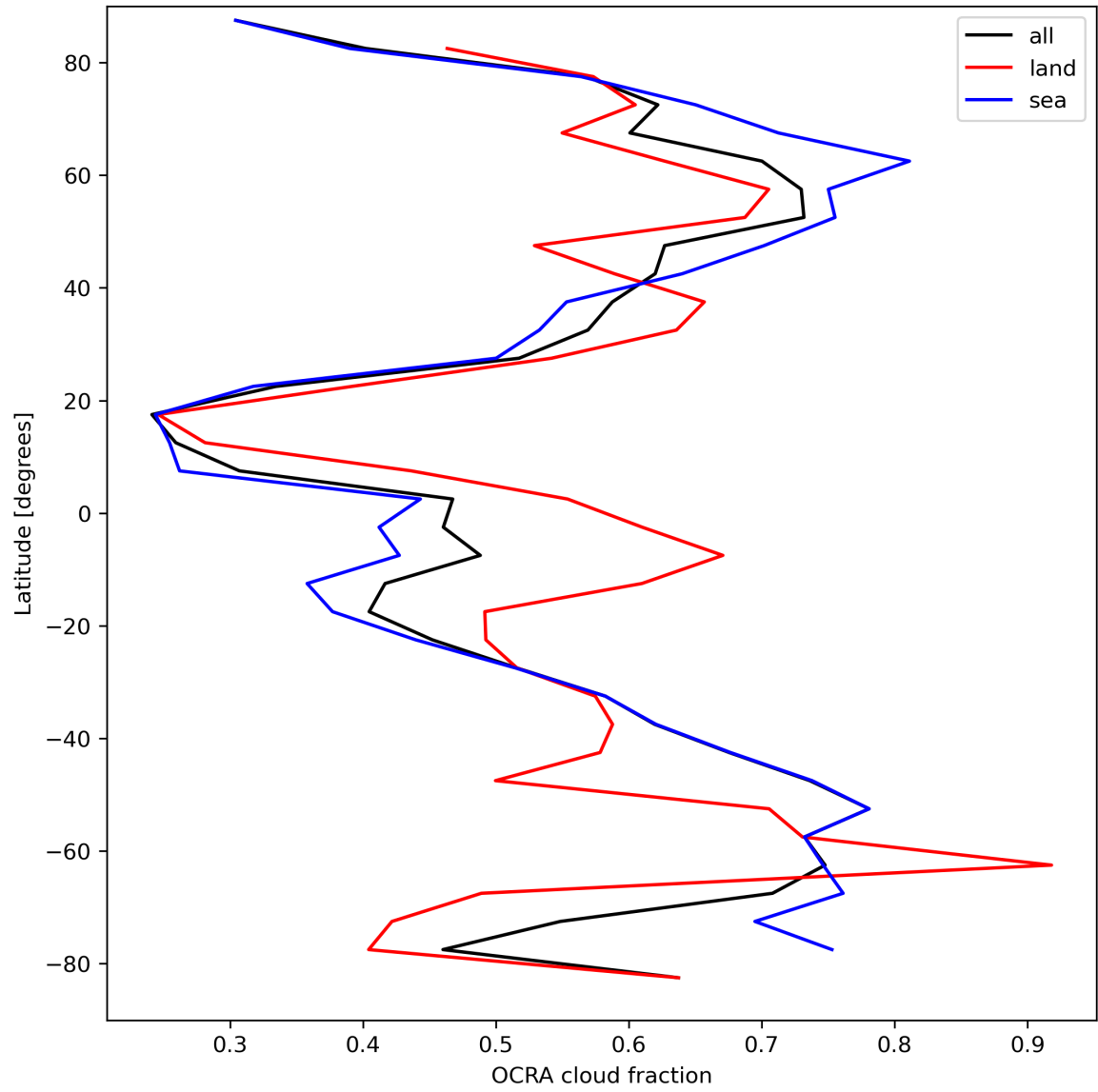
Figure 34: Zonal average of “OCRA cloud fraction” for 2024-03-31 to 2024-04-02.
