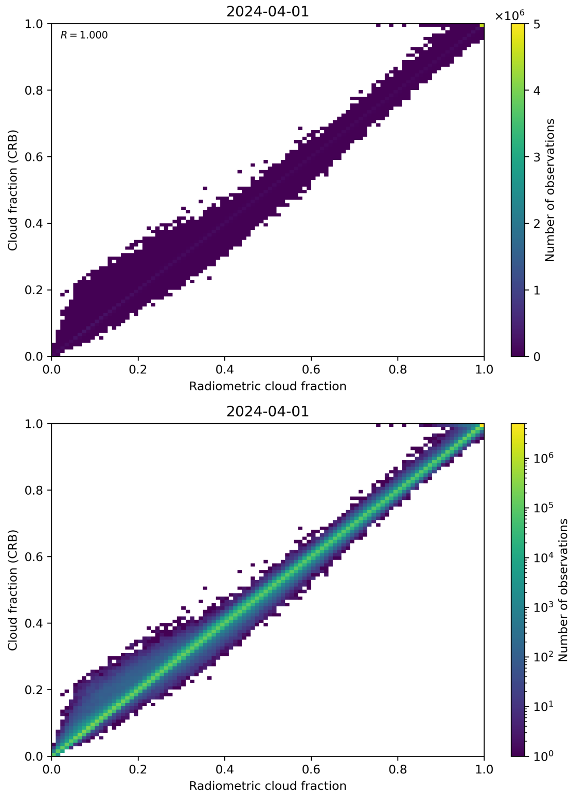
Figure 73: Scatter density plot of “Radiometric cloud fraction” against “Cloud fraction (CRB)” for 2024-03-31 to 2024-04-02.
