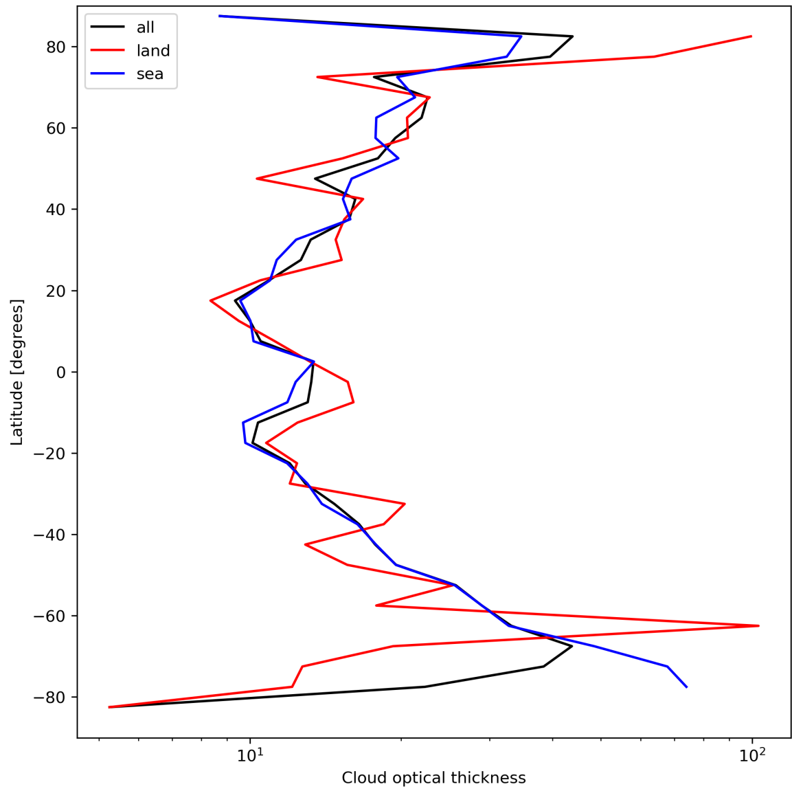
Figure 25: Zonal average of “Cloud optical thickness” for 2024-03-31 to 2024-04-02.
