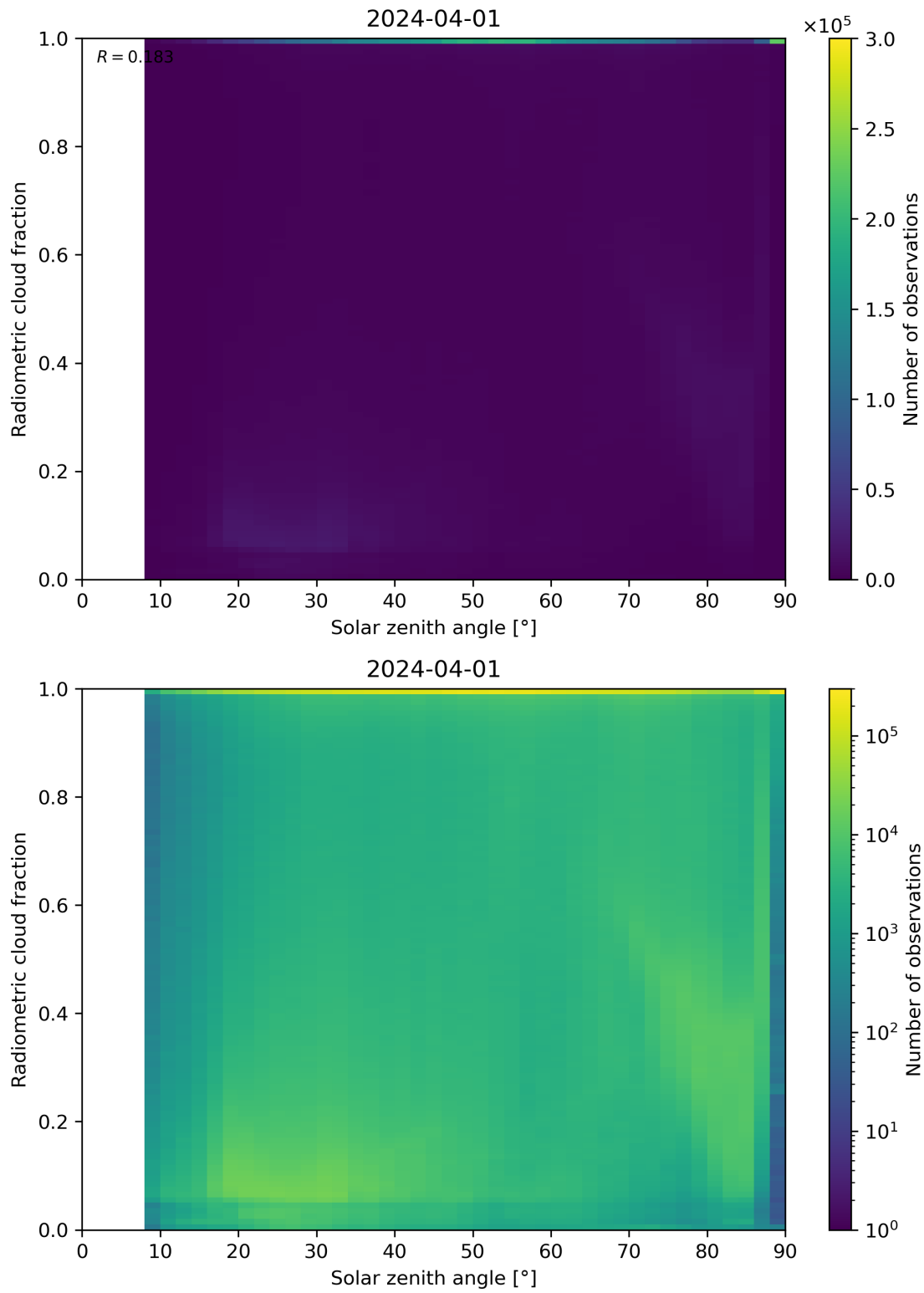
Figure 99: Scatter density plot of “Solar zenith angle” against “Radiometric cloud fraction” for 2024-03-31 to 2024-04-02.
