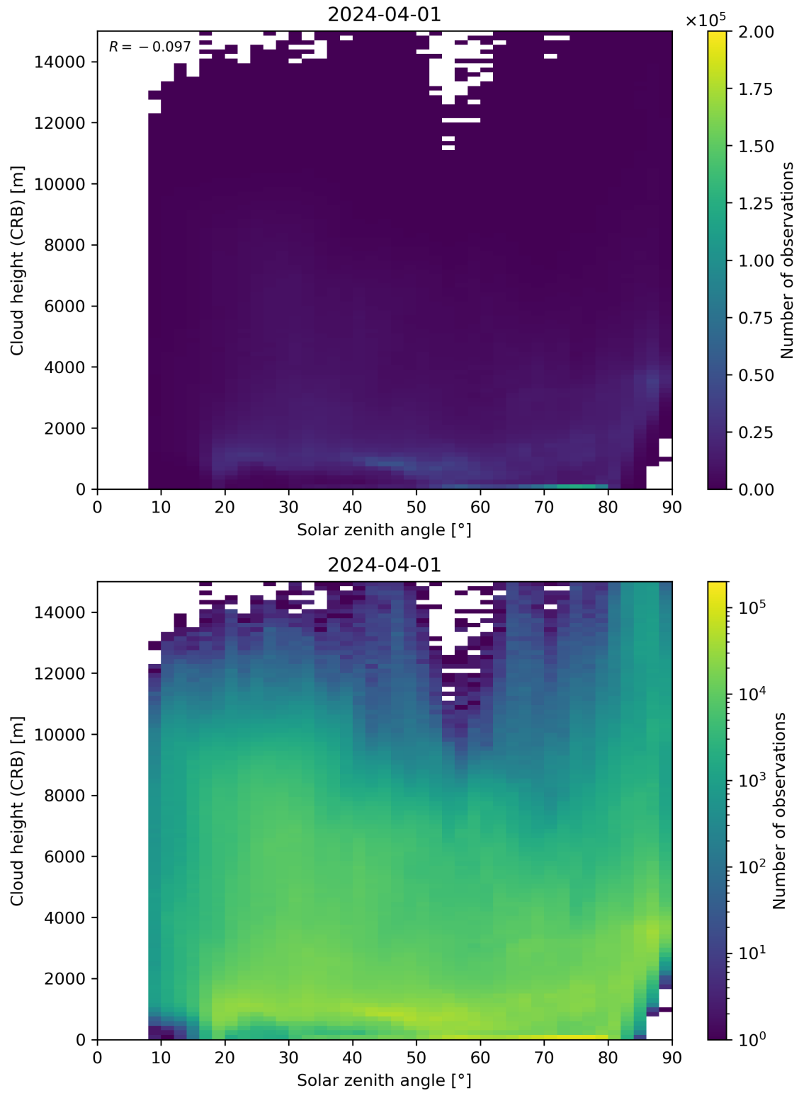
Figure 102: Scatter density plot of “Solar zenith angle” against “Cloud height (CRB)” for 2024-03-31 to 2024-04-02.
