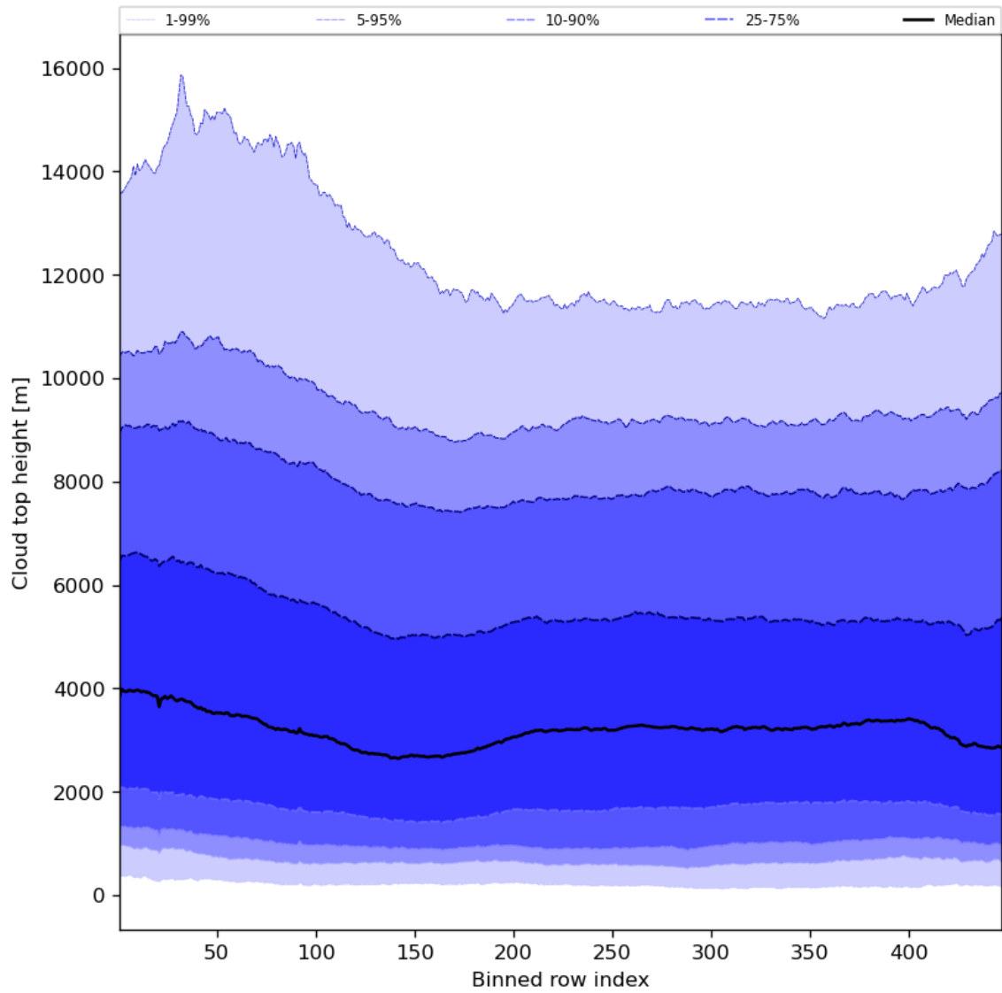
Figure 56: Along track statistics of “Cloud top height” for 2024-03-31 to 2024-04-02
