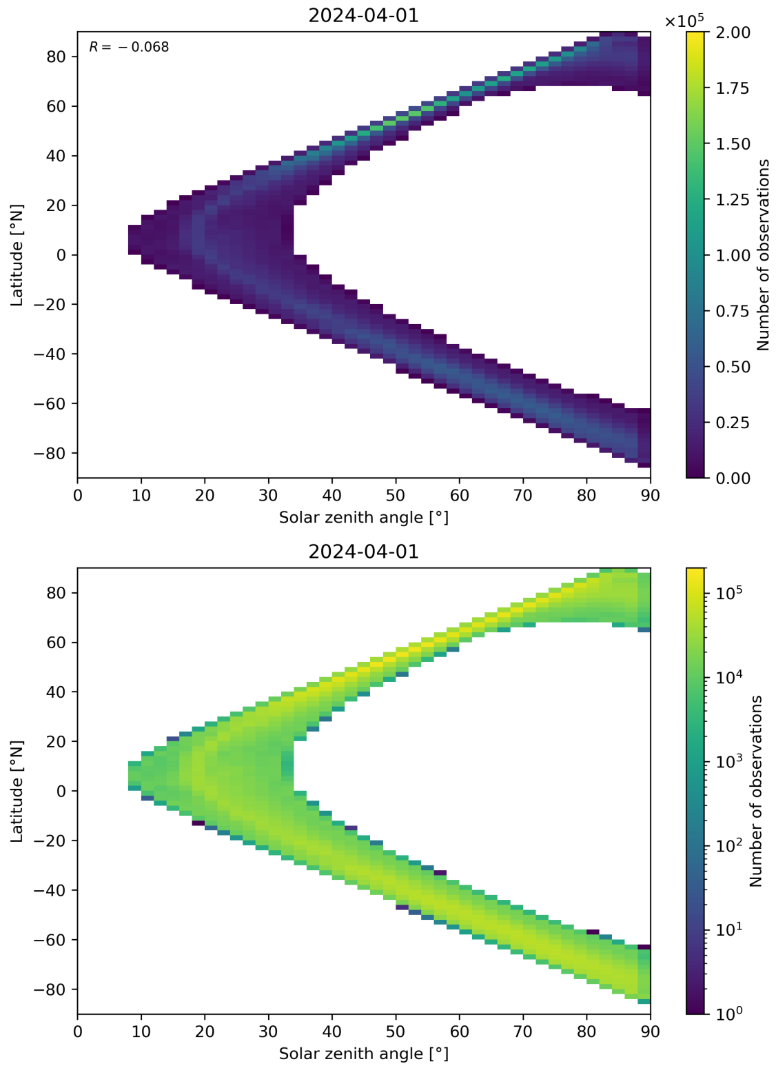
Figure 105: Scatter density plot of “Solar zenith angle” against “Latitude” for 2024-03-31 to 2024-04-02.
