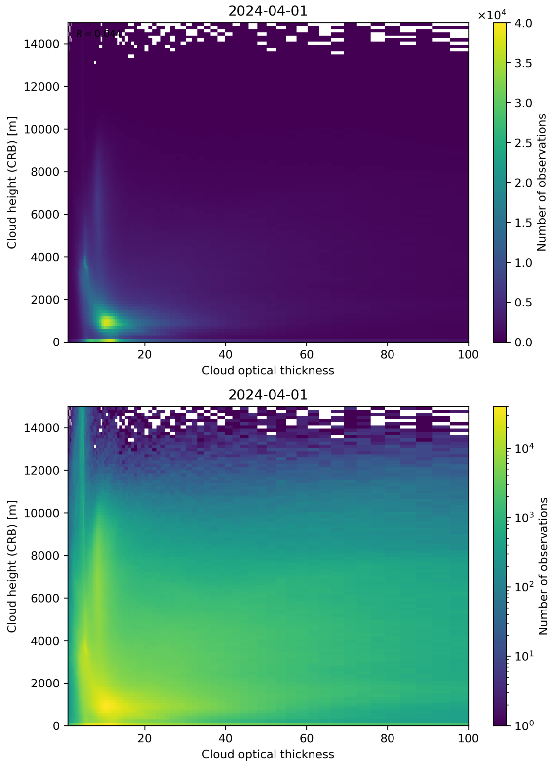
Figure 85: Scatter density plot of “Cloud optical thickness” against “Cloud height (CRB)” for 2024-03-31 to 2024-04-02.
