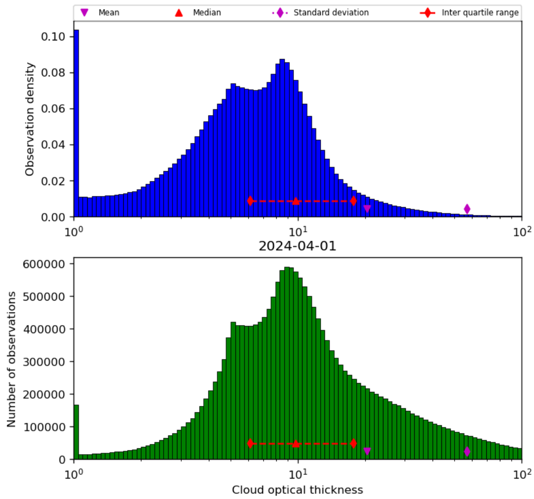
Figure 41: Histogram of “Cloud optical thickness” for 2024-03-31 to 2024-04-02
