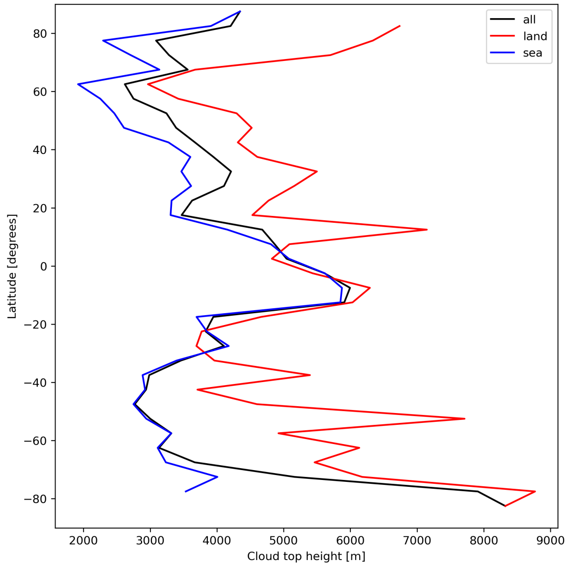
Figure 24: Zonal average of “Cloud top height” for 2024-03-31 to 2024-04-02.
