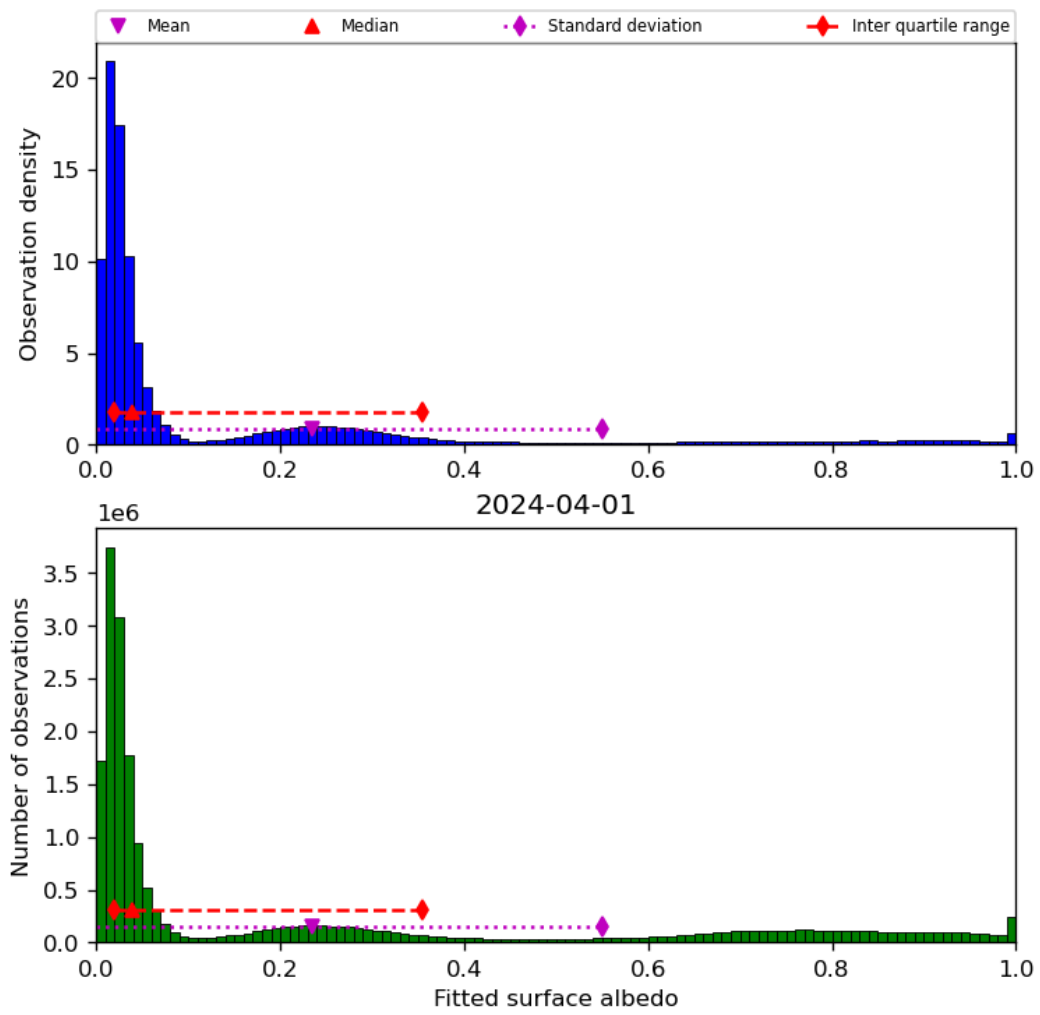
Figure 45: Histogram of “Fitted surface albedo” for 2024-03-31 to 2024-04-02
