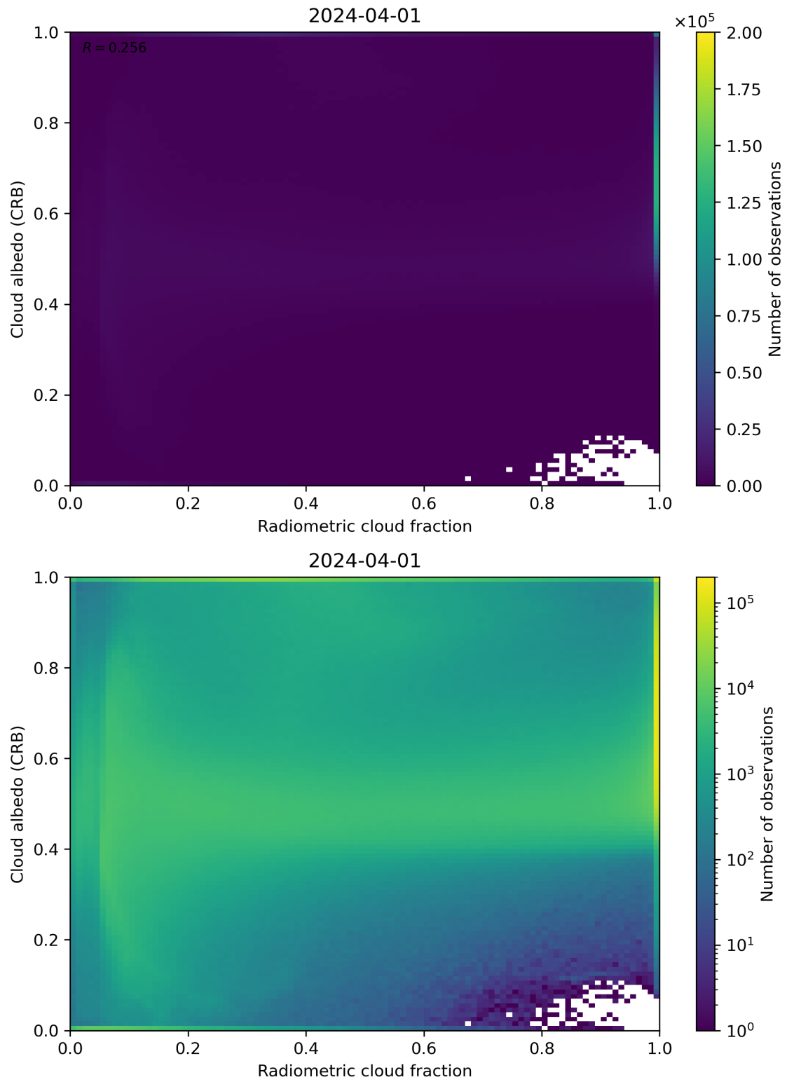
Figure 71: Scatter density plot of “Radiometric cloud fraction” against “Cloud albedo (CRB)” for 2024-03-31 to 2024-04-02.
