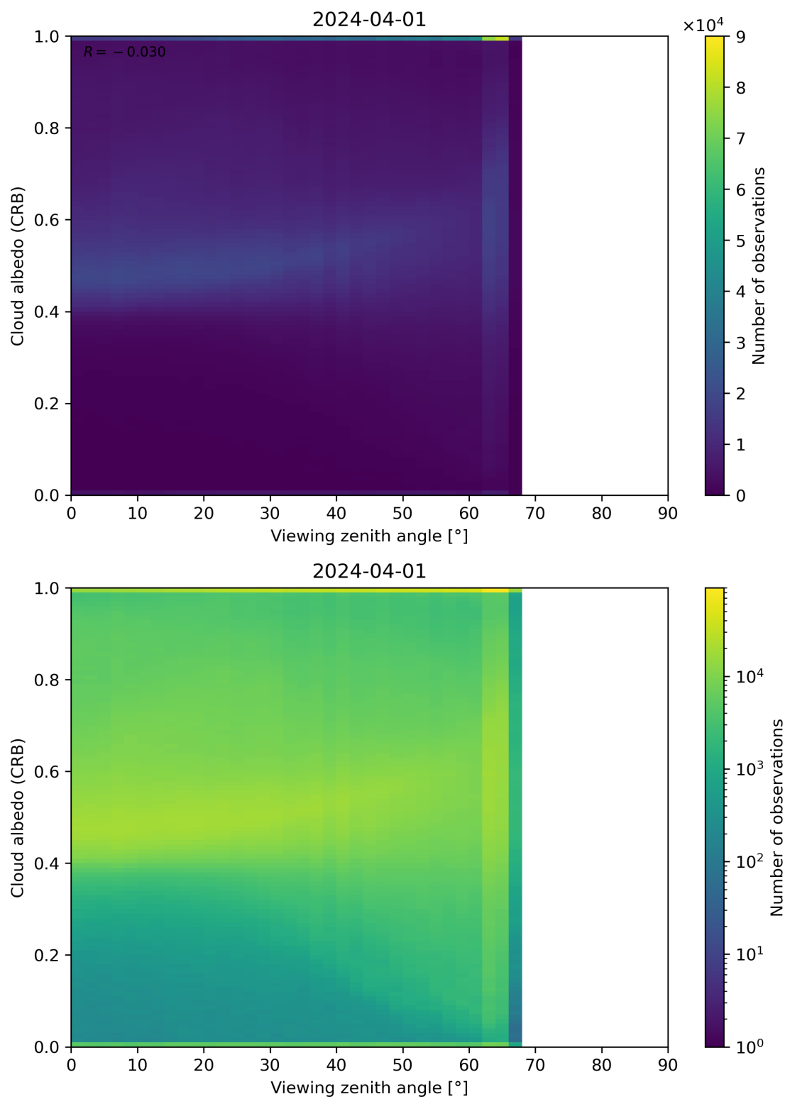
Figure 106: Scatter density plot of “Viewing zenith angle” against “Cloud albedo (CRB)” for 2024-03-31 to 2024-04-02.
